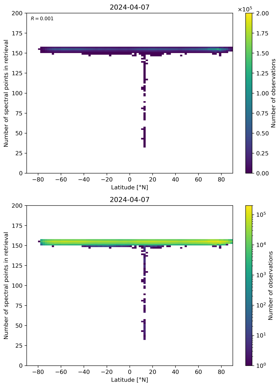
Figure 57: Scatter density plot of “Latitude” against “Number of spectral points in retrieval” for 2024-04-06 to 2024-04-08.
