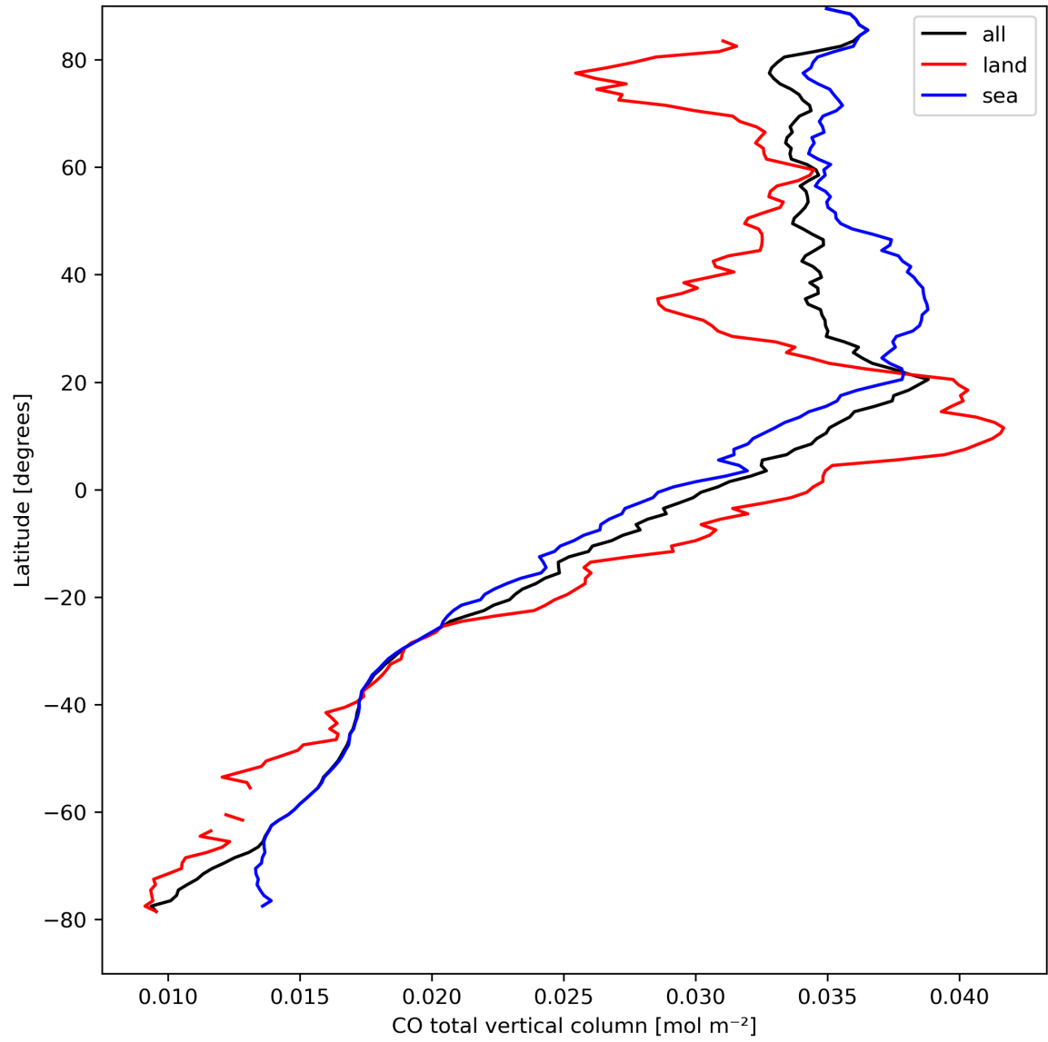
Figure 10: Zonal average of “CO total vertical column” for 2024-04-06 to 2024-04-08.
