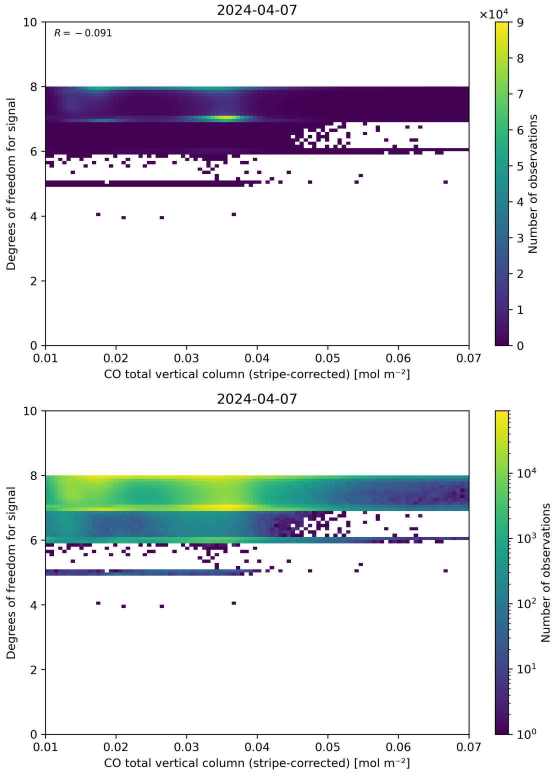
Figure 38: Scatter density plot of “CO total vertical column (stripe-corrected)” against “Degrees of freedom for signal” for 2024-04-06 to 2024-04-08.
