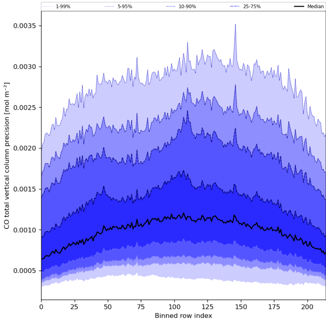
Figure 28: Along track statistics of “CO total vertical column precision” for 2024-04-06 to 2024-04-08
