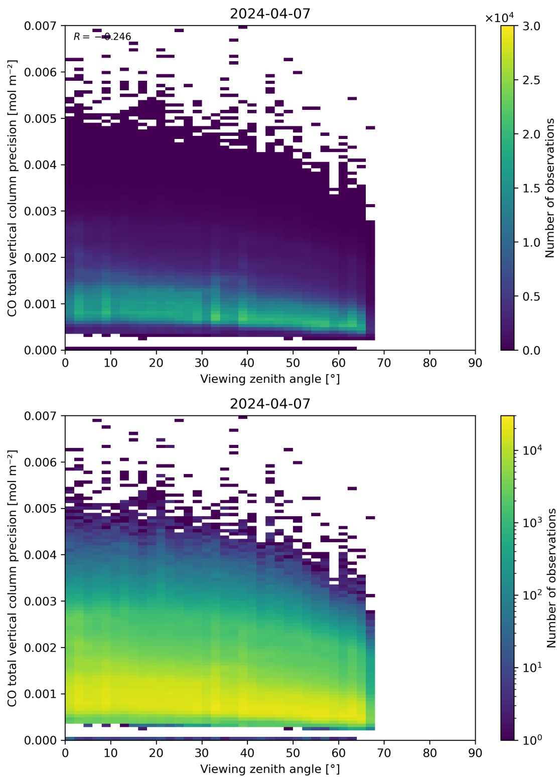
Figure 71: Scatter density plot of “Viewing zenith angle” against “CO total vertical column precision” for 2024-04-06 to 2024-04-08.
