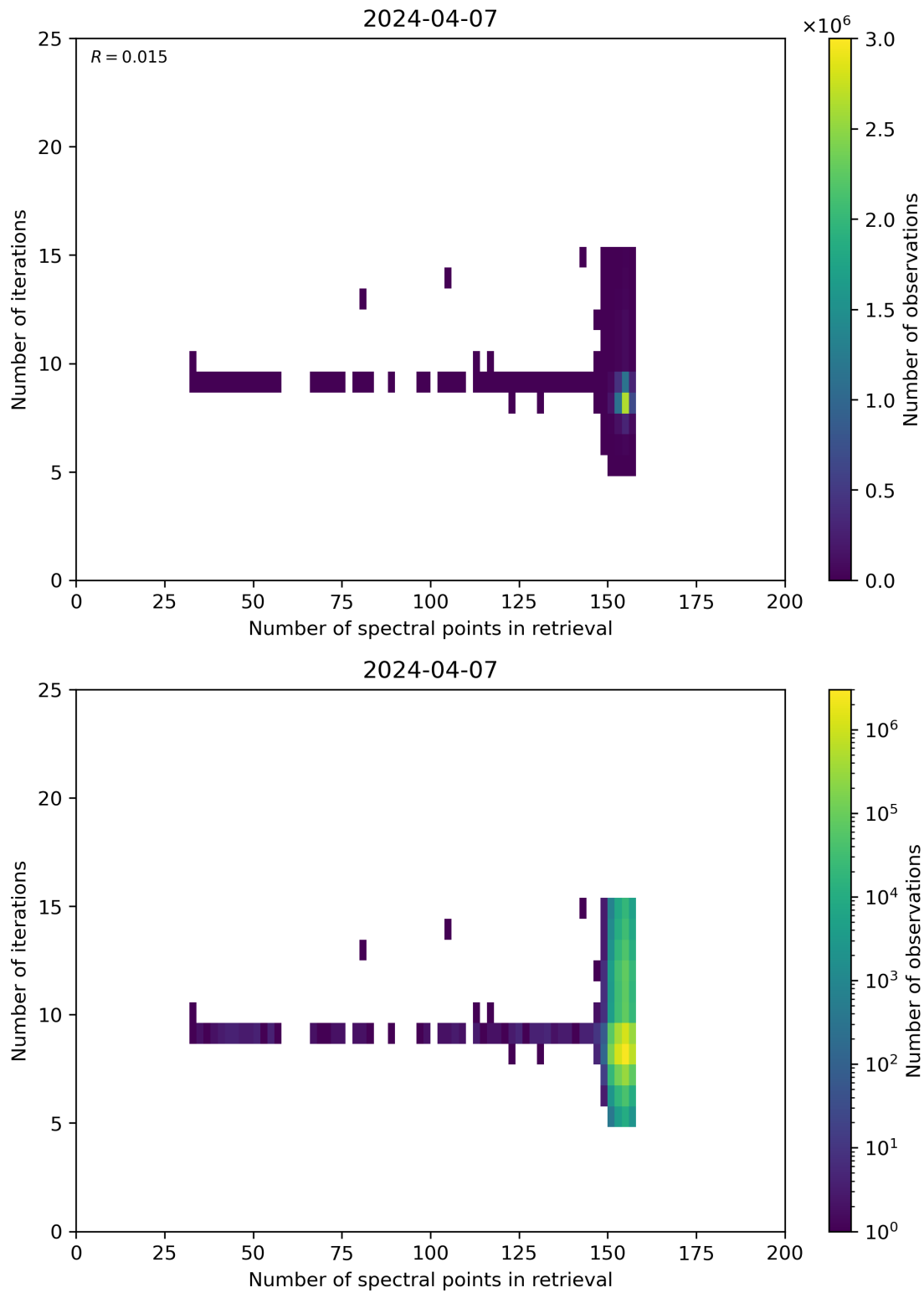
Figure 60: Scatter density plot of “Number of spectral points in retrieval” against “Number of iterations” for 2024-04-06 to 2024-04-08.
