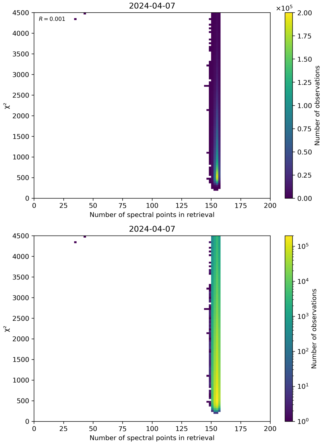
Figure 58: Scatter density plot of “Number of spectral points in retrieval” against “ \chi^2 ” for 2024-04-06 to 2024-04-08.
