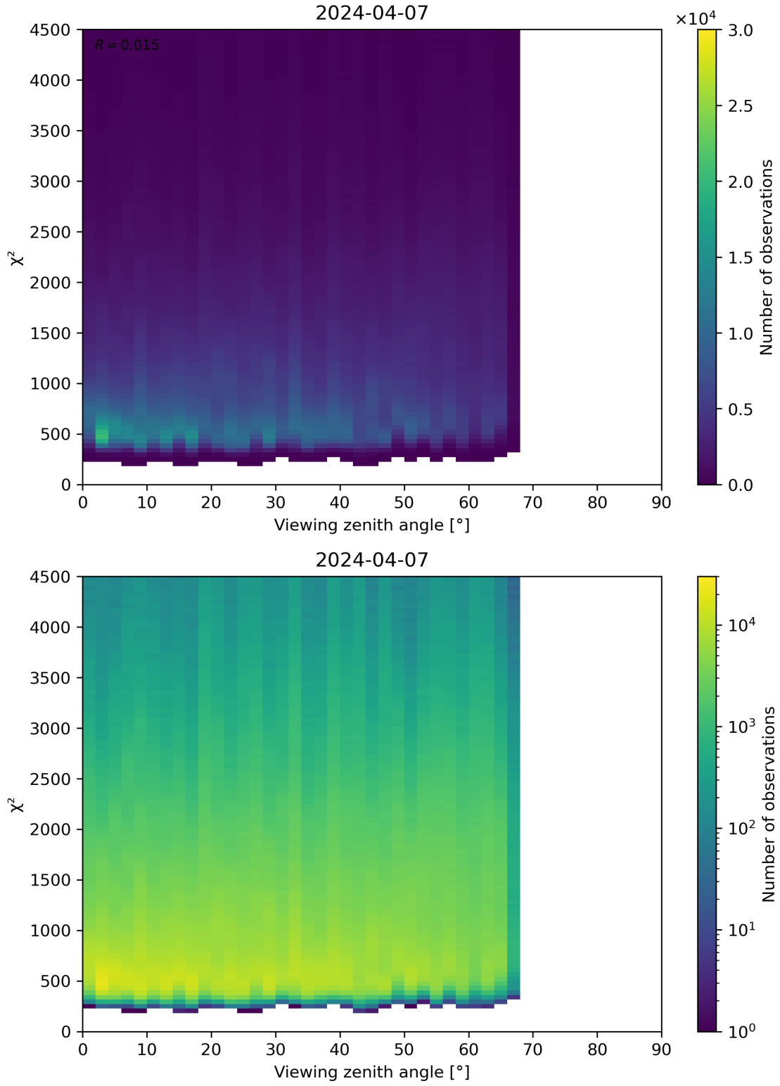
Figure 72: Scatter density plot of “Viewing zenith angle” against “ \chi^2 ” for 2024-04-06 to 2024-04-08.
