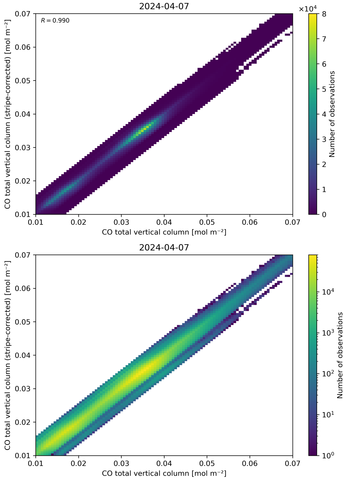
Figure 33: Scatter density plot of “CO total vertical column” against “CO total vertical column (stripe-corrected)” for 2024-04-06 to 2024-04-08.
