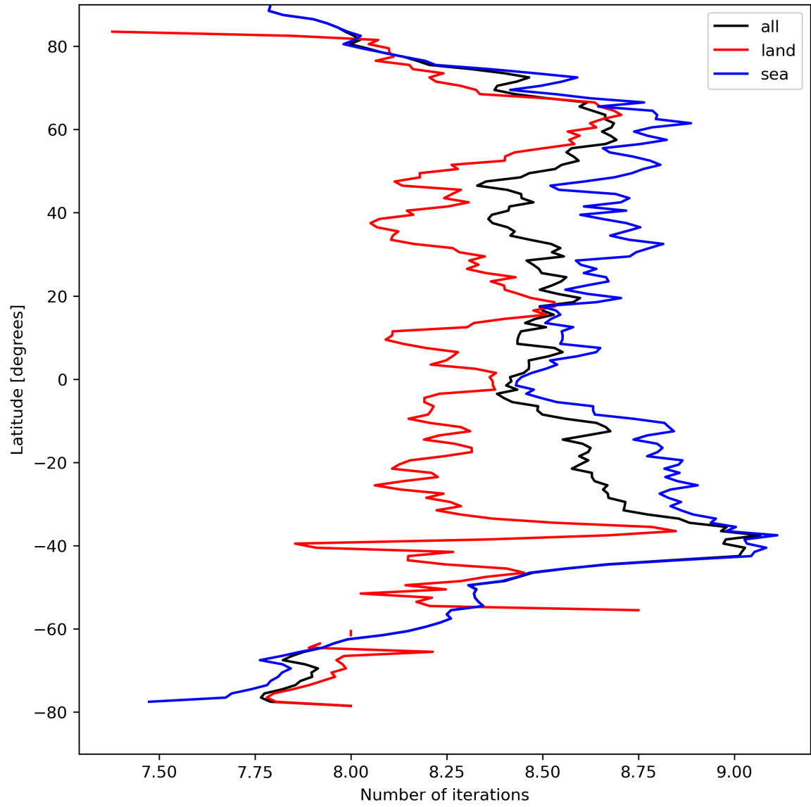
Figure 16: Zonal average of “Number of iterations” for 2024-04-06 to 2024-04-08.
