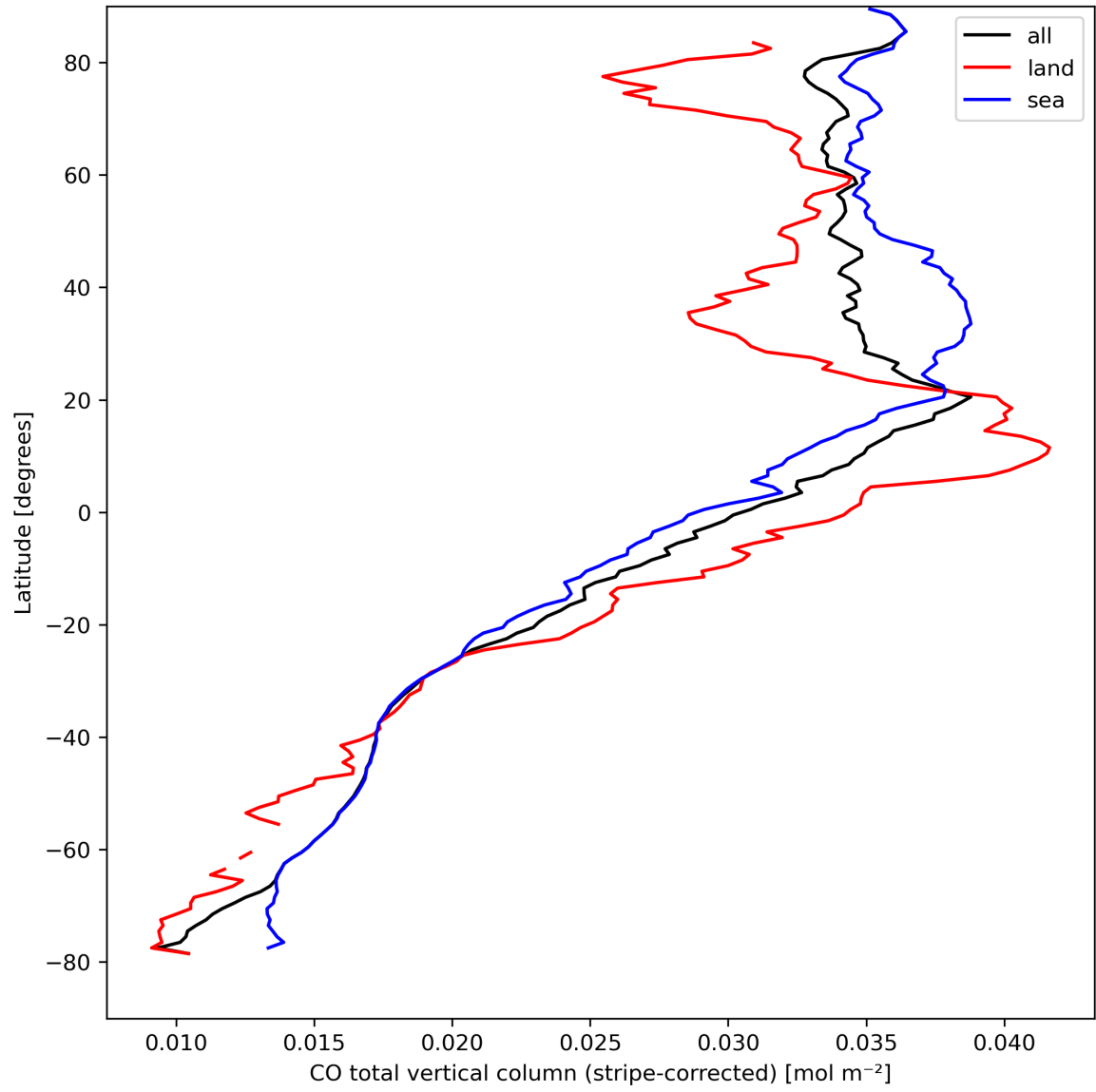
Figure 11: Zonal average of “CO total vertical column (stripe-corrected)” for 2024-04-06 to 2024-04-08.
