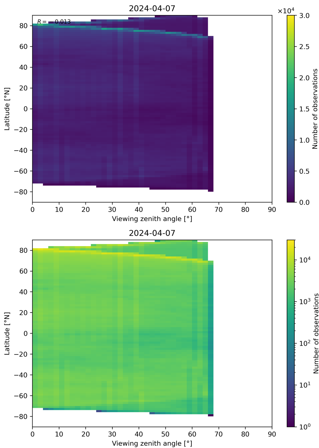
Figure 74: Scatter density plot of “Viewing zenith angle” against “Latitude” for 2024-04-06 to 2024-04-08.
