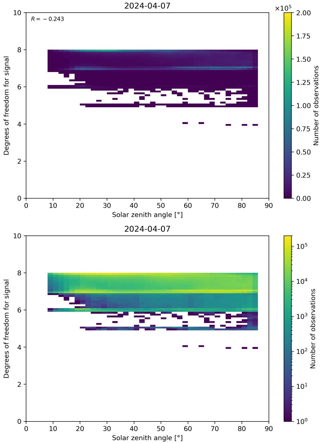
Figure 65: Scatter density plot of “Solar zenith angle” against “Degrees of freedom for signal” for 2024-04-06 to 2024-04-08.
