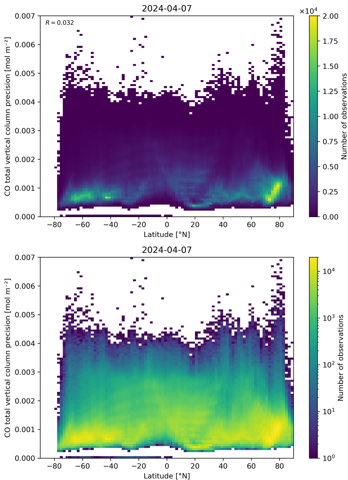
Figure 53: Scatter density plot of “Latitude” against “CO total vertical column precision” for 2024-04-06 to 2024-04-08.
