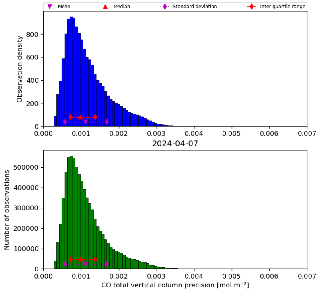
Figure 20: Histogram of “CO total vertical column precision” for 2024-04-06 to 2024-04-08
