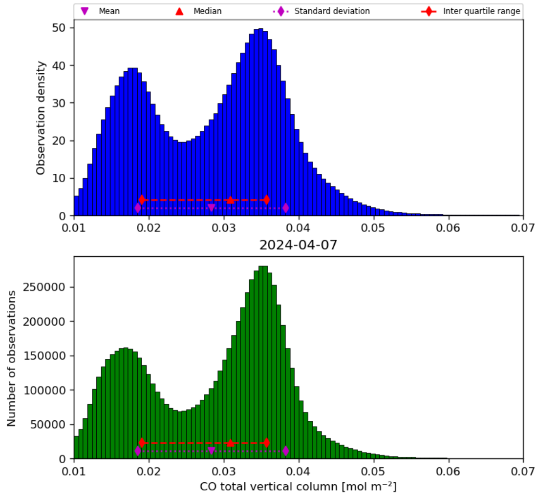
Figure 18: Histogram of “CO total vertical column” for 2024-04-06 to 2024-04-08
