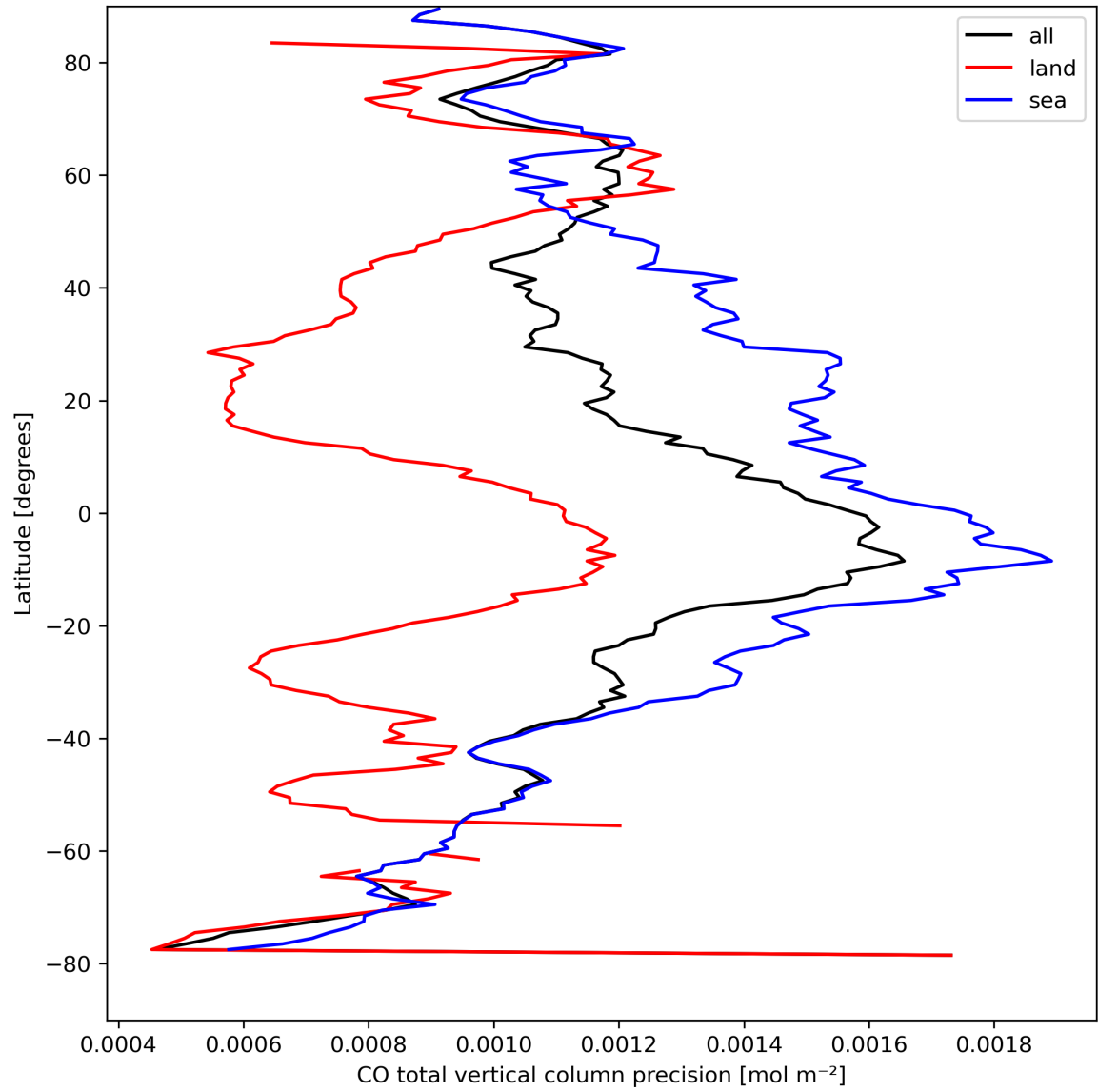
Figure 12: Zonal average of “CO total vertical column precision” for 2024-04-06 to 2024-04-08.
