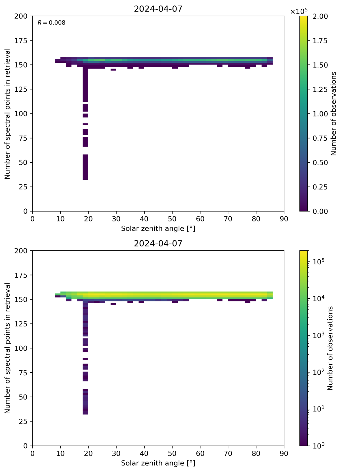
Figure 68: Scatter density plot of “Solar zenith angle” against “Number of spectral points in retrieval” for 2024-04-06 to 2024-04-08.
