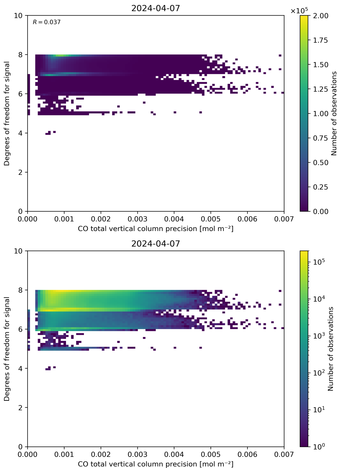
Figure 45: Scatter density plot of “CO total vertical column precision” against “Degrees of freedom for signal” for 2024-04-06 to 2024-04-08.
