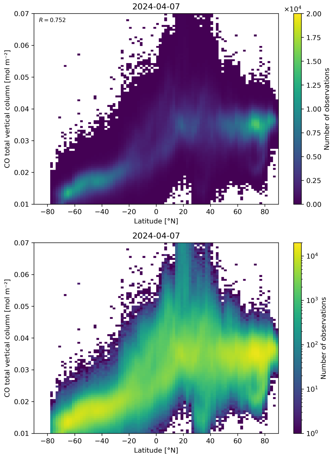
Figure 51: Scatter density plot of “Latitude” against “CO total vertical column” for 2024-04-06 to 2024-04-08.
