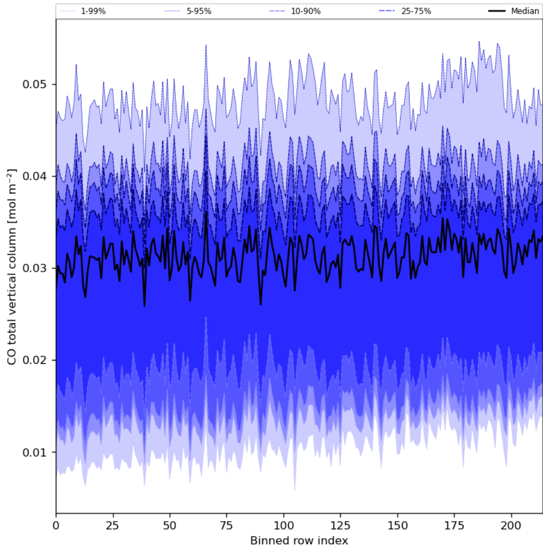
Figure 26: Along track statistics of “CO total vertical column” for 2024-04-06 to 2024-04-08
