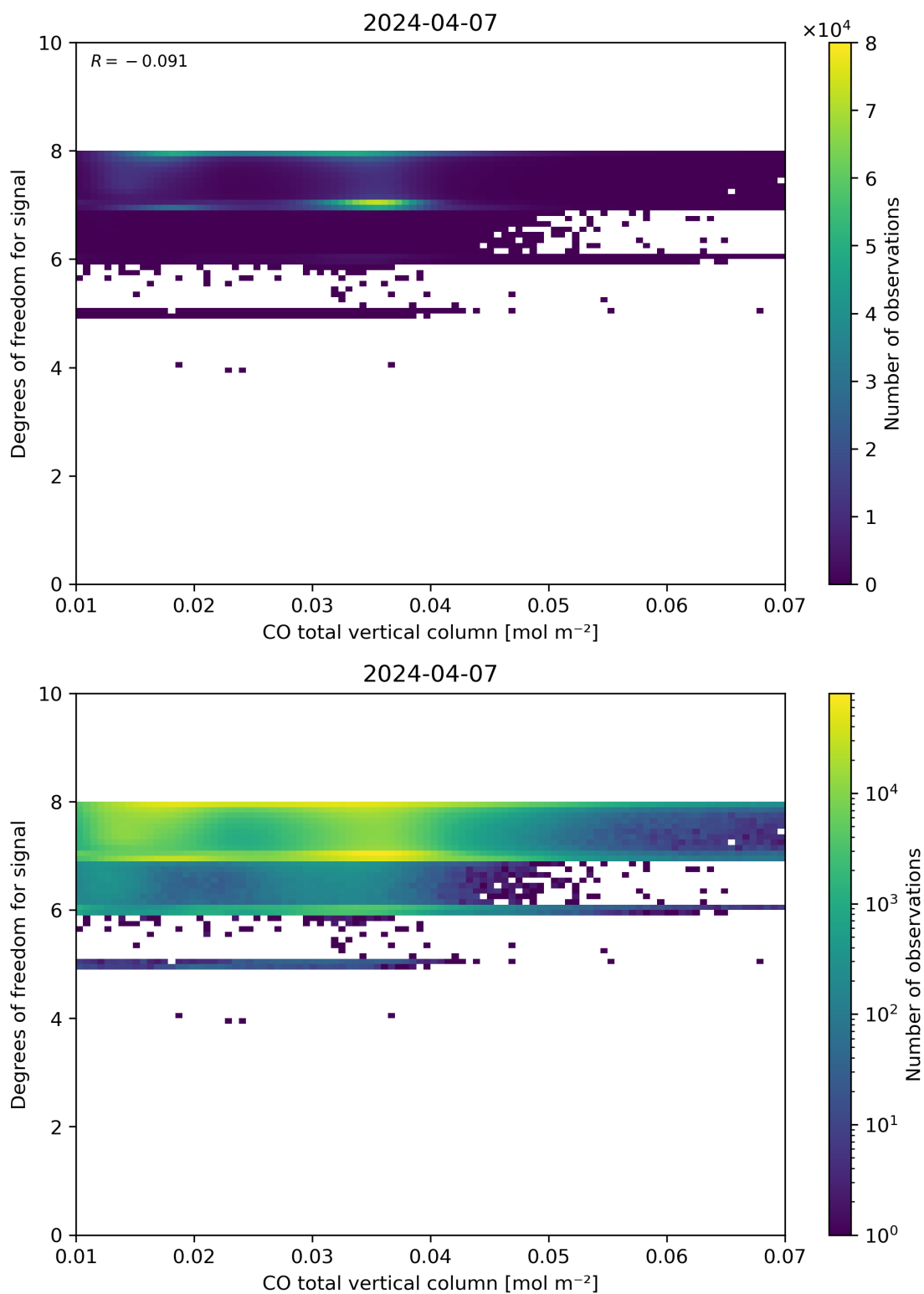
Figure 41: Scatter density plot of “CO total vertical column” against “Degrees of freedom for signal” for 2024-04-06 to 2024-04-08.
