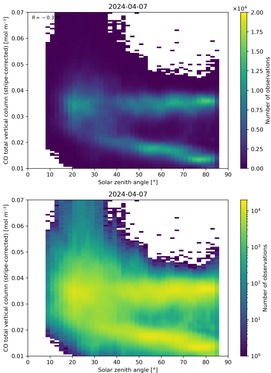
Figure 62: Scatter density plot of “Solar zenith angle” against “CO total vertical column (stripe-corrected)” for 2024-04-06 to 2024-04-08.
