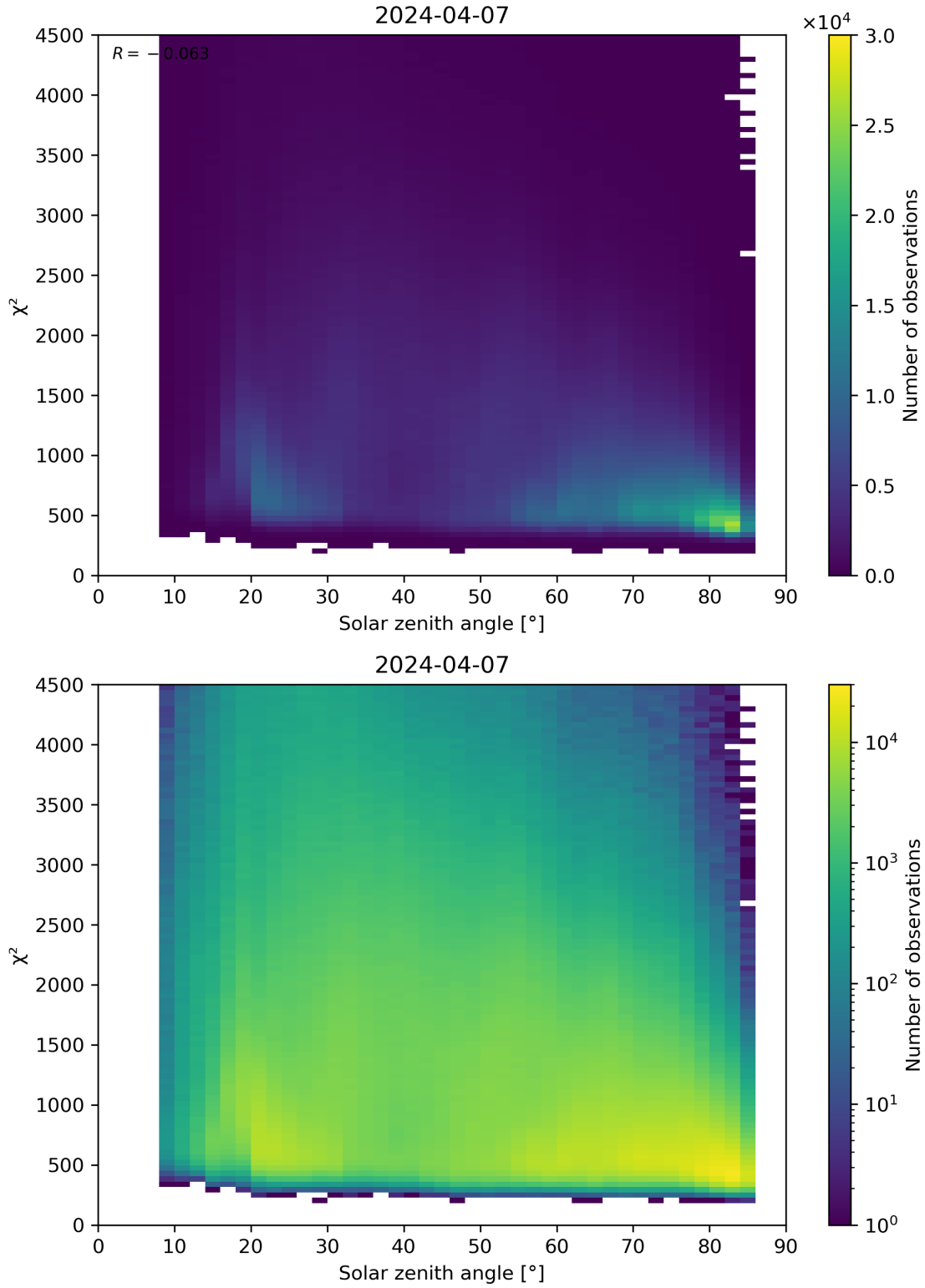
Figure 64: Scatter density plot of “Solar zenith angle” against “ \chi^2 ” for 2024-04-06 to 2024-04-08.
