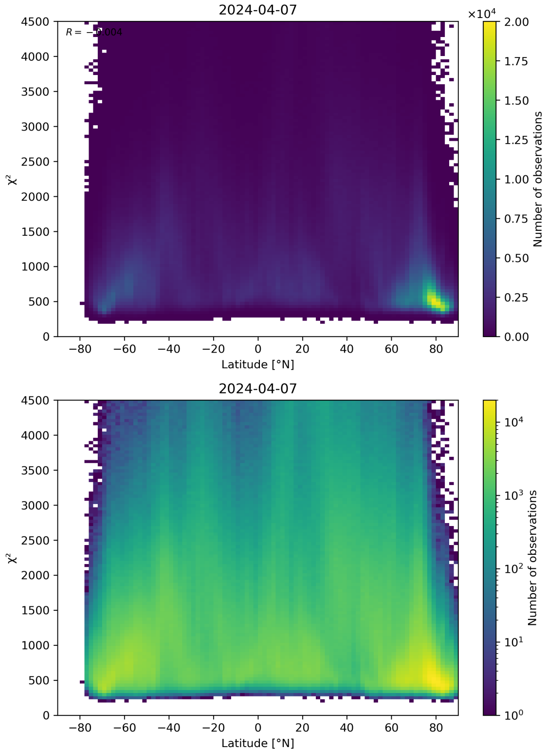
Figure 54: Scatter density plot of “Latitude” against “ \chi^2 ” for 2024-04-06 to 2024-04-08.
