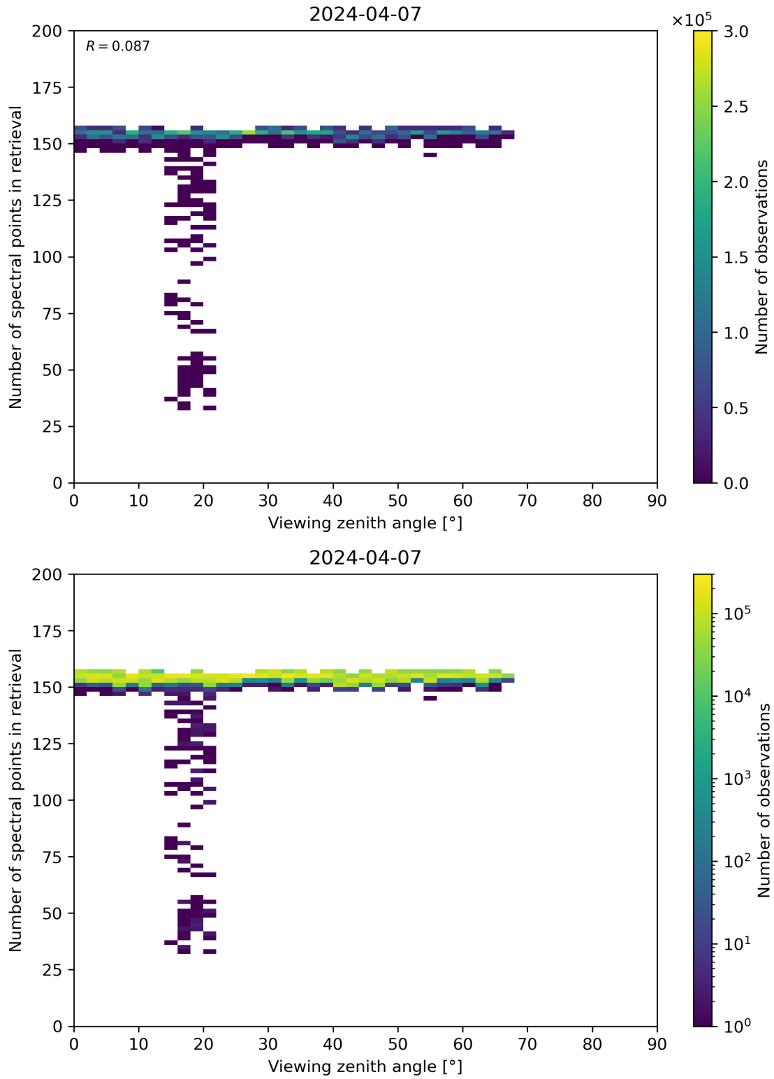
Figure 76: Scatter density plot of “Viewing zenith angle” against “Number of spectral points in retrieval” for 2024-04-06 to 2024-04-08.
