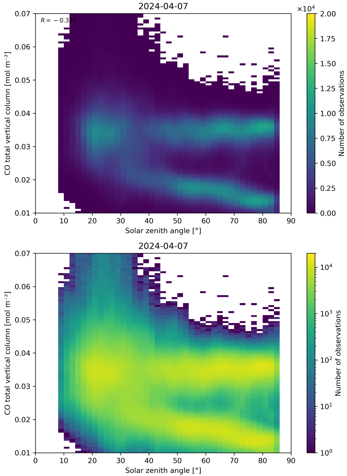
Figure 61: Scatter density plot of “Solar zenith angle” against “CO total vertical column” for 2024-04-06 to 2024-04-08.
