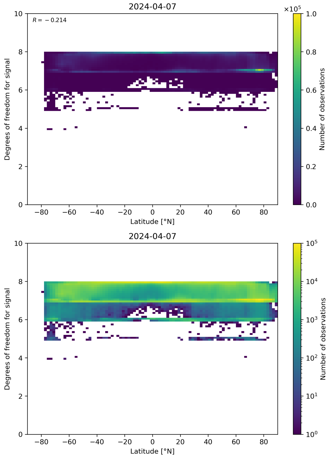
Figure 55: Scatter density plot of “Latitude” against “Degrees of freedom for signal” for 2024-04-06 to 2024-04-08.
