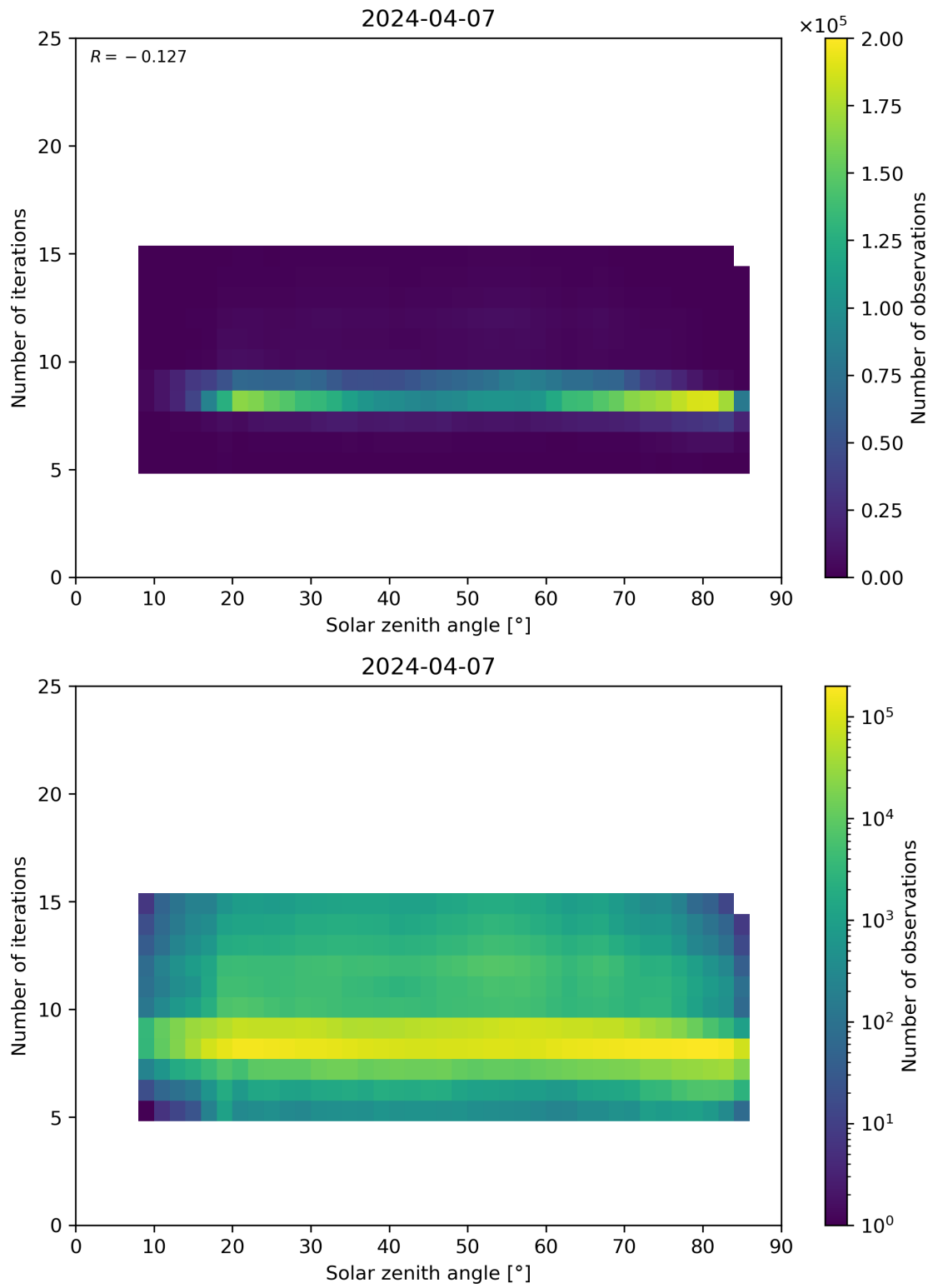
Figure 67: Scatter density plot of “Solar zenith angle” against “Number of iterations” for 2024-04-06 to 2024-04-08.
