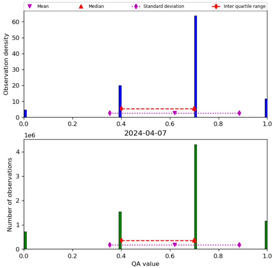
Figure 17: Histogram of “QA value” for 2024-04-06 to 2024-04-08
