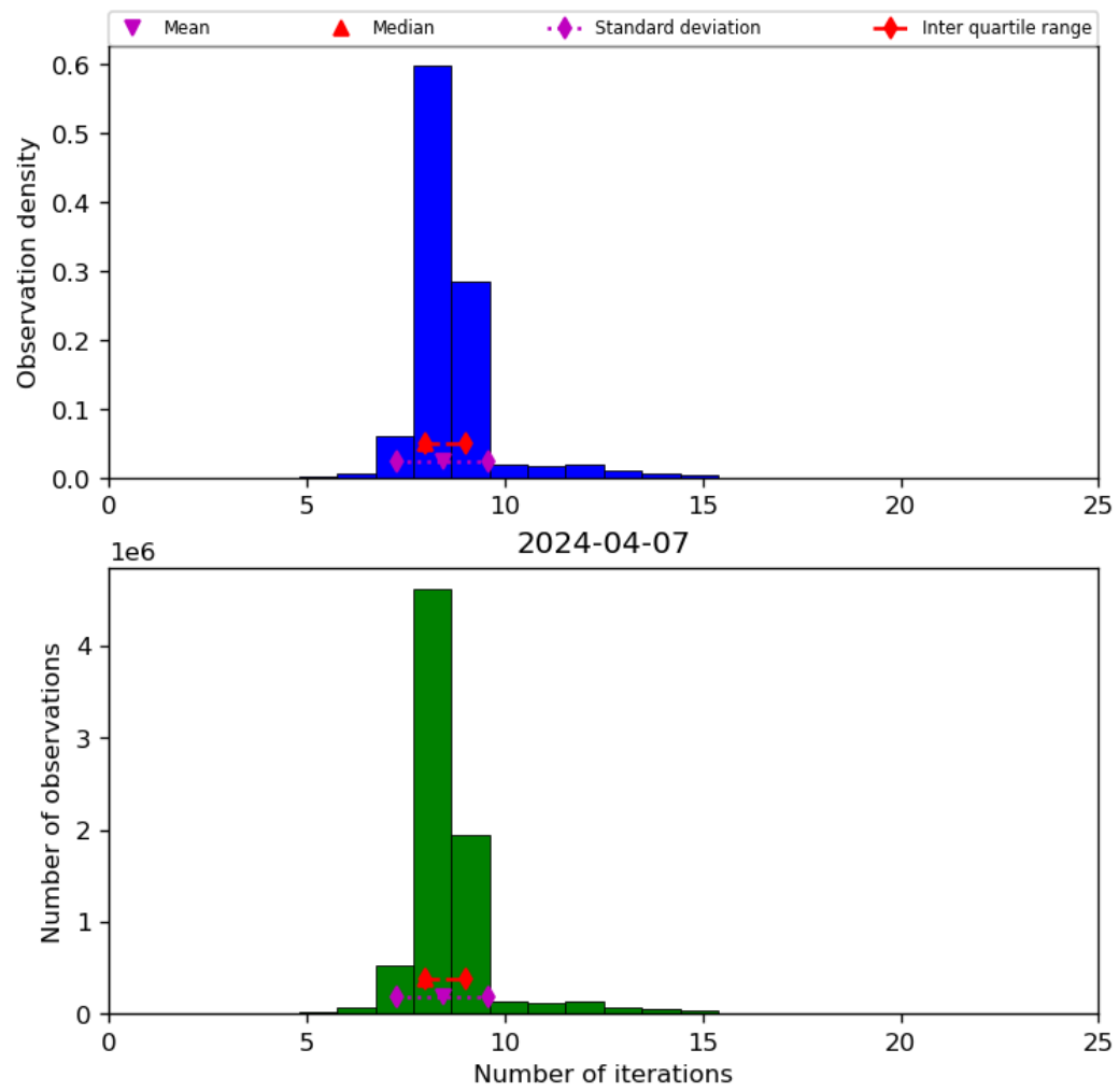
Figure 24: Histogram of “Number of iterations” for 2024-04-06 to 2024-04-08
