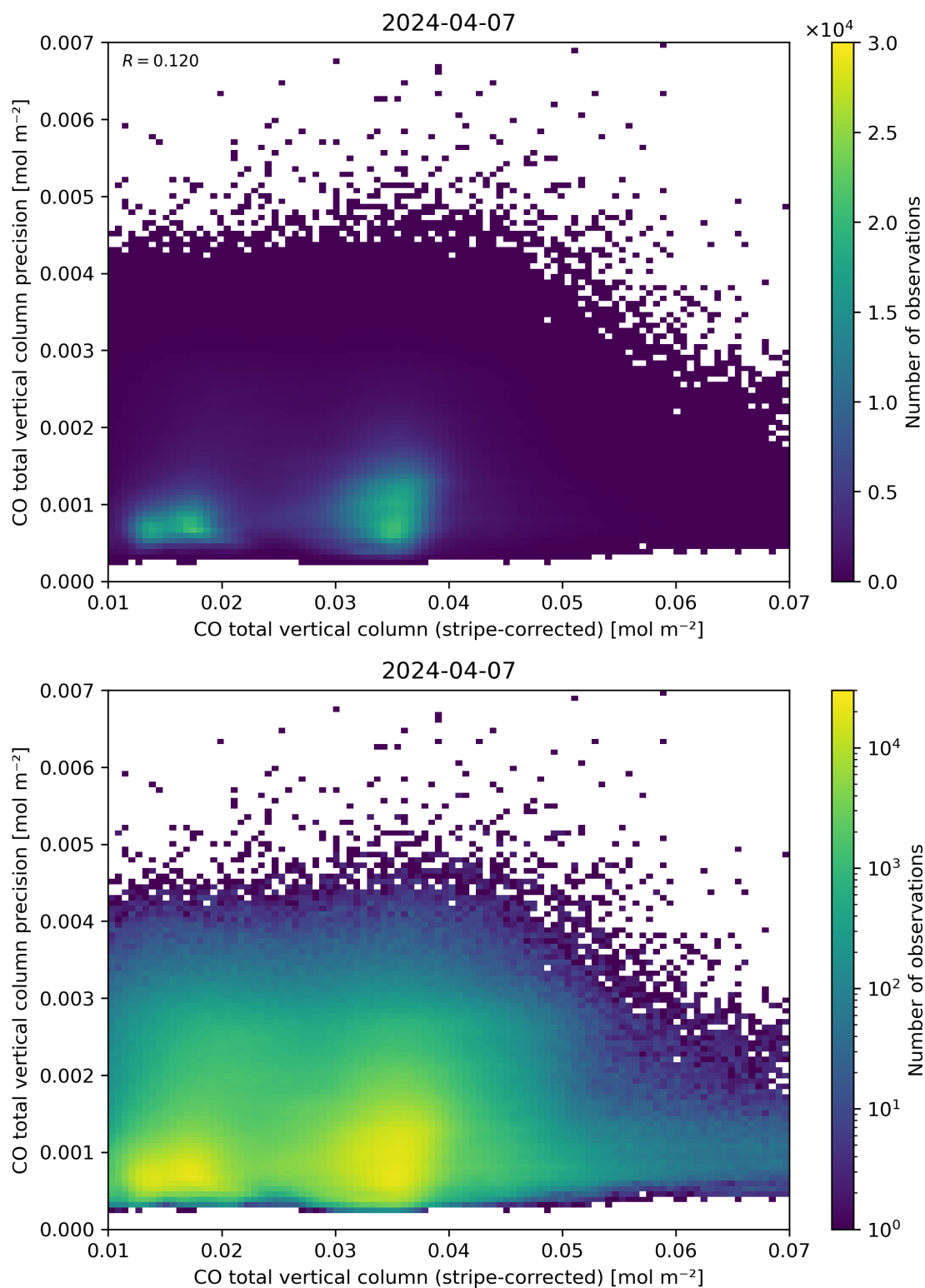
Figure 36: Scatter density plot of “CO total vertical column (stripe-corrected)” against “CO total vertical column precision” for 2024-04-06 to 2024-04-08.
