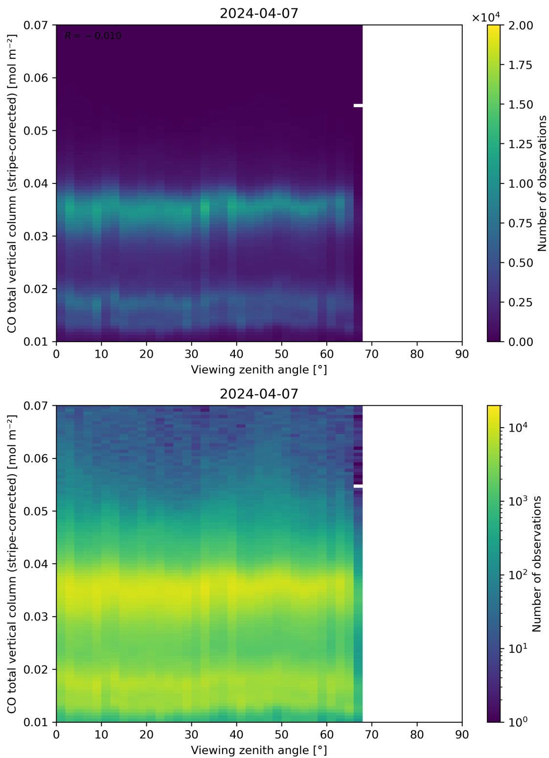
Figure 70: Scatter density plot of “Viewing zenith angle” against “CO total vertical column (stripe-corrected)” for 2024-04-06 to 2024-04-08.
