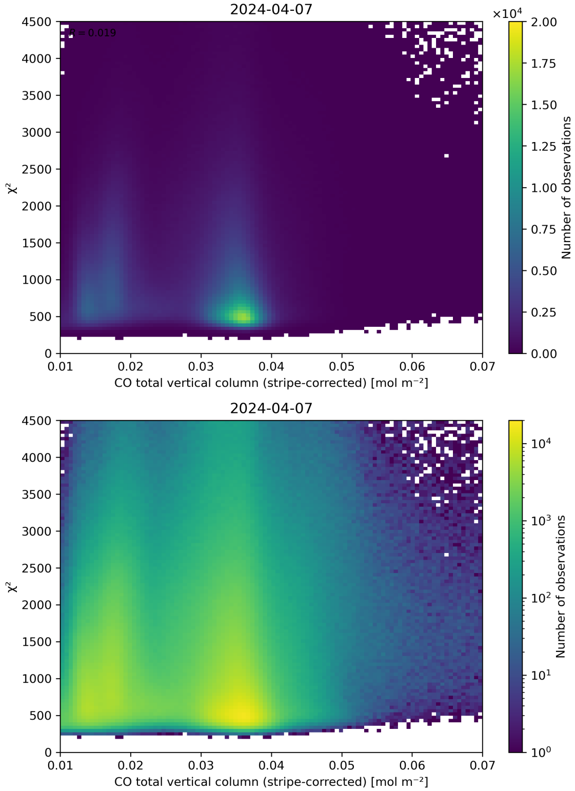
Figure 37: Scatter density plot of “CO total vertical column (stripe-corrected)” against “ \chi^2 ” for 2024-04-06 to 2024-04-08.
