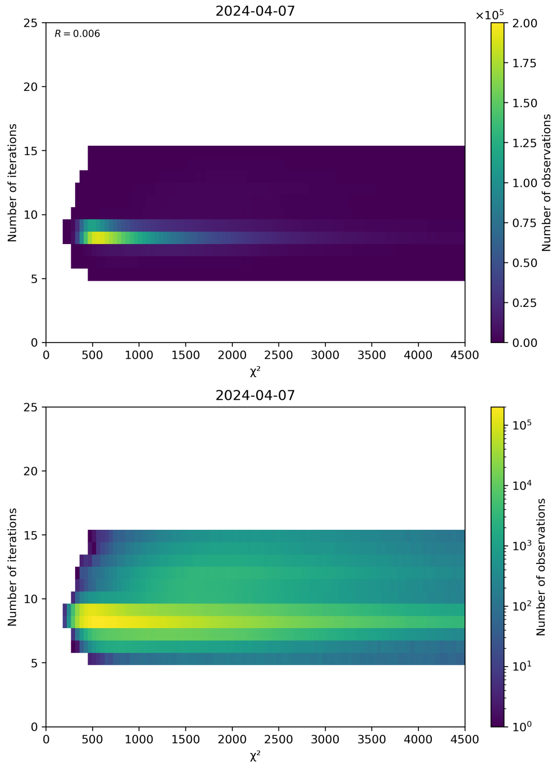
Figure 49: Scatter density plot of “ \chi^2 ” against “Number of iterations” for 2024-04-06 to 2024-04-08.
