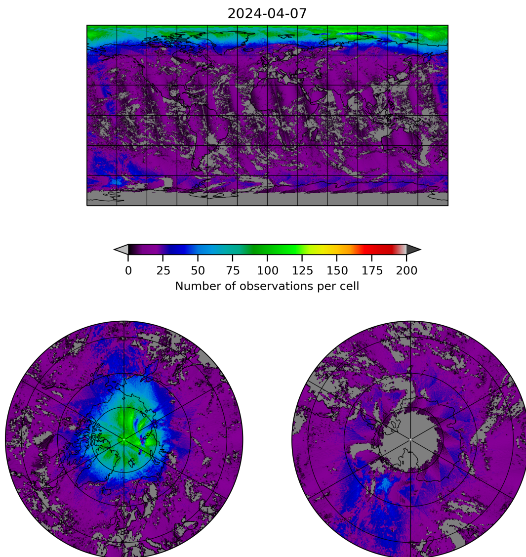
Figure 8: Map of the number of observations for 2024-04-06 to 2024-04-08
