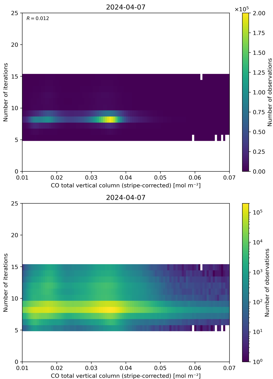
Figure 39: Scatter density plot of “CO total vertical column (stripe-corrected)” against “Number of iterations” for 2024-04-06 to 2024-04-08.
