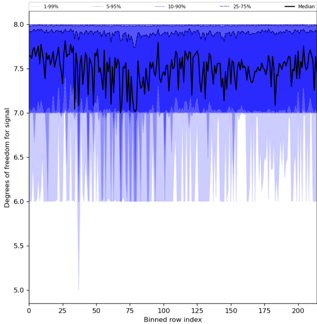
Figure 31: Along track statistics of “Degrees of freedom for signal” for 2024-04-06 to 2024-04-08
