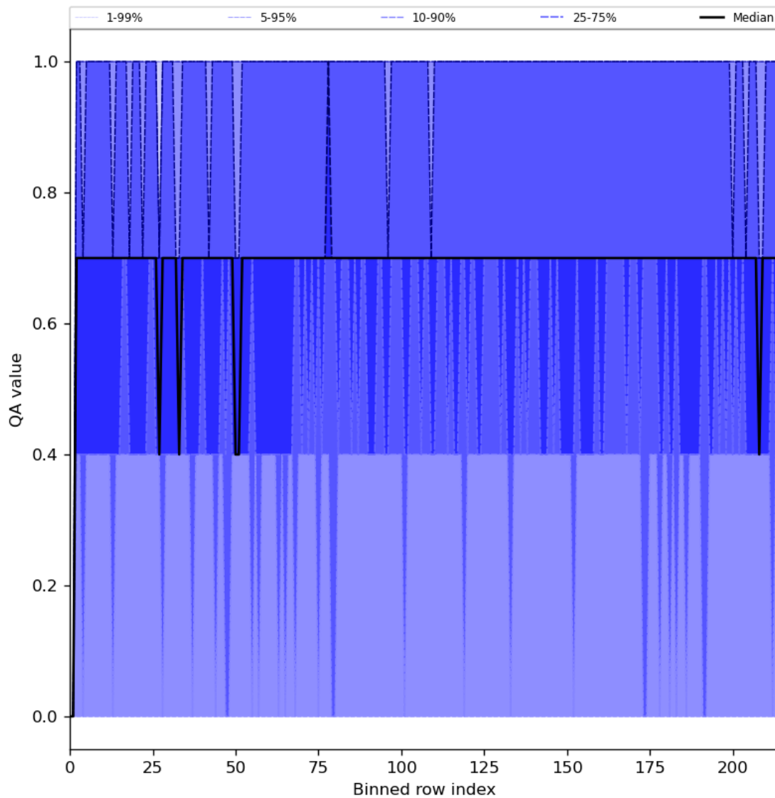
Figure 25: Along track statistics of “QA value” for 2024-04-06 to 2024-04-08
