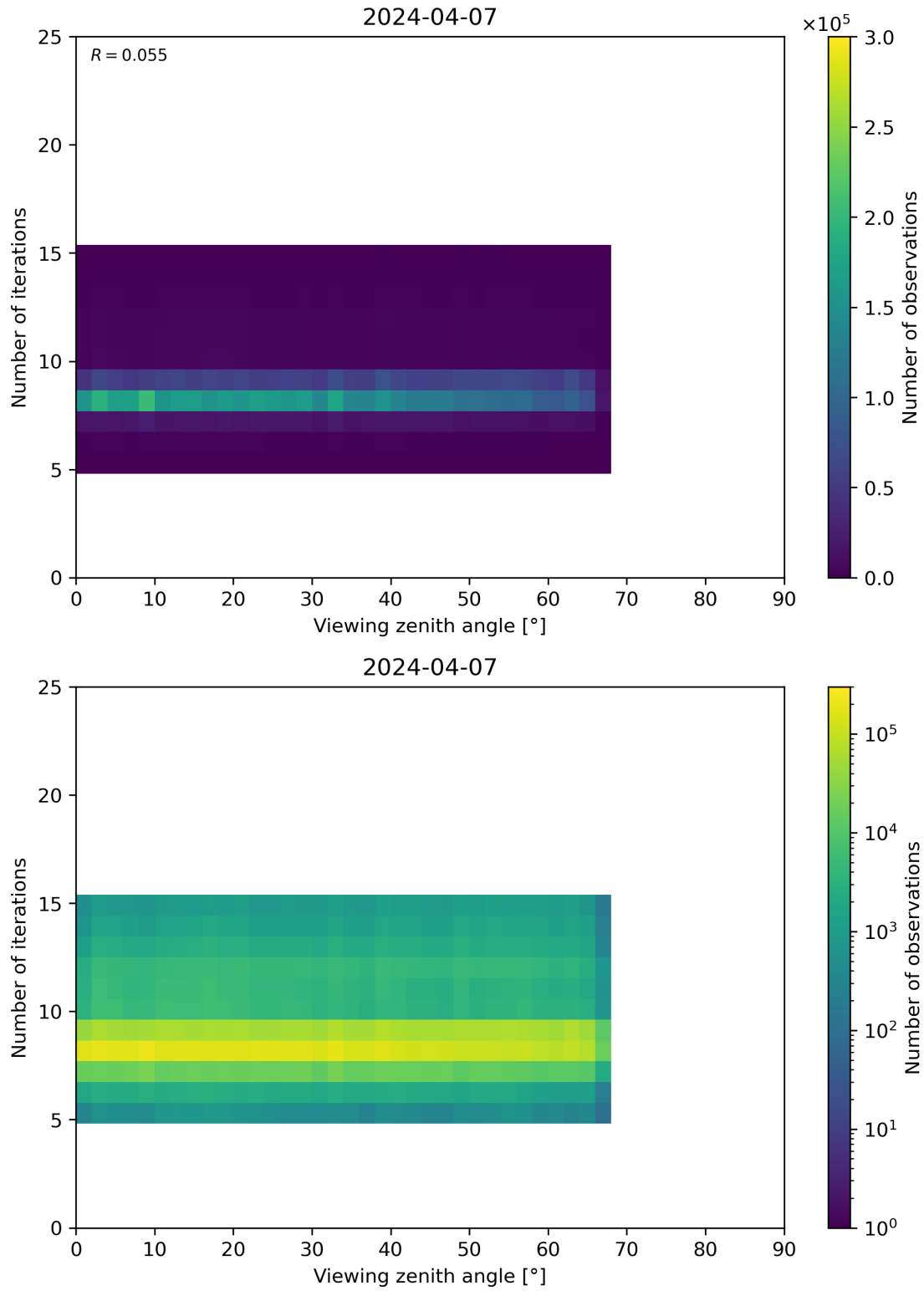
Figure 75: Scatter density plot of “Viewing zenith angle” against “Number of iterations” for 2024-04-06 to 2024-04-08.
