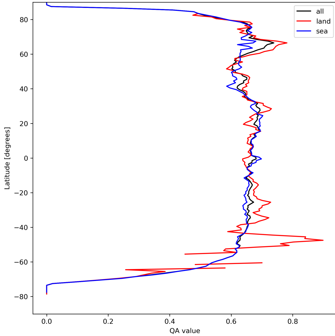
Figure 9: Zonal average of “QA value” for 2024-04-06 to 2024-04-08.
