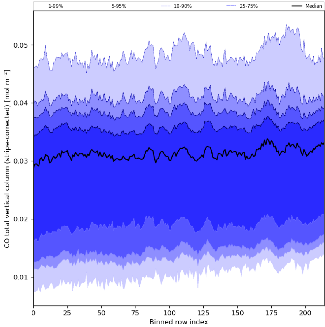
Figure 27: Along track statistics of “CO total vertical column (stripe-corrected)” for 2024-04-06 to 2024-04-08
