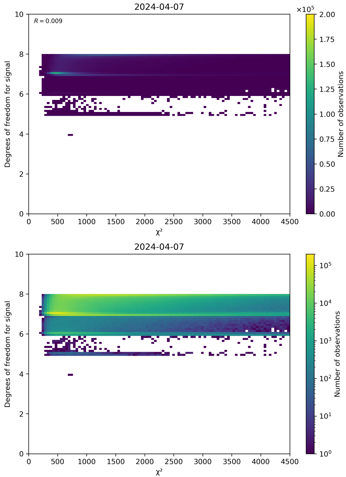
Figure 48: Scatter density plot of “ \chi^2 ” against “Degrees of freedom for signal” for 2024-04-06 to 2024-04-08.
