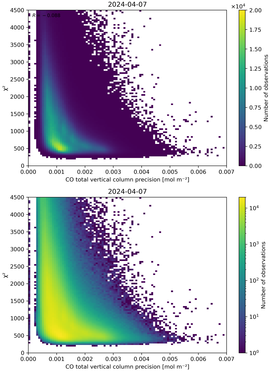
Figure 44: Scatter density plot of “CO total vertical column precision” against “ \chi^2 ” for 2024-04-06 to 2024-04-08.
