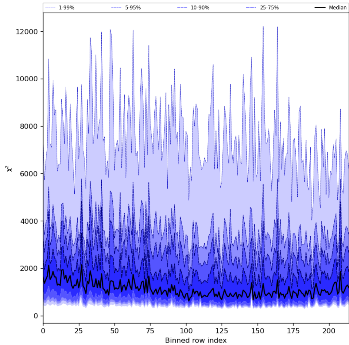
Figure 30: Along track statistics of “ \chi^2 ” for 2024-04-06 to 2024-04-08
