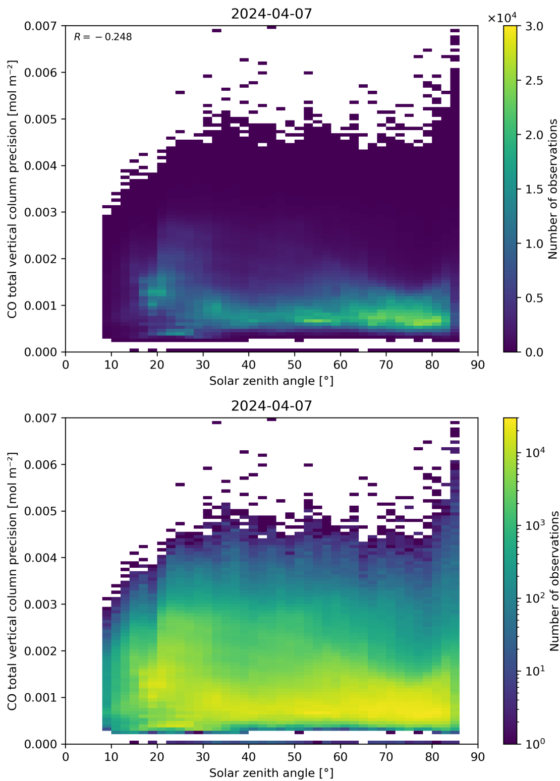
Figure 63: Scatter density plot of “Solar zenith angle” against “CO total vertical column precision” for 2024-04-06 to 2024-04-08.
