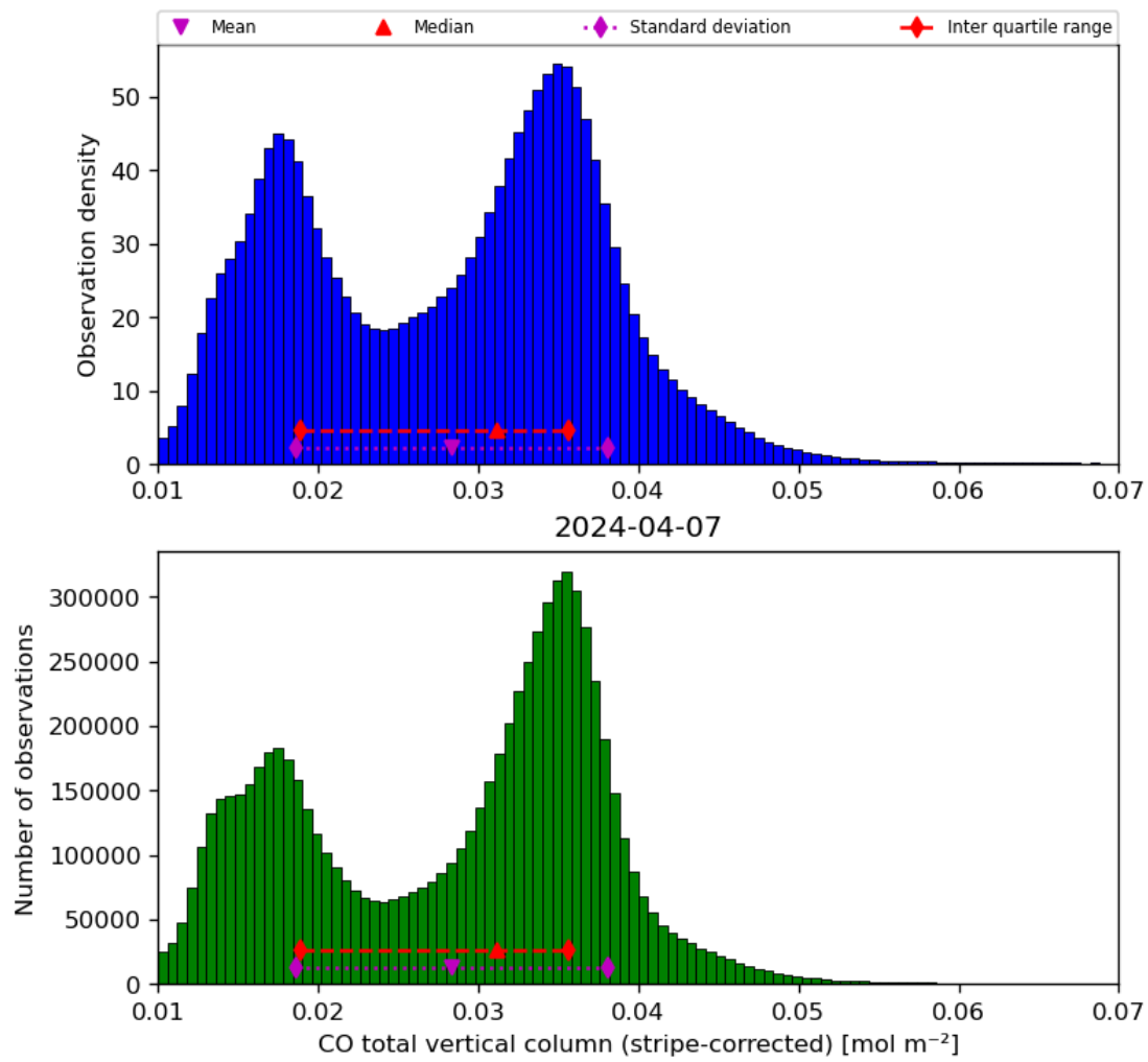
Figure 19: Histogram of “CO total vertical column (stripe-corrected)” for 2024-04-06 to 2024-04-08
