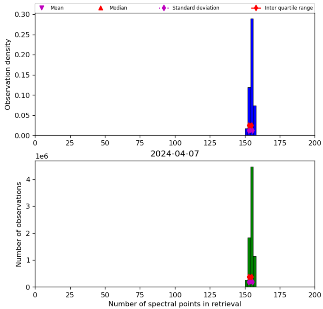
Figure 21: Histogram of “Number of spectral points in retrieval” for 2024-04-06 to 2024-04-08
