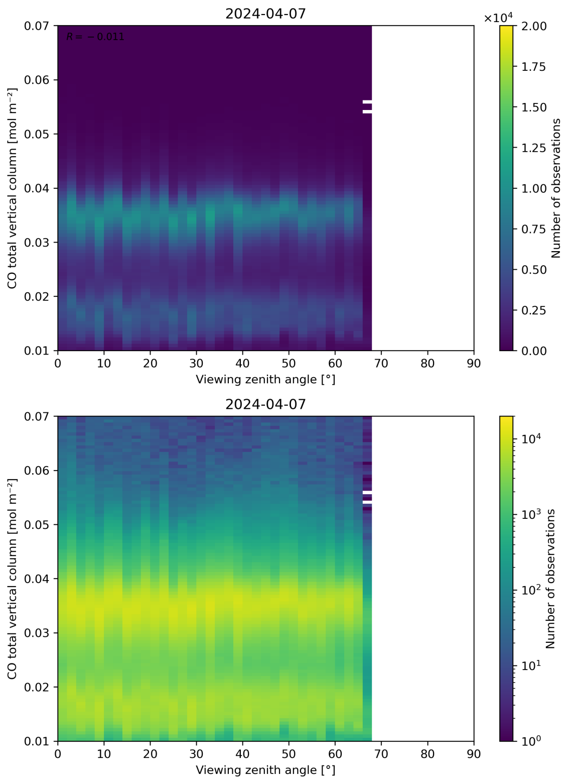
Figure 69: Scatter density plot of “Viewing zenith angle” against “CO total vertical column” for 2024-04-06 to 2024-04-08.
