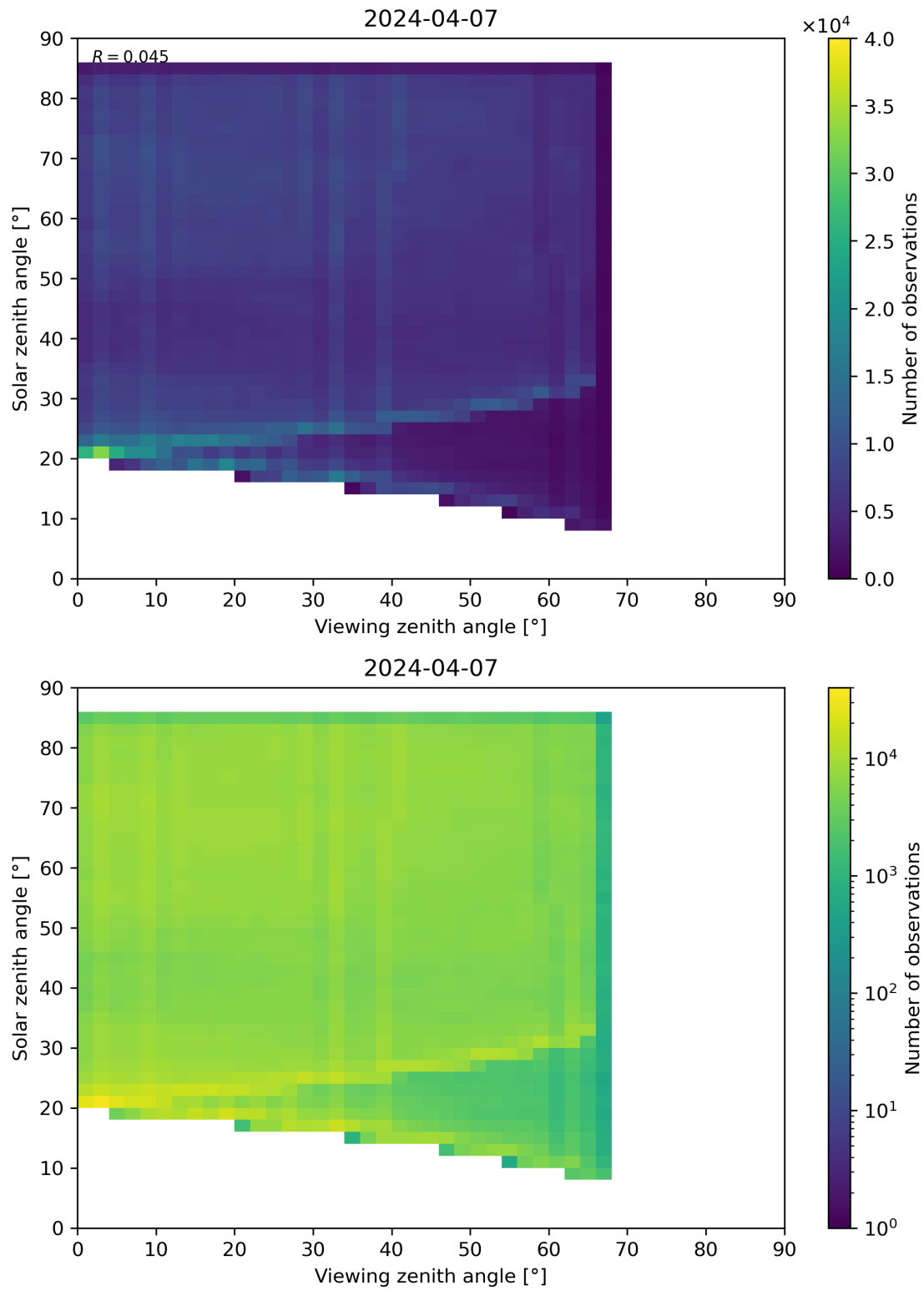
Figure 77: Scatter density plot of “Viewing zenith angle” against “Solar zenith angle” for 2024-04-06 to 2024-04-08.
