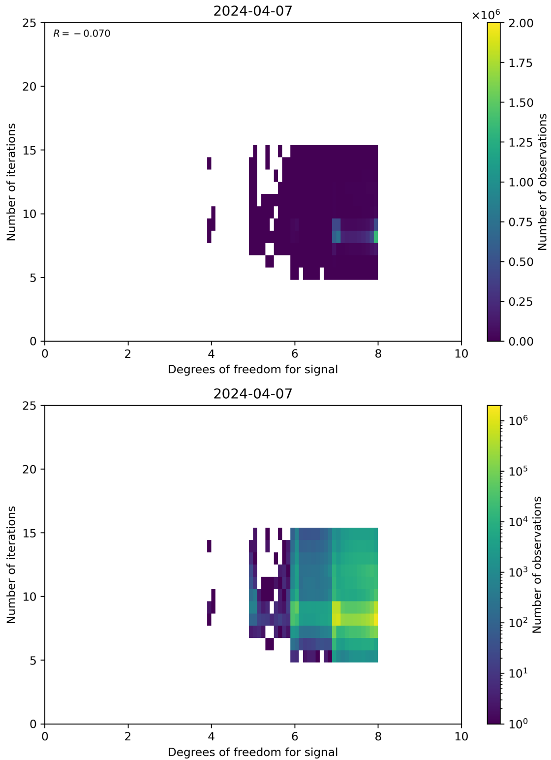
Figure 50: Scatter density plot of “Degrees of freedom for signal” against “Number of iterations” for 2024-04-06 to 2024-04-08.
