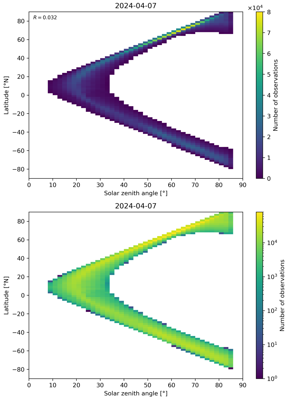
Figure 66: Scatter density plot of “Solar zenith angle” against “Latitude” for 2024-04-06 to 2024-04-08.
