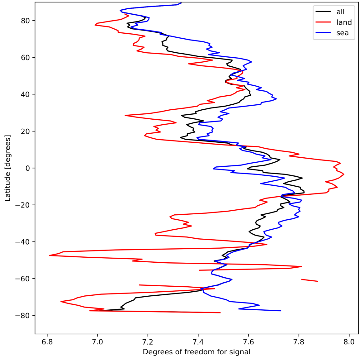
Figure 15: Zonal average of “Degrees of freedom for signal” for 2024-04-06 to 2024-04-08.
