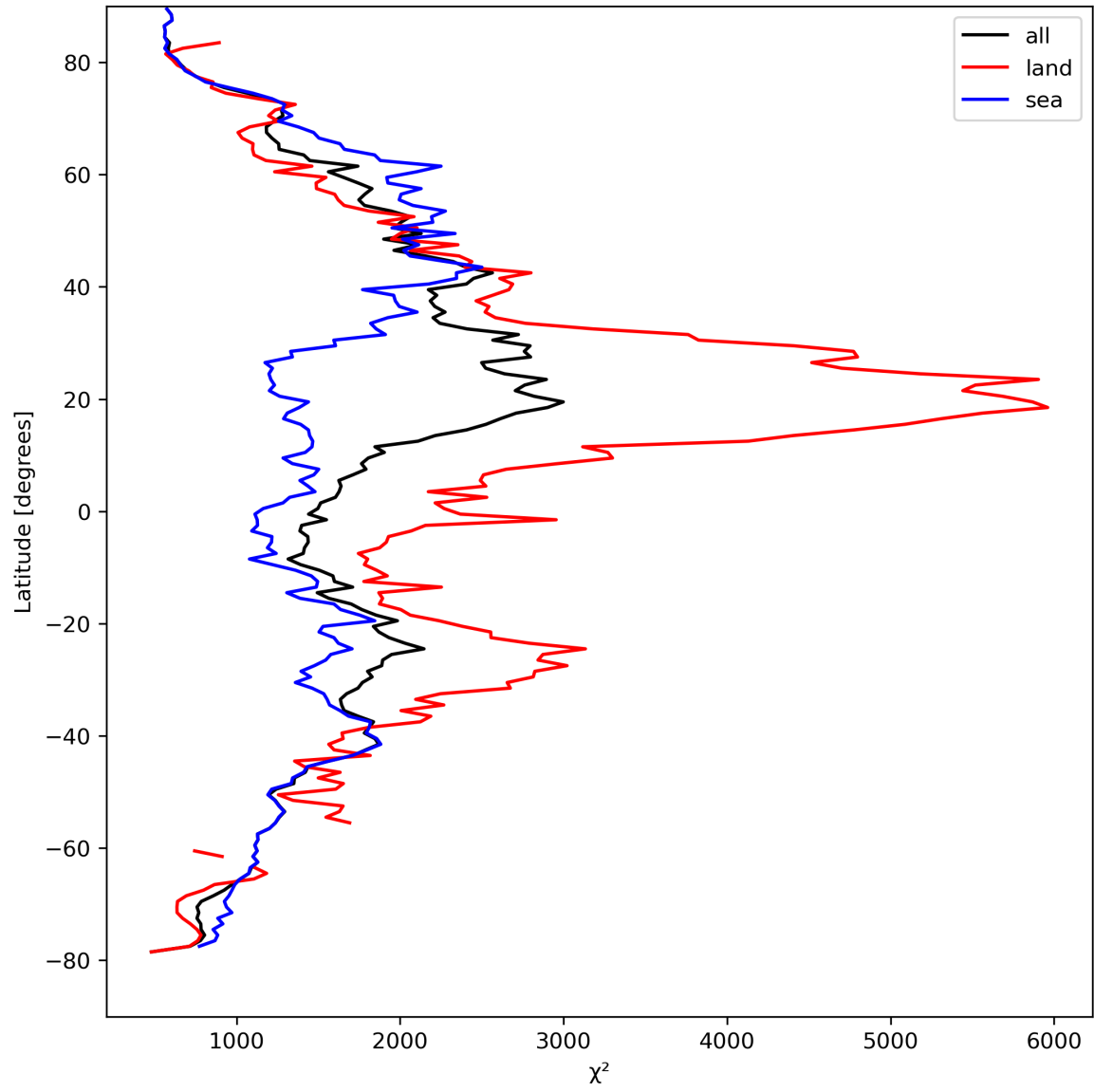
Figure 14: Zonal average of “ \chi^2 ” for 2024-04-06 to 2024-04-08.
