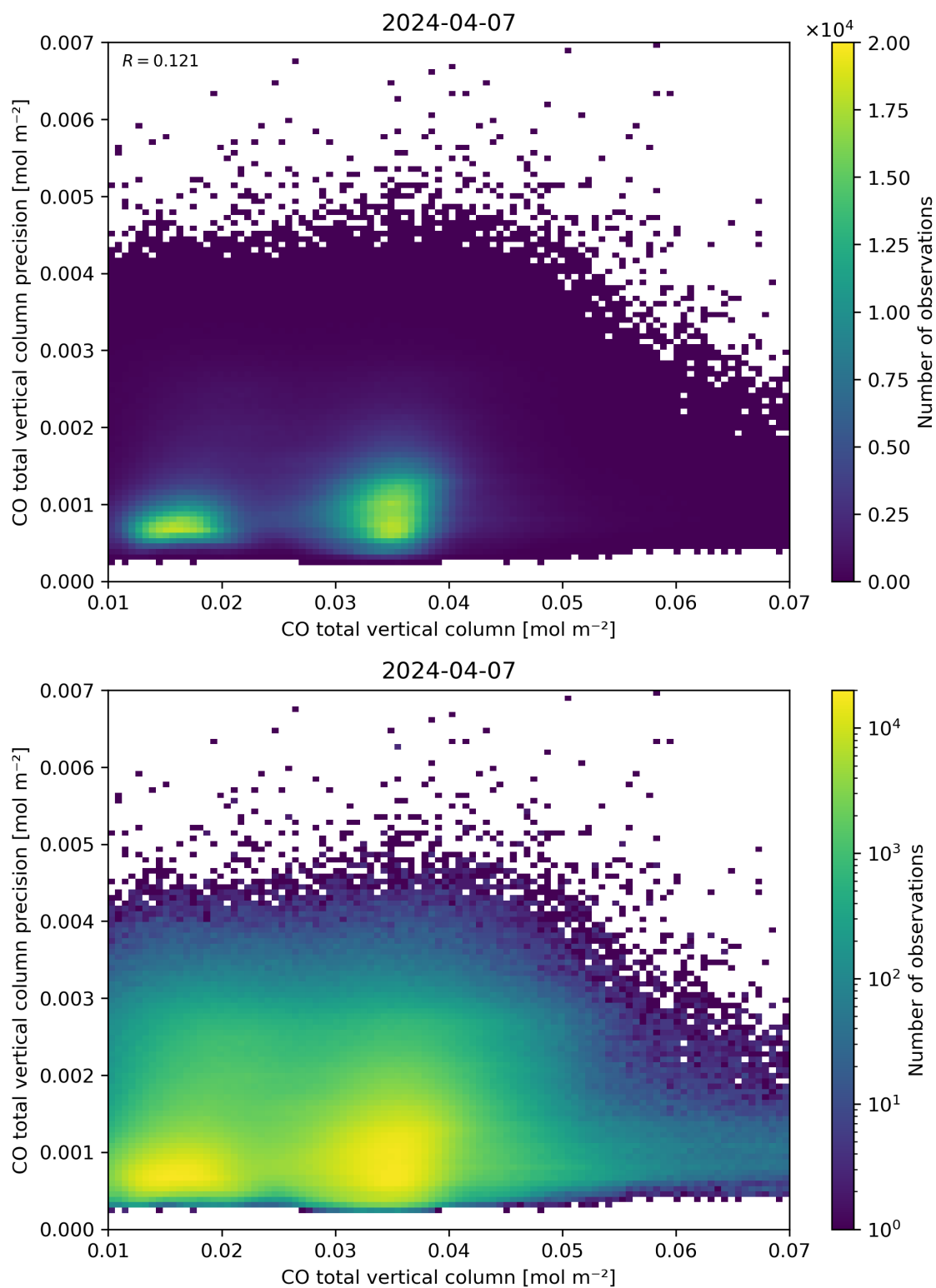
Figure 34: Scatter density plot of “CO total vertical column” against “CO total vertical column precision” for 2024-04-06 to 2024-04-08.
