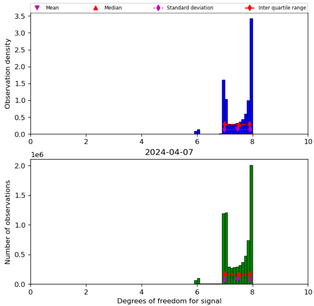
Figure 23: Histogram of “Degrees of freedom for signal” for 2024-04-06 to 2024-04-08
