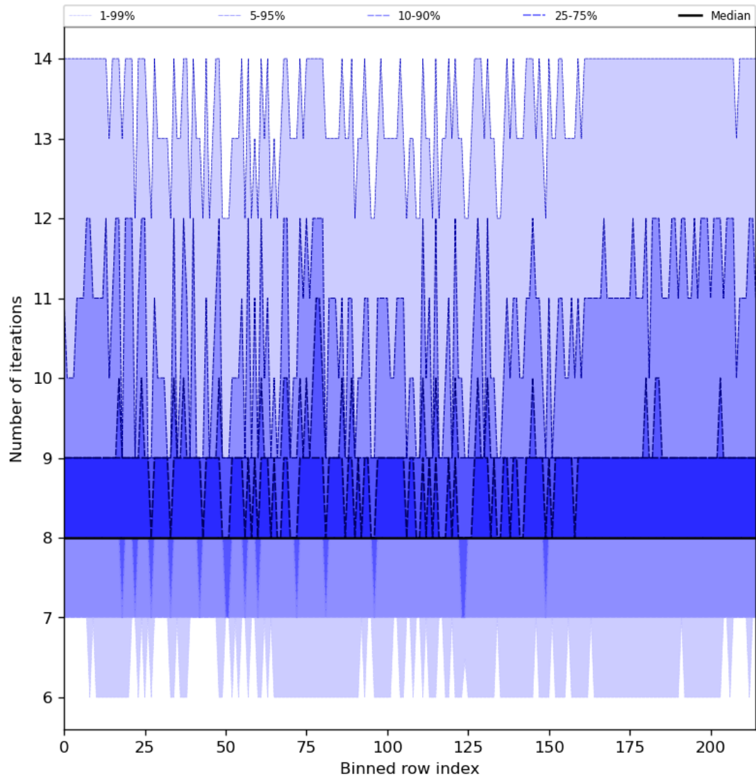
Figure 32: Along track statistics of “Number of iterations” for 2024-04-06 to 2024-04-08
