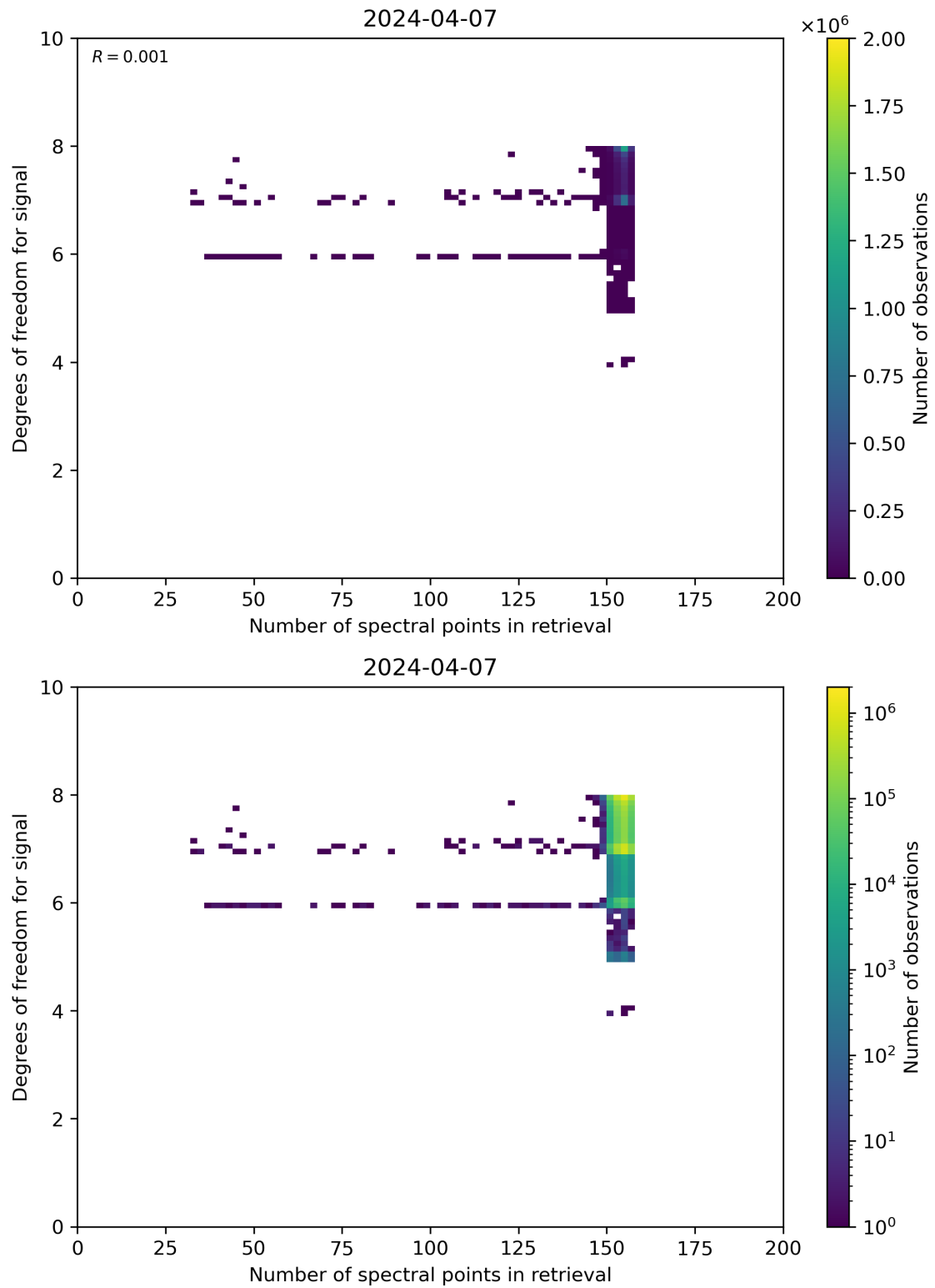
Figure 59: Scatter density plot of “Number of spectral points in retrieval” against “Degrees of freedom for signal” for 2024-04-06 to 2024-04-08.
