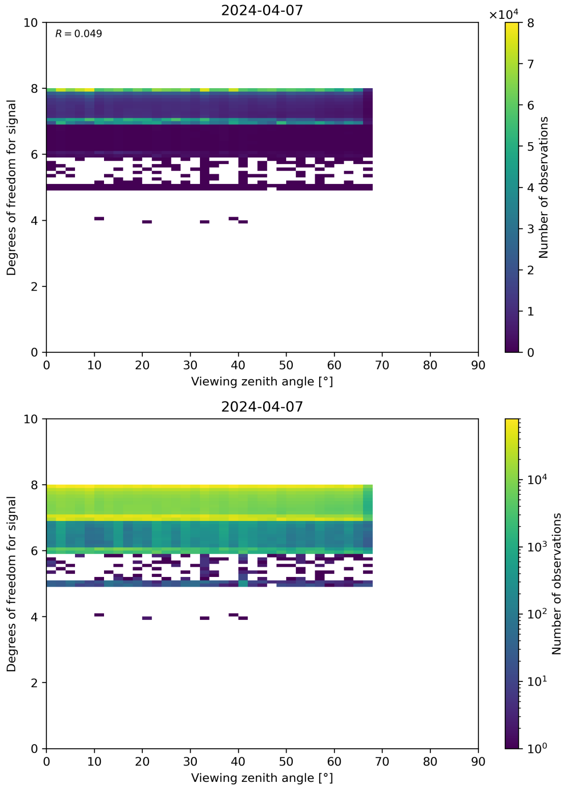
Figure 73: Scatter density plot of “Viewing zenith angle” against “Degrees of freedom for signal” for 2024-04-06 to 2024-04-08.
