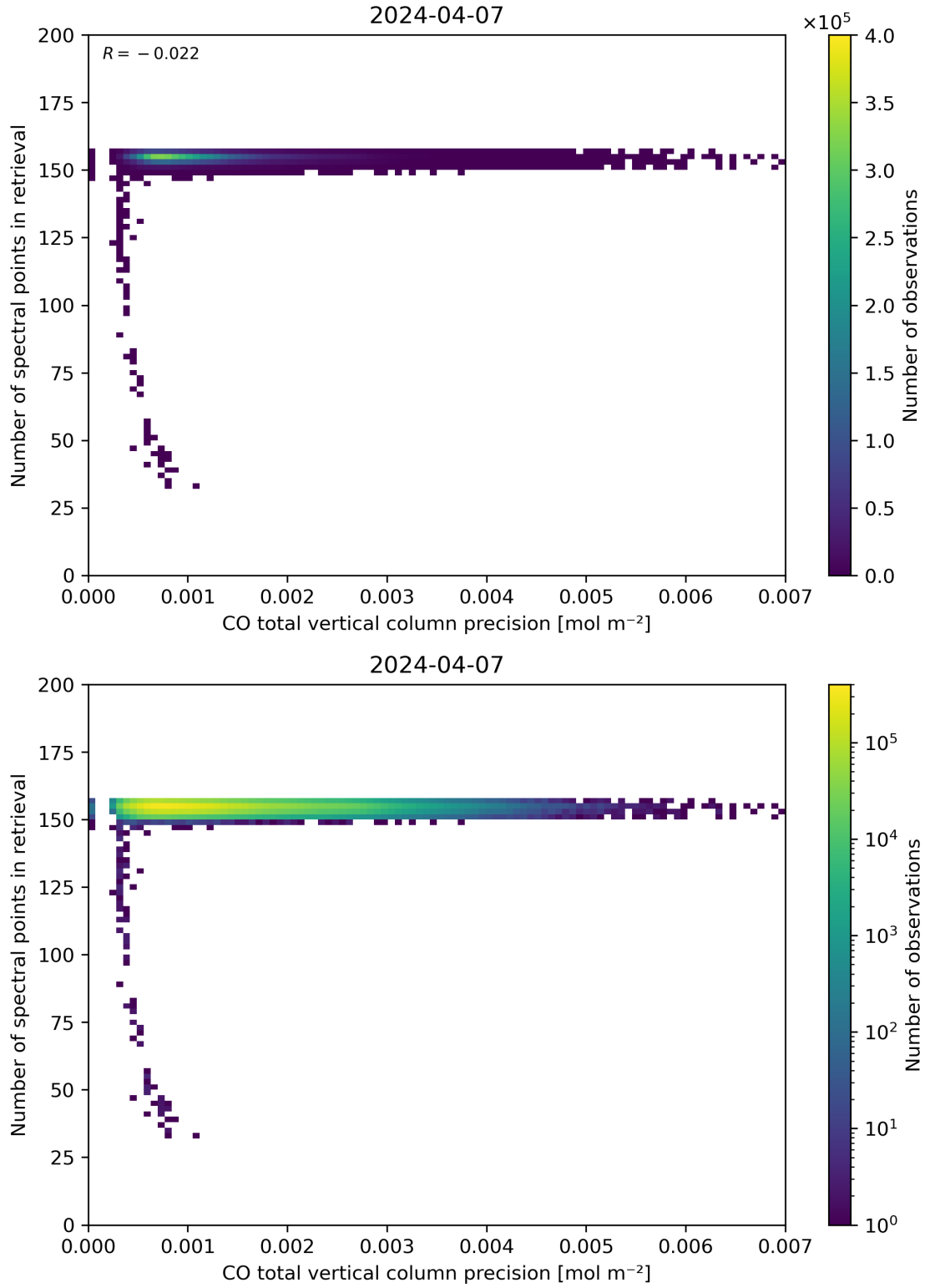
Figure 47: Scatter density plot of “CO total vertical column precision” against “Number of spectral points in retrieval” for 2024-04-06 to 2024-04-08.
