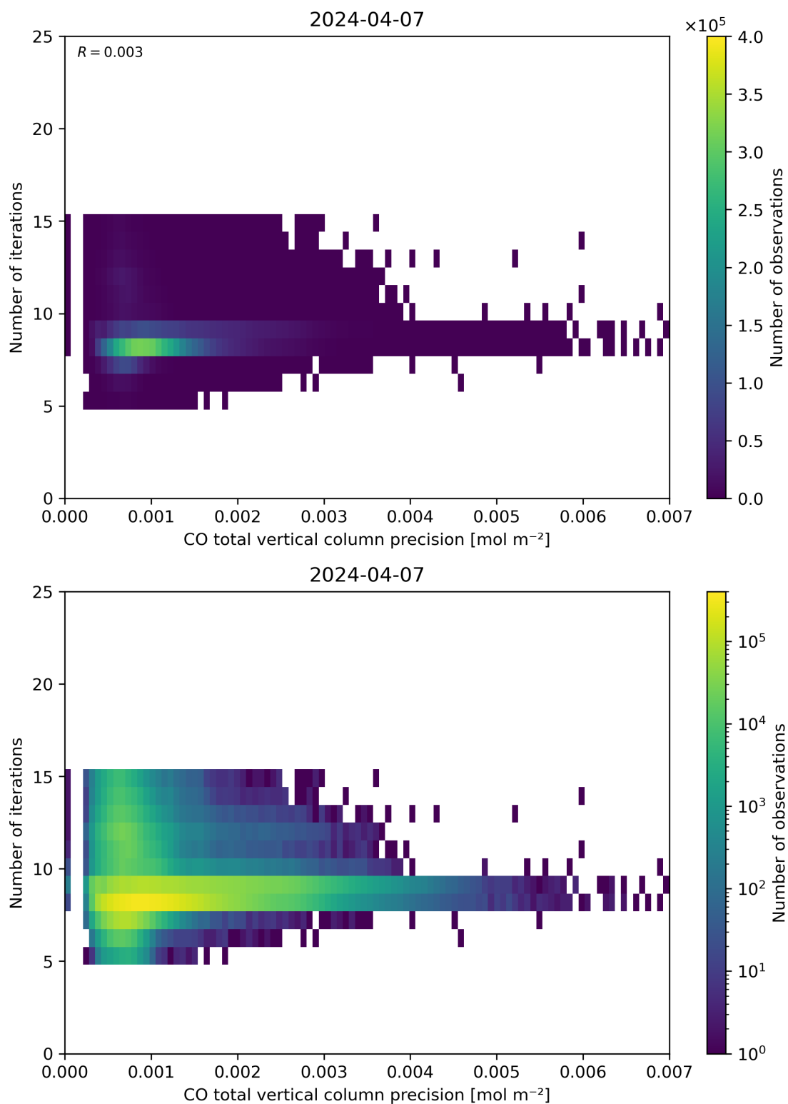
Figure 46: Scatter density plot of “CO total vertical column precision” against “Number of iterations” for 2024-04-06 to 2024-04-08.
