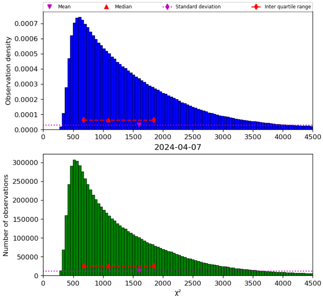
Figure 22: Histogram of “ \chi^2 ” for 2024-04-06 to 2024-04-08
