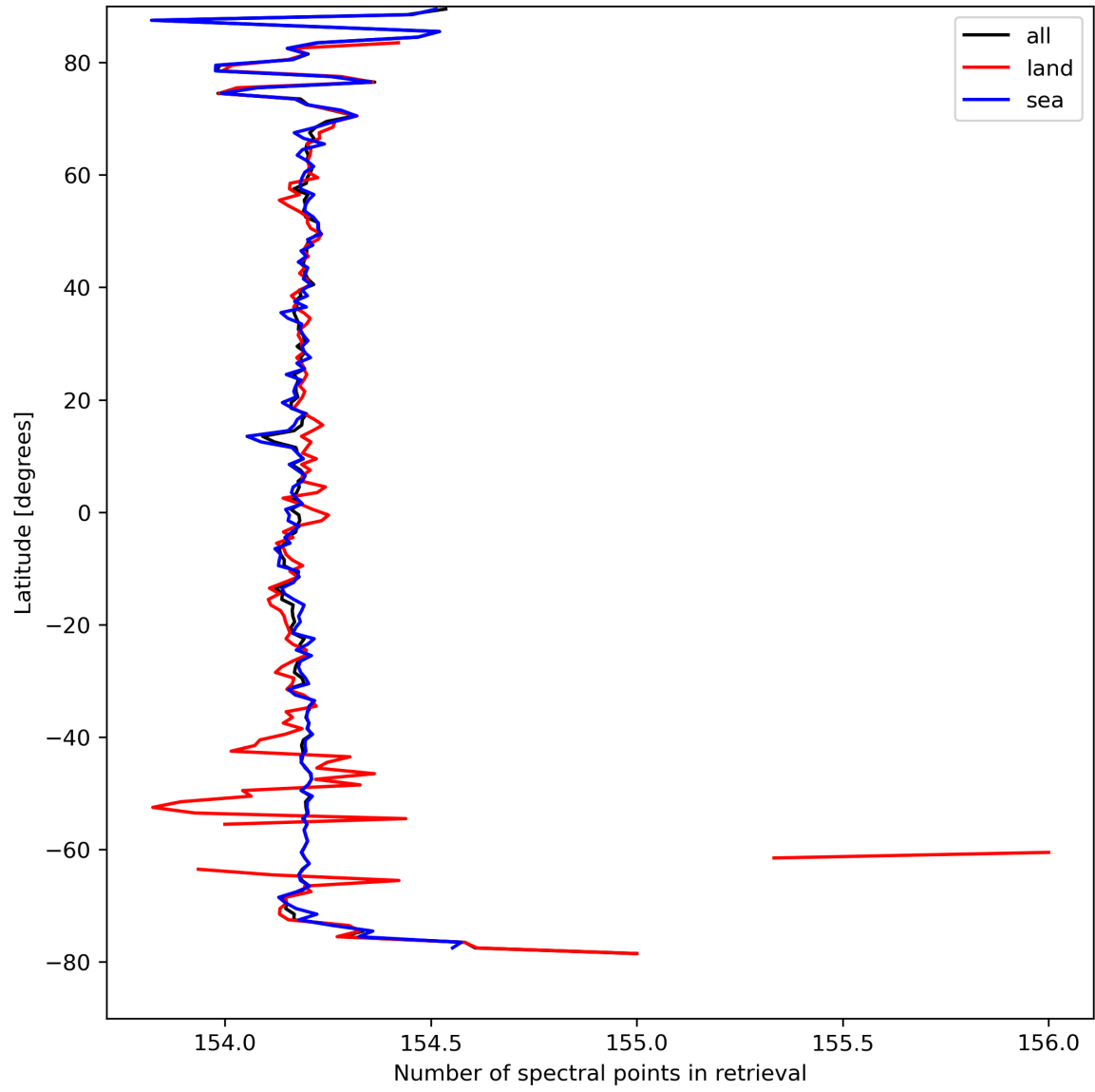
Figure 13: Zonal average of “Number of spectral points in retrieval” for 2024-04-06 to 2024-04-08.
