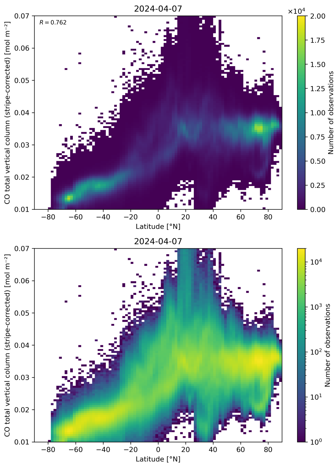
Figure 52: Scatter density plot of “Latitude” against “CO total vertical column (stripe-corrected)” for 2024-04-06 to 2024-04-08.
