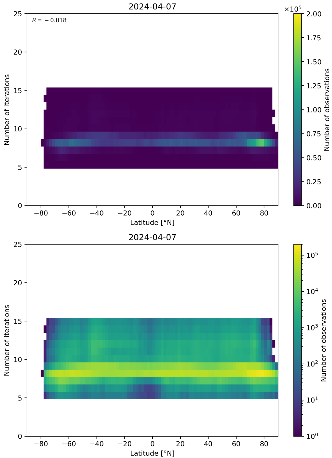
Figure 56: Scatter density plot of “Latitude” against “Number of iterations” for 2024-04-06 to 2024-04-08.
