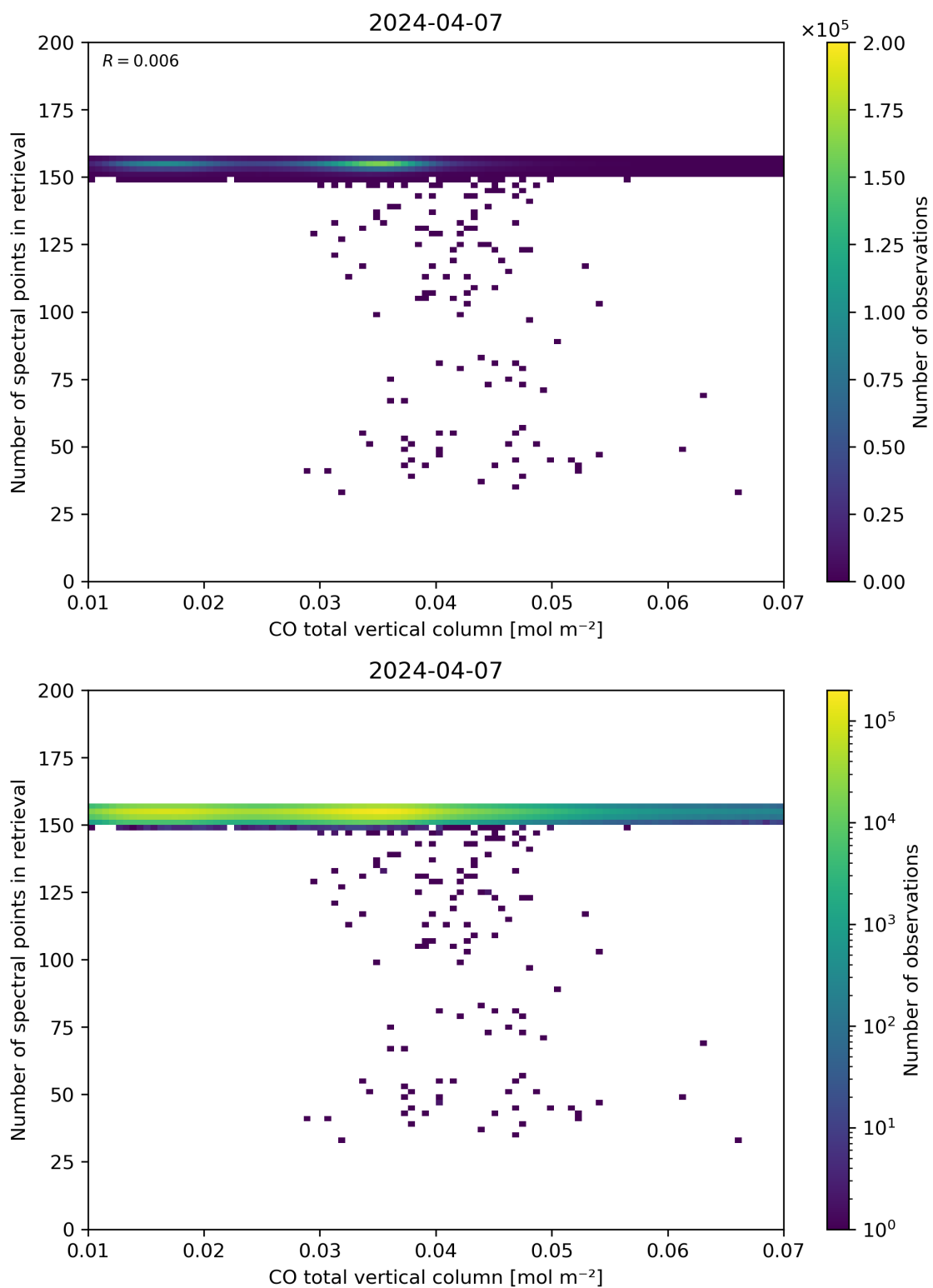
Figure 43: Scatter density plot of “CO total vertical column” against “Number of spectral points in retrieval” for 2024-04-06 to 2024-04-08.
