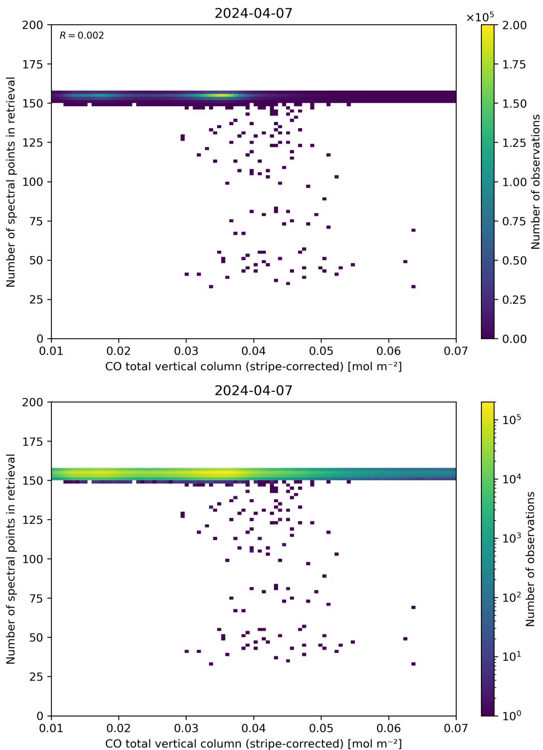
Figure 40: Scatter density plot of “CO total vertical column (stripe-corrected)” against “Number of spectral points in retrieval” for 2024-04-06 to 2024-04-08.
