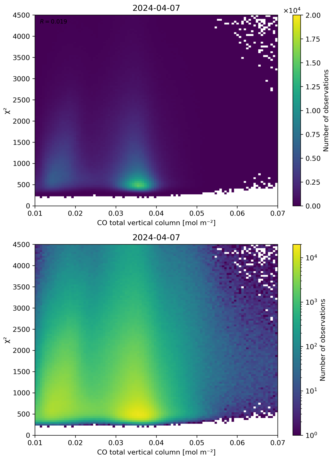
Figure 35: Scatter density plot of “CO total vertical column” against “ \chi^2 ” for 2024-04-06 to 2024-04-08.
