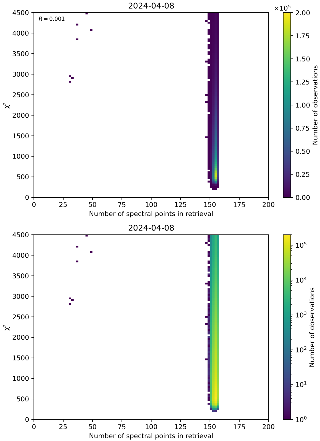
Figure 58: Scatter density plot of “Number of spectral points in retrieval” against “ \chi^2 ” for 2024-04-07 to 2024-04-09.
