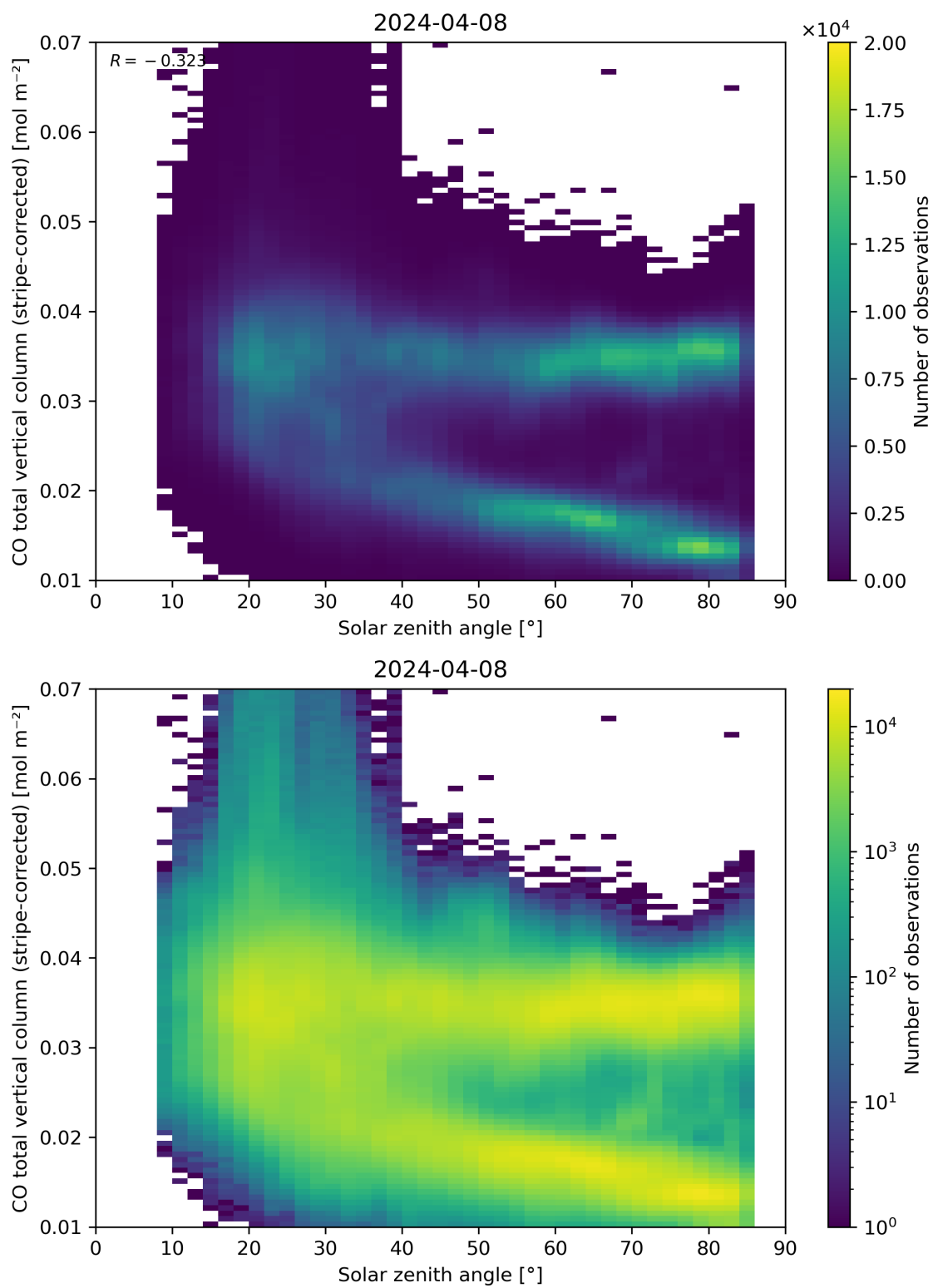
Figure 62: Scatter density plot of “Solar zenith angle” against “CO total vertical column (stripe-corrected)” for 2024-04-07 to 2024-04-09.
