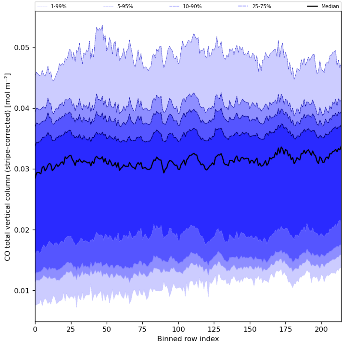
Figure 27: Along track statistics of “CO total vertical column (stripe-corrected)” for 2024-04-07 to 2024-04-09
