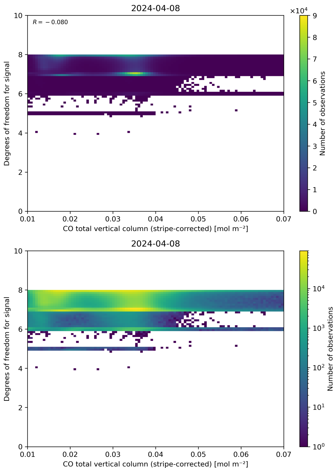
Figure 38: Scatter density plot of “CO total vertical column (stripe-corrected)” against “Degrees of freedom for signal” for 2024-04-07 to 2024-04-09.
