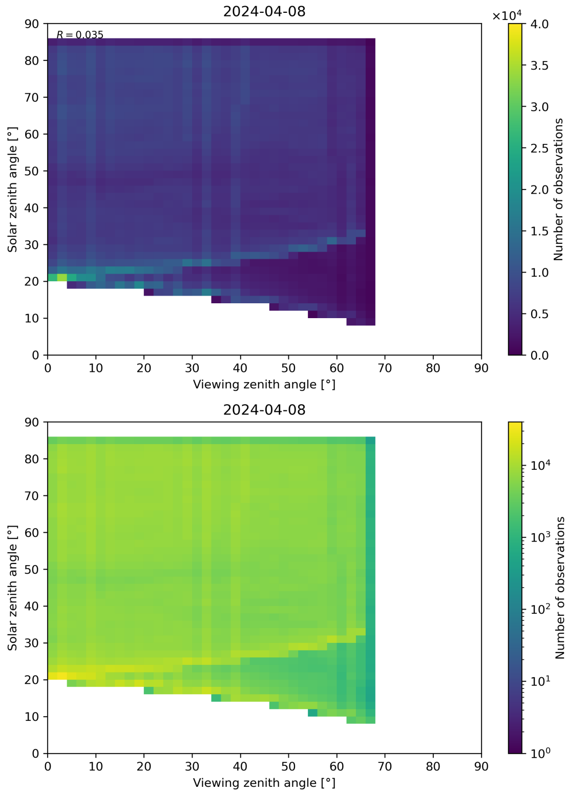
Figure 77: Scatter density plot of “Viewing zenith angle” against “Solar zenith angle” for 2024-04-07 to 2024-04-09.
