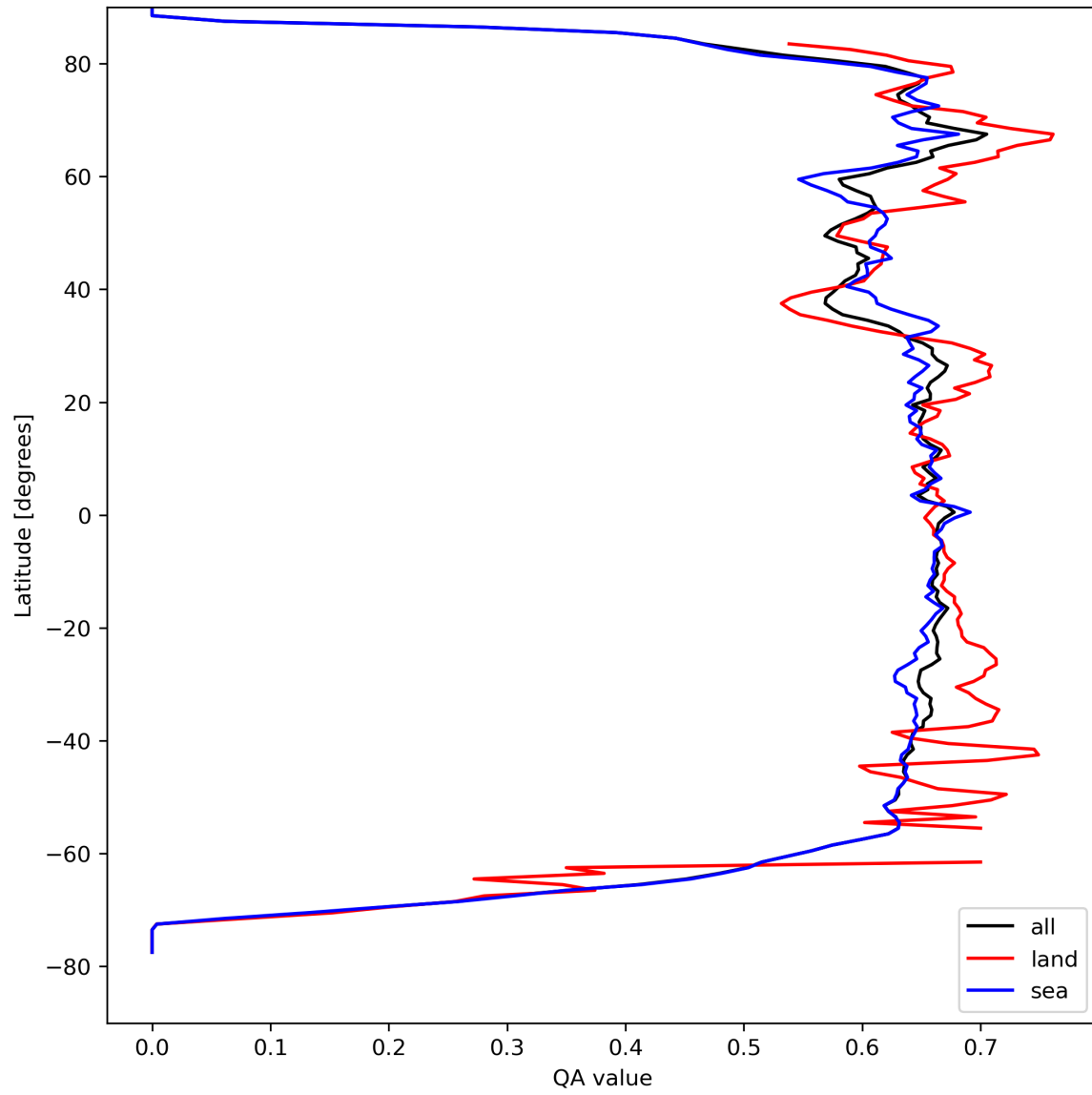
Figure 9: Zonal average of “QA value” for 2024-04-07 to 2024-04-09.
