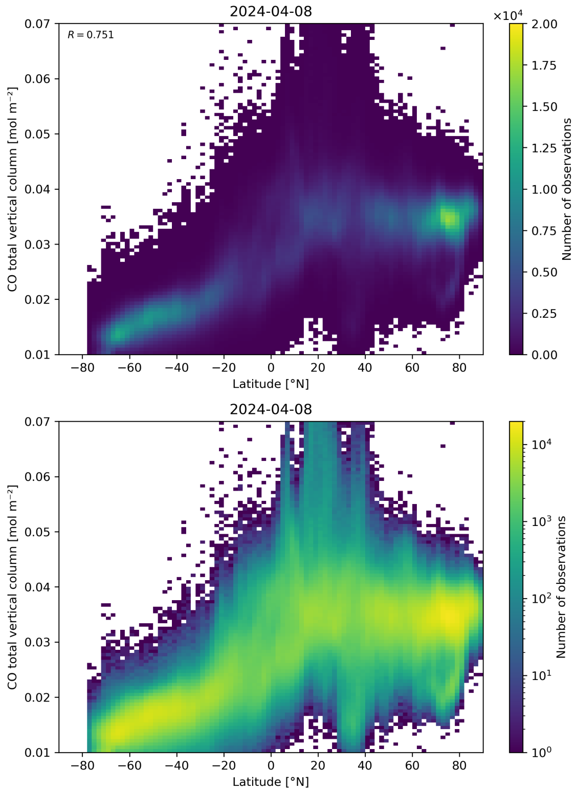
Figure 51: Scatter density plot of “Latitude” against “CO total vertical column” for 2024-04-07 to 2024-04-09.
