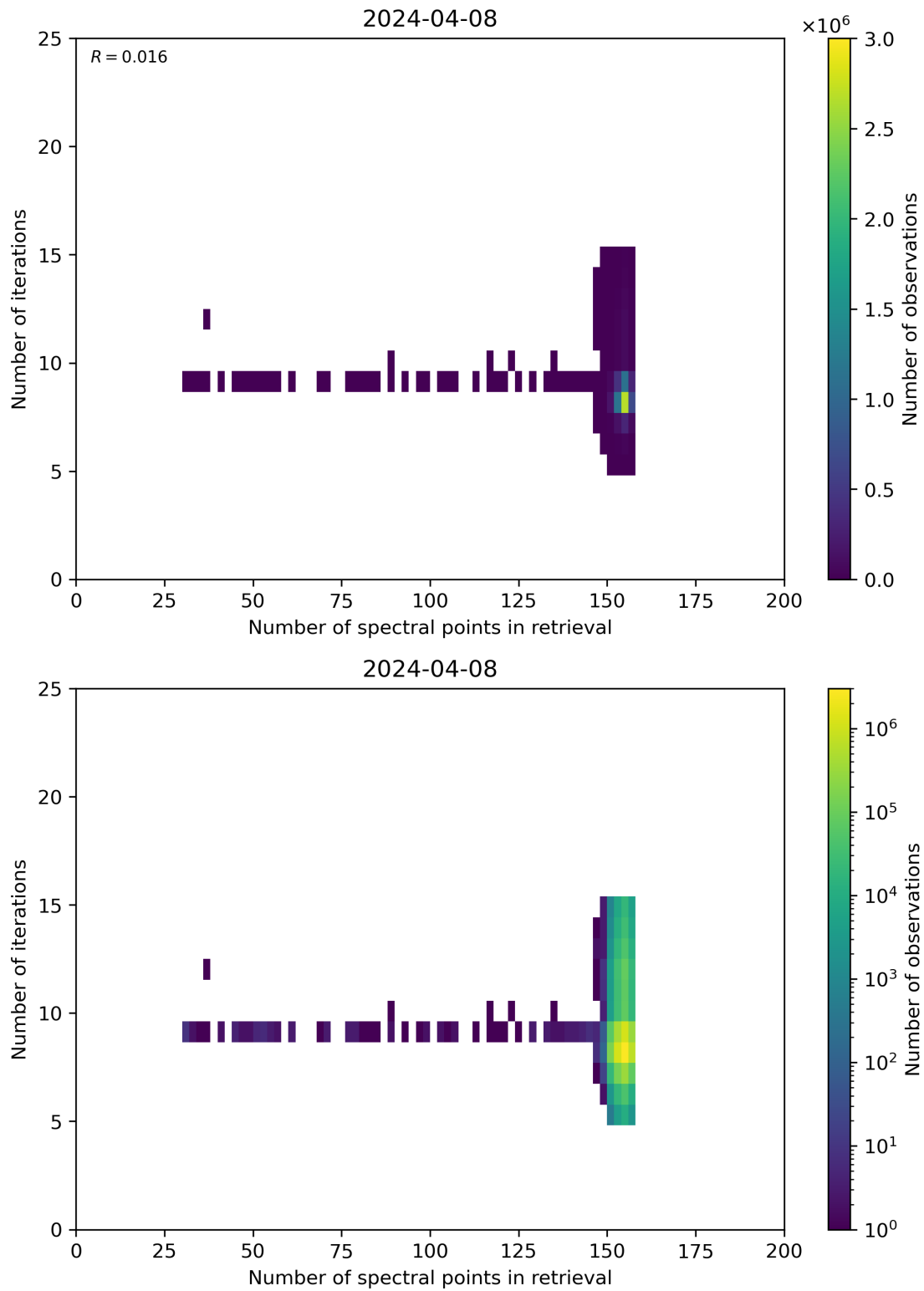
Figure 60: Scatter density plot of “Number of spectral points in retrieval” against “Number of iterations” for 2024-04-07 to 2024-04-09.
