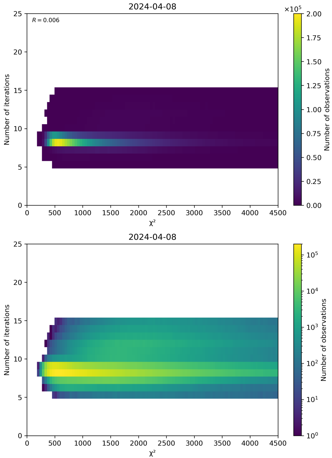
Figure 49: Scatter density plot of “ \chi^2 ” against “Number of iterations” for 2024-04-07 to 2024-04-09.
