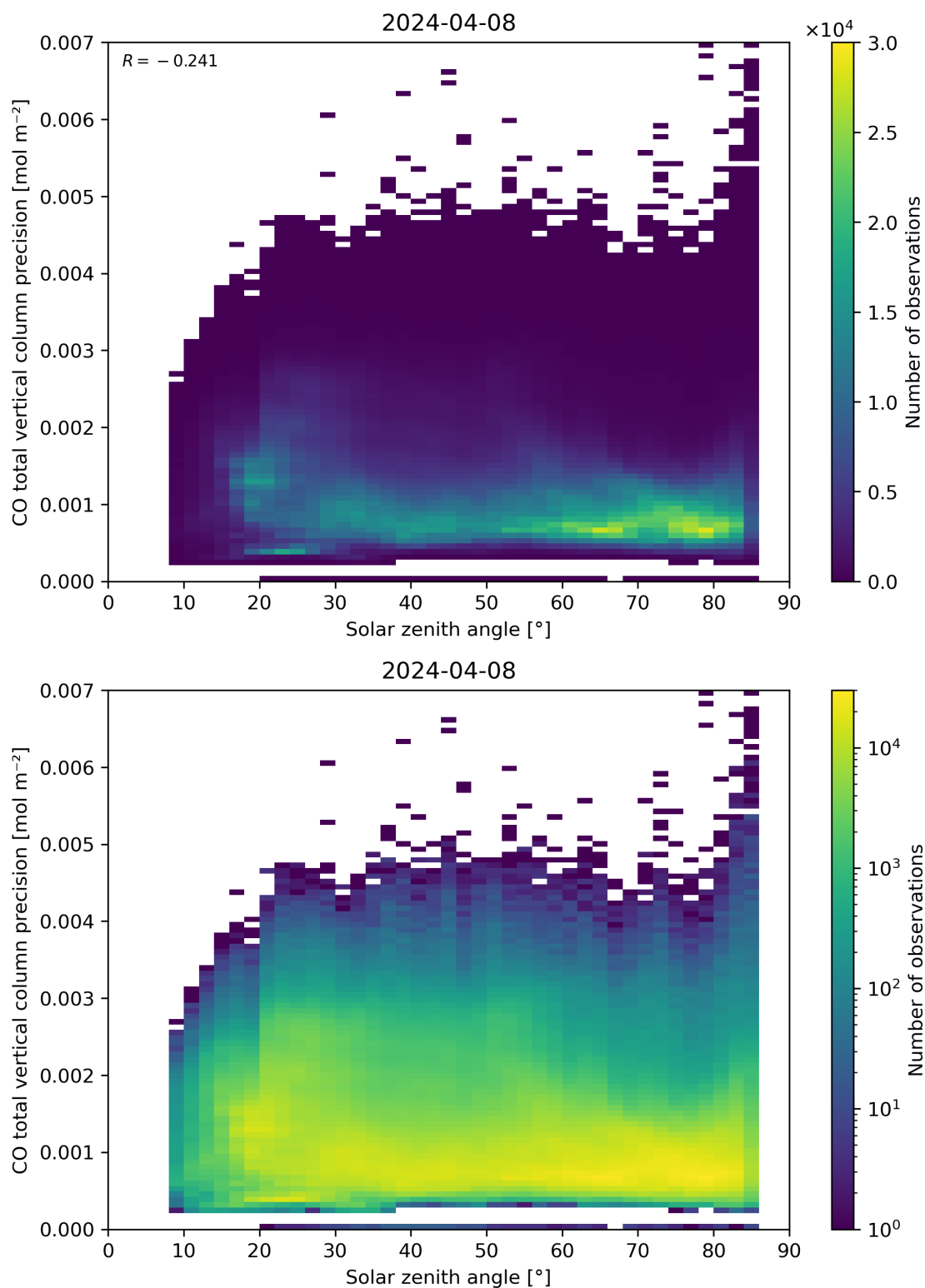
Figure 63: Scatter density plot of “Solar zenith angle” against “CO total vertical column precision” for 2024-04-07 to 2024-04-09.
