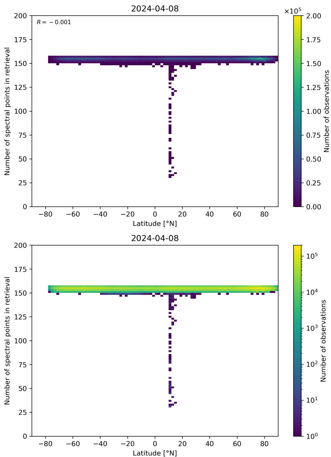
Figure 57: Scatter density plot of “Latitude” against “Number of spectral points in retrieval” for 2024-04-07 to 2024-04-09.
