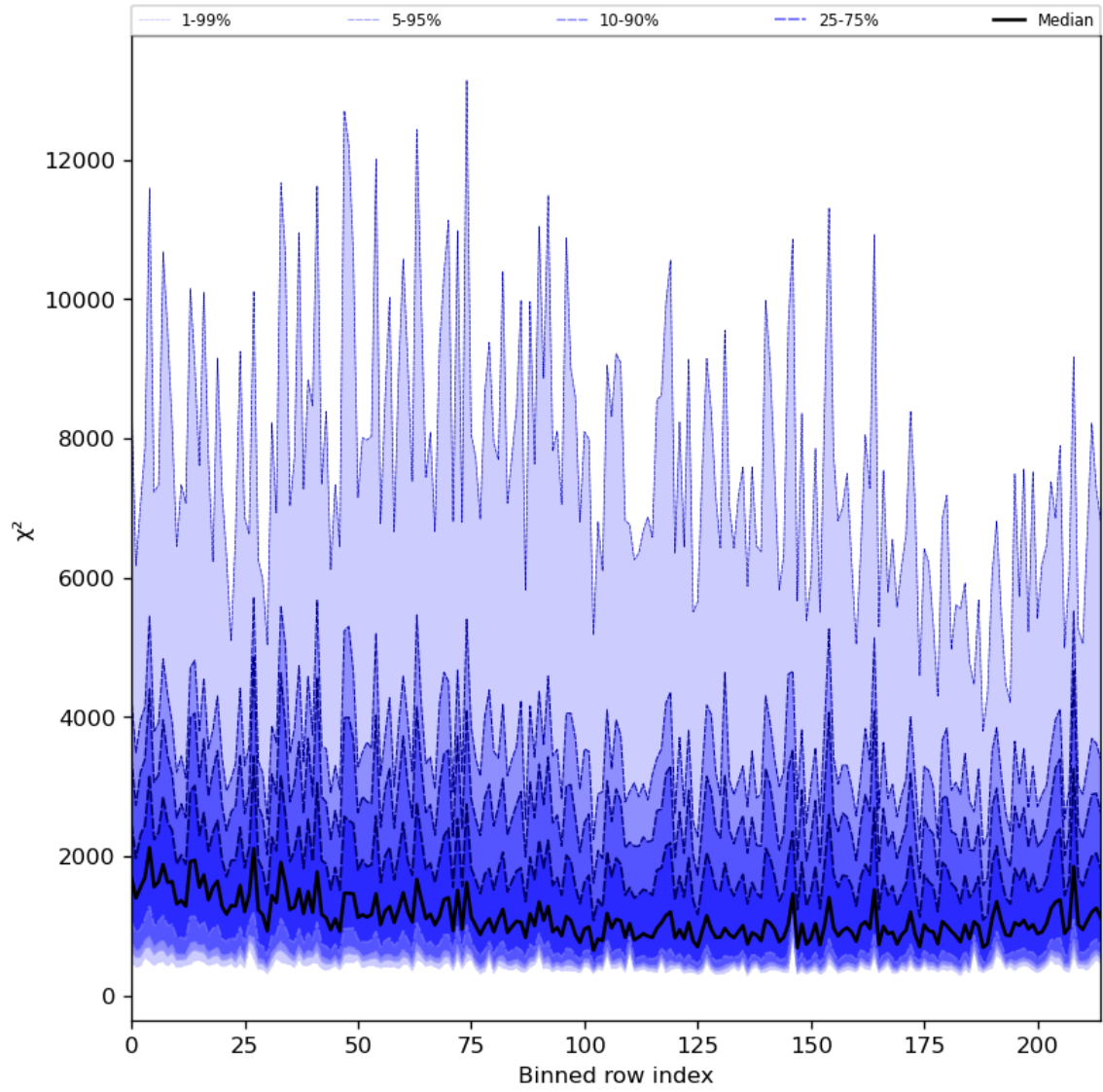
Figure 30: Along track statistics of “ \chi^2 ” for 2024-04-07 to 2024-04-09
