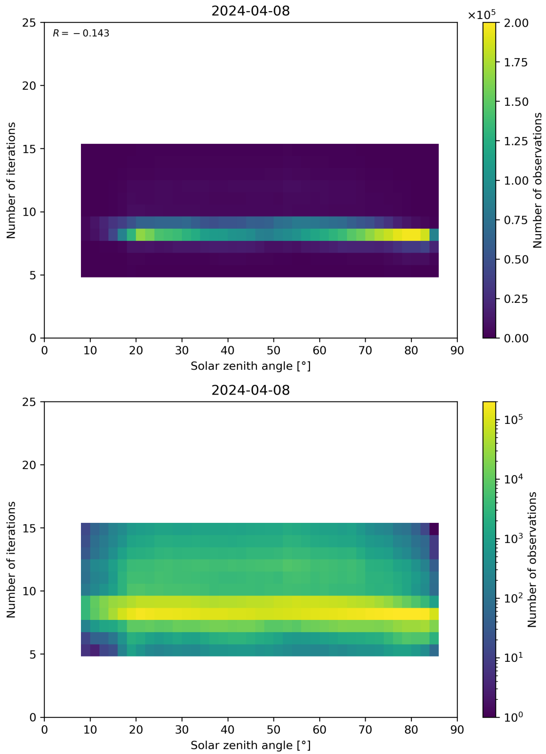
Figure 67: Scatter density plot of “Solar zenith angle” against “Number of iterations” for 2024-04-07 to 2024-04-09.
