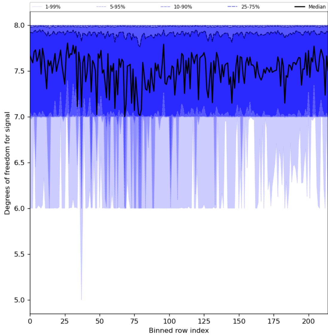
Figure 31: Along track statistics of “Degrees of freedom for signal” for 2024-04-07 to 2024-04-09
