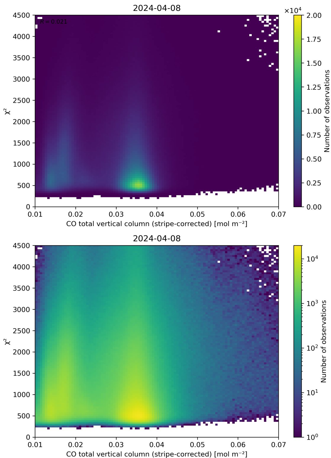
Figure 37: Scatter density plot of “CO total vertical column (stripe-corrected)” against “ \chi^2 ” for 2024-04-07 to 2024-04-09.
