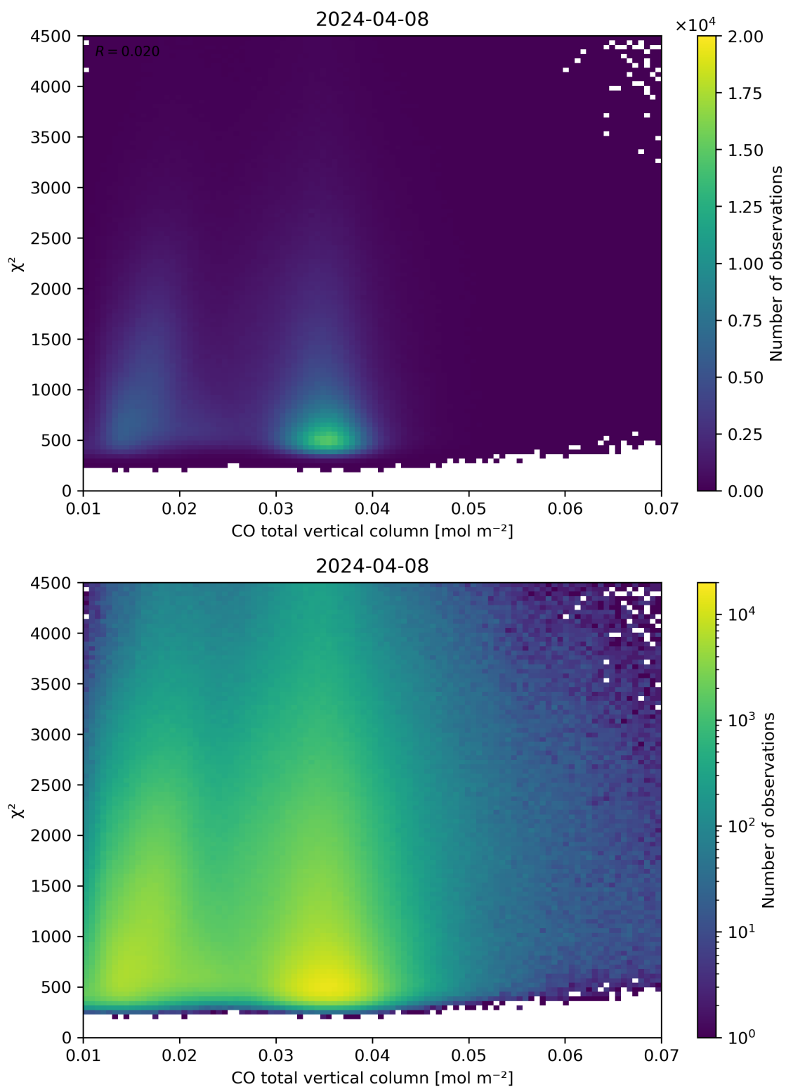
Figure 35: Scatter density plot of “CO total vertical column” against “ \chi^2 ” for 2024-04-07 to 2024-04-09.
