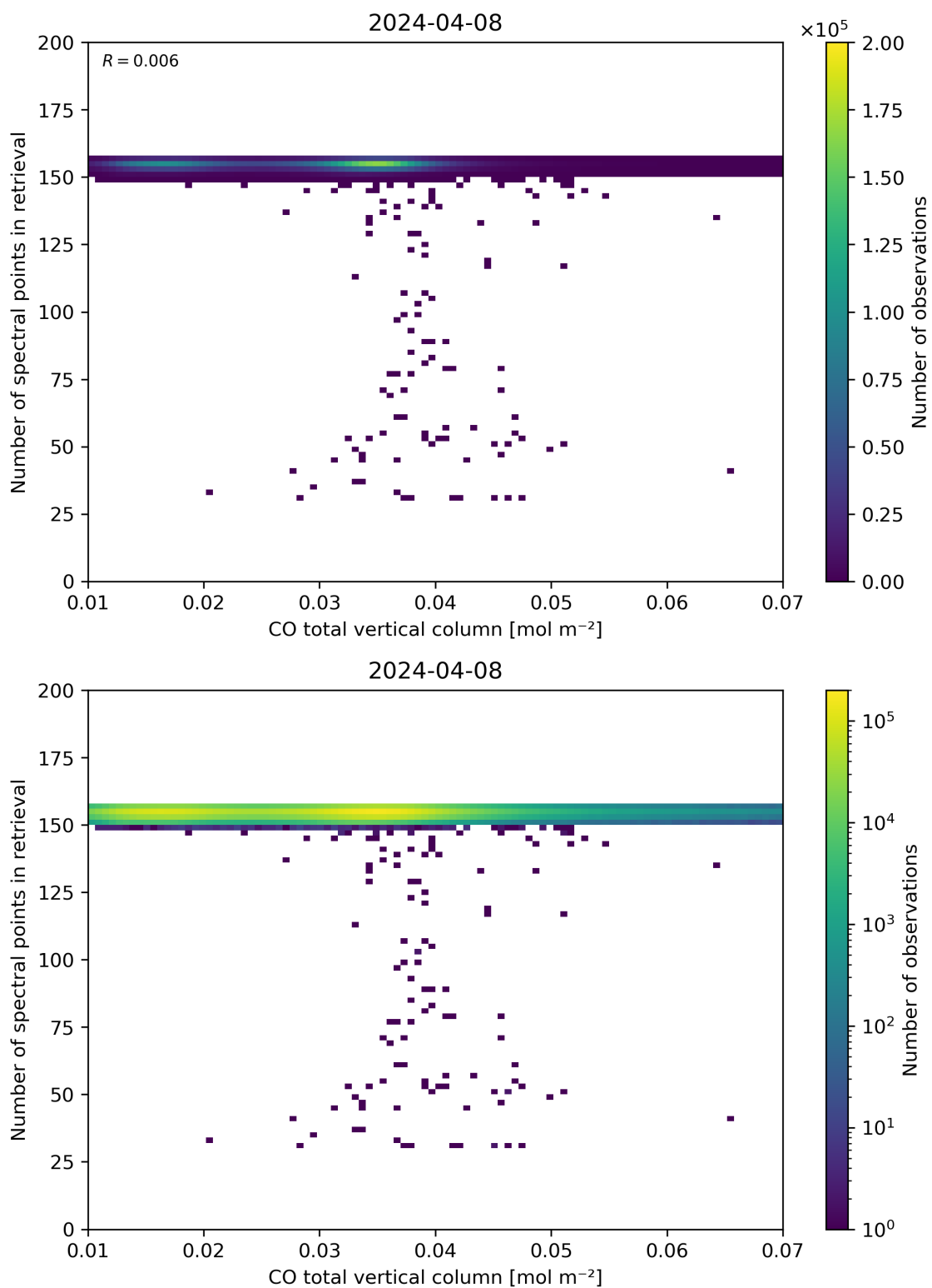
Figure 43: Scatter density plot of “CO total vertical column” against “Number of spectral points in retrieval” for 2024-04-07 to 2024-04-09.
