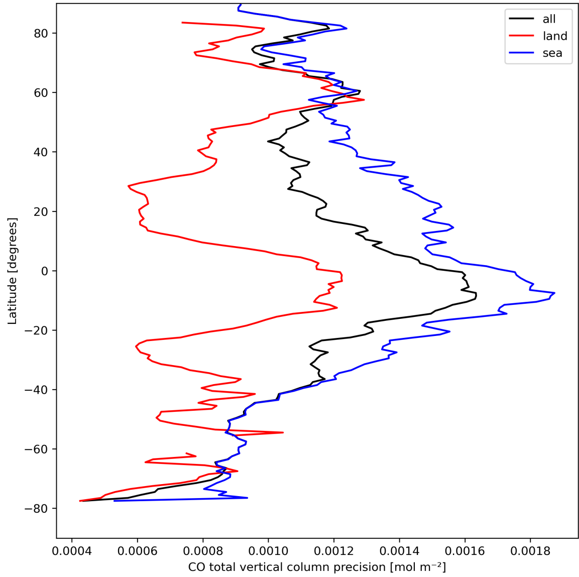
Figure 12: Zonal average of “CO total vertical column precision” for 2024-04-07 to 2024-04-09.
