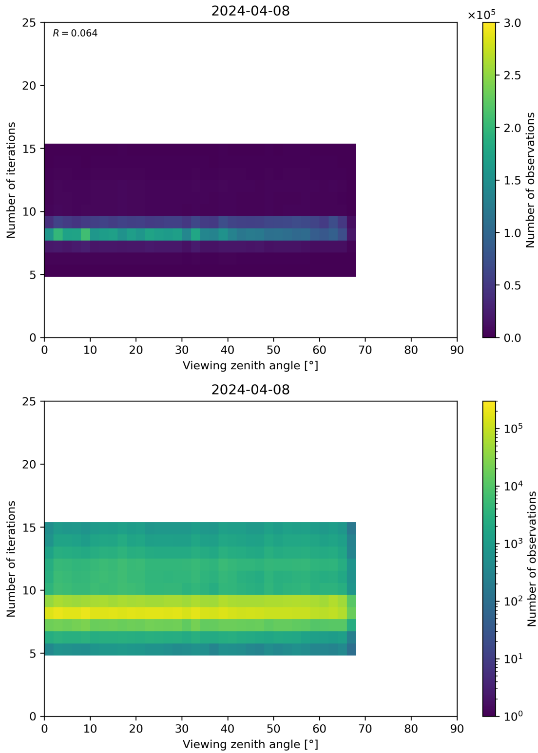
Figure 75: Scatter density plot of “Viewing zenith angle” against “Number of iterations” for 2024-04-07 to 2024-04-09.
