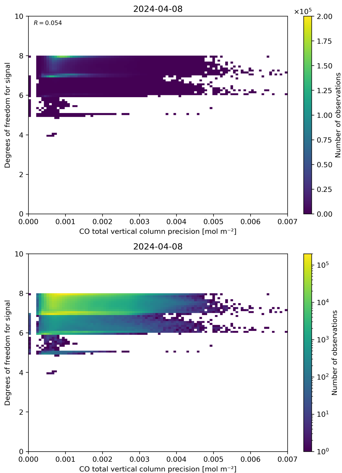
Figure 45: Scatter density plot of “CO total vertical column precision” against “Degrees of freedom for signal” for 2024-04-07 to 2024-04-09.
