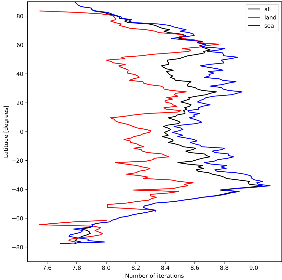
Figure 16: Zonal average of “Number of iterations” for 2024-04-07 to 2024-04-09.
