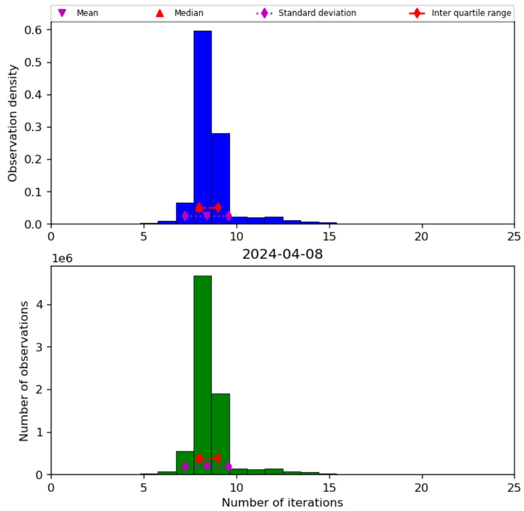
Figure 24: Histogram of “Number of iterations” for 2024-04-07 to 2024-04-09
