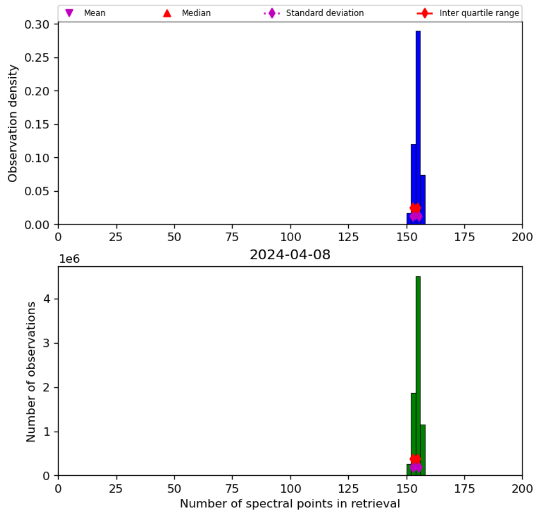
Figure 21: Histogram of “Number of spectral points in retrieval” for 2024-04-07 to 2024-04-09
