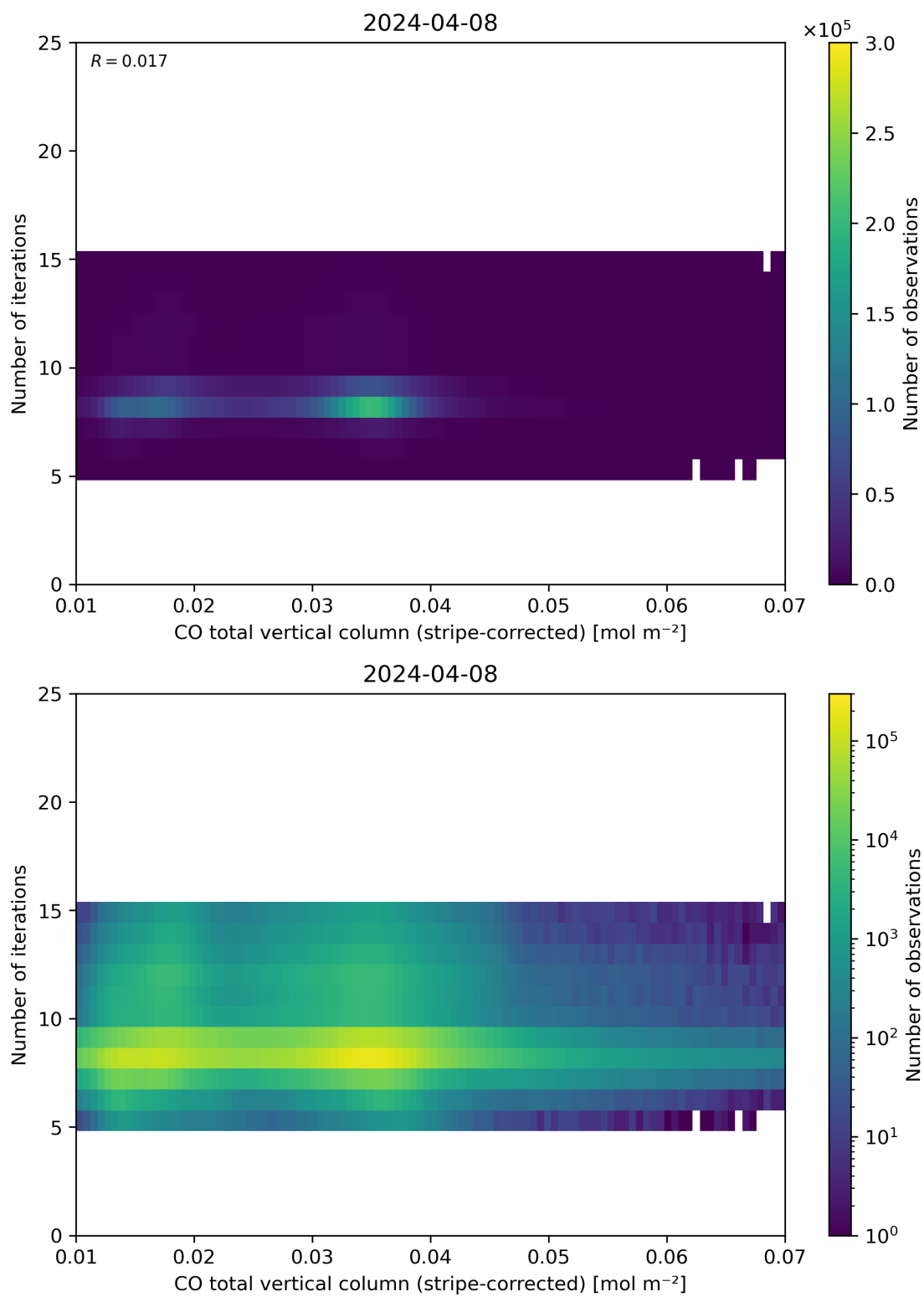
Figure 39: Scatter density plot of “CO total vertical column (stripe-corrected)” against “Number of iterations” for 2024-04-07 to 2024-04-09.
