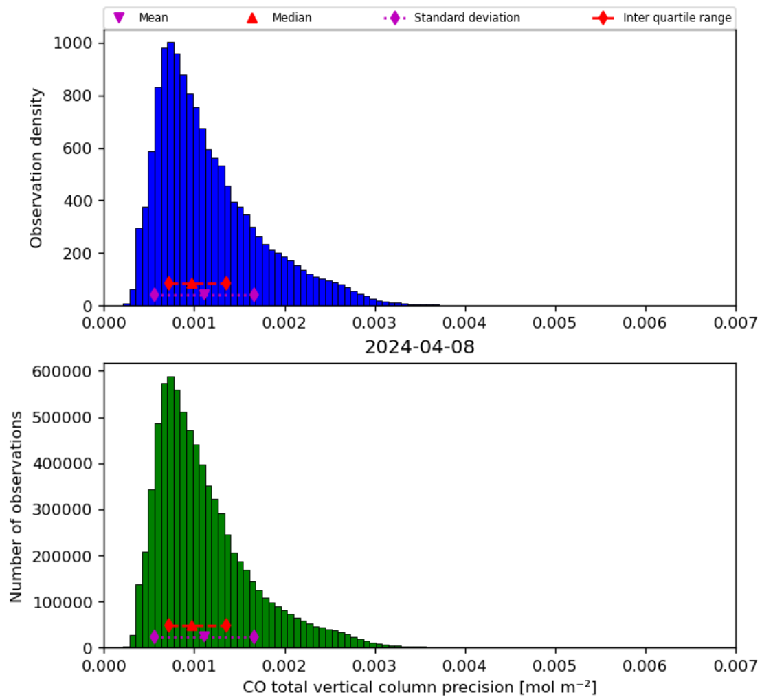
Figure 20: Histogram of “CO total vertical column precision” for 2024-04-07 to 2024-04-09
