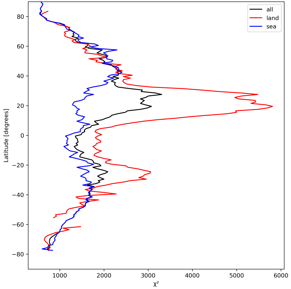
Figure 14: Zonal average of “ \chi^2 ” for 2024-04-07 to 2024-04-09.
