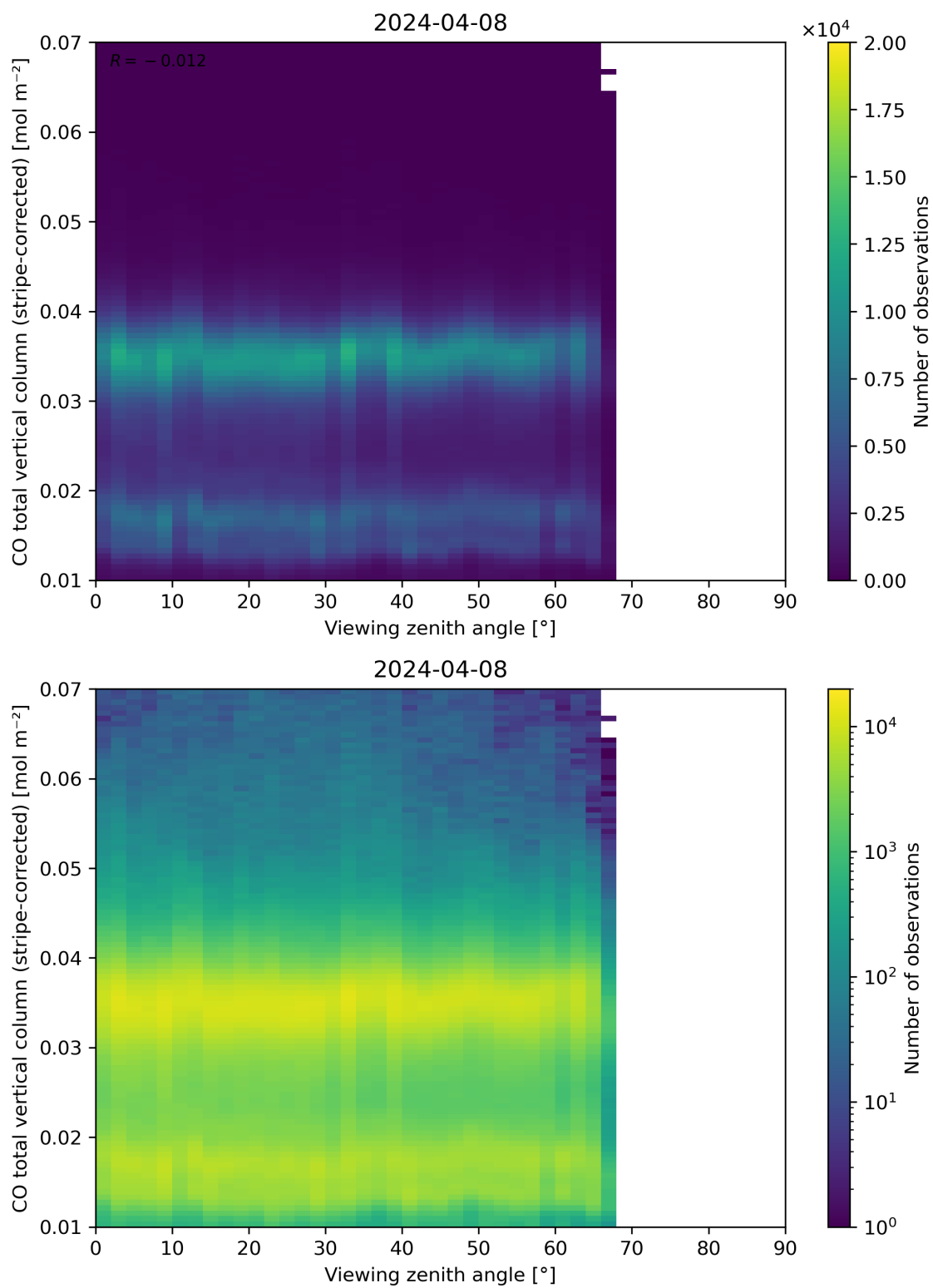
Figure 70: Scatter density plot of “Viewing zenith angle” against “CO total vertical column (stripe-corrected)” for 2024-04-07 to 2024-04-09.
