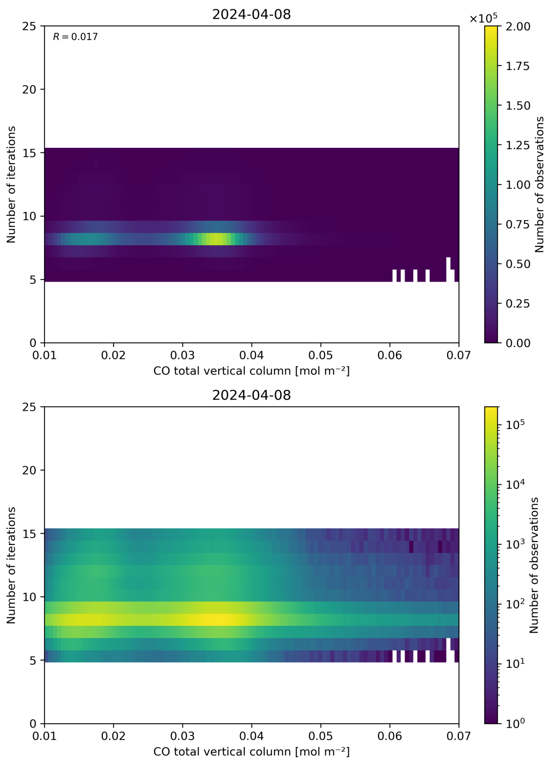
Figure 42: Scatter density plot of “CO total vertical column” against “Number of iterations” for 2024-04-07 to 2024-04-09.
