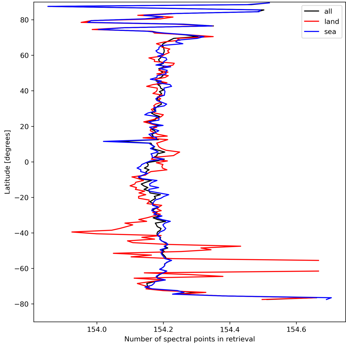
Figure 13: Zonal average of “Number of spectral points in retrieval” for 2024-04-07 to 2024-04-09.
