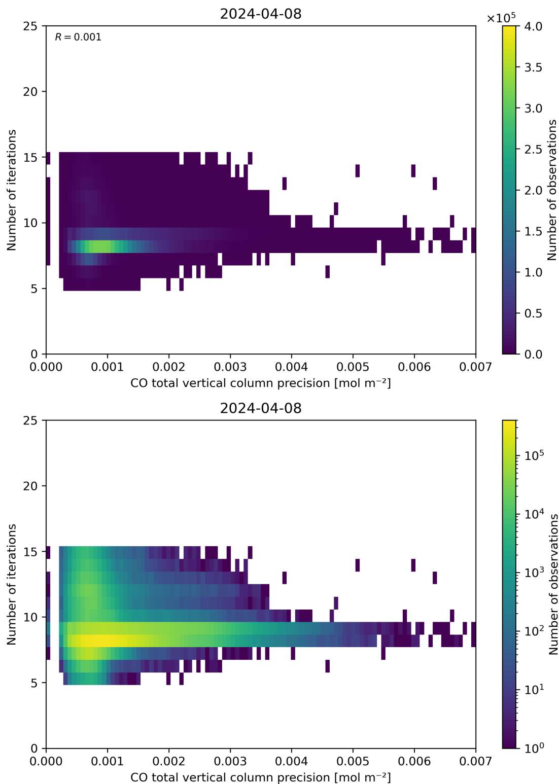
Figure 46: Scatter density plot of “CO total vertical column precision” against “Number of iterations” for 2024-04-07 to 2024-04-09.
