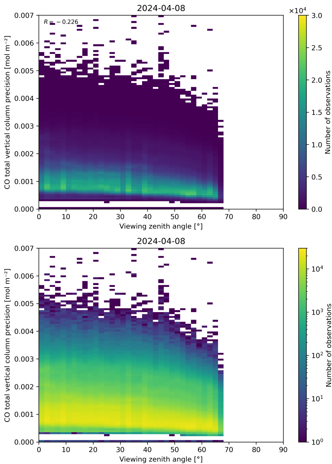
Figure 71: Scatter density plot of “Viewing zenith angle” against “CO total vertical column precision” for 2024-04-07 to 2024-04-09.
