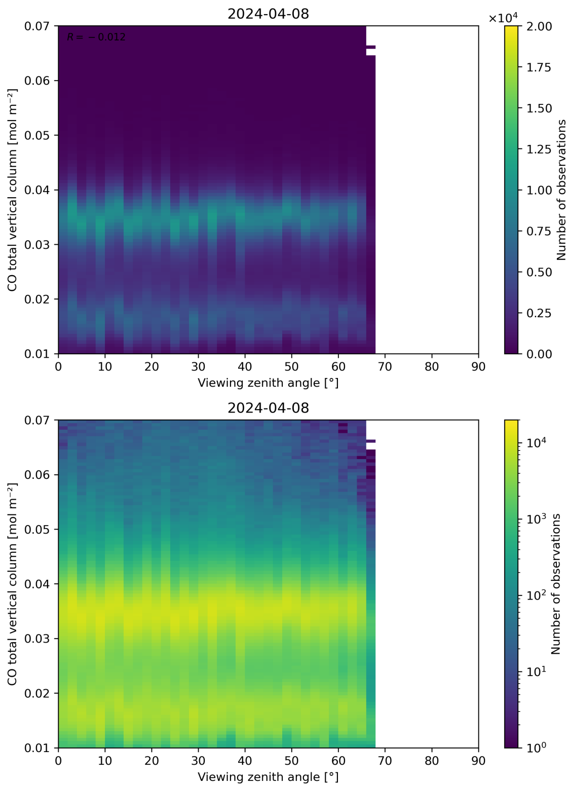
Figure 69: Scatter density plot of “Viewing zenith angle” against “CO total vertical column” for 2024-04-07 to 2024-04-09.
