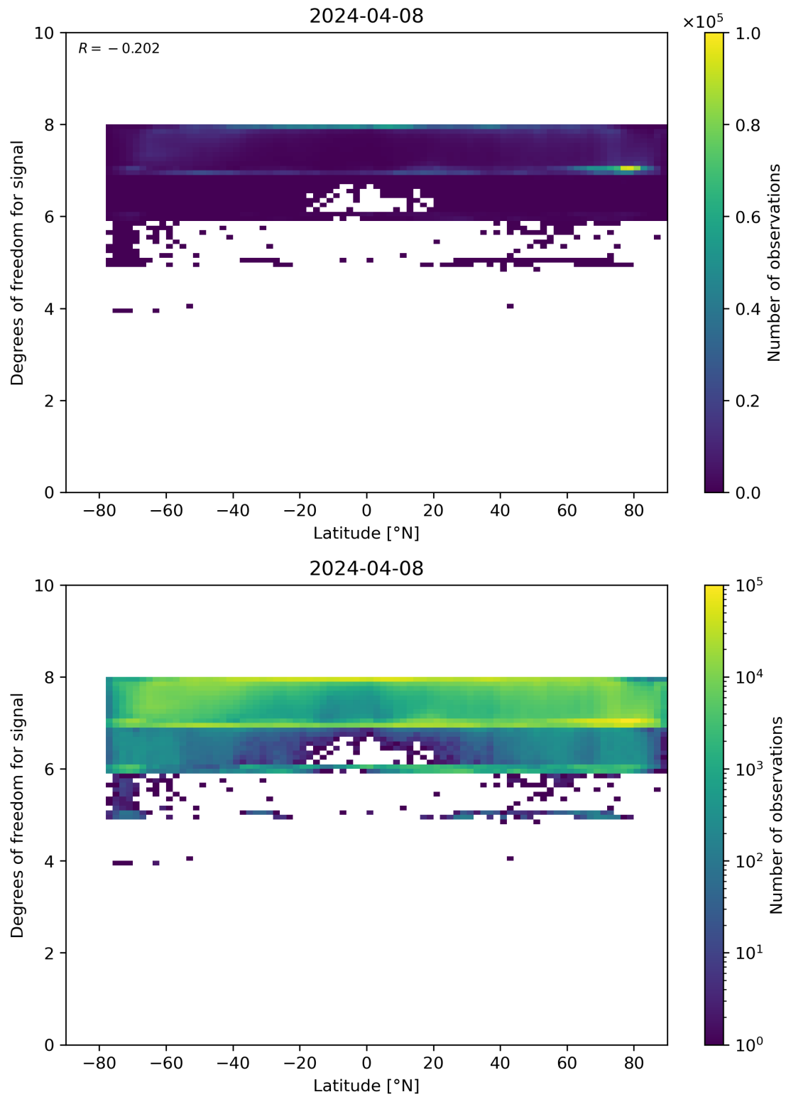
Figure 55: Scatter density plot of “Latitude” against “Degrees of freedom for signal” for 2024-04-07 to 2024-04-09.
