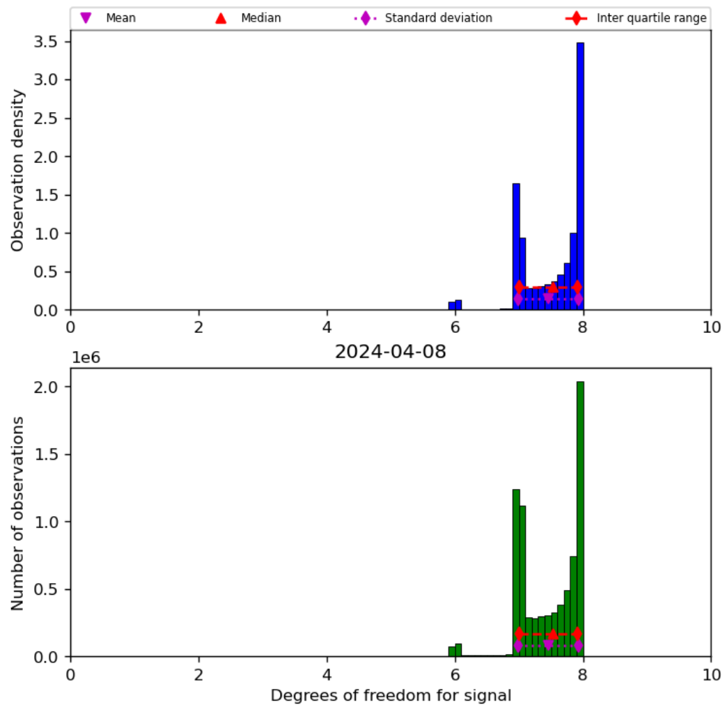
Figure 23: Histogram of “Degrees of freedom for signal” for 2024-04-07 to 2024-04-09
