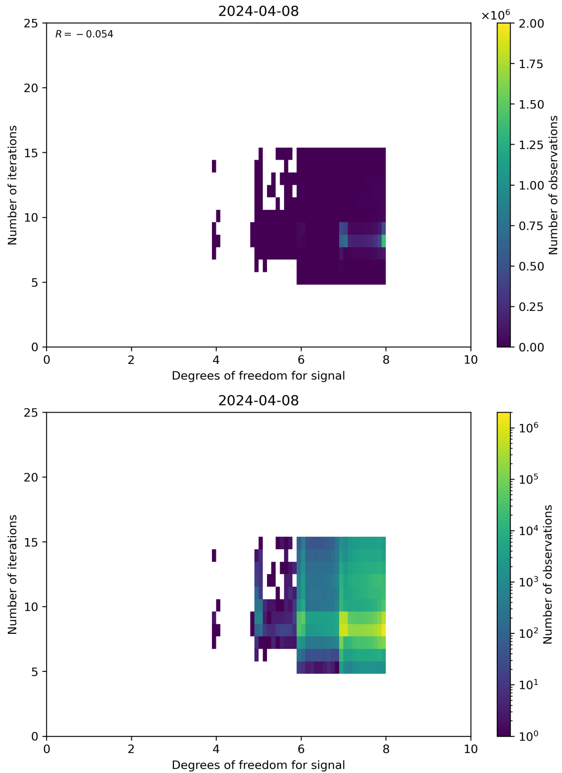
Figure 50: Scatter density plot of “Degrees of freedom for signal” against “Number of iterations” for 2024-04-07 to 2024-04-09.
