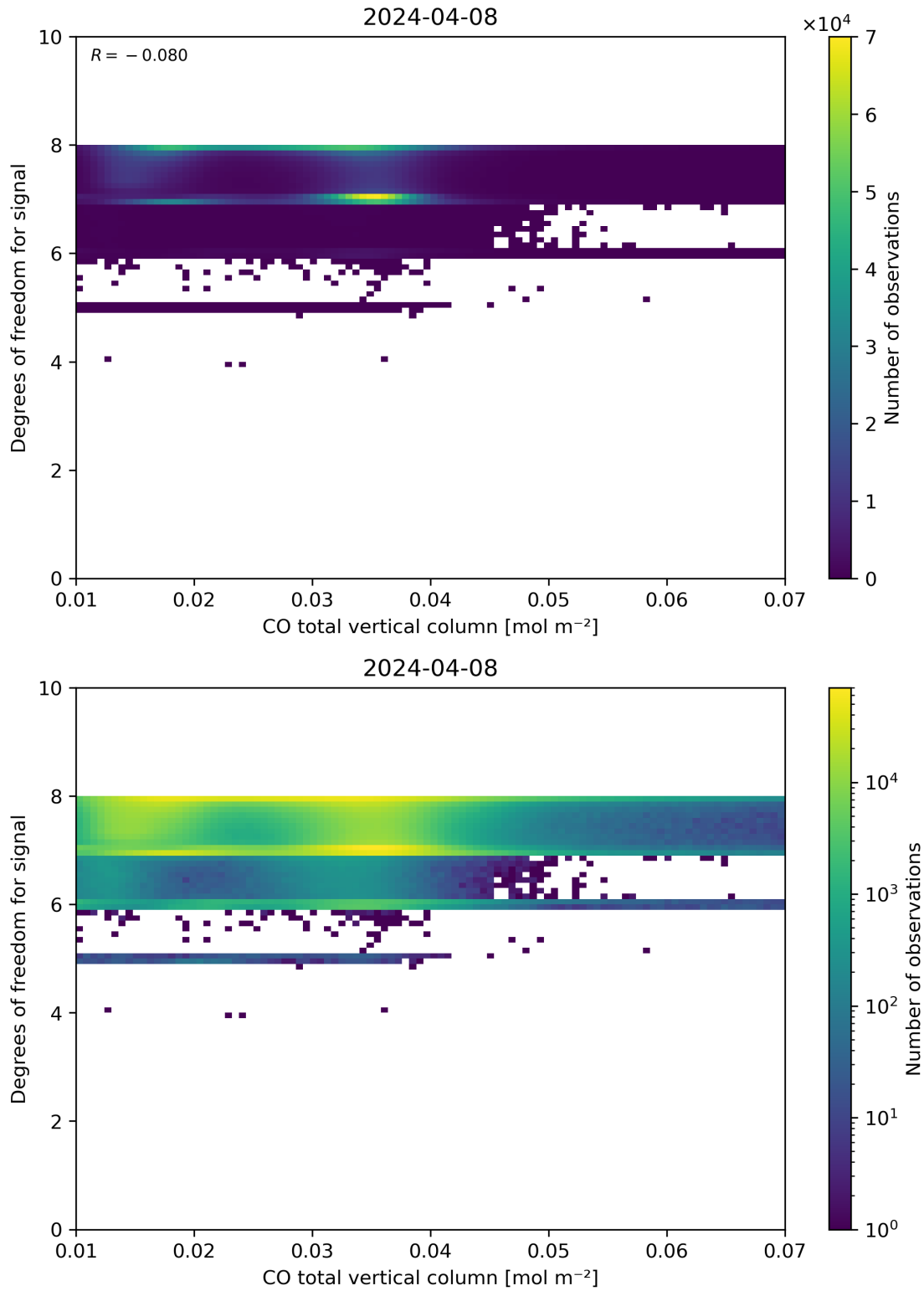
Figure 41: Scatter density plot of “CO total vertical column” against “Degrees of freedom for signal” for 2024-04-07 to 2024-04-09.
