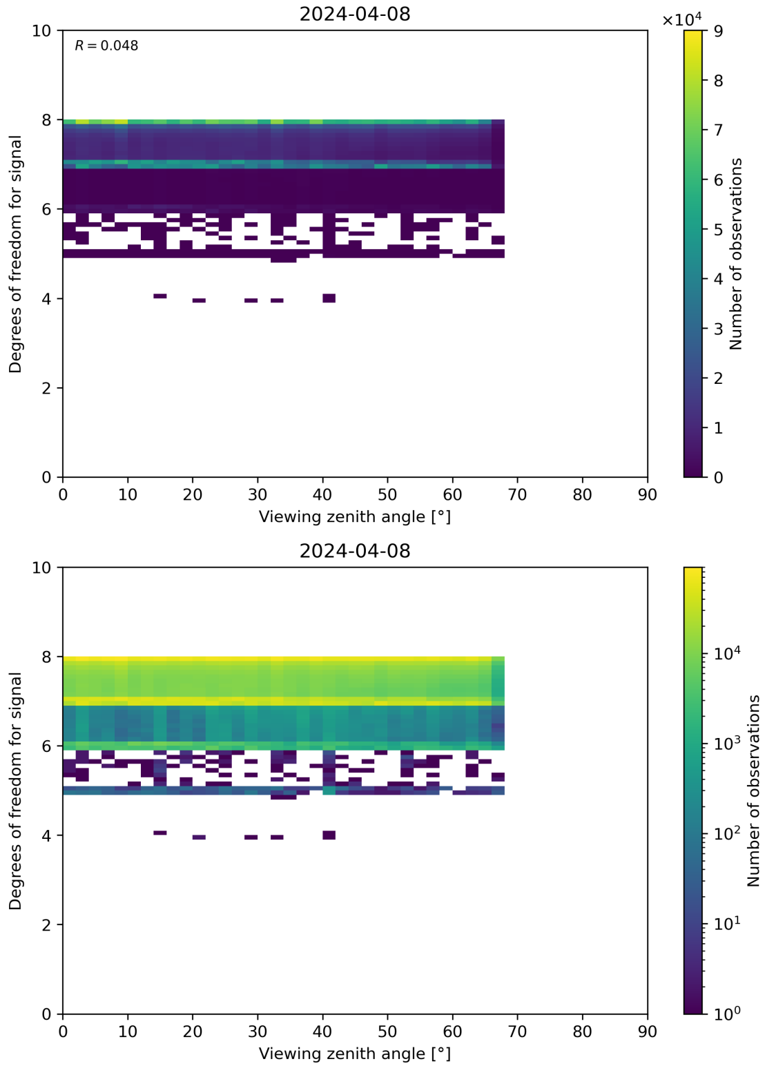
Figure 73: Scatter density plot of “Viewing zenith angle” against “Degrees of freedom for signal” for 2024-04-07 to 2024-04-09.
