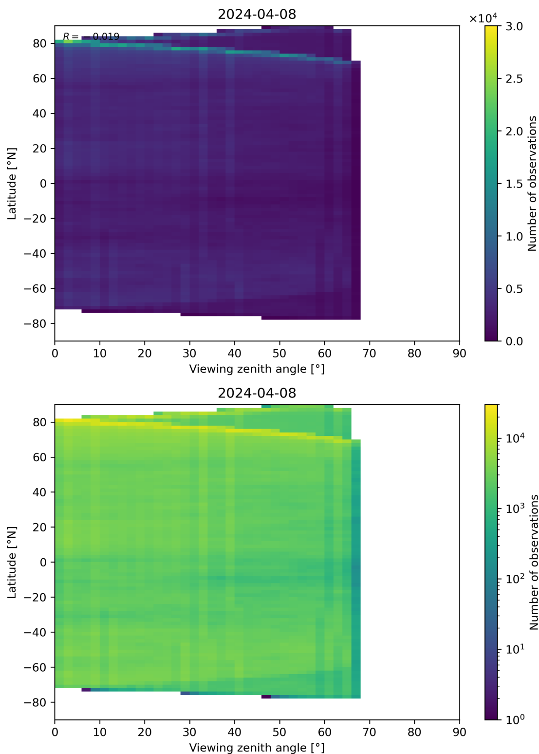
Figure 74: Scatter density plot of “Viewing zenith angle” against “Latitude” for 2024-04-07 to 2024-04-09.
