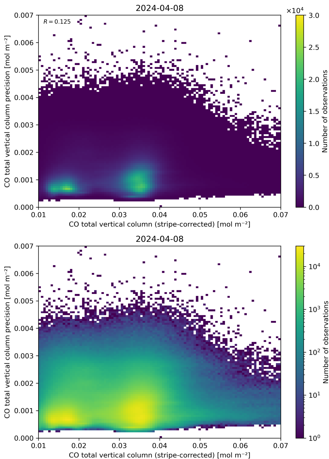
Figure 36: Scatter density plot of “CO total vertical column (stripe-corrected)” against “CO total vertical column precision” for 2024-04-07 to 2024-04-09.
