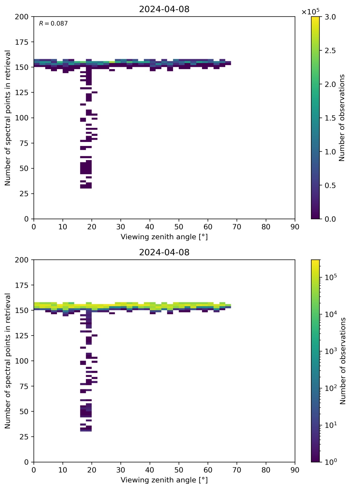
Figure 76: Scatter density plot of “Viewing zenith angle” against “Number of spectral points in retrieval” for 2024-04-07 to 2024-04-09.
