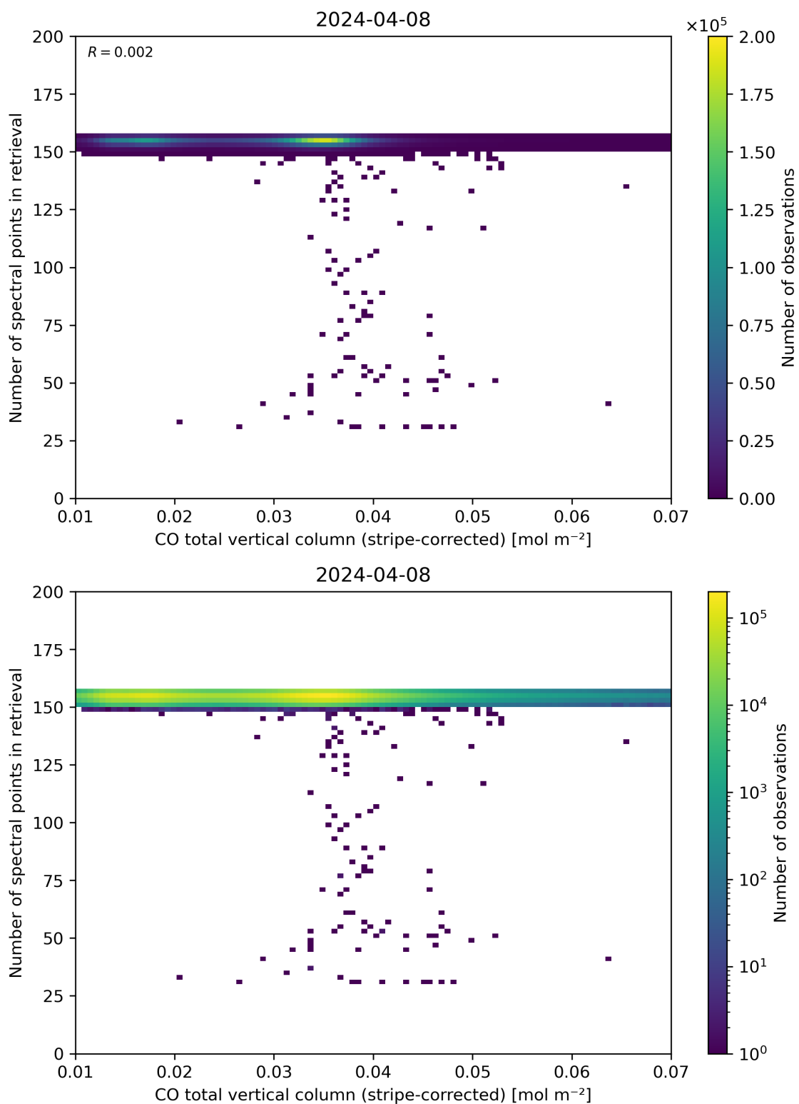
Figure 40: Scatter density plot of “CO total vertical column (stripe-corrected)” against “Number of spectral points in retrieval” for 2024-04-07 to 2024-04-09.
