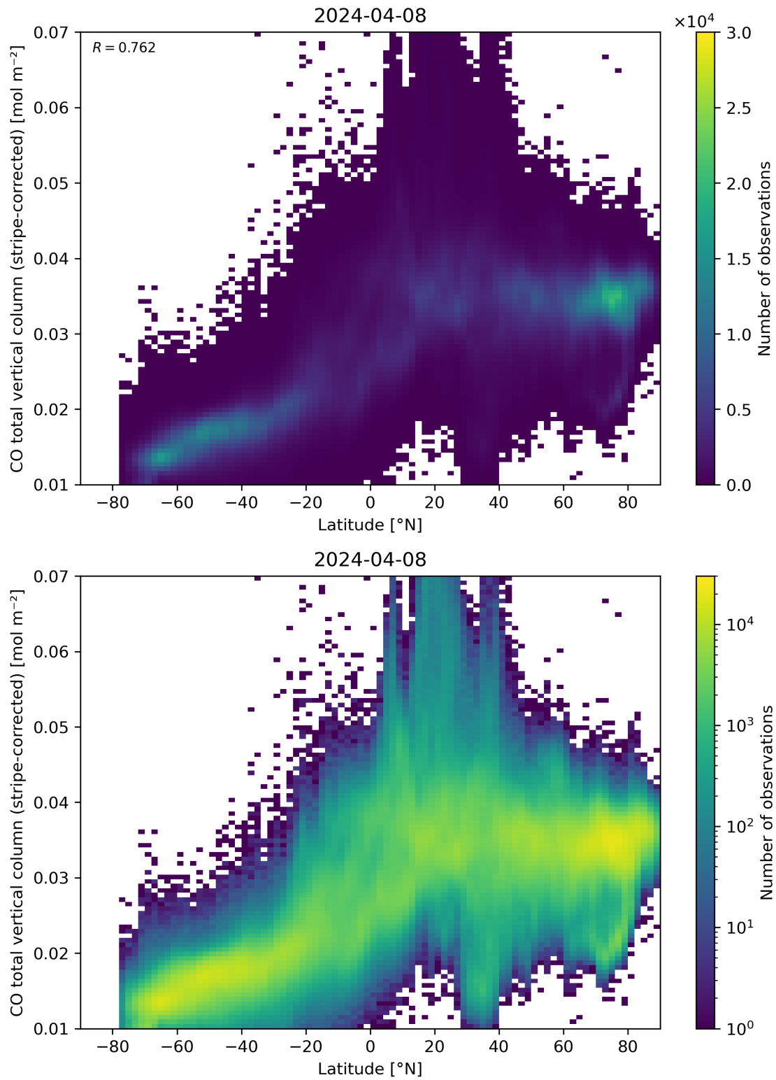
Figure 52: Scatter density plot of “Latitude” against “CO total vertical column (stripe-corrected)” for 2024-04-07 to 2024-04-09.
