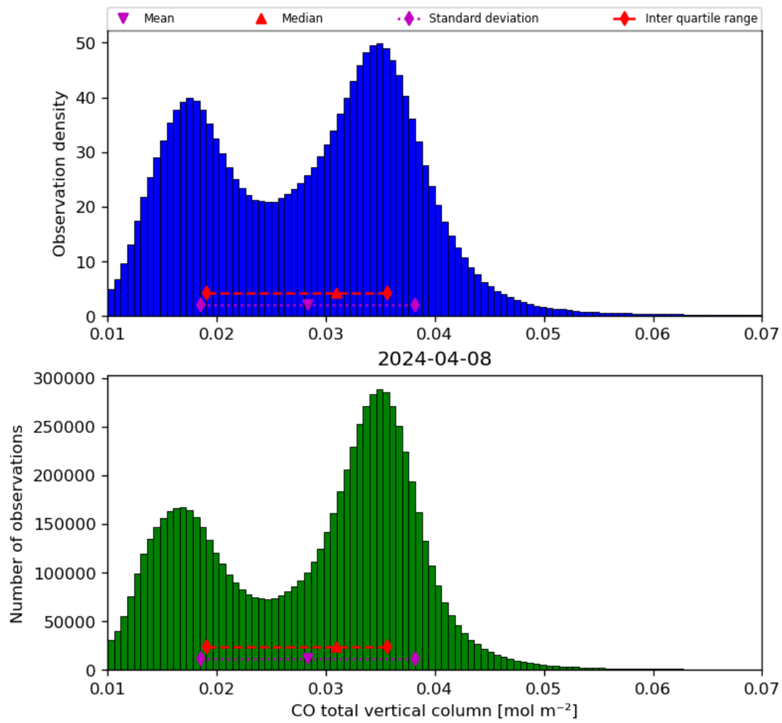
Figure 18: Histogram of “CO total vertical column” for 2024-04-07 to 2024-04-09
