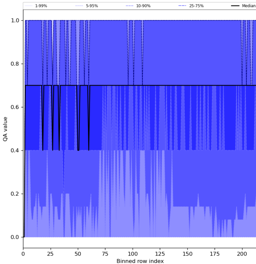
Figure 25: Along track statistics of “QA value” for 2024-04-07 to 2024-04-09
