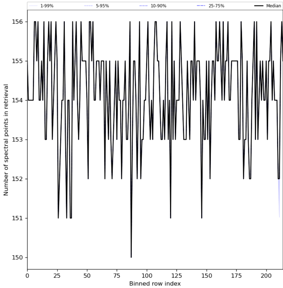
Figure 29: Along track statistics of “Number of spectral points in retrieval” for 2024-04-07 to 2024-04-09
