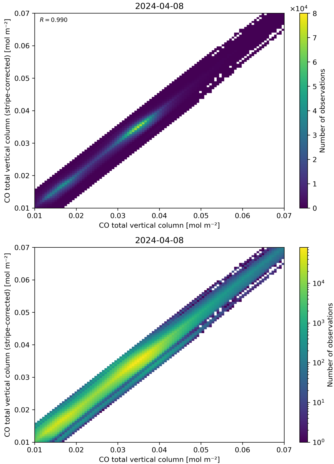
Figure 33: Scatter density plot of “CO total vertical column” against “CO total vertical column (stripe-corrected)” for 2024-04-07 to 2024-04-09.
