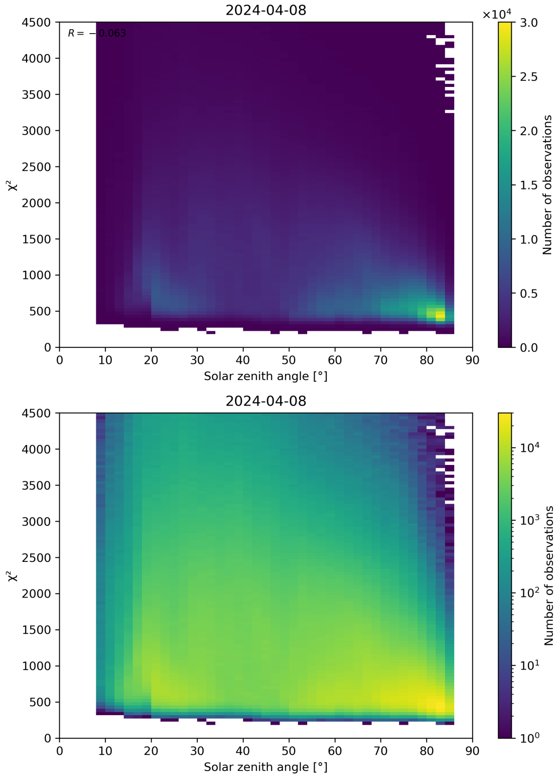
Figure 64: Scatter density plot of “Solar zenith angle” against “ \chi^2 ” for 2024-04-07 to 2024-04-09.
