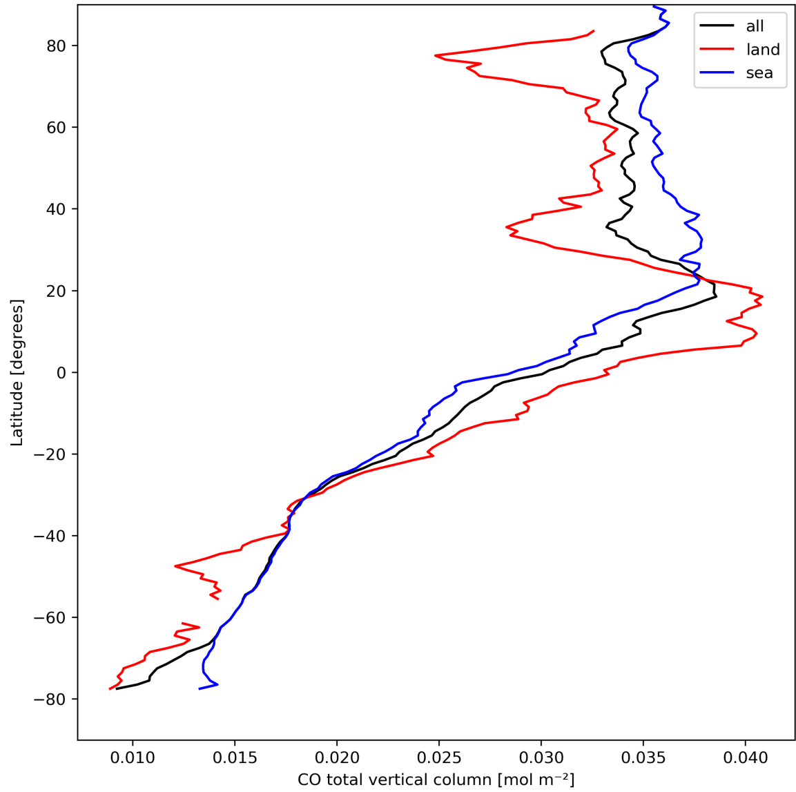
Figure 10: Zonal average of “CO total vertical column” for 2024-04-07 to 2024-04-09.
