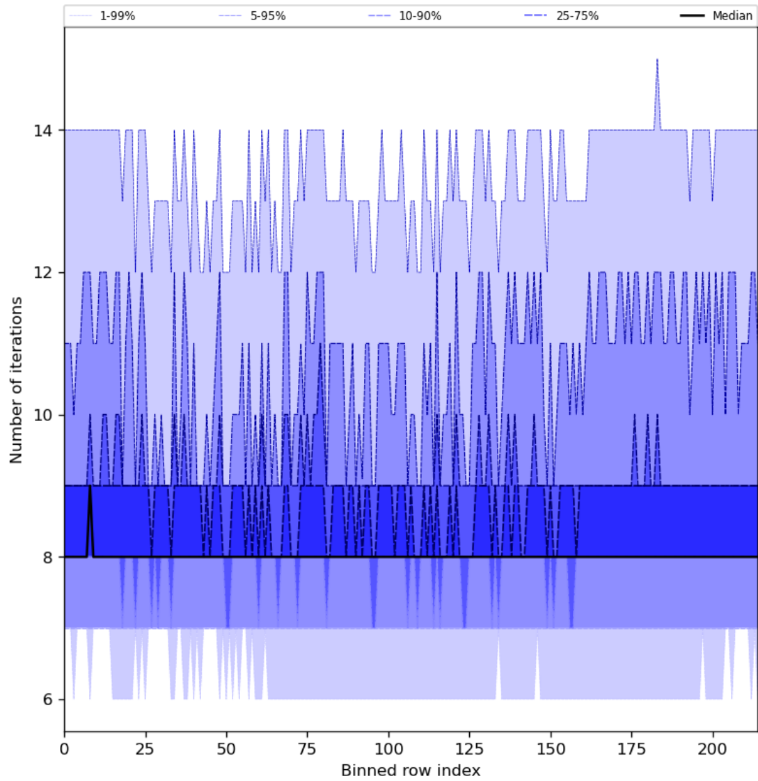
Figure 32: Along track statistics of “Number of iterations” for 2024-04-07 to 2024-04-09
