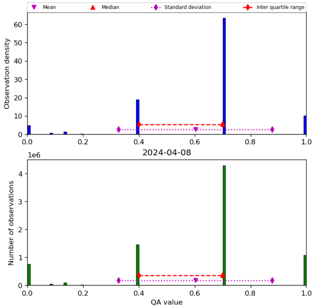
Figure 17: Histogram of “QA value” for 2024-04-07 to 2024-04-09
