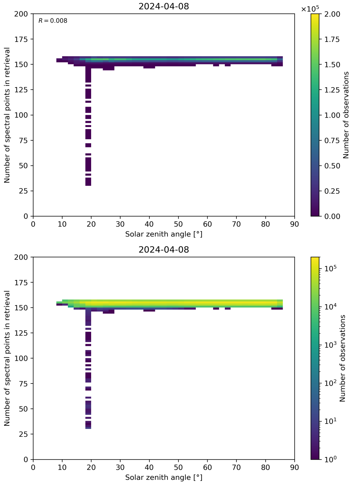
Figure 68: Scatter density plot of “Solar zenith angle” against “Number of spectral points in retrieval” for 2024-04-07 to 2024-04-09.
