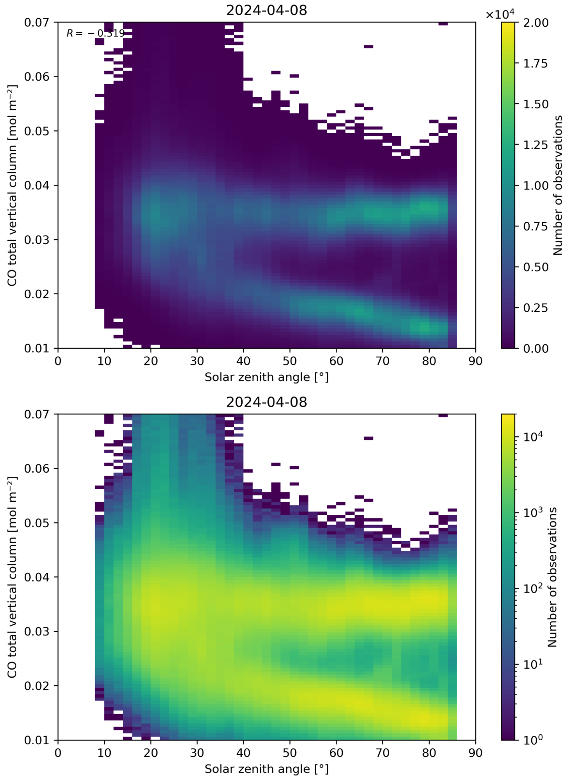
Figure 61: Scatter density plot of “Solar zenith angle” against “CO total vertical column” for 2024-04-07 to 2024-04-09.
