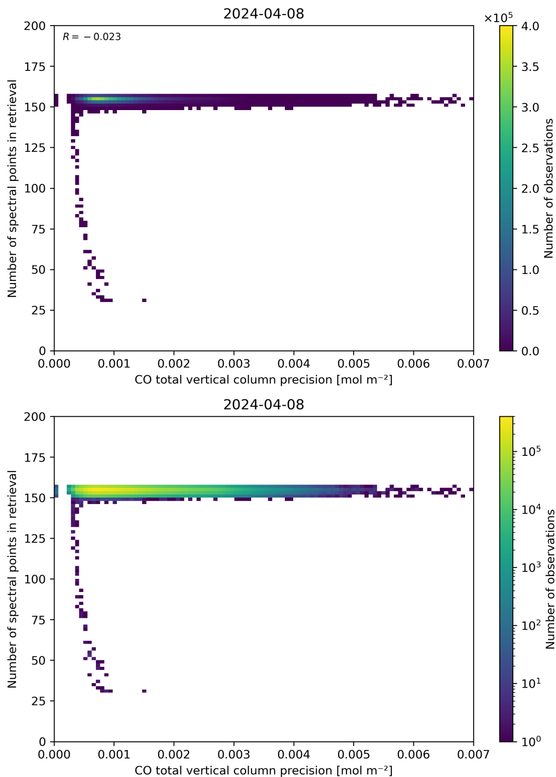
Figure 47: Scatter density plot of “CO total vertical column precision” against “Number of spectral points in retrieval” for 2024-04-07 to 2024-04-09.
