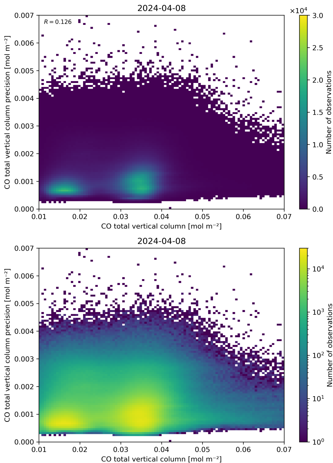
Figure 34: Scatter density plot of “CO total vertical column” against “CO total vertical column precision” for 2024-04-07 to 2024-04-09.
