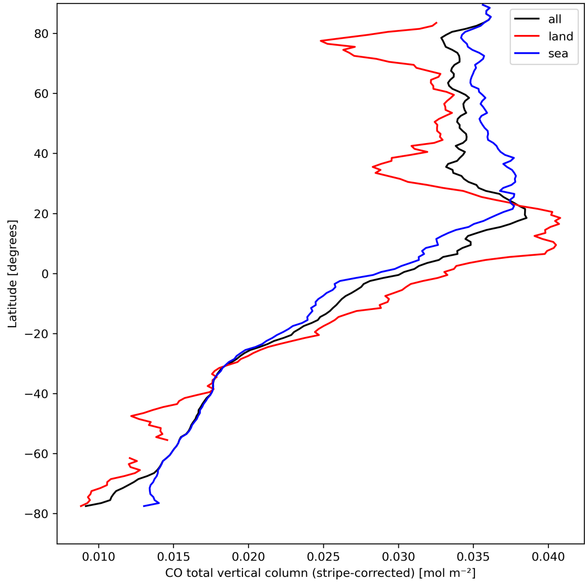
Figure 11: Zonal average of “CO total vertical column (stripe-corrected)” for 2024-04-07 to 2024-04-09.
