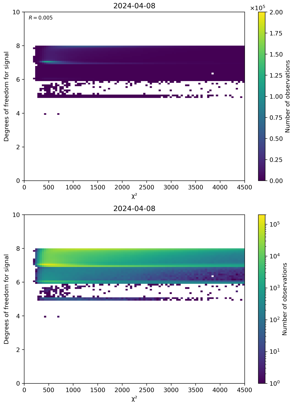
Figure 48: Scatter density plot of “ \chi^2 ” against “Degrees of freedom for signal” for 2024-04-07 to 2024-04-09.
