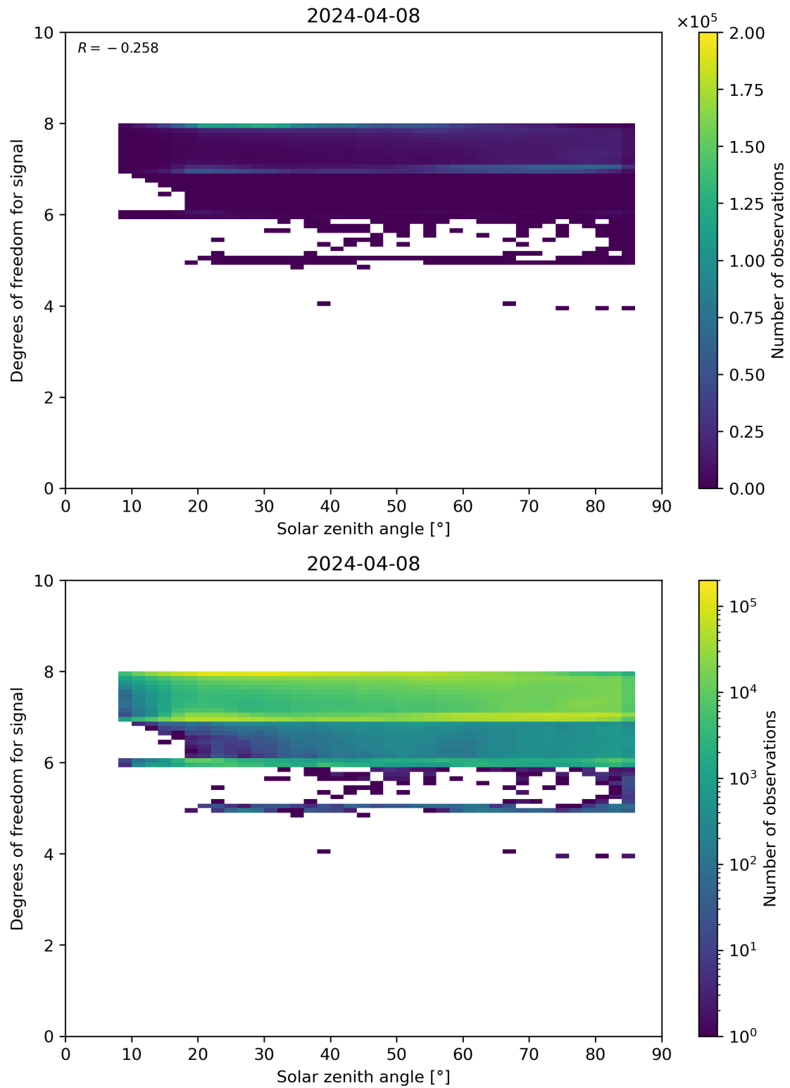
Figure 65: Scatter density plot of “Solar zenith angle” against “Degrees of freedom for signal” for 2024-04-07 to 2024-04-09.
