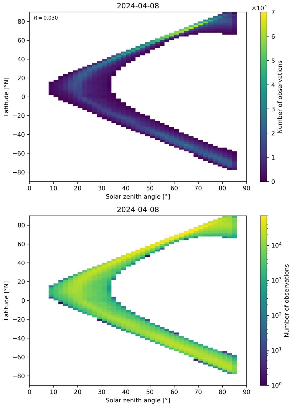
Figure 66: Scatter density plot of “Solar zenith angle” against “Latitude” for 2024-04-07 to 2024-04-09.
