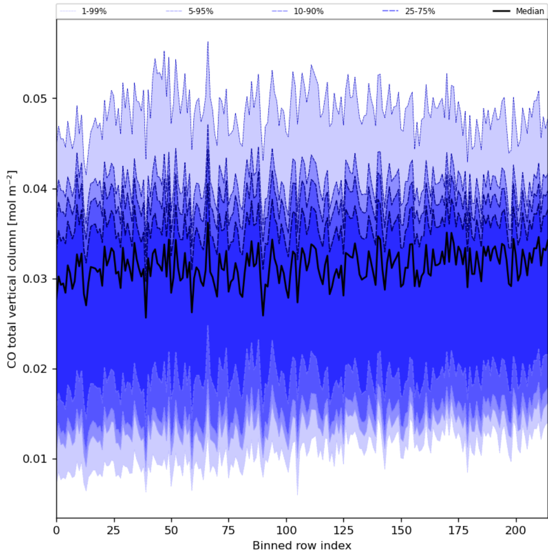
Figure 26: Along track statistics of “CO total vertical column” for 2024-04-07 to 2024-04-09
