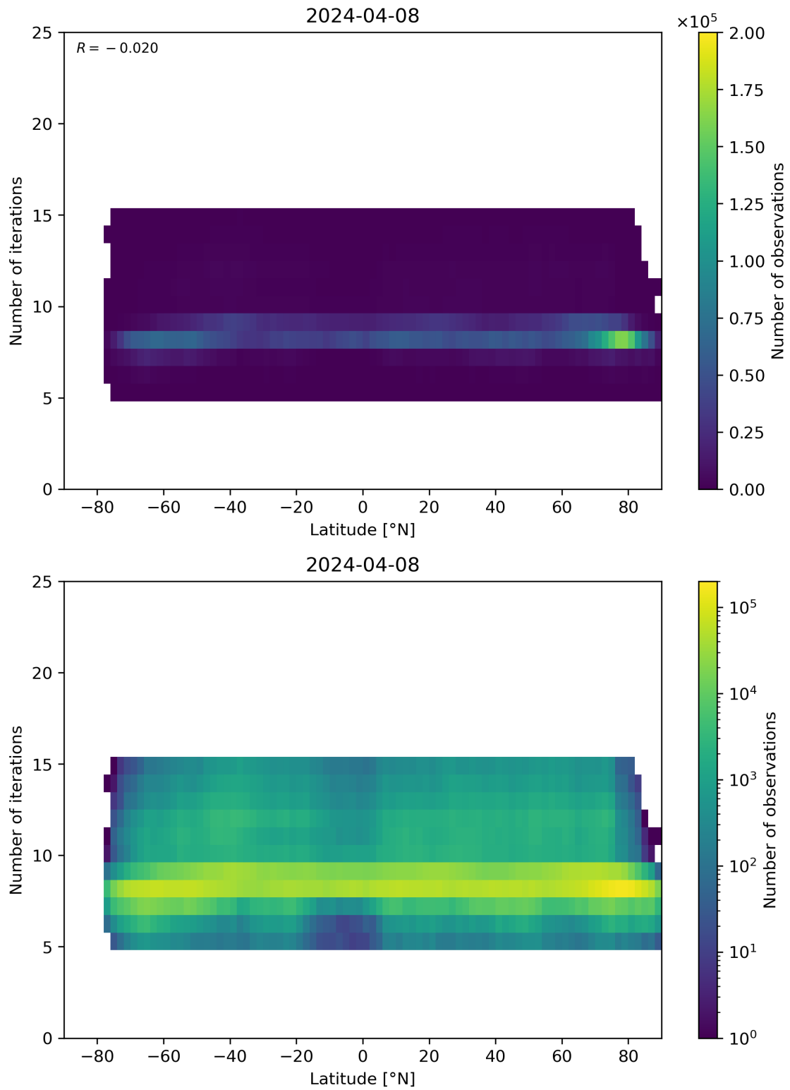
Figure 56: Scatter density plot of “Latitude” against “Number of iterations” for 2024-04-07 to 2024-04-09.
