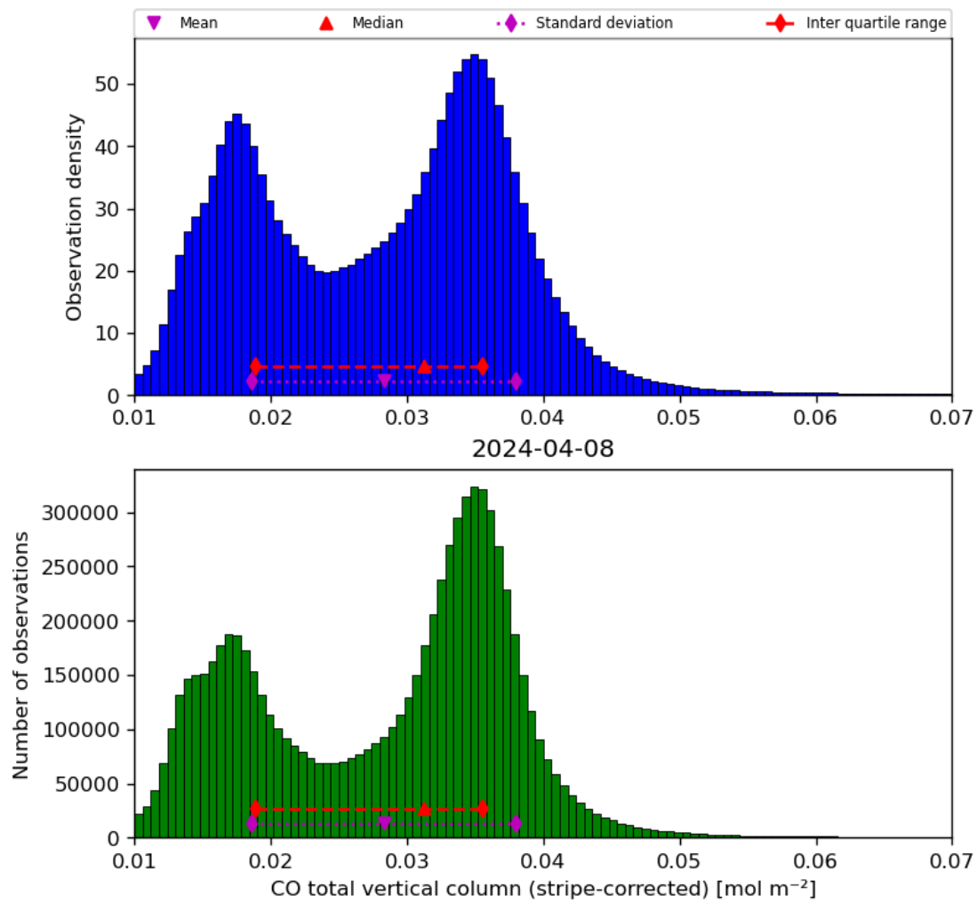
Figure 19: Histogram of “CO total vertical column (stripe-corrected)” for 2024-04-07 to 2024-04-09
