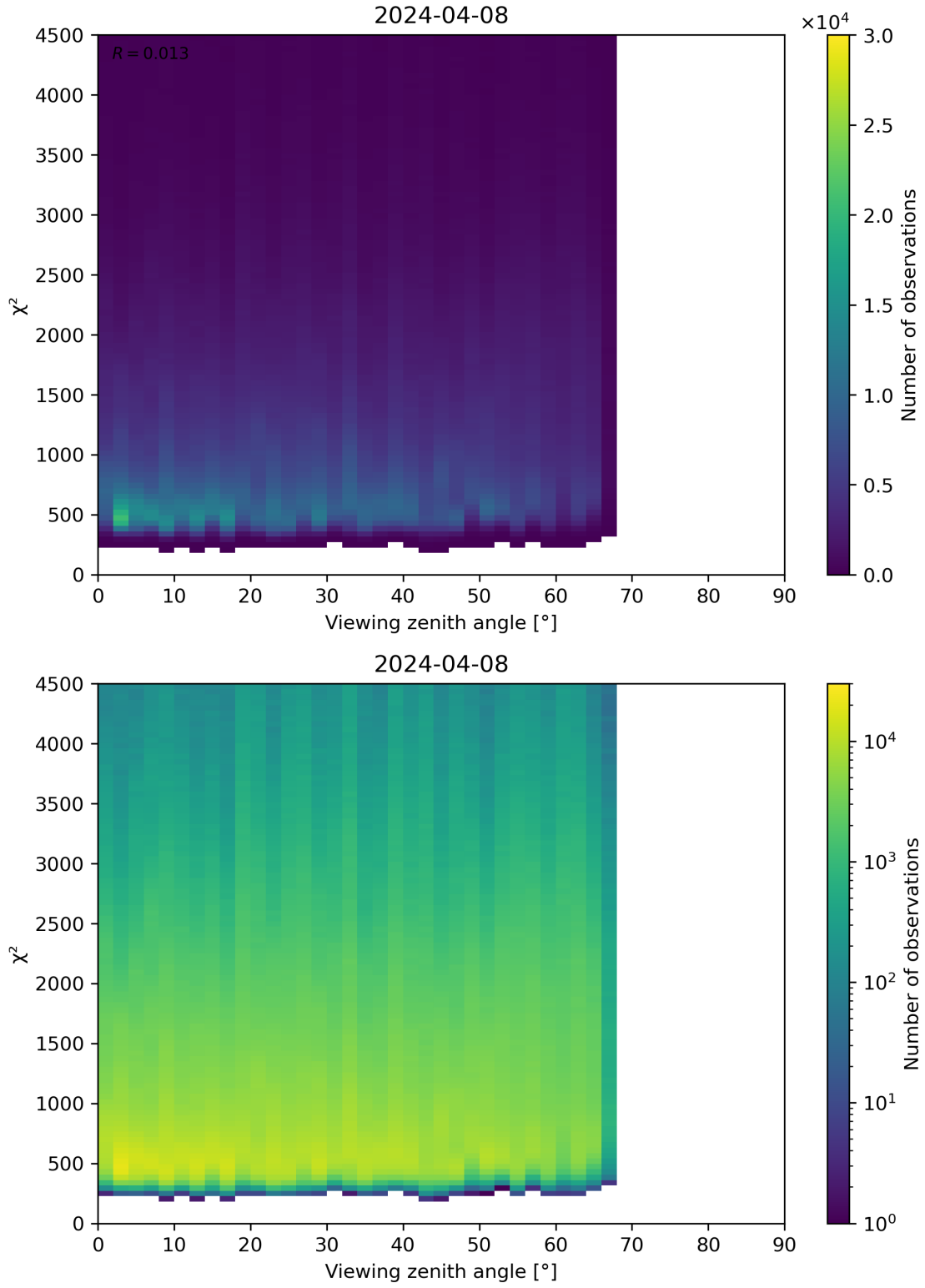
Figure 72: Scatter density plot of “Viewing zenith angle” against “ \chi^2 ” for 2024-04-07 to 2024-04-09.
