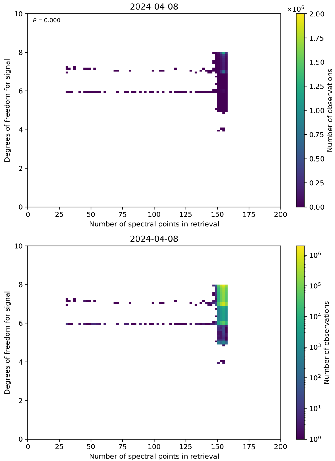
Figure 59: Scatter density plot of “Number of spectral points in retrieval” against “Degrees of freedom for signal” for 2024-04-07 to 2024-04-09.
