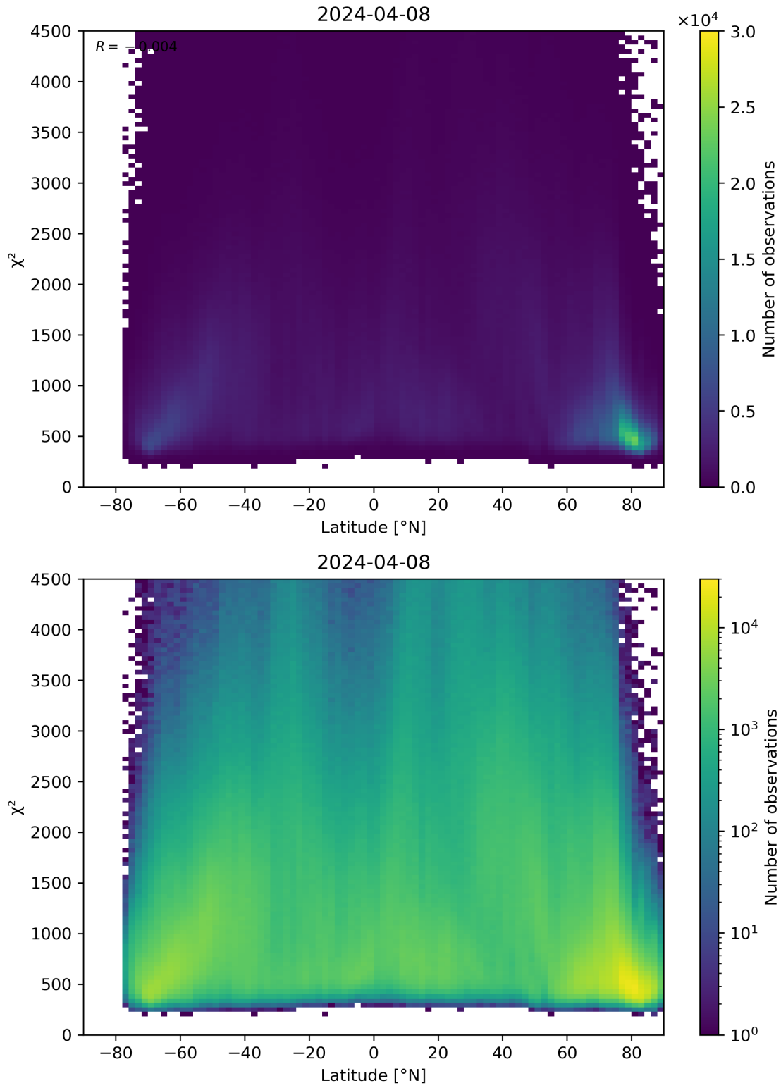
Figure 54: Scatter density plot of “Latitude” against “ \chi^2 ” for 2024-04-07 to 2024-04-09.
