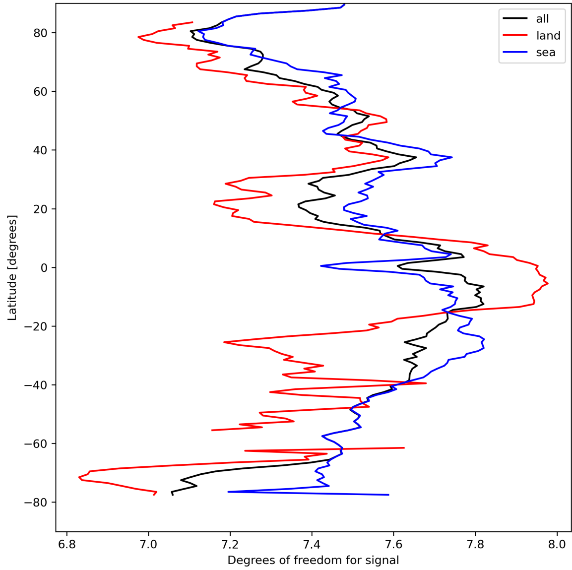
Figure 15: Zonal average of “Degrees of freedom for signal” for 2024-04-07 to 2024-04-09.
