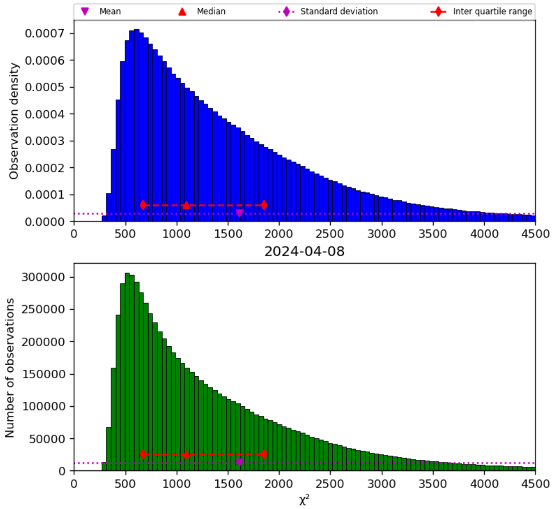
Figure 22: Histogram of “ \chi^2 ” for 2024-04-07 to 2024-04-09
