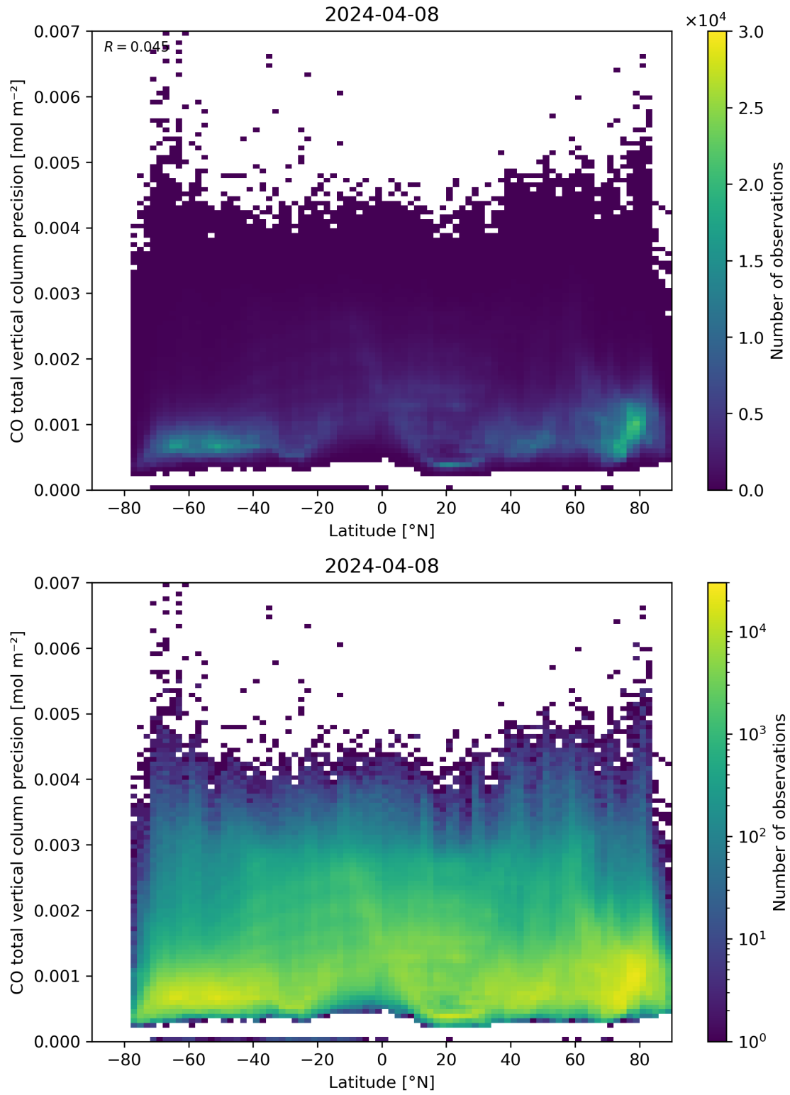
Figure 53: Scatter density plot of “Latitude” against “CO total vertical column precision” for 2024-04-07 to 2024-04-09.
