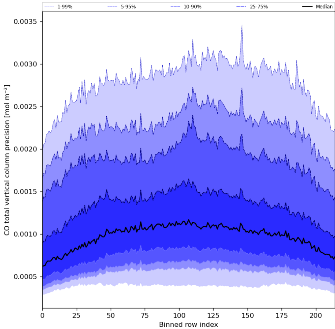
Figure 28: Along track statistics of “CO total vertical column precision” for 2024-04-07 to 2024-04-09
