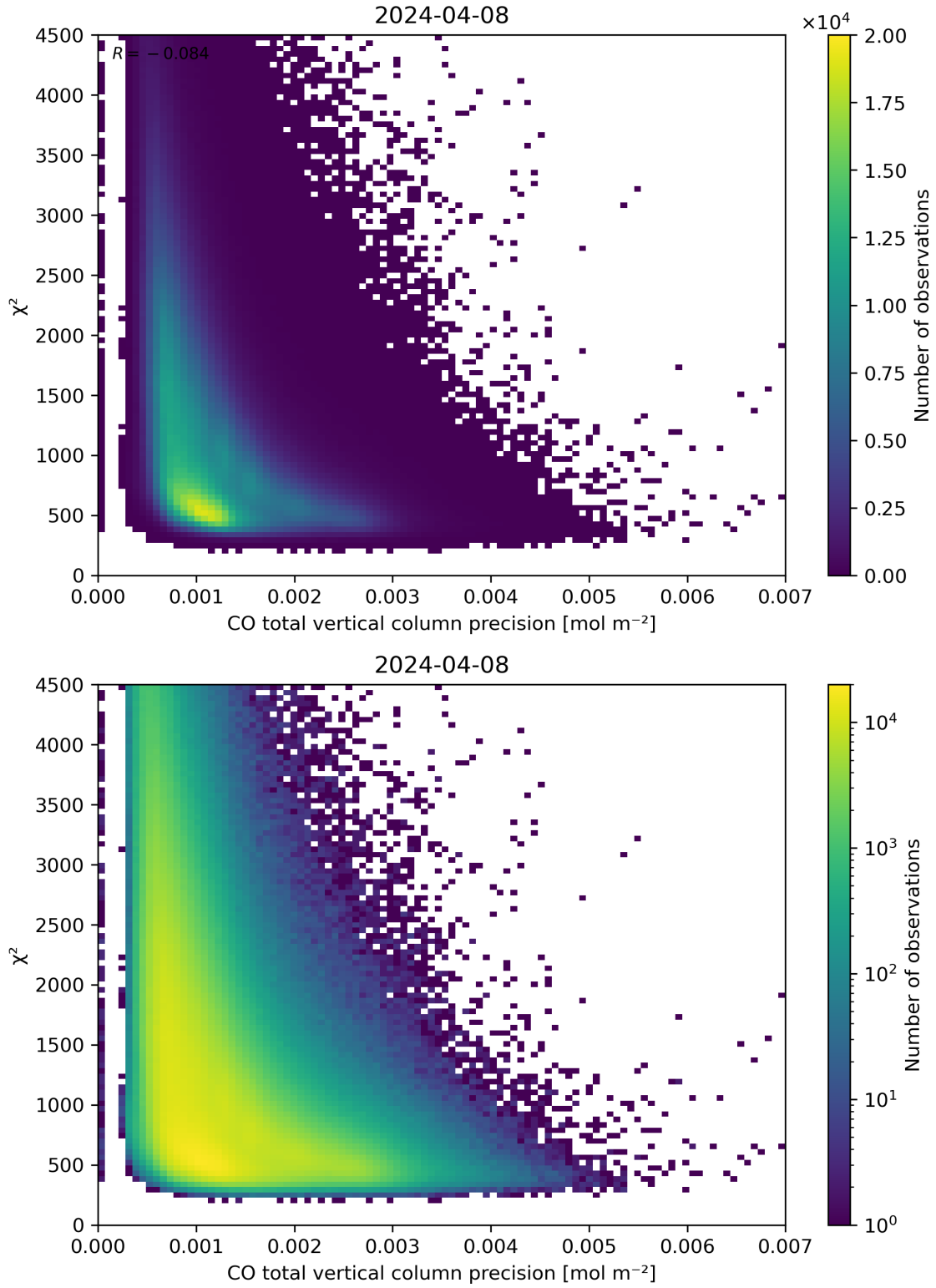
Figure 44: Scatter density plot of “CO total vertical column precision” against “ \chi^2 ” for 2024-04-07 to 2024-04-09.
