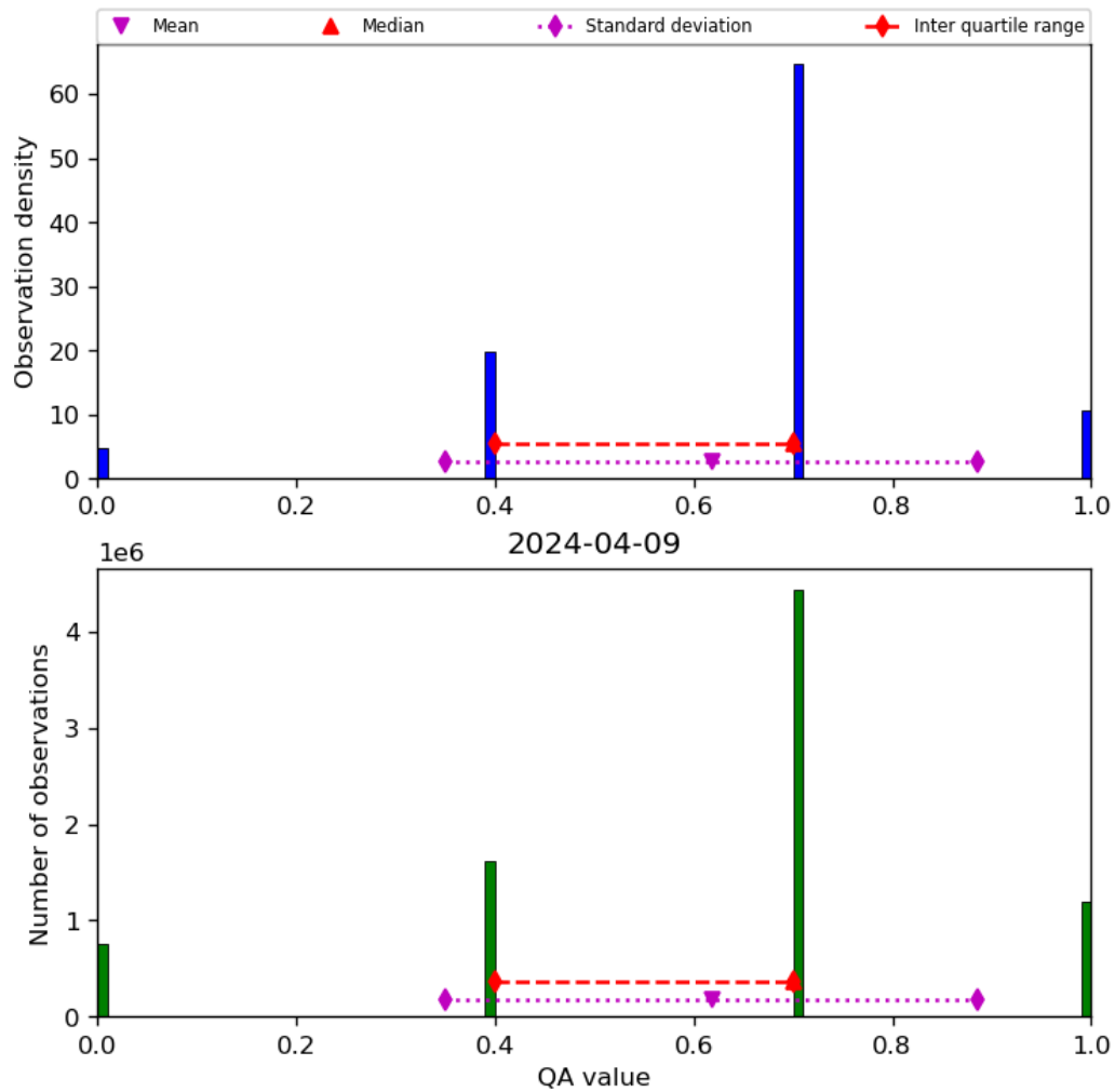
Figure 17: Histogram of “QA value” for 2024-04-08 to 2024-04-10
