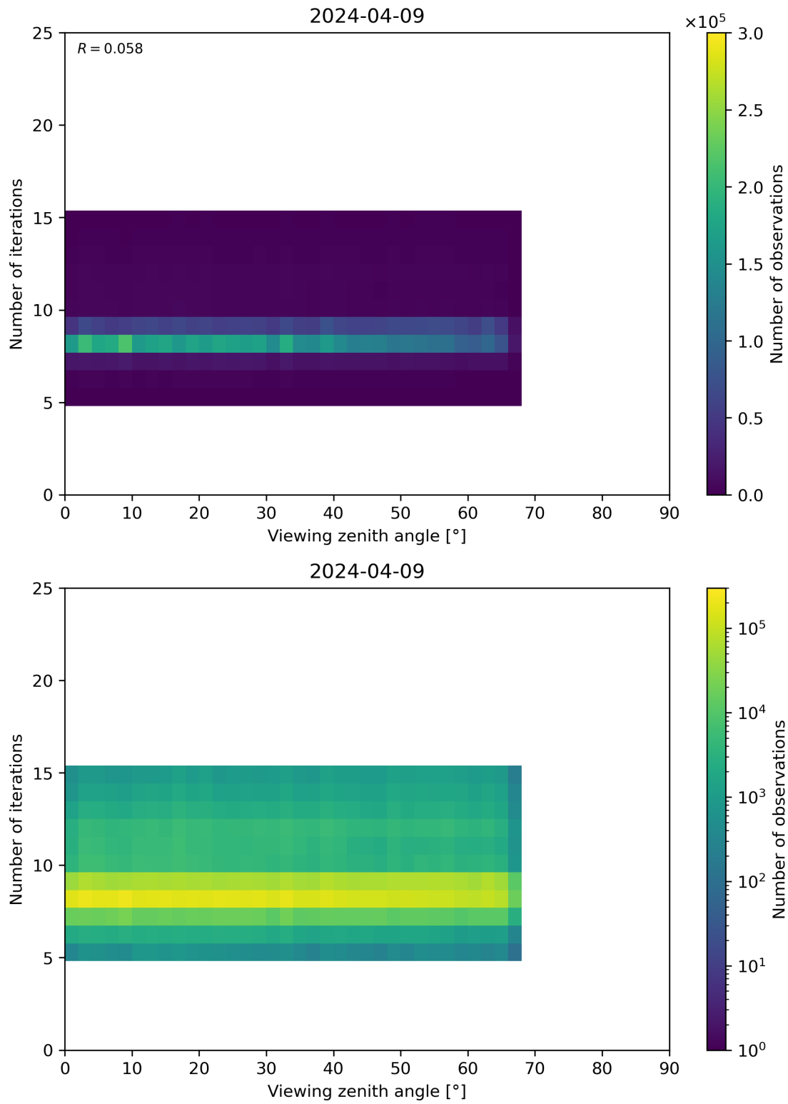
Figure 75: Scatter density plot of “Viewing zenith angle” against “Number of iterations” for 2024-04-08 to 2024-04-10.
