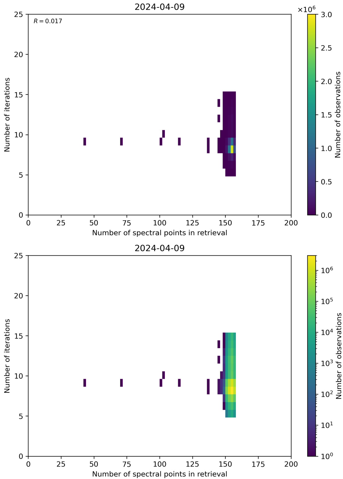
Figure 60: Scatter density plot of “Number of spectral points in retrieval” against “Number of iterations” for 2024-04-08 to 2024-04-10.
