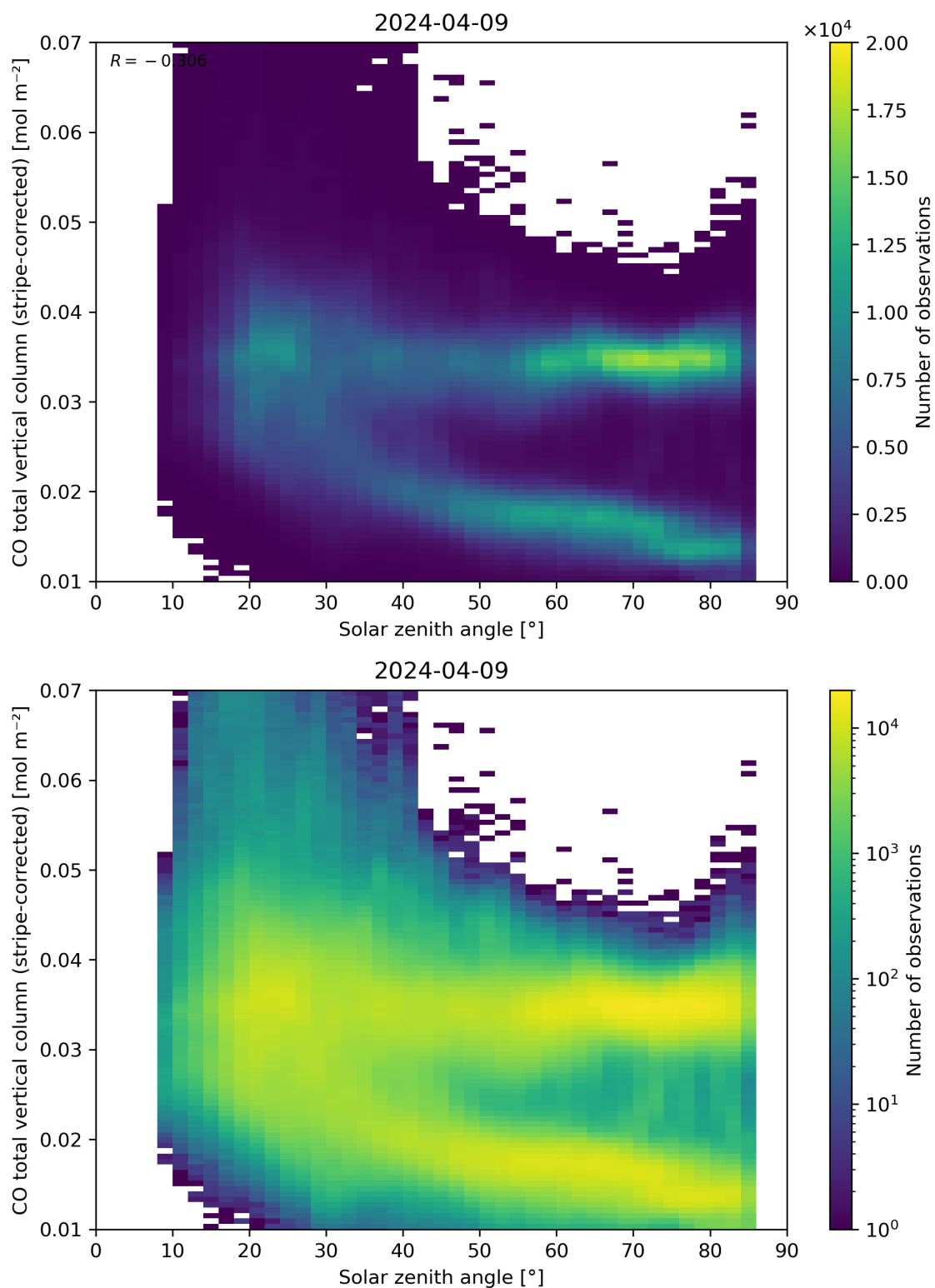
Figure 62: Scatter density plot of “Solar zenith angle” against “CO total vertical column (stripe-corrected)” for 2024-04-08 to 2024-04-10.
