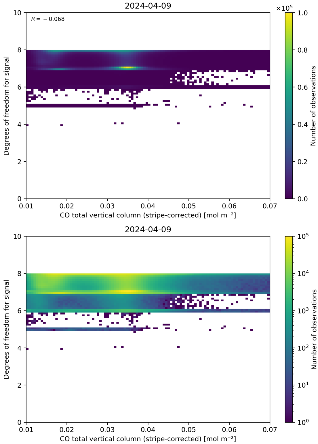
Figure 38: Scatter density plot of “CO total vertical column (stripe-corrected)” against “Degrees of freedom for signal” for 2024-04-08 to 2024-04-10.
