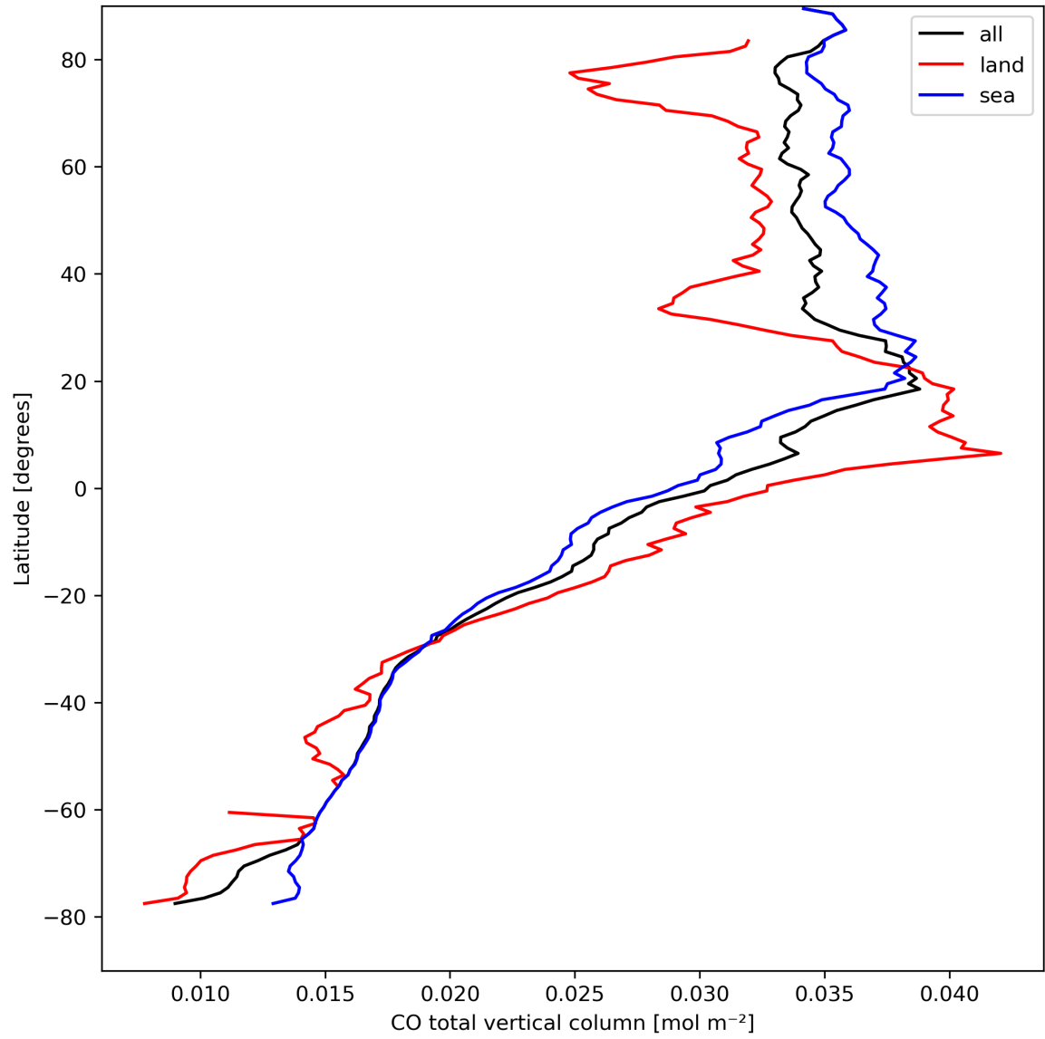
Figure 10: Zonal average of “CO total vertical column” for 2024-04-08 to 2024-04-10.
