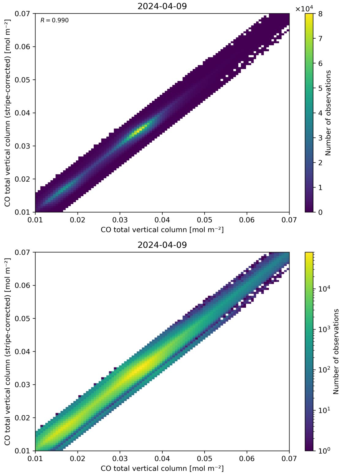
Figure 33: Scatter density plot of “CO total vertical column” against “CO total vertical column (stripe-corrected)” for 2024-04-08 to 2024-04-10.
