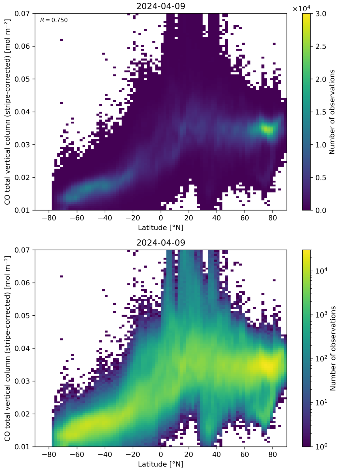
Figure 52: Scatter density plot of “Latitude” against “CO total vertical column (stripe-corrected)” for 2024-04-08 to 2024-04-10.
