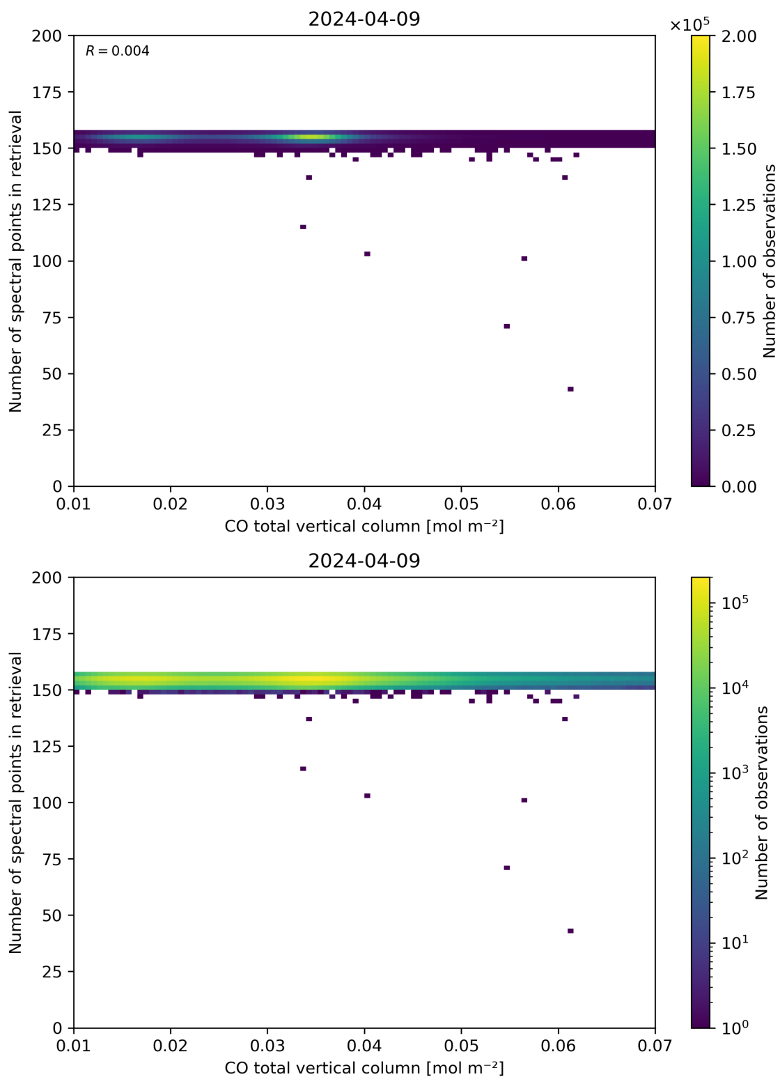
Figure 43: Scatter density plot of “CO total vertical column” against “Number of spectral points in retrieval” for 2024-04-08 to 2024-04-10.
