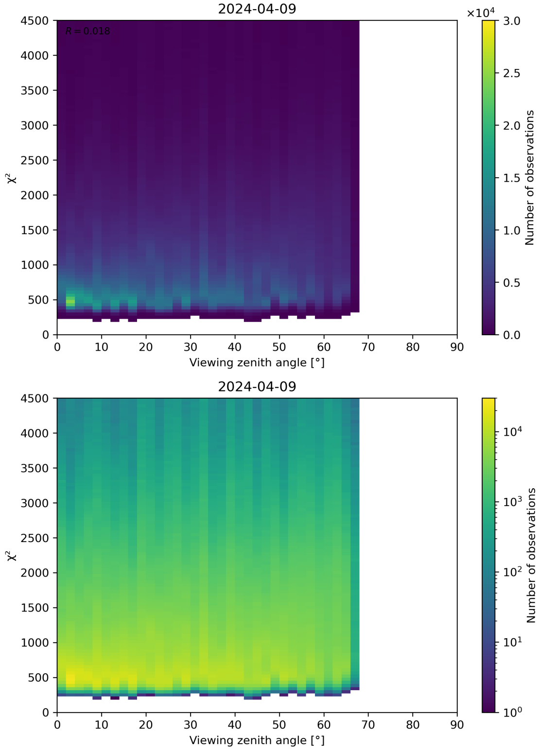
Figure 72: Scatter density plot of “Viewing zenith angle” against “ \chi^2 ” for 2024-04-08 to 2024-04-10.
