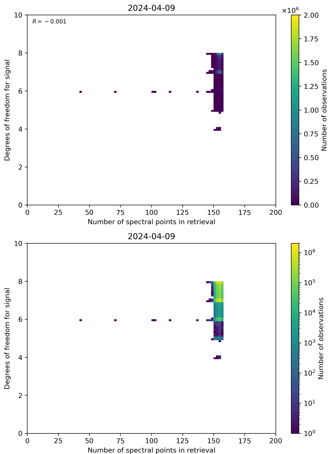
Figure 59: Scatter density plot of “Number of spectral points in retrieval” against “Degrees of freedom for signal” for 2024-04-08 to 2024-04-10.
