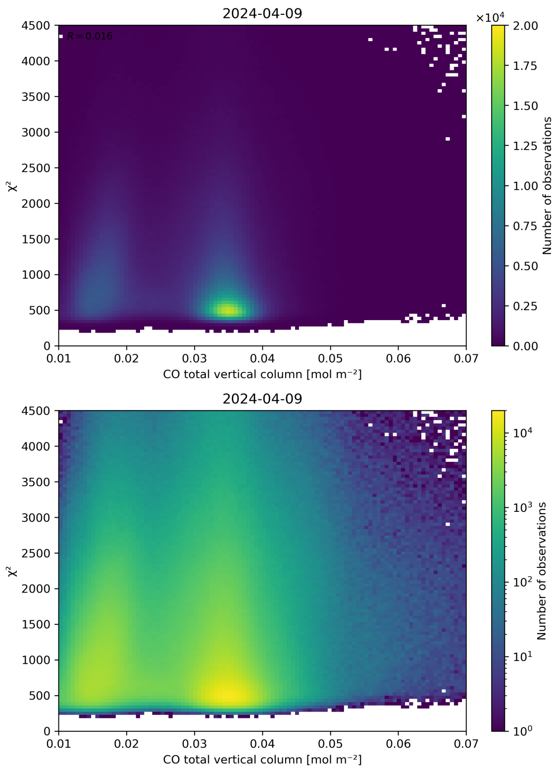
Figure 35: Scatter density plot of “CO total vertical column” against “ \chi^2 ” for 2024-04-08 to 2024-04-10.
