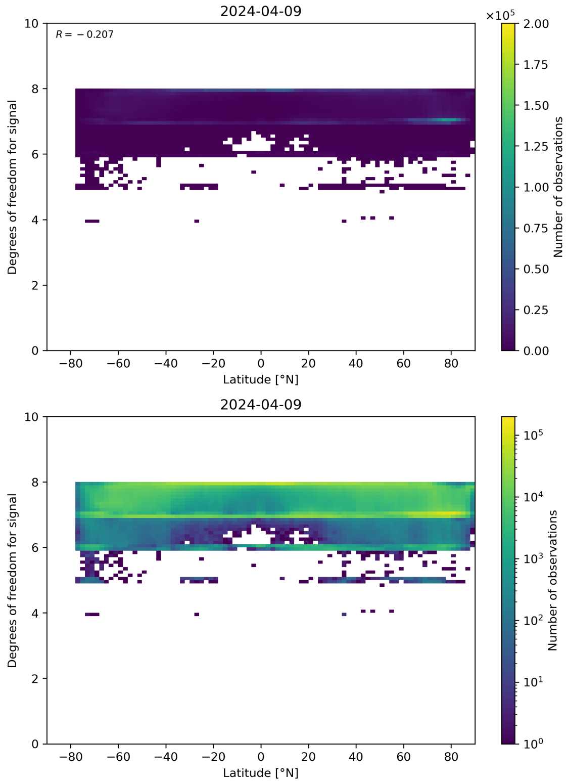
Figure 55: Scatter density plot of “Latitude” against “Degrees of freedom for signal” for 2024-04-08 to 2024-04-10.
