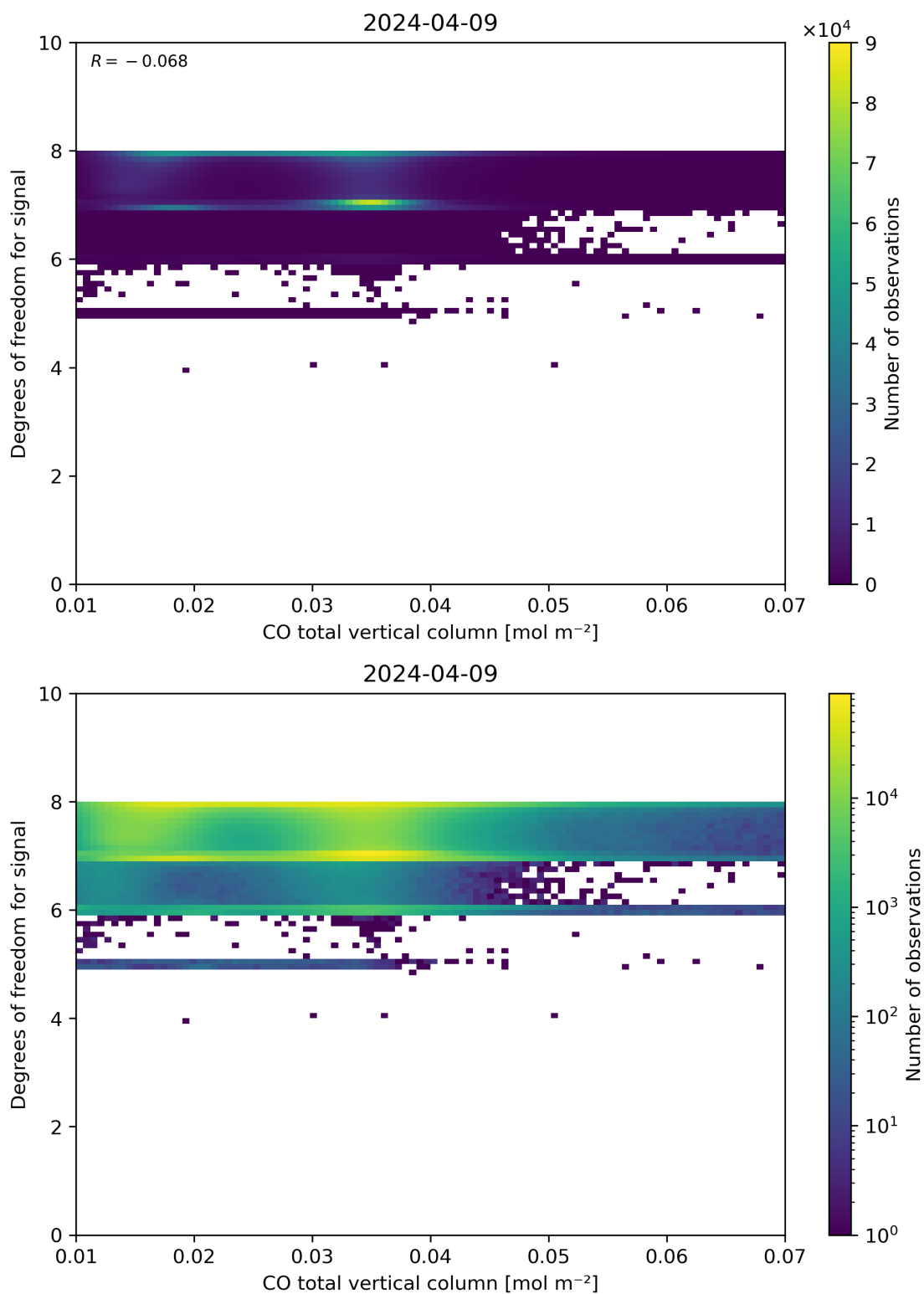
Figure 41: Scatter density plot of “CO total vertical column” against “Degrees of freedom for signal” for 2024-04-08 to 2024-04-10.
