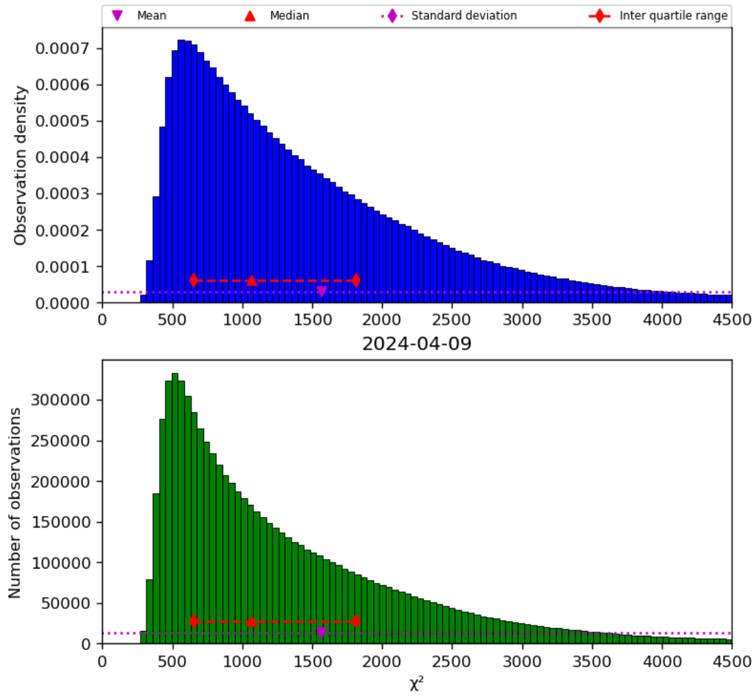
Figure 22: Histogram of “ \chi^2 ” for 2024-04-08 to 2024-04-10
