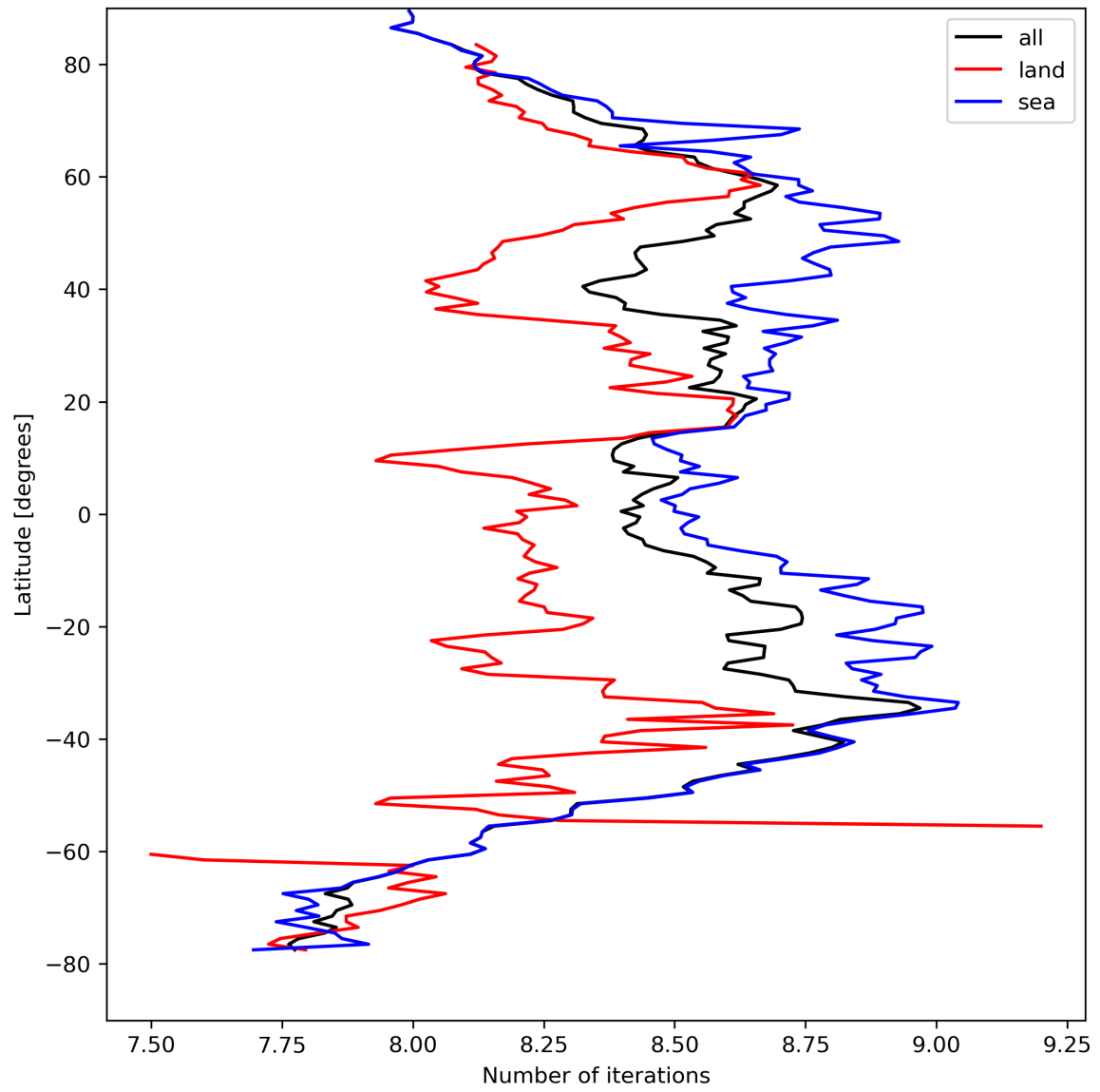
Figure 16: Zonal average of “Number of iterations” for 2024-04-08 to 2024-04-10.
