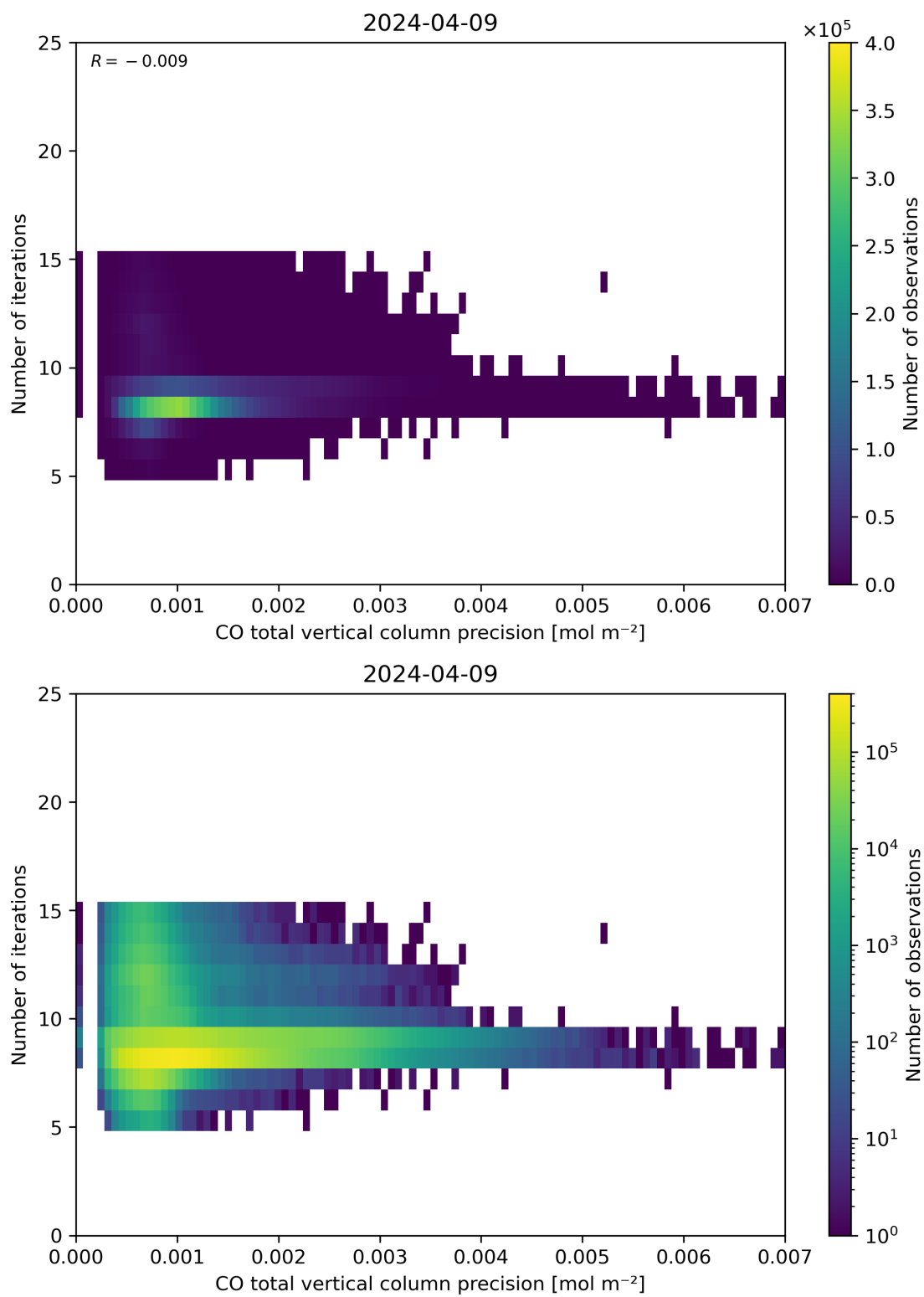
Figure 46: Scatter density plot of “CO total vertical column precision” against “Number of iterations” for 2024-04-08 to 2024-04-10.
