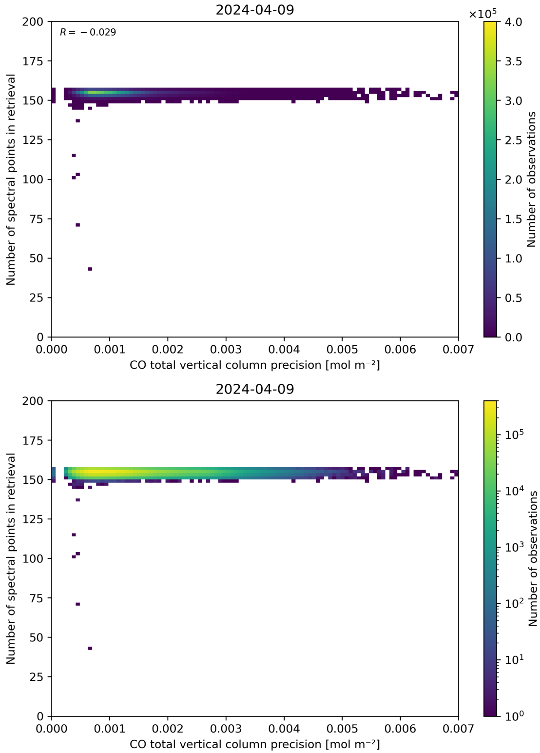
Figure 47: Scatter density plot of “CO total vertical column precision” against “Number of spectral points in retrieval” for 2024-04-08 to 2024-04-10.
