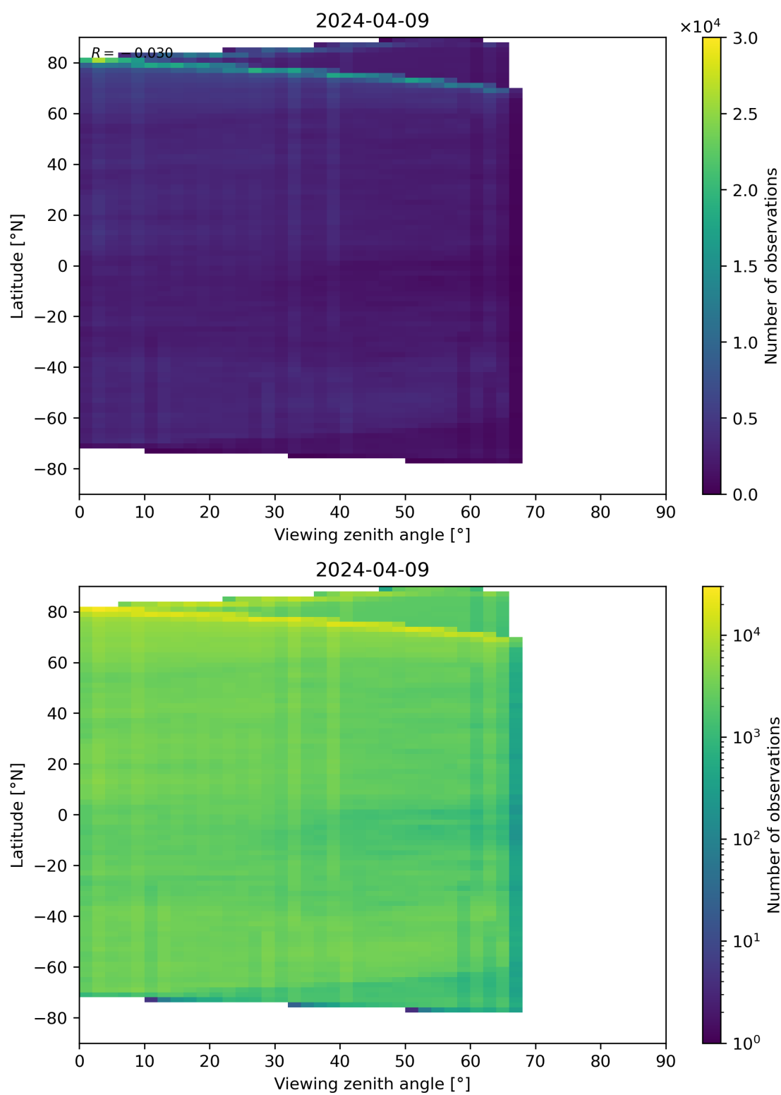
Figure 74: Scatter density plot of “Viewing zenith angle” against “Latitude” for 2024-04-08 to 2024-04-10.
