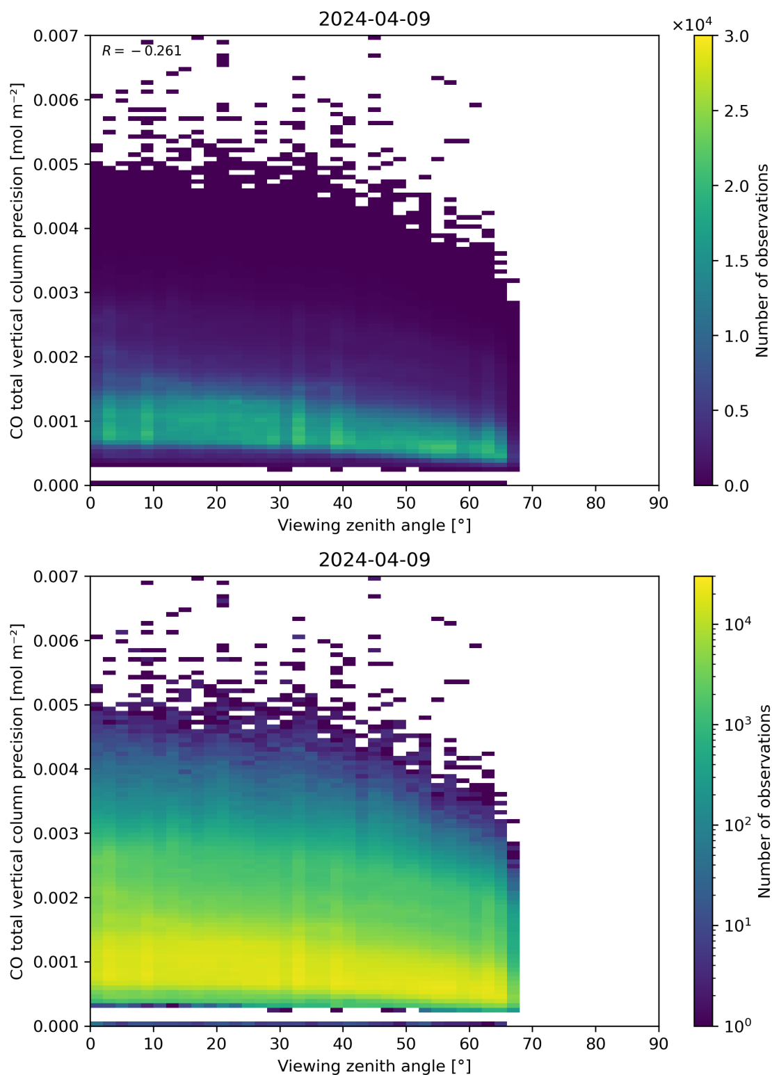
Figure 71: Scatter density plot of “Viewing zenith angle” against “CO total vertical column precision” for 2024-04-08 to 2024-04-10.
