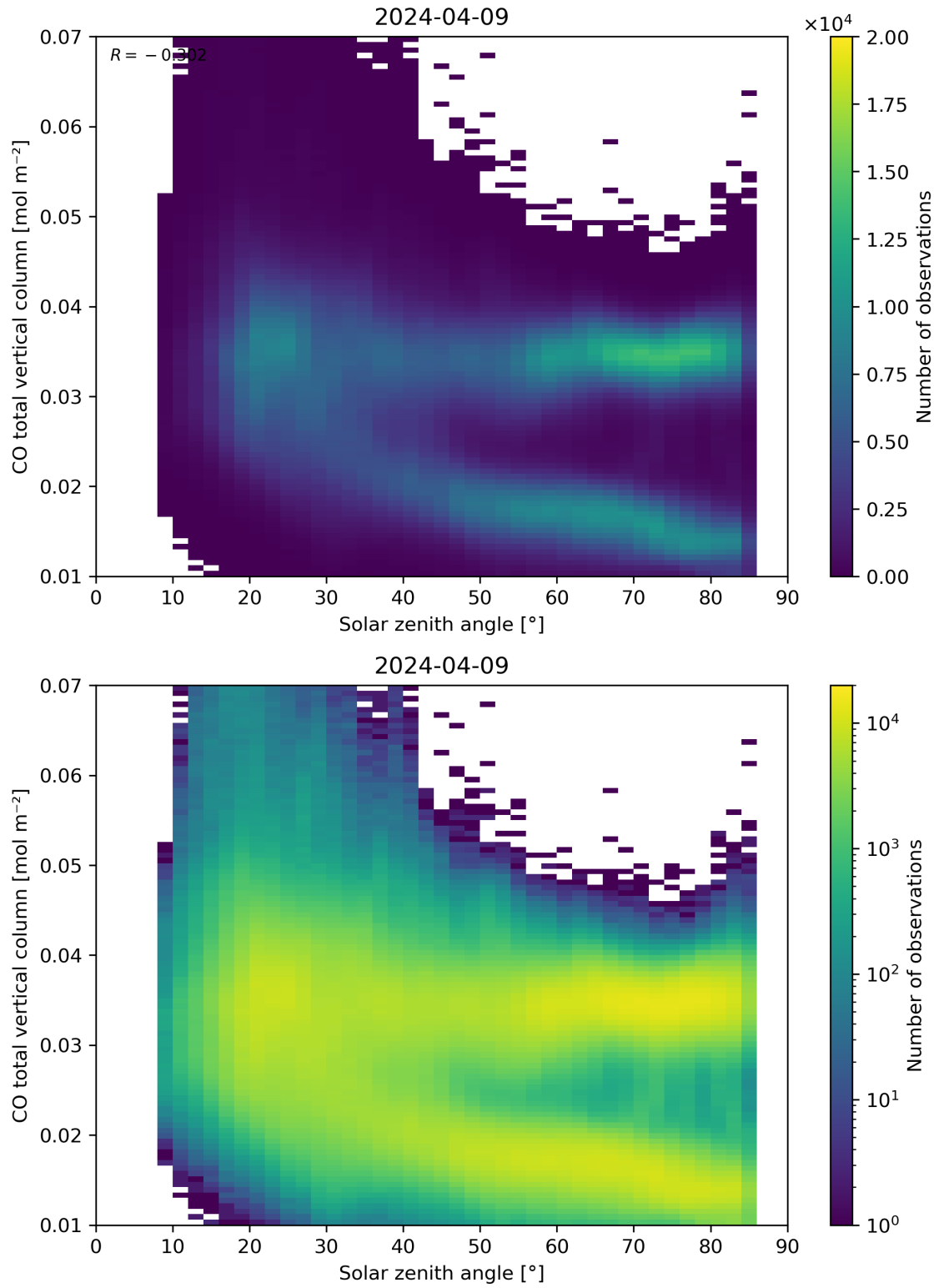
Figure 61: Scatter density plot of “Solar zenith angle” against “CO total vertical column” for 2024-04-08 to 2024-04-10.
