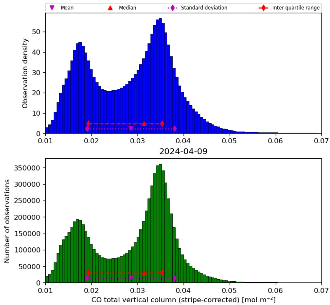
Figure 19: Histogram of “CO total vertical column (stripe-corrected)” for 2024-04-08 to 2024-04-10
