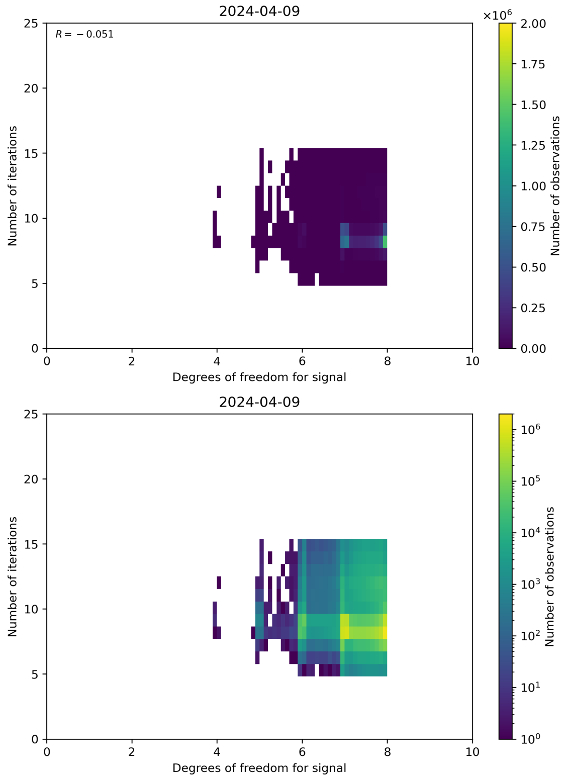
Figure 50: Scatter density plot of “Degrees of freedom for signal” against “Number of iterations” for 2024-04-08 to 2024-04-10.
