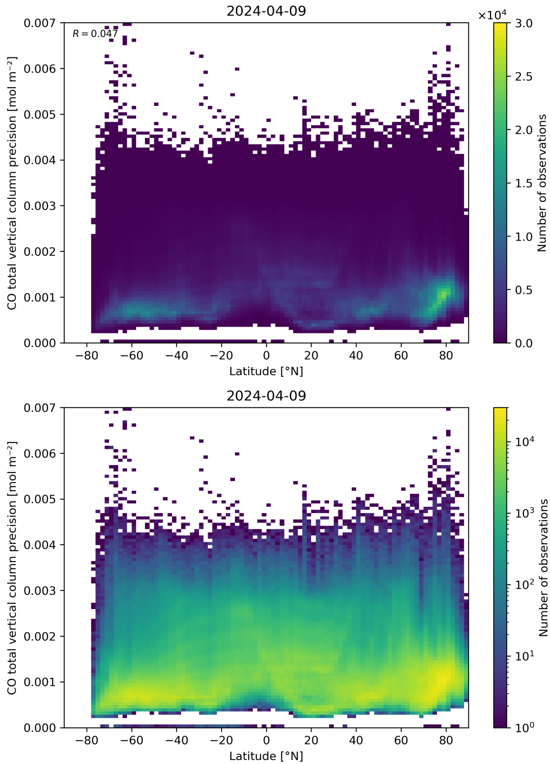
Figure 53: Scatter density plot of “Latitude” against “CO total vertical column precision” for 2024-04-08 to 2024-04-10.
