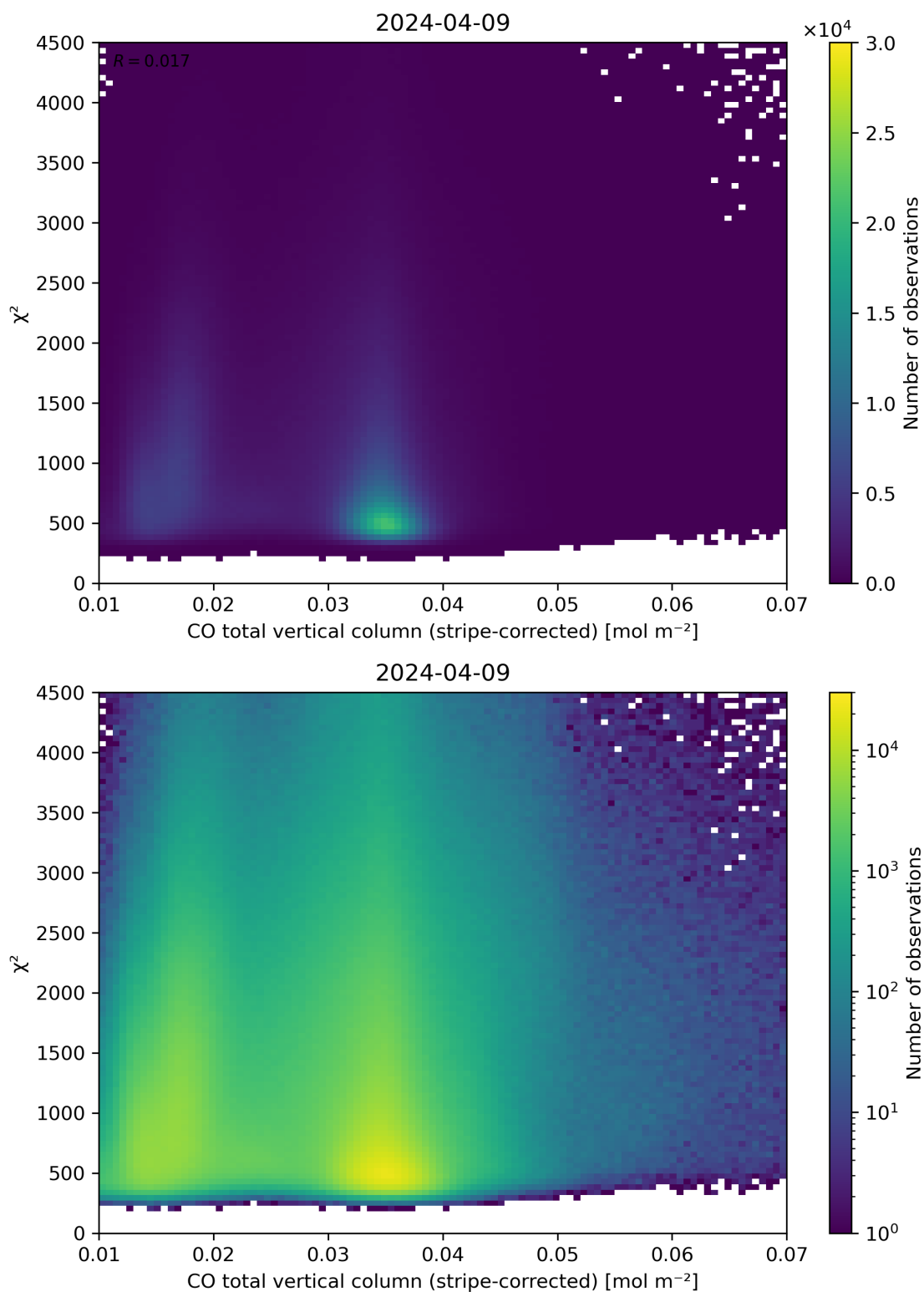
Figure 37: Scatter density plot of “CO total vertical column (stripe-corrected)” against “ \chi^2 ” for 2024-04-08 to 2024-04-10.
