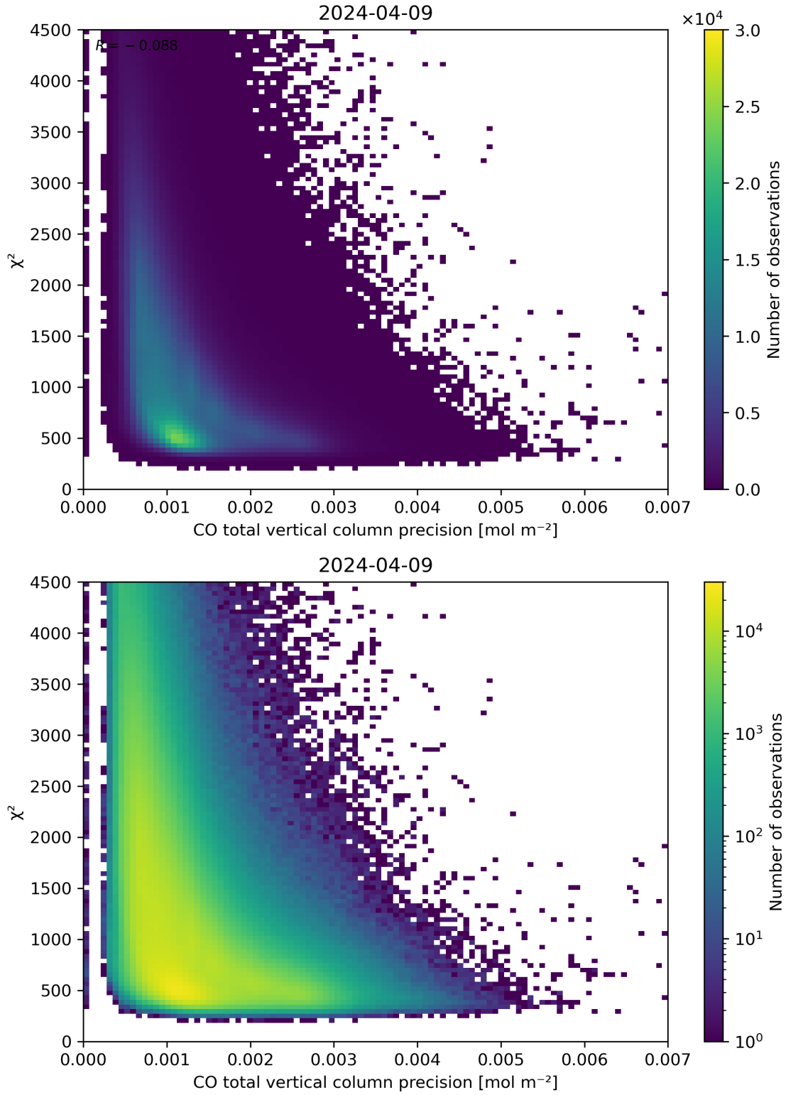
Figure 44: Scatter density plot of “CO total vertical column precision” against “ \chi^2 ” for 2024-04-08 to 2024-04-10.
