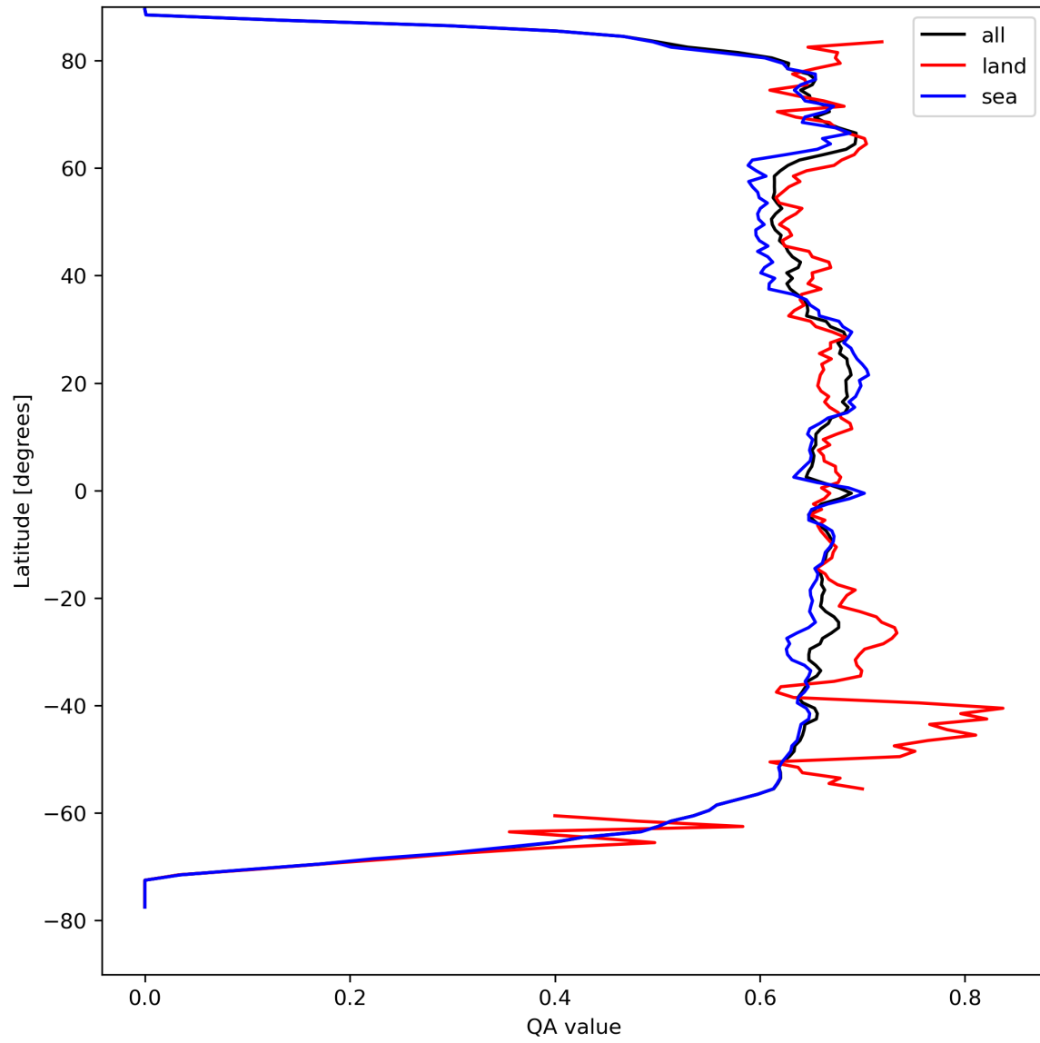
Figure 9: Zonal average of “QA value” for 2024-04-08 to 2024-04-10.
