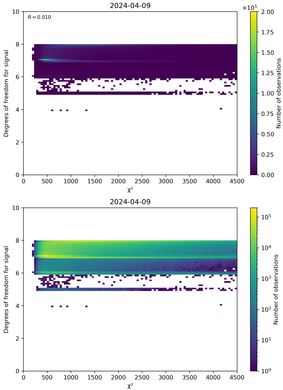
Figure 48: Scatter density plot of “ \chi^2 ” against “Degrees of freedom for signal” for 2024-04-08 to 2024-04-10.
