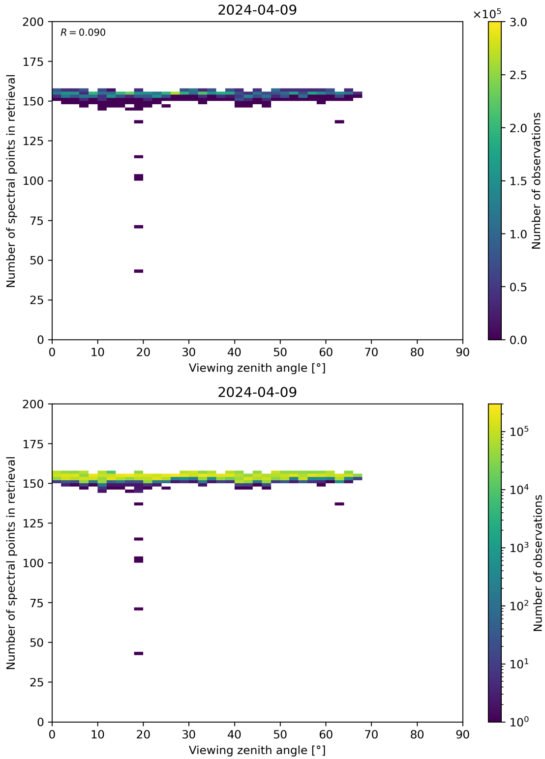
Figure 76: Scatter density plot of “Viewing zenith angle” against “Number of spectral points in retrieval” for 2024-04-08 to 2024-04-10.
