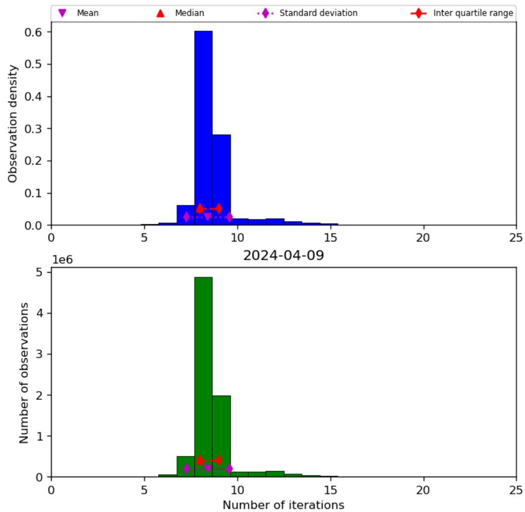
Figure 24: Histogram of “Number of iterations” for 2024-04-08 to 2024-04-10
