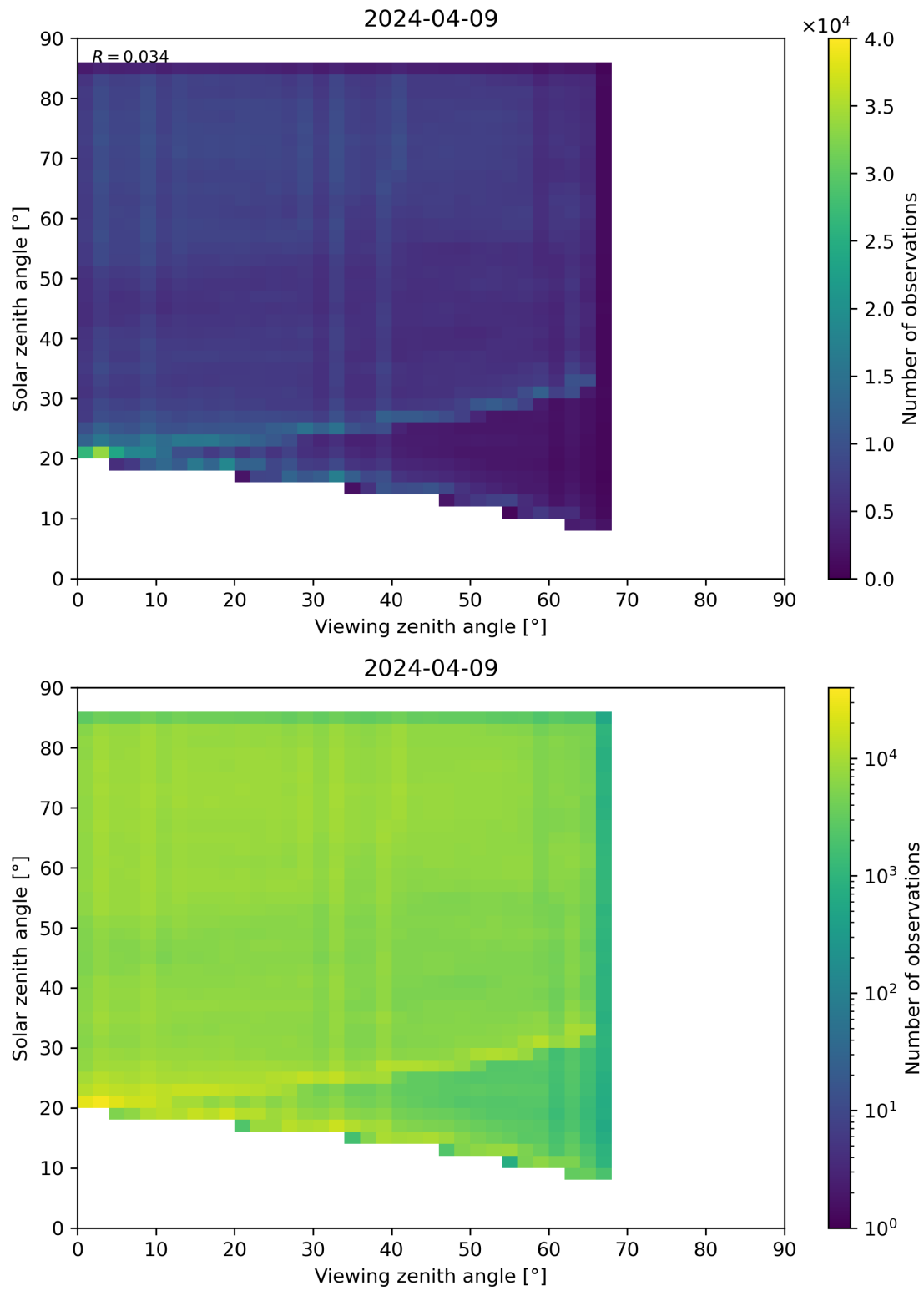
Figure 77: Scatter density plot of “Viewing zenith angle” against “Solar zenith angle” for 2024-04-08 to 2024-04-10.
