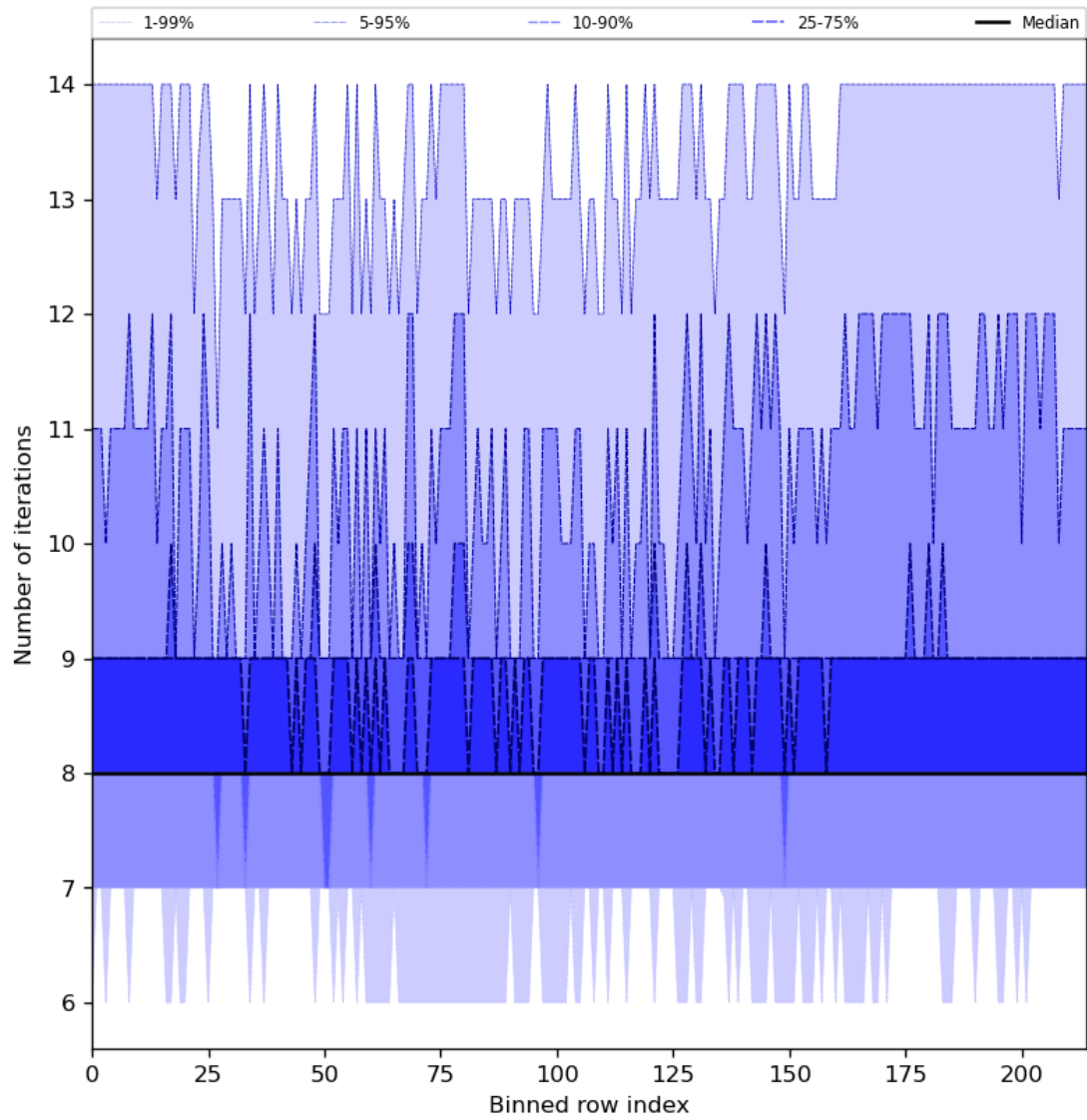
Figure 32: Along track statistics of “Number of iterations” for 2024-04-08 to 2024-04-10
