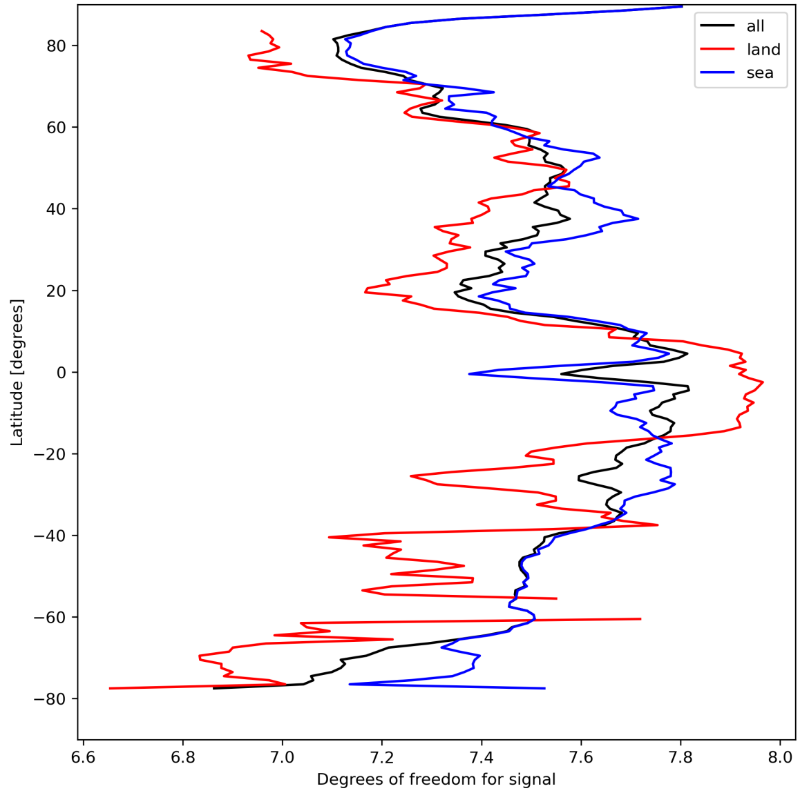
Figure 15: Zonal average of “Degrees of freedom for signal” for 2024-04-08 to 2024-04-10.
