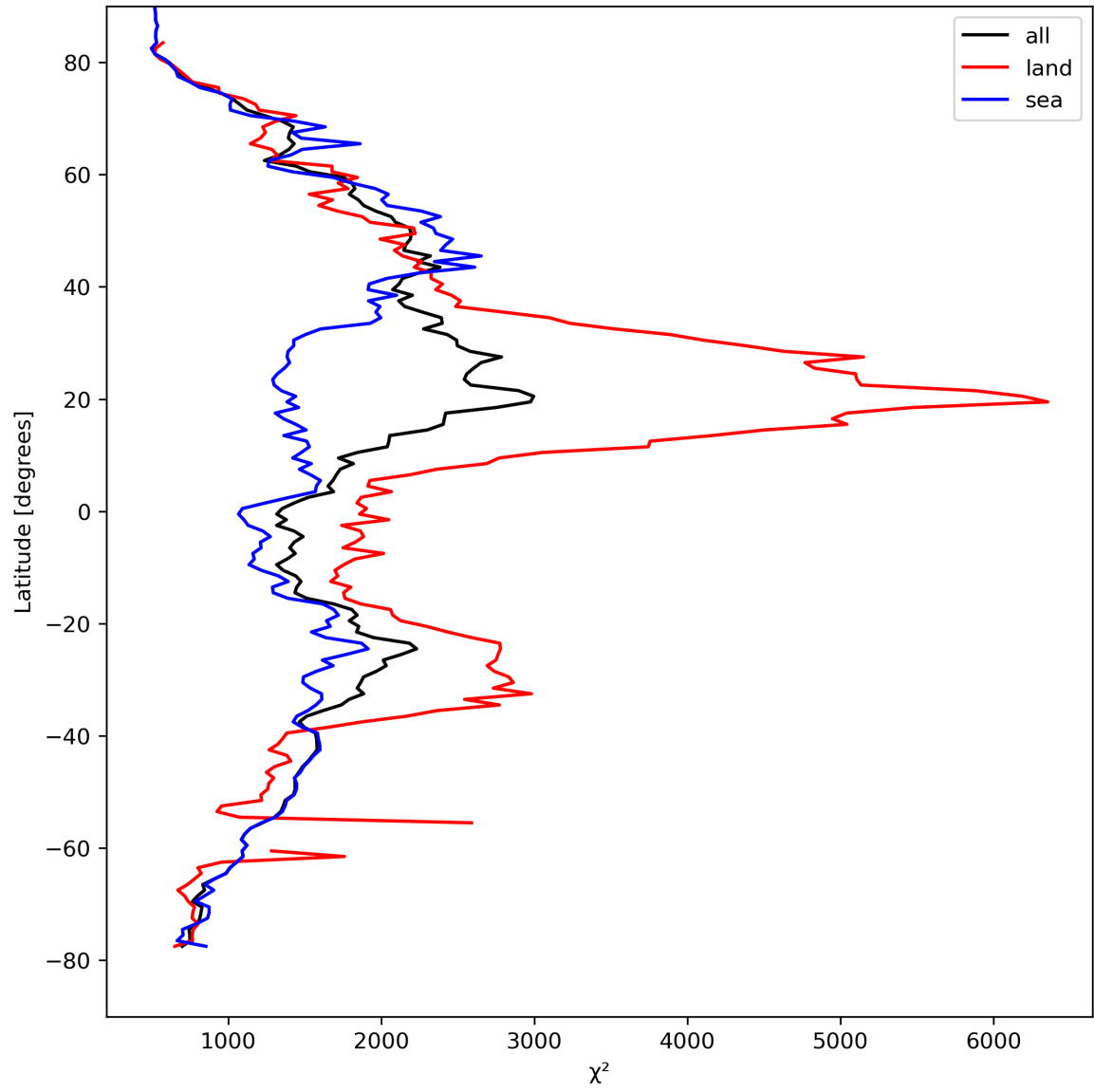
Figure 14: Zonal average of “ \chi^2 ” for 2024-04-08 to 2024-04-10.
