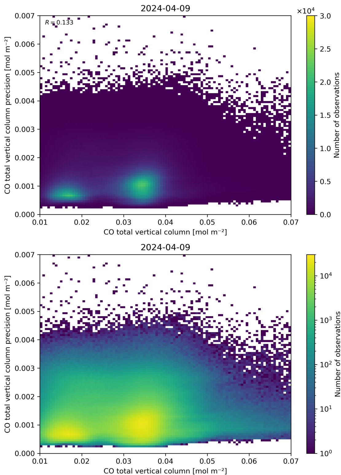
Figure 34: Scatter density plot of “CO total vertical column” against “CO total vertical column precision” for 2024-04-08 to 2024-04-10.
