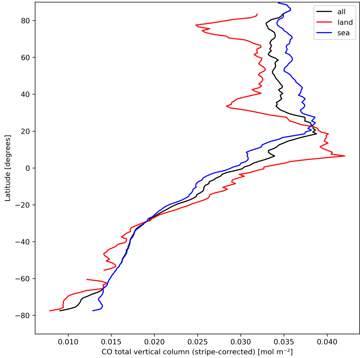
Figure 11: Zonal average of “CO total vertical column (stripe-corrected)” for 2024-04-08 to 2024-04-10.
