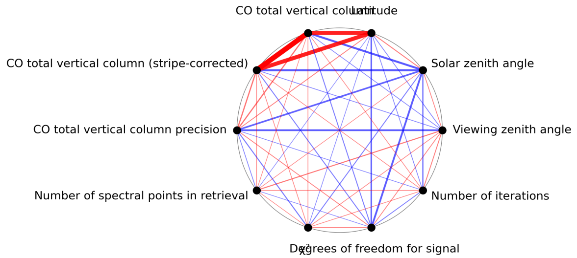
Figure 1: Map of correlation graph for 2024-04-08 to 2024-04-10.
