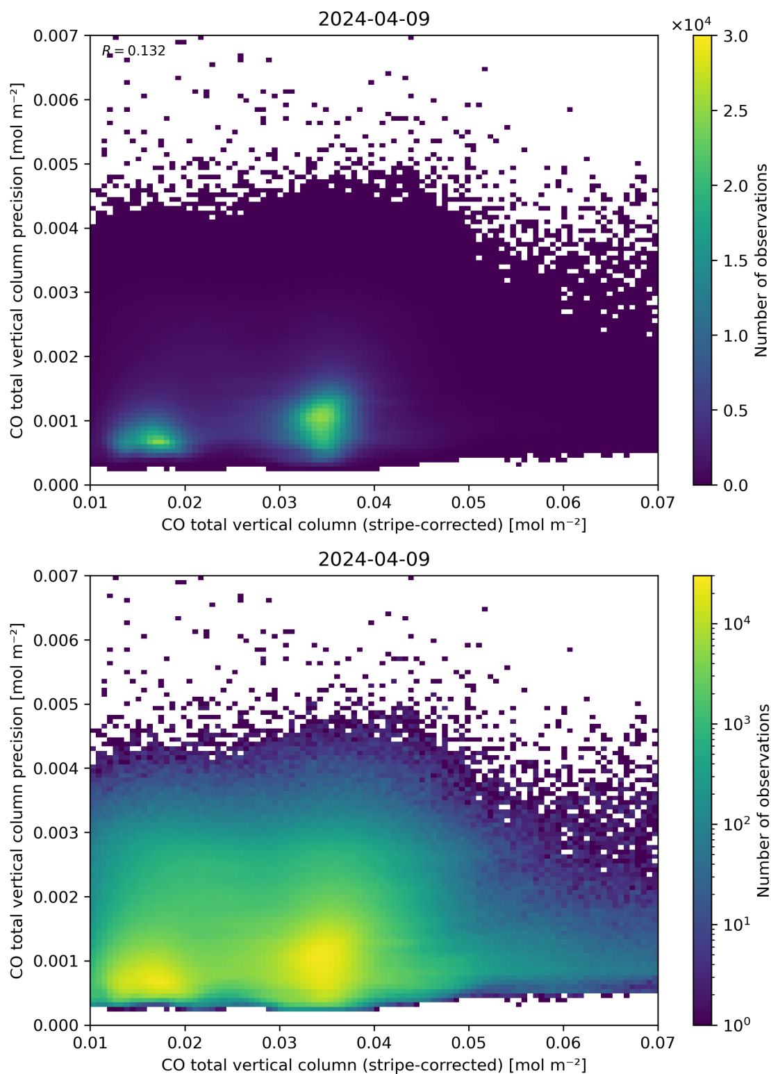
Figure 36: Scatter density plot of “CO total vertical column (stripe-corrected)” against “CO total vertical column precision” for 2024-04-08 to 2024-04-10.
