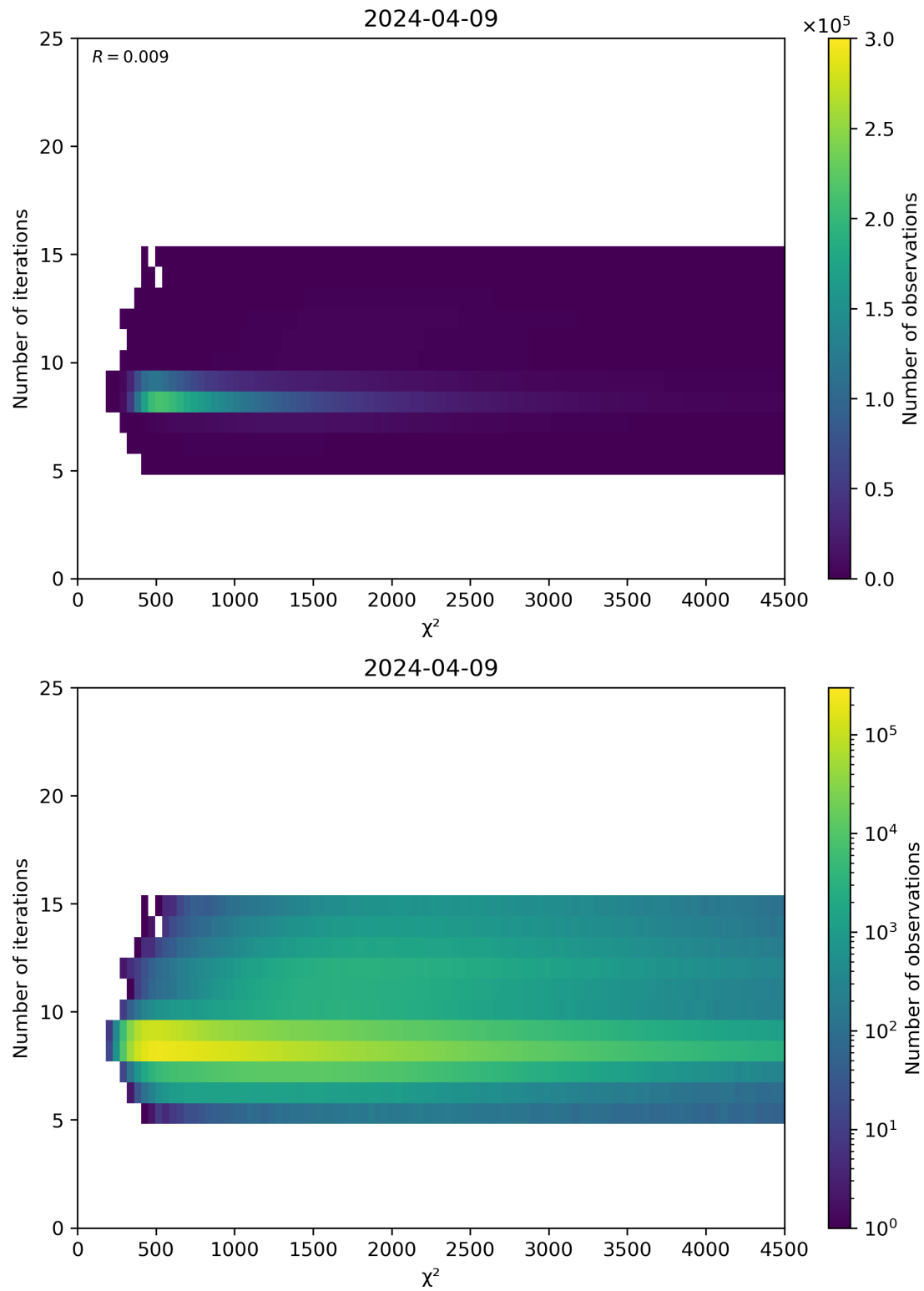
Figure 49: Scatter density plot of “ \chi^2 ” against “Number of iterations” for 2024-04-08 to 2024-04-10.
