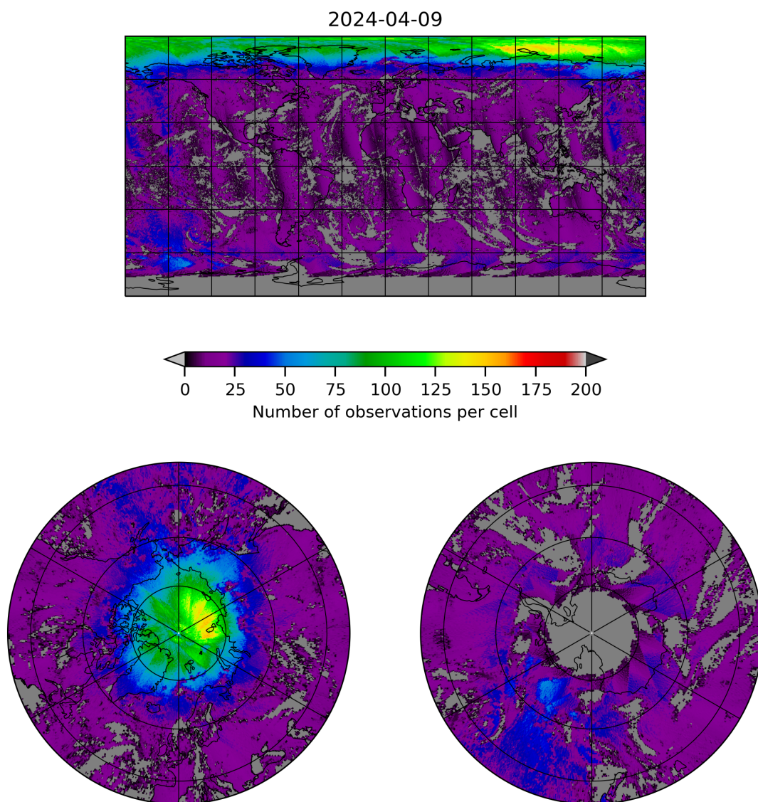
Figure 8: Map of the number of observations for 2024-04-08 to 2024-04-10
