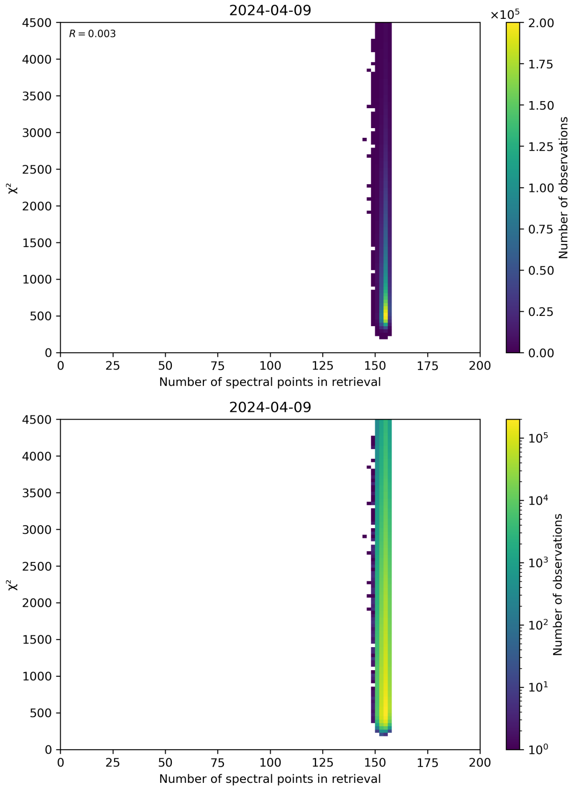
Figure 58: Scatter density plot of “Number of spectral points in retrieval” against “ \chi^2 ” for 2024-04-08 to 2024-04-10.
