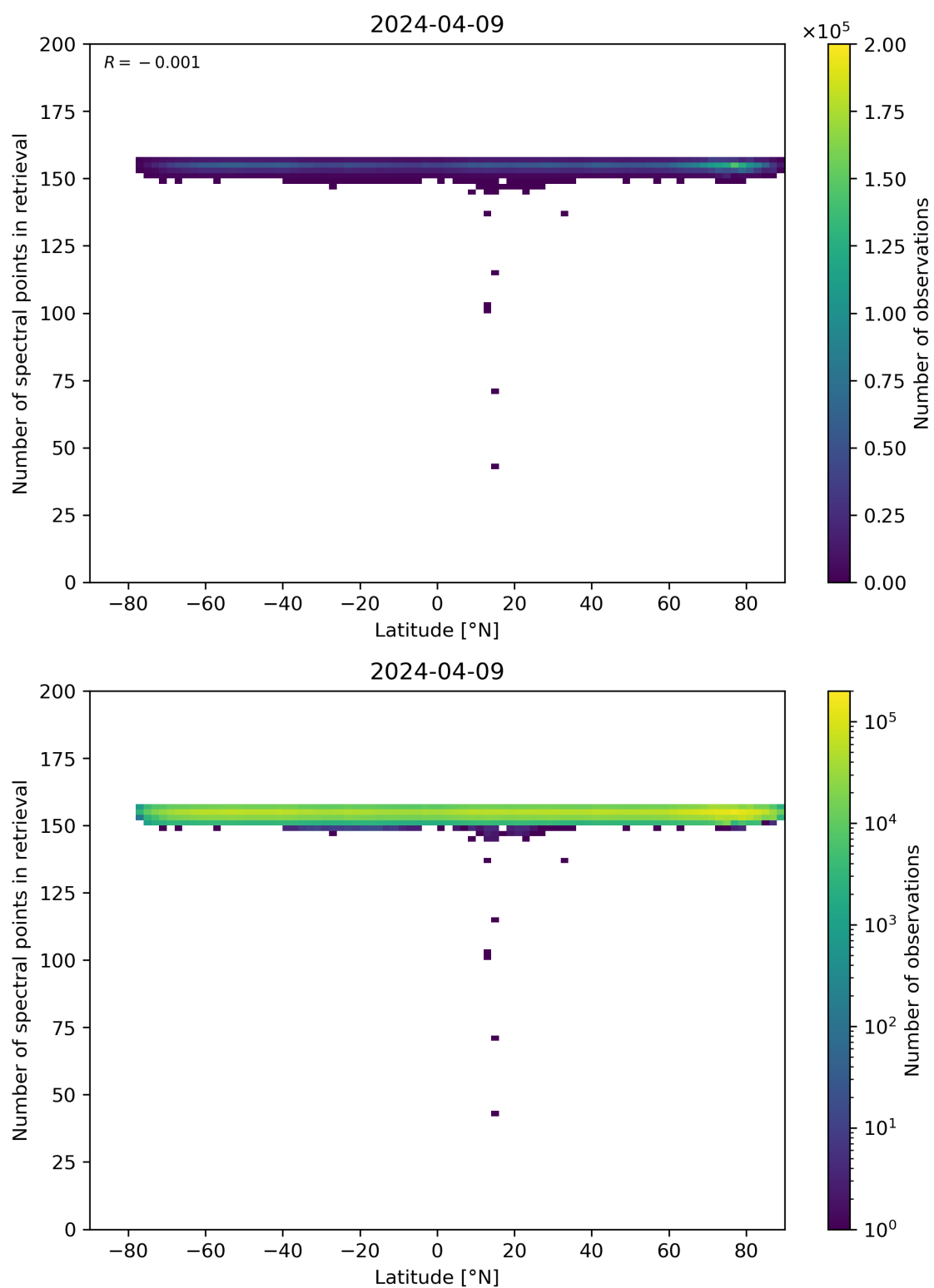
Figure 57: Scatter density plot of “Latitude” against “Number of spectral points in retrieval” for 2024-04-08 to 2024-04-10.
