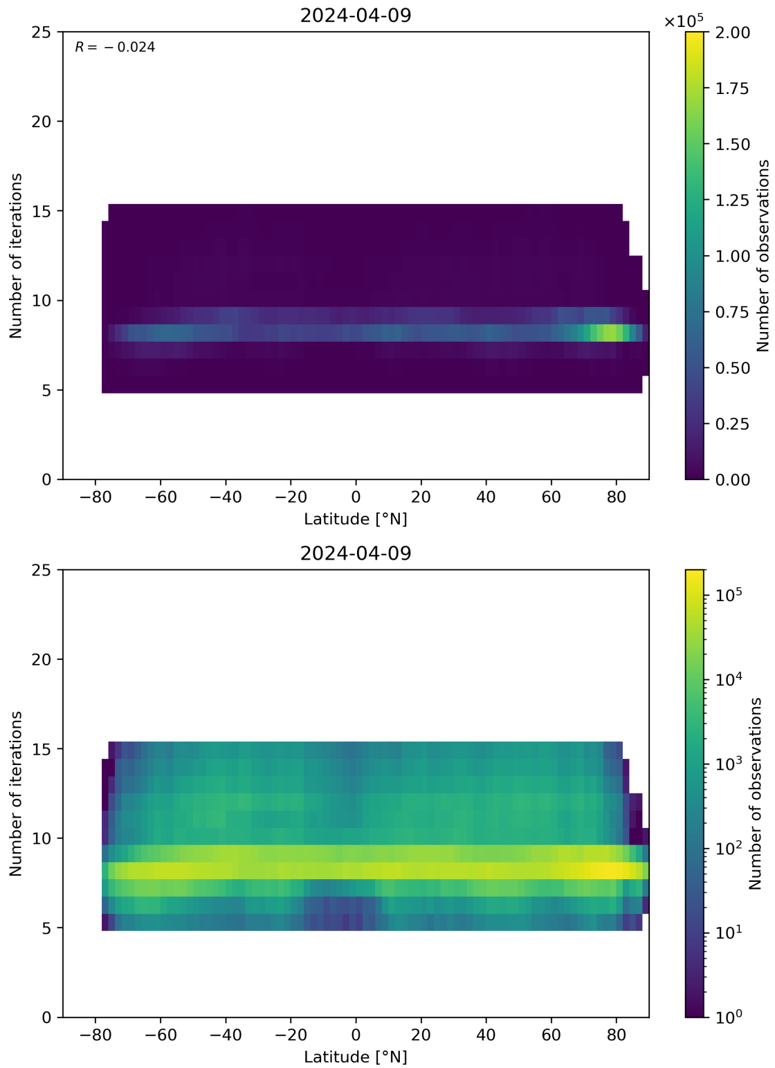
Figure 56: Scatter density plot of “Latitude” against “Number of iterations” for 2024-04-08 to 2024-04-10.
