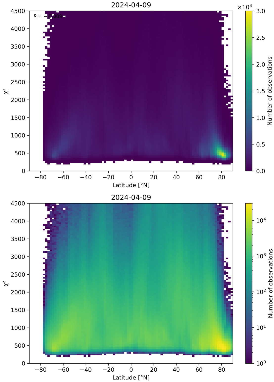
Figure 54: Scatter density plot of “Latitude” against “ \chi^2 ” for 2024-04-08 to 2024-04-10.
