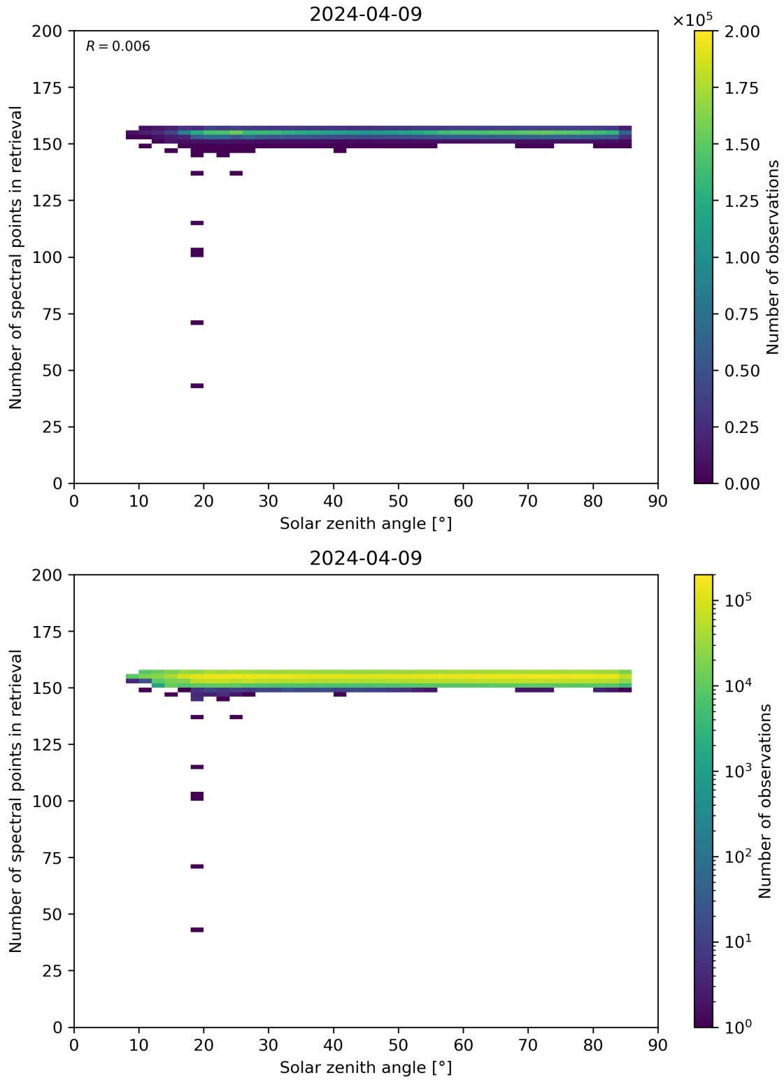
Figure 68: Scatter density plot of “Solar zenith angle” against “Number of spectral points in retrieval” for 2024-04-08 to 2024-04-10.
