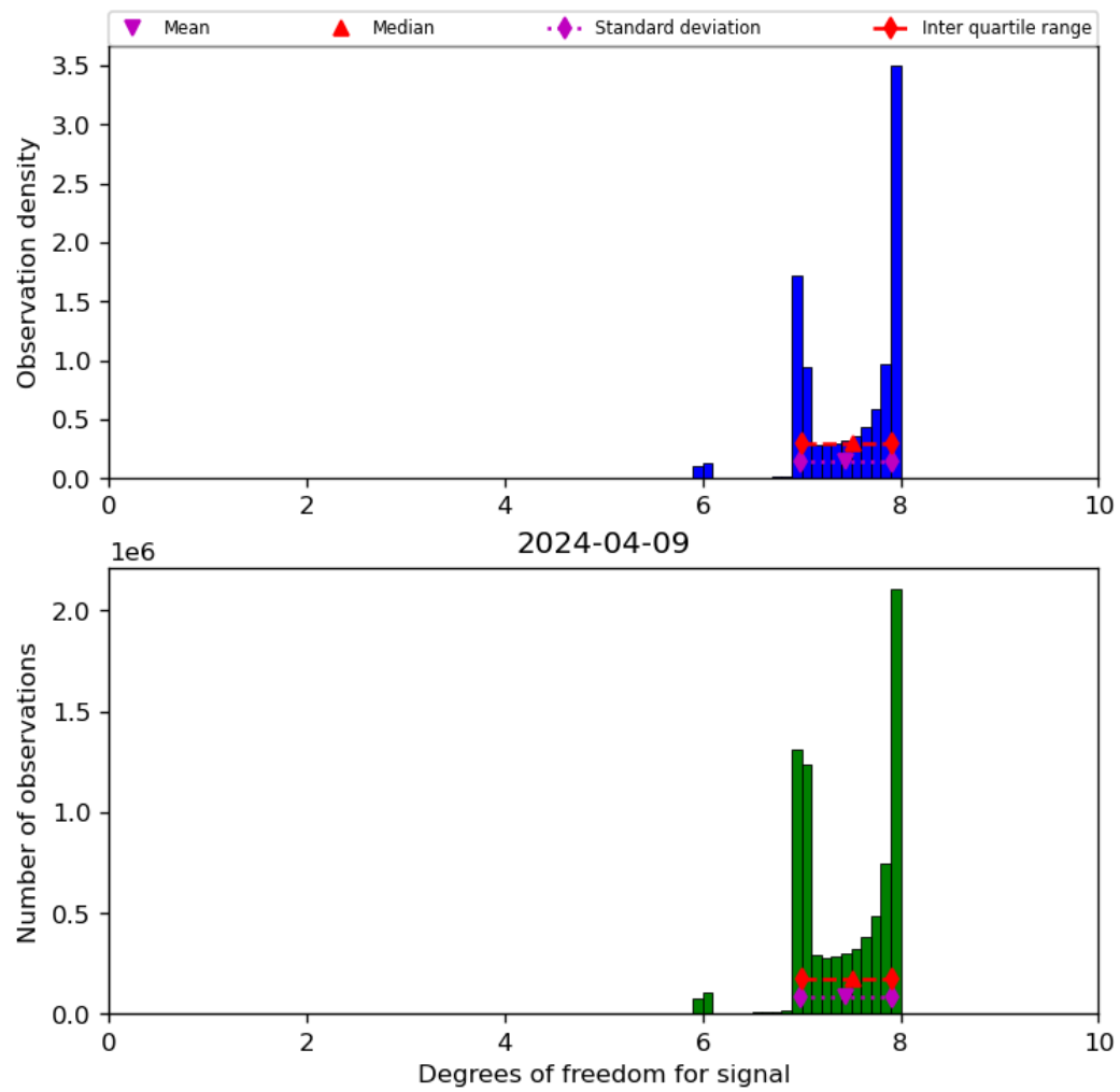
Figure 23: Histogram of “Degrees of freedom for signal” for 2024-04-08 to 2024-04-10
