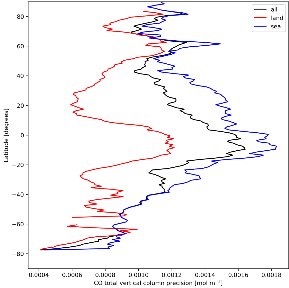
Figure 12: Zonal average of "CO total vertical column precision" for 2024-04-08 to 2024-04-10.
