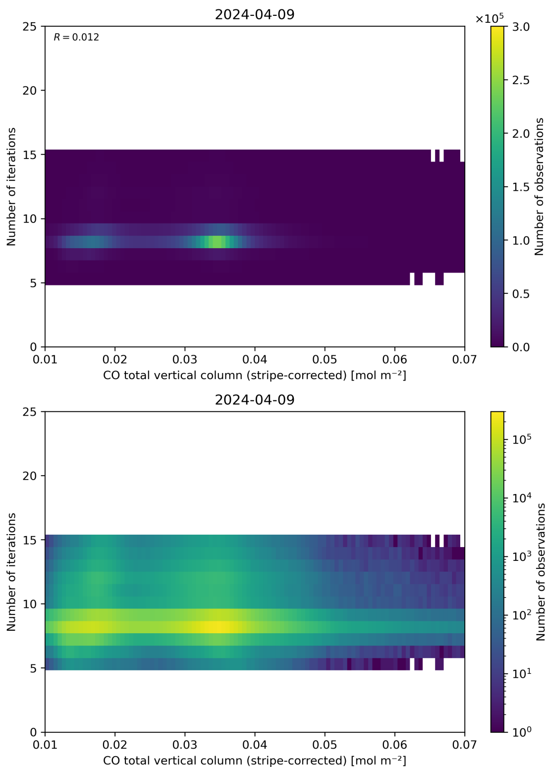
Figure 39: Scatter density plot of “CO total vertical column (stripe-corrected)” against “Number of iterations” for 2024-04-08 to 2024-04-10.
