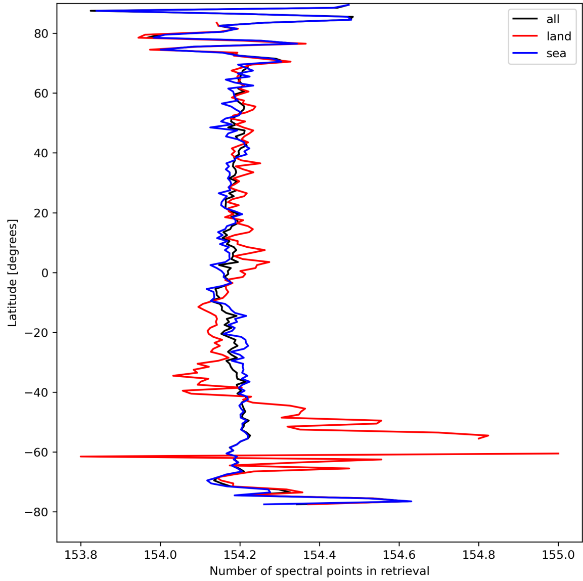
Figure 13: Zonal average of “Number of spectral points in retrieval” for 2024-04-08 to 2024-04-10.
