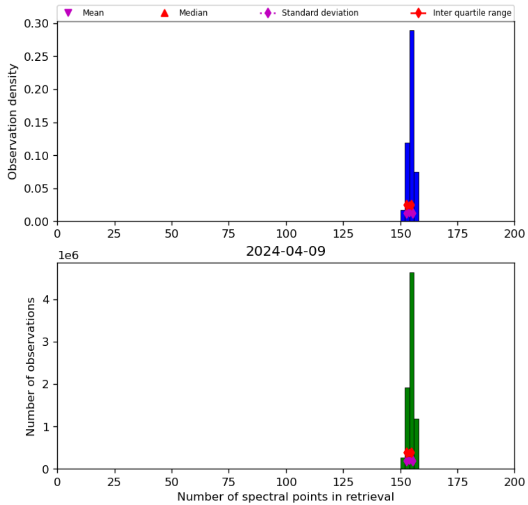
Figure 21: Histogram of “Number of spectral points in retrieval” for 2024-04-08 to 2024-04-10
