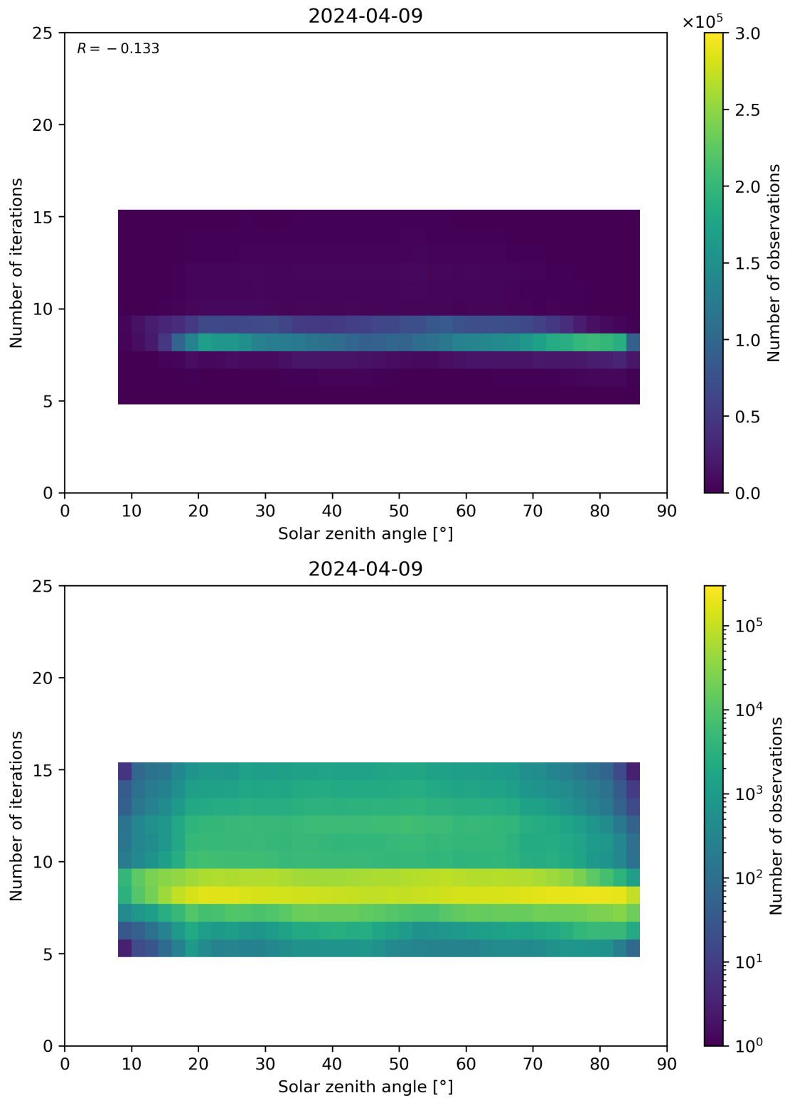
Figure 67: Scatter density plot of “Solar zenith angle” against “Number of iterations” for 2024-04-08 to 2024-04-10.
