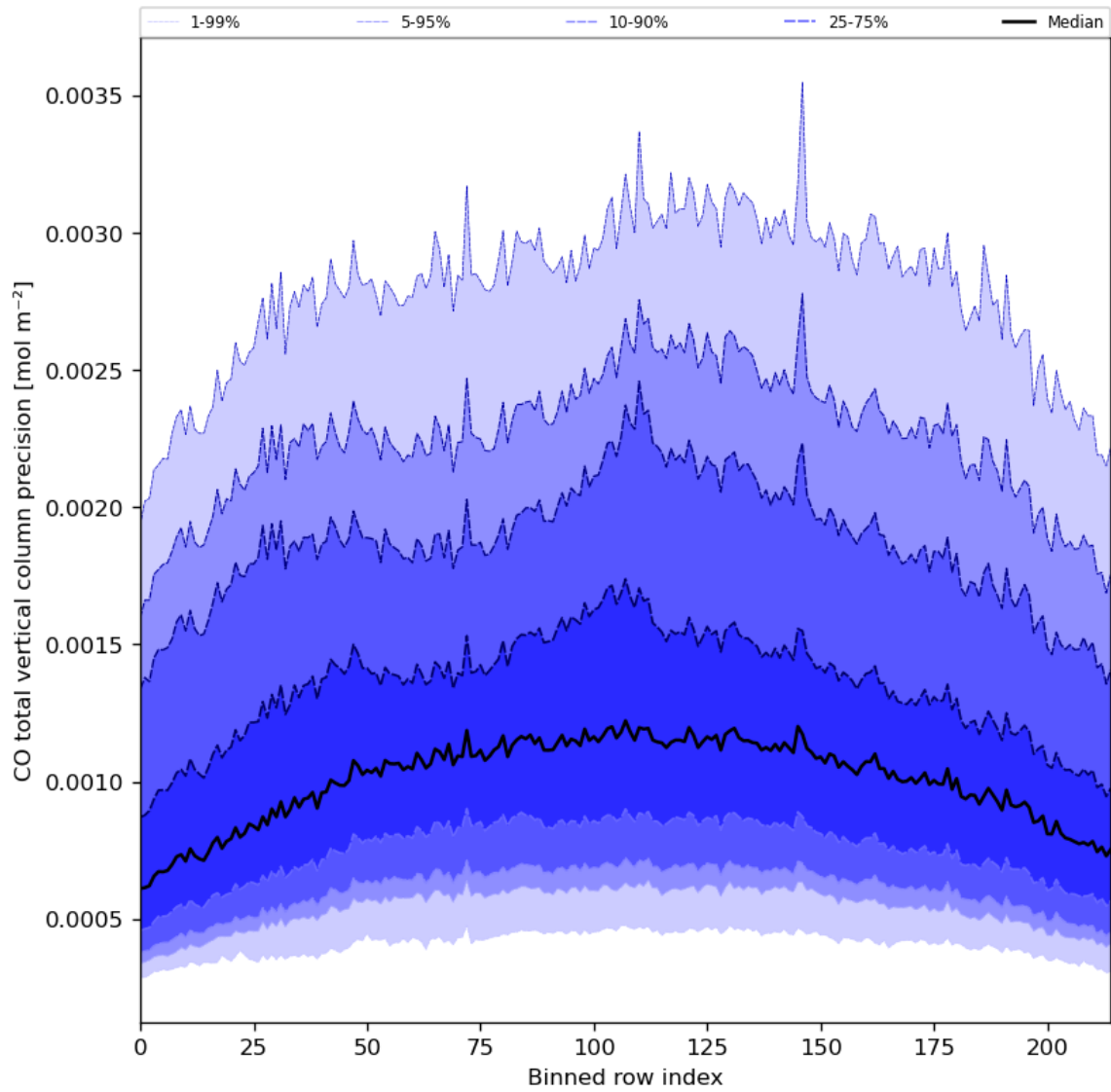
Figure 28: Along track statistics of “CO total vertical column precision” for 2024-04-08 to 2024-04-10
