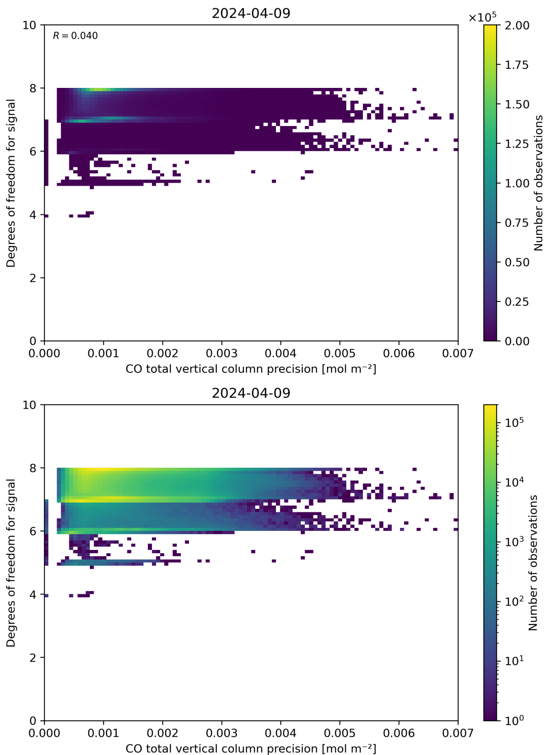
Figure 45: Scatter density plot of “CO total vertical column precision” against “Degrees of freedom for signal” for 2024-04-08 to 2024-04-10.
