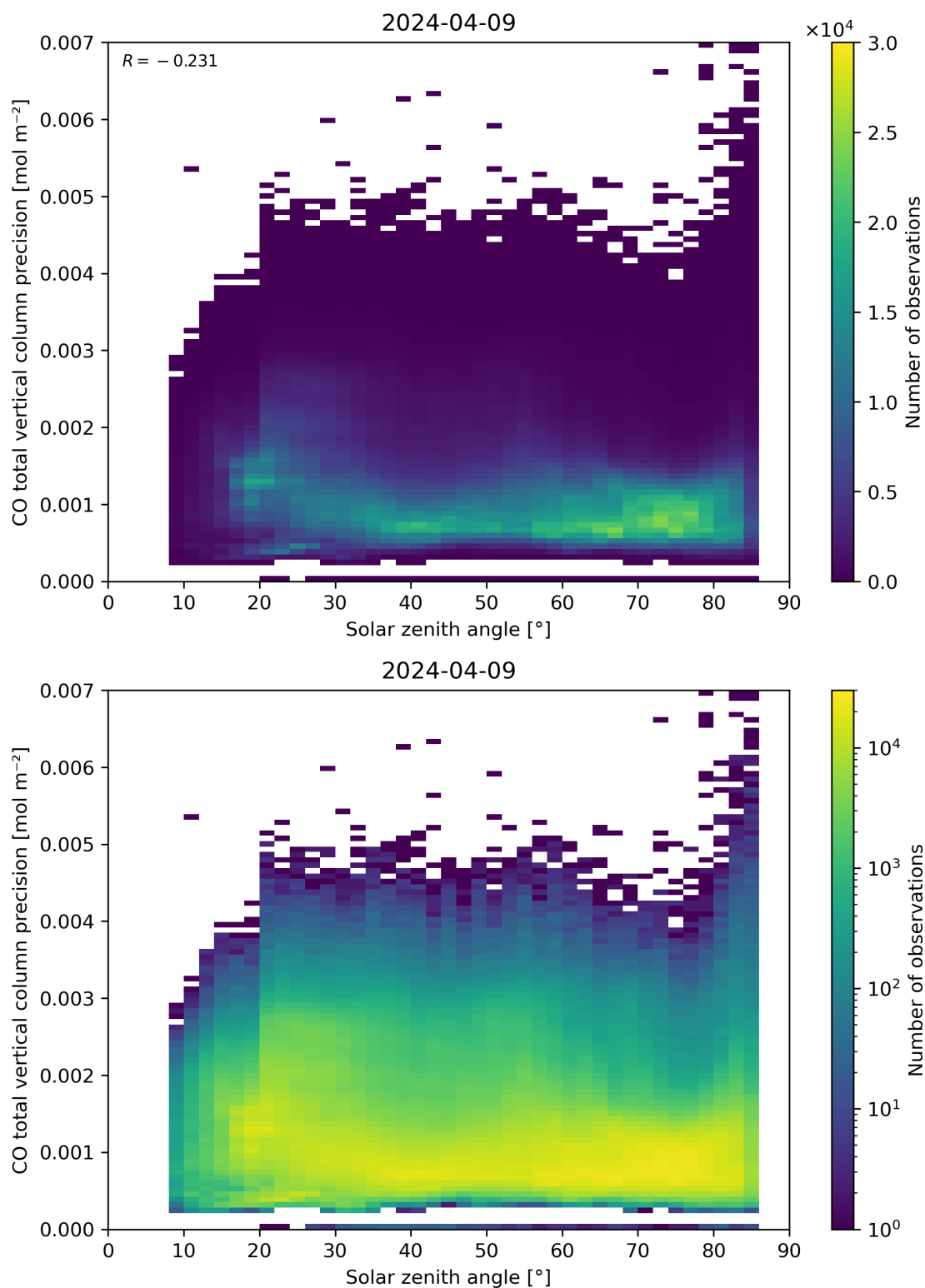
Figure 63: Scatter density plot of “Solar zenith angle” against “CO total vertical column precision” for 2024-04-08 to 2024-04-10.
