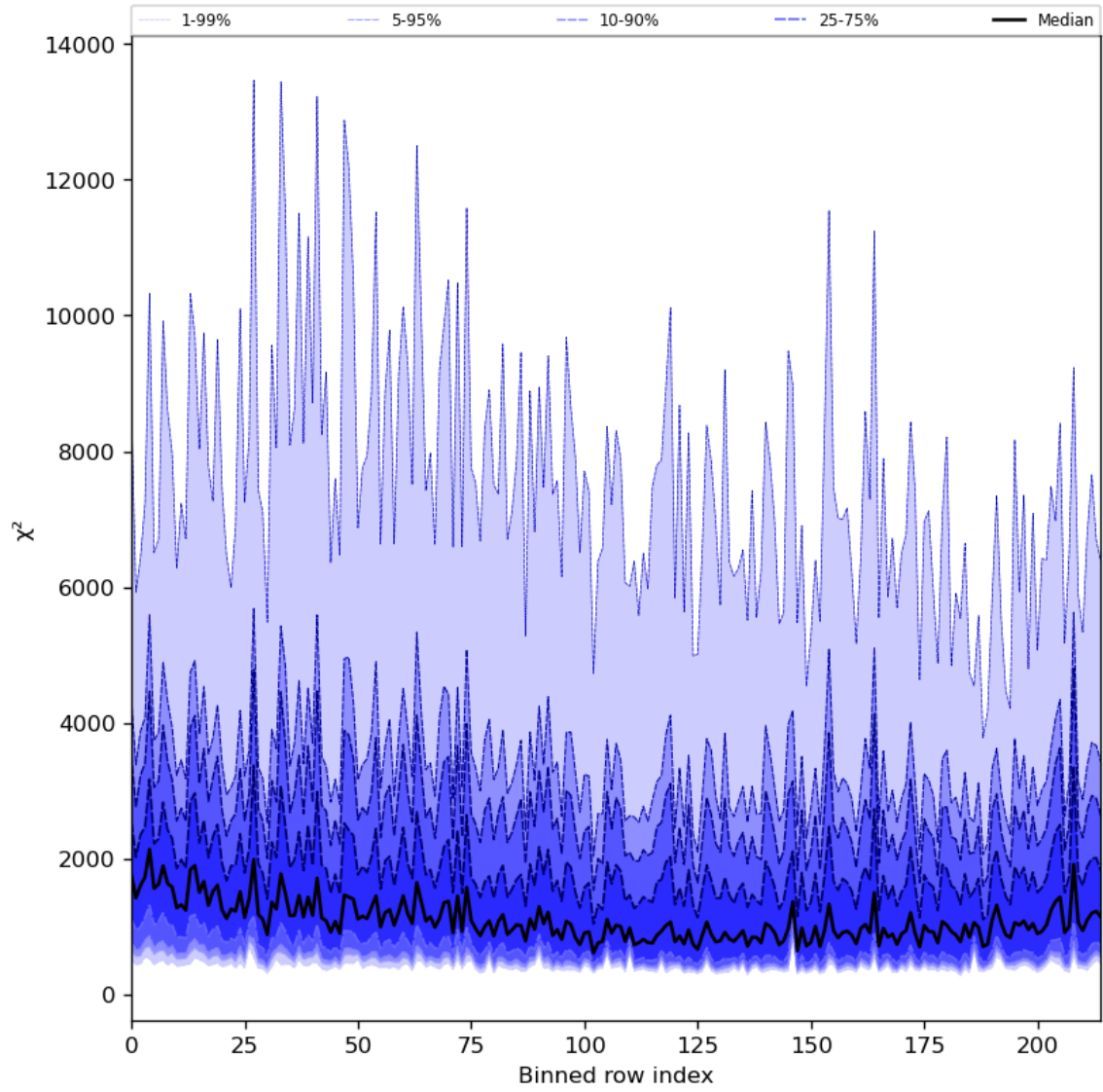
Figure 30: Along track statistics of “ \chi^2 ” for 2024-04-08 to 2024-04-10
