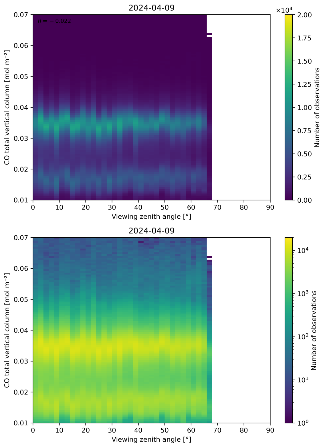
Figure 69: Scatter density plot of “Viewing zenith angle” against “CO total vertical column” for 2024-04-08 to 2024-04-10.
