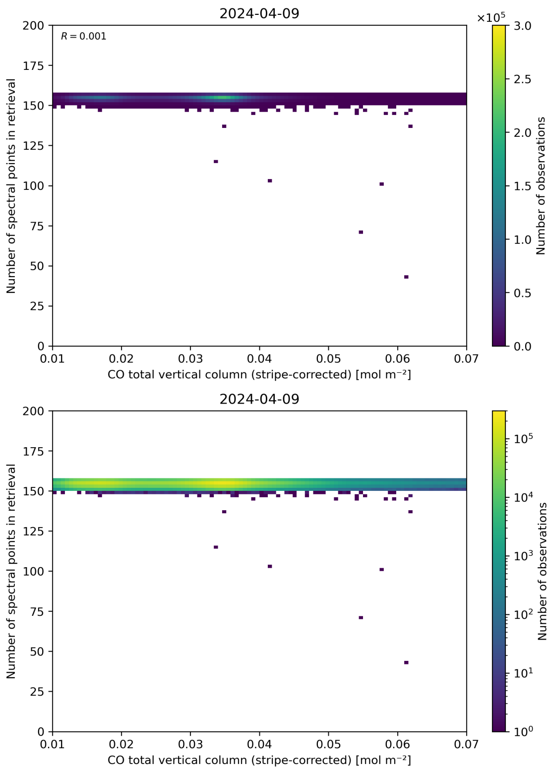
Figure 40: Scatter density plot of “CO total vertical column (stripe-corrected)” against “Number of spectral points in retrieval” for 2024-04-08 to 2024-04-10.
