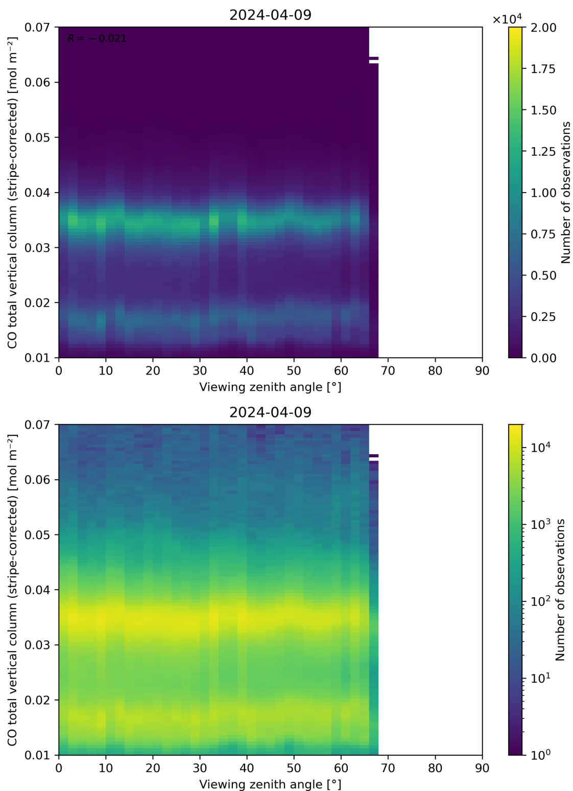
Figure 70: Scatter density plot of “Viewing zenith angle” against “CO total vertical column (stripe-corrected)” for 2024-04-08 to 2024-04-10.
