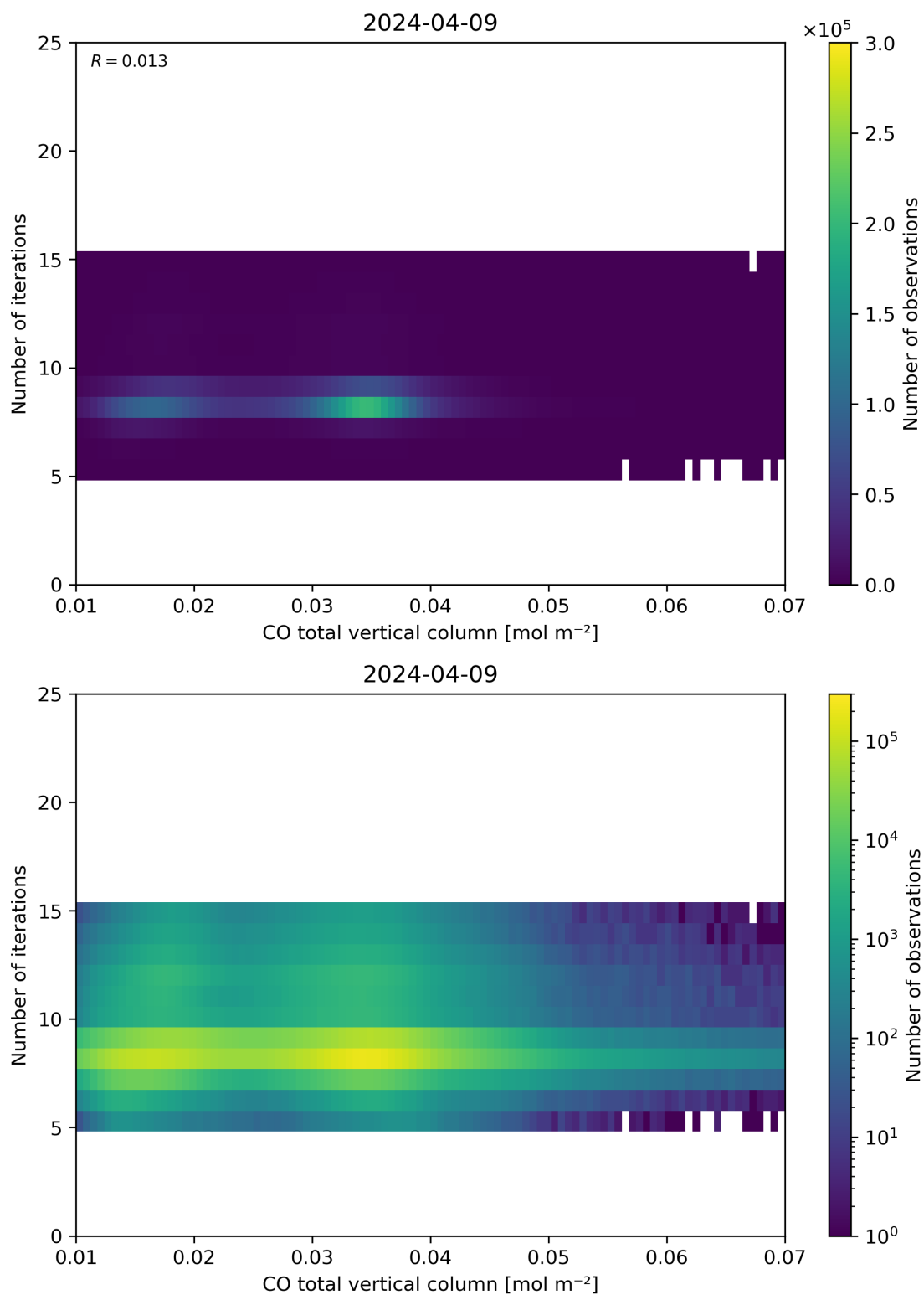
Figure 42: Scatter density plot of “CO total vertical column” against “Number of iterations” for 2024-04-08 to 2024-04-10.
