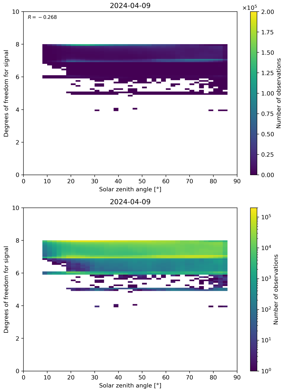
Figure 65: Scatter density plot of “Solar zenith angle” against “Degrees of freedom for signal” for 2024-04-08 to 2024-04-10.
