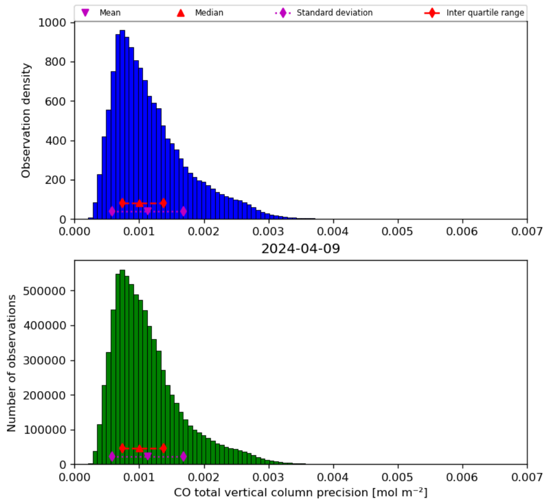
Figure 20: Histogram of “CO total vertical column precision” for 2024-04-08 to 2024-04-10
