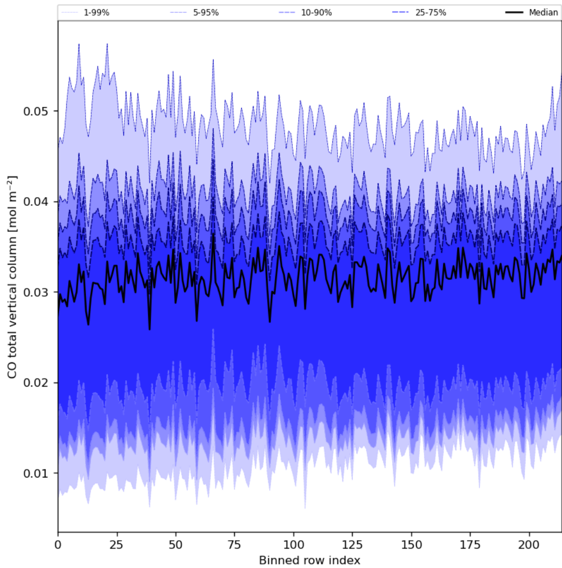
Figure 26: Along track statistics of "CO total vertical column" for 2024-04-08 to 2024-04-10
