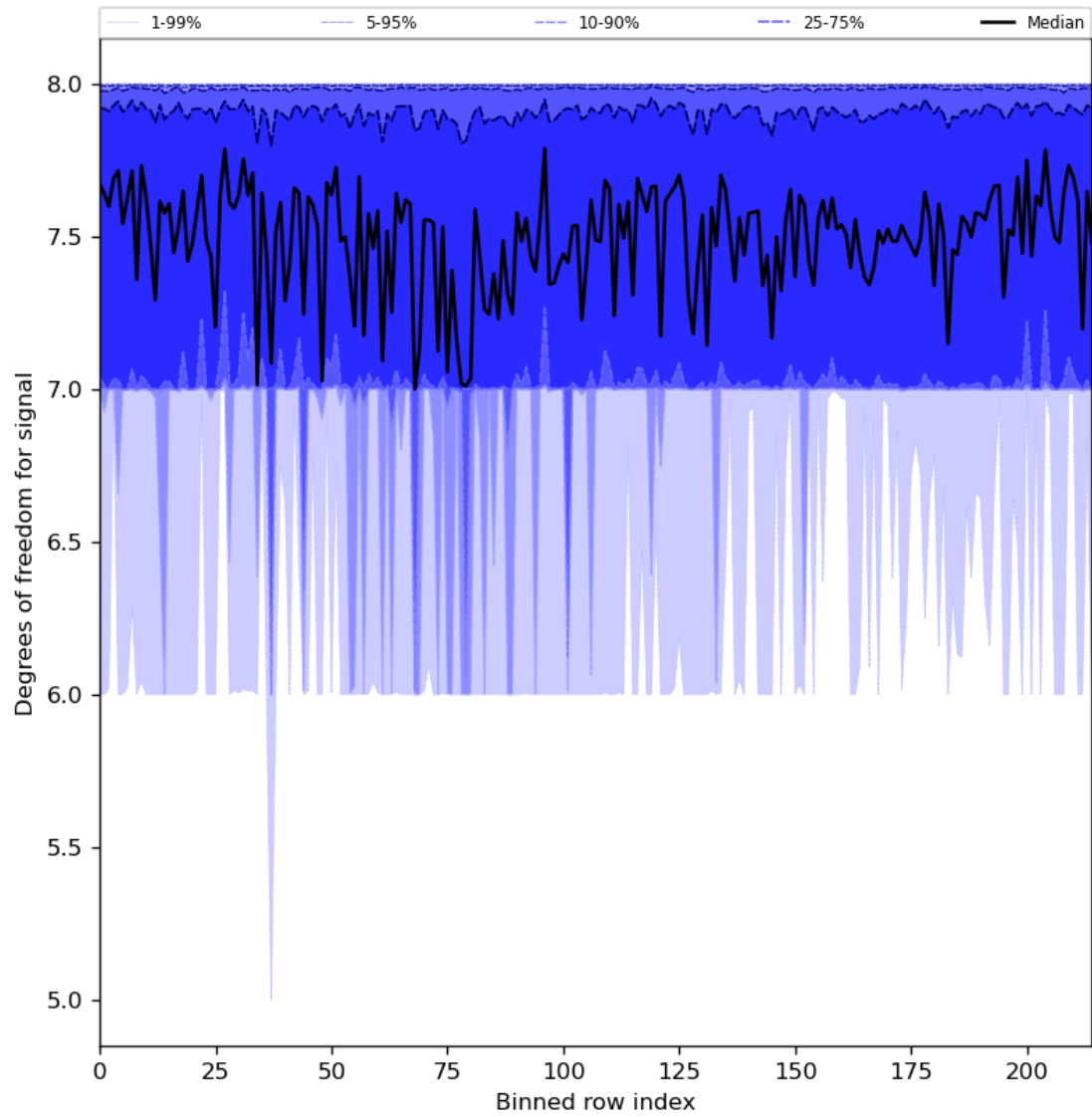
Figure 31: Along track statistics of “Degrees of freedom for signal” for 2024-04-08 to 2024-04-10
