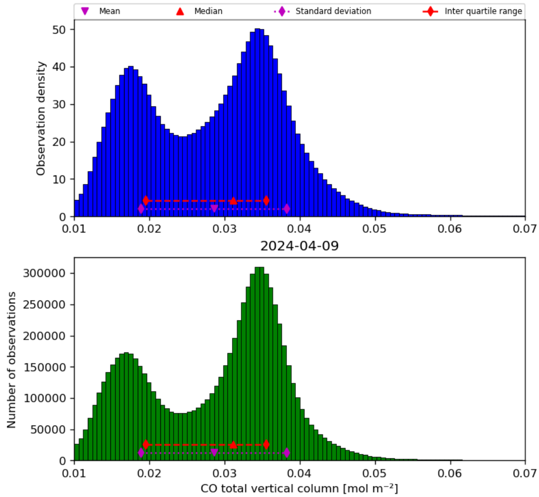
Figure 18: Histogram of “CO total vertical column” for 2024-04-08 to 2024-04-10
