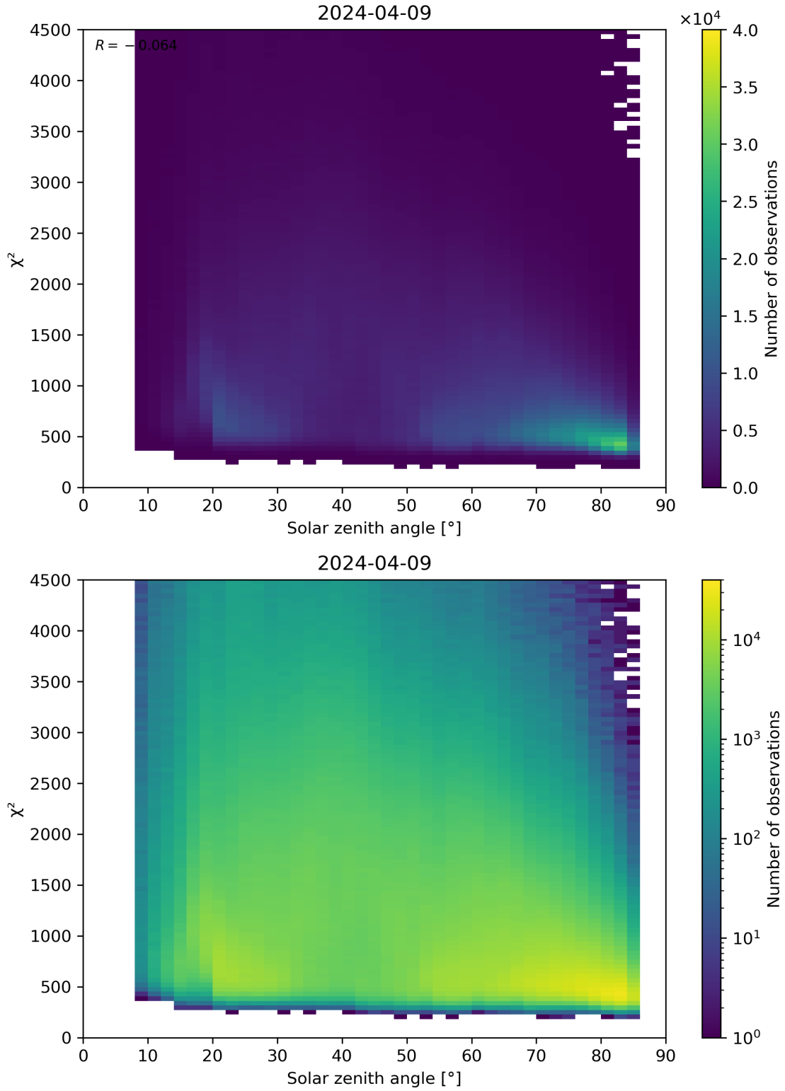
Figure 64: Scatter density plot of “Solar zenith angle” against “ \chi^2 ” for 2024-04-08 to 2024-04-10.
