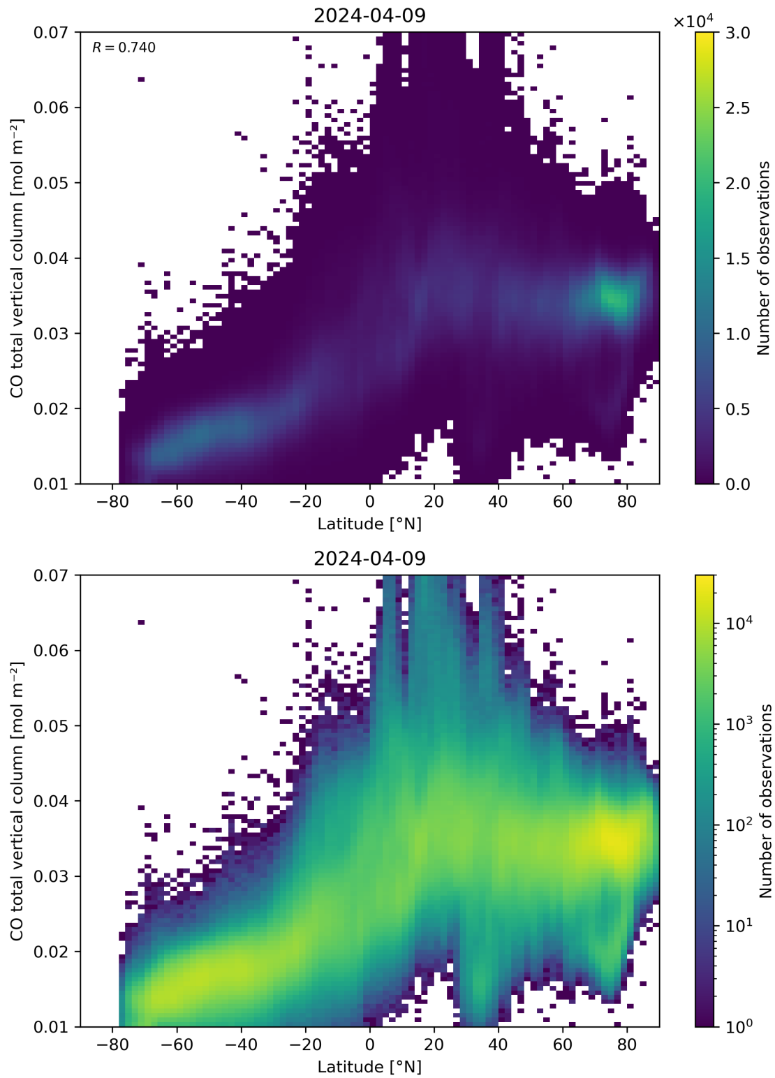
Figure 51: Scatter density plot of “Latitude” against “CO total vertical column” for 2024-04-08 to 2024-04-10.
