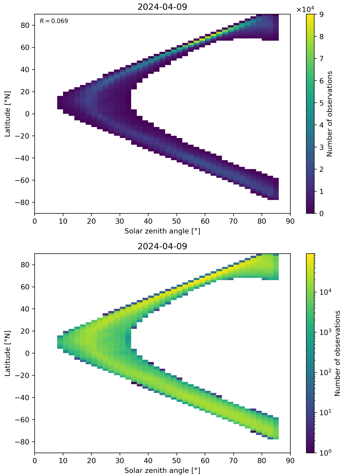
Figure 66: Scatter density plot of “Solar zenith angle” against “Latitude” for 2024-04-08 to 2024-04-10.
