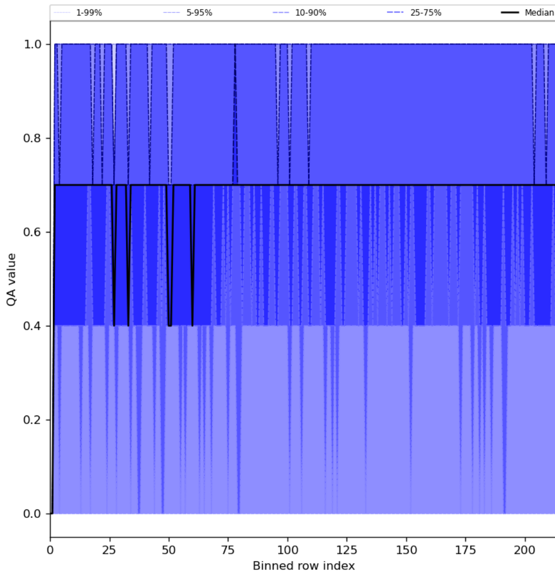
Figure 25: Along track statistics of “QA value” for 2024-04-08 to 2024-04-10
