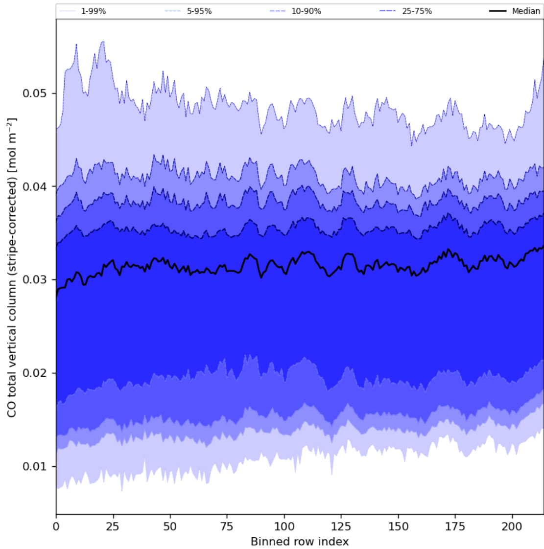
Figure 27: Along track statistics of “CO total vertical column (stripe-corrected)” for 2024-04-08 to 2024-04-10
