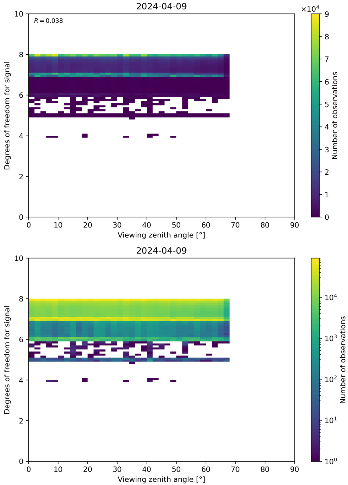
Figure 73: Scatter density plot of “Viewing zenith angle” against “Degrees of freedom for signal” for 2024-04-08 to 2024-04-10.
