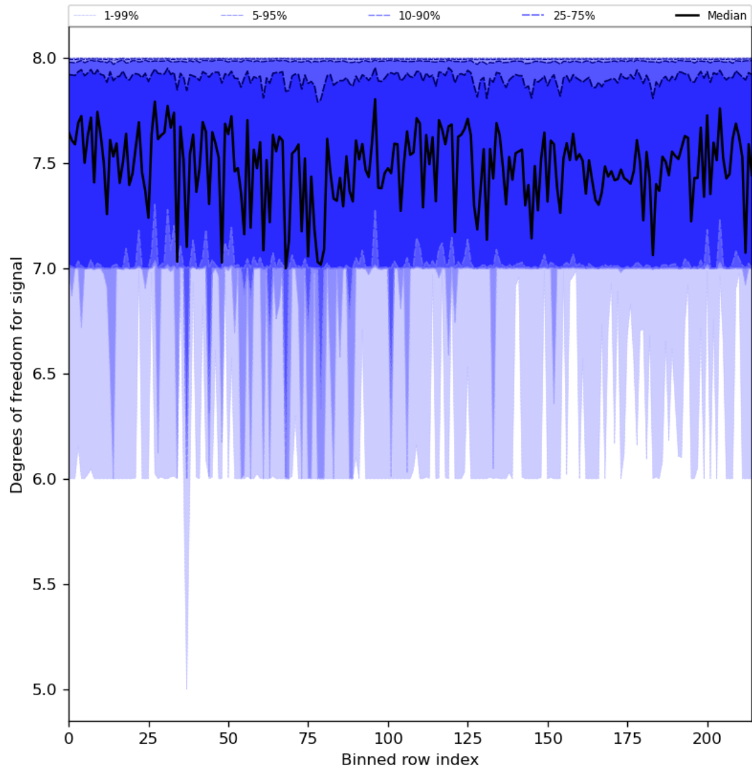
Figure 31: Along track statistics of “Degrees of freedom for signal” for 2024-04-10 to 2024-04-11
