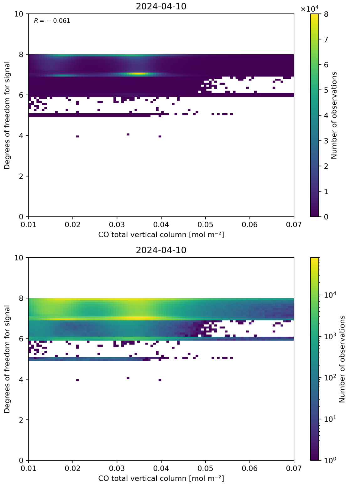
Figure 41: Scatter density plot of “CO total vertical column” against “Degrees of freedom for signal” for 2024-04-10 to 2024-04-11.
