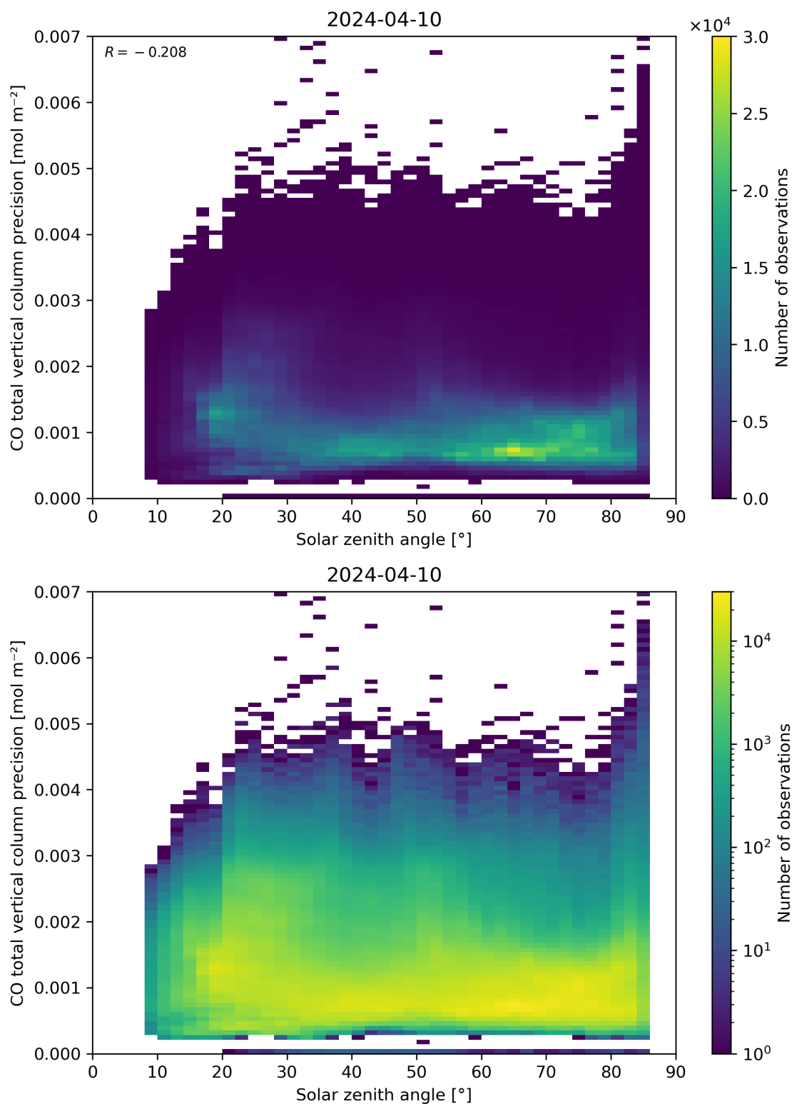
Figure 63: Scatter density plot of “Solar zenith angle” against “CO total vertical column precision” for 2024-04-10 to 2024-04-11.
