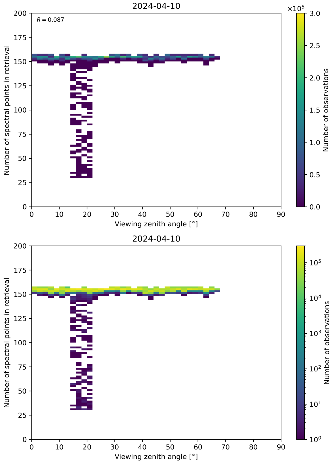
Figure 76: Scatter density plot of “Viewing zenith angle” against “Number of spectral points in retrieval” for 2024-04-10 to 2024-04-11.
