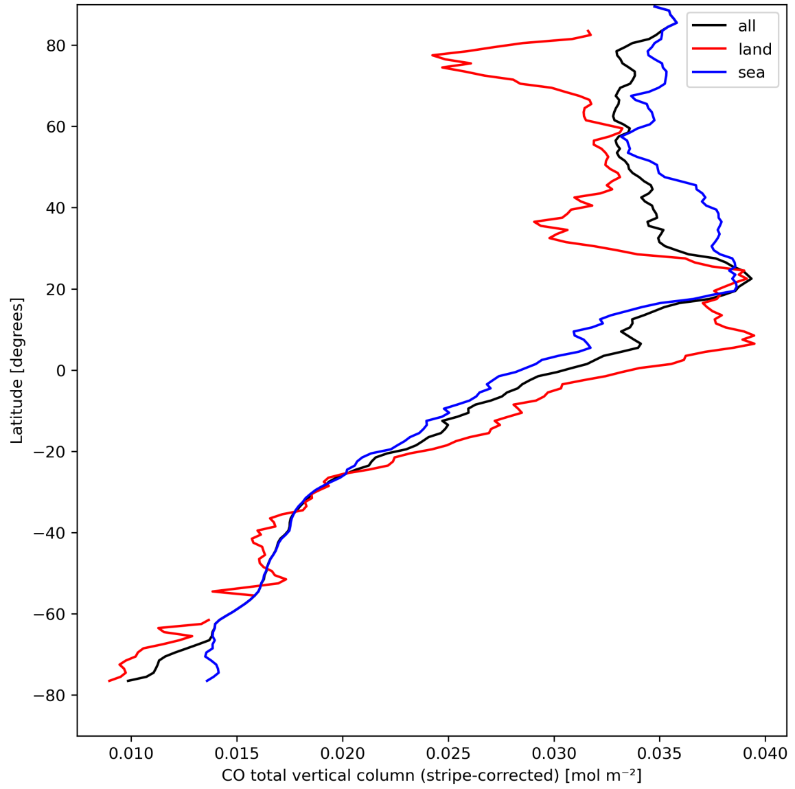
Figure 11: Zonal average of “CO total vertical column (stripe-corrected)” for 2024-04-10 to 2024-04-11.
