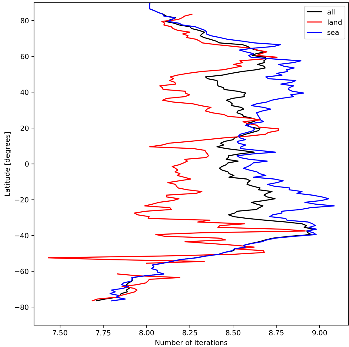
Figure 16: Zonal average of “Number of iterations” for 2024-04-10 to 2024-04-11.
