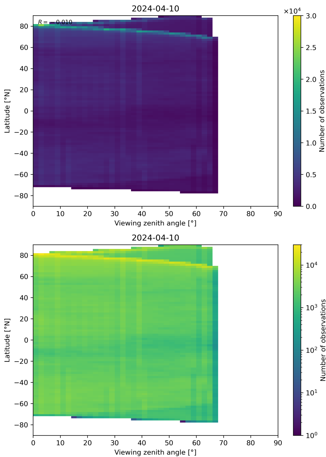
Figure 74: Scatter density plot of “Viewing zenith angle” against “Latitude” for 2024-04-10 to 2024-04-11.
