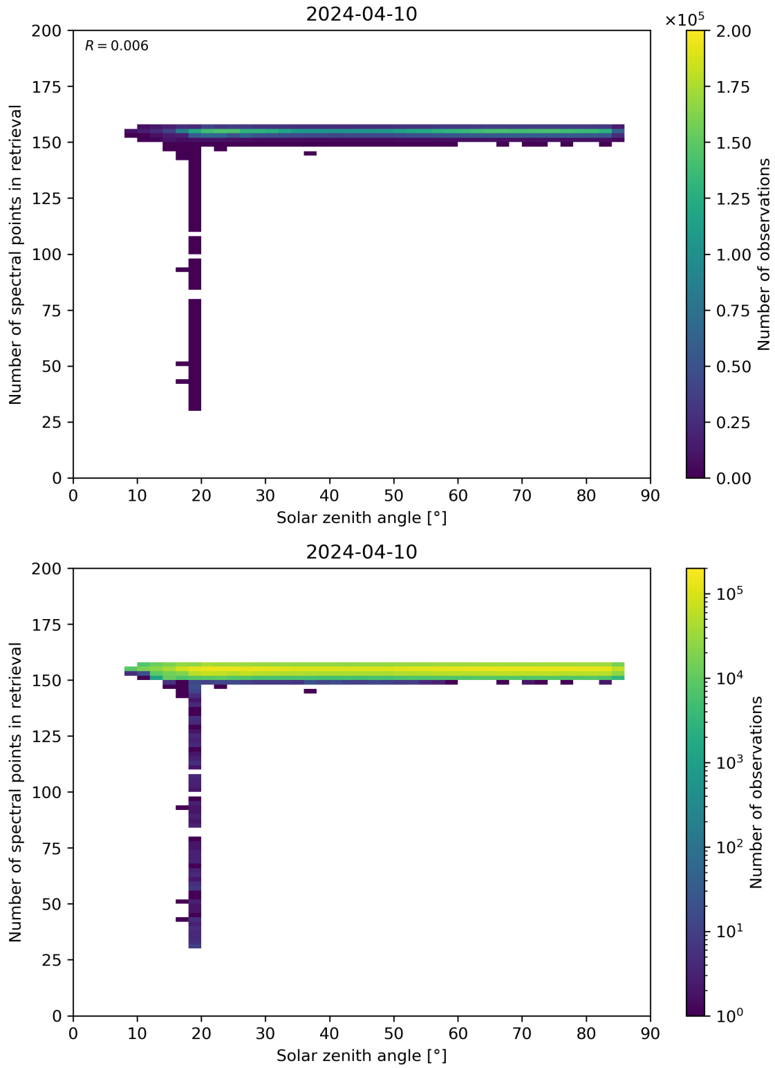
Figure 68: Scatter density plot of “Solar zenith angle” against “Number of spectral points in retrieval” for 2024-04-10 to 2024-04-11.
