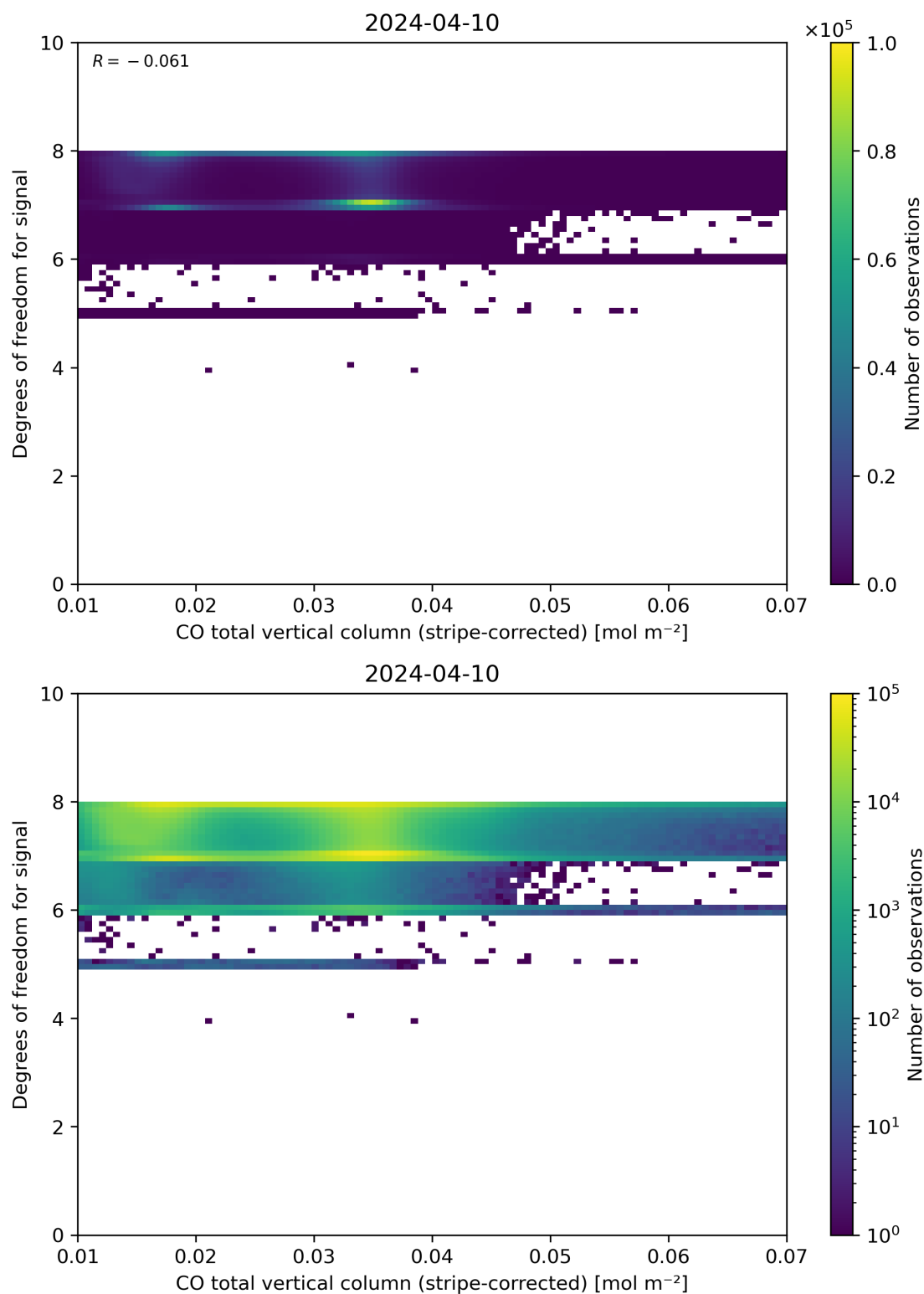
Figure 38: Scatter density plot of “CO total vertical column (stripe-corrected)” against “Degrees of freedom for signal” for 2024-04-10 to 2024-04-11.
