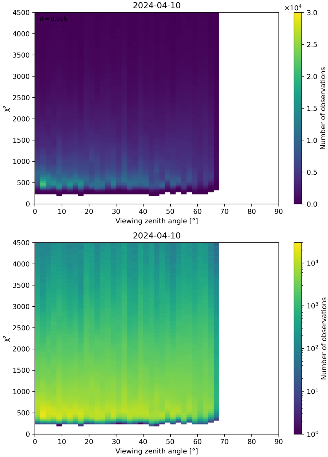
Figure 72: Scatter density plot of “Viewing zenith angle” against “ \chi^2 ” for 2024-04-10 to 2024-04-11.
