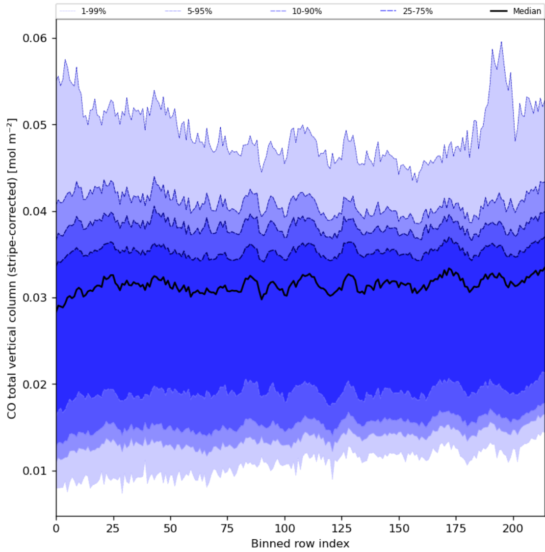
Figure 27: Along track statistics of “CO total vertical column (stripe-corrected)” for 2024-04-10 to 2024-04-11
