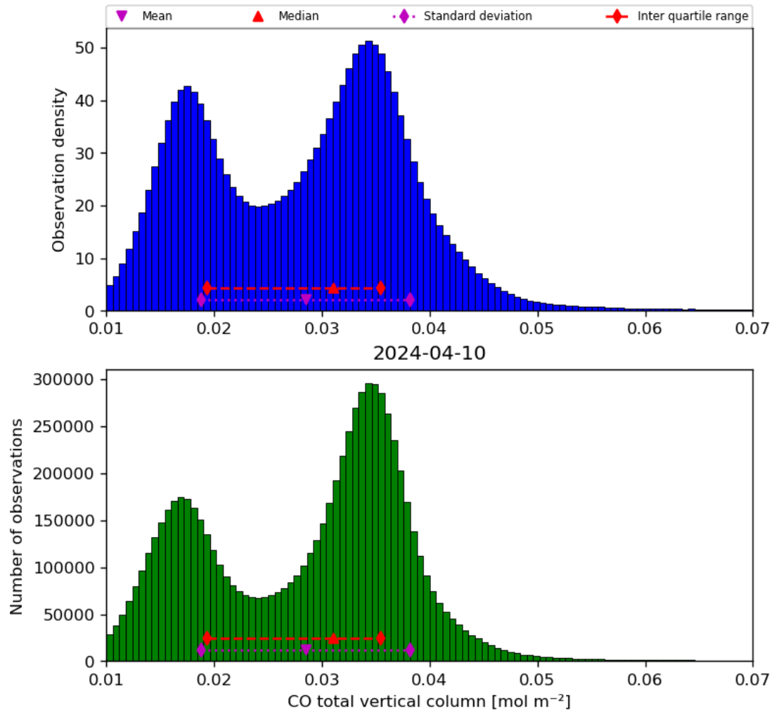
Figure 18: Histogram of “CO total vertical column” for 2024-04-10 to 2024-04-11
