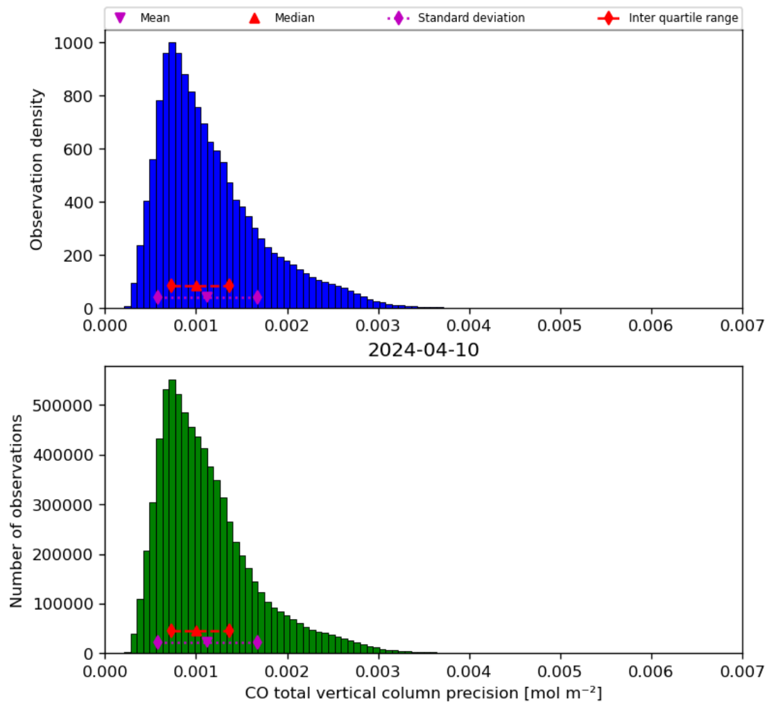
Figure 20: Histogram of “CO total vertical column precision” for 2024-04-10 to 2024-04-11
