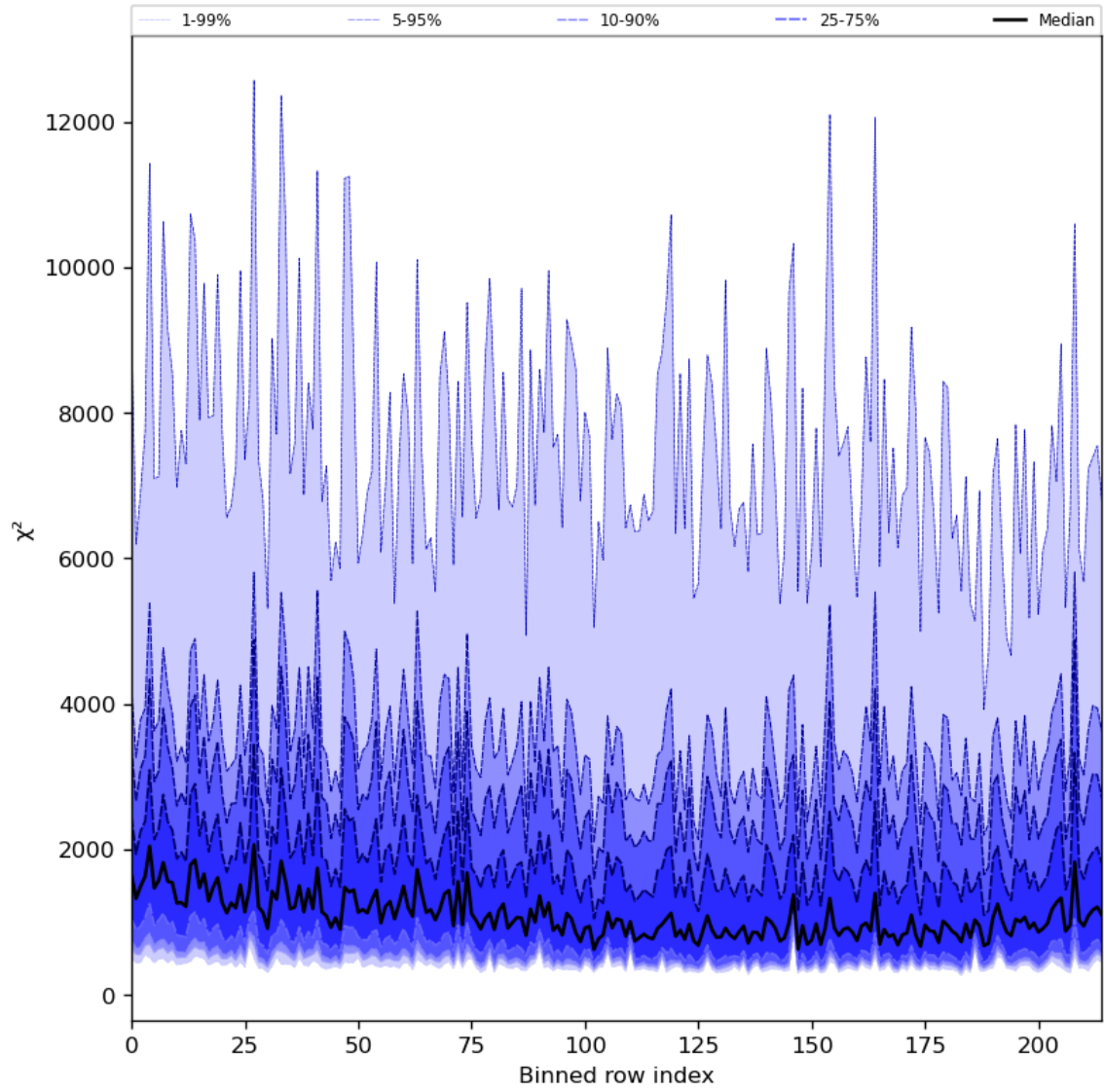
Figure 30: Along track statistics of “ \chi^2 ” for 2024-04-10 to 2024-04-11
