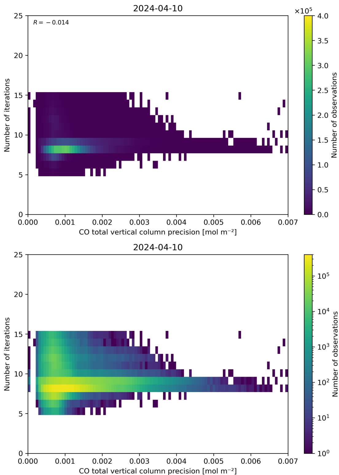
Figure 46: Scatter density plot of “CO total vertical column precision” against “Number of iterations” for 2024-04-10 to 2024-04-11.
