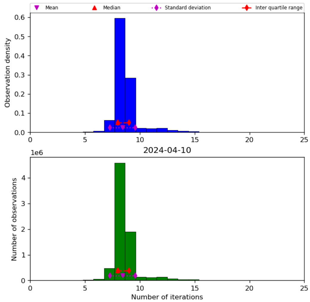
Figure 24: Histogram of “Number of iterations” for 2024-04-10 to 2024-04-11
