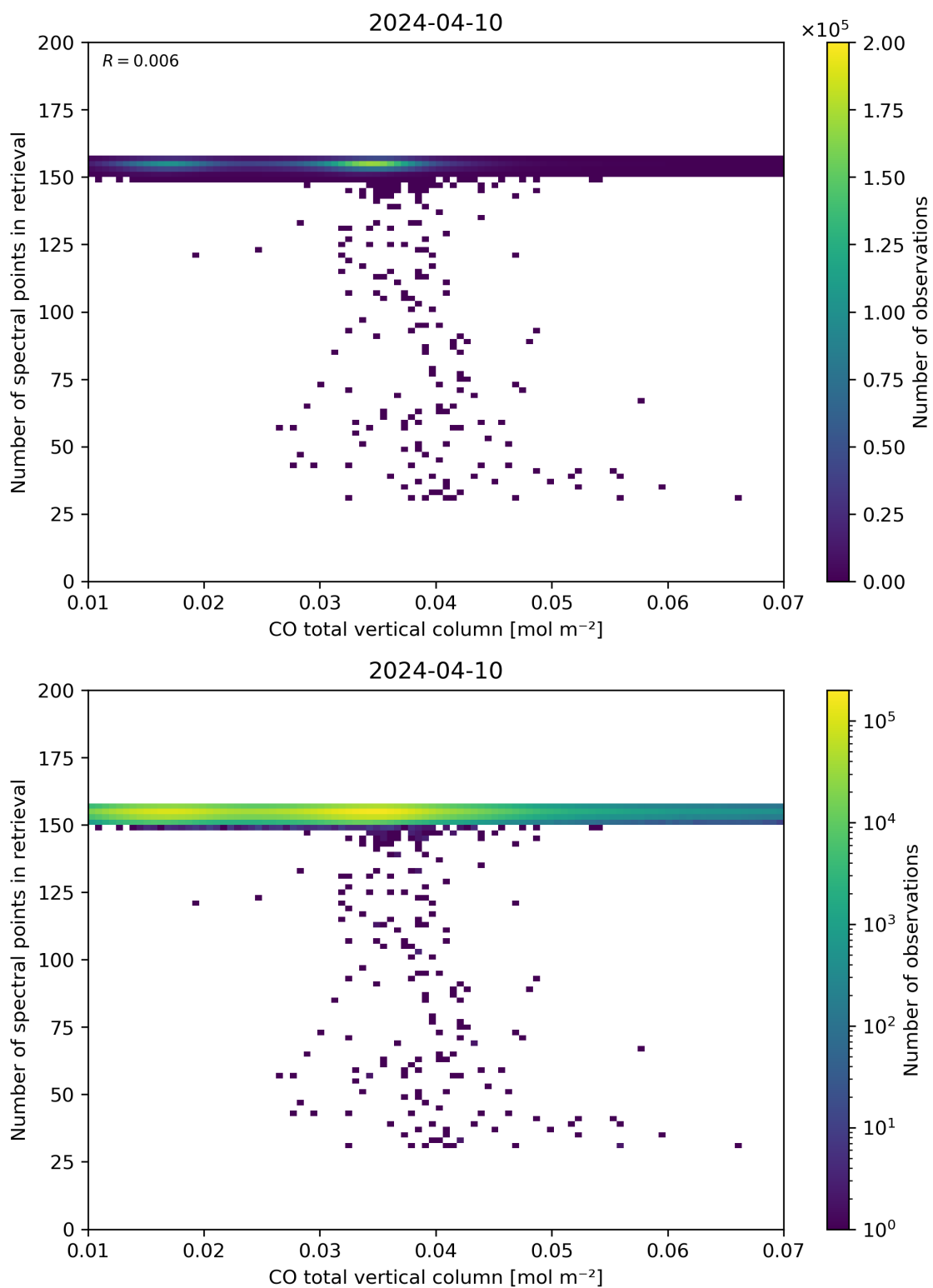
Figure 43: Scatter density plot of “CO total vertical column” against “Number of spectral points in retrieval” for 2024-04-10 to 2024-04-11.
