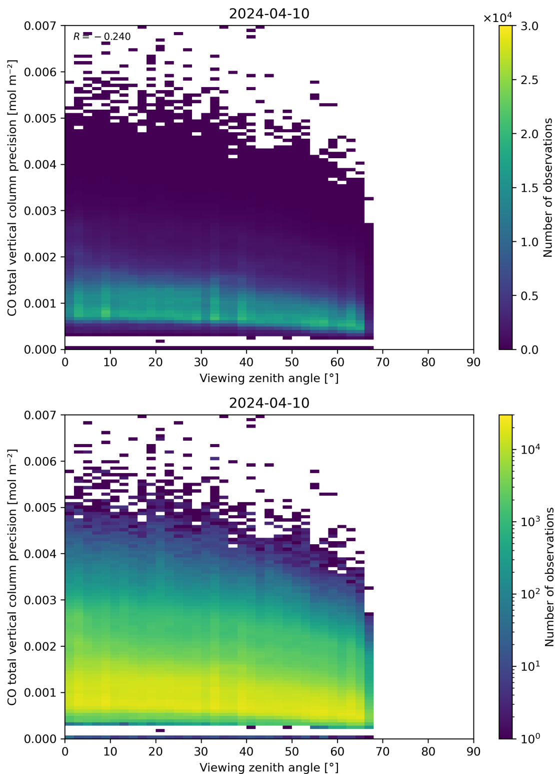
Figure 71: Scatter density plot of “Viewing zenith angle” against “CO total vertical column precision” for 2024-04-10 to 2024-04-11.
