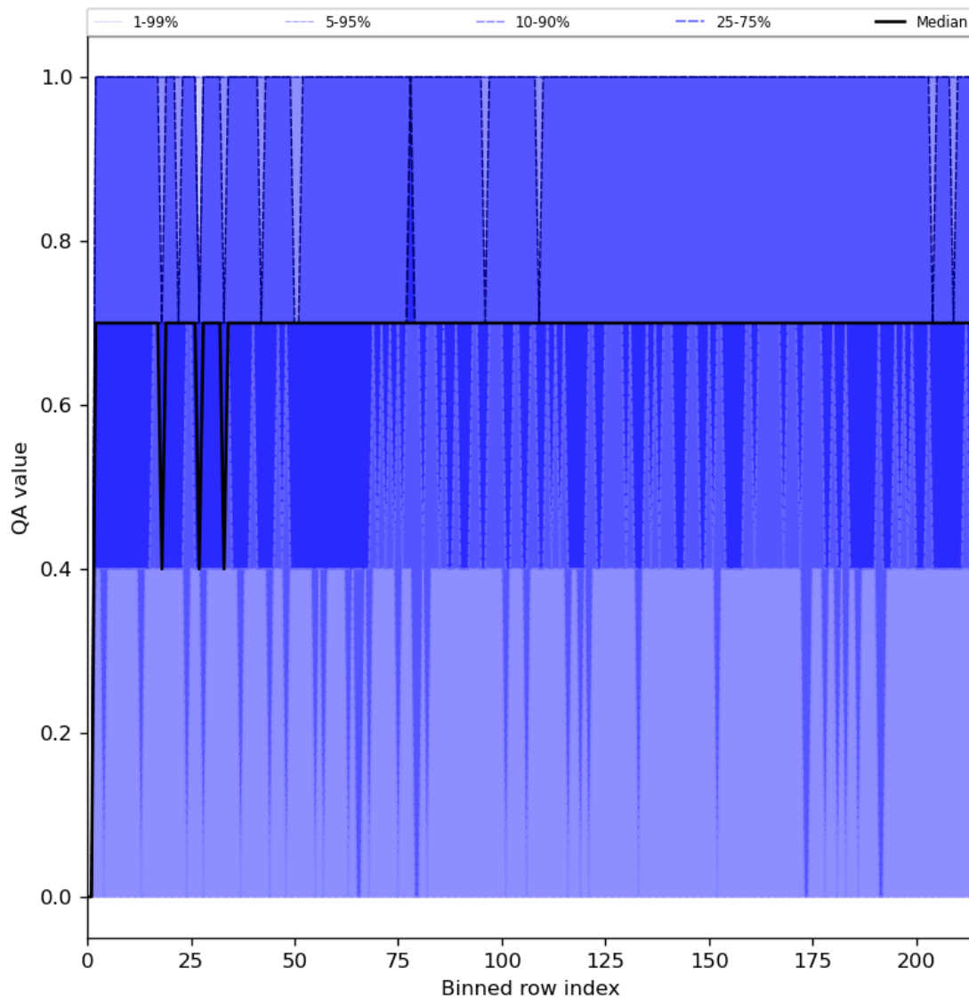
Figure 25: Along track statistics of “QA value” for 2024-04-10 to 2024-04-11
