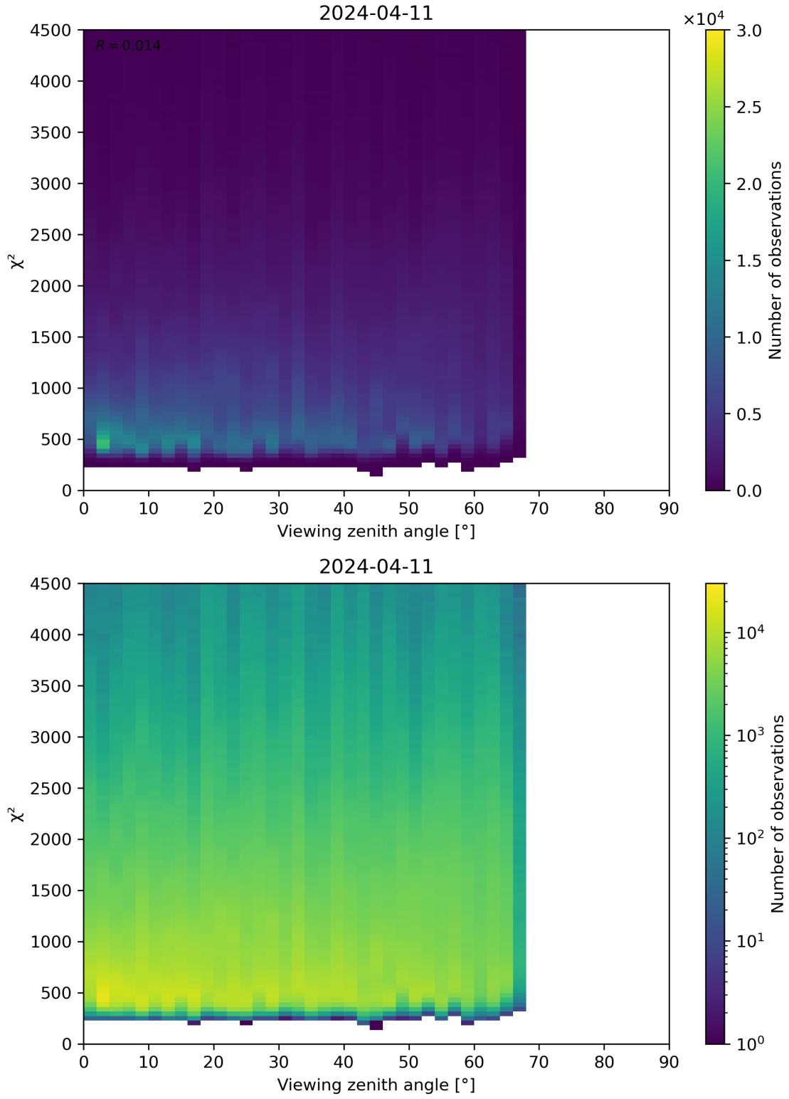
Figure 72: Scatter density plot of “Viewing zenith angle” against “ \chi^2 ” for 2024-04-10 to 2024-04-12.
