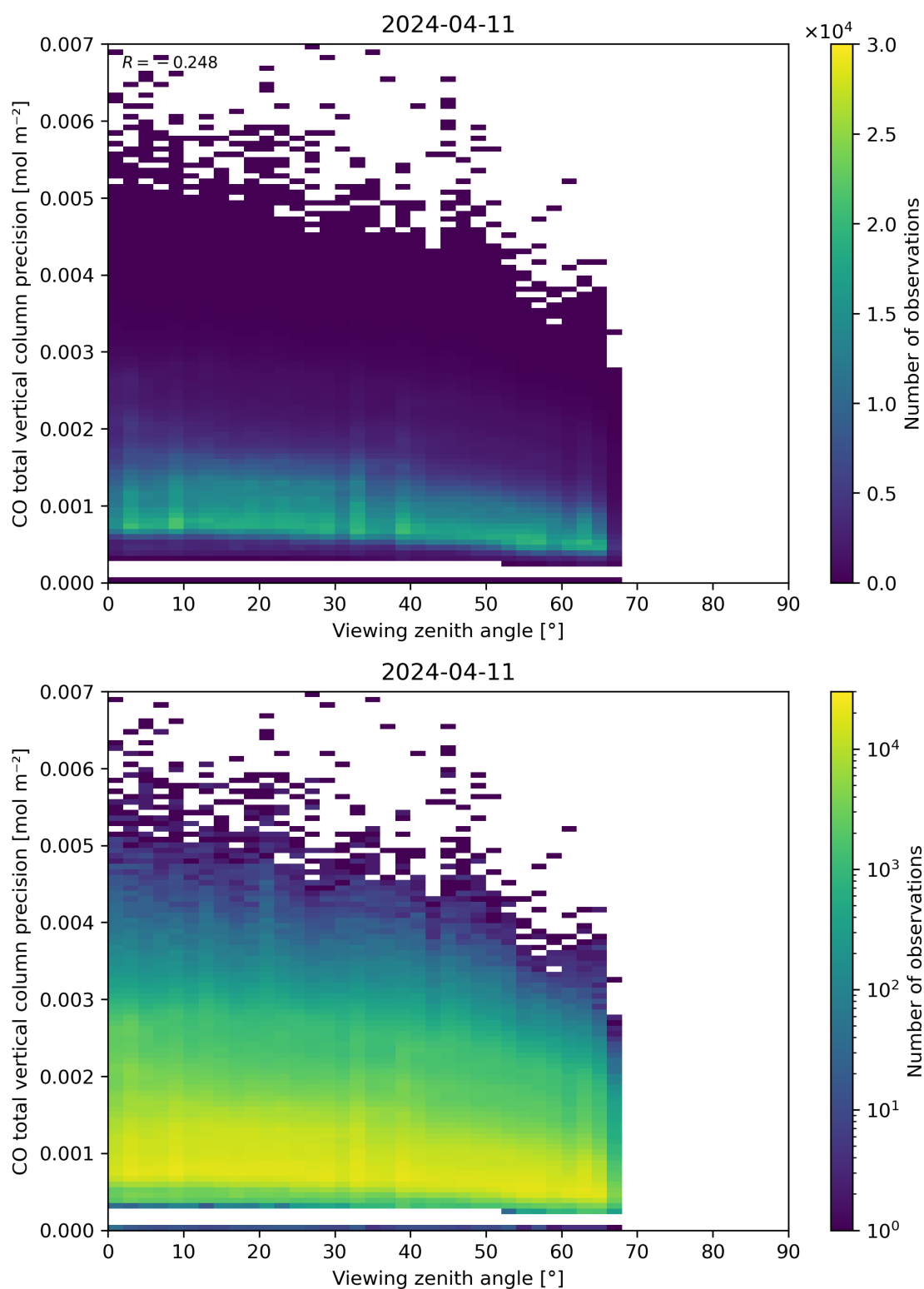
Figure 71: Scatter density plot of “Viewing zenith angle” against “CO total vertical column precision” for 2024-04-10 to 2024-04-12.
