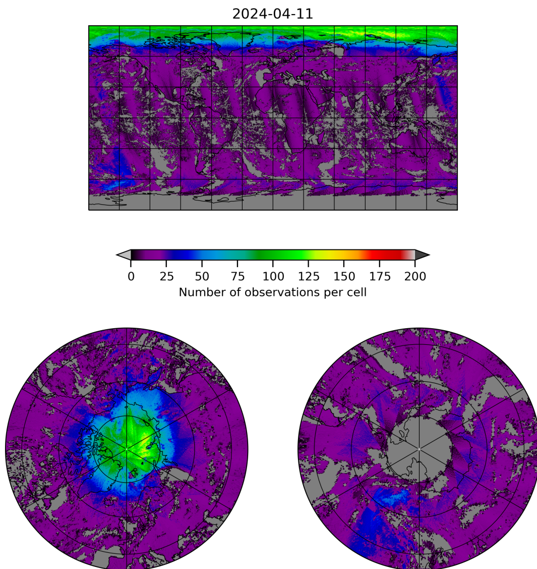
Figure 8: Map of the number of observations for 2024-04-10 to 2024-04-12
