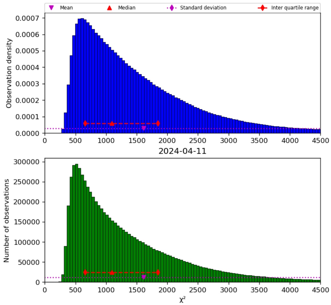
Figure 22: Histogram of “ \chi^2 ” for 2024-04-10 to 2024-04-12
