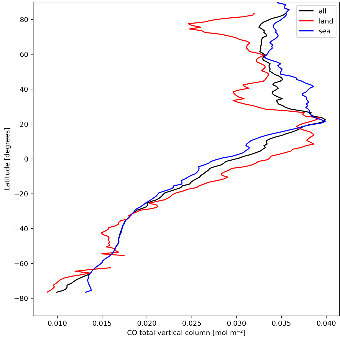
Figure 10: Zonal average of “CO total vertical column” for 2024-04-10 to 2024-04-12.
