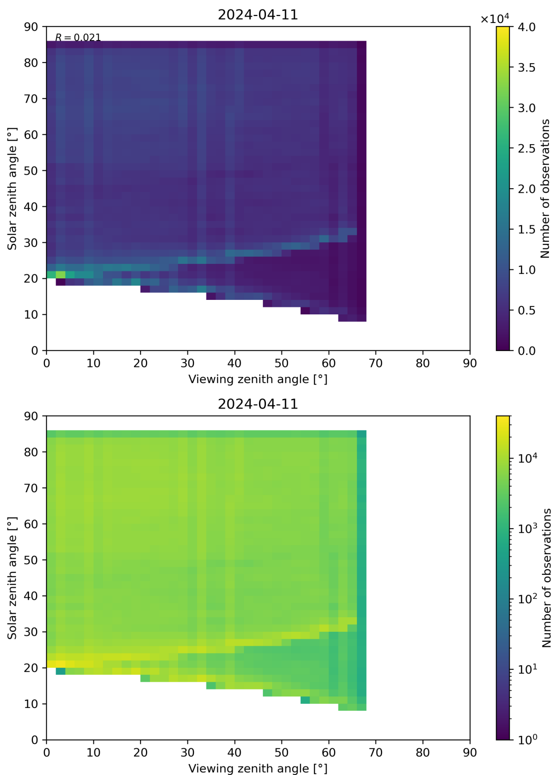
Figure 77: Scatter density plot of “Viewing zenith angle” against “Solar zenith angle” for 2024-04-10 to 2024-04-12.
