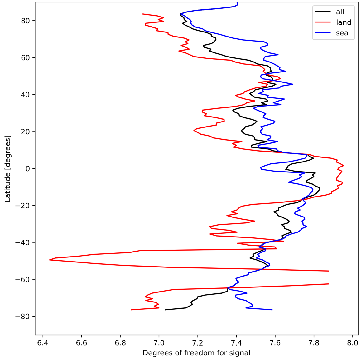
Figure 15: Zonal average of “Degrees of freedom for signal” for 2024-04-10 to 2024-04-12.
