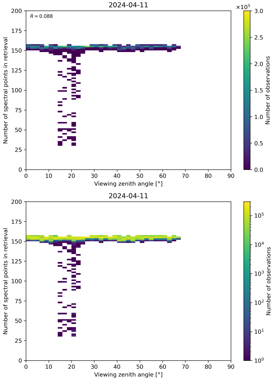
Figure 76: Scatter density plot of “Viewing zenith angle” against “Number of spectral points in retrieval” for 2024-04-10 to 2024-04-12.
