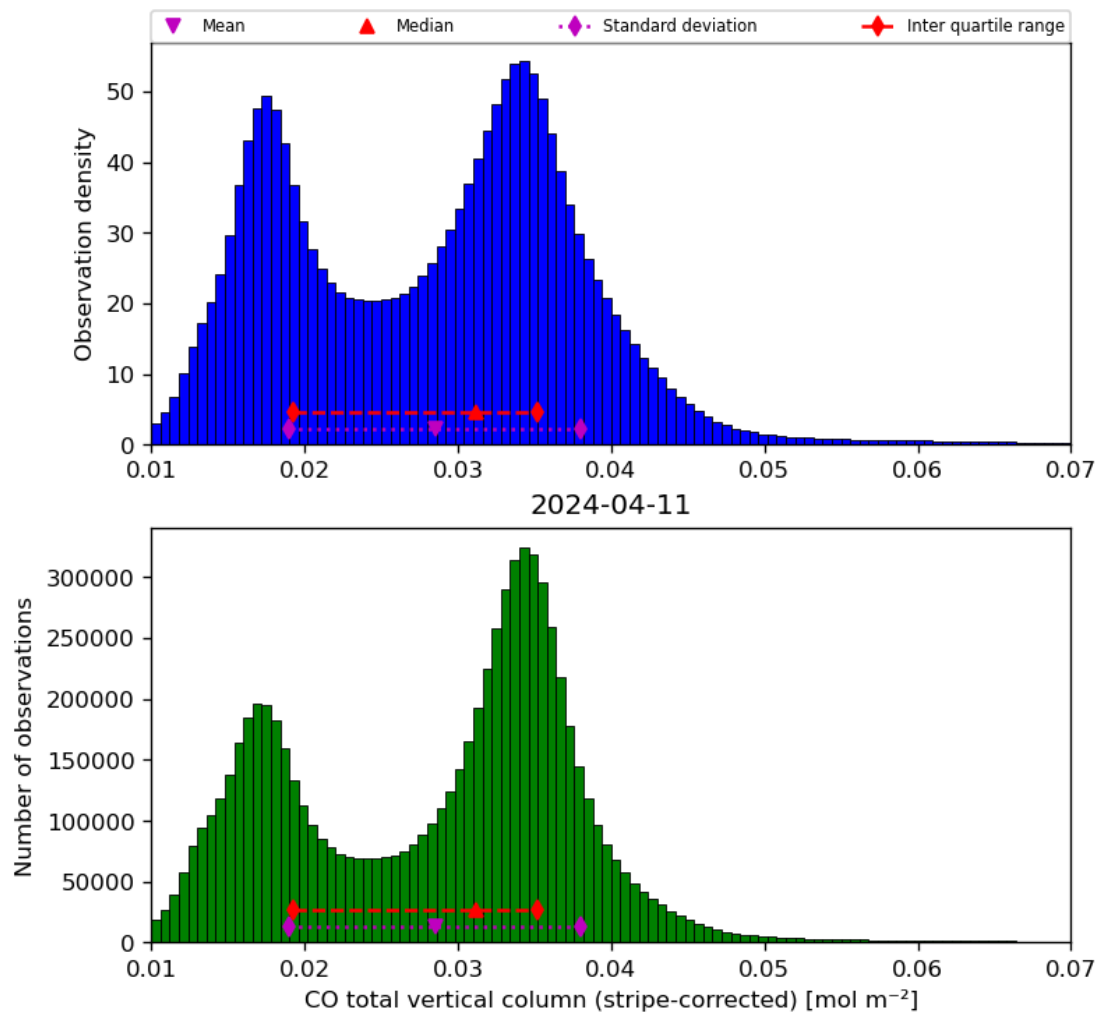
Figure 19: Histogram of “CO total vertical column (stripe-corrected)” for 2024-04-10 to 2024-04-12
