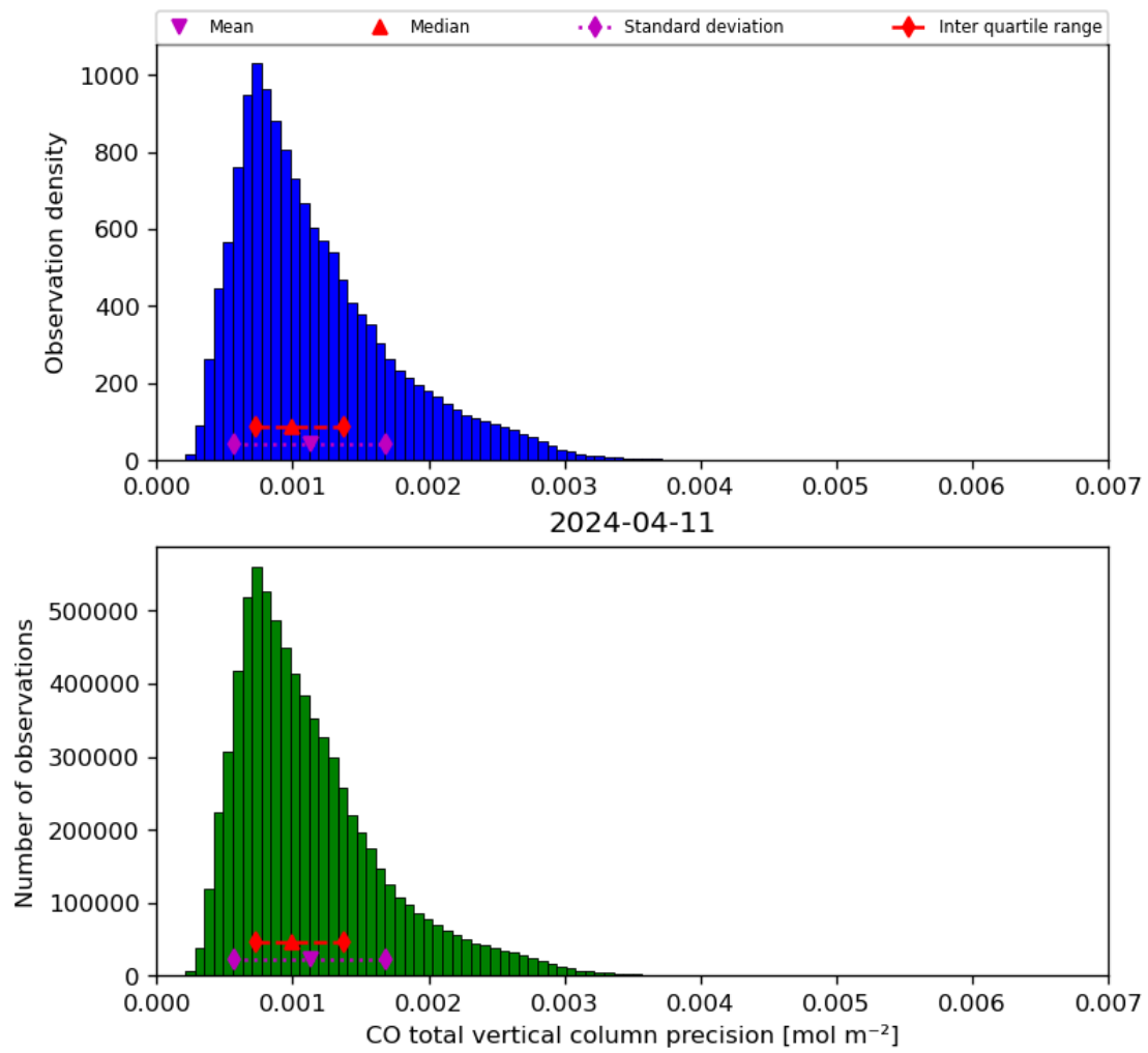
Figure 20: Histogram of “CO total vertical column precision” for 2024-04-10 to 2024-04-12
