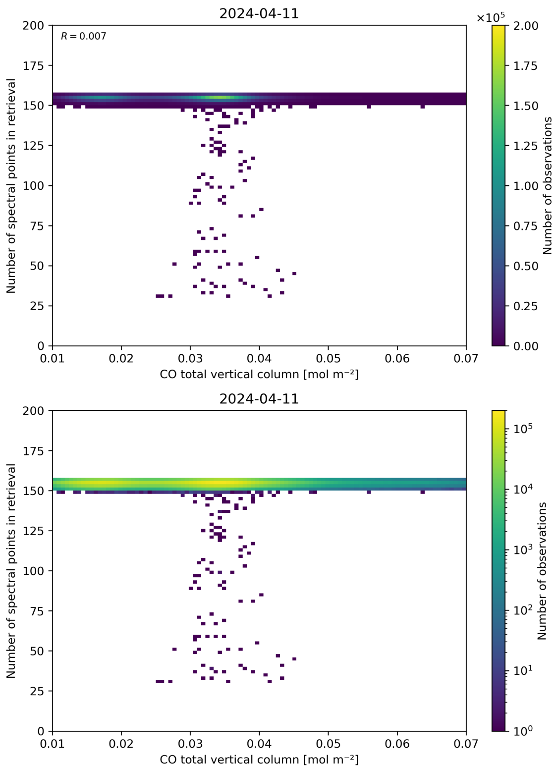
Figure 43: Scatter density plot of “CO total vertical column” against “Number of spectral points in retrieval” for 2024-04-10 to 2024-04-12.
