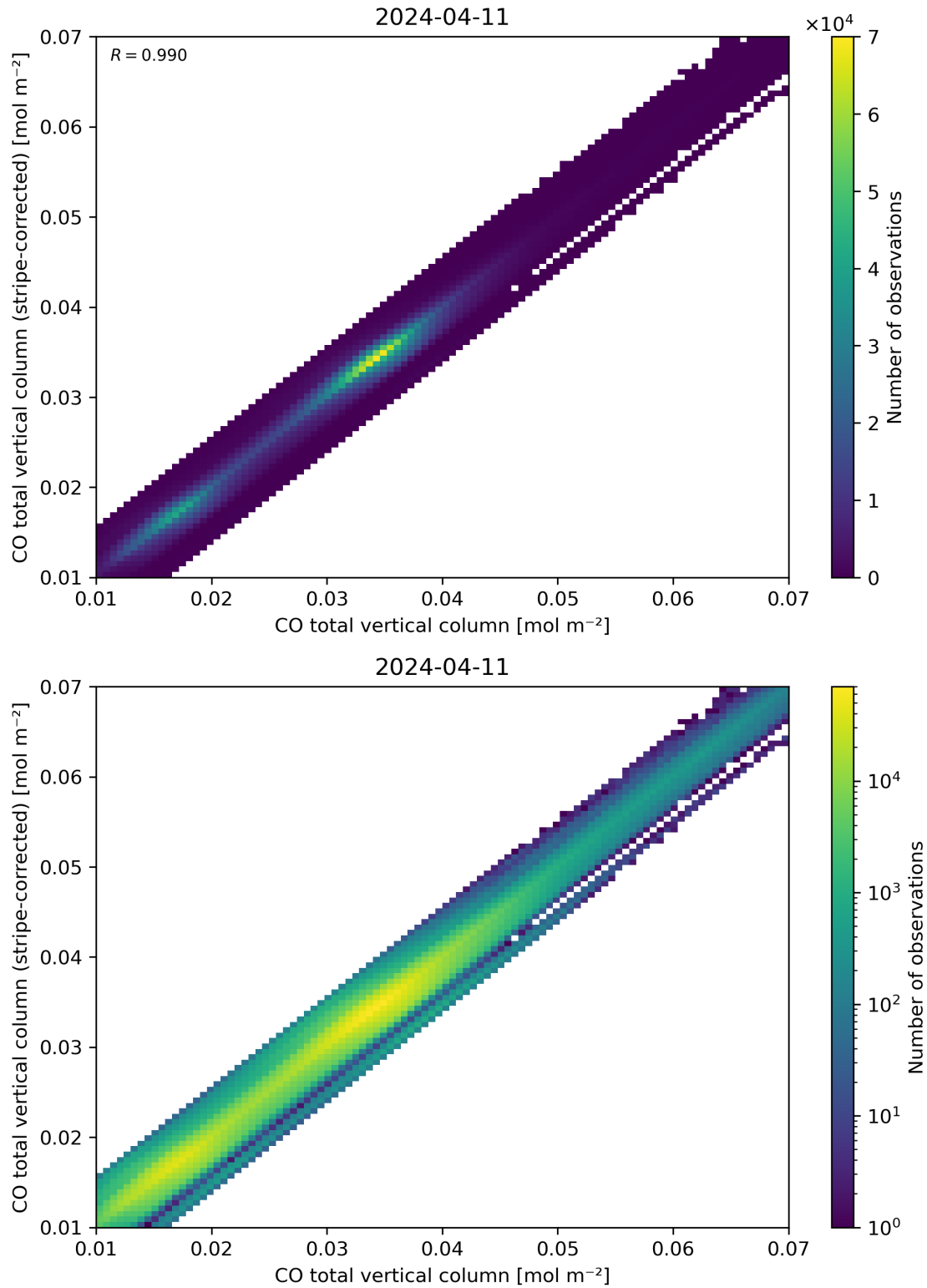
Figure 33: Scatter density plot of “CO total vertical column” against “CO total vertical column (stripe-corrected)” for 2024-04-10 to 2024-04-12.
