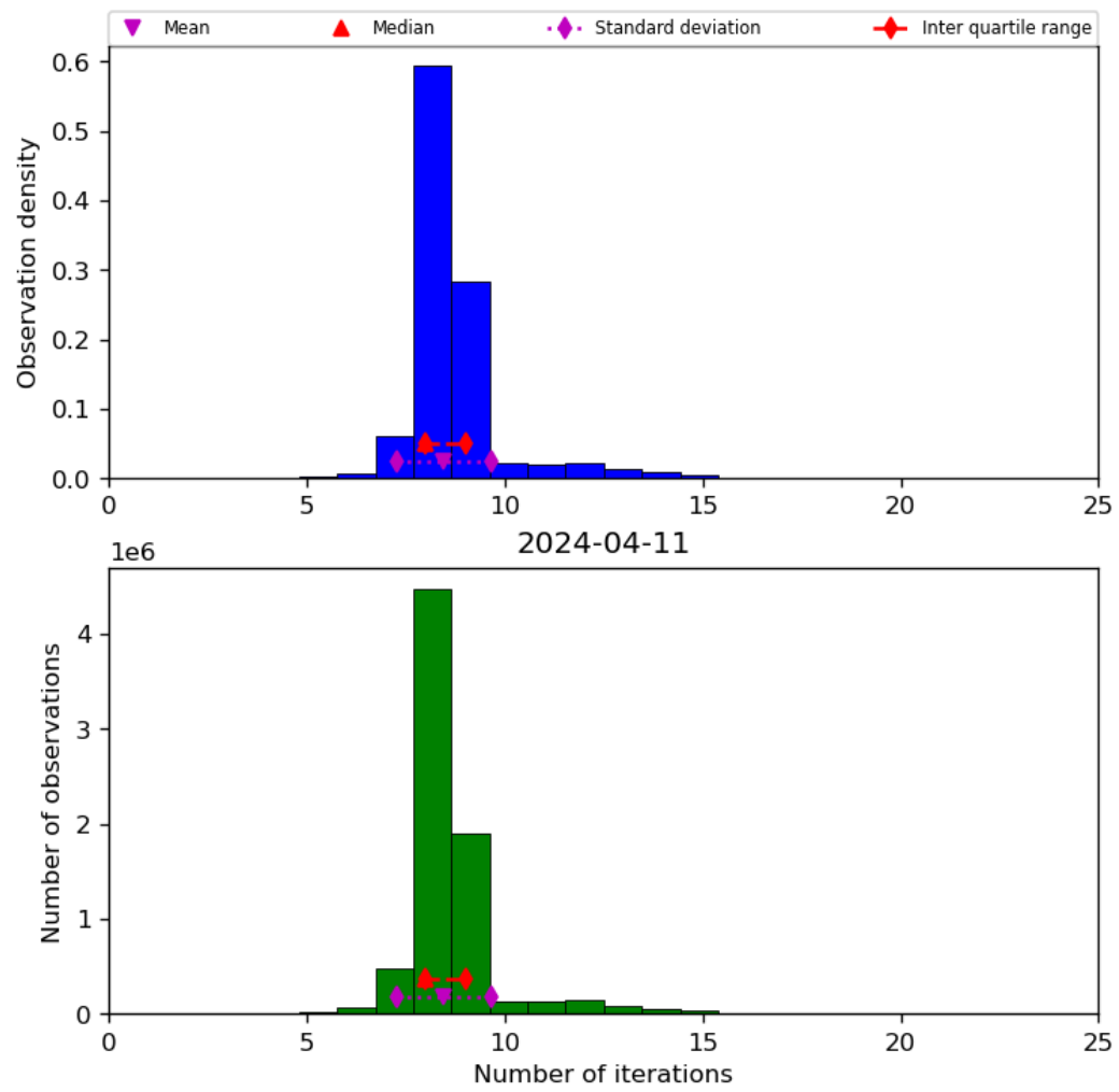
Figure 24: Histogram of “Number of iterations” for 2024-04-10 to 2024-04-12
