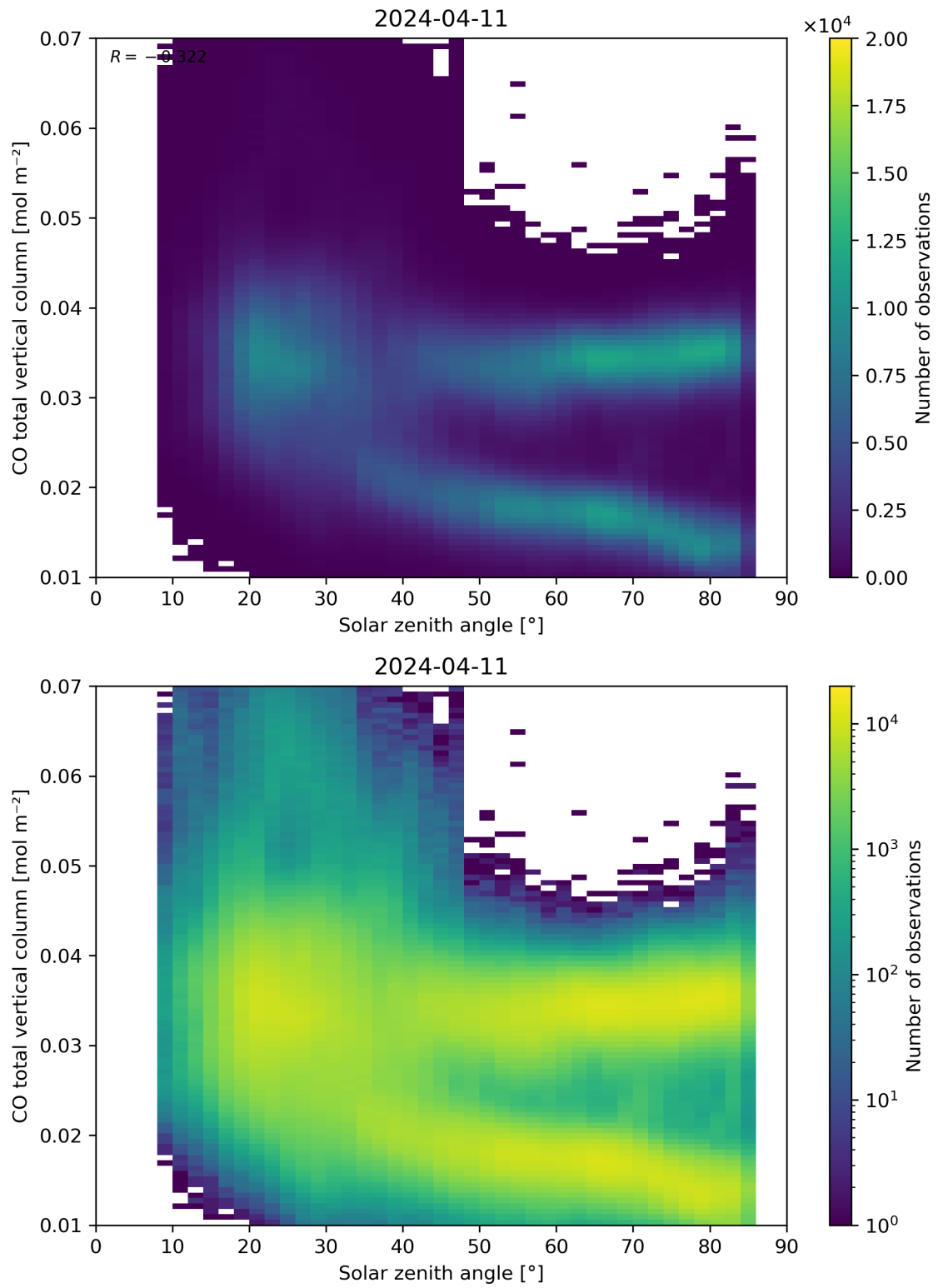
Figure 61: Scatter density plot of “Solar zenith angle” against “CO total vertical column” for 2024-04-10 to 2024-04-12.
