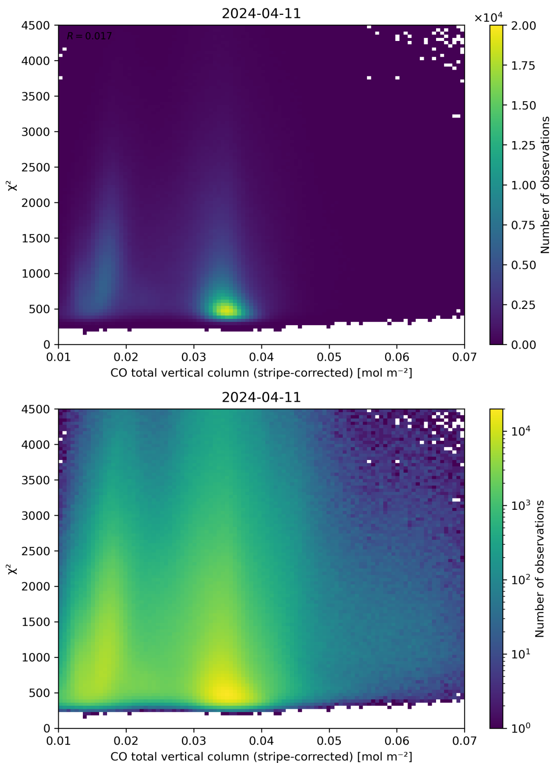
Figure 37: Scatter density plot of “CO total vertical column (stripe-corrected)” against “ \chi^2 ” for 2024-04-10 to 2024-04-12.
