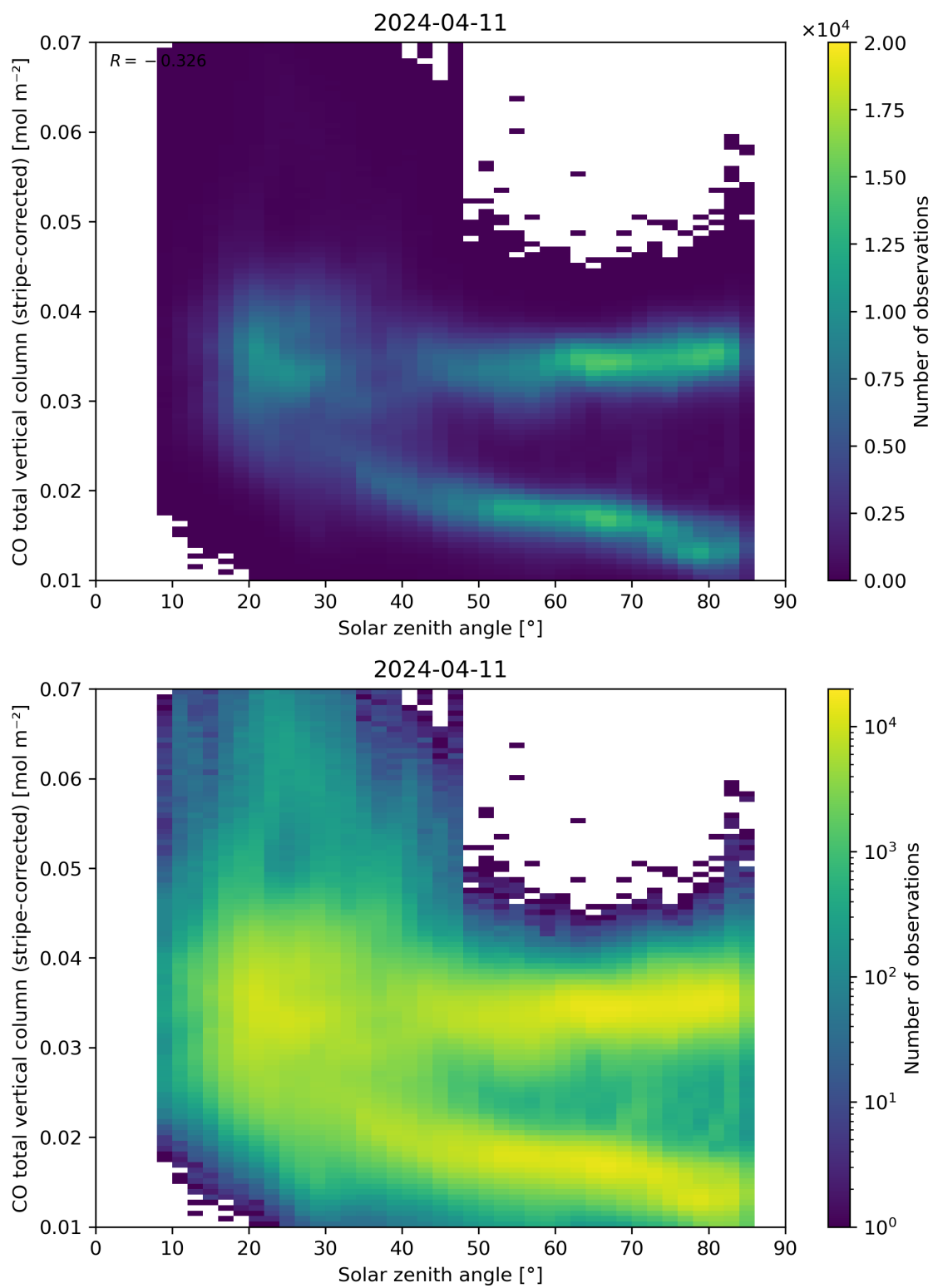
Figure 62: Scatter density plot of “Solar zenith angle” against “CO total vertical column (stripe-corrected)” for 2024-04-10 to 2024-04-12.
