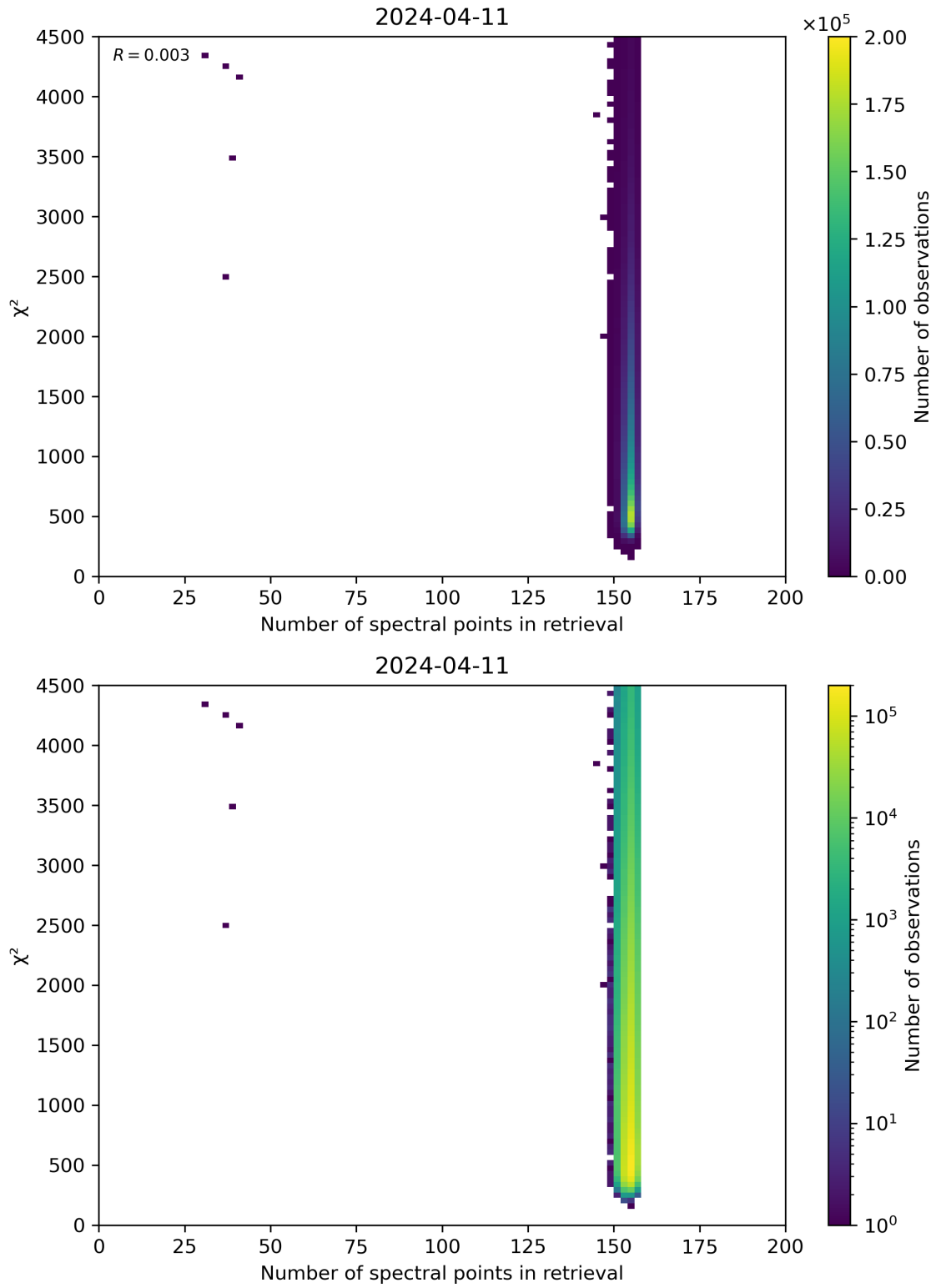
Figure 58: Scatter density plot of “Number of spectral points in retrieval” against “ \chi^2 ” for 2024-04-10 to 2024-04-12.
