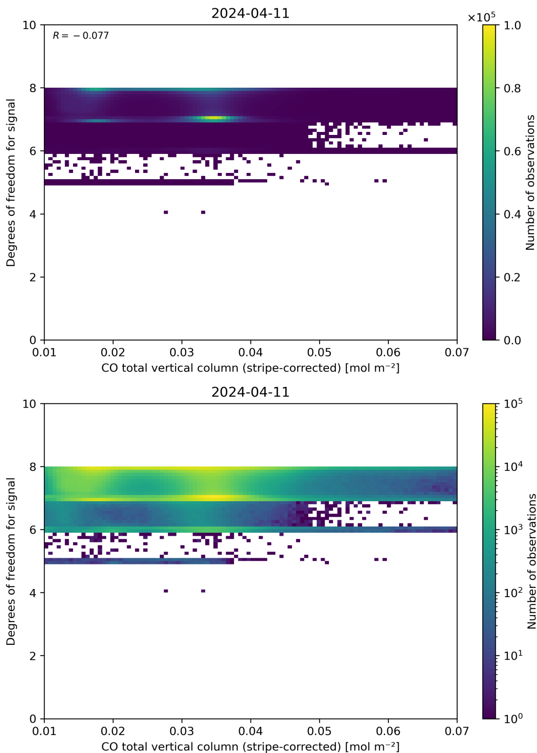
Figure 38: Scatter density plot of “CO total vertical column (stripe-corrected)” against “Degrees of freedom for signal” for 2024-04-10 to 2024-04-12.
