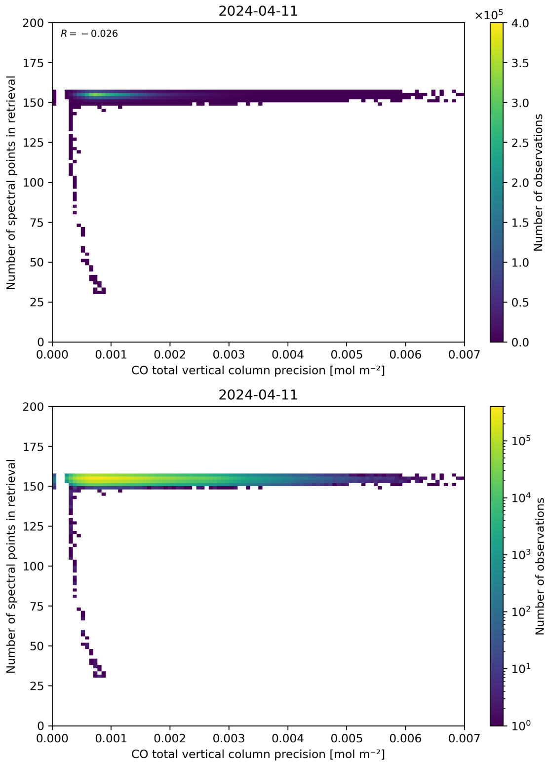
Figure 47: Scatter density plot of “CO total vertical column precision” against “Number of spectral points in retrieval” for 2024-04-10 to 2024-04-12.
