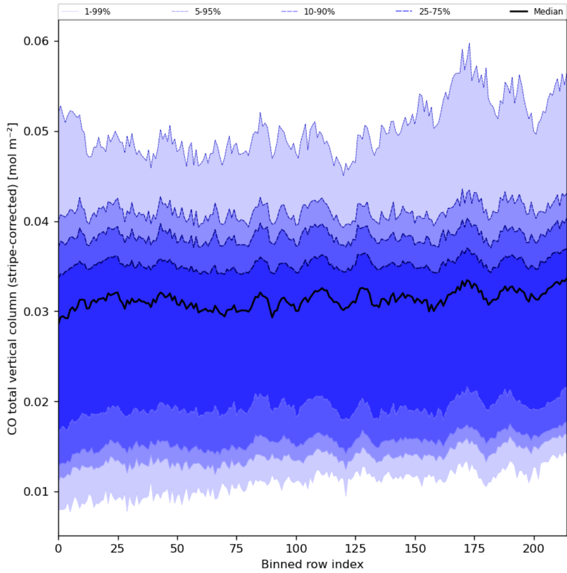
Figure 27: Along track statistics of “CO total vertical column (stripe-corrected)” for 2024-04-10 to 2024-04-12
