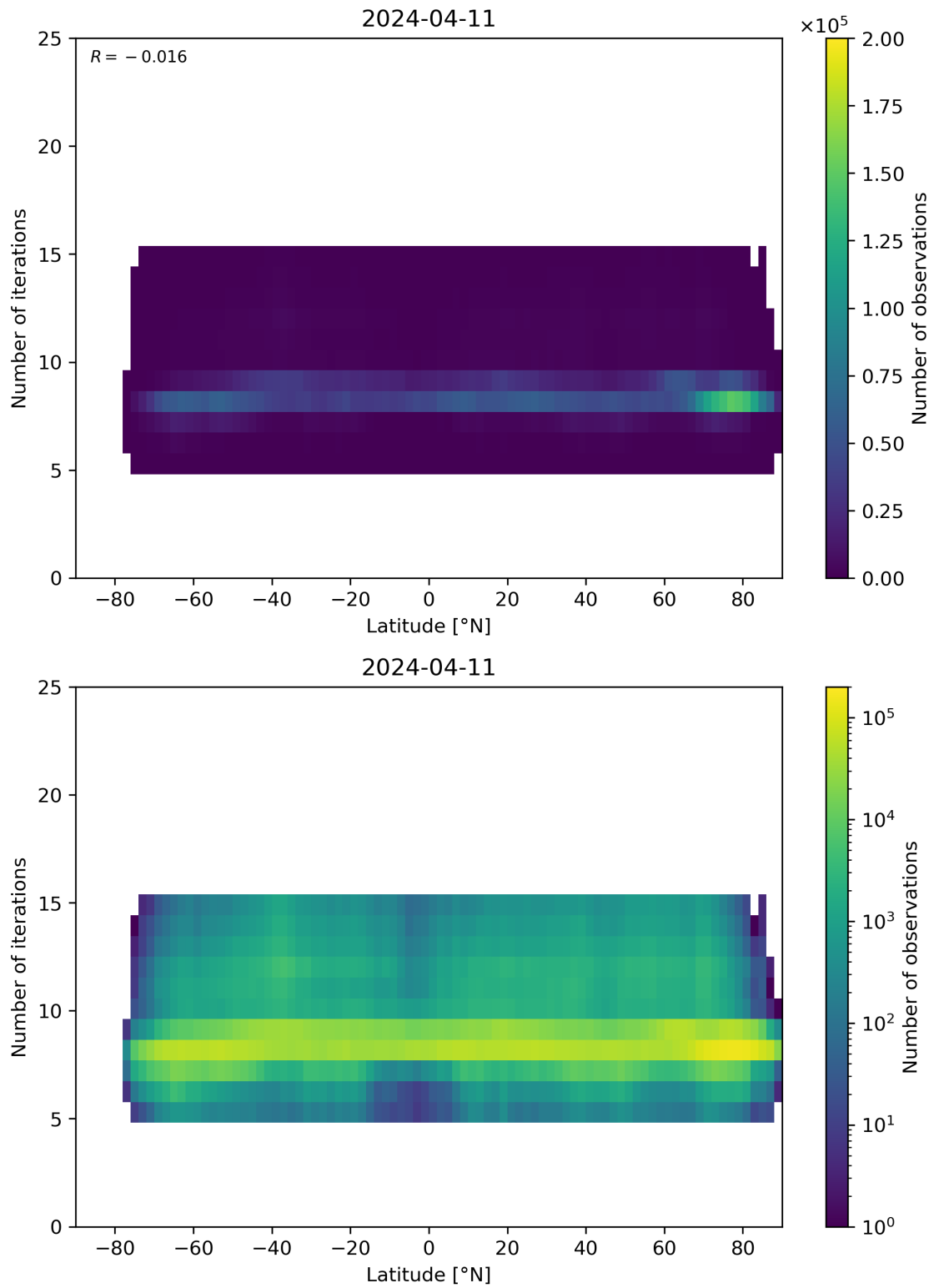
Figure 56: Scatter density plot of “Latitude” against “Number of iterations” for 2024-04-10 to 2024-04-12.
