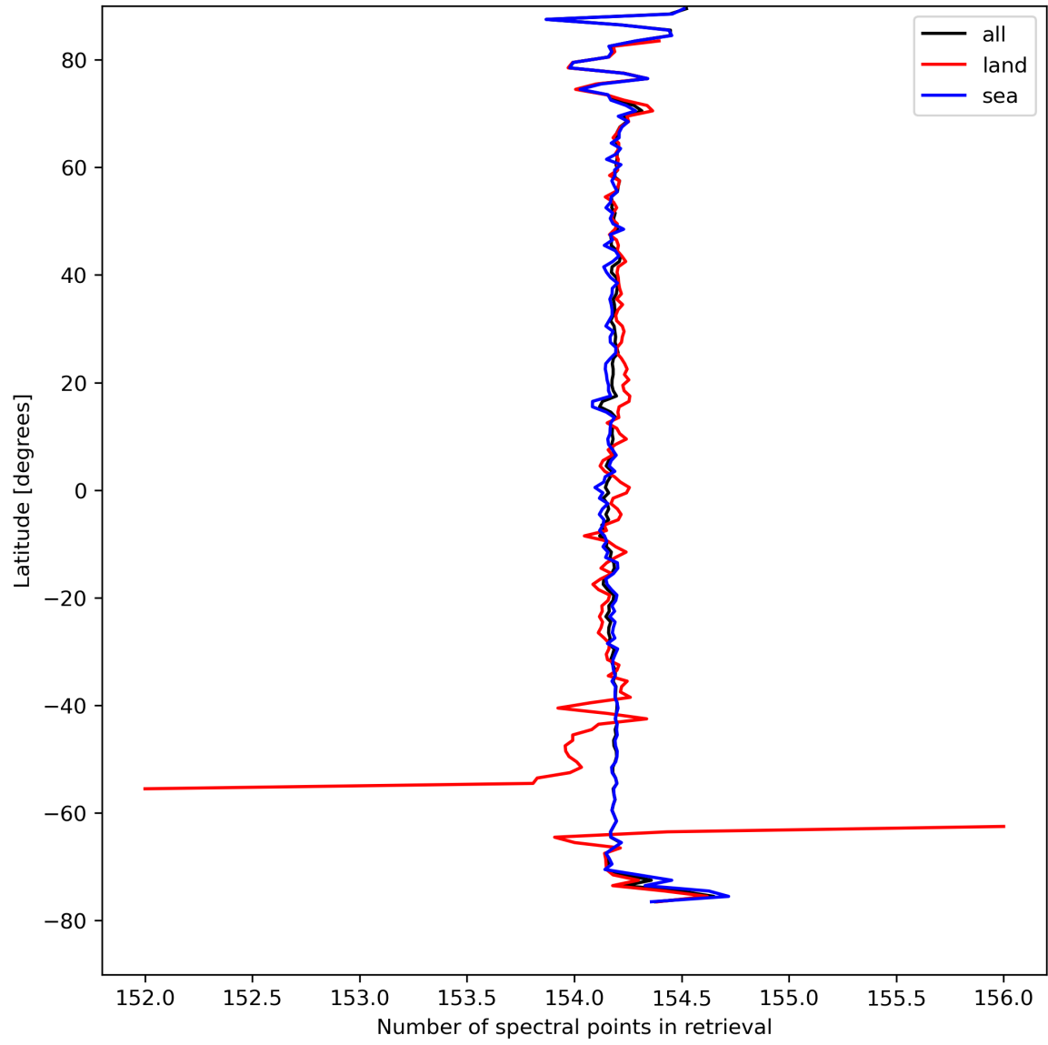
Figure 13: Zonal average of “Number of spectral points in retrieval” for 2024-04-10 to 2024-04-12.
