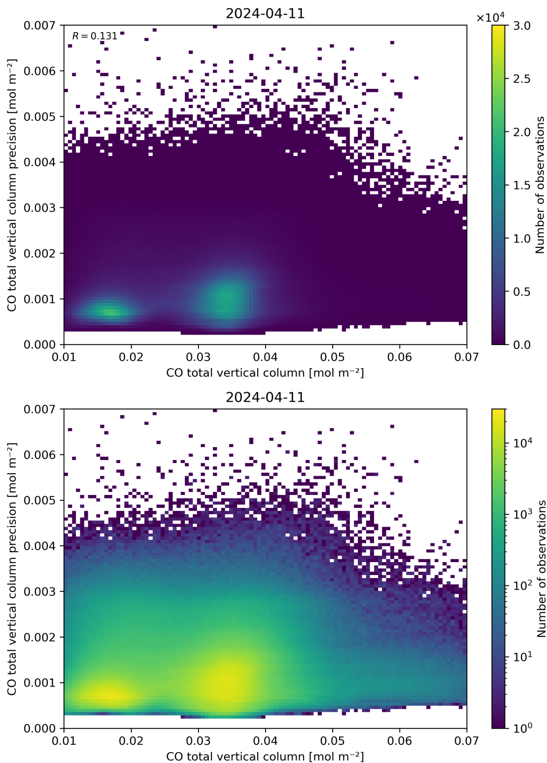
Figure 34: Scatter density plot of “CO total vertical column” against “CO total vertical column precision” for 2024-04-10 to 2024-04-12.
