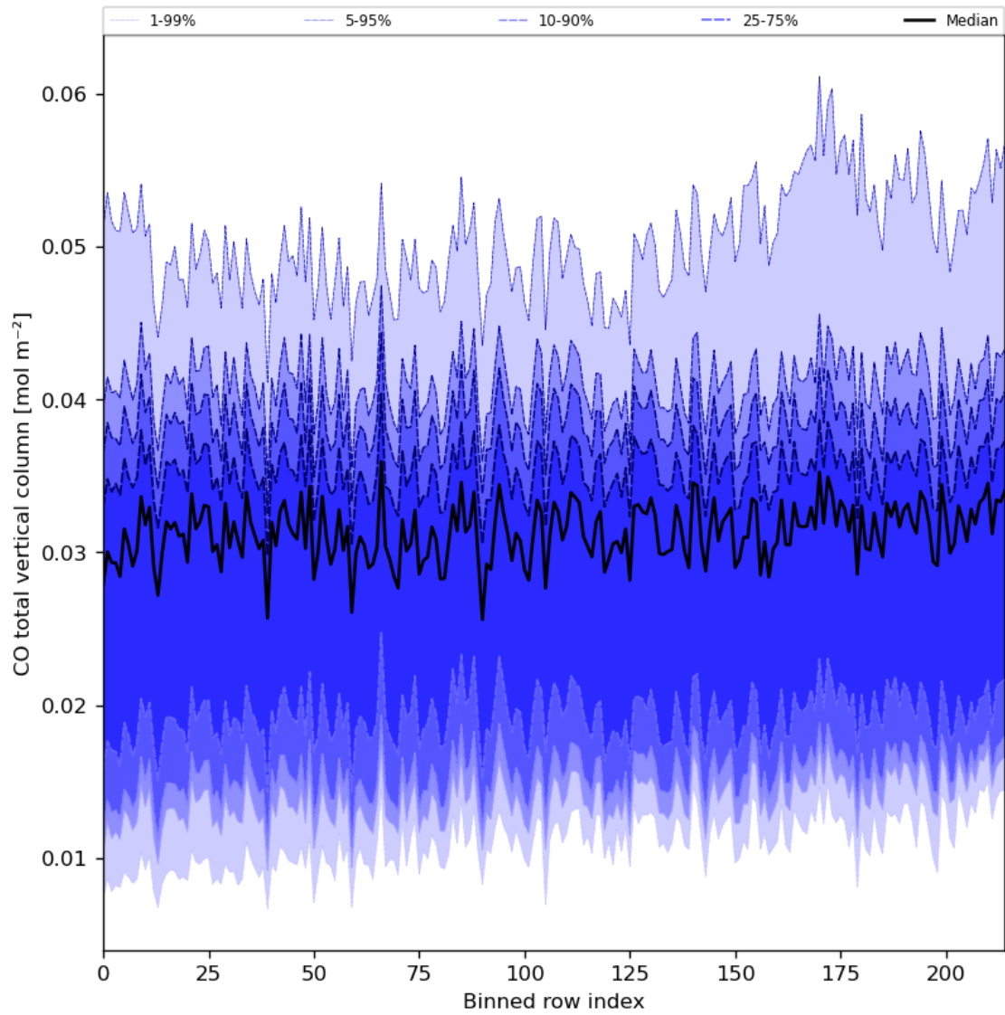
Figure 26: Along track statistics of “CO total vertical column” for 2024-04-10 to 2024-04-12
