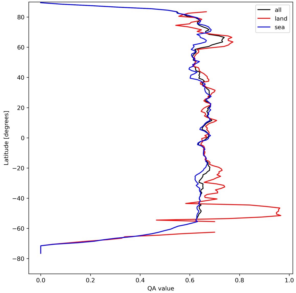
Figure 9: Zonal average of “QA value” for 2024-04-10 to 2024-04-12.
