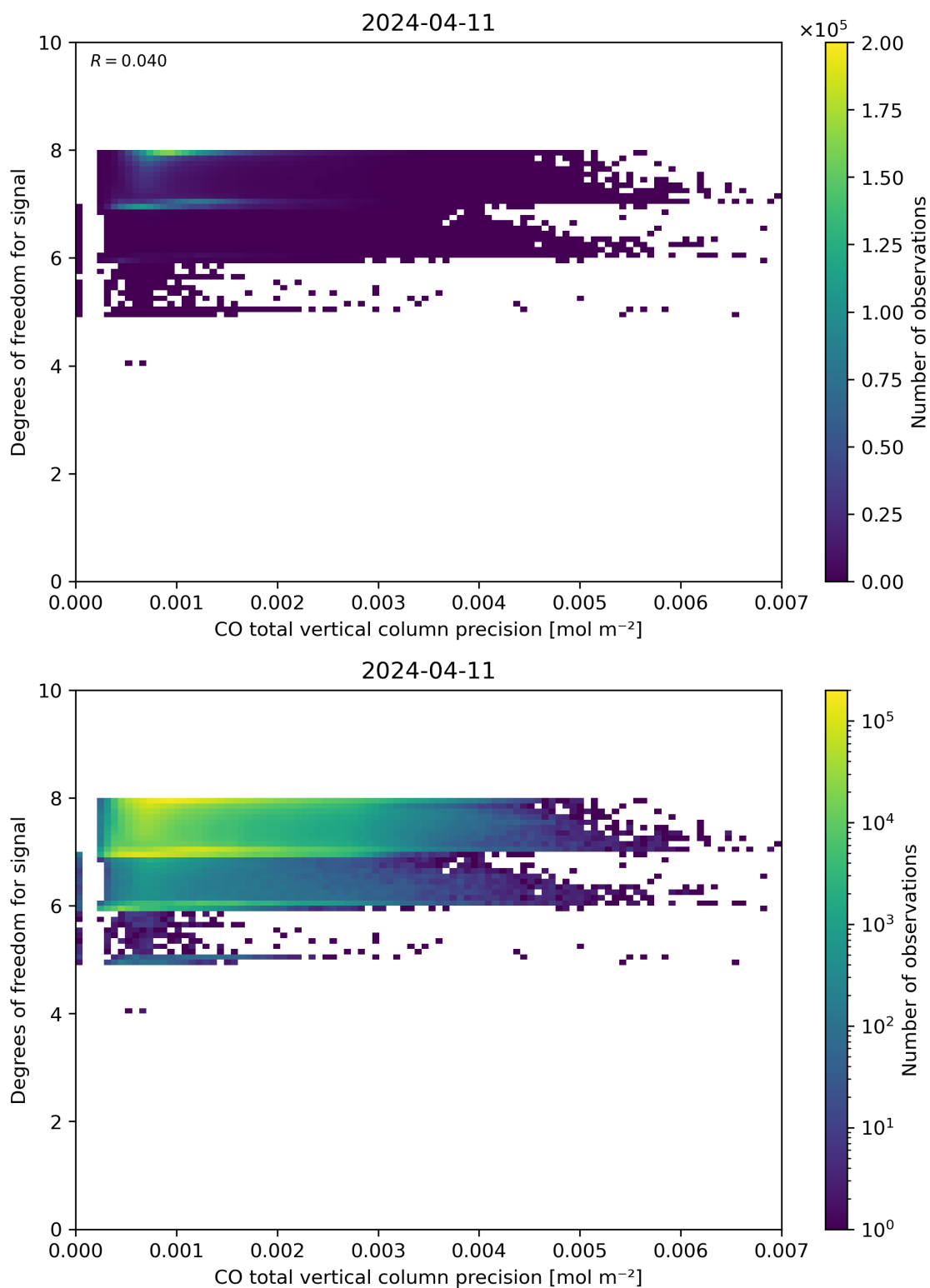
Figure 45: Scatter density plot of “CO total vertical column precision” against “Degrees of freedom for signal” for 2024-04-10 to 2024-04-12.
