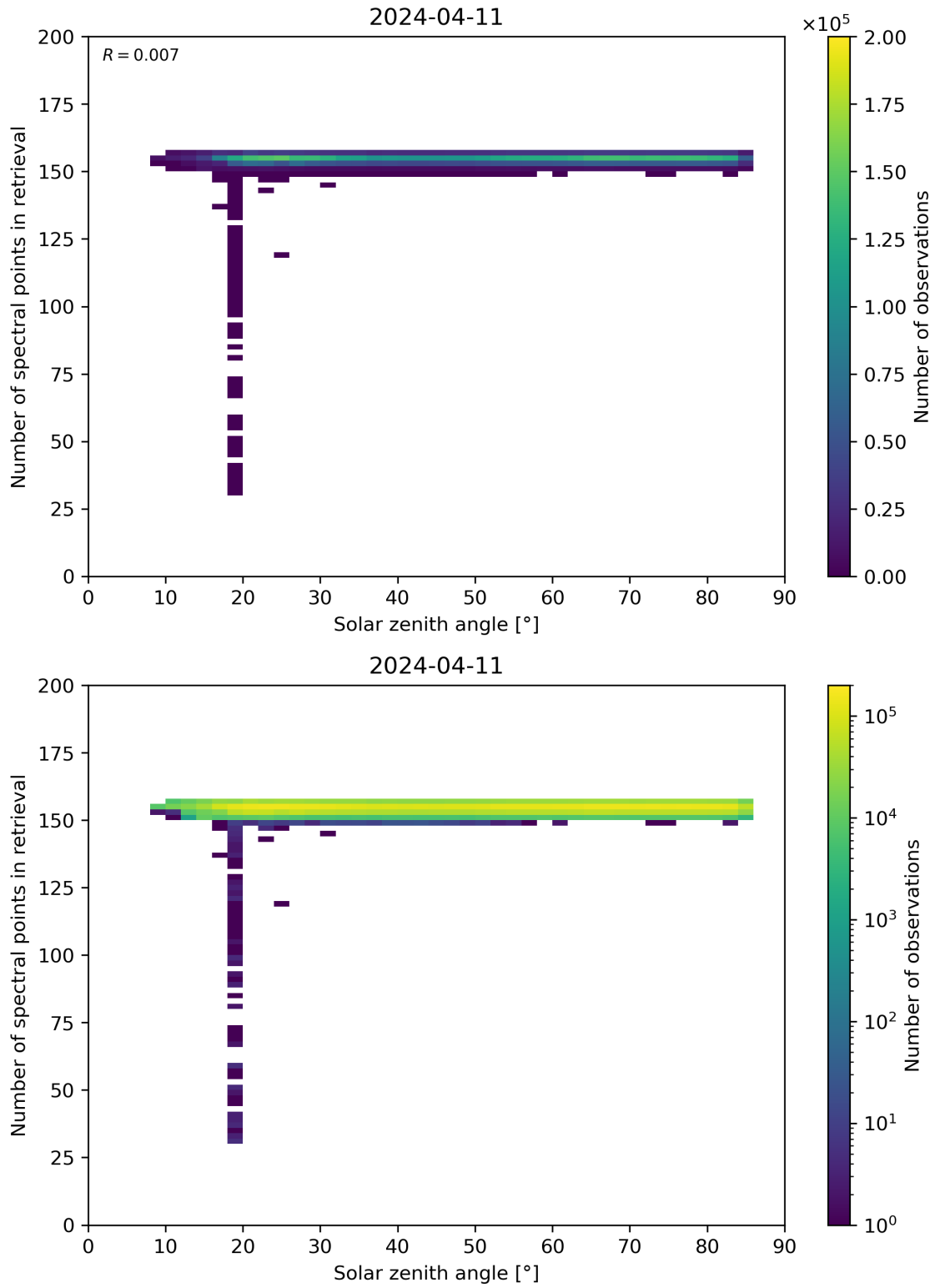
Figure 68: Scatter density plot of “Solar zenith angle” against “Number of spectral points in retrieval” for 2024-04-10 to 2024-04-12.
