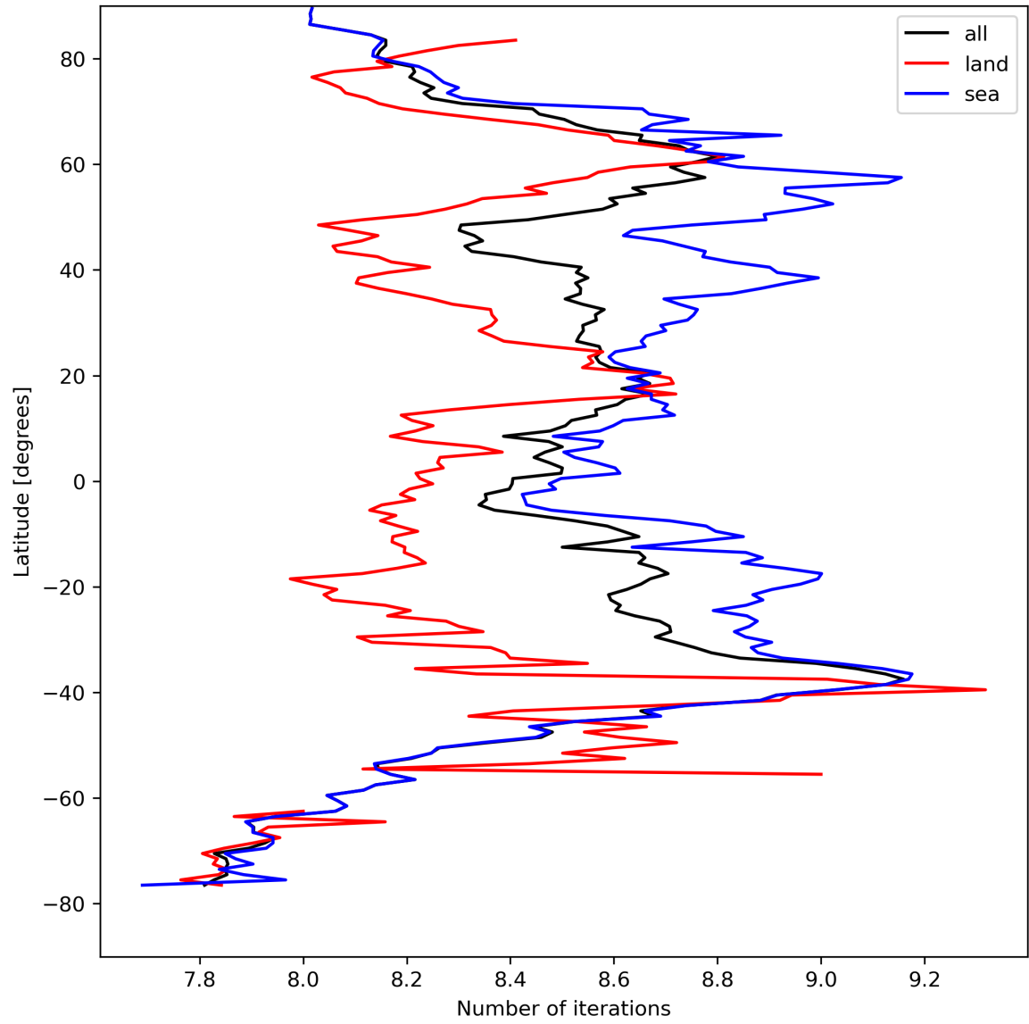
Figure 16: Zonal average of “Number of iterations” for 2024-04-10 to 2024-04-12.
