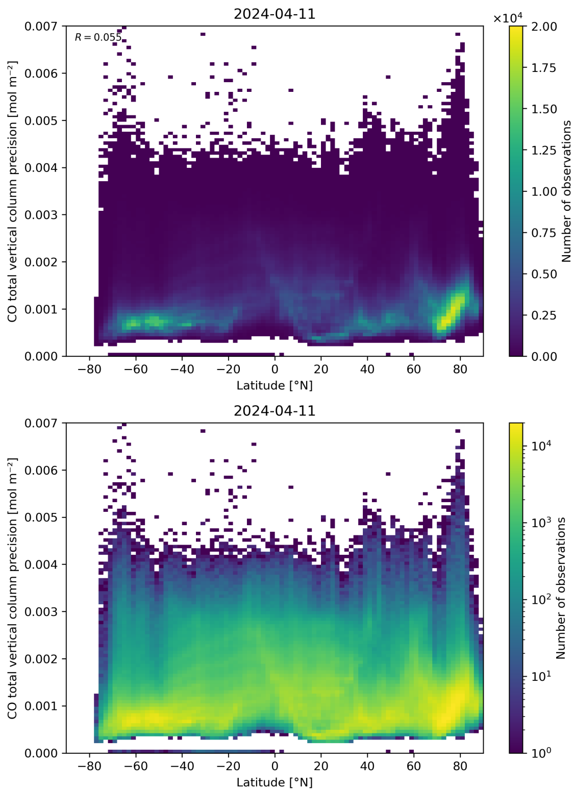
Figure 53: Scatter density plot of “Latitude” against “CO total vertical column precision” for 2024-04-10 to 2024-04-12.
