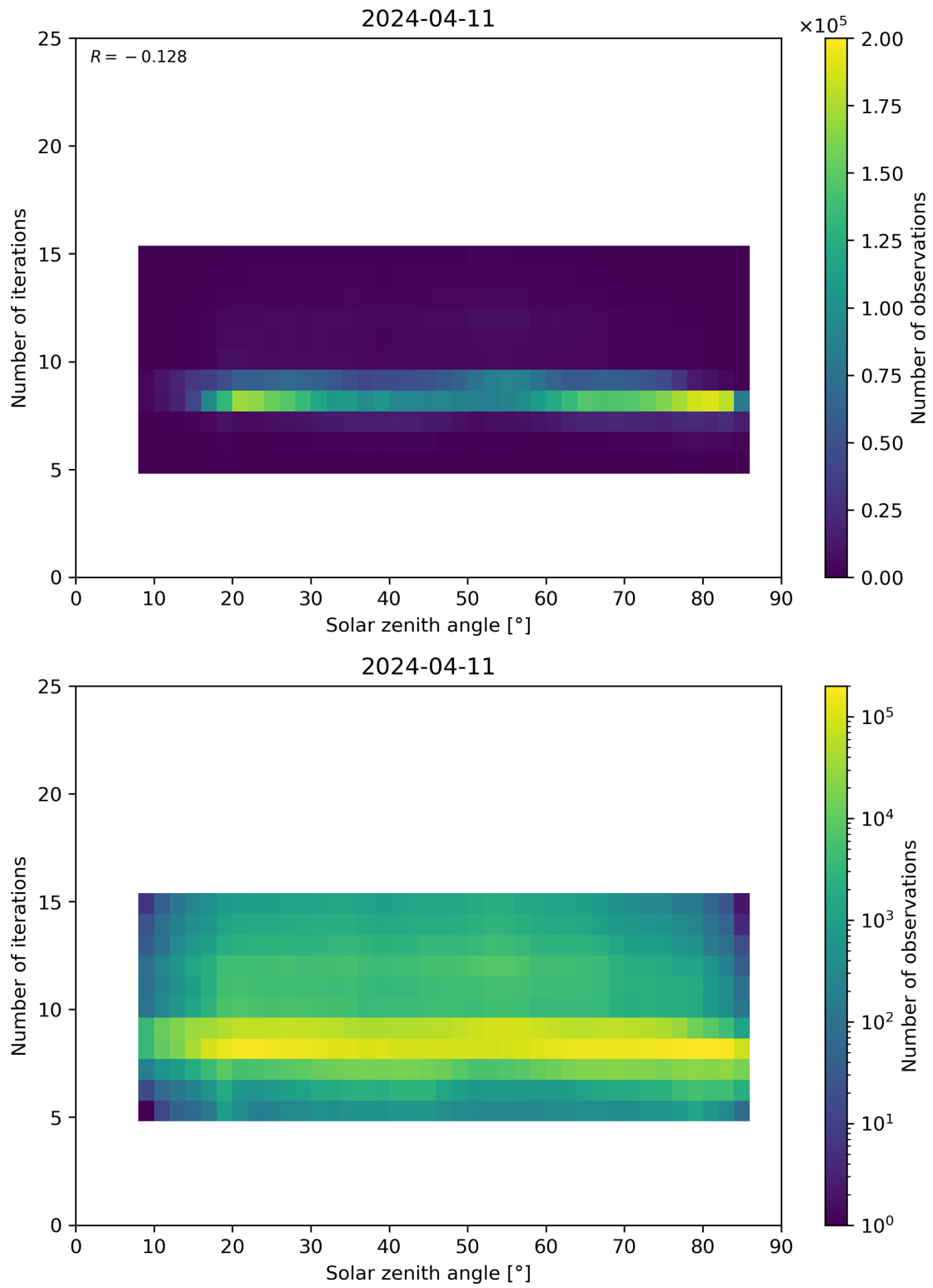
Figure 67: Scatter density plot of “Solar zenith angle” against “Number of iterations” for 2024-04-10 to 2024-04-12.
