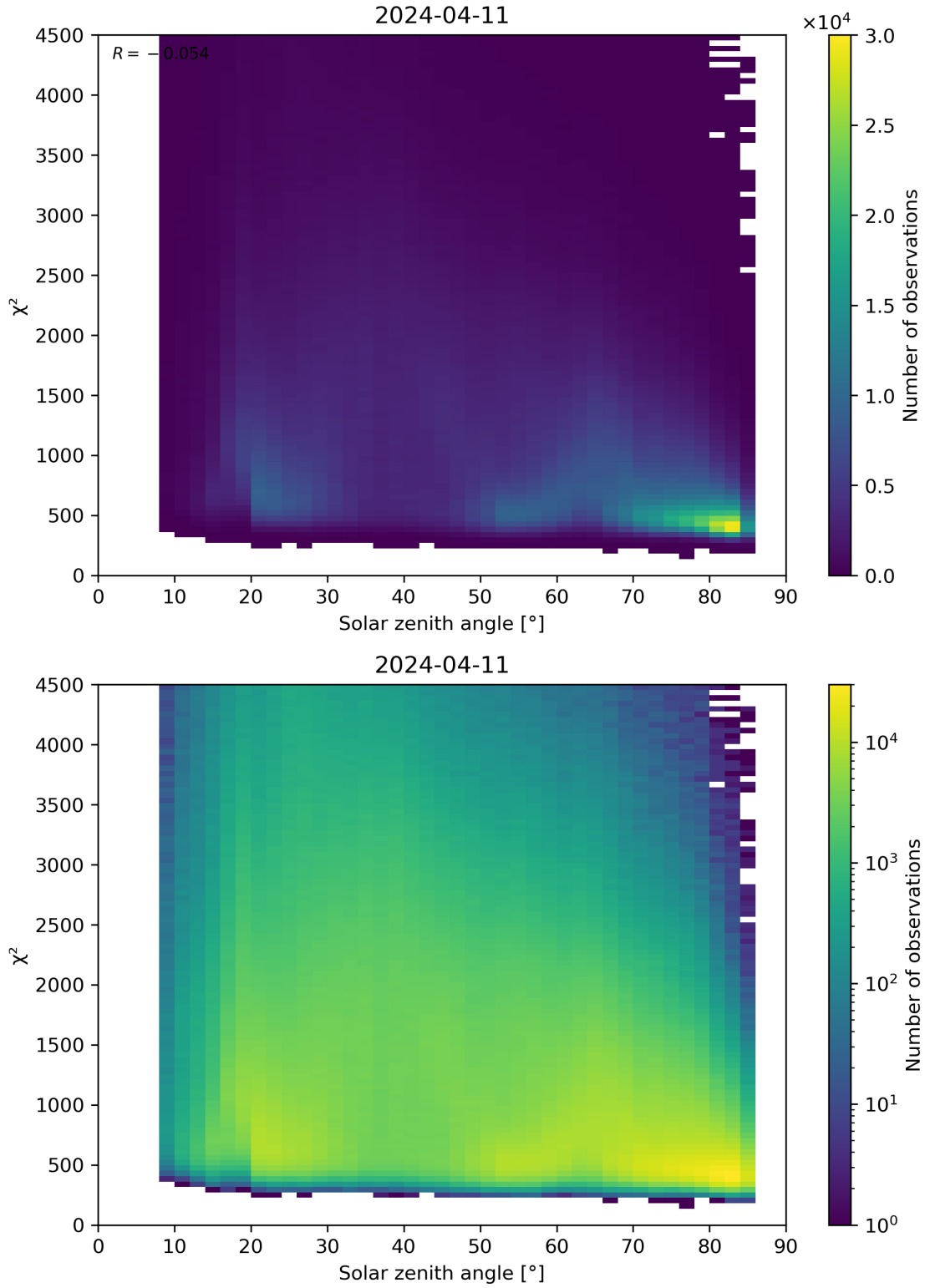
Figure 64: Scatter density plot of “Solar zenith angle” against “ \chi^2 ” for 2024-04-10 to 2024-04-12.
