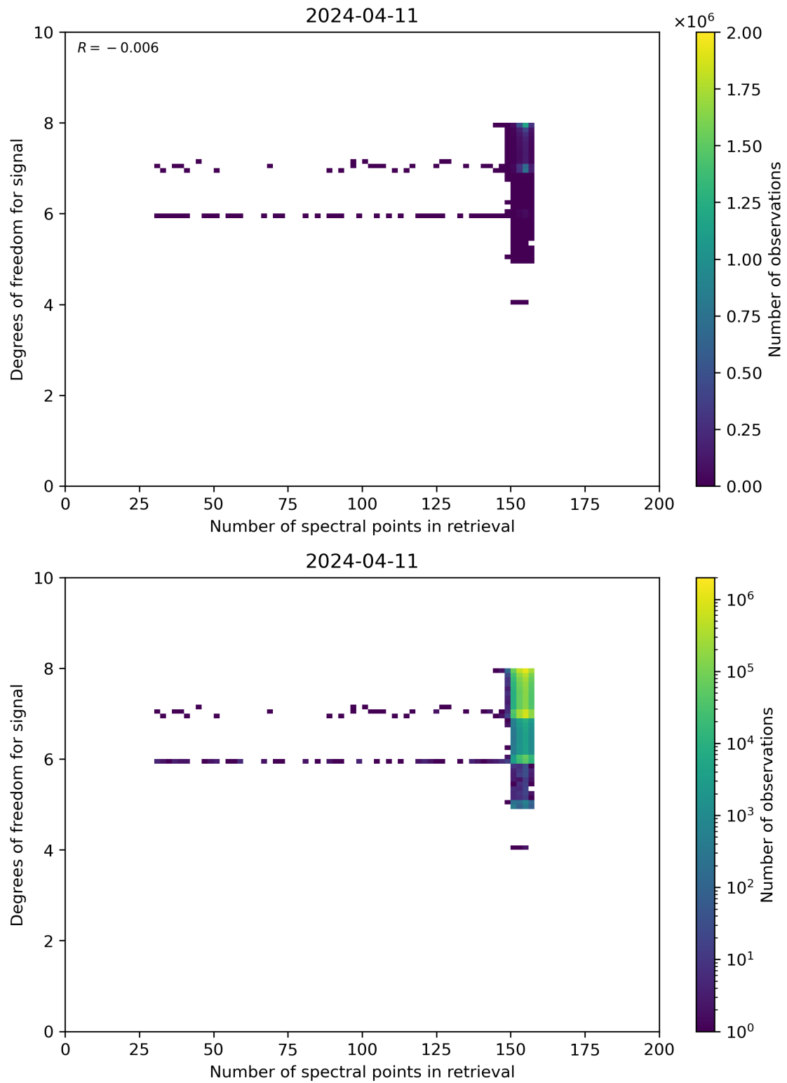
Figure 59: Scatter density plot of “Number of spectral points in retrieval” against “Degrees of freedom for signal” for 2024-04-10 to 2024-04-12.
