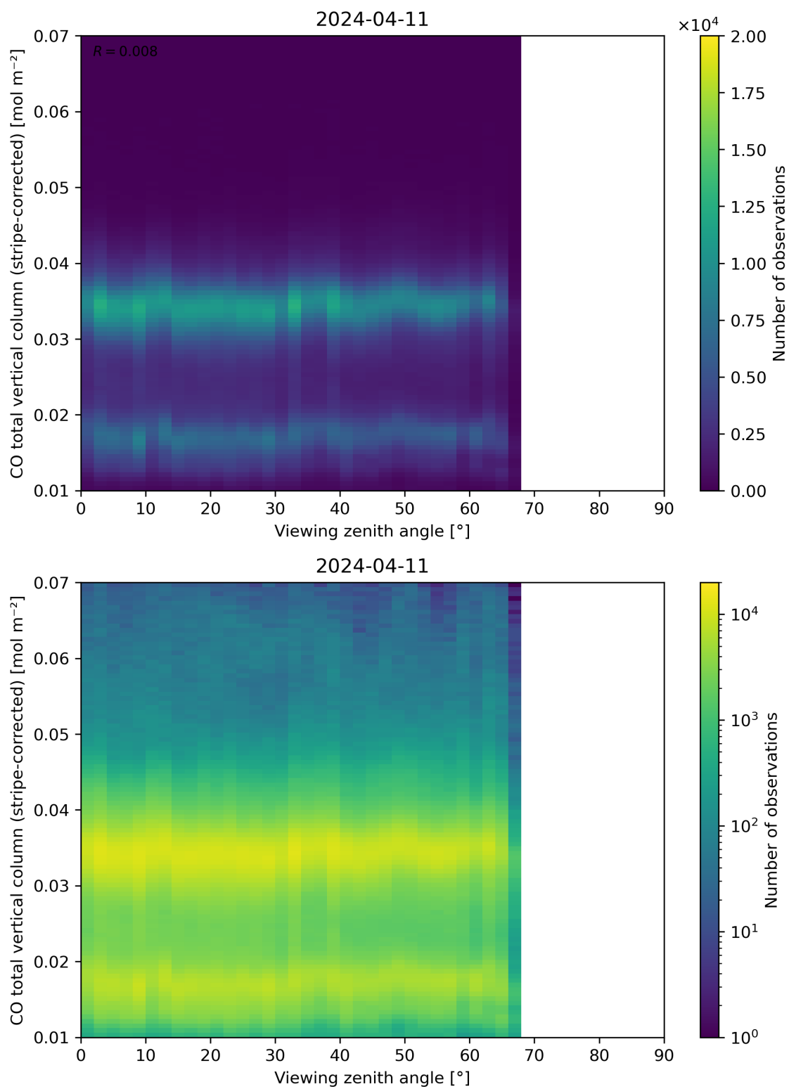
Figure 70: Scatter density plot of “Viewing zenith angle” against “CO total vertical column (stripe-corrected)” for 2024-04-10 to 2024-04-12.
