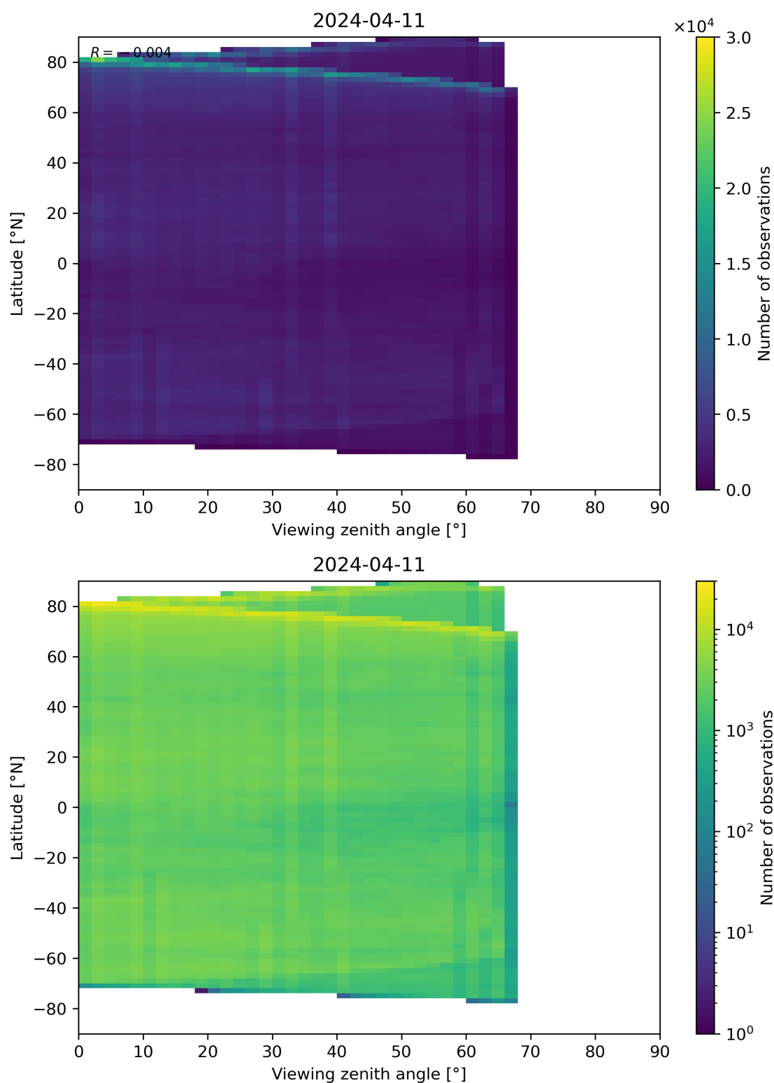
Figure 74: Scatter density plot of “Viewing zenith angle” against “Latitude” for 2024-04-10 to 2024-04-12.
