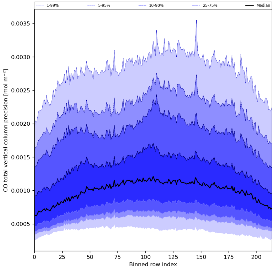
Figure 28: Along track statistics of “CO total vertical column precision” for 2024-04-10 to 2024-04-12
