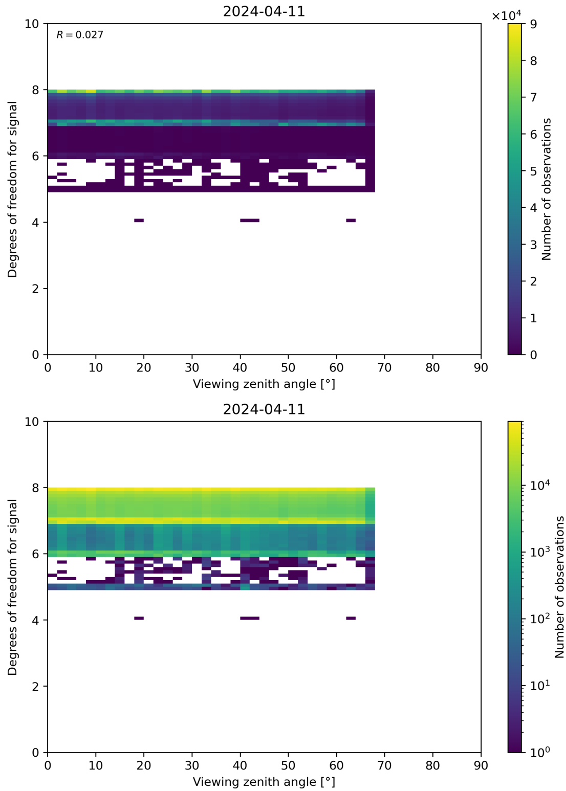
Figure 73: Scatter density plot of “Viewing zenith angle” against “Degrees of freedom for signal” for 2024-04-10 to 2024-04-12.
