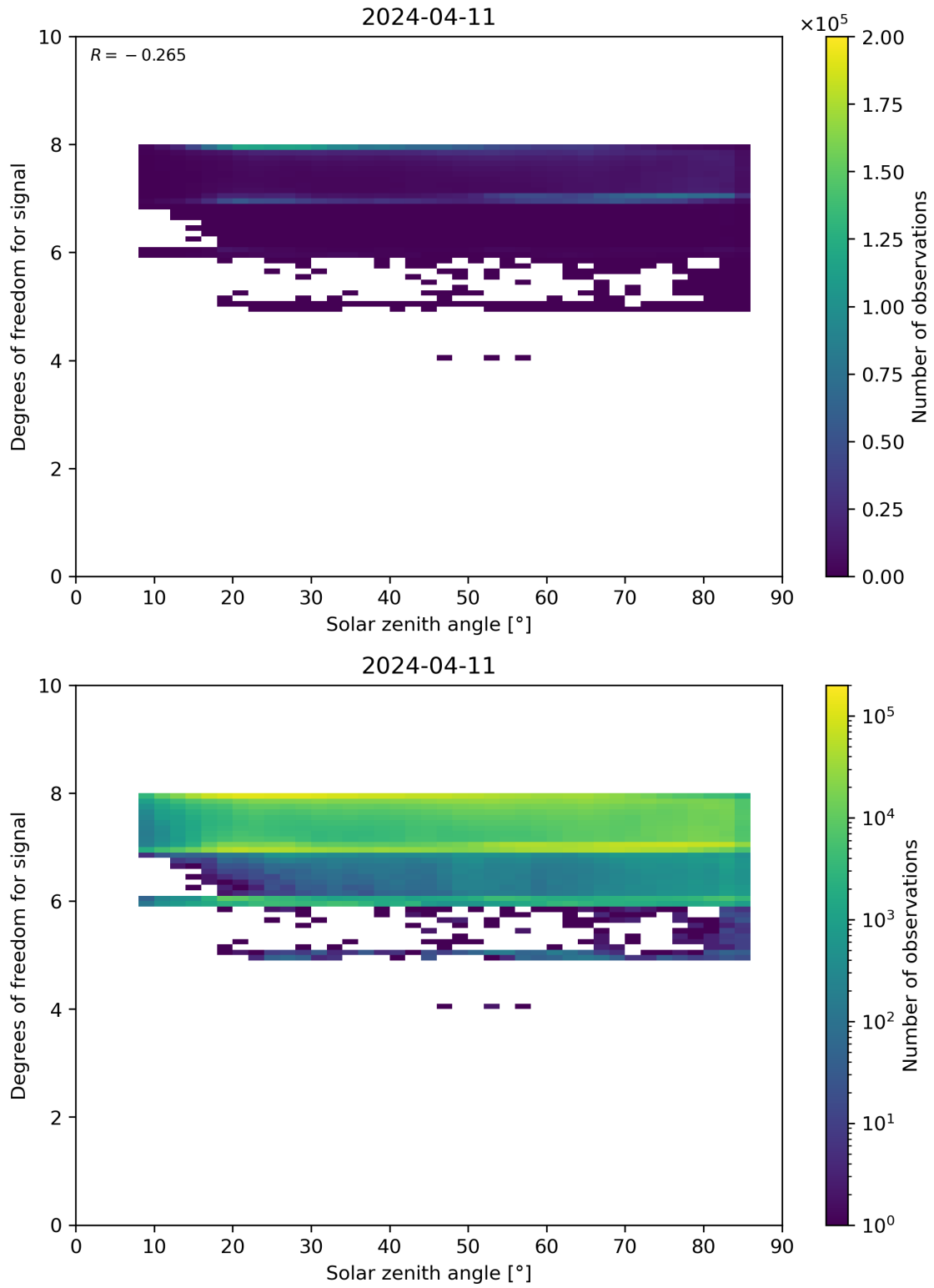
Figure 65: Scatter density plot of “Solar zenith angle” against “Degrees of freedom for signal” for 2024-04-10 to 2024-04-12.
