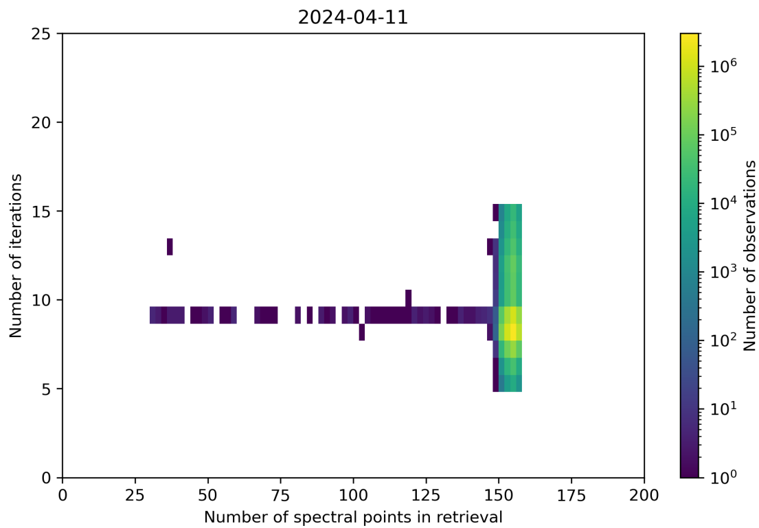
Figure 60: Scatter density plot of “Number of spectral points in retrieval” against “Number of iterations” for 2024-04-10 to 2024-04-12.
