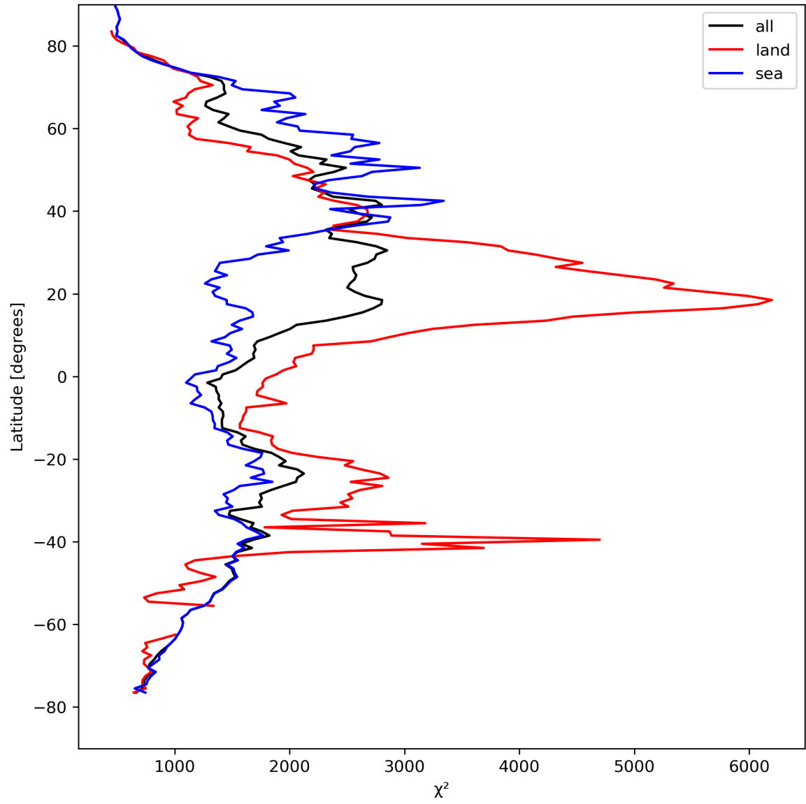
Figure 14: Zonal average of “ \chi^2 ” for 2024-04-10 to 2024-04-12.
