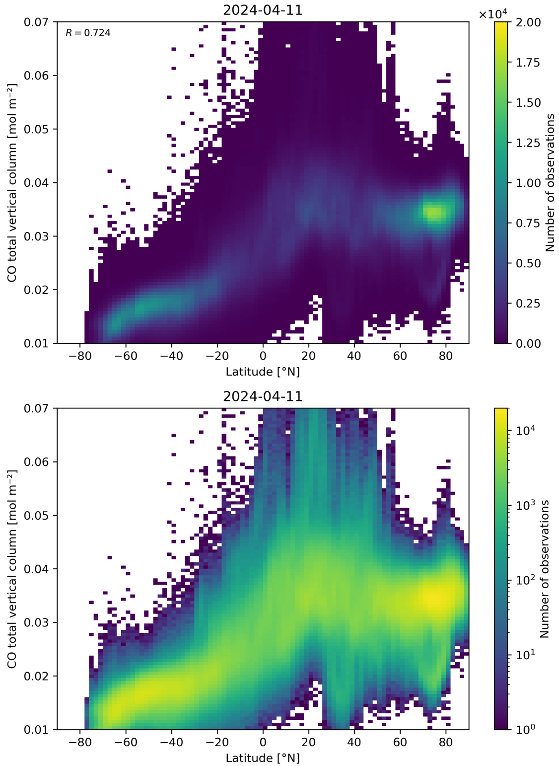
Figure 51: Scatter density plot of “Latitude” against “CO total vertical column” for 2024-04-10 to 2024-04-12.
