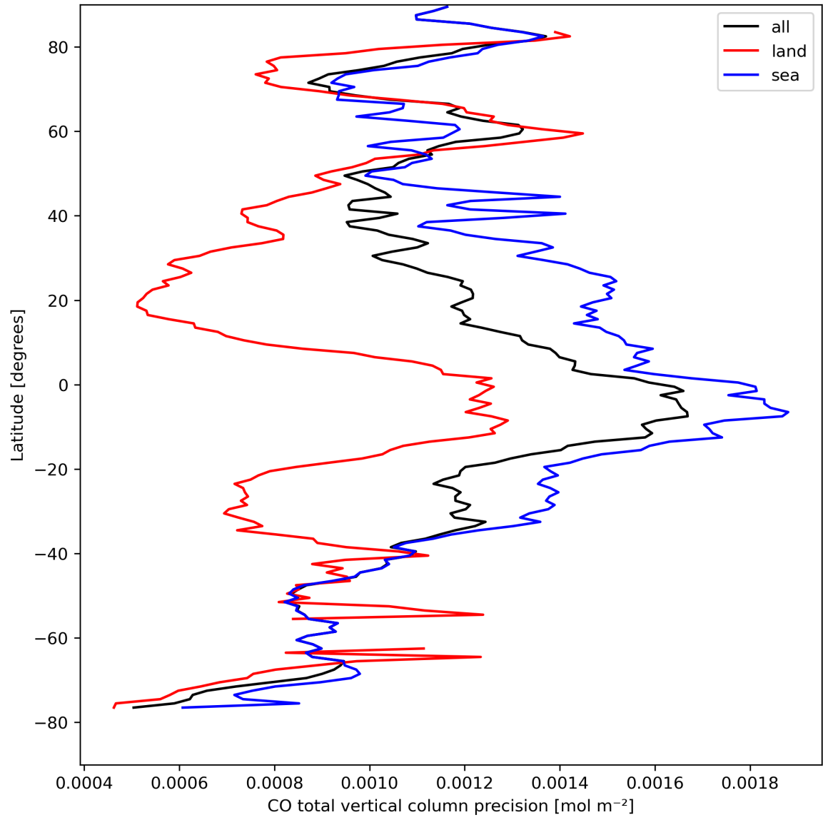
Figure 12: Zonal average of "CO total vertical column precision" for 2024-04-10 to 2024-04-12.
