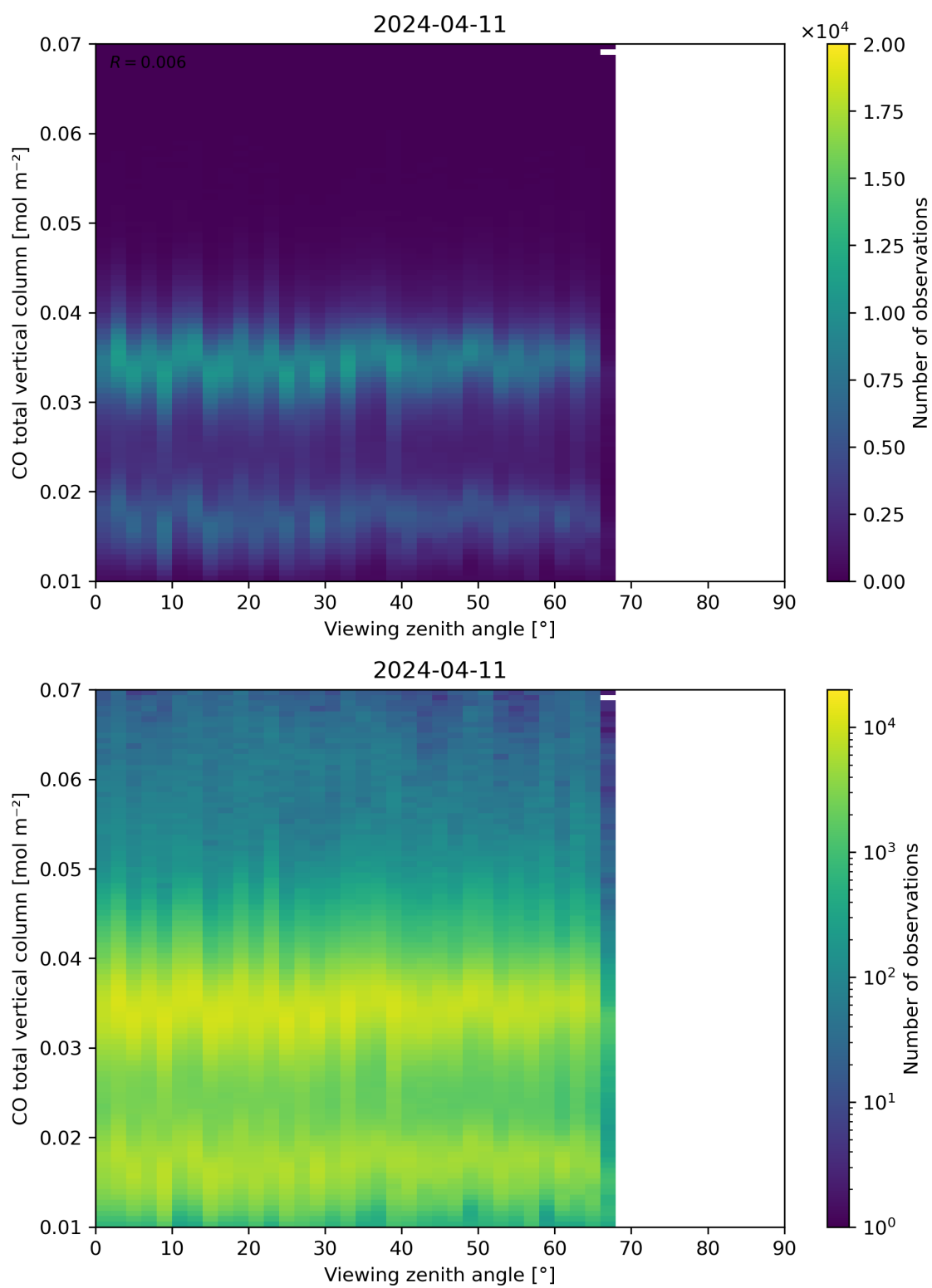
Figure 69: Scatter density plot of “Viewing zenith angle” against “CO total vertical column” for 2024-04-10 to 2024-04-12.
