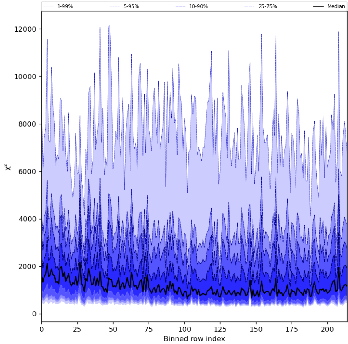
Figure 30: Along track statistics of “ \chi^2 ” for 2024-04-10 to 2024-04-12
