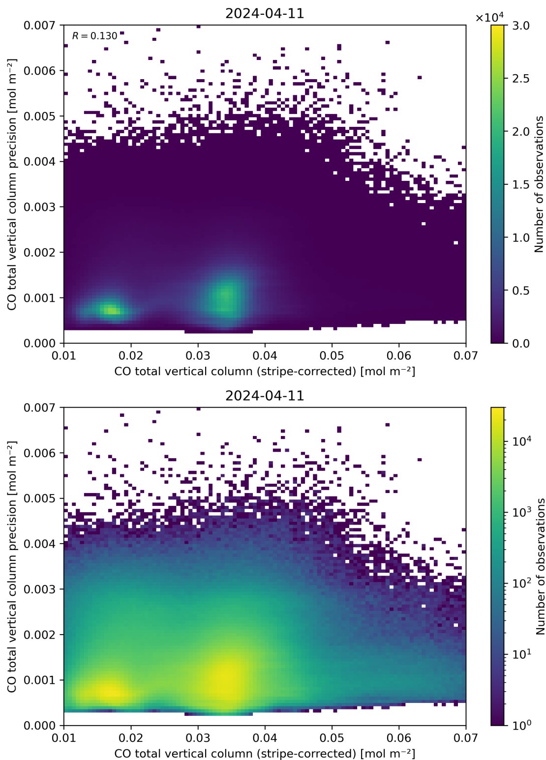
Figure 36: Scatter density plot of “CO total vertical column (stripe-corrected)” against “CO total vertical column precision” for 2024-04-10 to 2024-04-12.
