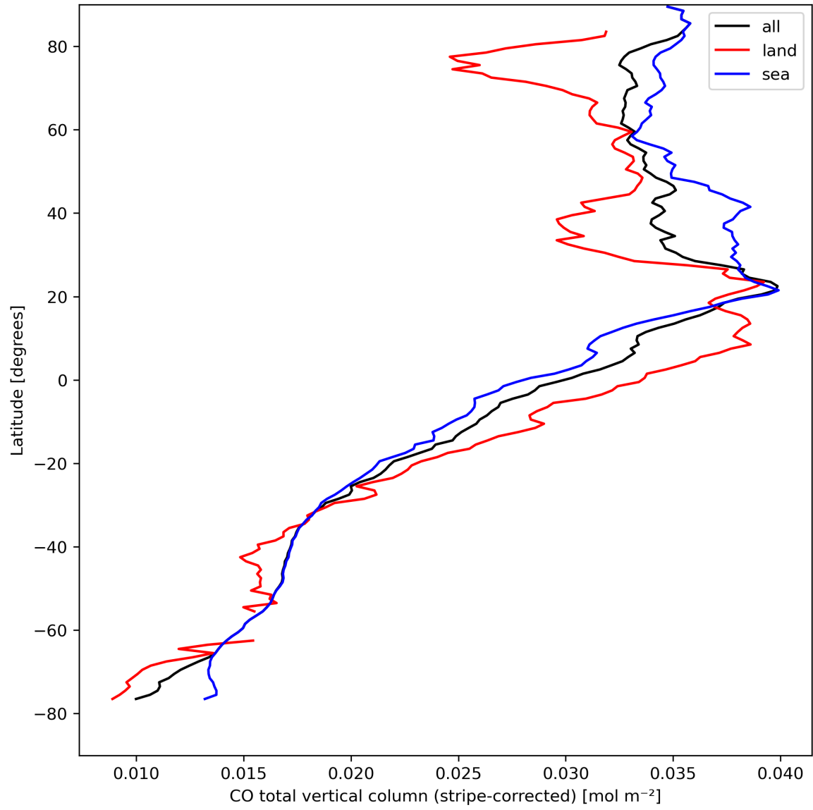
Figure 11: Zonal average of “CO total vertical column (stripe-corrected)” for 2024-04-10 to 2024-04-12.
