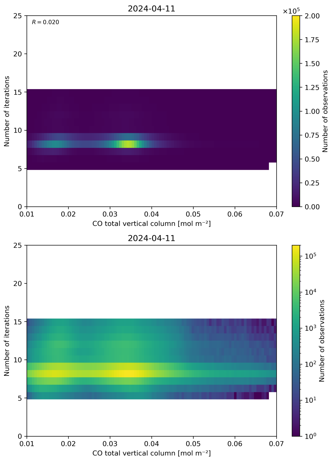
Figure 42: Scatter density plot of “CO total vertical column” against “Number of iterations” for 2024-04-10 to 2024-04-12.
