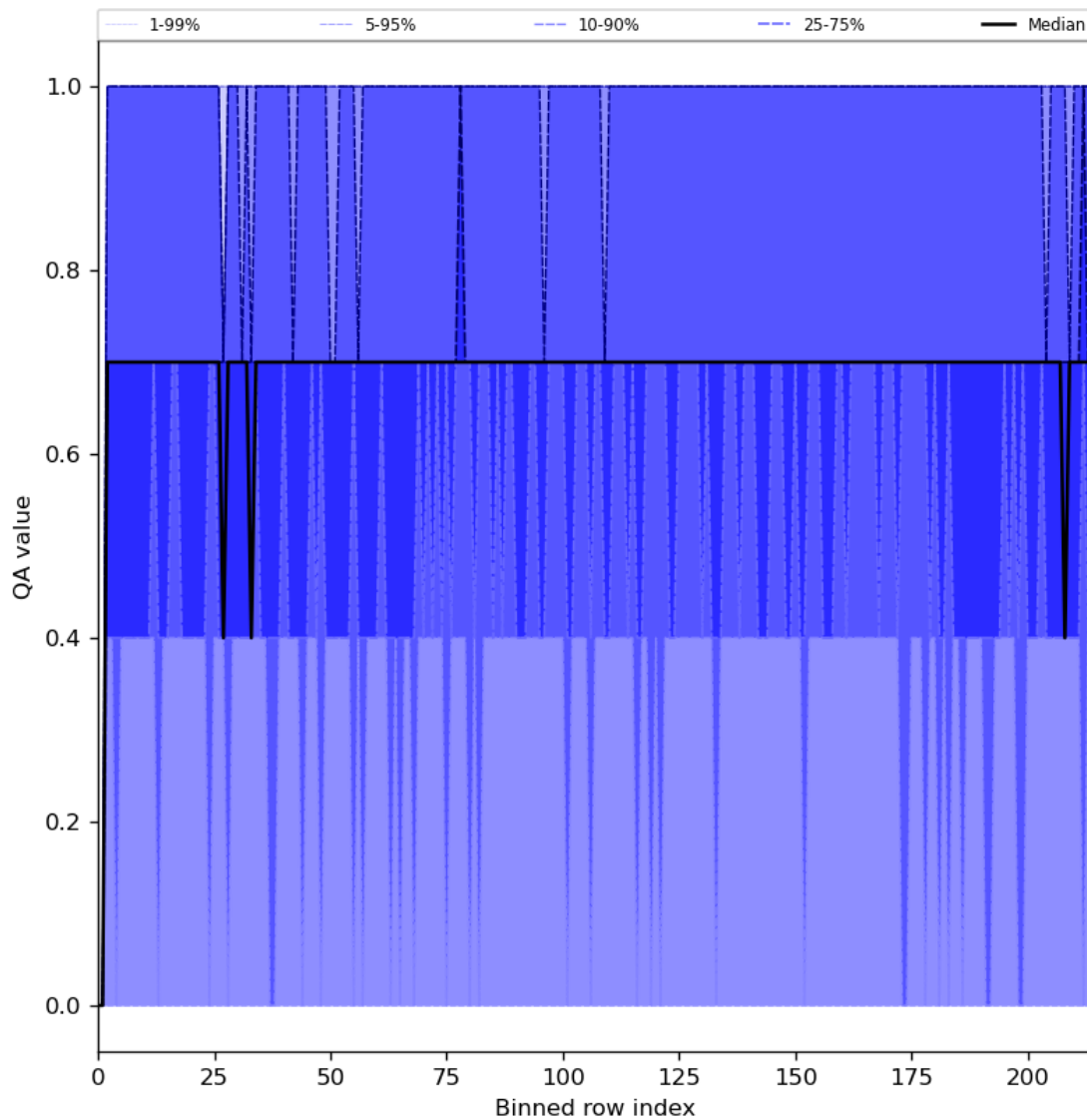
Figure 25: Along track statistics of “QA value” for 2024-04-10 to 2024-04-12
