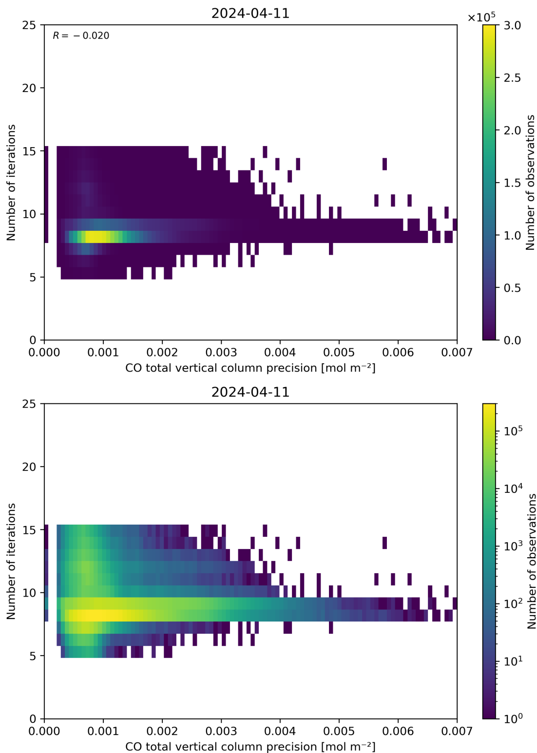
Figure 46: Scatter density plot of “CO total vertical column precision” against “Number of iterations” for 2024-04-10 to 2024-04-12.
