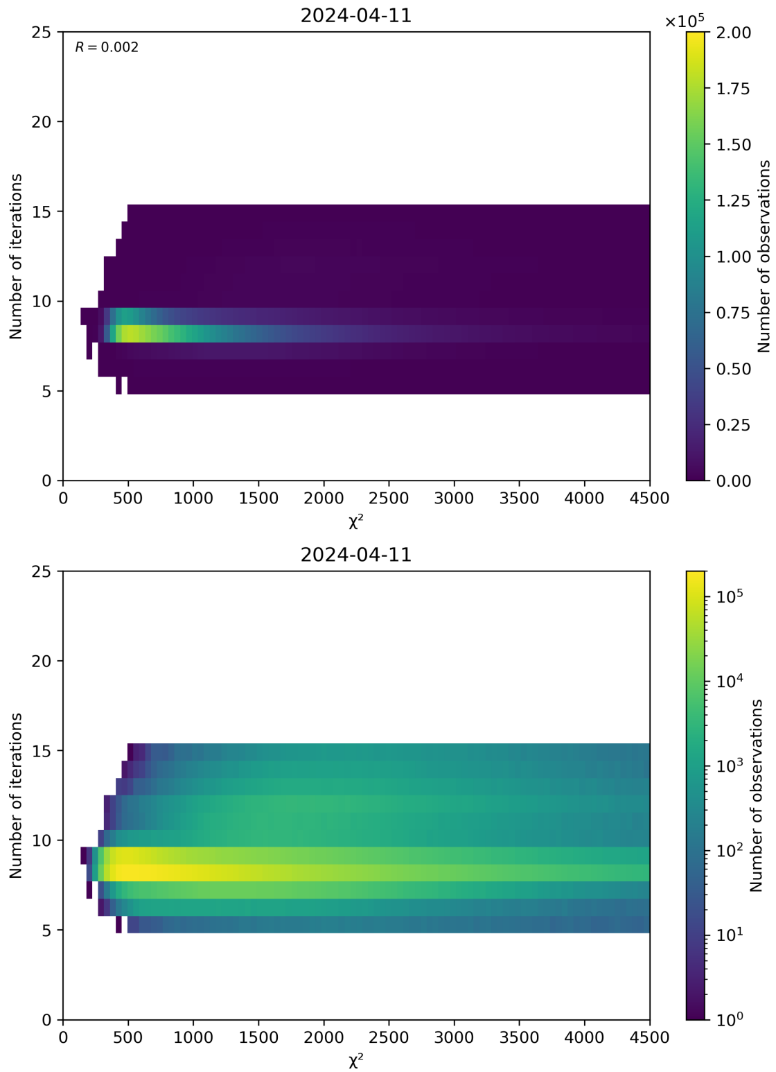
Figure 49: Scatter density plot of “ \chi^2 ” against “Number of iterations” for 2024-04-10 to 2024-04-12.
