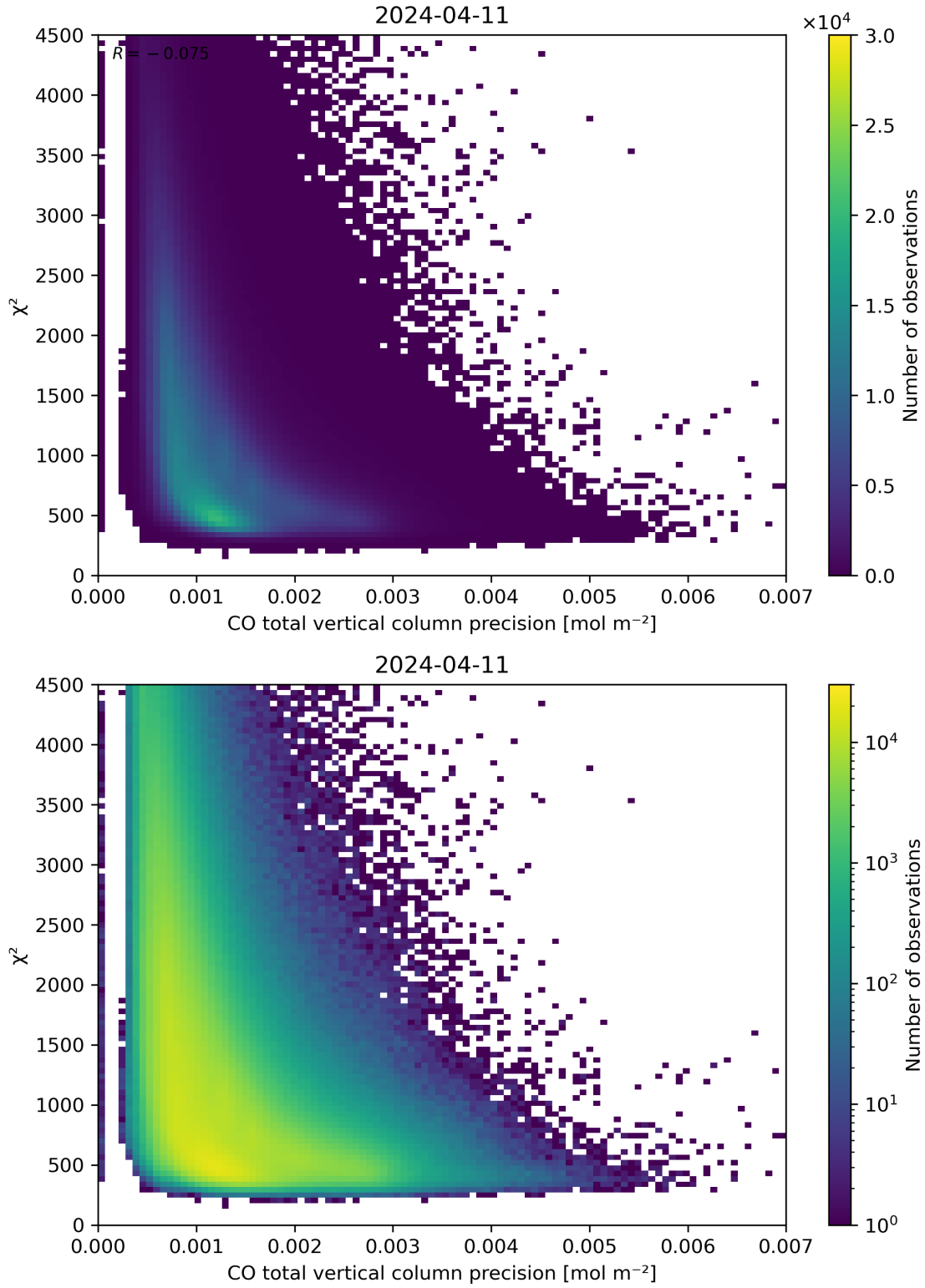
Figure 44: Scatter density plot of “CO total vertical column precision” against “ \chi^2 ” for 2024-04-10 to 2024-04-12.
