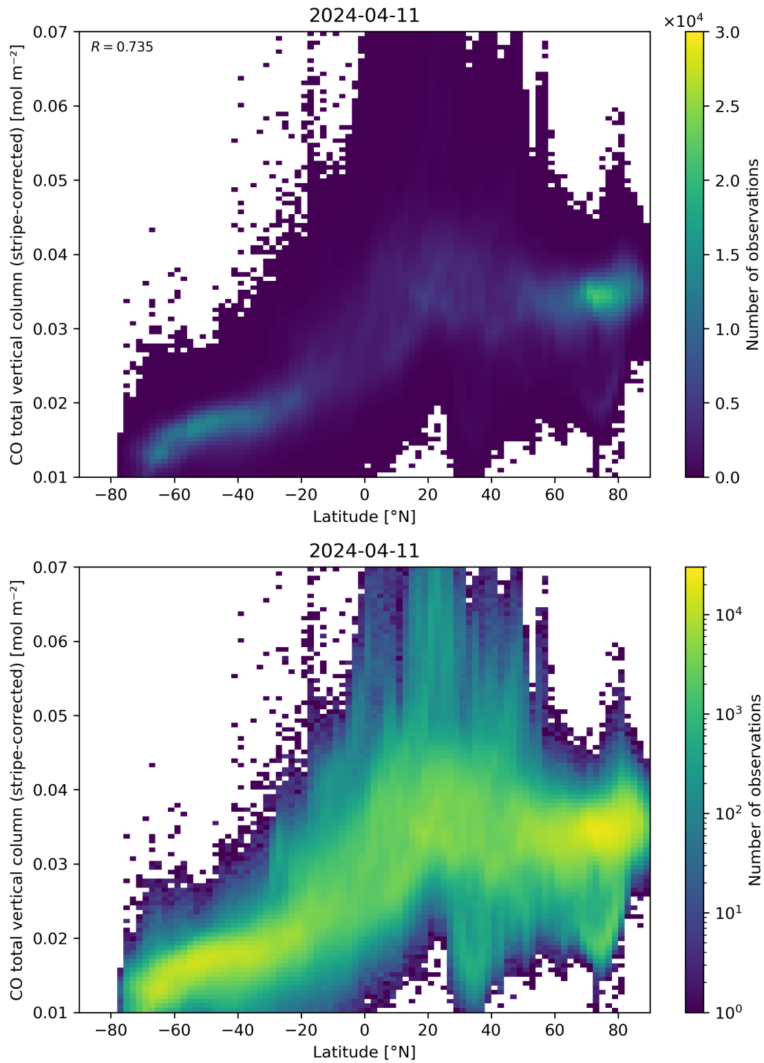
Figure 52: Scatter density plot of “Latitude” against “CO total vertical column (stripe-corrected)” for 2024-04-10 to 2024-04-12.
