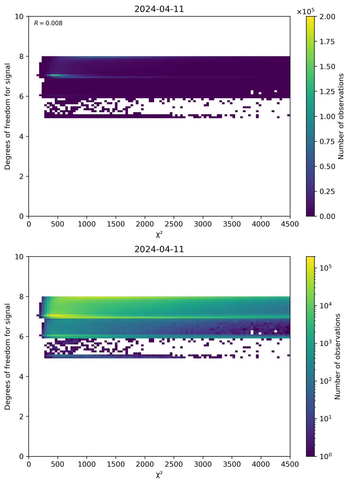
Figure 48: Scatter density plot of “ \chi^2 ” against “Degrees of freedom for signal” for 2024-04-10 to 2024-04-12.
