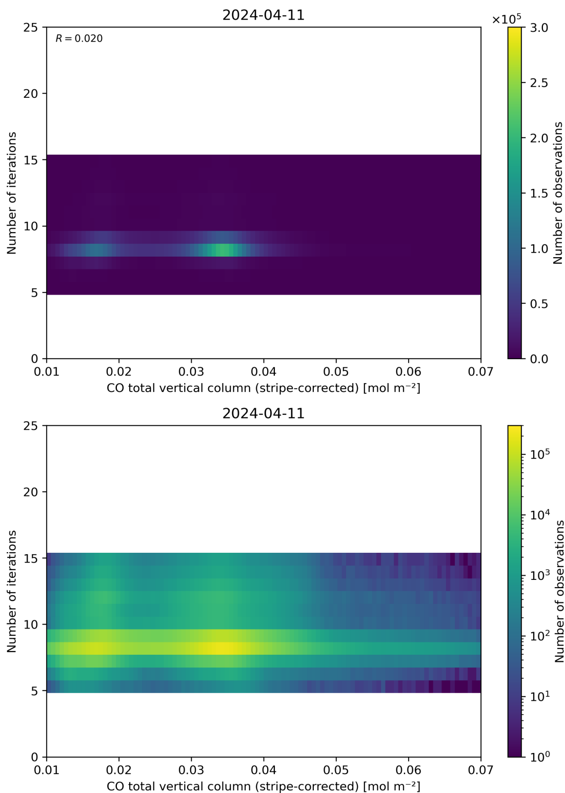
Figure 39: Scatter density plot of “CO total vertical column (stripe-corrected)” against “Number of iterations” for 2024-04-10 to 2024-04-12.
