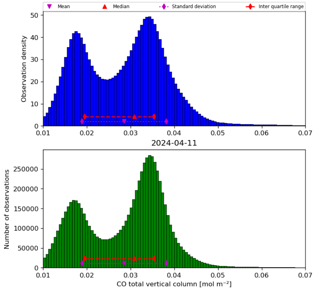
Figure 18: Histogram of “CO total vertical column” for 2024-04-10 to 2024-04-12
