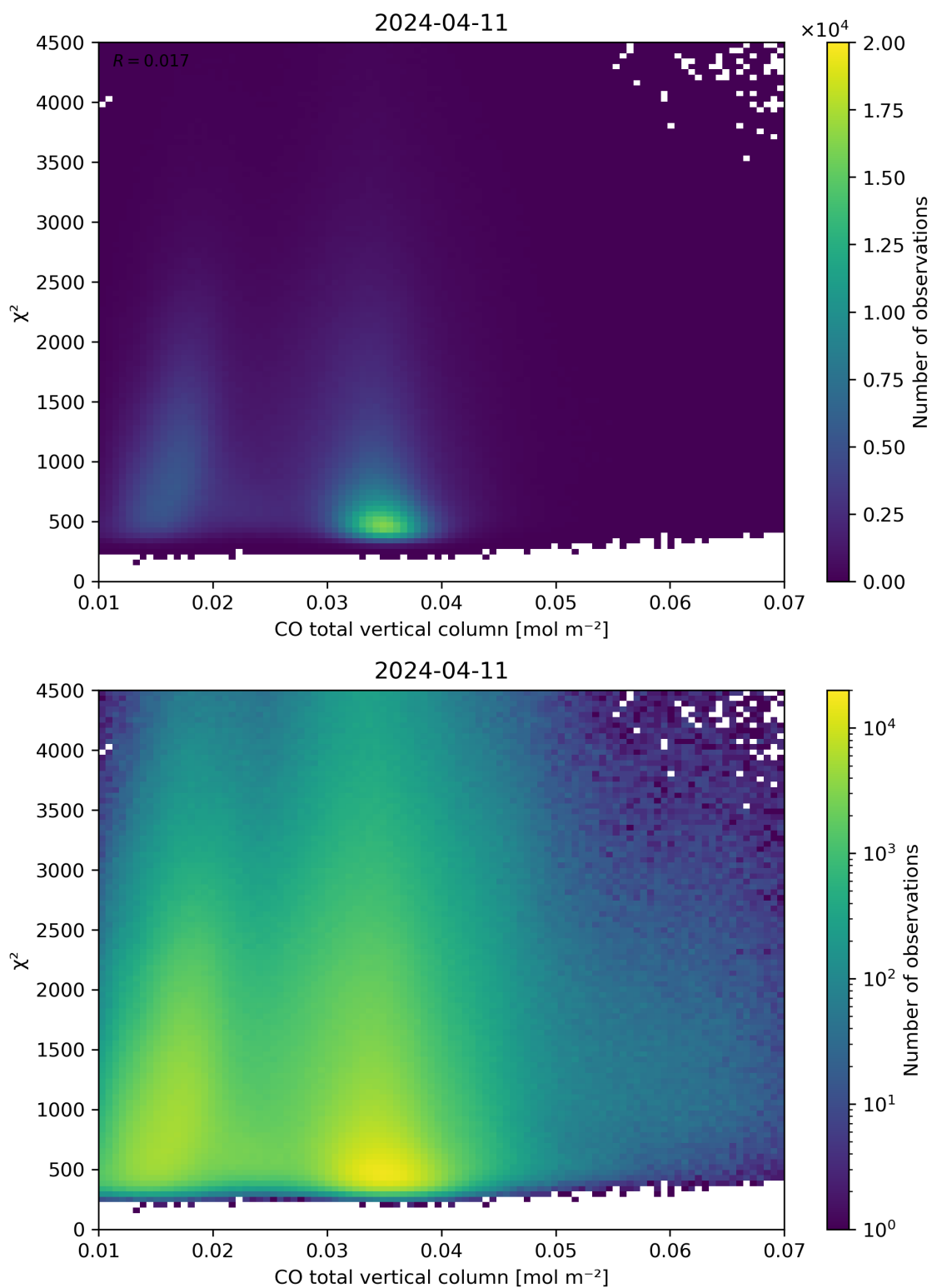
Figure 35: Scatter density plot of “CO total vertical column” against “ \chi^2 ” for 2024-04-10 to 2024-04-12.
