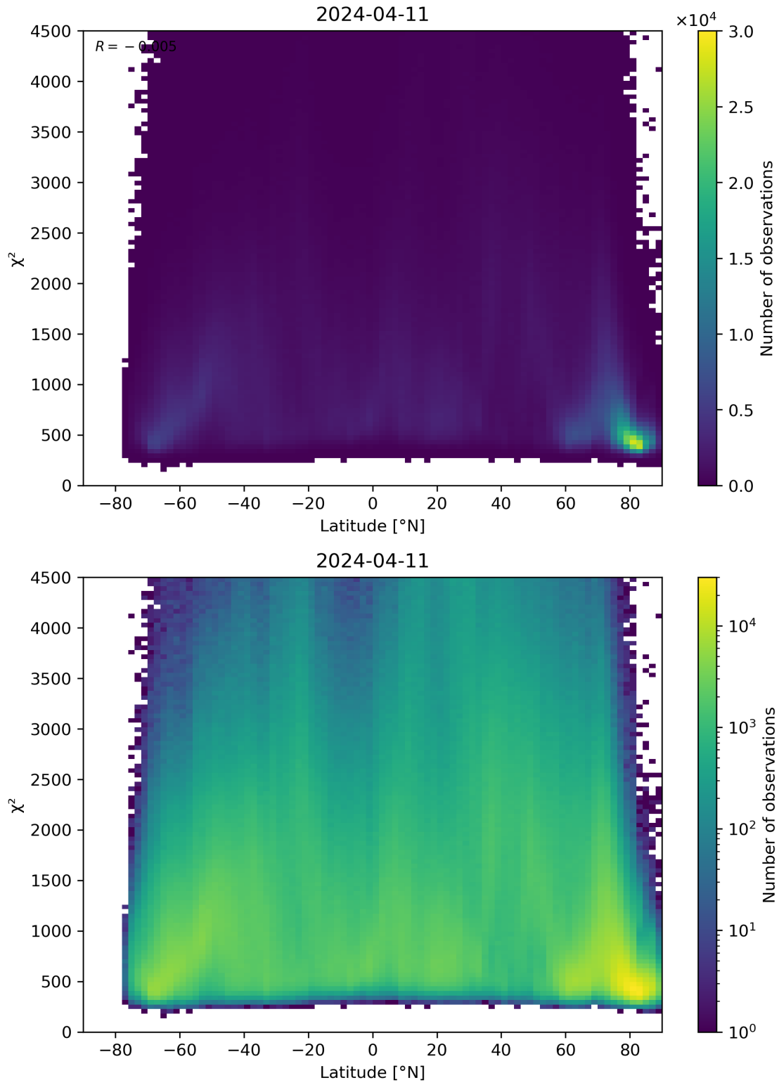
Figure 54: Scatter density plot of “Latitude” against “ \chi^2 ” for 2024-04-10 to 2024-04-12.
