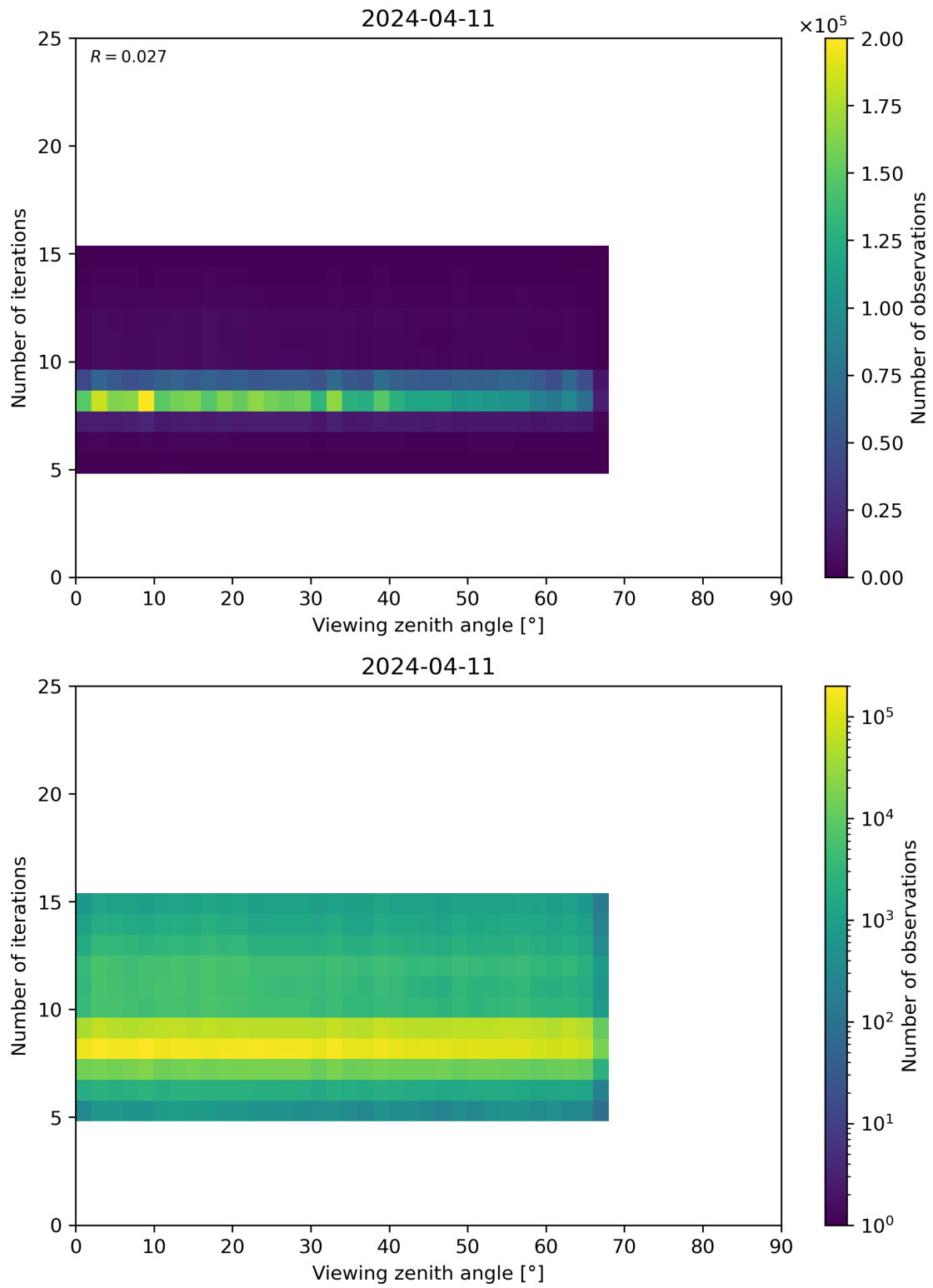
Figure 75: Scatter density plot of “Viewing zenith angle” against “Number of iterations” for 2024-04-10 to 2024-04-12.
