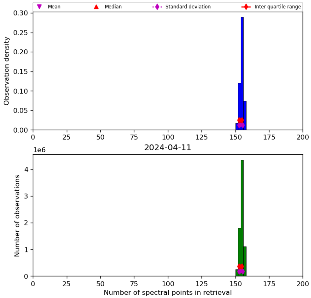
Figure 21: Histogram of “Number of spectral points in retrieval” for 2024-04-10 to 2024-04-12
