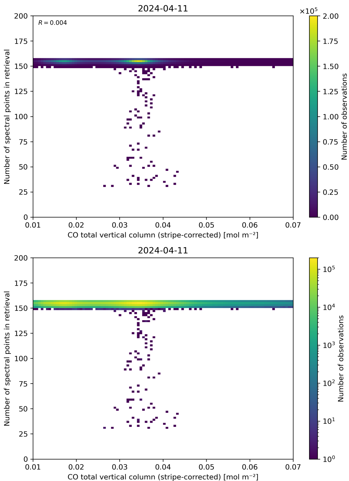
Figure 40: Scatter density plot of “CO total vertical column (stripe-corrected)” against “Number of spectral points in retrieval” for 2024-04-10 to 2024-04-12.
