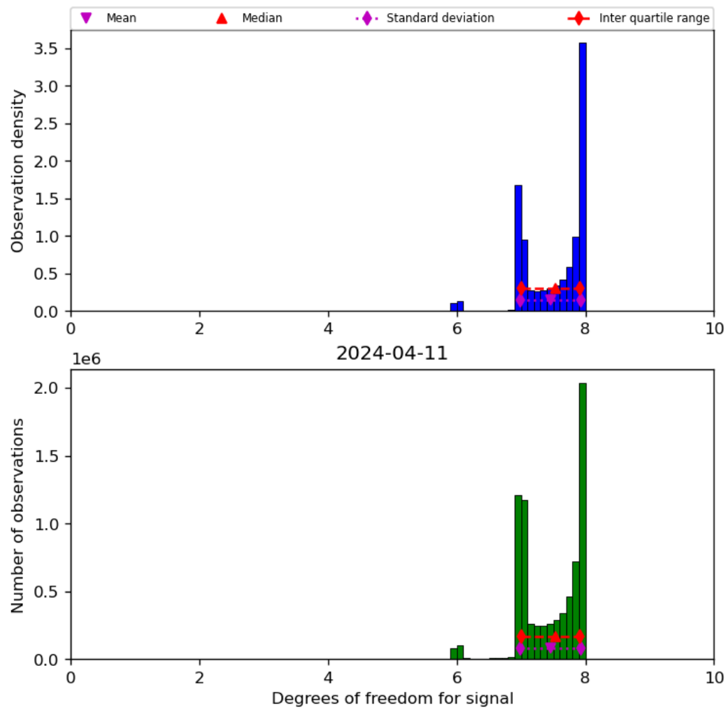
Figure 23: Histogram of “Degrees of freedom for signal” for 2024-04-10 to 2024-04-12
