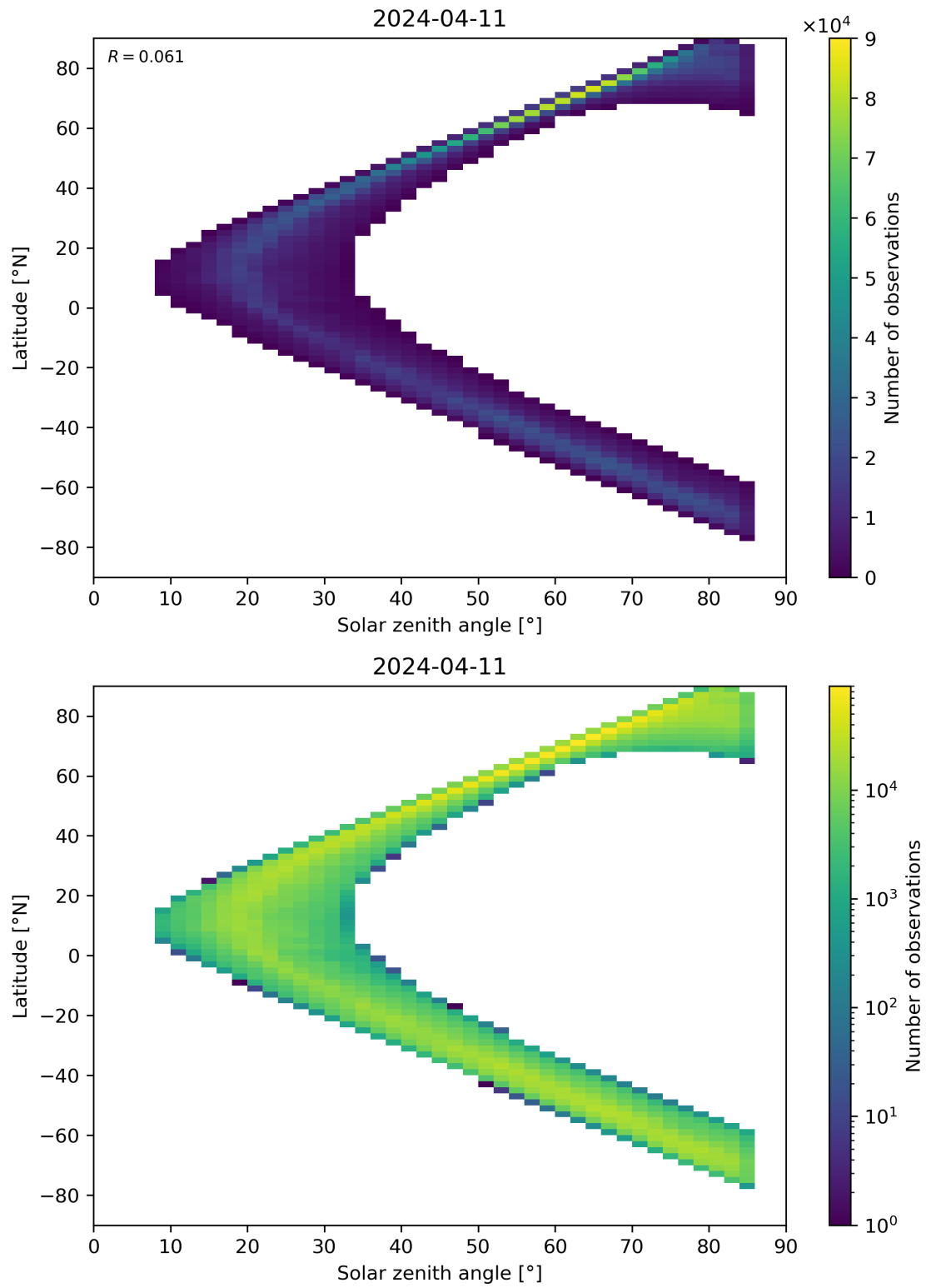
Figure 66: Scatter density plot of “Solar zenith angle” against “Latitude” for 2024-04-10 to 2024-04-12.
