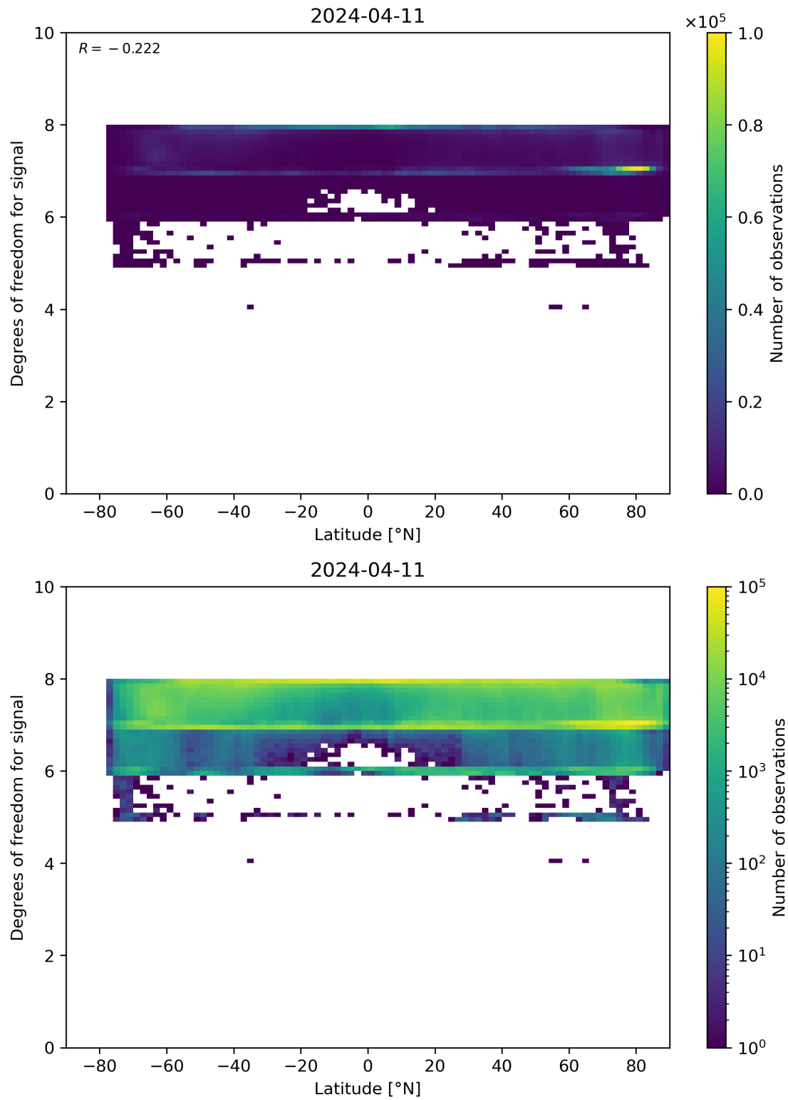
Figure 55: Scatter density plot of “Latitude” against “Degrees of freedom for signal” for 2024-04-10 to 2024-04-12.
