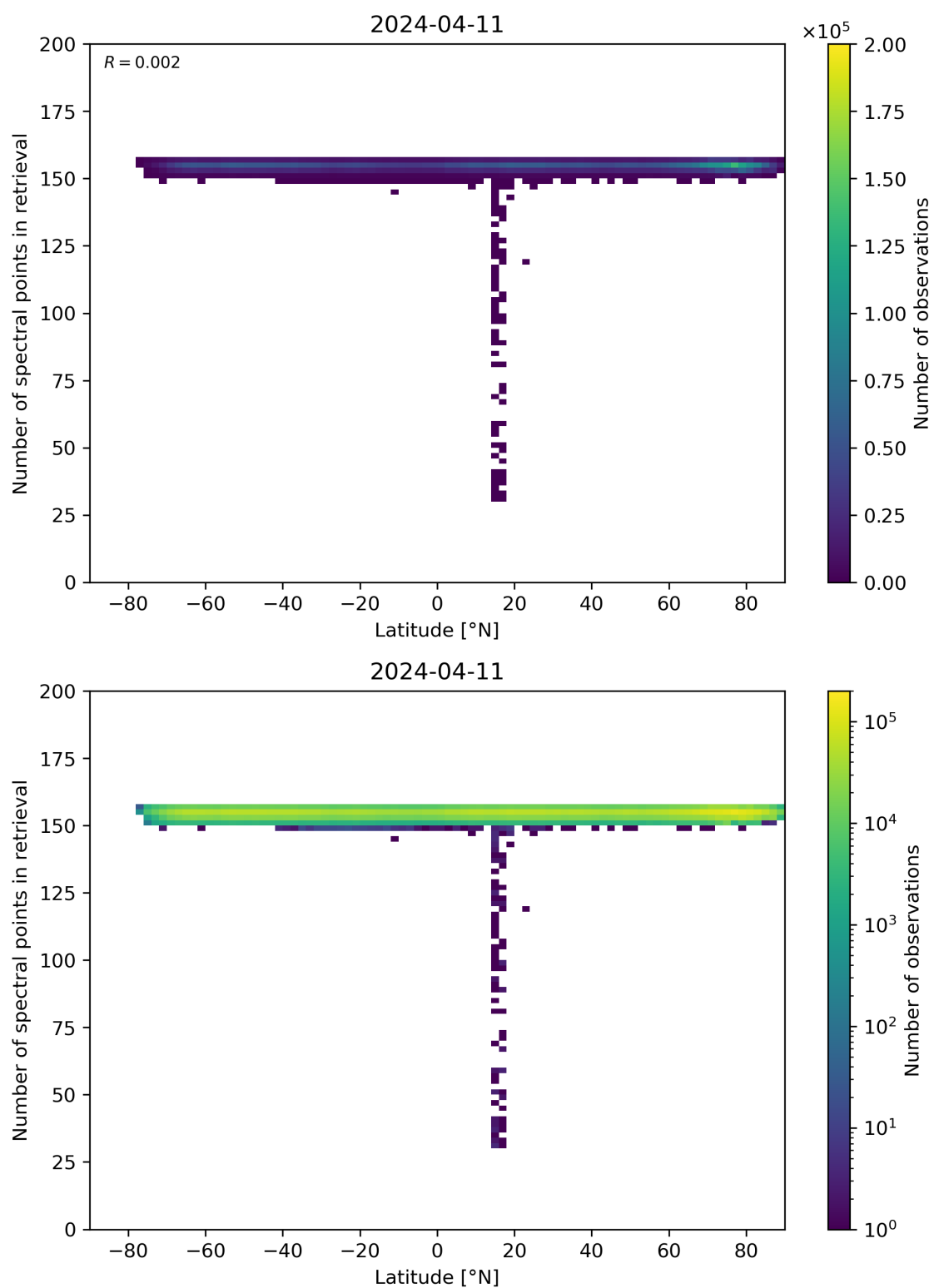
Figure 57: Scatter density plot of “Latitude” against “Number of spectral points in retrieval” for 2024-04-10 to 2024-04-12.
