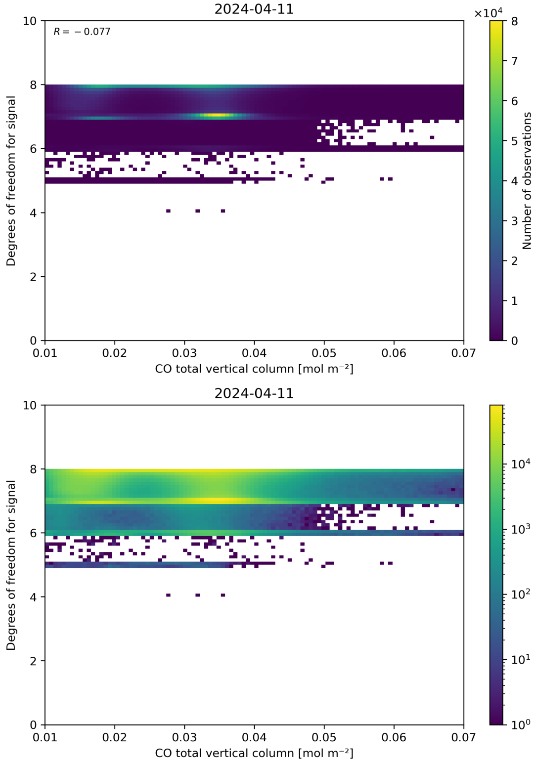
Figure 41: Scatter density plot of “CO total vertical column” against “Degrees of freedom for signal” for 2024-04-10 to 2024-04-12.
