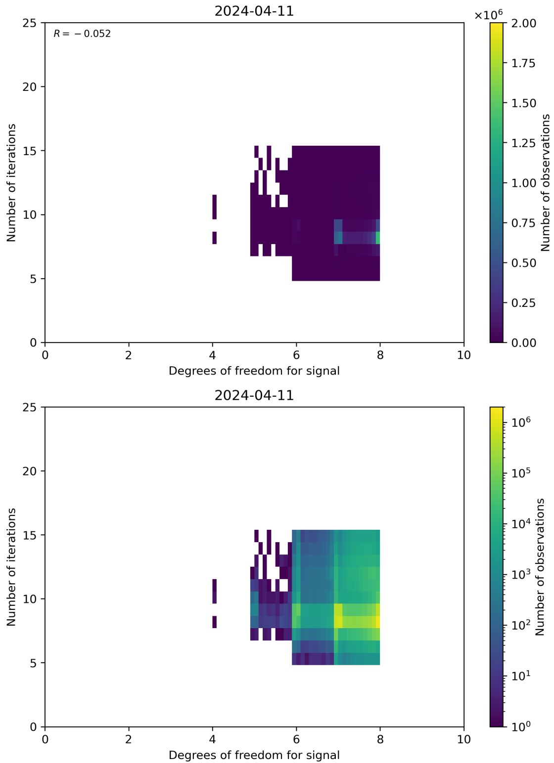
Figure 50: Scatter density plot of “Degrees of freedom for signal” against “Number of iterations” for 2024-04-10 to 2024-04-12.
