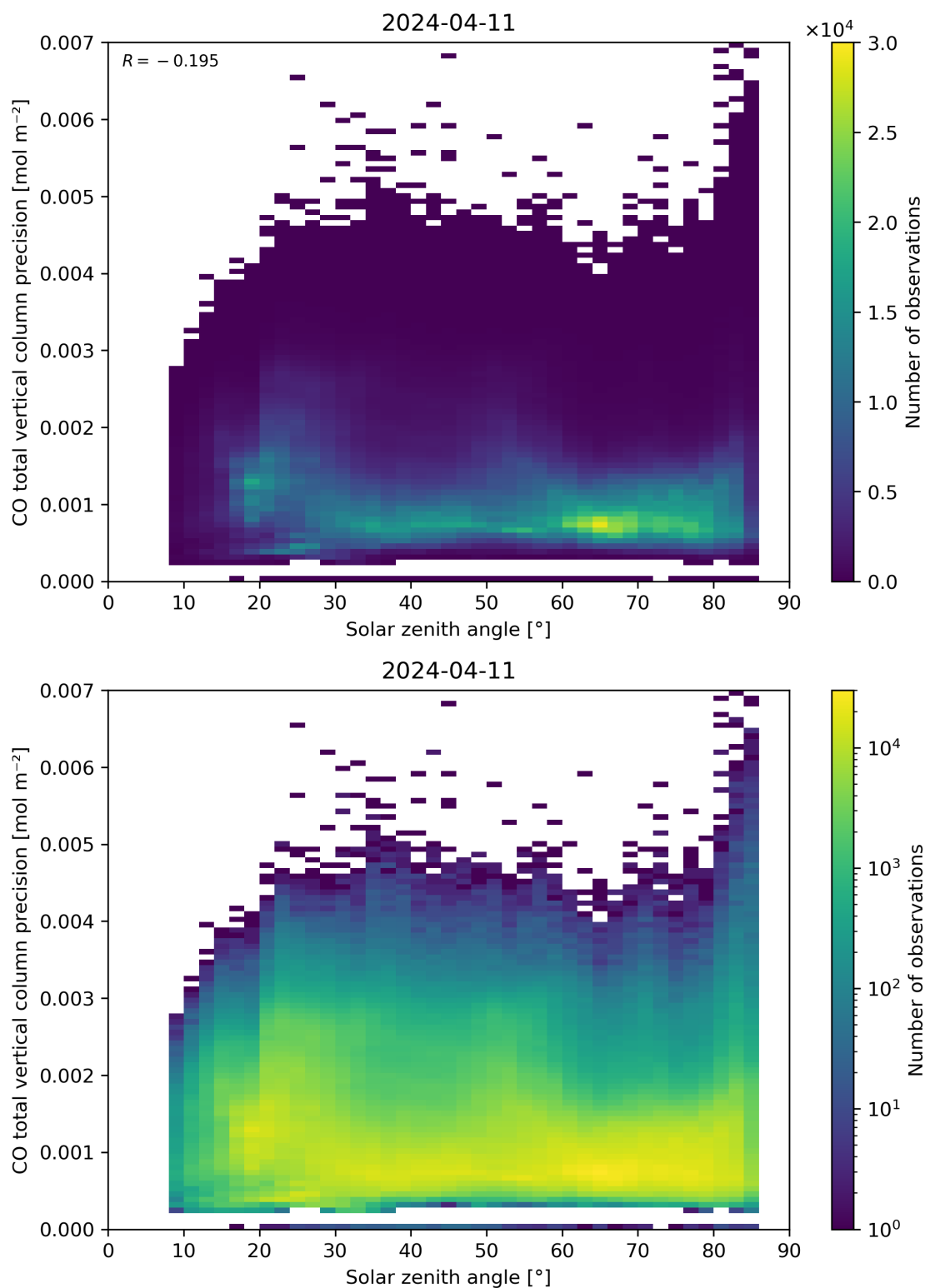
Figure 63: Scatter density plot of “Solar zenith angle” against “CO total vertical column precision” for 2024-04-10 to 2024-04-12.
