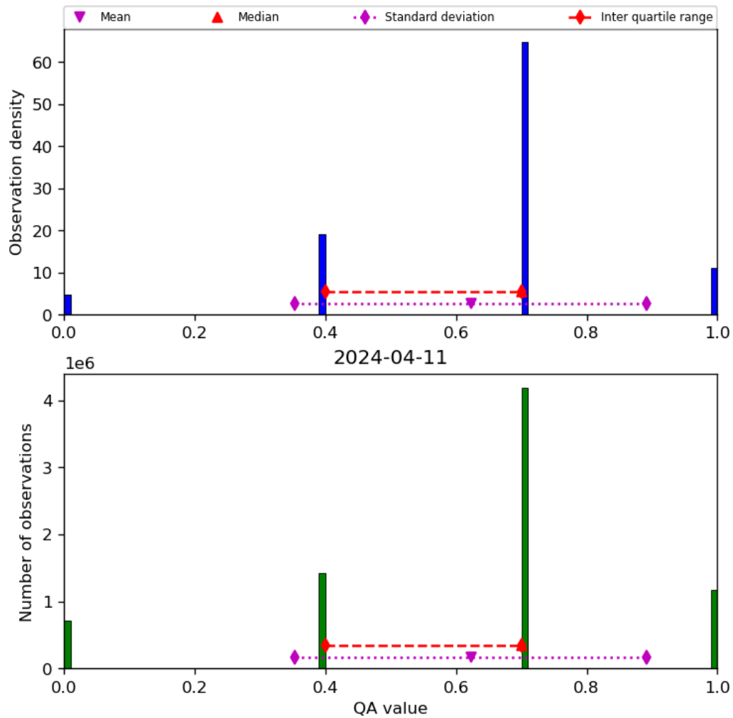
Figure 17: Histogram of “QA value” for 2024-04-10 to 2024-04-12
