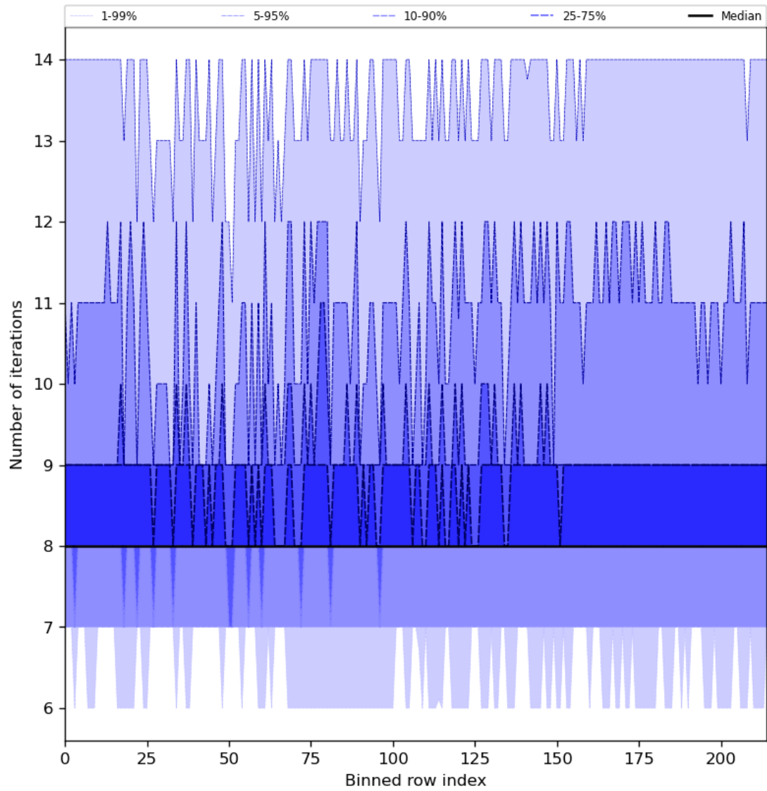
Figure 32: Along track statistics of “Number of iterations” for 2024-04-10 to 2024-04-12
