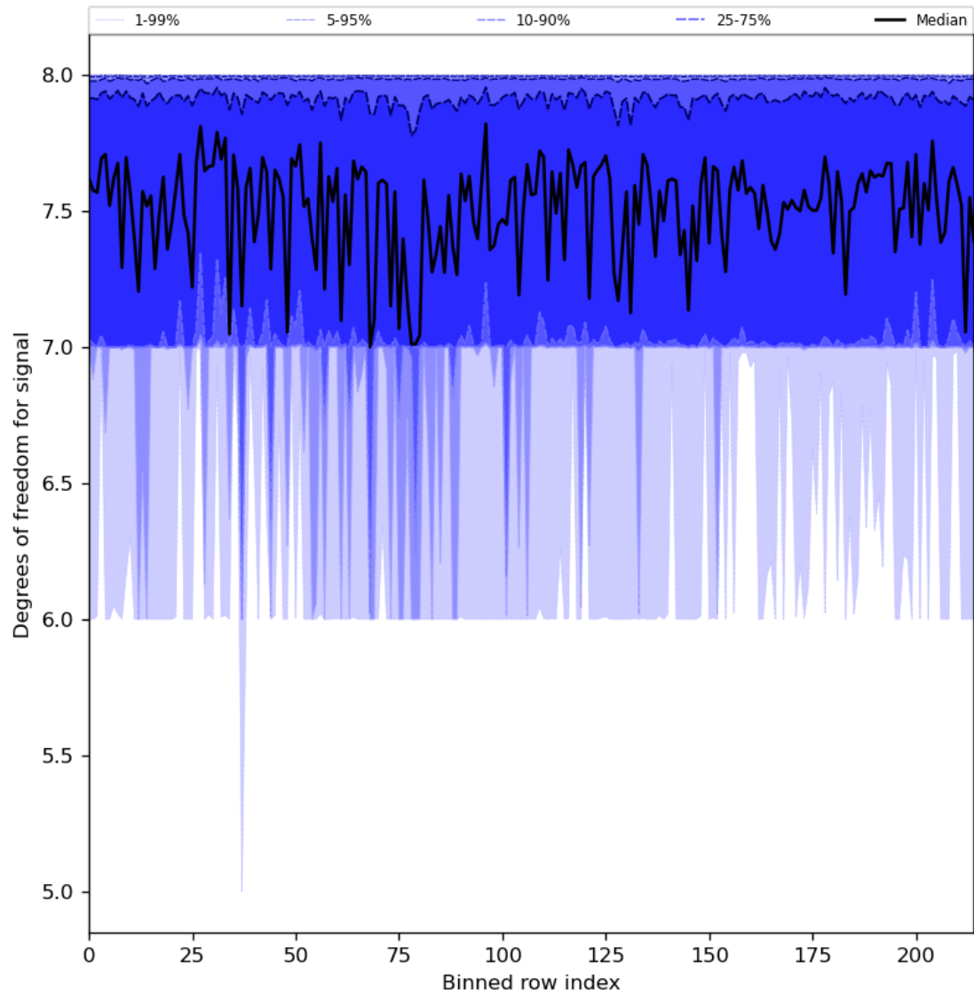
Figure 31: Along track statistics of “Degrees of freedom for signal” for 2024-04-10 to 2024-04-12
