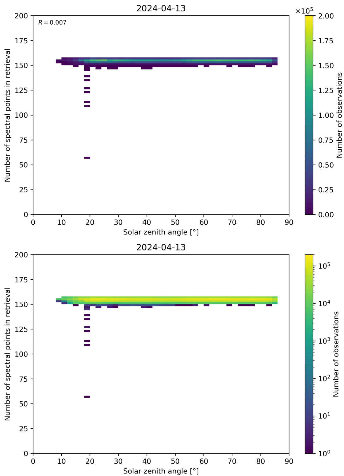
Figure 68: Scatter density plot of “Solar zenith angle” against “Number of spectral points in retrieval” for 2024-04-12 to 2024-04-14.
