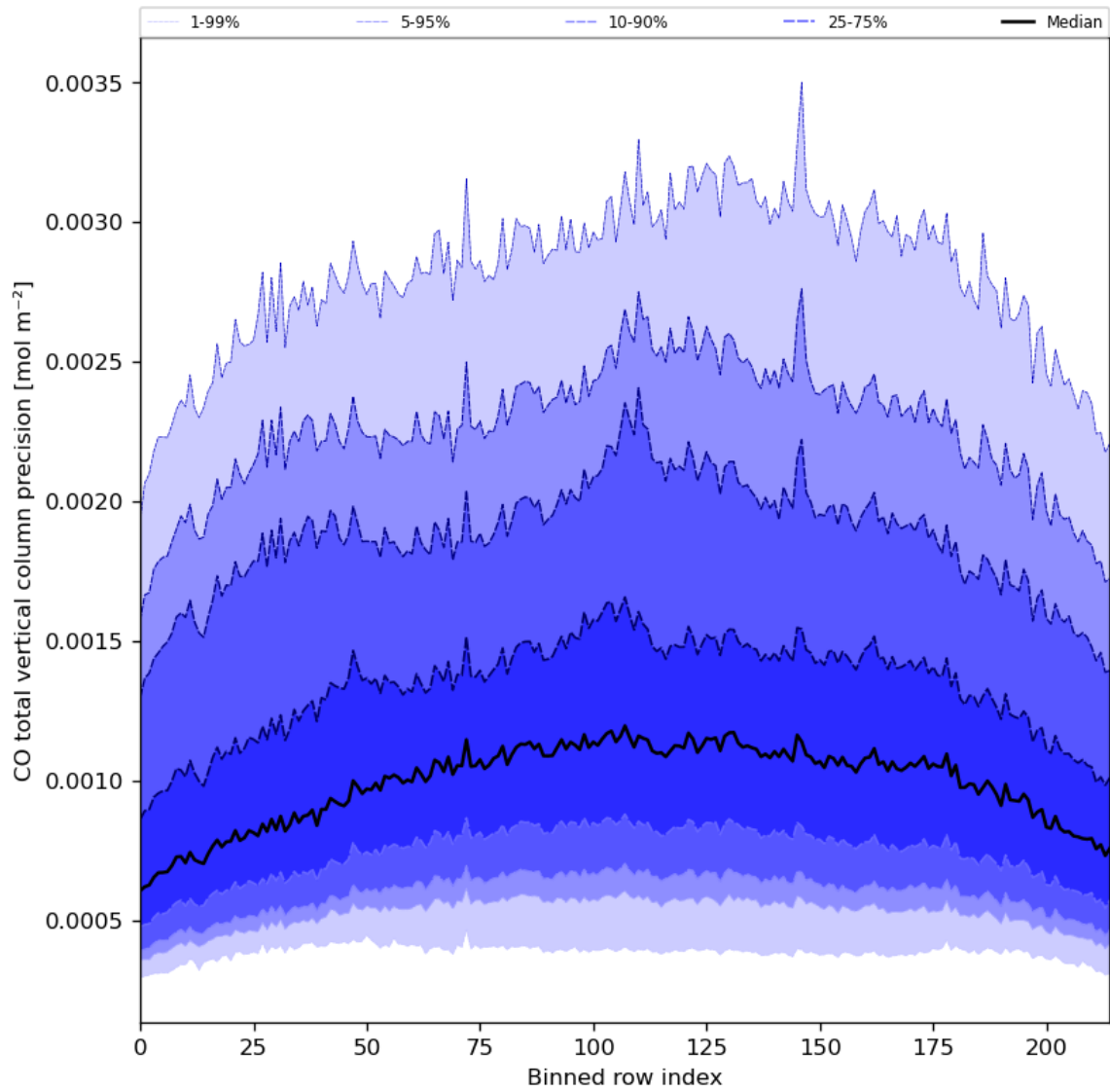
Figure 28: Along track statistics of “CO total vertical column precision” for 2024-04-12 to 2024-04-14
