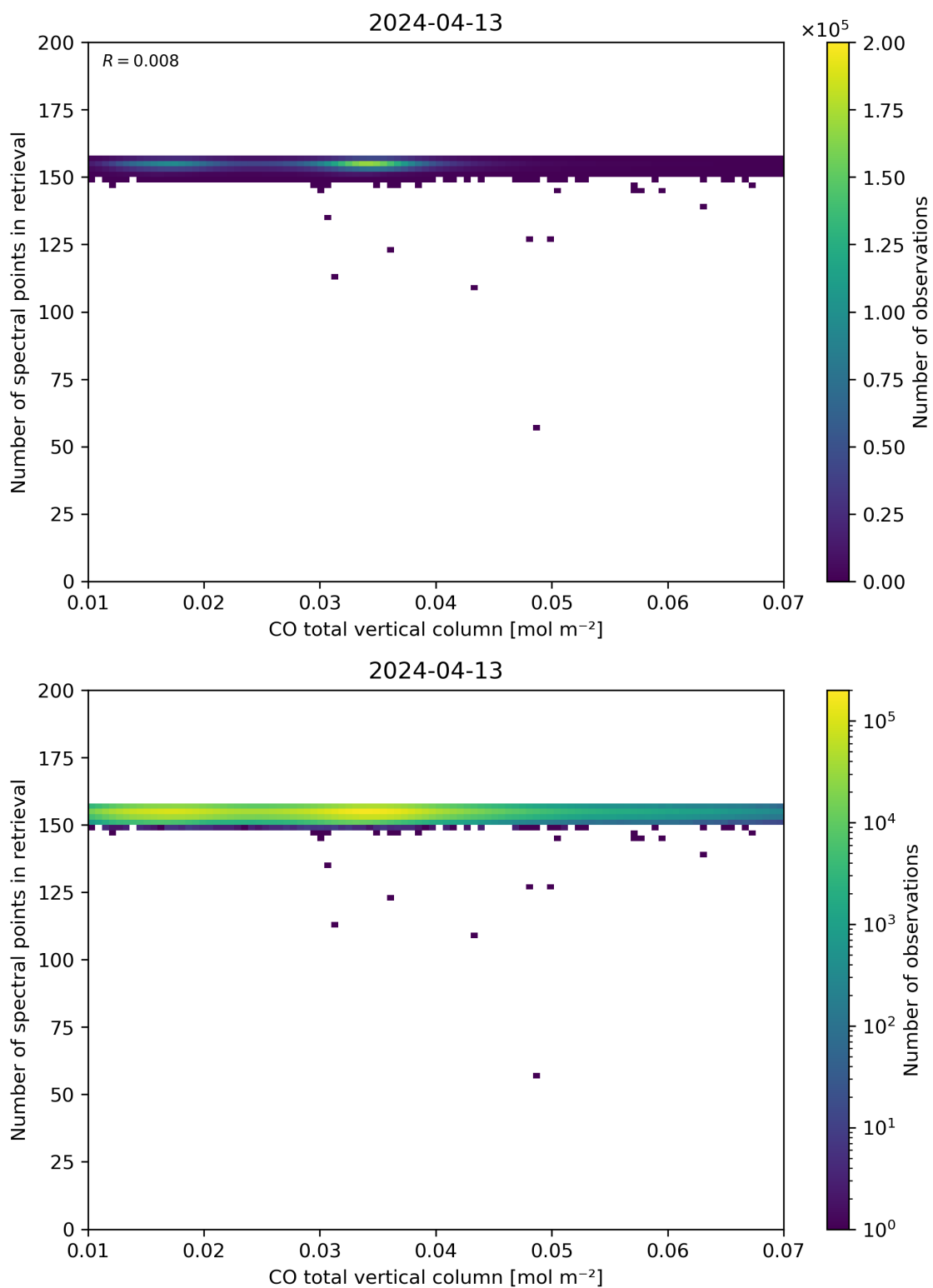
Figure 43: Scatter density plot of “CO total vertical column” against “Number of spectral points in retrieval” for 2024-04-12 to 2024-04-14.
