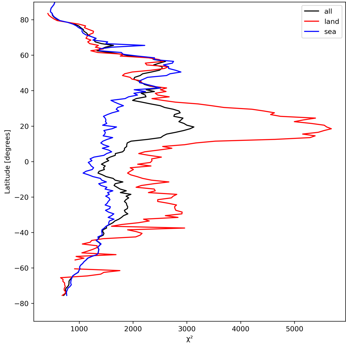
Figure 14: Zonal average of “ \chi^2 ” for 2024-04-12 to 2024-04-14.
