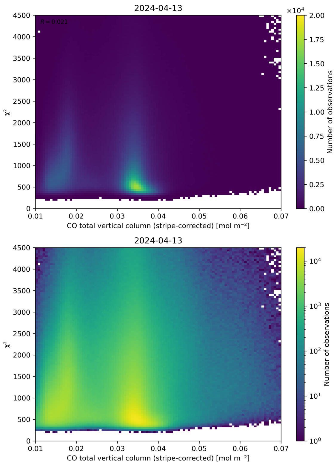
Figure 37: Scatter density plot of “CO total vertical column (stripe-corrected)” against “ \chi^2 ” for 2024-04-12 to 2024-04-14.
