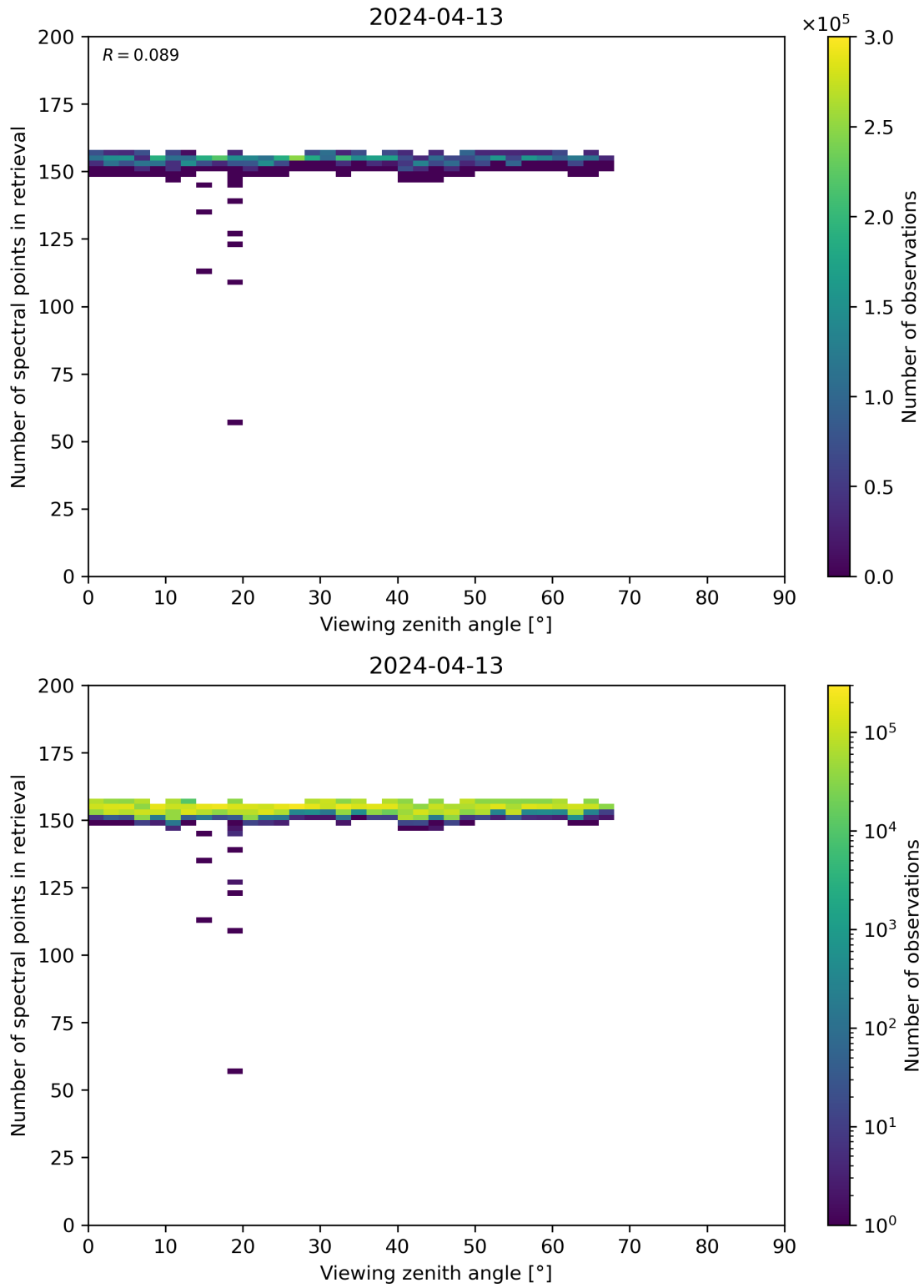
Figure 76: Scatter density plot of “Viewing zenith angle” against “Number of spectral points in retrieval” for 2024-04-12 to 2024-04-14.
