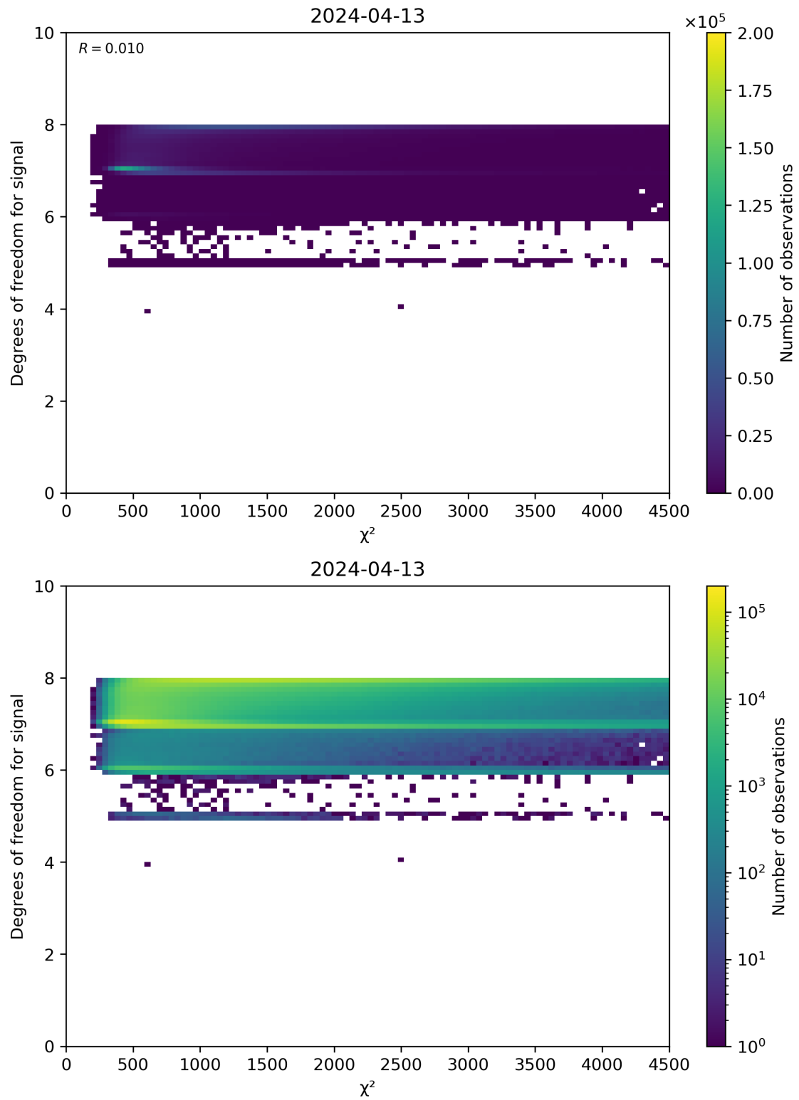
Figure 48: Scatter density plot of “ \chi^2 ” against “Degrees of freedom for signal” for 2024-04-12 to 2024-04-14.
