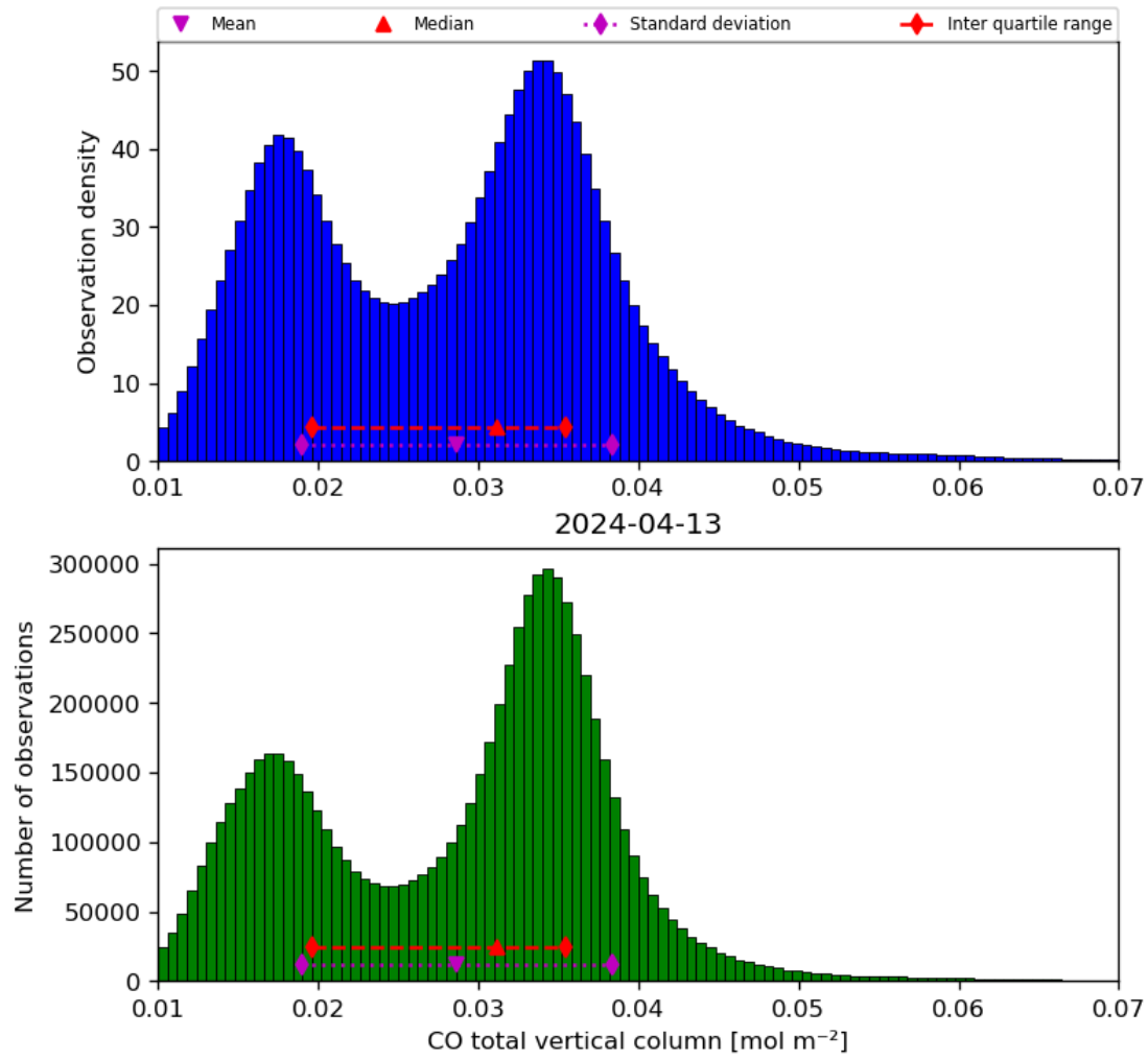
Figure 18: Histogram of “CO total vertical column” for 2024-04-12 to 2024-04-14
