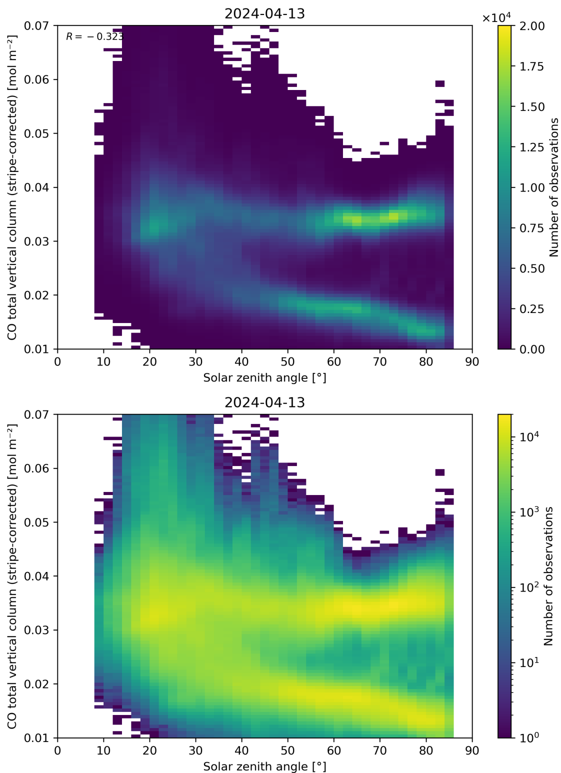
Figure 62: Scatter density plot of “Solar zenith angle” against “CO total vertical column (stripe-corrected)” for 2024-04-12 to 2024-04-14.
