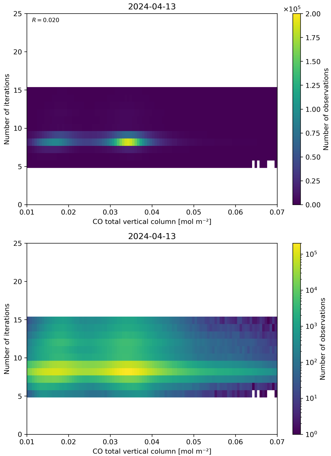
Figure 42: Scatter density plot of “CO total vertical column” against “Number of iterations” for 2024-04-12 to 2024-04-14.
