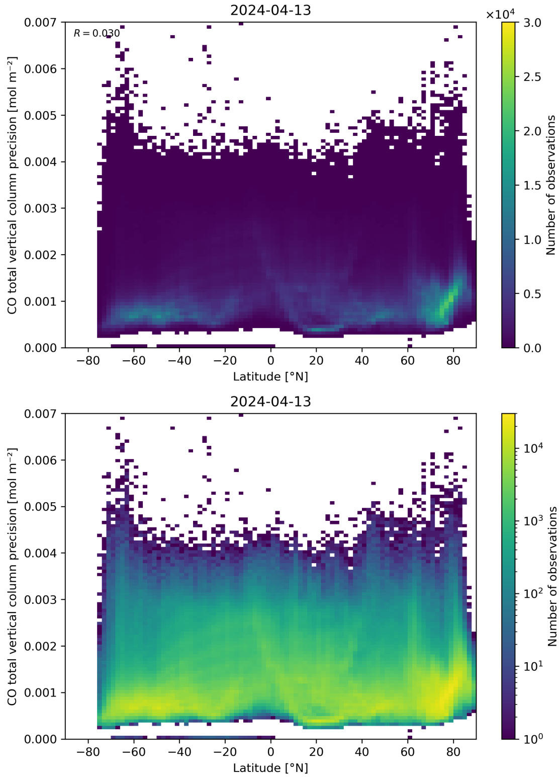
Figure 53: Scatter density plot of “Latitude” against “CO total vertical column precision” for 2024-04-12 to 2024-04-14.
