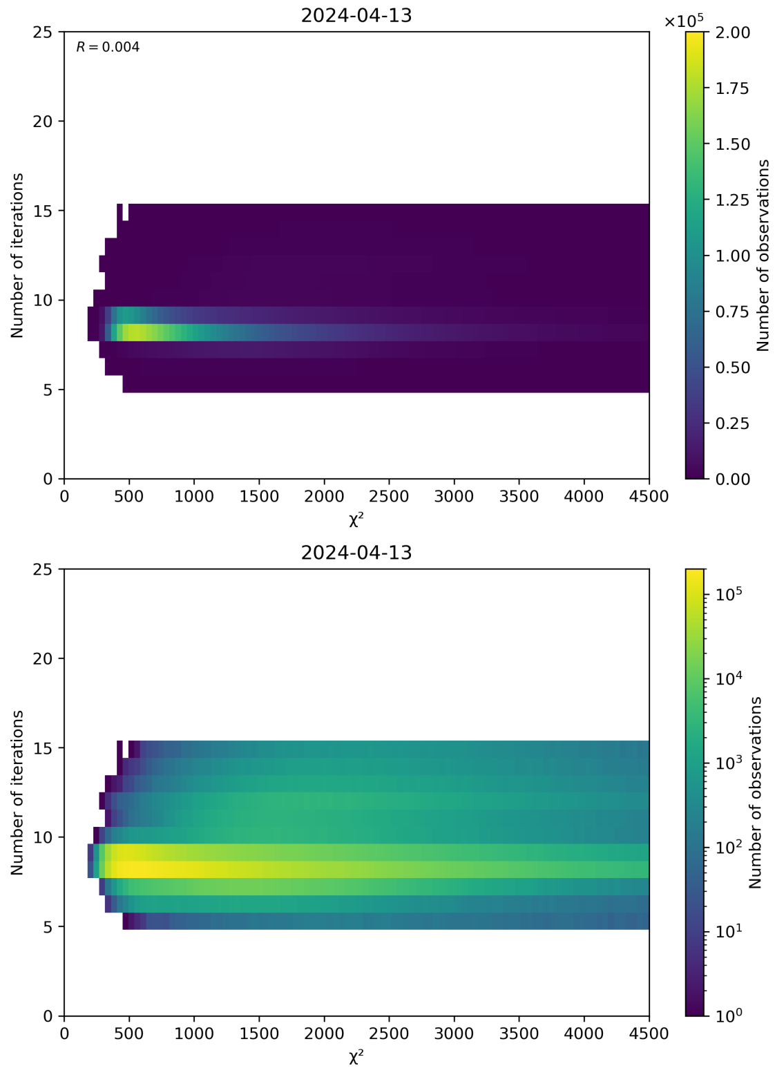
Figure 49: Scatter density plot of “ \chi^2 ” against “Number of iterations” for 2024-04-12 to 2024-04-14.
