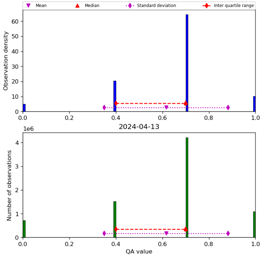
Figure 17: Histogram of “QA value” for 2024-04-12 to 2024-04-14
