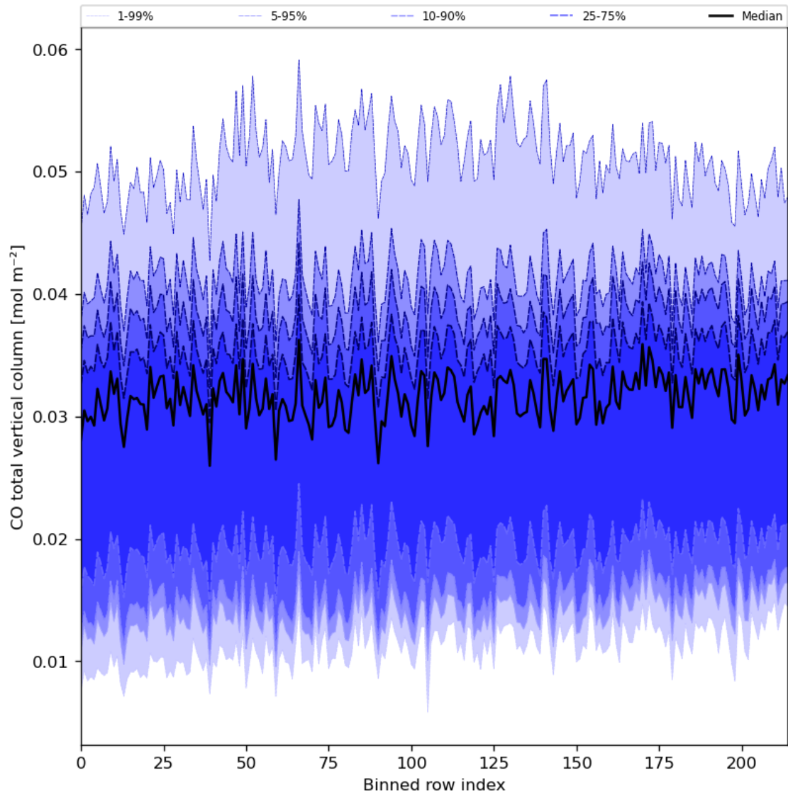
Figure 26: Along track statistics of “CO total vertical column” for 2024-04-12 to 2024-04-14
