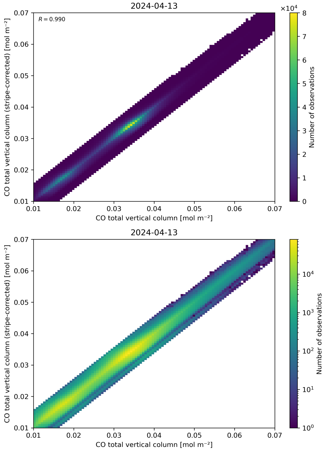
Figure 33: Scatter density plot of “CO total vertical column” against “CO total vertical column (stripe-corrected)” for 2024-04-12 to 2024-04-14.
