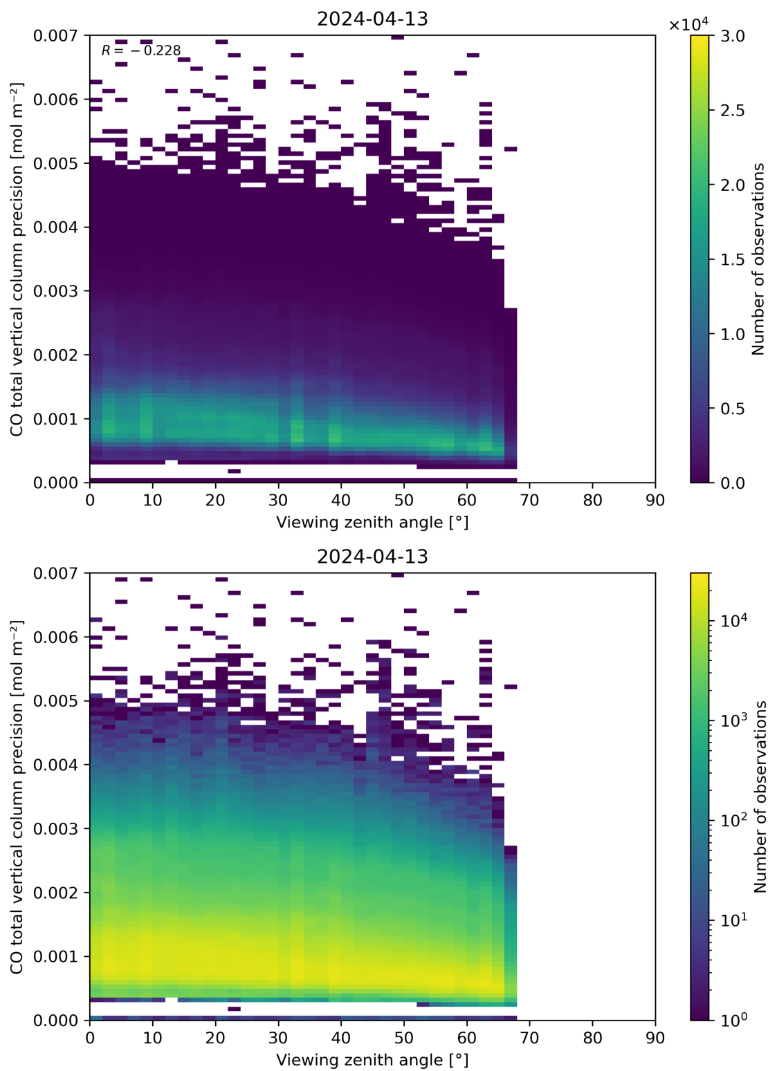
Figure 71: Scatter density plot of “Viewing zenith angle” against “CO total vertical column precision” for 2024-04-12 to 2024-04-14.
