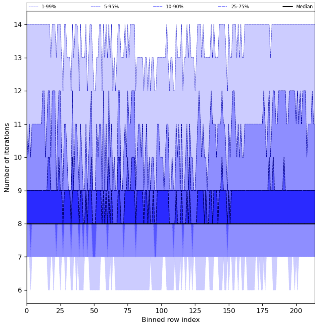
Figure 32: Along track statistics of “Number of iterations” for 2024-04-12 to 2024-04-14
