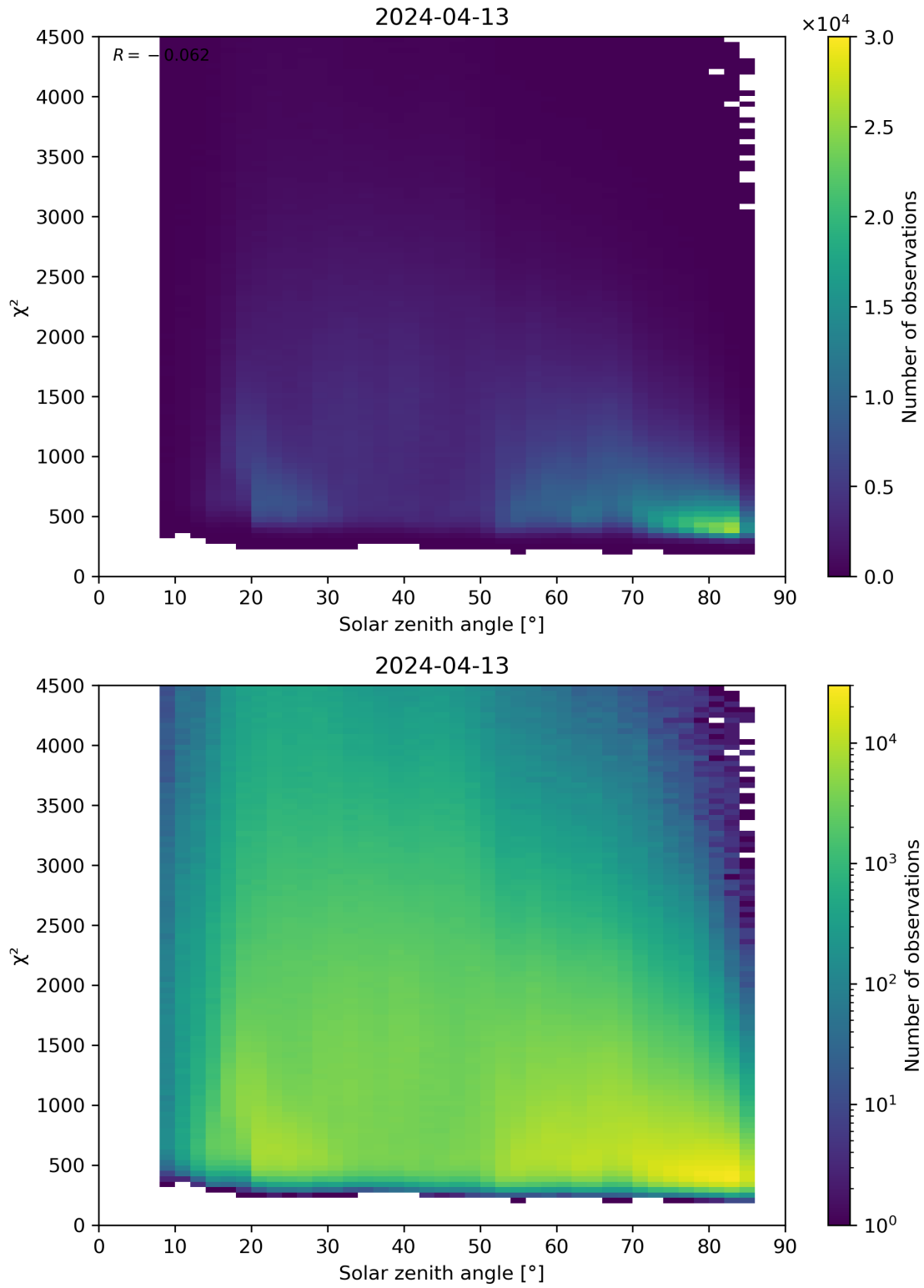
Figure 64: Scatter density plot of “Solar zenith angle” against “ \chi^2 ” for 2024-04-12 to 2024-04-14.
