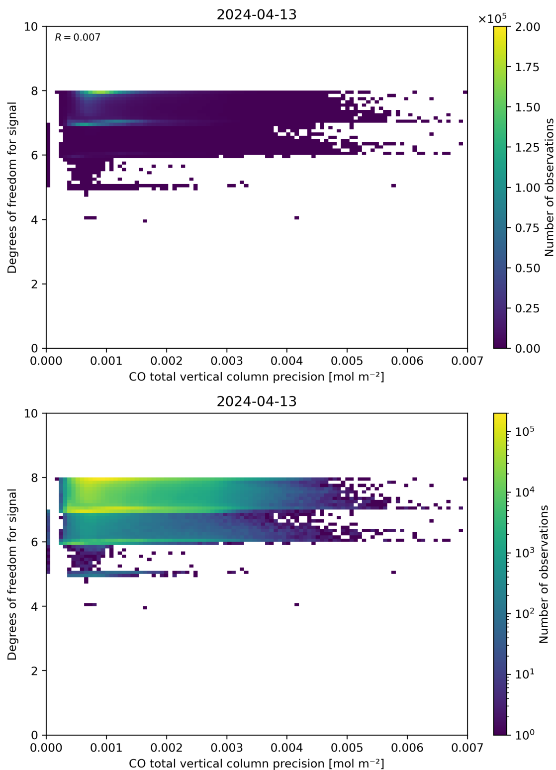
Figure 45: Scatter density plot of “CO total vertical column precision” against “Degrees of freedom for signal” for 2024-04-12 to 2024-04-14.
