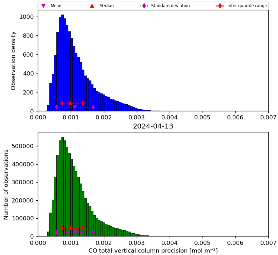
Figure 20: Histogram of “CO total vertical column precision” for 2024-04-12 to 2024-04-14
