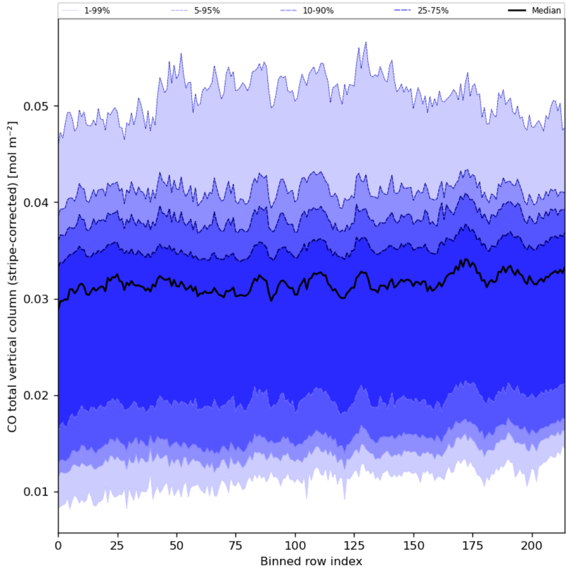
Figure 27: Along track statistics of “CO total vertical column (stripe-corrected)” for 2024-04-12 to 2024-04-14
