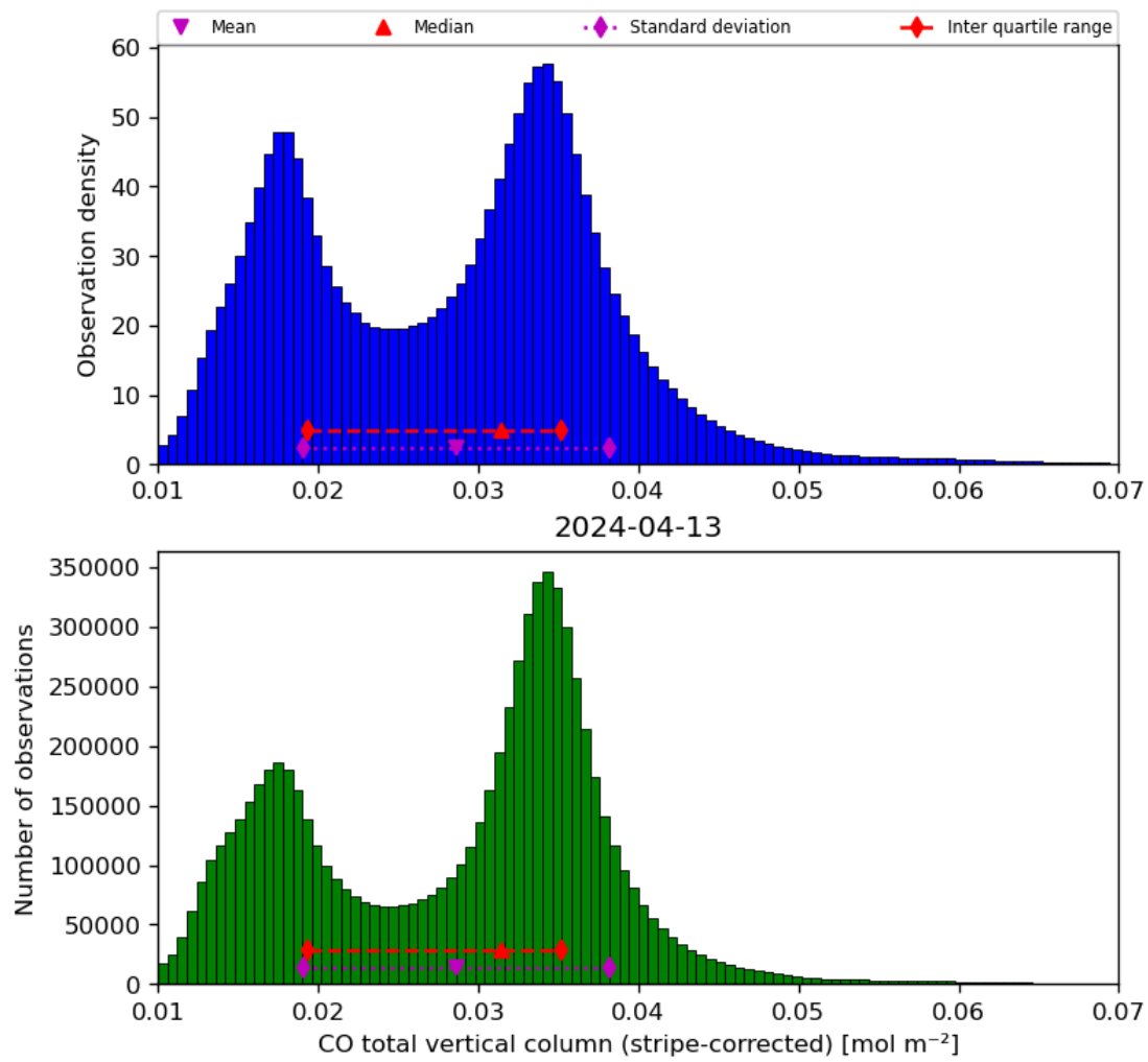
Figure 19: Histogram of “CO total vertical column (stripe-corrected)” for 2024-04-12 to 2024-04-14
