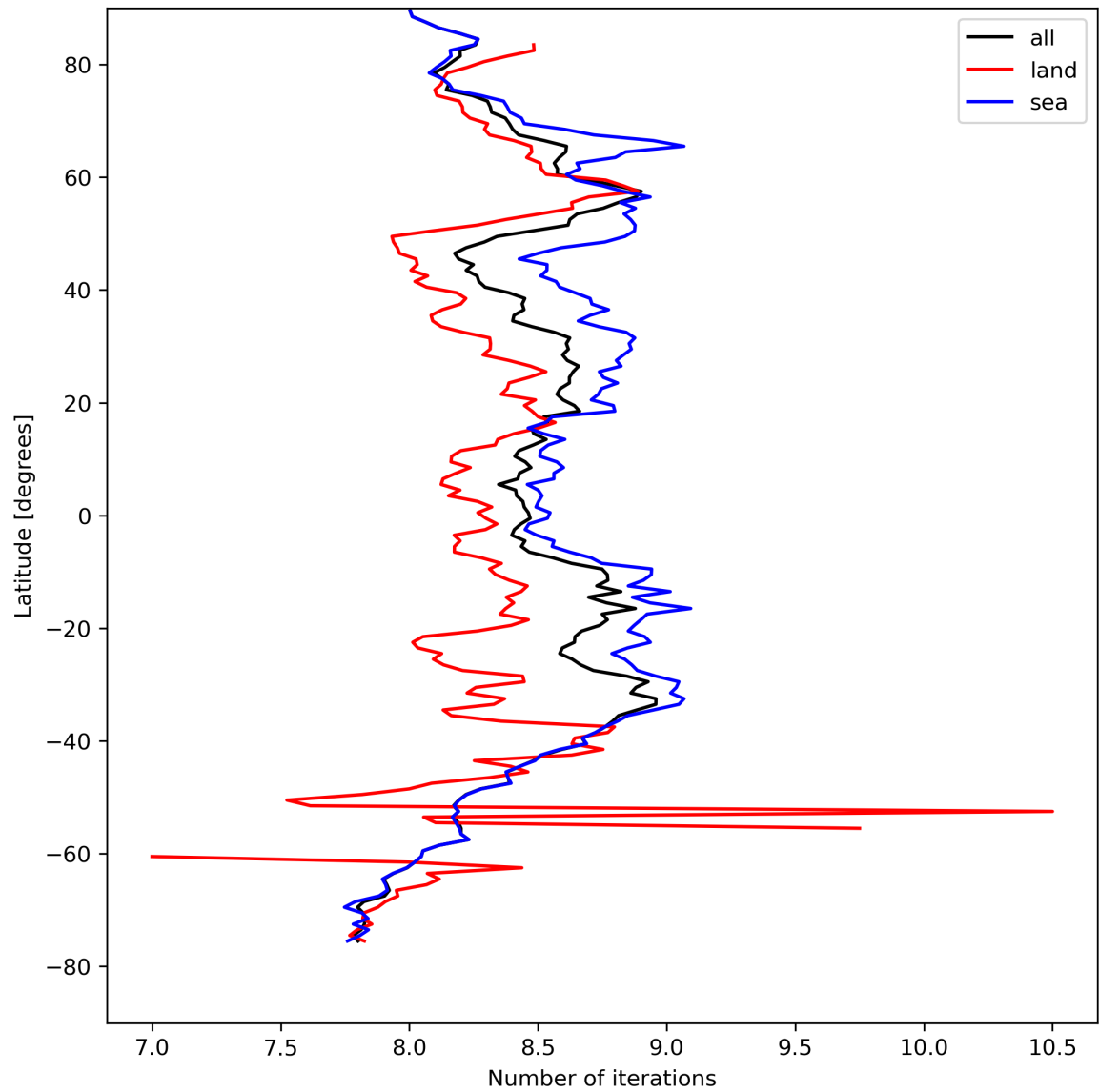
Figure 16: Zonal average of “Number of iterations” for 2024-04-12 to 2024-04-14.
