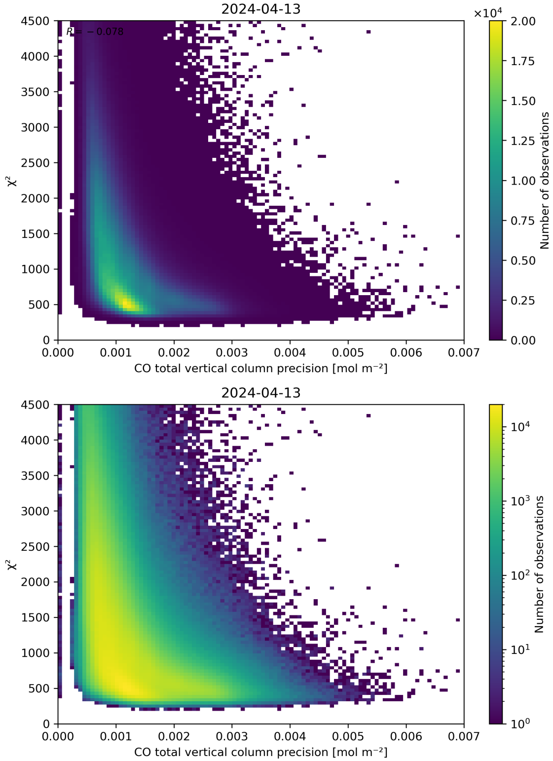
Figure 44: Scatter density plot of “CO total vertical column precision” against “ \chi^2 ” for 2024-04-12 to 2024-04-14.
