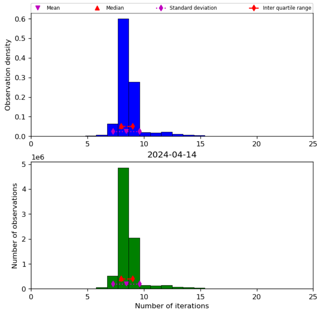
Figure 24: Histogram of “Number of iterations” for 2024-04-13 to 2024-04-15
