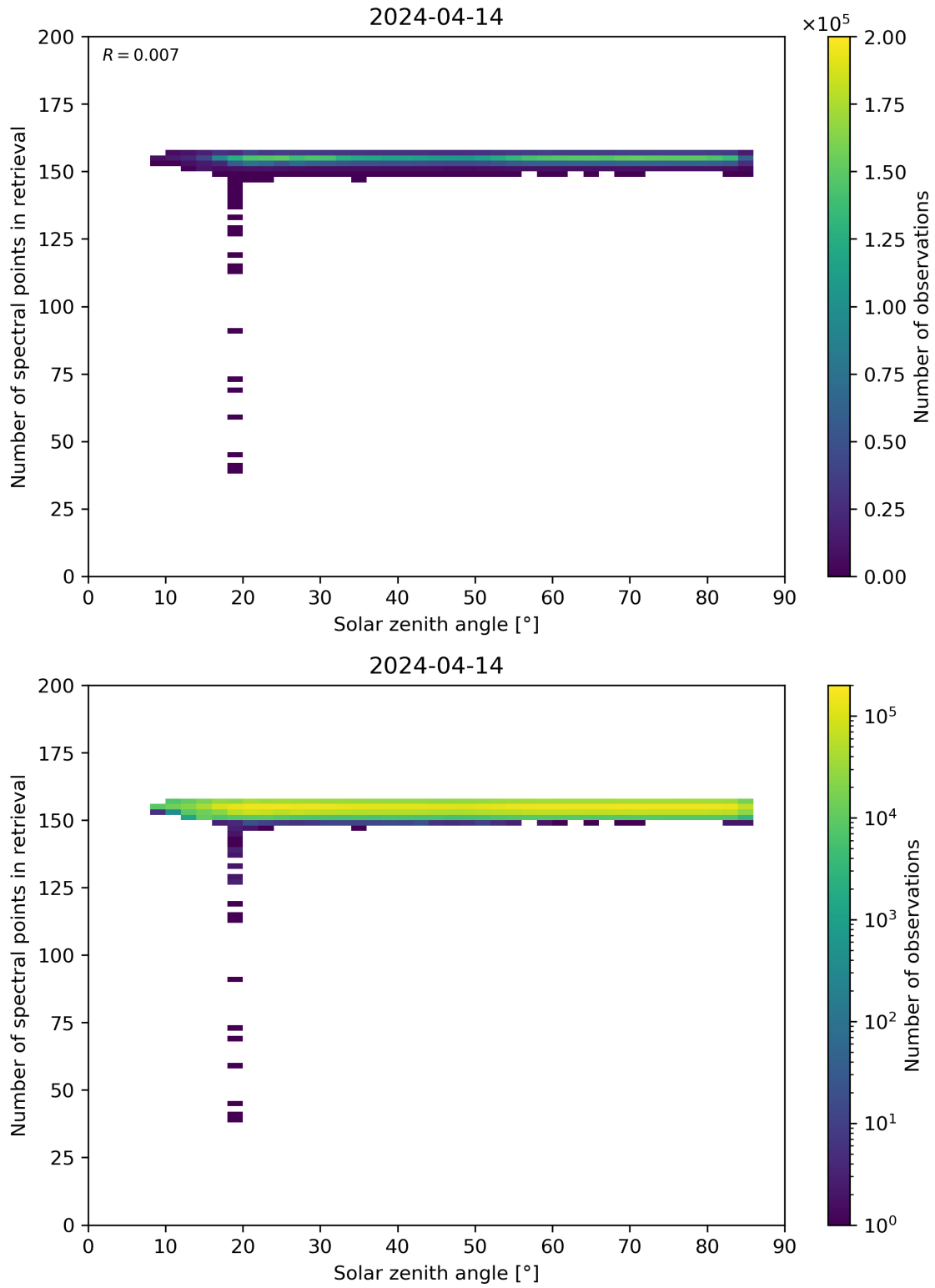
Figure 68: Scatter density plot of “Solar zenith angle” against “Number of spectral points in retrieval” for 2024-04-13 to 2024-04-15.
