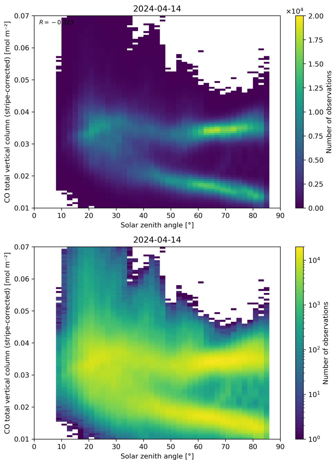
Figure 62: Scatter density plot of “Solar zenith angle” against “CO total vertical column (stripe-corrected)” for 2024-04-13 to 2024-04-15.
