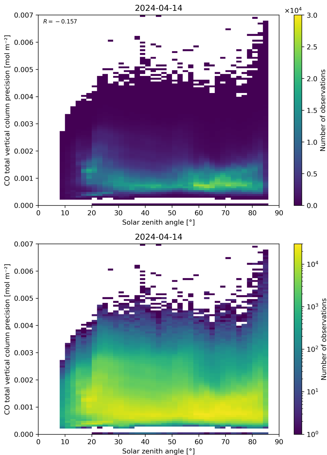
Figure 63: Scatter density plot of “Solar zenith angle” against “CO total vertical column precision” for 2024-04-13 to 2024-04-15.
