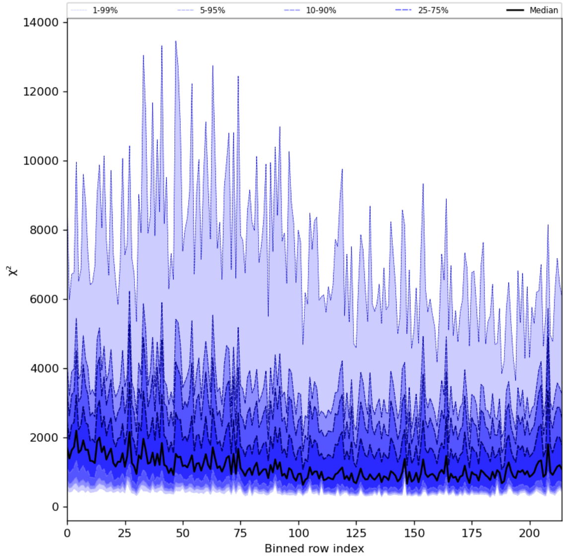
Figure 30: Along track statistics of “ \chi^2 ” for 2024-04-13 to 2024-04-15
