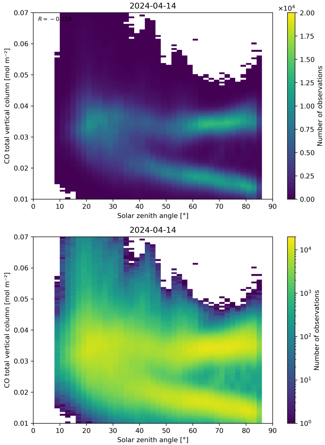
Figure 61: Scatter density plot of “Solar zenith angle” against “CO total vertical column” for 2024-04-13 to 2024-04-15.
