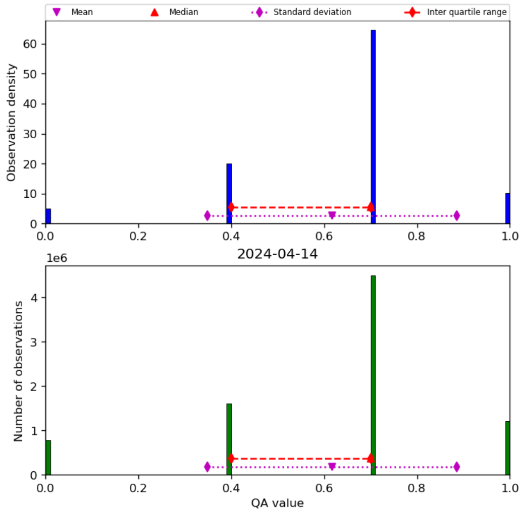
Figure 17: Histogram of “QA value” for 2024-04-13 to 2024-04-15
