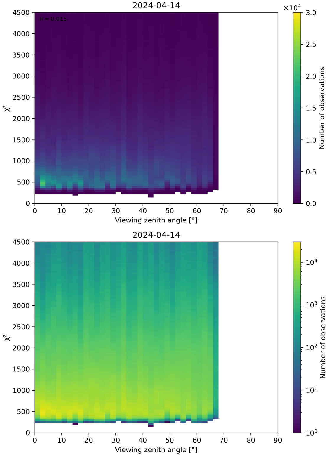
Figure 72: Scatter density plot of “Viewing zenith angle” against “ \chi^2 ” for 2024-04-13 to 2024-04-15.
