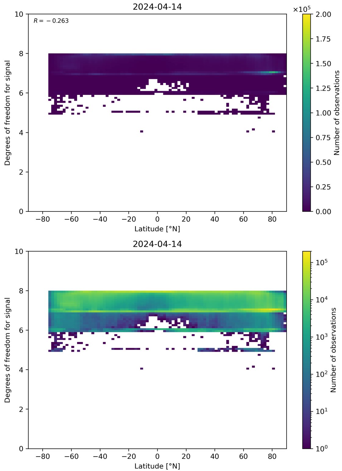
Figure 55: Scatter density plot of “Latitude” against “Degrees of freedom for signal” for 2024-04-13 to 2024-04-15.
