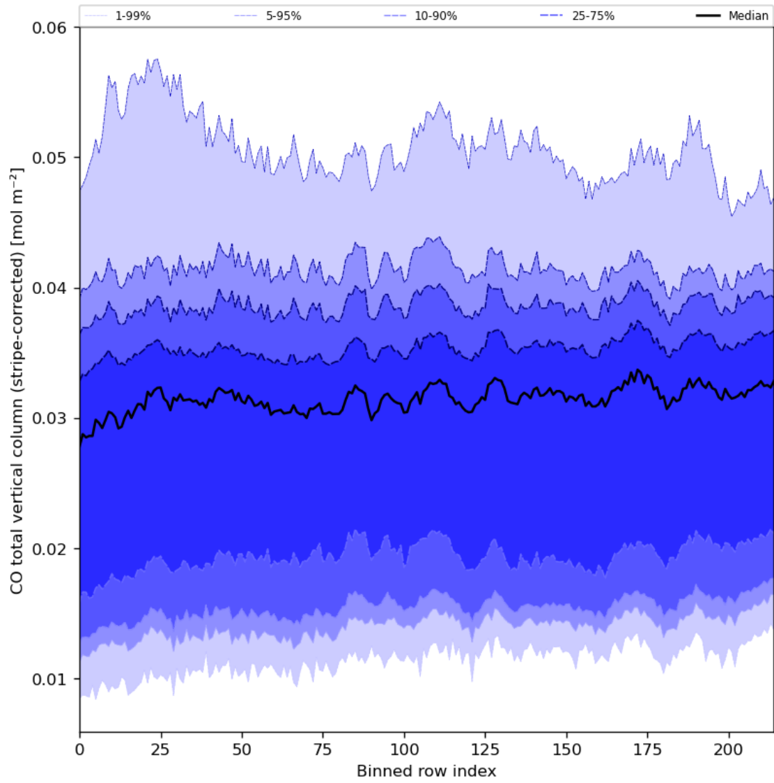
Figure 27: Along track statistics of “CO total vertical column (stripe-corrected)” for 2024-04-13 to 2024-04-15
