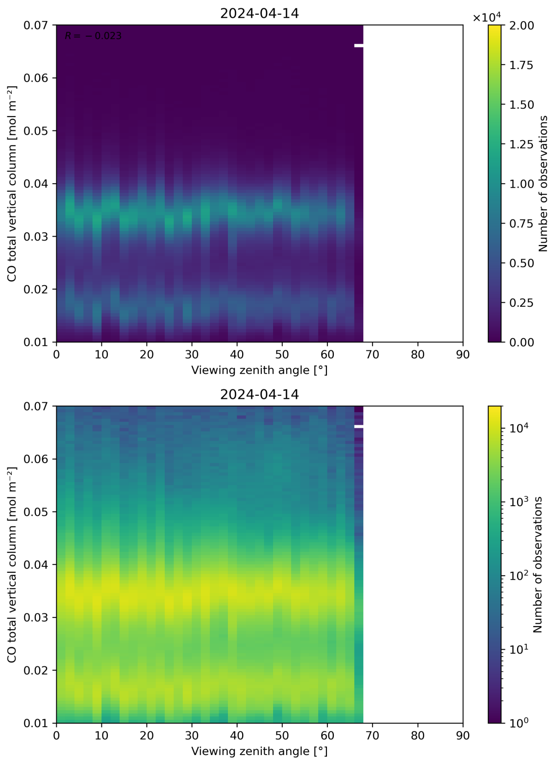
Figure 69: Scatter density plot of “Viewing zenith angle” against “CO total vertical column” for 2024-04-13 to 2024-04-15.
