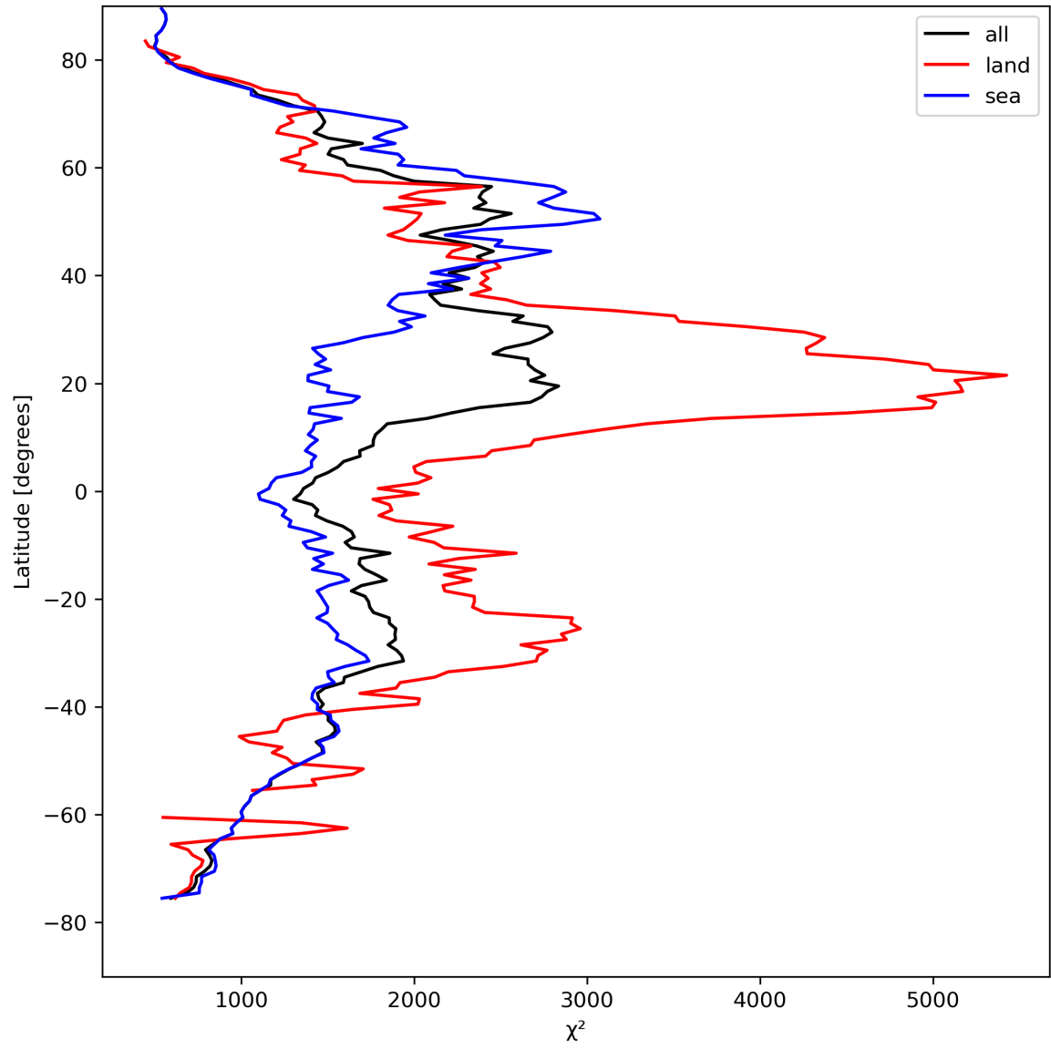
Figure 14: Zonal average of “ \chi^2 ” for 2024-04-13 to 2024-04-15.
