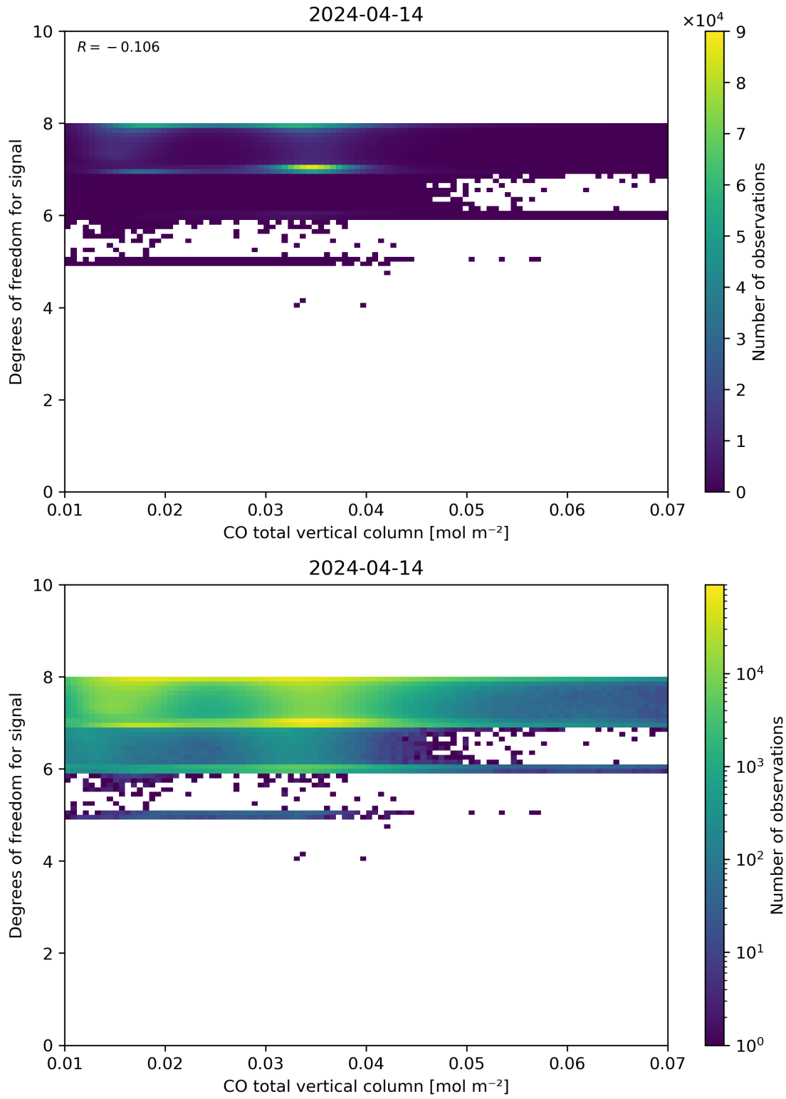
Figure 41: Scatter density plot of “CO total vertical column” against “Degrees of freedom for signal” for 2024-04-13 to 2024-04-15.
