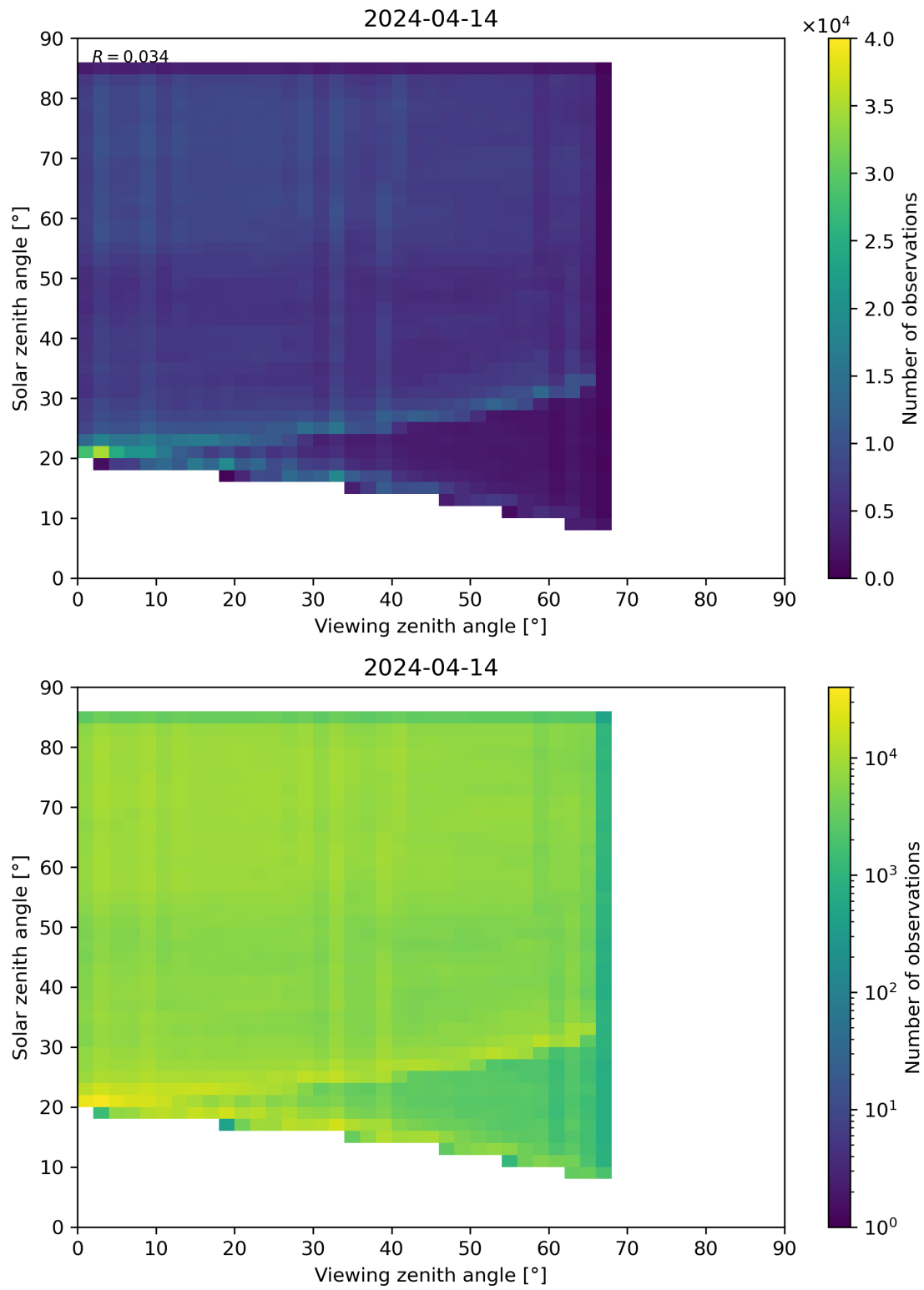
Figure 77: Scatter density plot of “Viewing zenith angle” against “Solar zenith angle” for 2024-04-13 to 2024-04-15.
