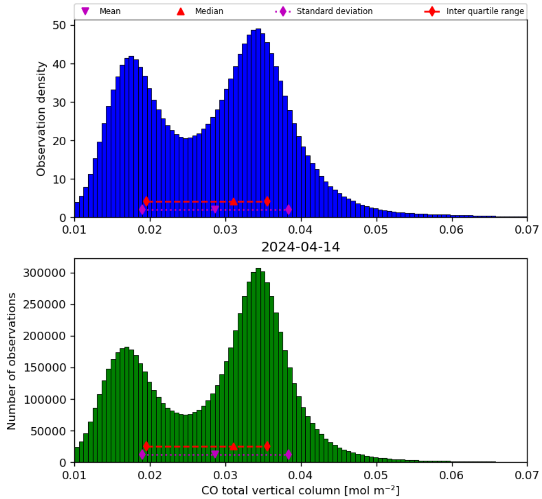
Figure 18: Histogram of “CO total vertical column” for 2024-04-13 to 2024-04-15
