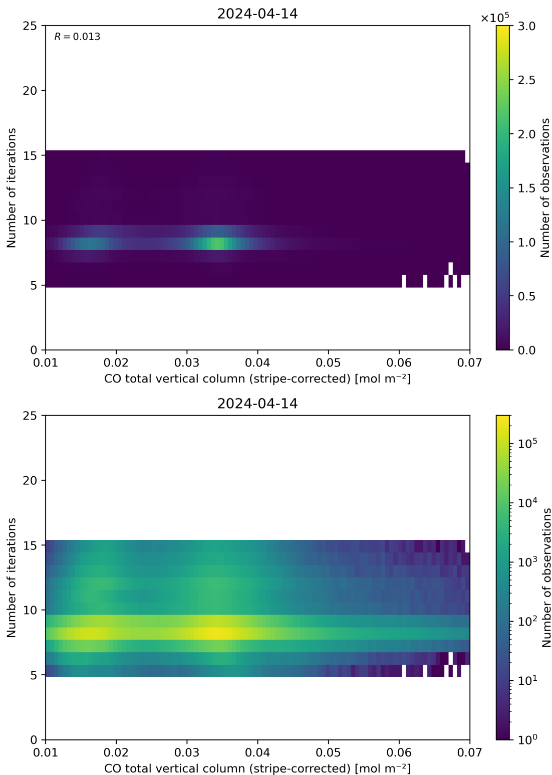
Figure 39: Scatter density plot of “CO total vertical column (stripe-corrected)” against “Number of iterations” for 2024-04-13 to 2024-04-15.
