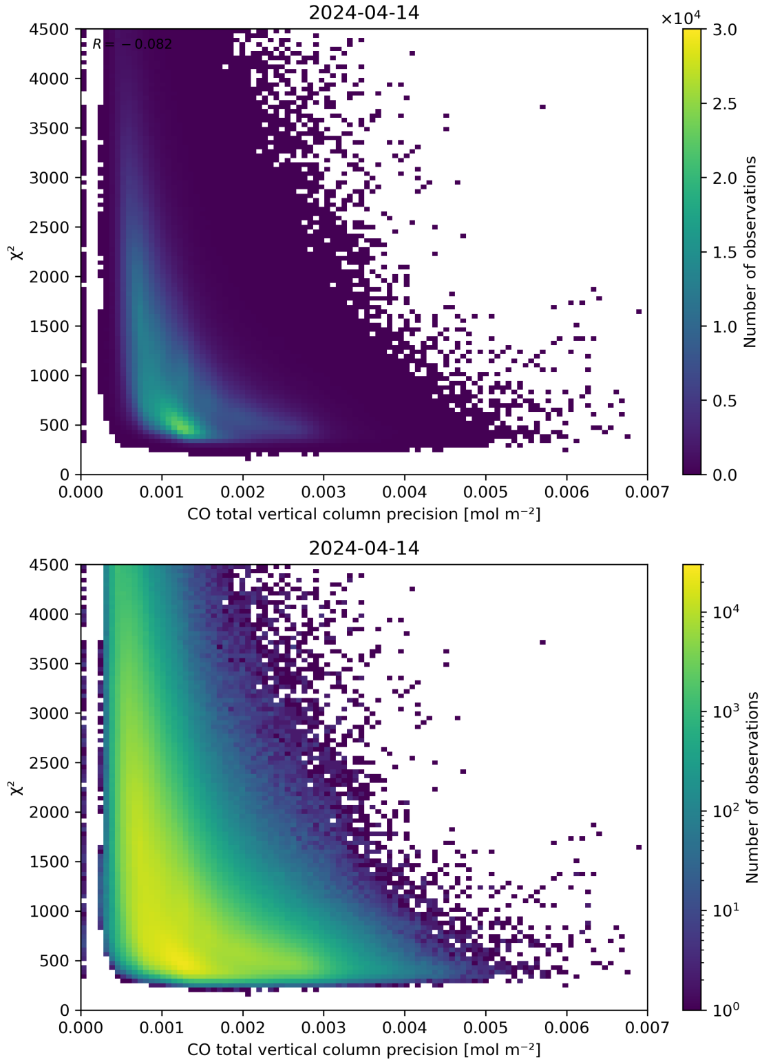
Figure 44: Scatter density plot of “CO total vertical column precision” against “ \chi^2 ” for 2024-04-13 to 2024-04-15.
