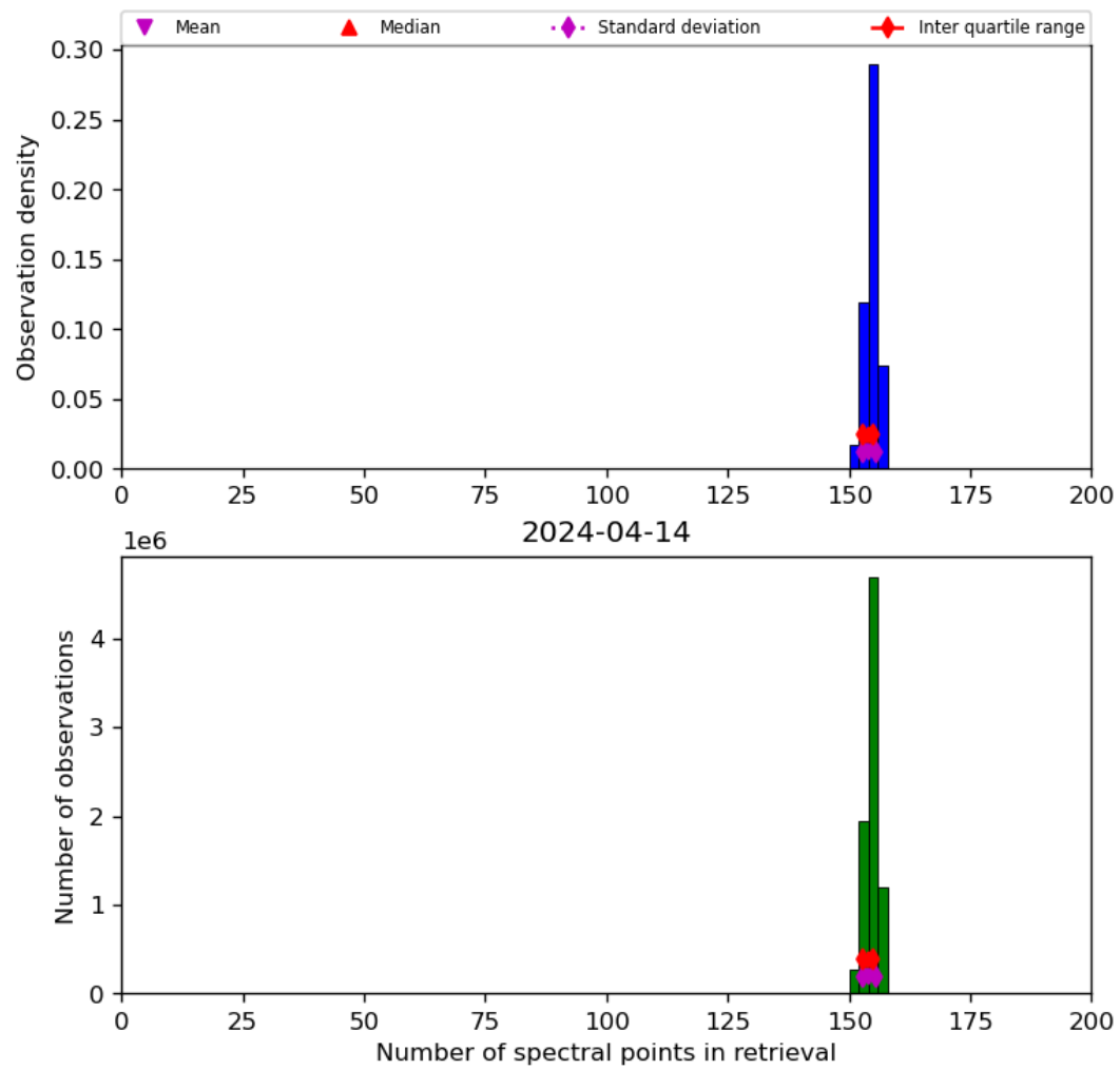
Figure 21: Histogram of “Number of spectral points in retrieval” for 2024-04-13 to 2024-04-15
