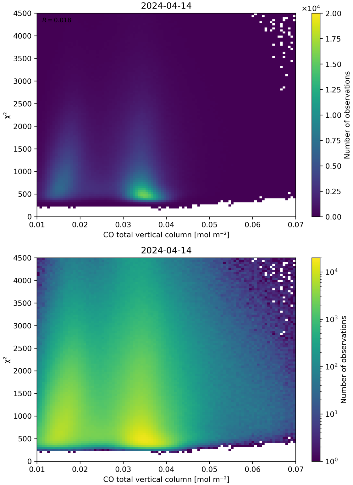
Figure 35: Scatter density plot of “CO total vertical column” against “ \chi^2 ” for 2024-04-13 to 2024-04-15.
