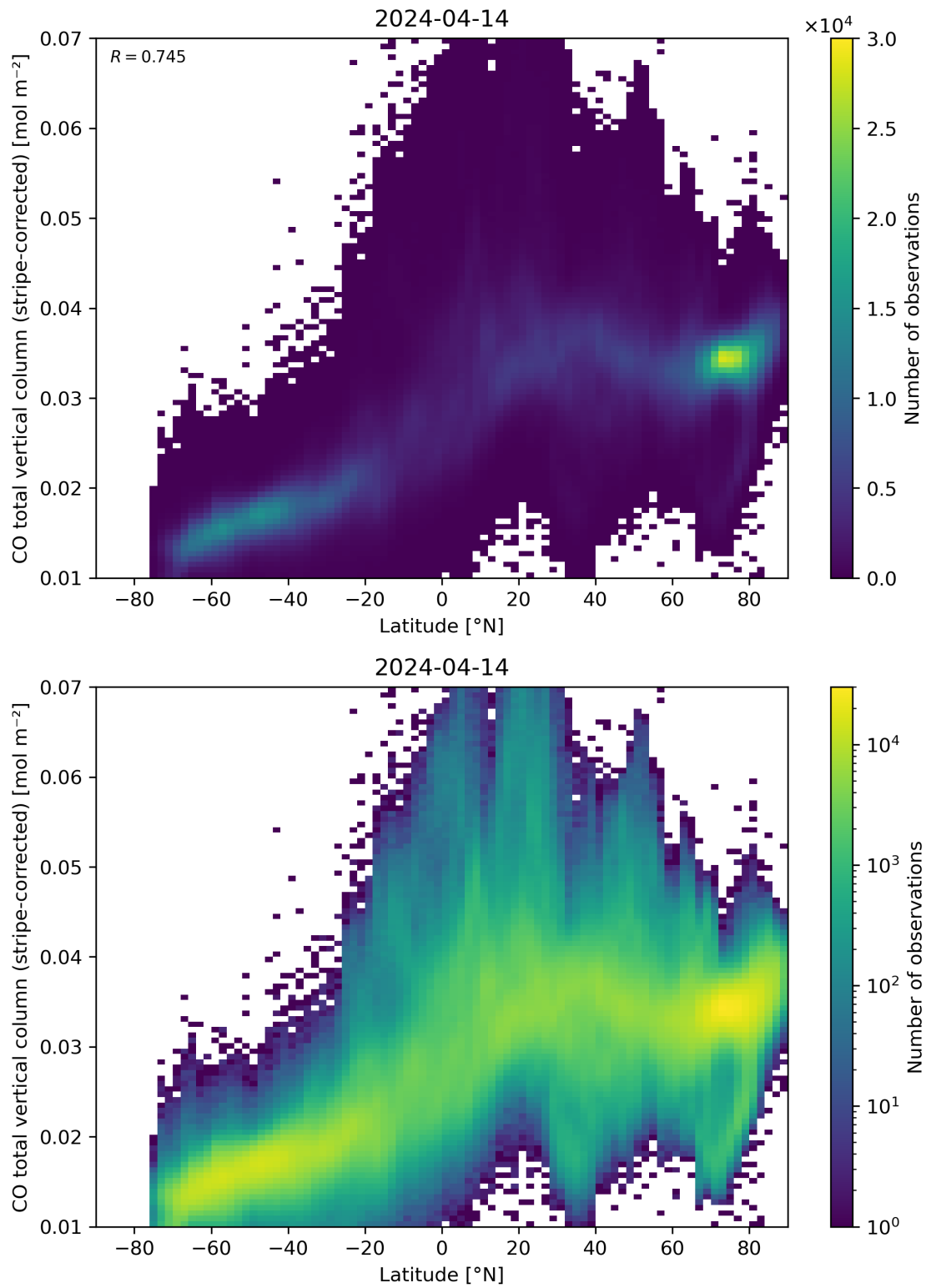
Figure 52: Scatter density plot of “Latitude” against “CO total vertical column (stripe-corrected)” for 2024-04-13 to 2024-04-15.
