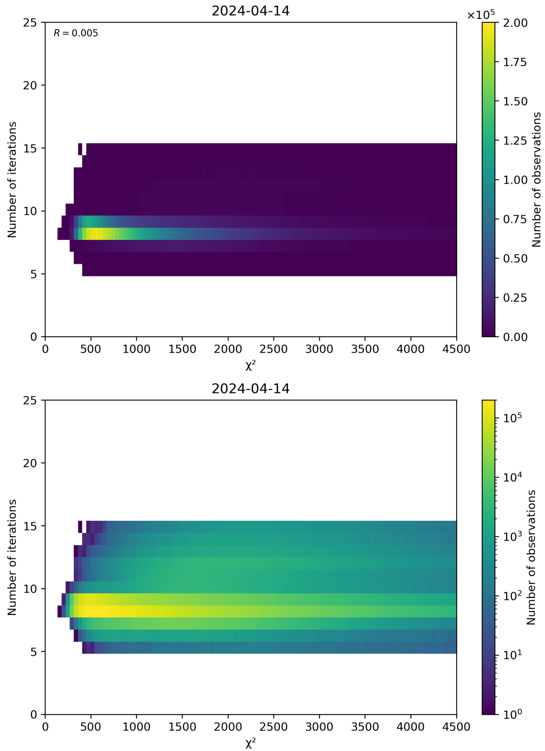
Figure 49: Scatter density plot of “ \chi^2 ” against “Number of iterations” for 2024-04-13 to 2024-04-15.
