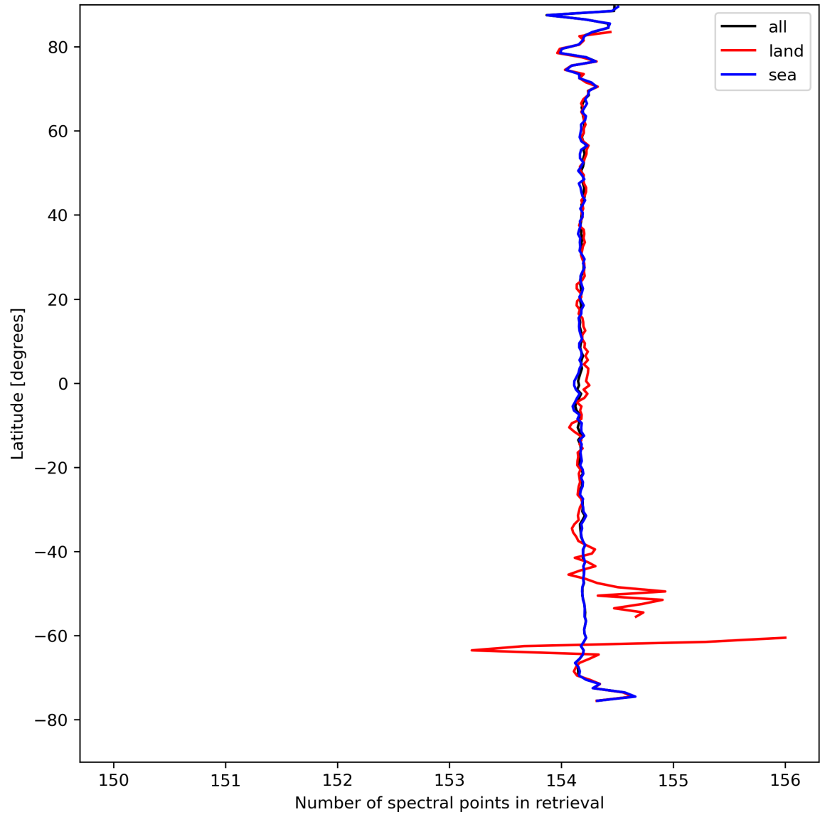
Figure 13: Zonal average of “Number of spectral points in retrieval” for 2024-04-13 to 2024-04-15.
