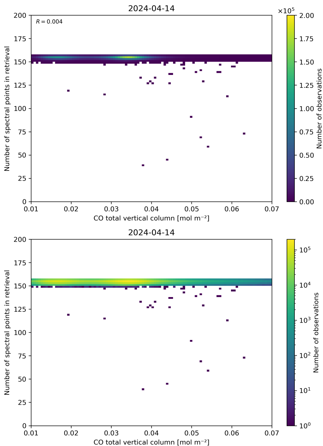
Figure 43: Scatter density plot of “CO total vertical column” against “Number of spectral points in retrieval” for 2024-04-13 to 2024-04-15.
