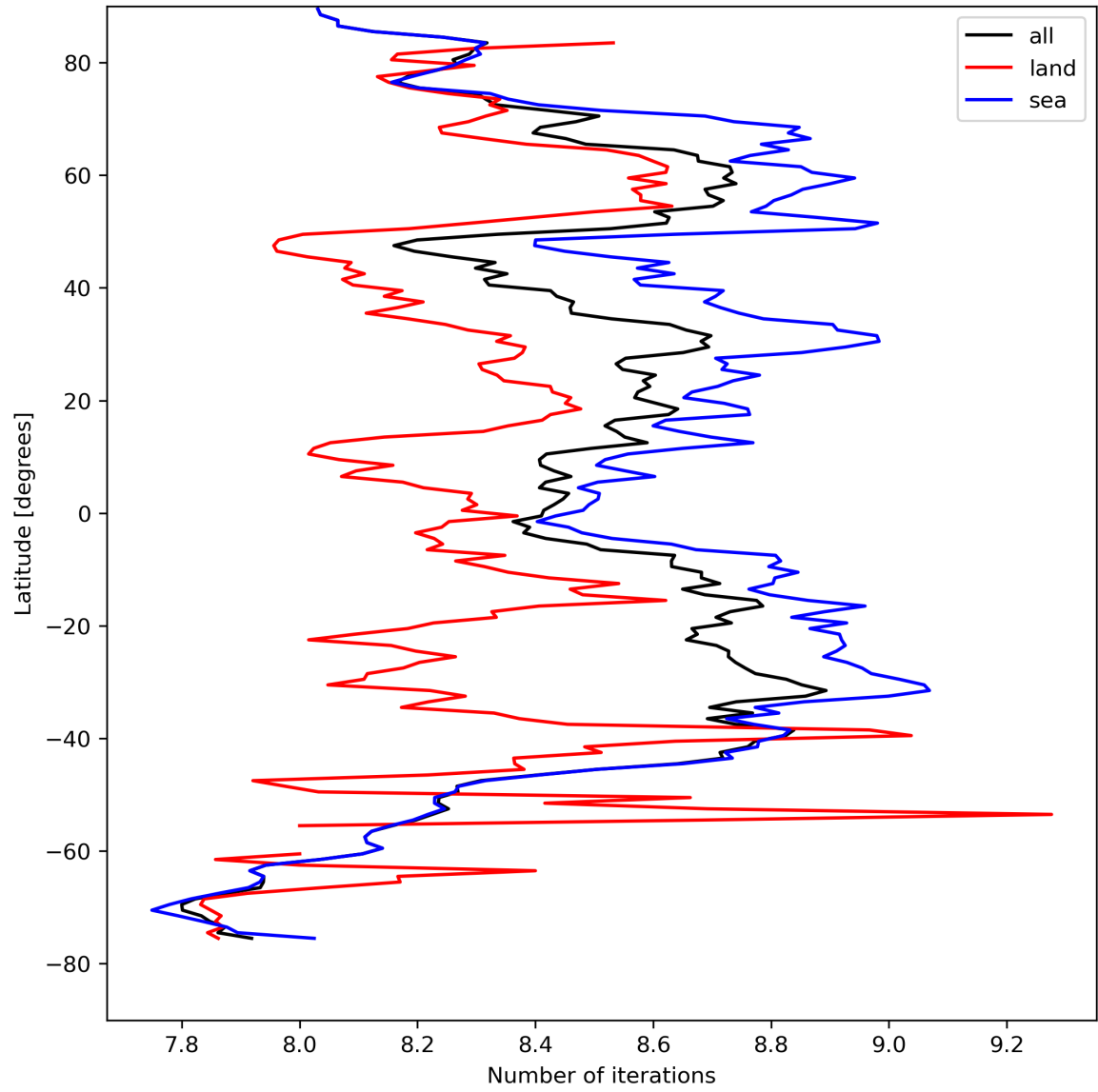
Figure 16: Zonal average of “Number of iterations” for 2024-04-13 to 2024-04-15.
