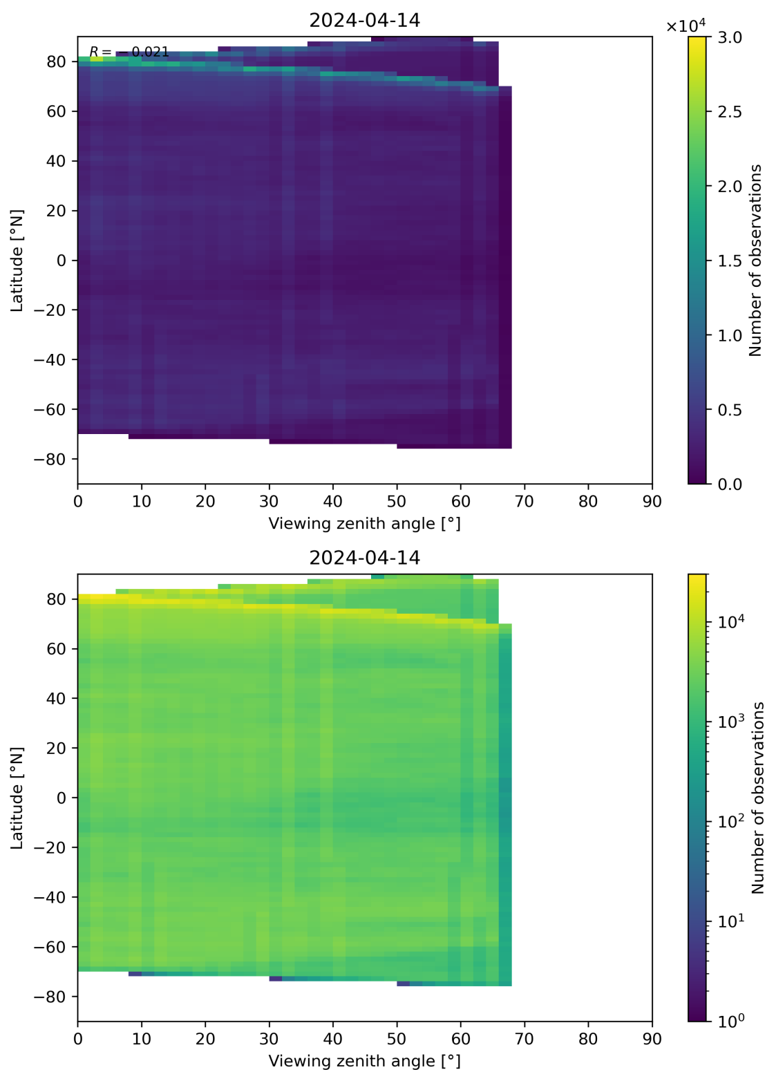
Figure 74: Scatter density plot of “Viewing zenith angle” against “Latitude” for 2024-04-13 to 2024-04-15.
