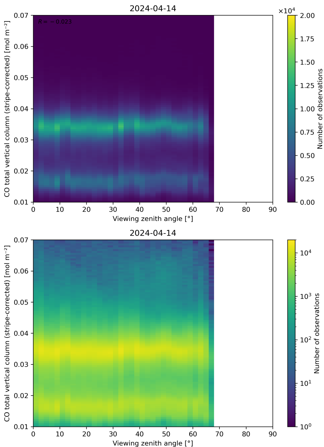
Figure 70: Scatter density plot of “Viewing zenith angle” against “CO total vertical column (stripe-corrected)” for 2024-04-13 to 2024-04-15.
