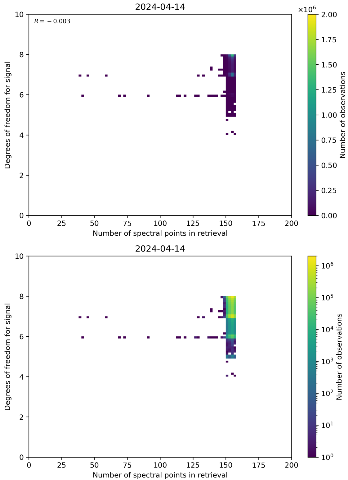
Figure 59: Scatter density plot of “Number of spectral points in retrieval” against “Degrees of freedom for signal” for 2024-04-13 to 2024-04-15.
