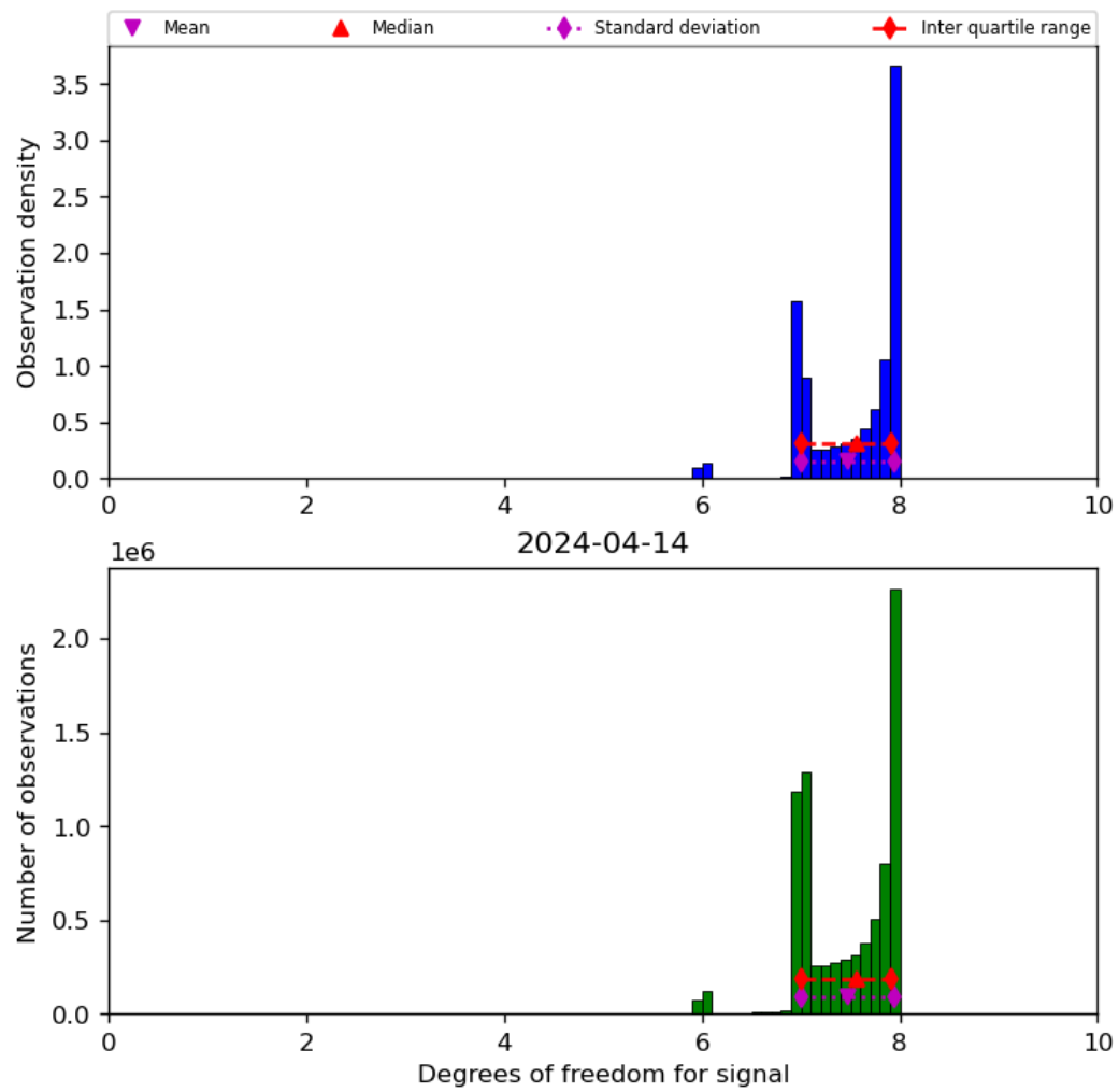
Figure 23: Histogram of “Degrees of freedom for signal” for 2024-04-13 to 2024-04-15
