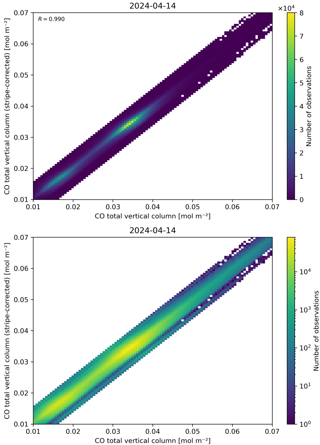
Figure 33: Scatter density plot of “CO total vertical column” against “CO total vertical column (stripe-corrected)” for 2024-04-13 to 2024-04-15.
