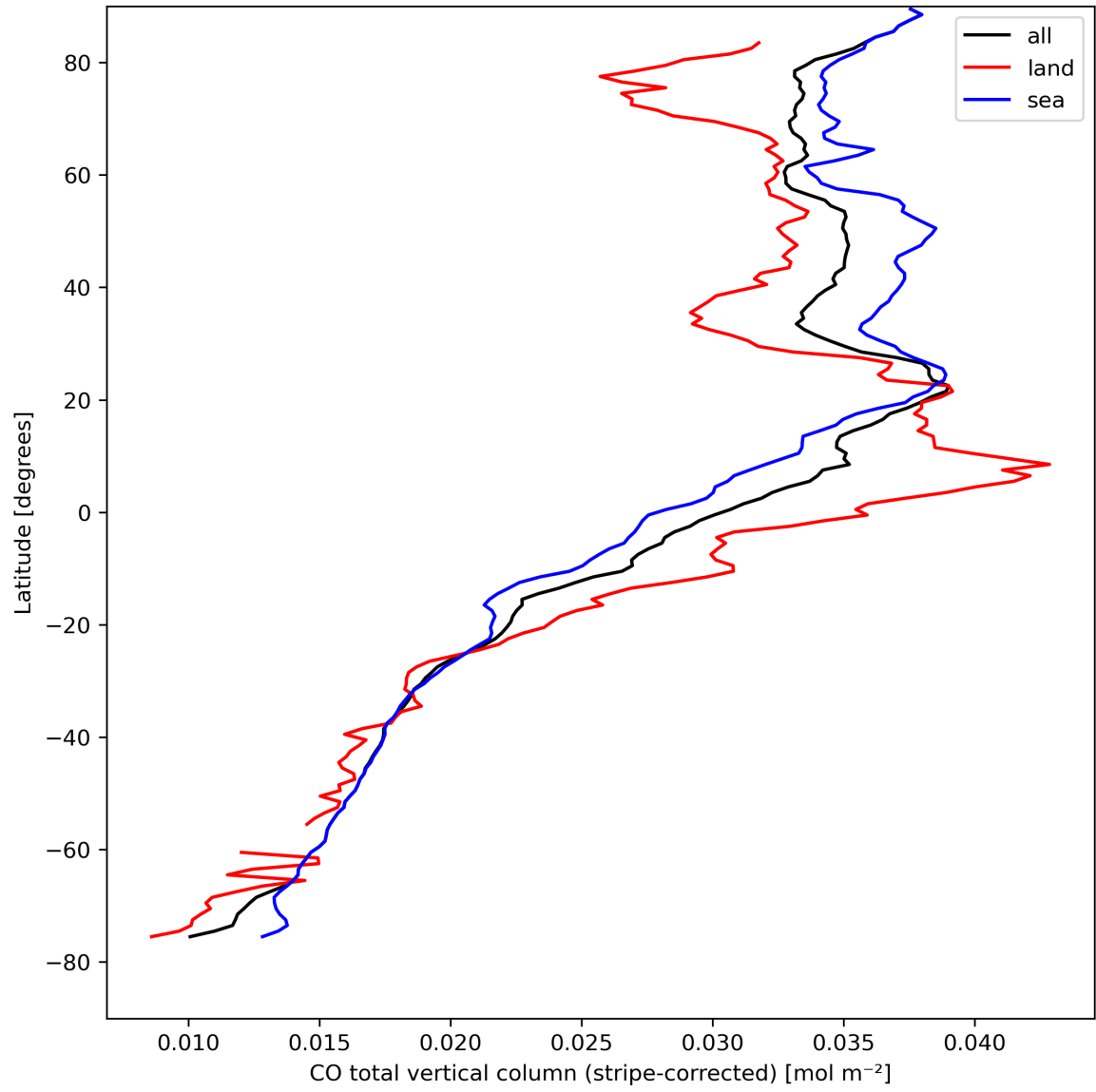
Figure 11: Zonal average of “CO total vertical column (stripe-corrected)” for 2024-04-13 to 2024-04-15.
