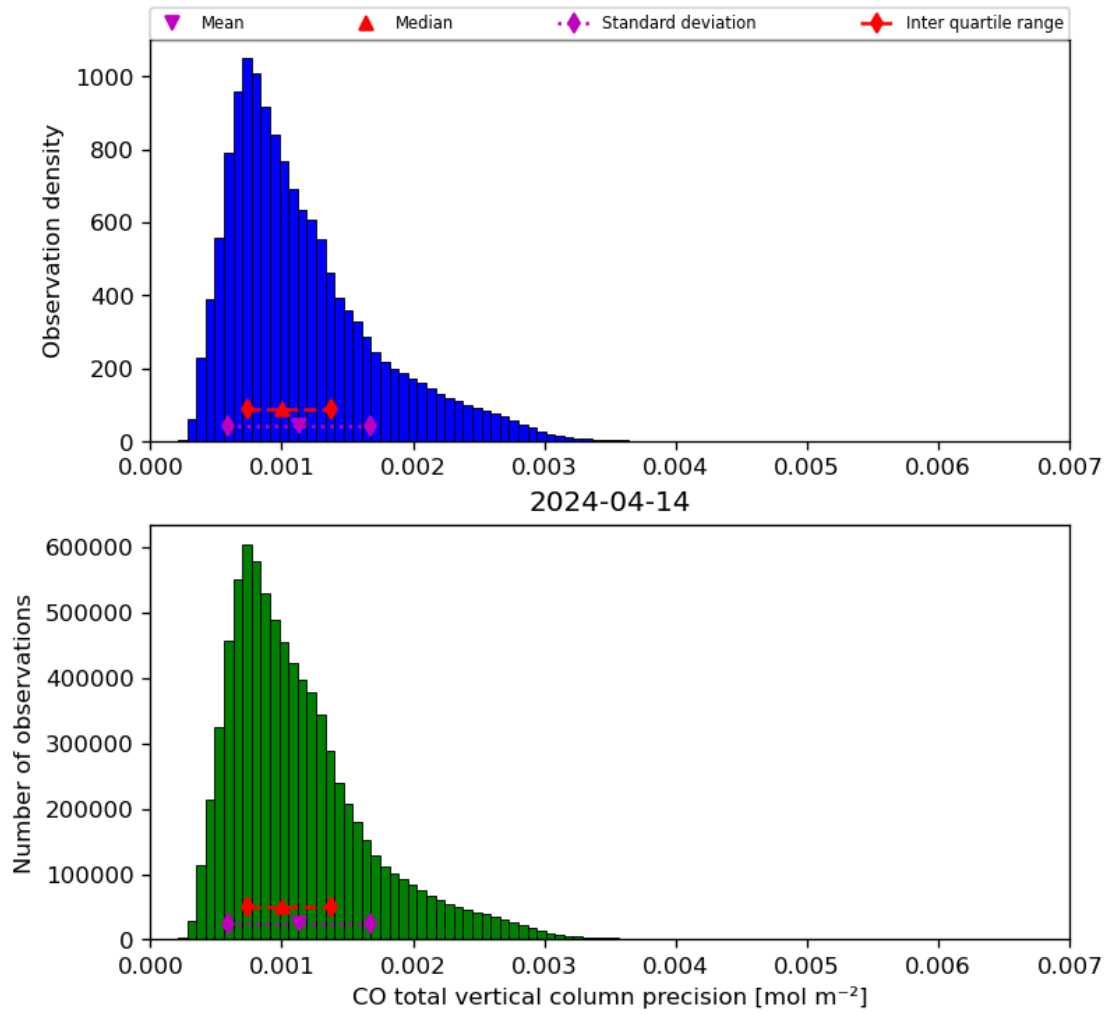
Figure 20: Histogram of “CO total vertical column precision” for 2024-04-13 to 2024-04-15
