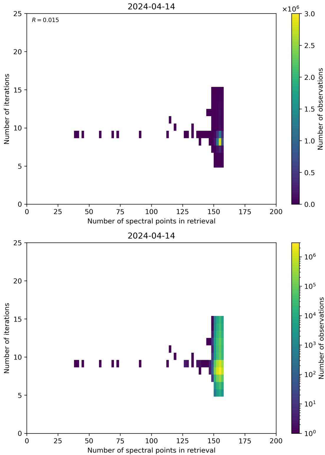
Figure 60: Scatter density plot of “Number of spectral points in retrieval” against “Number of iterations” for 2024-04-13 to 2024-04-15.
