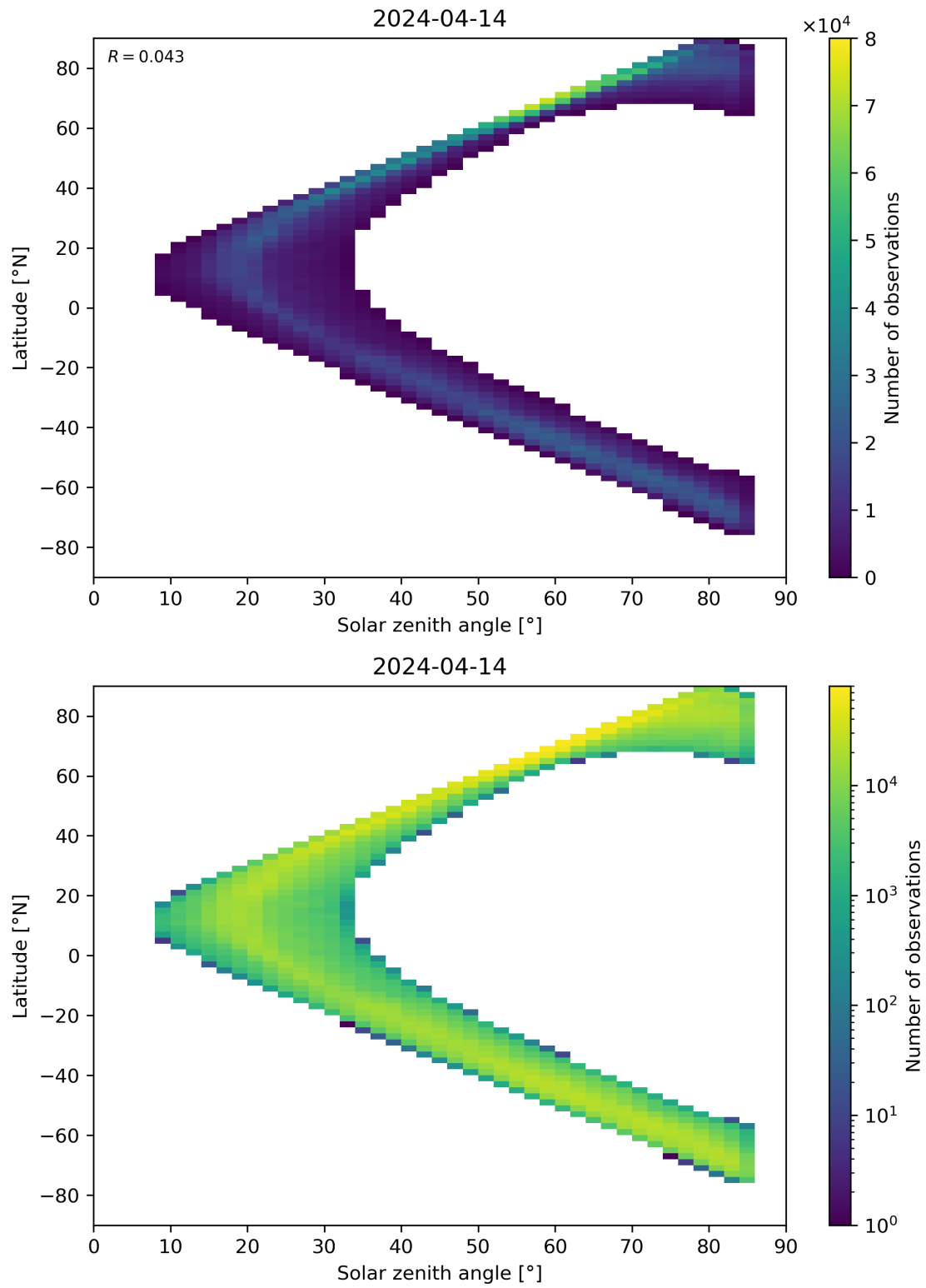
Figure 66: Scatter density plot of “Solar zenith angle” against “Latitude” for 2024-04-13 to 2024-04-15.
