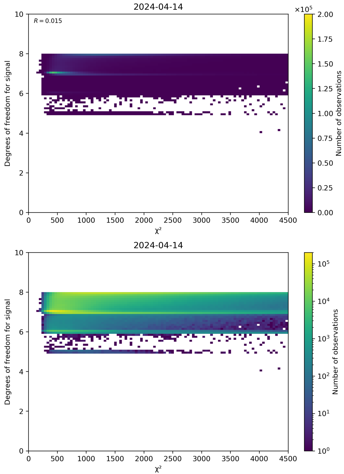
Figure 48: Scatter density plot of “ \chi^2 ” against “Degrees of freedom for signal” for 2024-04-13 to 2024-04-15.
