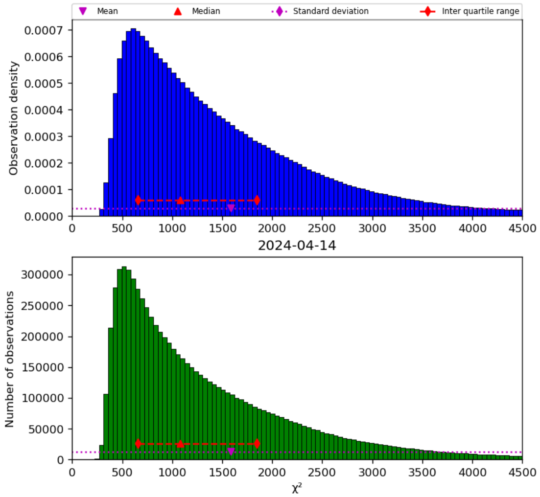
Figure 22: Histogram of " \chi^2 " for 2024-04-13 to 2024-04-15
