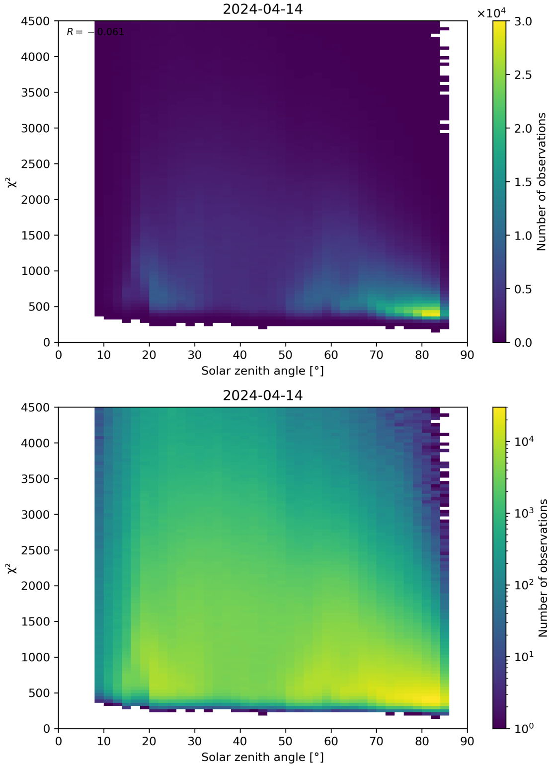
Figure 64: Scatter density plot of “Solar zenith angle” against “ \chi^2 ” for 2024-04-13 to 2024-04-15.
