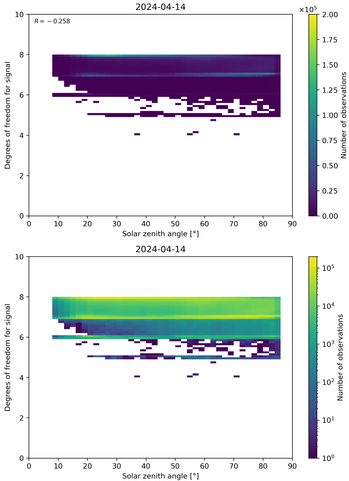
Figure 65: Scatter density plot of “Solar zenith angle” against “Degrees of freedom for signal” for 2024-04-13 to 2024-04-15.
