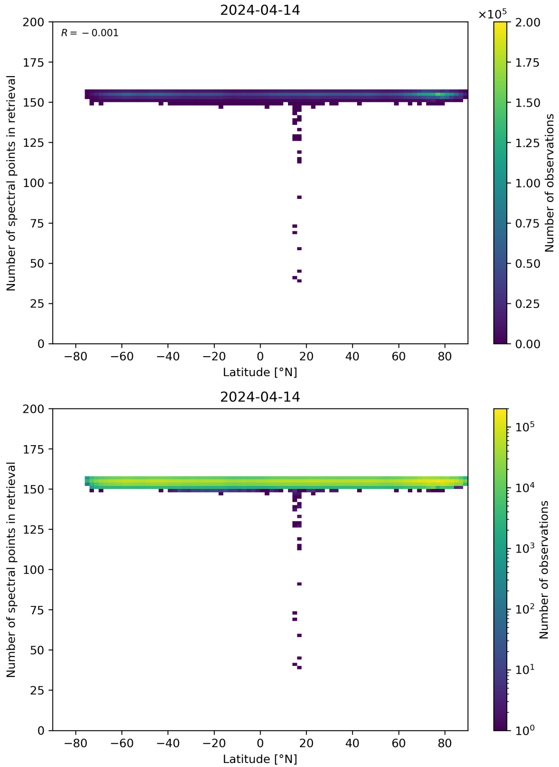
Figure 57: Scatter density plot of “Latitude” against “Number of spectral points in retrieval” for 2024-04-13 to 2024-04-15.
