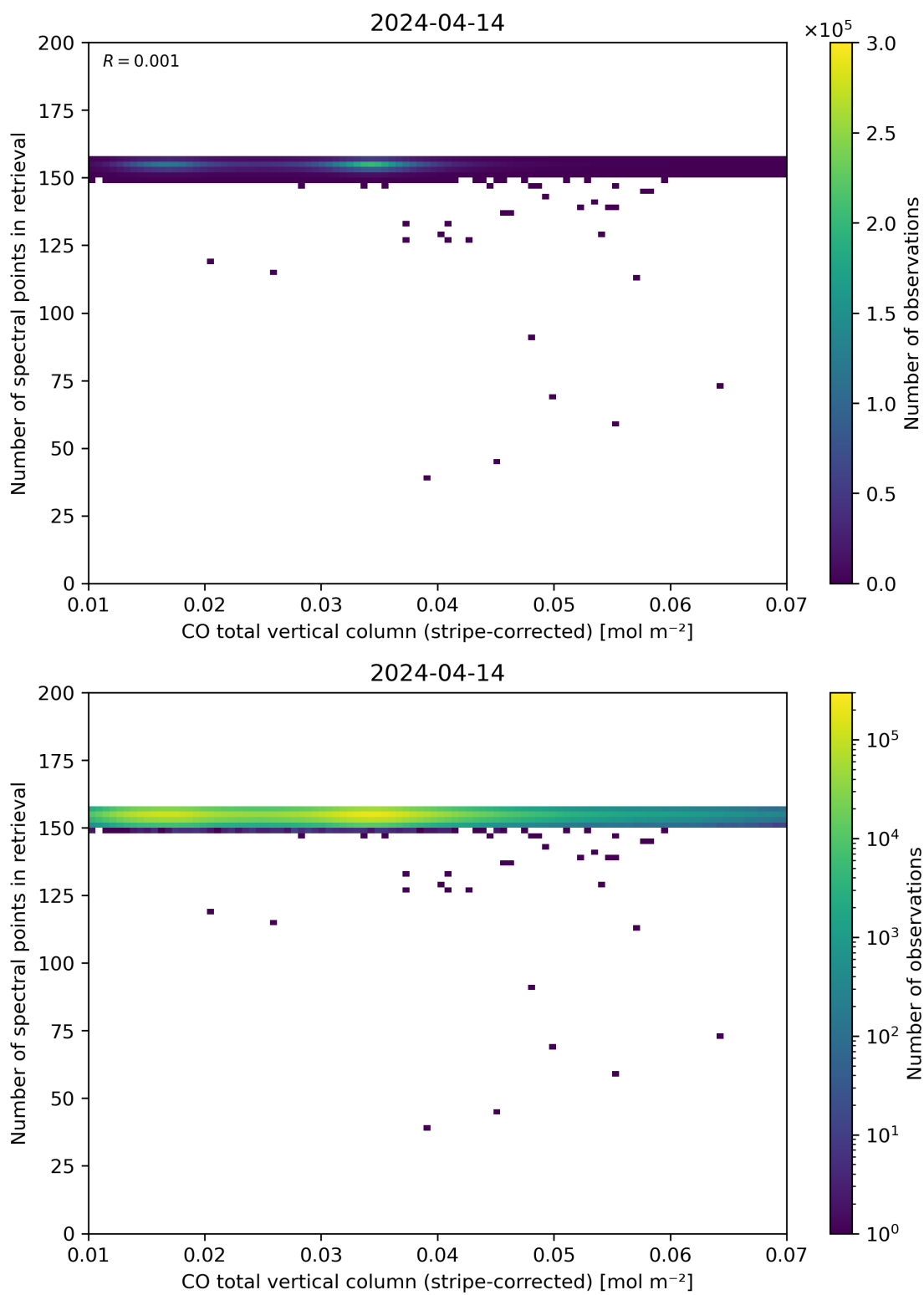
Figure 40: Scatter density plot of “CO total vertical column (stripe-corrected)” against “Number of spectral points in retrieval” for 2024-04-13 to 2024-04-15.
