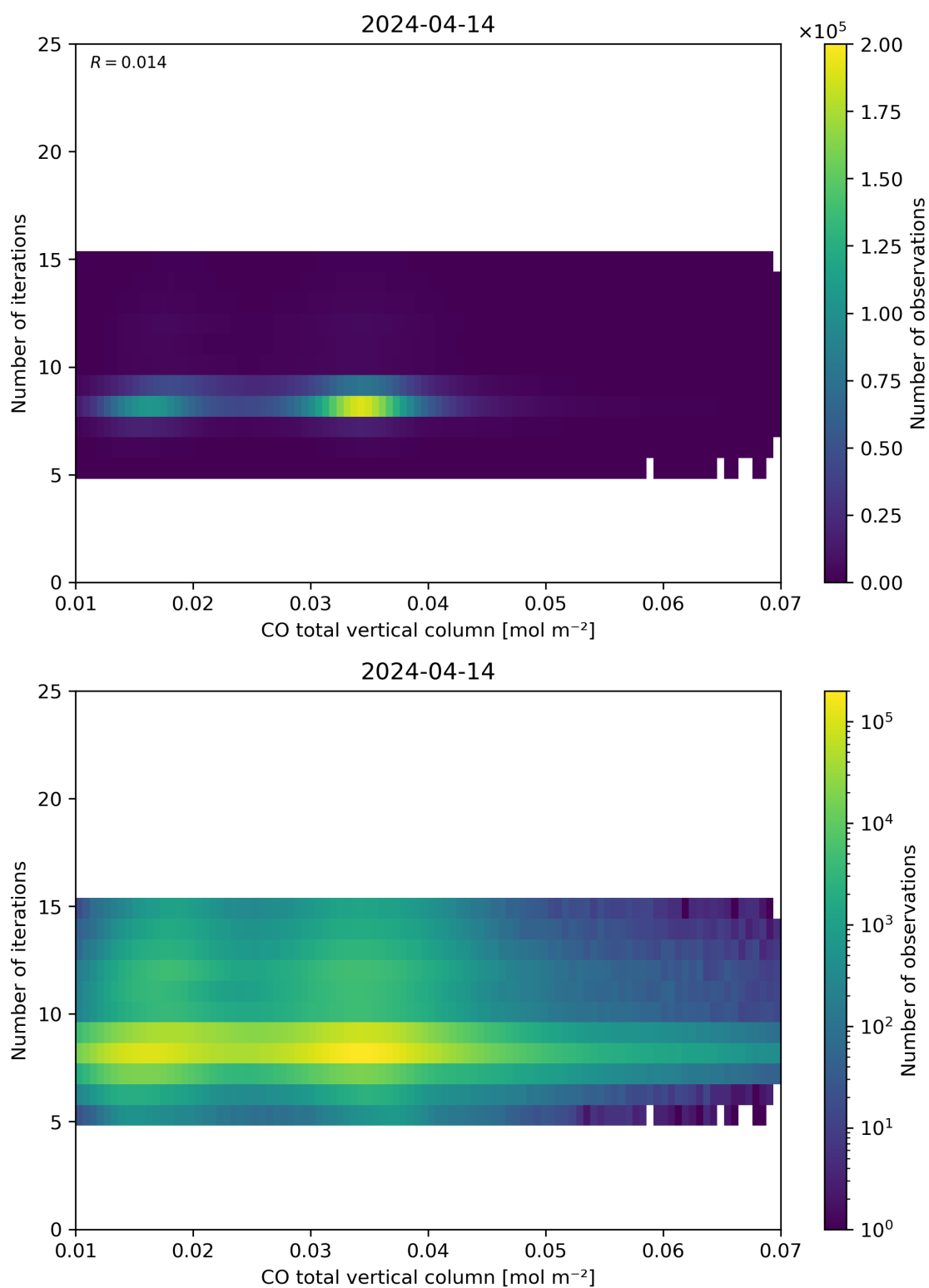
Figure 42: Scatter density plot of “CO total vertical column” against “Number of iterations” for 2024-04-13 to 2024-04-15.
