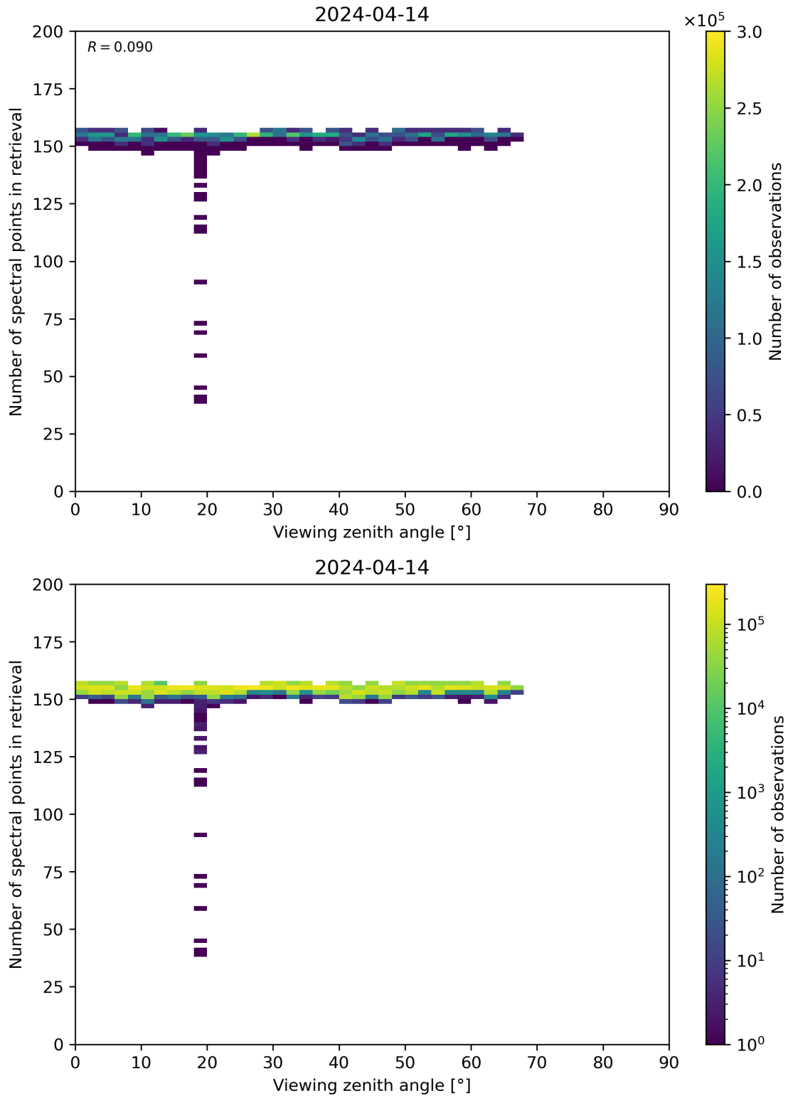
Figure 76: Scatter density plot of “Viewing zenith angle” against “Number of spectral points in retrieval” for 2024-04-13 to 2024-04-15.
