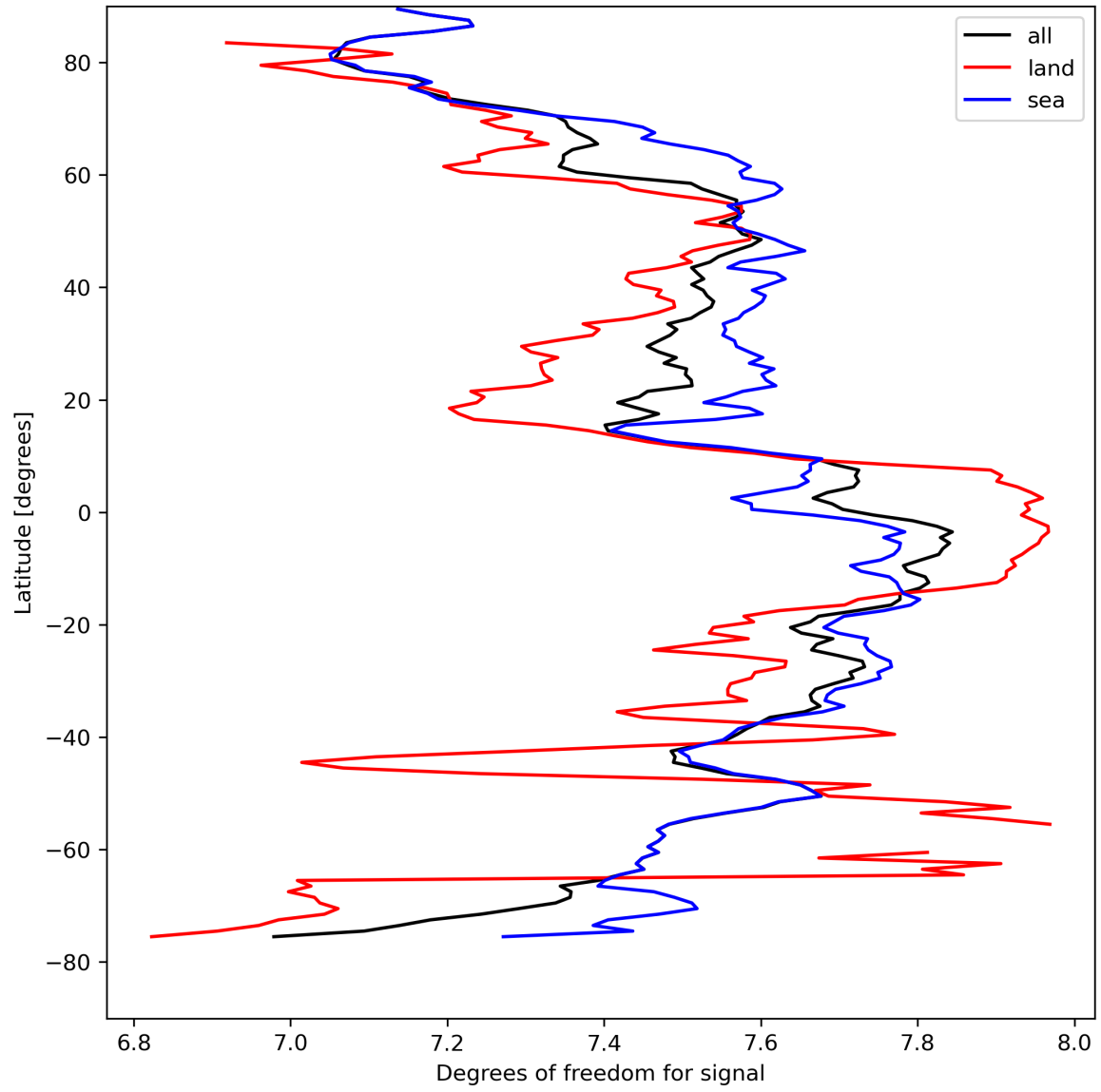
Figure 15: Zonal average of “Degrees of freedom for signal” for 2024-04-13 to 2024-04-15.
