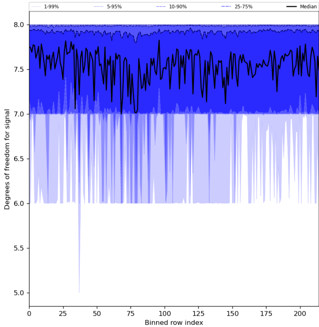
Figure 31: Along track statistics of “Degrees of freedom for signal” for 2024-04-13 to 2024-04-15
