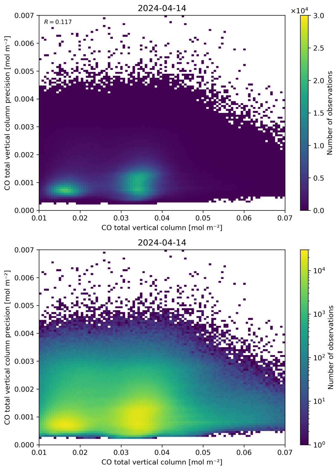
Figure 34: Scatter density plot of “CO total vertical column” against “CO total vertical column precision” for 2024-04-13 to 2024-04-15.
