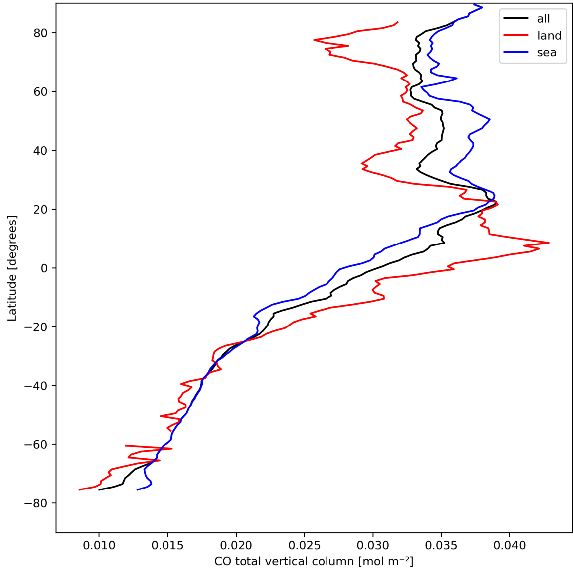
Figure 10: Zonal average of “CO total vertical column” for 2024-04-13 to 2024-04-15.
