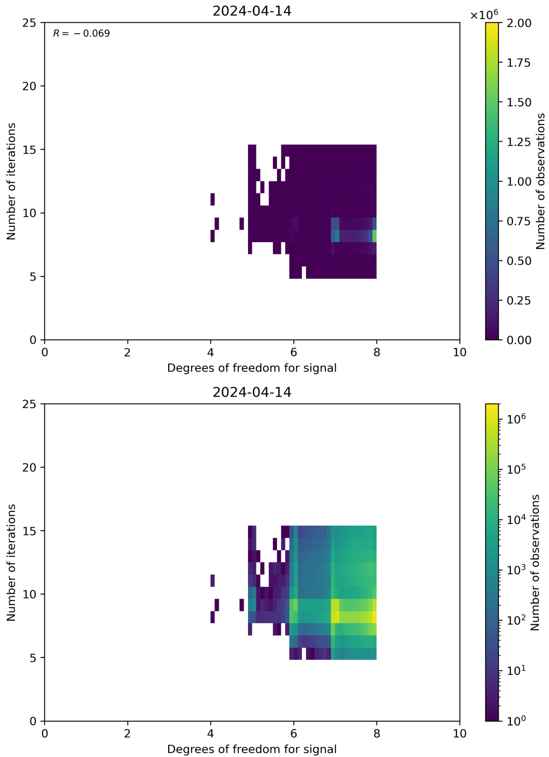
Figure 50: Scatter density plot of “Degrees of freedom for signal” against “Number of iterations” for 2024-04-13 to 2024-04-15.
