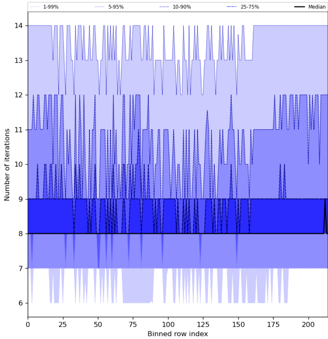
Figure 32: Along track statistics of “Number of iterations” for 2024-04-13 to 2024-04-15
