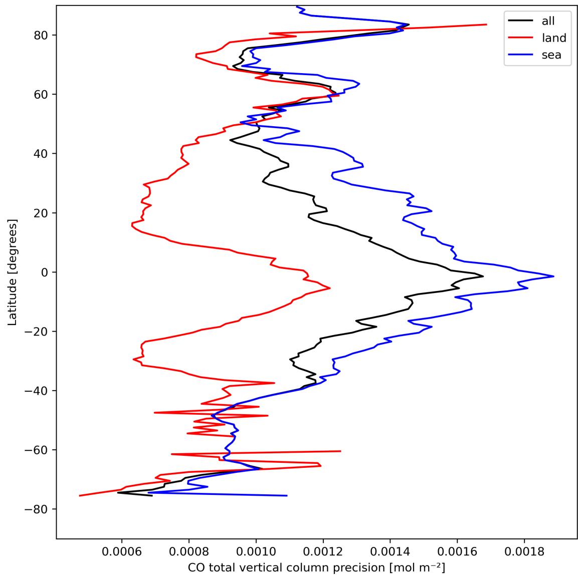
Figure 12: Zonal average of “CO total vertical column precision” for 2024-04-13 to 2024-04-15.
