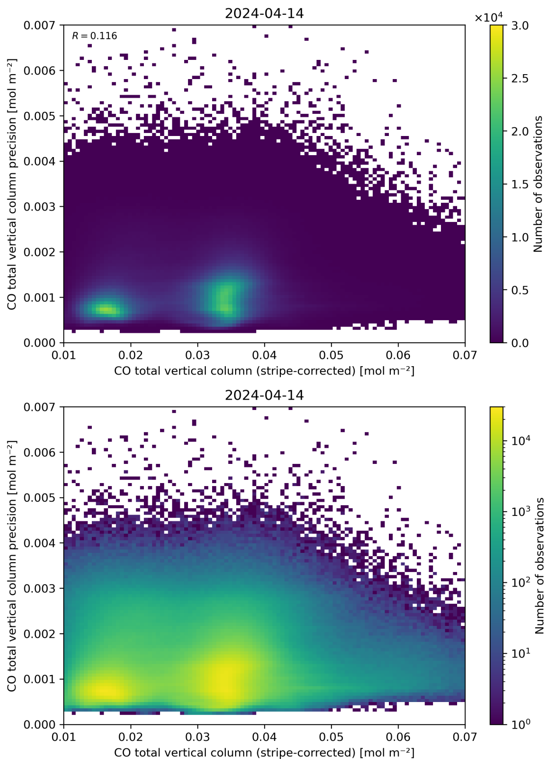
Figure 36: Scatter density plot of “CO total vertical column (stripe-corrected)” against “CO total vertical column precision” for 2024-04-13 to 2024-04-15.
