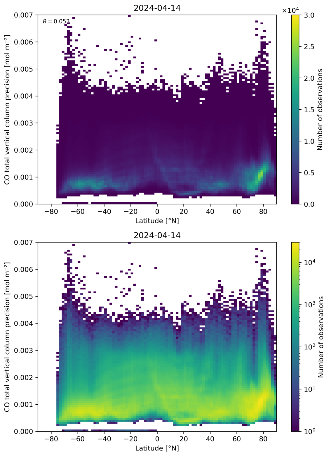
Figure 53: Scatter density plot of “Latitude” against “CO total vertical column precision” for 2024-04-13 to 2024-04-15.
