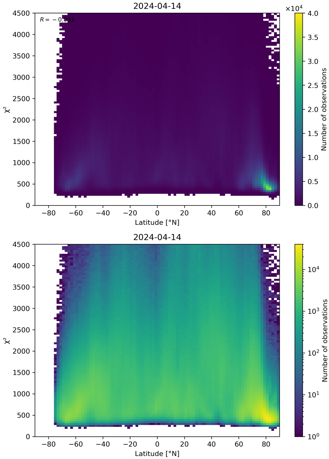
Figure 54: Scatter density plot of “Latitude” against “ \chi^2 ” for 2024-04-13 to 2024-04-15.
