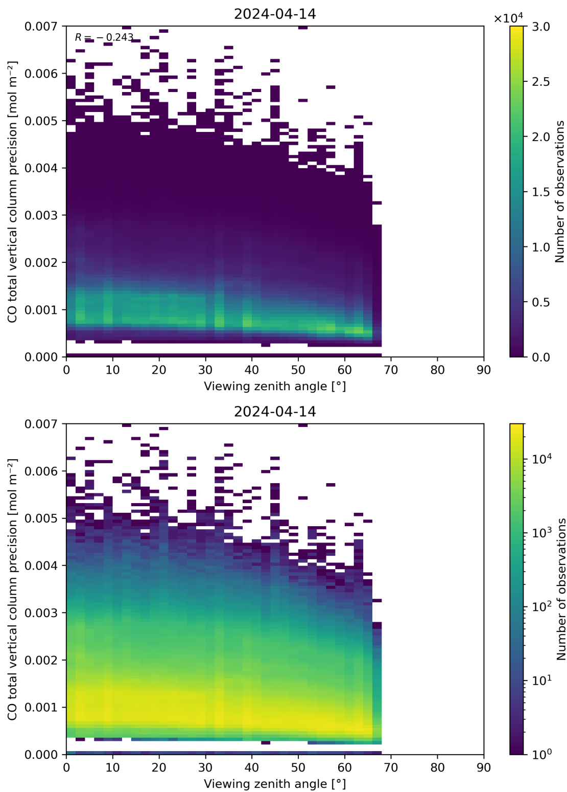
Figure 71: Scatter density plot of “Viewing zenith angle” against “CO total vertical column precision” for 2024-04-13 to 2024-04-15.
