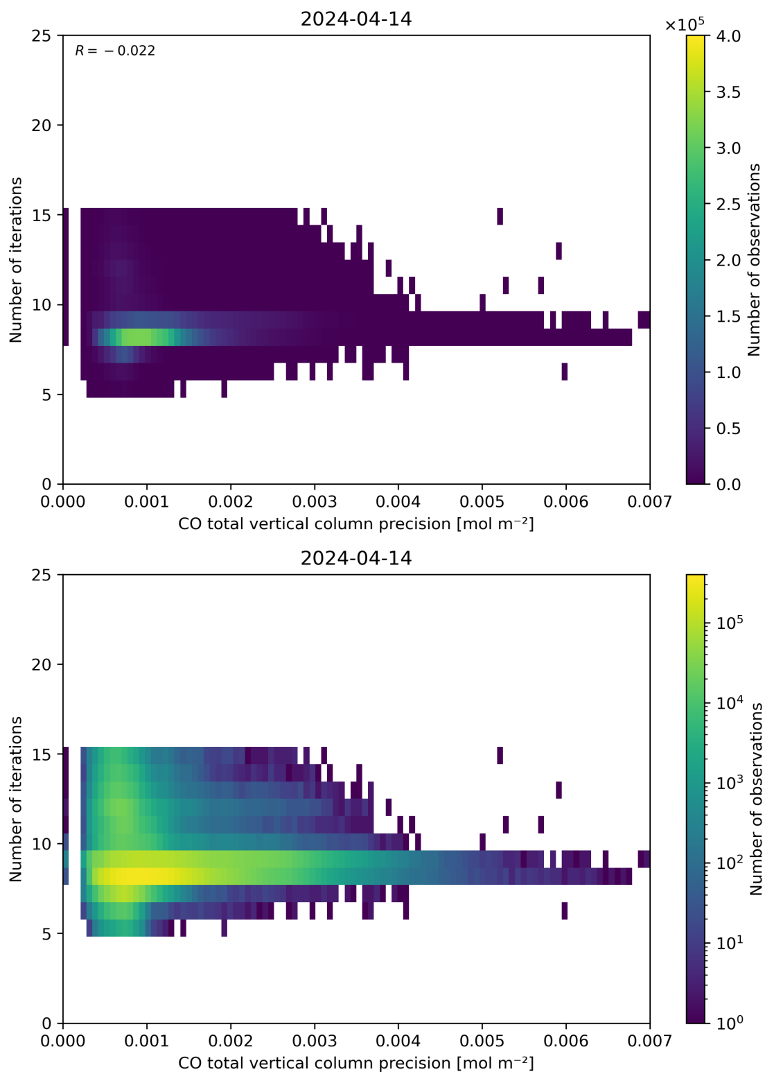
Figure 46: Scatter density plot of “CO total vertical column precision” against “Number of iterations” for 2024-04-13 to 2024-04-15.
