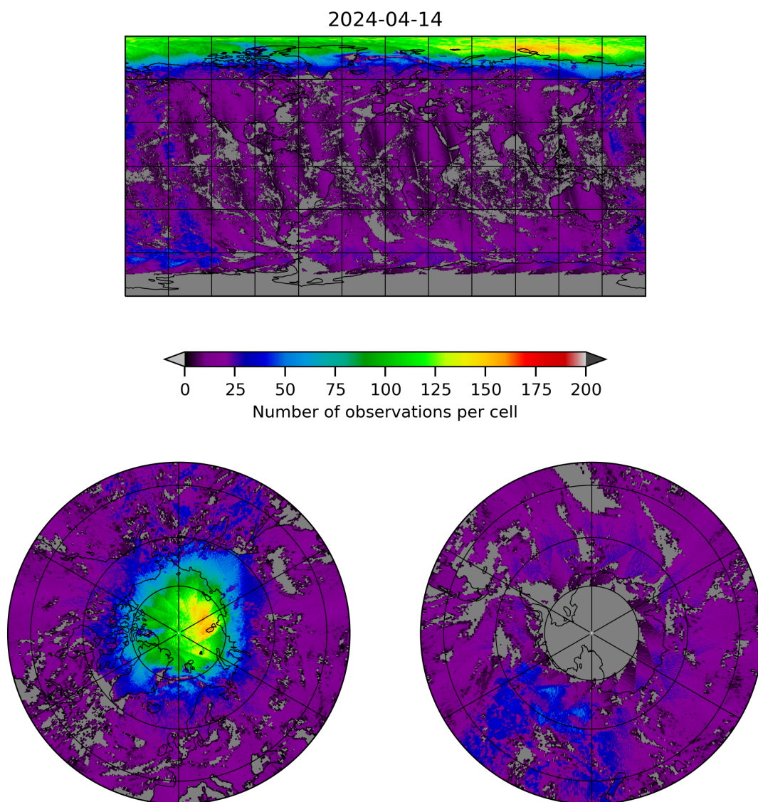
Figure 8: Map of the number of observations for 2024-04-13 to 2024-04-15
