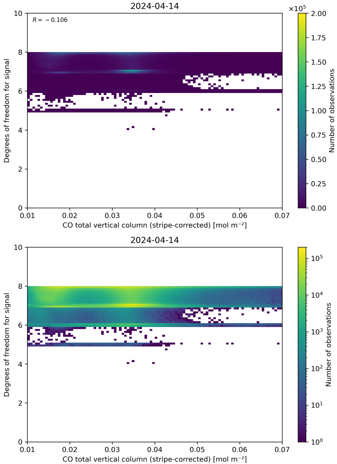
Figure 38: Scatter density plot of “CO total vertical column (stripe-corrected)” against “Degrees of freedom for signal” for 2024-04-13 to 2024-04-15.
