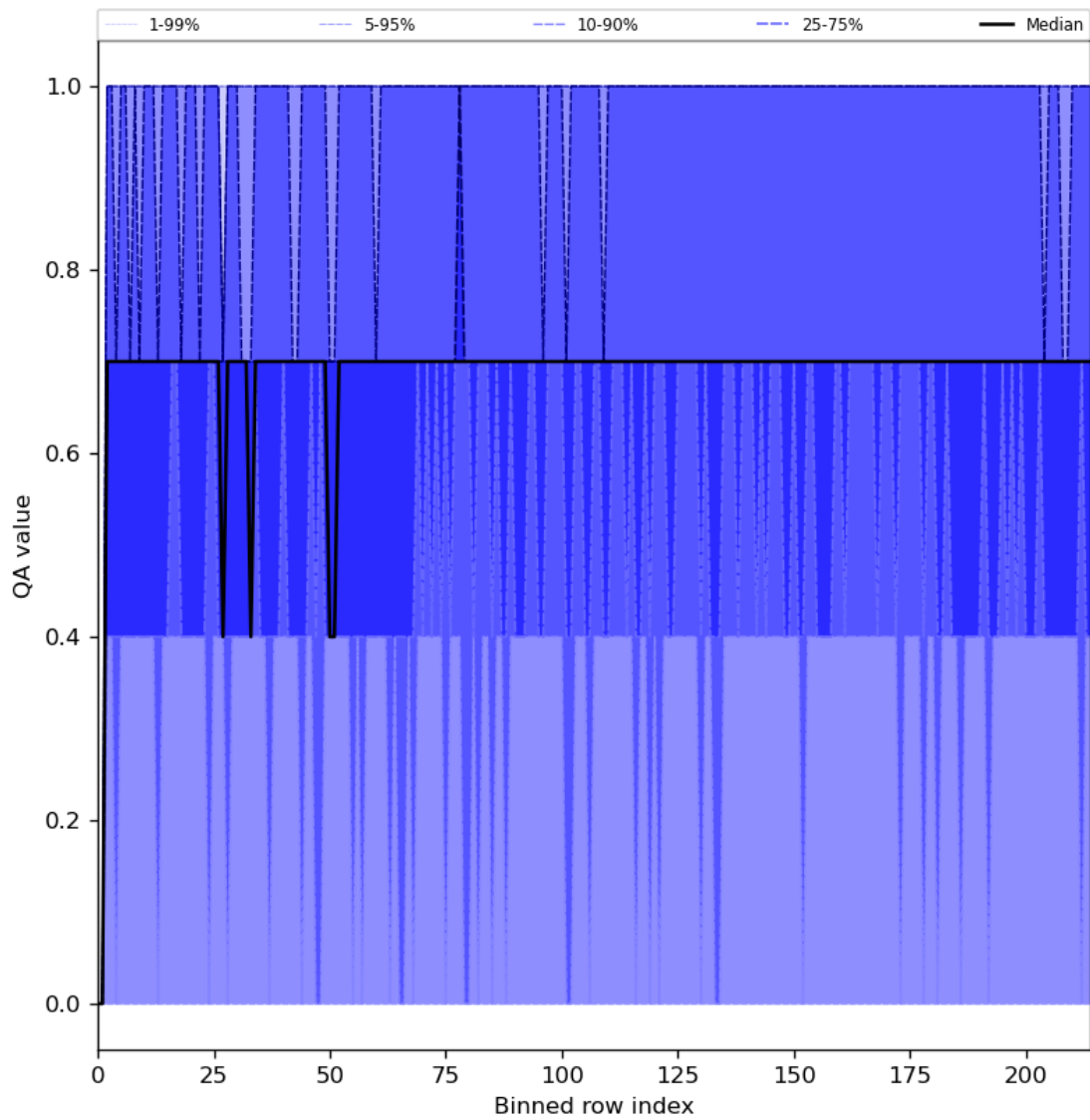
Figure 25: Along track statistics of “QA value” for 2024-04-13 to 2024-04-15
