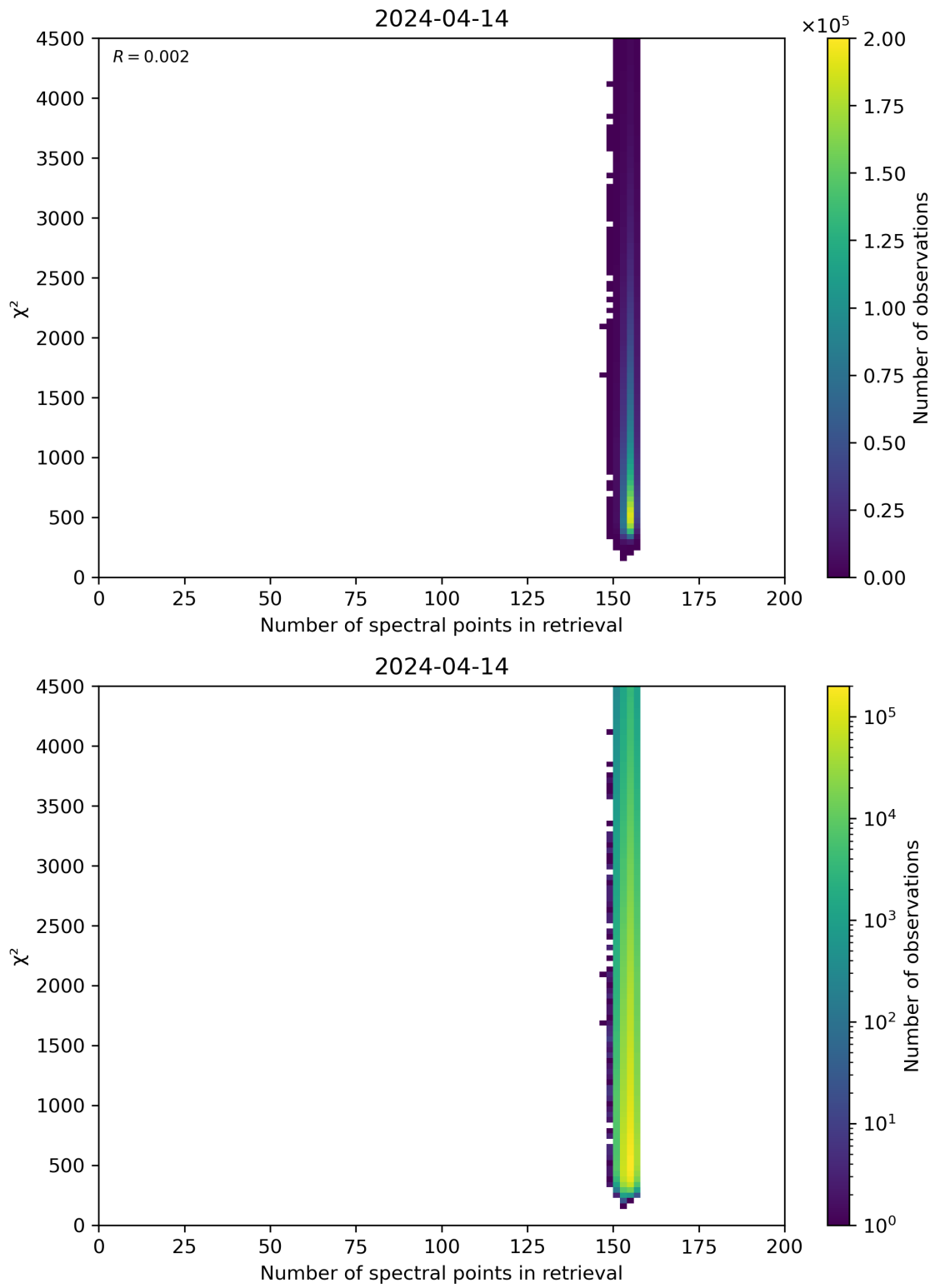
Figure 58: Scatter density plot of “Number of spectral points in retrieval” against “ \chi^2 ” for 2024-04-13 to 2024-04-15.
