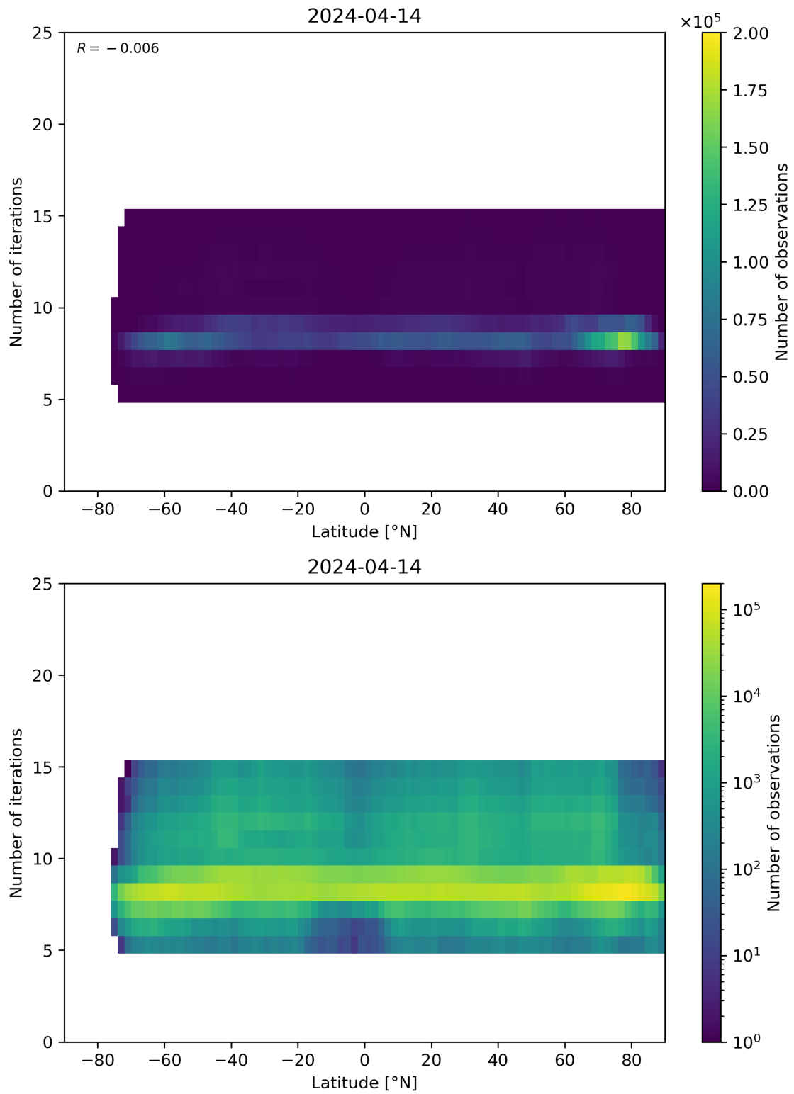
Figure 56: Scatter density plot of “Latitude” against “Number of iterations” for 2024-04-13 to 2024-04-15.
