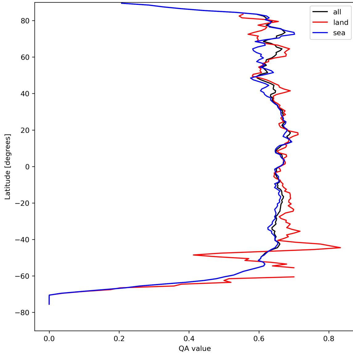
Figure 9: Zonal average of “QA value” for 2024-04-13 to 2024-04-15.
