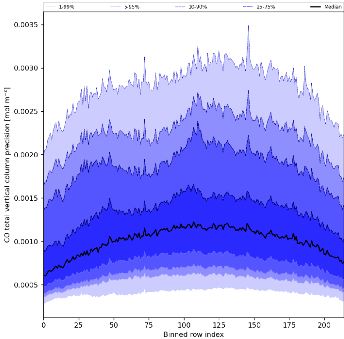
Figure 28: Along track statistics of “CO total vertical column precision” for 2024-04-13 to 2024-04-15
