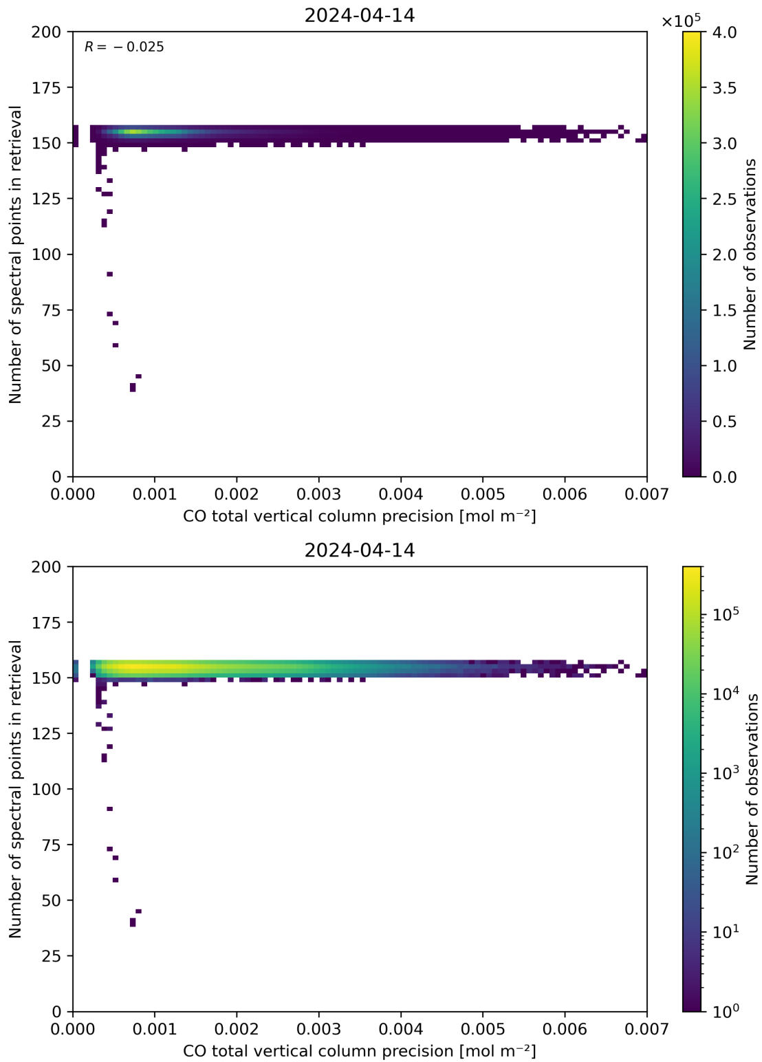
Figure 47: Scatter density plot of “CO total vertical column precision” against “Number of spectral points in retrieval” for 2024-04-13 to 2024-04-15.
