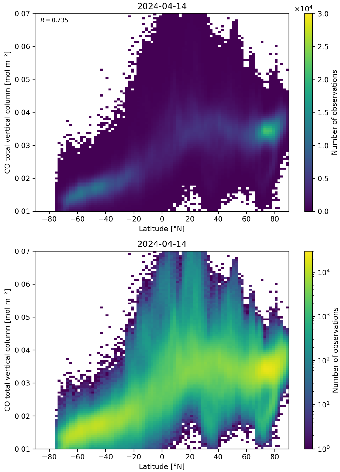
Figure 51: Scatter density plot of “Latitude” against “CO total vertical column” for 2024-04-13 to 2024-04-15.
