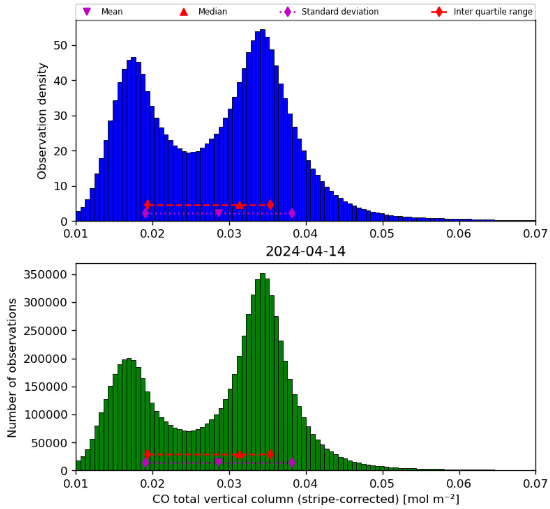
Figure 19: Histogram of “CO total vertical column (stripe-corrected)” for 2024-04-13 to 2024-04-15
