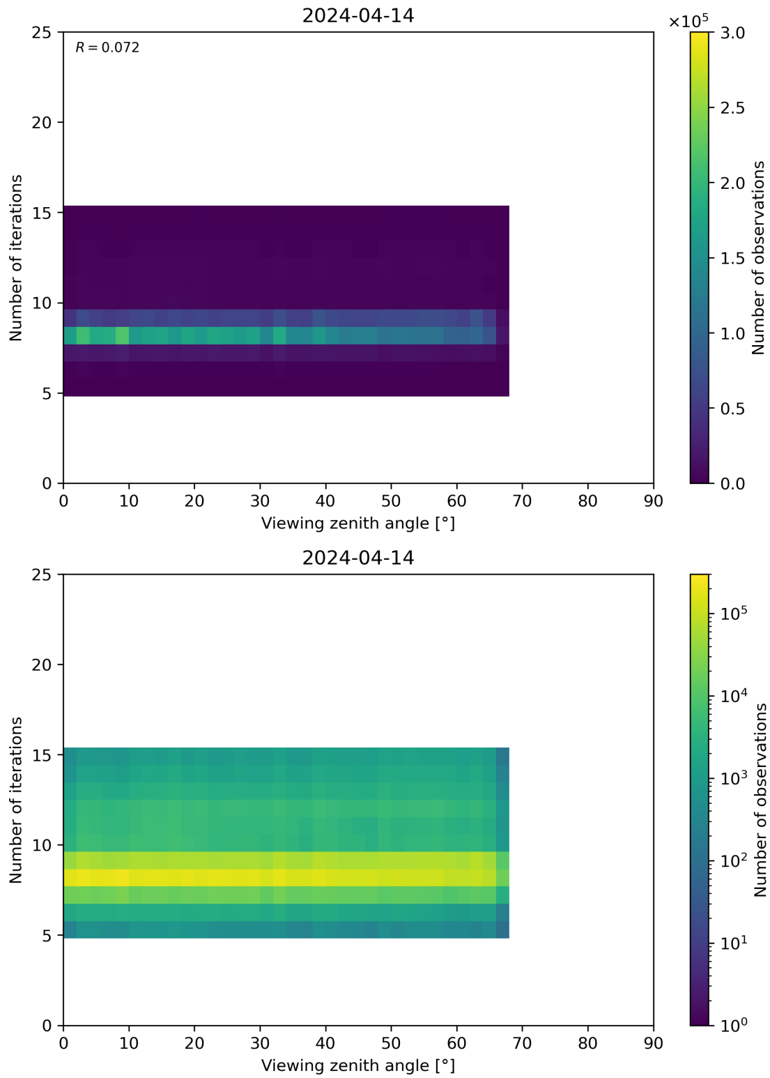
Figure 75: Scatter density plot of “Viewing zenith angle” against “Number of iterations” for 2024-04-13 to 2024-04-15.
