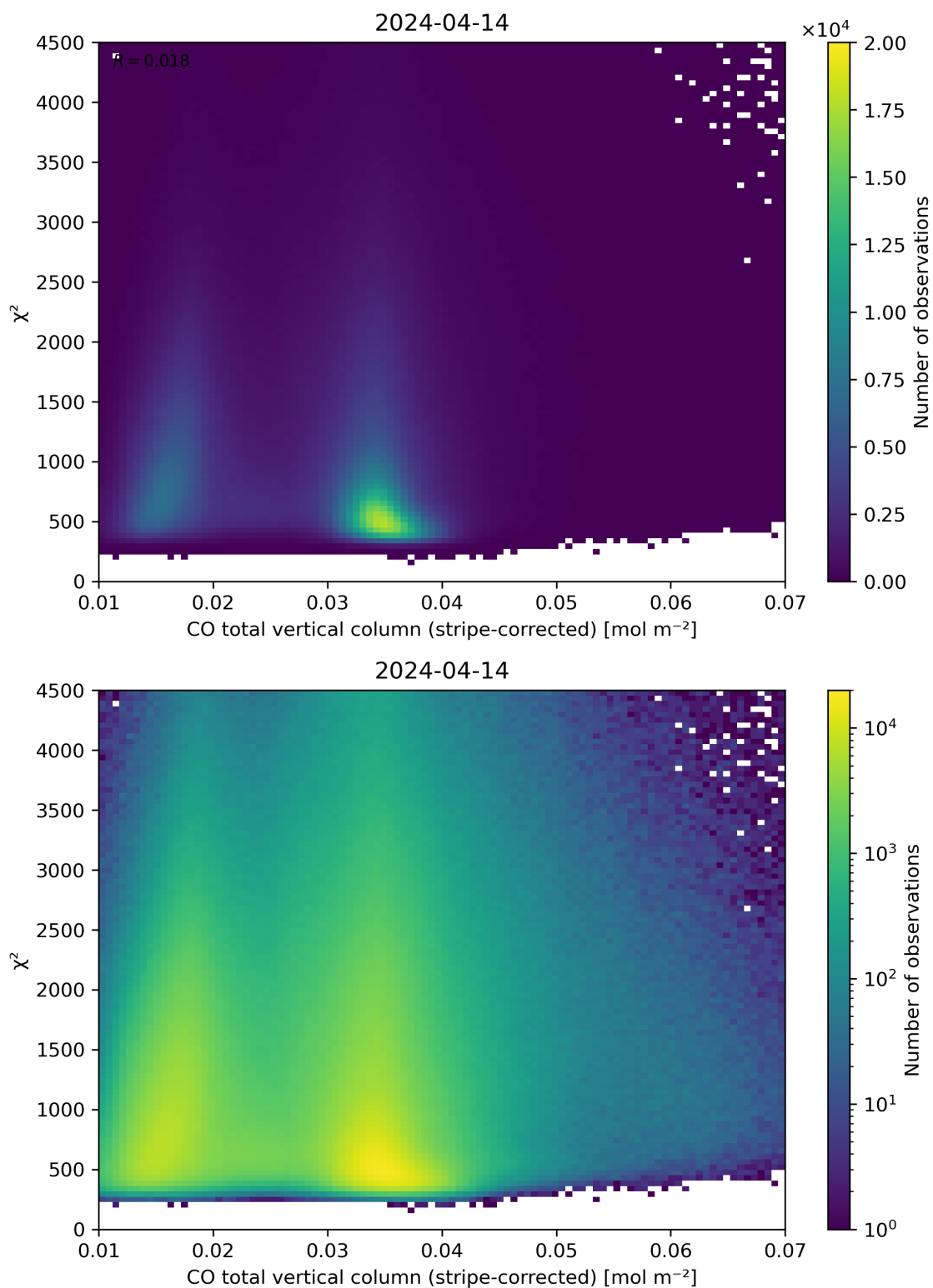
Figure 37: Scatter density plot of “CO total vertical column (stripe-corrected)” against “ \chi^2 ” for 2024-04-13 to 2024-04-15.
