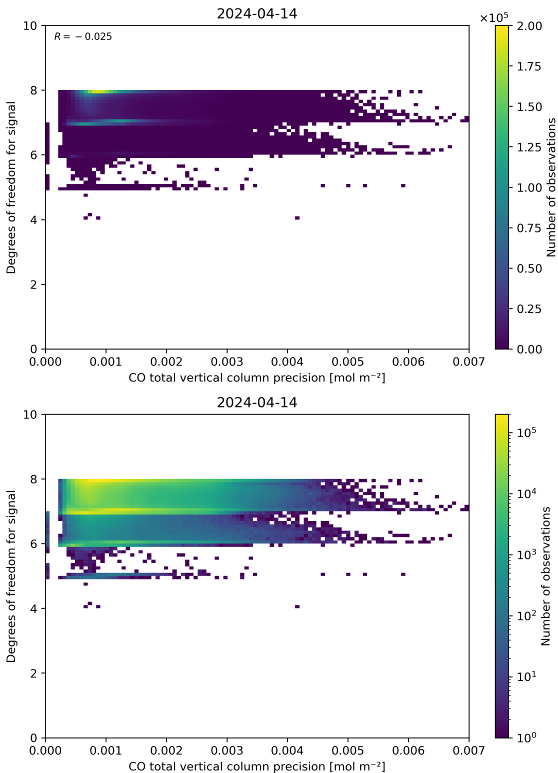
Figure 45: Scatter density plot of “CO total vertical column precision” against “Degrees of freedom for signal” for 2024-04-13 to 2024-04-15.
