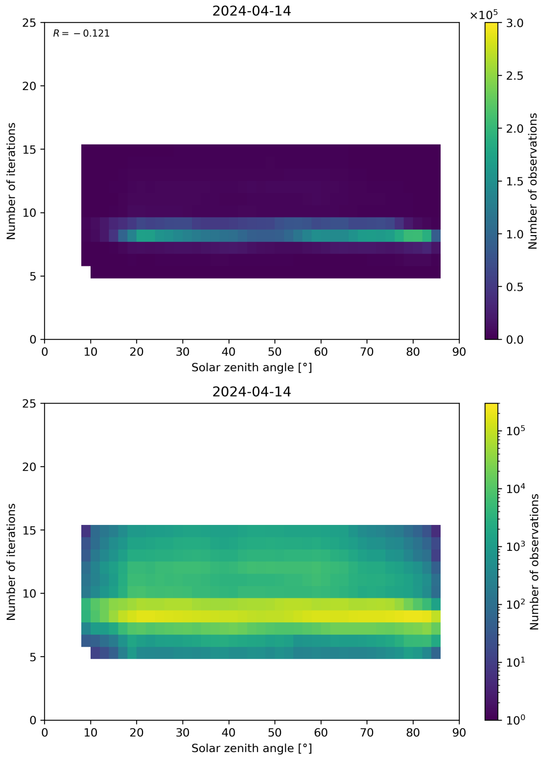
Figure 67: Scatter density plot of “Solar zenith angle” against “Number of iterations” for 2024-04-13 to 2024-04-15.
