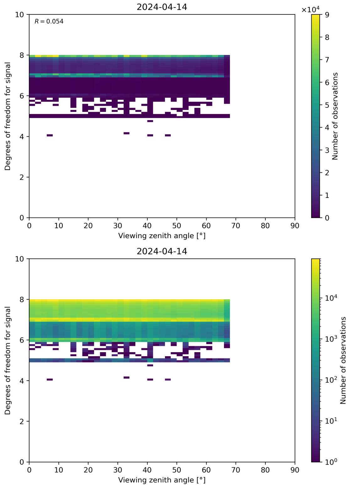
Figure 73: Scatter density plot of “Viewing zenith angle” against “Degrees of freedom for signal” for 2024-04-13 to 2024-04-15.
