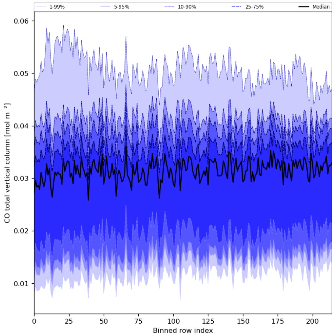
Figure 26: Along track statistics of “CO total vertical column” for 2024-04-13 to 2024-04-15
