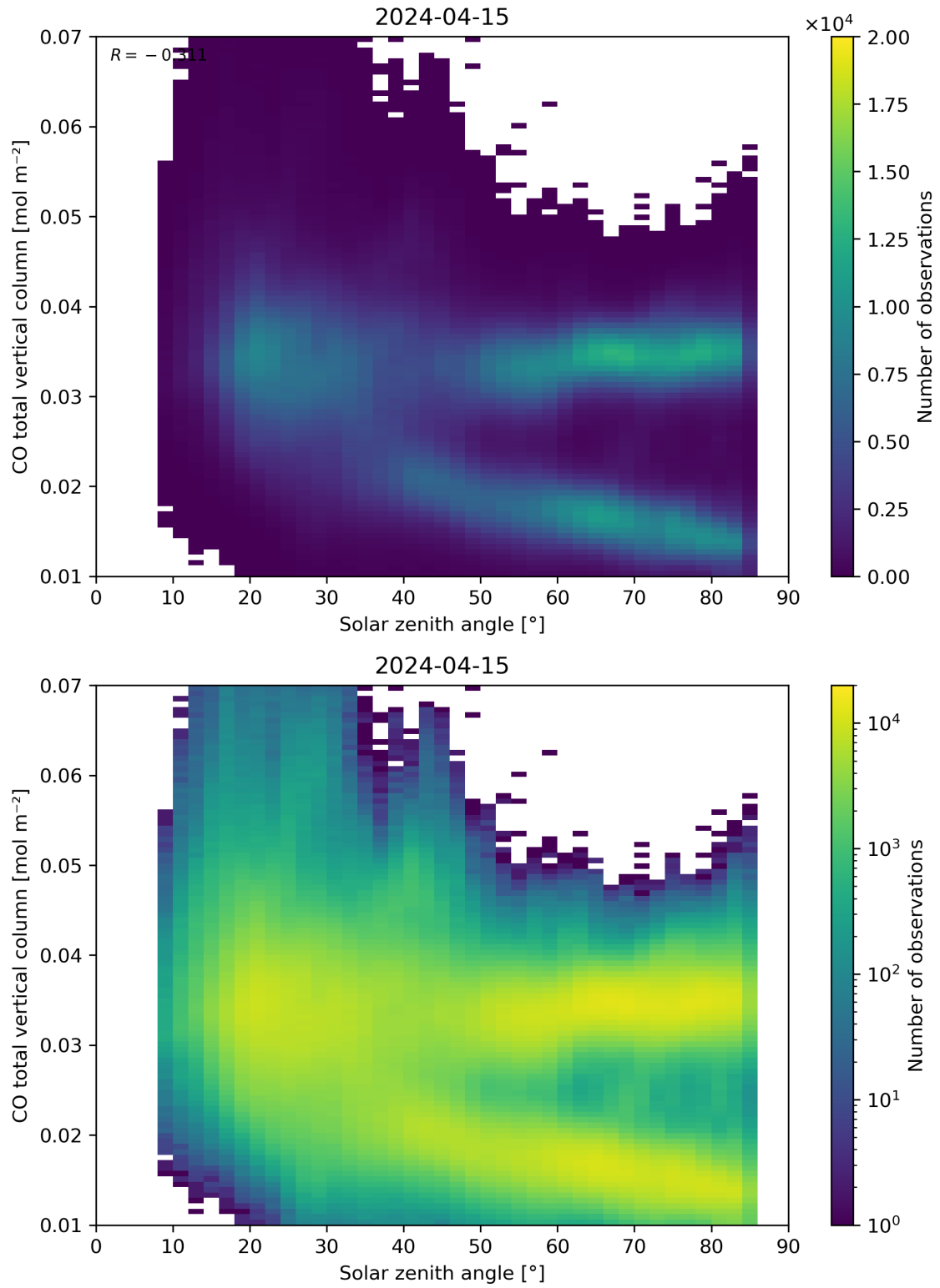
Figure 61: Scatter density plot of “Solar zenith angle” against “CO total vertical column” for 2024-04-15 to 2024-04-16.
