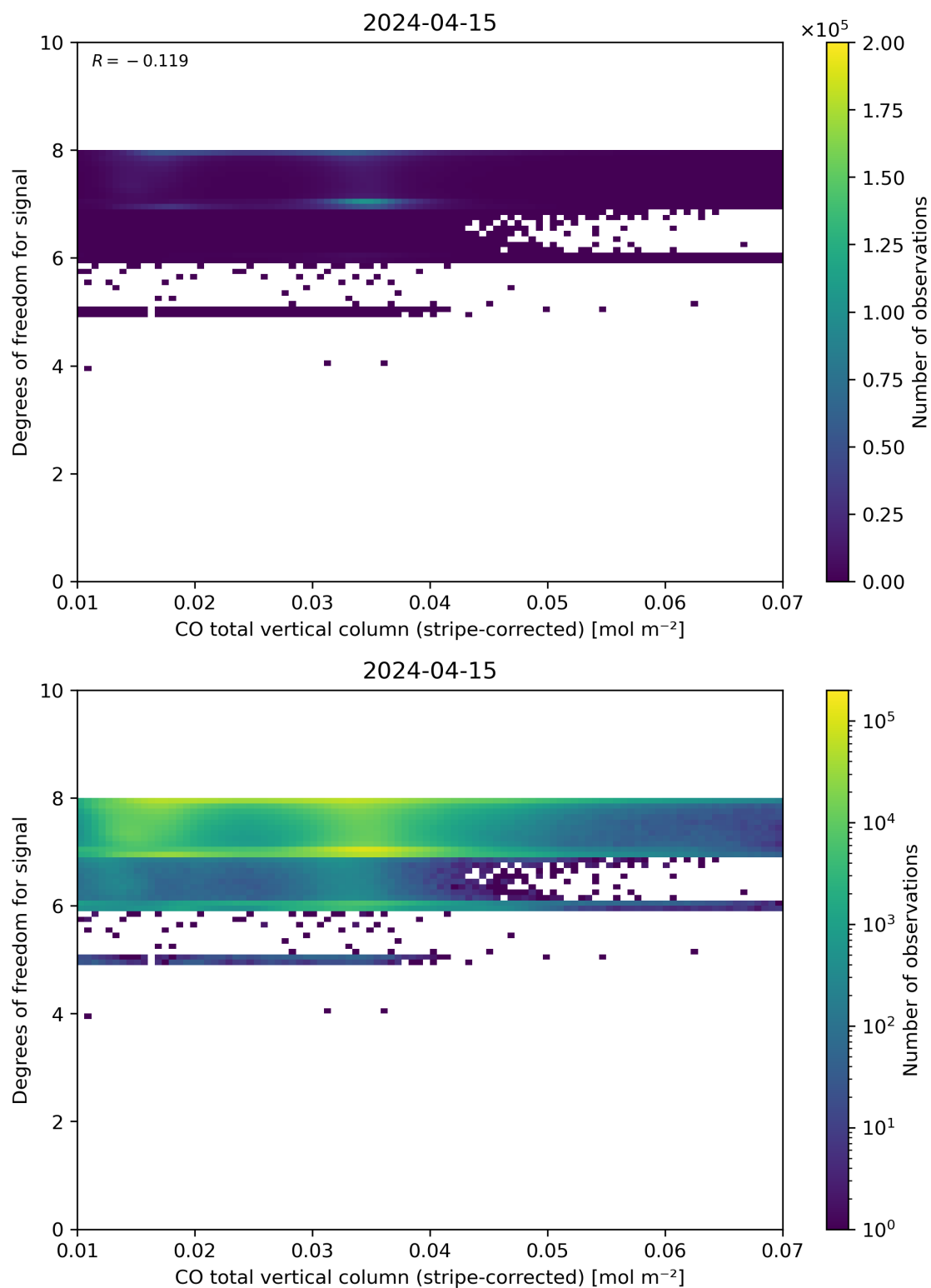
Figure 38: Scatter density plot of “CO total vertical column (stripe-corrected)” against “Degrees of freedom for signal” for 2024-04-15 to 2024-04-16.
