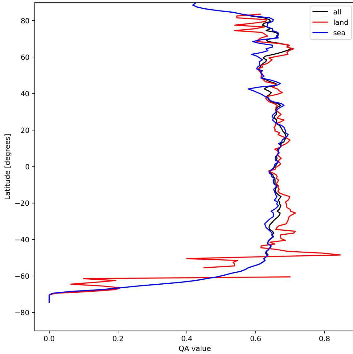
Figure 9: Zonal average of “QA value” for 2024-04-15 to 2024-04-16.
