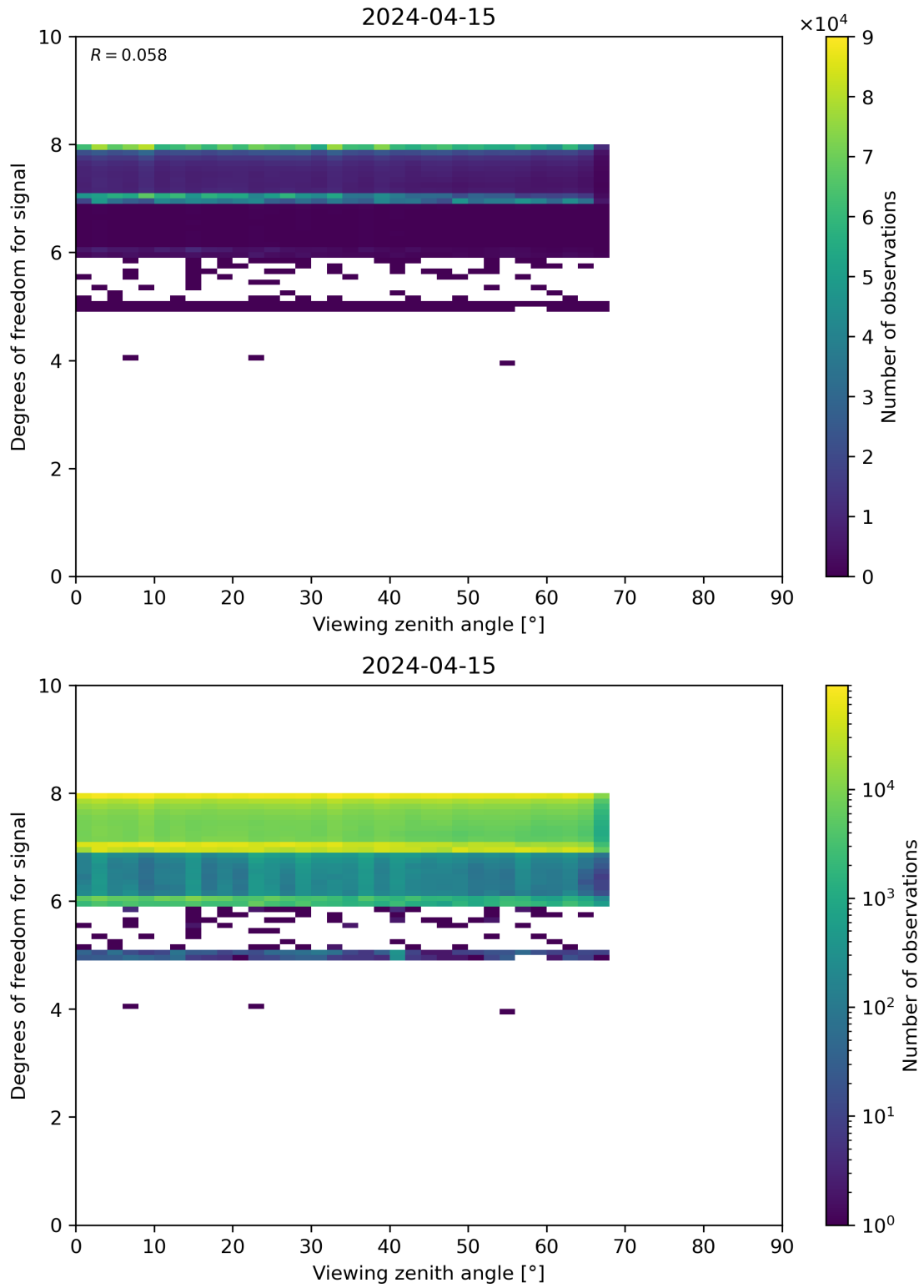
Figure 73: Scatter density plot of “Viewing zenith angle” against “Degrees of freedom for signal” for 2024-04-15 to 2024-04-16.
