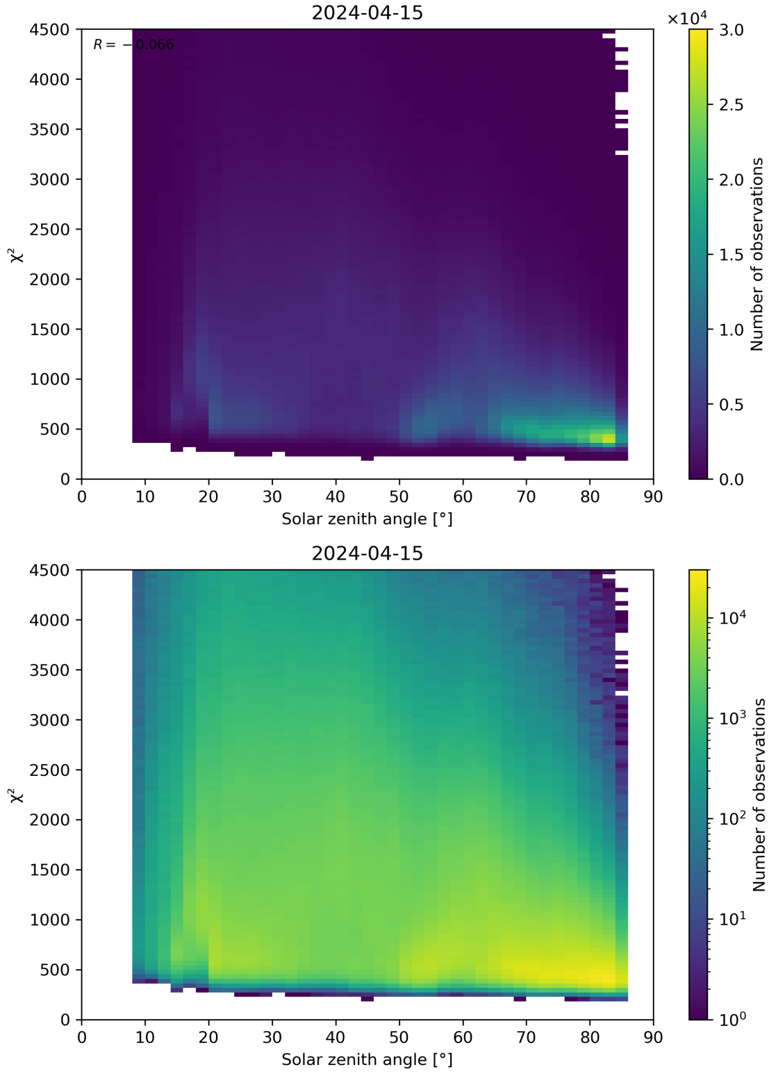
Figure 64: Scatter density plot of “Solar zenith angle” against “ \chi^2 ” for 2024-04-15 to 2024-04-16.
