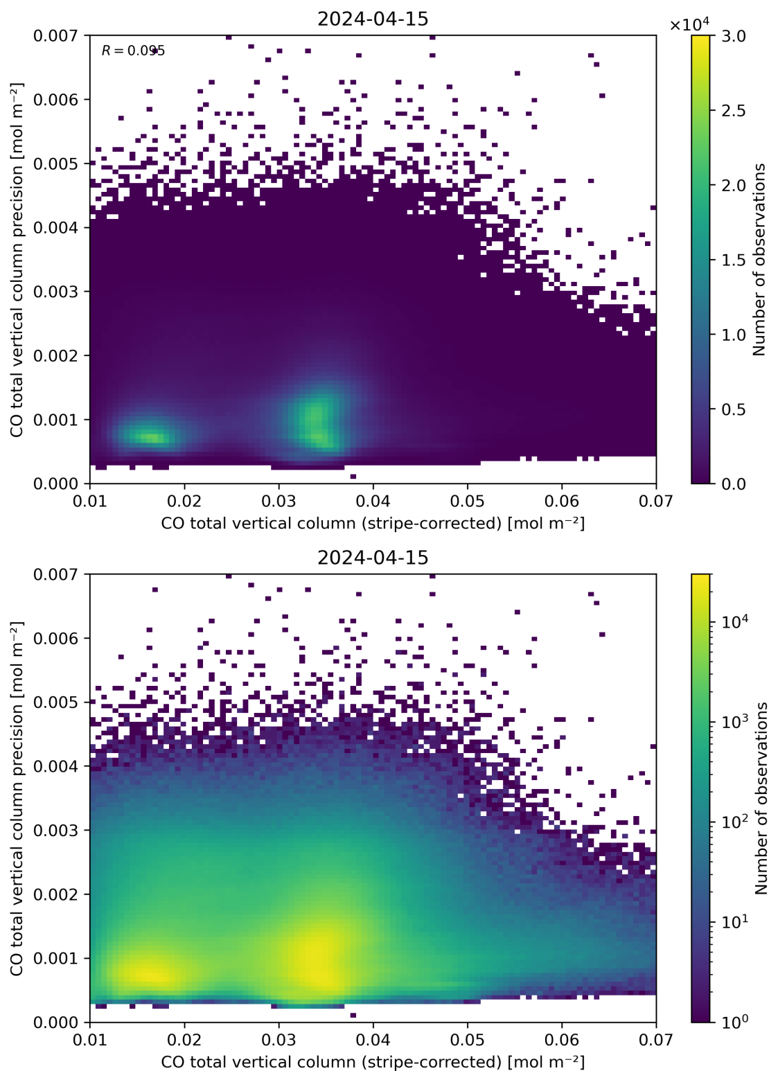
Figure 36: Scatter density plot of “CO total vertical column (stripe-corrected)” against “CO total vertical column precision” for 2024-04-15 to 2024-04-16.
