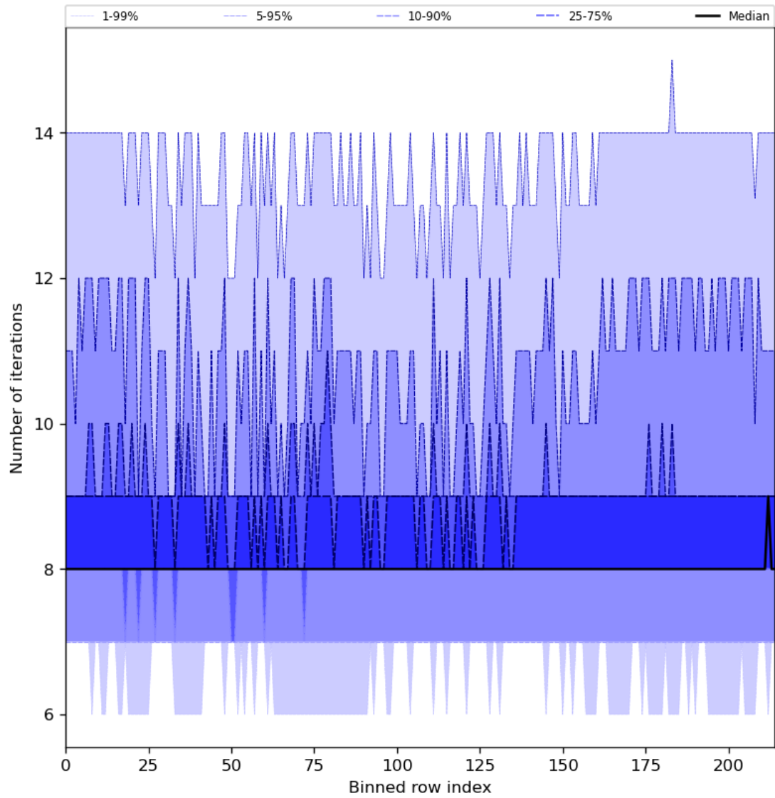
Figure 32: Along track statistics of “Number of iterations” for 2024-04-15 to 2024-04-16
