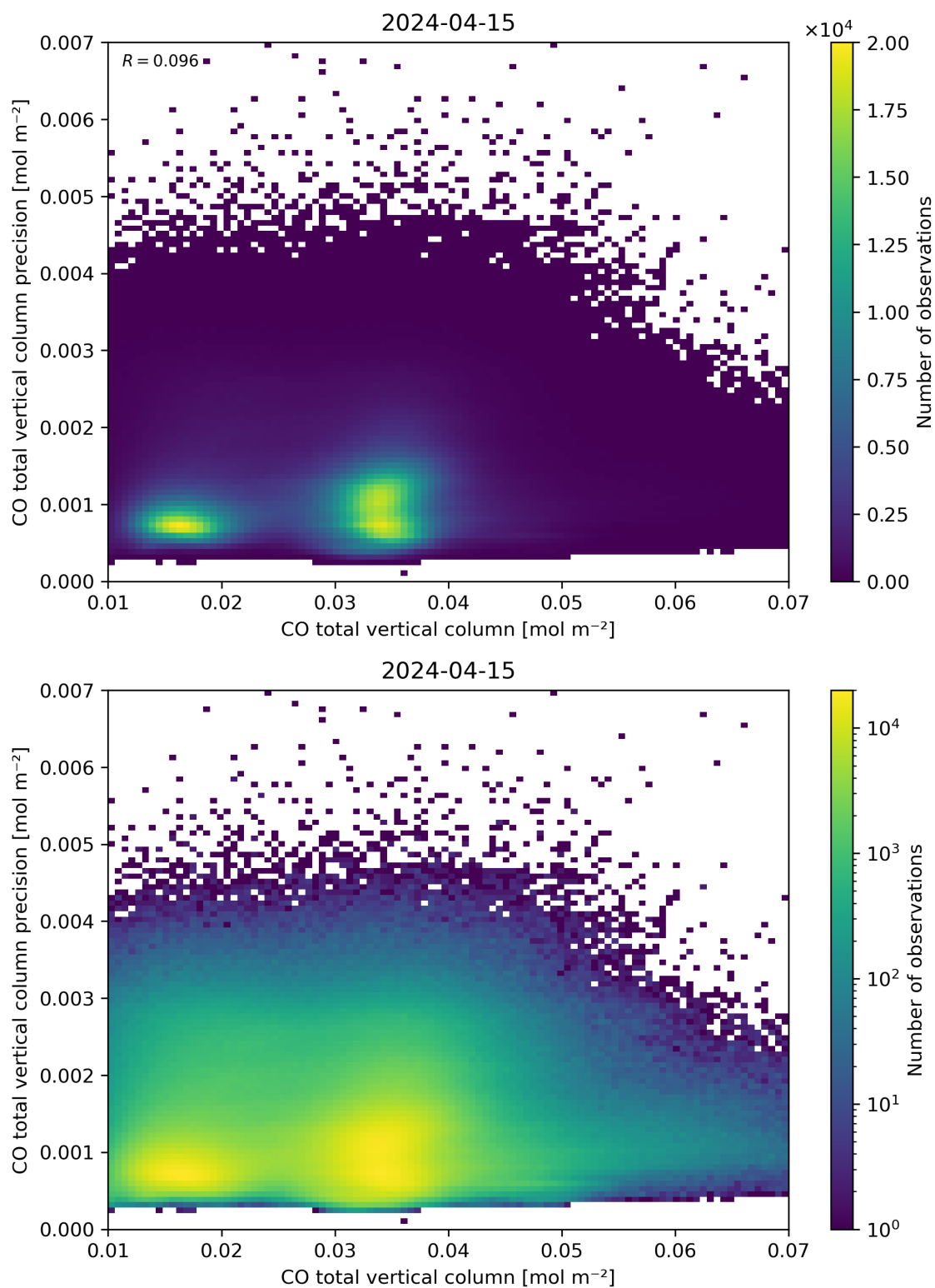
Figure 34: Scatter density plot of “CO total vertical column” against “CO total vertical column precision” for 2024-04-15 to 2024-04-16.
