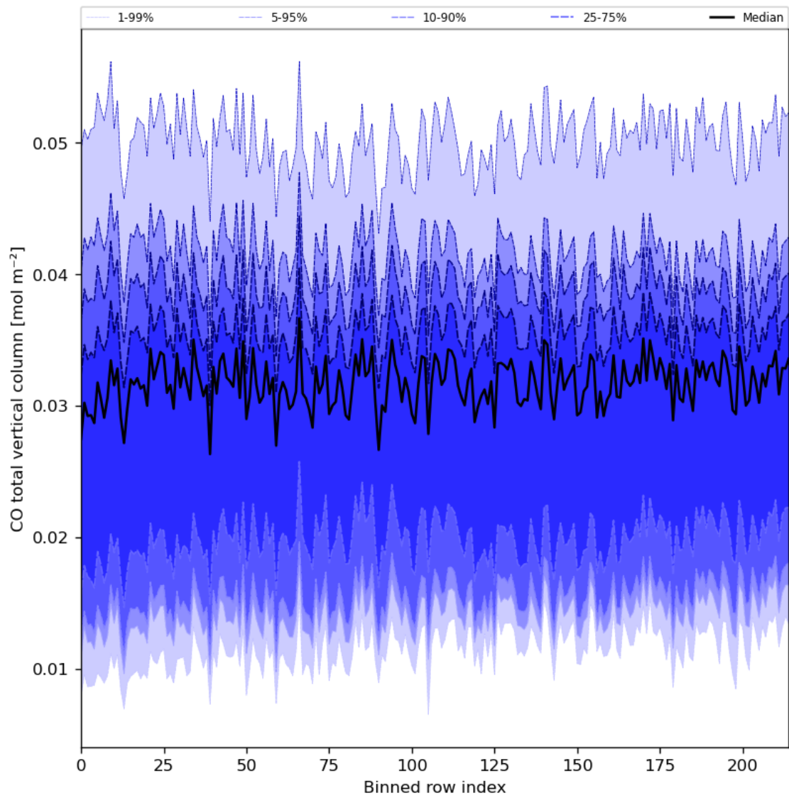
Figure 26: Along track statistics of “CO total vertical column” for 2024-04-15 to 2024-04-16
