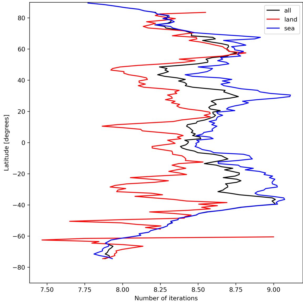
Figure 16: Zonal average of “Number of iterations” for 2024-04-15 to 2024-04-16.
