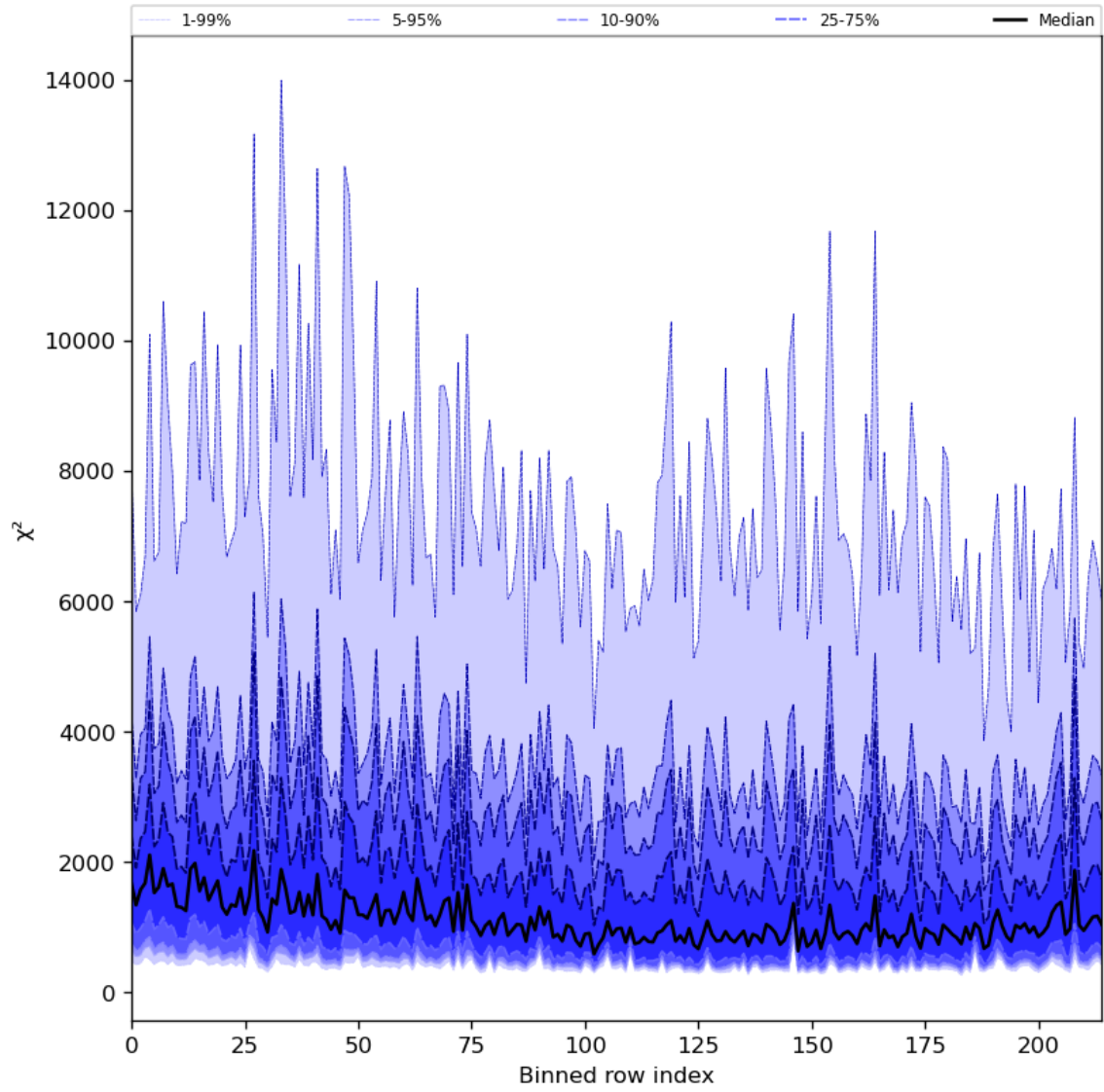
Figure 30: Along track statistics of “ \chi^2 ” for 2024-04-15 to 2024-04-16
