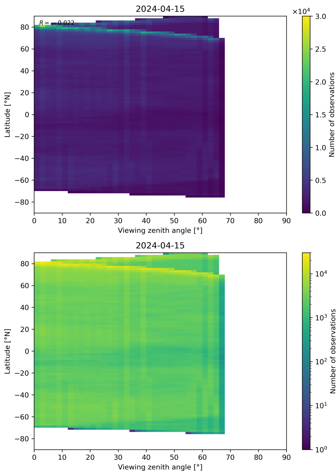
Figure 74: Scatter density plot of “Viewing zenith angle” against “Latitude” for 2024-04-15 to 2024-04-16.
