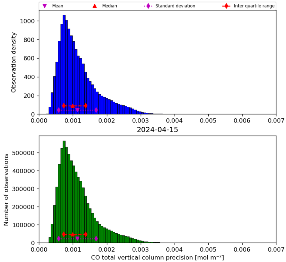
Figure 20: Histogram of “CO total vertical column precision” for 2024-04-15 to 2024-04-16
