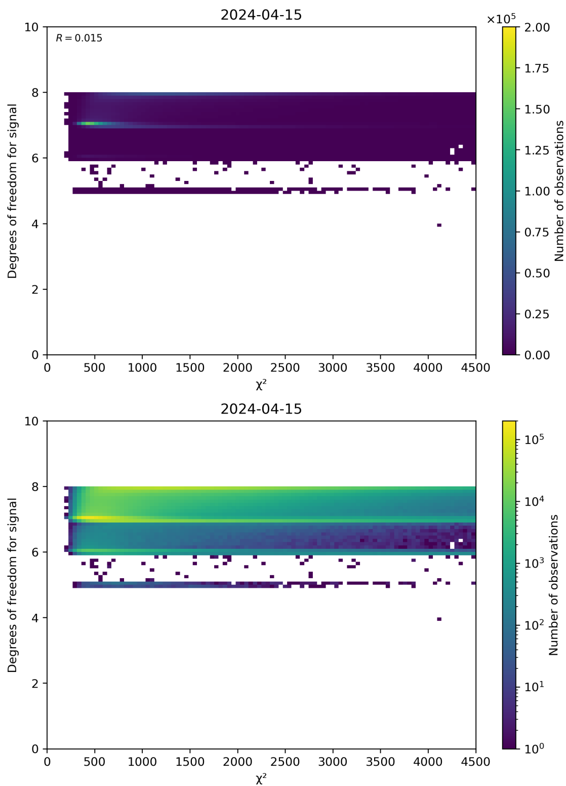
Figure 48: Scatter density plot of " \chi^2 " against "Degrees of freedom for signal" for 2024-04-15 to 2024-04-16.
