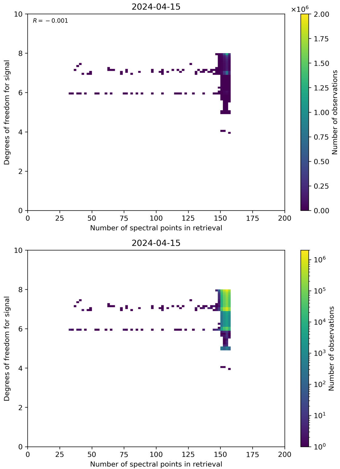
Figure 59: Scatter density plot of “Number of spectral points in retrieval” against “Degrees of freedom for signal” for 2024-04-15 to 2024-04-16.
