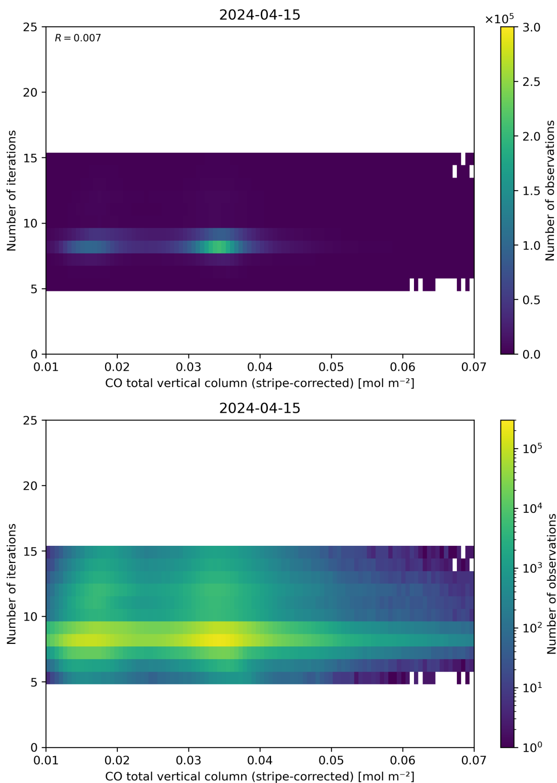
Figure 39: Scatter density plot of “CO total vertical column (stripe-corrected)” against “Number of iterations” for 2024-04-15 to 2024-04-16.
