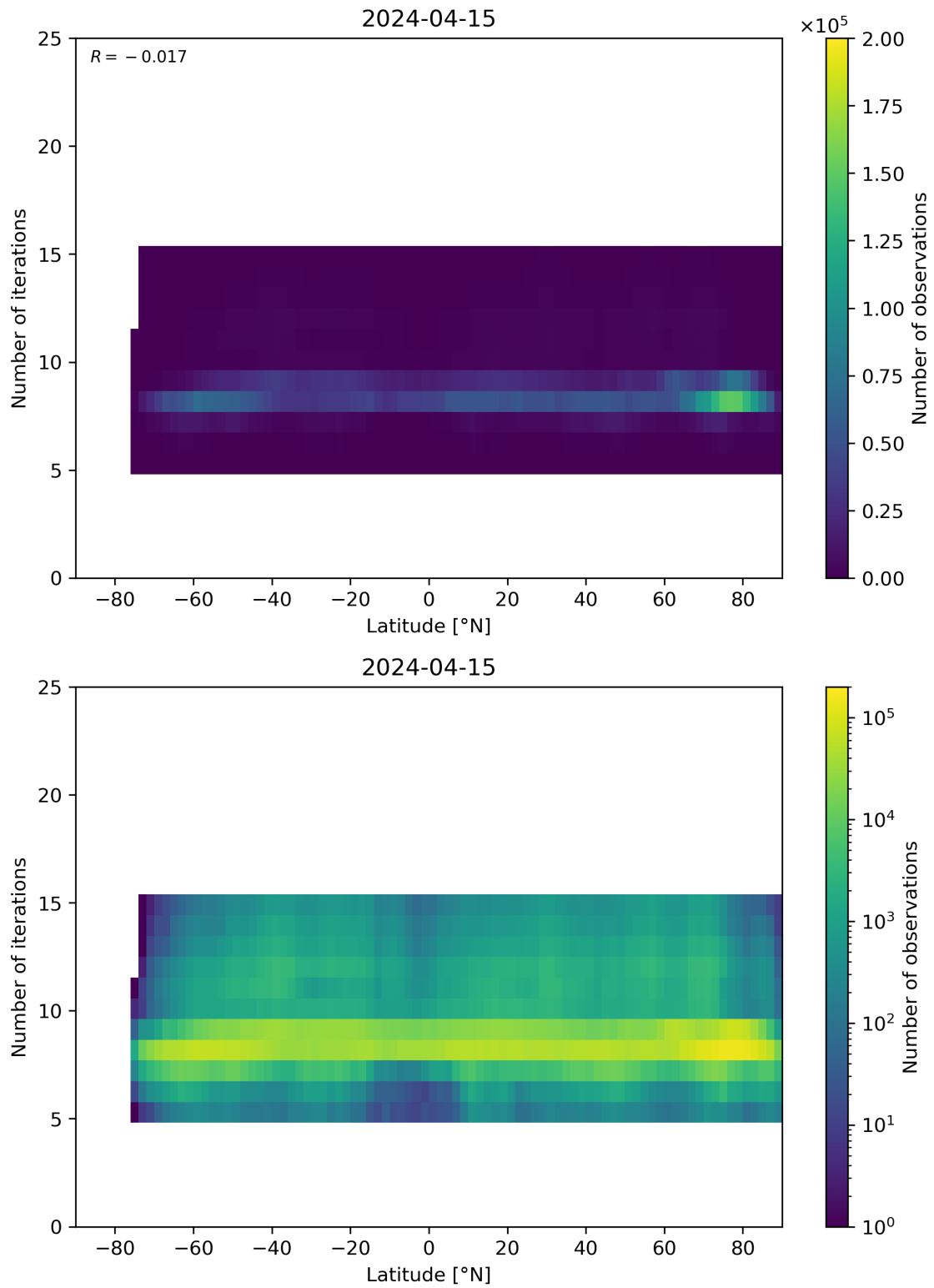
Figure 56: Scatter density plot of “Latitude” against “Number of iterations” for 2024-04-15 to 2024-04-16.
