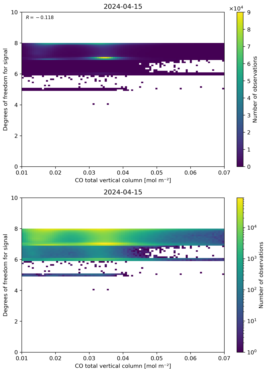
Figure 41: Scatter density plot of “CO total vertical column” against “Degrees of freedom for signal” for 2024-04-15 to 2024-04-16.
