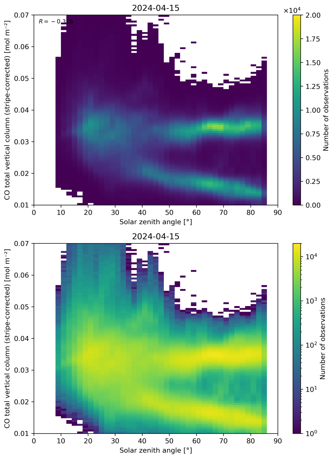
Figure 62: Scatter density plot of “Solar zenith angle” against “CO total vertical column (stripe-corrected)” for 2024-04-15 to 2024-04-16.
