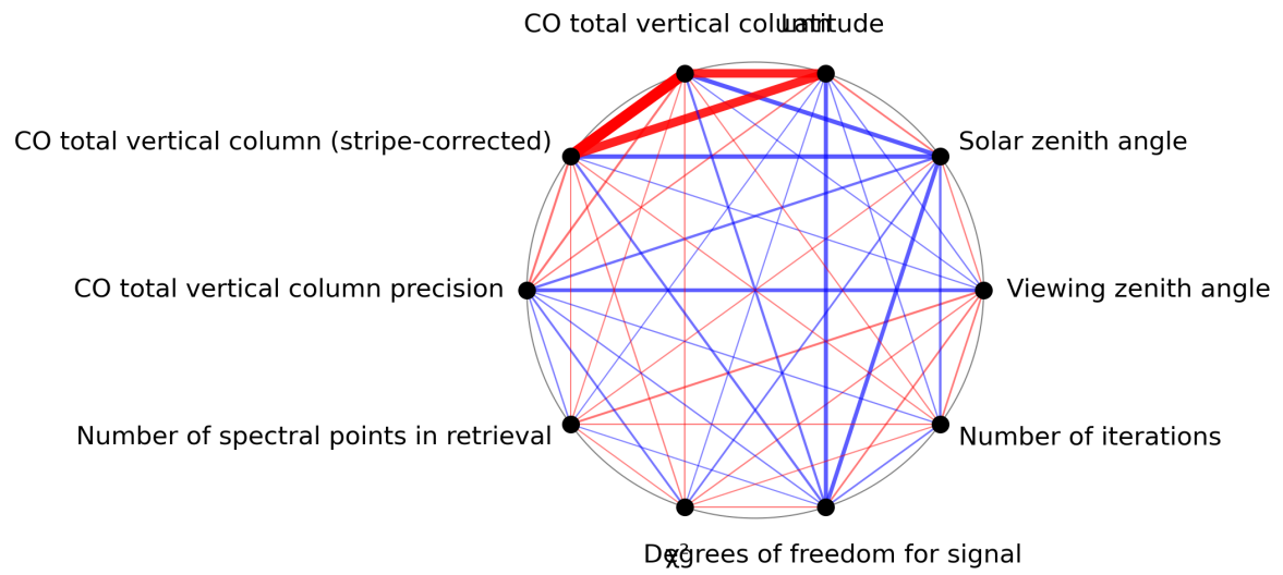
Figure 1: Map of correlation graph for 2024-04-15 to 2024-04-16.
