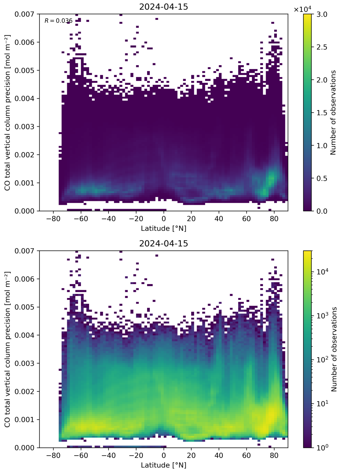
Figure 53: Scatter density plot of “Latitude” against “CO total vertical column precision” for 2024-04-15 to 2024-04-16.
