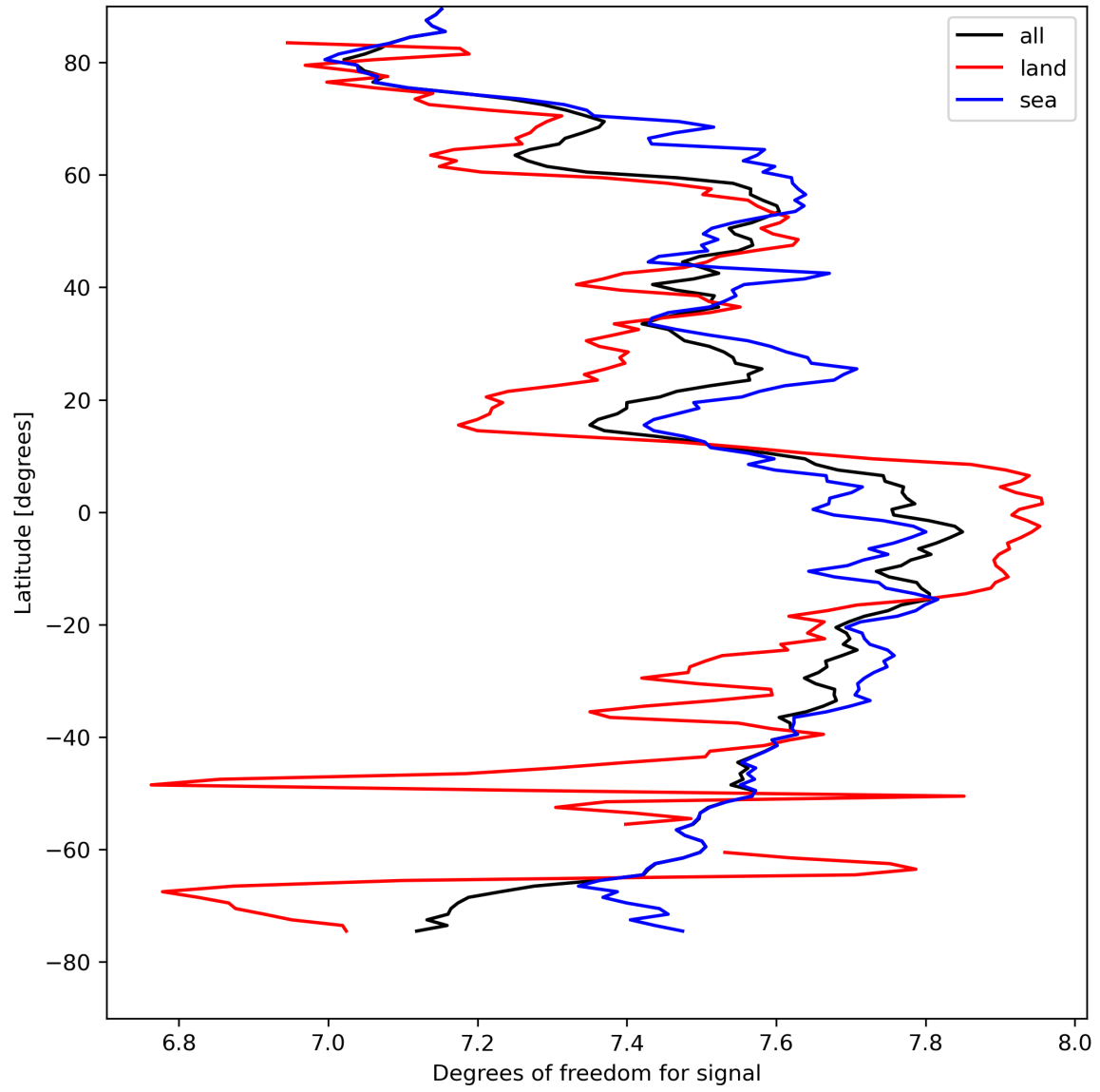
Figure 15: Zonal average of “Degrees of freedom for signal” for 2024-04-15 to 2024-04-16.
