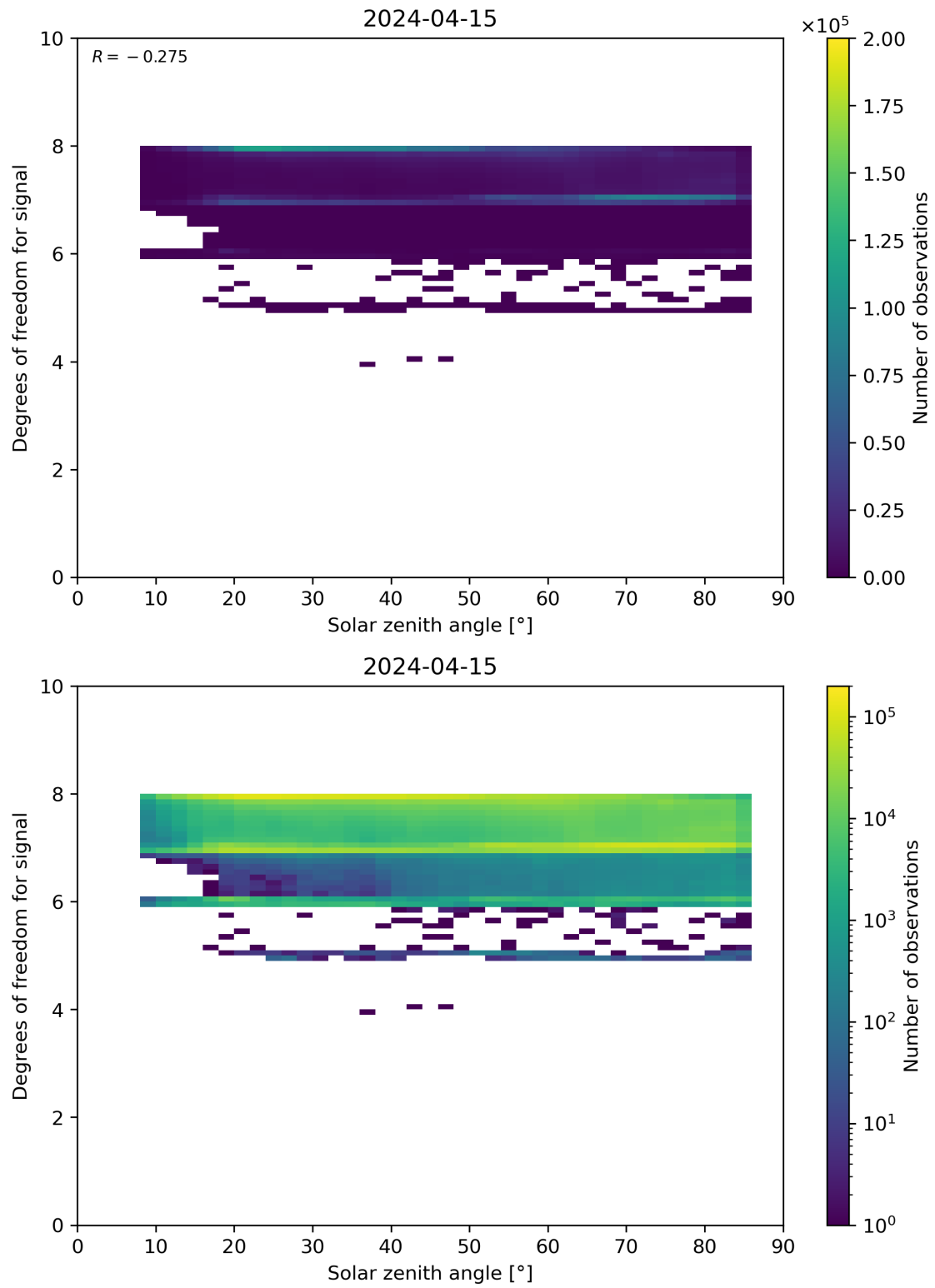
Figure 65: Scatter density plot of “Solar zenith angle” against “Degrees of freedom for signal” for 2024-04-15 to 2024-04-16.
