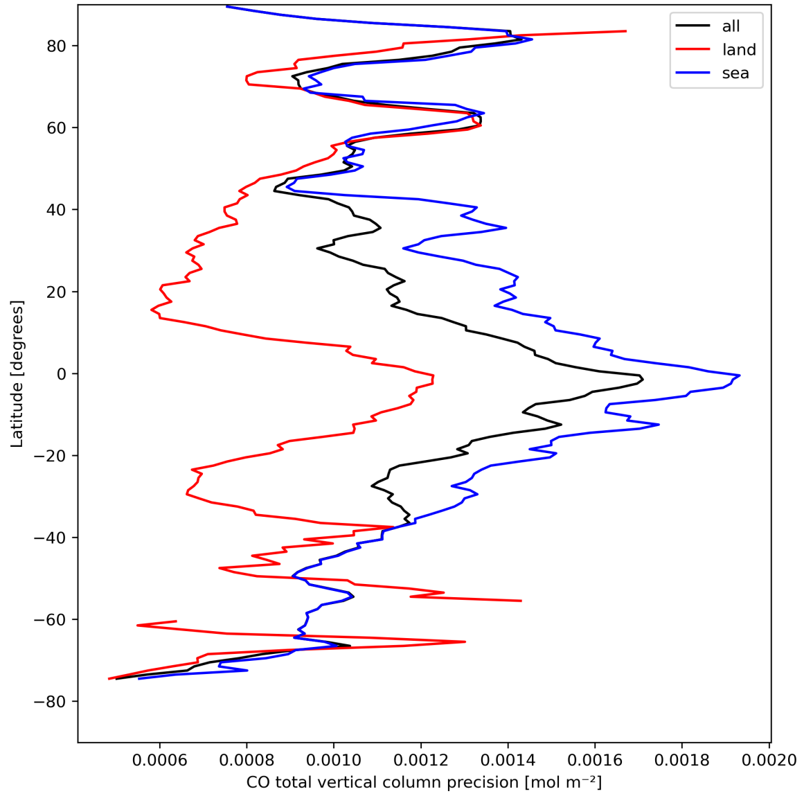
Figure 12: Zonal average of “CO total vertical column precision” for 2024-04-15 to 2024-04-16.
