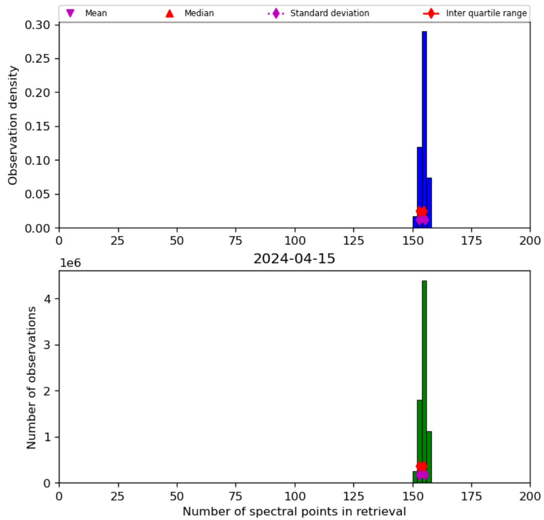
Figure 21: Histogram of “Number of spectral points in retrieval” for 2024-04-15 to 2024-04-16
