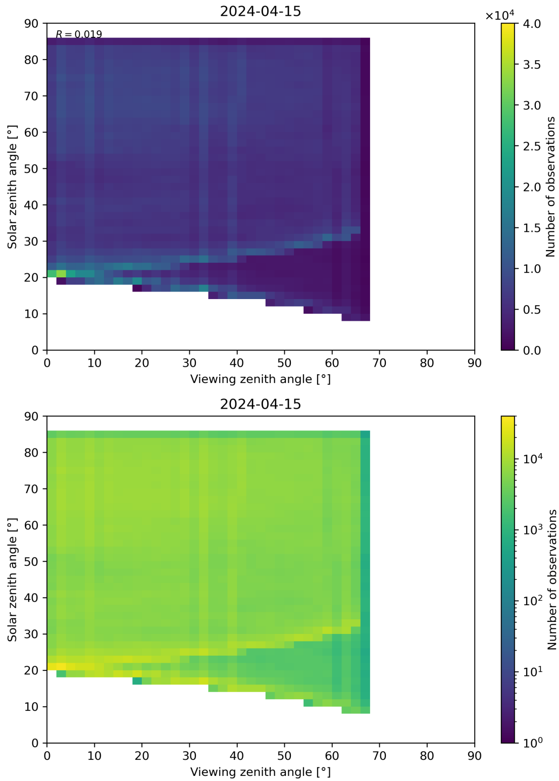
Figure 77: Scatter density plot of “Viewing zenith angle” against “Solar zenith angle” for 2024-04-15 to 2024-04-16.
