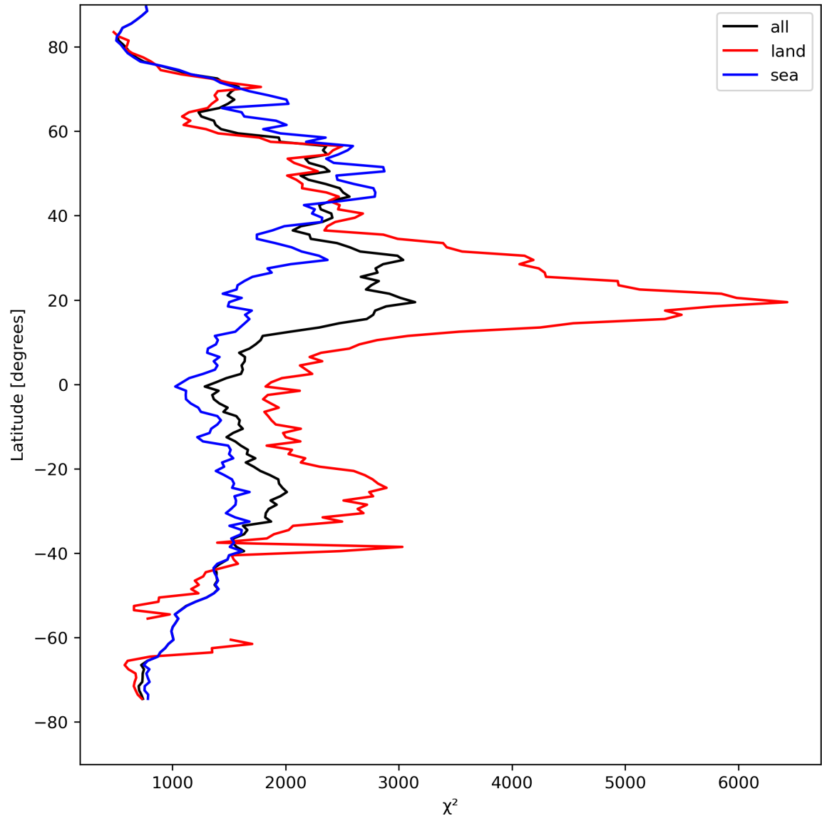
Figure 14: Zonal average of “ \chi^2 ” for 2024-04-15 to 2024-04-16.
