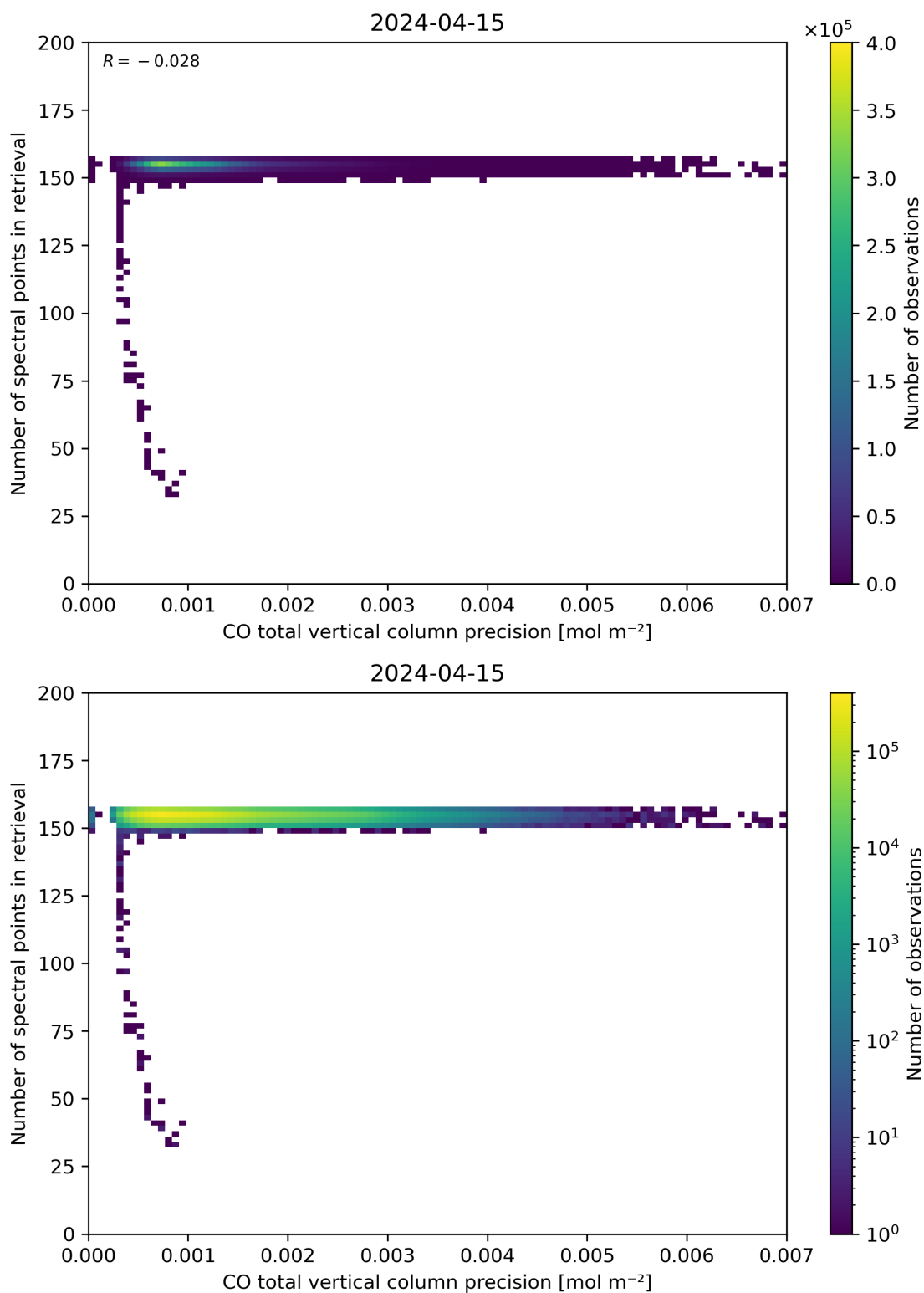
Figure 47: Scatter density plot of “CO total vertical column precision” against “Number of spectral points in retrieval” for 2024-04-15 to 2024-04-16.
