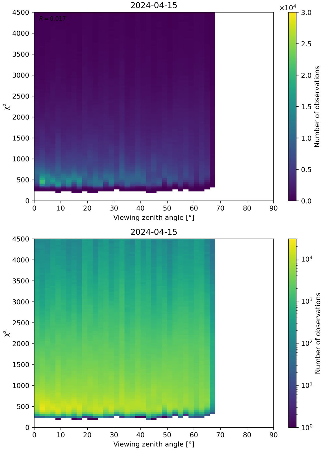
Figure 72: Scatter density plot of “Viewing zenith angle” against “ \chi^2 ” for 2024-04-15 to 2024-04-16.
