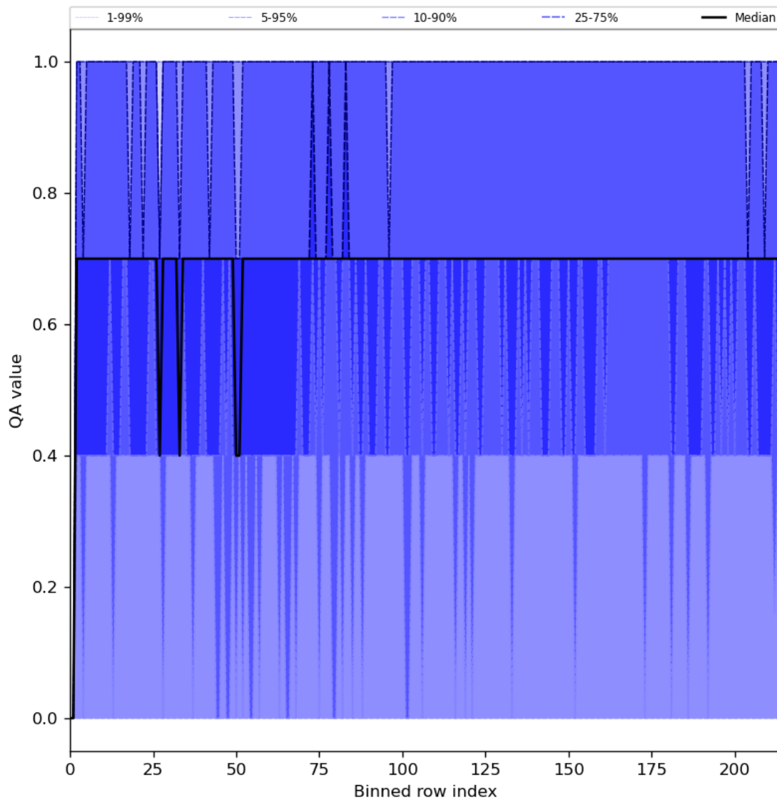
Figure 25: Along track statistics of "QA value" for 2024-04-15 to 2024-04-16
