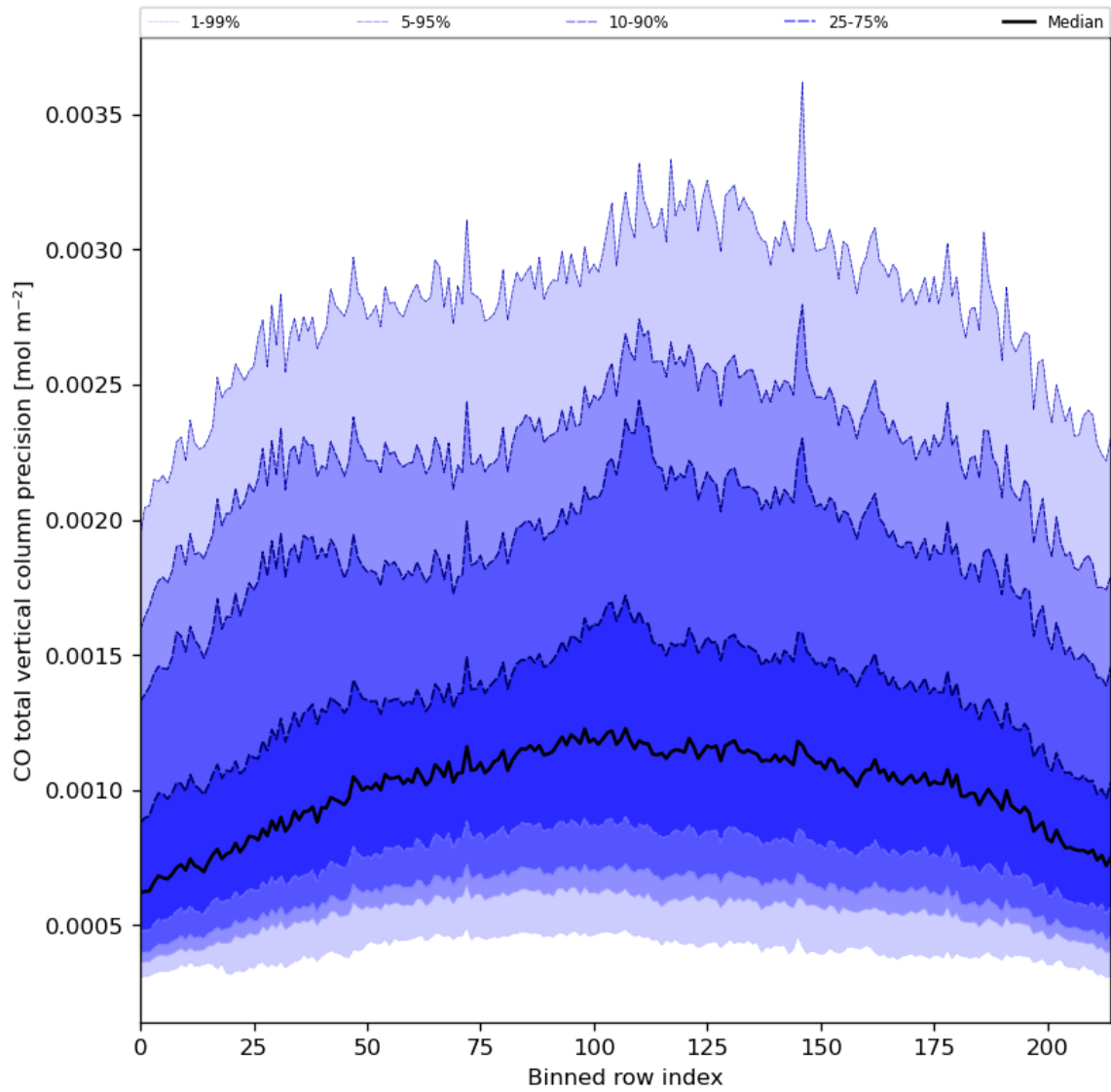
Figure 28: Along track statistics of “CO total vertical column precision” for 2024-04-15 to 2024-04-16
