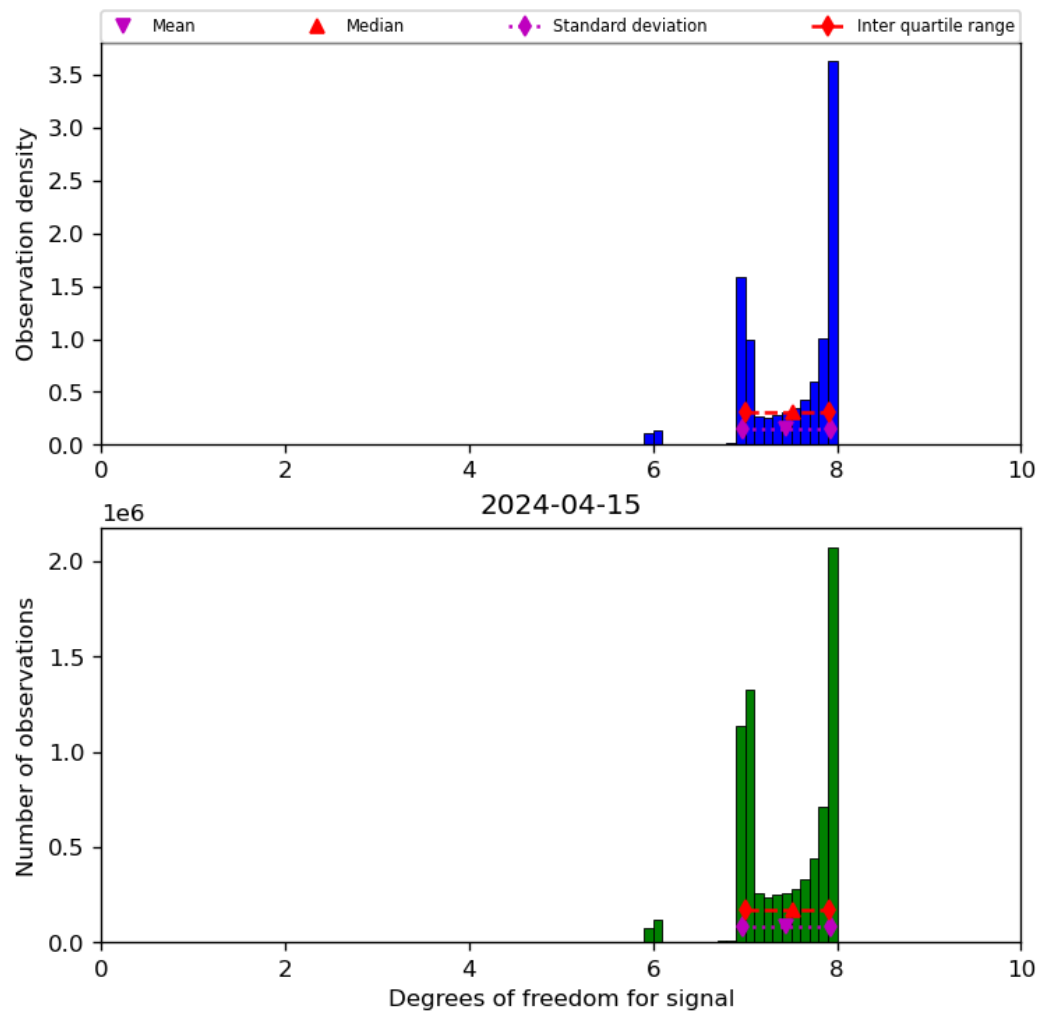
Figure 23: Histogram of “Degrees of freedom for signal” for 2024-04-15 to 2024-04-16
