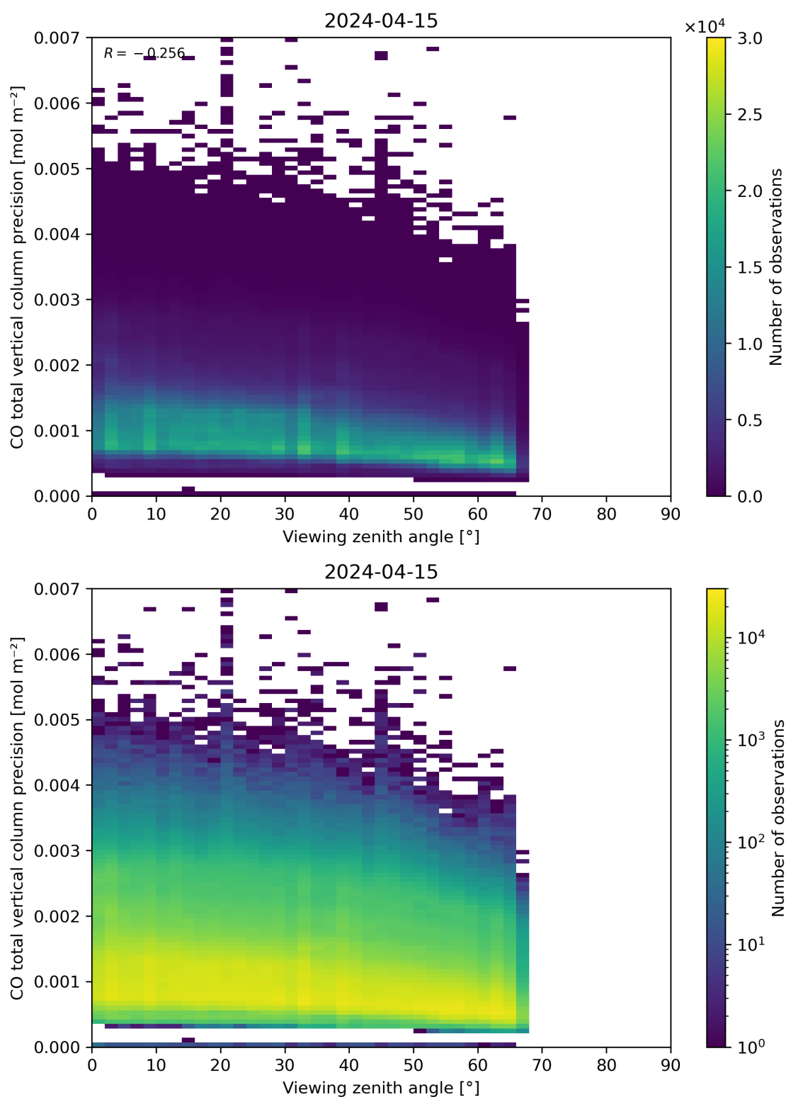
Figure 71: Scatter density plot of “Viewing zenith angle” against “CO total vertical column precision” for 2024-04-15 to 2024-04-16.
