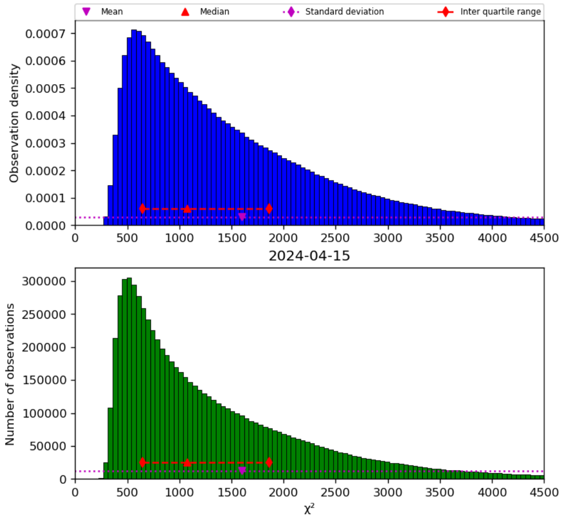
Figure 22: Histogram of “ \chi^2 ” for 2024-04-15 to 2024-04-16
