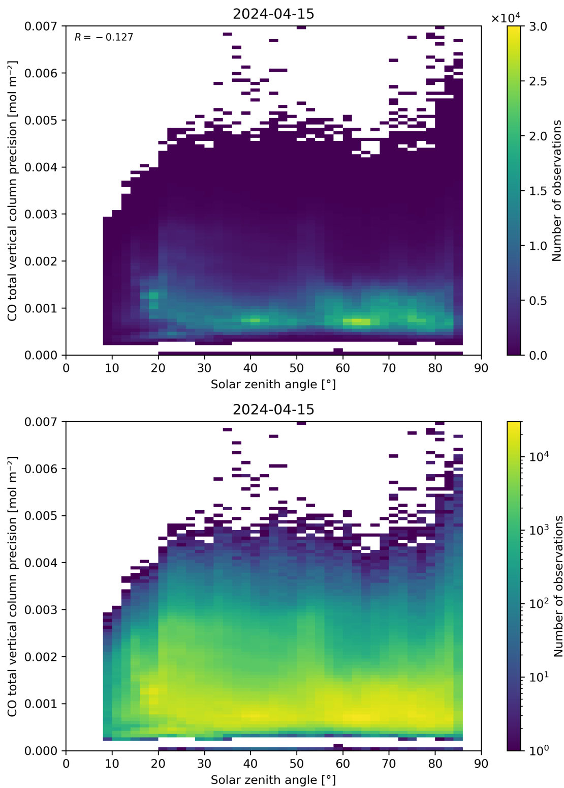
Figure 63: Scatter density plot of “Solar zenith angle” against “CO total vertical column precision” for 2024-04-15 to 2024-04-16.
