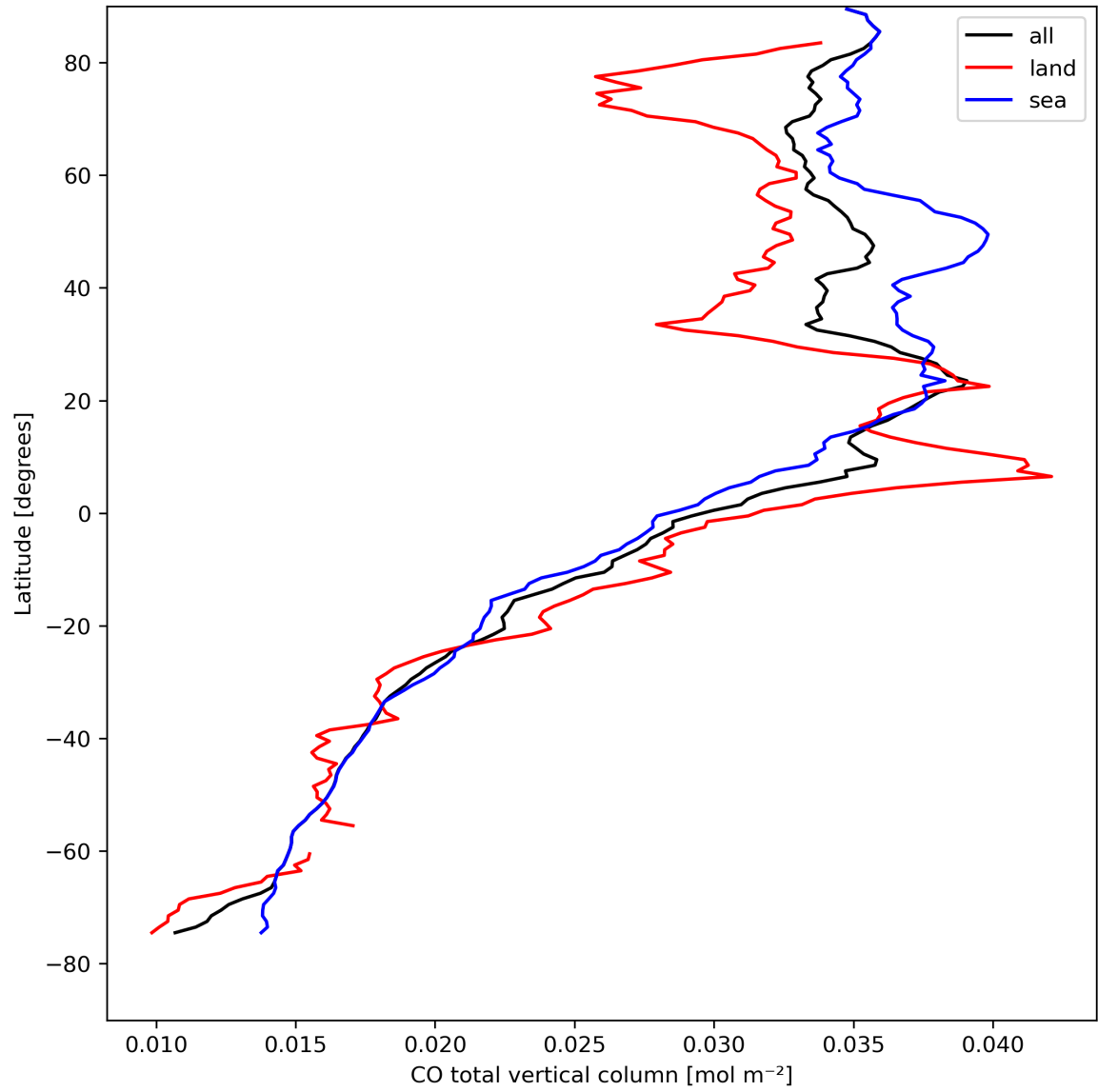
Figure 10: Zonal average of “CO total vertical column” for 2024-04-15 to 2024-04-16.
