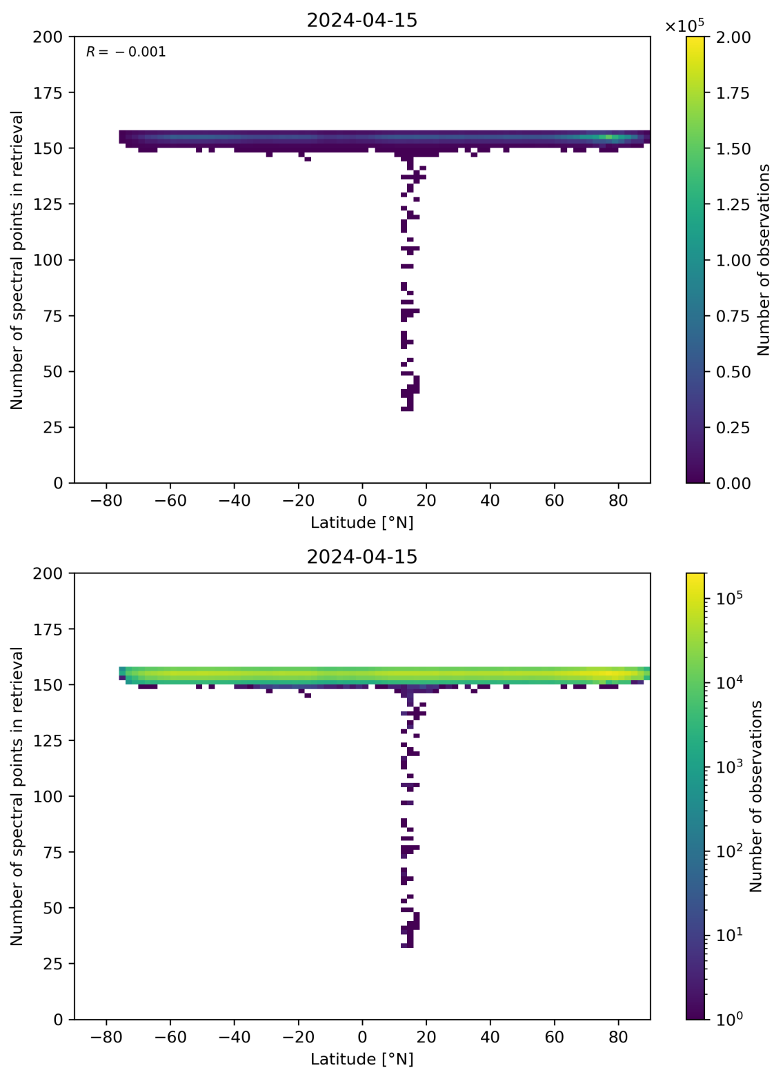
Figure 57: Scatter density plot of “Latitude” against “Number of spectral points in retrieval” for 2024-04-15 to 2024-04-16.
