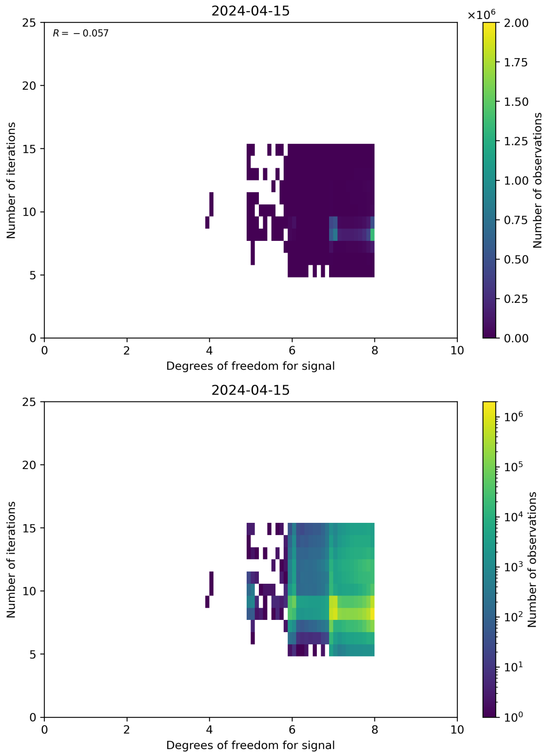
Figure 50: Scatter density plot of “Degrees of freedom for signal” against “Number of iterations” for 2024-04-15 to 2024-04-16.
