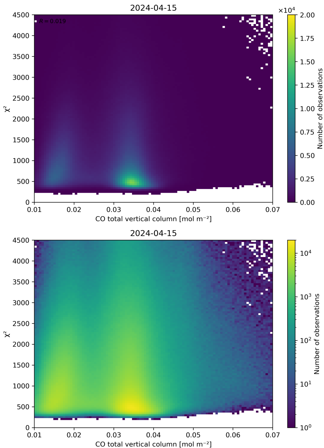
Figure 35: Scatter density plot of “CO total vertical column” against “ \chi^2 ” for 2024-04-15 to 2024-04-16.
