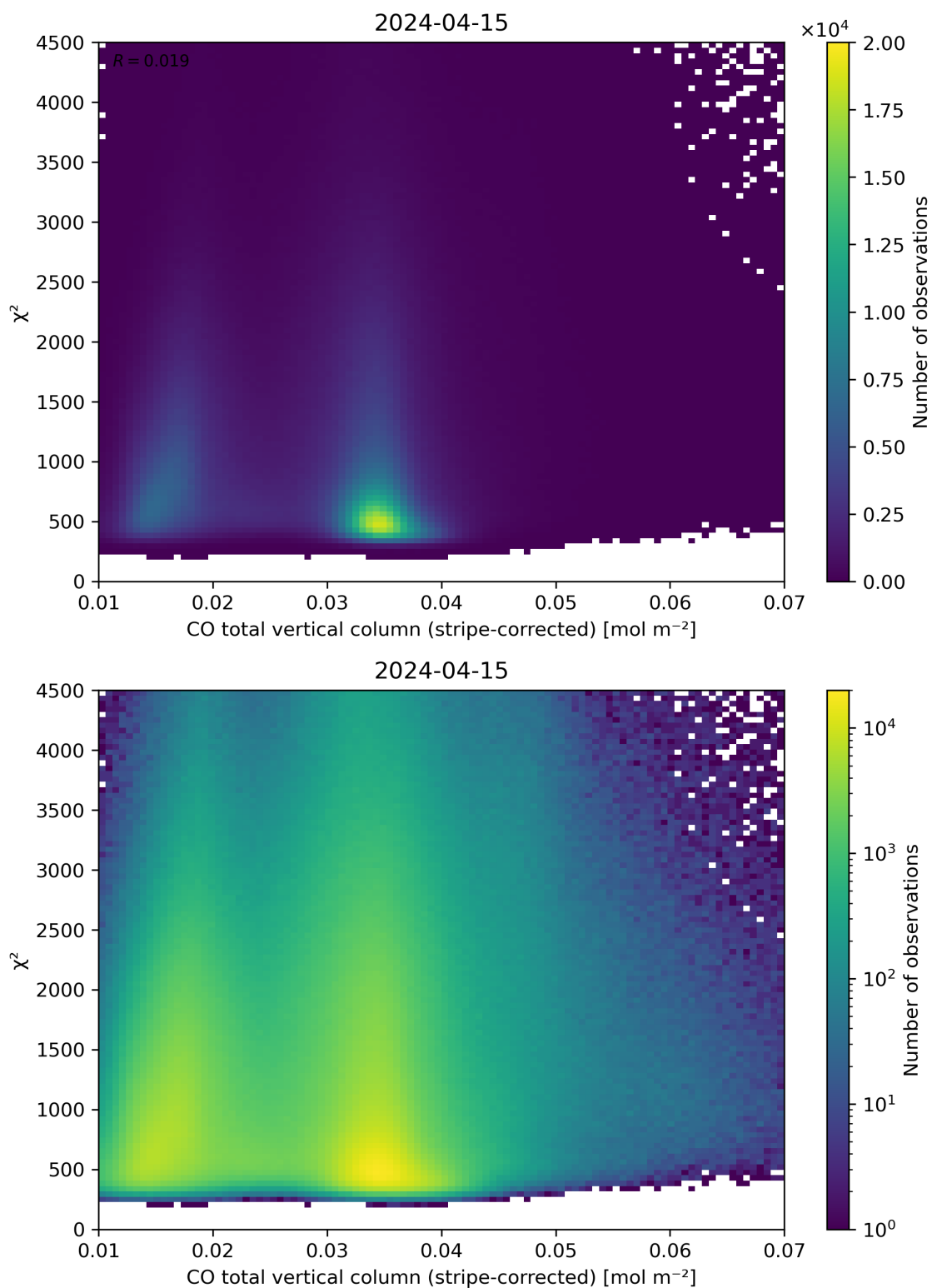
Figure 37: Scatter density plot of “CO total vertical column (stripe-corrected)” against “ \chi^2 ” for 2024-04-15 to 2024-04-16.
