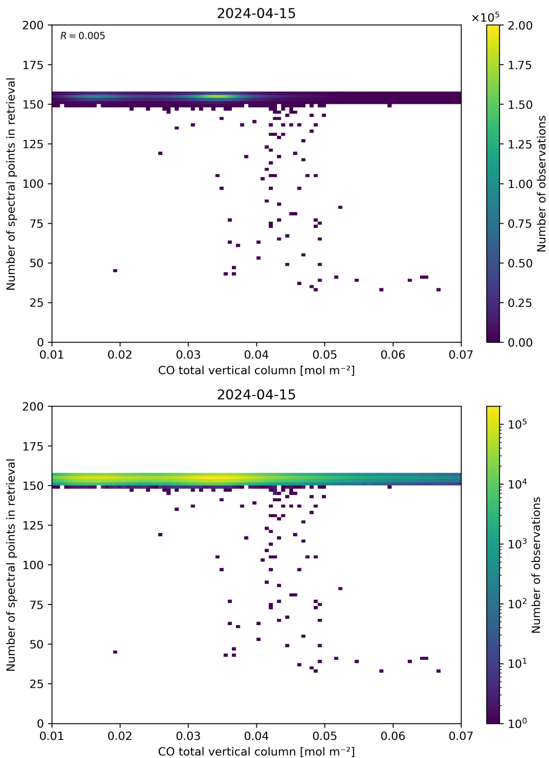
Figure 43: Scatter density plot of “CO total vertical column” against “Number of spectral points in retrieval” for 2024-04-15 to 2024-04-16.
