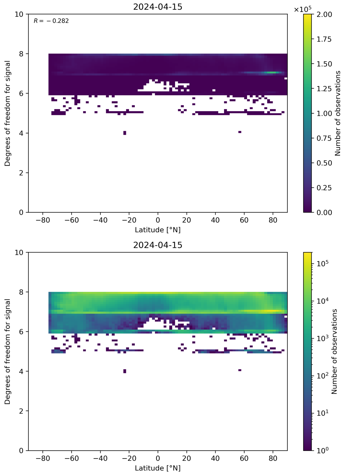
Figure 55: Scatter density plot of “Latitude” against “Degrees of freedom for signal” for 2024-04-15 to 2024-04-16.
