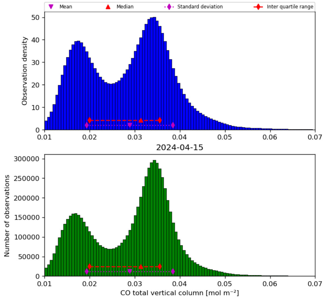
Figure 18: Histogram of “CO total vertical column” for 2024-04-15 to 2024-04-16
