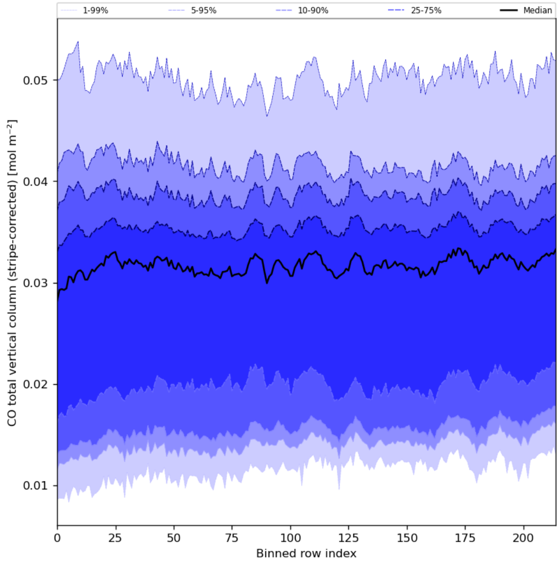
Figure 27: Along track statistics of “CO total vertical column (stripe-corrected)” for 2024-04-15 to 2024-04-16
