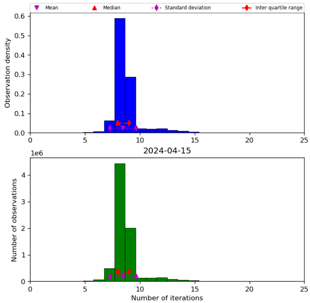
Figure 24: Histogram of “Number of iterations” for 2024-04-15 to 2024-04-16
