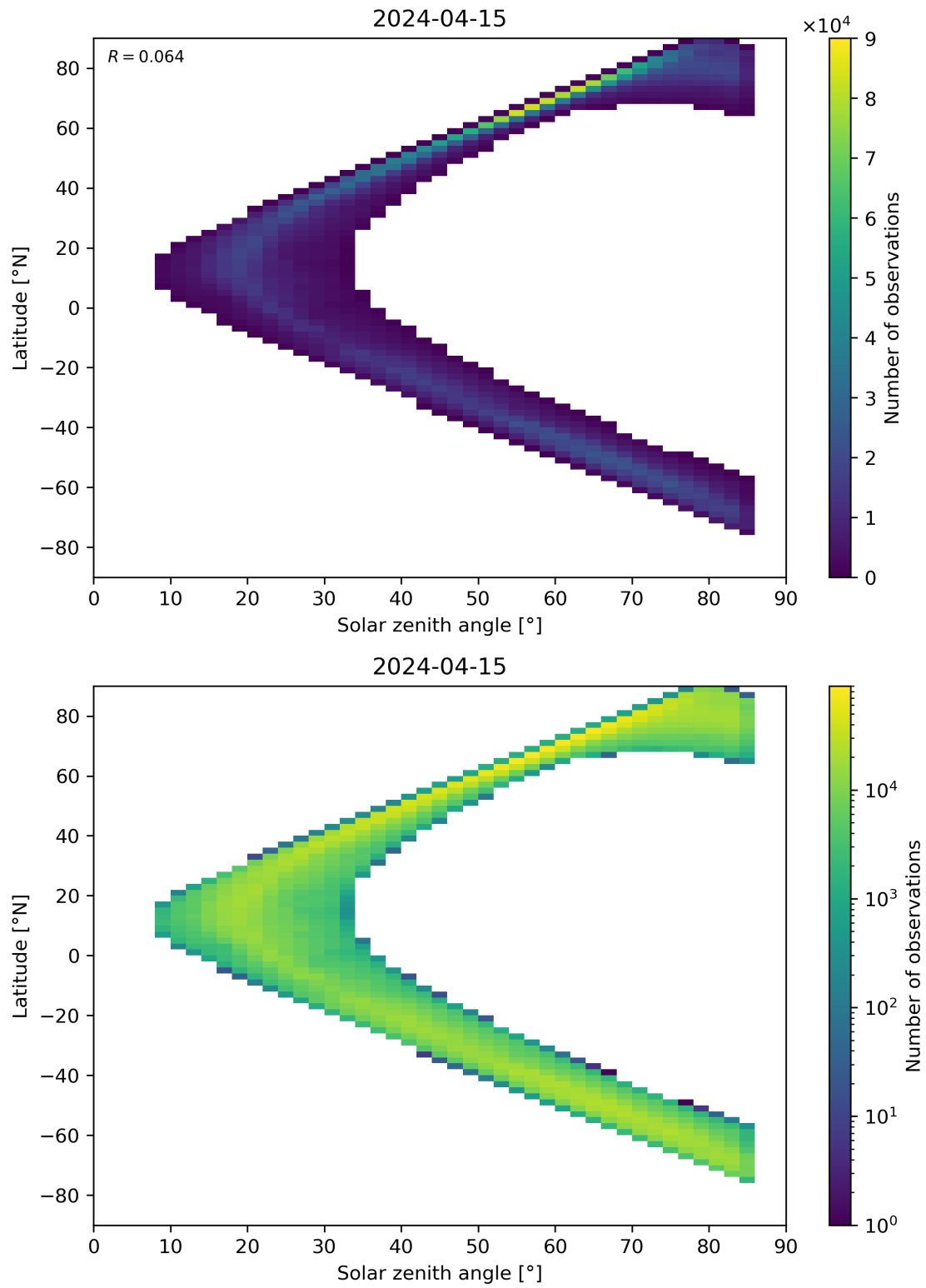
Figure 66: Scatter density plot of “Solar zenith angle” against “Latitude” for 2024-04-15 to 2024-04-16.
