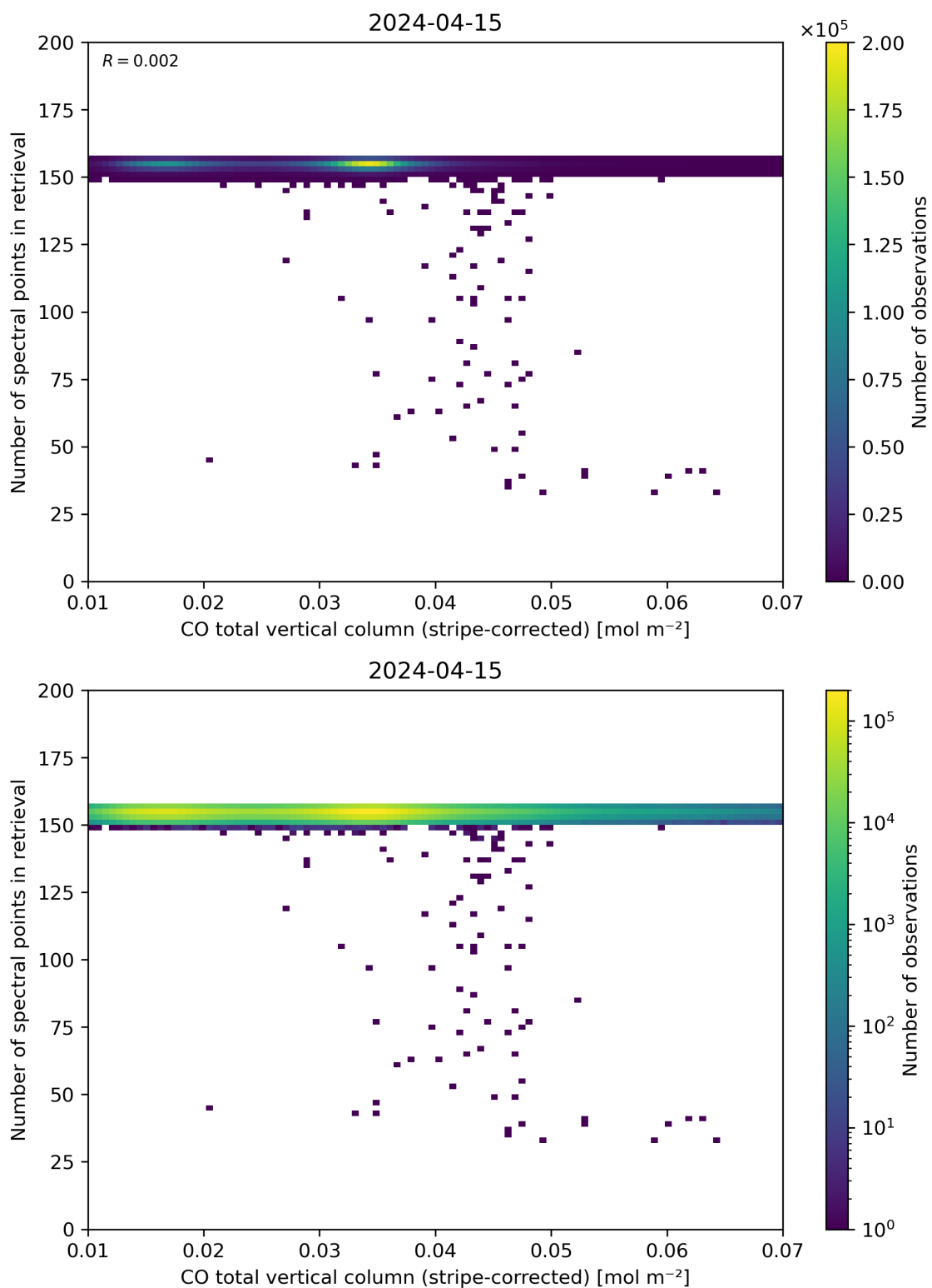
Figure 40: Scatter density plot of “CO total vertical column (stripe-corrected)” against “Number of spectral points in retrieval” for 2024-04-15 to 2024-04-16.
