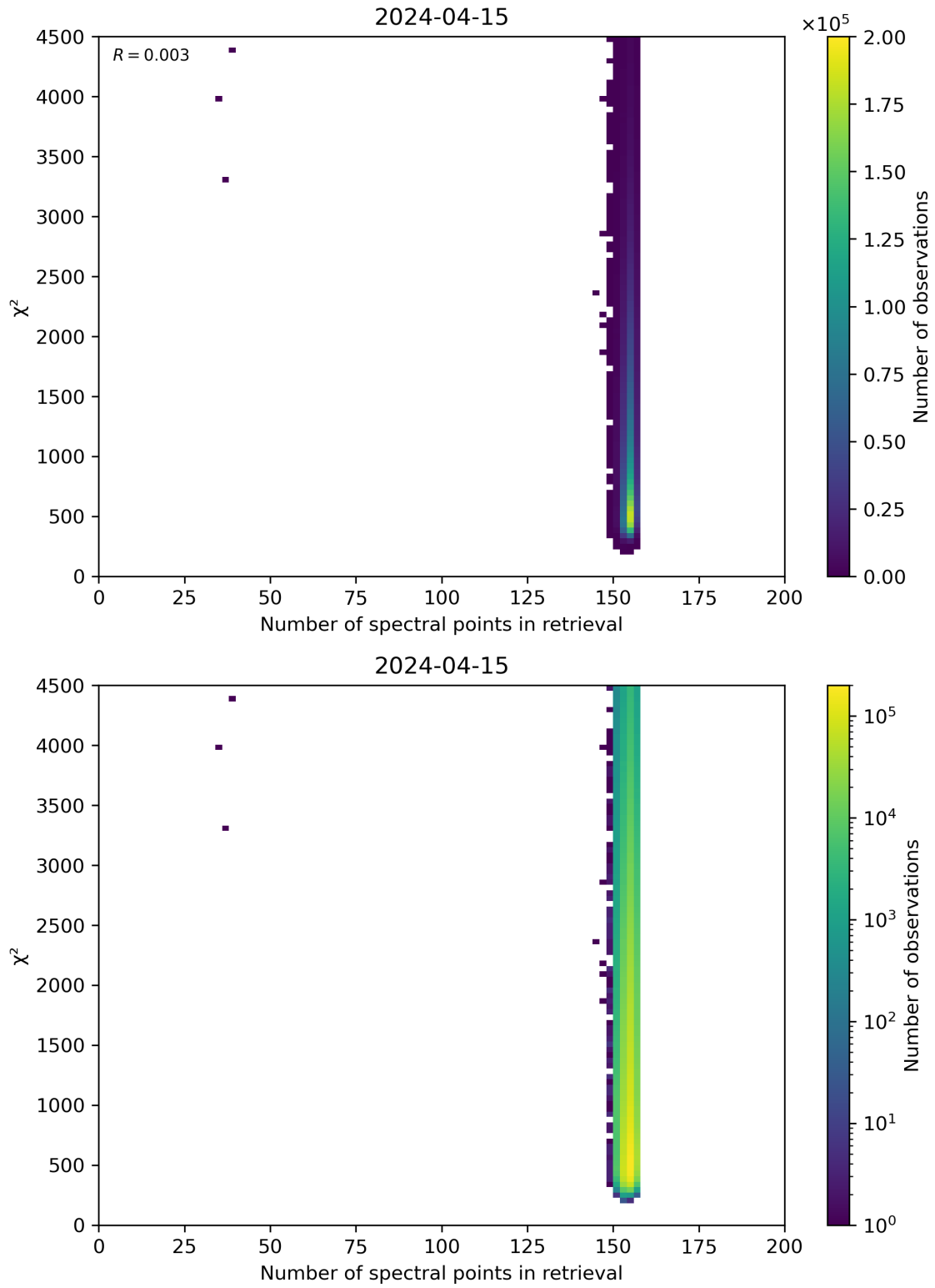
Figure 58: Scatter density plot of “Number of spectral points in retrieval” against “ \chi^2 ” for 2024-04-15 to 2024-04-16.
