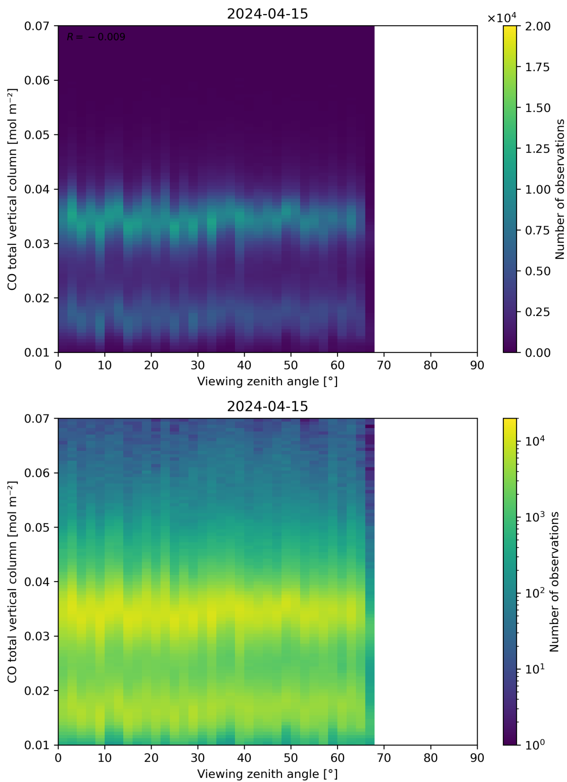
Figure 69: Scatter density plot of “Viewing zenith angle” against “CO total vertical column” for 2024-04-15 to 2024-04-16.
