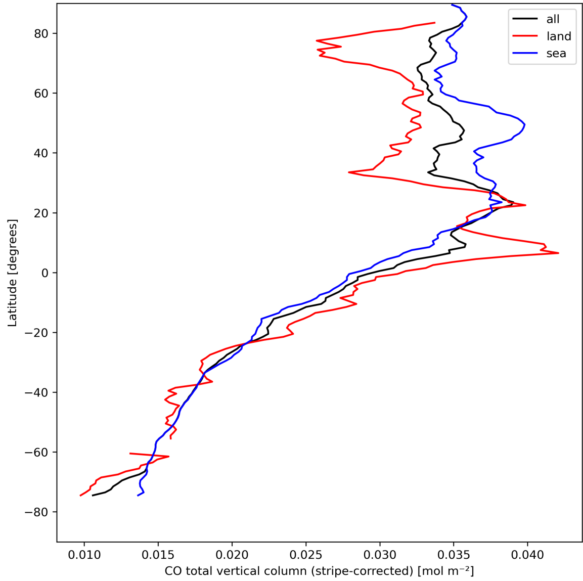
Figure 11: Zonal average of “CO total vertical column (stripe-corrected)” for 2024-04-15 to 2024-04-16.
