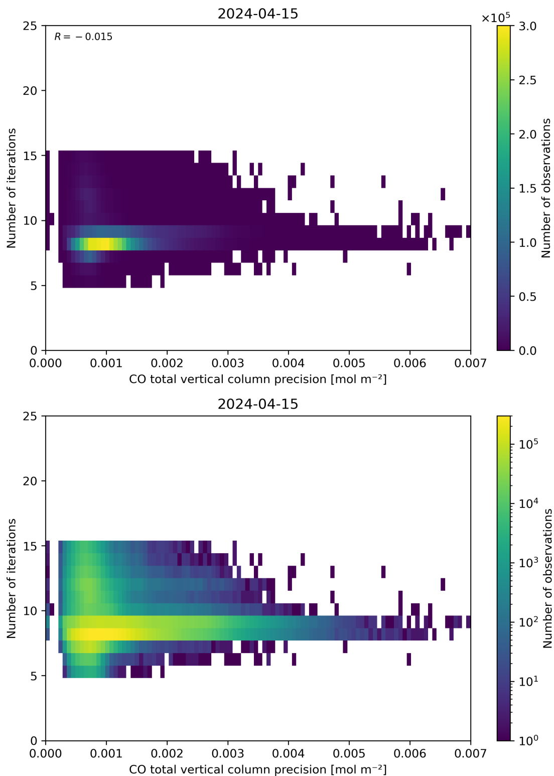
Figure 46: Scatter density plot of “CO total vertical column precision” against “Number of iterations” for 2024-04-15 to 2024-04-16.
