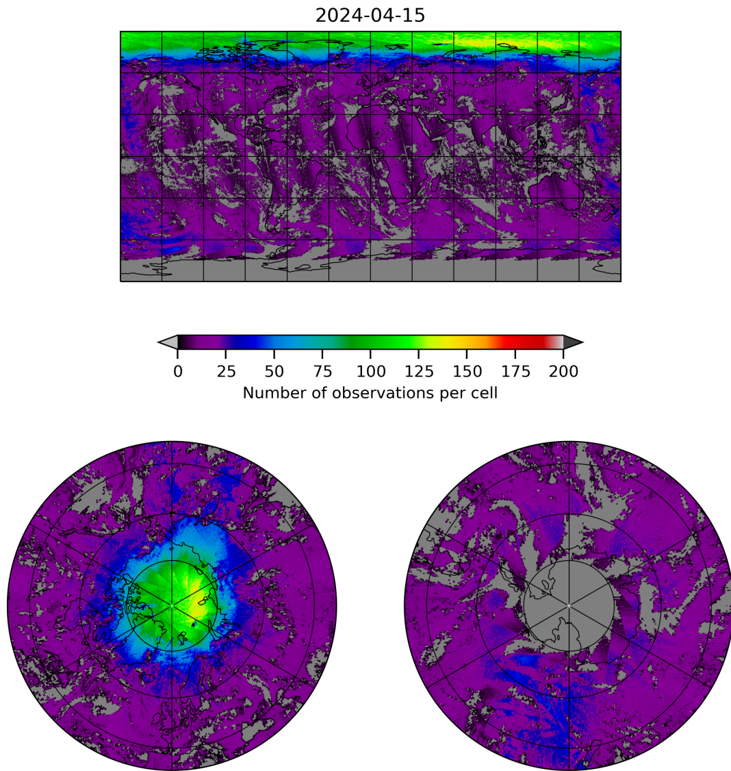
Figure 8: Map of the number of observations for 2024-04-15 to 2024-04-16
