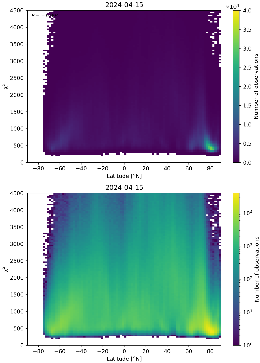
Figure 54: Scatter density plot of “Latitude” against “ \chi^2 ” for 2024-04-15 to 2024-04-16.
