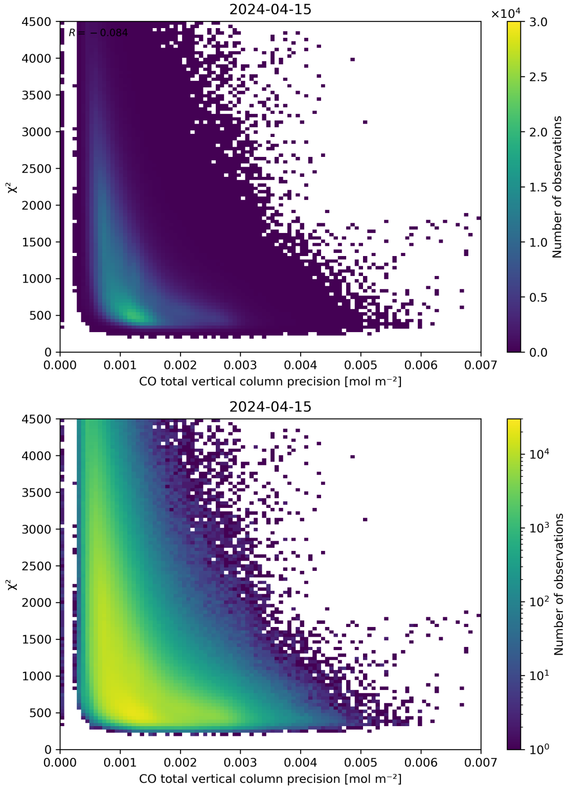
Figure 44: Scatter density plot of “CO total vertical column precision” against “ \chi^2 ” for 2024-04-15 to 2024-04-16.
