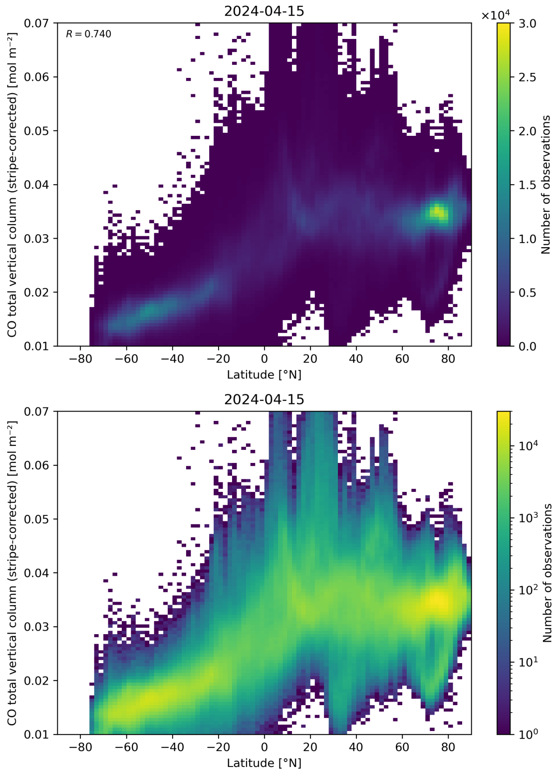
Figure 52: Scatter density plot of “Latitude” against “CO total vertical column (stripe-corrected)” for 2024-04-15 to 2024-04-16.
