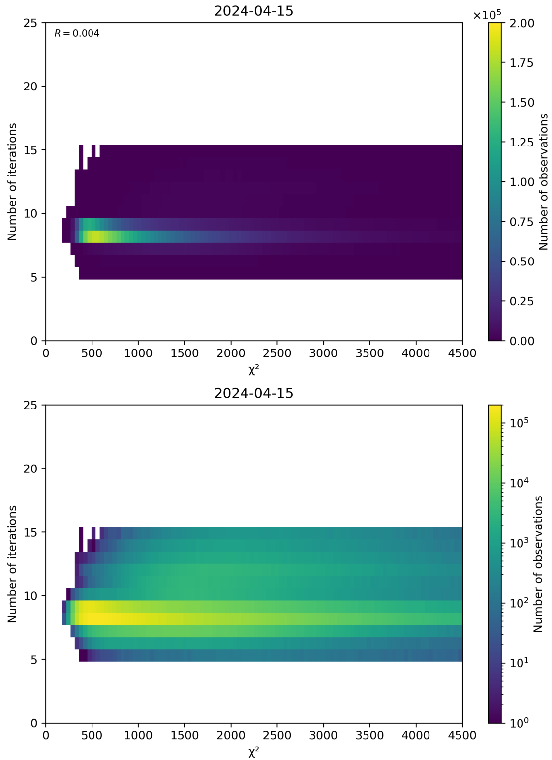
Figure 49: Scatter density plot of “ \chi^2 ” against “Number of iterations” for 2024-04-15 to 2024-04-16.
