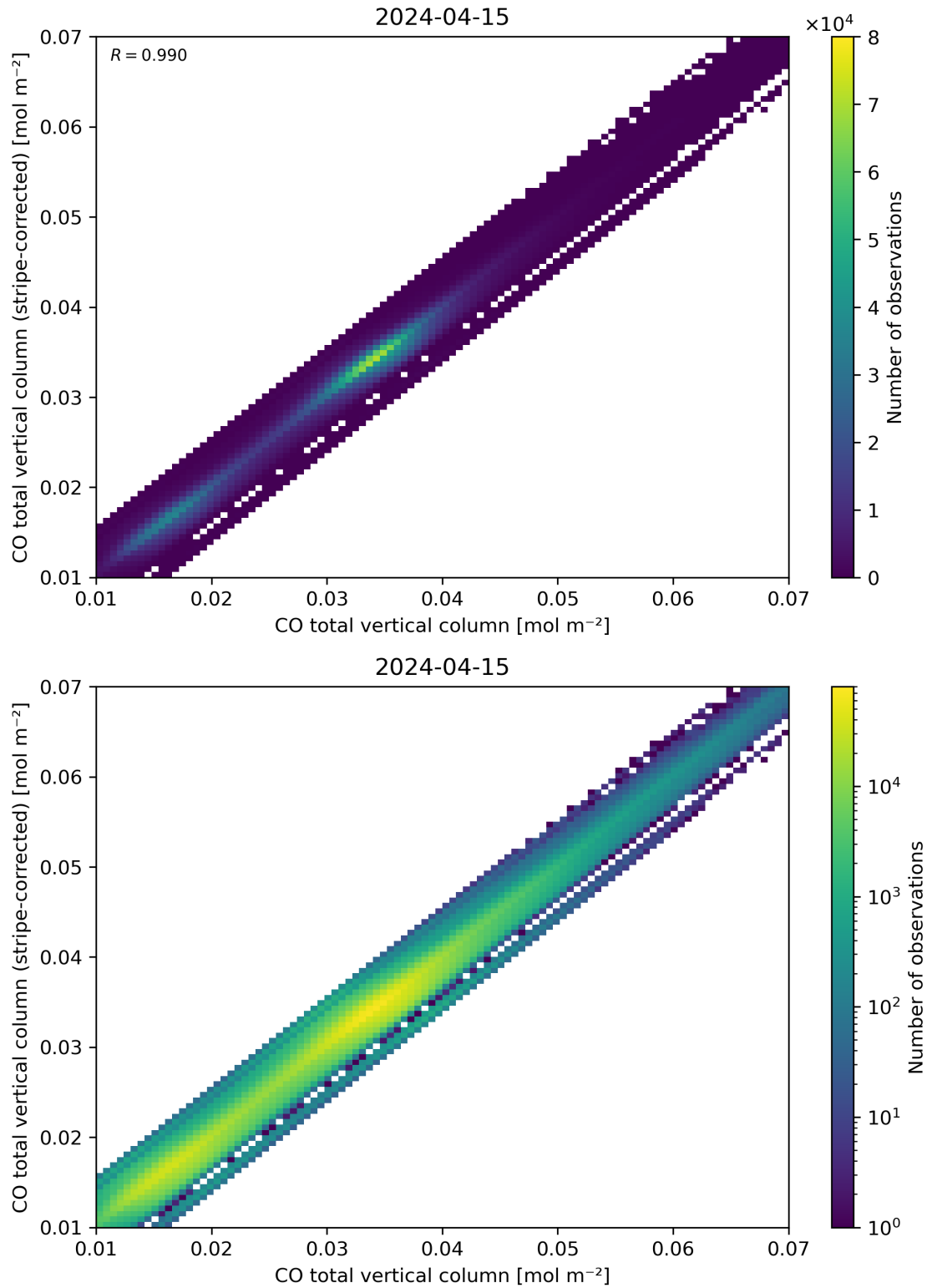
Figure 33: Scatter density plot of “CO total vertical column” against “CO total vertical column (stripe-corrected)” for 2024-04-15 to 2024-04-16.
