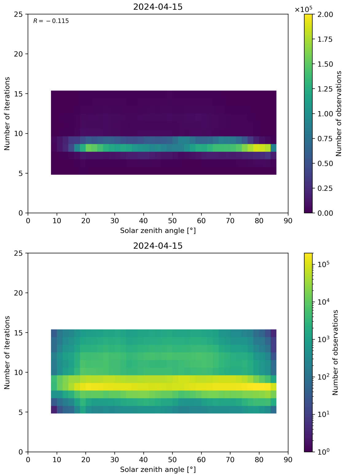
Figure 67: Scatter density plot of “Solar zenith angle” against “Number of iterations” for 2024-04-15 to 2024-04-16.
