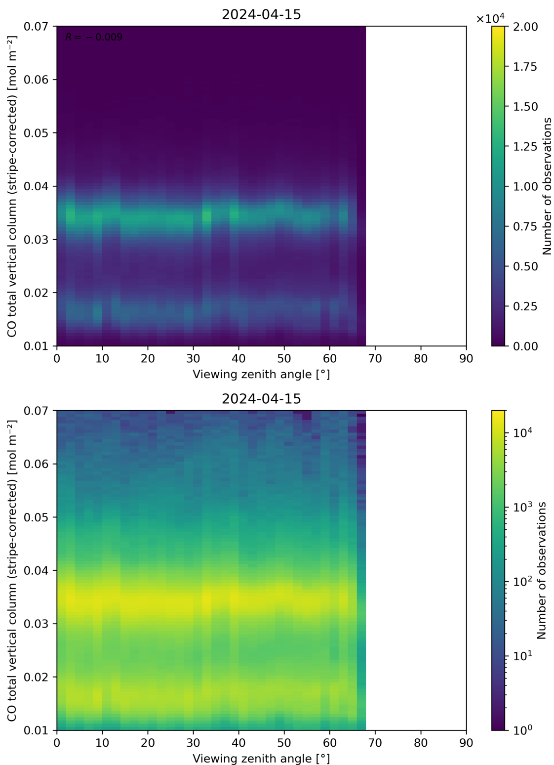
Figure 70: Scatter density plot of “Viewing zenith angle” against “CO total vertical column (stripe-corrected)” for 2024-04-15 to 2024-04-16.
