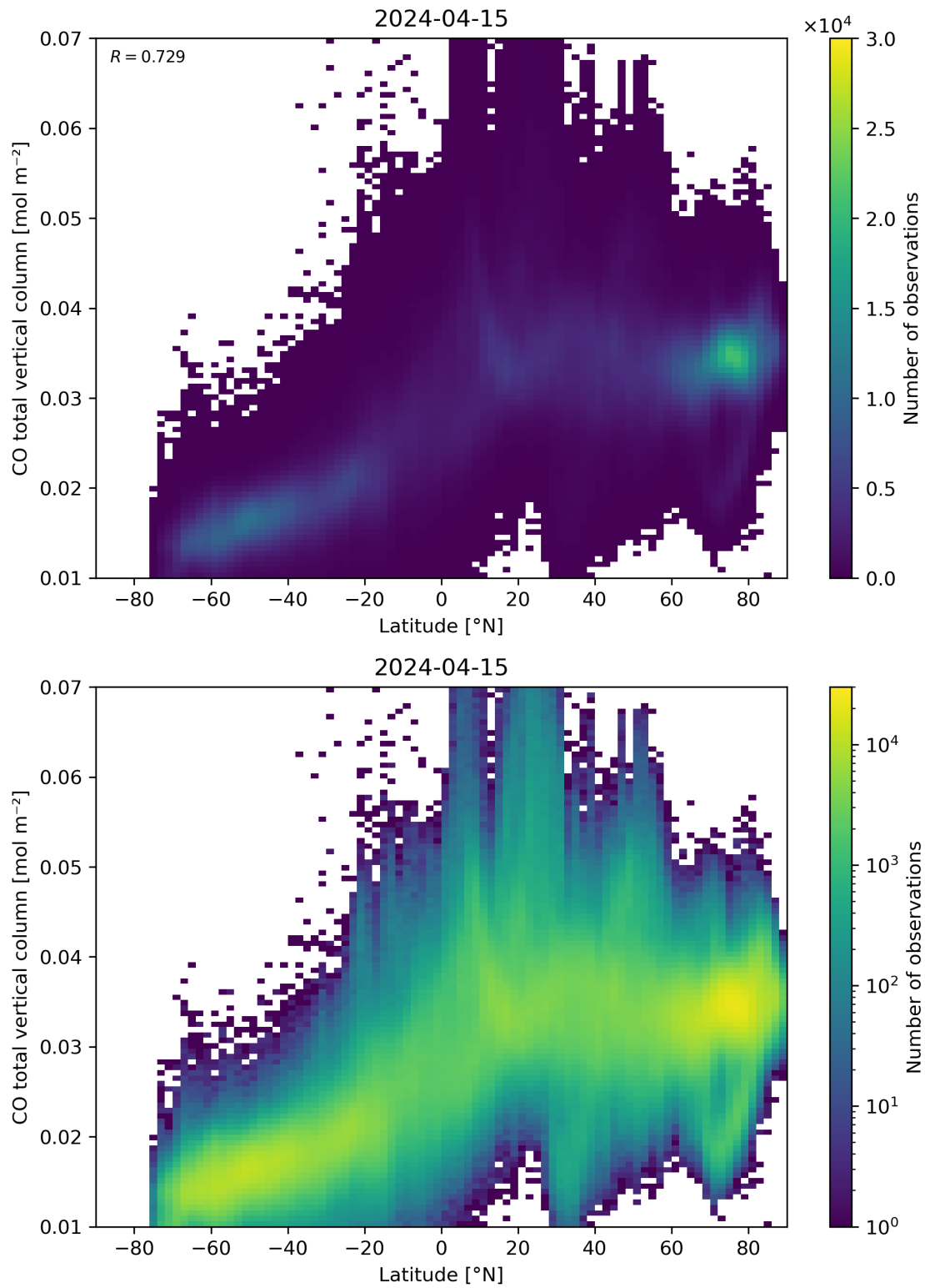
Figure 51: Scatter density plot of “Latitude” against “CO total vertical column” for 2024-04-15 to 2024-04-16.
