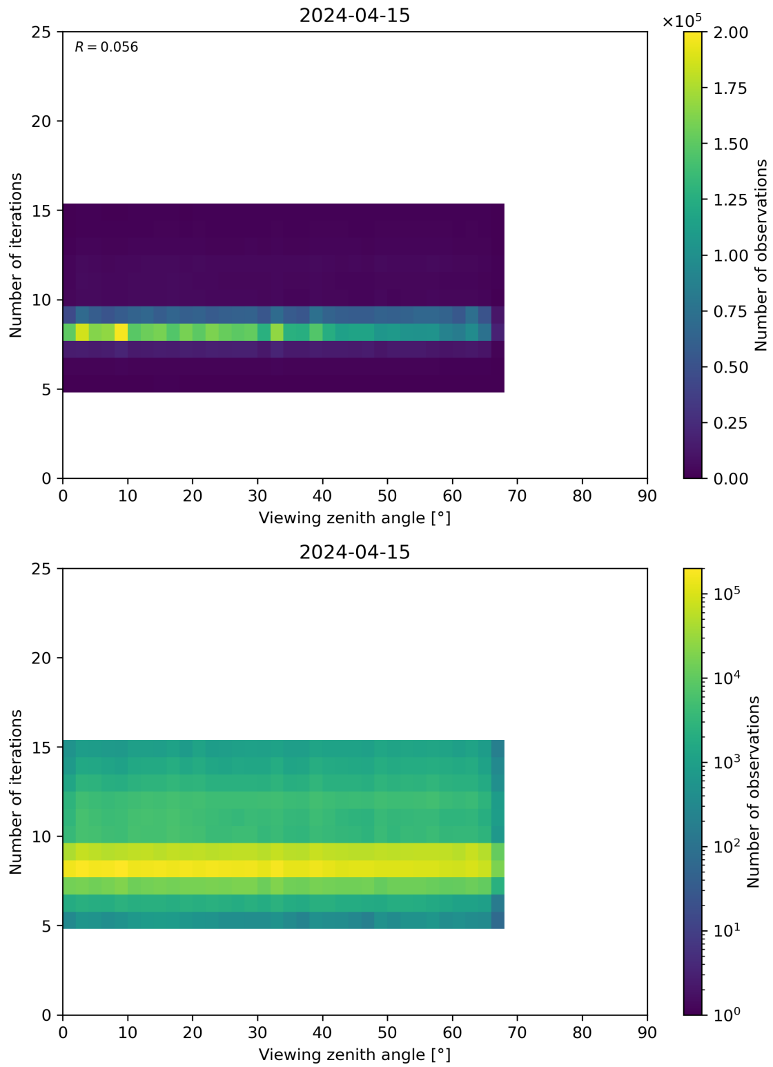
Figure 75: Scatter density plot of “Viewing zenith angle” against “Number of iterations” for 2024-04-15 to 2024-04-16.
