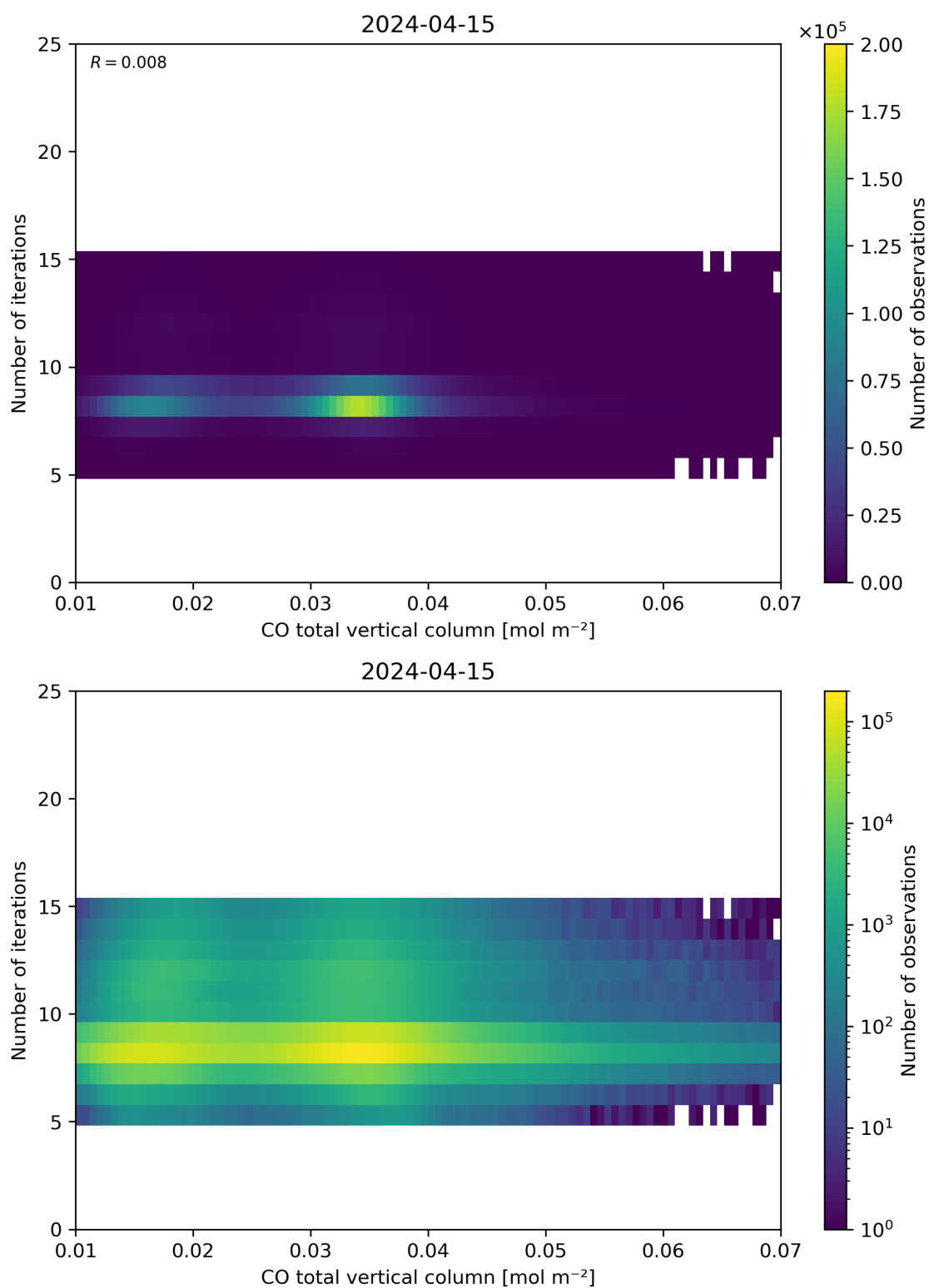
Figure 42: Scatter density plot of “CO total vertical column” against “Number of iterations” for 2024-04-15 to 2024-04-16.
