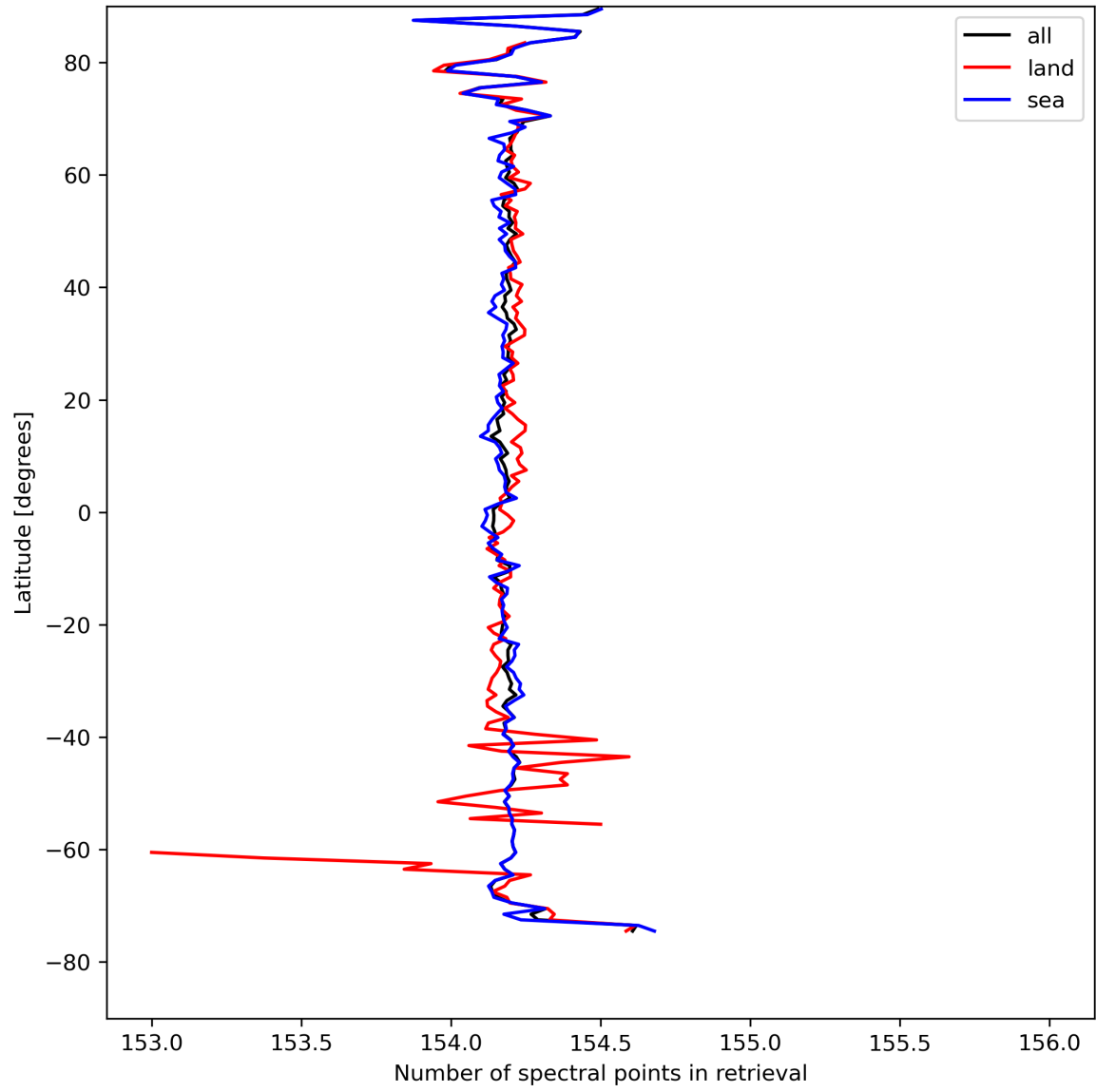
Figure 13: Zonal average of “Number of spectral points in retrieval” for 2024-04-15 to 2024-04-16.
