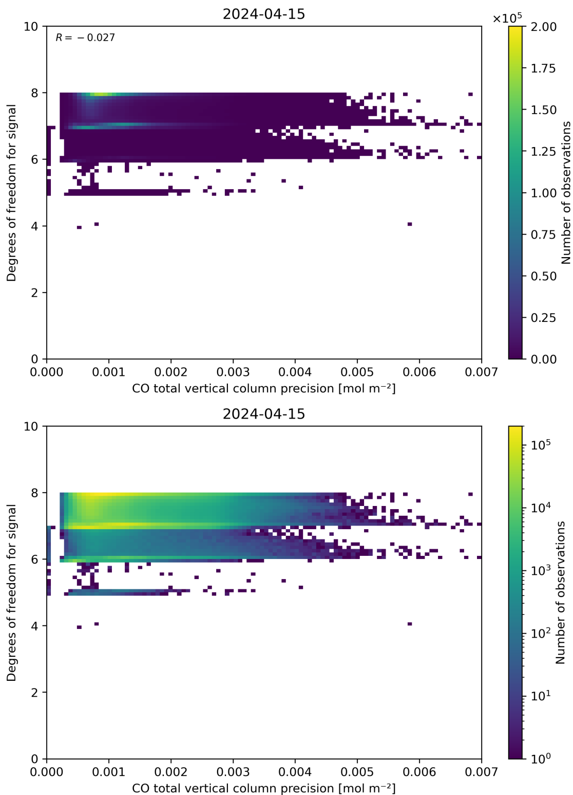
Figure 45: Scatter density plot of “CO total vertical column precision” against “Degrees of freedom for signal” for 2024-04-15 to 2024-04-16.
