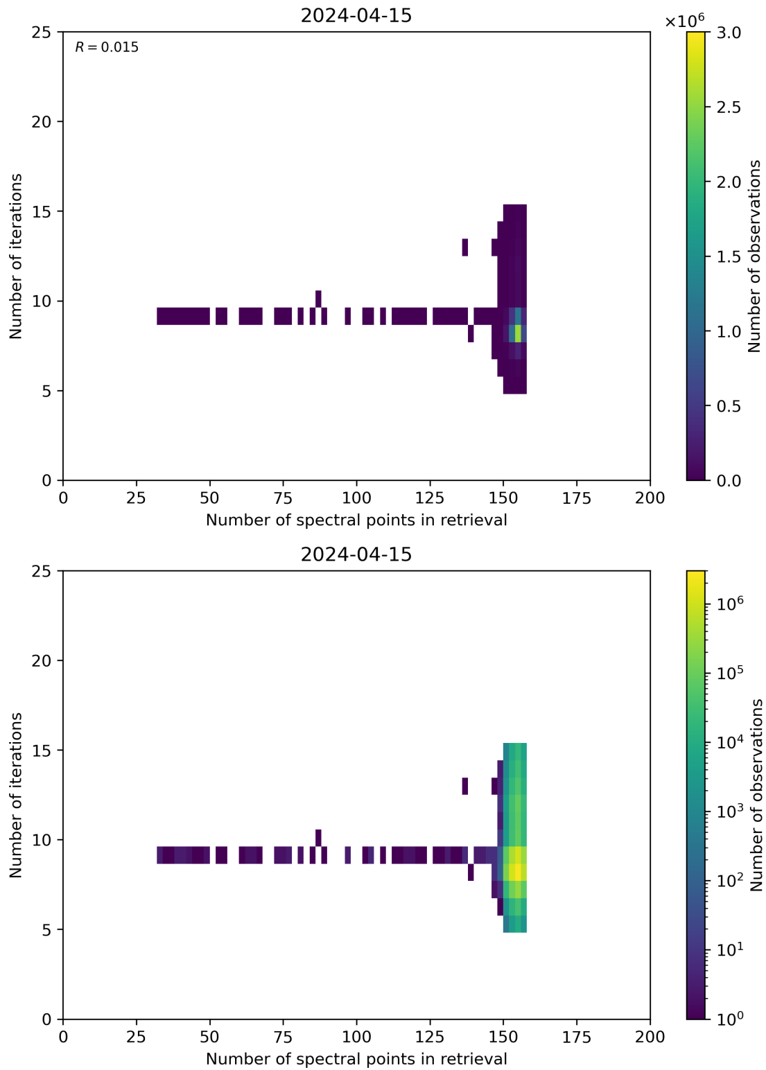
Figure 60: Scatter density plot of “Number of spectral points in retrieval” against “Number of iterations” for 2024-04-15 to 2024-04-16.
