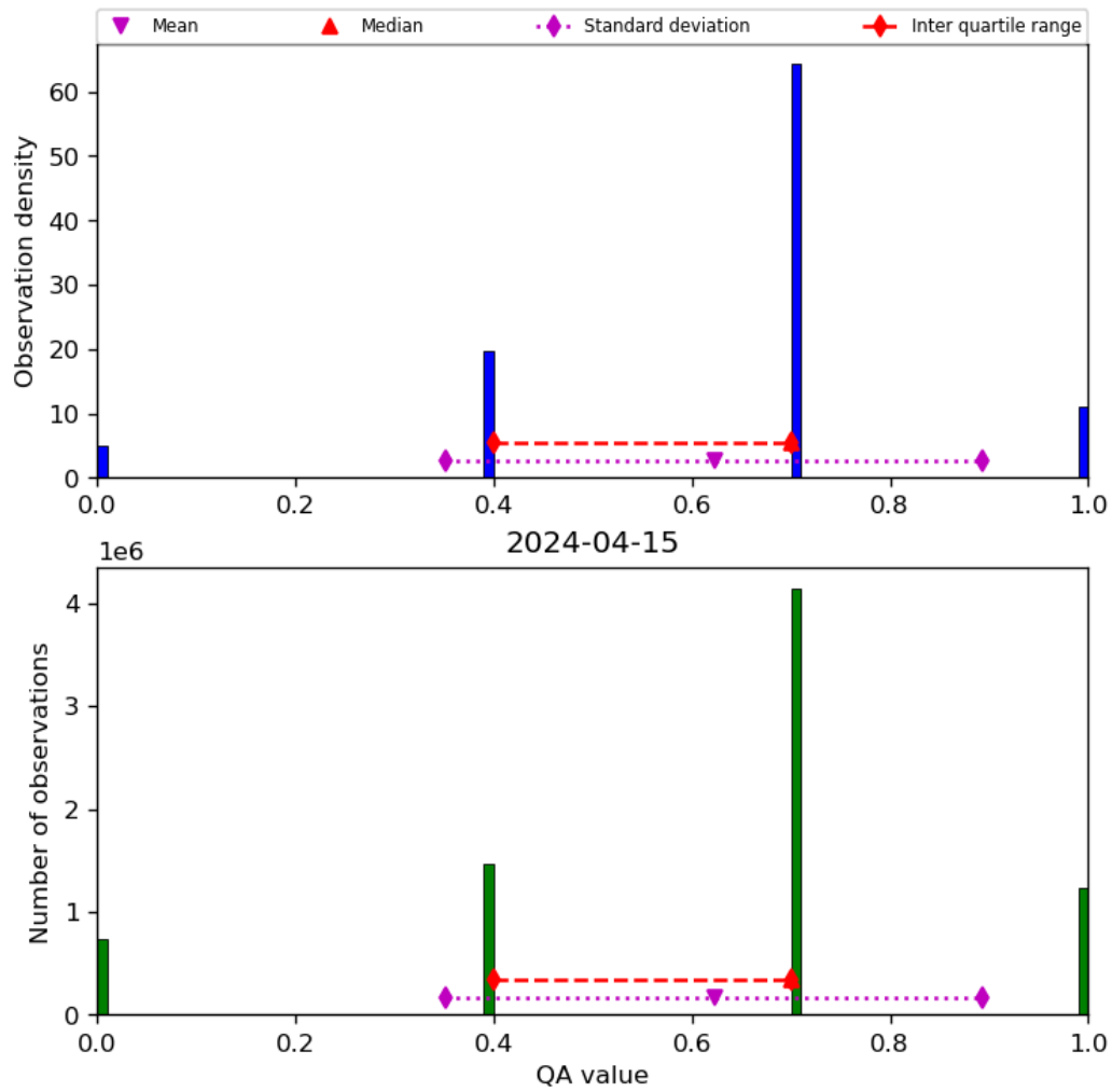
Figure 17: Histogram of “QA value” for 2024-04-15 to 2024-04-16
