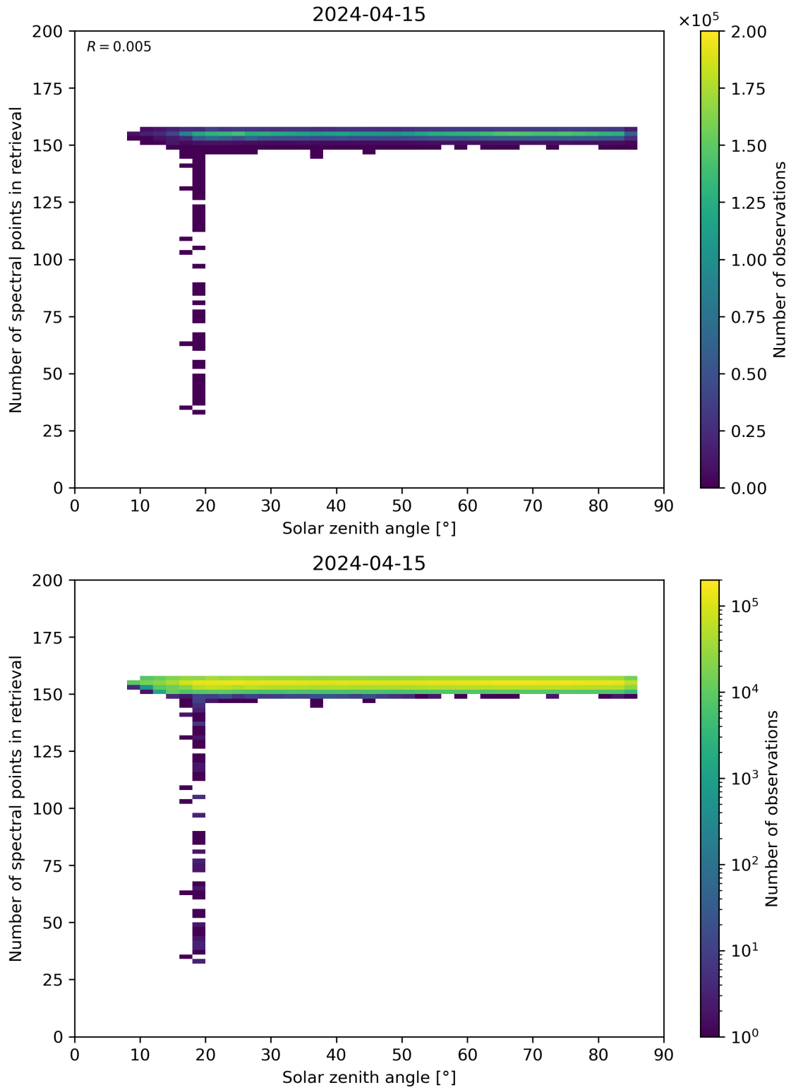
Figure 68: Scatter density plot of “Solar zenith angle” against “Number of spectral points in retrieval” for 2024-04-15 to 2024-04-16.
