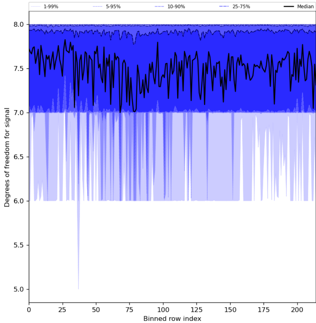
Figure 31: Along track statistics of “Degrees of freedom for signal” for 2024-04-15 to 2024-04-16
