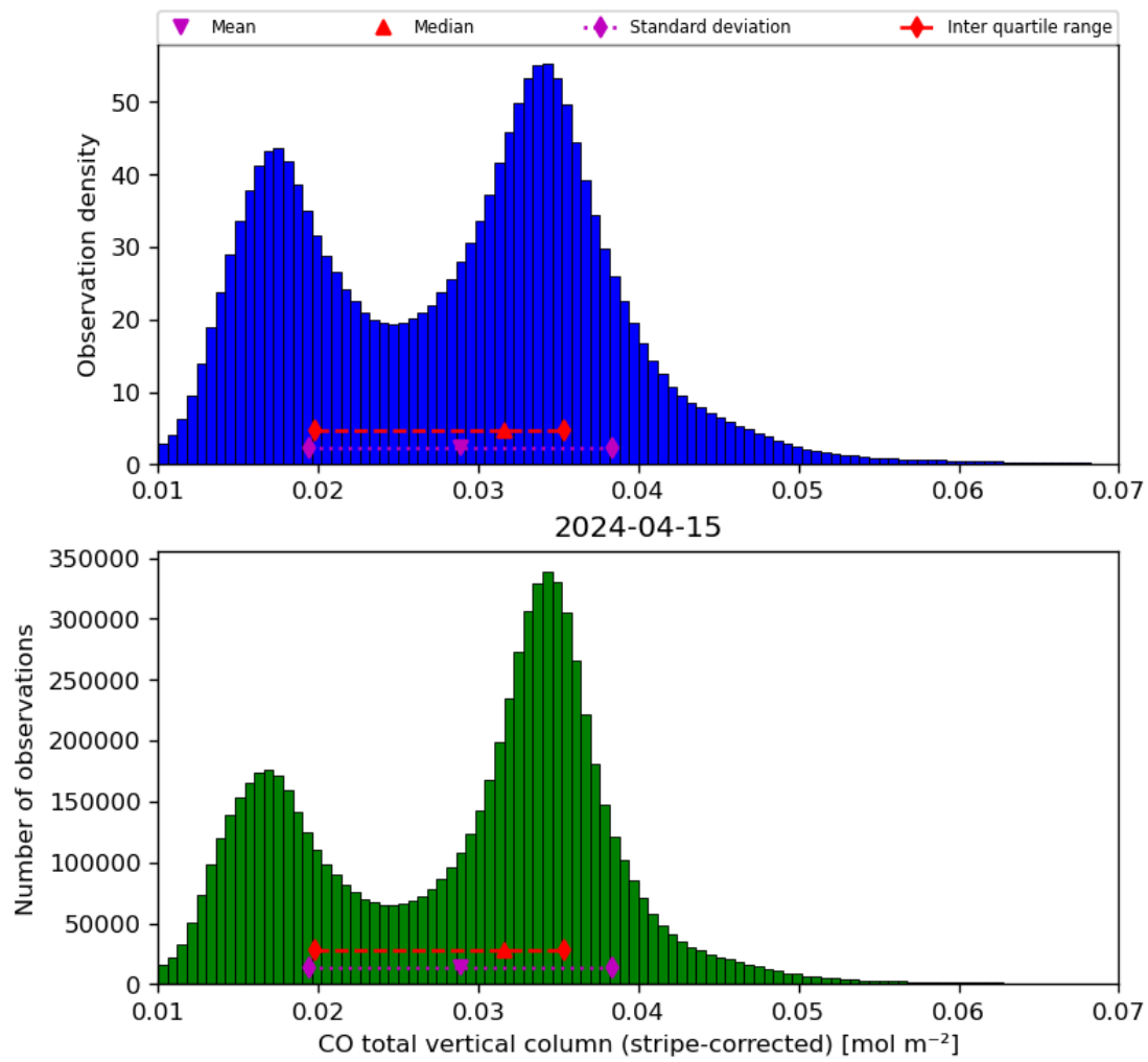
Figure 19: Histogram of “CO total vertical column (stripe-corrected)” for 2024-04-15 to 2024-04-16
