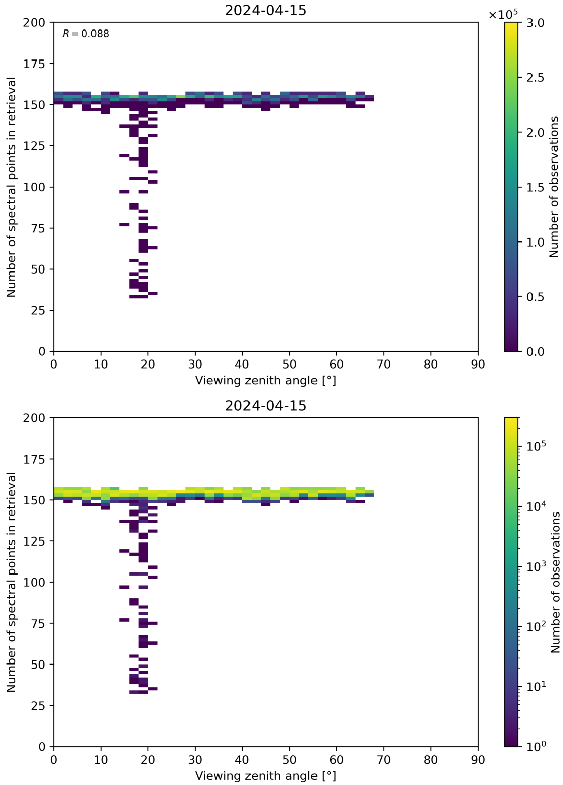
Figure 76: Scatter density plot of “Viewing zenith angle” against “Number of spectral points in retrieval” for 2024-04-15 to 2024-04-16.
