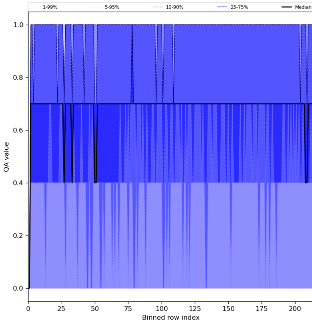
Figure 25: Along track statistics of “QA value” for 2024-04-16 to 2024-04-17
