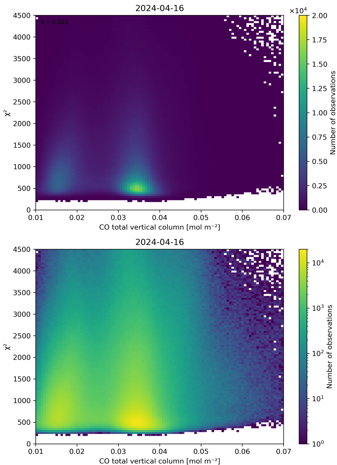
Figure 35: Scatter density plot of “CO total vertical column” against “ \chi^2 ” for 2024-04-16 to 2024-04-17.
