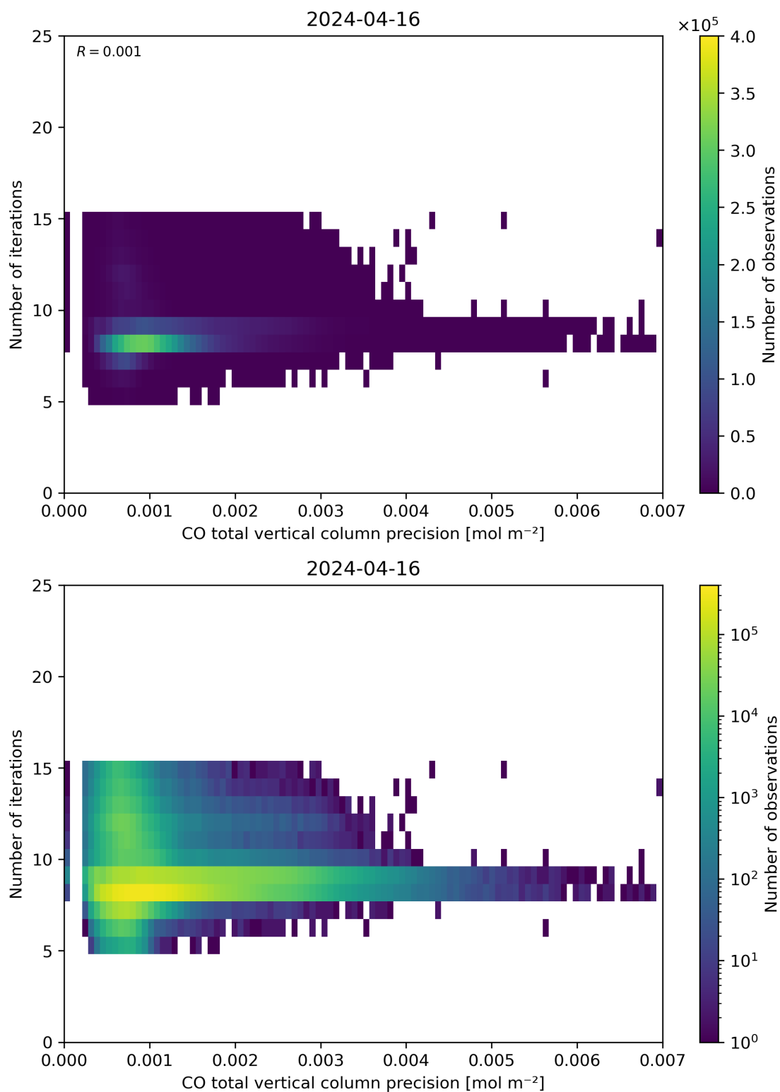
Figure 46: Scatter density plot of “CO total vertical column precision” against “Number of iterations” for 2024-04-16 to 2024-04-17.
