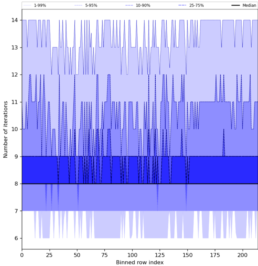
Figure 32: Along track statistics of “Number of iterations” for 2024-04-16 to 2024-04-17
