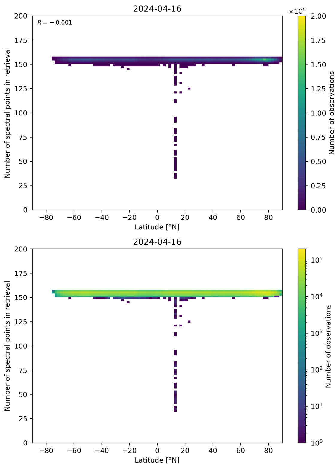
Figure 57: Scatter density plot of “Latitude” against “Number of spectral points in retrieval” for 2024-04-16 to 2024-04-17.
