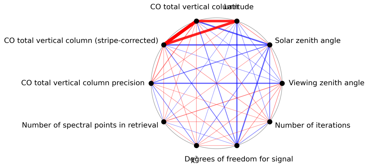
Figure 1: Map of correlation graph for 2024-04-16 to 2024-04-17.
