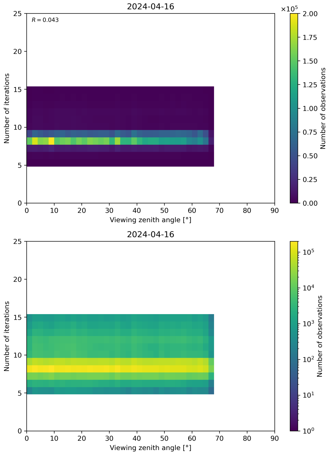
Figure 75: Scatter density plot of “Viewing zenith angle” against “Number of iterations” for 2024-04-16 to 2024-04-17.
