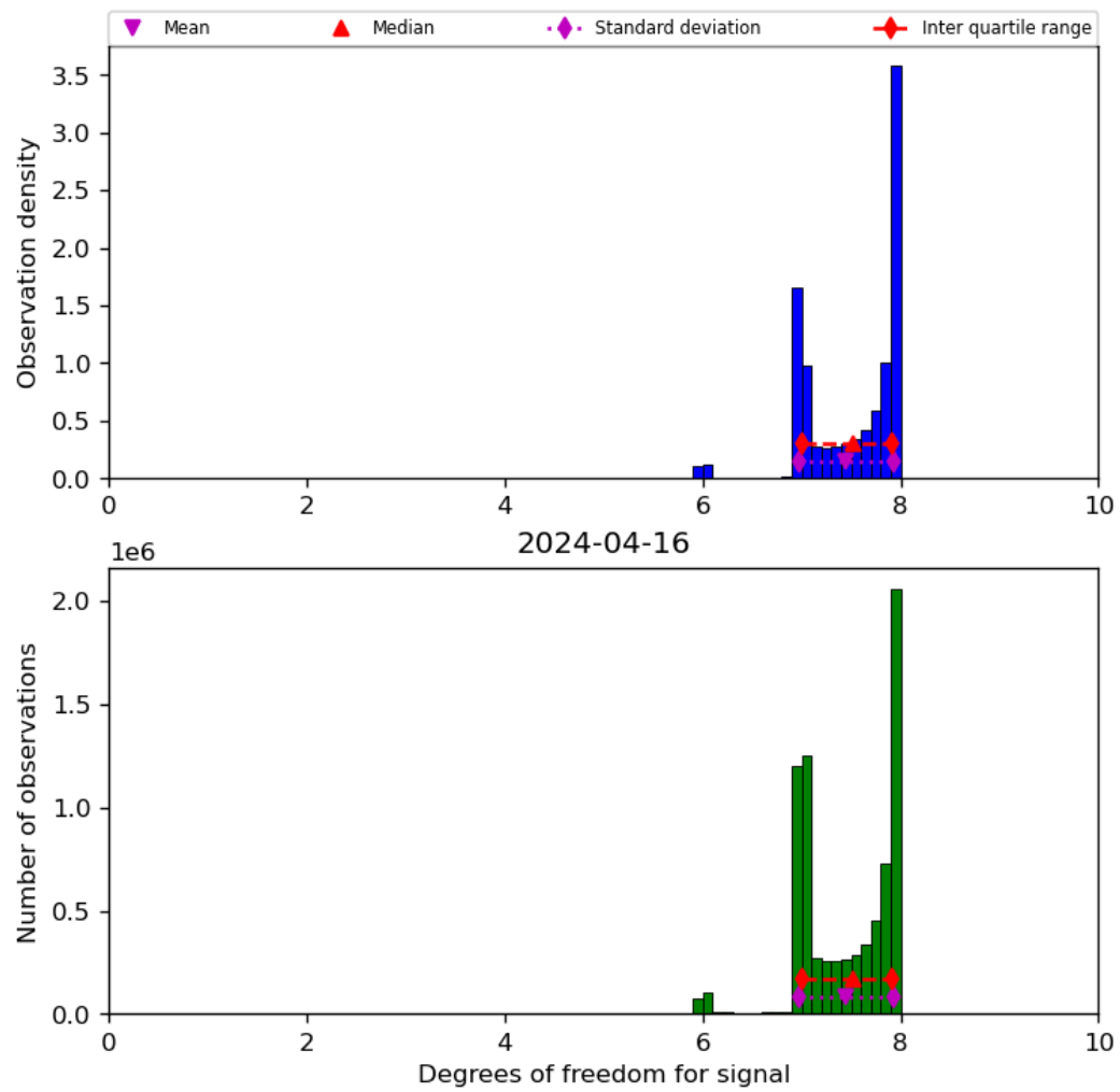
Figure 23: Histogram of “Degrees of freedom for signal” for 2024-04-16 to 2024-04-17
