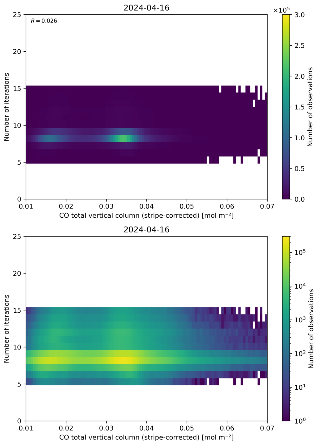
Figure 39: Scatter density plot of “CO total vertical column (stripe-corrected)” against “Number of iterations” for 2024-04-16 to 2024-04-17.
