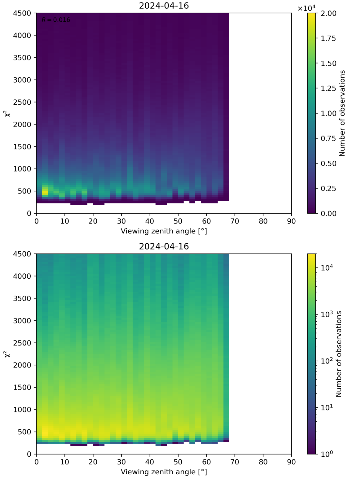
Figure 72: Scatter density plot of “Viewing zenith angle” against “ \chi^2 ” for 2024-04-16 to 2024-04-17.
