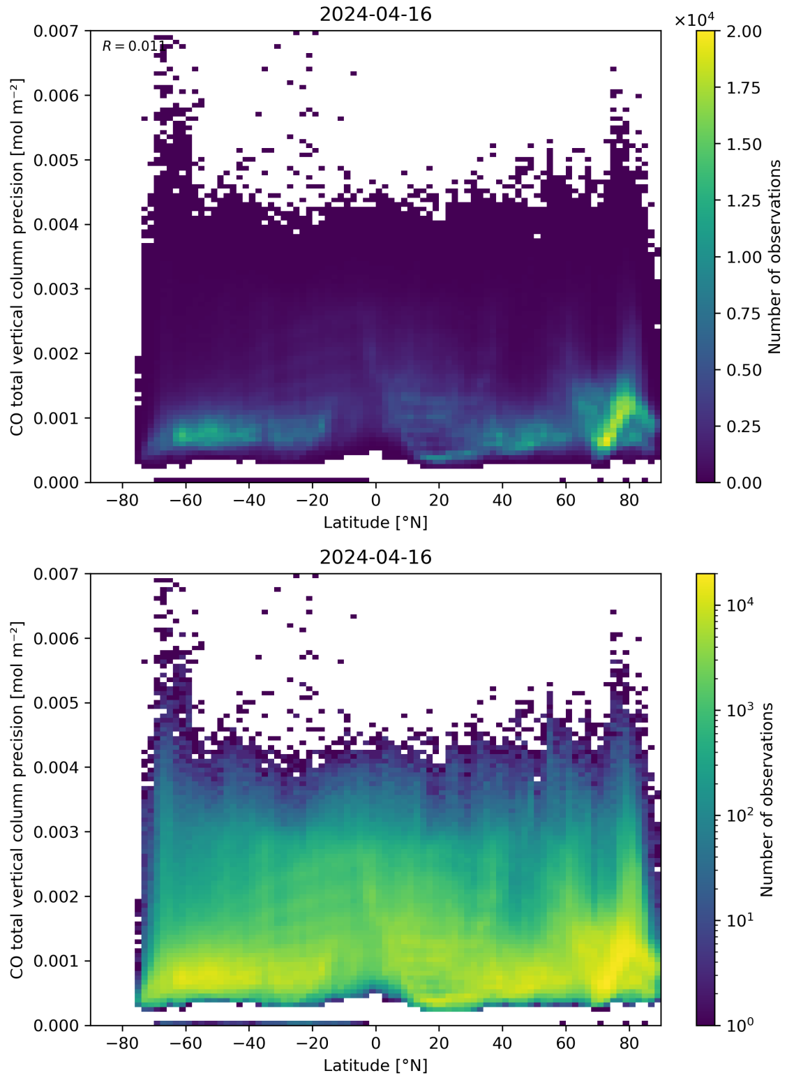
Figure 53: Scatter density plot of “Latitude” against “CO total vertical column precision” for 2024-04-16 to 2024-04-17.
