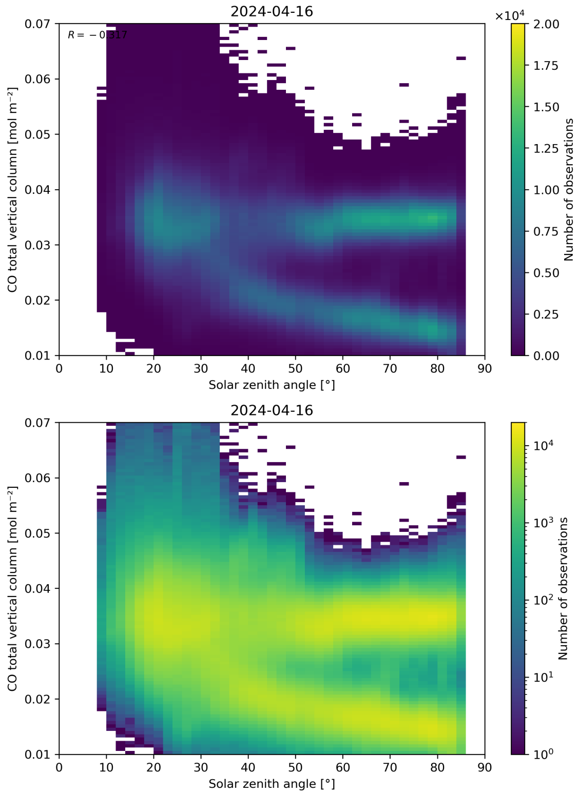
Figure 61: Scatter density plot of “Solar zenith angle” against “CO total vertical column” for 2024-04-16 to 2024-04-17.
