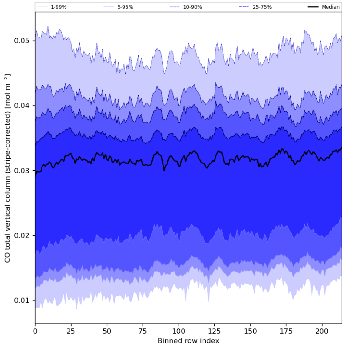
Figure 27: Along track statistics of “CO total vertical column (stripe-corrected)” for 2024-04-16 to 2024-04-17
