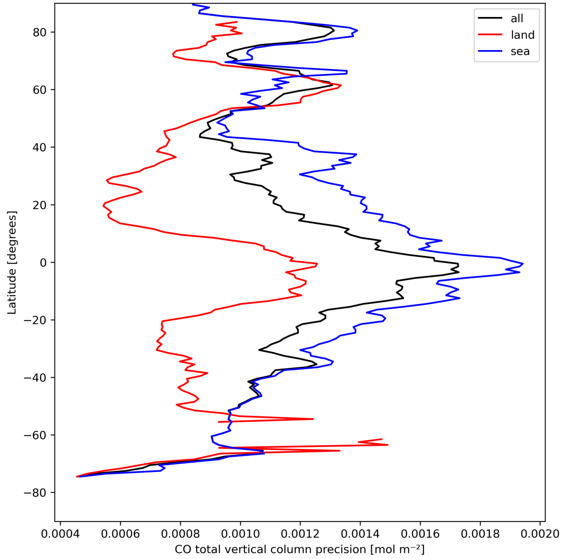
Figure 12: Zonal average of “CO total vertical column precision” for 2024-04-16 to 2024-04-17.
