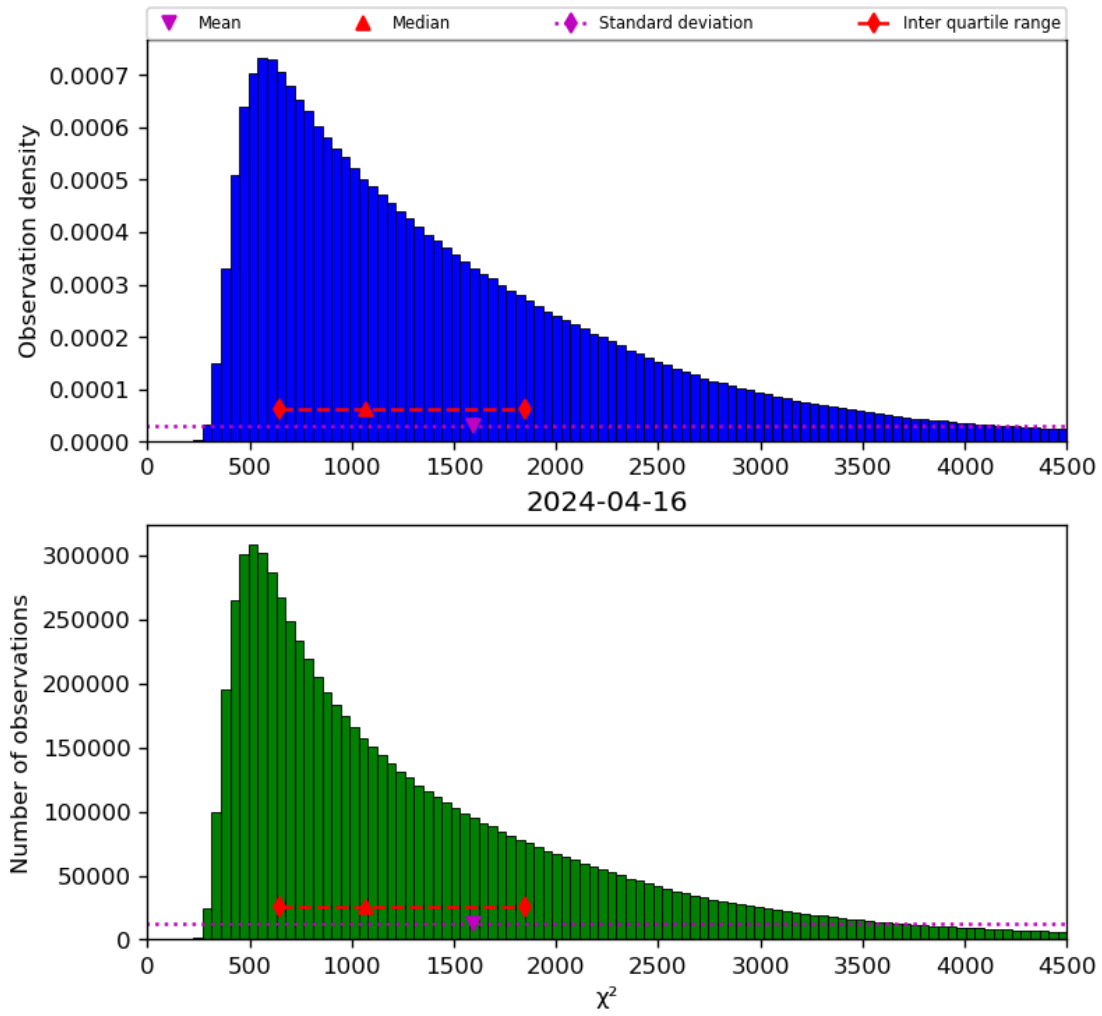
Figure 22: Histogram of “ \chi^2 ” for 2024-04-16 to 2024-04-17
