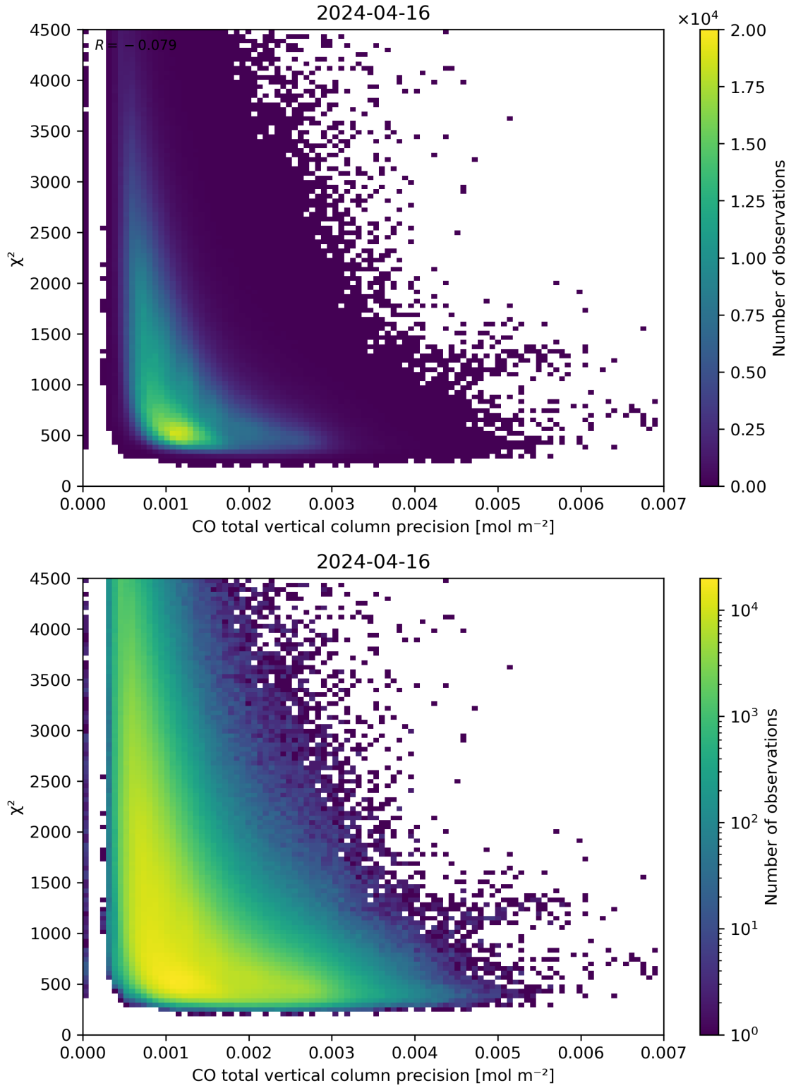
Figure 44: Scatter density plot of “CO total vertical column precision” against “ \chi^2 ” for 2024-04-16 to 2024-04-17.
