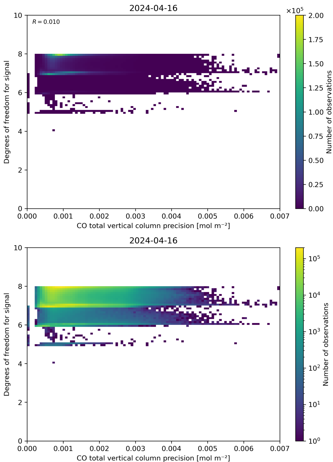
Figure 45: Scatter density plot of “CO total vertical column precision” against “Degrees of freedom for signal” for 2024-04-16 to 2024-04-17.
