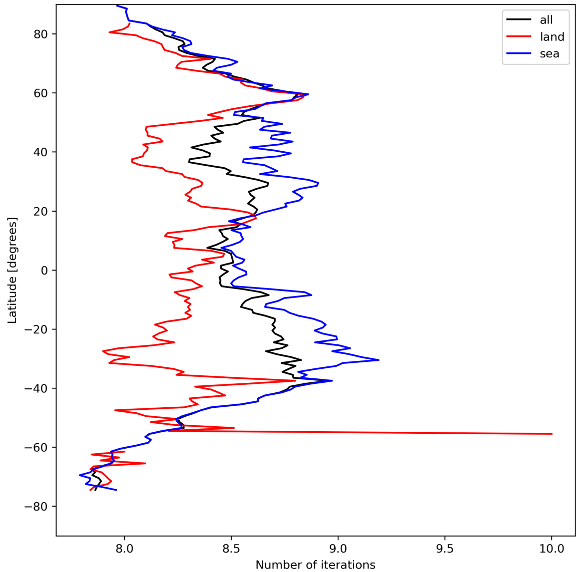
Figure 16: Zonal average of “Number of iterations” for 2024-04-16 to 2024-04-17.
