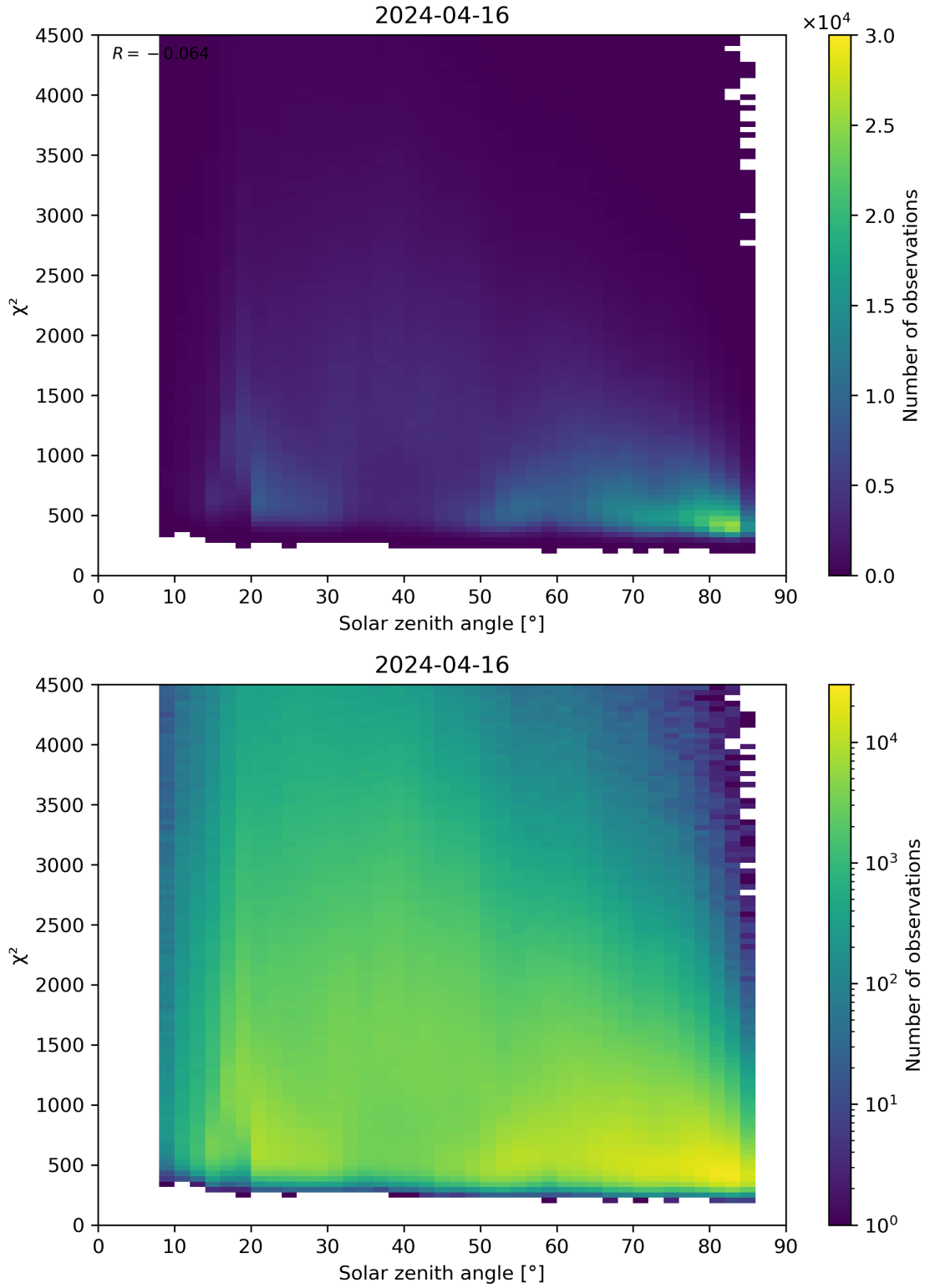
Figure 64: Scatter density plot of “Solar zenith angle” against “ \chi^2 ” for 2024-04-16 to 2024-04-17.
