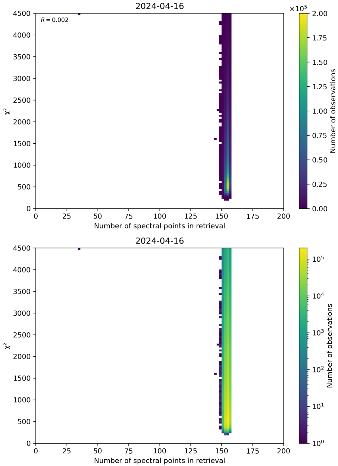
Figure 58: Scatter density plot of “Number of spectral points in retrieval” against “ \chi^2 ” for 2024-04-16 to 2024-04-17.
