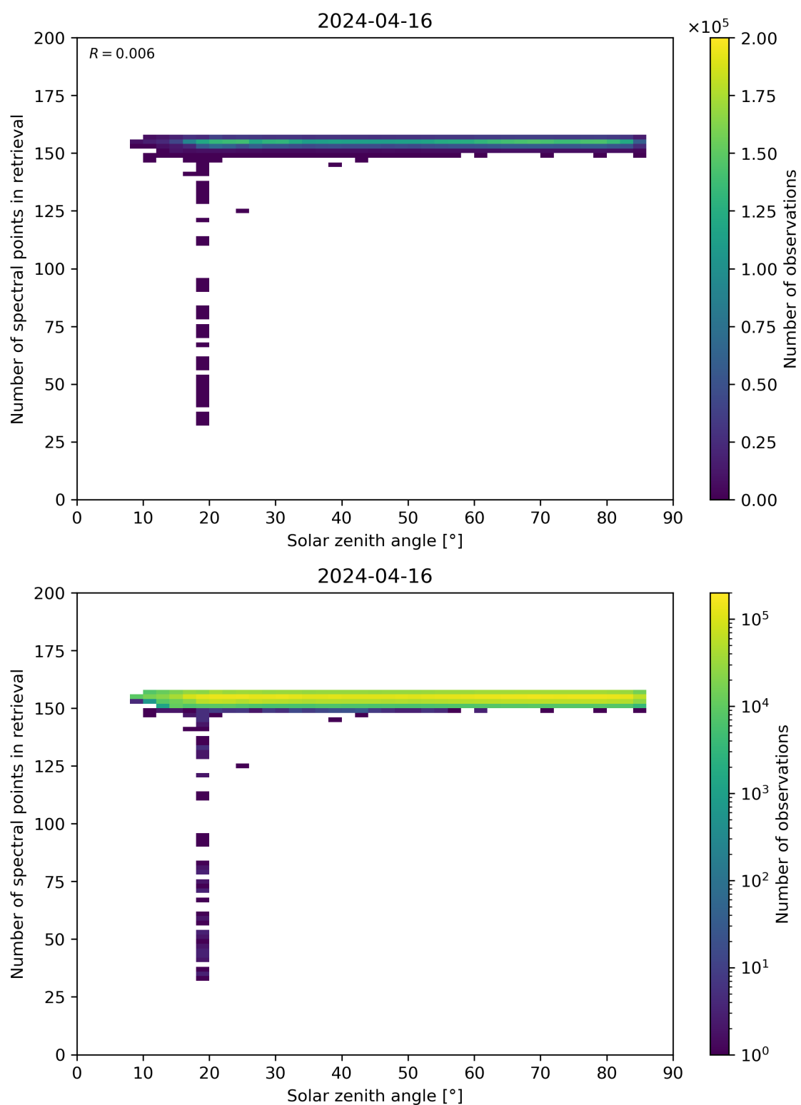
Figure 68: Scatter density plot of “Solar zenith angle” against “Number of spectral points in retrieval” for 2024-04-16 to 2024-04-17.
