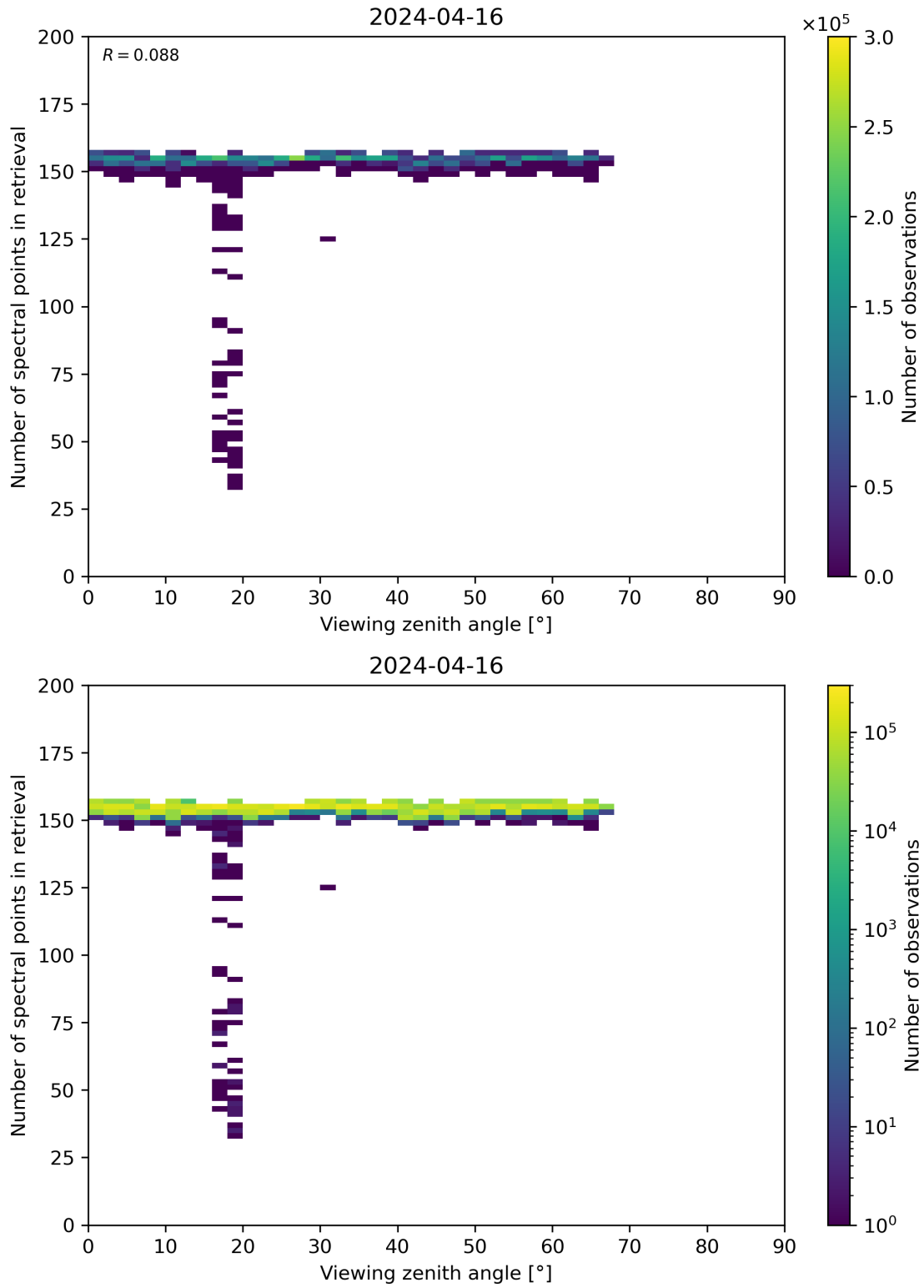
Figure 76: Scatter density plot of “Viewing zenith angle” against “Number of spectral points in retrieval” for 2024-04-16 to 2024-04-17.
