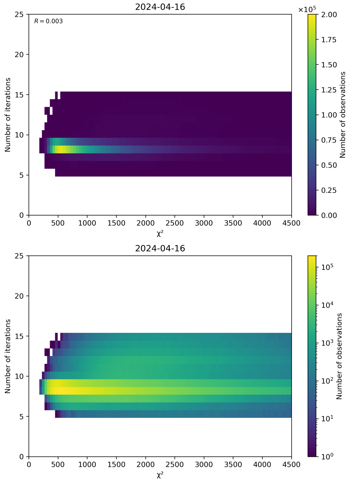
Figure 49: Scatter density plot of “ \chi^2 ” against “Number of iterations” for 2024-04-16 to 2024-04-17.
