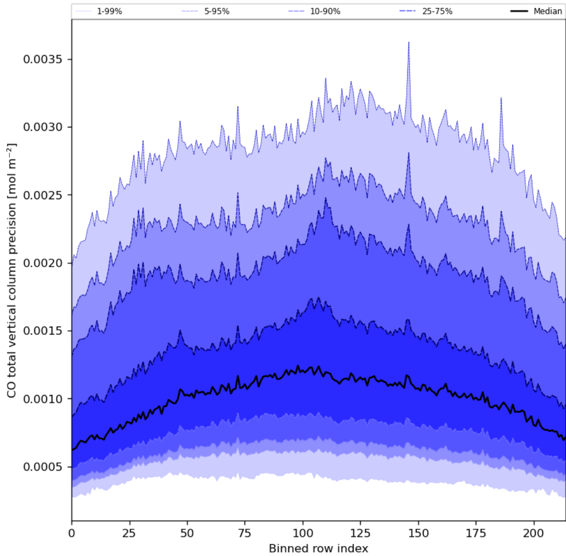
Figure 28: Along track statistics of “CO total vertical column precision” for 2024-04-16 to 2024-04-17
