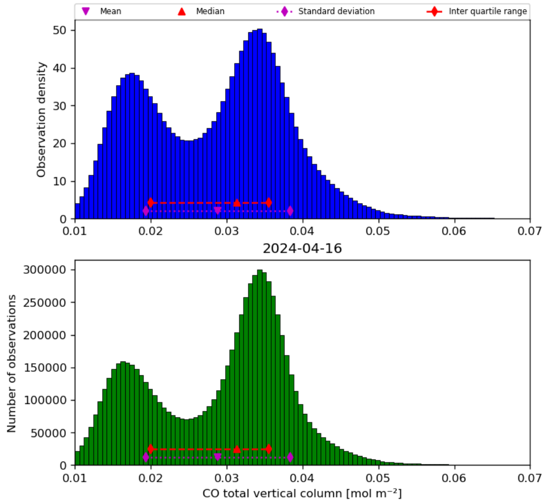
Figure 18: Histogram of “CO total vertical column” for 2024-04-16 to 2024-04-17
