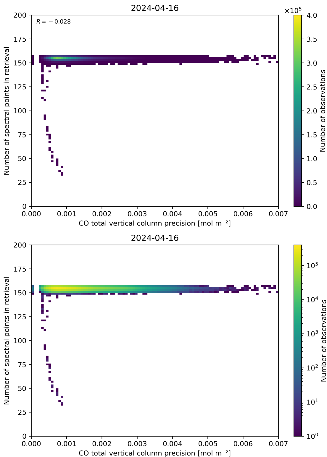
Figure 47: Scatter density plot of “CO total vertical column precision” against “Number of spectral points in retrieval” for 2024-04-16 to 2024-04-17.
