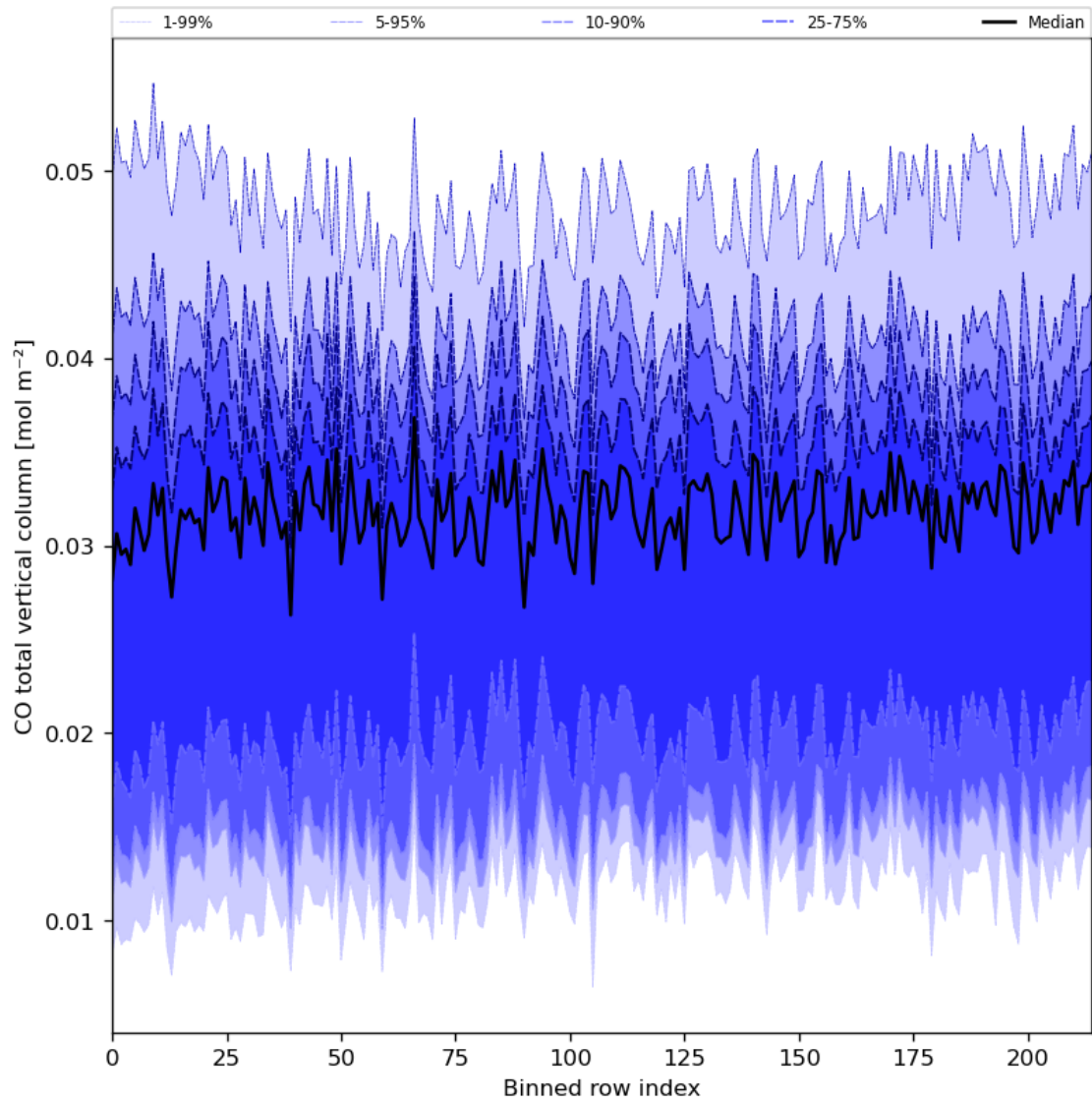
Figure 26: Along track statistics of “CO total vertical column” for 2024-04-16 to 2024-04-17
