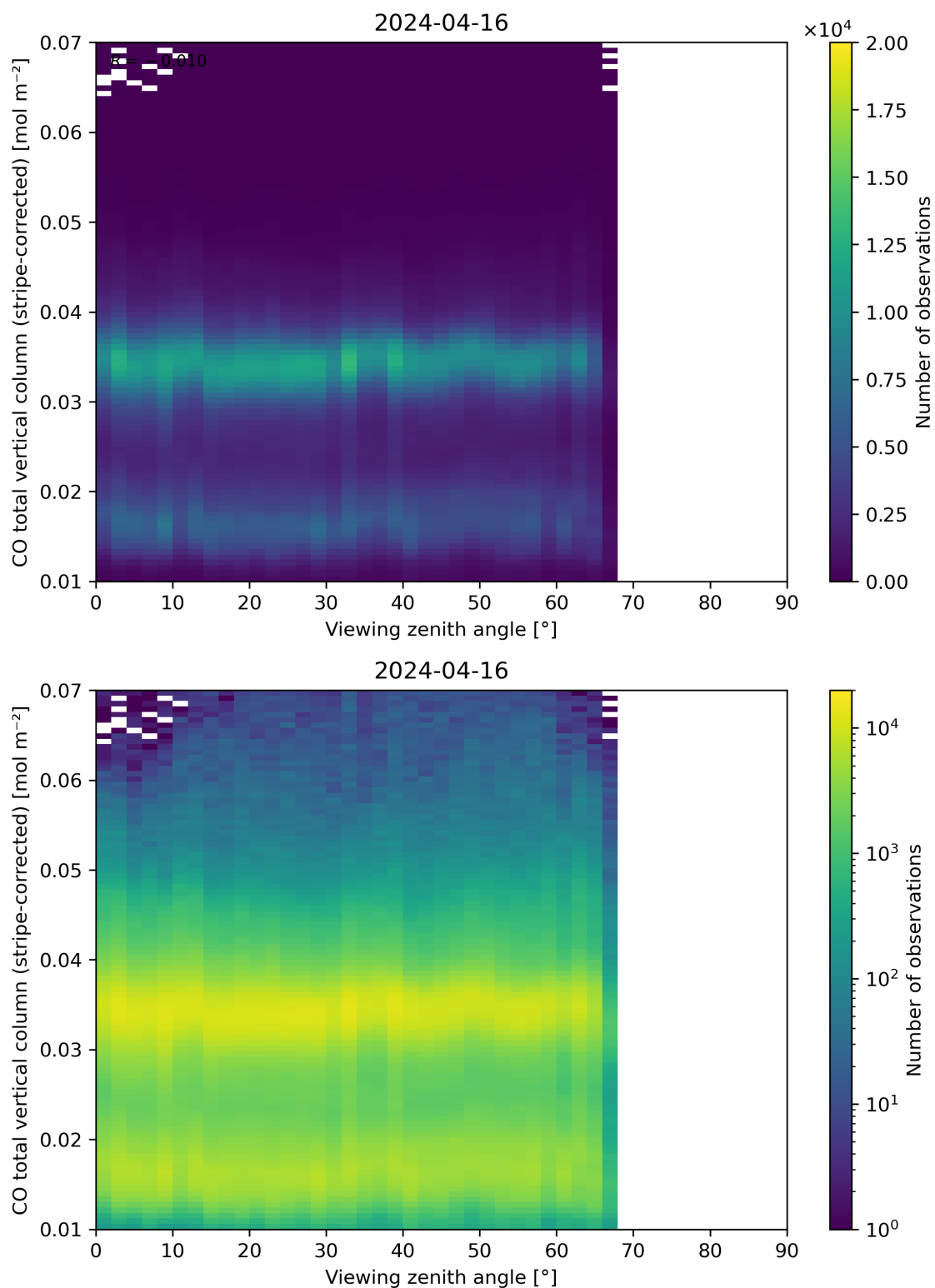
Figure 70: Scatter density plot of “Viewing zenith angle” against “CO total vertical column (stripe-corrected)” for 2024-04-16 to 2024-04-17.
