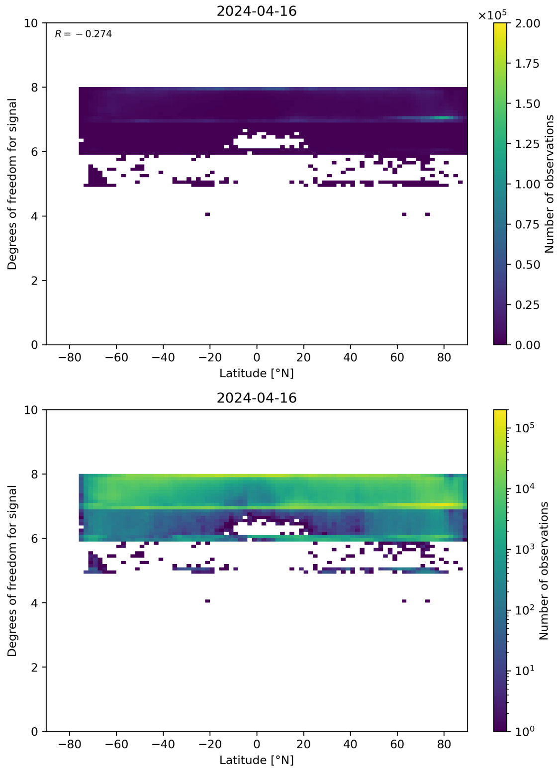
Figure 55: Scatter density plot of “Latitude” against “Degrees of freedom for signal” for 2024-04-16 to 2024-04-17.
