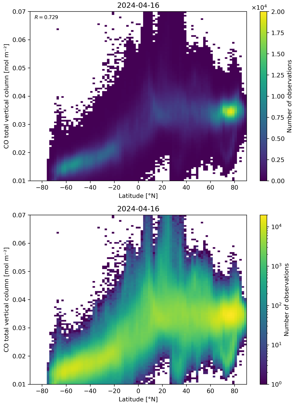
Figure 51: Scatter density plot of “Latitude” against “CO total vertical column” for 2024-04-16 to 2024-04-17.
