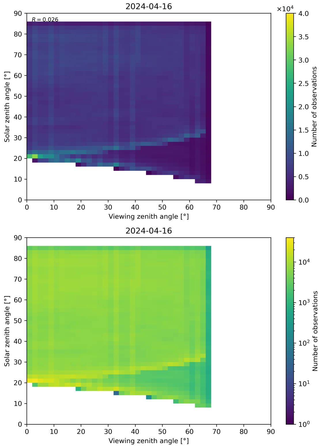
Figure 77: Scatter density plot of “Viewing zenith angle” against “Solar zenith angle” for 2024-04-16 to 2024-04-17.
