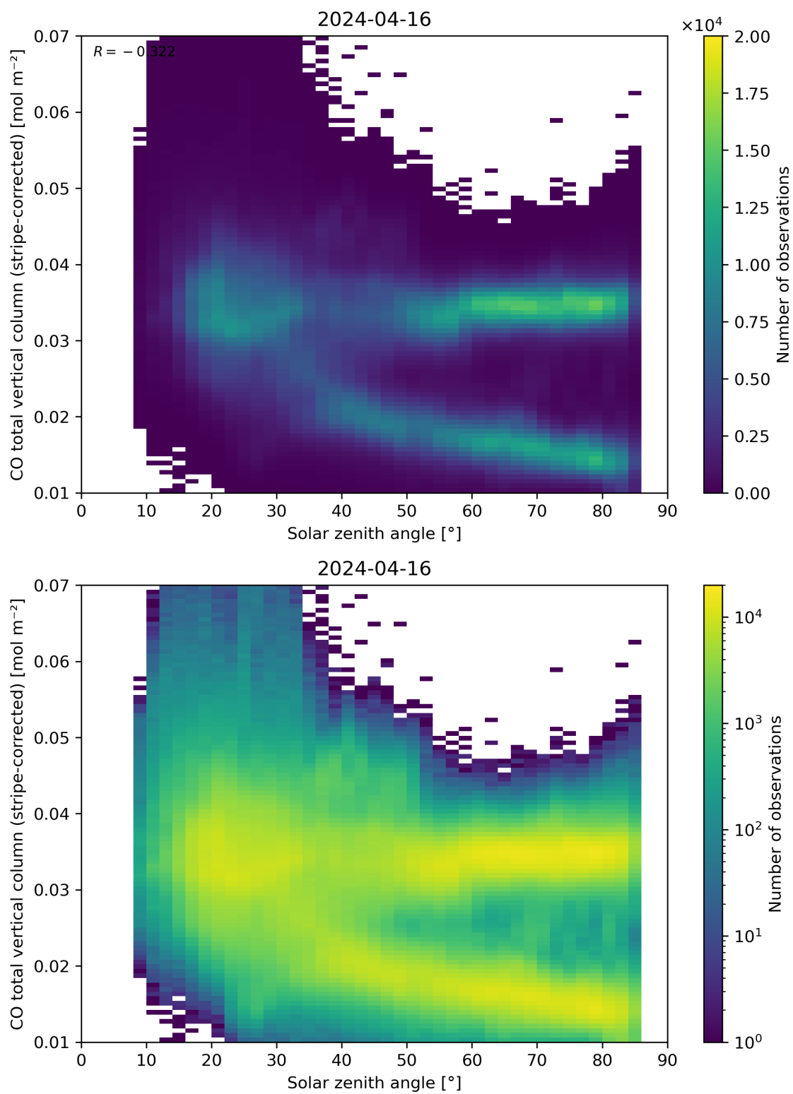
Figure 62: Scatter density plot of “Solar zenith angle” against “CO total vertical column (stripe-corrected)” for 2024-04-16 to 2024-04-17.
