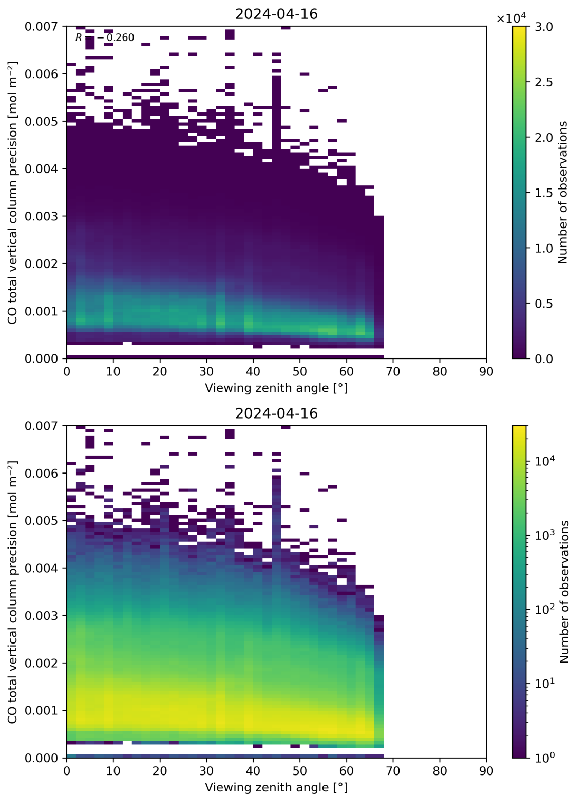
Figure 71: Scatter density plot of “Viewing zenith angle” against “CO total vertical column precision” for 2024-04-16 to 2024-04-17.
