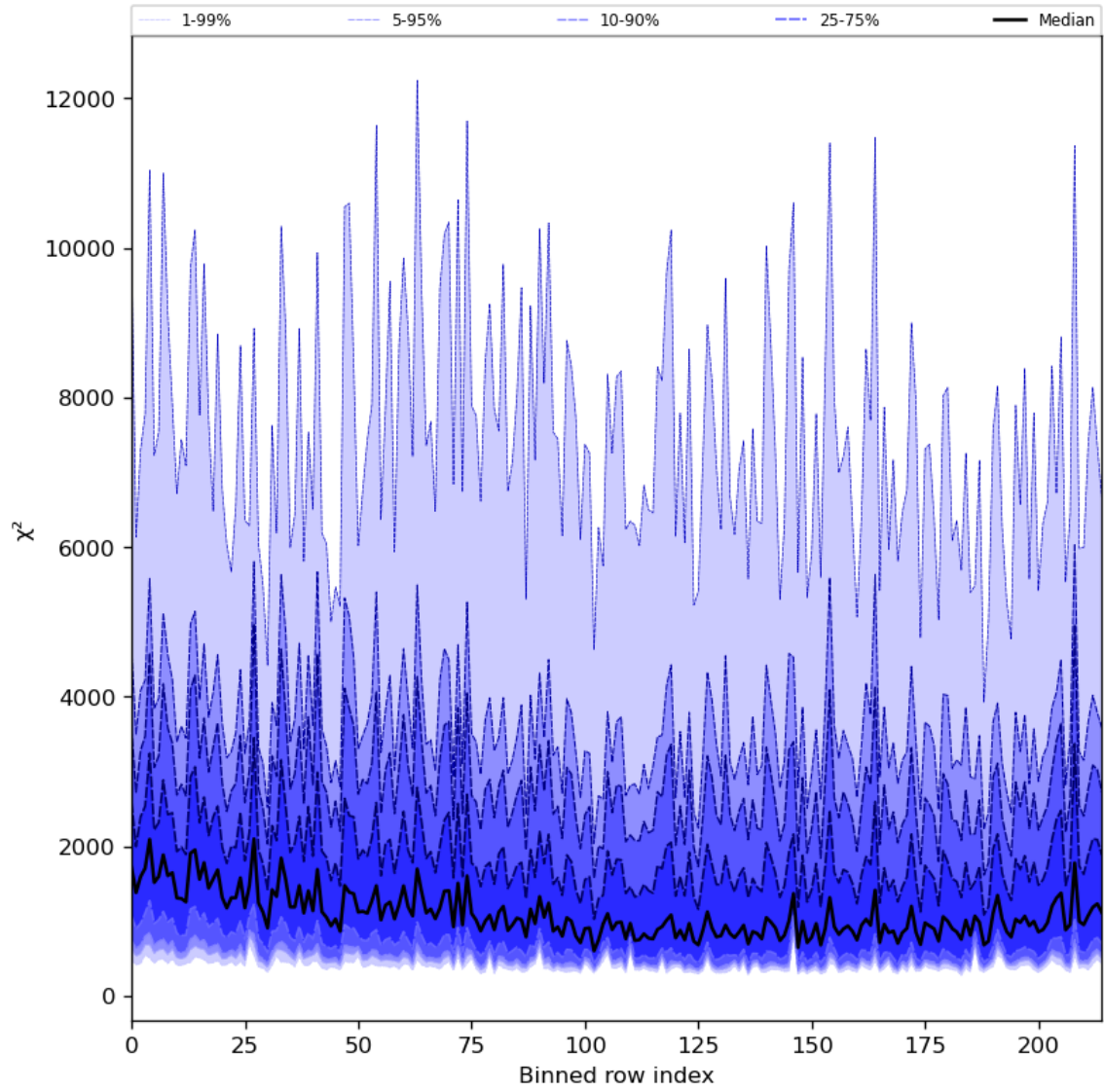
Figure 30: Along track statistics of “ \chi^2 ” for 2024-04-16 to 2024-04-17
