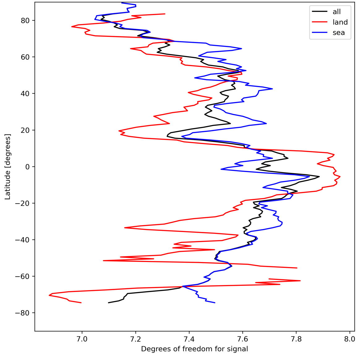
Figure 15: Zonal average of “Degrees of freedom for signal” for 2024-04-16 to 2024-04-17.
