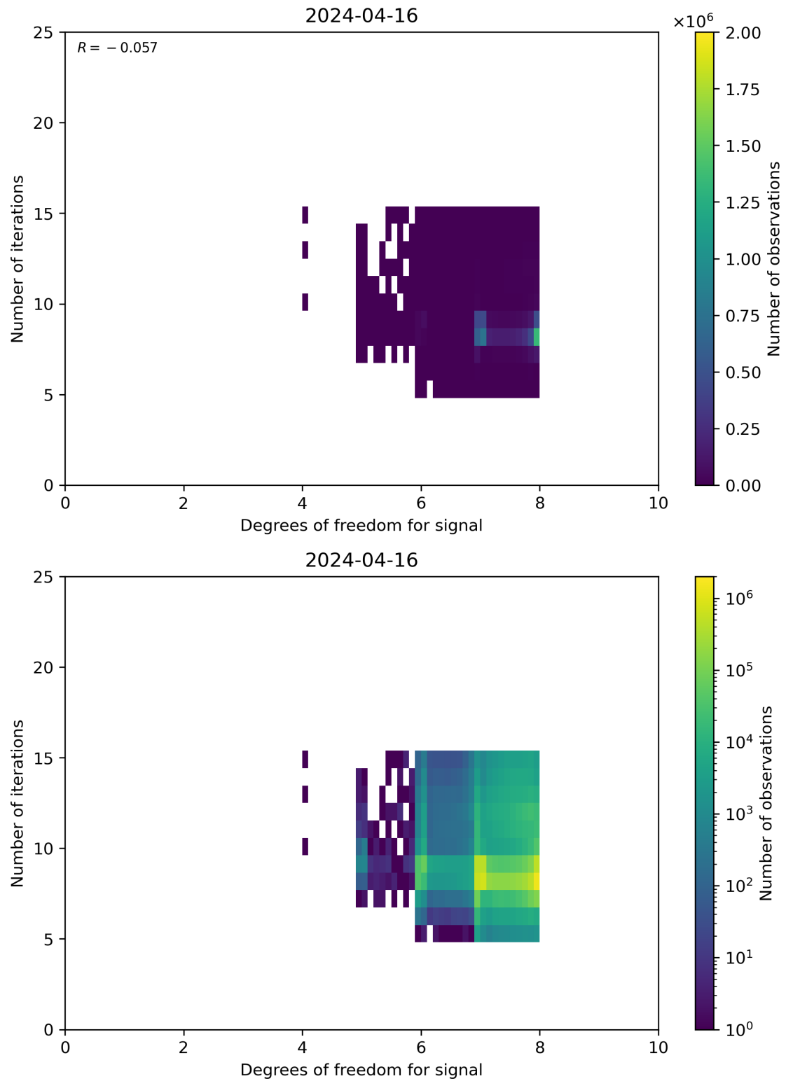
Figure 50: Scatter density plot of “Degrees of freedom for signal” against “Number of iterations” for 2024-04-16 to 2024-04-17.
