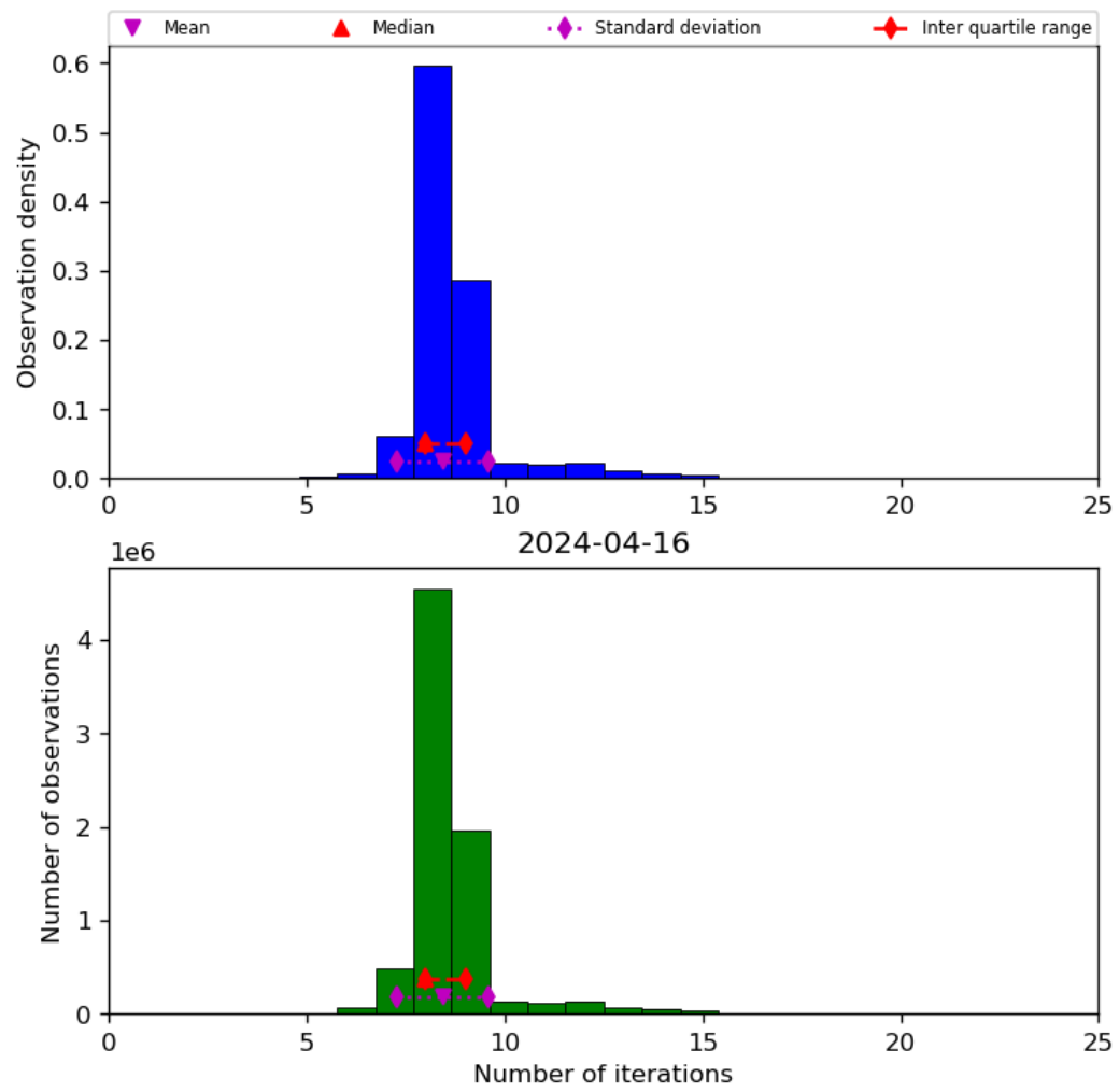
Figure 24: Histogram of “Number of iterations” for 2024-04-16 to 2024-04-17
