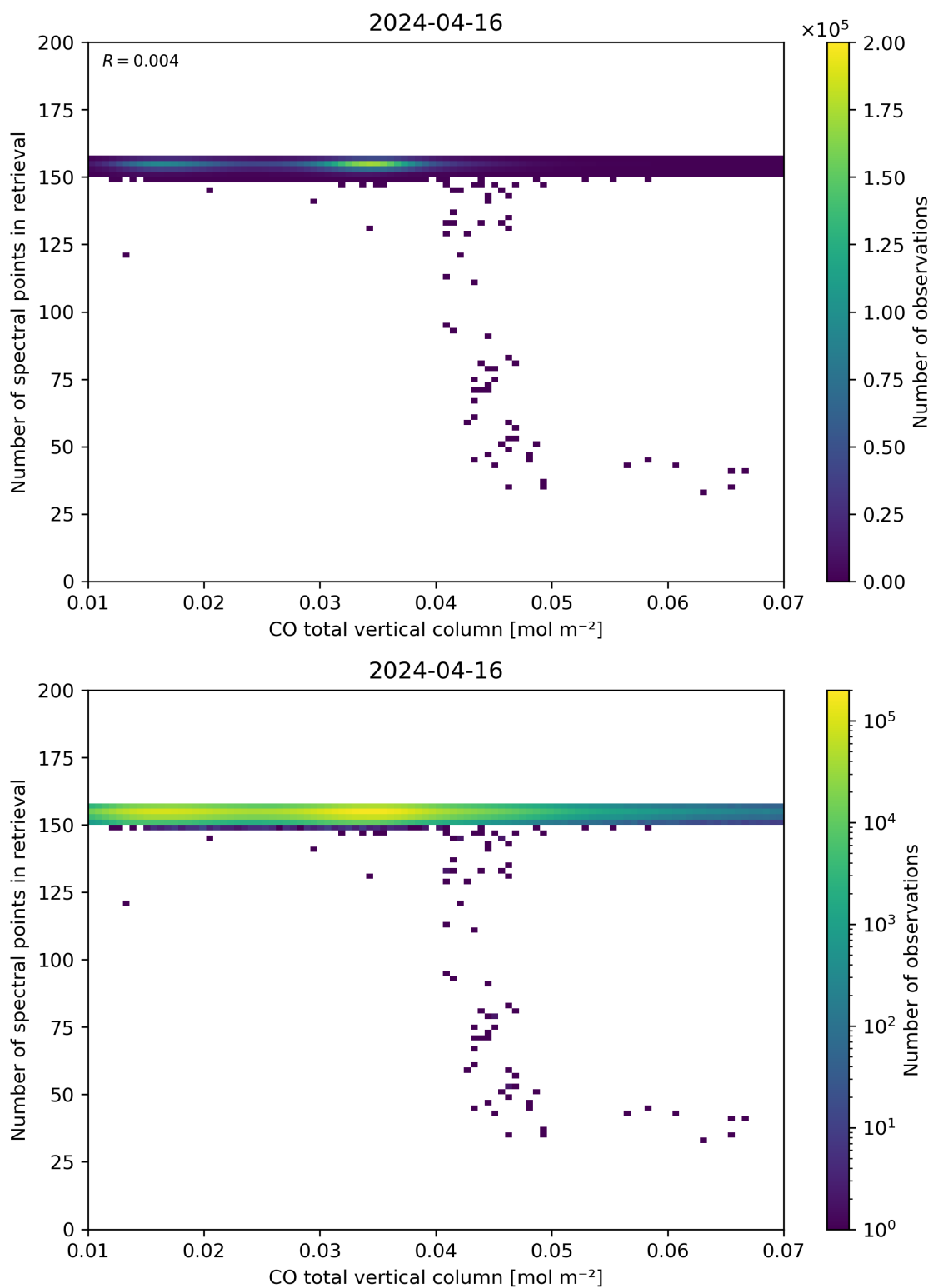
Figure 43: Scatter density plot of “CO total vertical column” against “Number of spectral points in retrieval” for 2024-04-16 to 2024-04-17.
