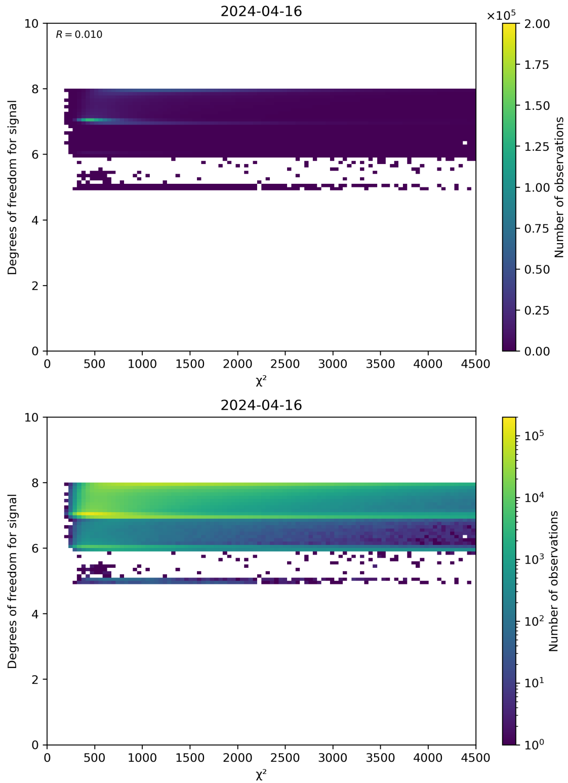
Figure 48: Scatter density plot of “ \chi^2 ” against “Degrees of freedom for signal” for 2024-04-16 to 2024-04-17.
