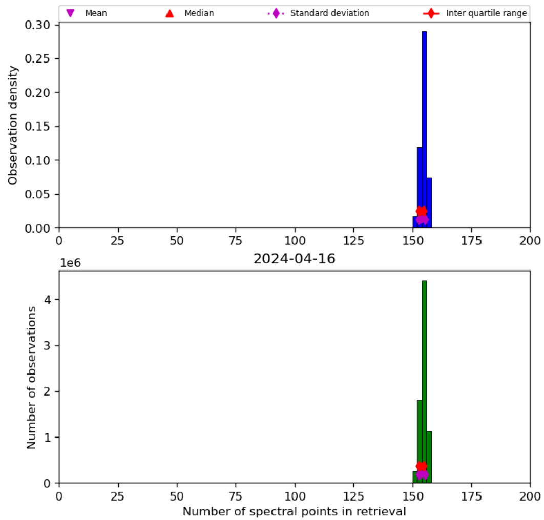
Figure 21: Histogram of “Number of spectral points in retrieval” for 2024-04-16 to 2024-04-17
