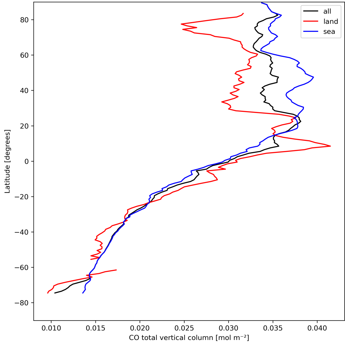
Figure 10: Zonal average of “CO total vertical column” for 2024-04-16 to 2024-04-17.
