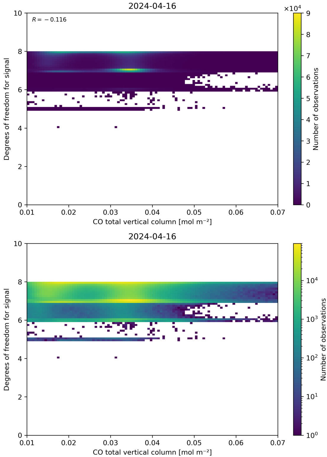
Figure 41: Scatter density plot of “CO total vertical column” against “Degrees of freedom for signal” for 2024-04-16 to 2024-04-17.
