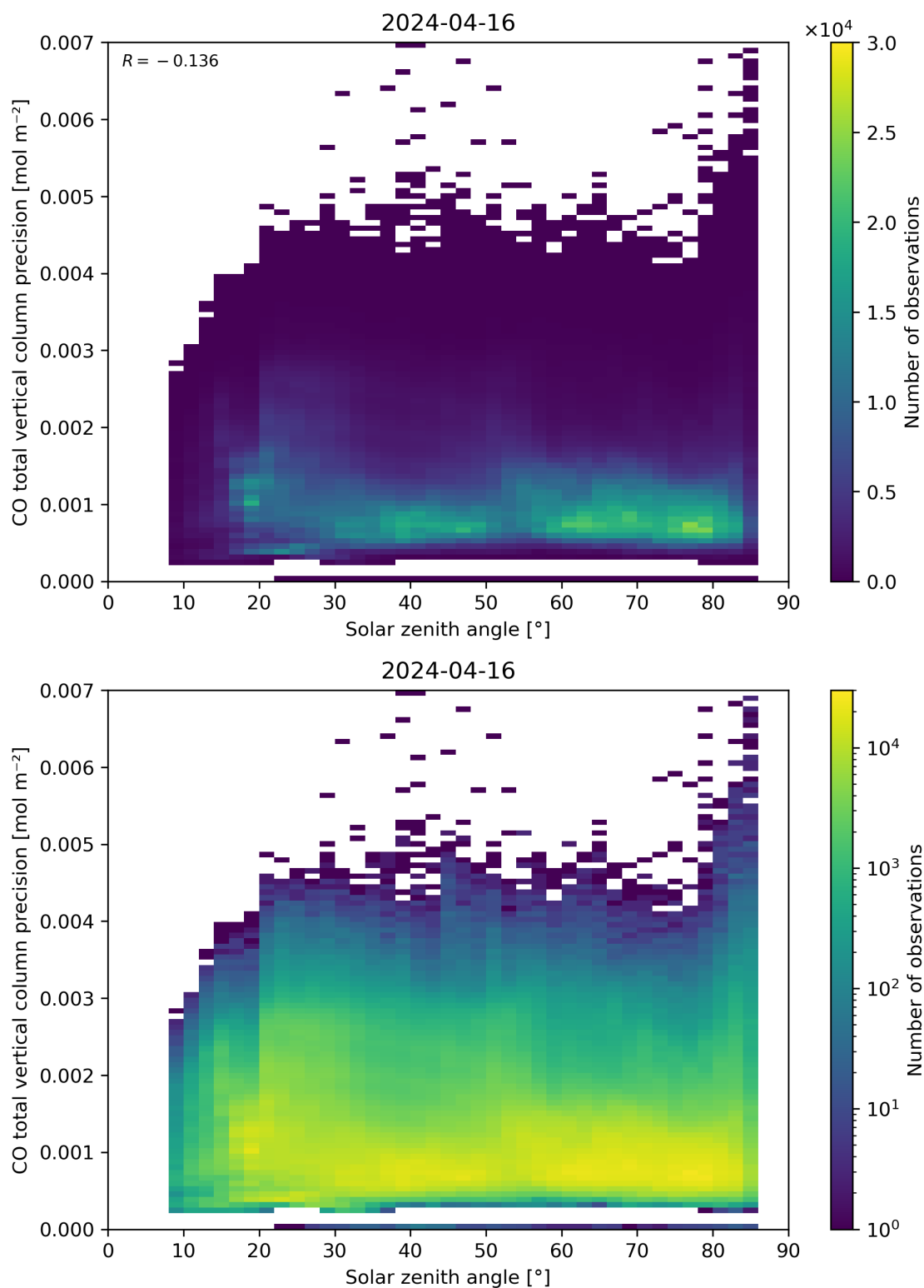
Figure 63: Scatter density plot of “Solar zenith angle” against “CO total vertical column precision” for 2024-04-16 to 2024-04-17.
