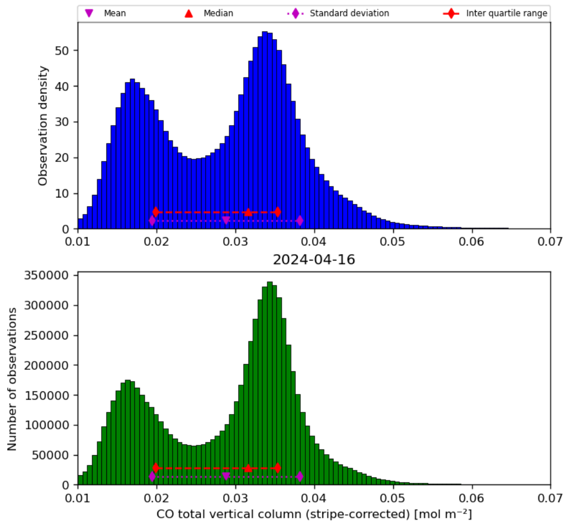
Figure 19: Histogram of “CO total vertical column (stripe-corrected)” for 2024-04-16 to 2024-04-17
