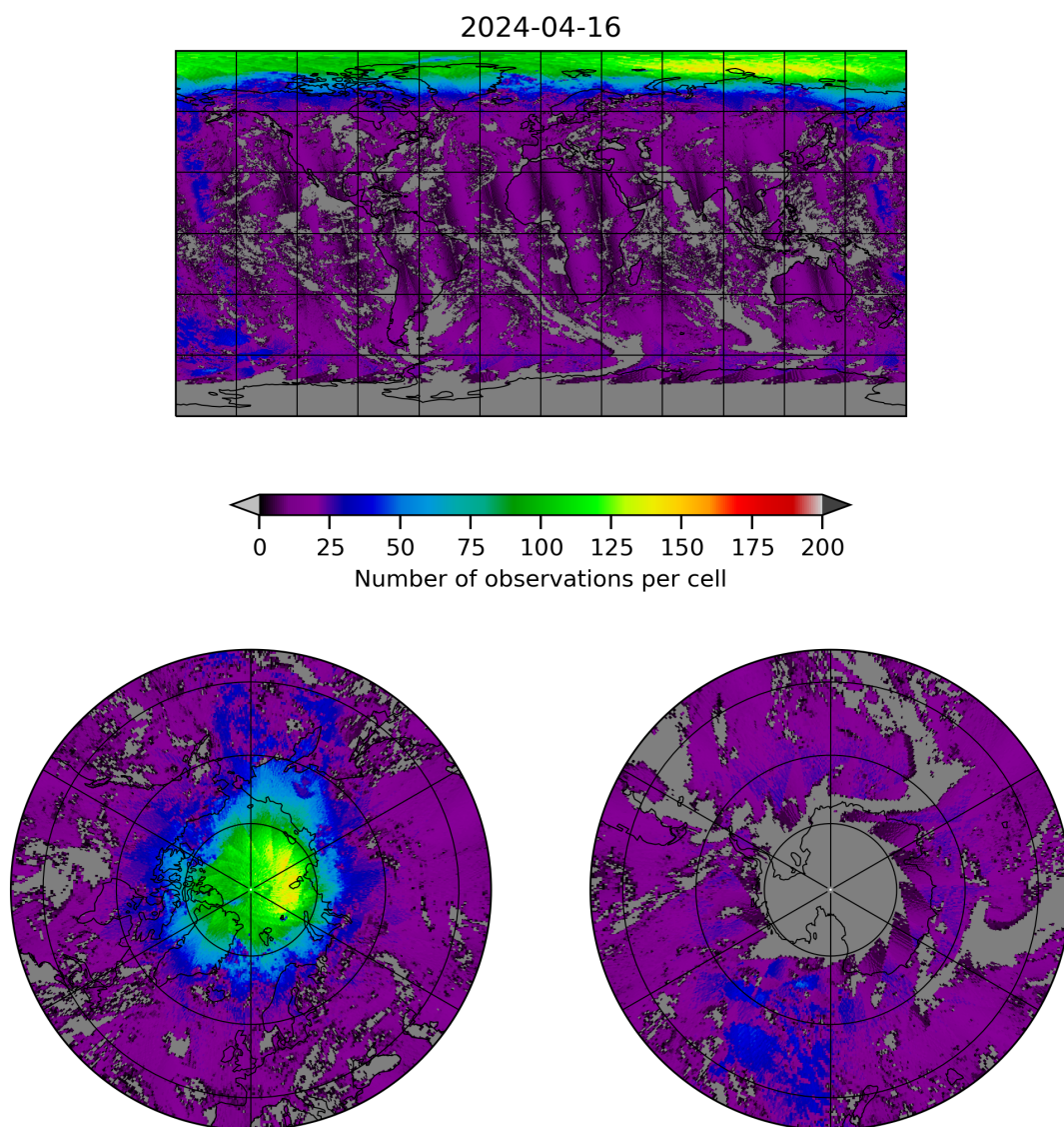
Figure 8: Map of the number of observations for 2024-04-16 to 2024-04-17
