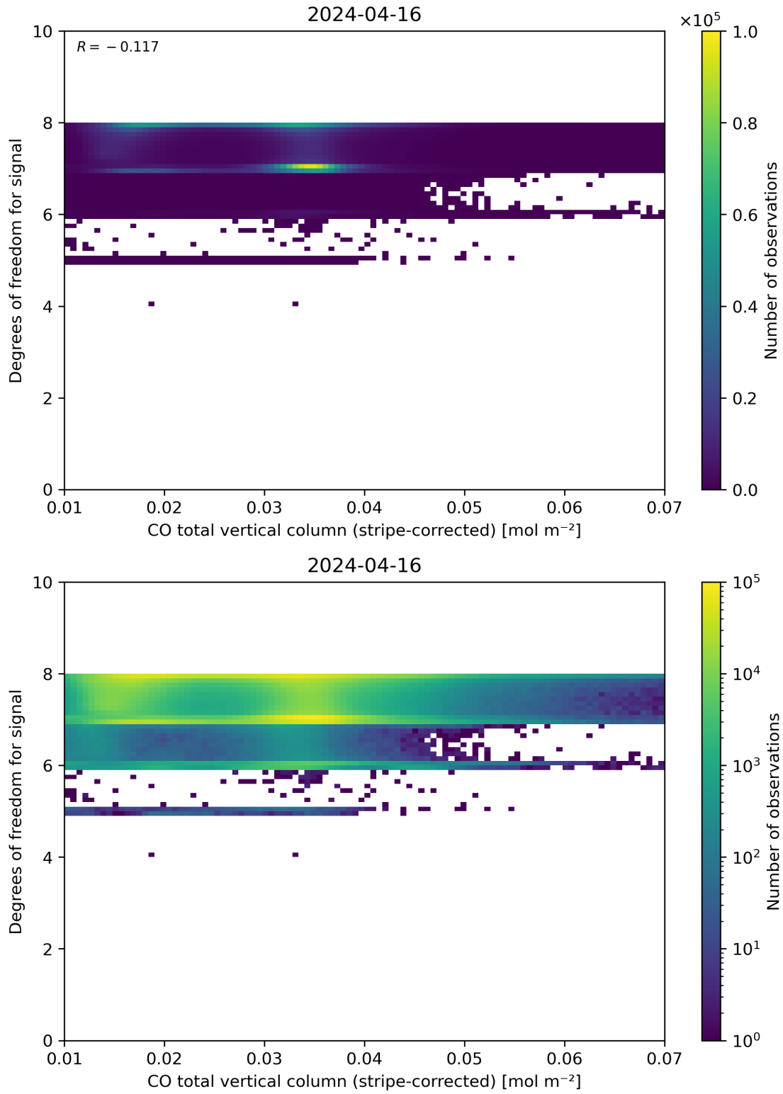
Figure 38: Scatter density plot of “CO total vertical column (stripe-corrected)” against “Degrees of freedom for signal” for 2024-04-16 to 2024-04-17.
