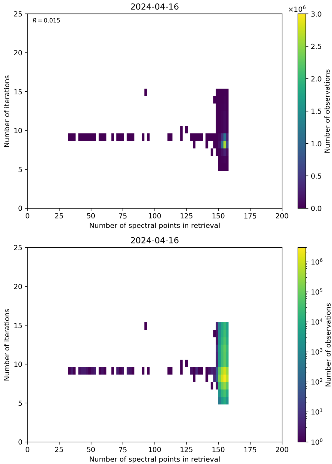
Figure 60: Scatter density plot of “Number of spectral points in retrieval” against “Number of iterations” for 2024-04-16 to 2024-04-17.
