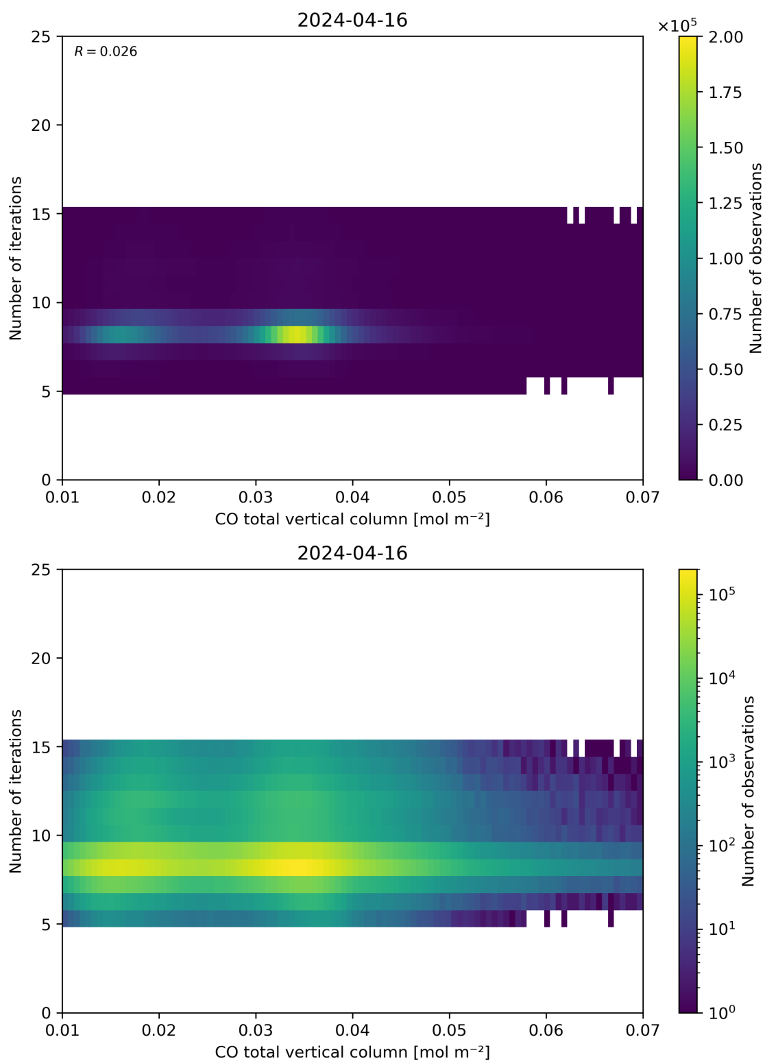
Figure 42: Scatter density plot of “CO total vertical column” against “Number of iterations” for 2024-04-16 to 2024-04-17.
