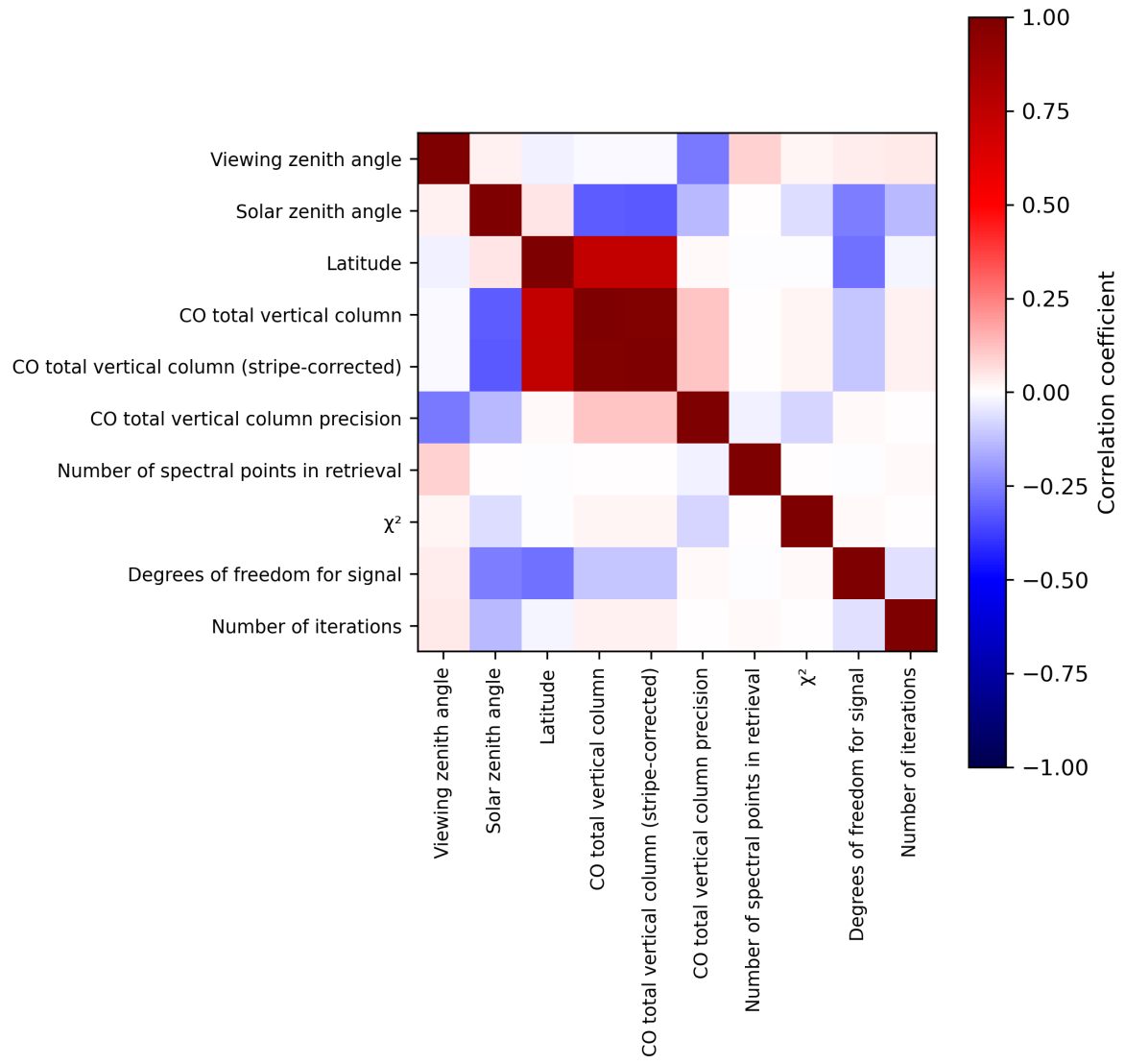
Figure 2: Map of correlation matrix for 2024-04-16 to 2024-04-17.
