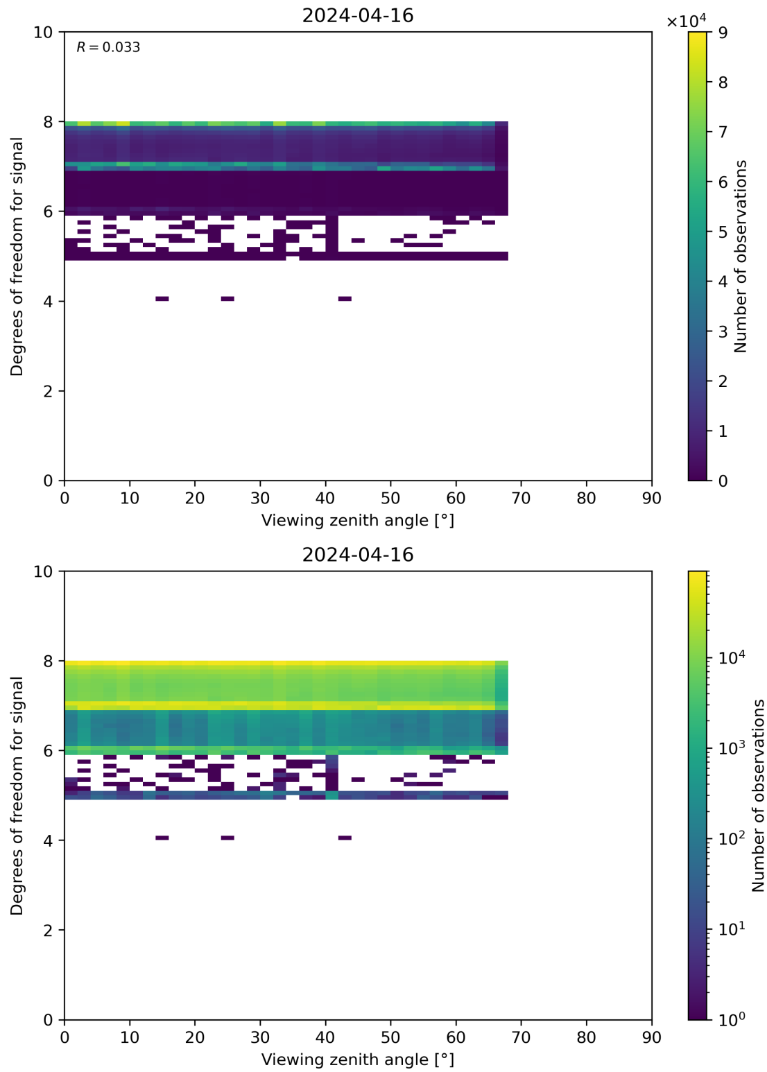
Figure 73: Scatter density plot of “Viewing zenith angle” against “Degrees of freedom for signal” for 2024-04-16 to 2024-04-17.
