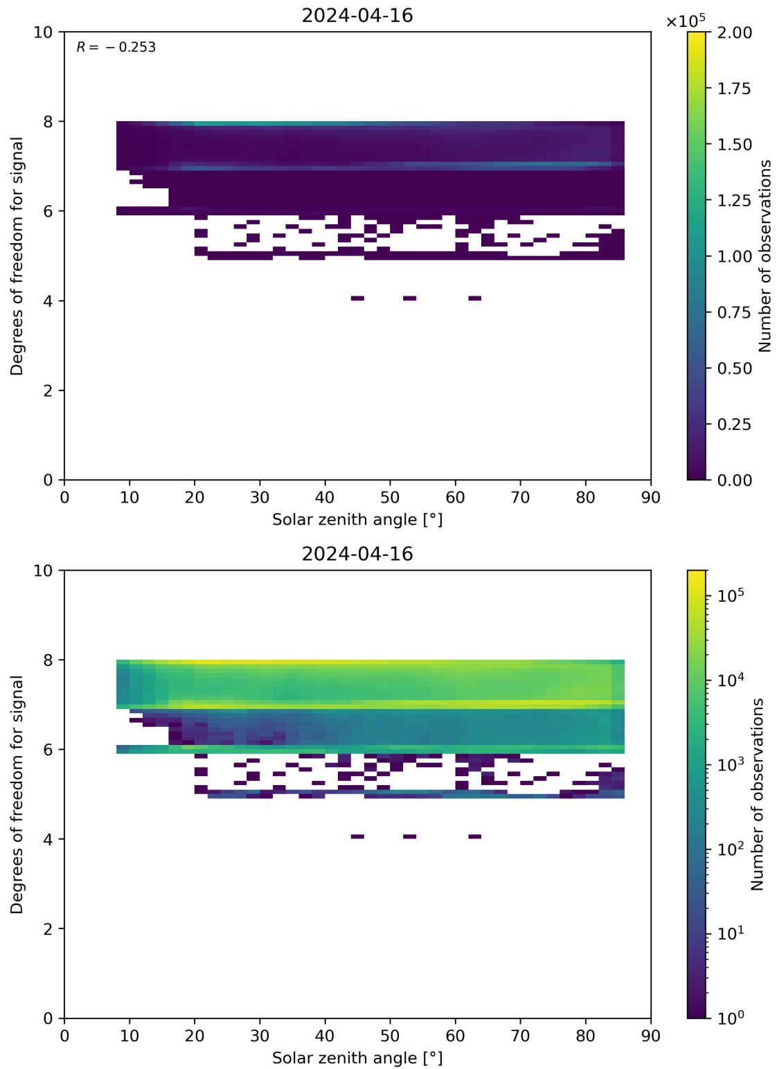
Figure 65: Scatter density plot of “Solar zenith angle” against “Degrees of freedom for signal” for 2024-04-16 to 2024-04-17.
