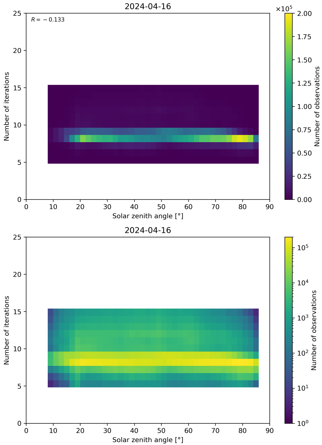
Figure 67: Scatter density plot of “Solar zenith angle” against “Number of iterations” for 2024-04-16 to 2024-04-17.
