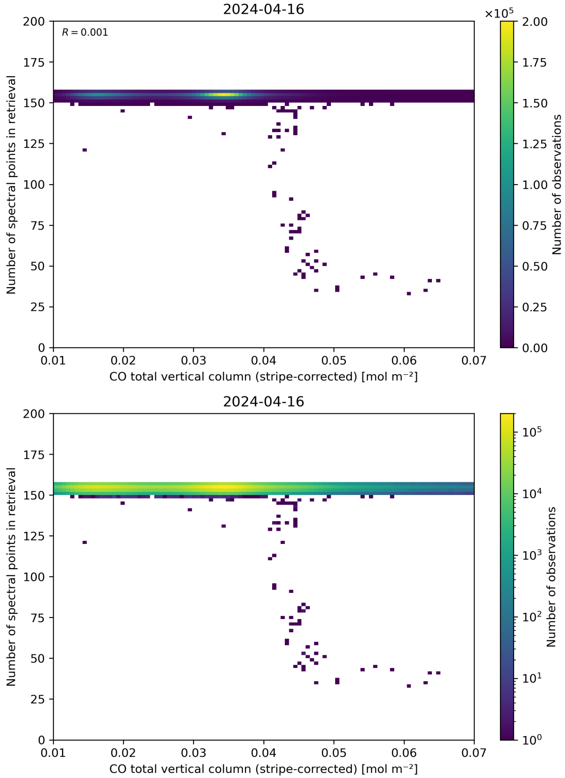
Figure 40: Scatter density plot of “CO total vertical column (stripe-corrected)” against “Number of spectral points in retrieval” for 2024-04-16 to 2024-04-17.
