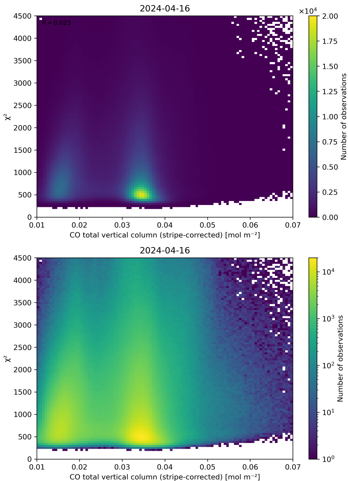
Figure 37: Scatter density plot of “CO total vertical column (stripe-corrected)” against “ \chi^2 ” for 2024-04-16 to 2024-04-17.
