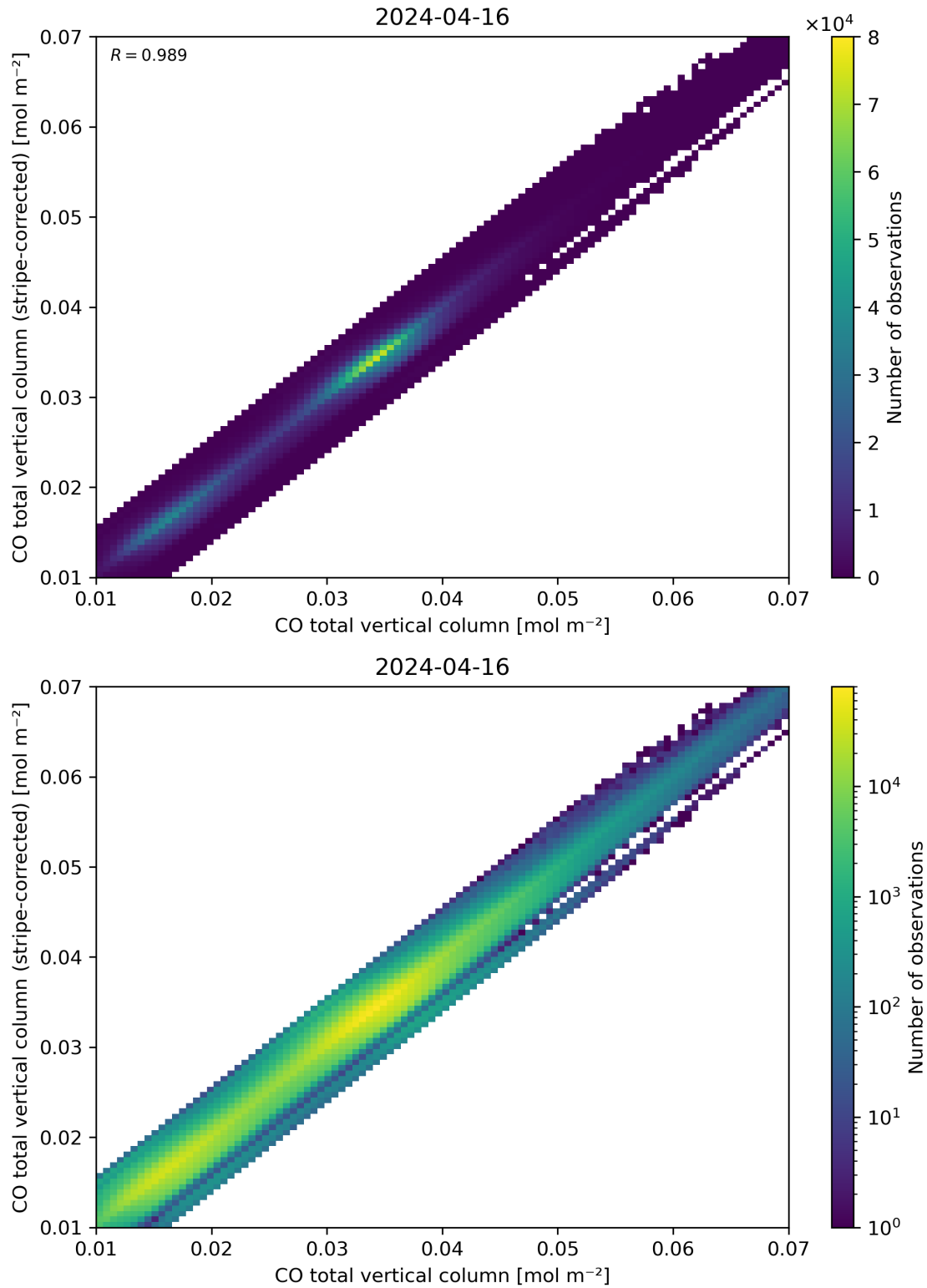
Figure 33: Scatter density plot of “CO total vertical column” against “CO total vertical column (stripe-corrected)” for 2024-04-16 to 2024-04-17.
