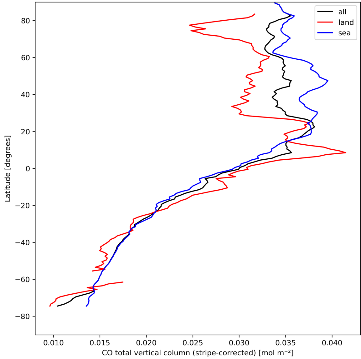
Figure 11: Zonal average of “CO total vertical column (stripe-corrected)” for 2024-04-16 to 2024-04-17.
