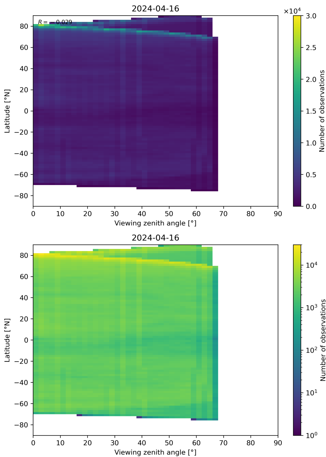
Figure 74: Scatter density plot of “Viewing zenith angle” against “Latitude” for 2024-04-16 to 2024-04-17.
