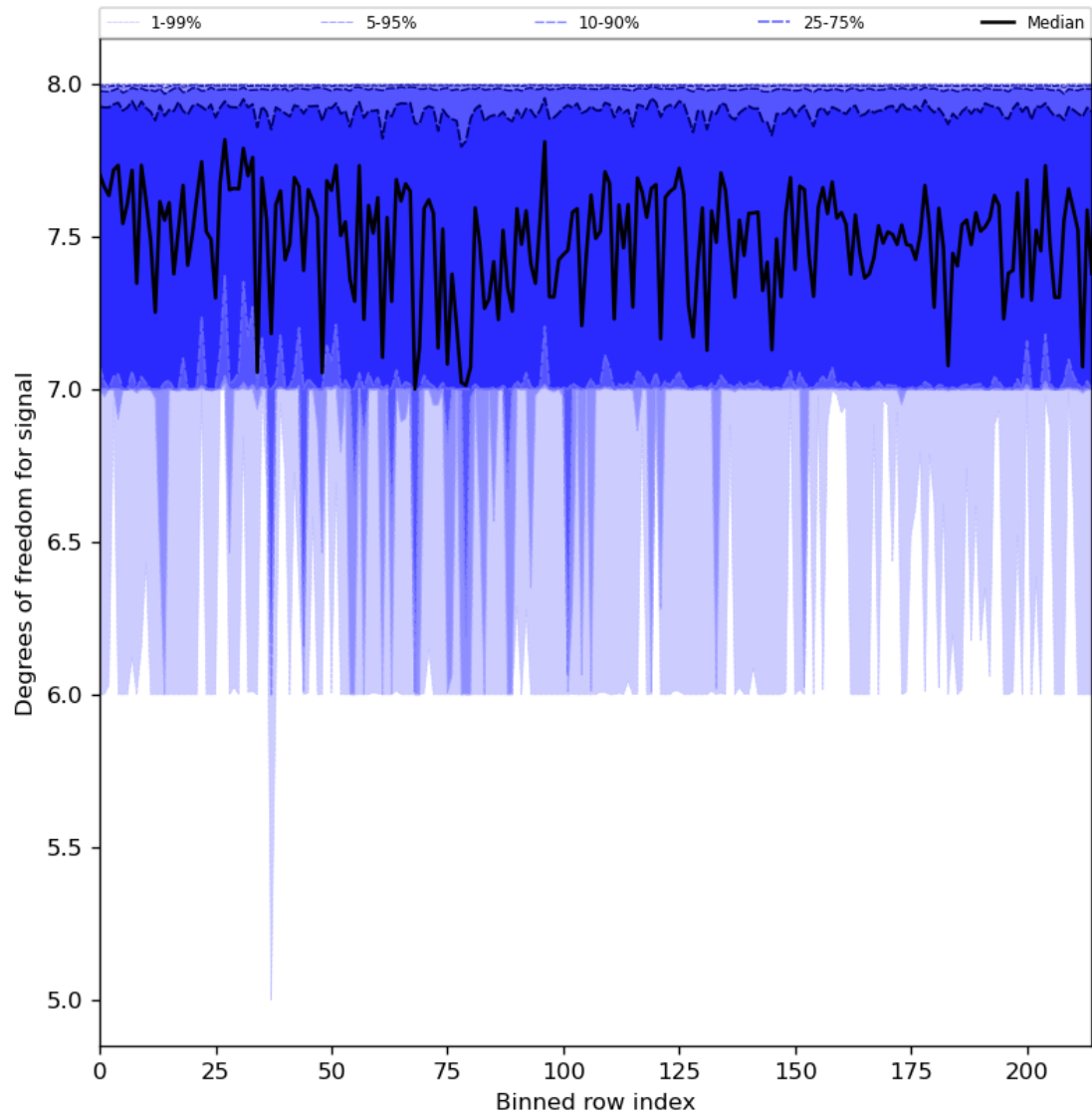
Figure 31: Along track statistics of “Degrees of freedom for signal” for 2024-04-16 to 2024-04-17
