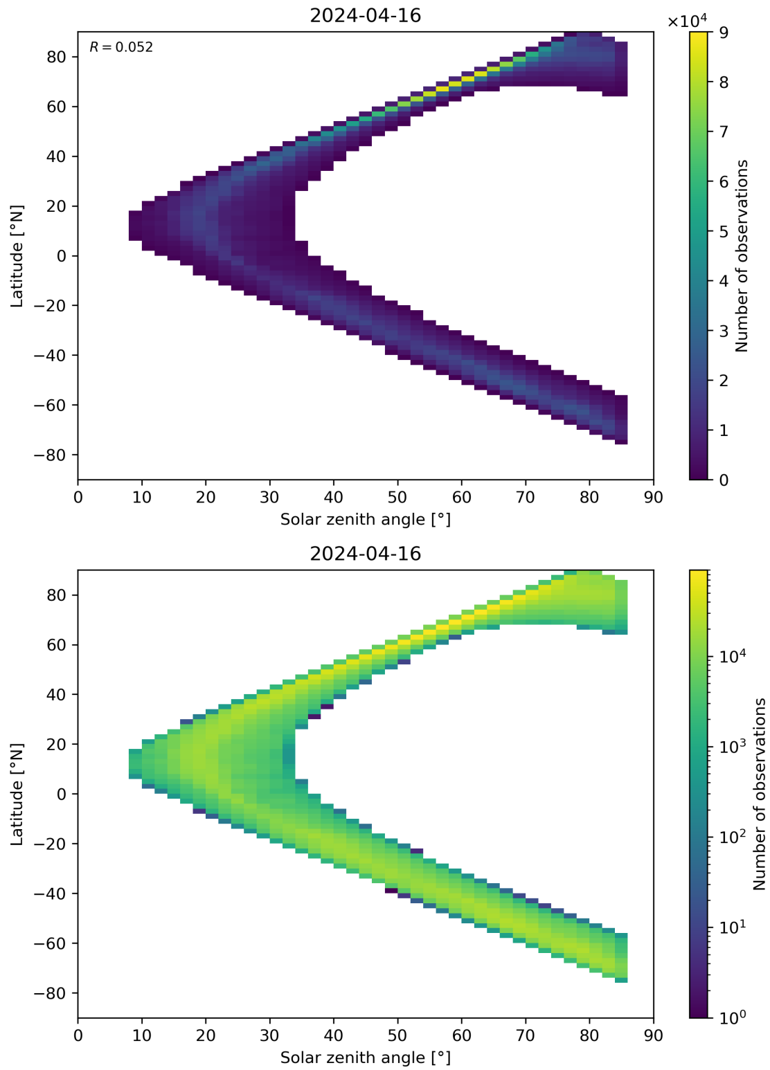
Figure 66: Scatter density plot of “Solar zenith angle” against “Latitude” for 2024-04-16 to 2024-04-17.
