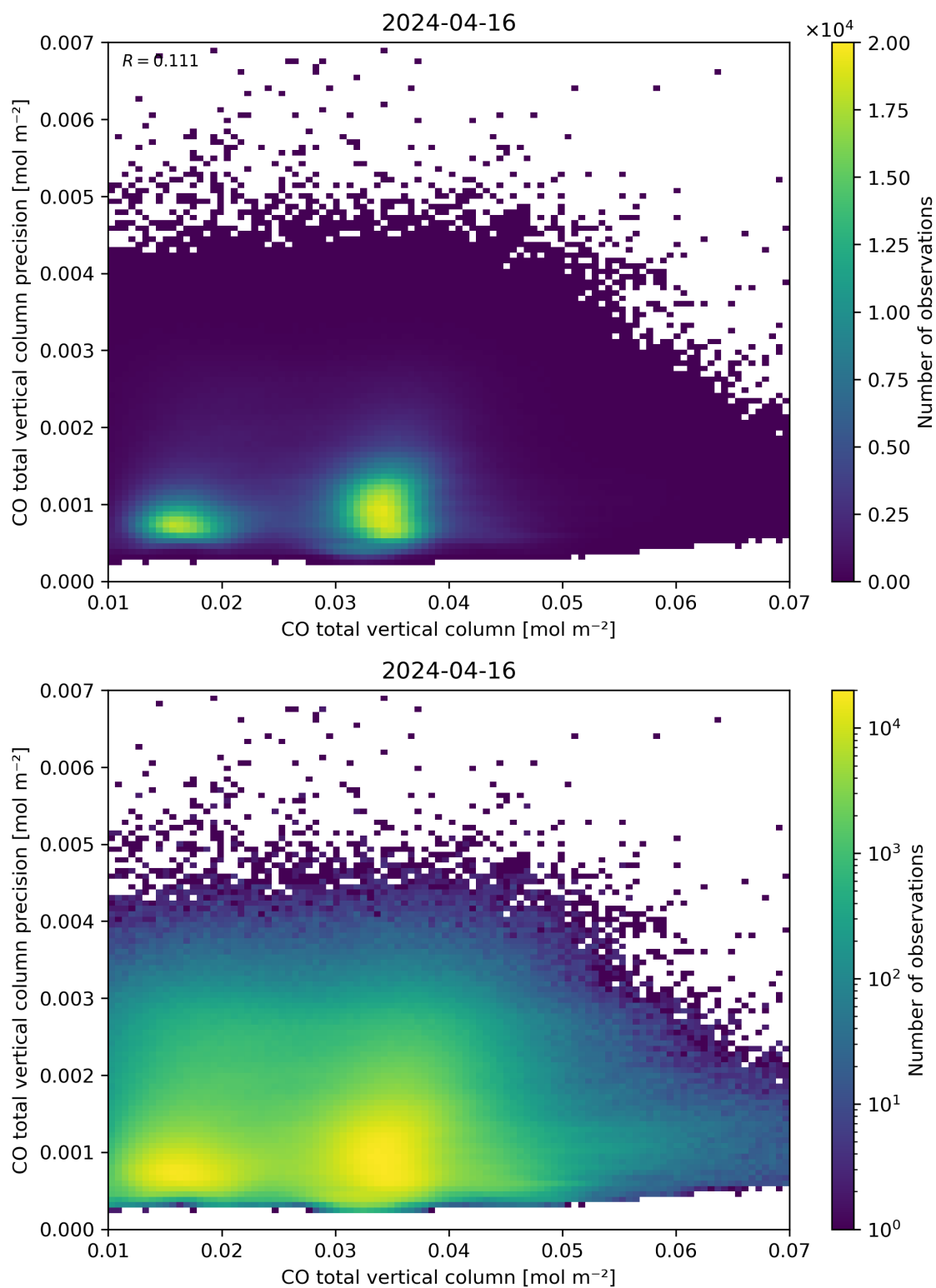
Figure 34: Scatter density plot of “CO total vertical column” against “CO total vertical column precision” for 2024-04-16 to 2024-04-17.
