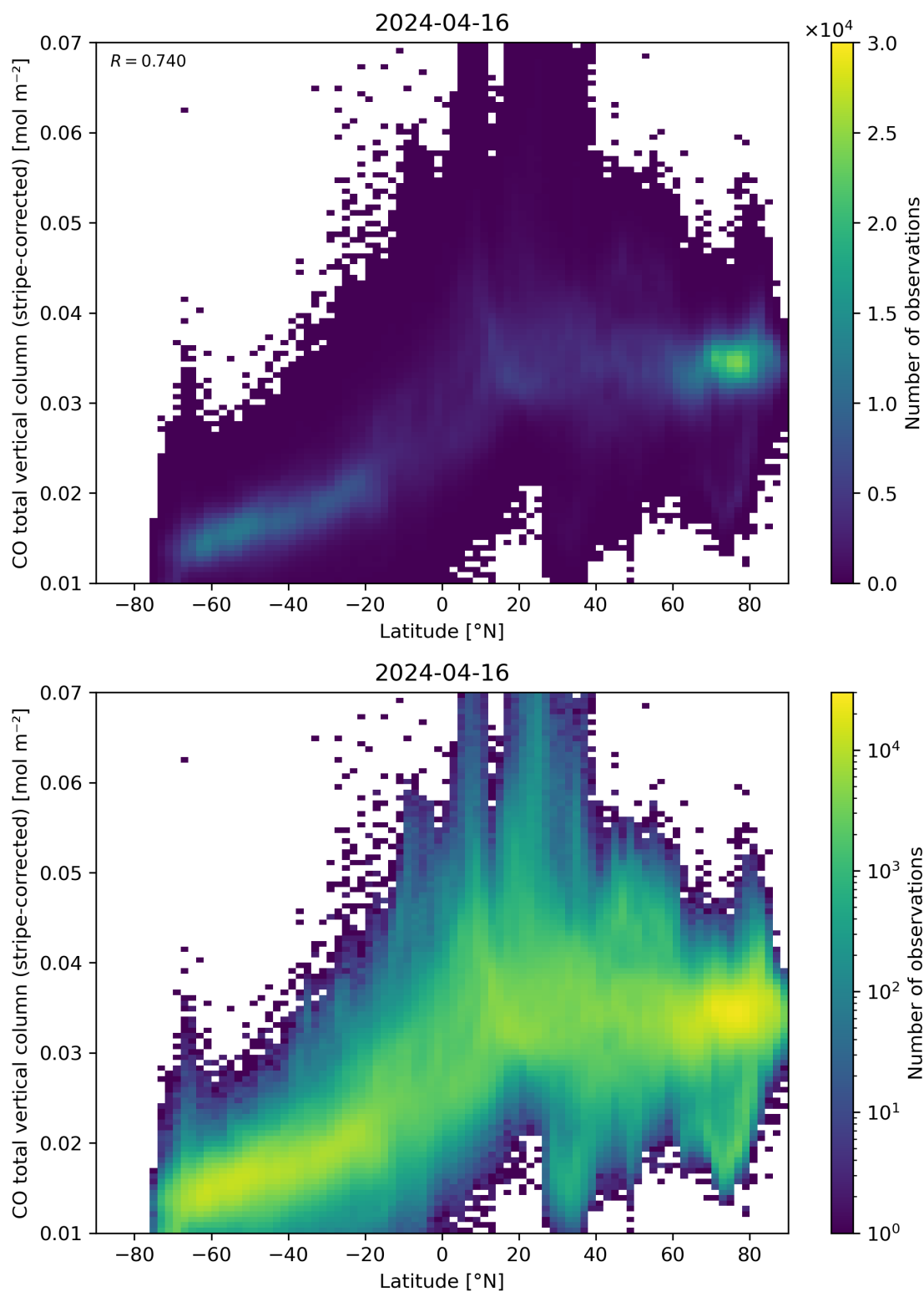
Figure 52: Scatter density plot of “Latitude” against “CO total vertical column (stripe-corrected)” for 2024-04-16 to 2024-04-17.
