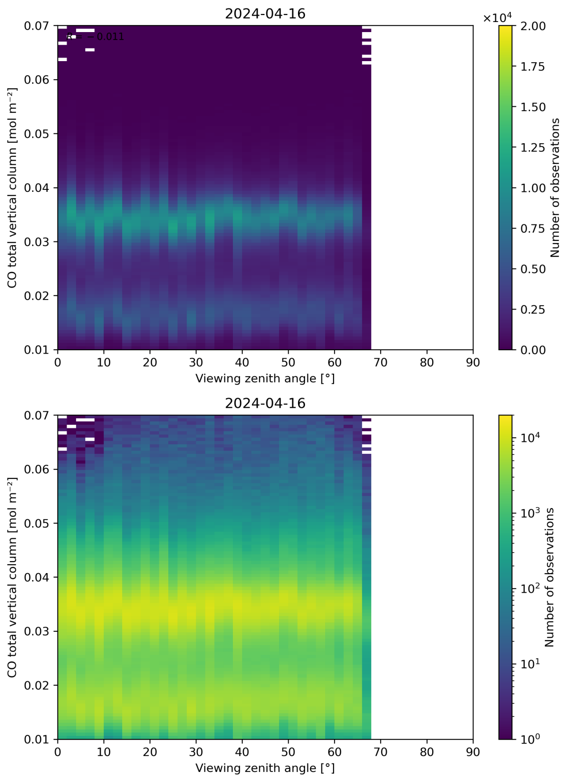
Figure 69: Scatter density plot of “Viewing zenith angle” against “CO total vertical column” for 2024-04-16 to 2024-04-17.
