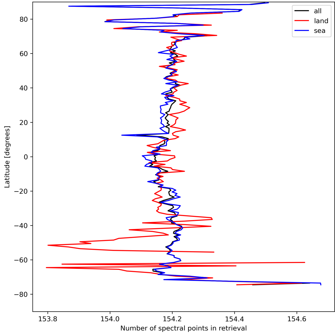
Figure 13: Zonal average of “Number of spectral points in retrieval” for 2024-04-16 to 2024-04-17.
