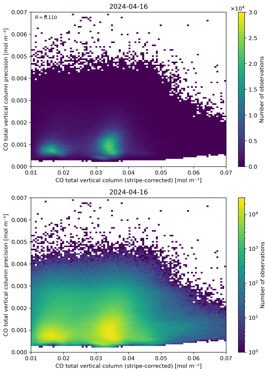
Figure 36: Scatter density plot of “CO total vertical column (stripe-corrected)” against “CO total vertical column precision” for 2024-04-16 to 2024-04-17.
