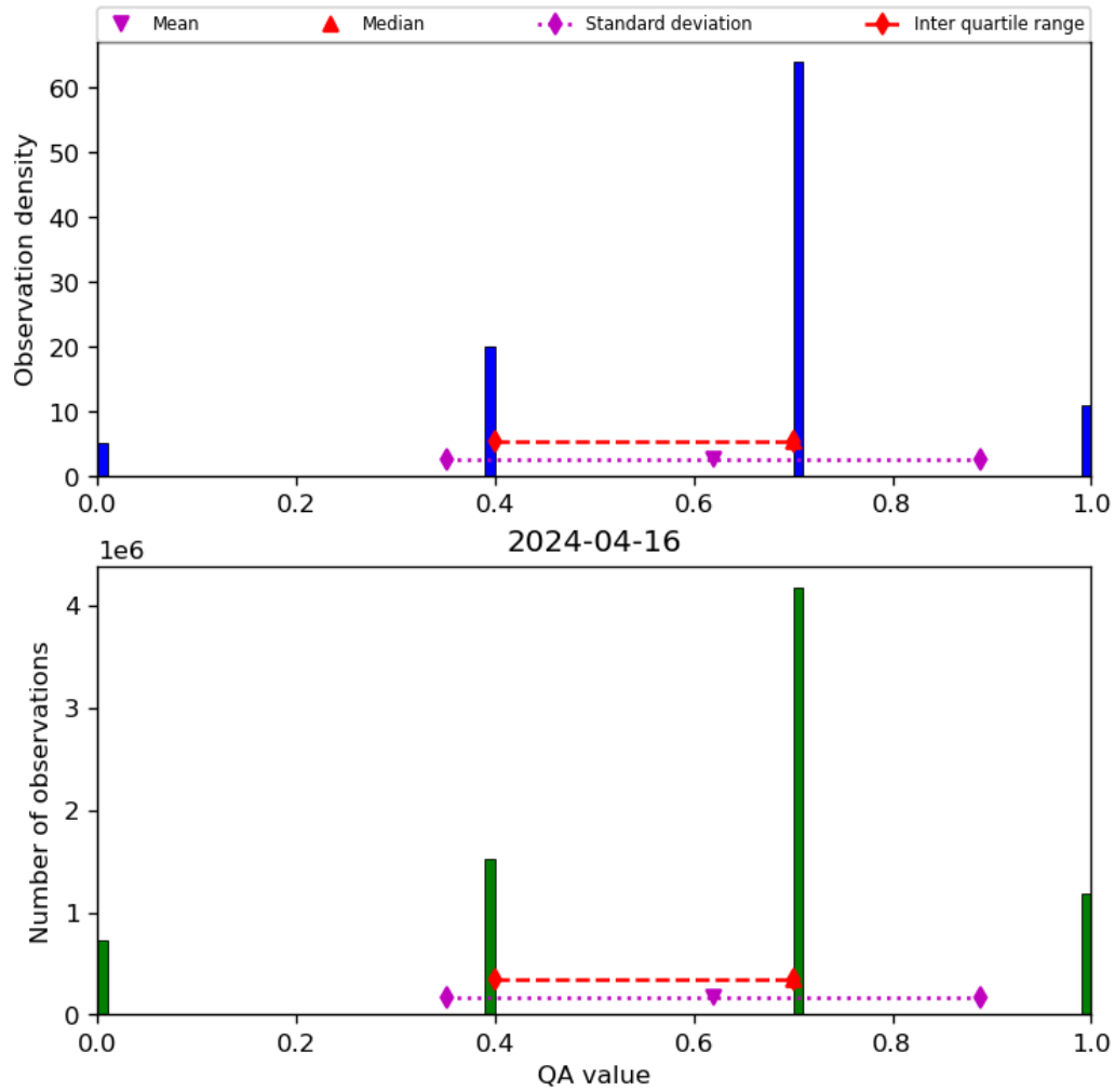
Figure 17: Histogram of “QA value” for 2024-04-16 to 2024-04-17
