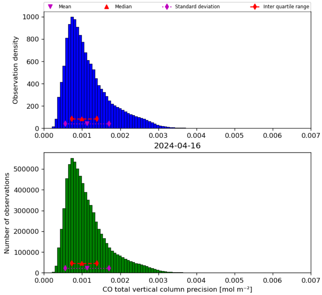
Figure 20: Histogram of “CO total vertical column precision” for 2024-04-16 to 2024-04-17
