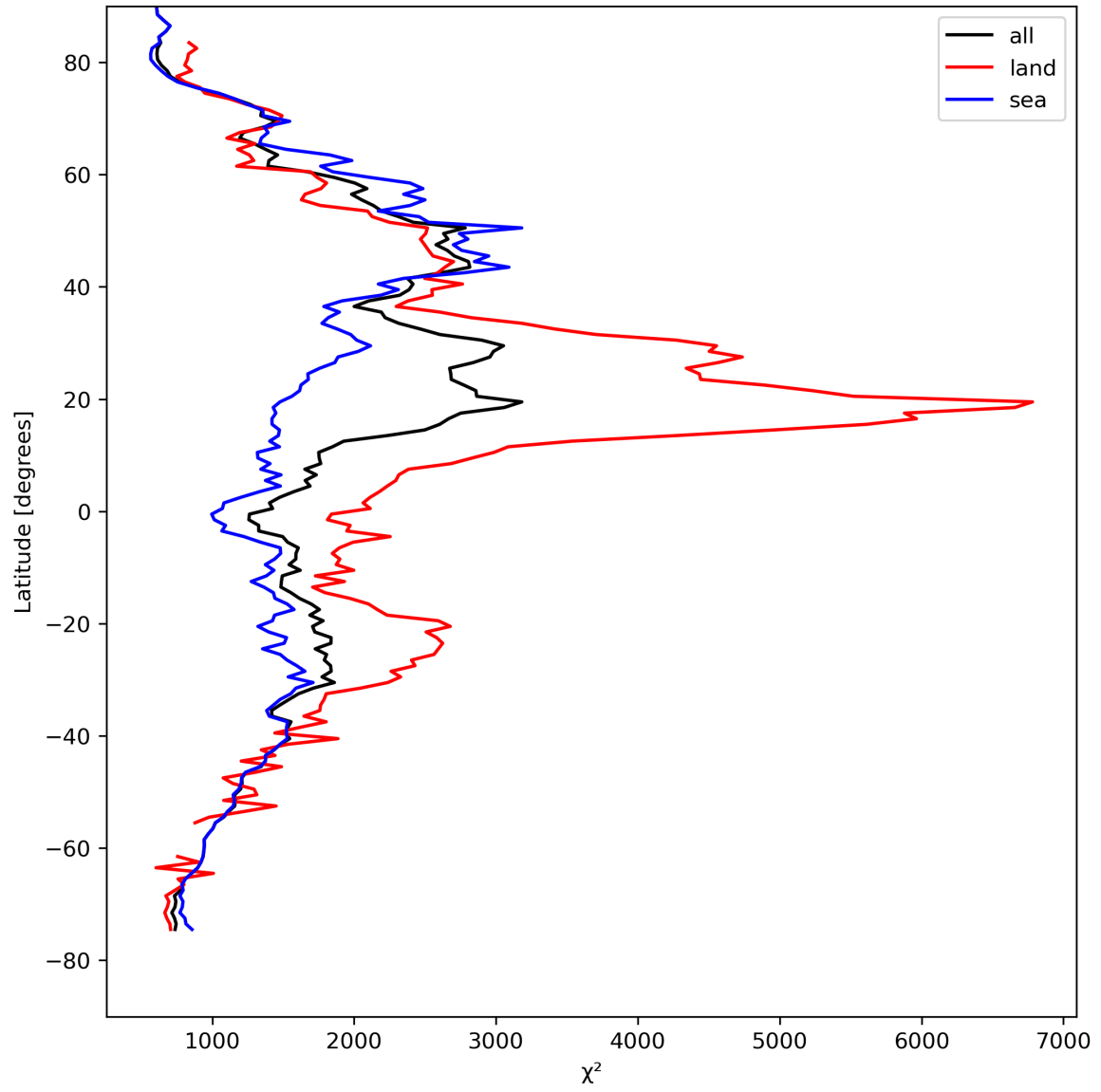
Figure 14: Zonal average of “ \chi^2 ” for 2024-04-16 to 2024-04-17.
