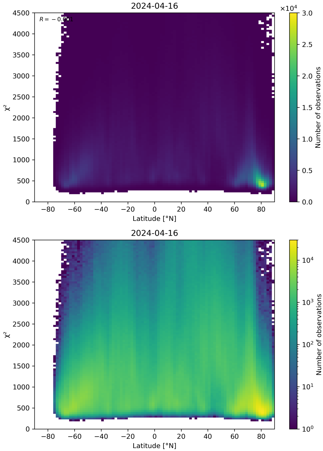
Figure 54: Scatter density plot of “Latitude” against “ \chi^2 ” for 2024-04-16 to 2024-04-17.
