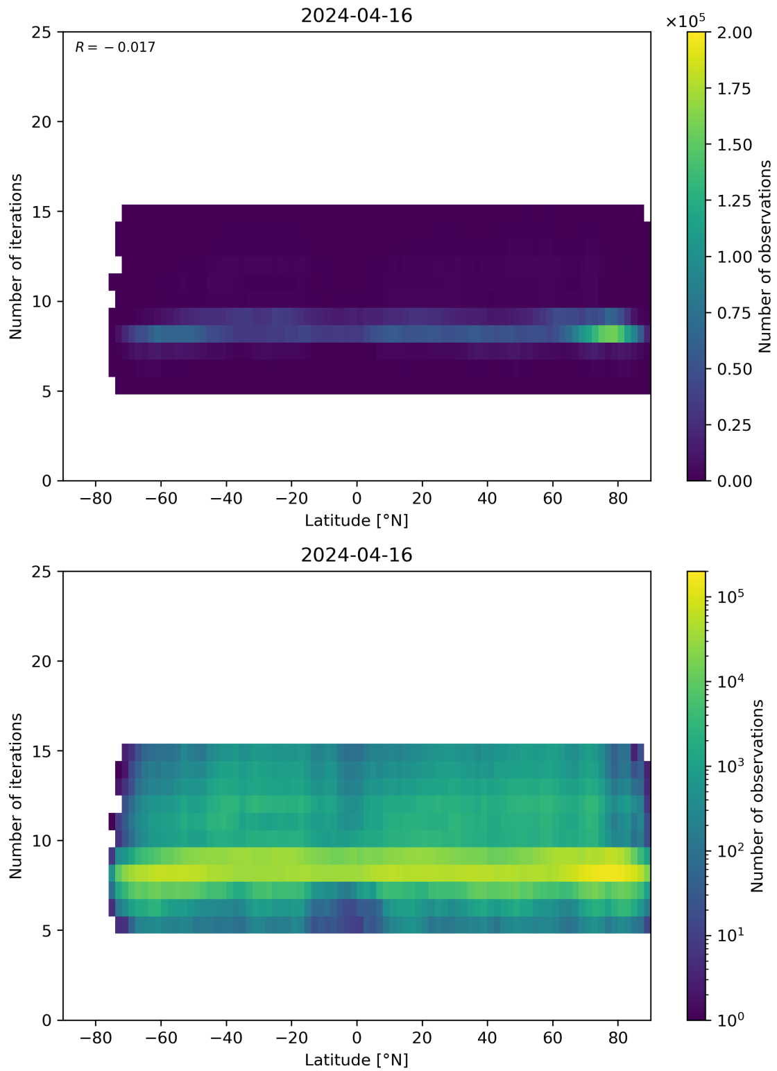
Figure 56: Scatter density plot of “Latitude” against “Number of iterations” for 2024-04-16 to 2024-04-17.
