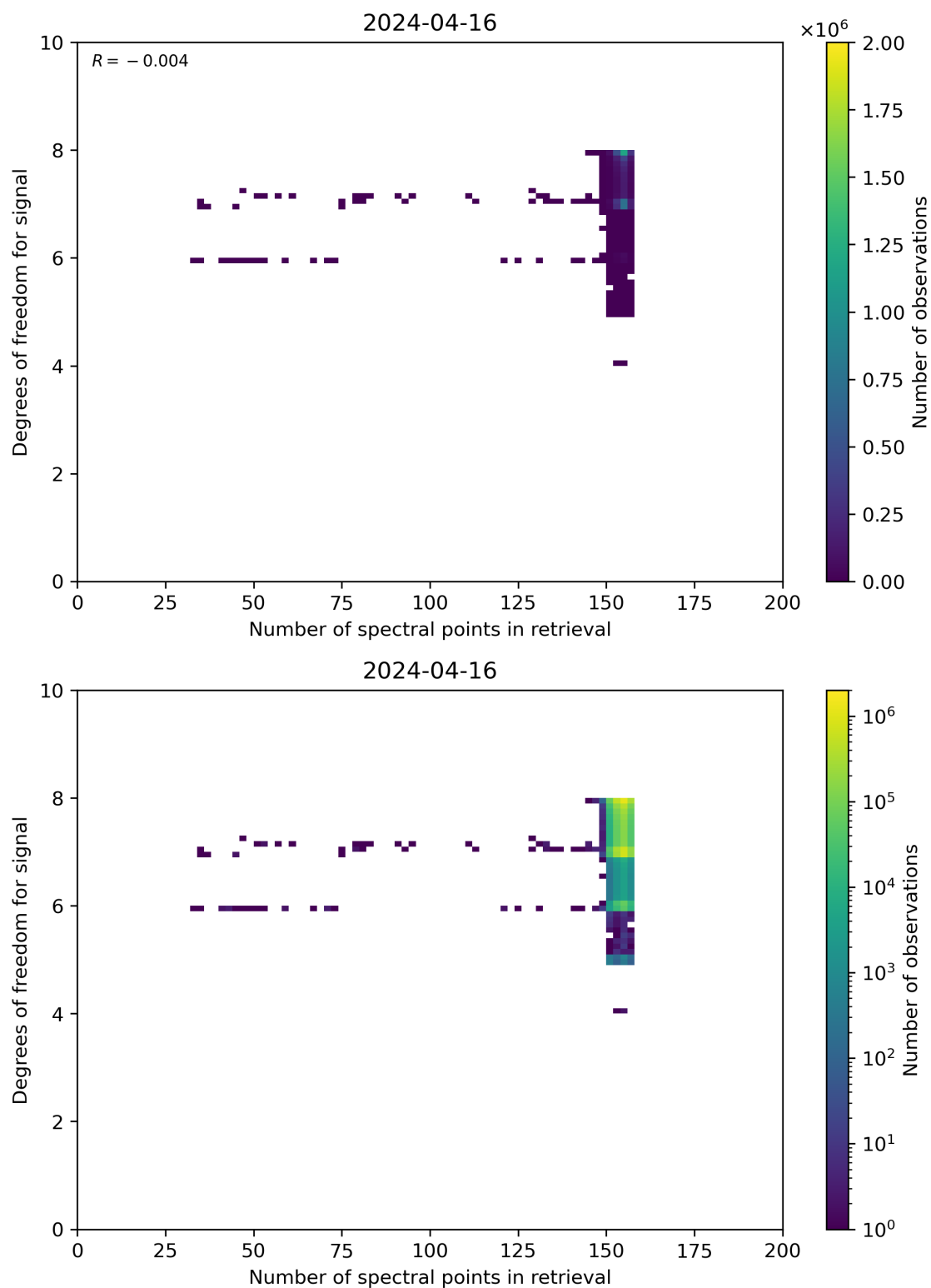
Figure 59: Scatter density plot of “Number of spectral points in retrieval” against “Degrees of freedom for signal” for 2024-04-16 to 2024-04-17.
