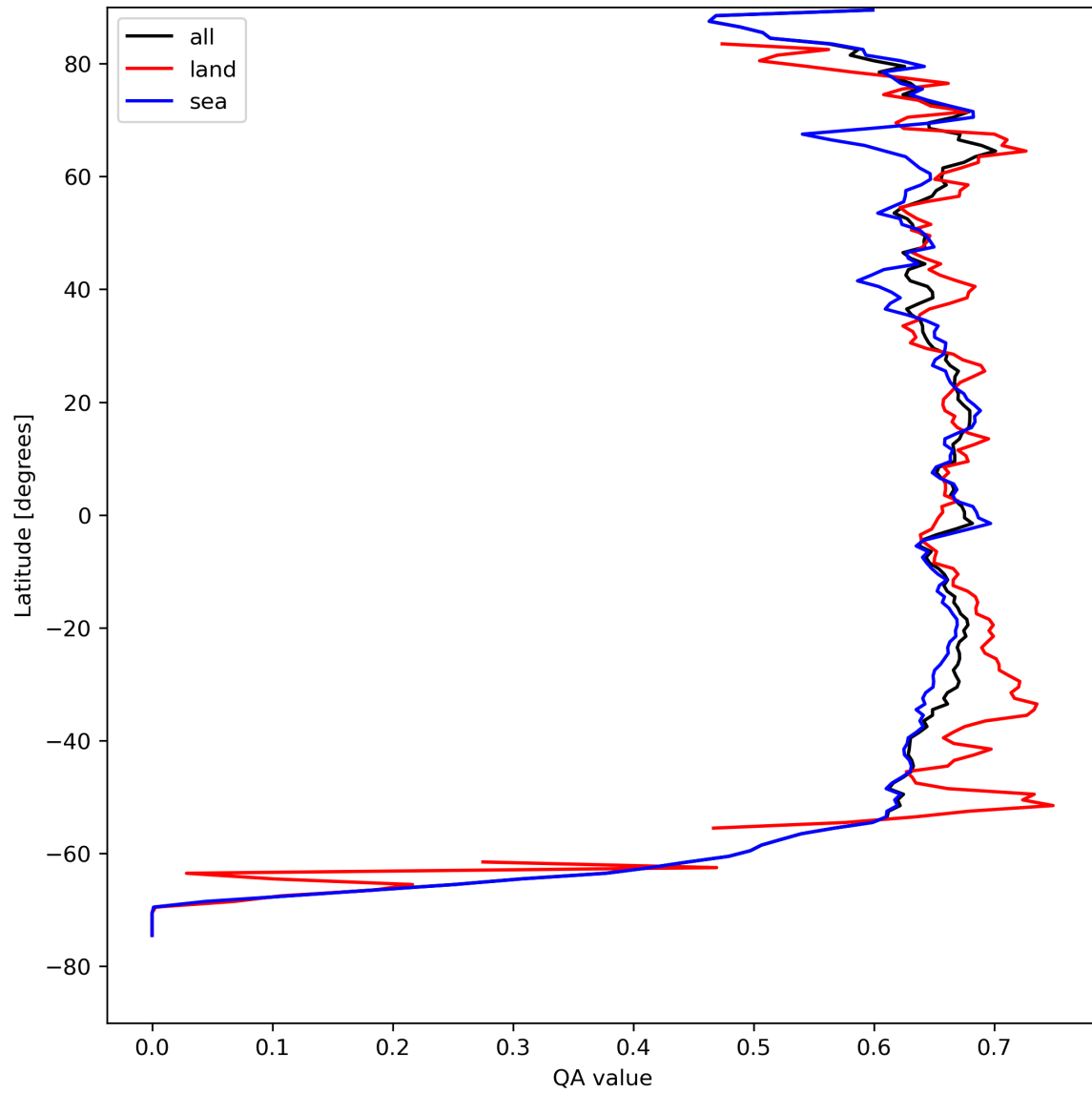
Figure 9: Zonal average of “QA value” for 2024-04-16 to 2024-04-17.
