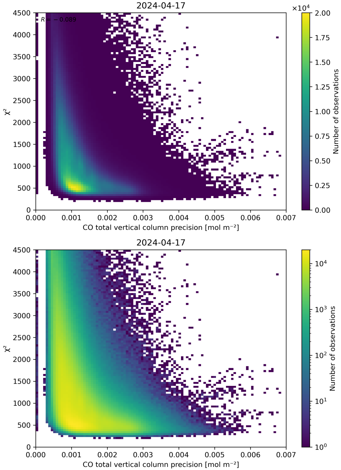
Figure 44: Scatter density plot of “CO total vertical column precision” against “ \chi^2 ” for 2024-04-16 to 2024-04-18.
