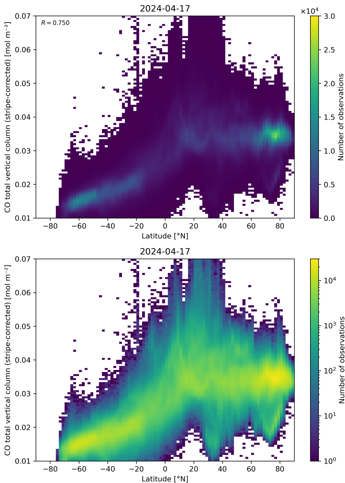
Figure 52: Scatter density plot of “Latitude” against “CO total vertical column (stripe-corrected)” for 2024-04-16 to 2024-04-18.
