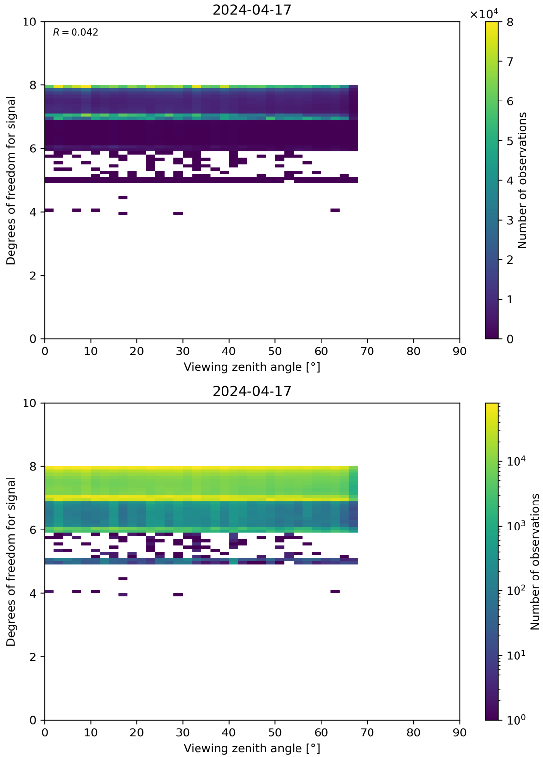
Figure 73: Scatter density plot of “Viewing zenith angle” against “Degrees of freedom for signal” for 2024-04-16 to 2024-04-18.
