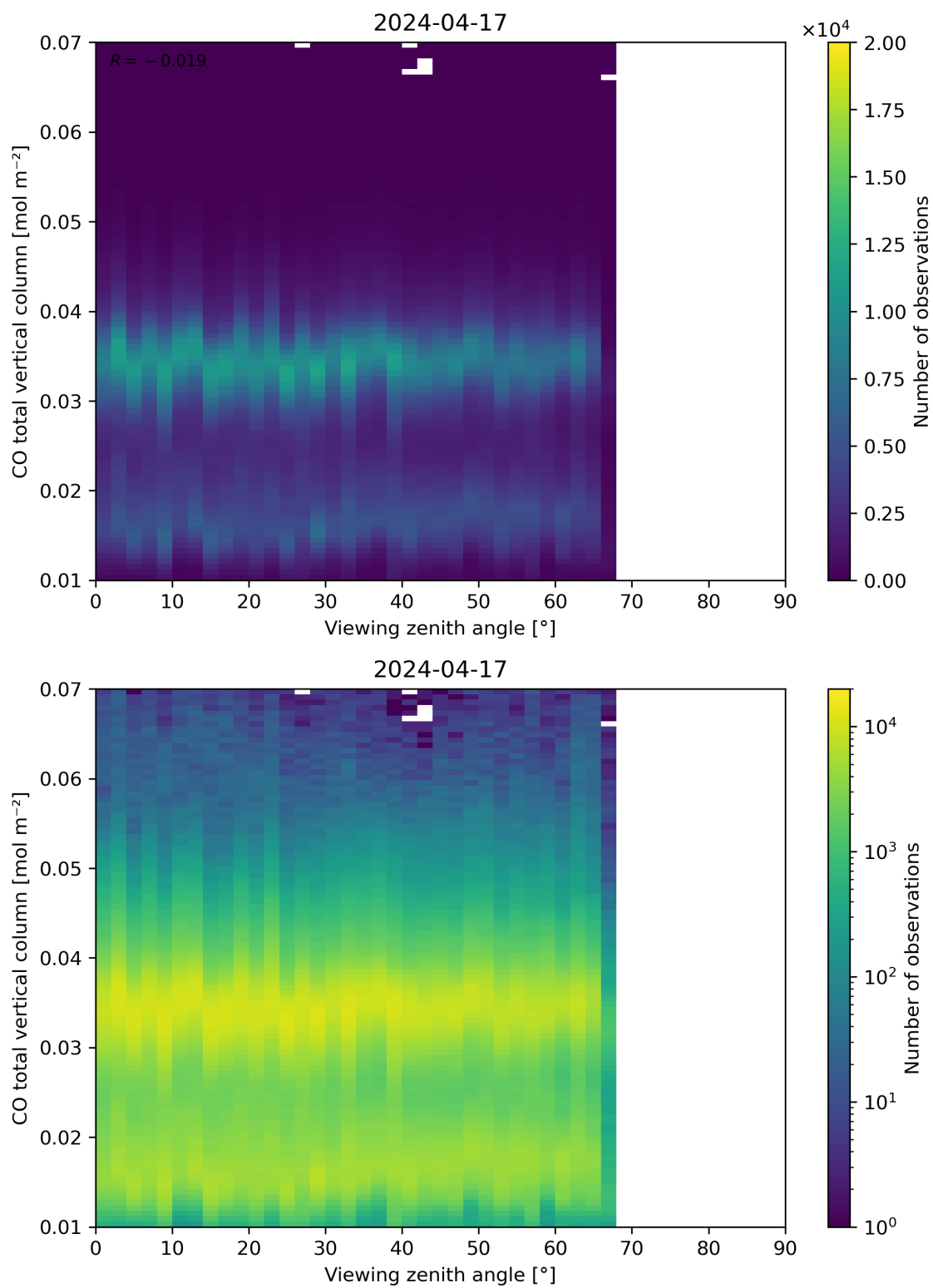
Figure 69: Scatter density plot of “Viewing zenith angle” against “CO total vertical column” for 2024-04-16 to 2024-04-18.
