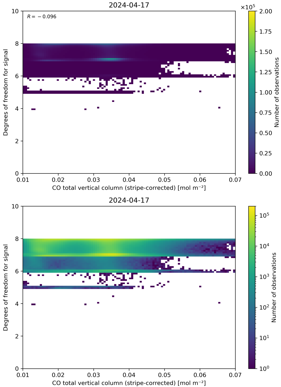
Figure 38: Scatter density plot of “CO total vertical column (stripe-corrected)” against “Degrees of freedom for signal” for 2024-04-16 to 2024-04-18.
