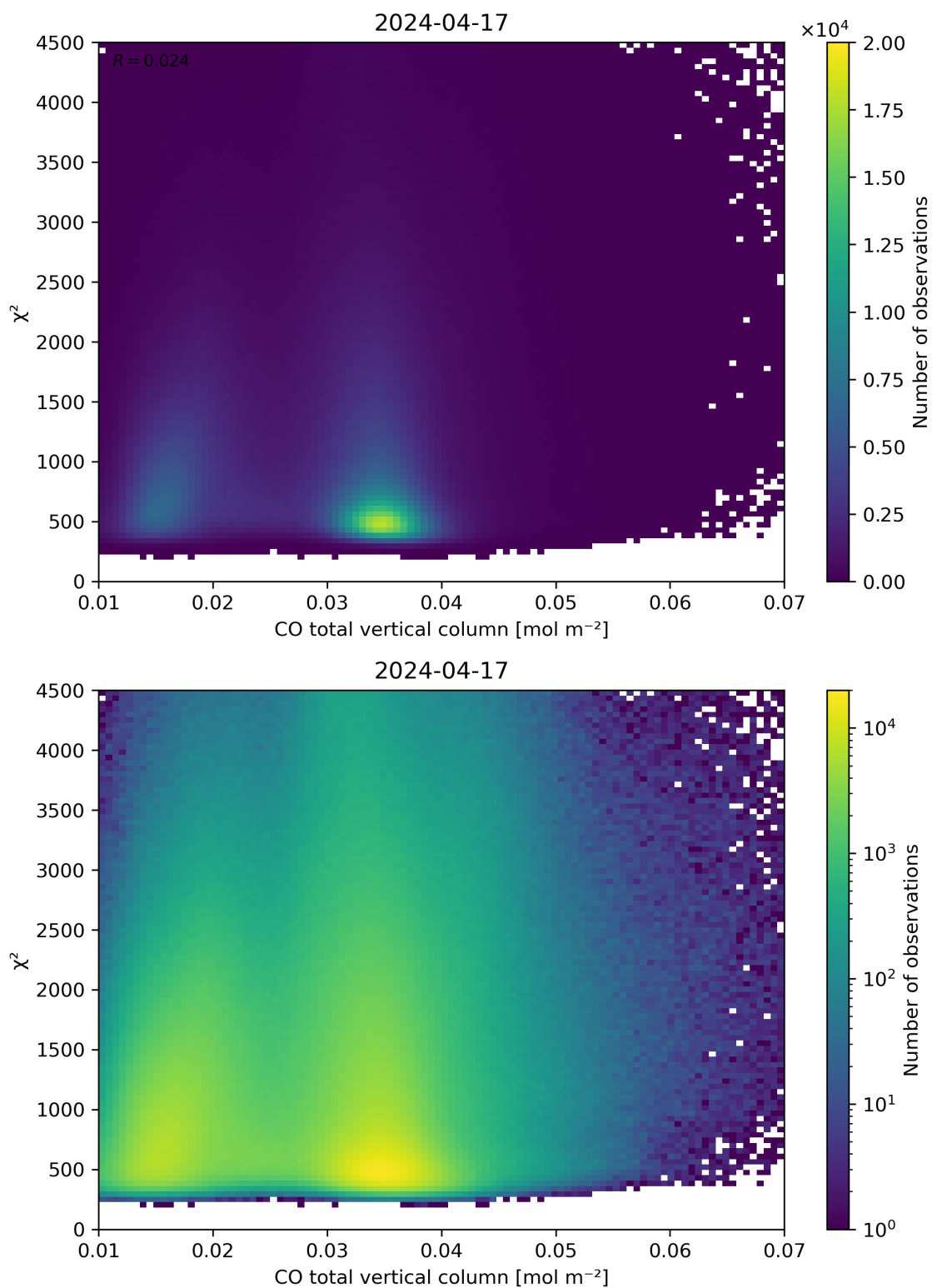
Figure 35: Scatter density plot of “CO total vertical column” against “ \chi^2 ” for 2024-04-16 to 2024-04-18.
