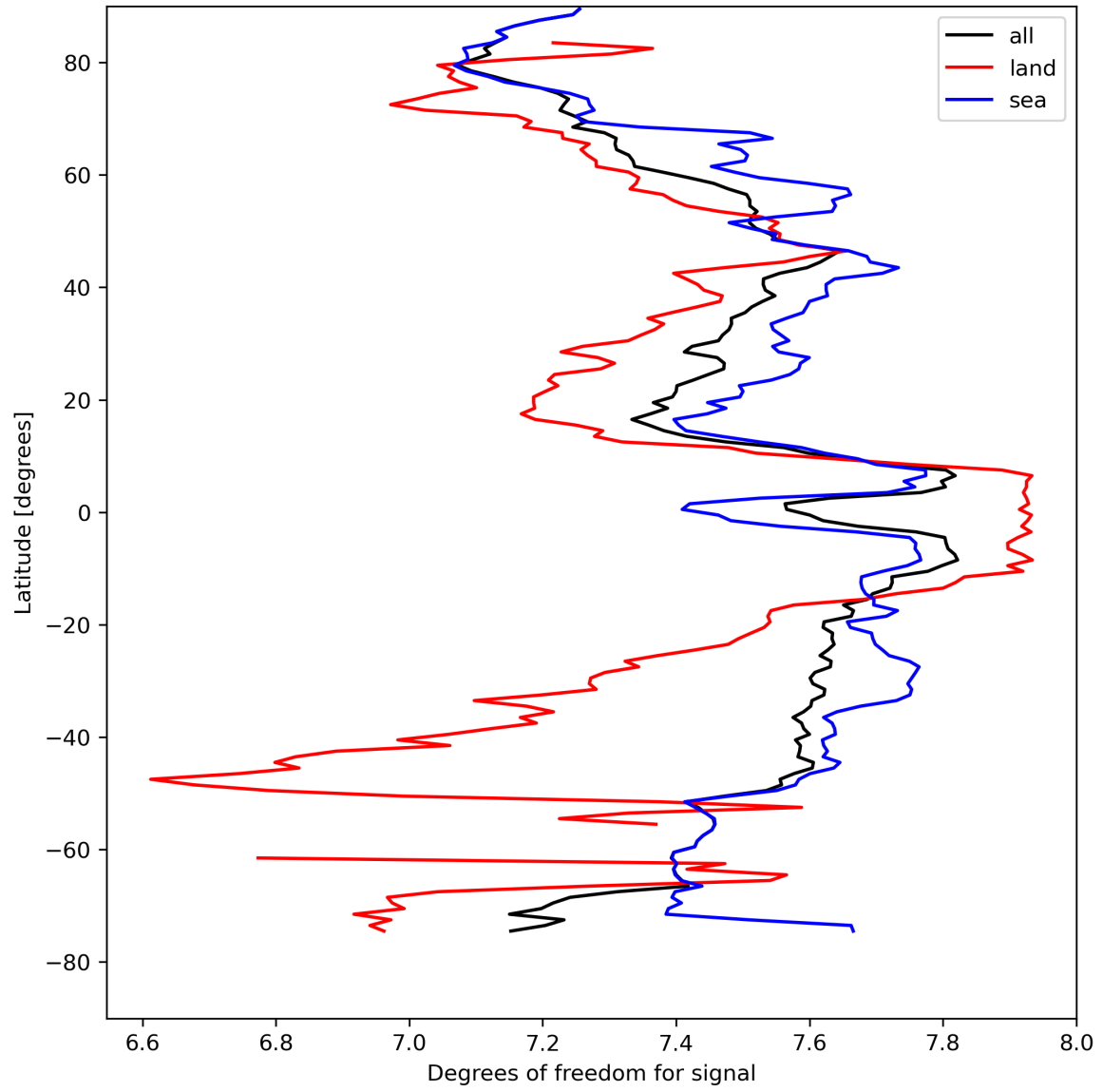
Figure 15: Zonal average of “Degrees of freedom for signal” for 2024-04-16 to 2024-04-18.
