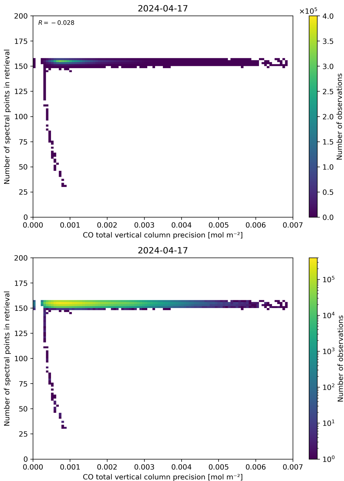
Figure 47: Scatter density plot of “CO total vertical column precision” against “Number of spectral points in retrieval” for 2024-04-16 to 2024-04-18.
