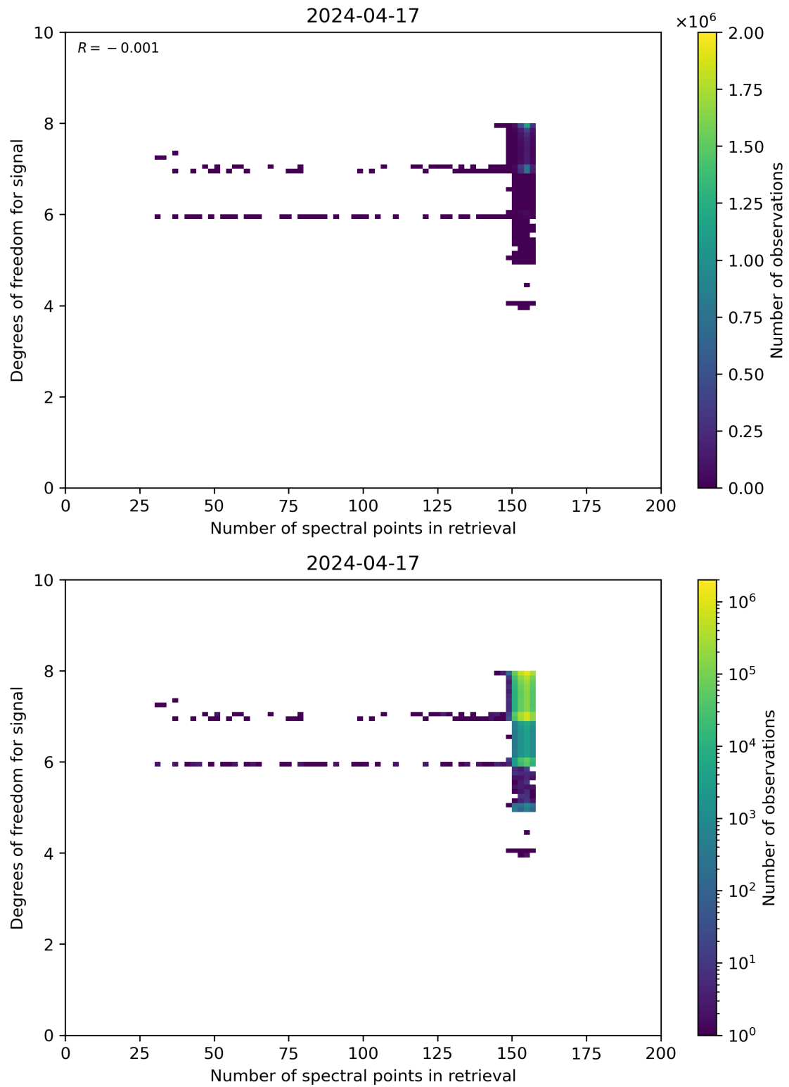
Figure 59: Scatter density plot of “Number of spectral points in retrieval” against “Degrees of freedom for signal” for 2024-04-16 to 2024-04-18.
