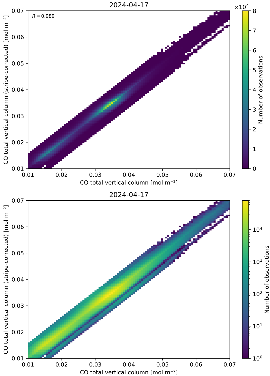
Figure 33: Scatter density plot of “CO total vertical column” against “CO total vertical column (stripe-corrected)” for 2024-04-16 to 2024-04-18.
