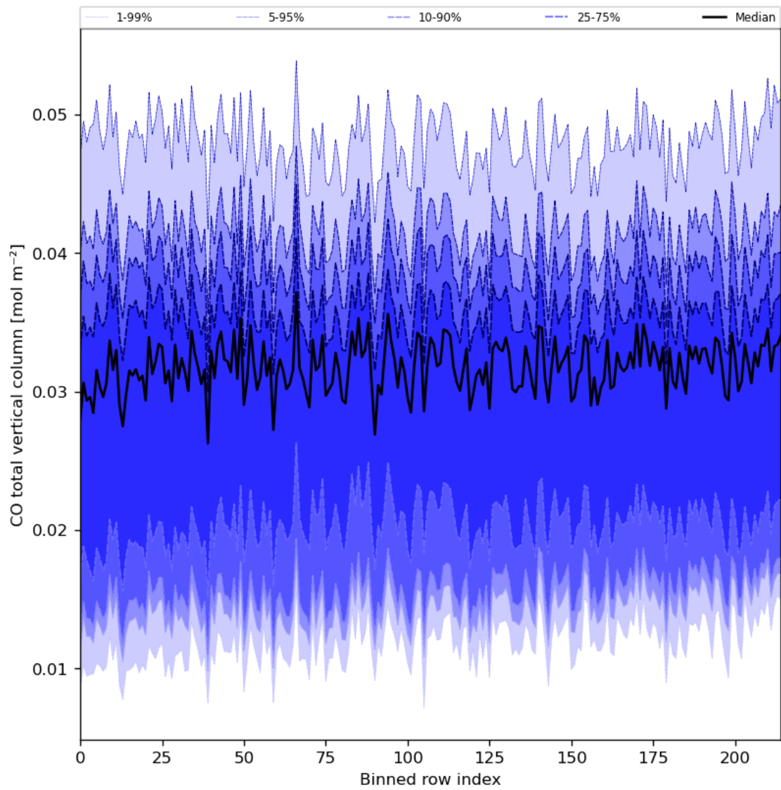
Figure 26: Along track statistics of “CO total vertical column” for 2024-04-16 to 2024-04-18
