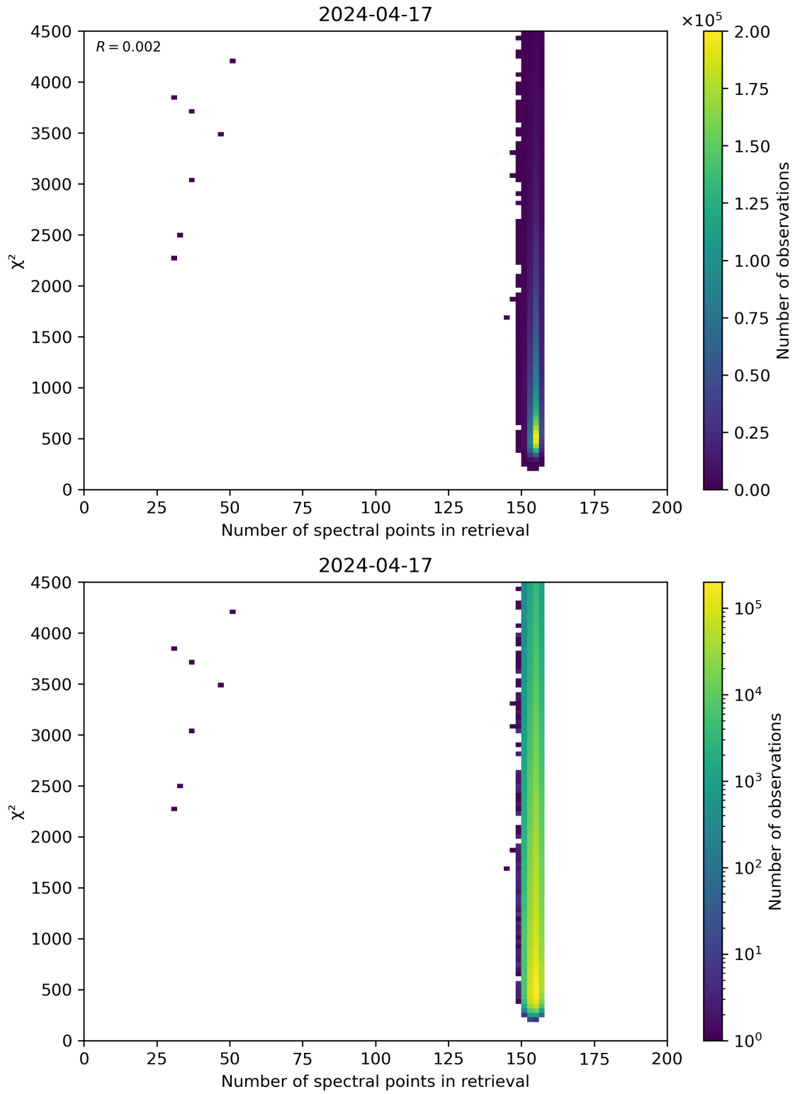
Figure 58: Scatter density plot of “Number of spectral points in retrieval” against “ \chi^2 ” for 2024-04-16 to 2024-04-18.
