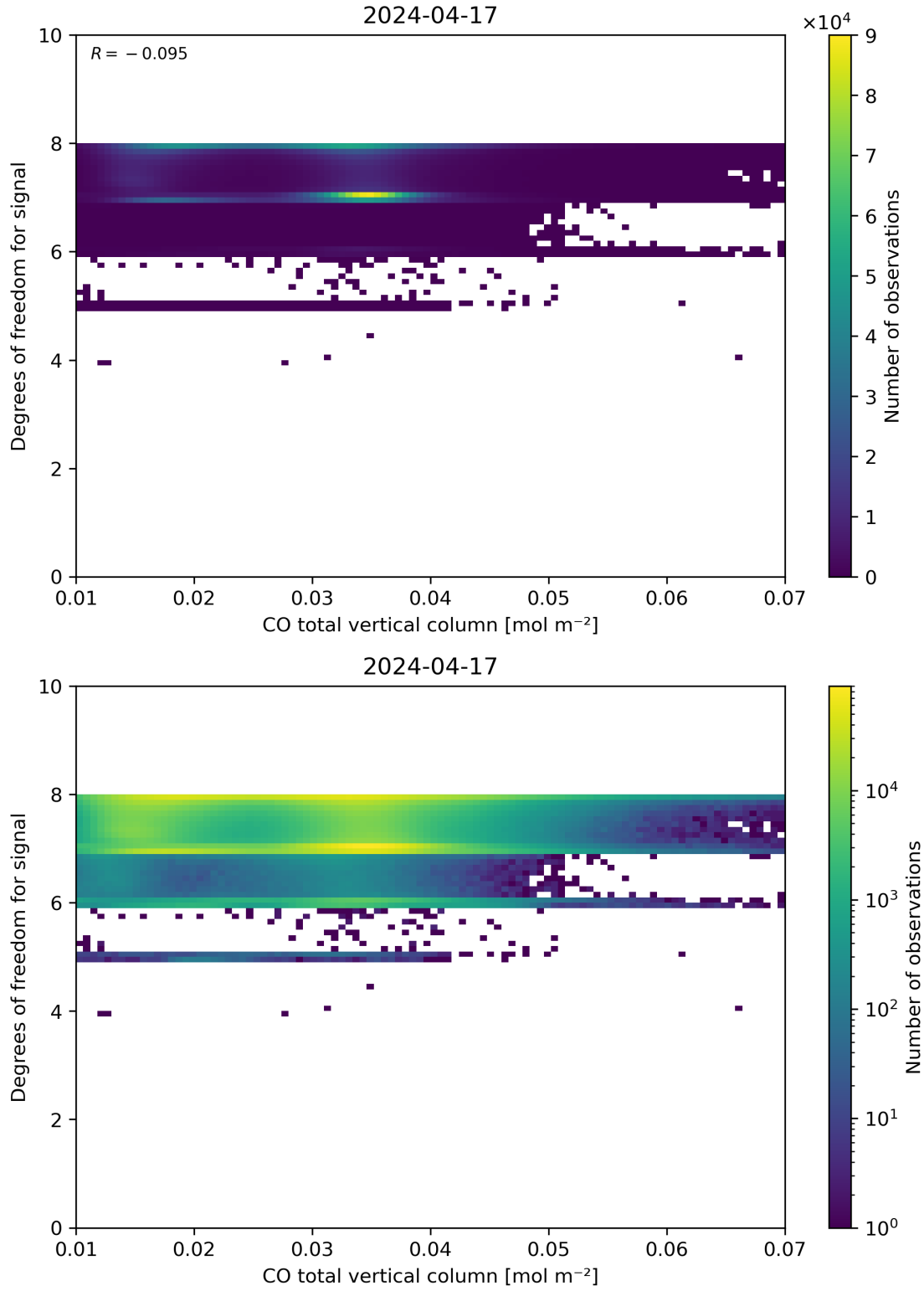
Figure 41: Scatter density plot of “CO total vertical column” against “Degrees of freedom for signal” for 2024-04-16 to 2024-04-18.
