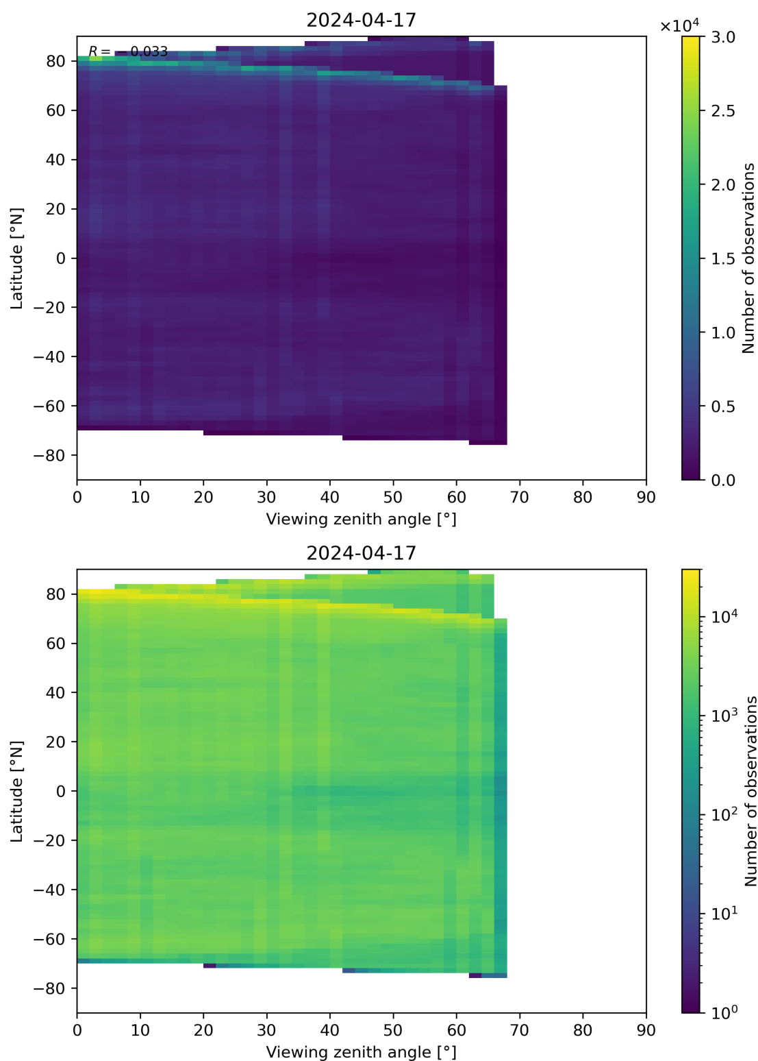
Figure 74: Scatter density plot of “Viewing zenith angle” against “Latitude” for 2024-04-16 to 2024-04-18.
