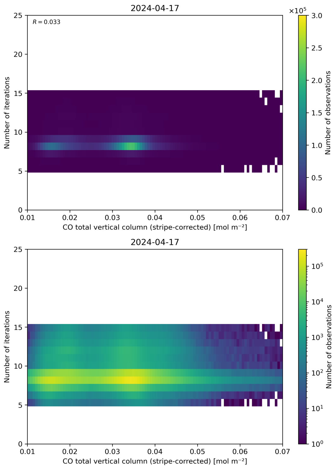
Figure 39: Scatter density plot of “CO total vertical column (stripe-corrected)” against “Number of iterations” for 2024-04-16 to 2024-04-18.
