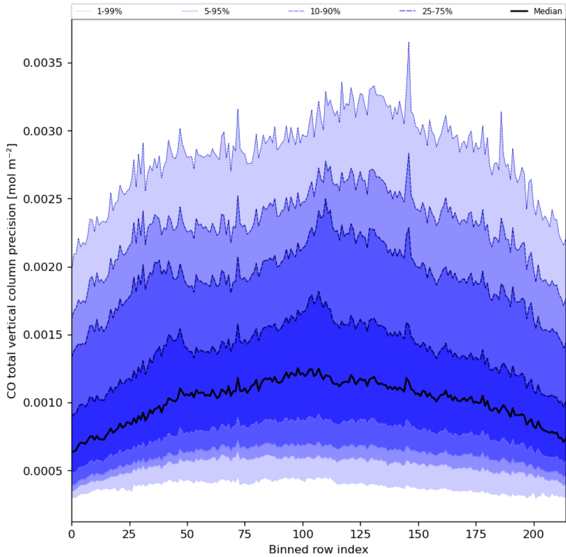
Figure 28: Along track statistics of “CO total vertical column precision” for 2024-04-16 to 2024-04-18
