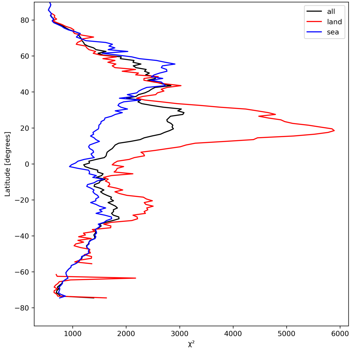
Figure 14: Zonal average of “ \chi^2 ” for 2024-04-16 to 2024-04-18.
