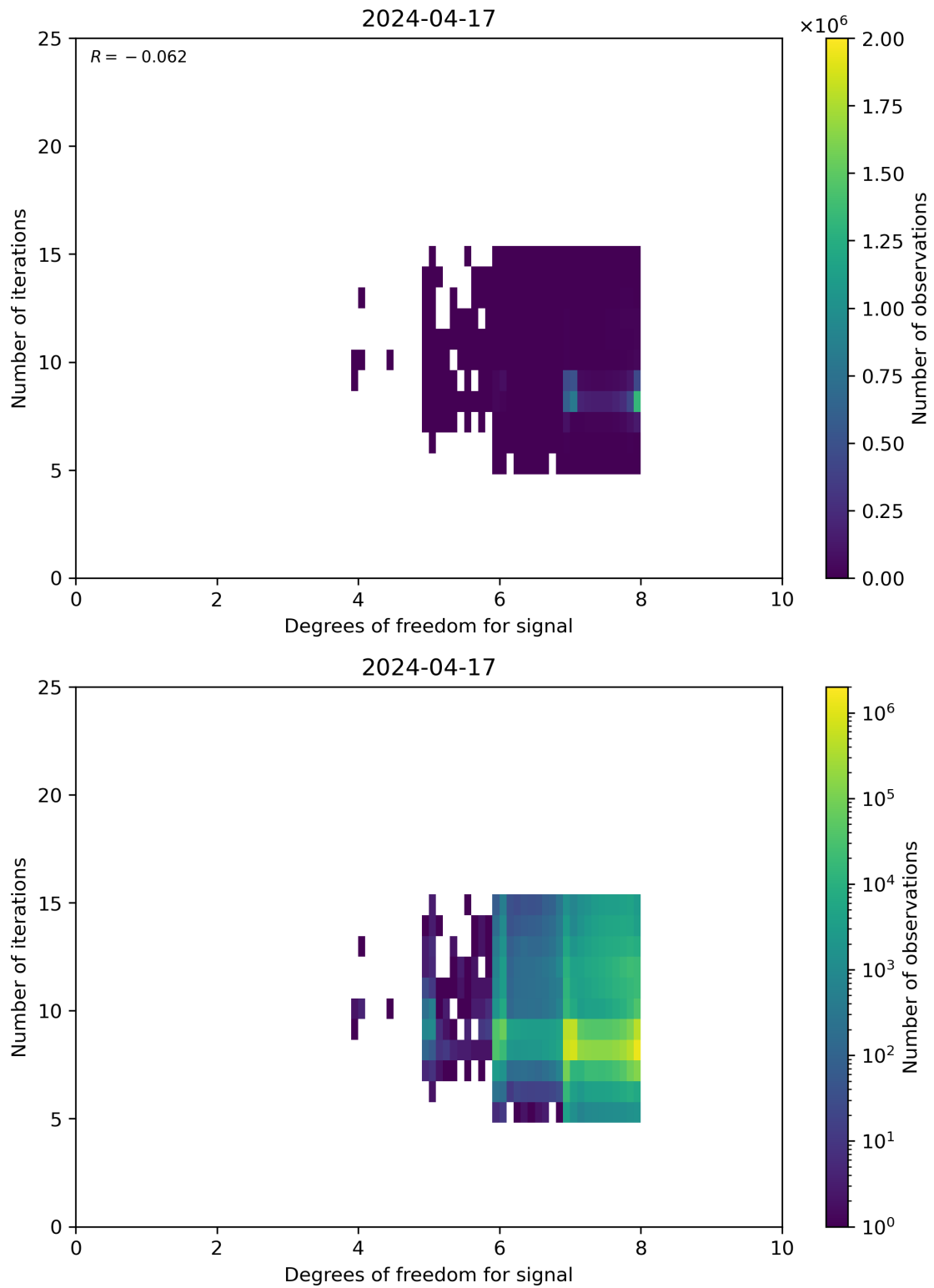
Figure 50: Scatter density plot of “Degrees of freedom for signal” against “Number of iterations” for 2024-04-16 to 2024-04-18.
