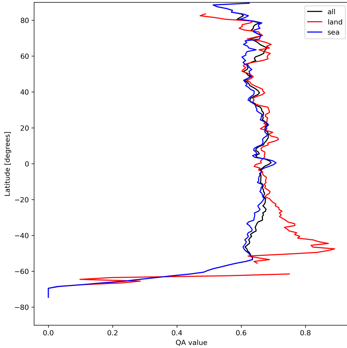
Figure 9: Zonal average of “QA value” for 2024-04-16 to 2024-04-18.
