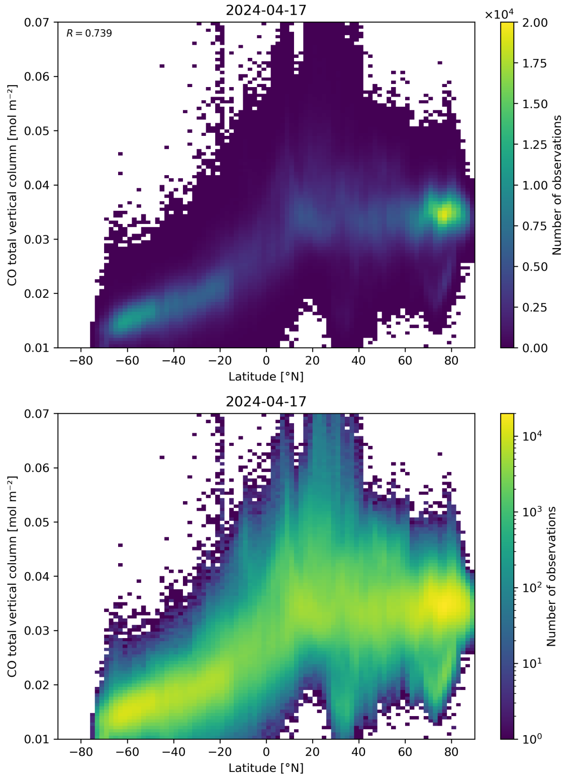
Figure 51: Scatter density plot of “Latitude” against “CO total vertical column” for 2024-04-16 to 2024-04-18.
