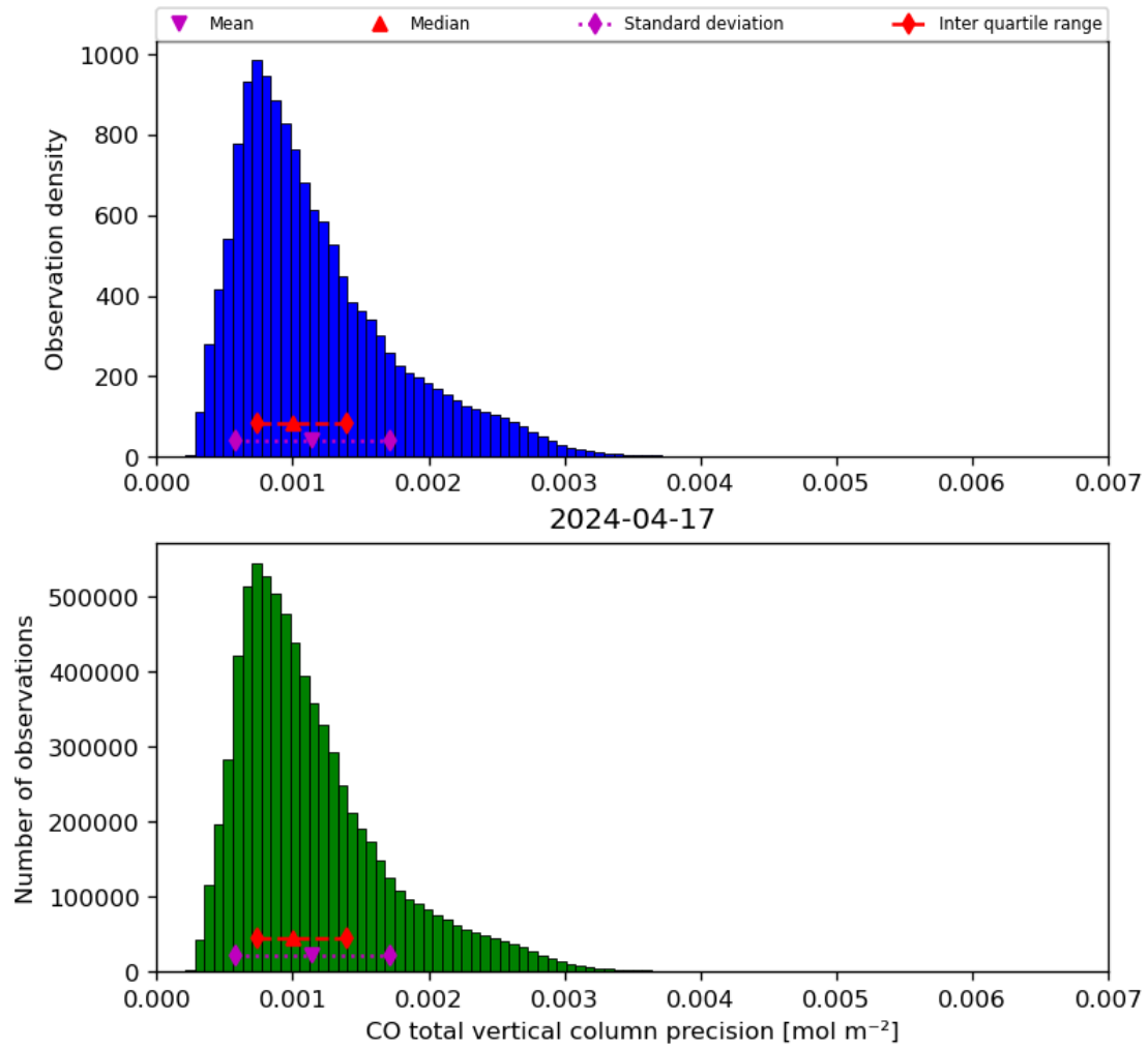
Figure 20: Histogram of “CO total vertical column precision” for 2024-04-16 to 2024-04-18
