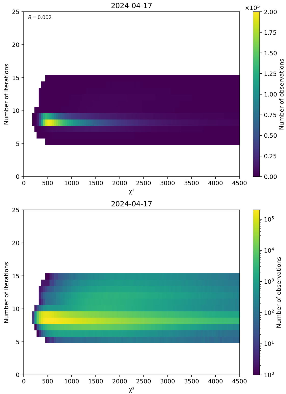
Figure 49: Scatter density plot of “ \chi^2 ” against “Number of iterations” for 2024-04-16 to 2024-04-18.
