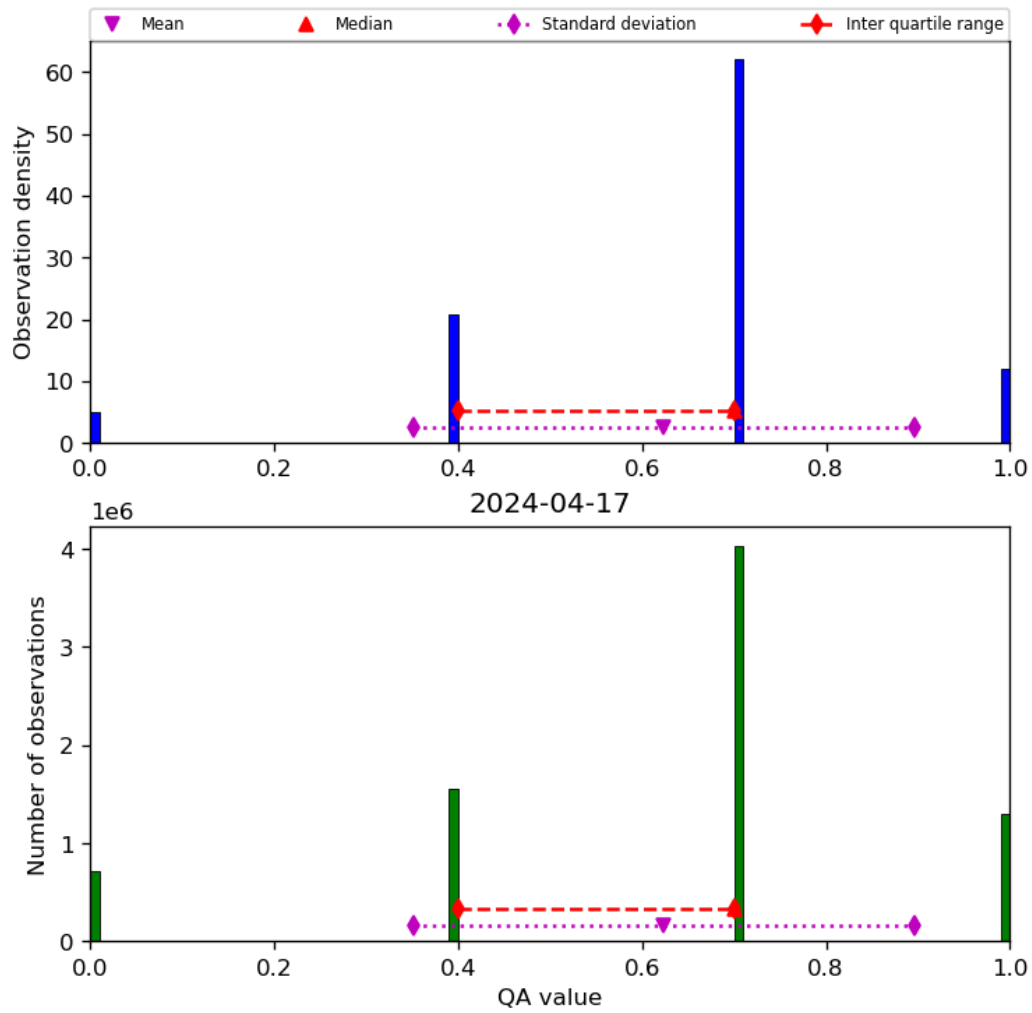
Figure 17: Histogram of “QA value” for 2024-04-16 to 2024-04-18
