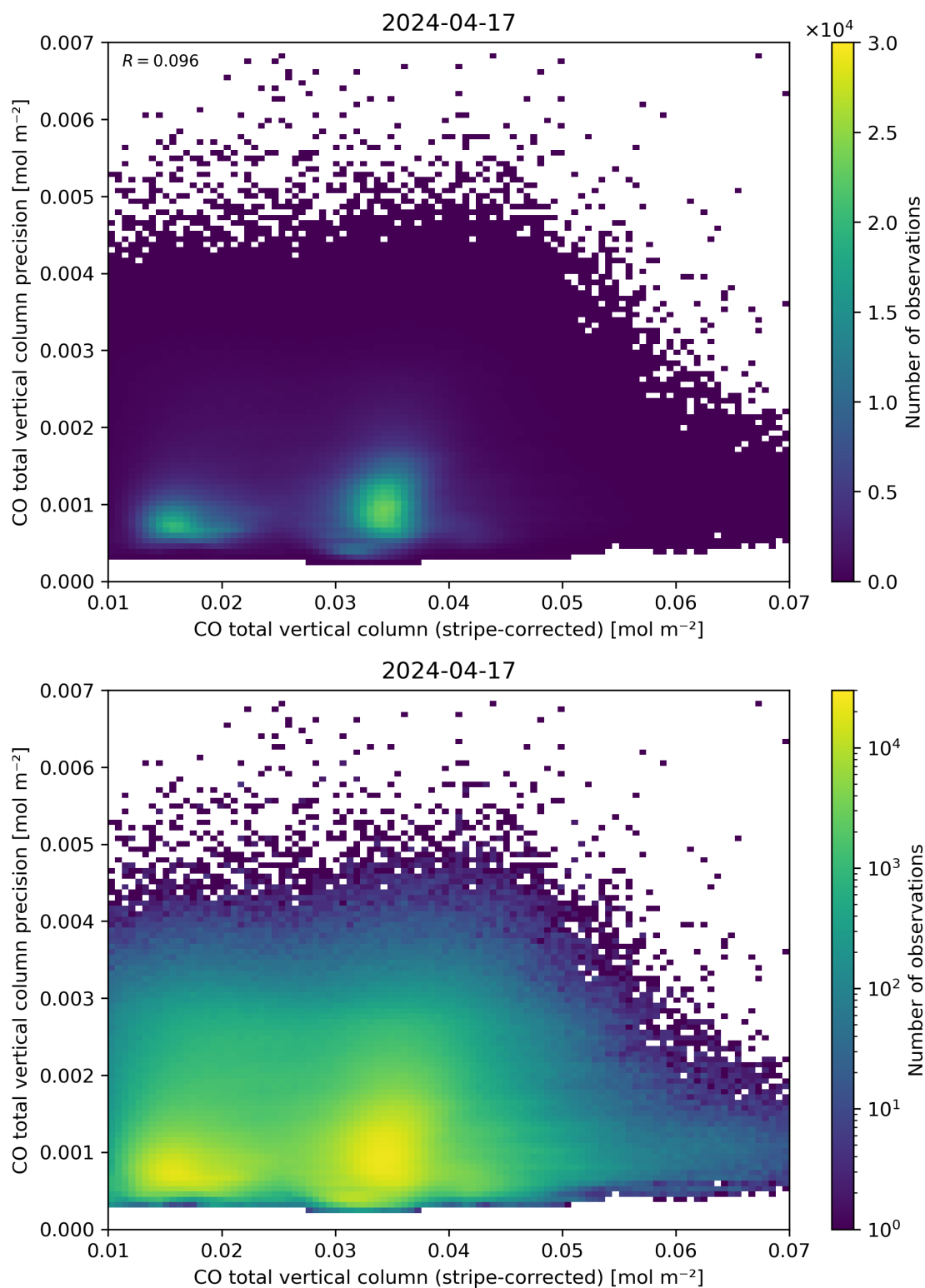
Figure 36: Scatter density plot of “CO total vertical column (stripe-corrected)” against “CO total vertical column precision” for 2024-04-16 to 2024-04-18.
