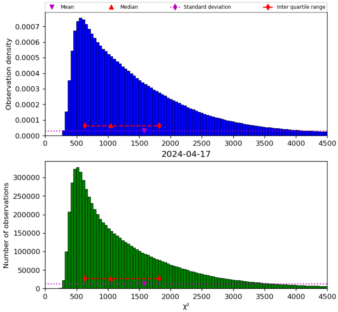
Figure 22: Histogram of “ \chi^2 ” for 2024-04-16 to 2024-04-18
