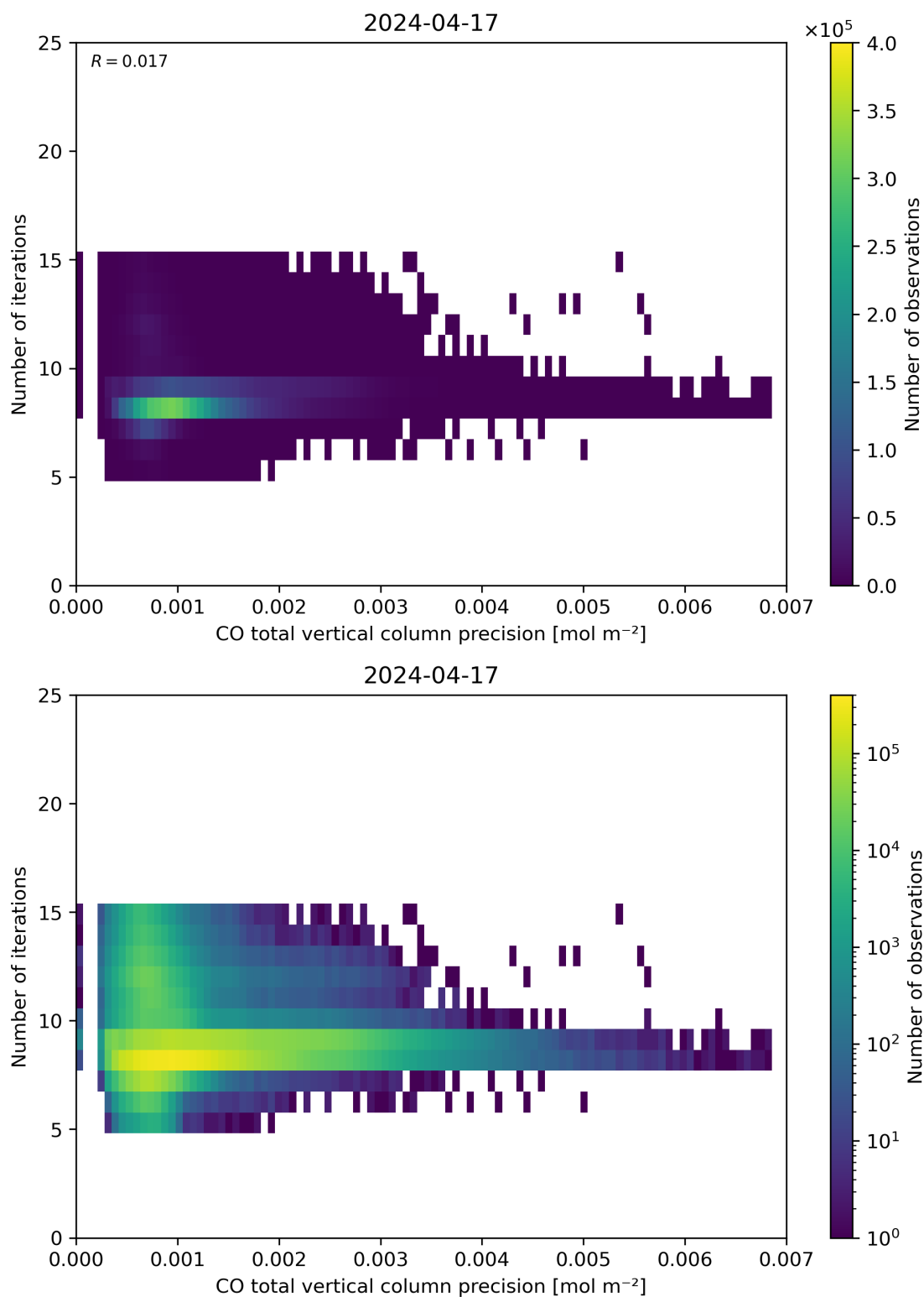
Figure 46: Scatter density plot of “CO total vertical column precision” against “Number of iterations” for 2024-04-16 to 2024-04-18.
