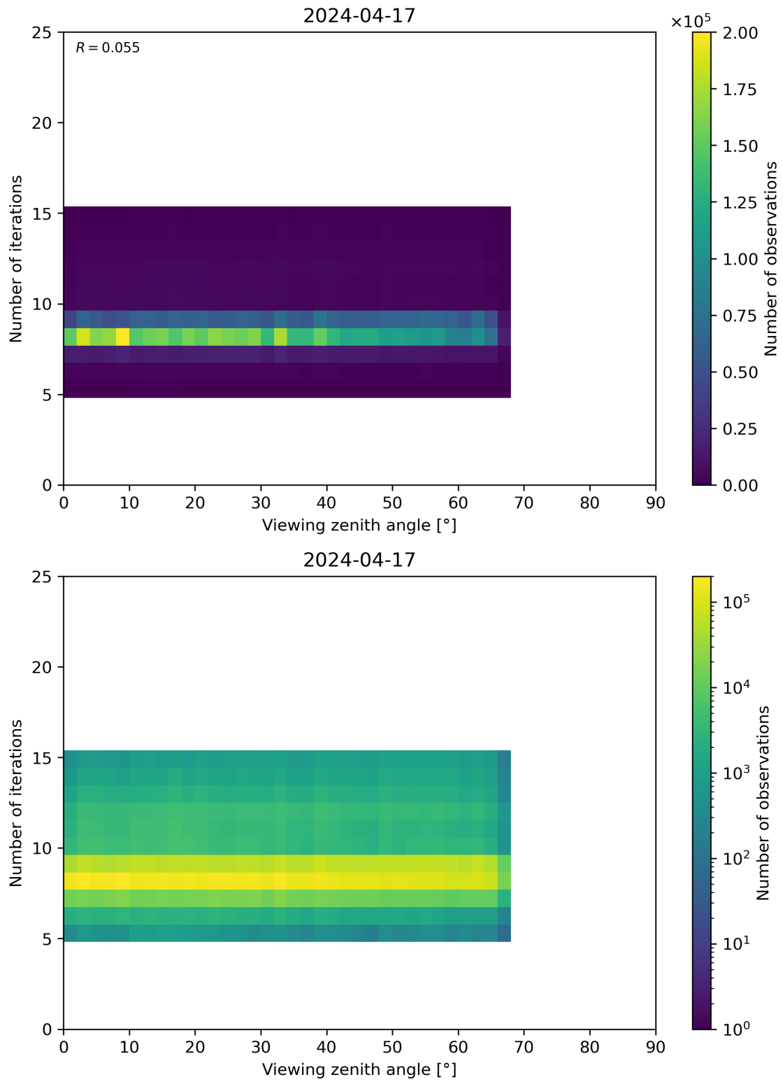
Figure 75: Scatter density plot of “Viewing zenith angle” against “Number of iterations” for 2024-04-16 to 2024-04-18.
