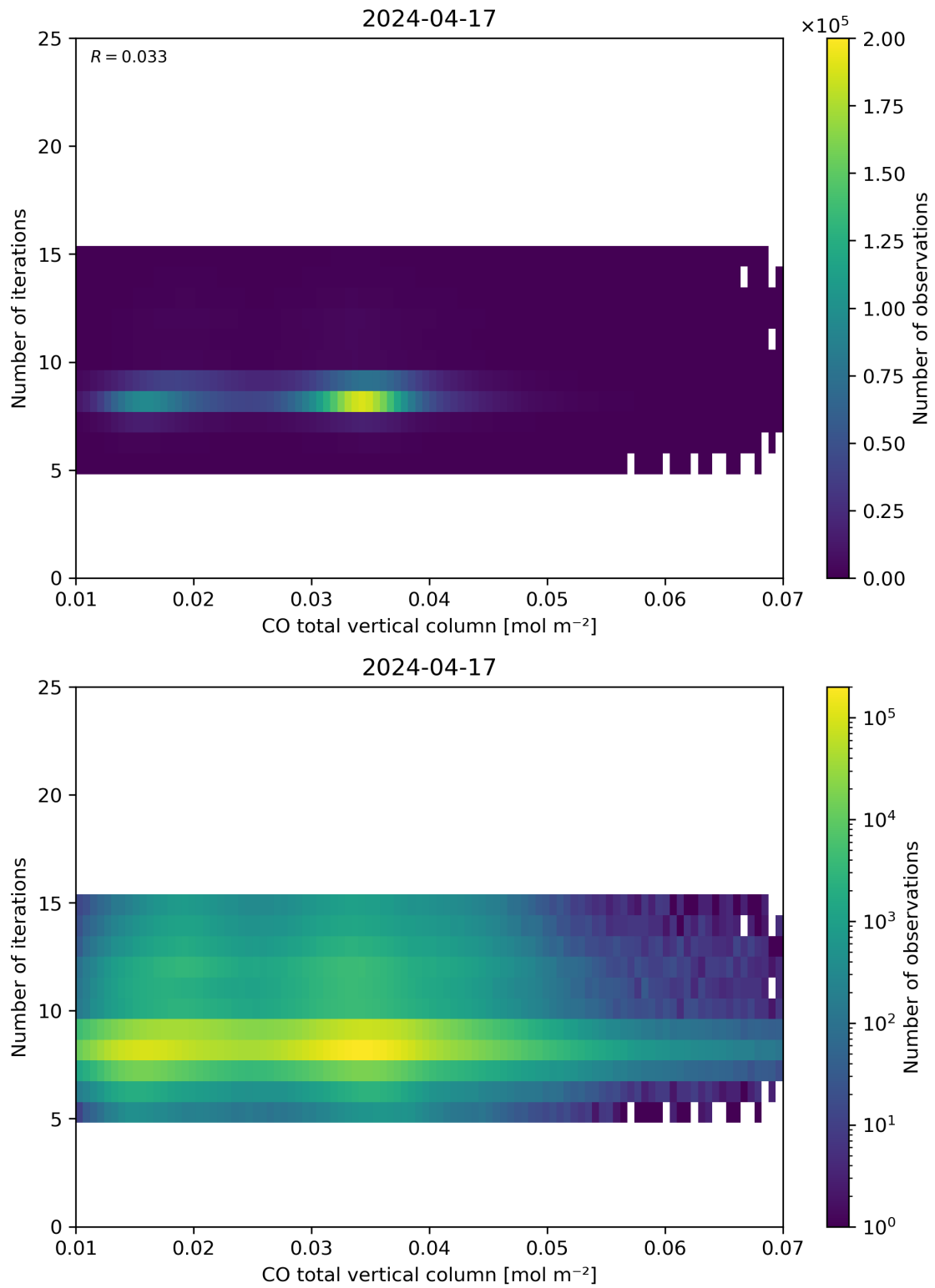
Figure 42: Scatter density plot of “CO total vertical column” against “Number of iterations” for 2024-04-16 to 2024-04-18.
