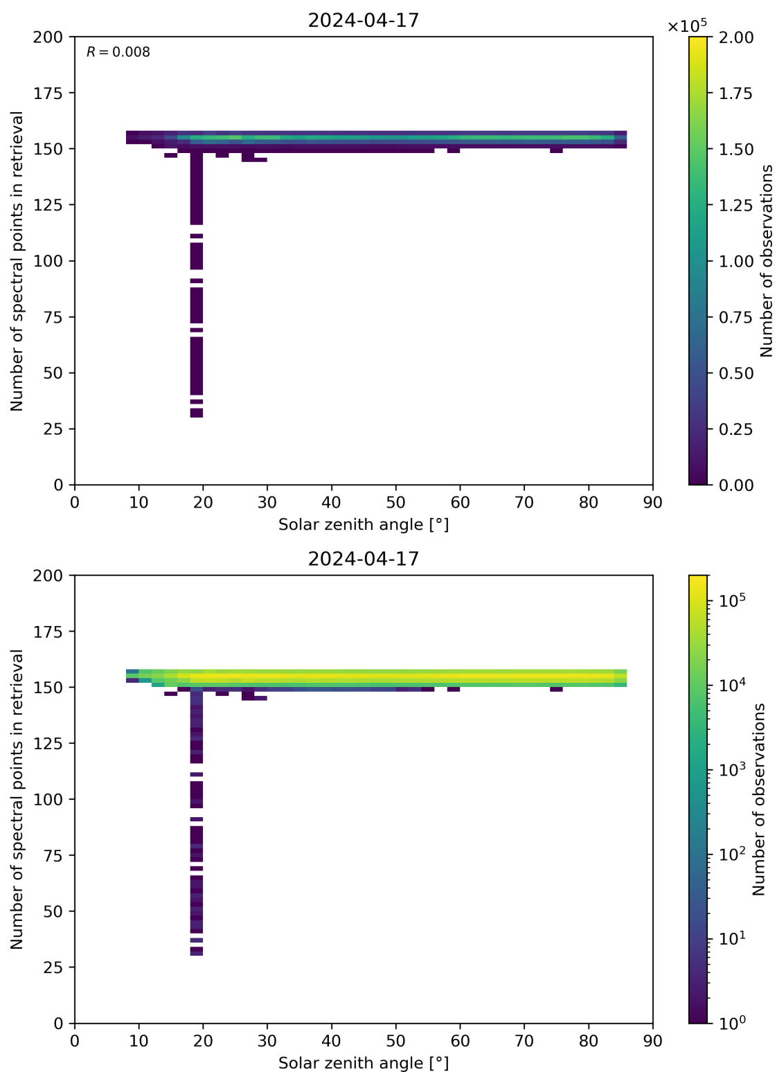
Figure 68: Scatter density plot of “Solar zenith angle” against “Number of spectral points in retrieval” for 2024-04-16 to 2024-04-18.
