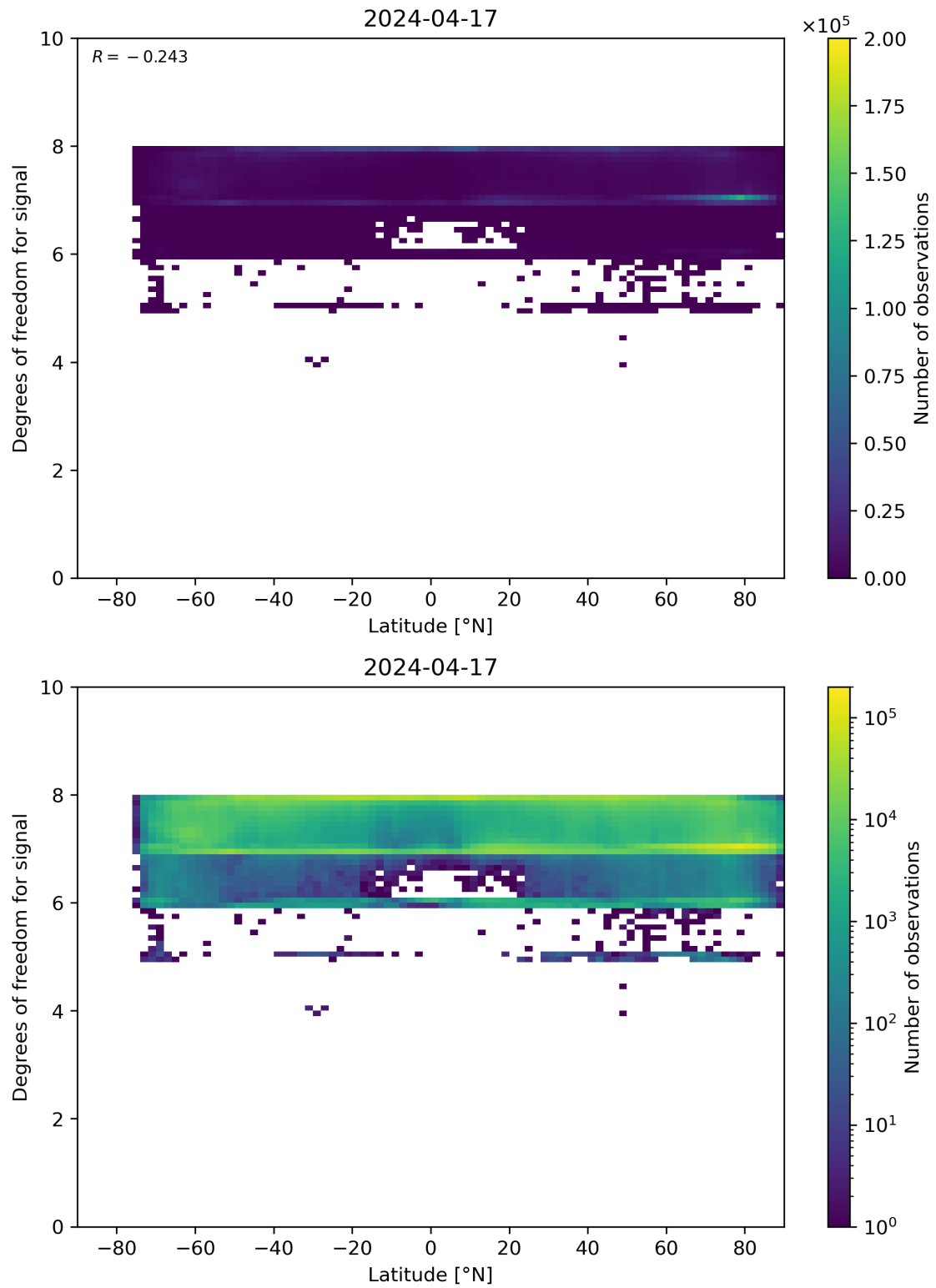
Figure 55: Scatter density plot of “Latitude” against “Degrees of freedom for signal” for 2024-04-16 to 2024-04-18.
