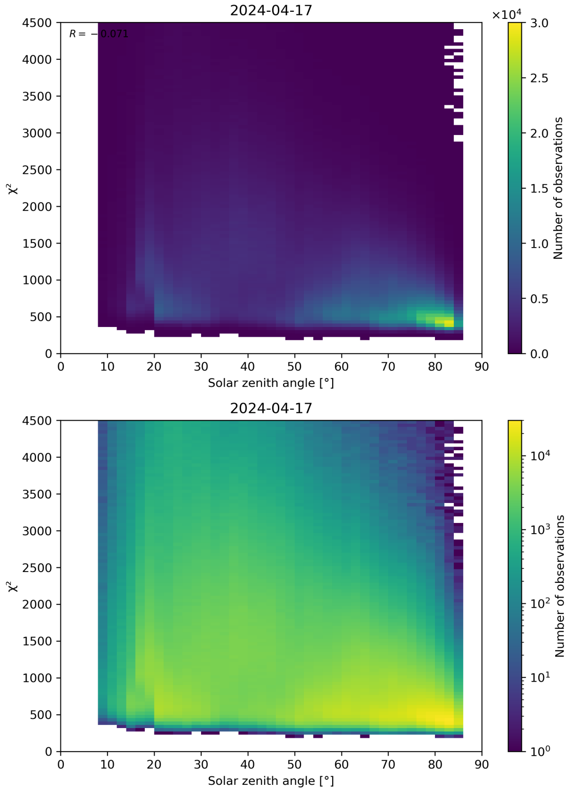
Figure 64: Scatter density plot of “Solar zenith angle” against “ \chi^2 ” for 2024-04-16 to 2024-04-18.
