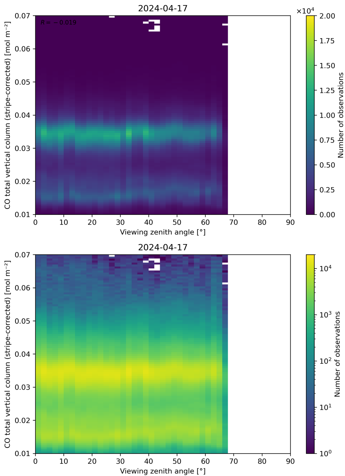
Figure 70: Scatter density plot of “Viewing zenith angle” against “CO total vertical column (stripe-corrected)” for 2024-04-16 to 2024-04-18.
