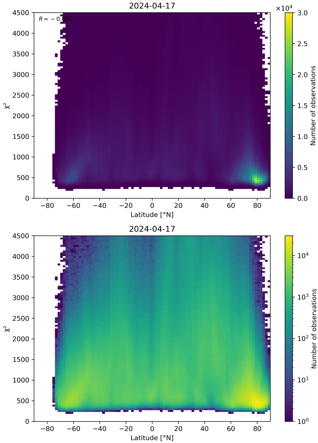
Figure 54: Scatter density plot of “Latitude” against “ \chi^2 ” for 2024-04-16 to 2024-04-18.
