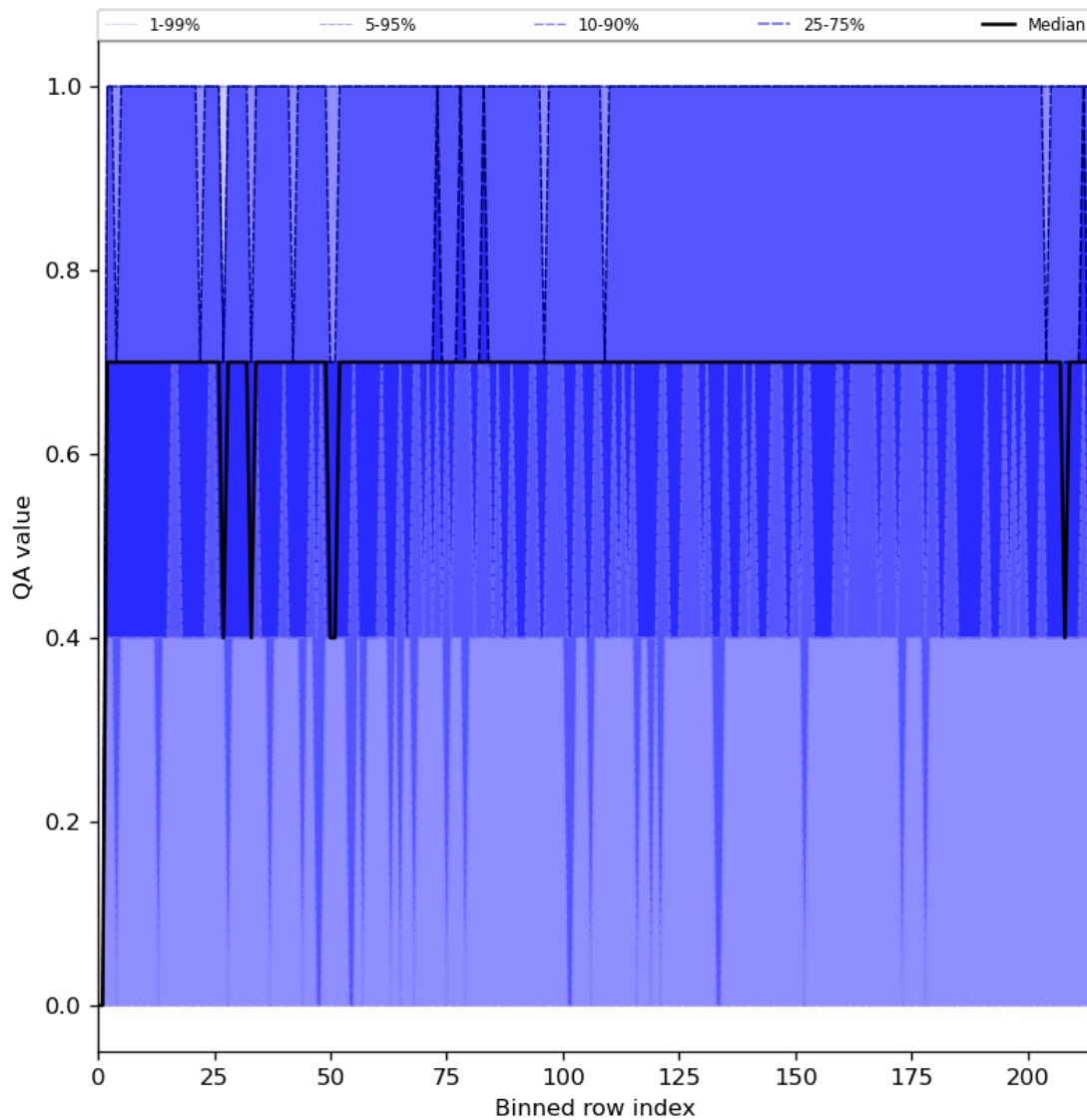
Figure 25: Along track statistics of “QA value” for 2024-04-16 to 2024-04-18
