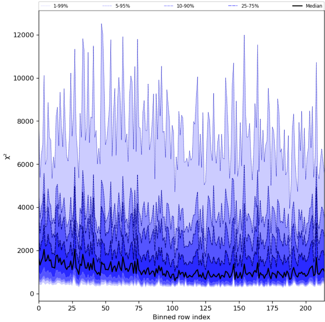
Figure 30: Along track statistics of “ \chi^2 ” for 2024-04-16 to 2024-04-18
