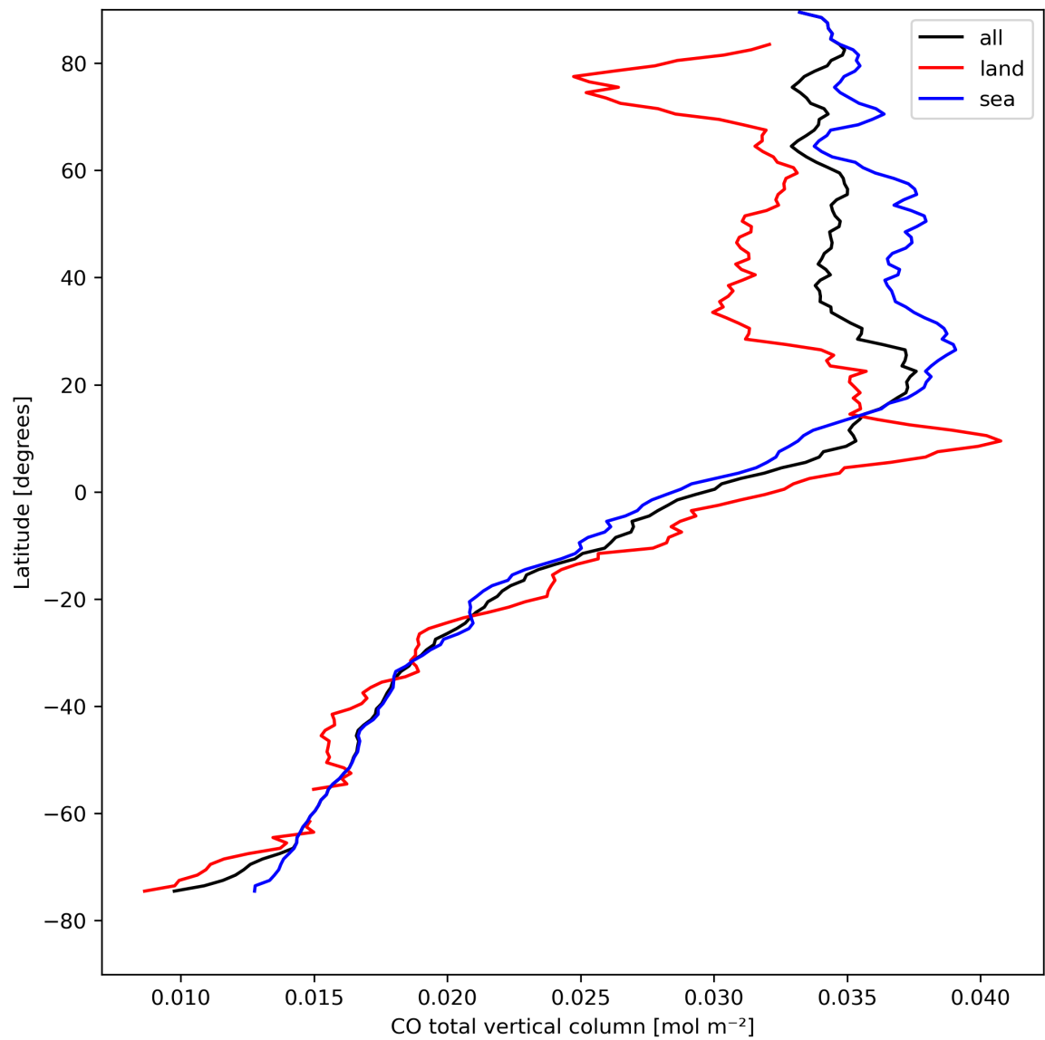
Figure 10: Zonal average of “CO total vertical column” for 2024-04-16 to 2024-04-18.
