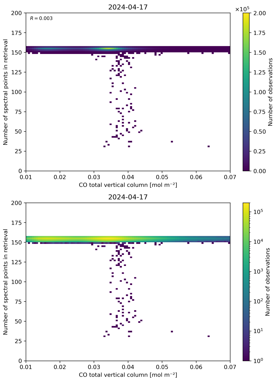
Figure 43: Scatter density plot of “CO total vertical column” against “Number of spectral points in retrieval” for 2024-04-16 to 2024-04-18.
