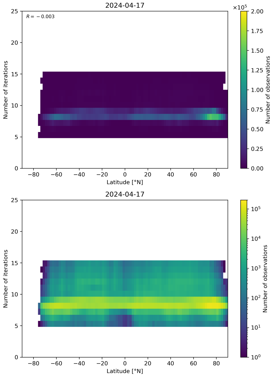
Figure 56: Scatter density plot of “Latitude” against “Number of iterations” for 2024-04-16 to 2024-04-18.
