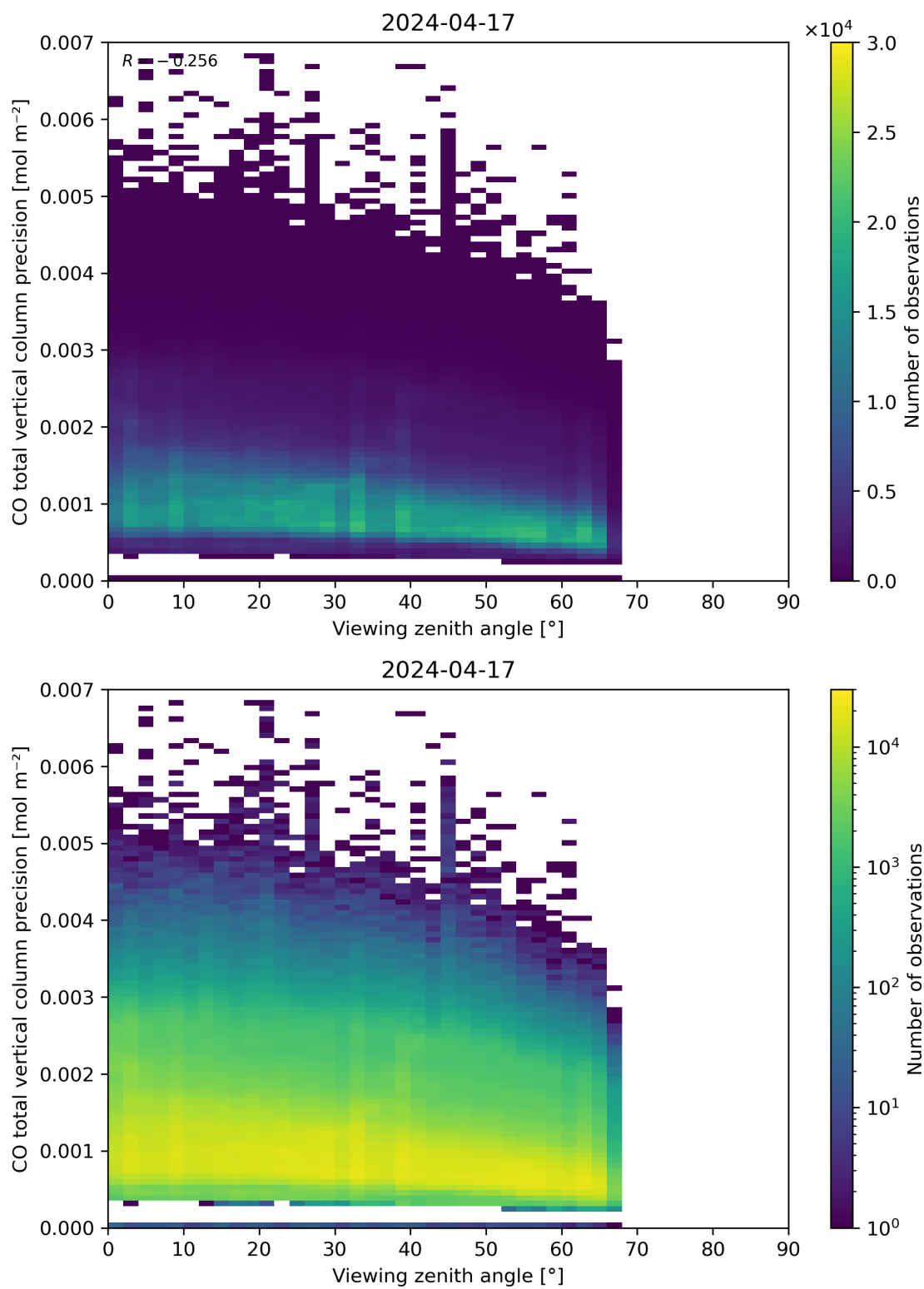
Figure 71: Scatter density plot of “Viewing zenith angle” against “CO total vertical column precision” for 2024-04-16 to 2024-04-18.
