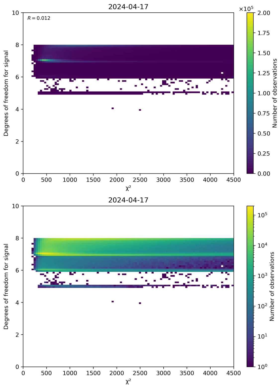
Figure 48: Scatter density plot of “ \chi^2 ” against “Degrees of freedom for signal” for 2024-04-16 to 2024-04-18.
