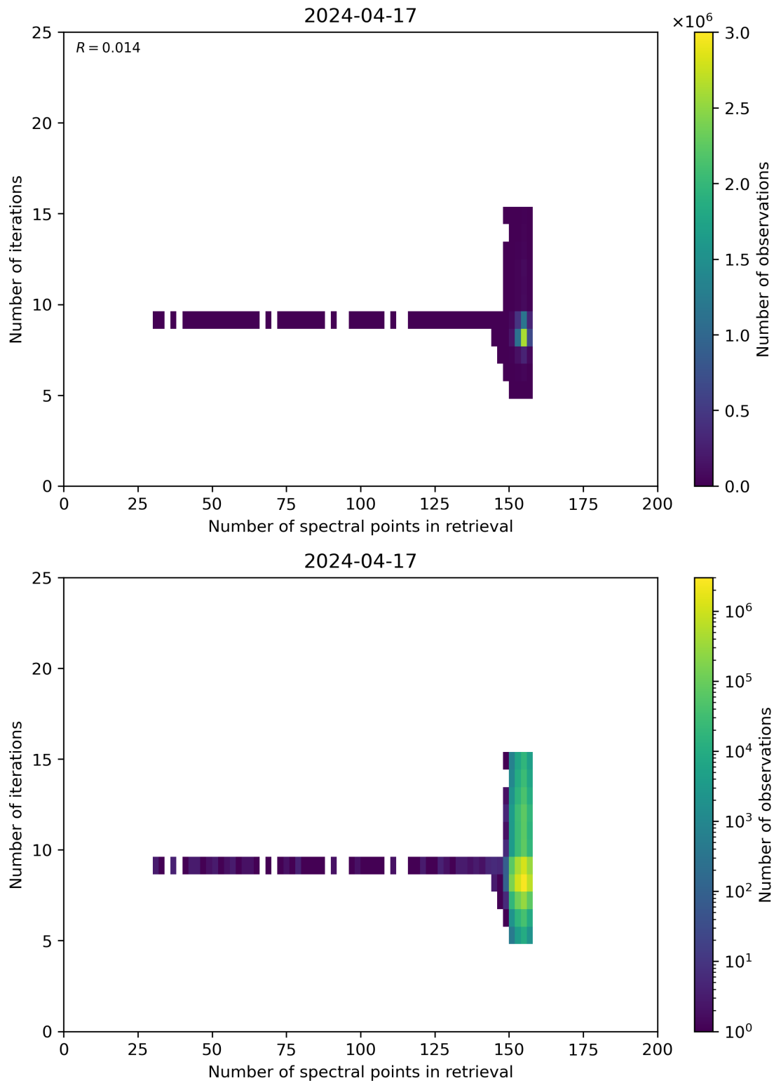
Figure 60: Scatter density plot of “Number of spectral points in retrieval” against “Number of iterations” for 2024-04-16 to 2024-04-18.
