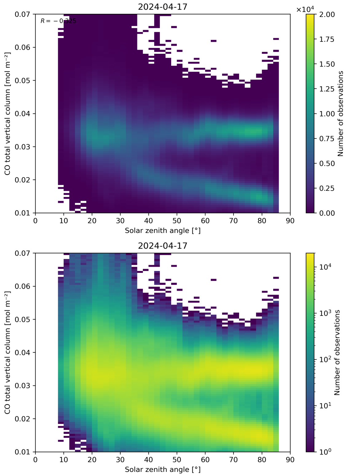
Figure 61: Scatter density plot of “Solar zenith angle” against “CO total vertical column” for 2024-04-16 to 2024-04-18.
