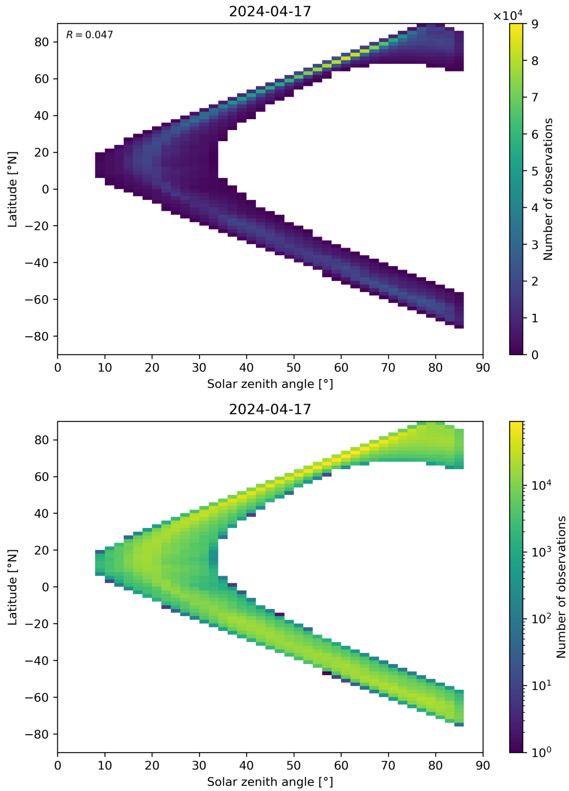
Figure 66: Scatter density plot of “Solar zenith angle” against “Latitude” for 2024-04-16 to 2024-04-18.
