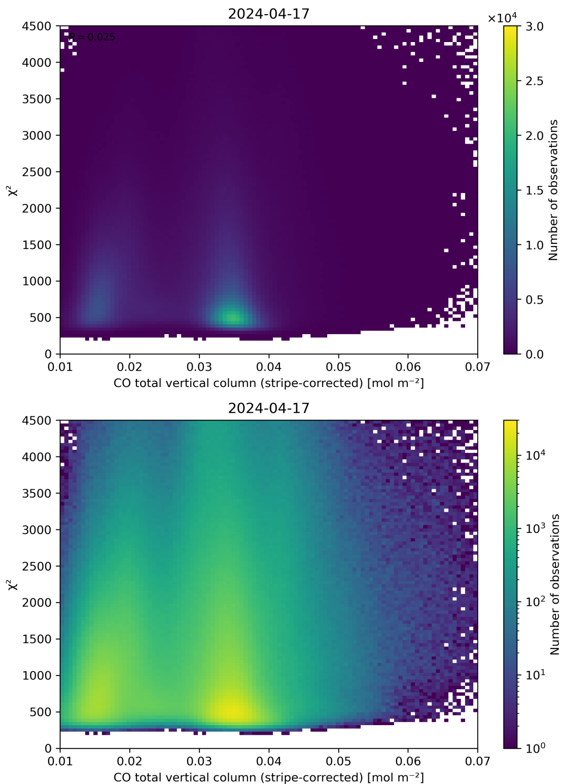
Figure 37: Scatter density plot of “CO total vertical column (stripe-corrected)” against “ \chi^2 ” for 2024-04-16 to 2024-04-18.
