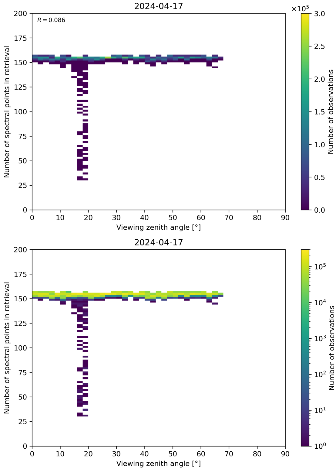
Figure 76: Scatter density plot of “Viewing zenith angle” against “Number of spectral points in retrieval” for 2024-04-16 to 2024-04-18.
