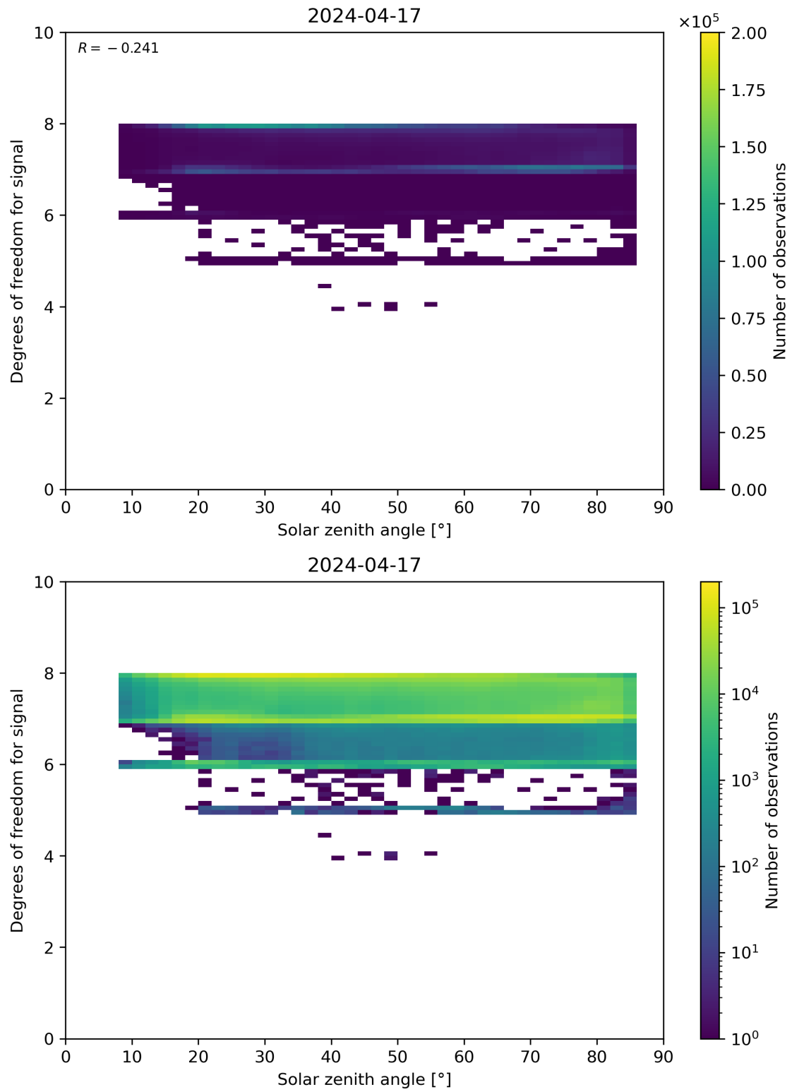
Figure 65: Scatter density plot of “Solar zenith angle” against “Degrees of freedom for signal” for 2024-04-16 to 2024-04-18.
