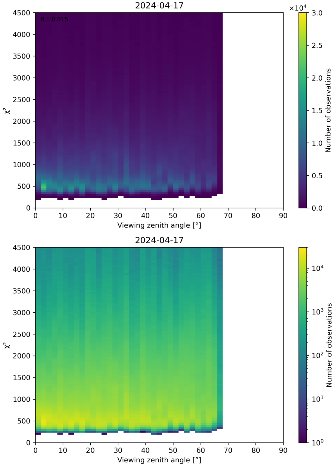
Figure 72: Scatter density plot of “Viewing zenith angle” against “ \chi^2 ” for 2024-04-16 to 2024-04-18.
