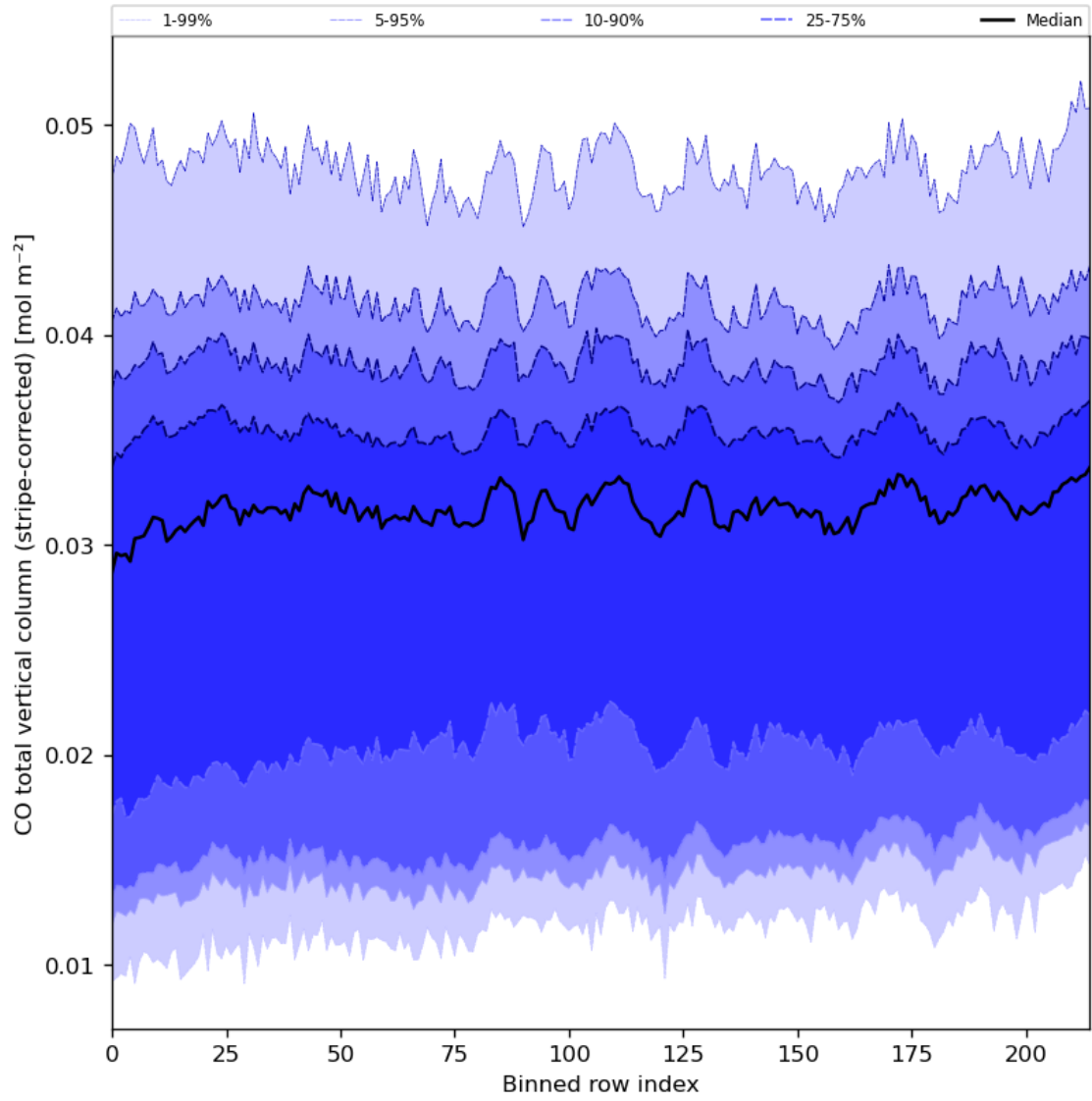
Figure 27: Along track statistics of “CO total vertical column (stripe-corrected)” for 2024-04-16 to 2024-04-18
