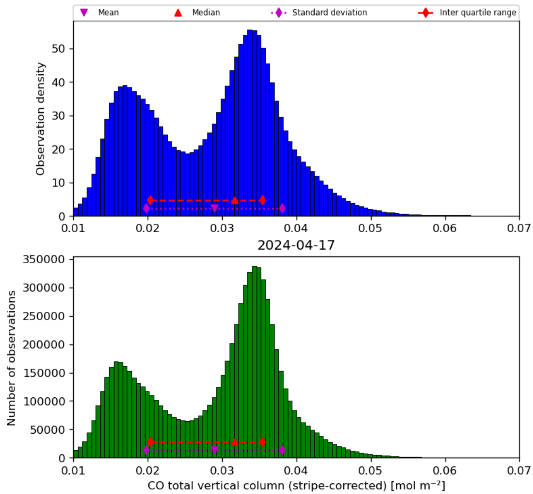
Figure 19: Histogram of “CO total vertical column (stripe-corrected)” for 2024-04-16 to 2024-04-18
