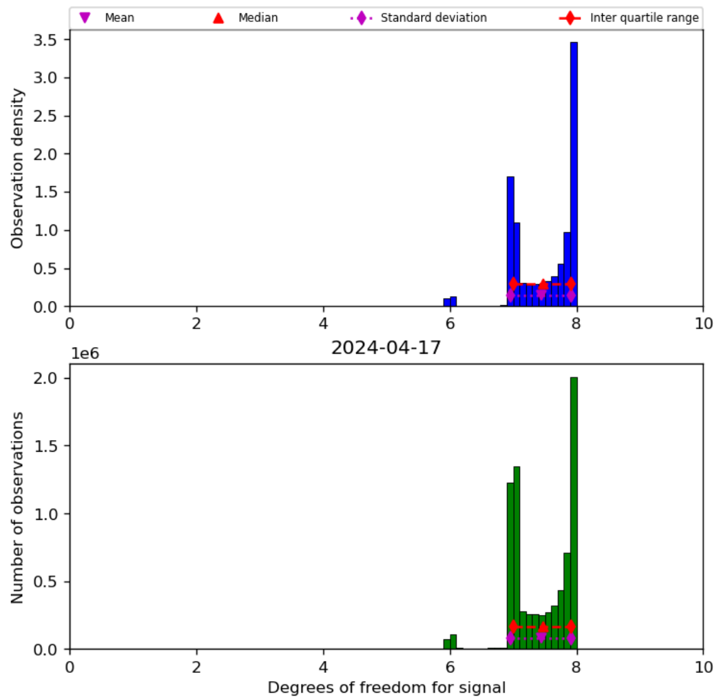
Figure 23: Histogram of “Degrees of freedom for signal” for 2024-04-16 to 2024-04-18
