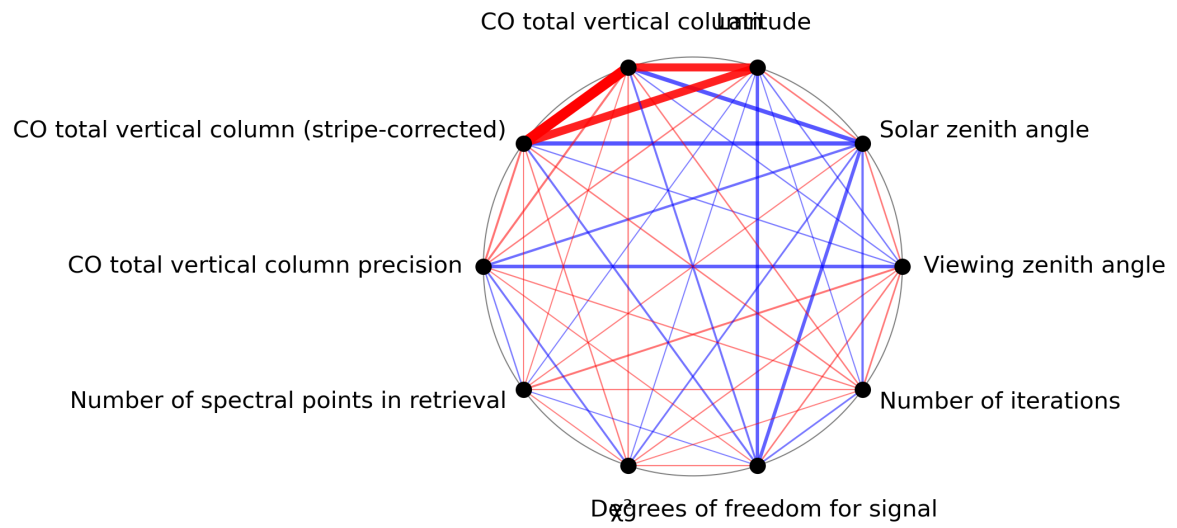
Figure 1: Map of correlation graph for 2024-04-16 to 2024-04-18.
