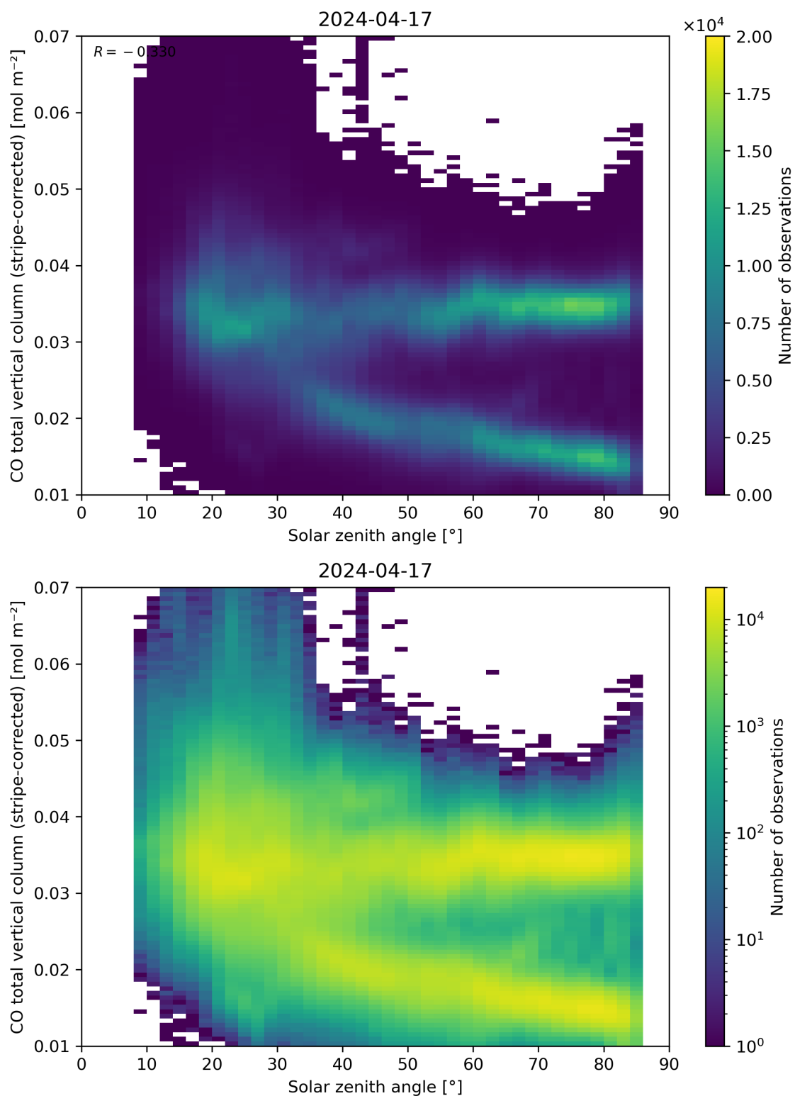
Figure 62: Scatter density plot of “Solar zenith angle” against “CO total vertical column (stripe-corrected)” for 2024-04-16 to 2024-04-18.
