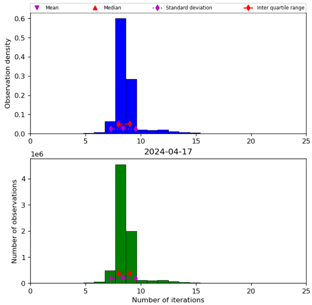
Figure 24: Histogram of “Number of iterations” for 2024-04-16 to 2024-04-18
