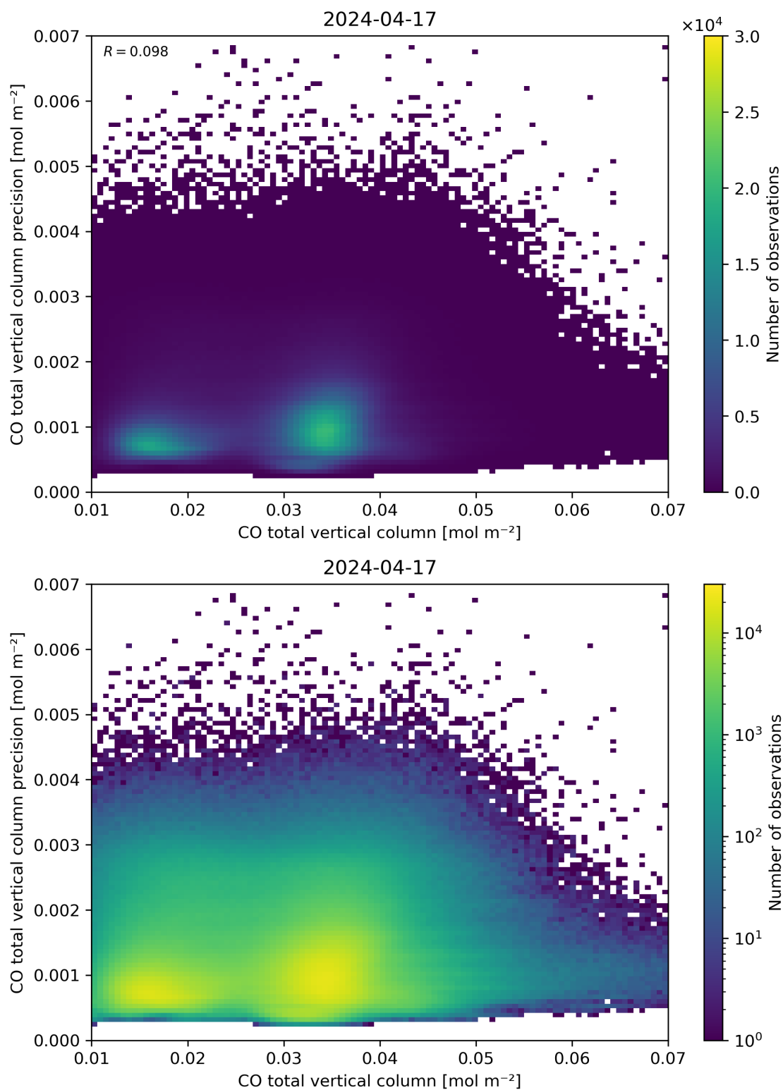
Figure 34: Scatter density plot of “CO total vertical column” against “CO total vertical column precision” for 2024-04-16 to 2024-04-18.
