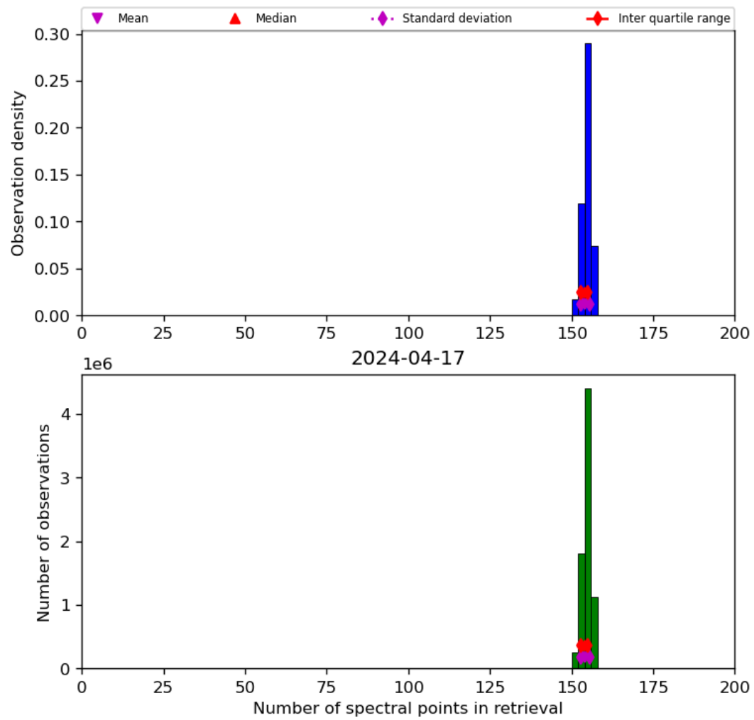
Figure 21: Histogram of “Number of spectral points in retrieval” for 2024-04-16 to 2024-04-18
