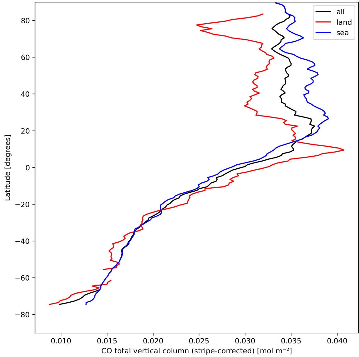
Figure 11: Zonal average of “CO total vertical column (stripe-corrected)” for 2024-04-16 to 2024-04-18.
