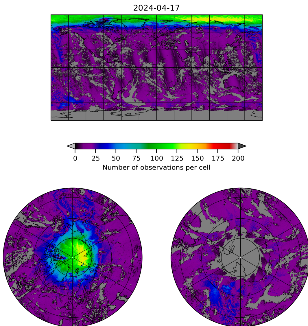
Figure 8: Map of the number of observations for 2024-04-16 to 2024-04-18
