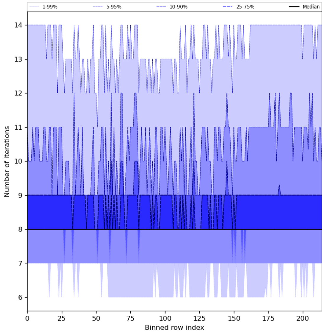
Figure 32: Along track statistics of “Number of iterations” for 2024-04-16 to 2024-04-18
