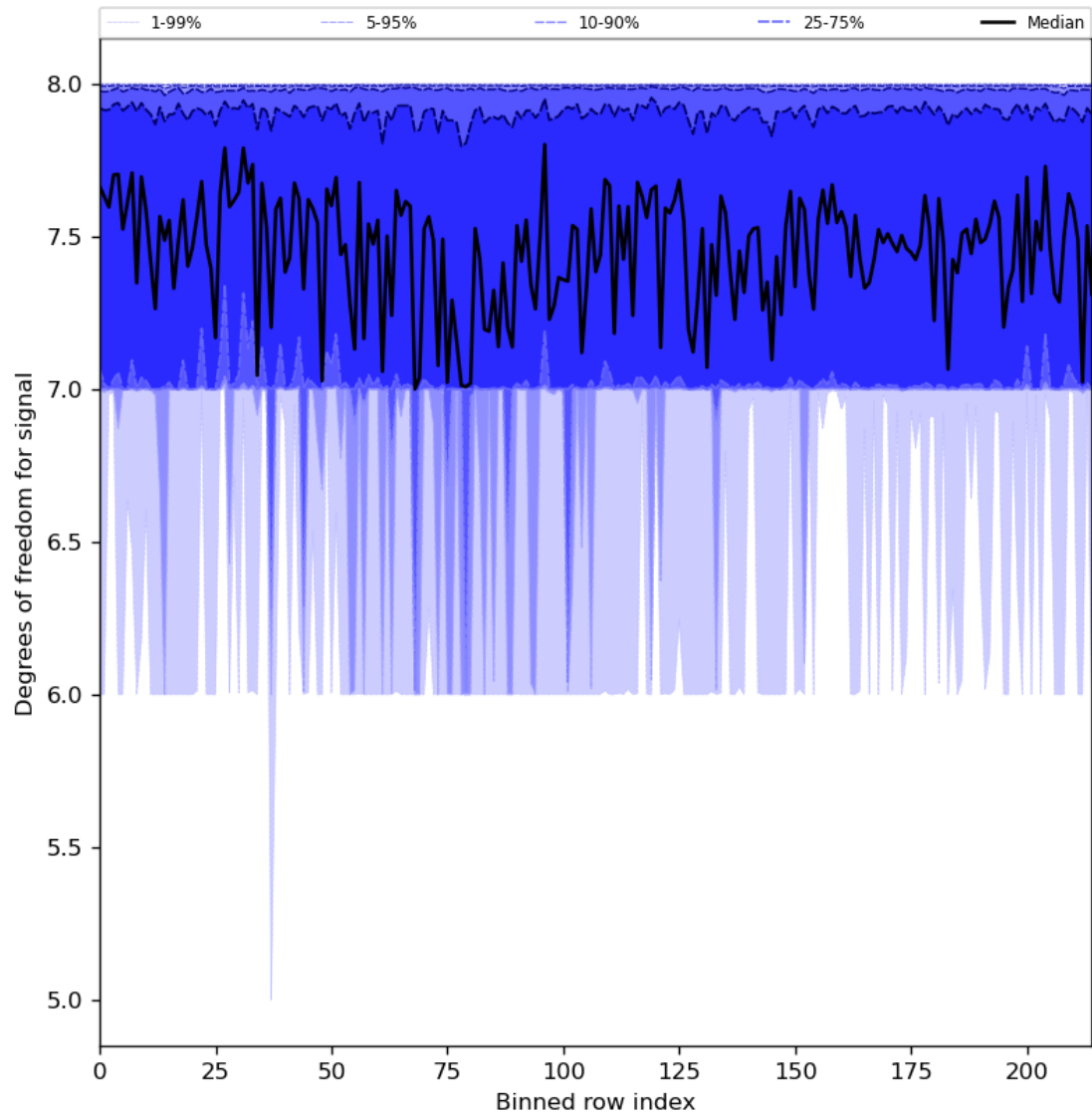
Figure 31: Along track statistics of “Degrees of freedom for signal” for 2024-04-16 to 2024-04-18
