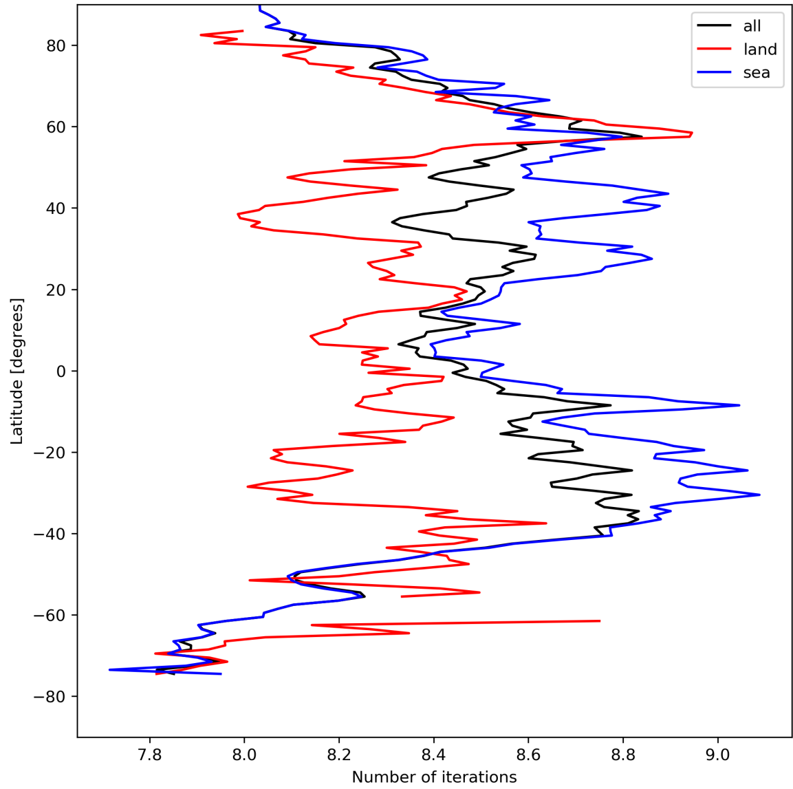
Figure 16: Zonal average of “Number of iterations” for 2024-04-16 to 2024-04-18.
