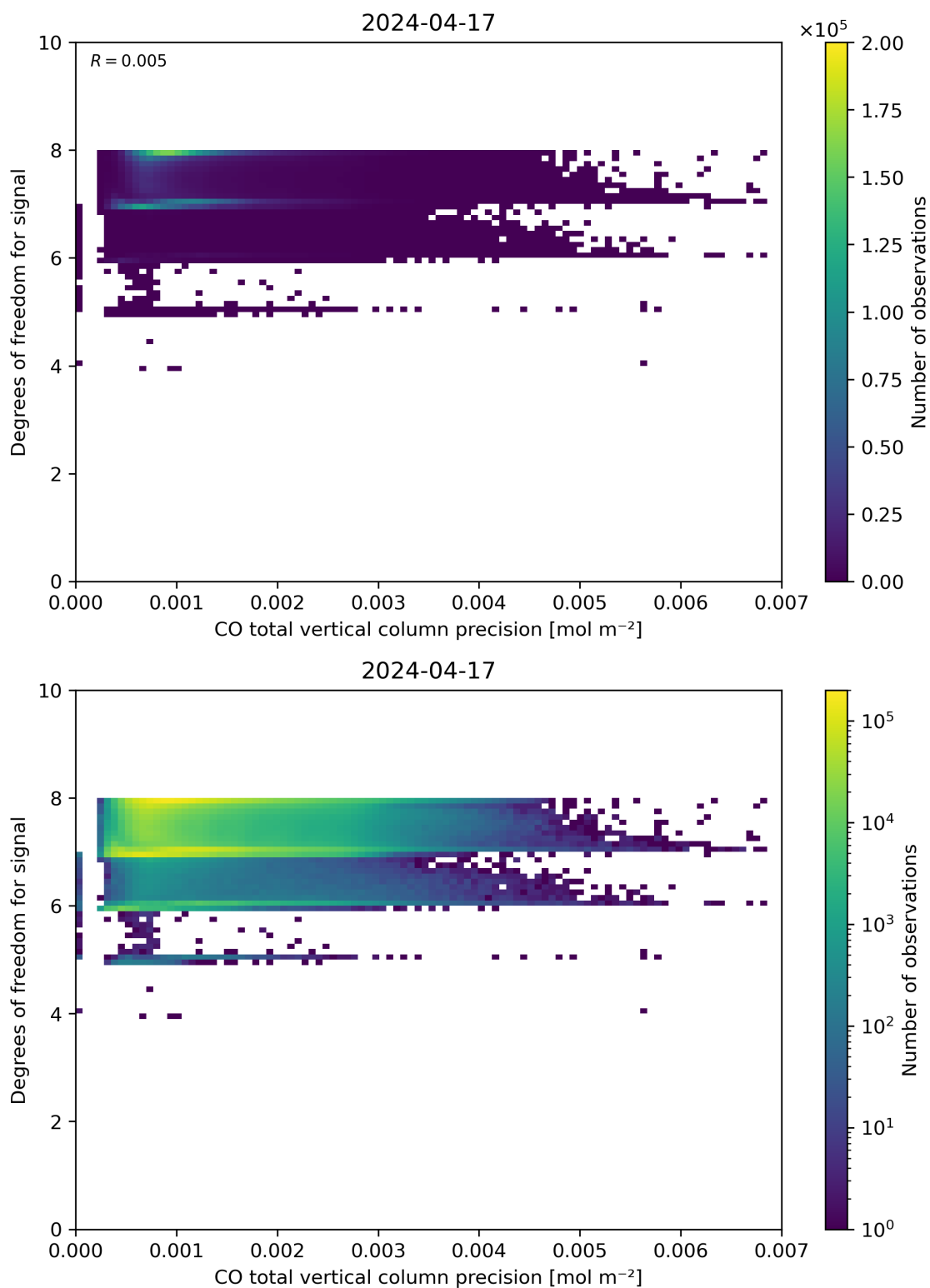
Figure 45: Scatter density plot of “CO total vertical column precision” against “Degrees of freedom for signal” for 2024-04-16 to 2024-04-18.
