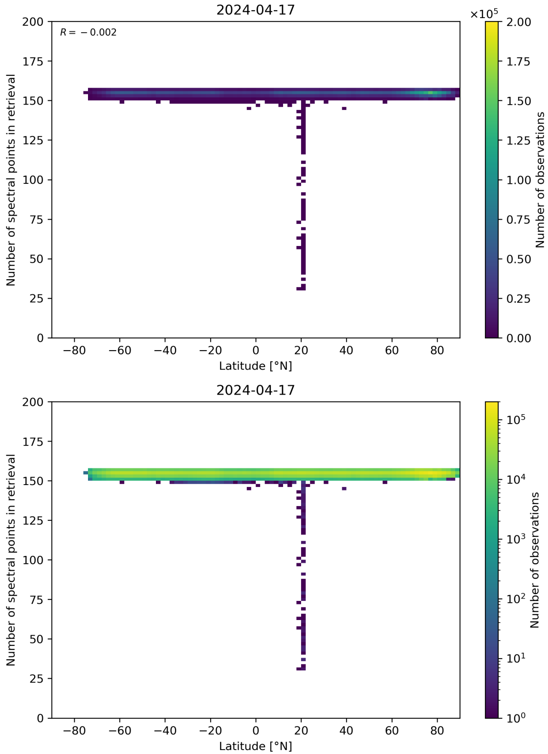
Figure 57: Scatter density plot of “Latitude” against “Number of spectral points in retrieval” for 2024-04-16 to 2024-04-18.
