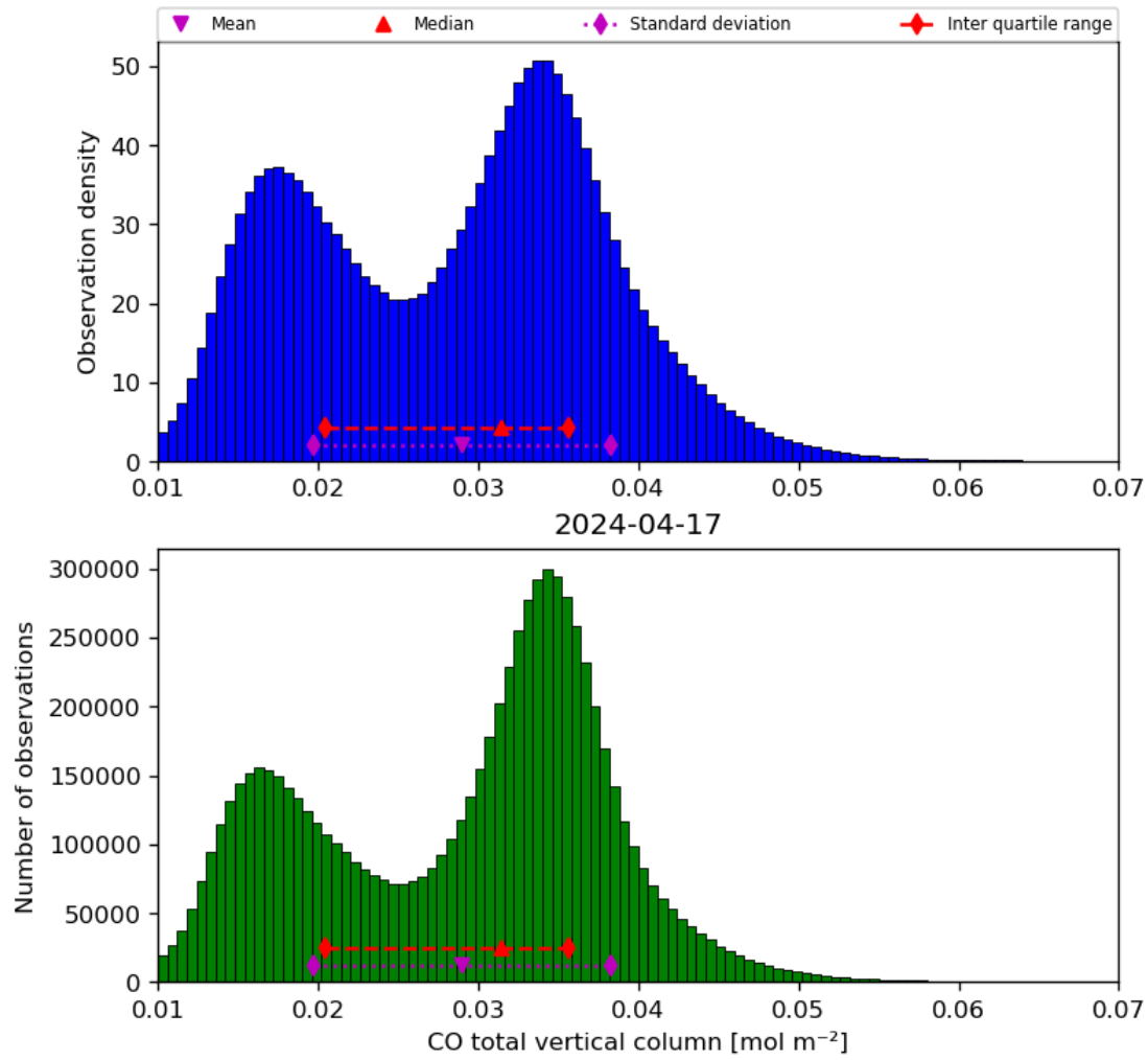
Figure 18: Histogram of “CO total vertical column” for 2024-04-16 to 2024-04-18
