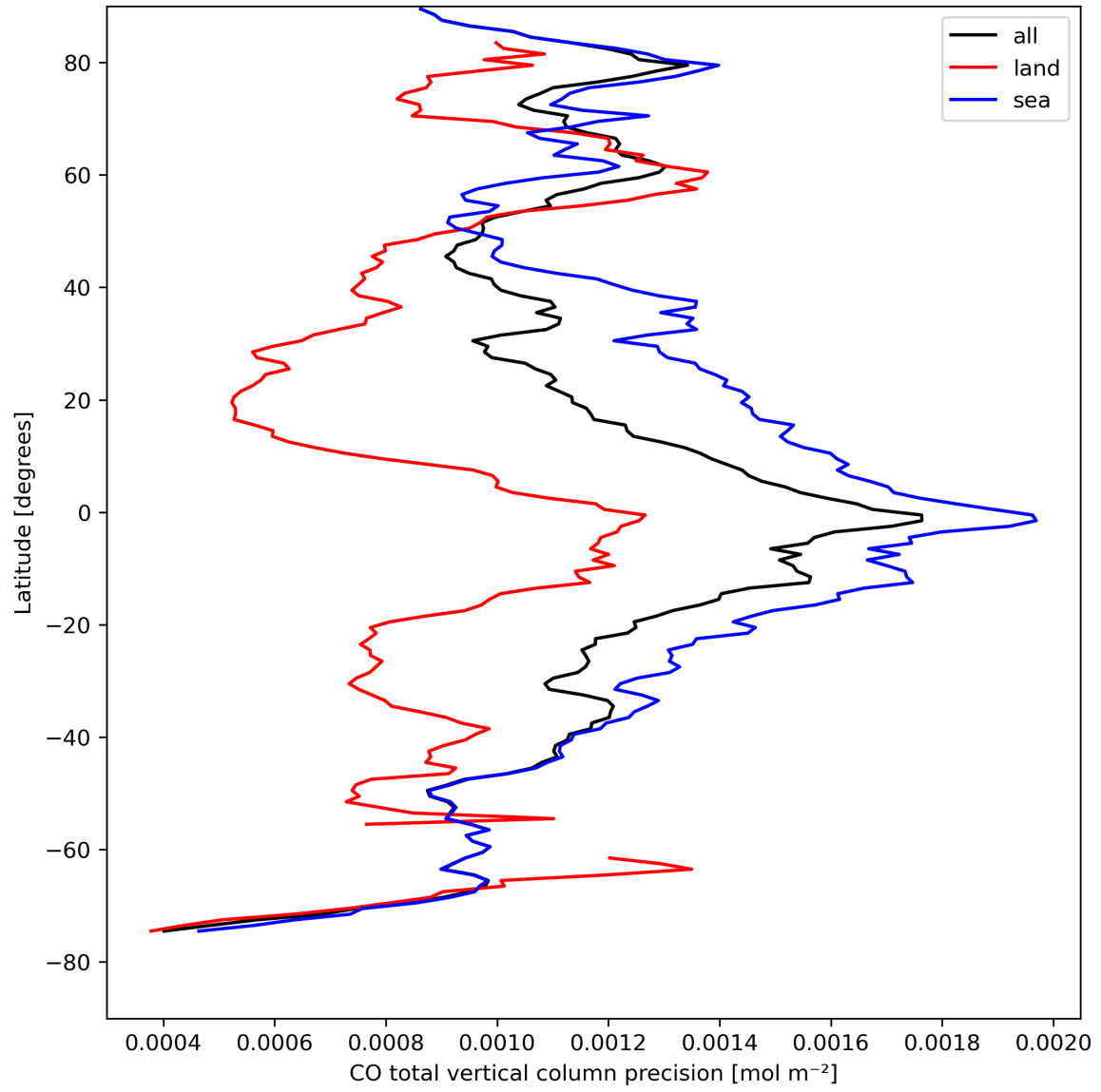
Figure 12: Zonal average of "CO total vertical column precision" for 2024-04-16 to 2024-04-18.
