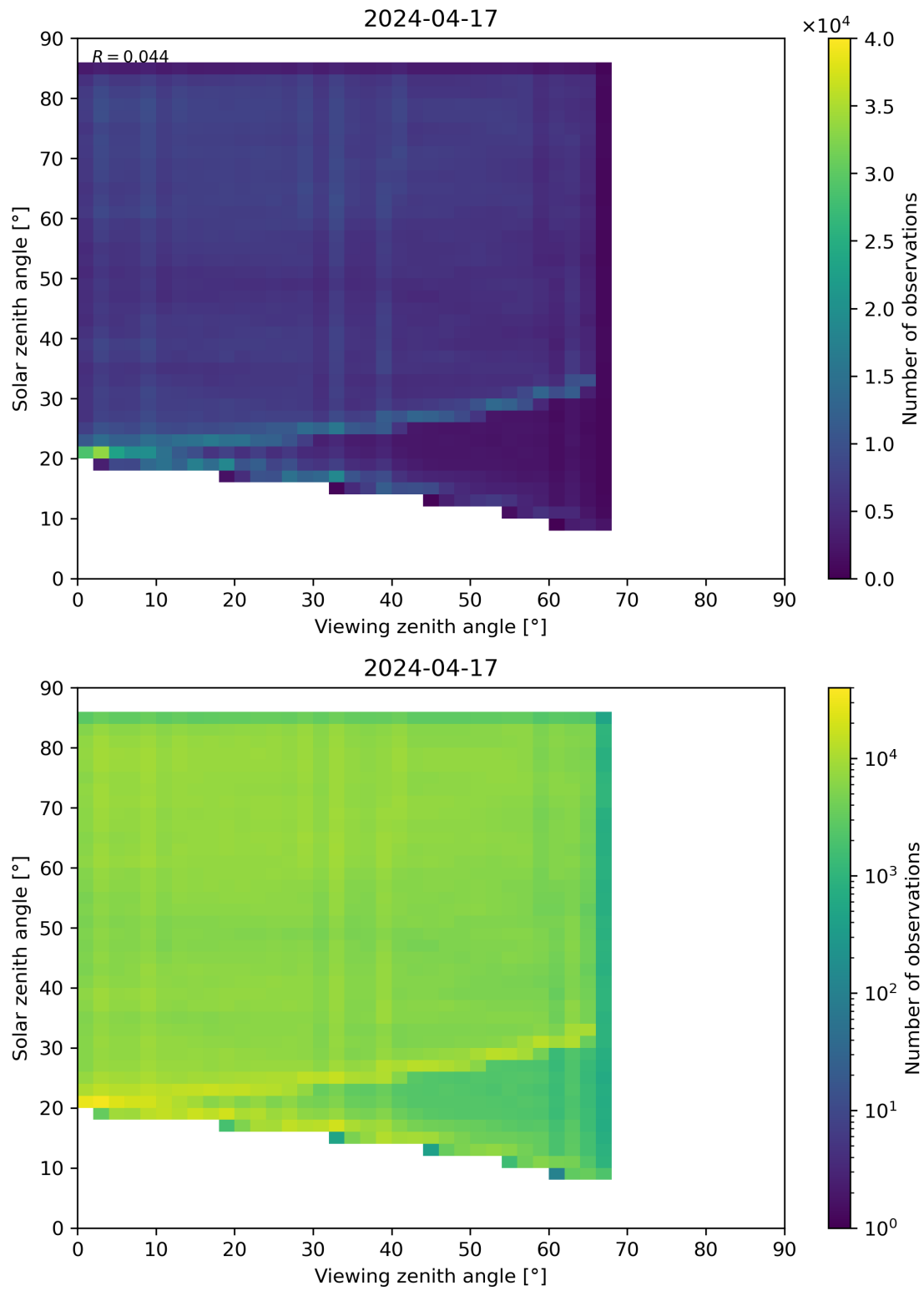
Figure 77: Scatter density plot of “Viewing zenith angle” against “Solar zenith angle” for 2024-04-16 to 2024-04-18.
