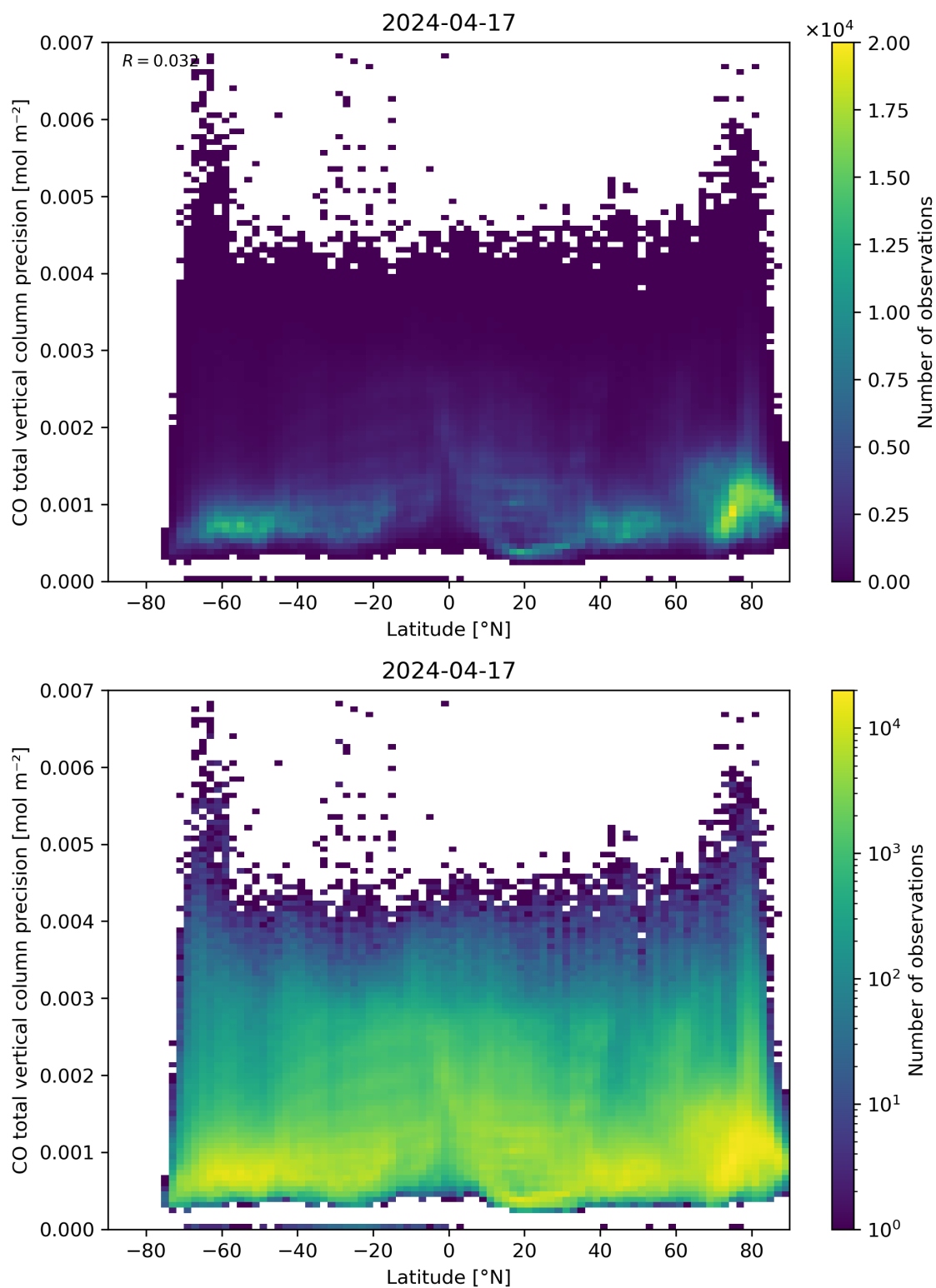
Figure 53: Scatter density plot of “Latitude” against “CO total vertical column precision” for 2024-04-16 to 2024-04-18.
