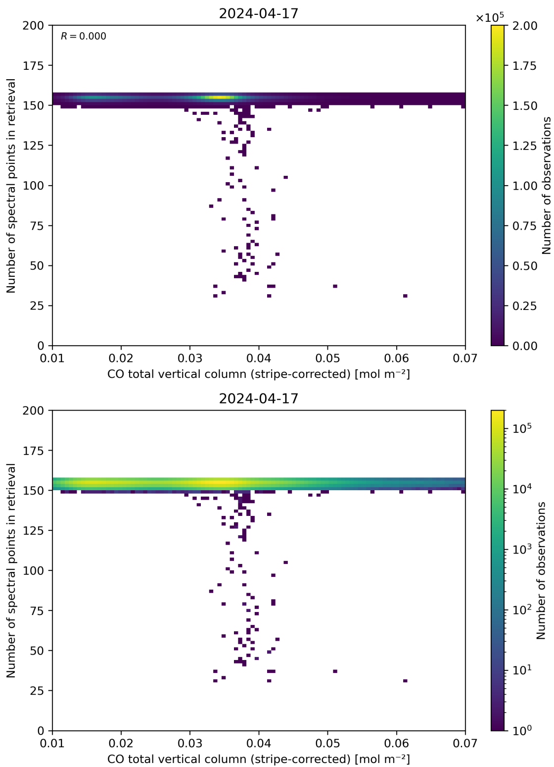
Figure 40: Scatter density plot of “CO total vertical column (stripe-corrected)” against “Number of spectral points in retrieval” for 2024-04-16 to 2024-04-18.
