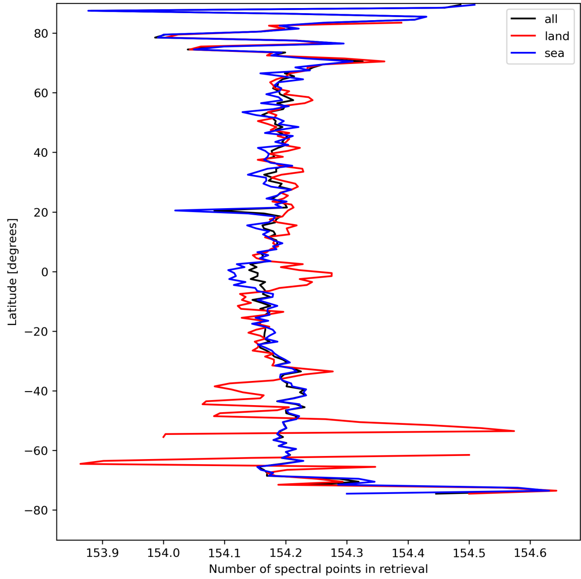
Figure 13: Zonal average of “Number of spectral points in retrieval” for 2024-04-16 to 2024-04-18.
