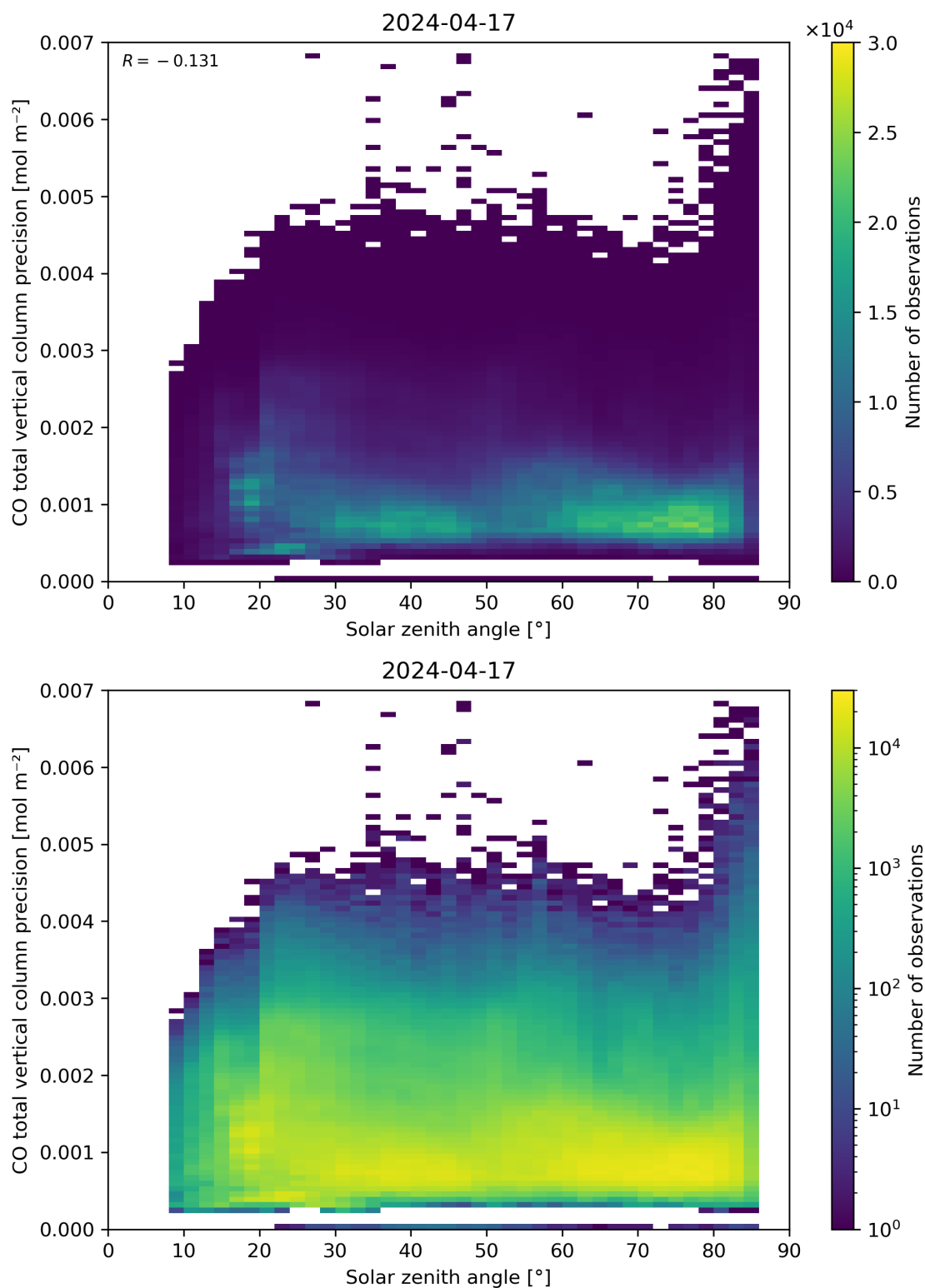
Figure 63: Scatter density plot of “Solar zenith angle” against “CO total vertical column precision” for 2024-04-16 to 2024-04-18.
