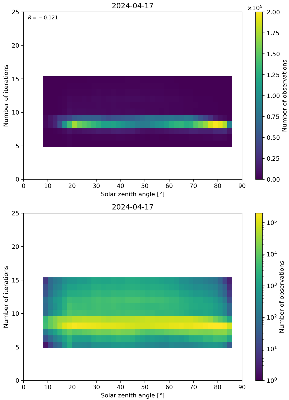
Figure 67: Scatter density plot of “Solar zenith angle” against “Number of iterations” for 2024-04-16 to 2024-04-18.
