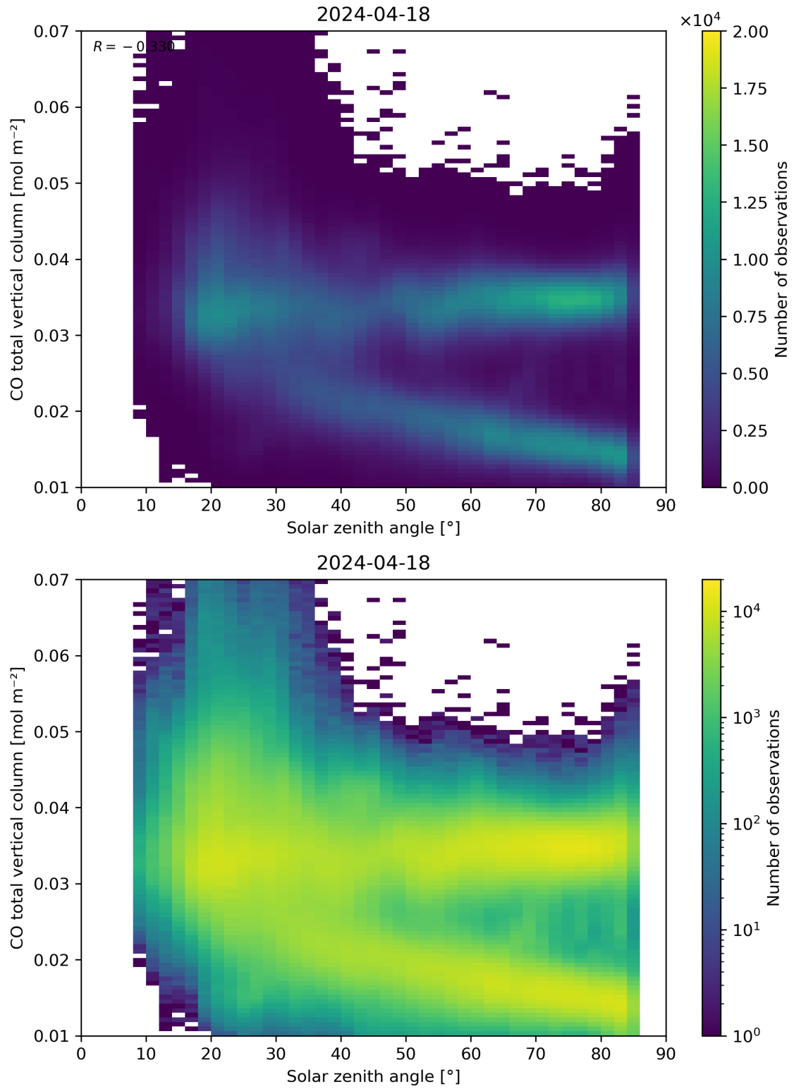
Figure 61: Scatter density plot of “Solar zenith angle” against “CO total vertical column” for 2024-04-17 to 2024-04-19.
