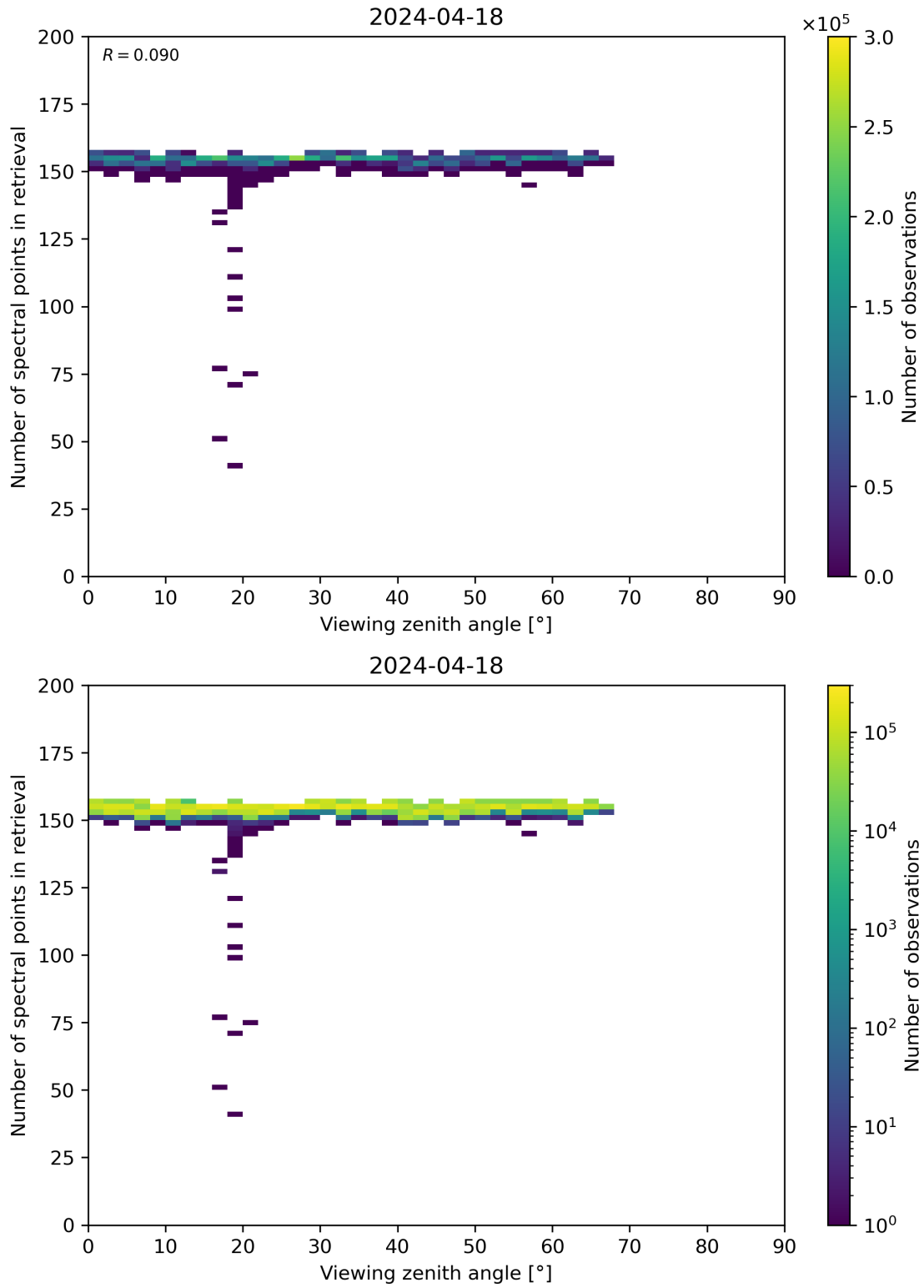
Figure 76: Scatter density plot of “Viewing zenith angle” against “Number of spectral points in retrieval” for 2024-04-17 to 2024-04-19.
