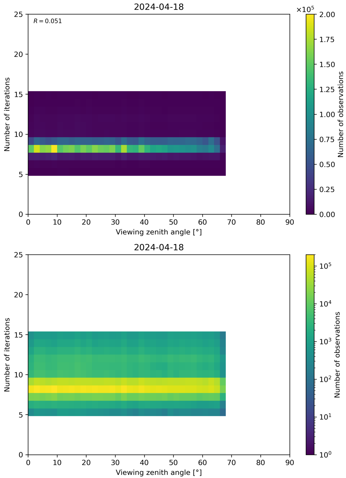
Figure 75: Scatter density plot of “Viewing zenith angle” against “Number of iterations” for 2024-04-17 to 2024-04-19.
