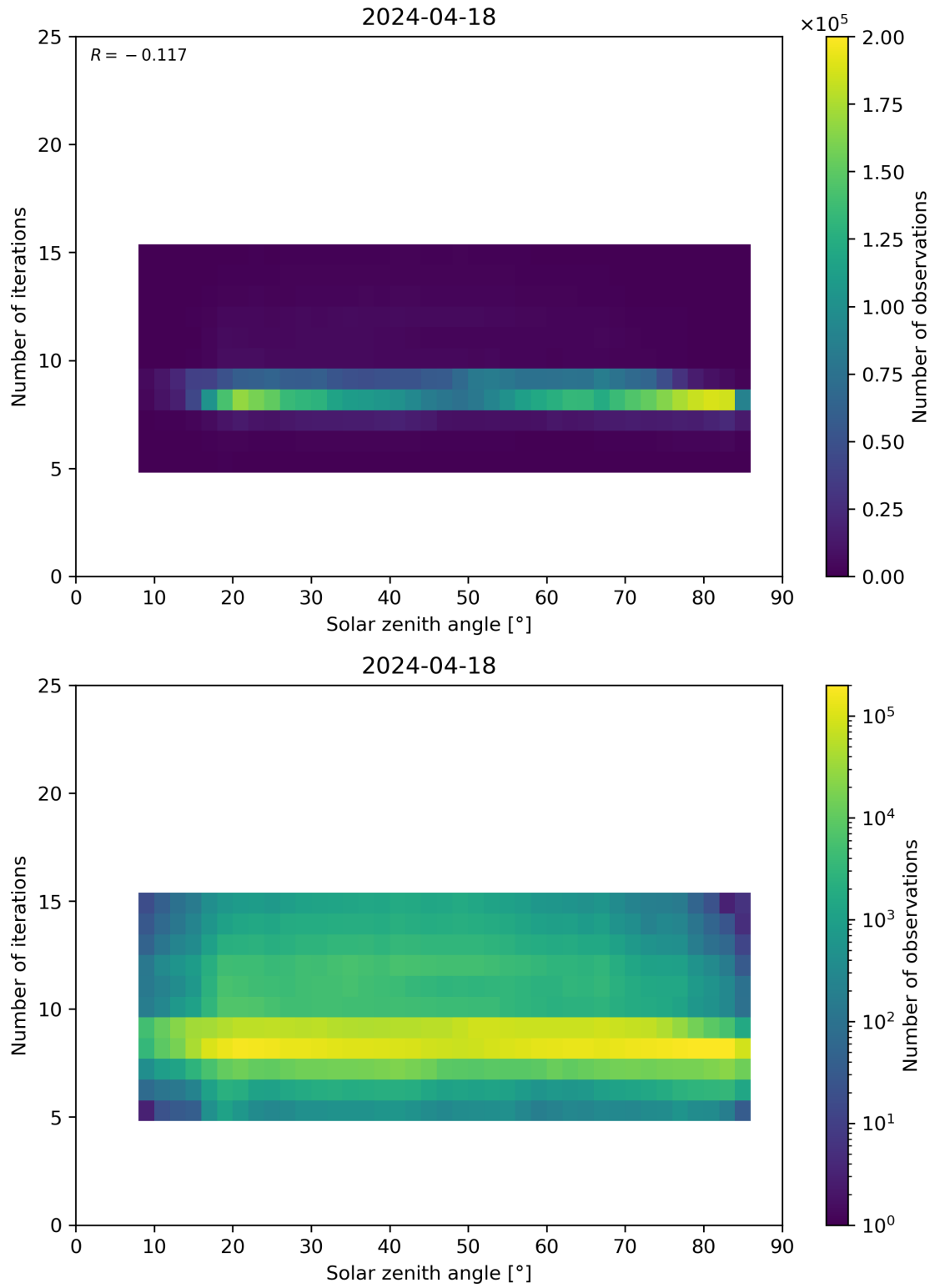
Figure 67: Scatter density plot of “Solar zenith angle” against “Number of iterations” for 2024-04-17 to 2024-04-19.
