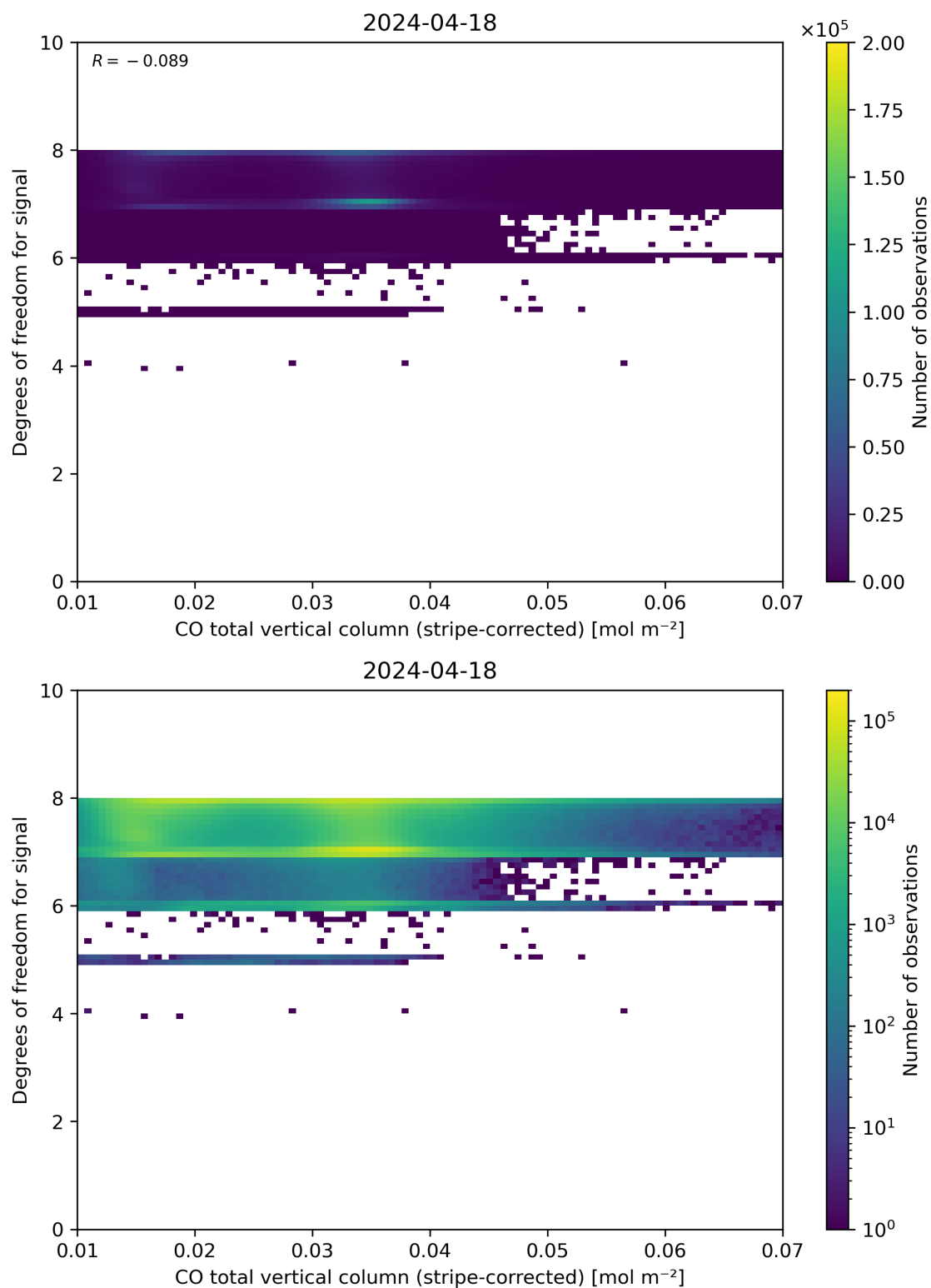
Figure 38: Scatter density plot of “CO total vertical column (stripe-corrected)” against “Degrees of freedom for signal” for 2024-04-17 to 2024-04-19.
