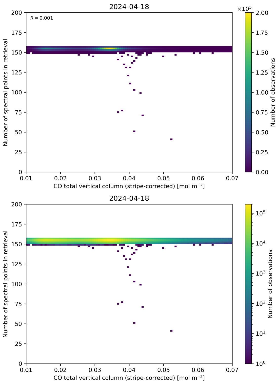
Figure 40: Scatter density plot of “CO total vertical column (stripe-corrected)” against “Number of spectral points in retrieval” for 2024-04-17 to 2024-04-19.
