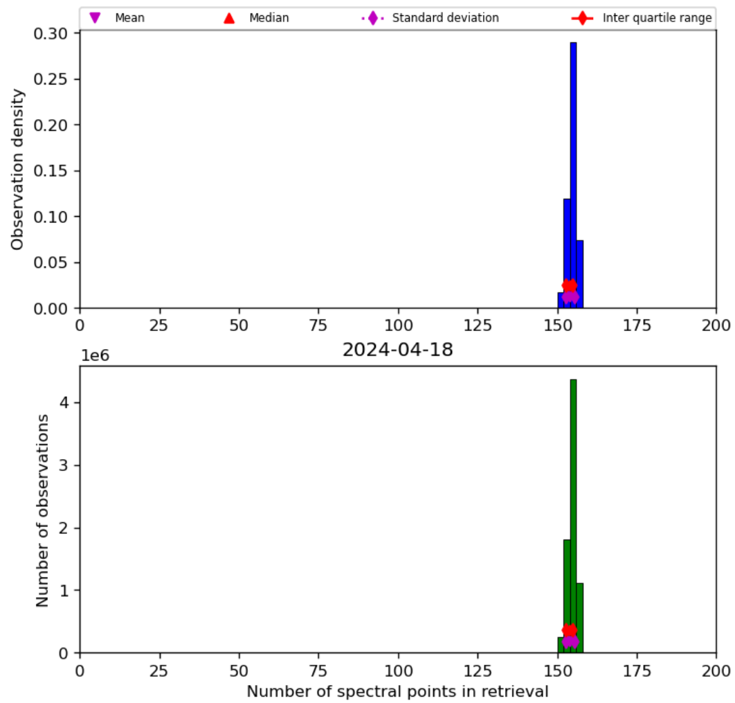
Figure 21: Histogram of “Number of spectral points in retrieval” for 2024-04-17 to 2024-04-19
