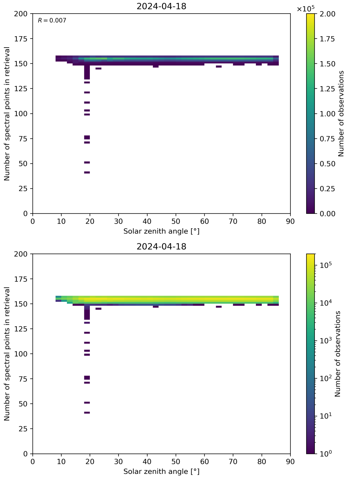
Figure 68: Scatter density plot of “Solar zenith angle” against “Number of spectral points in retrieval” for 2024-04-17 to 2024-04-19.
