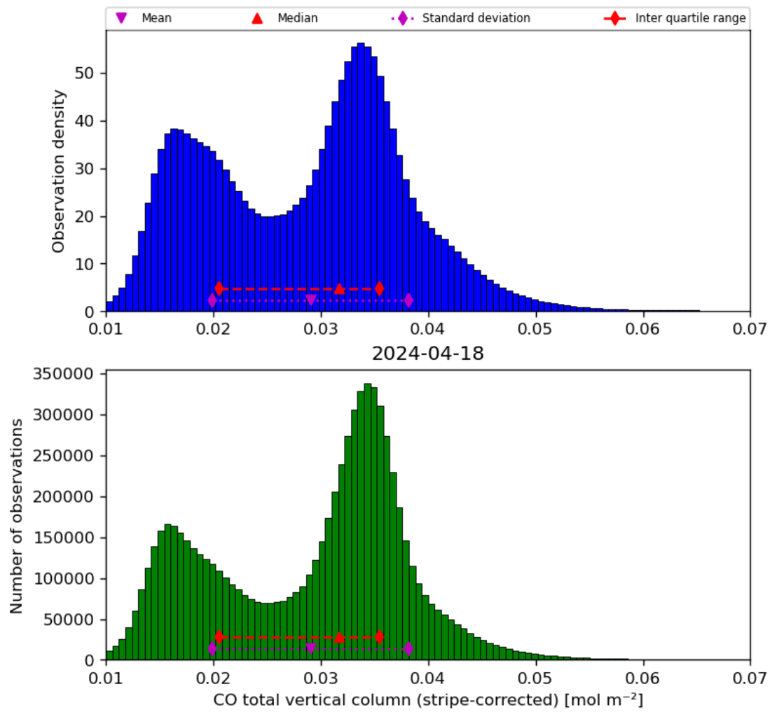
Figure 19: Histogram of “CO total vertical column (stripe-corrected)” for 2024-04-17 to 2024-04-19
