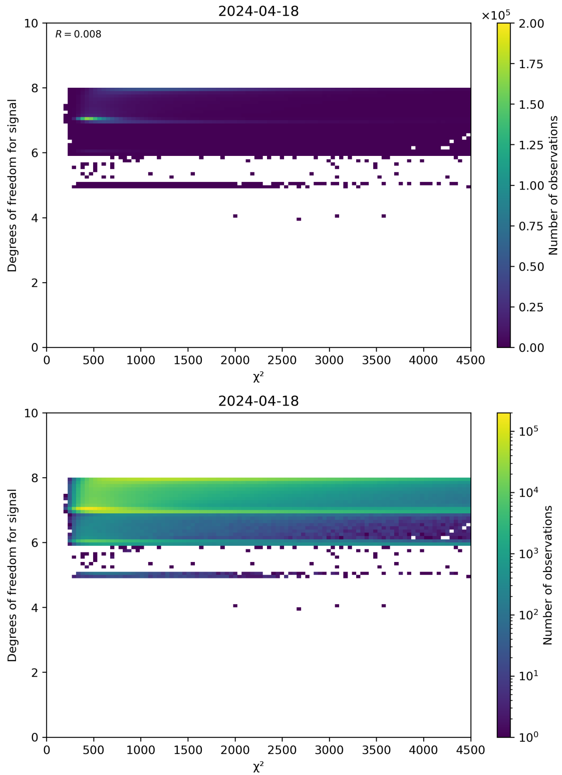
Figure 48: Scatter density plot of “ \chi^2 ” against “Degrees of freedom for signal” for 2024-04-17 to 2024-04-19.
