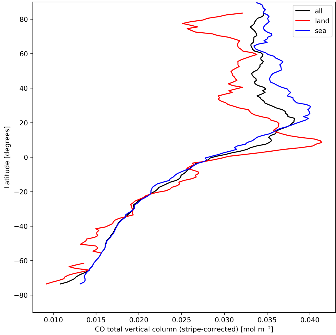
Figure 11: Zonal average of “CO total vertical column (stripe-corrected)” for 2024-04-17 to 2024-04-19.
