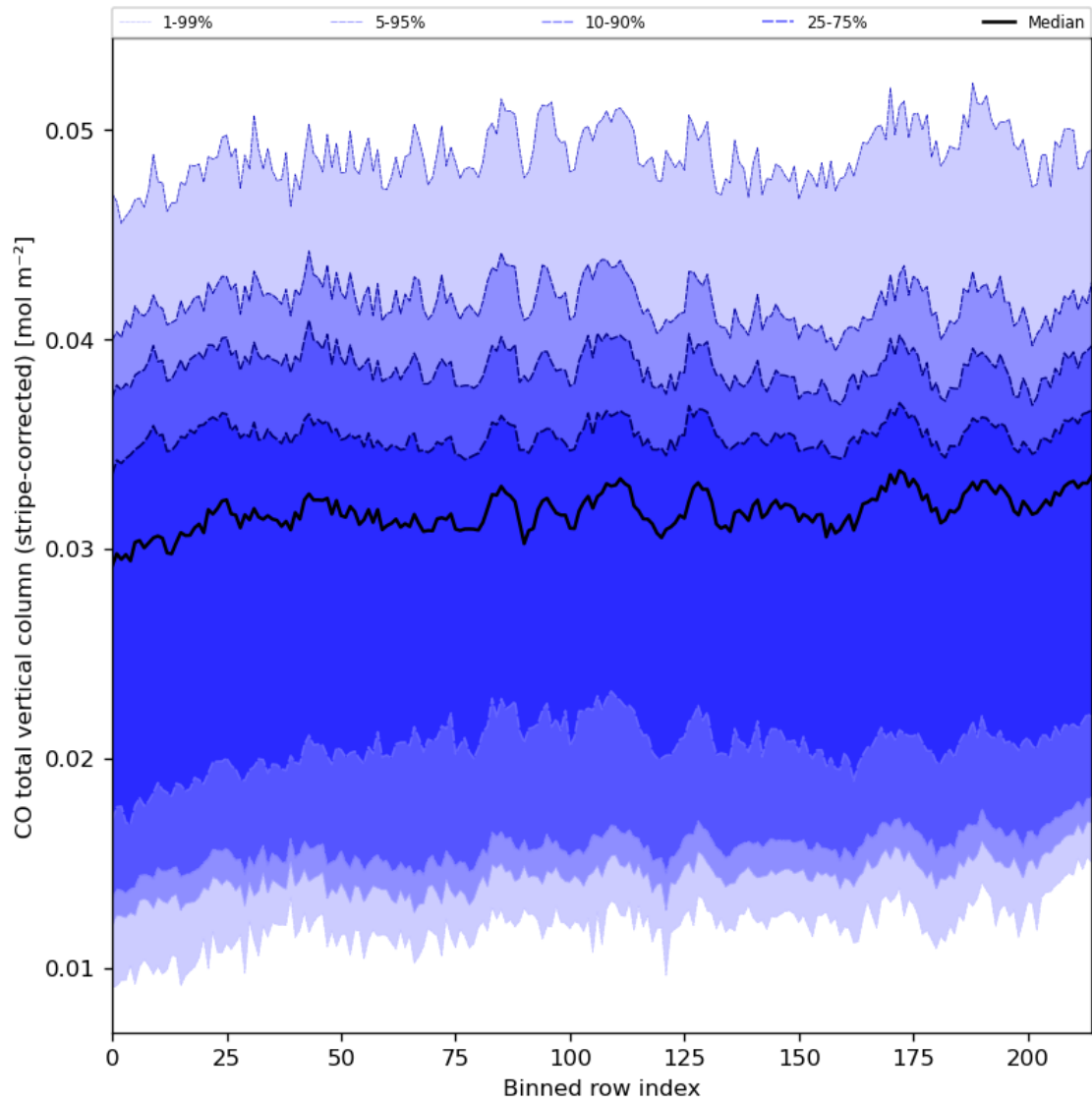
Figure 27: Along track statistics of “CO total vertical column (stripe-corrected)” for 2024-04-17 to 2024-04-19
