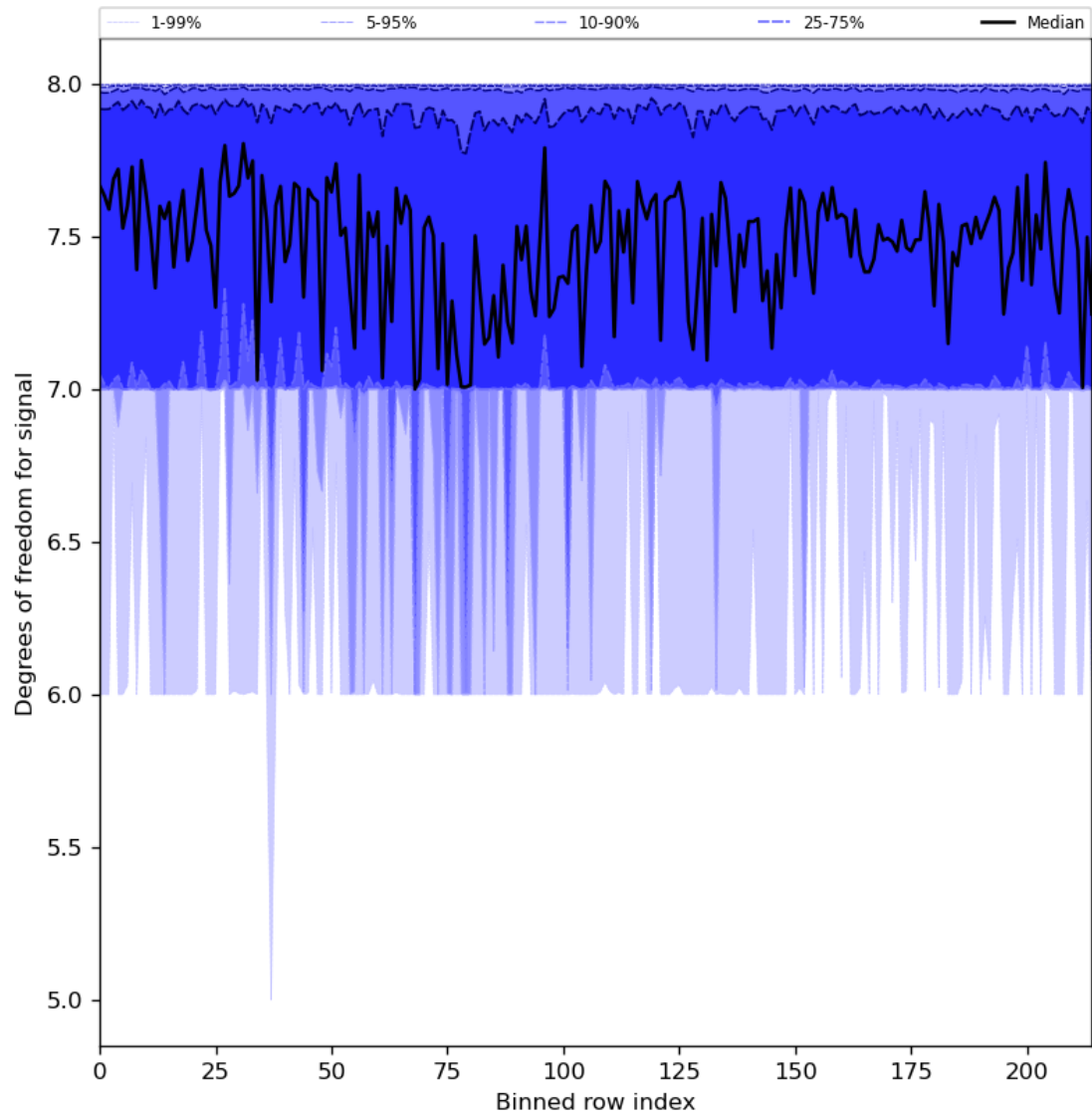
Figure 31: Along track statistics of “Degrees of freedom for signal” for 2024-04-17 to 2024-04-19
