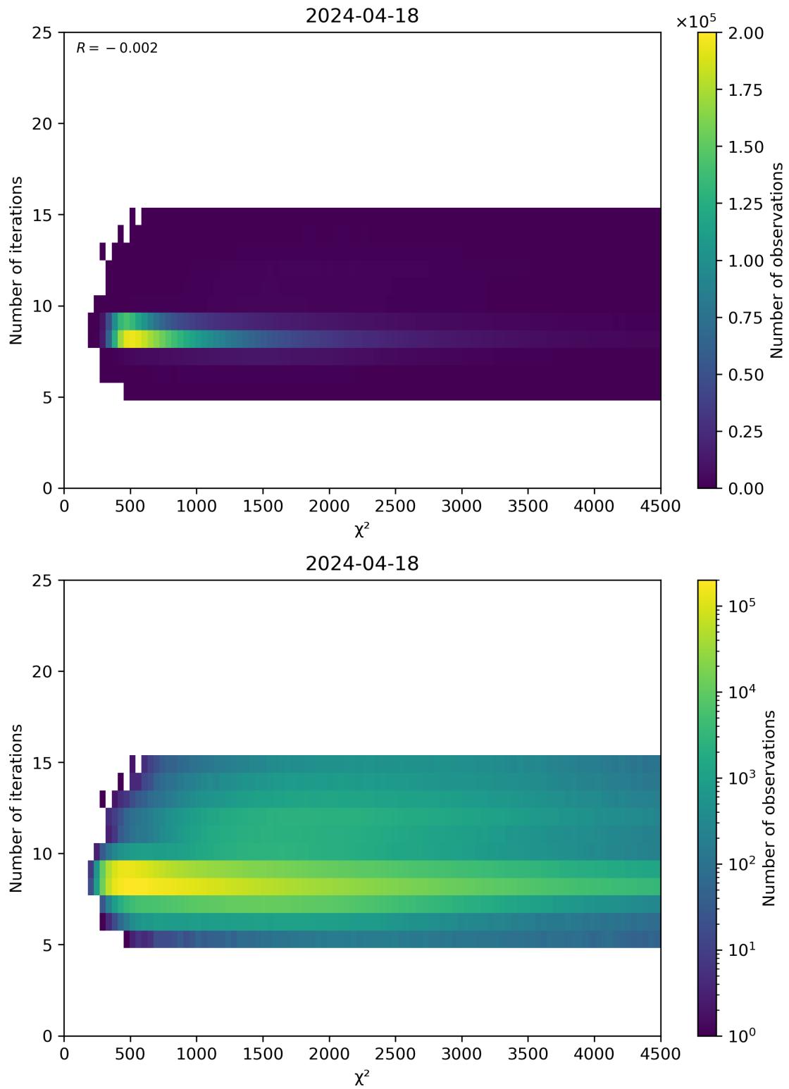
Figure 49: Scatter density plot of “ \chi^2 ” against “Number of iterations” for 2024-04-17 to 2024-04-19.
