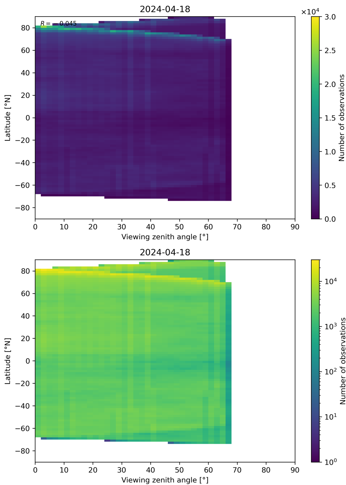
Figure 74: Scatter density plot of “Viewing zenith angle” against “Latitude” for 2024-04-17 to 2024-04-19.
