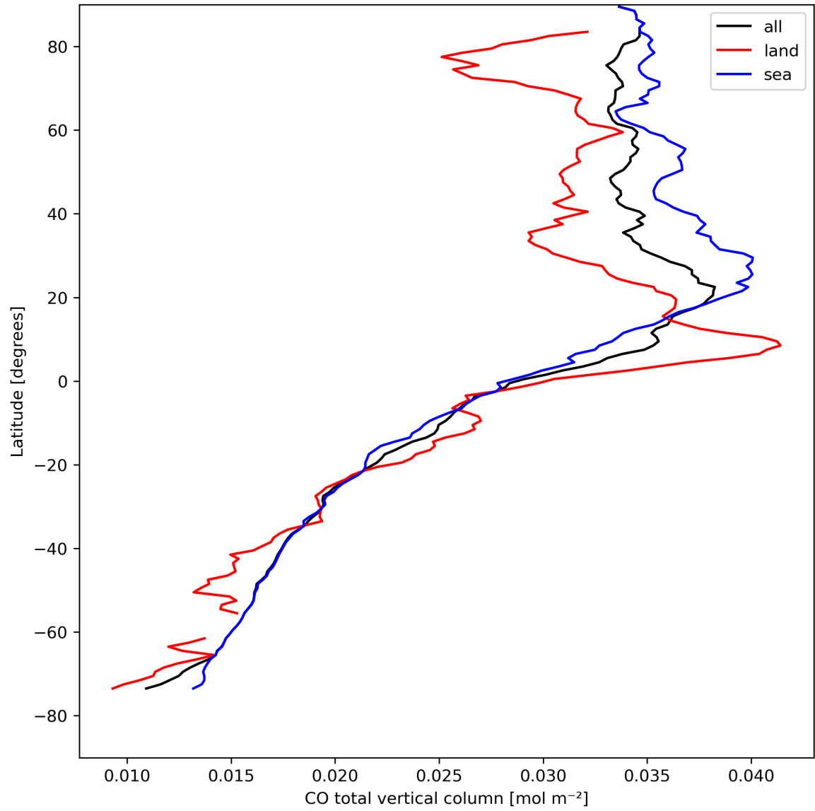
Figure 10: Zonal average of “CO total vertical column” for 2024-04-17 to 2024-04-19.
