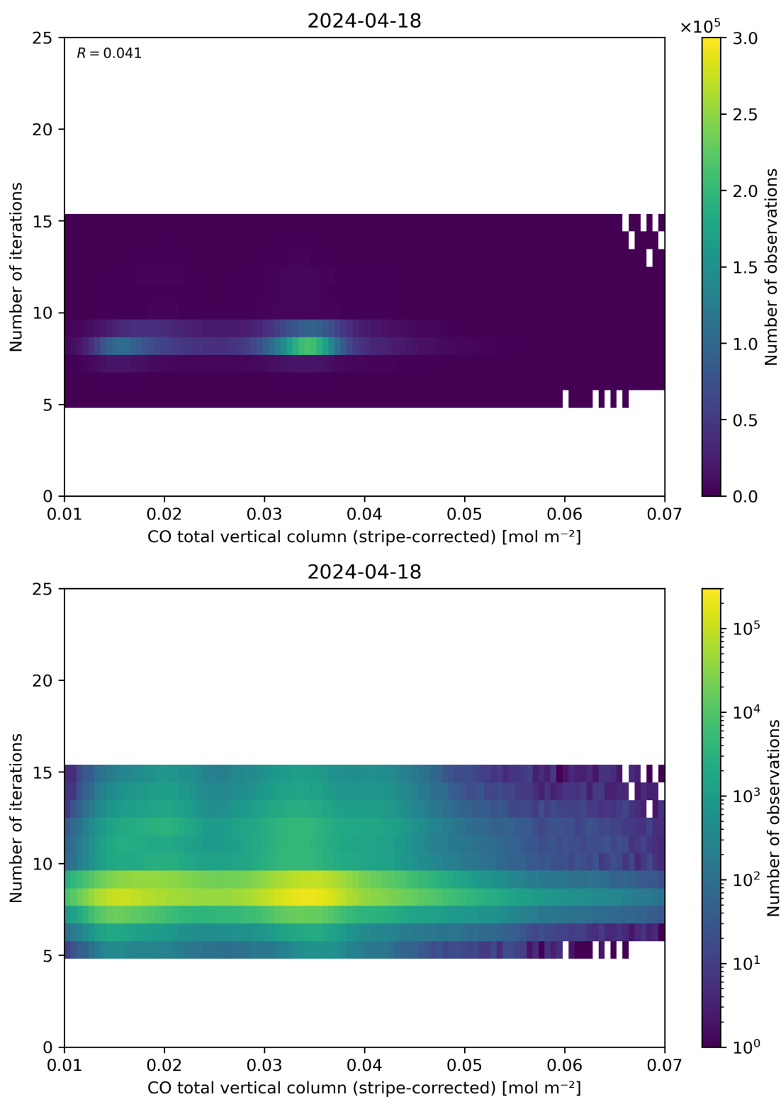
Figure 39: Scatter density plot of “CO total vertical column (stripe-corrected)” against “Number of iterations” for 2024-04-17 to 2024-04-19.
