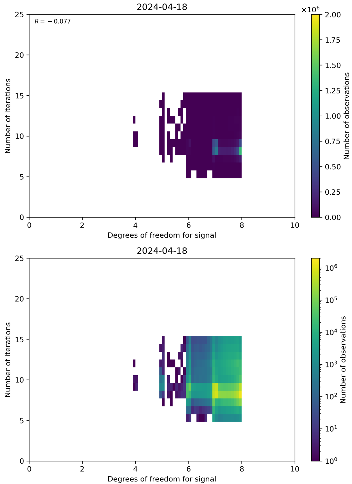
Figure 50: Scatter density plot of “Degrees of freedom for signal” against “Number of iterations” for 2024-04-17 to 2024-04-19.
