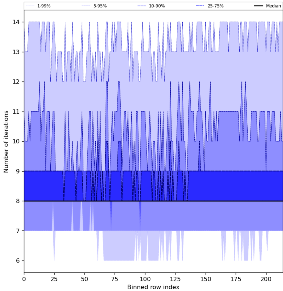
Figure 32: Along track statistics of “Number of iterations” for 2024-04-17 to 2024-04-19
