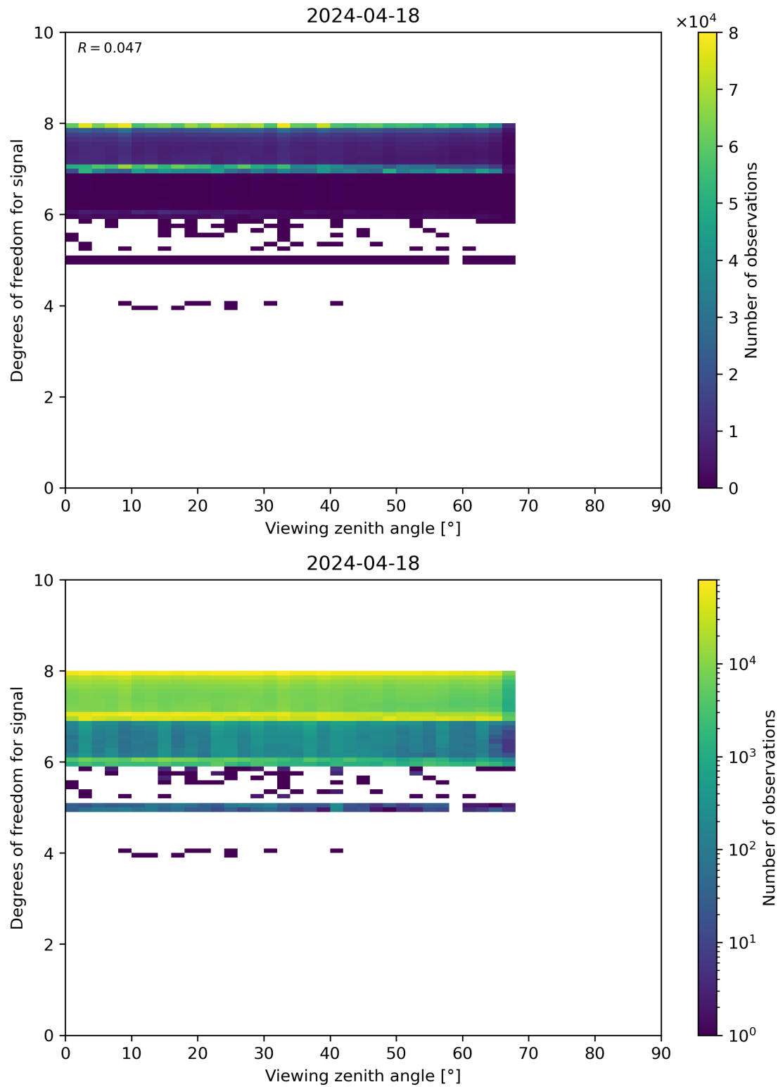
Figure 73: Scatter density plot of “Viewing zenith angle” against “Degrees of freedom for signal” for 2024-04-17 to 2024-04-19.
