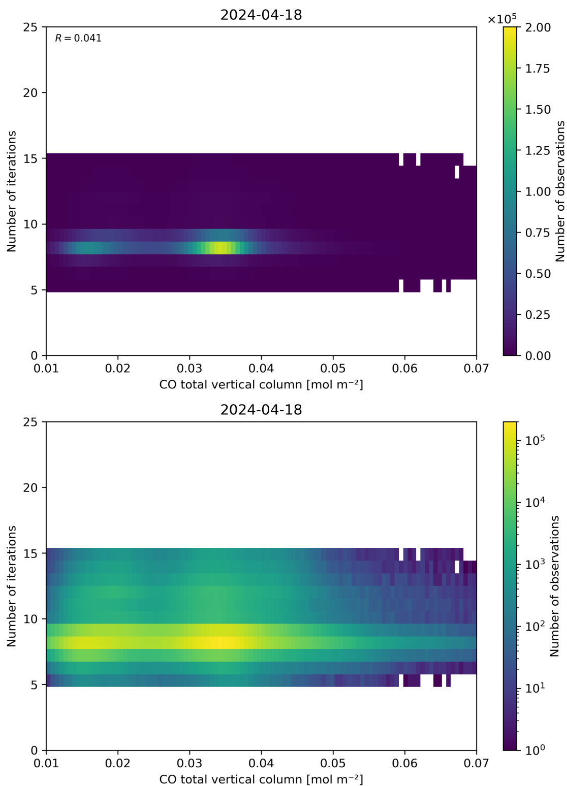
Figure 42: Scatter density plot of “CO total vertical column” against “Number of iterations” for 2024-04-17 to 2024-04-19.
