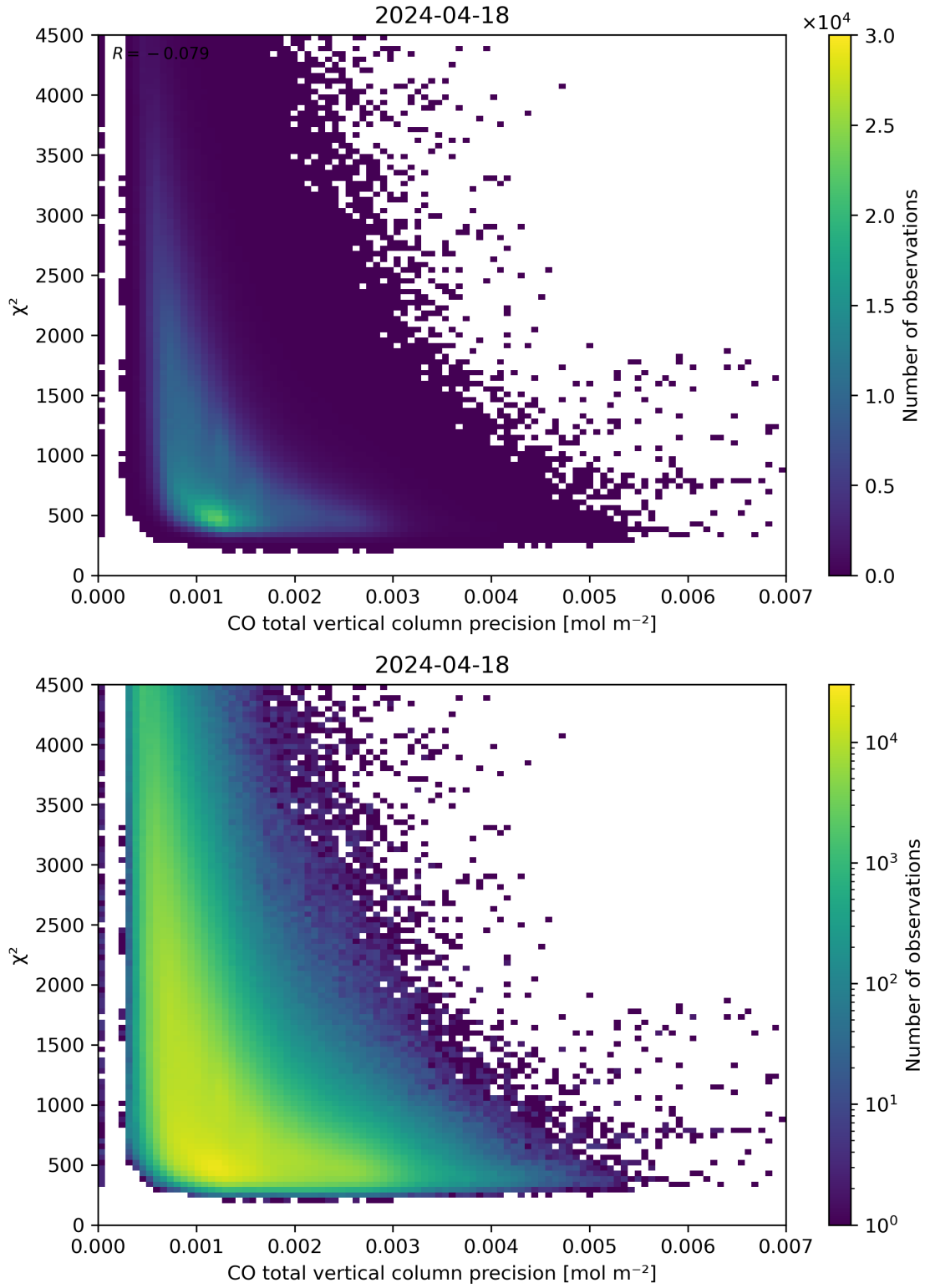
Figure 44: Scatter density plot of “CO total vertical column precision” against “ \chi^2 ” for 2024-04-17 to 2024-04-19.
