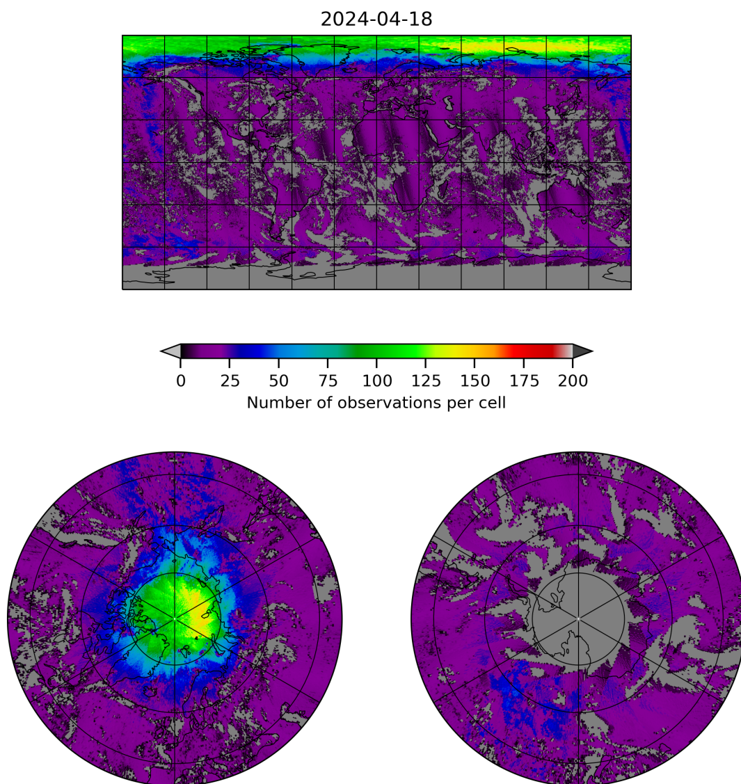
Figure 8: Map of the number of observations for 2024-04-17 to 2024-04-19
