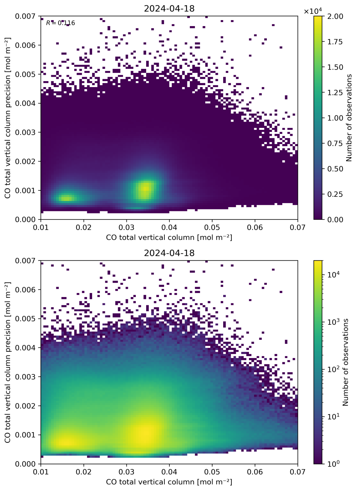
Figure 34: Scatter density plot of “CO total vertical column” against “CO total vertical column precision” for 2024-04-17 to 2024-04-19.
