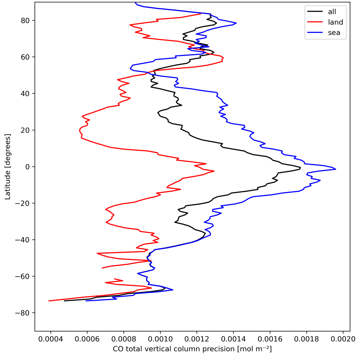
Figure 12: Zonal average of “CO total vertical column precision” for 2024-04-17 to 2024-04-19.
