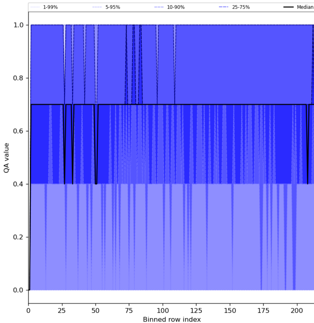
Figure 25: Along track statistics of “QA value” for 2024-04-17 to 2024-04-19
