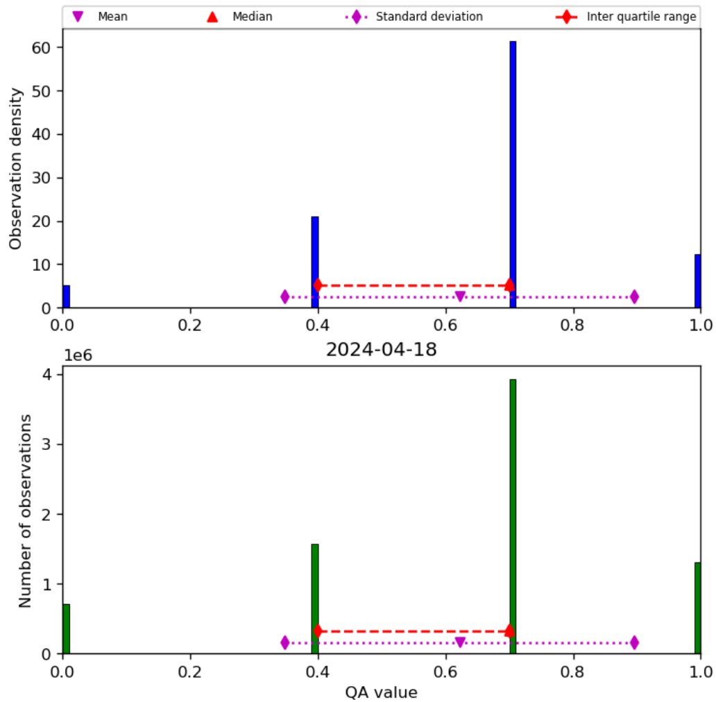
Figure 17: Histogram of “QA value” for 2024-04-17 to 2024-04-19
