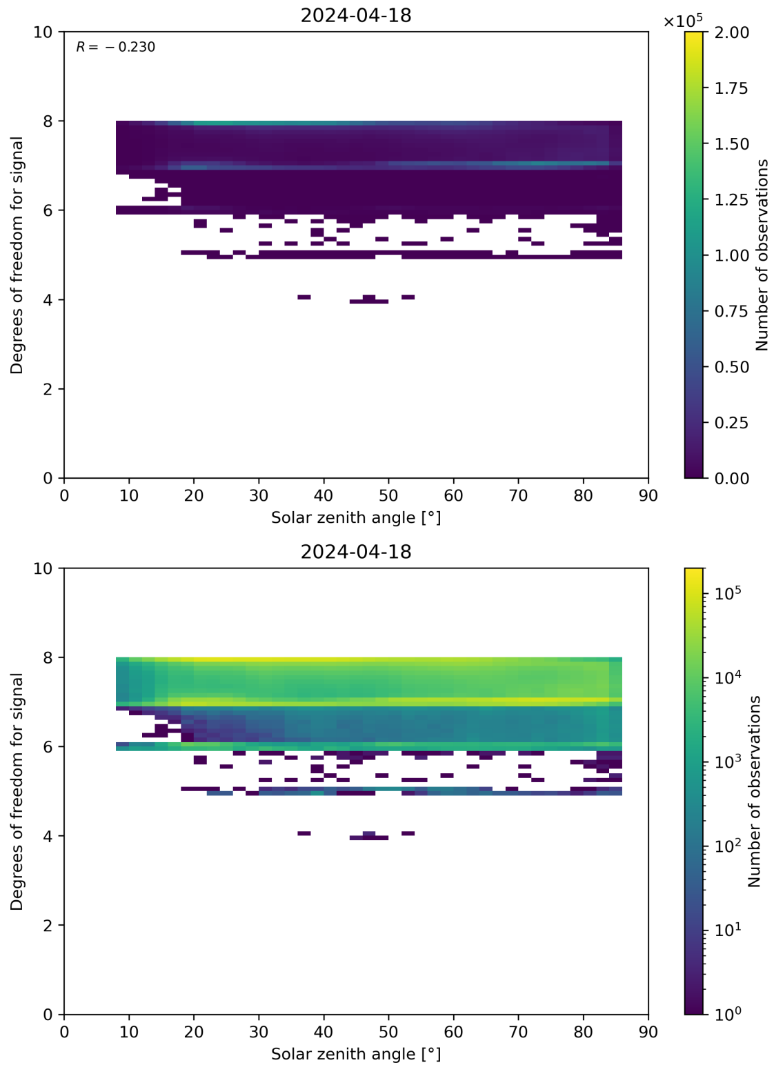
Figure 65: Scatter density plot of “Solar zenith angle” against “Degrees of freedom for signal” for 2024-04-17 to 2024-04-19.
