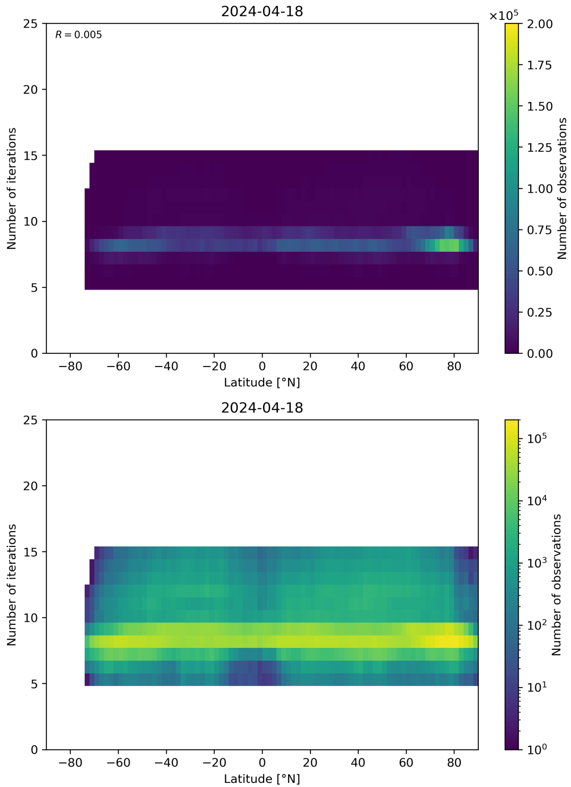
Figure 56: Scatter density plot of “Latitude” against “Number of iterations” for 2024-04-17 to 2024-04-19.
