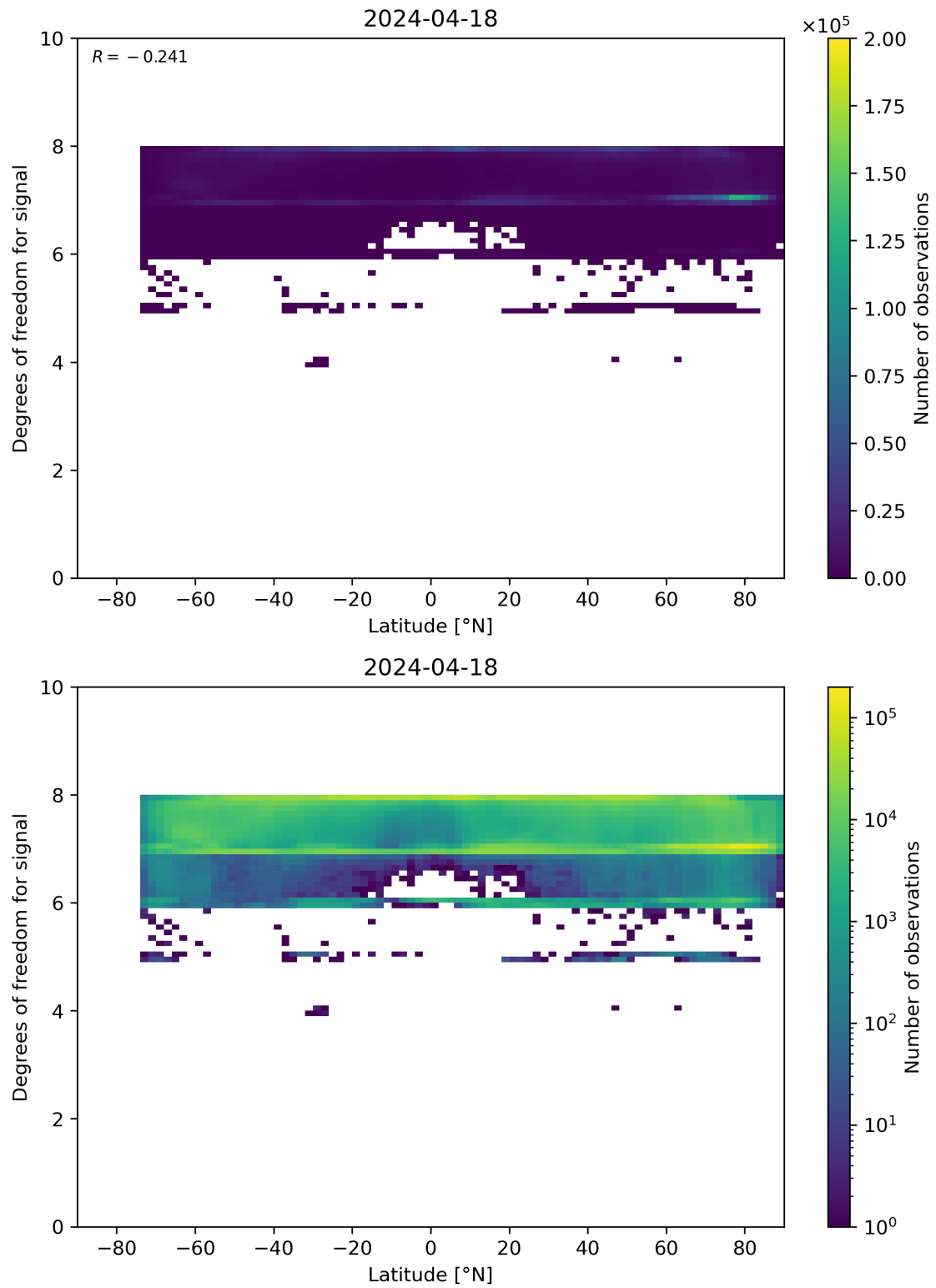
Figure 55: Scatter density plot of “Latitude” against “Degrees of freedom for signal” for 2024-04-17 to 2024-04-19.
