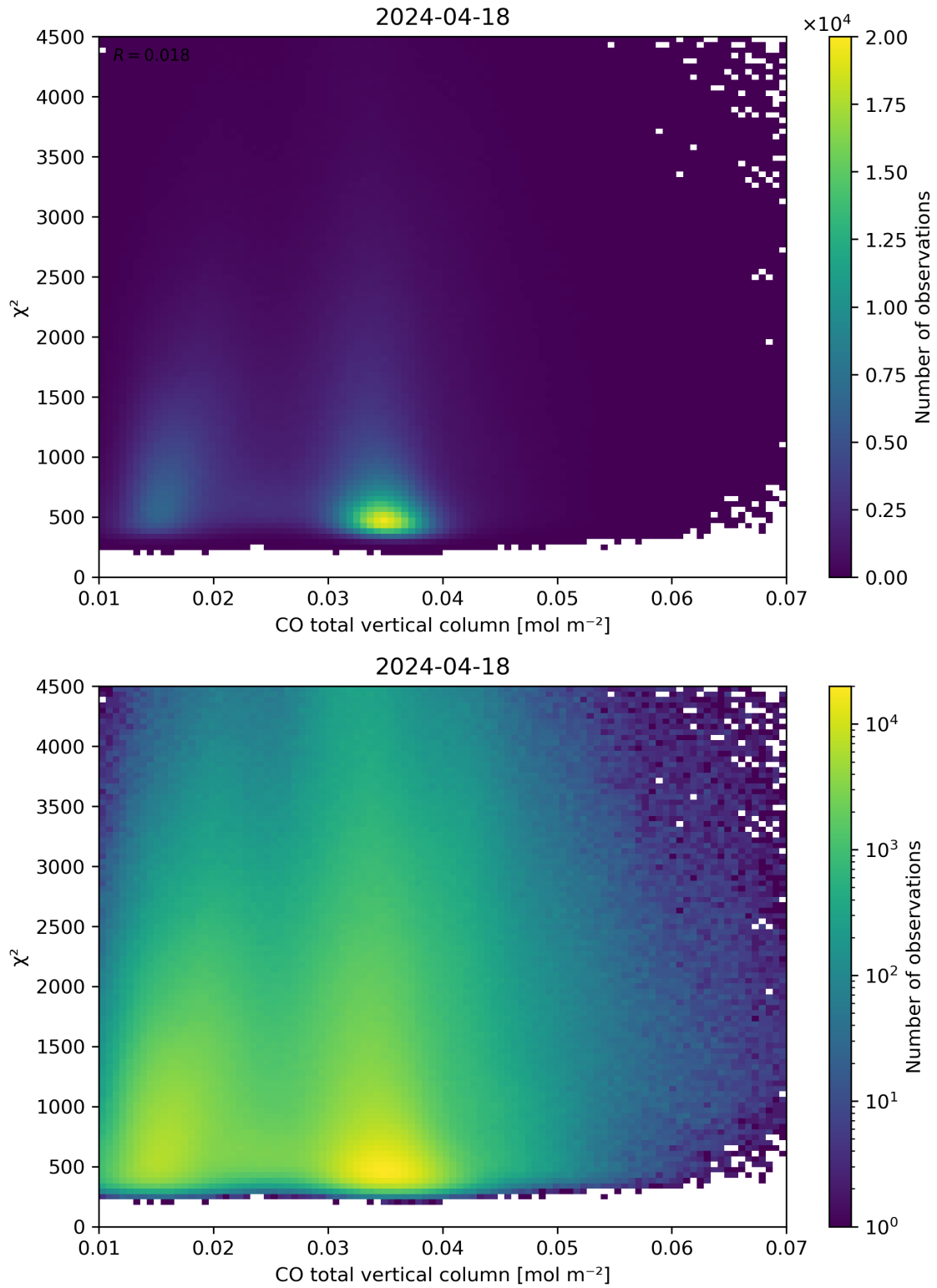
Figure 35: Scatter density plot of “CO total vertical column” against “ \chi^2 ” for 2024-04-17 to 2024-04-19.
