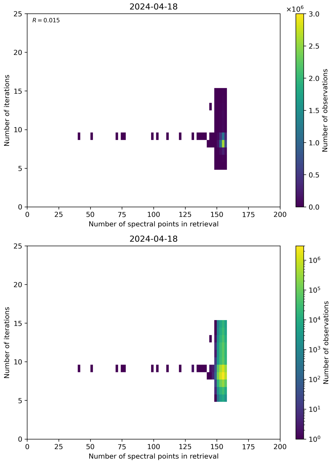
Figure 60: Scatter density plot of “Number of spectral points in retrieval” against “Number of iterations” for 2024-04-17 to 2024-04-19.
