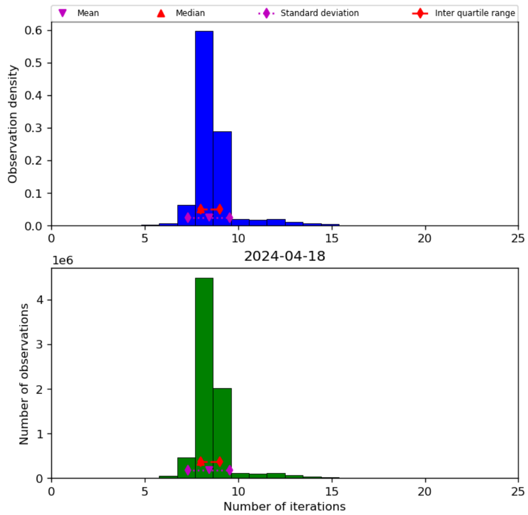
Figure 24: Histogram of “Number of iterations” for 2024-04-17 to 2024-04-19
