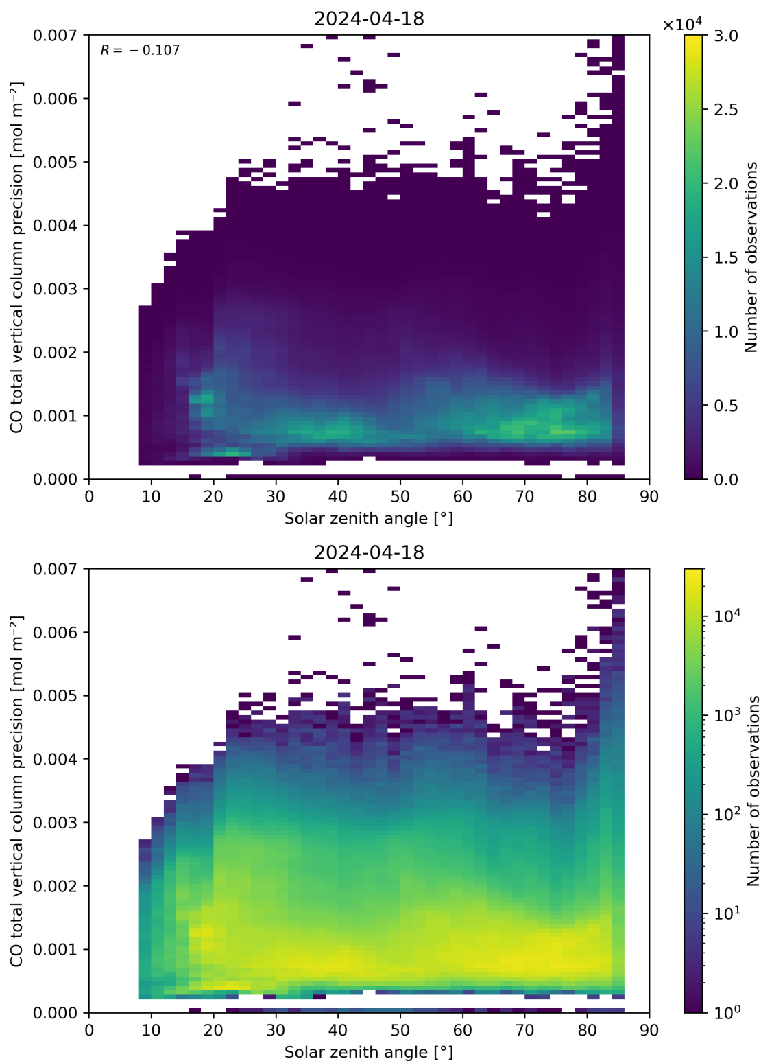
Figure 63: Scatter density plot of “Solar zenith angle” against “CO total vertical column precision” for 2024-04-17 to 2024-04-19.
