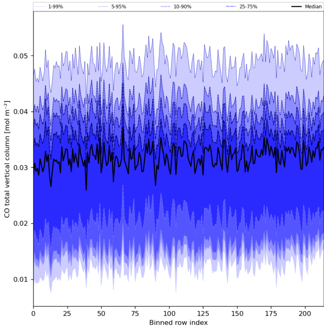
Figure 26: Along track statistics of “CO total vertical column” for 2024-04-17 to 2024-04-19
