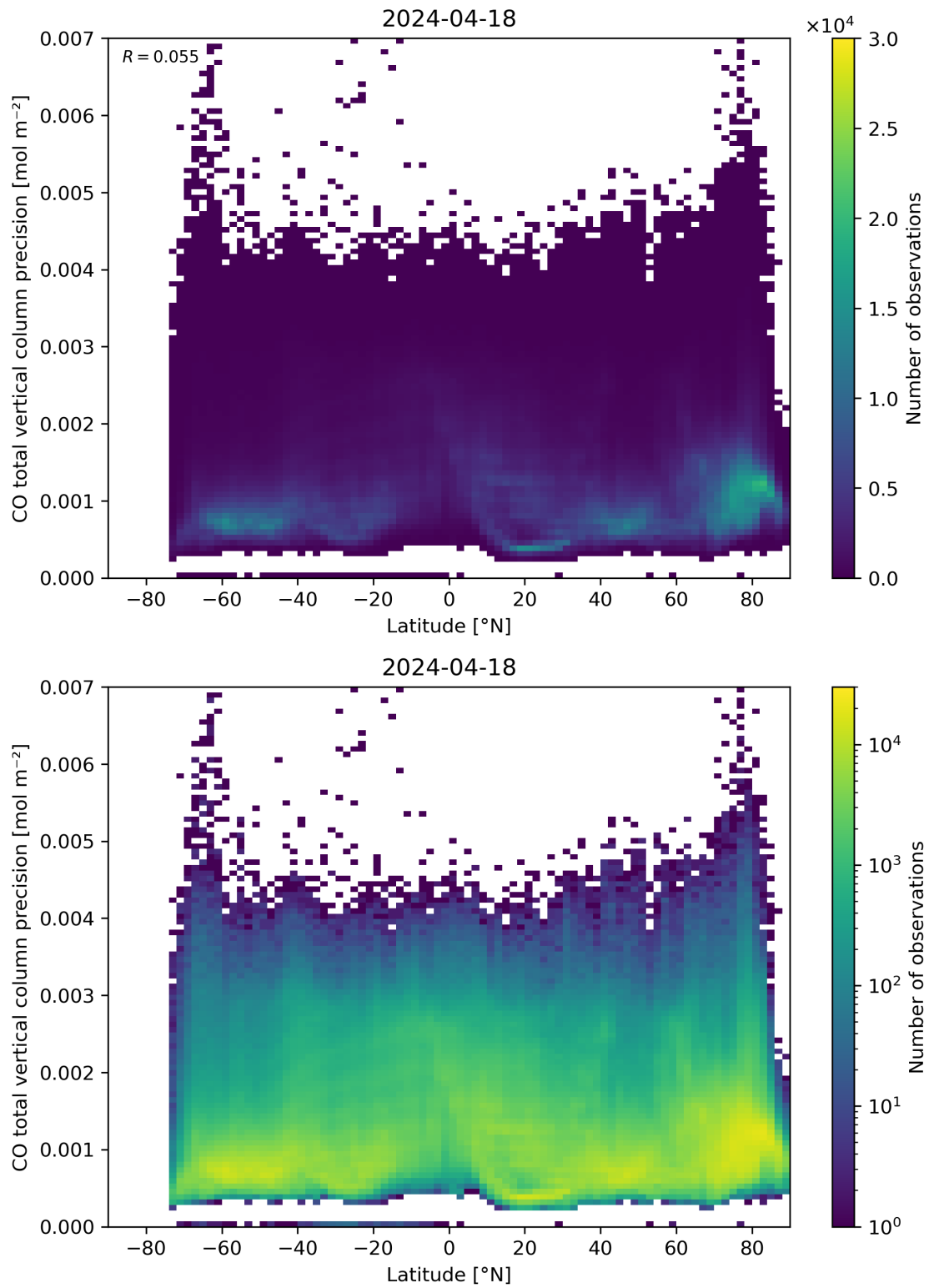
Figure 53: Scatter density plot of “Latitude” against “CO total vertical column precision” for 2024-04-17 to 2024-04-19.
