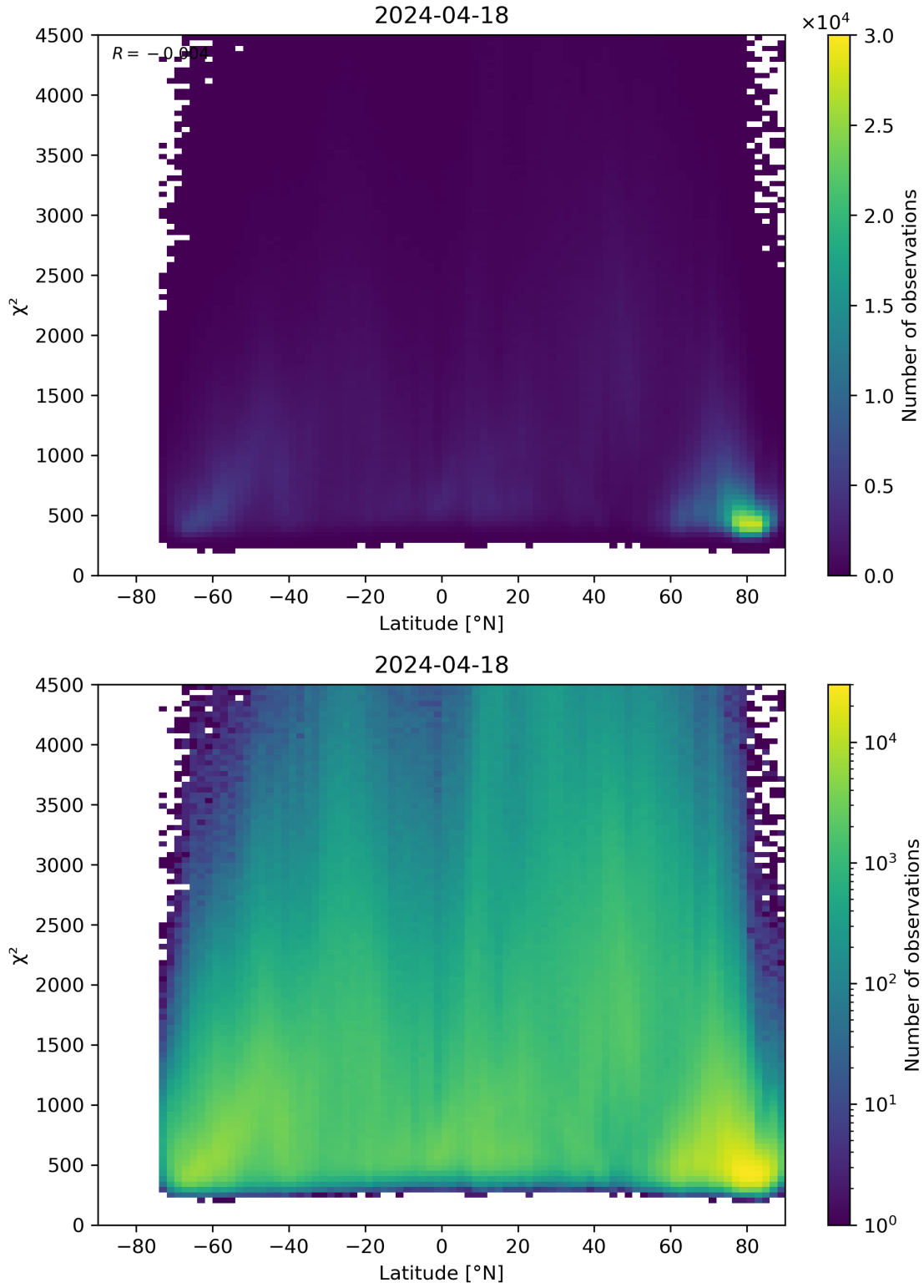
Figure 54: Scatter density plot of “Latitude” against “ \chi^2 ” for 2024-04-17 to 2024-04-19.
