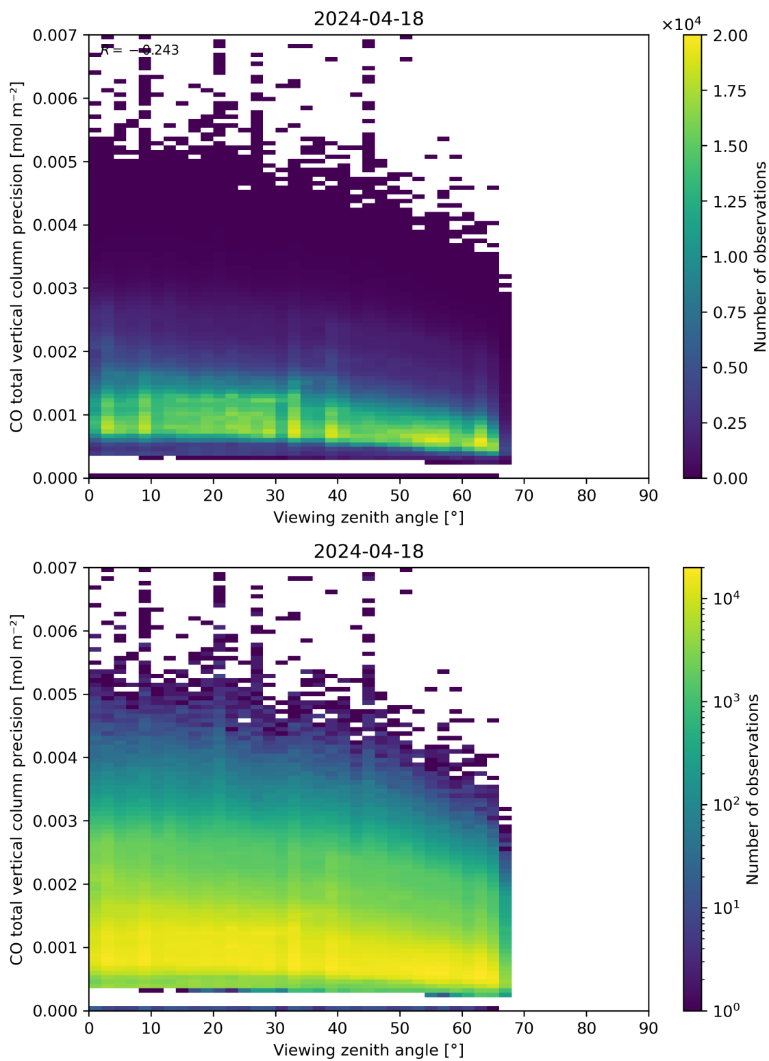
Figure 71: Scatter density plot of “Viewing zenith angle” against “CO total vertical column precision” for 2024-04-17 to 2024-04-19.
