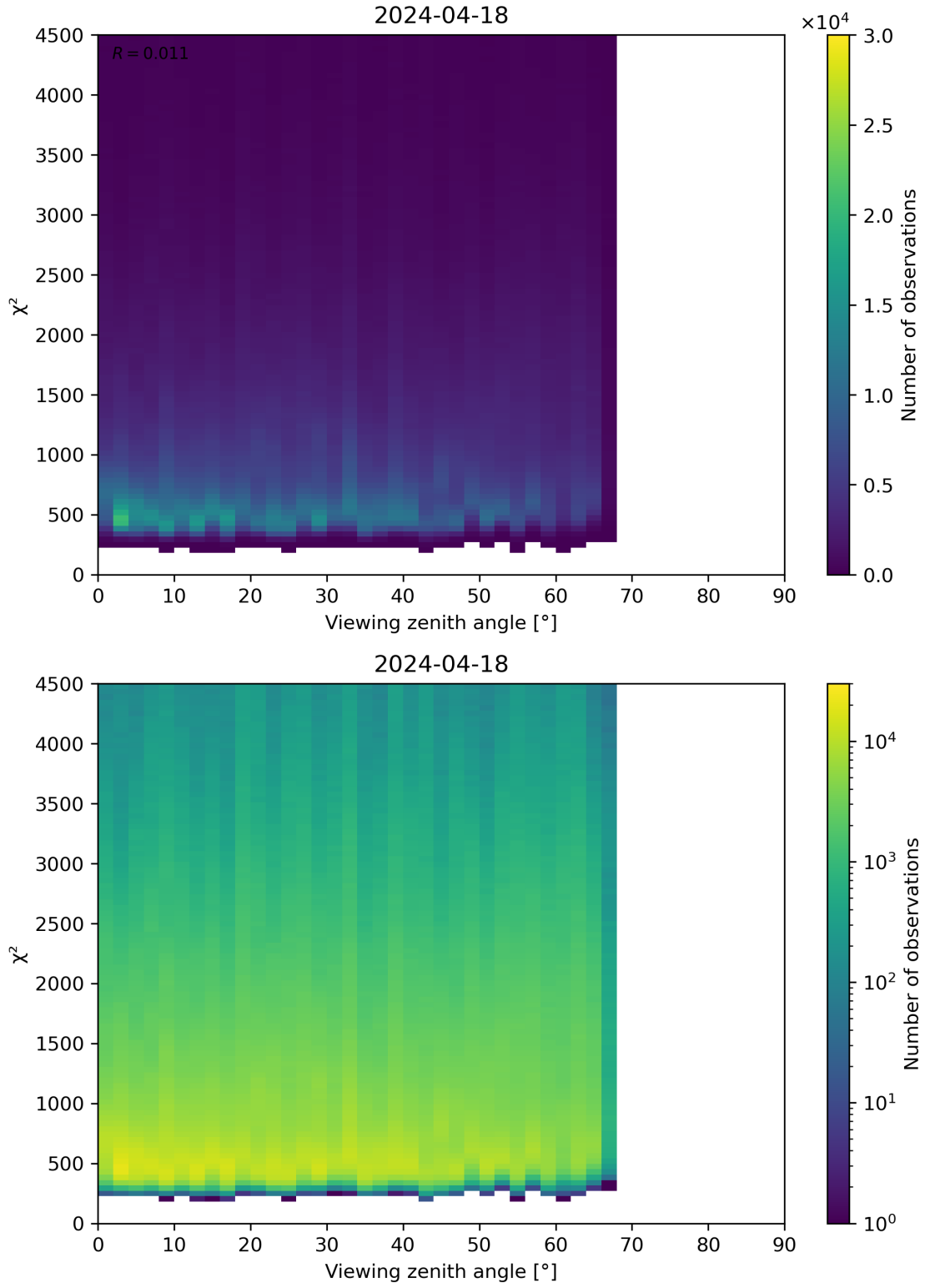
Figure 72: Scatter density plot of “Viewing zenith angle” against “ \chi^2 ” for 2024-04-17 to 2024-04-19.
