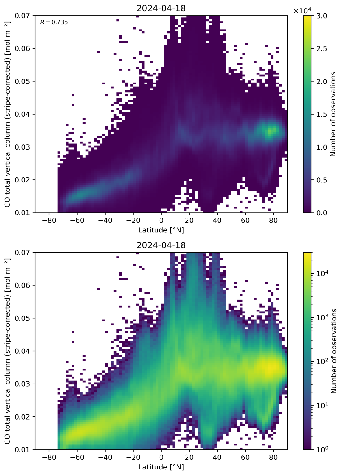
Figure 52: Scatter density plot of “Latitude” against “CO total vertical column (stripe-corrected)” for 2024-04-17 to 2024-04-19.
