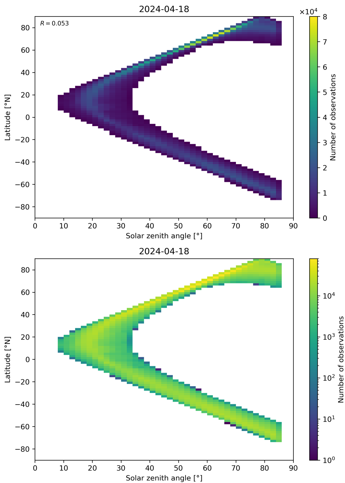
Figure 66: Scatter density plot of “Solar zenith angle” against “Latitude” for 2024-04-17 to 2024-04-19.
