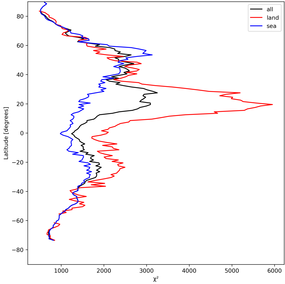
Figure 14: Zonal average of “ \chi^2 ” for 2024-04-17 to 2024-04-19.
