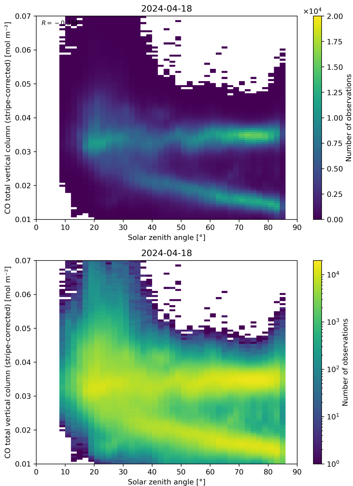
Figure 62: Scatter density plot of “Solar zenith angle” against “CO total vertical column (stripe-corrected)” for 2024-04-17 to 2024-04-19.
