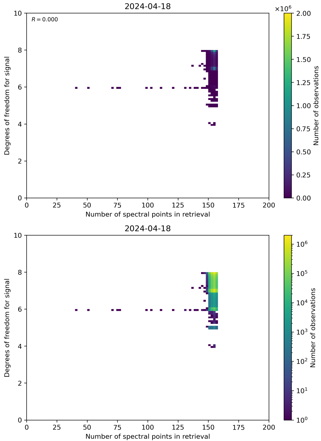
Figure 59: Scatter density plot of “Number of spectral points in retrieval” against “Degrees of freedom for signal” for 2024-04-17 to 2024-04-19.
