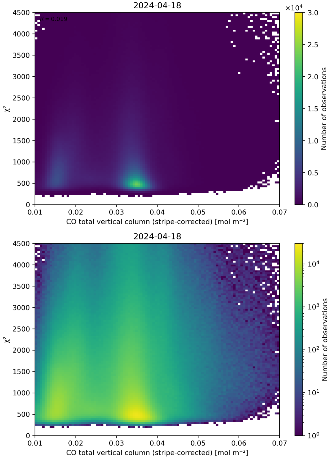
Figure 37: Scatter density plot of “CO total vertical column (stripe-corrected)” against “ \chi^2 ” for 2024-04-17 to 2024-04-19.
