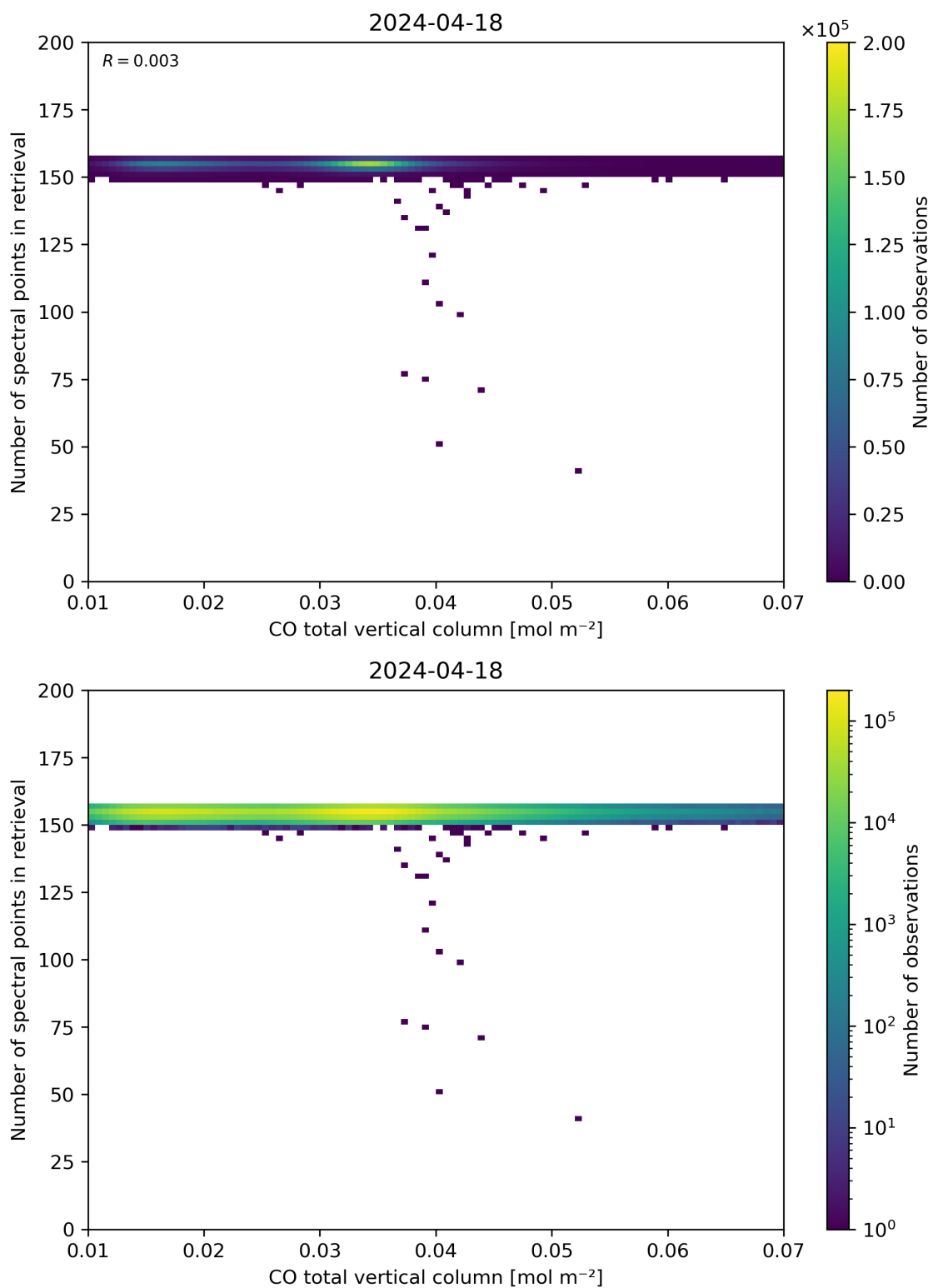
Figure 43: Scatter density plot of “CO total vertical column” against “Number of spectral points in retrieval” for 2024-04-17 to 2024-04-19.
