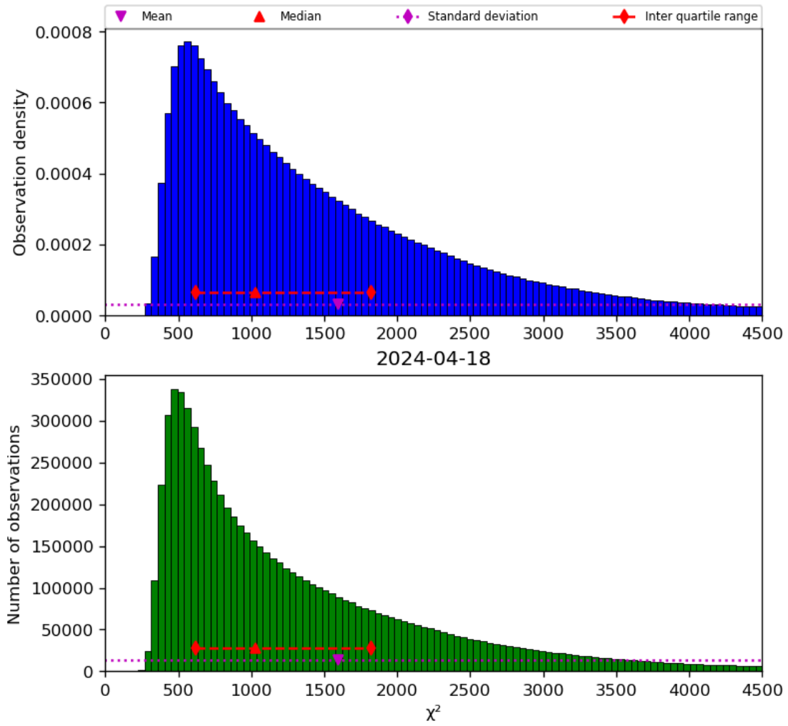
Figure 22: Histogram of “ \chi^2 ” for 2024-04-17 to 2024-04-19
