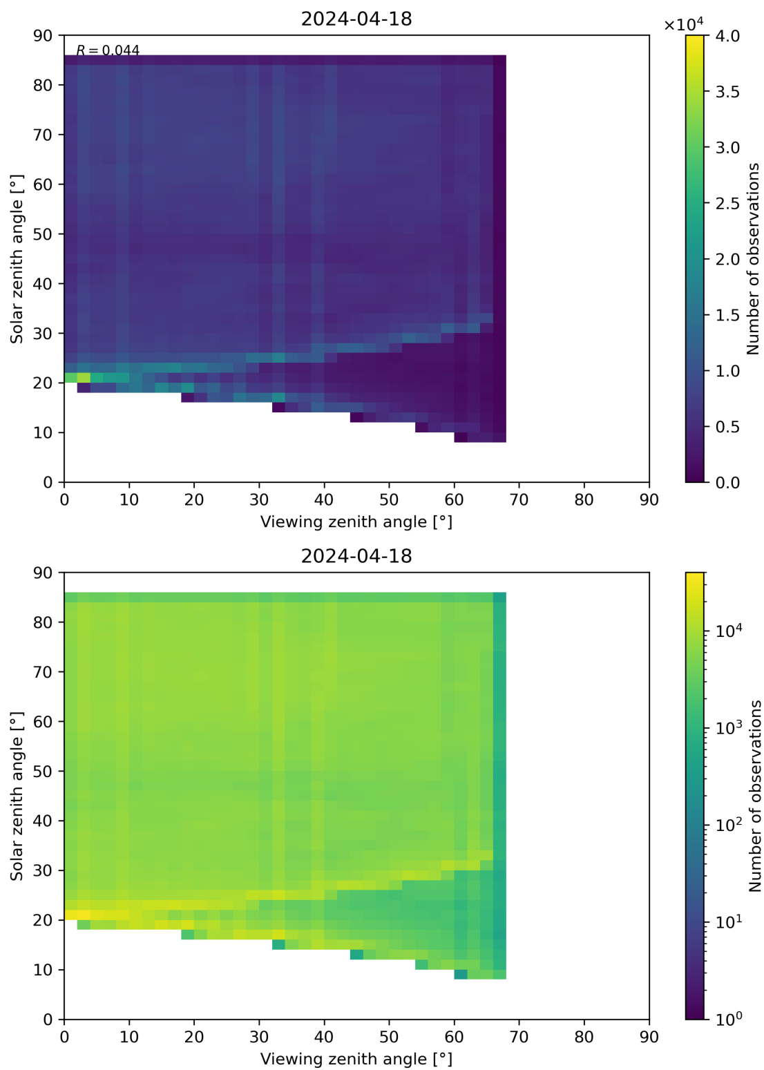
Figure 77: Scatter density plot of “Viewing zenith angle” against “Solar zenith angle” for 2024-04-17 to 2024-04-19.
