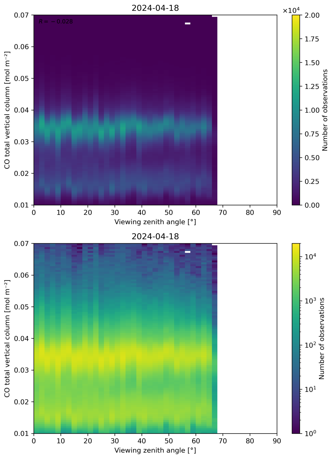
Figure 69: Scatter density plot of “Viewing zenith angle” against “CO total vertical column” for 2024-04-17 to 2024-04-19.
