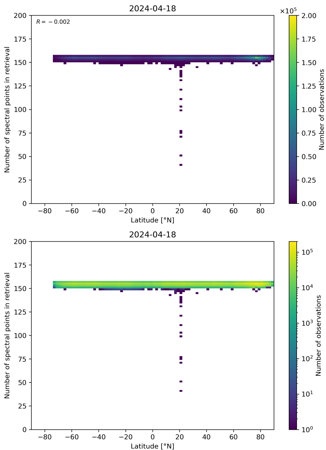
Figure 57: Scatter density plot of “Latitude” against “Number of spectral points in retrieval” for 2024-04-17 to 2024-04-19.
