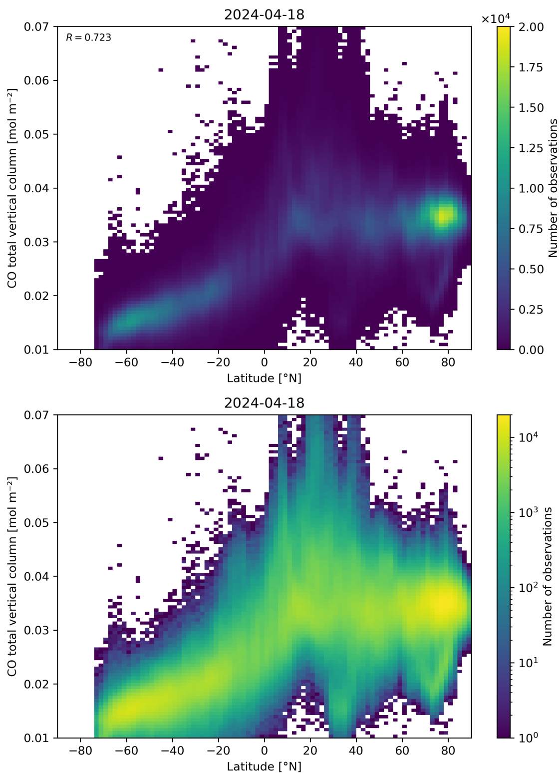
Figure 51: Scatter density plot of “Latitude” against “CO total vertical column” for 2024-04-17 to 2024-04-19.
