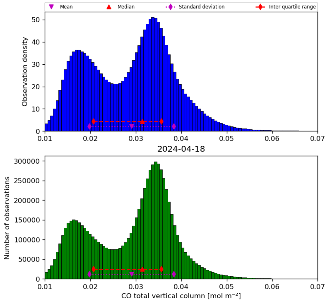
Figure 18: Histogram of “CO total vertical column” for 2024-04-17 to 2024-04-19
