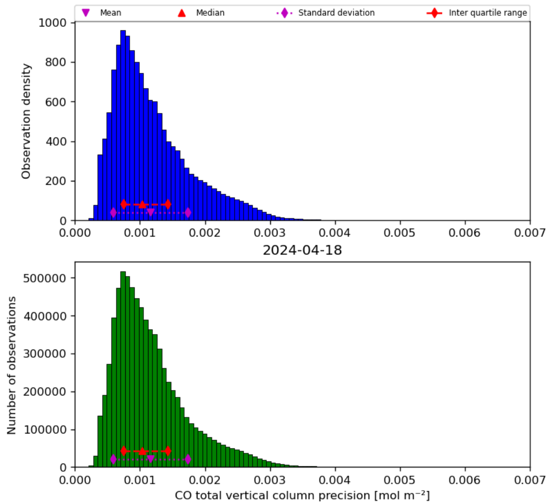
Figure 20: Histogram of “CO total vertical column precision” for 2024-04-17 to 2024-04-19
