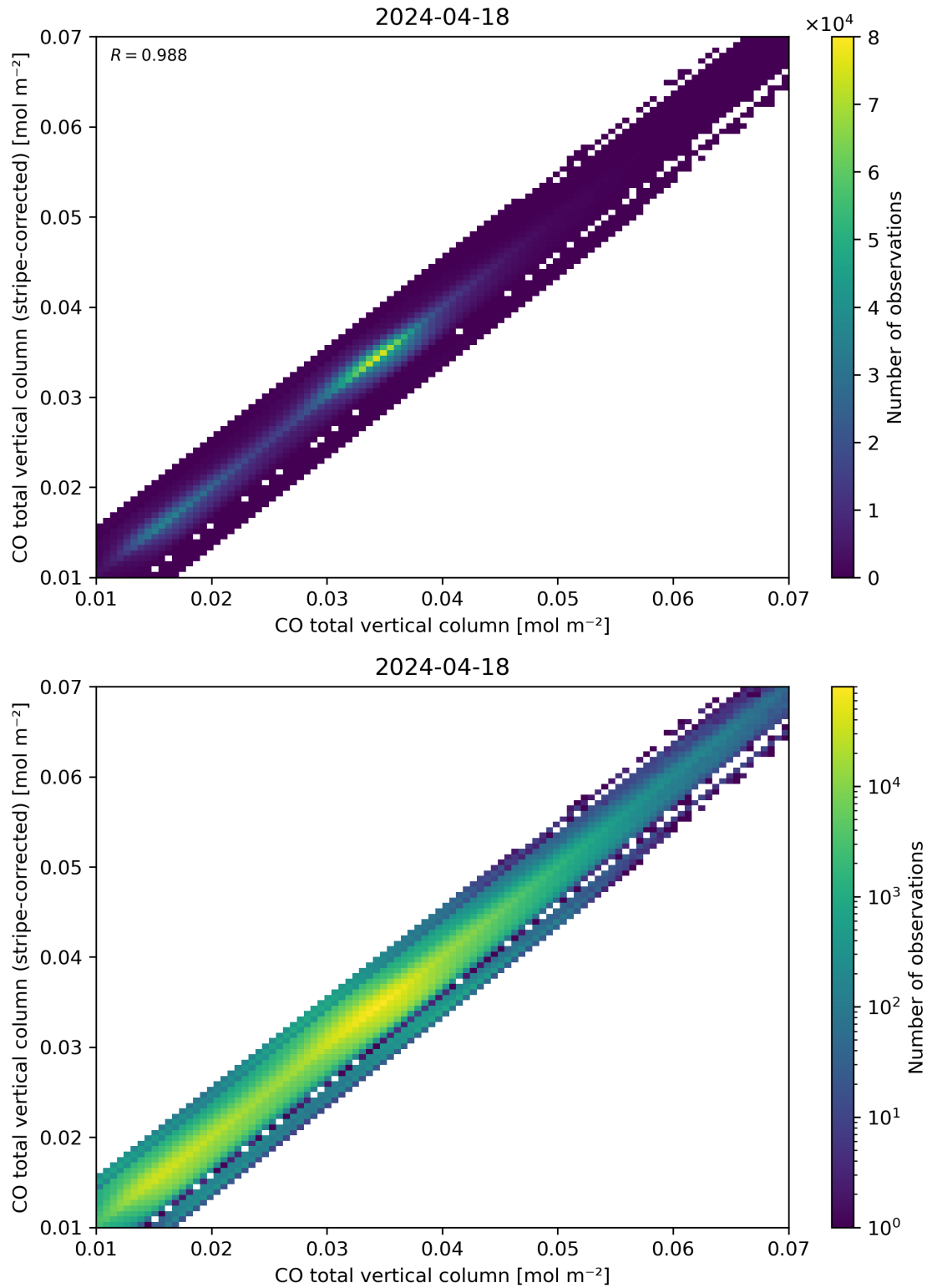
Figure 33: Scatter density plot of “CO total vertical column” against “CO total vertical column (stripe-corrected)” for 2024-04-17 to 2024-04-19.
