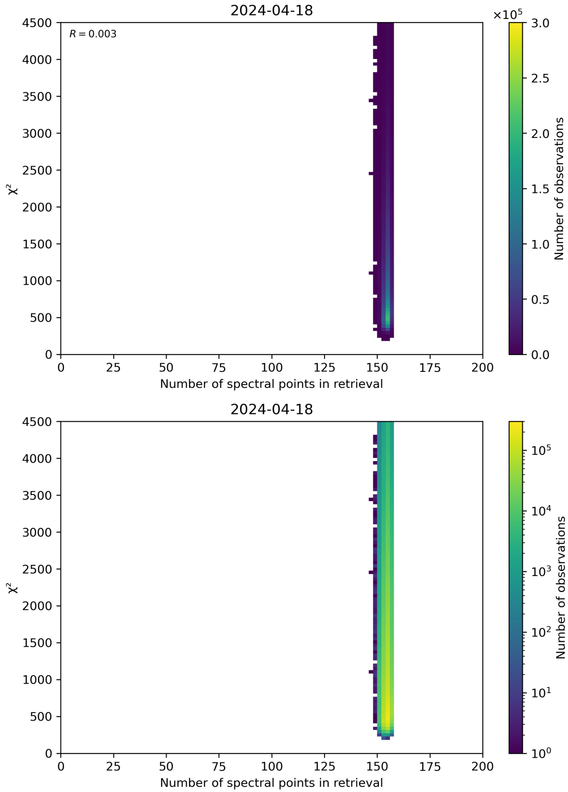
Figure 58: Scatter density plot of “Number of spectral points in retrieval” against “ \chi^2 ” for 2024-04-17 to 2024-04-19.
