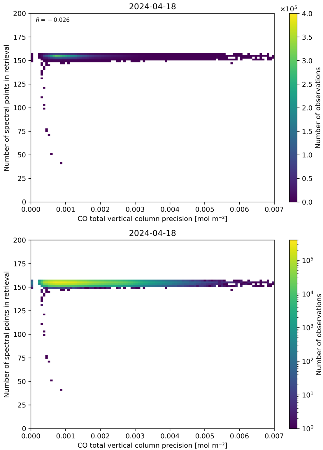
Figure 47: Scatter density plot of “CO total vertical column precision” against “Number of spectral points in retrieval” for 2024-04-17 to 2024-04-19.
