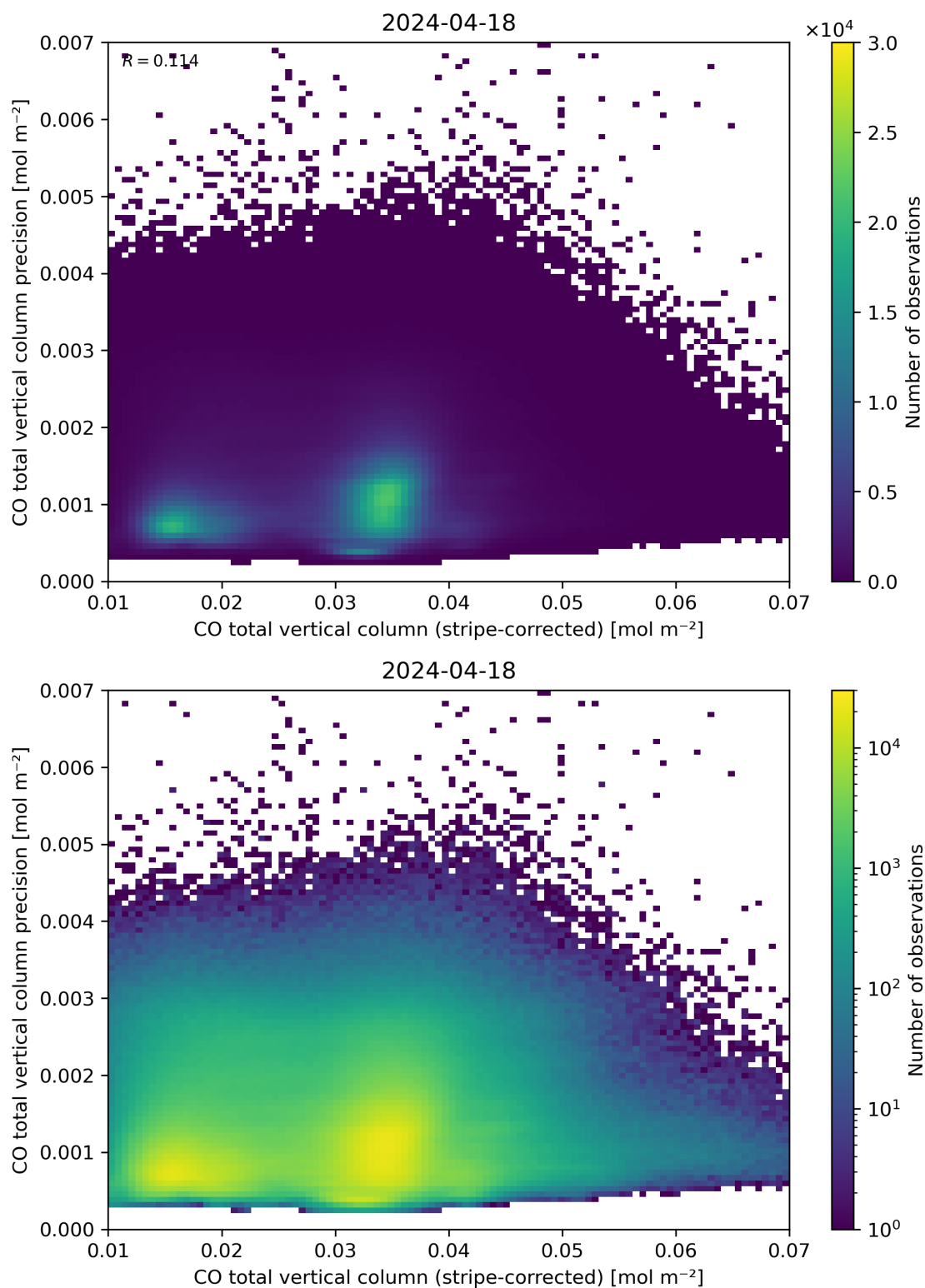
Figure 36: Scatter density plot of “CO total vertical column (stripe-corrected)” against “CO total vertical column precision” for 2024-04-17 to 2024-04-19.
