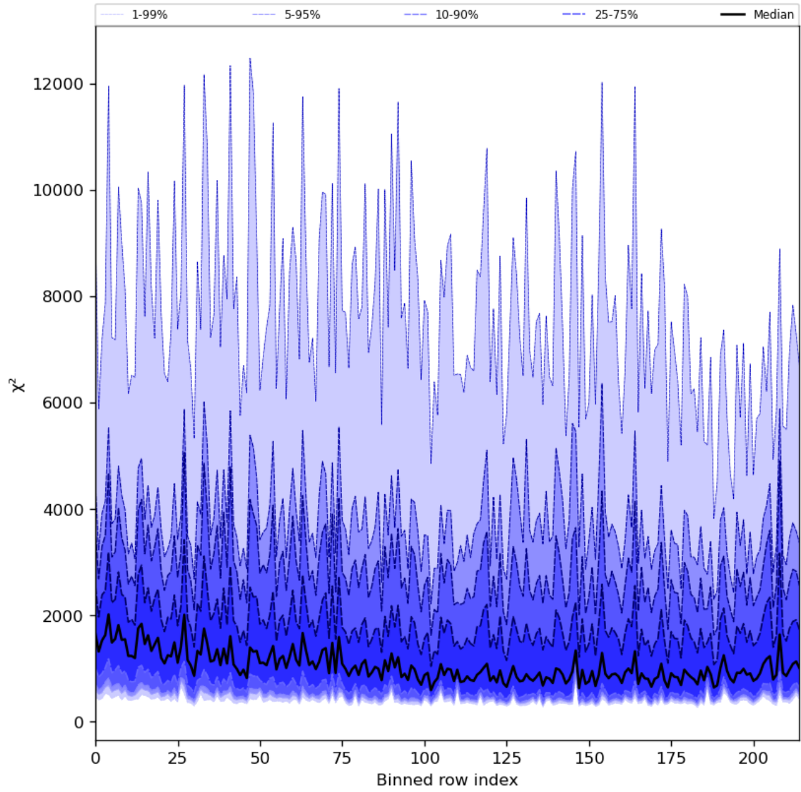
Figure 30: Along track statistics of “ \chi^2 ” for 2024-04-17 to 2024-04-19
