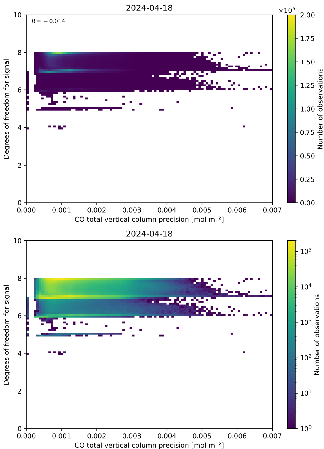
Figure 45: Scatter density plot of “CO total vertical column precision” against “Degrees of freedom for signal” for 2024-04-17 to 2024-04-19.
