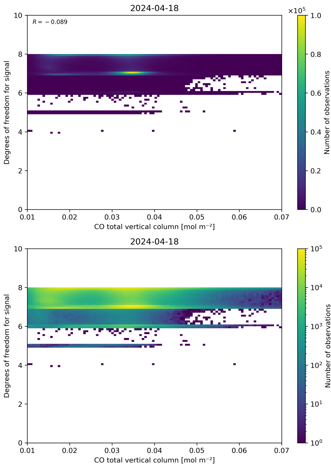
Figure 41: Scatter density plot of “CO total vertical column” against “Degrees of freedom for signal” for 2024-04-17 to 2024-04-19.
