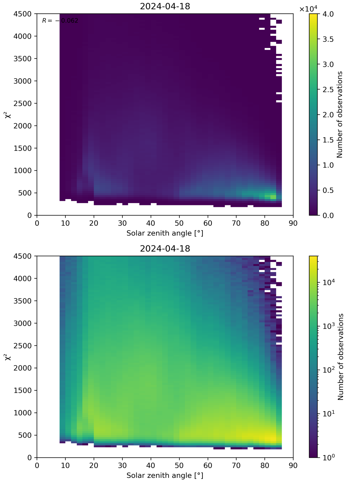
Figure 64: Scatter density plot of “Solar zenith angle” against “ \chi^2 ” for 2024-04-17 to 2024-04-19.
