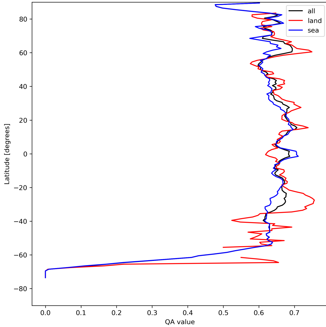
Figure 9: Zonal average of “QA value” for 2024-04-17 to 2024-04-19.
