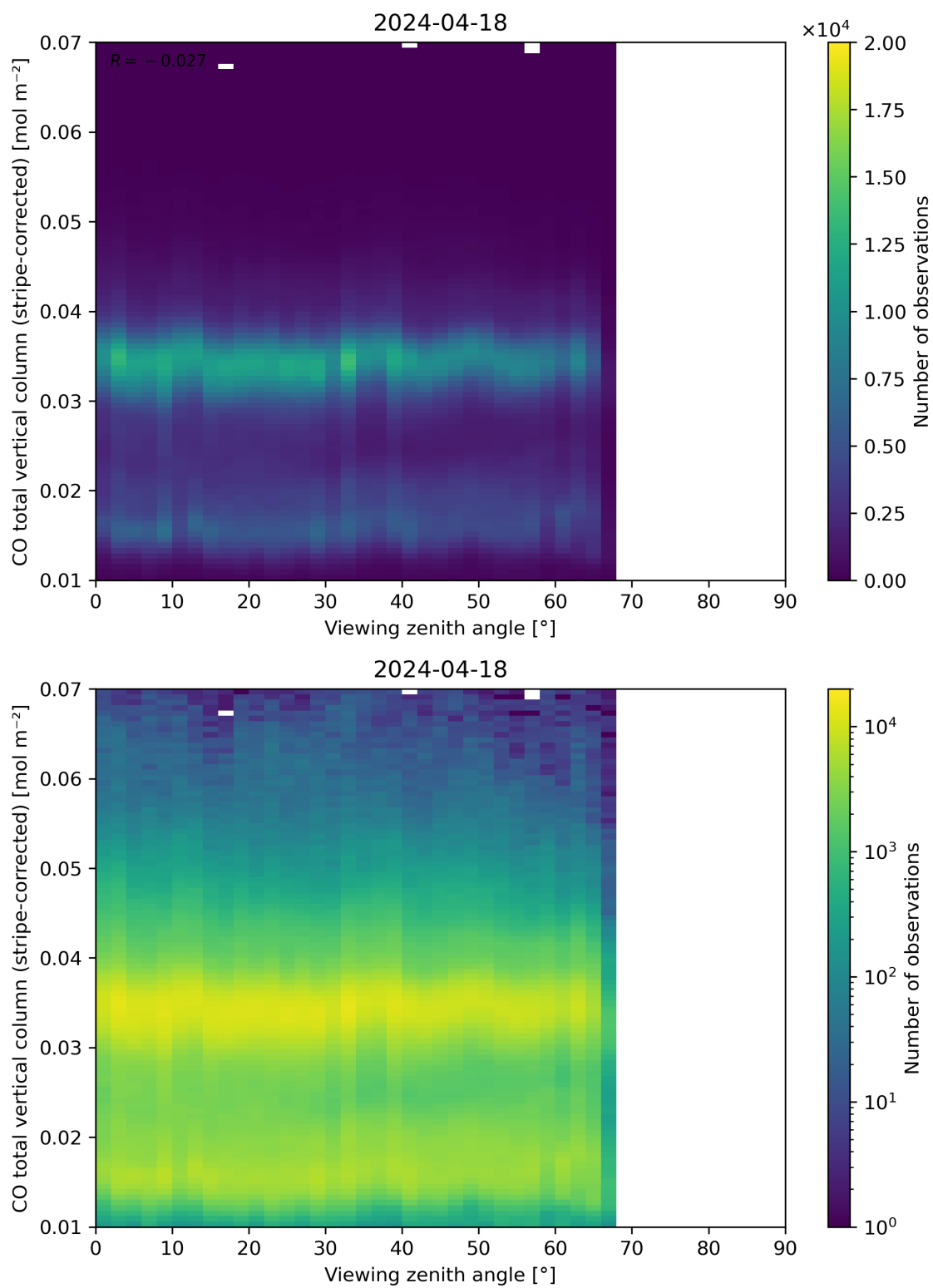
Figure 70: Scatter density plot of “Viewing zenith angle” against “CO total vertical column (stripe-corrected)” for 2024-04-17 to 2024-04-19.
