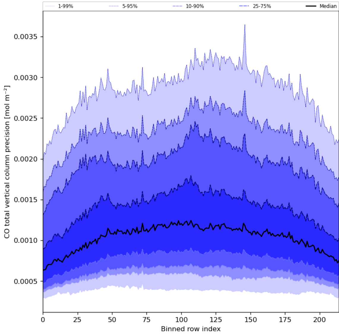
Figure 28: Along track statistics of “CO total vertical column precision” for 2024-04-17 to 2024-04-19
