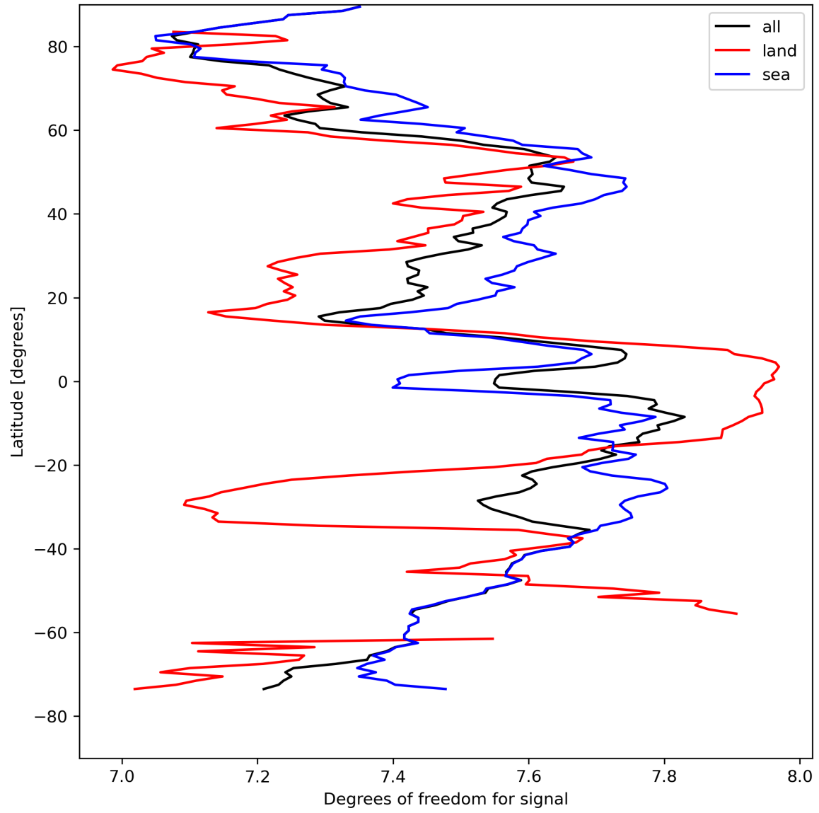
Figure 15: Zonal average of “Degrees of freedom for signal” for 2024-04-17 to 2024-04-19.
