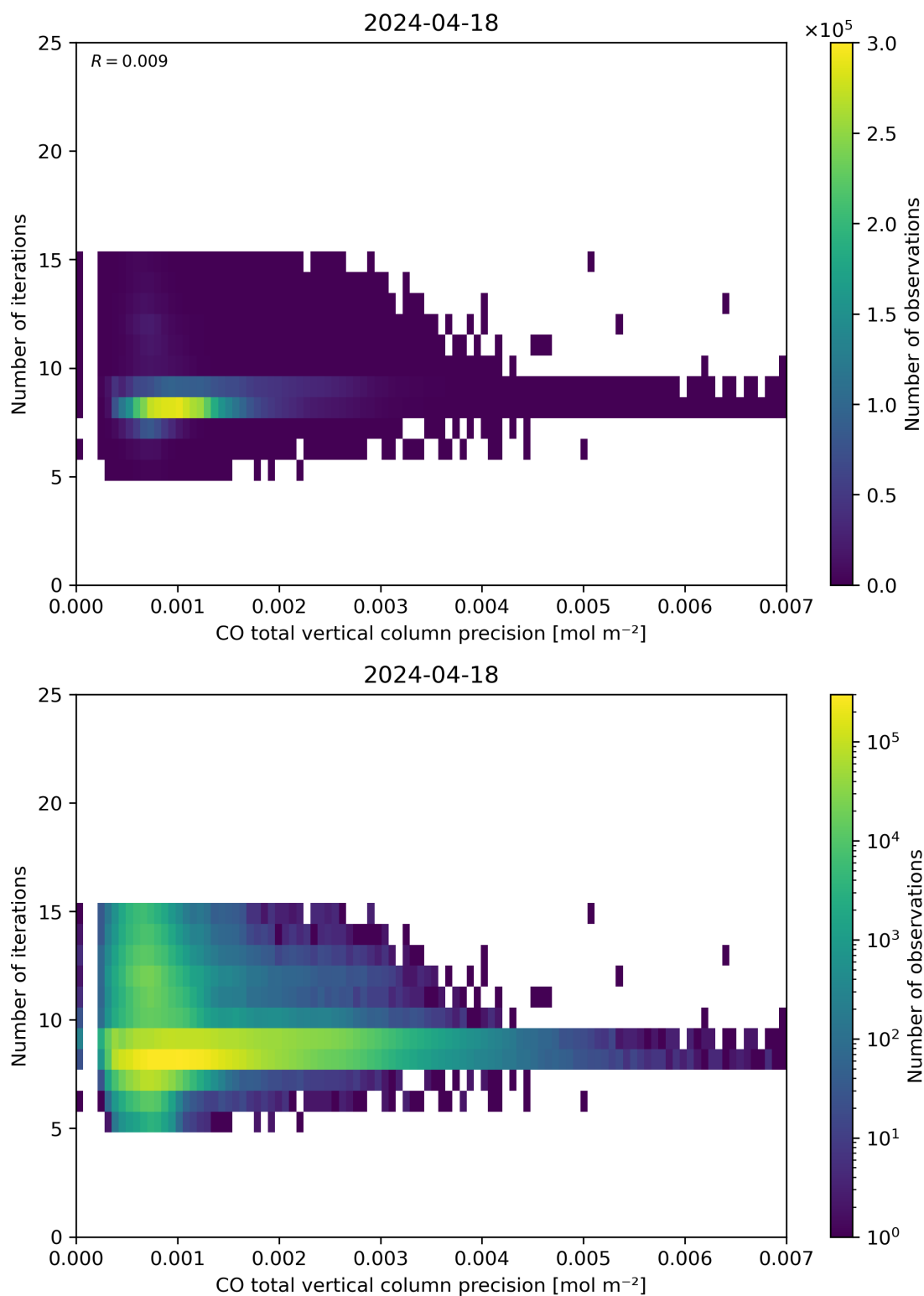
Figure 46: Scatter density plot of “CO total vertical column precision” against “Number of iterations” for 2024-04-17 to 2024-04-19.
