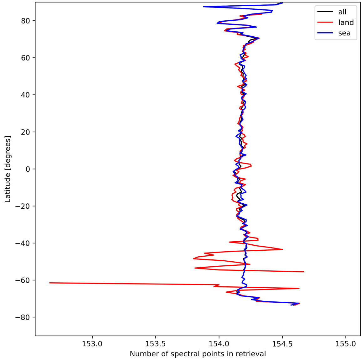
Figure 13: Zonal average of “Number of spectral points in retrieval” for 2024-04-17 to 2024-04-19.
