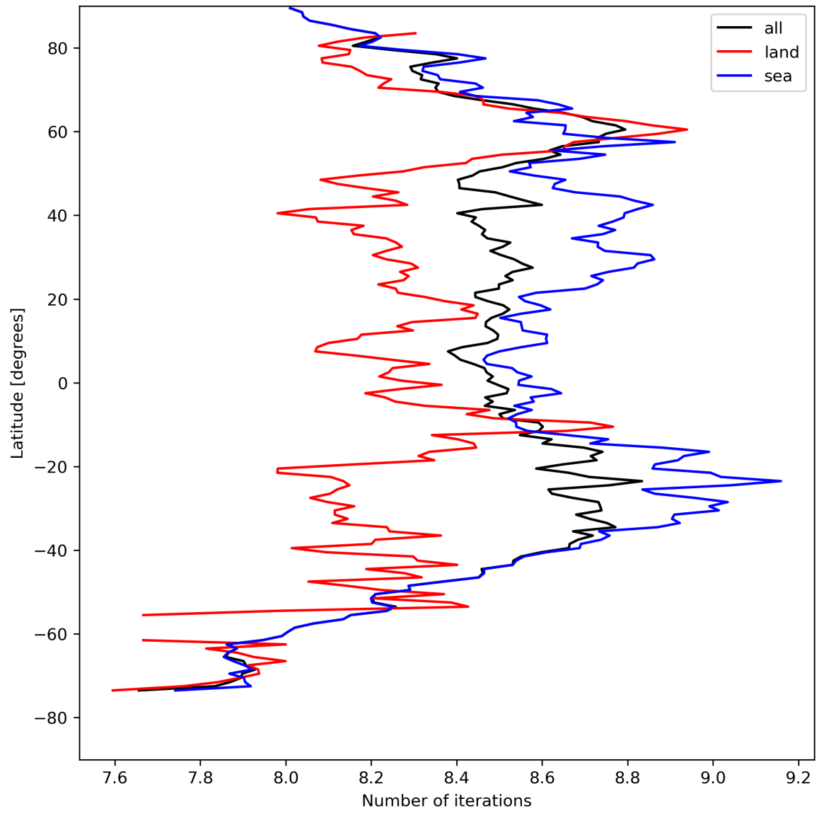
Figure 16: Zonal average of “Number of iterations” for 2024-04-17 to 2024-04-19.
