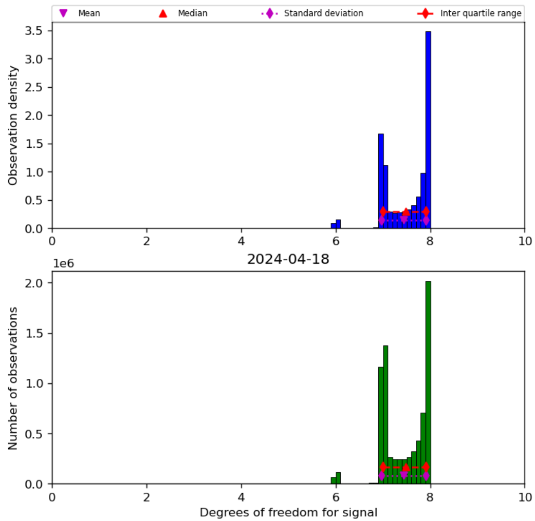
Figure 23: Histogram of “Degrees of freedom for signal” for 2024-04-17 to 2024-04-19
