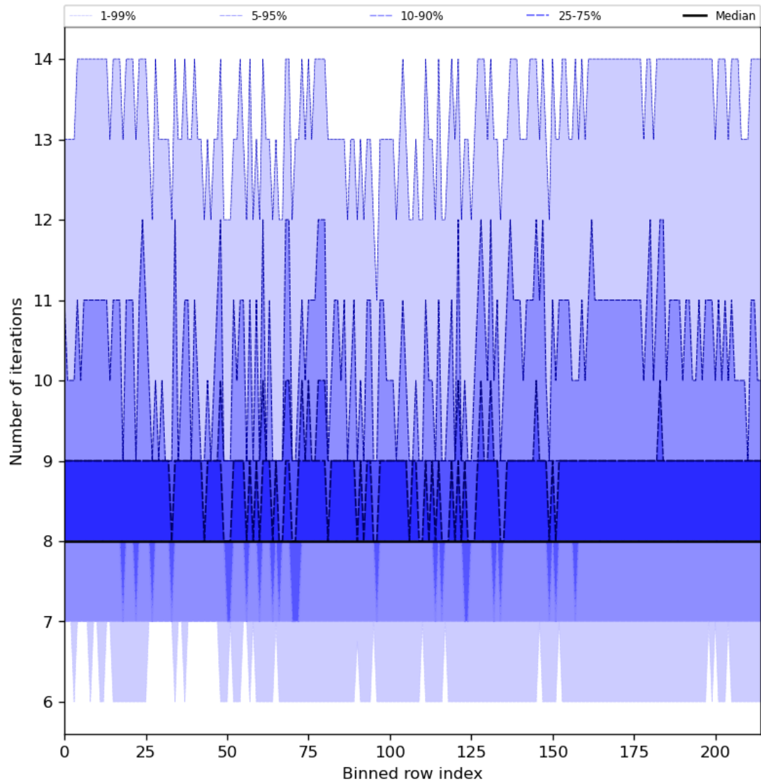
Figure 32: Along track statistics of “Number of iterations” for 2024-04-19 to 2024-04-21
