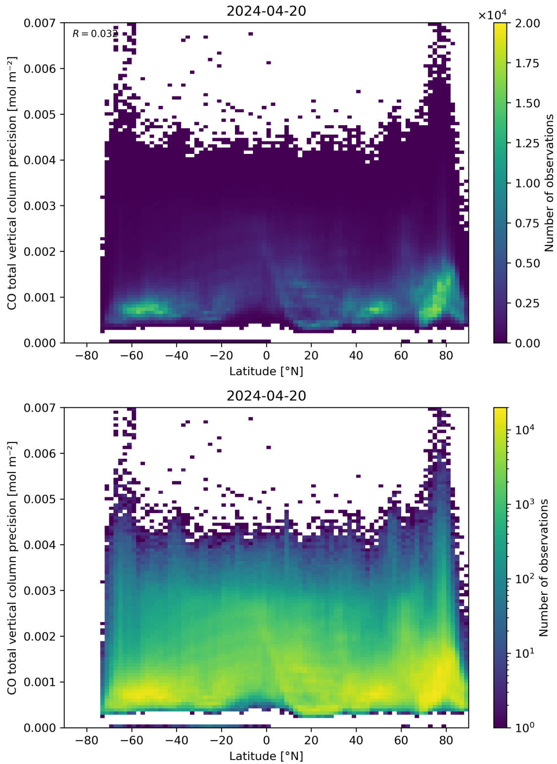
Figure 53: Scatter density plot of “Latitude” against “CO total vertical column precision” for 2024-04-19 to 2024-04-21.
