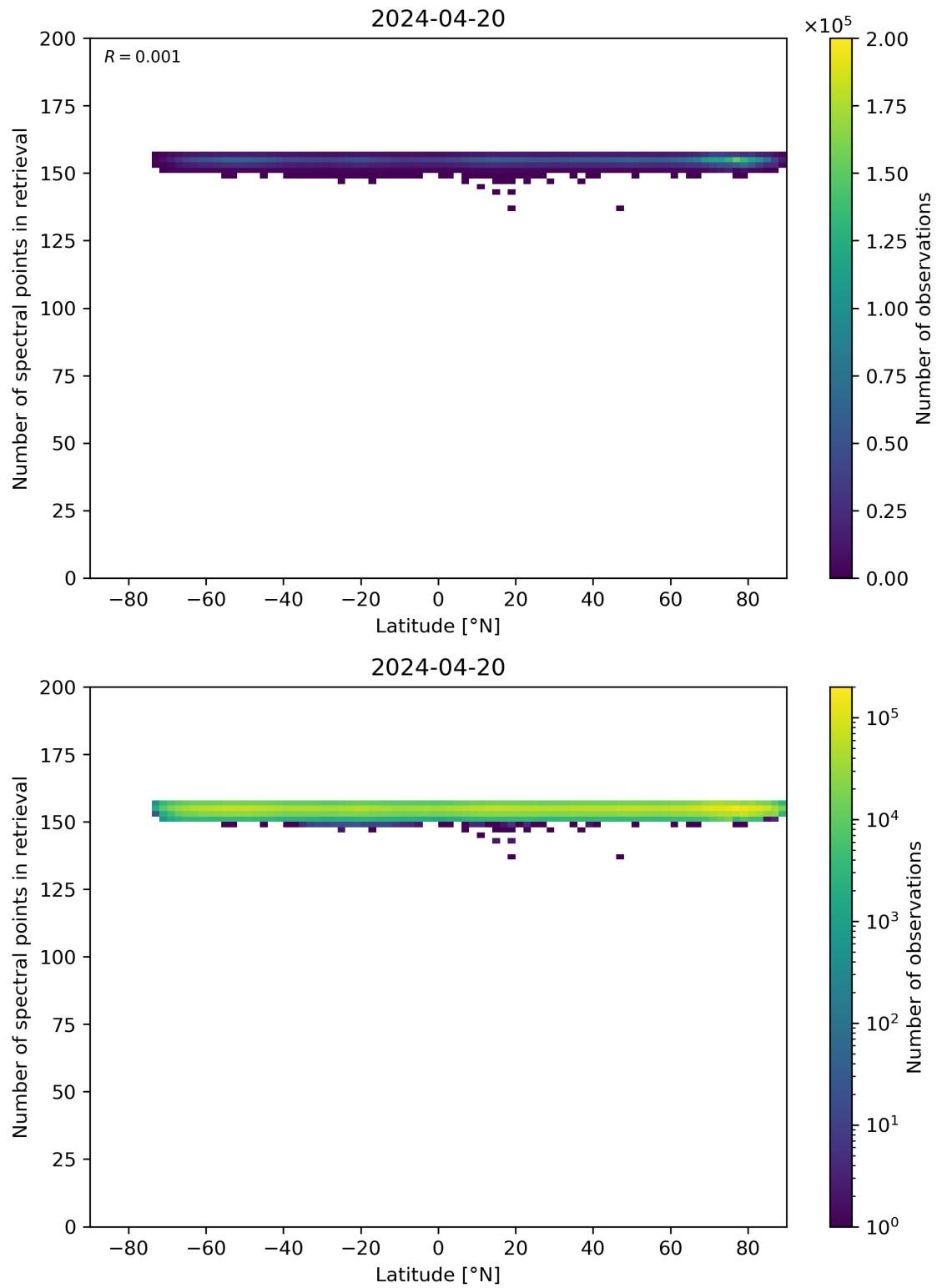
Figure 57: Scatter density plot of “Latitude” against “Number of spectral points in retrieval” for 2024-04-19 to 2024-04-21.
