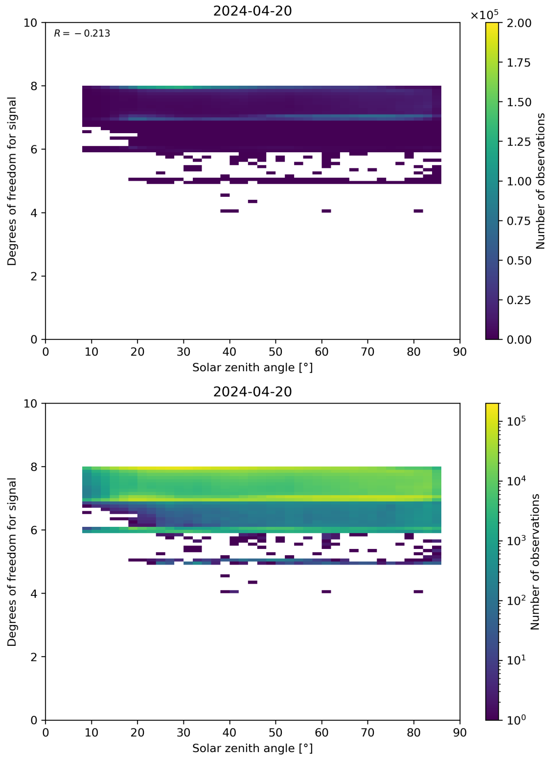
Figure 65: Scatter density plot of “Solar zenith angle” against “Degrees of freedom for signal” for 2024-04-19 to 2024-04-21.
