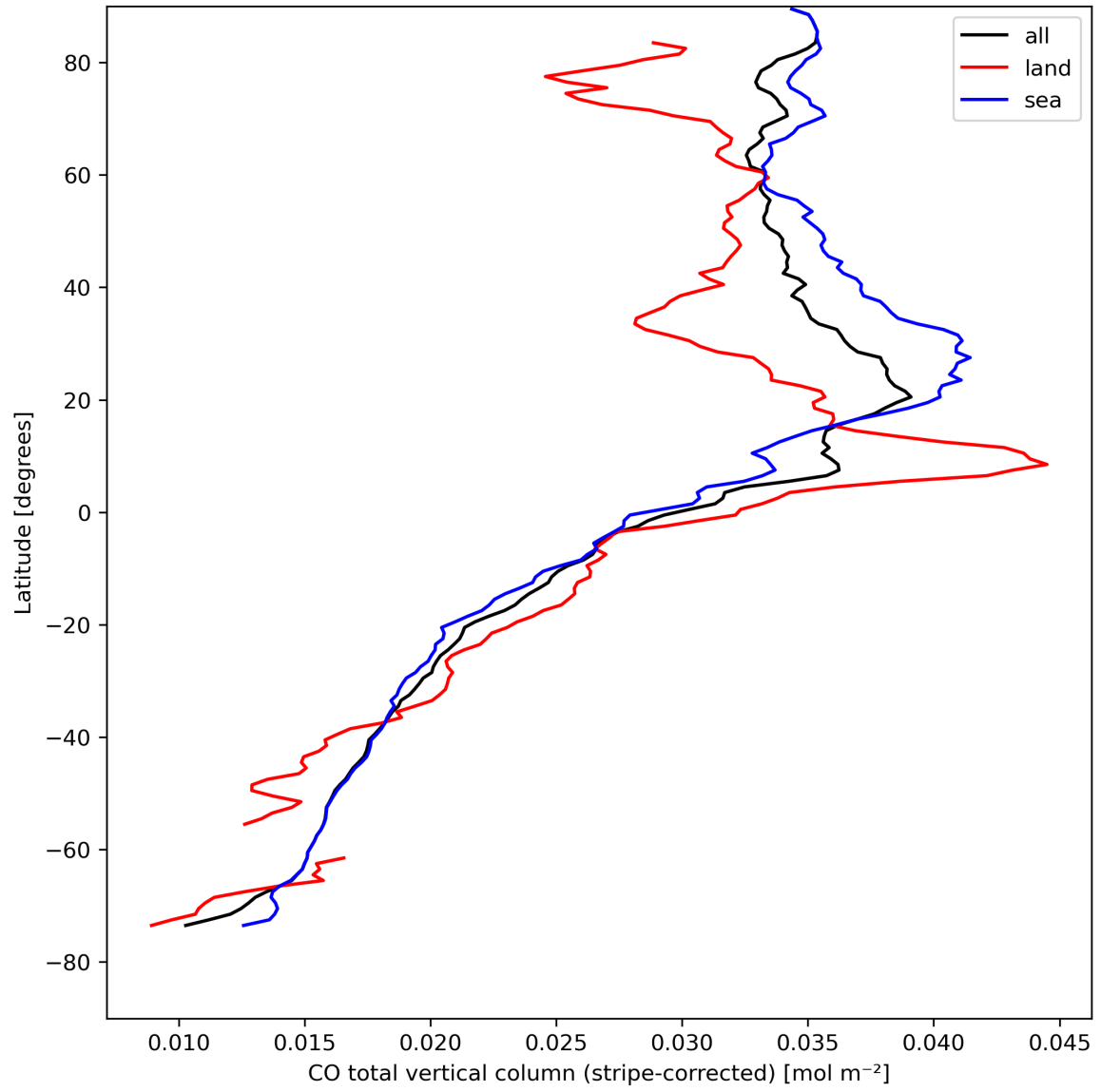
Figure 11: Zonal average of “CO total vertical column (stripe-corrected)” for 2024-04-19 to 2024-04-21.
