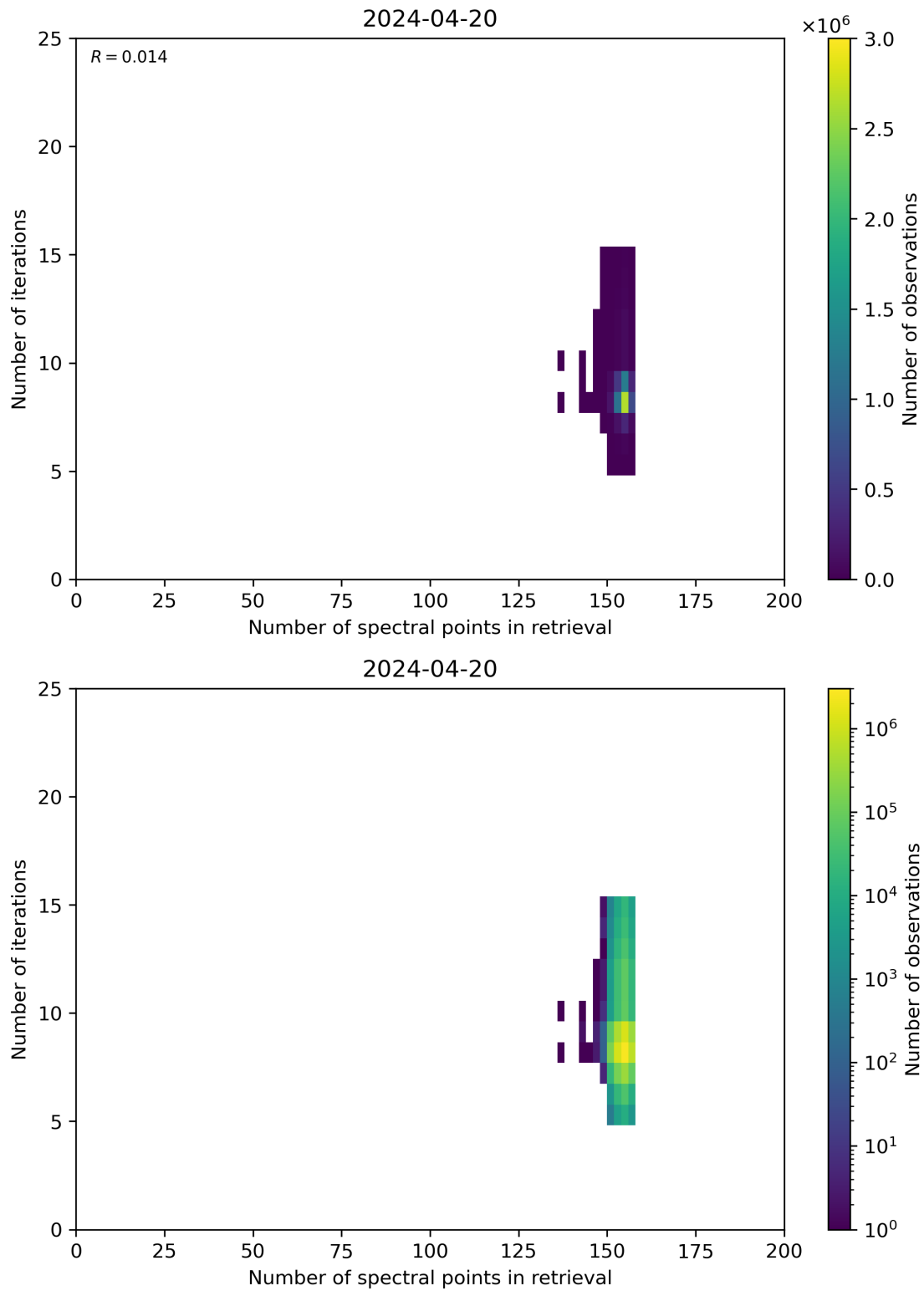
Figure 60: Scatter density plot of “Number of spectral points in retrieval” against “Number of iterations” for 2024-04-19 to 2024-04-21.
