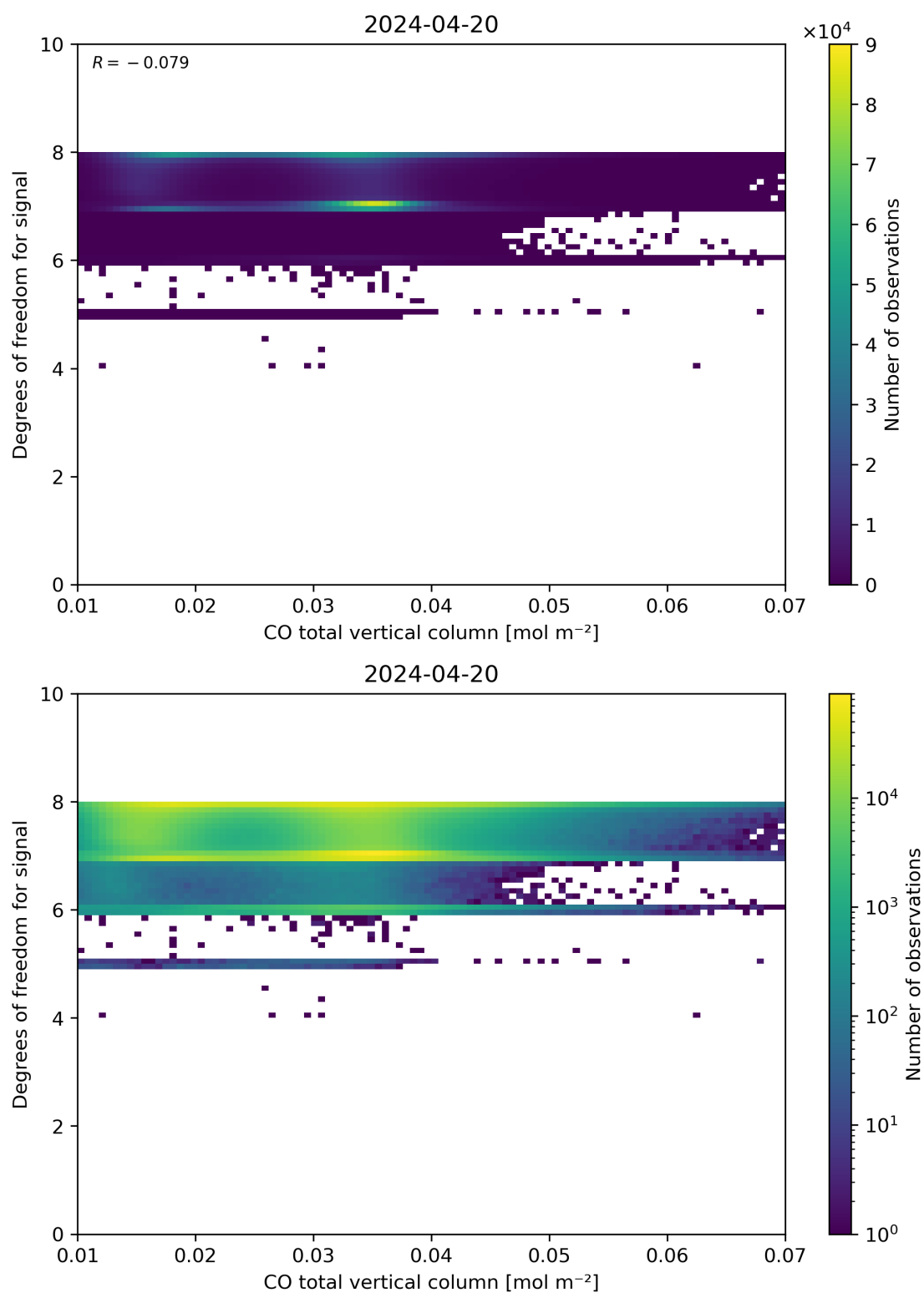
Figure 41: Scatter density plot of “CO total vertical column” against “Degrees of freedom for signal” for 2024-04-19 to 2024-04-21.
