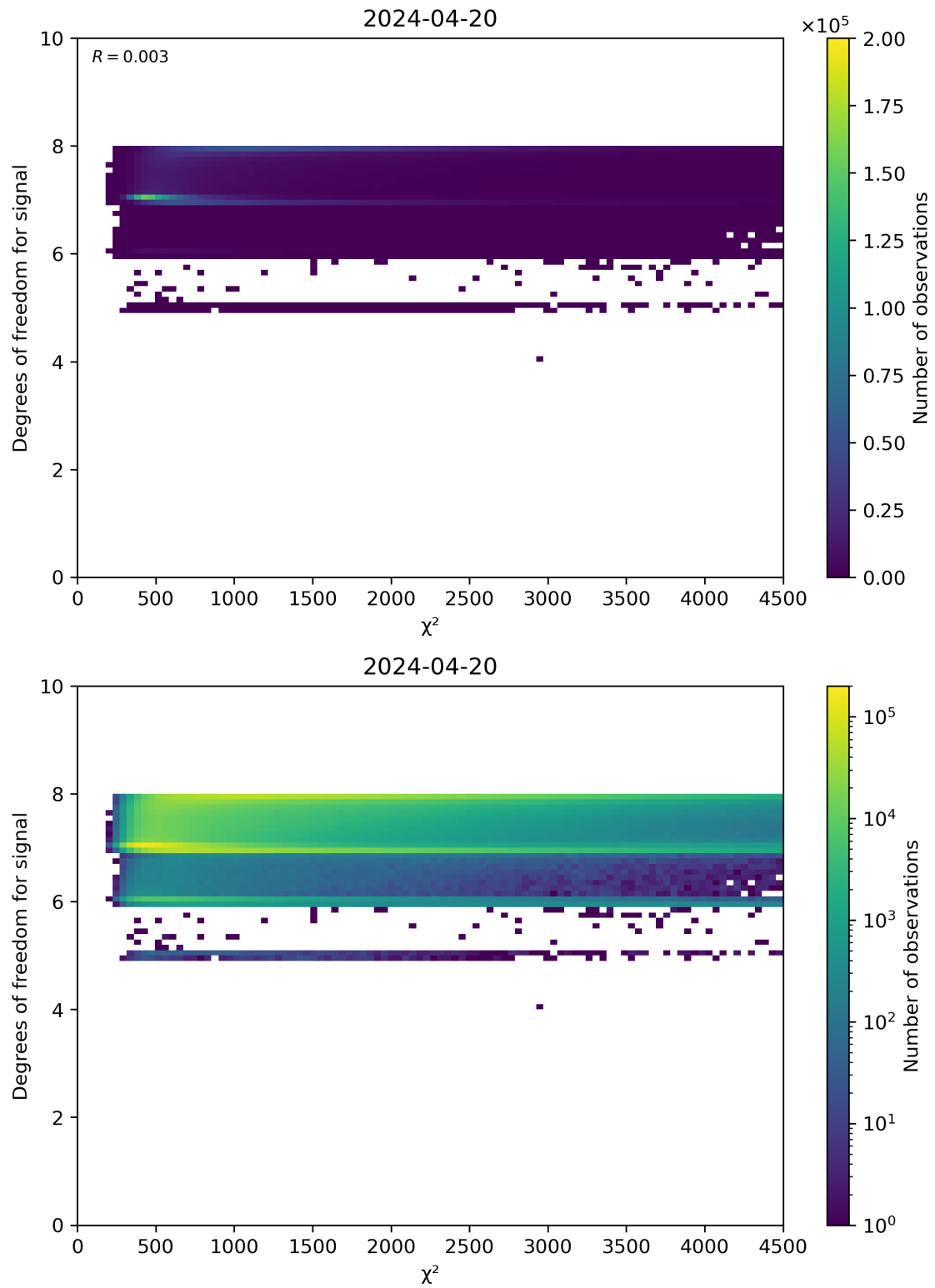
Figure 48: Scatter density plot of “ \chi^2 ” against “Degrees of freedom for signal” for 2024-04-19 to 2024-04-21.
