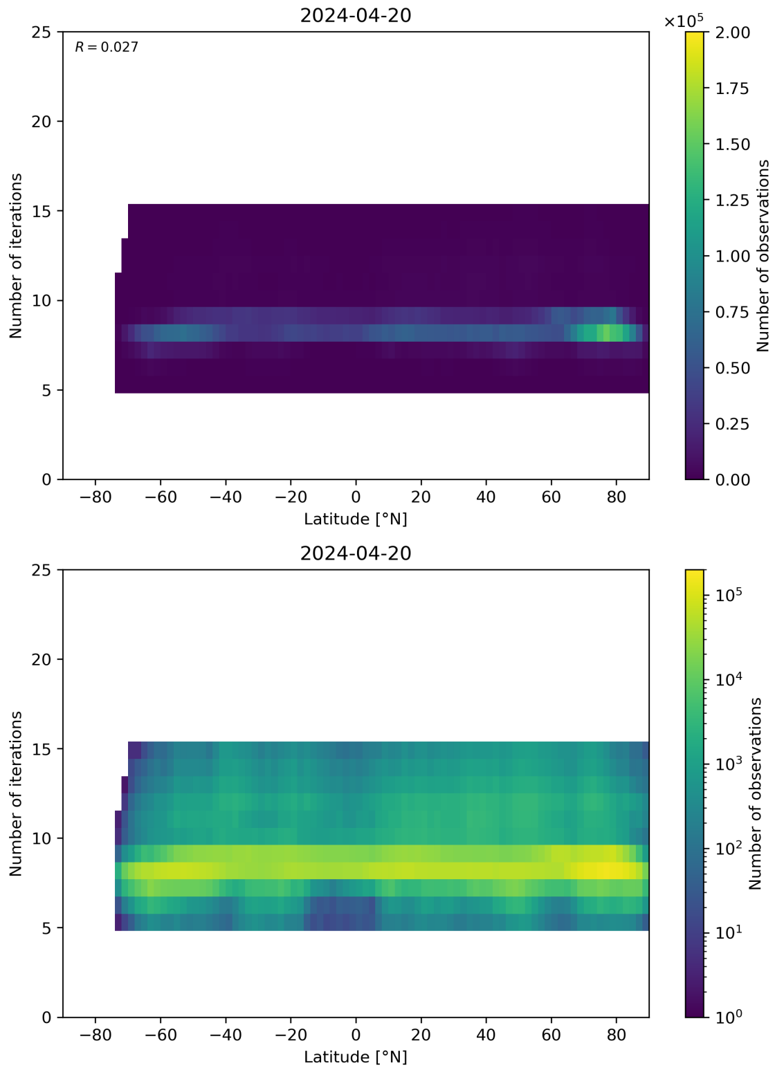
Figure 56: Scatter density plot of “Latitude” against “Number of iterations” for 2024-04-19 to 2024-04-21.
