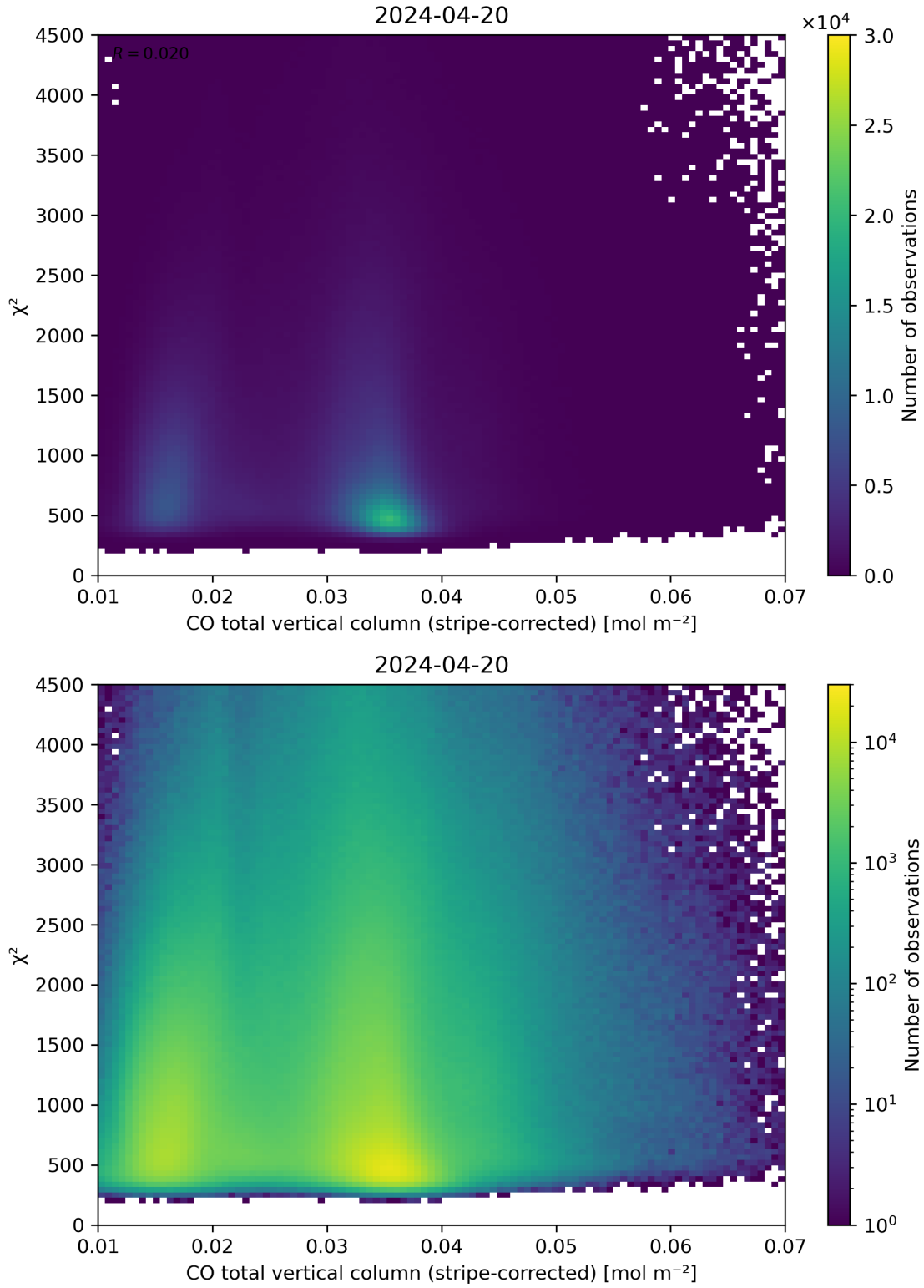
Figure 37: Scatter density plot of “CO total vertical column (stripe-corrected)” against “ \chi^2 ” for 2024-04-19 to 2024-04-21.
