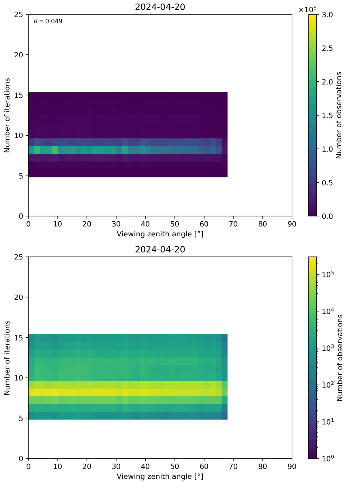
Figure 75: Scatter density plot of “Viewing zenith angle” against “Number of iterations” for 2024-04-19 to 2024-04-21.
