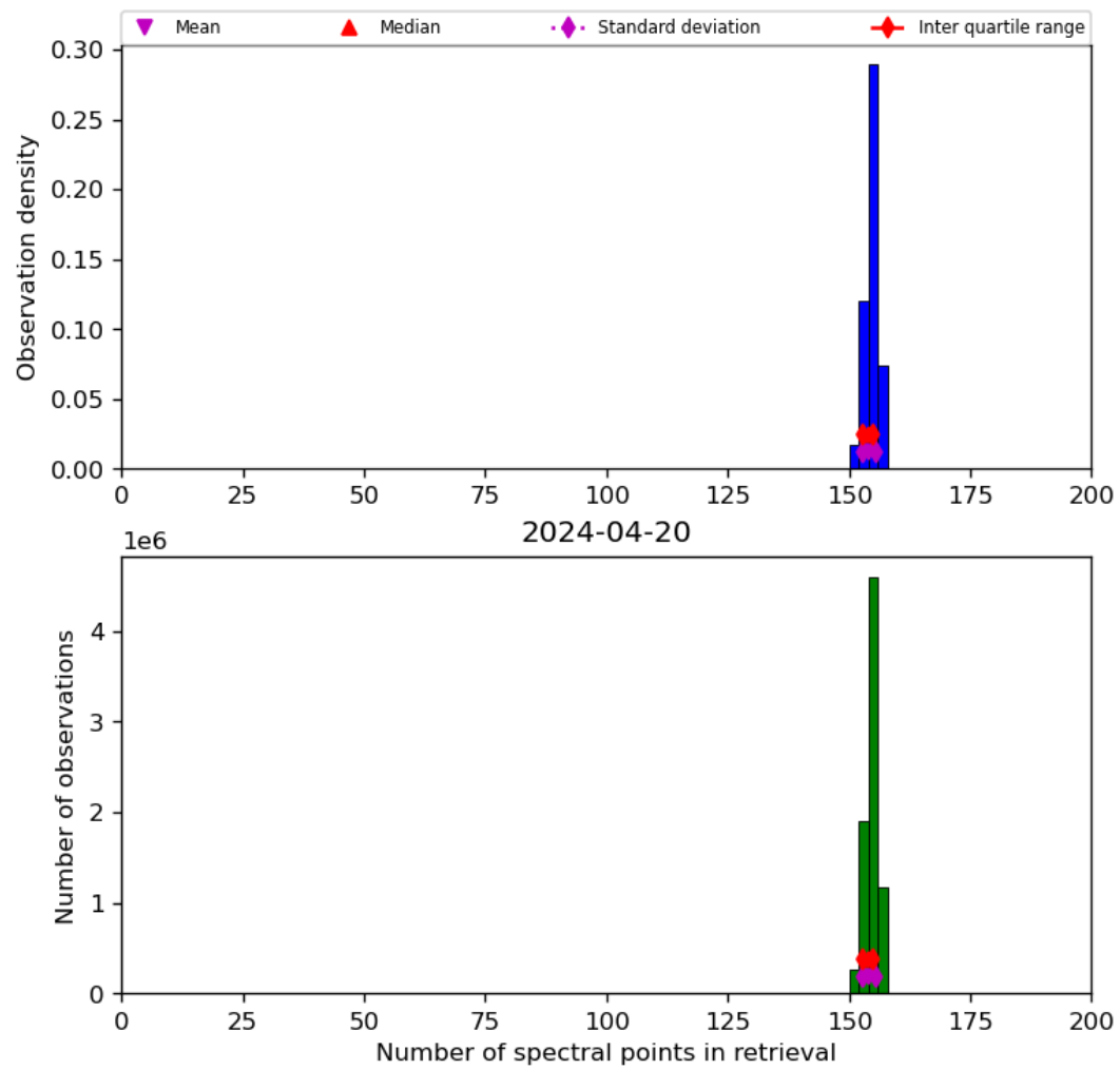
Figure 21: Histogram of “Number of spectral points in retrieval” for 2024-04-19 to 2024-04-21
