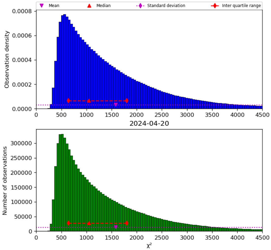
Figure 22: Histogram of “ \chi^2 ” for 2024-04-19 to 2024-04-21
