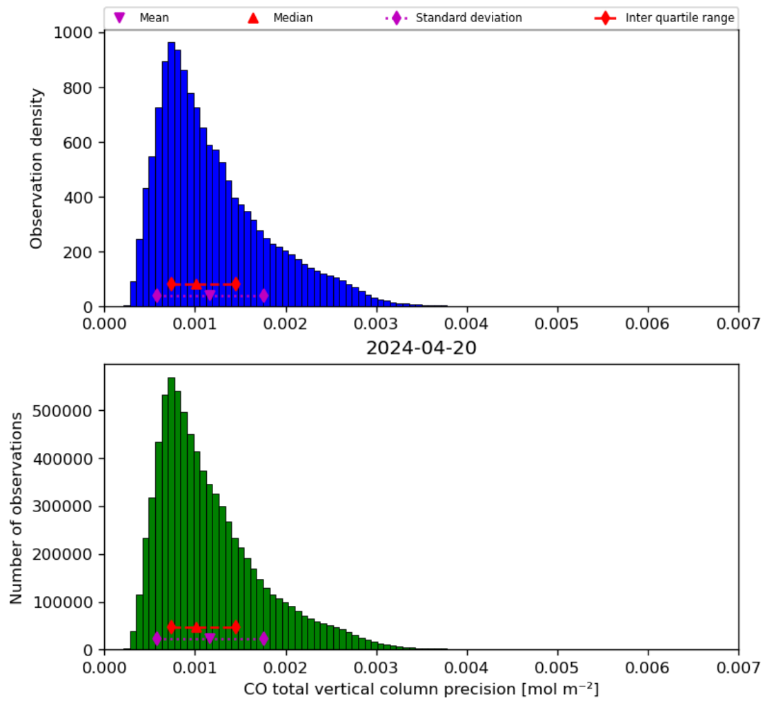
Figure 20: Histogram of “CO total vertical column precision” for 2024-04-19 to 2024-04-21
