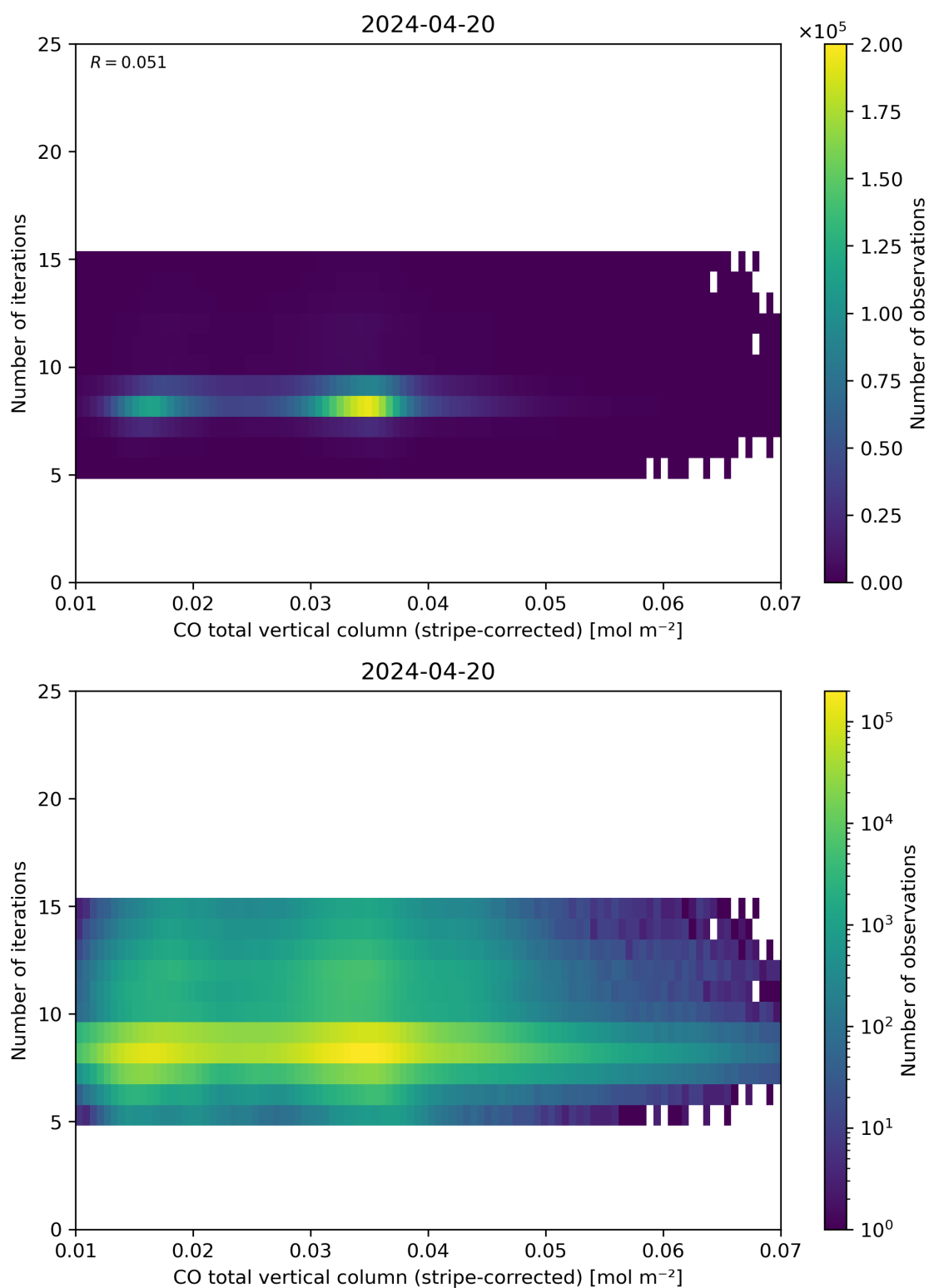
Figure 39: Scatter density plot of “CO total vertical column (stripe-corrected)” against “Number of iterations” for 2024-04-19 to 2024-04-21.
