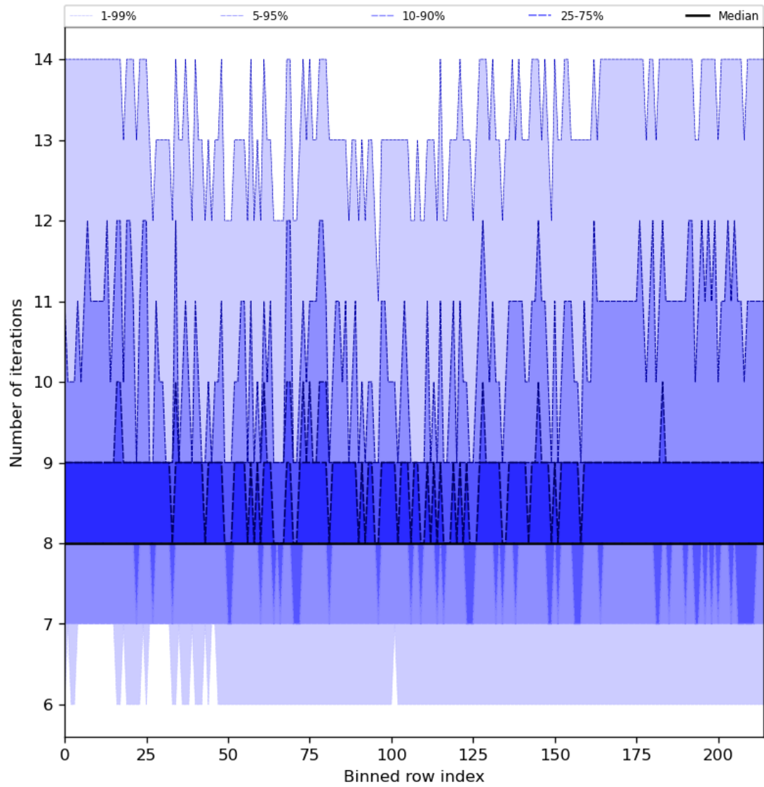
Figure 32: Along track statistics of “Number of iterations” for 2024-04-21 to 2024-04-22
