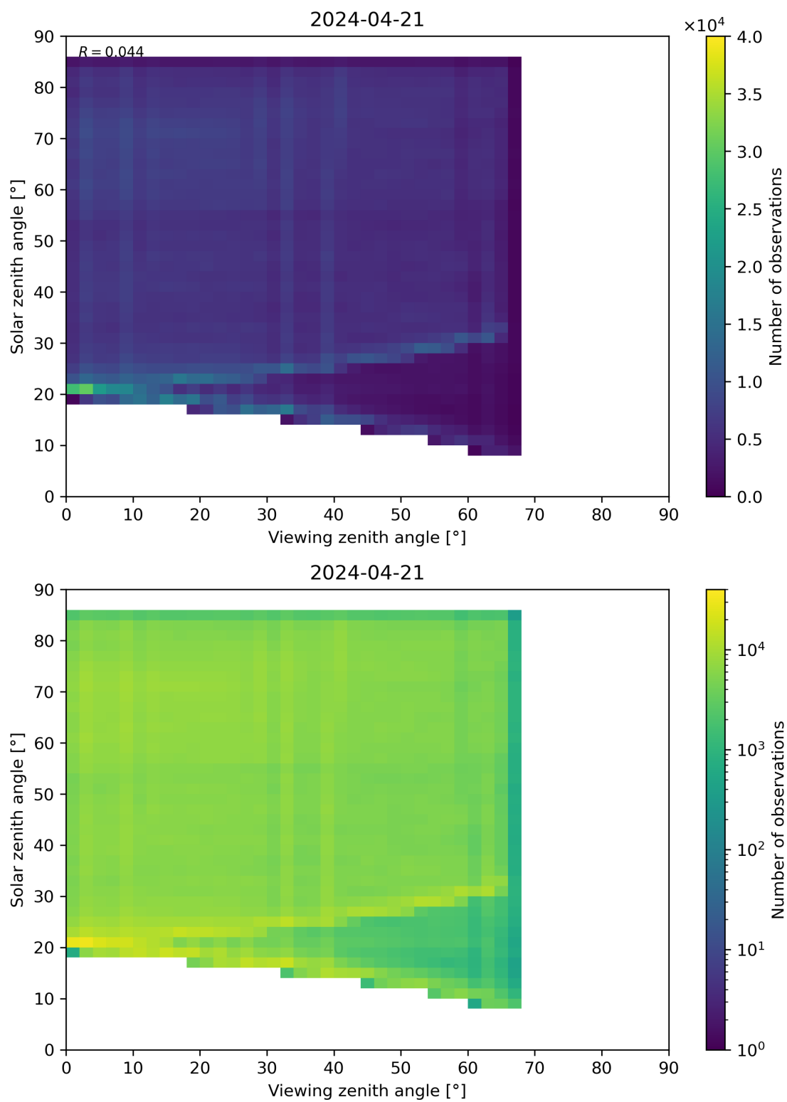
Figure 77: Scatter density plot of “Viewing zenith angle” against “Solar zenith angle” for 2024-04-21 to 2024-04-22.
