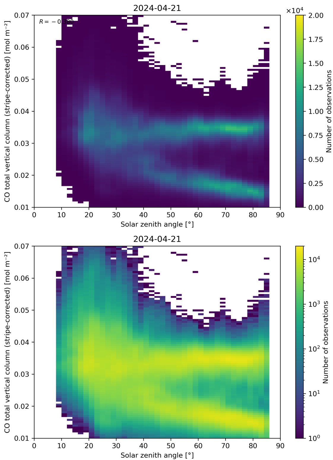
Figure 62: Scatter density plot of “Solar zenith angle” against “CO total vertical column (stripe-corrected)” for 2024-04-21 to 2024-04-22.
