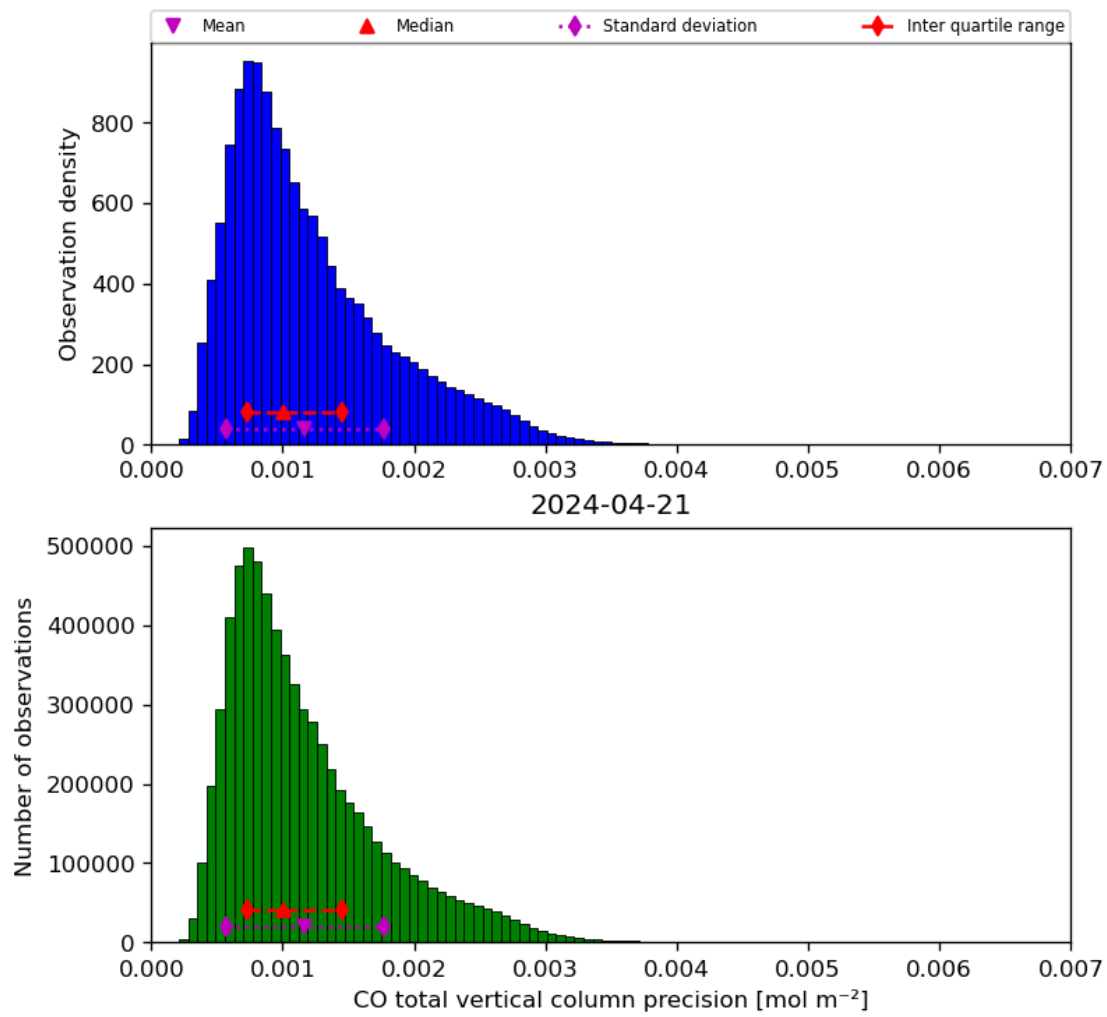
Figure 20: Histogram of “CO total vertical column precision” for 2024-04-21 to 2024-04-22
