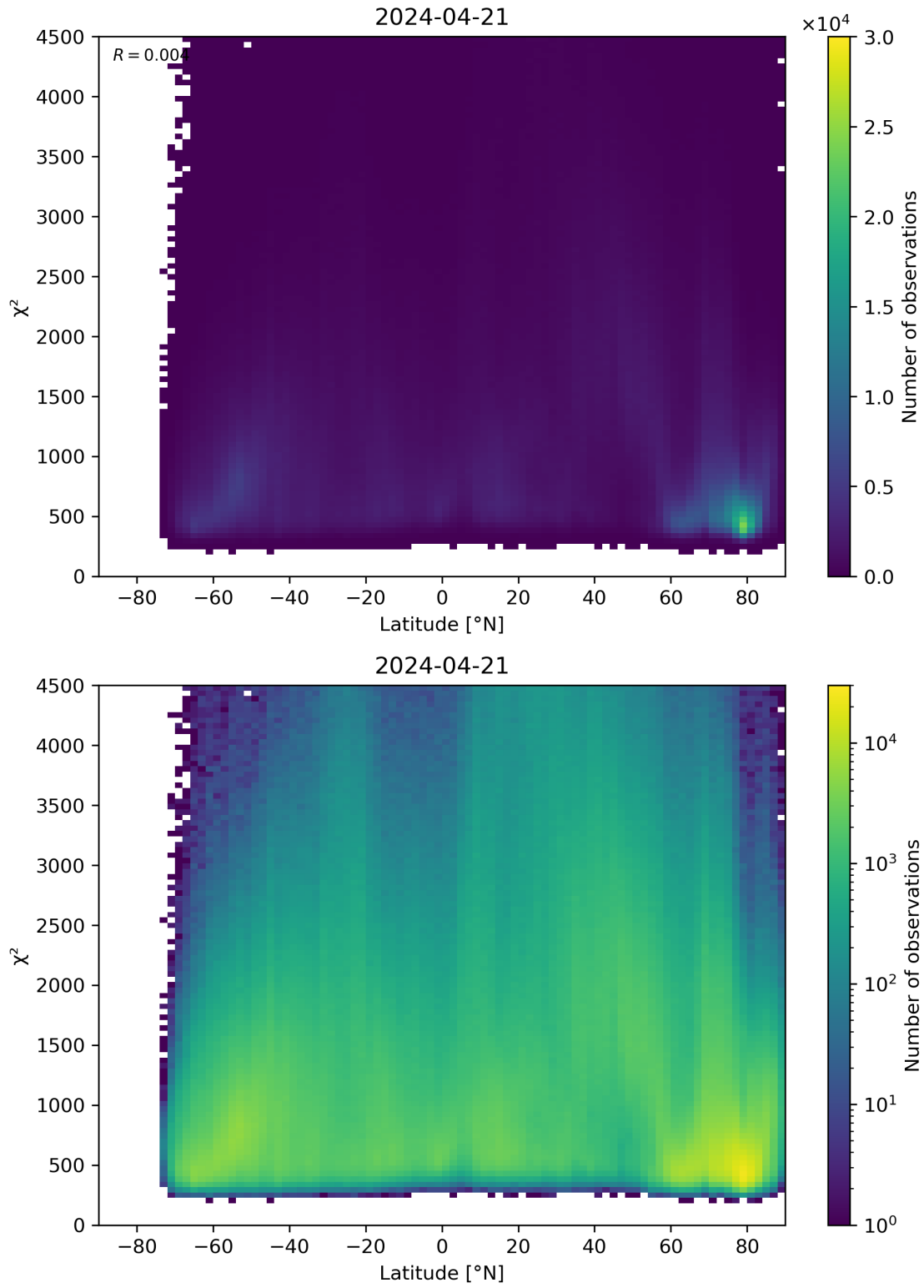
Figure 54: Scatter density plot of “Latitude” against “ \chi^2 ” for 2024-04-21 to 2024-04-22.
