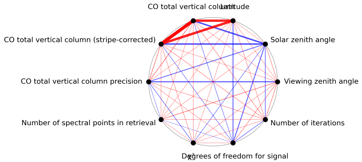
Figure 1: Map of correlation graph for 2024-04-21 to 2024-04-22.
