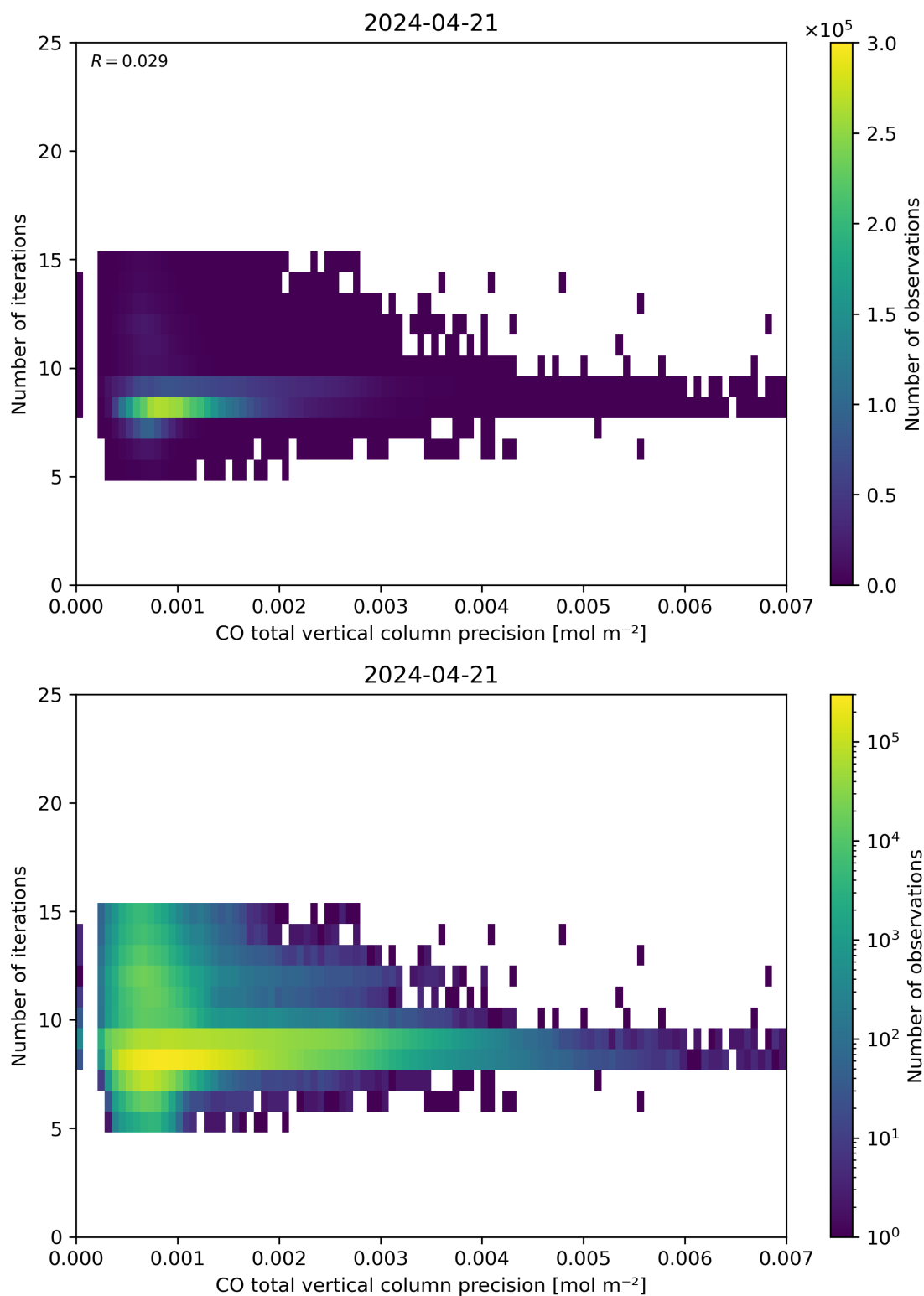
Figure 46: Scatter density plot of “CO total vertical column precision” against “Number of iterations” for 2024-04-21 to 2024-04-22.
