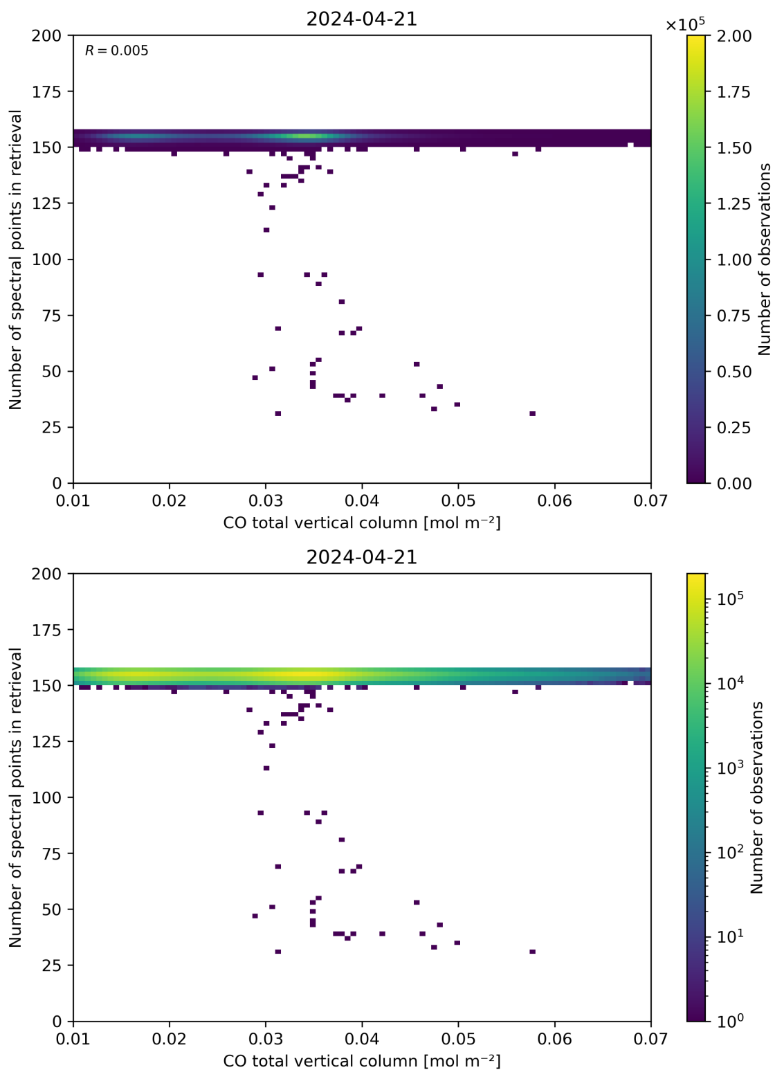
Figure 43: Scatter density plot of “CO total vertical column” against “Number of spectral points in retrieval” for 2024-04-21 to 2024-04-22.
