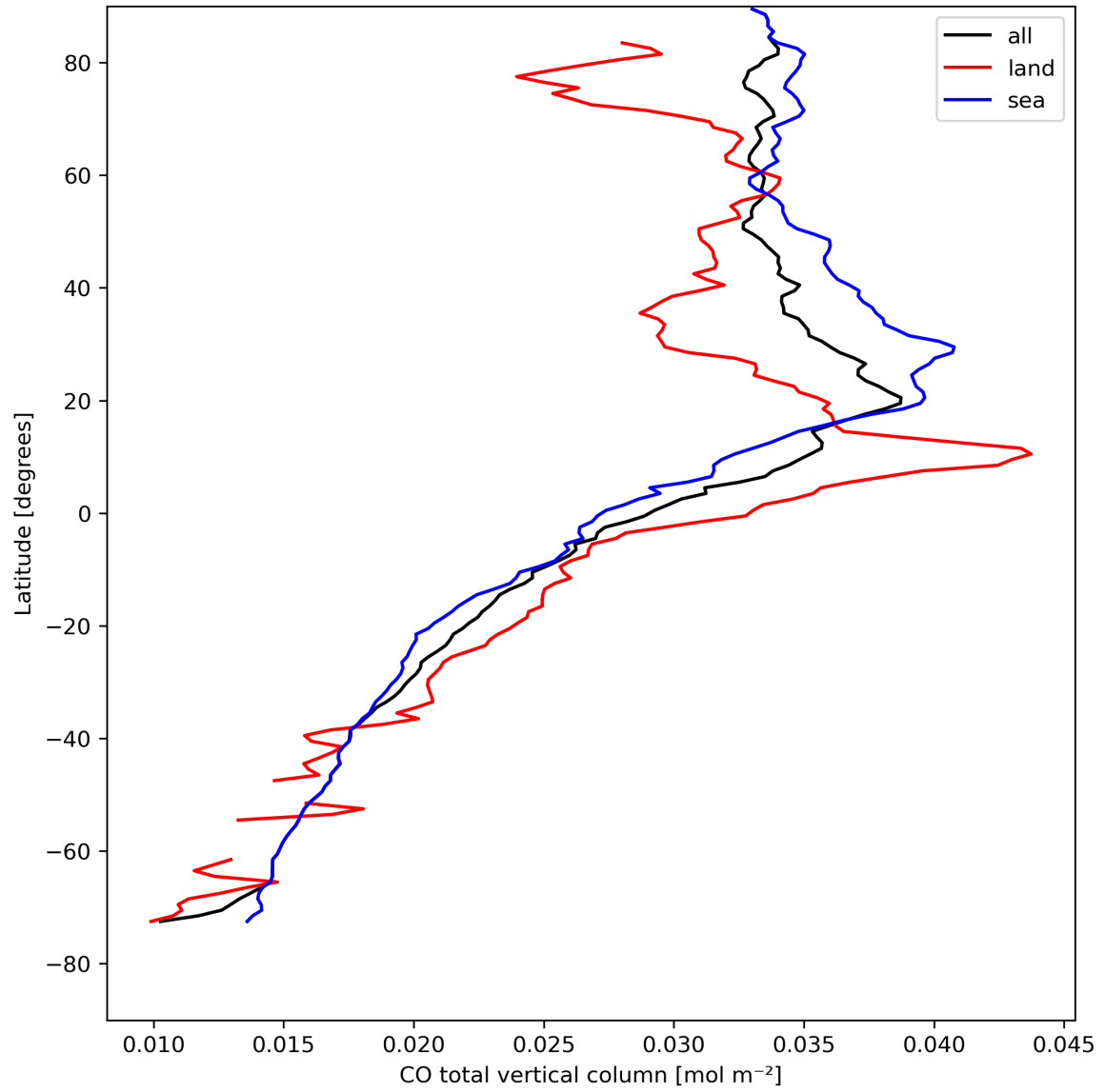
Figure 10: Zonal average of “CO total vertical column” for 2024-04-21 to 2024-04-22.
