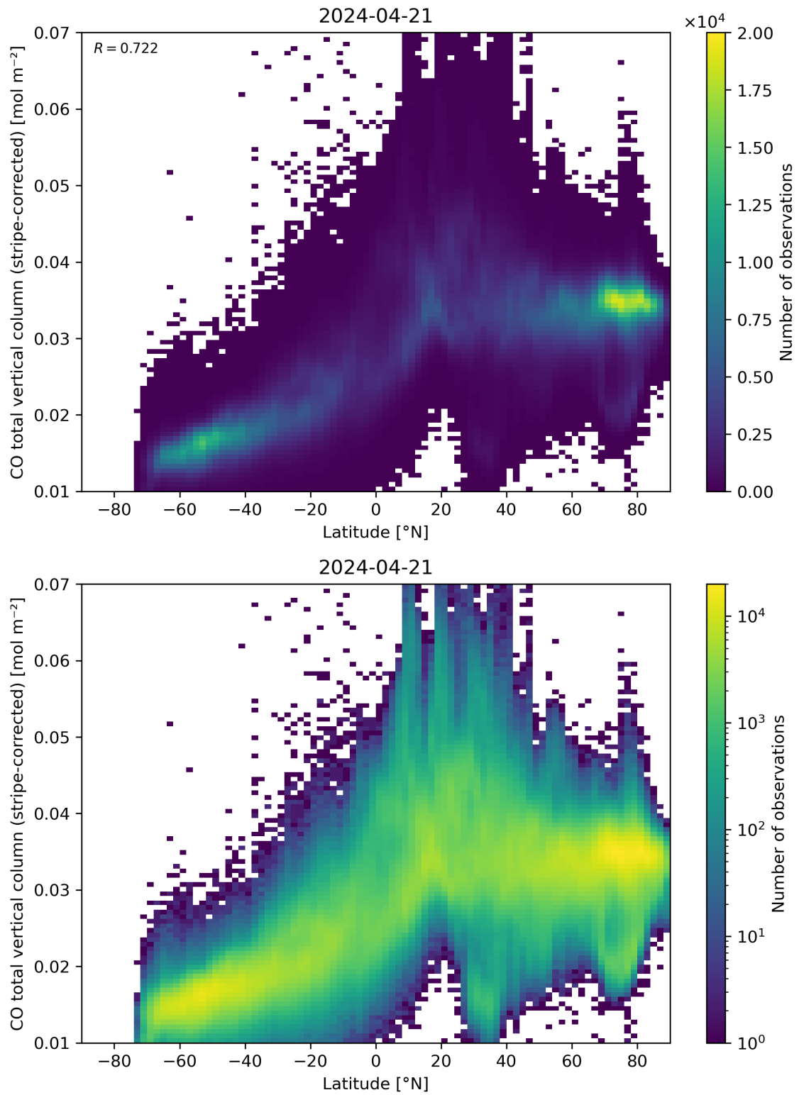
Figure 52: Scatter density plot of “Latitude” against “CO total vertical column (stripe-corrected)” for 2024-04-21 to 2024-04-22.
