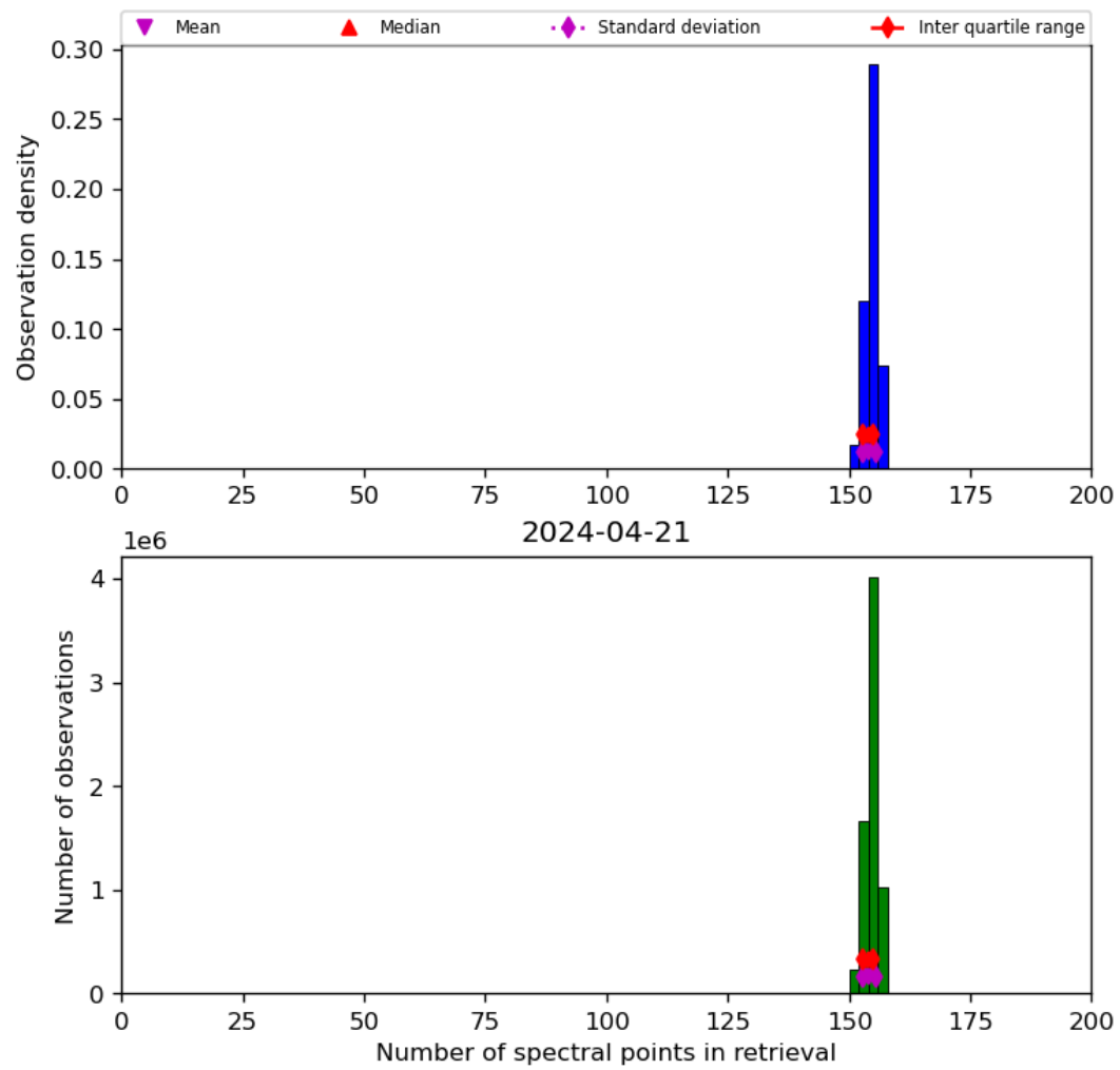
Figure 21: Histogram of “Number of spectral points in retrieval” for 2024-04-21 to 2024-04-22
