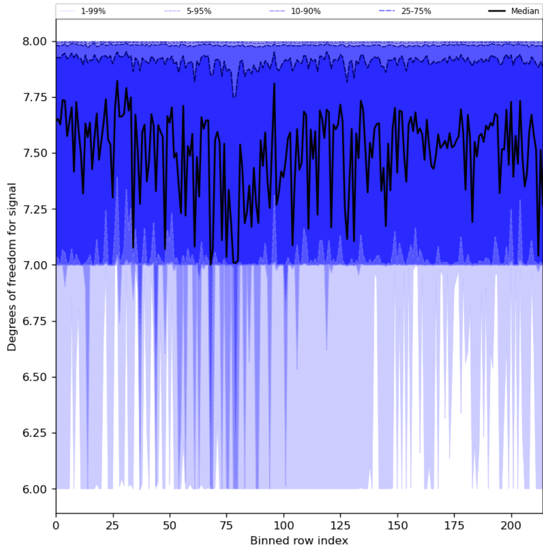
Figure 31: Along track statistics of “Degrees of freedom for signal” for 2024-04-21 to 2024-04-22
