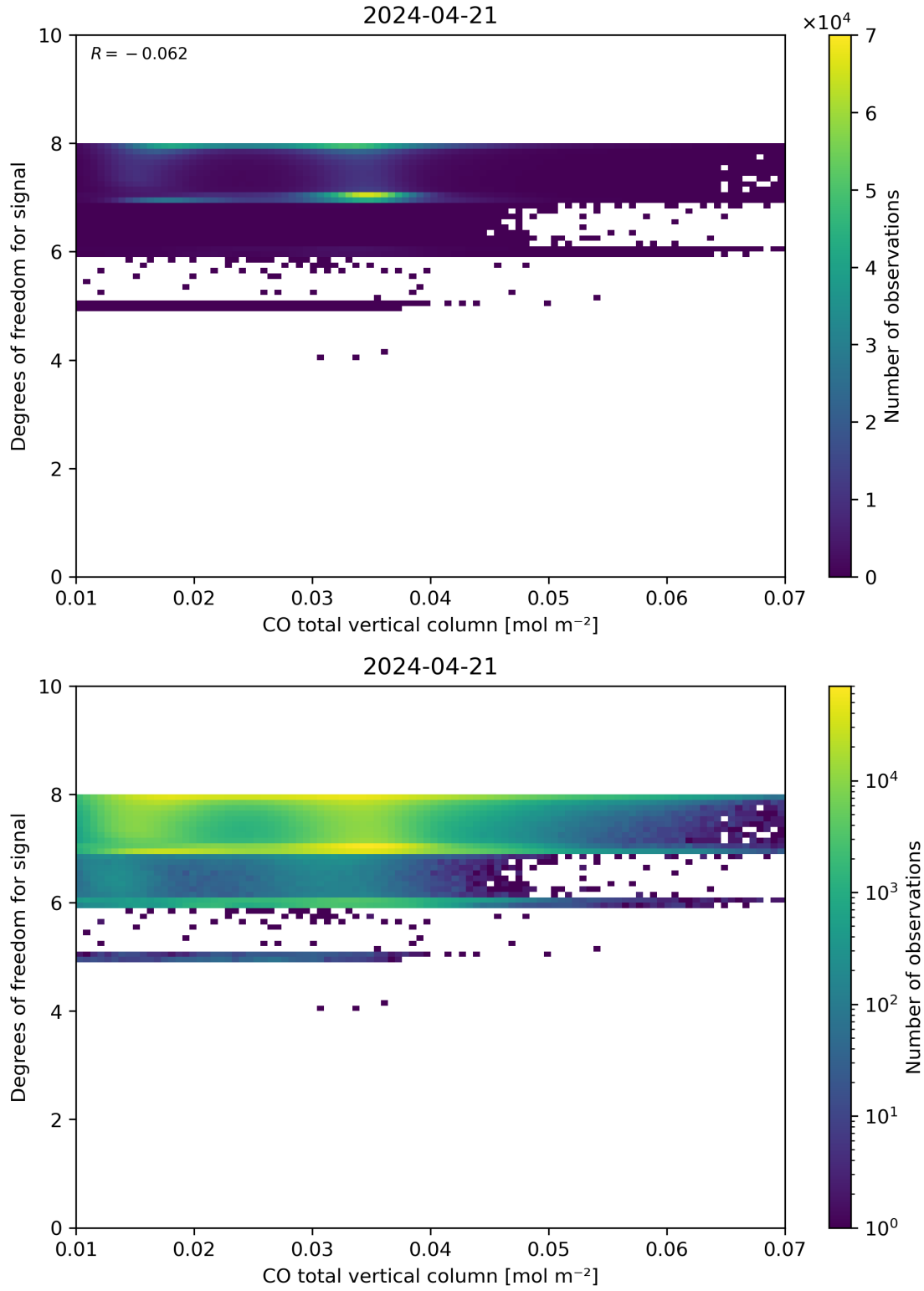
Figure 41: Scatter density plot of “CO total vertical column” against “Degrees of freedom for signal” for 2024-04-21 to 2024-04-22.
