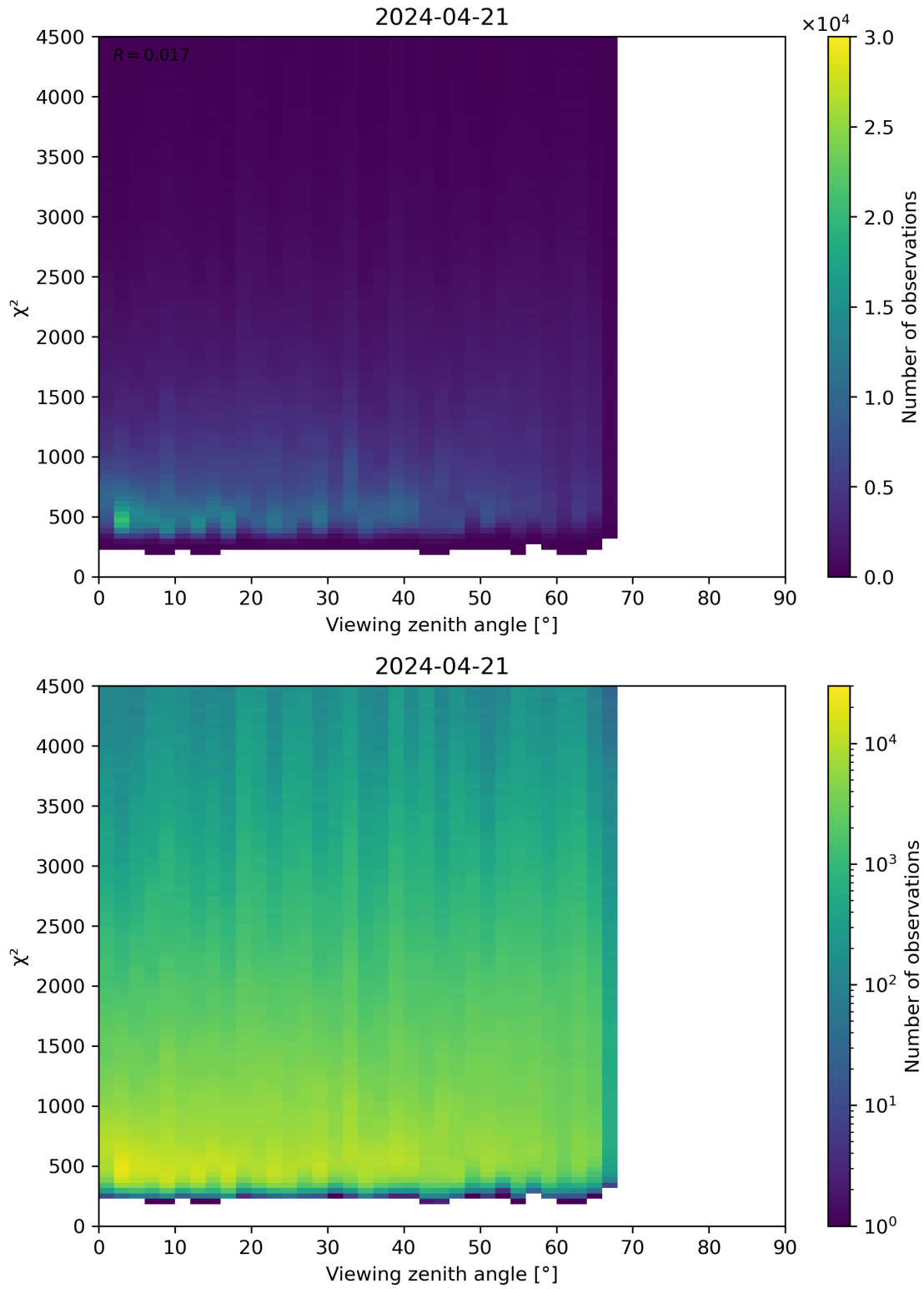
Figure 72: Scatter density plot of “Viewing zenith angle” against “ \chi^2 ” for 2024-04-21 to 2024-04-22.
