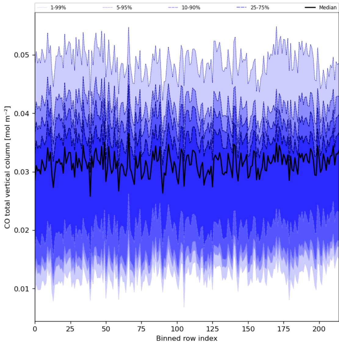
Figure 26: Along track statistics of "CO total vertical column" for 2024-04-21 to 2024-04-22
