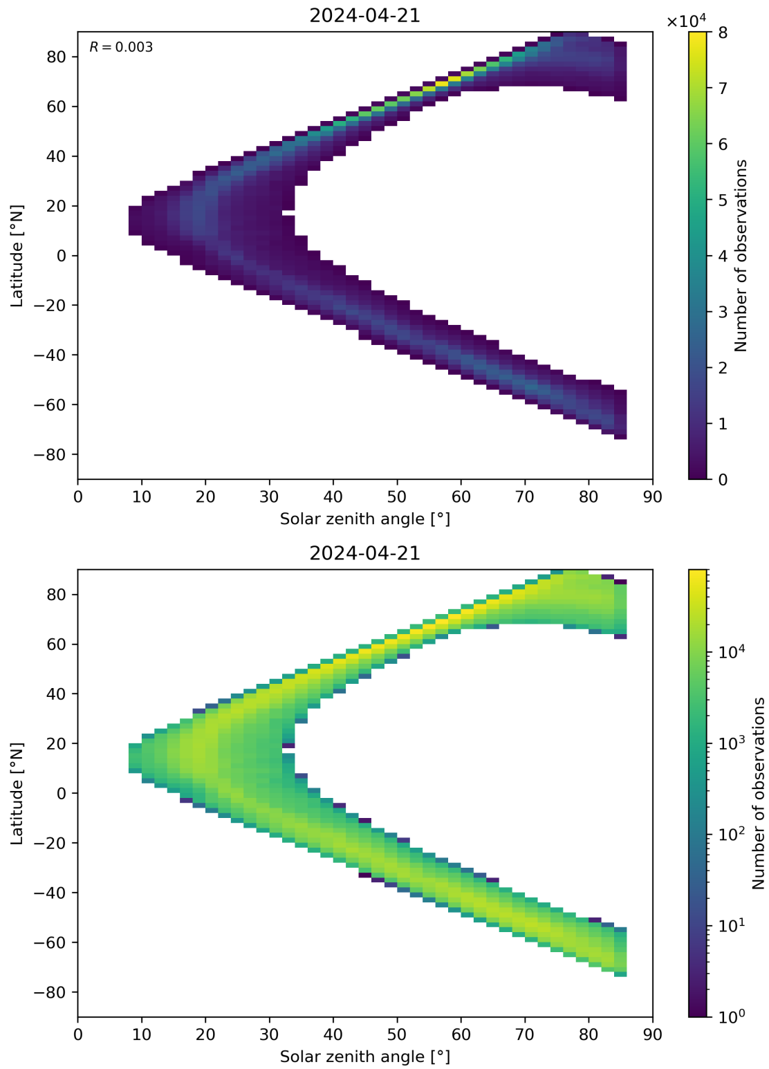
Figure 66: Scatter density plot of “Solar zenith angle” against “Latitude” for 2024-04-21 to 2024-04-22.
