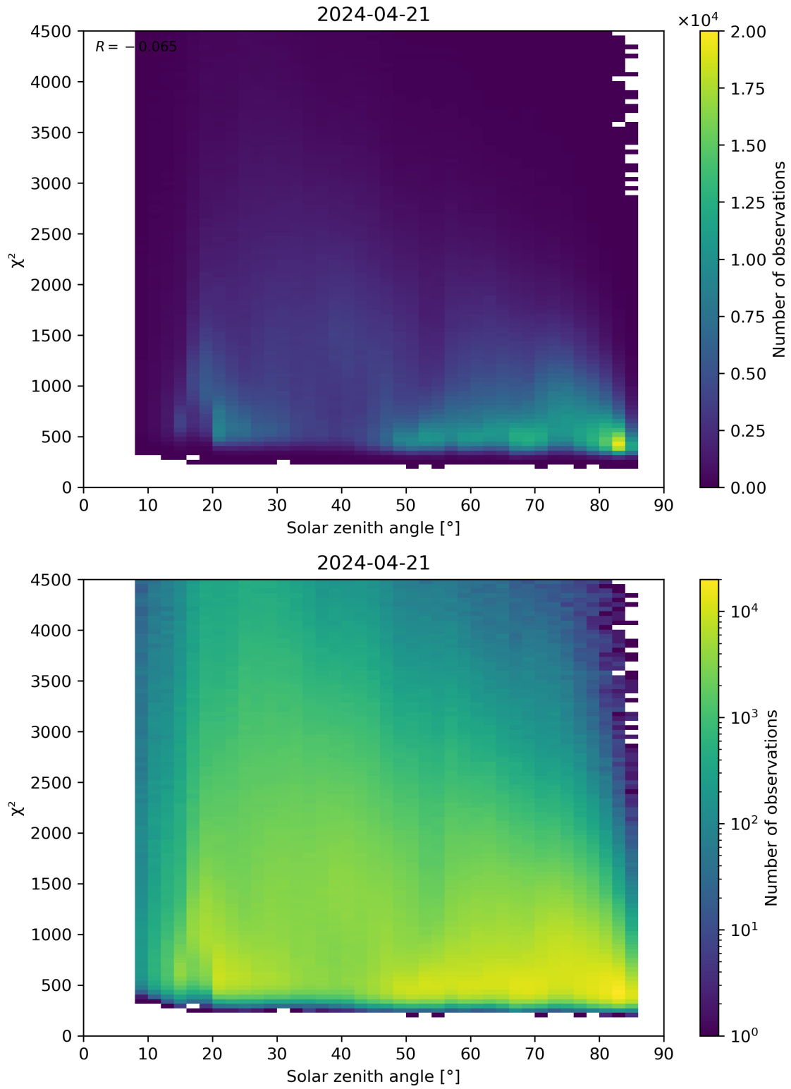
Figure 64: Scatter density plot of “Solar zenith angle” against “ \chi^2 ” for 2024-04-21 to 2024-04-22.
