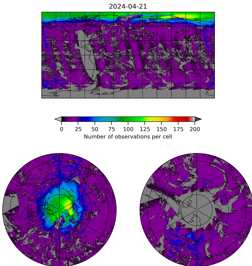
Figure 8: Map of the number of observations for 2024-04-21 to 2024-04-22
