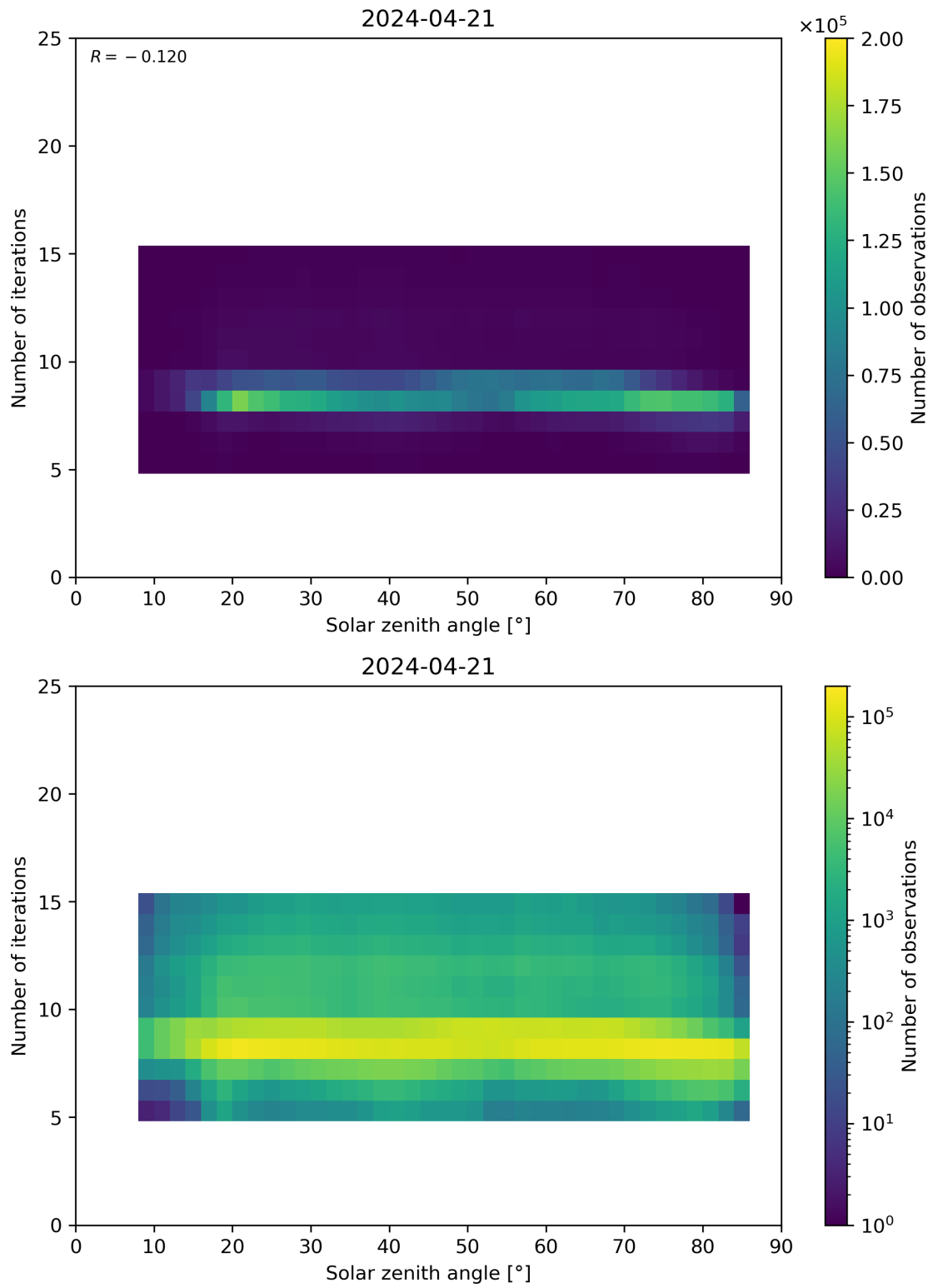
Figure 67: Scatter density plot of “Solar zenith angle” against “Number of iterations” for 2024-04-21 to 2024-04-22.
