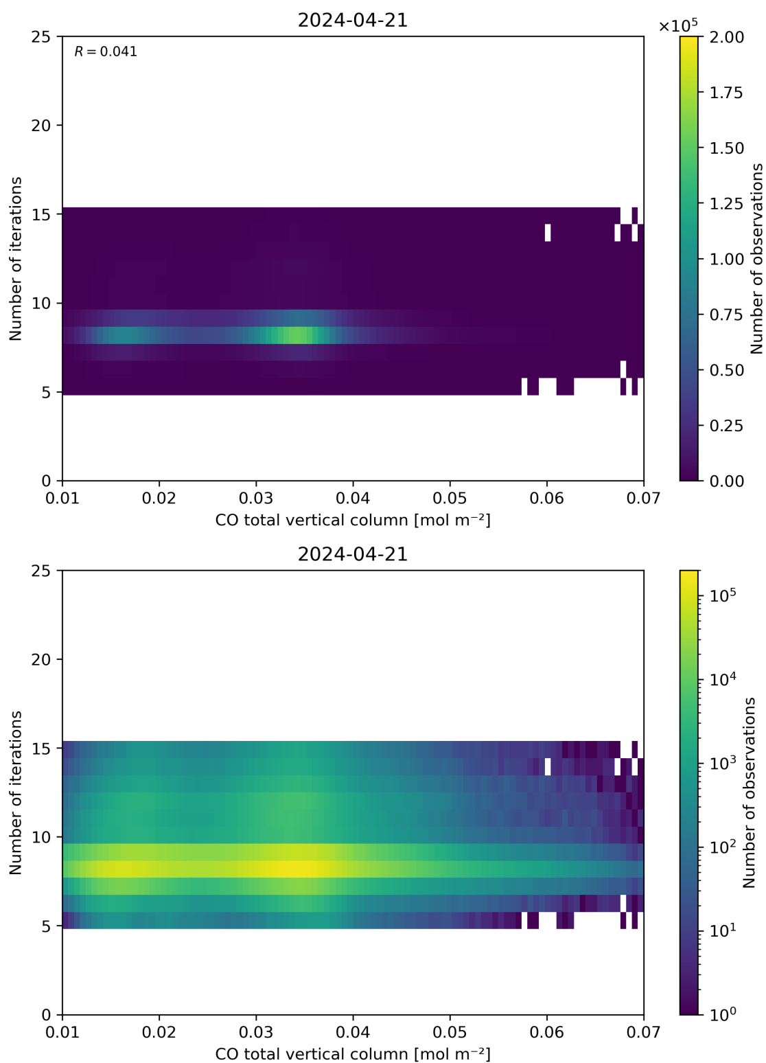
Figure 42: Scatter density plot of “CO total vertical column” against “Number of iterations” for 2024-04-21 to 2024-04-22.
