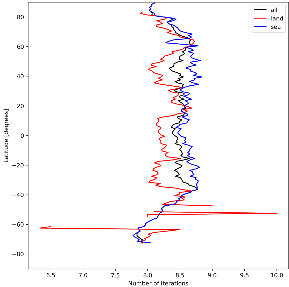
Figure 16: Zonal average of “Number of iterations” for 2024-04-21 to 2024-04-22.
