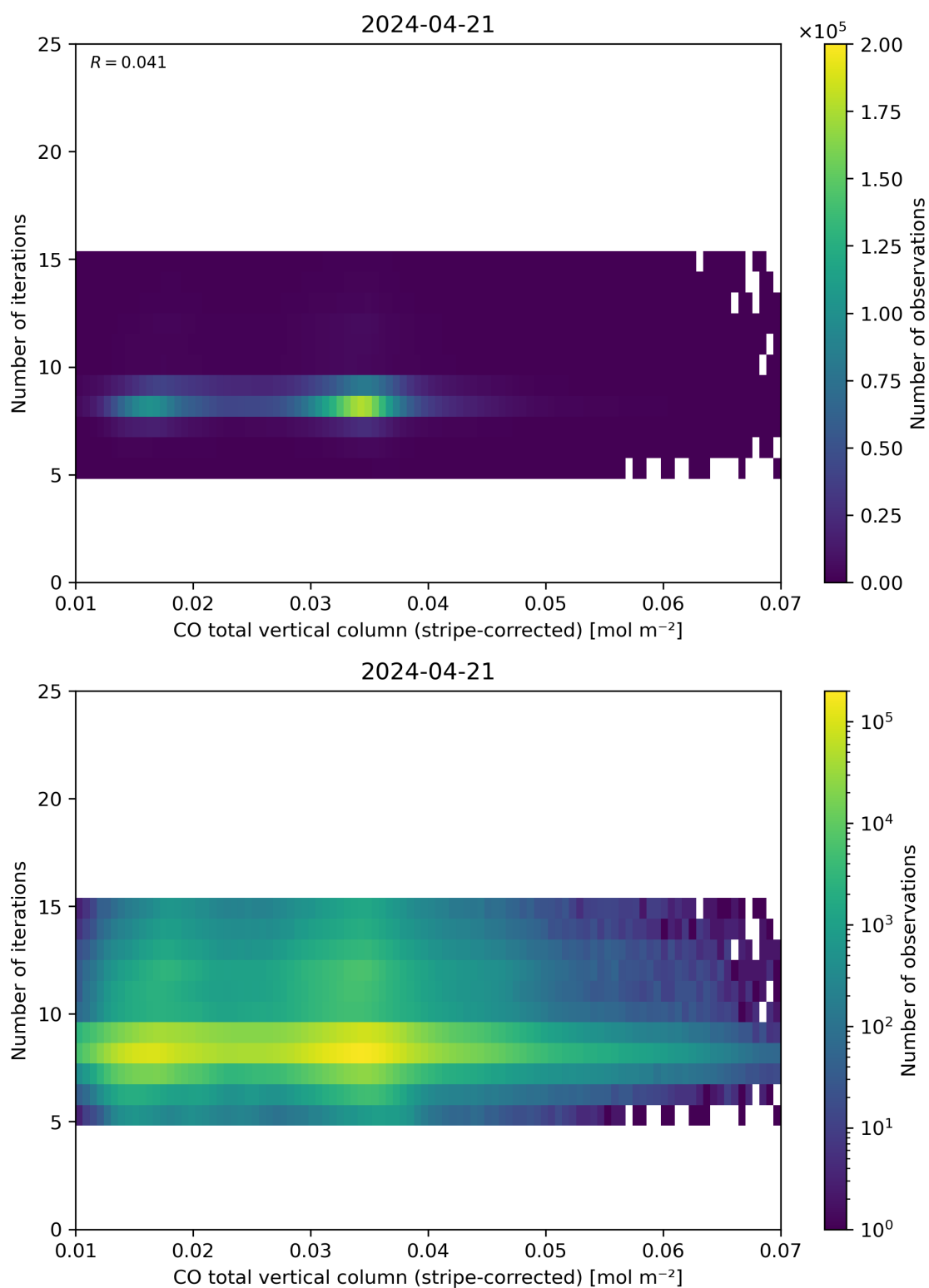
Figure 39: Scatter density plot of “CO total vertical column (stripe-corrected)” against “Number of iterations” for 2024-04-21 to 2024-04-22.
