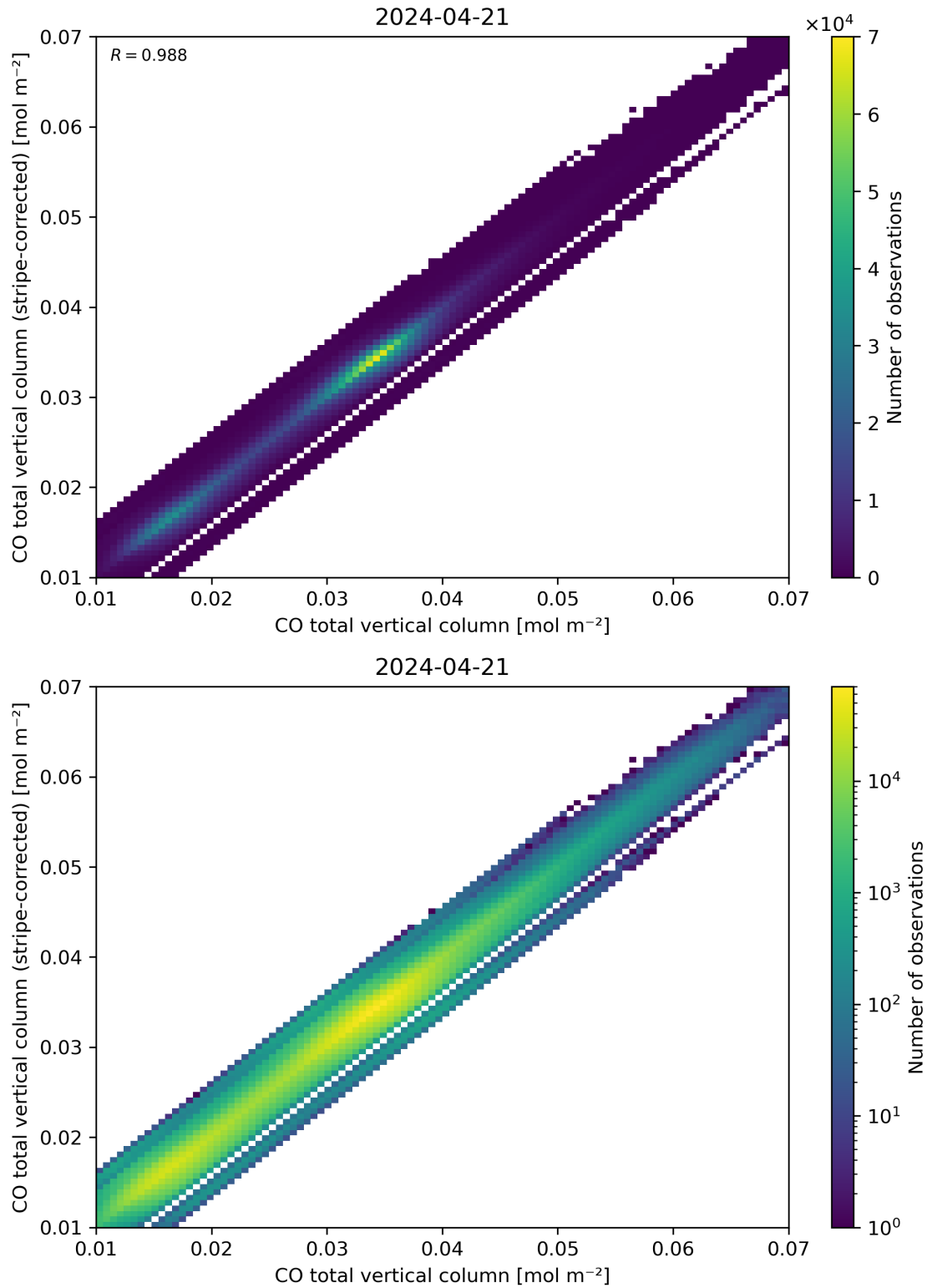
Figure 33: Scatter density plot of “CO total vertical column” against “CO total vertical column (stripe-corrected)” for 2024-04-21 to 2024-04-22.
