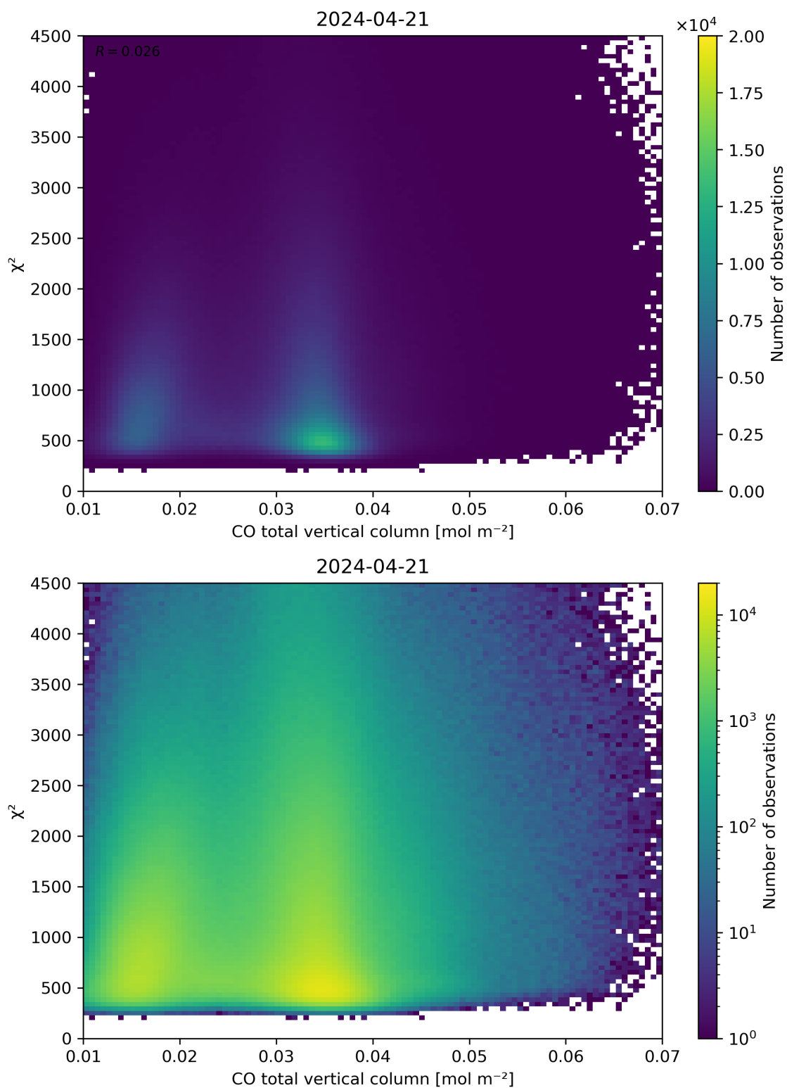
Figure 35: Scatter density plot of “CO total vertical column” against “ \chi^2 ” for 2024-04-21 to 2024-04-22.
