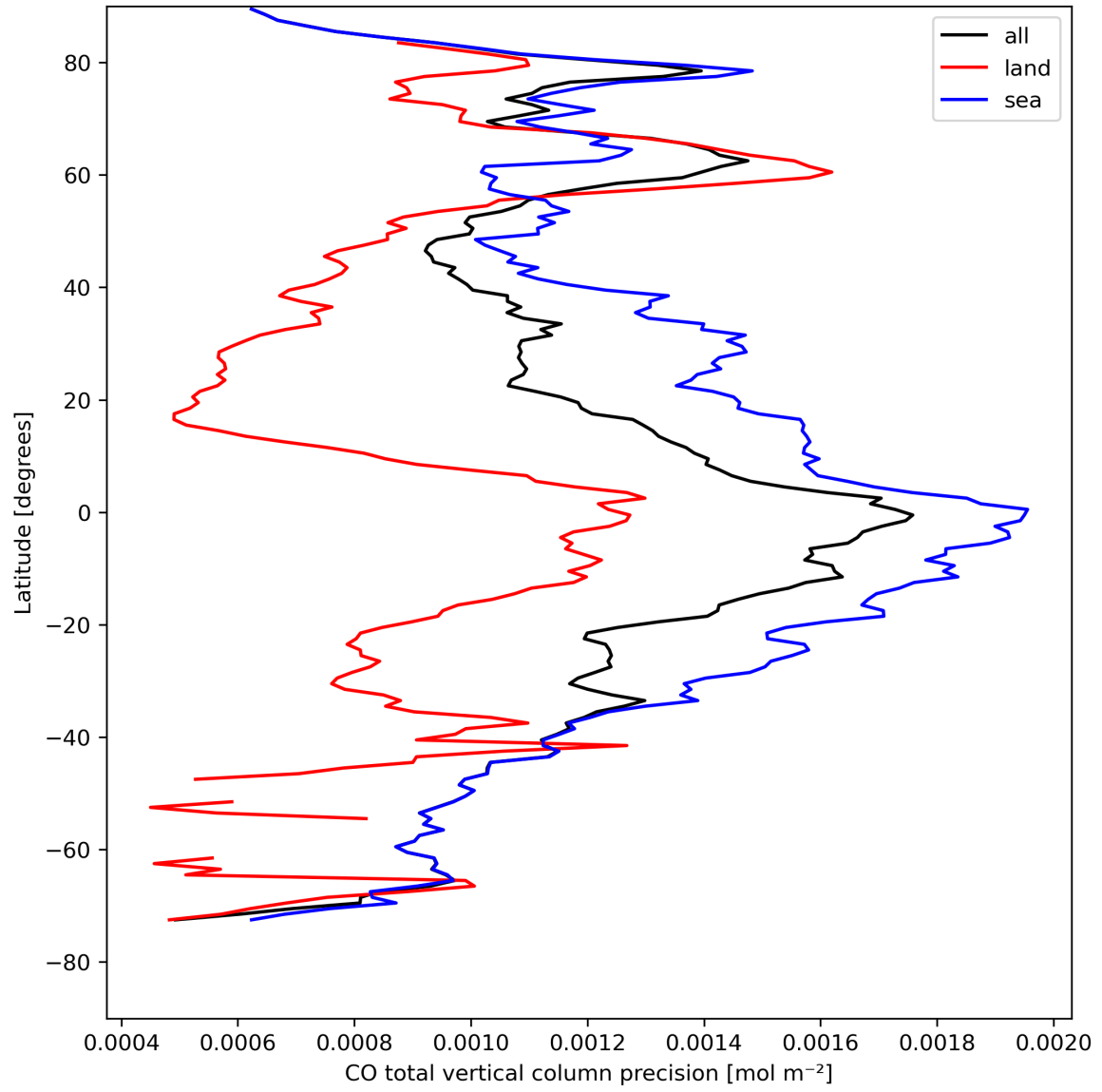
Figure 12: Zonal average of “CO total vertical column precision” for 2024-04-21 to 2024-04-22.
