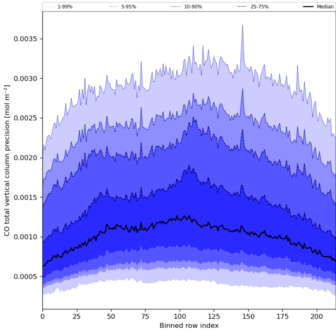
Figure 28: Along track statistics of “CO total vertical column precision” for 2024-04-21 to 2024-04-22
