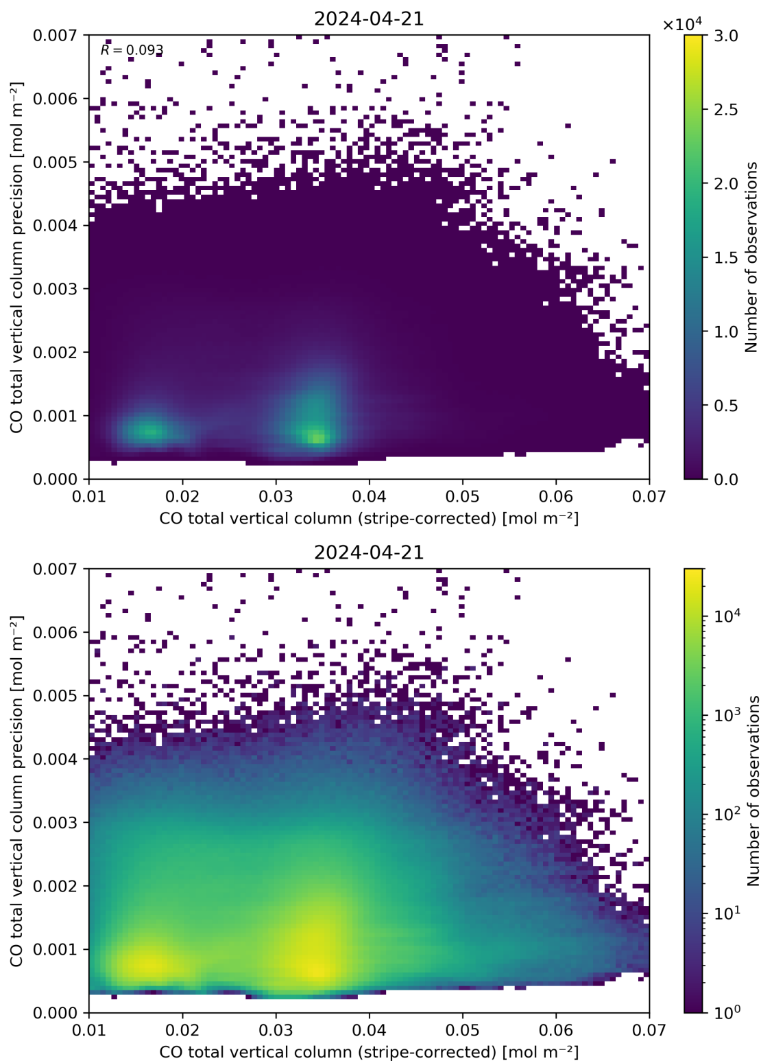
Figure 36: Scatter density plot of “CO total vertical column (stripe-corrected)” against “CO total vertical column precision” for 2024-04-21 to 2024-04-22.
