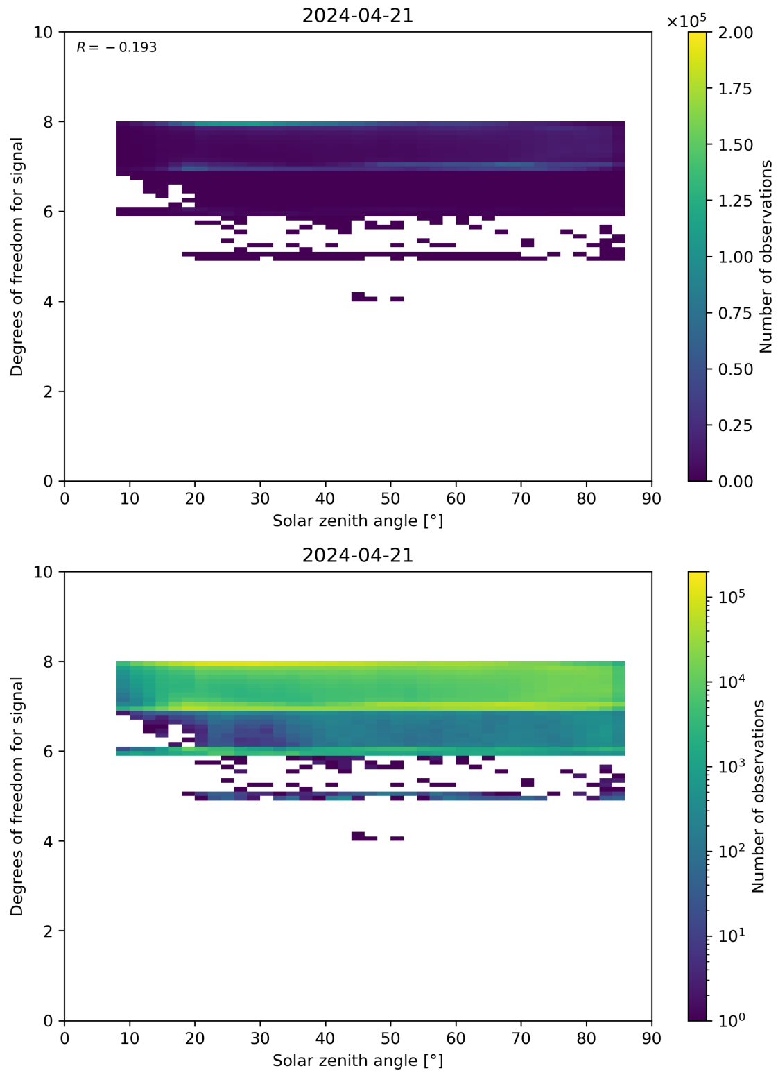
Figure 65: Scatter density plot of “Solar zenith angle” against “Degrees of freedom for signal” for 2024-04-21 to 2024-04-22.
