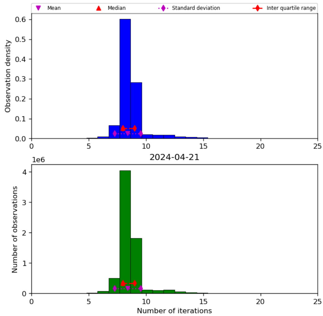
Figure 24: Histogram of “Number of iterations” for 2024-04-21 to 2024-04-22
