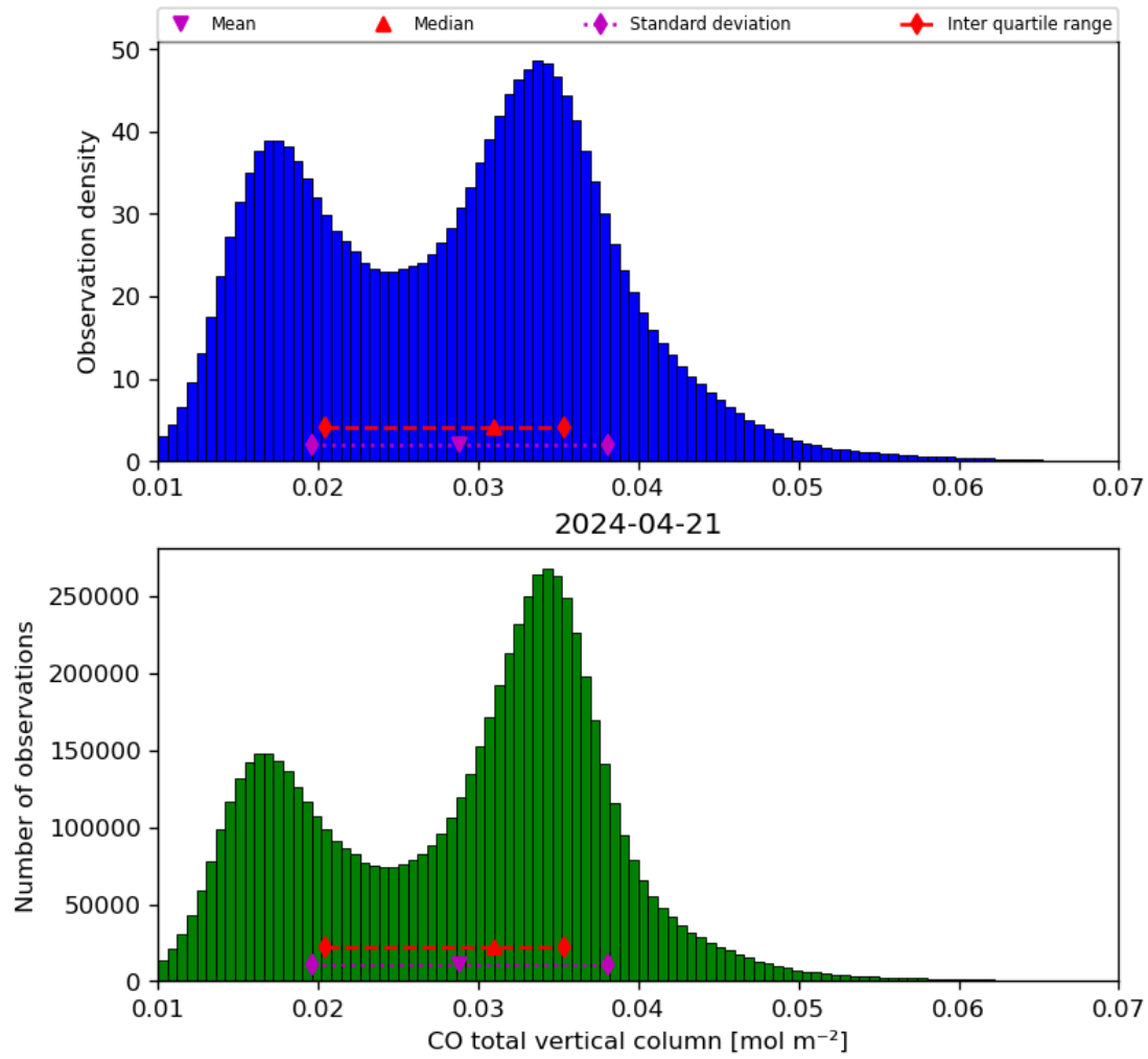
Figure 18: Histogram of “CO total vertical column” for 2024-04-21 to 2024-04-22
