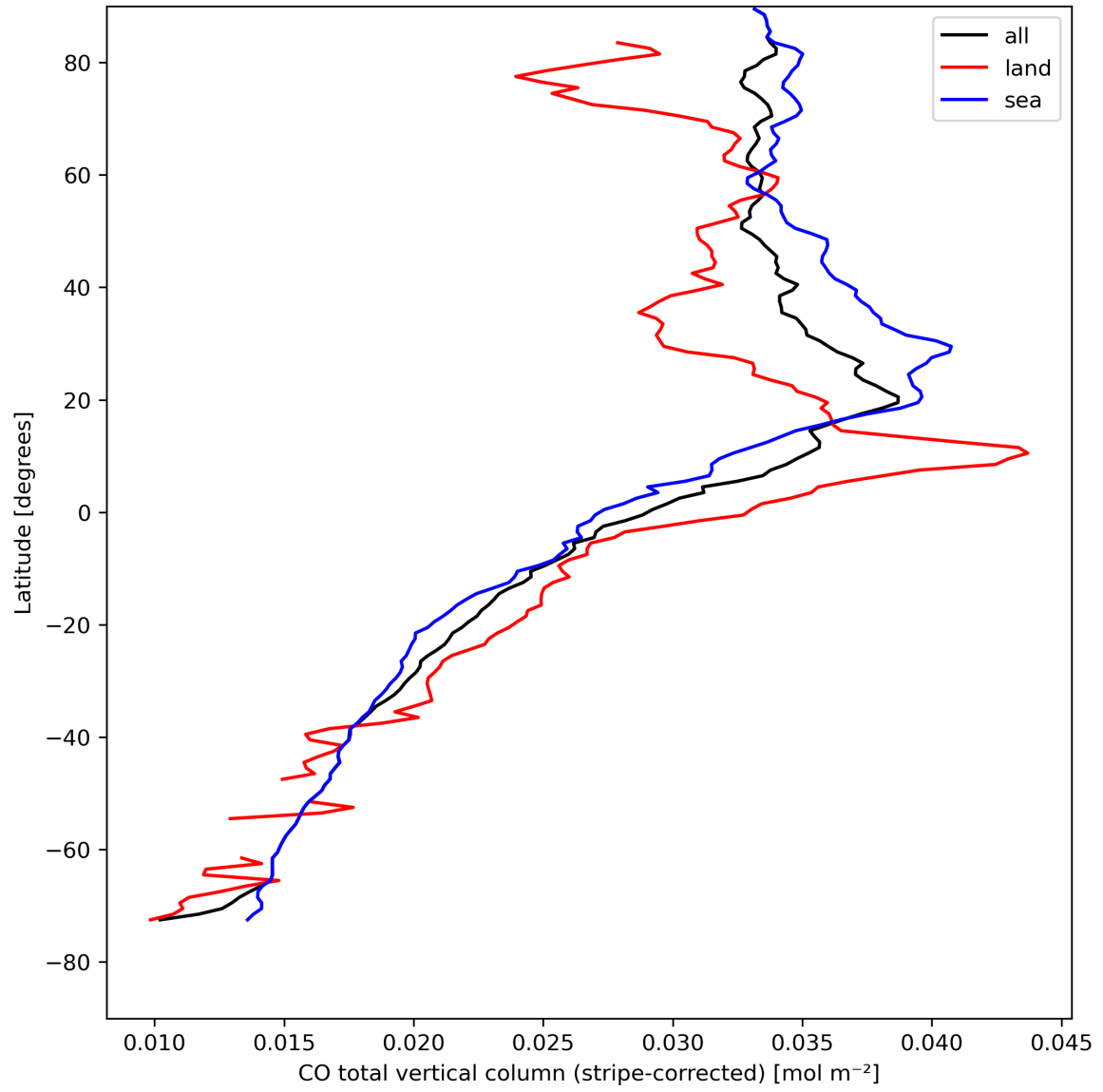
Figure 11: Zonal average of “CO total vertical column (stripe-corrected)” for 2024-04-21 to 2024-04-22.
