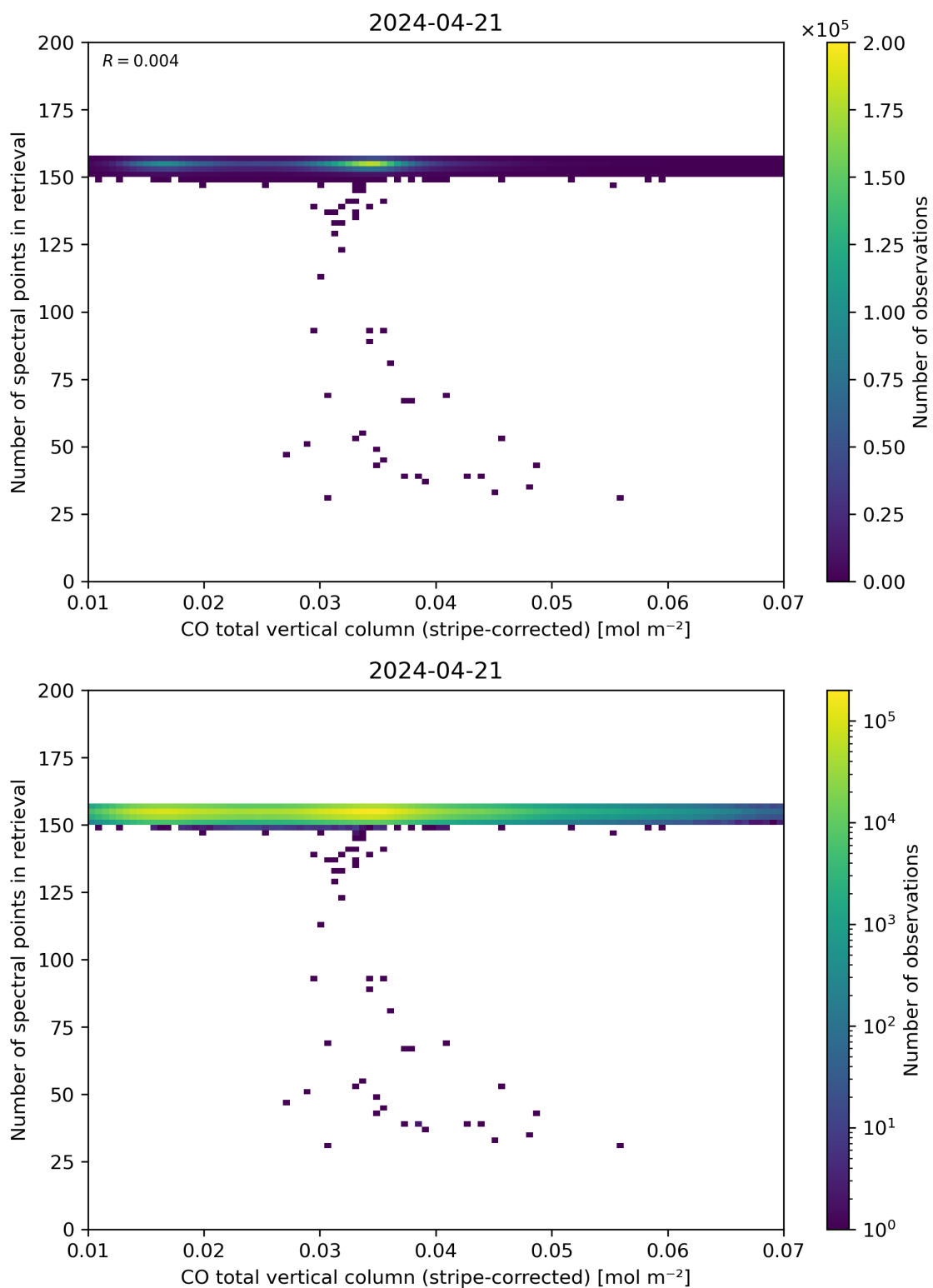
Figure 40: Scatter density plot of “CO total vertical column (stripe-corrected)” against “Number of spectral points in retrieval” for 2024-04-21 to 2024-04-22.
