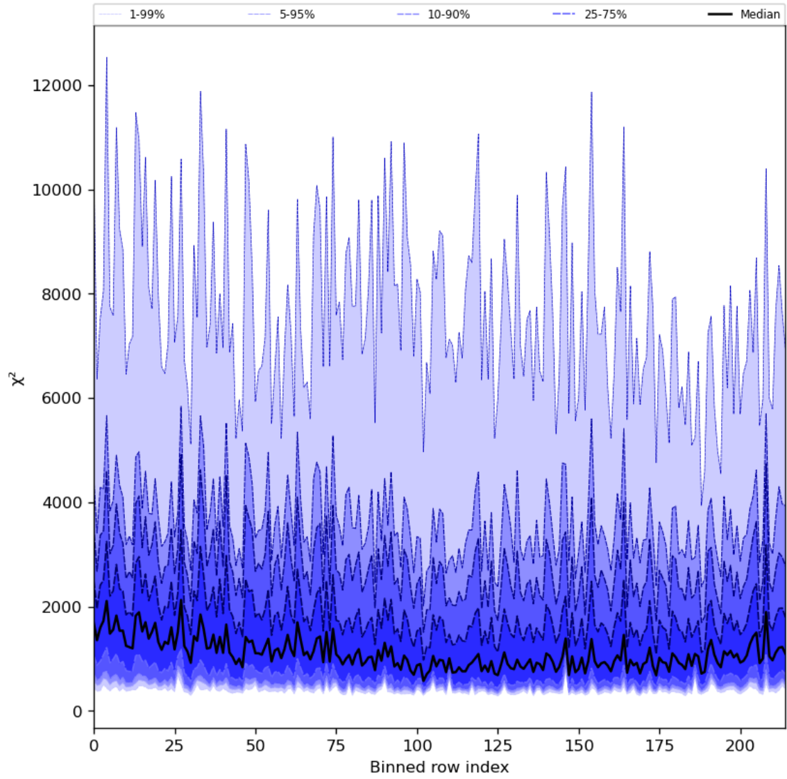
Figure 30: Along track statistics of “ \chi^2 ” for 2024-04-21 to 2024-04-22
