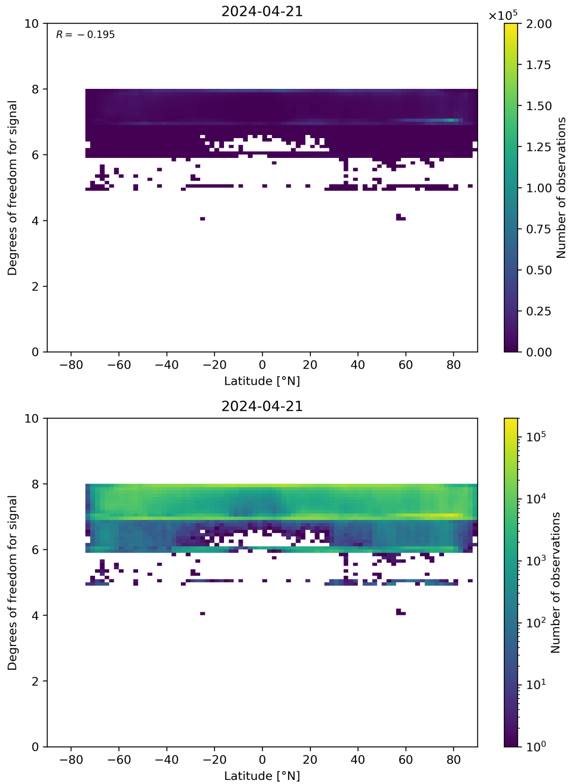
Figure 55: Scatter density plot of “Latitude” against “Degrees of freedom for signal” for 2024-04-21 to 2024-04-22.
