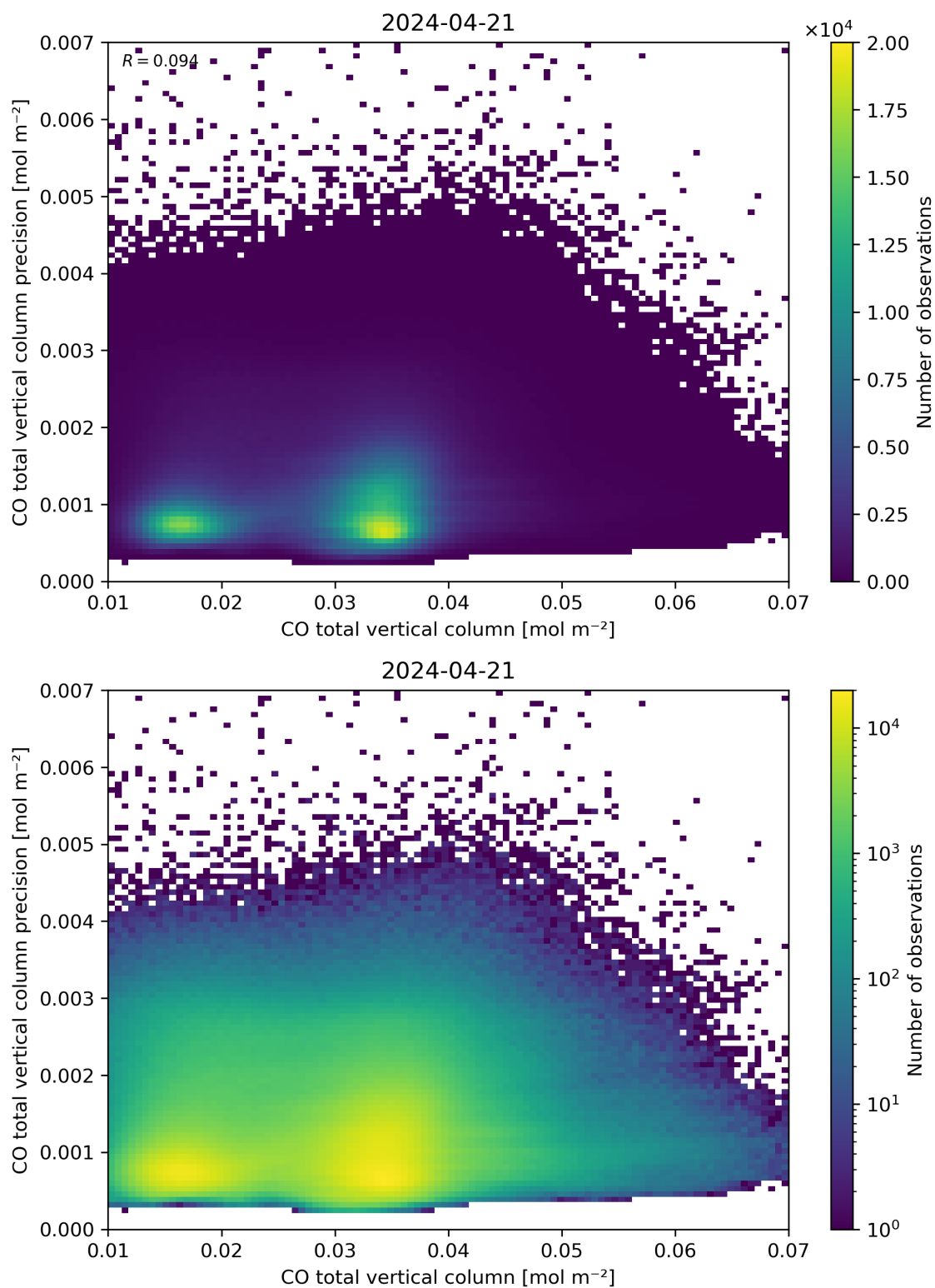
Figure 34: Scatter density plot of “CO total vertical column” against “CO total vertical column precision” for 2024-04-21 to 2024-04-22.
