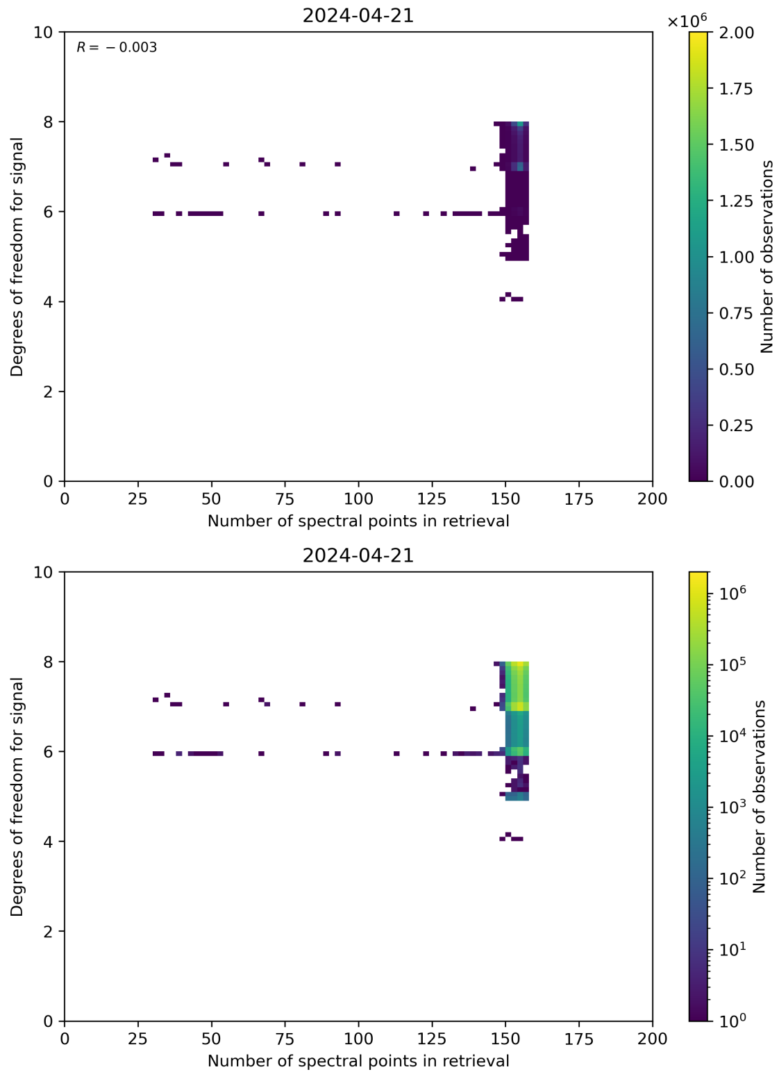
Figure 59: Scatter density plot of “Number of spectral points in retrieval” against “Degrees of freedom for signal” for 2024-04-21 to 2024-04-22.
