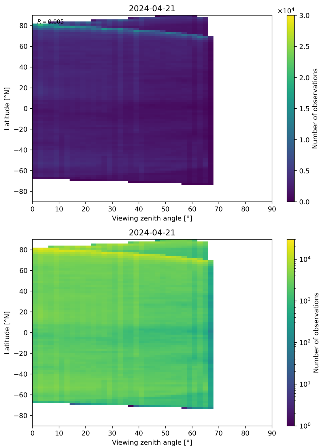
Figure 74: Scatter density plot of “Viewing zenith angle” against “Latitude” for 2024-04-21 to 2024-04-22.
