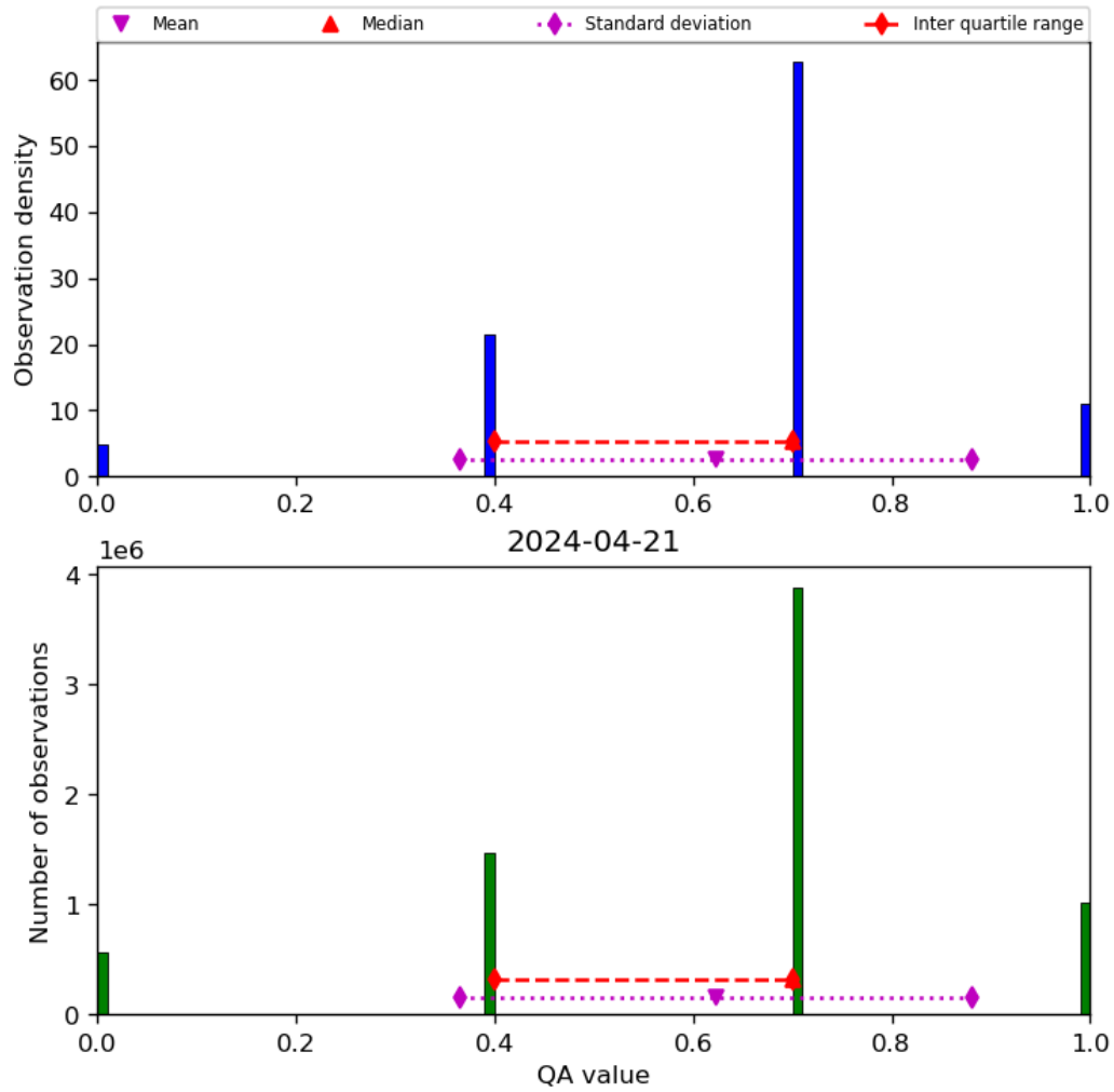
Figure 17: Histogram of “QA value” for 2024-04-21 to 2024-04-22
