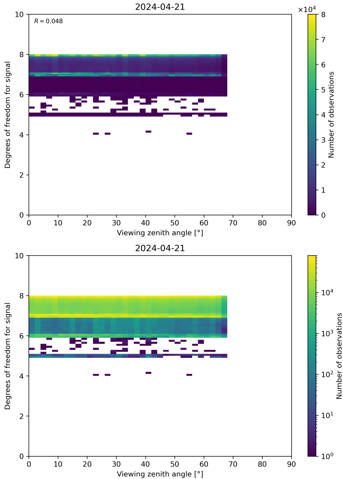
Figure 73: Scatter density plot of “Viewing zenith angle” against “Degrees of freedom for signal” for 2024-04-21 to 2024-04-22.
