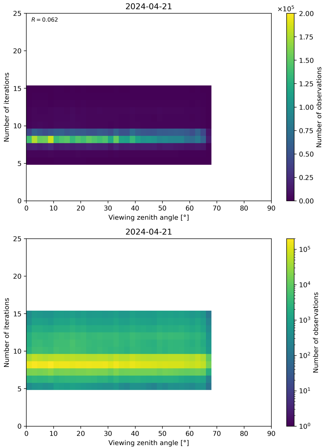
Figure 75: Scatter density plot of “Viewing zenith angle” against “Number of iterations” for 2024-04-21 to 2024-04-22.
