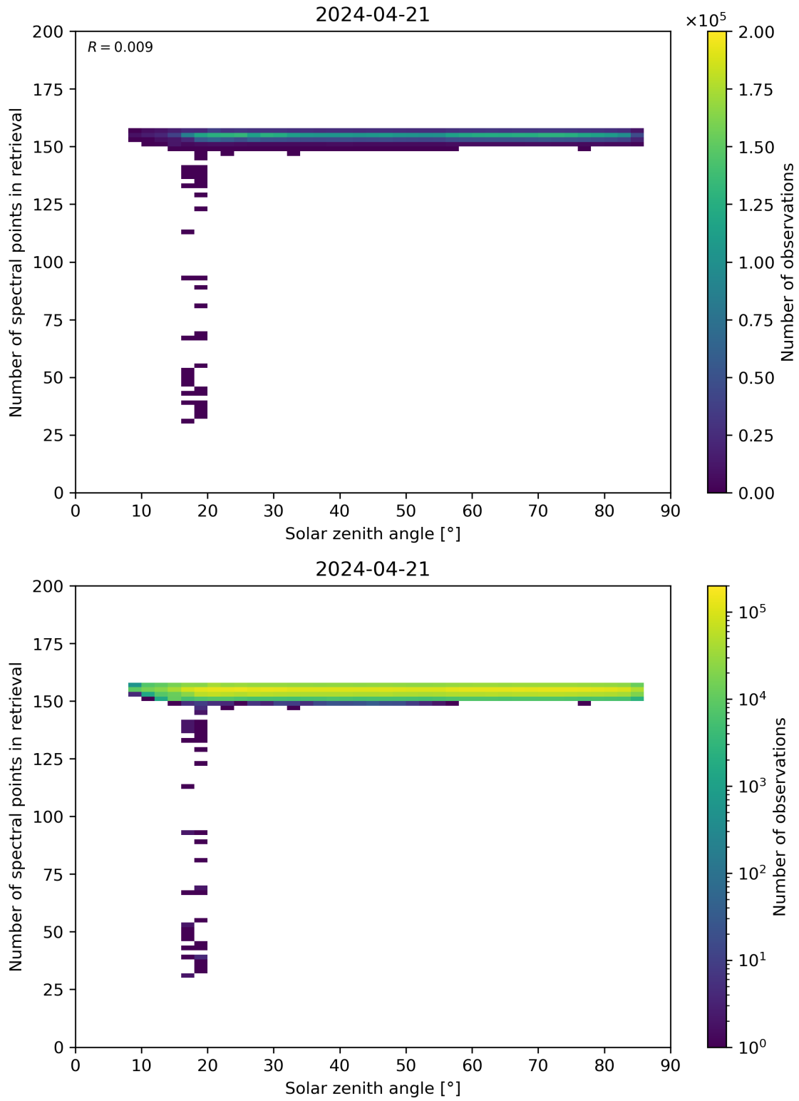
Figure 68: Scatter density plot of “Solar zenith angle” against “Number of spectral points in retrieval” for 2024-04-21 to 2024-04-22.
