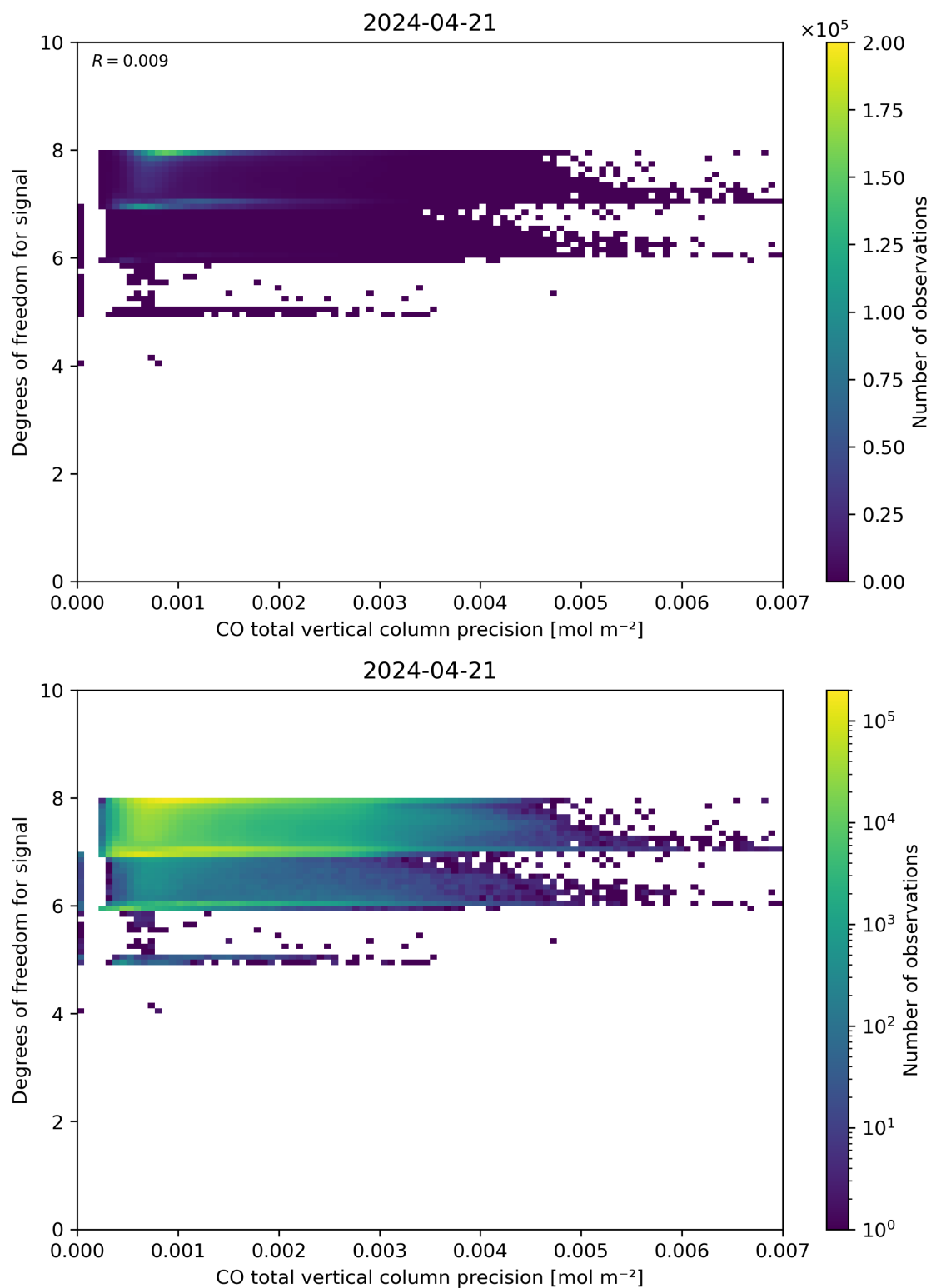
Figure 45: Scatter density plot of “CO total vertical column precision” against “Degrees of freedom for signal” for 2024-04-21 to 2024-04-22.
