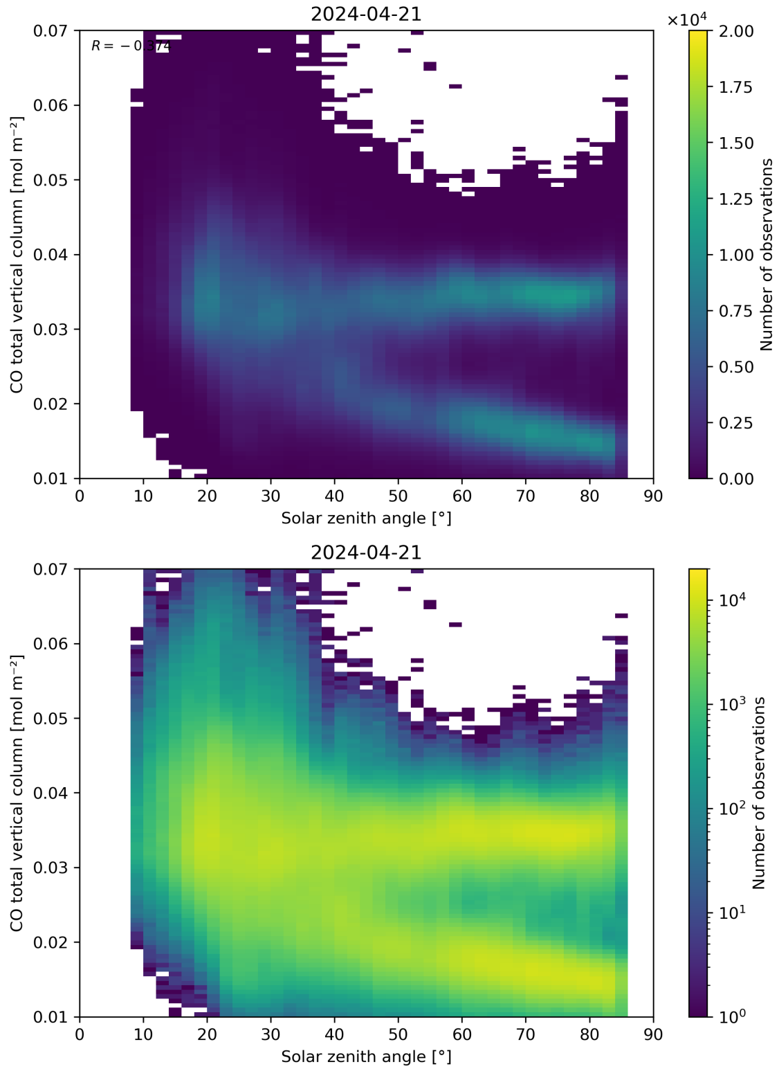
Figure 61: Scatter density plot of “Solar zenith angle” against “CO total vertical column” for 2024-04-21 to 2024-04-22.
