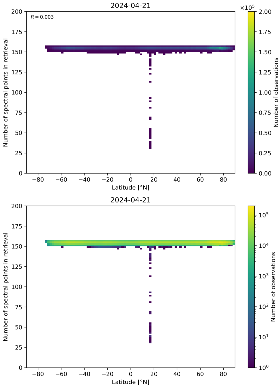
Figure 57: Scatter density plot of “Latitude” against “Number of spectral points in retrieval” for 2024-04-21 to 2024-04-22.
