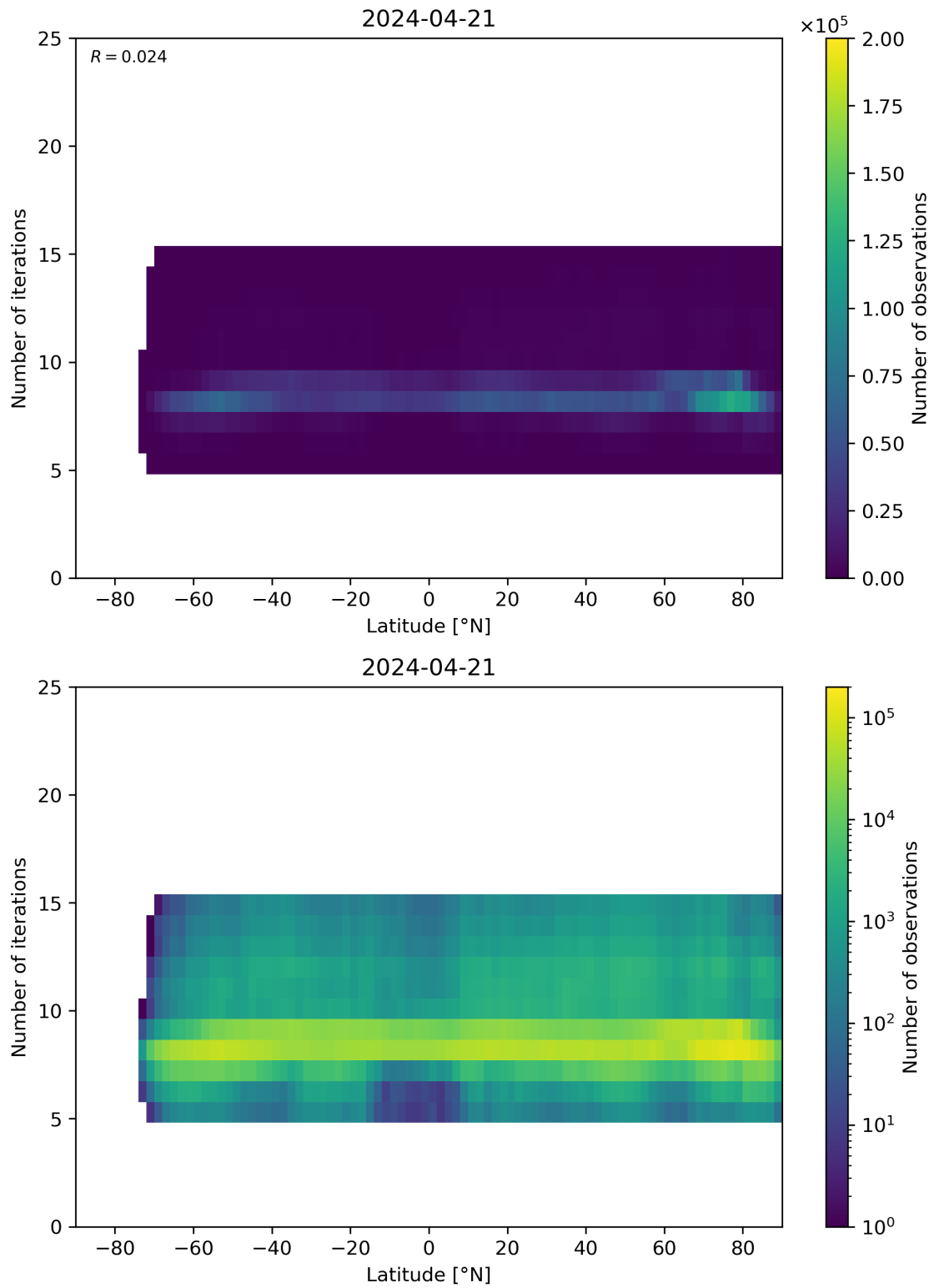
Figure 56: Scatter density plot of “Latitude” against “Number of iterations” for 2024-04-21 to 2024-04-22.
