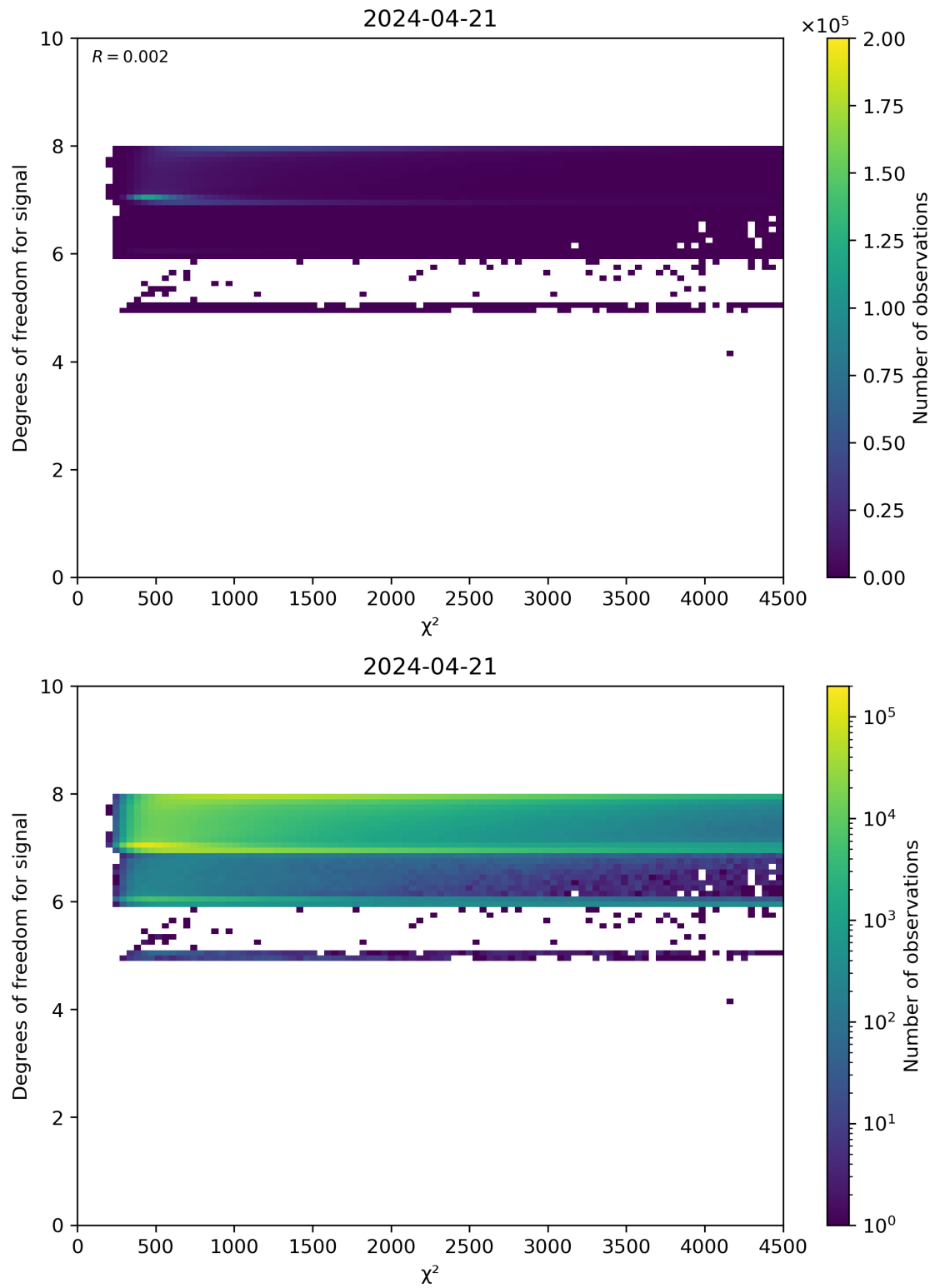
Figure 48: Scatter density plot of " \chi^2 " against "Degrees of freedom for signal" for 2024-04-21 to 2024-04-22.
