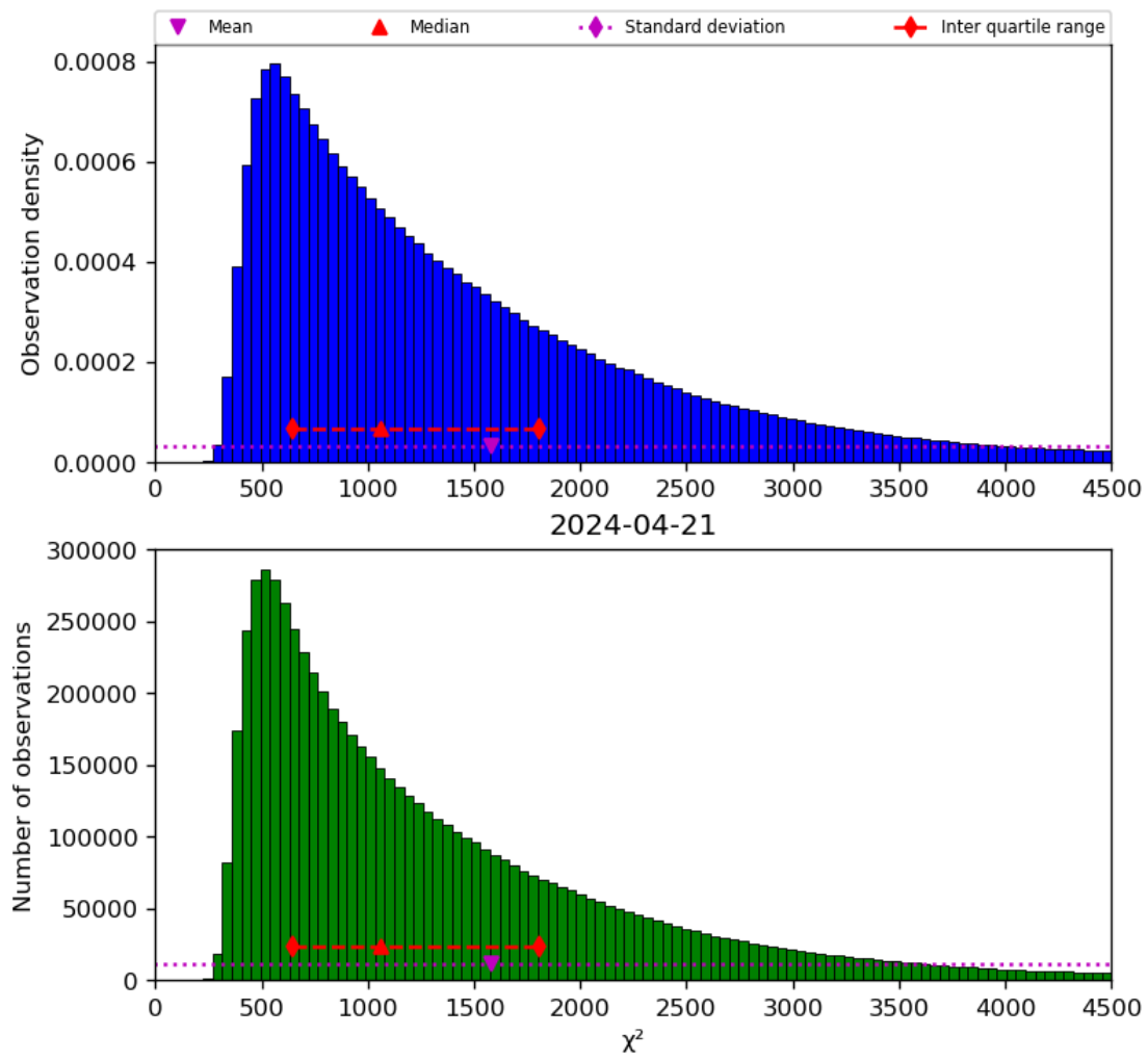
Figure 22: Histogram of “ \chi^2 ” for 2024-04-21 to 2024-04-22
