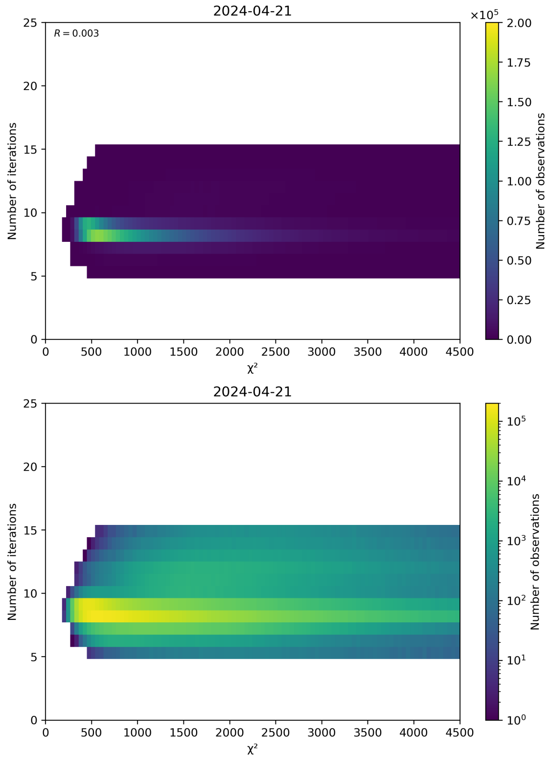
Figure 49: Scatter density plot of “ \chi^2 ” against “Number of iterations” for 2024-04-21 to 2024-04-22.
