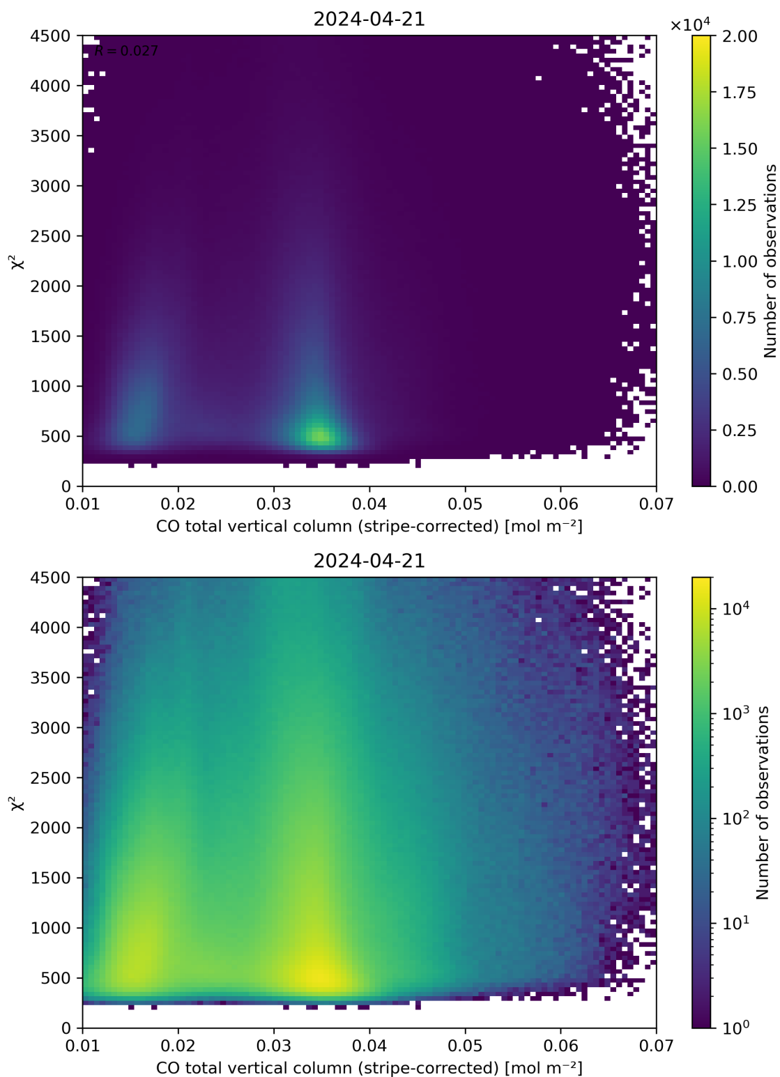
Figure 37: Scatter density plot of “CO total vertical column (stripe-corrected)” against “ \chi^2 ” for 2024-04-21 to 2024-04-22.
