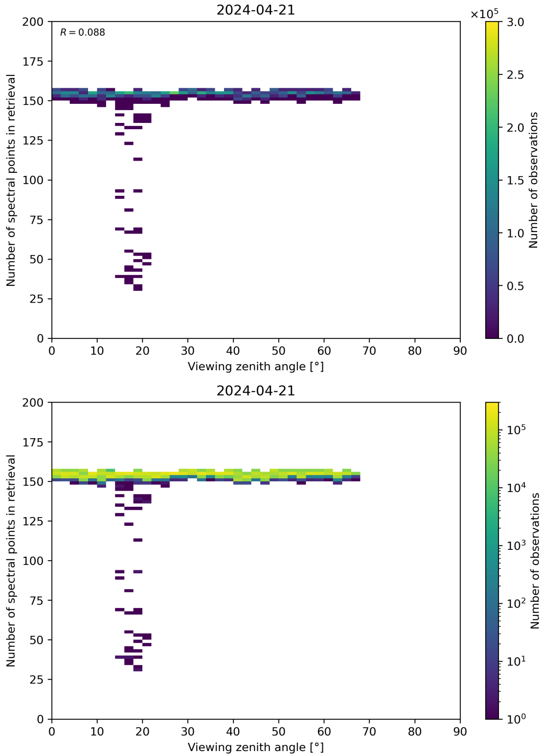
Figure 76: Scatter density plot of “Viewing zenith angle” against “Number of spectral points in retrieval” for 2024-04-21 to 2024-04-22.
