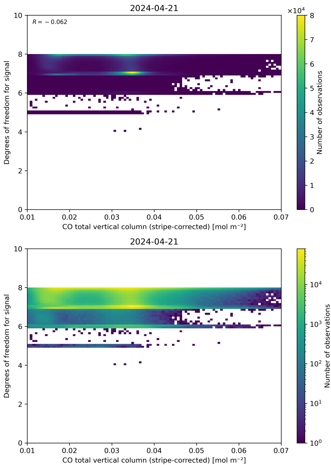
Figure 38: Scatter density plot of “CO total vertical column (stripe-corrected)” against “Degrees of freedom for signal” for 2024-04-21 to 2024-04-22.
