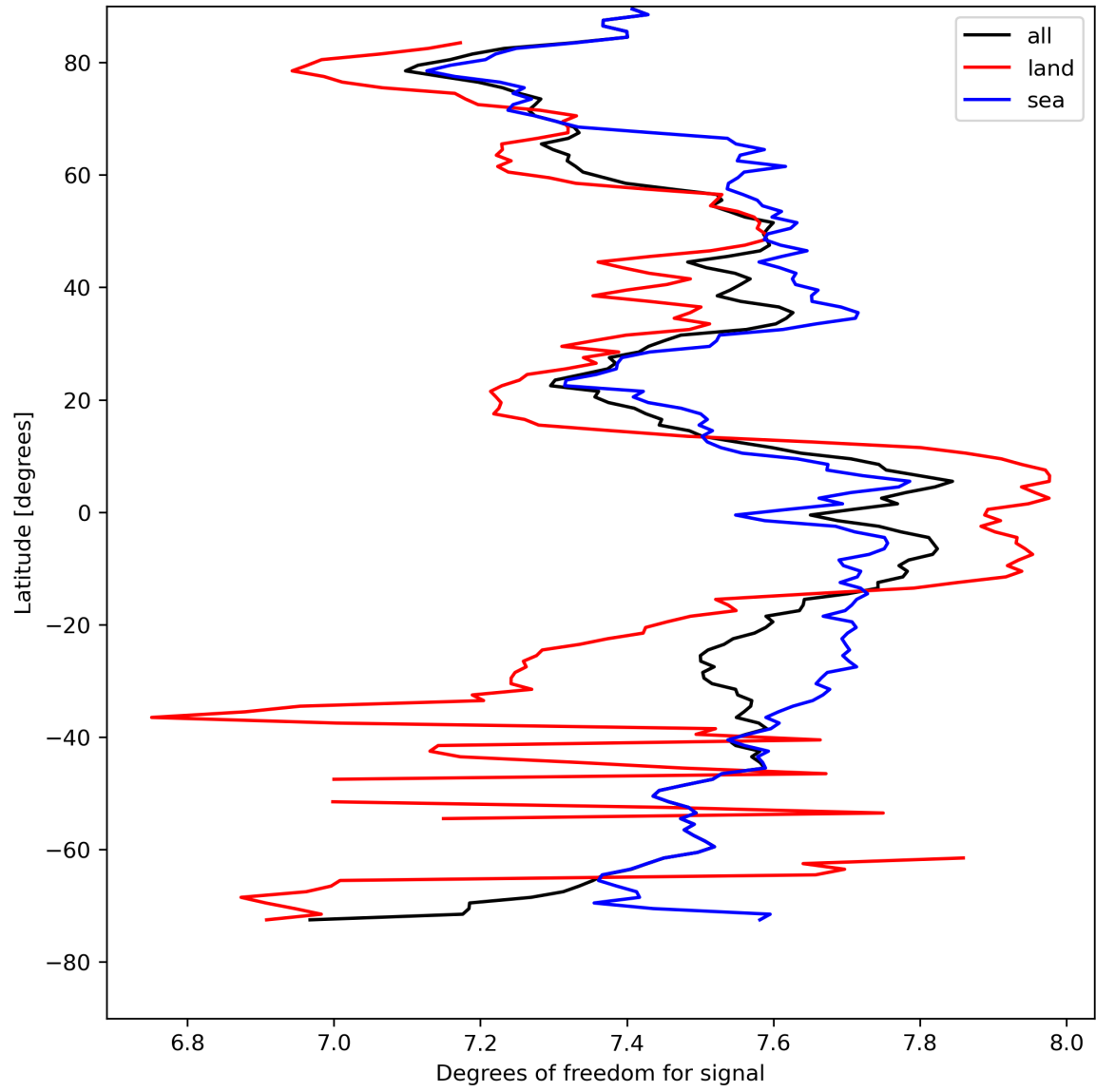
Figure 15: Zonal average of “Degrees of freedom for signal” for 2024-04-21 to 2024-04-22.
