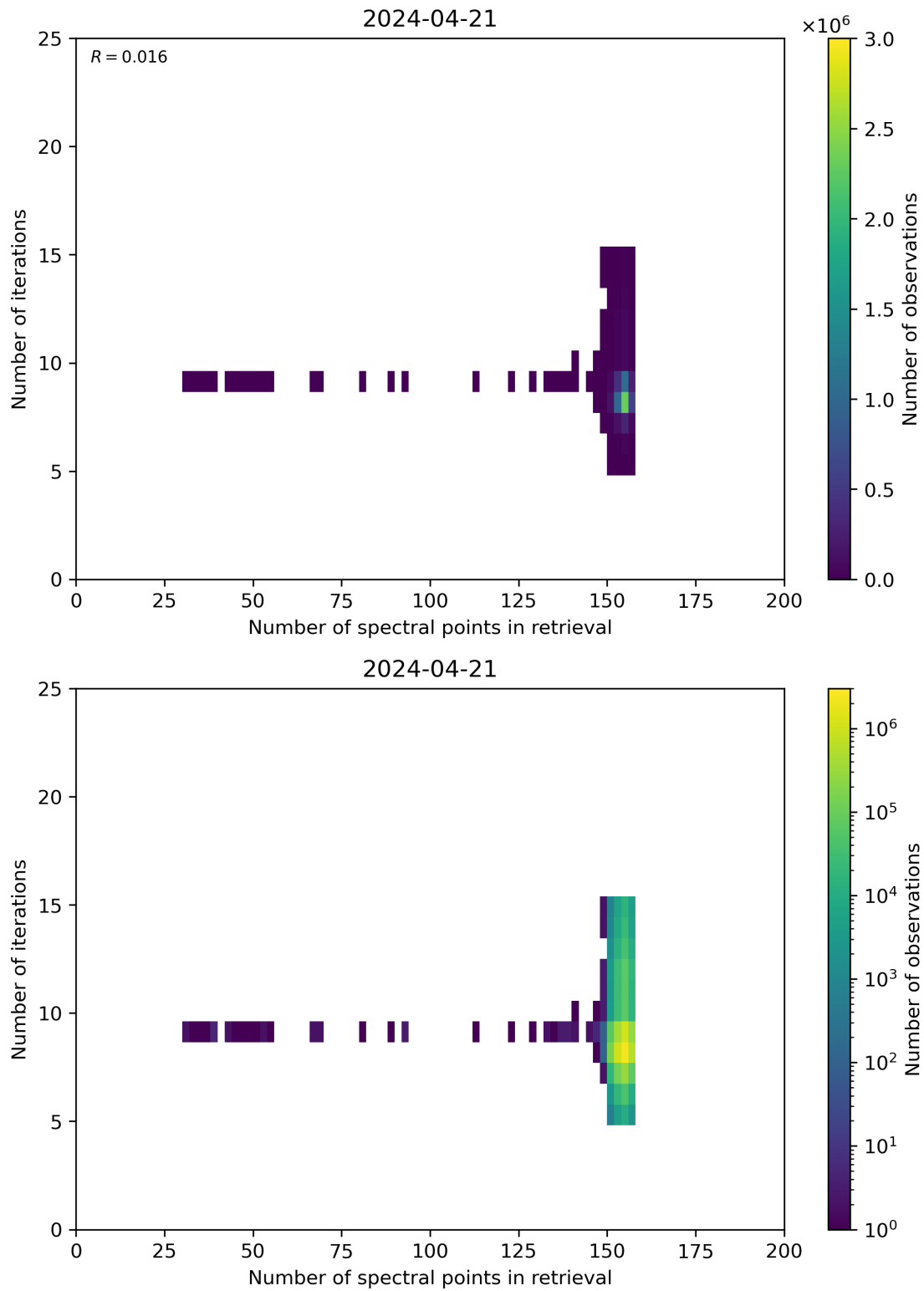
Figure 60: Scatter density plot of “Number of spectral points in retrieval” against “Number of iterations” for 2024-04-21 to 2024-04-22.
