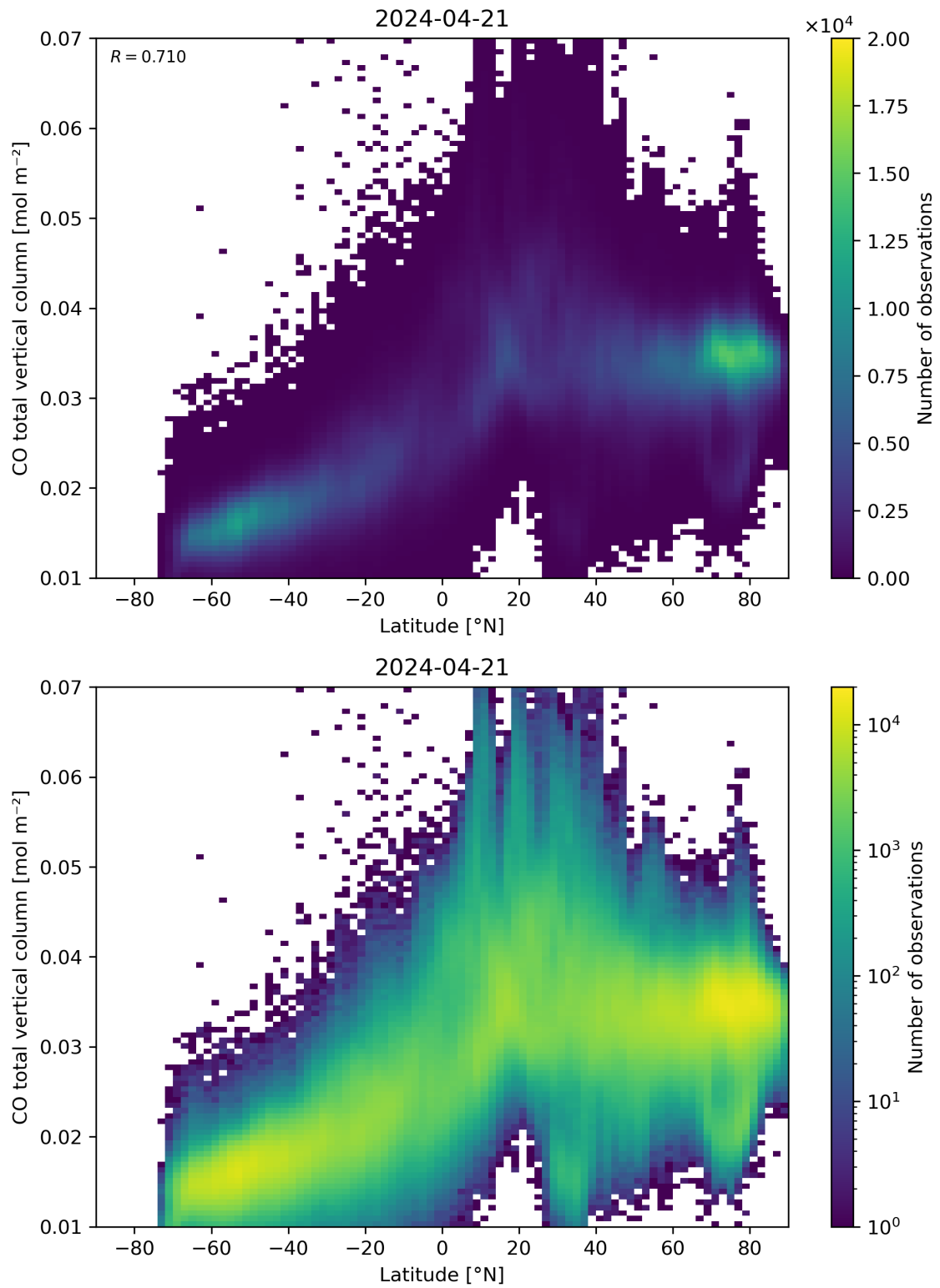
Figure 51: Scatter density plot of “Latitude” against “CO total vertical column” for 2024-04-21 to 2024-04-22.
