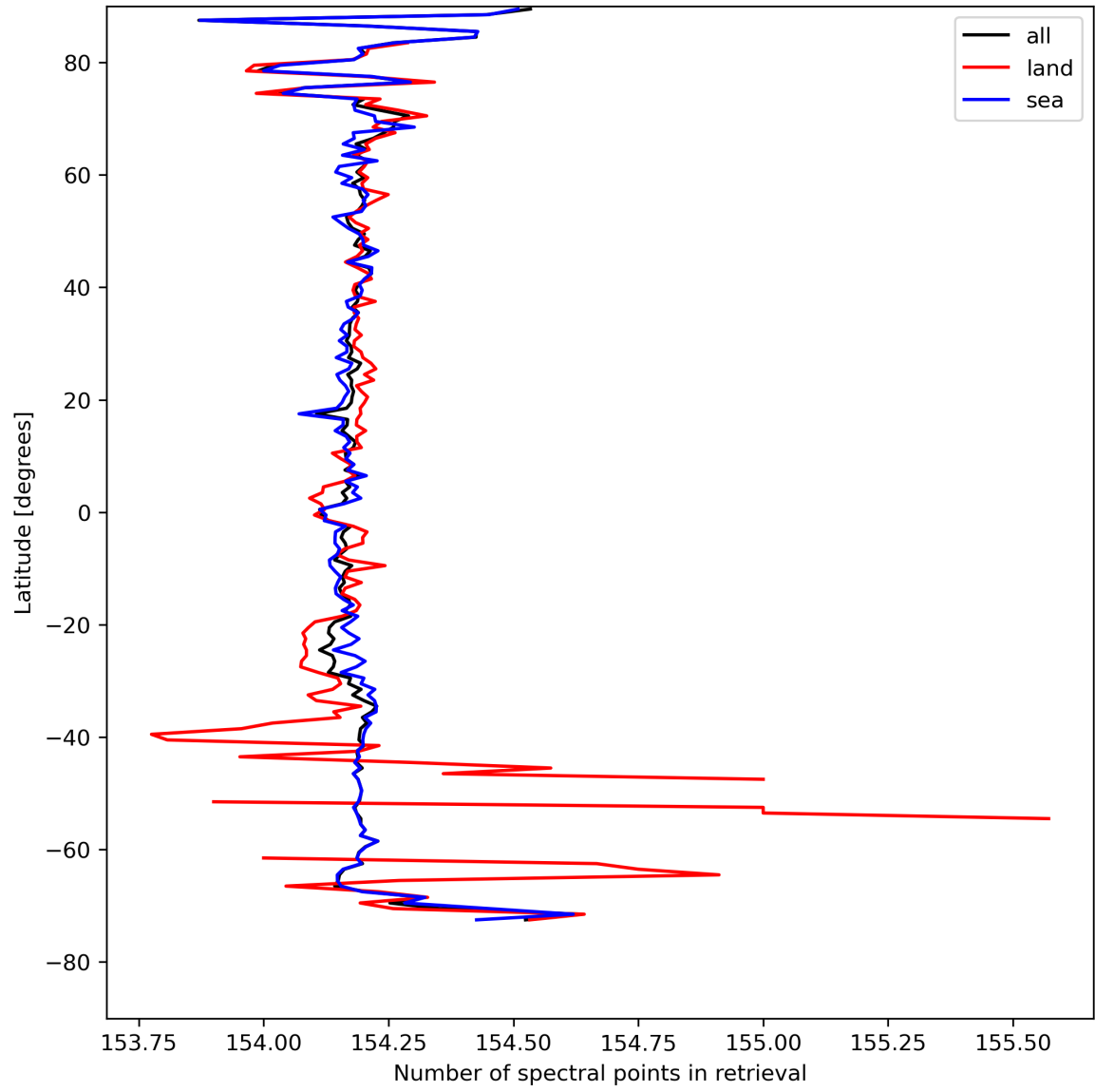
Figure 13: Zonal average of “Number of spectral points in retrieval” for 2024-04-21 to 2024-04-22.
