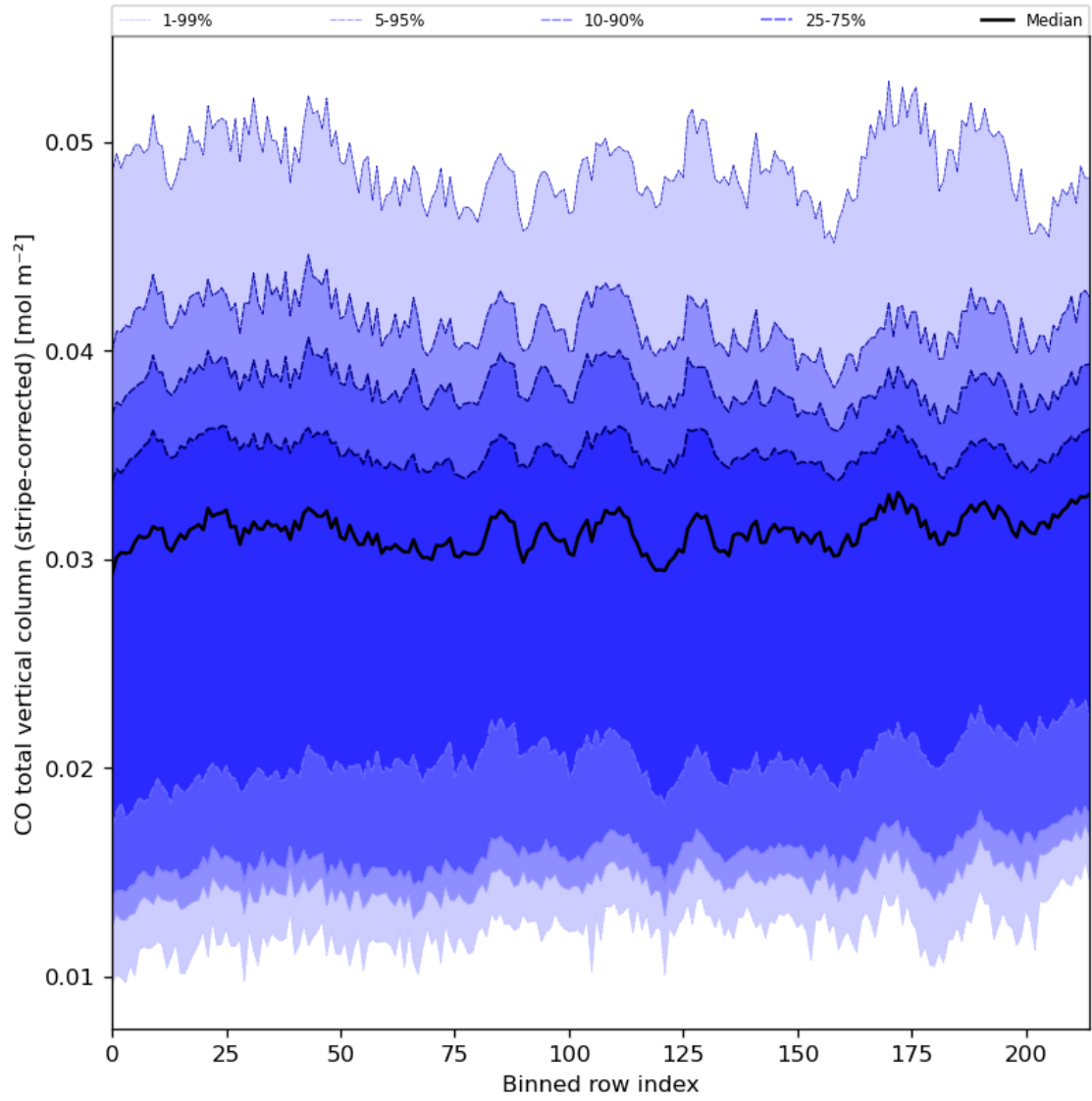
Figure 27: Along track statistics of “CO total vertical column (stripe-corrected)” for 2024-04-21 to 2024-04-22
