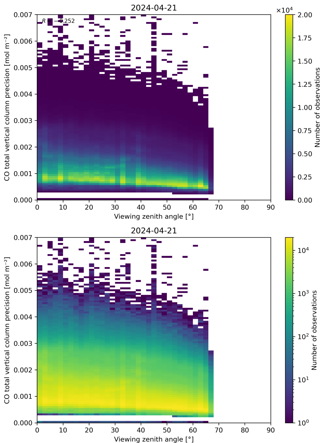
Figure 71: Scatter density plot of “Viewing zenith angle” against “CO total vertical column precision” for 2024-04-21 to 2024-04-22.
