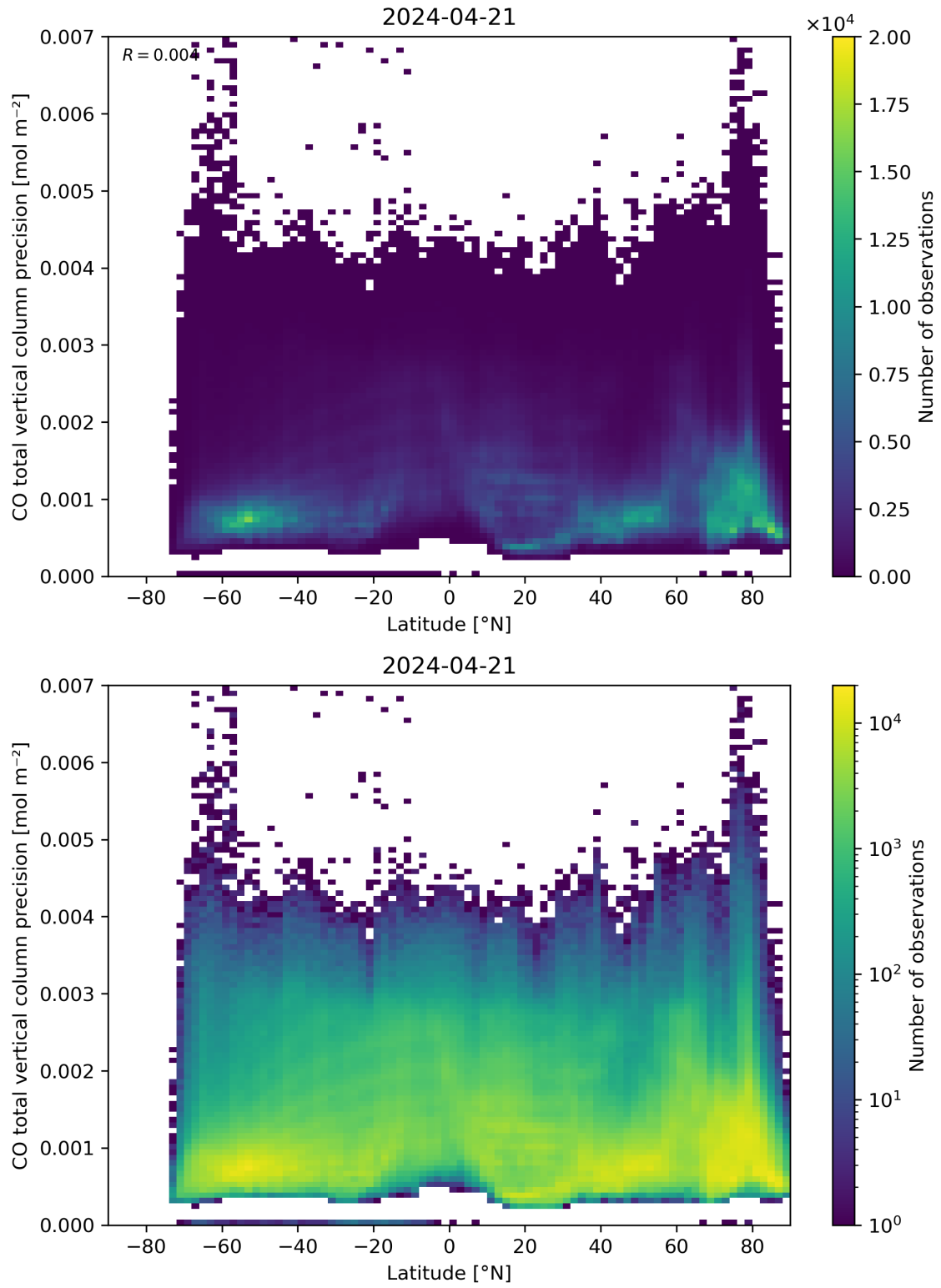
Figure 53: Scatter density plot of “Latitude” against “CO total vertical column precision” for 2024-04-21 to 2024-04-22.
