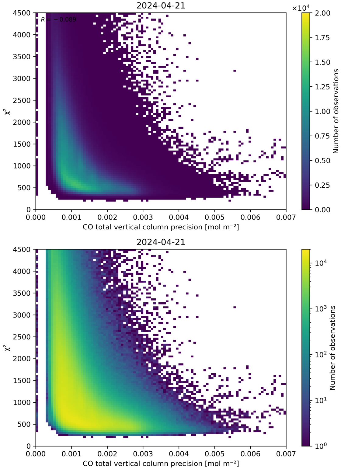
Figure 44: Scatter density plot of “CO total vertical column precision” against “ \chi^2 ” for 2024-04-21 to 2024-04-22.
