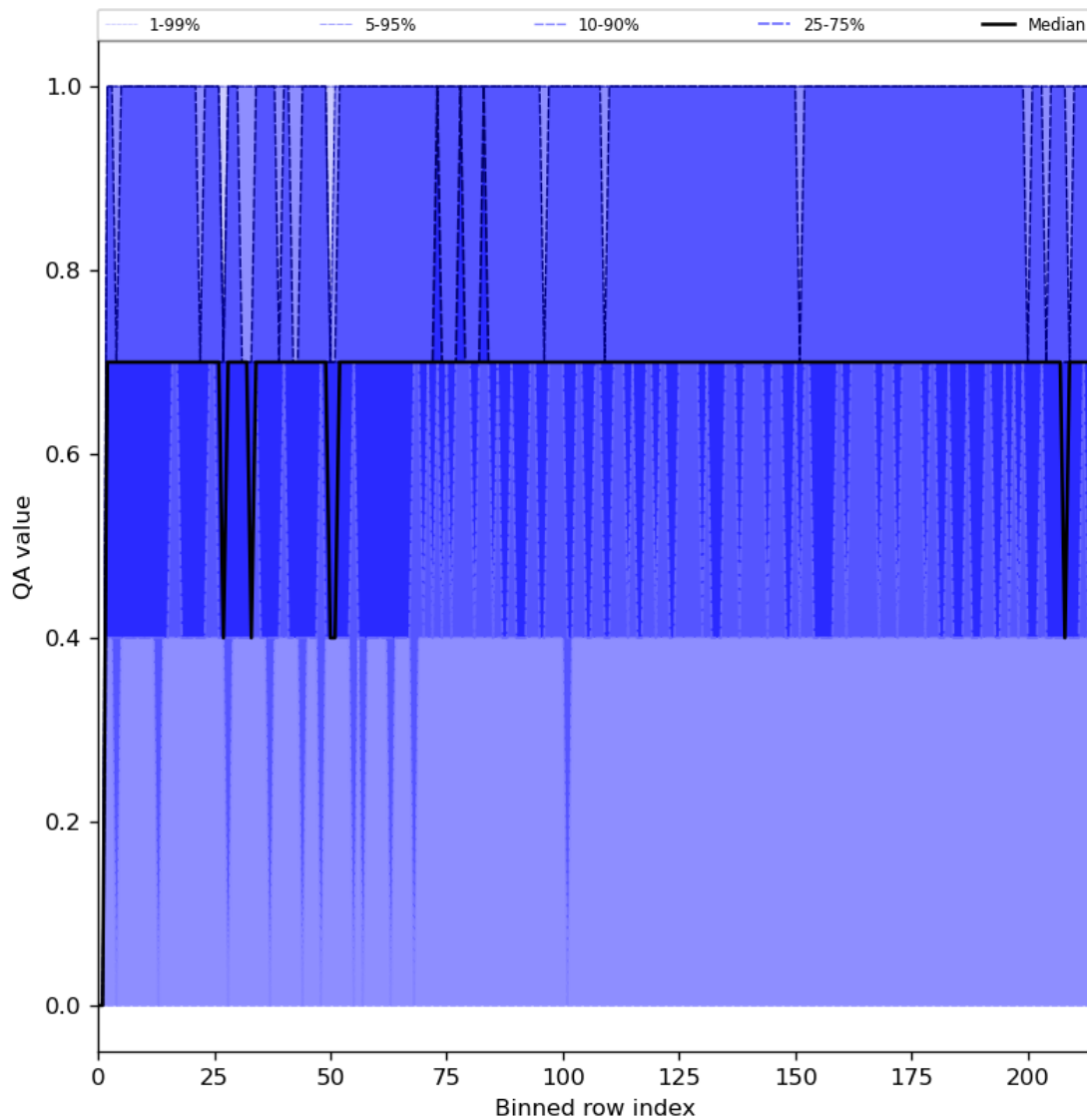
Figure 25: Along track statistics of "QA value" for 2024-04-21 to 2024-04-22
