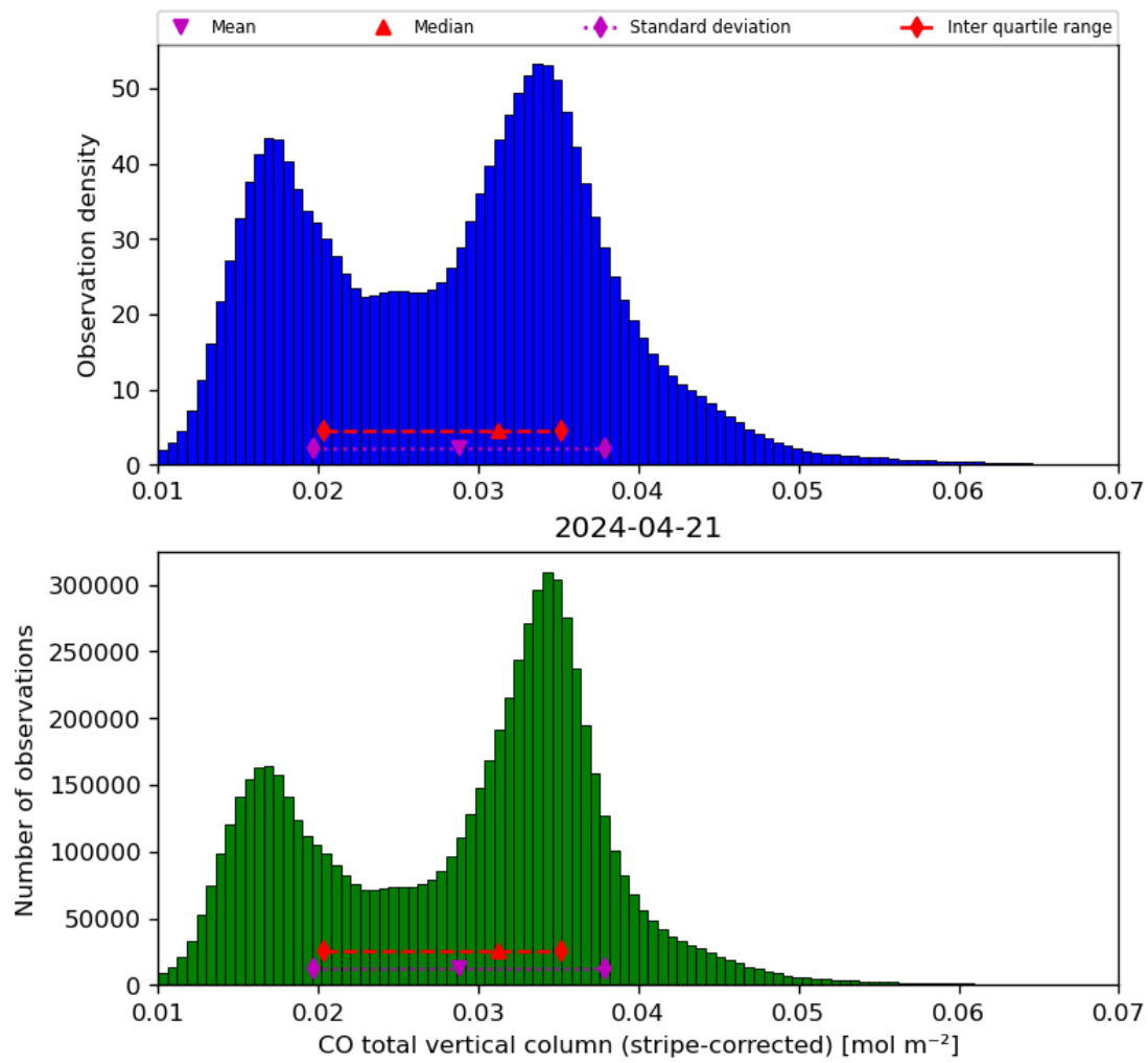
Figure 19: Histogram of “CO total vertical column (stripe-corrected)” for 2024-04-21 to 2024-04-22
