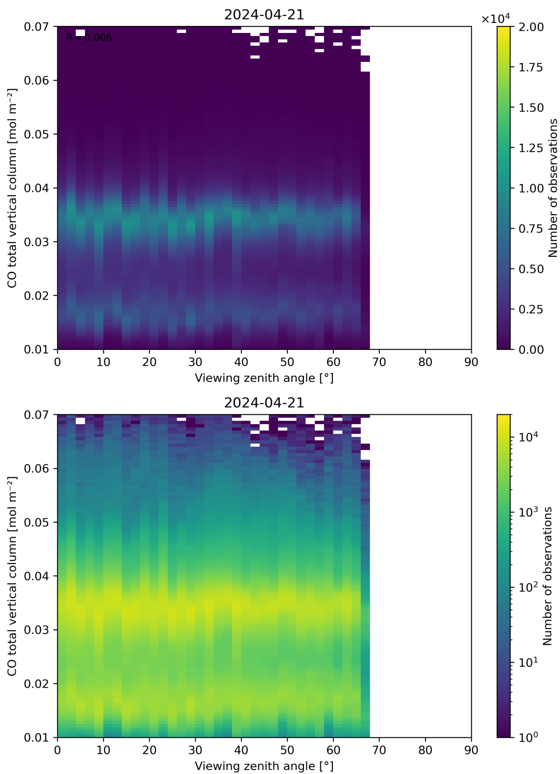
Figure 69: Scatter density plot of “Viewing zenith angle” against “CO total vertical column” for 2024-04-21 to 2024-04-22.
