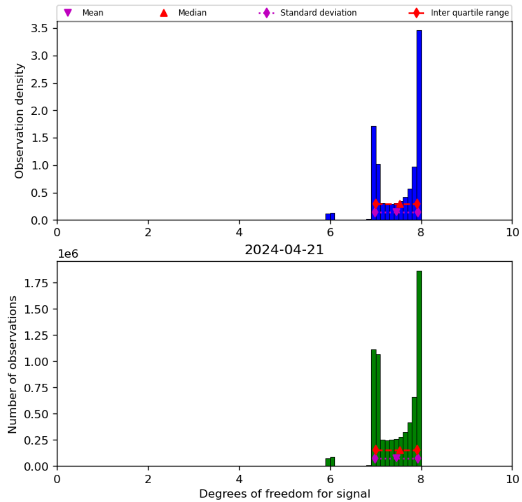
Figure 23: Histogram of “Degrees of freedom for signal” for 2024-04-21 to 2024-04-22
