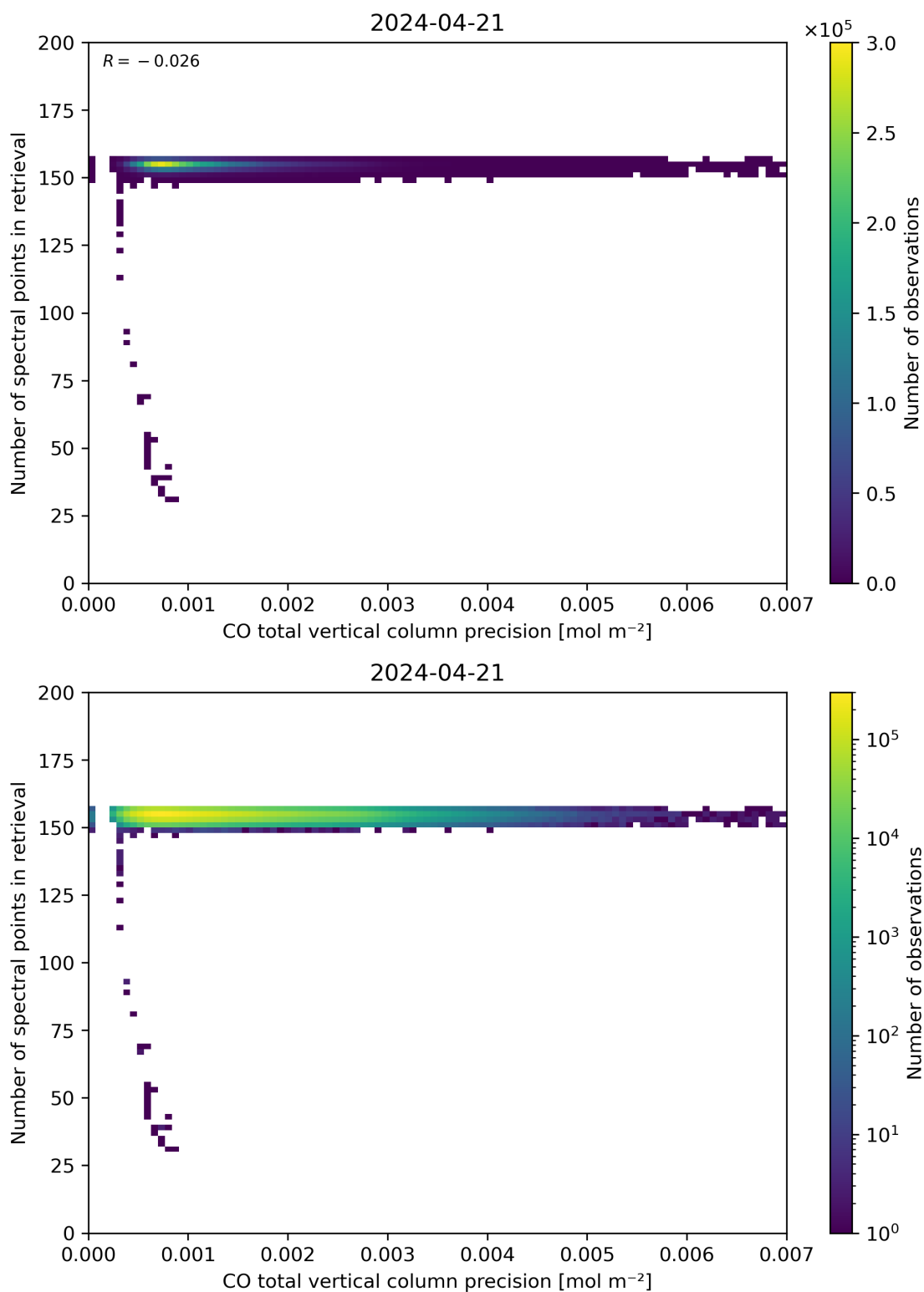
Figure 47: Scatter density plot of “CO total vertical column precision” against “Number of spectral points in retrieval” for 2024-04-21 to 2024-04-22.
