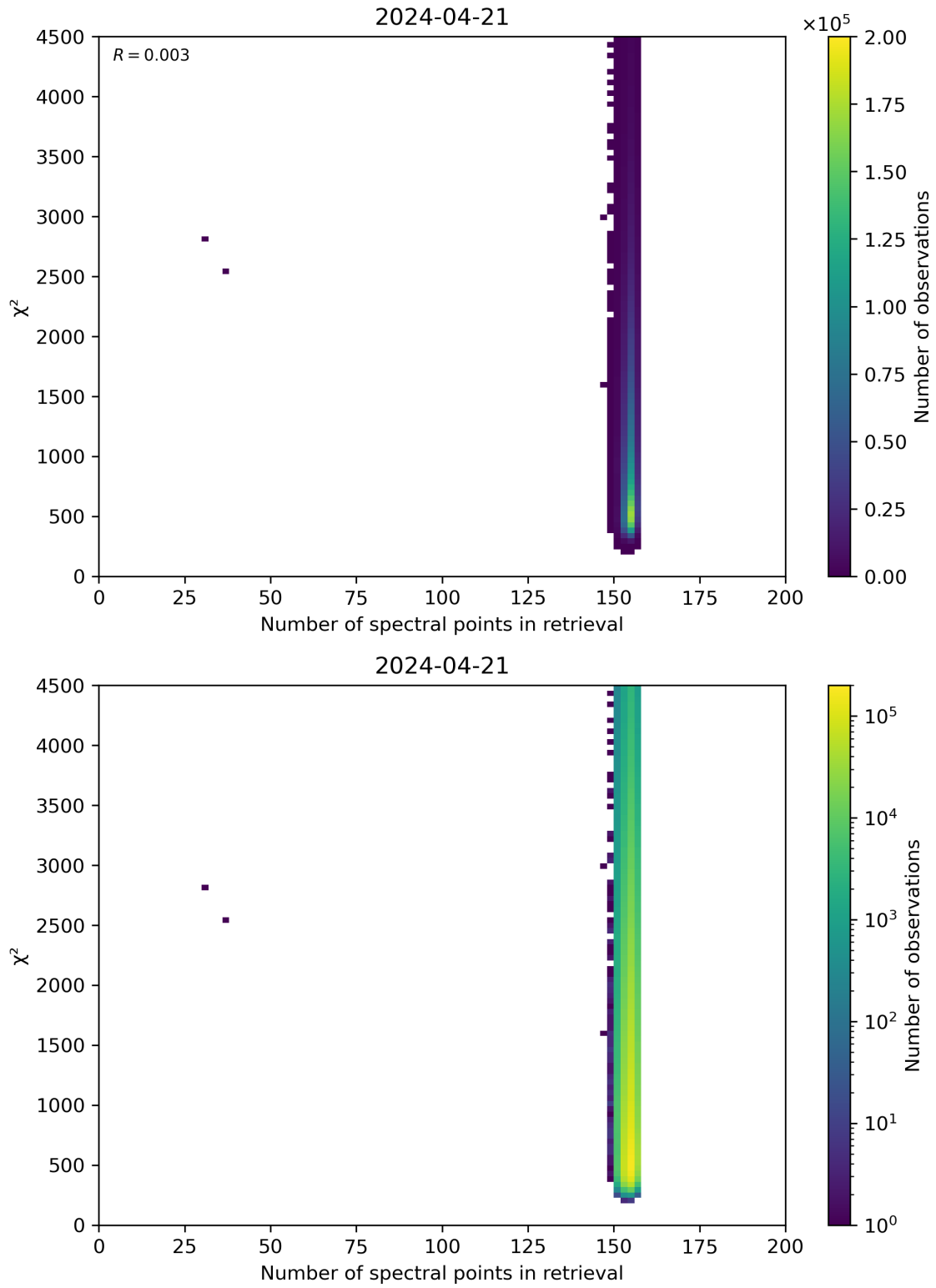
Figure 58: Scatter density plot of “Number of spectral points in retrieval” against “ \chi^2 ” for 2024-04-21 to 2024-04-22.
