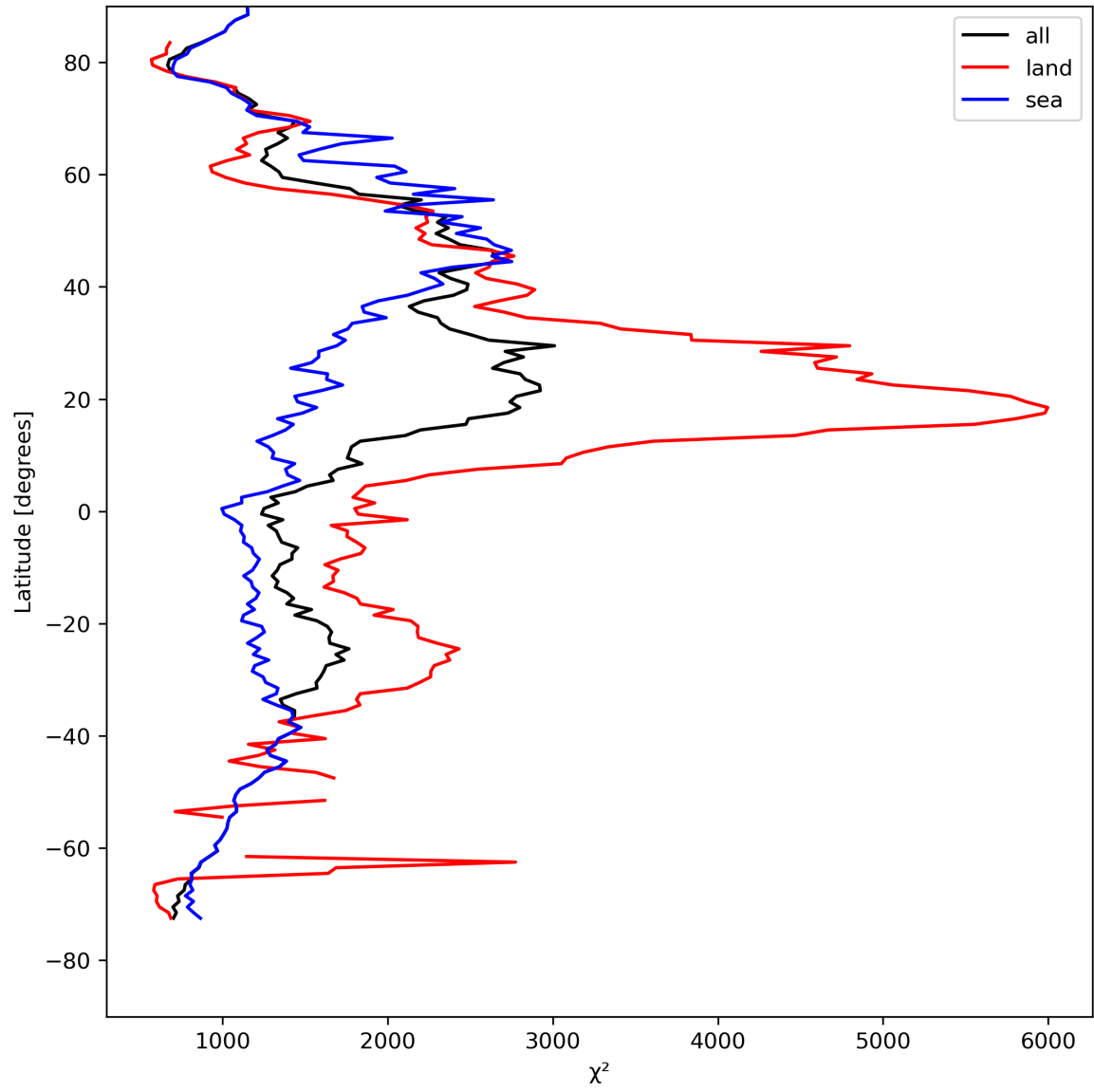
Figure 14: Zonal average of “ \chi^2 ” for 2024-04-21 to 2024-04-22.
