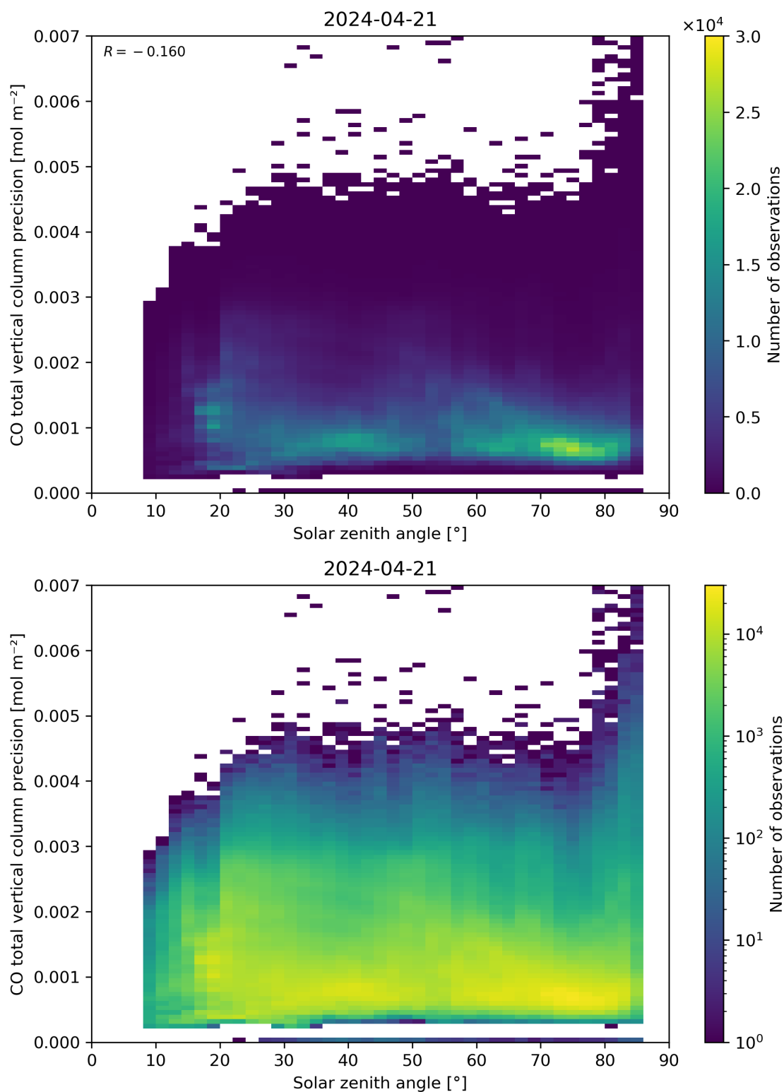
Figure 63: Scatter density plot of “Solar zenith angle” against “CO total vertical column precision” for 2024-04-21 to 2024-04-22.
