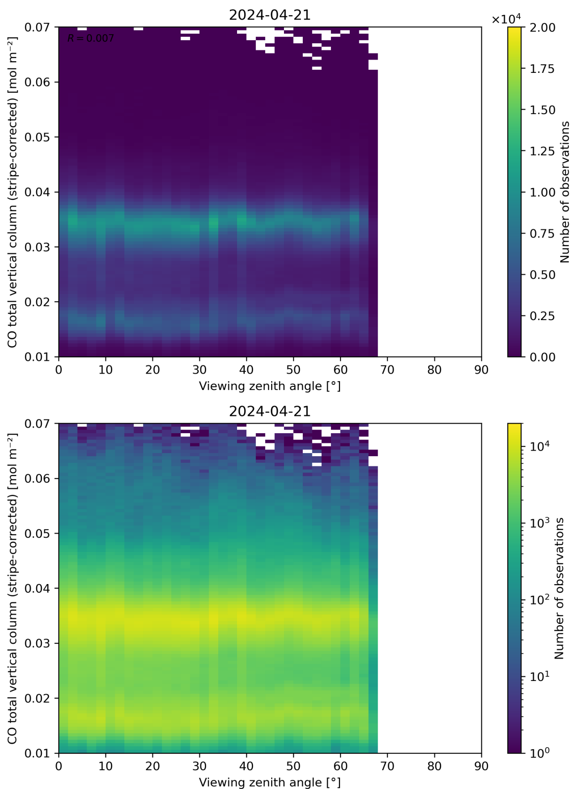
Figure 70: Scatter density plot of “Viewing zenith angle” against “CO total vertical column (stripe-corrected)” for 2024-04-21 to 2024-04-22.
