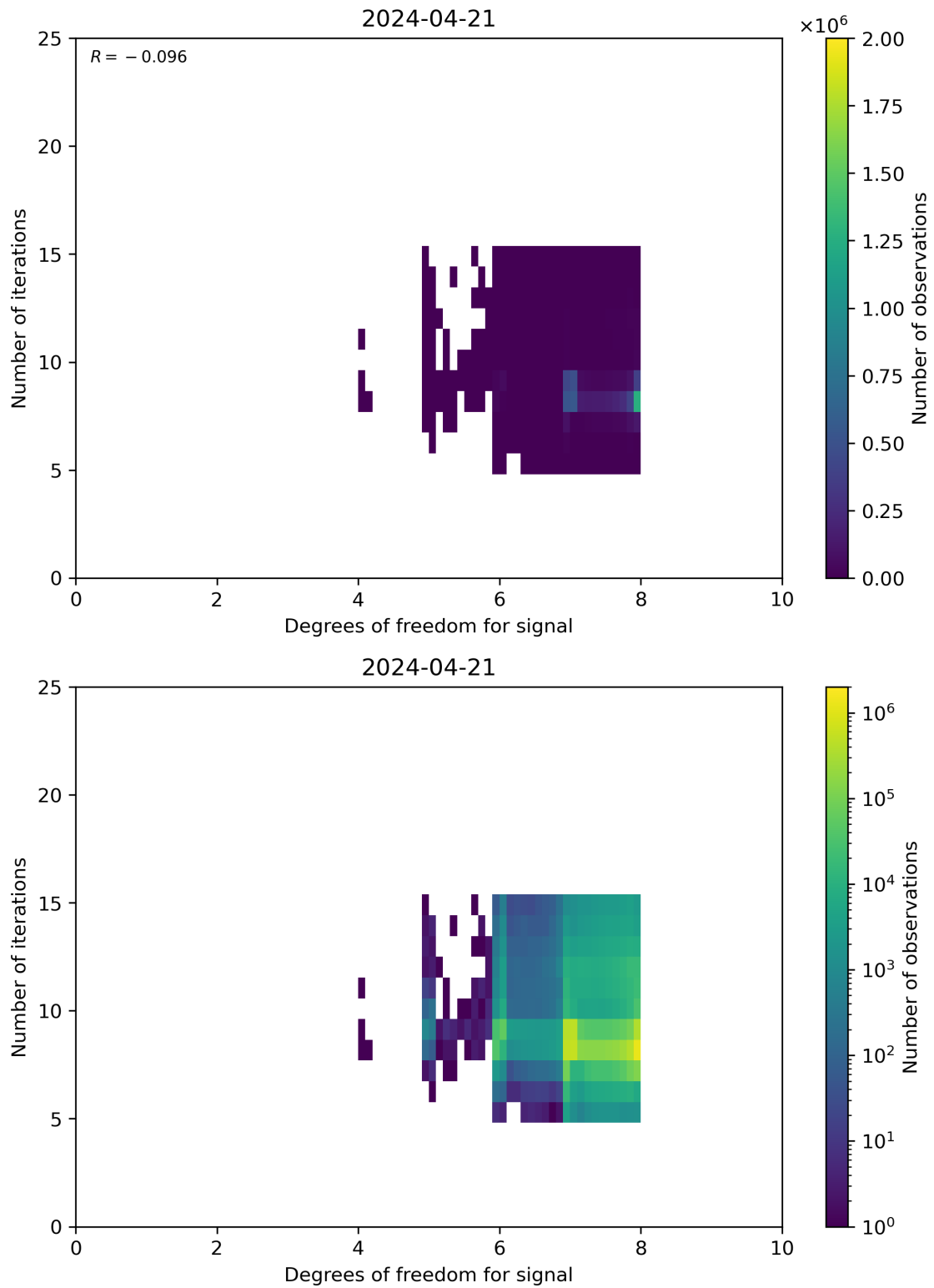
Figure 50: Scatter density plot of “Degrees of freedom for signal” against “Number of iterations” for 2024-04-21 to 2024-04-22.
