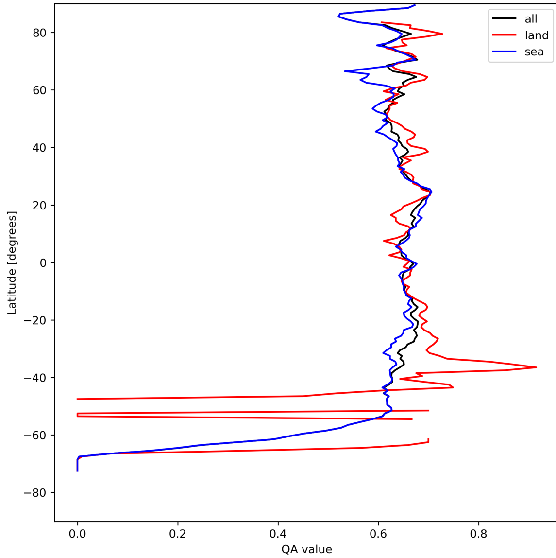
Figure 9: Zonal average of “QA value” for 2024-04-21 to 2024-04-22.
