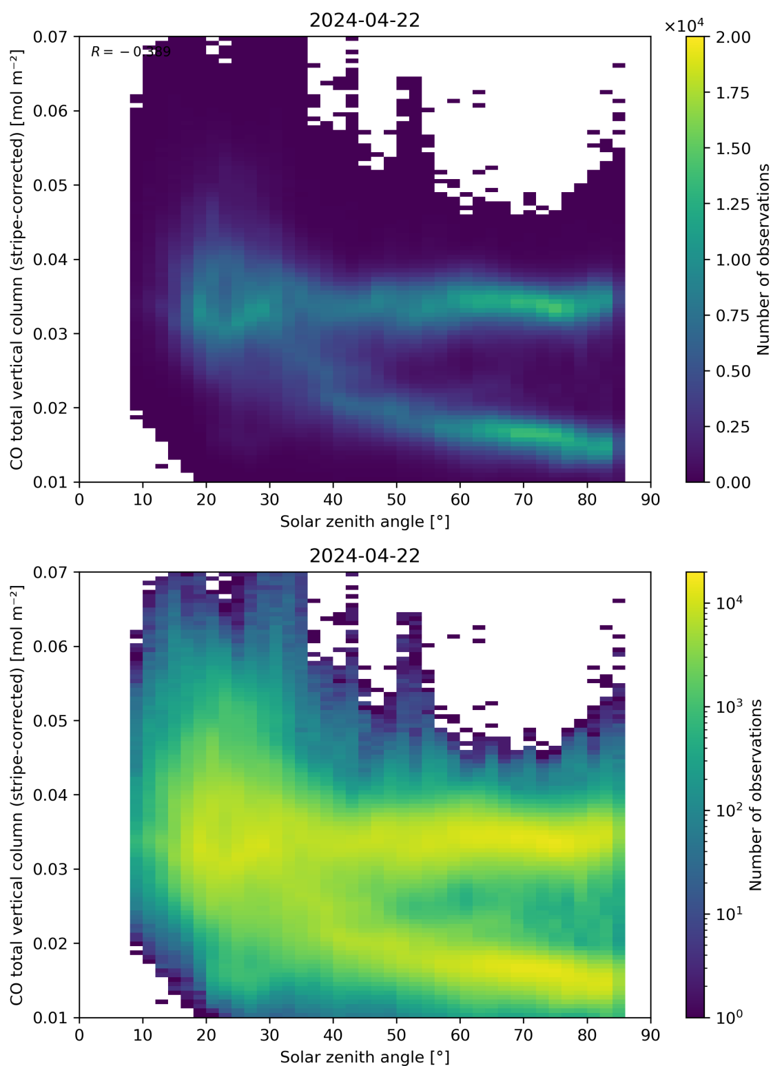
Figure 62: Scatter density plot of “Solar zenith angle” against “CO total vertical column (stripe-corrected)” for 2024-04-21 to 2024-04-23.
