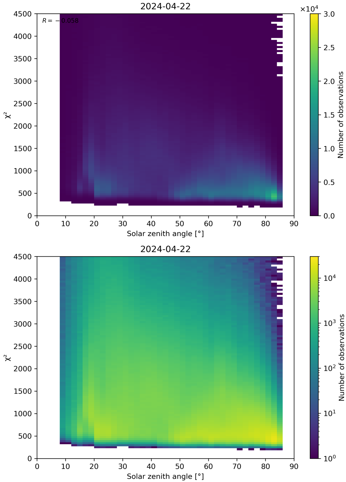
Figure 64: Scatter density plot of “Solar zenith angle” against “ \chi^2 ” for 2024-04-21 to 2024-04-23.
