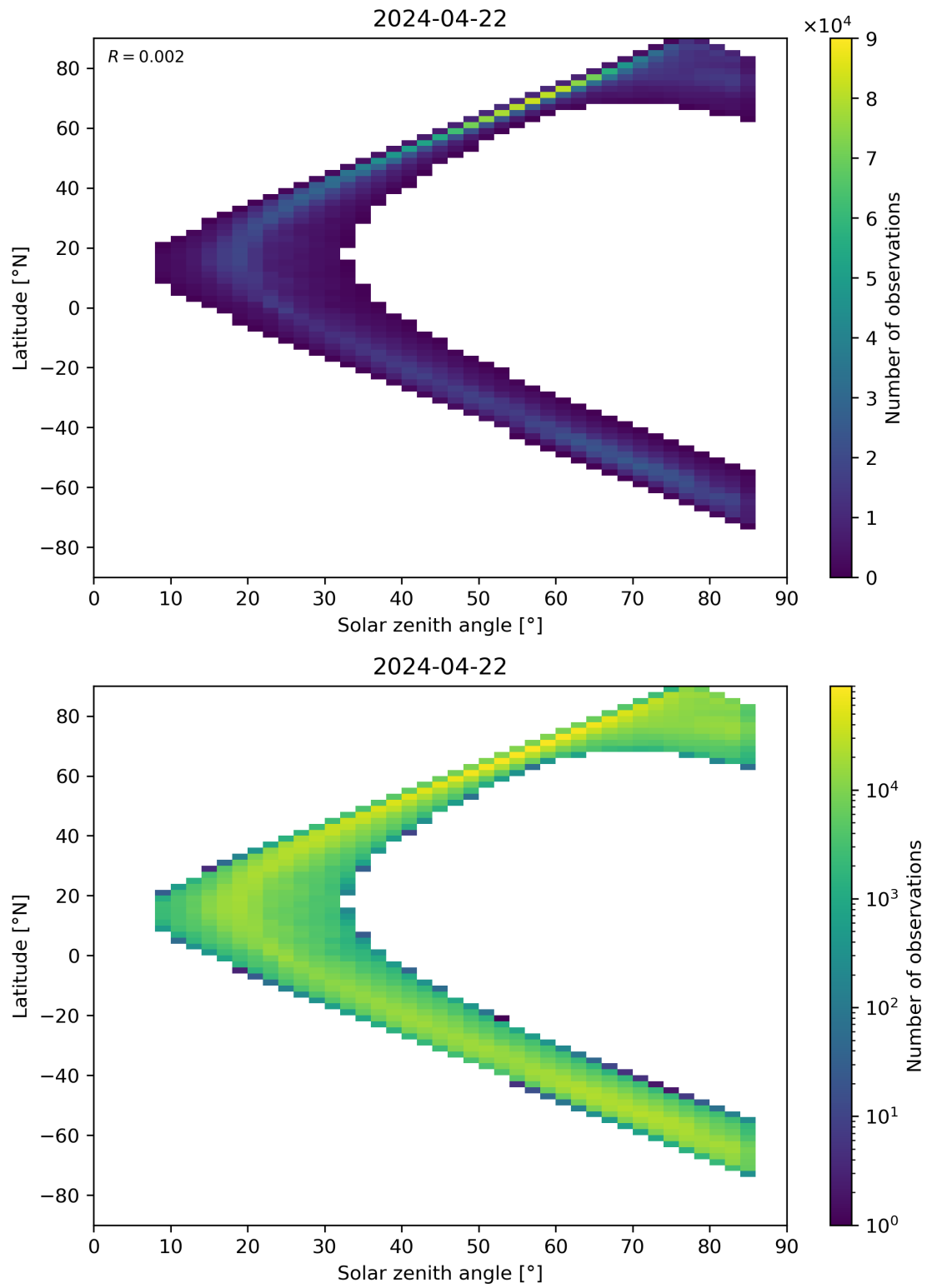
Figure 66: Scatter density plot of “Solar zenith angle” against “Latitude” for 2024-04-21 to 2024-04-23.
