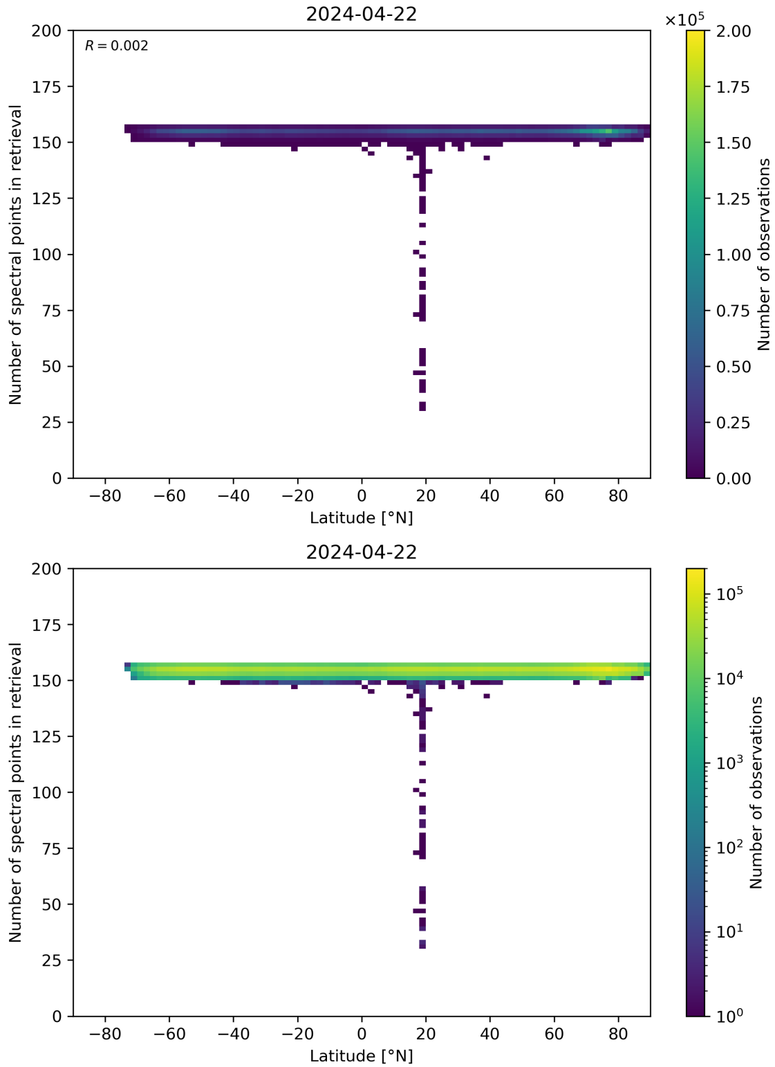
Figure 57: Scatter density plot of “Latitude” against “Number of spectral points in retrieval” for 2024-04-21 to 2024-04-23.
