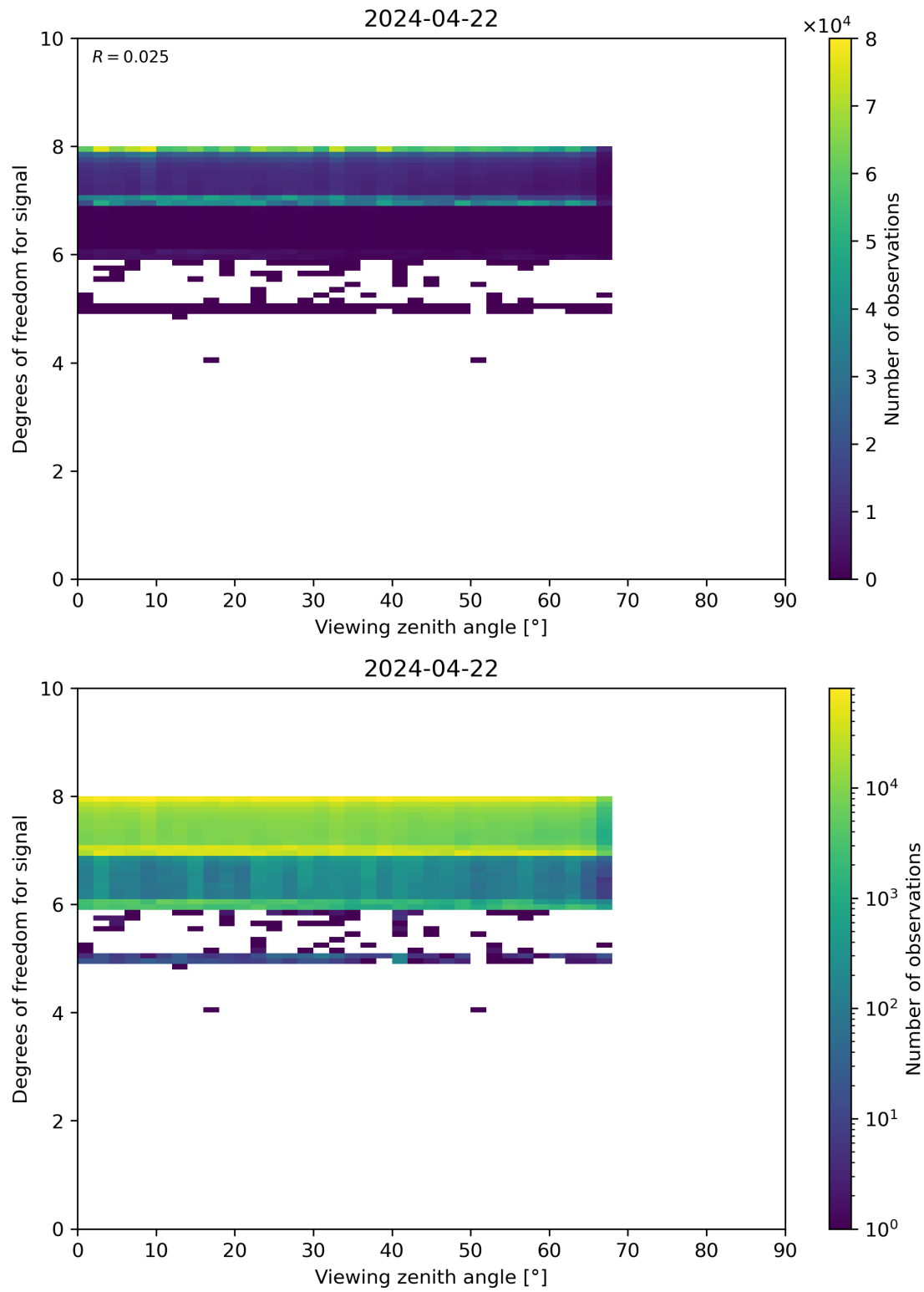
Figure 73: Scatter density plot of “Viewing zenith angle” against “Degrees of freedom for signal” for 2024-04-21 to 2024-04-23.
