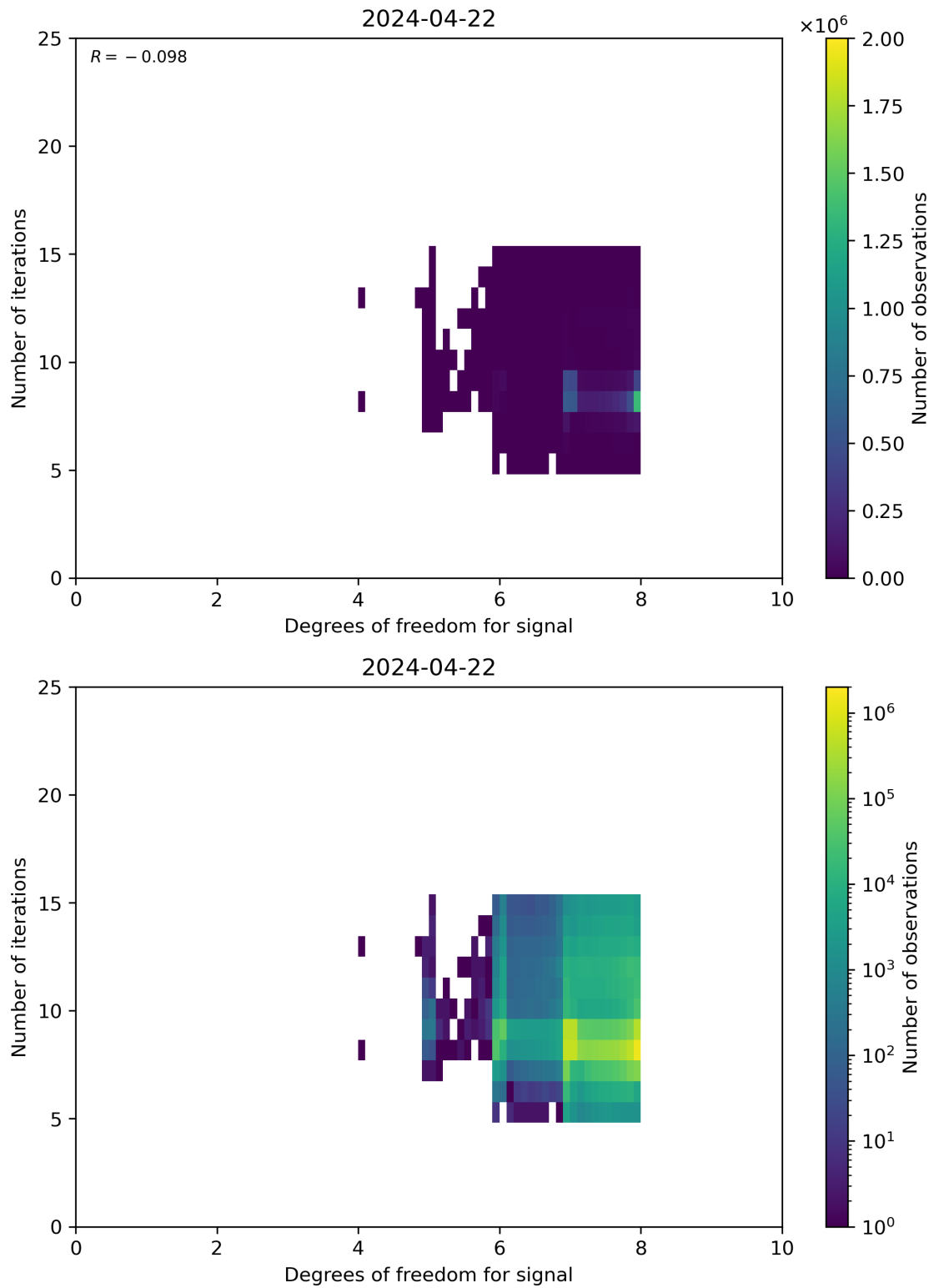
Figure 50: Scatter density plot of “Degrees of freedom for signal” against “Number of iterations” for 2024-04-21 to 2024-04-23.
