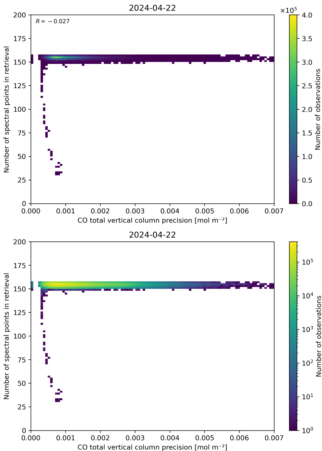
Figure 47: Scatter density plot of “CO total vertical column precision” against “Number of spectral points in retrieval” for 2024-04-21 to 2024-04-23.
