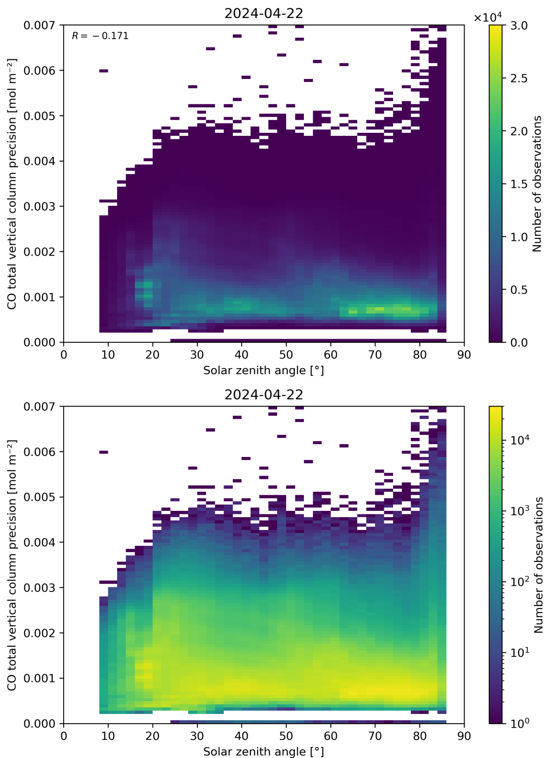
Figure 63: Scatter density plot of “Solar zenith angle” against “CO total vertical column precision” for 2024-04-21 to 2024-04-23.
