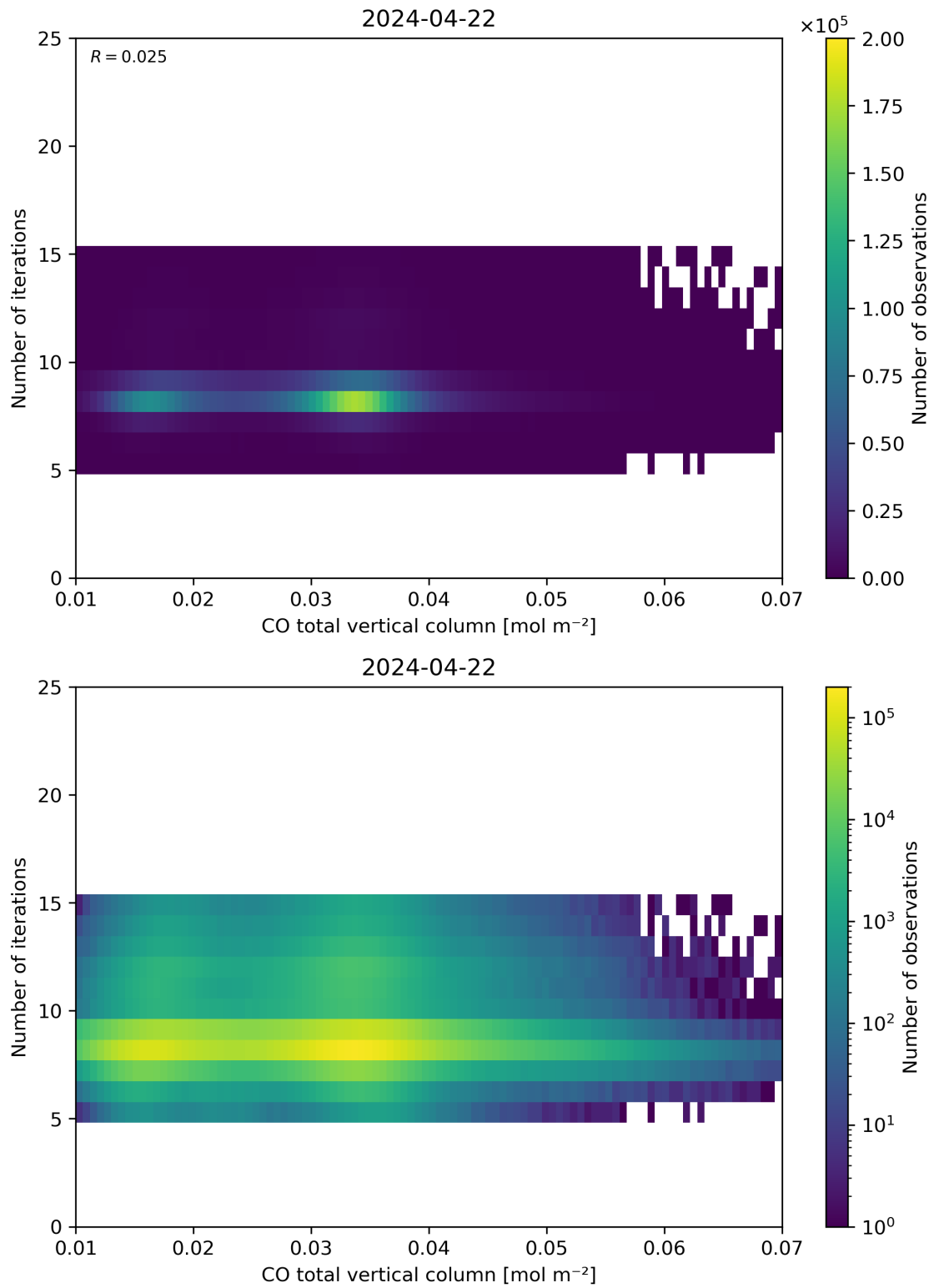
Figure 42: Scatter density plot of “CO total vertical column” against “Number of iterations” for 2024-04-21 to 2024-04-23.
