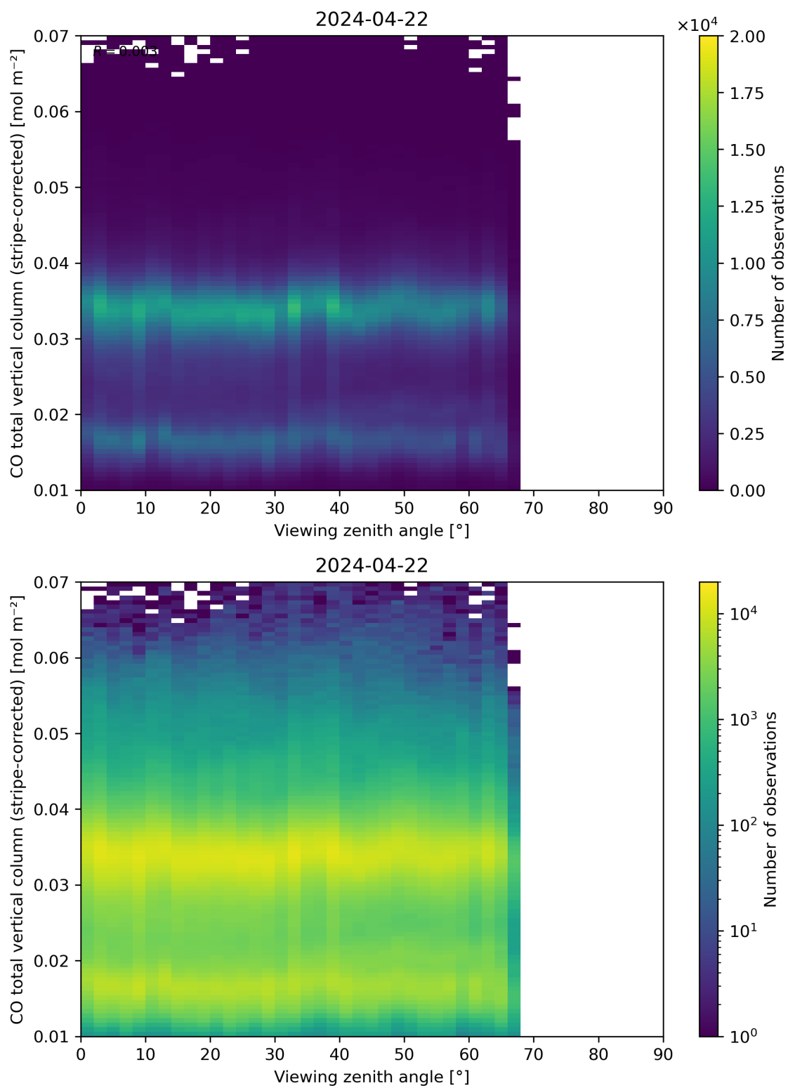
Figure 70: Scatter density plot of “Viewing zenith angle” against “CO total vertical column (stripe-corrected)” for 2024-04-21 to 2024-04-23.
