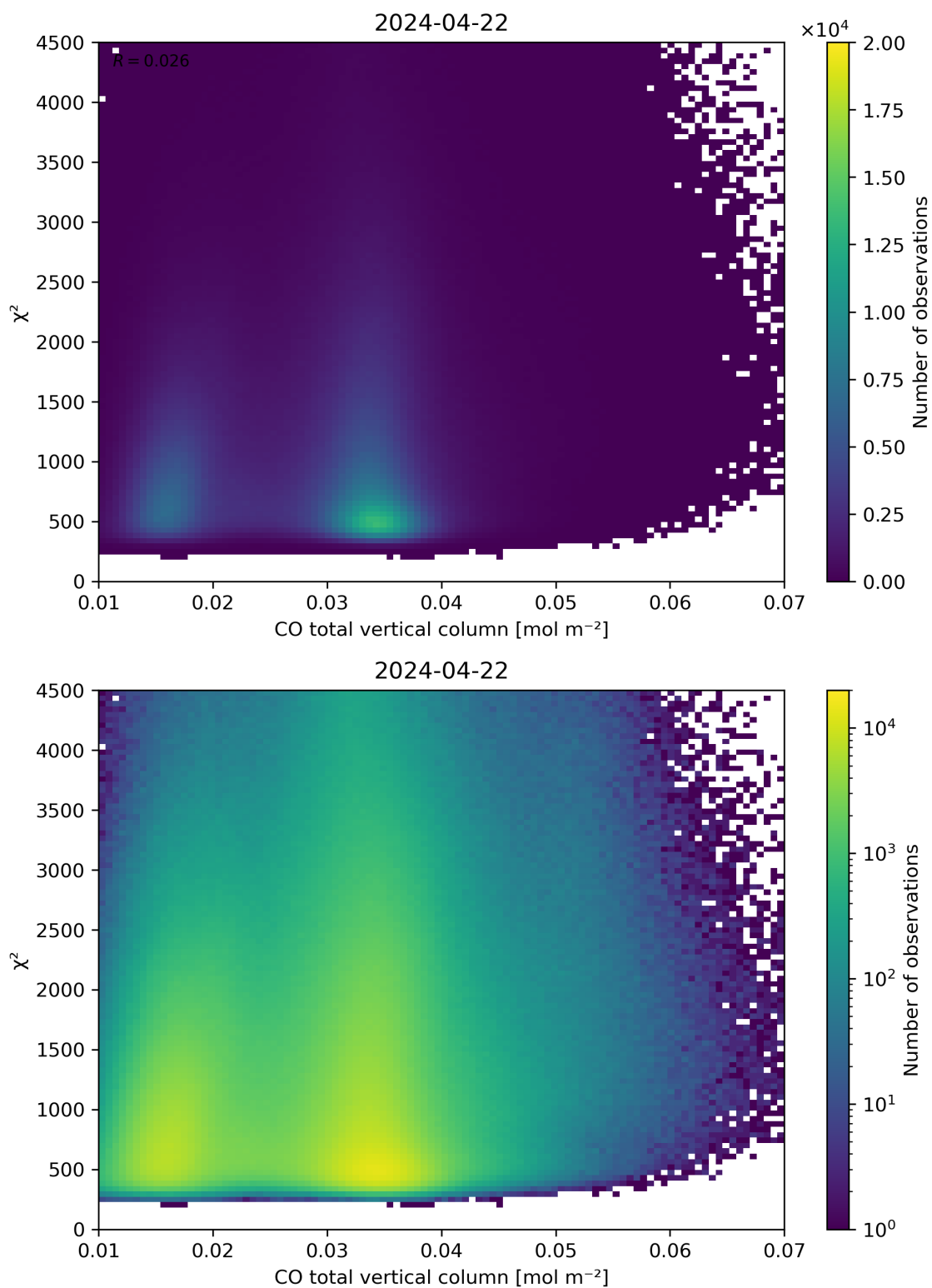
Figure 35: Scatter density plot of “CO total vertical column” against “ \chi^2 ” for 2024-04-21 to 2024-04-23.
