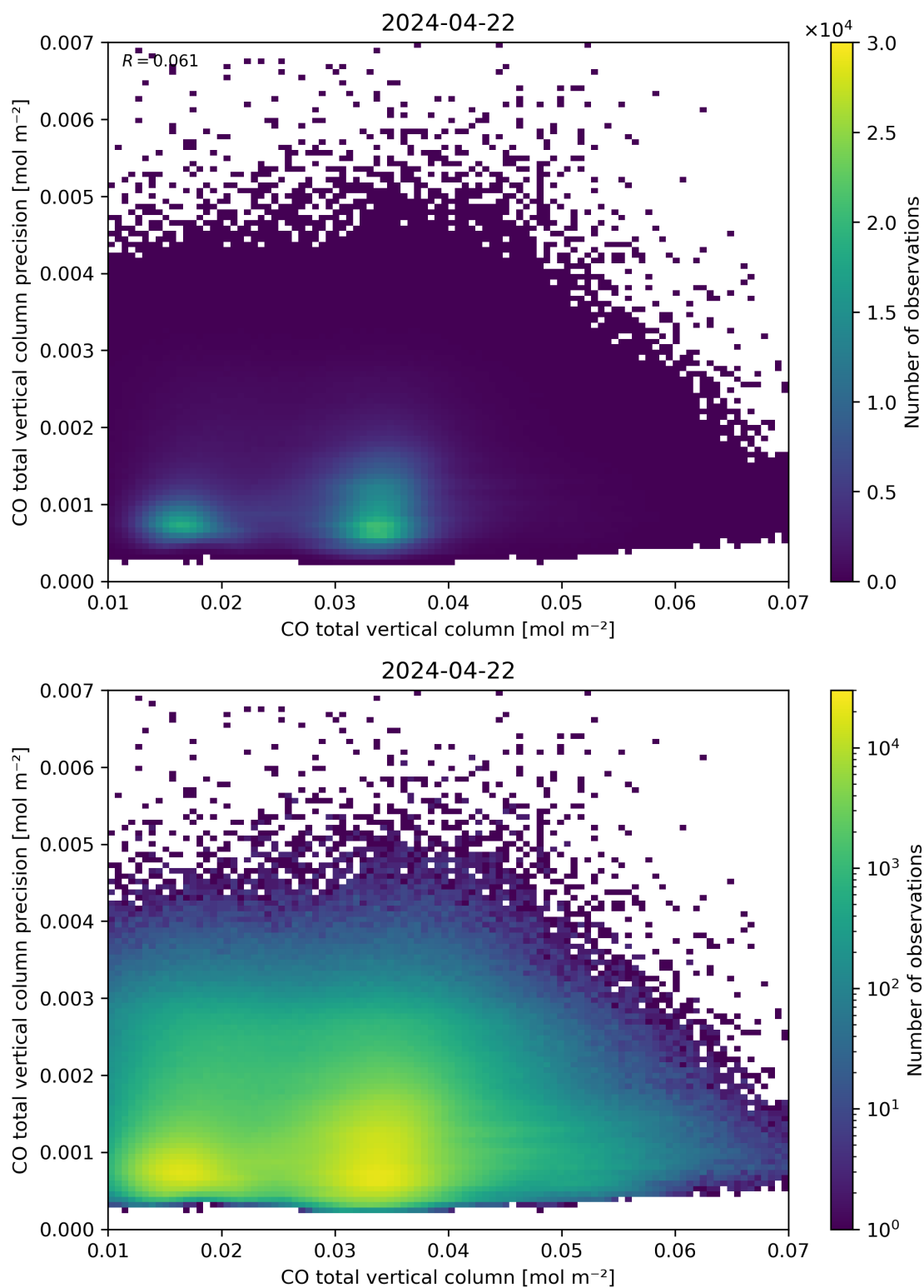
Figure 34: Scatter density plot of “CO total vertical column” against “CO total vertical column precision” for 2024-04-21 to 2024-04-23.
