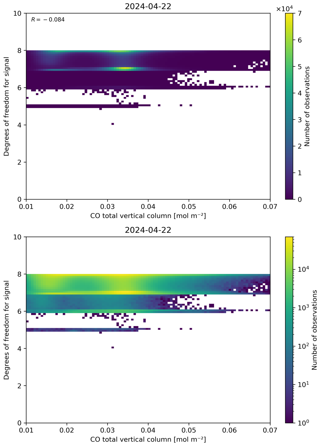
Figure 41: Scatter density plot of “CO total vertical column” against “Degrees of freedom for signal” for 2024-04-21 to 2024-04-23.
