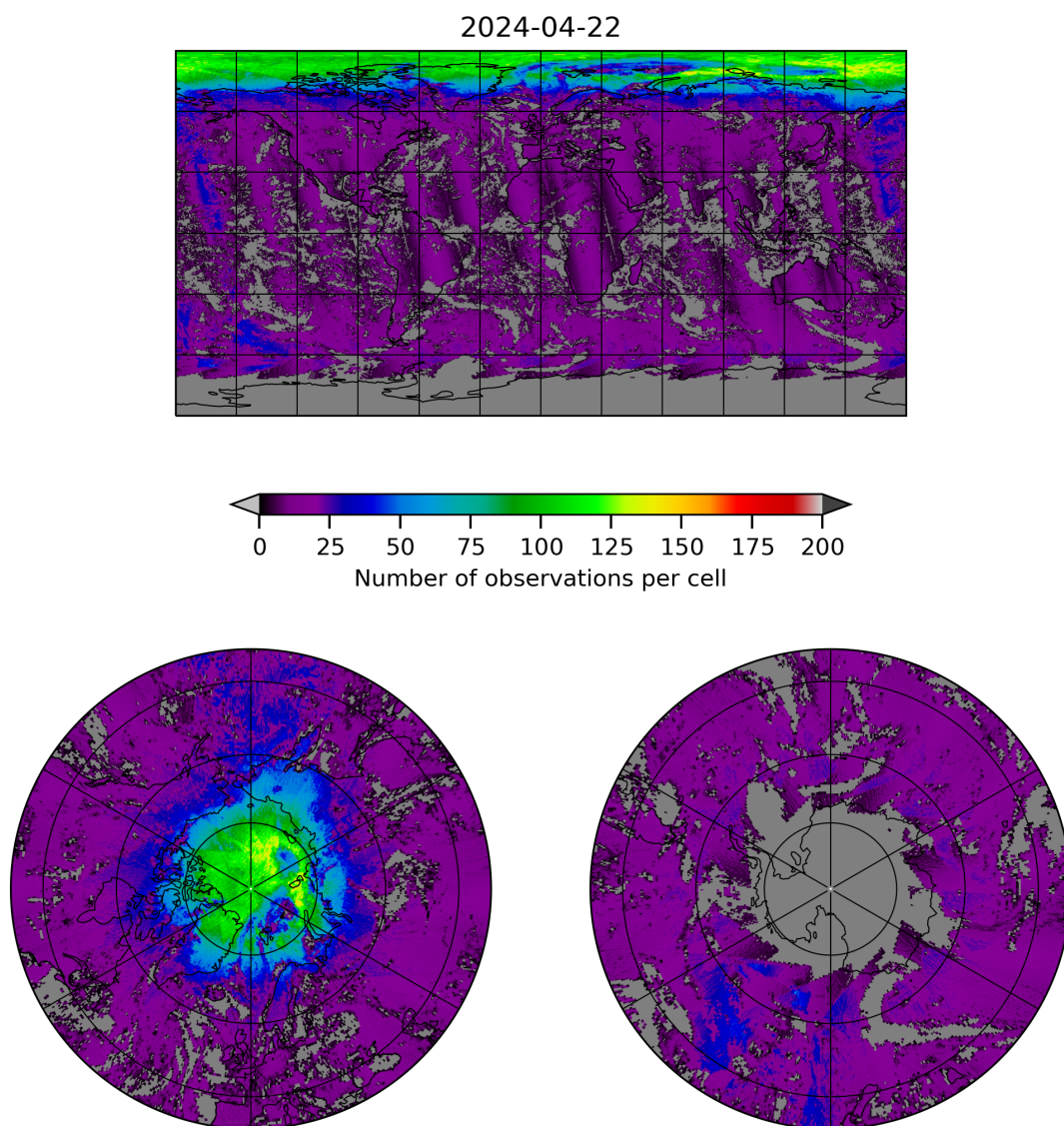
Figure 8: Map of the number of observations for 2024-04-21 to 2024-04-23
