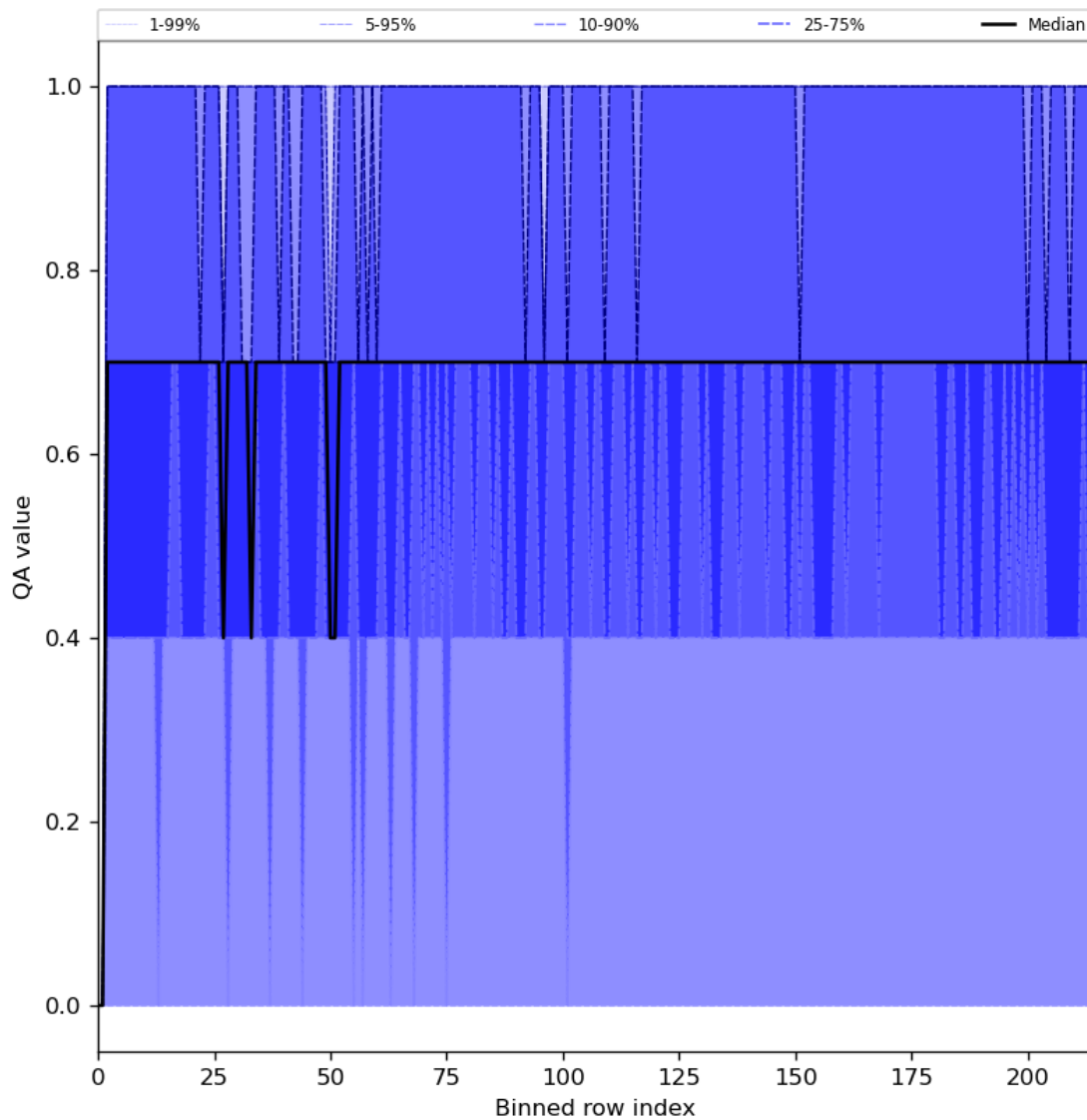
Figure 25: Along track statistics of “QA value” for 2024-04-21 to 2024-04-23
