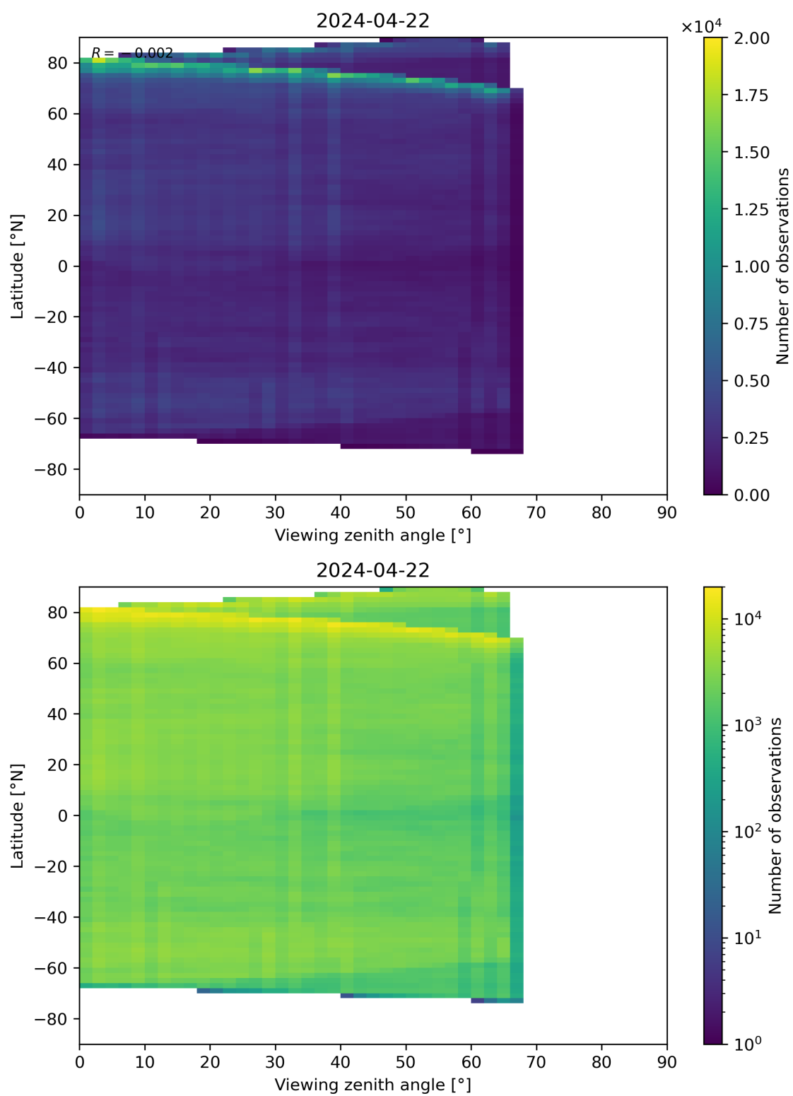
Figure 74: Scatter density plot of “Viewing zenith angle” against “Latitude” for 2024-04-21 to 2024-04-23.
