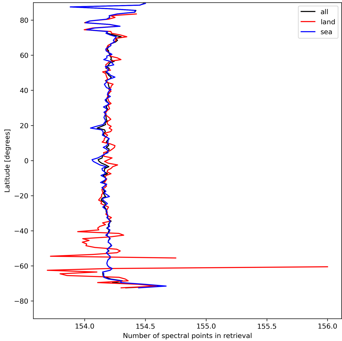
Figure 13: Zonal average of “Number of spectral points in retrieval” for 2024-04-21 to 2024-04-23.
