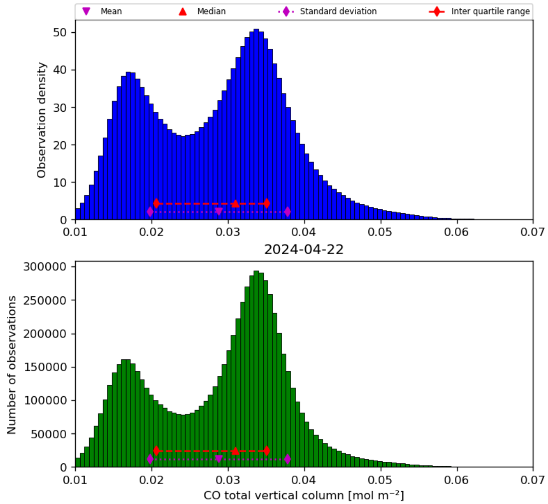
Figure 18: Histogram of “CO total vertical column” for 2024-04-21 to 2024-04-23
