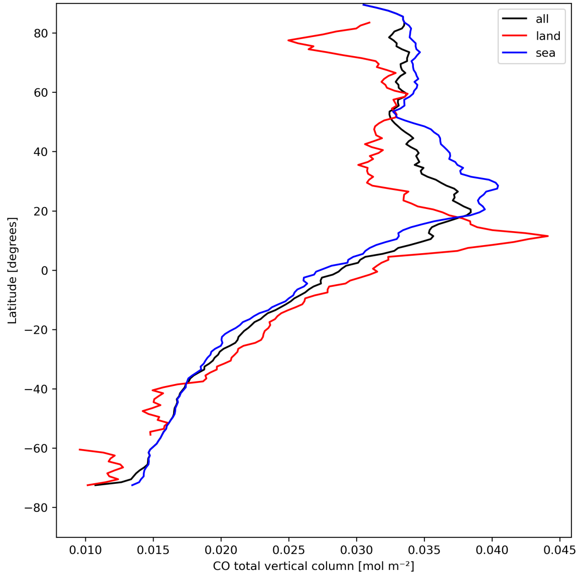
Figure 10: Zonal average of “CO total vertical column” for 2024-04-21 to 2024-04-23.
