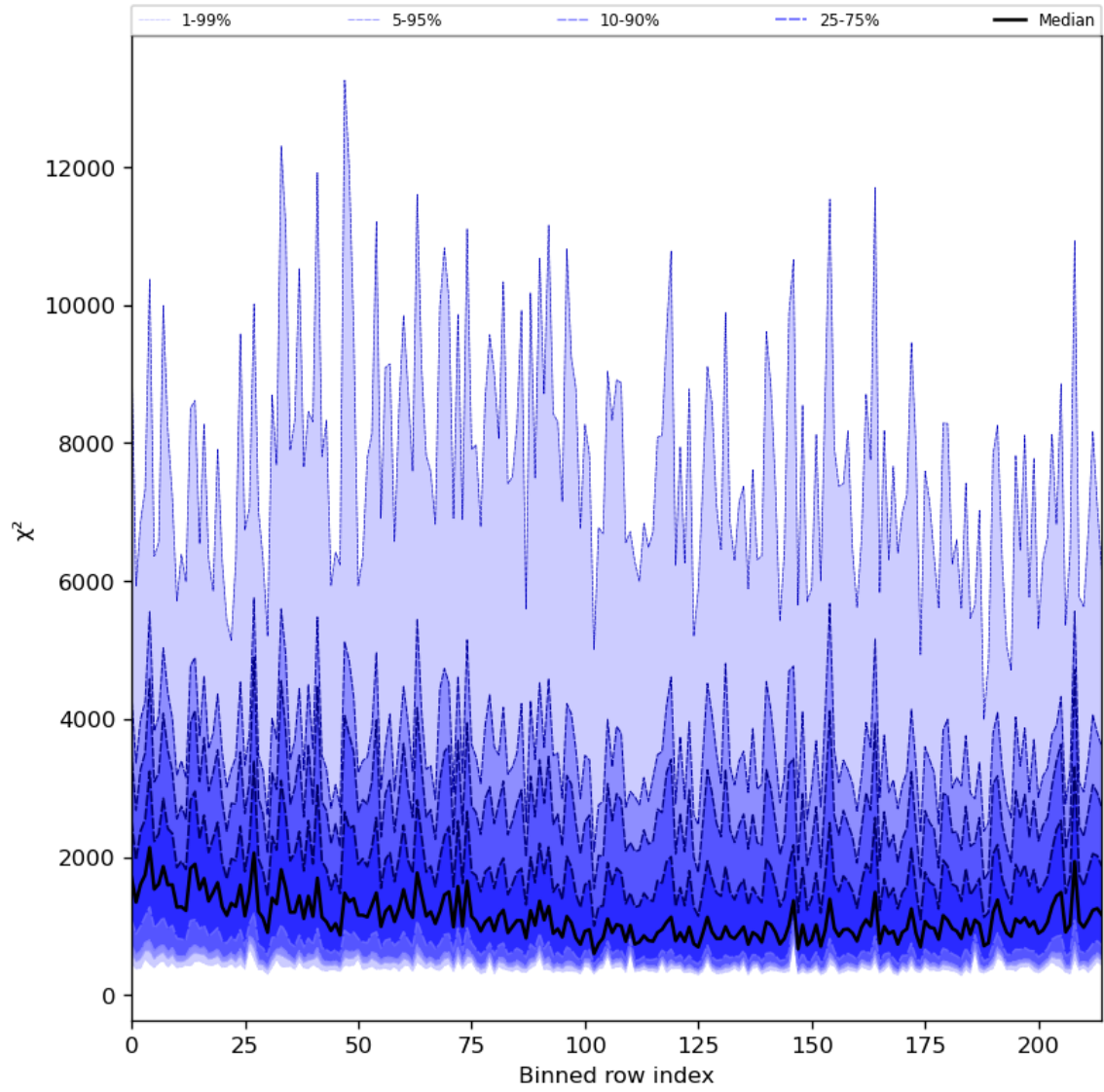
Figure 30: Along track statistics of “ \chi^2 ” for 2024-04-21 to 2024-04-23
