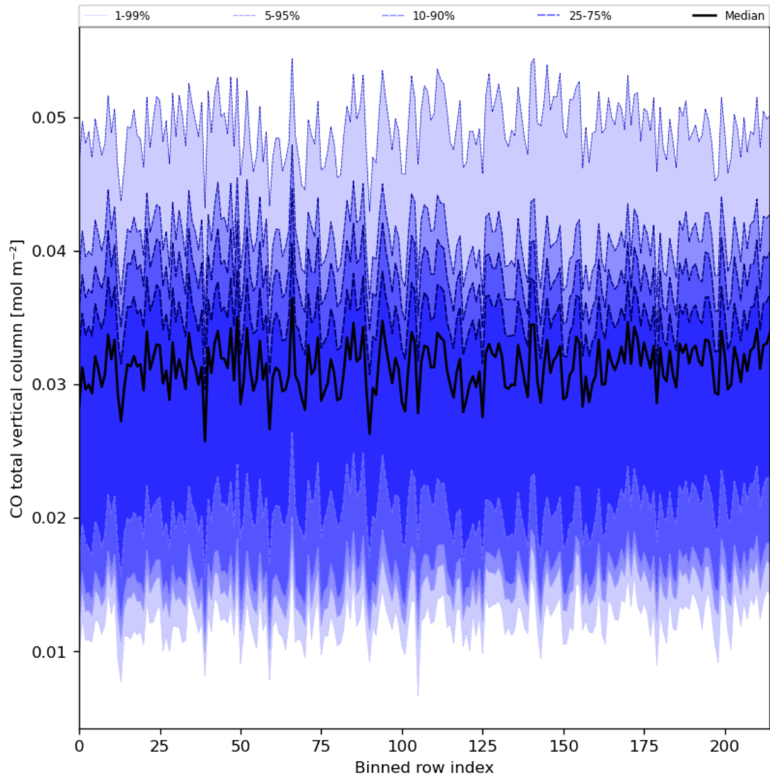
Figure 26: Along track statistics of “CO total vertical column” for 2024-04-21 to 2024-04-23
