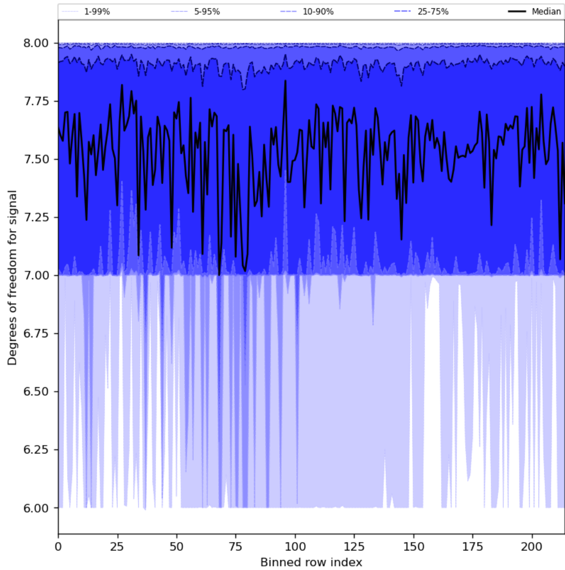
Figure 31: Along track statistics of “Degrees of freedom for signal” for 2024-04-21 to 2024-04-23
