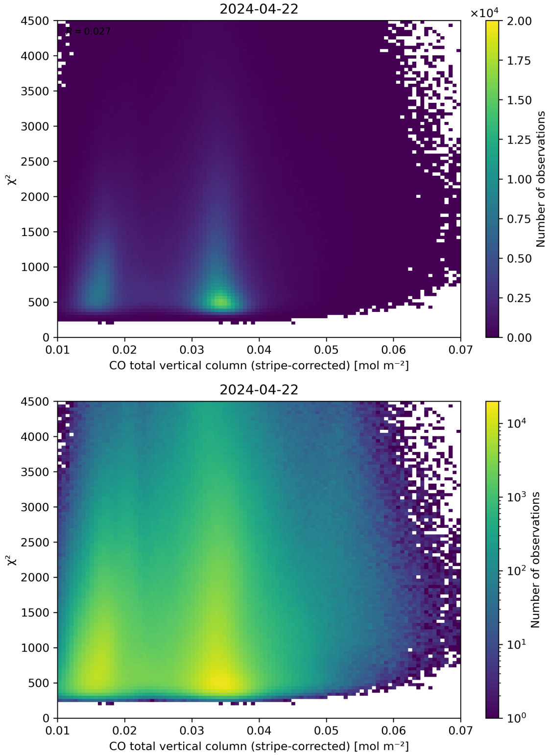
Figure 37: Scatter density plot of “CO total vertical column (stripe-corrected)” against “ \chi^2 ” for 2024-04-21 to 2024-04-23.
