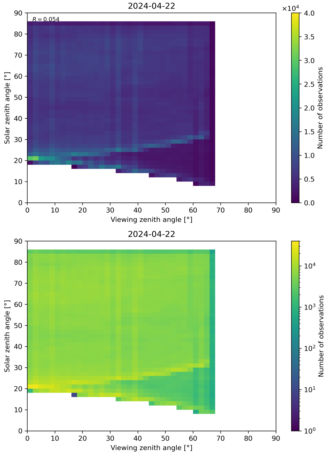
Figure 77: Scatter density plot of “Viewing zenith angle” against “Solar zenith angle” for 2024-04-21 to 2024-04-23.
