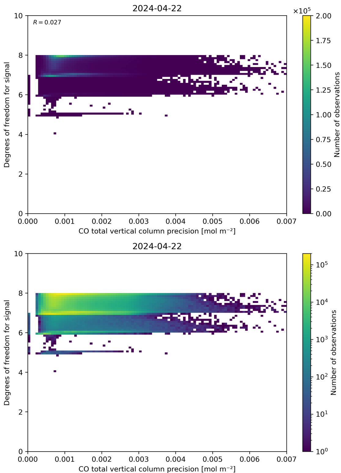
Figure 45: Scatter density plot of “CO total vertical column precision” against “Degrees of freedom for signal” for 2024-04-21 to 2024-04-23.
