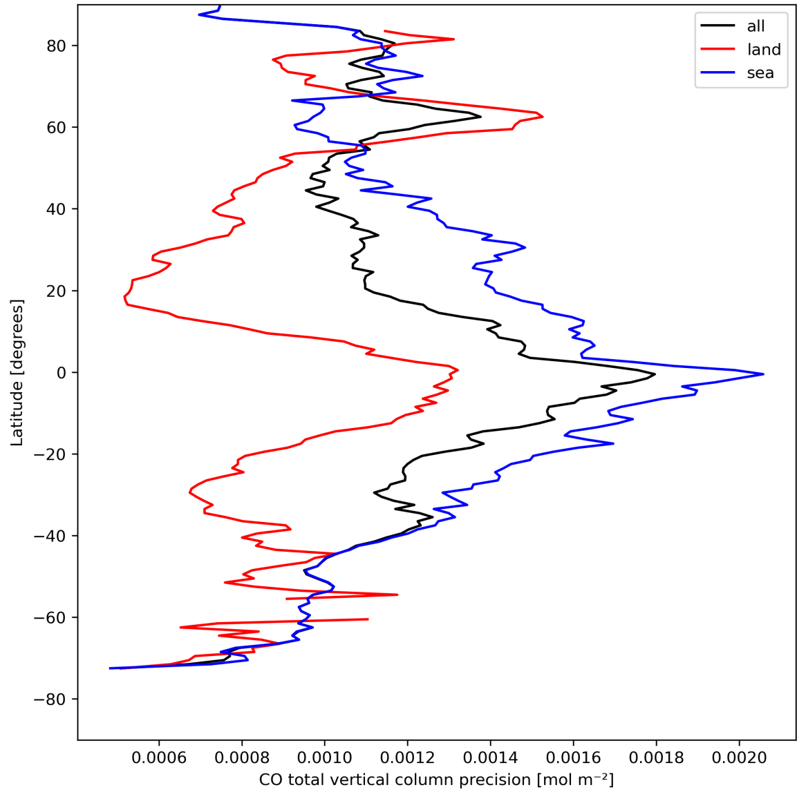
Figure 12: Zonal average of “CO total vertical column precision” for 2024-04-21 to 2024-04-23.
