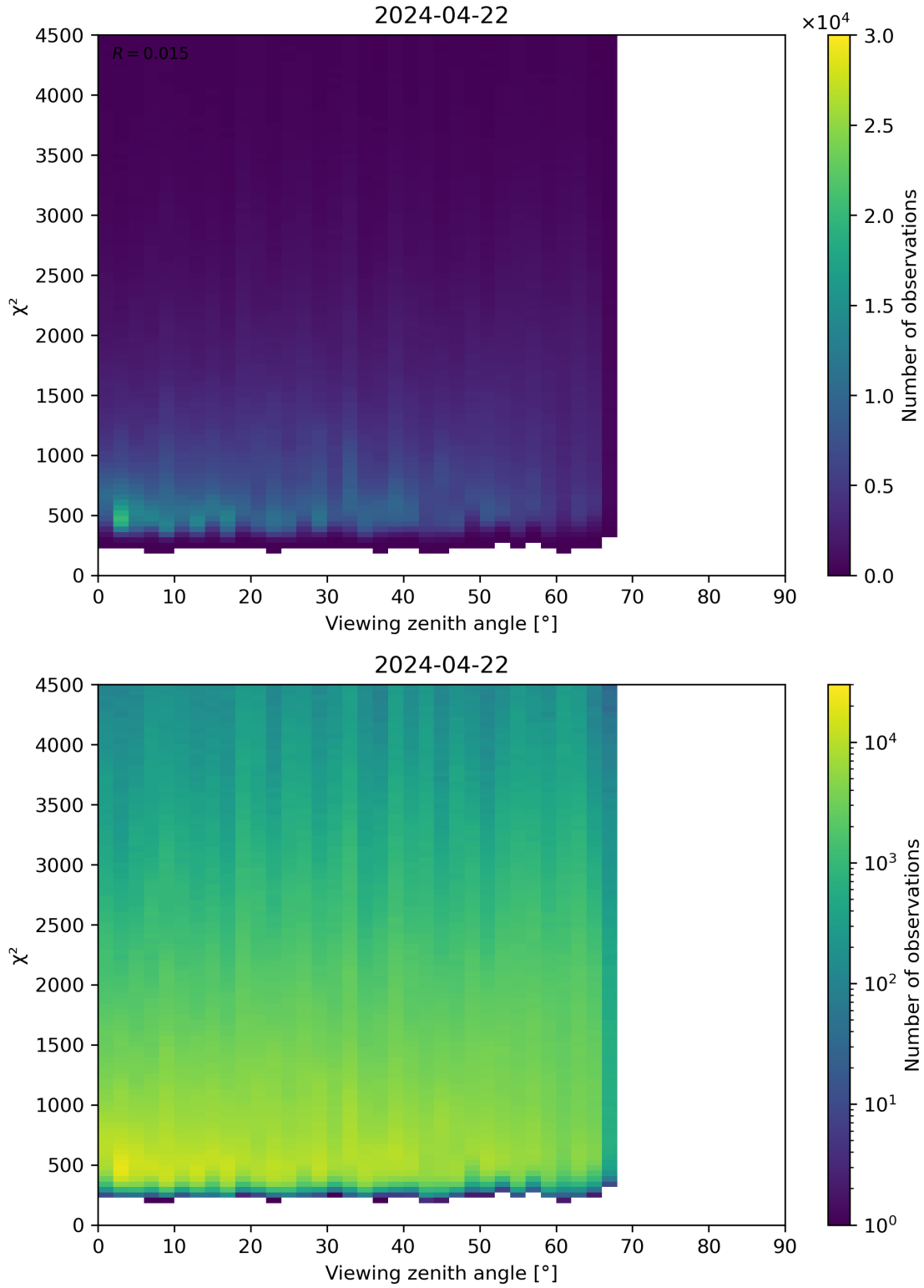
Figure 72: Scatter density plot of “Viewing zenith angle” against “ \chi^2 ” for 2024-04-21 to 2024-04-23.
