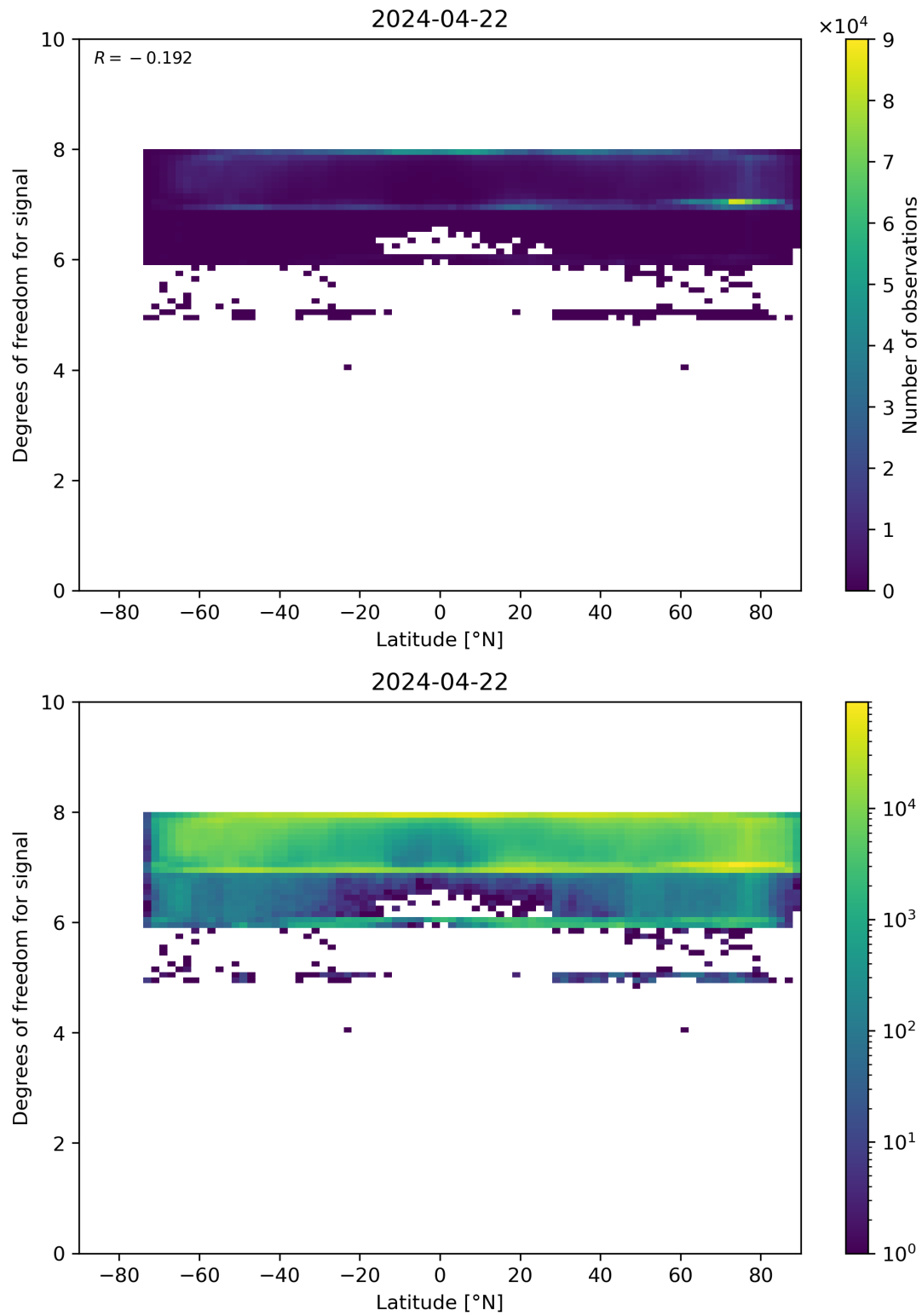
Figure 55: Scatter density plot of “Latitude” against “Degrees of freedom for signal” for 2024-04-21 to 2024-04-23.
