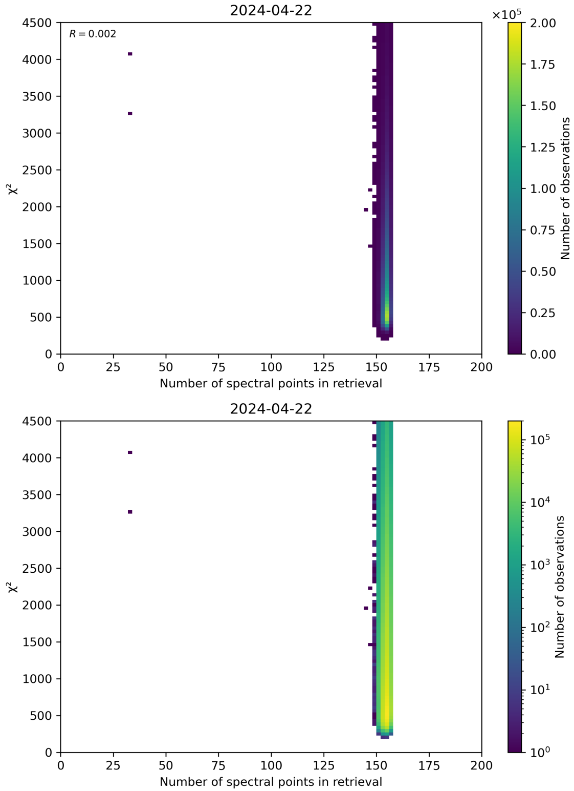
Figure 58: Scatter density plot of “Number of spectral points in retrieval” against “ \chi^2 ” for 2024-04-21 to 2024-04-23.
