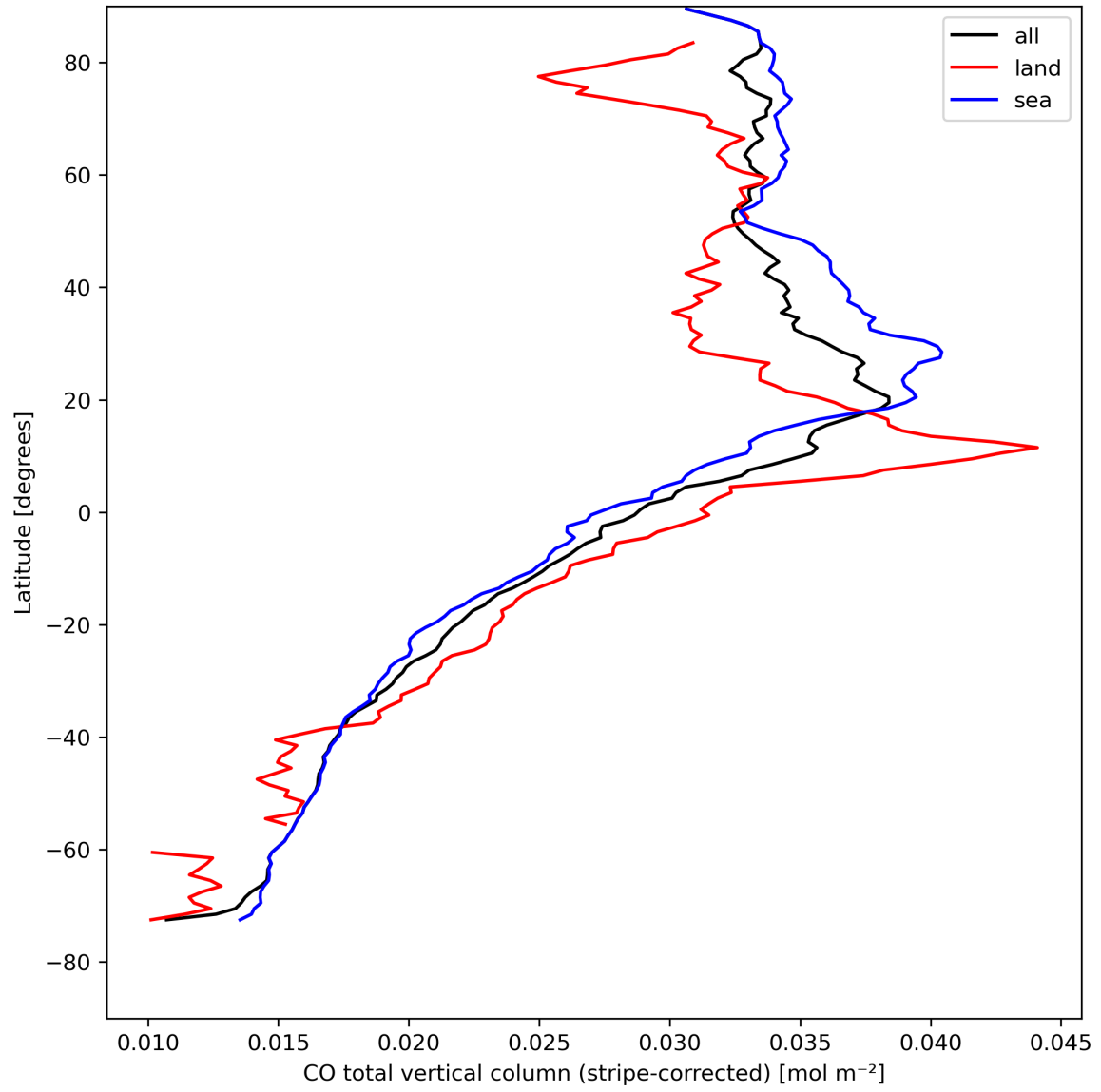
Figure 11: Zonal average of “CO total vertical column (stripe-corrected)” for 2024-04-21 to 2024-04-23.
