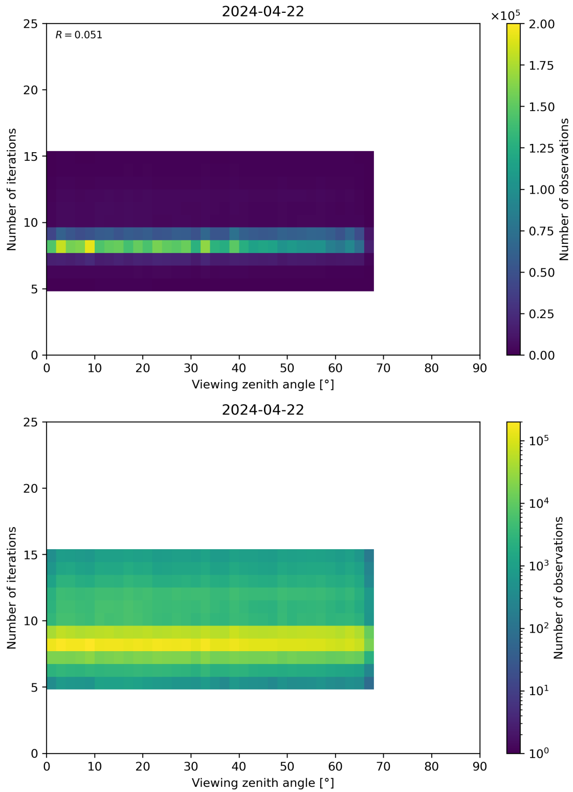
Figure 75: Scatter density plot of “Viewing zenith angle” against “Number of iterations” for 2024-04-21 to 2024-04-23.
