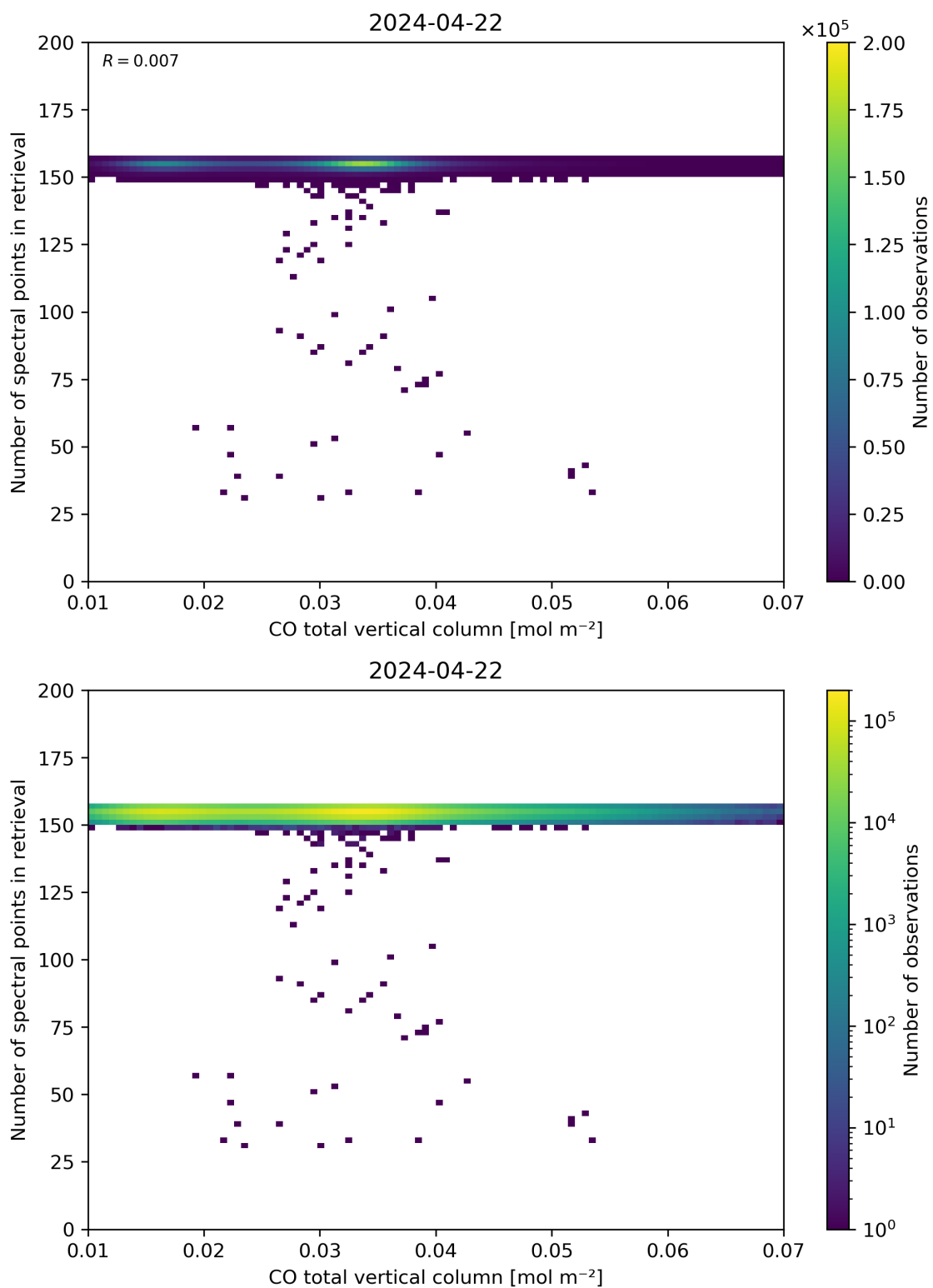
Figure 43: Scatter density plot of “CO total vertical column” against “Number of spectral points in retrieval” for 2024-04-21 to 2024-04-23.
