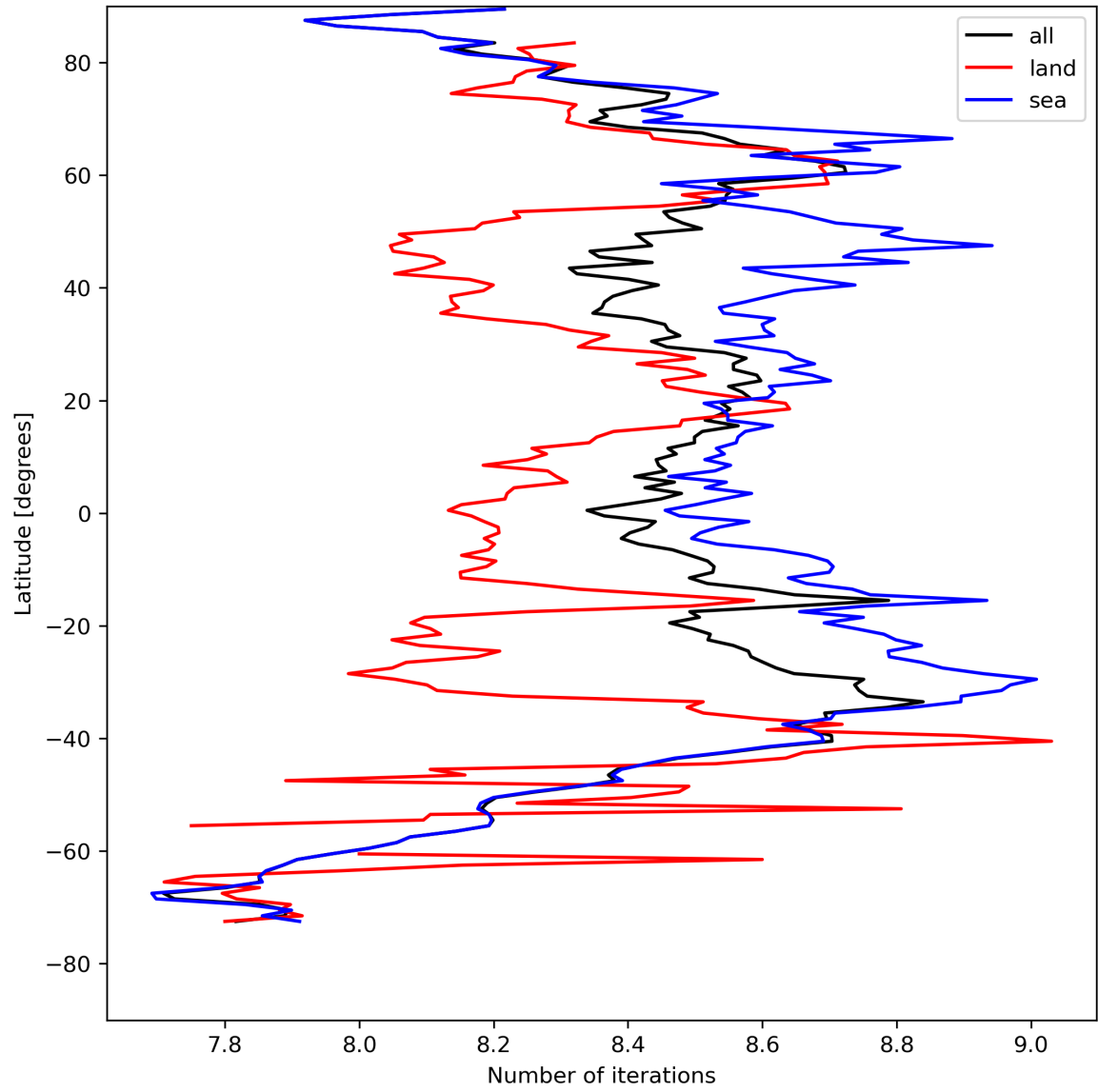
Figure 16: Zonal average of “Number of iterations” for 2024-04-21 to 2024-04-23.
