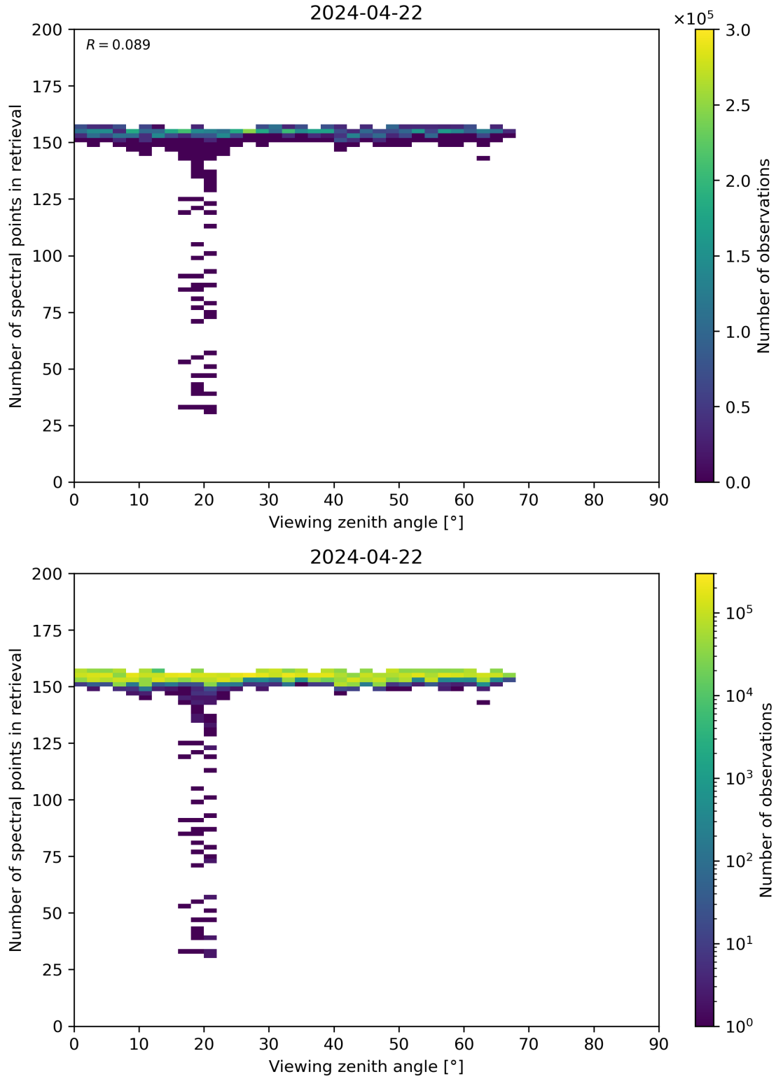
Figure 76: Scatter density plot of “Viewing zenith angle” against “Number of spectral points in retrieval” for 2024-04-21 to 2024-04-23.
