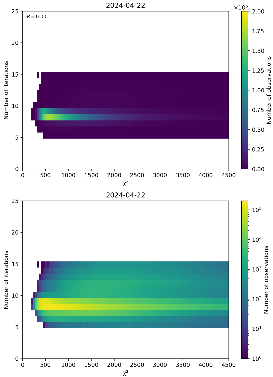
Figure 49: Scatter density plot of “ \chi^2 ” against “Number of iterations” for 2024-04-21 to 2024-04-23.
