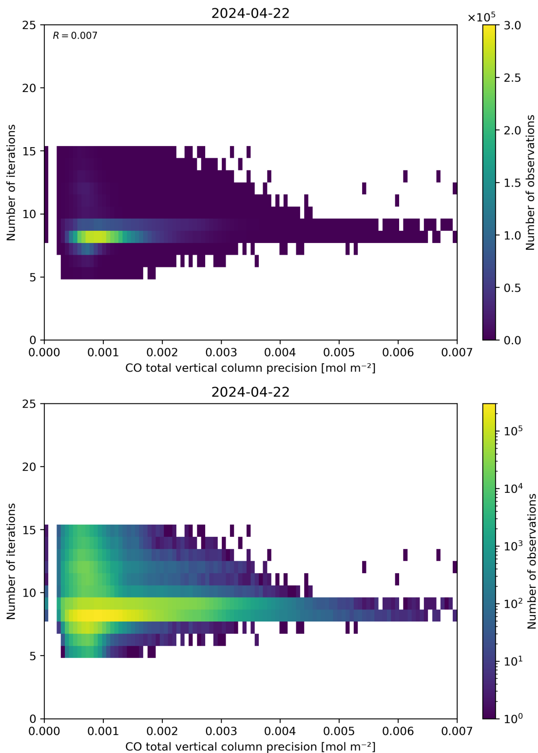
Figure 46: Scatter density plot of “CO total vertical column precision” against “Number of iterations” for 2024-04-21 to 2024-04-23.
