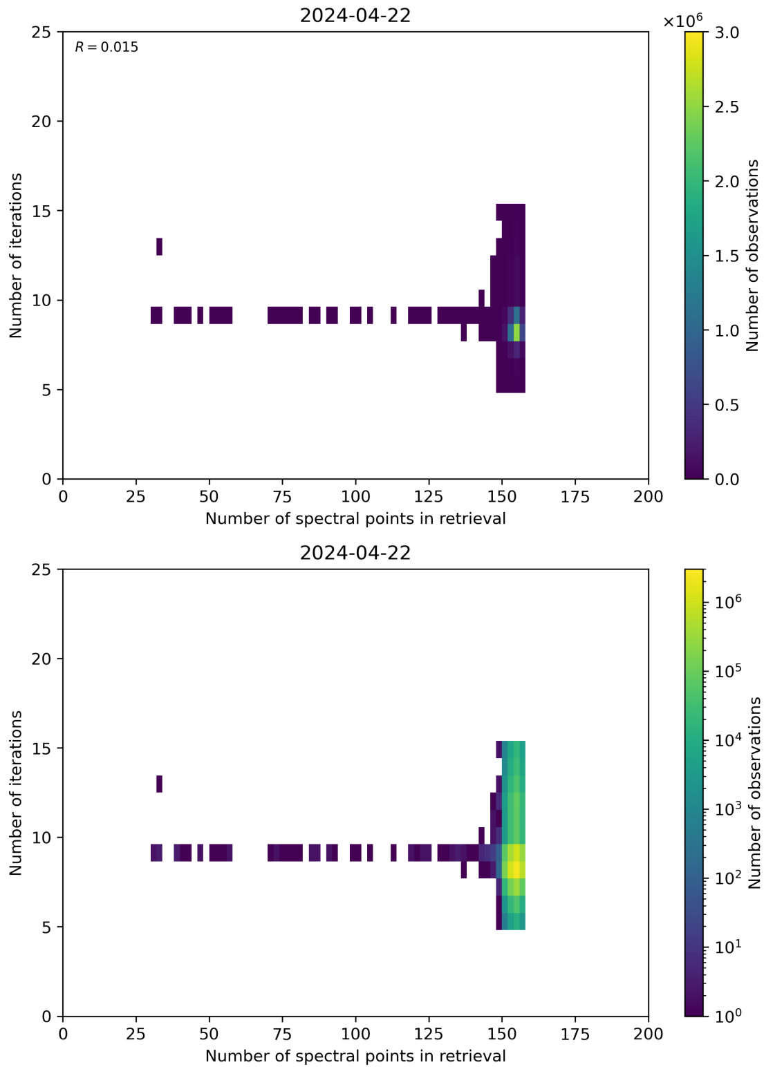
Figure 60: Scatter density plot of “Number of spectral points in retrieval” against “Number of iterations” for 2024-04-21 to 2024-04-23.
