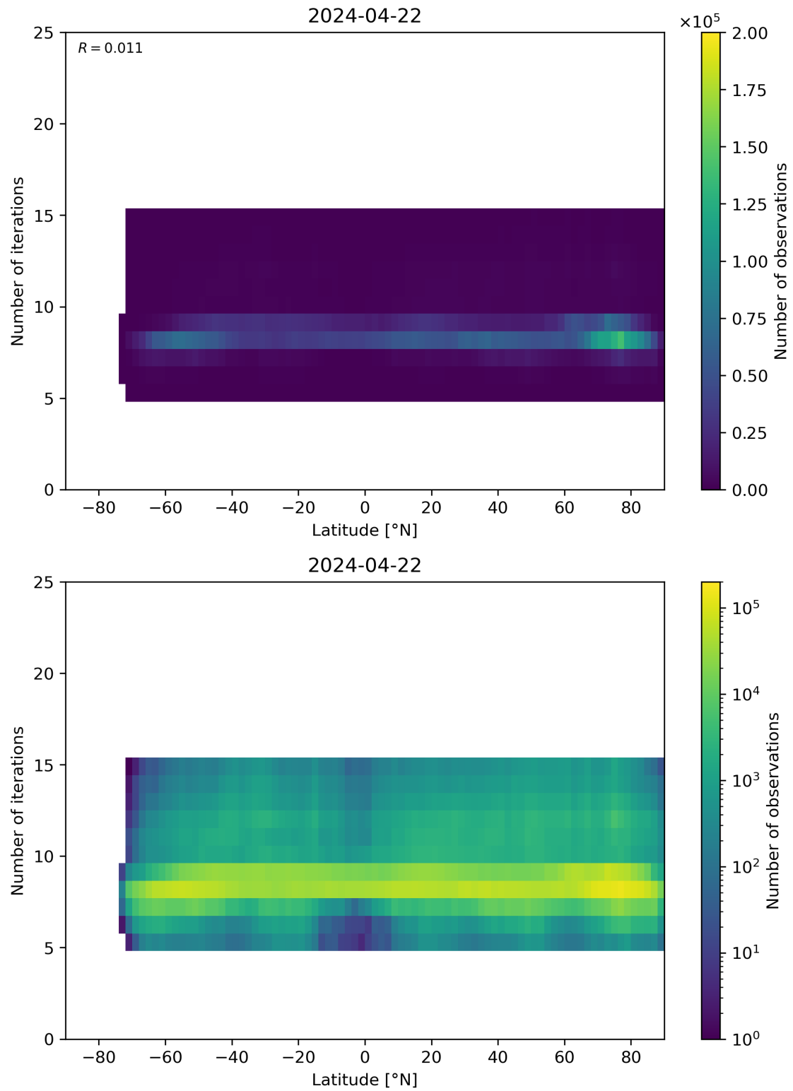
Figure 56: Scatter density plot of “Latitude” against “Number of iterations” for 2024-04-21 to 2024-04-23.
