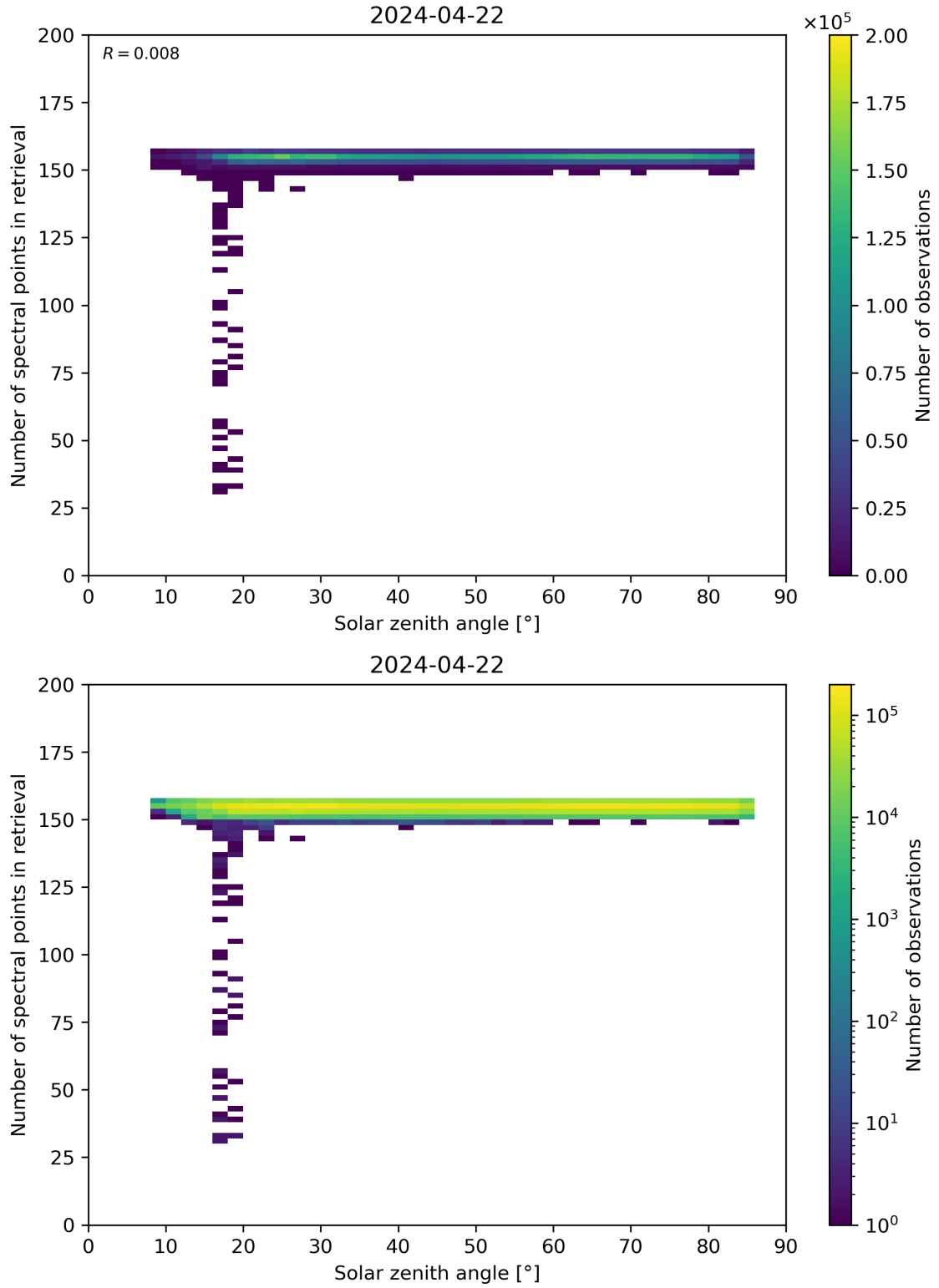
Figure 68: Scatter density plot of “Solar zenith angle” against “Number of spectral points in retrieval” for 2024-04-21 to 2024-04-23.
