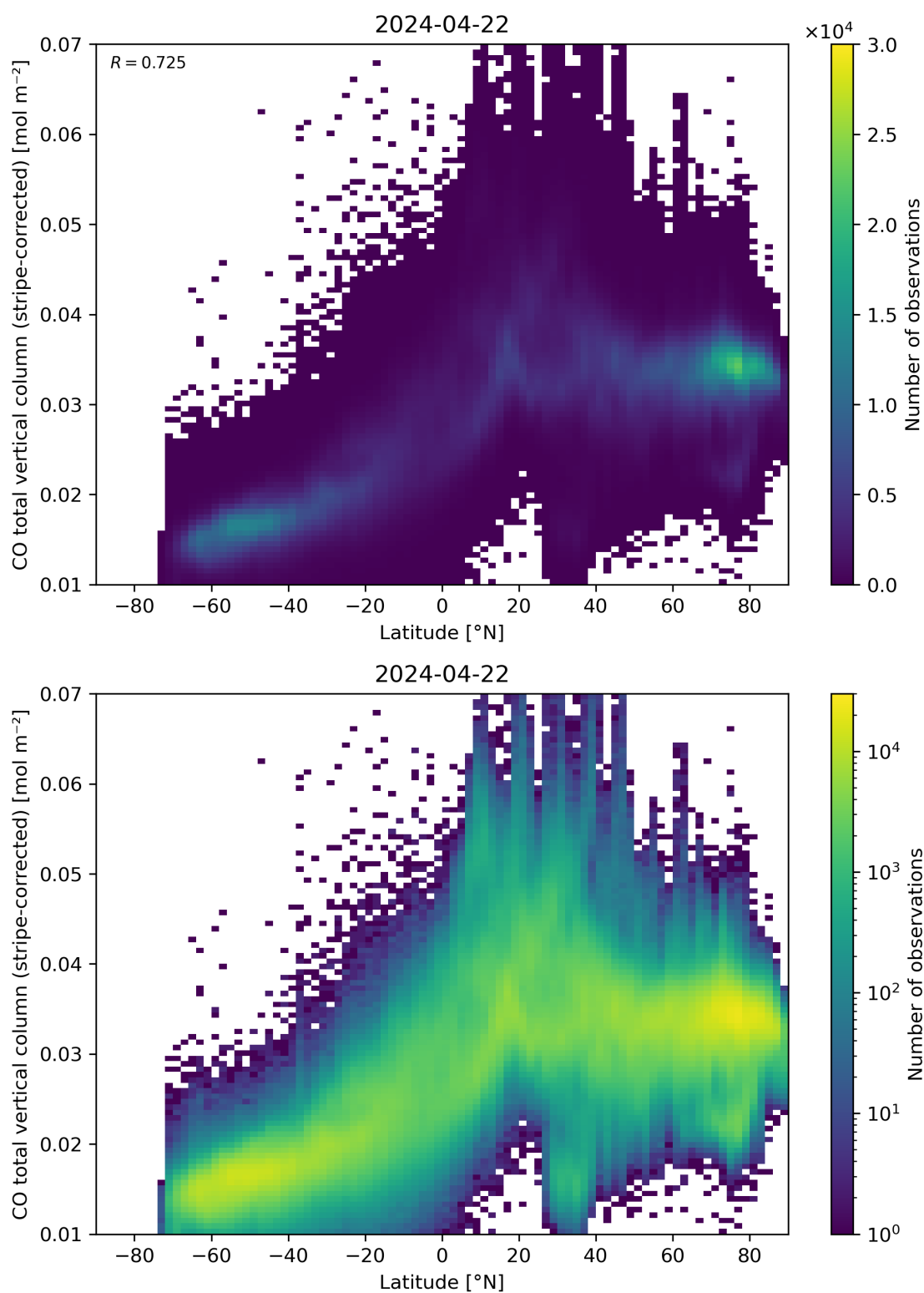
Figure 52: Scatter density plot of “Latitude” against “CO total vertical column (stripe-corrected)” for 2024-04-21 to 2024-04-23.
