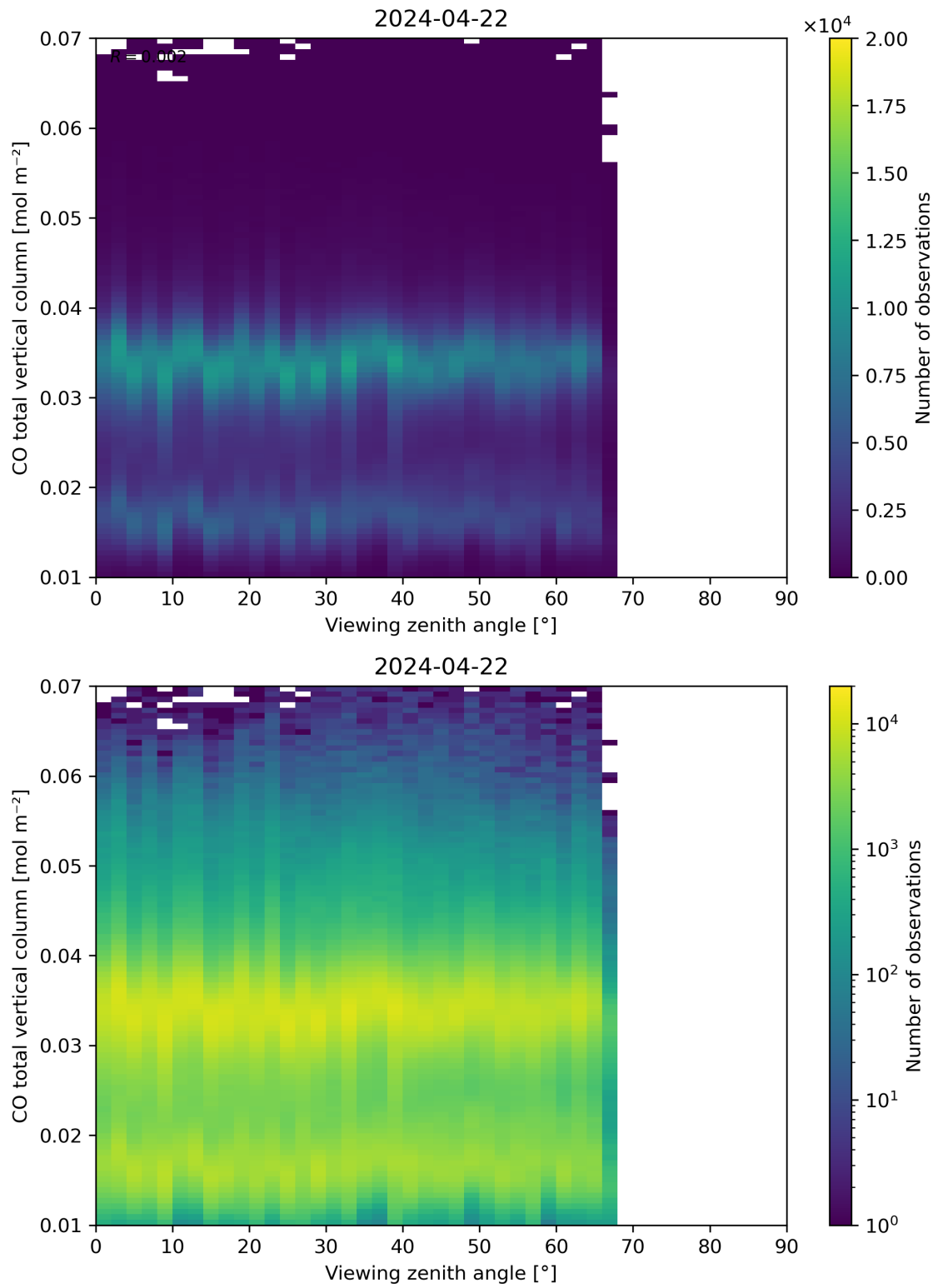
Figure 69: Scatter density plot of “Viewing zenith angle” against “CO total vertical column” for 2024-04-21 to 2024-04-23.
