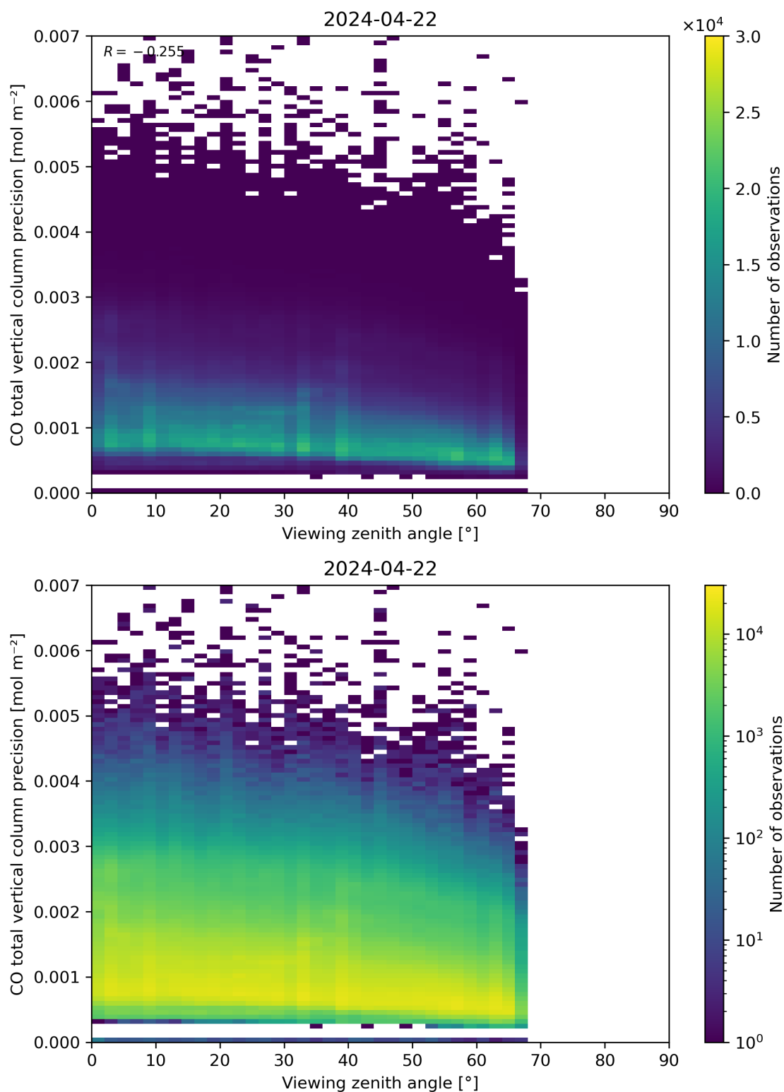
Figure 71: Scatter density plot of “Viewing zenith angle” against “CO total vertical column precision” for 2024-04-21 to 2024-04-23.
