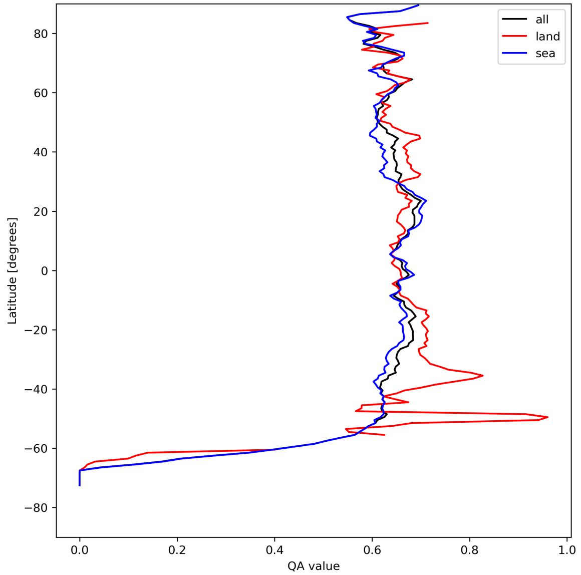
Figure 9: Zonal average of “QA value” for 2024-04-21 to 2024-04-23.
