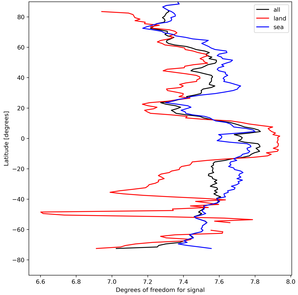
Figure 15: Zonal average of “Degrees of freedom for signal” for 2024-04-21 to 2024-04-23.
