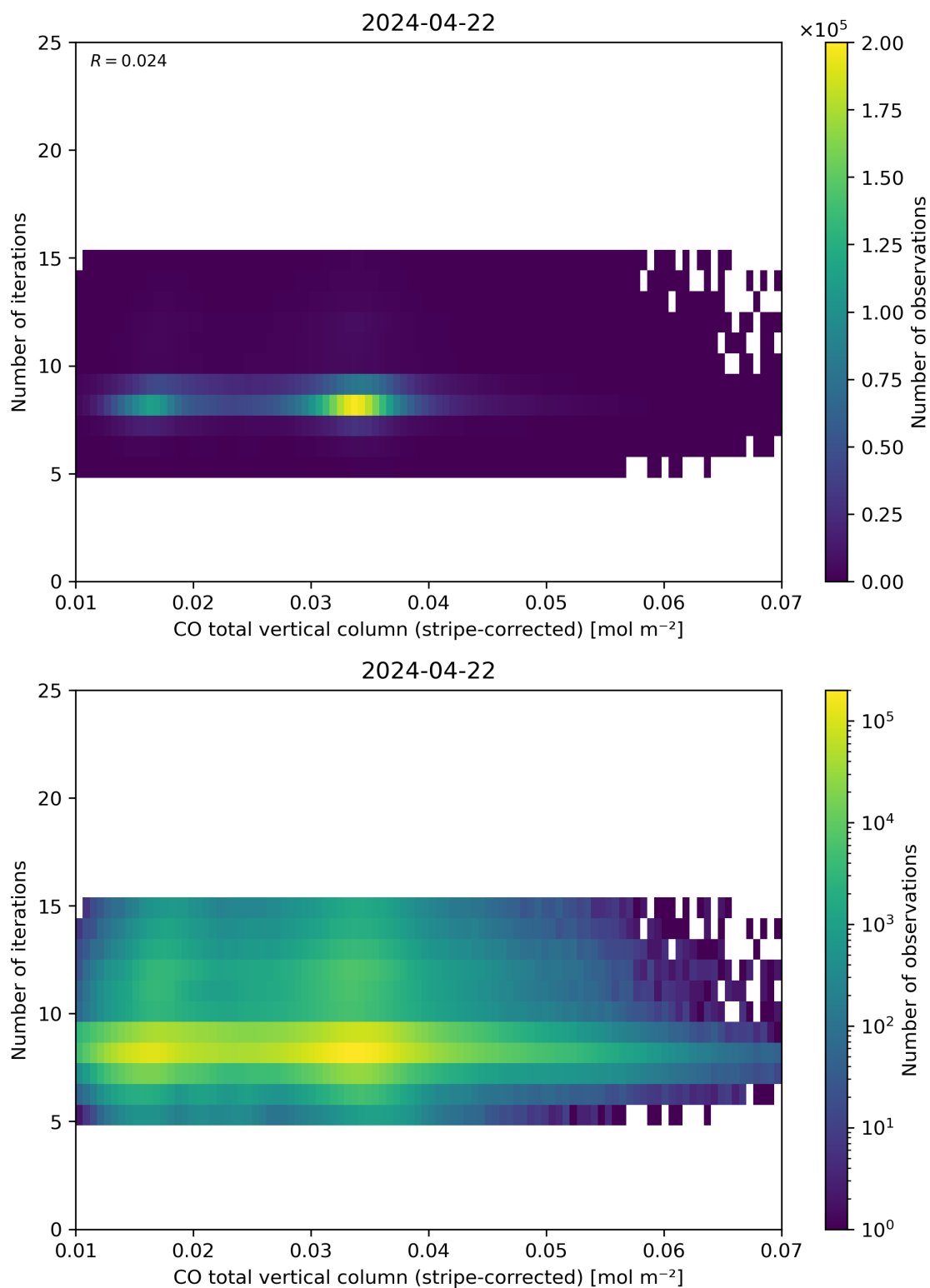
Figure 39: Scatter density plot of “CO total vertical column (stripe-corrected)” against “Number of iterations” for 2024-04-21 to 2024-04-23.
