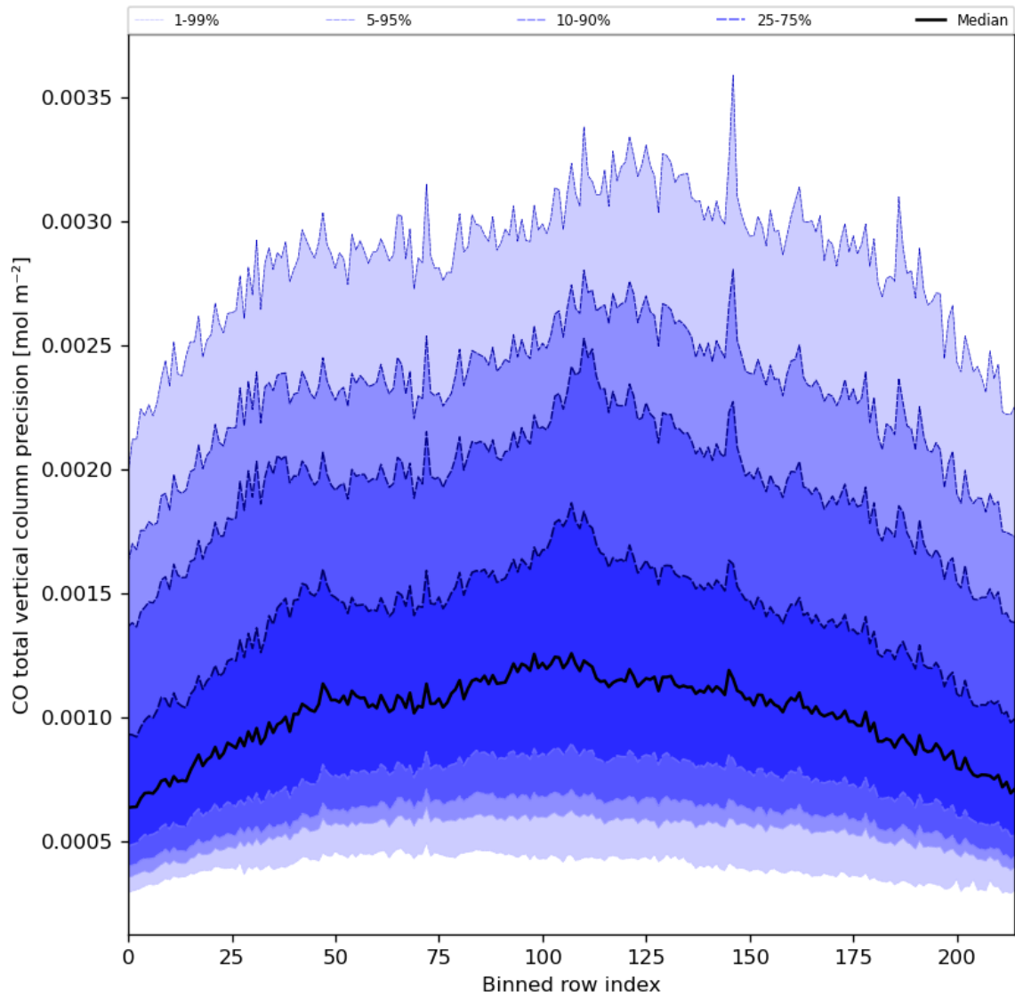
Figure 28: Along track statistics of “CO total vertical column precision” for 2024-04-21 to 2024-04-23
