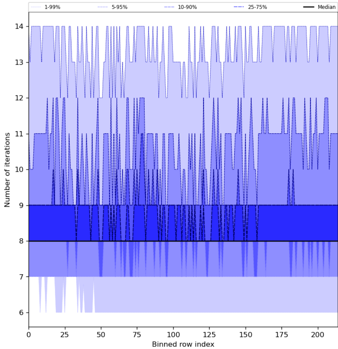
Figure 32: Along track statistics of “Number of iterations” for 2024-04-21 to 2024-04-23
