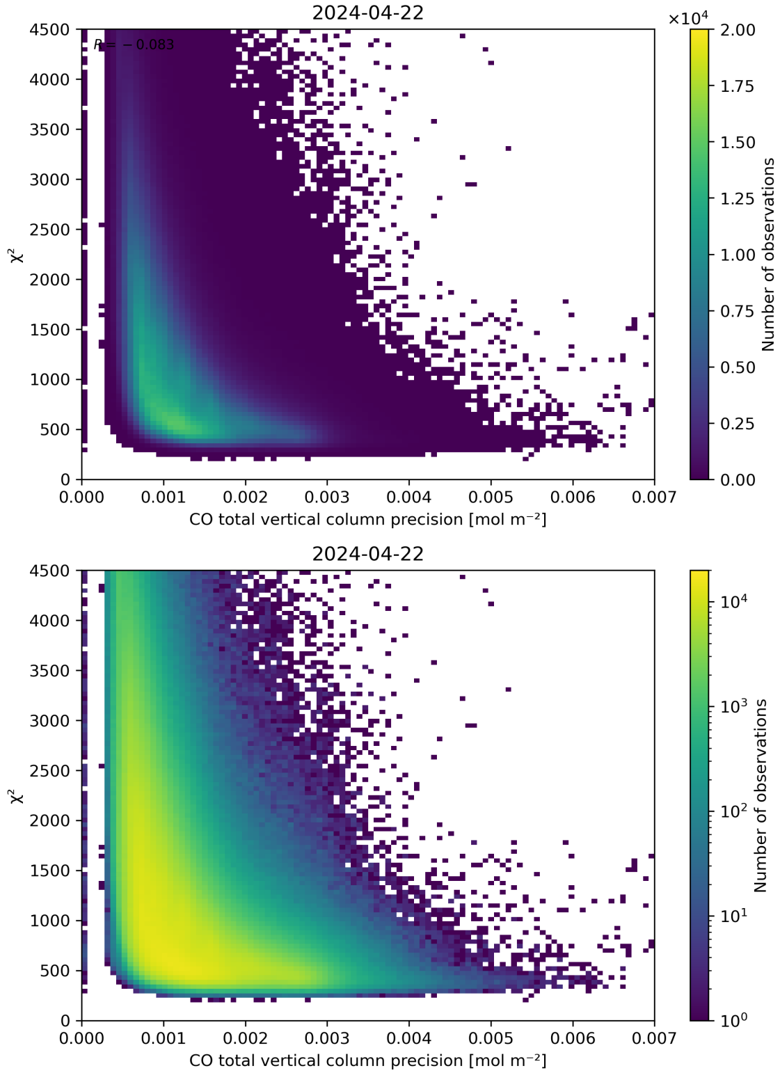
Figure 44: Scatter density plot of “CO total vertical column precision” against “ \chi^2 ” for 2024-04-21 to 2024-04-23.
