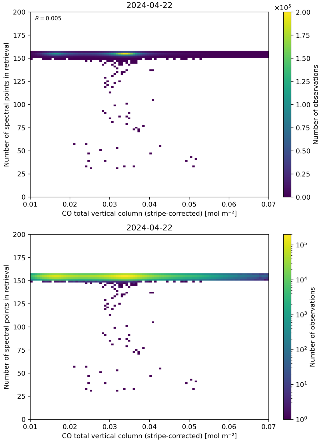
Figure 40: Scatter density plot of “CO total vertical column (stripe-corrected)” against “Number of spectral points in retrieval” for 2024-04-21 to 2024-04-23.
