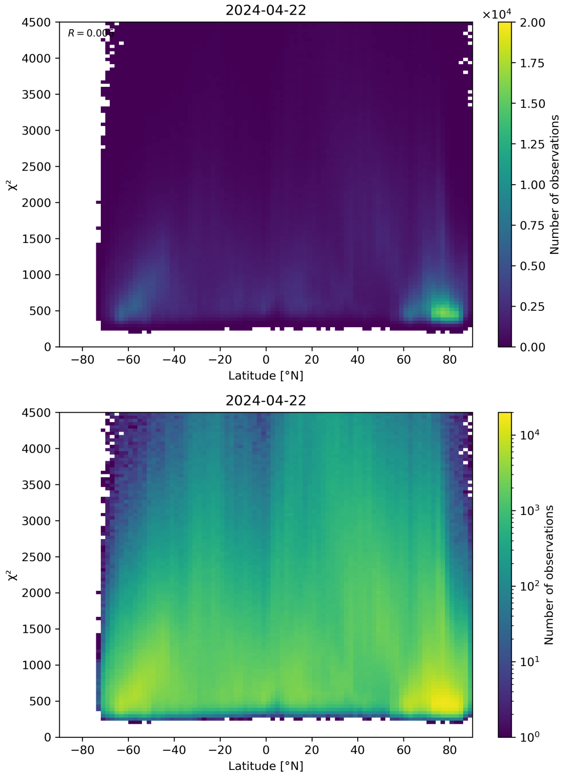
Figure 54: Scatter density plot of “Latitude” against “ \chi^2 ” for 2024-04-21 to 2024-04-23.
