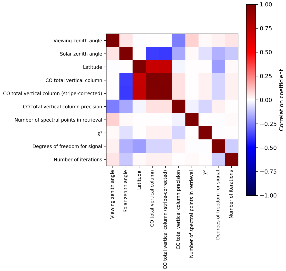
Figure 2: Map of correlation matrix for 2024-04-21 to 2024-04-23.
