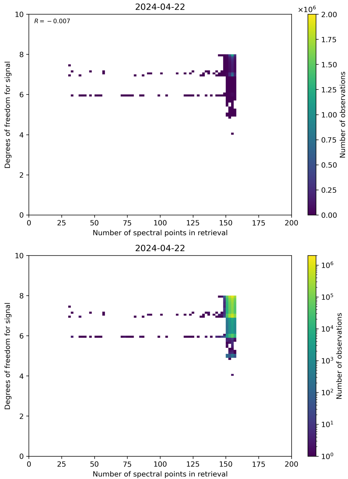
Figure 59: Scatter density plot of “Number of spectral points in retrieval” against “Degrees of freedom for signal” for 2024-04-21 to 2024-04-23.
