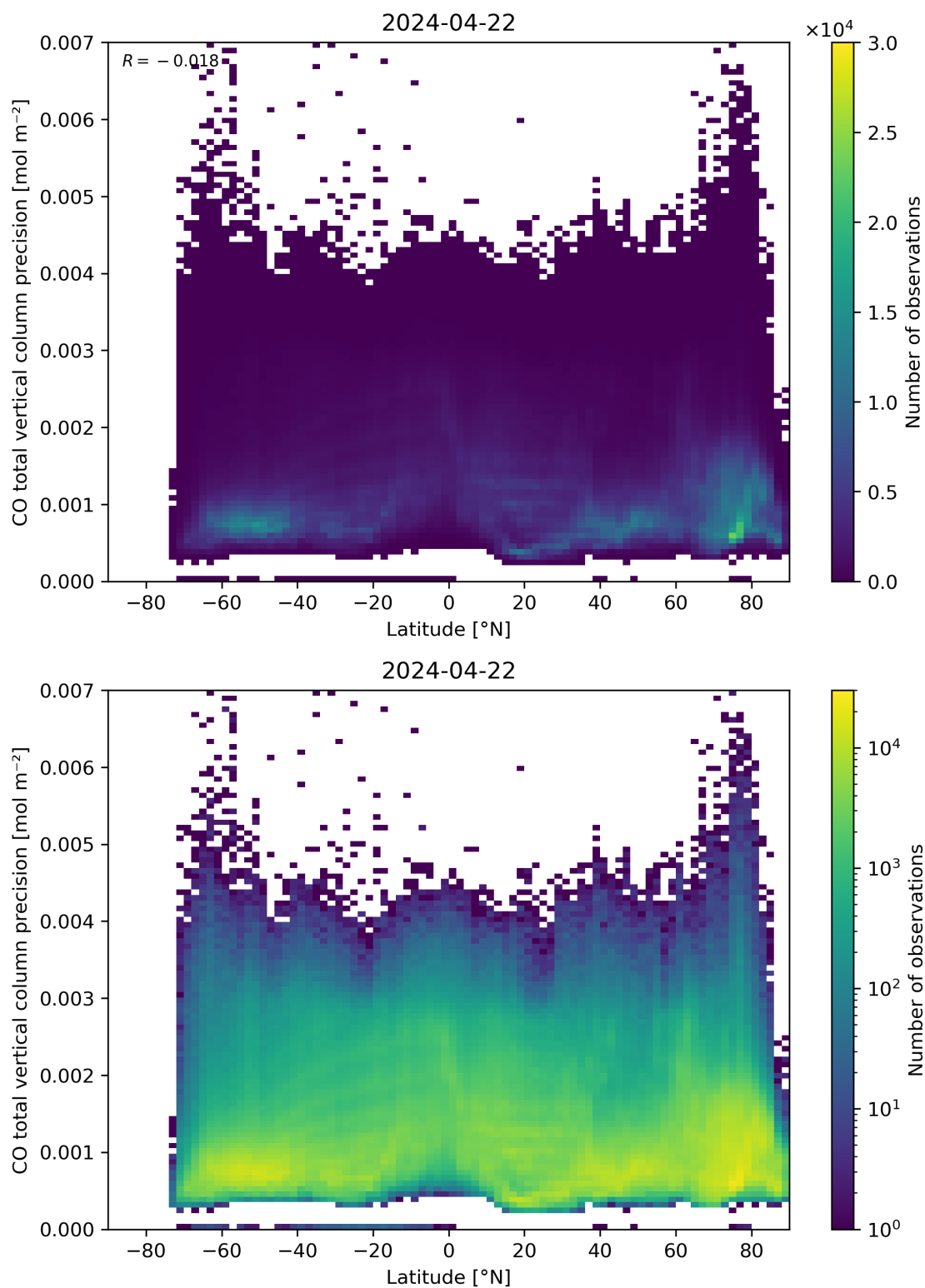
Figure 53: Scatter density plot of “Latitude” against “CO total vertical column precision” for 2024-04-21 to 2024-04-23.
