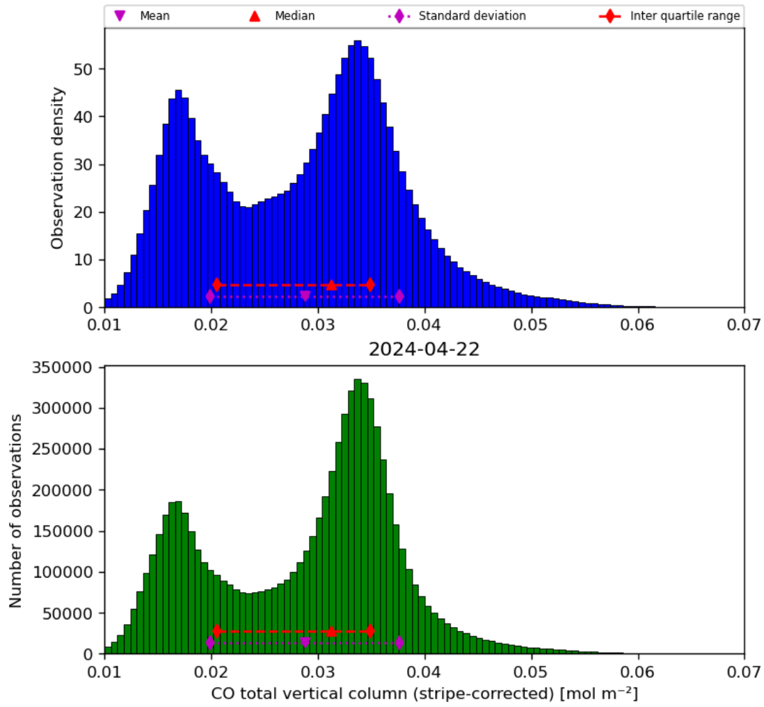
Figure 19: Histogram of “CO total vertical column (stripe-corrected)” for 2024-04-21 to 2024-04-23
