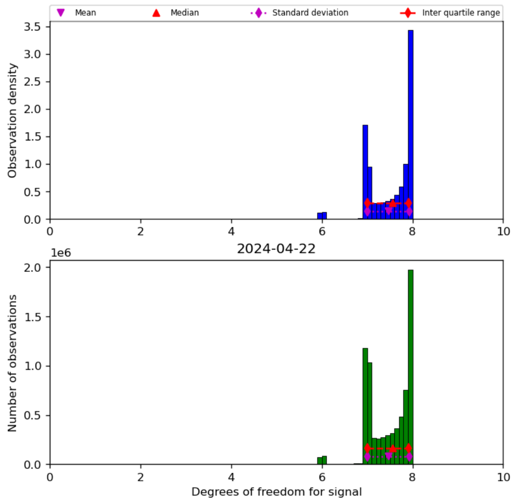
Figure 23: Histogram of “Degrees of freedom for signal” for 2024-04-21 to 2024-04-23
