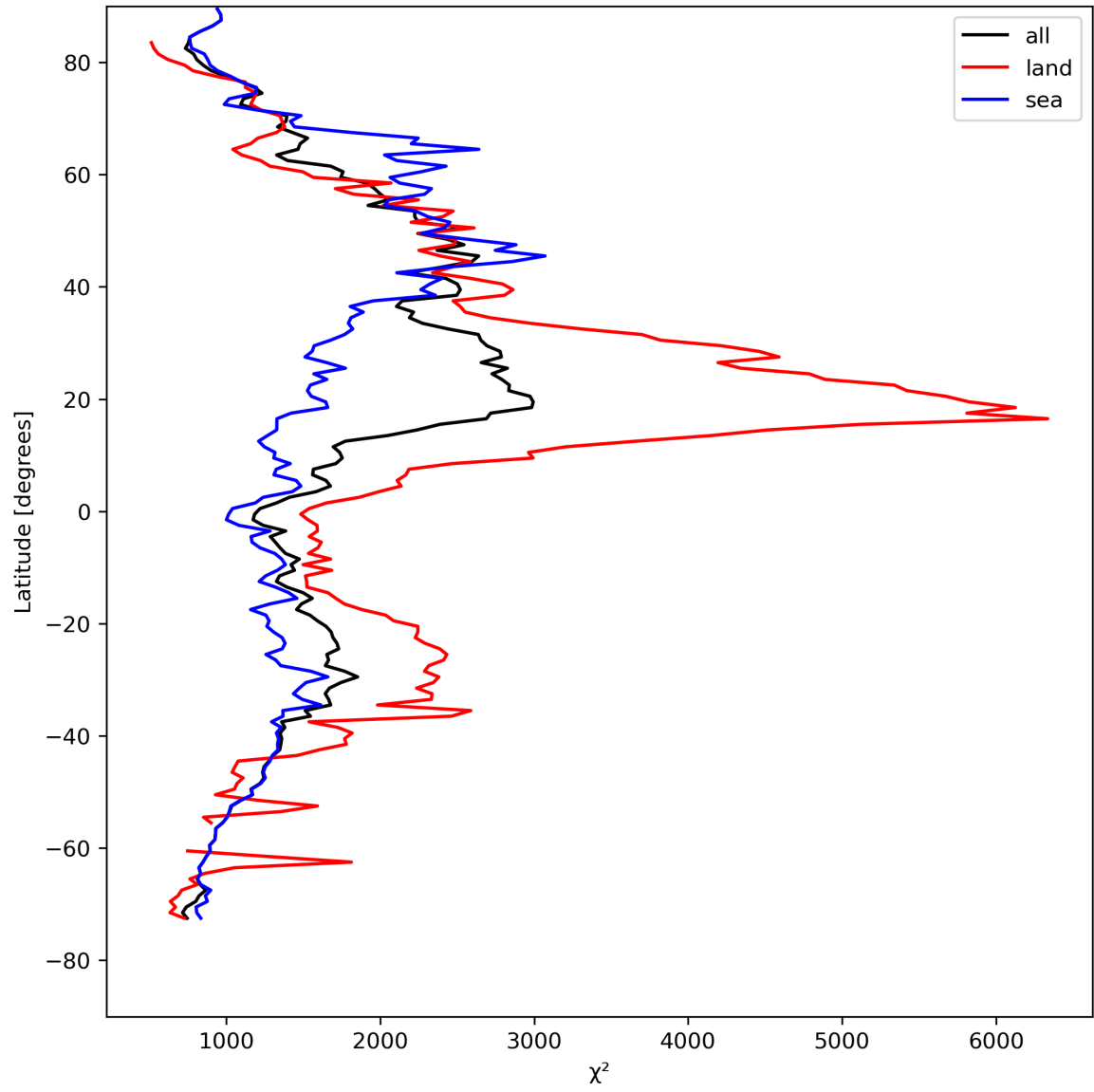
Figure 14: Zonal average of “ \chi^2 ” for 2024-04-21 to 2024-04-23.
