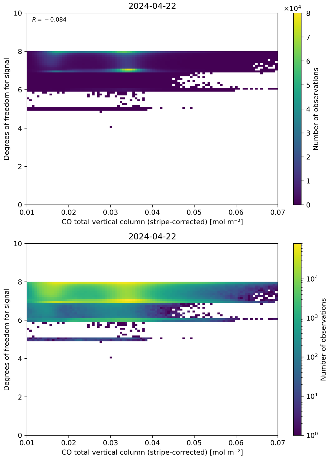
Figure 38: Scatter density plot of “CO total vertical column (stripe-corrected)” against “Degrees of freedom for signal” for 2024-04-21 to 2024-04-23.
