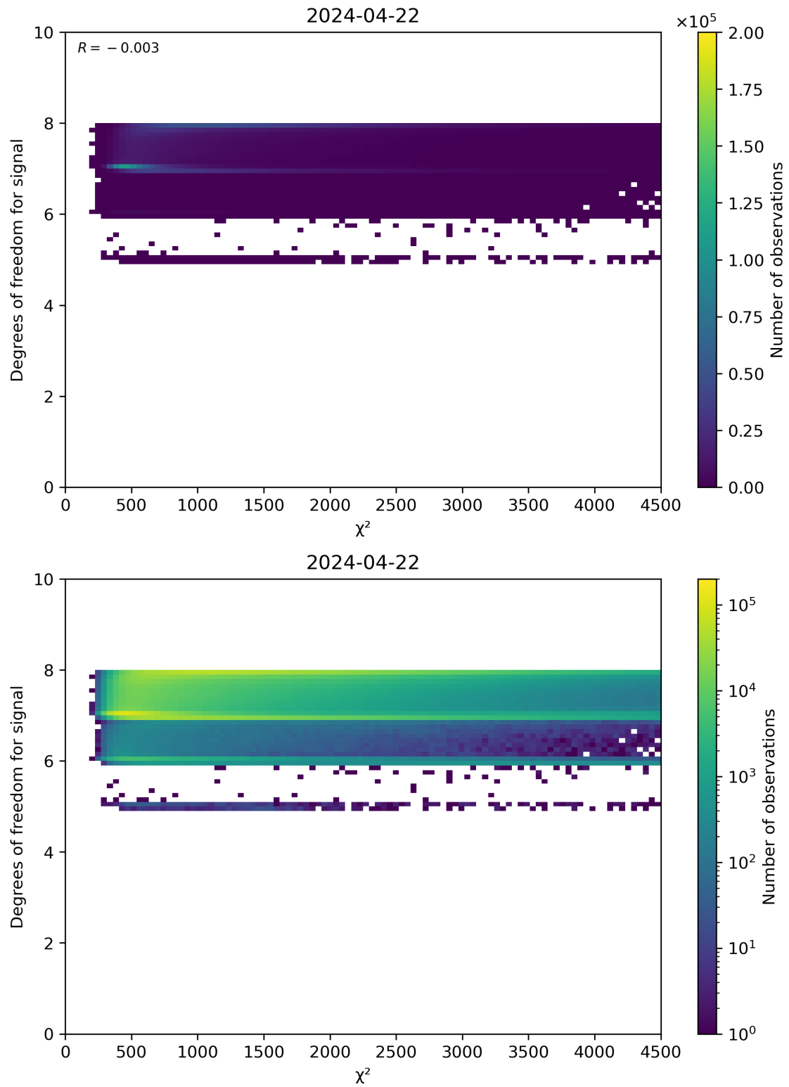
Figure 48: Scatter density plot of “ \chi^2 ” against “Degrees of freedom for signal” for 2024-04-21 to 2024-04-23.
