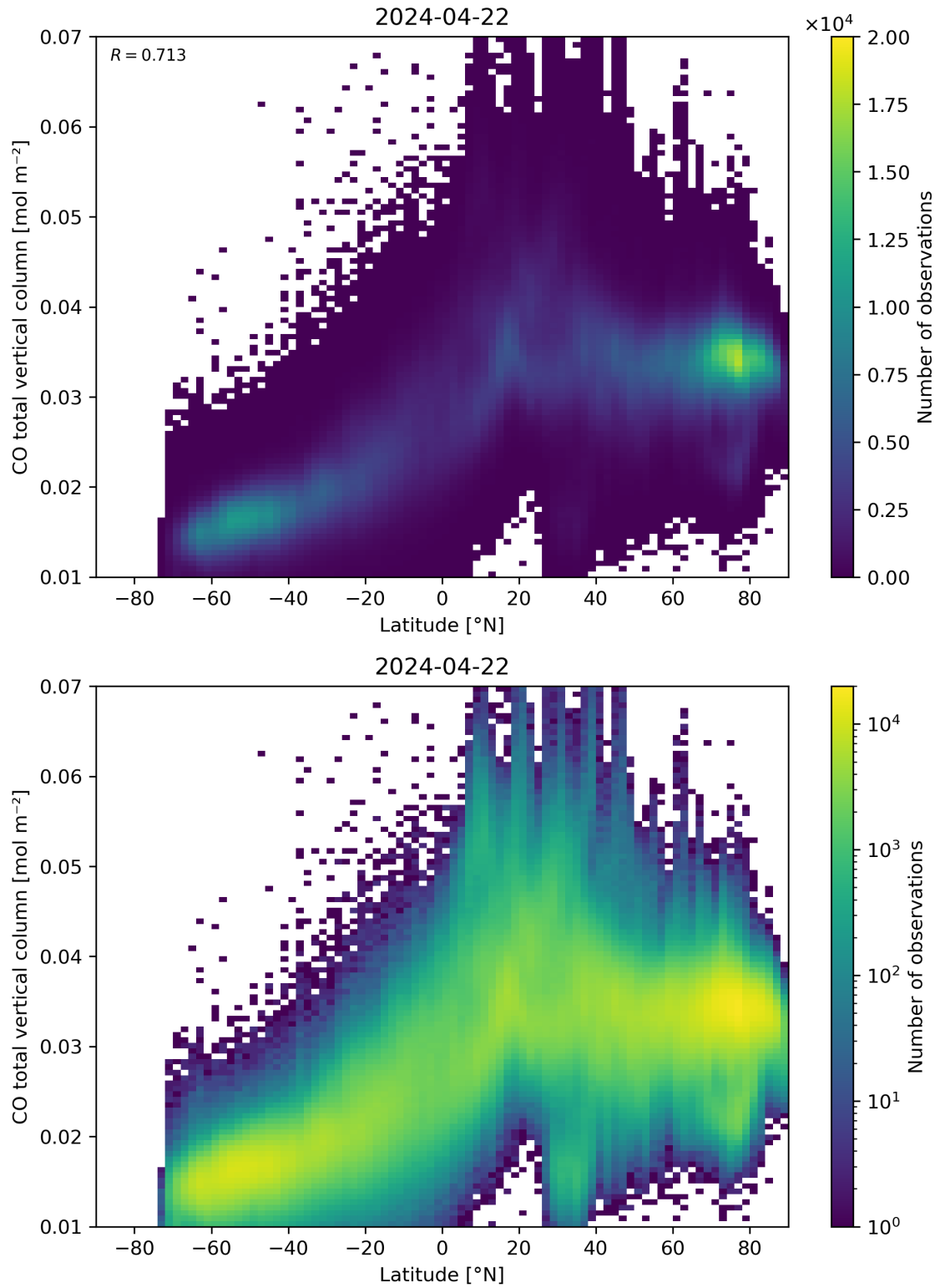
Figure 51: Scatter density plot of “Latitude” against “CO total vertical column” for 2024-04-21 to 2024-04-23.
