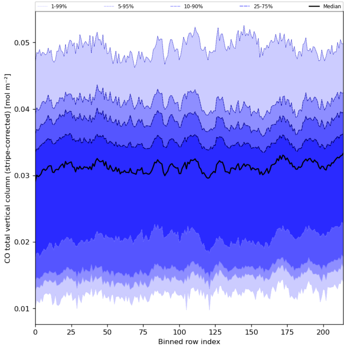
Figure 27: Along track statistics of “CO total vertical column (stripe-corrected)” for 2024-04-21 to 2024-04-23
