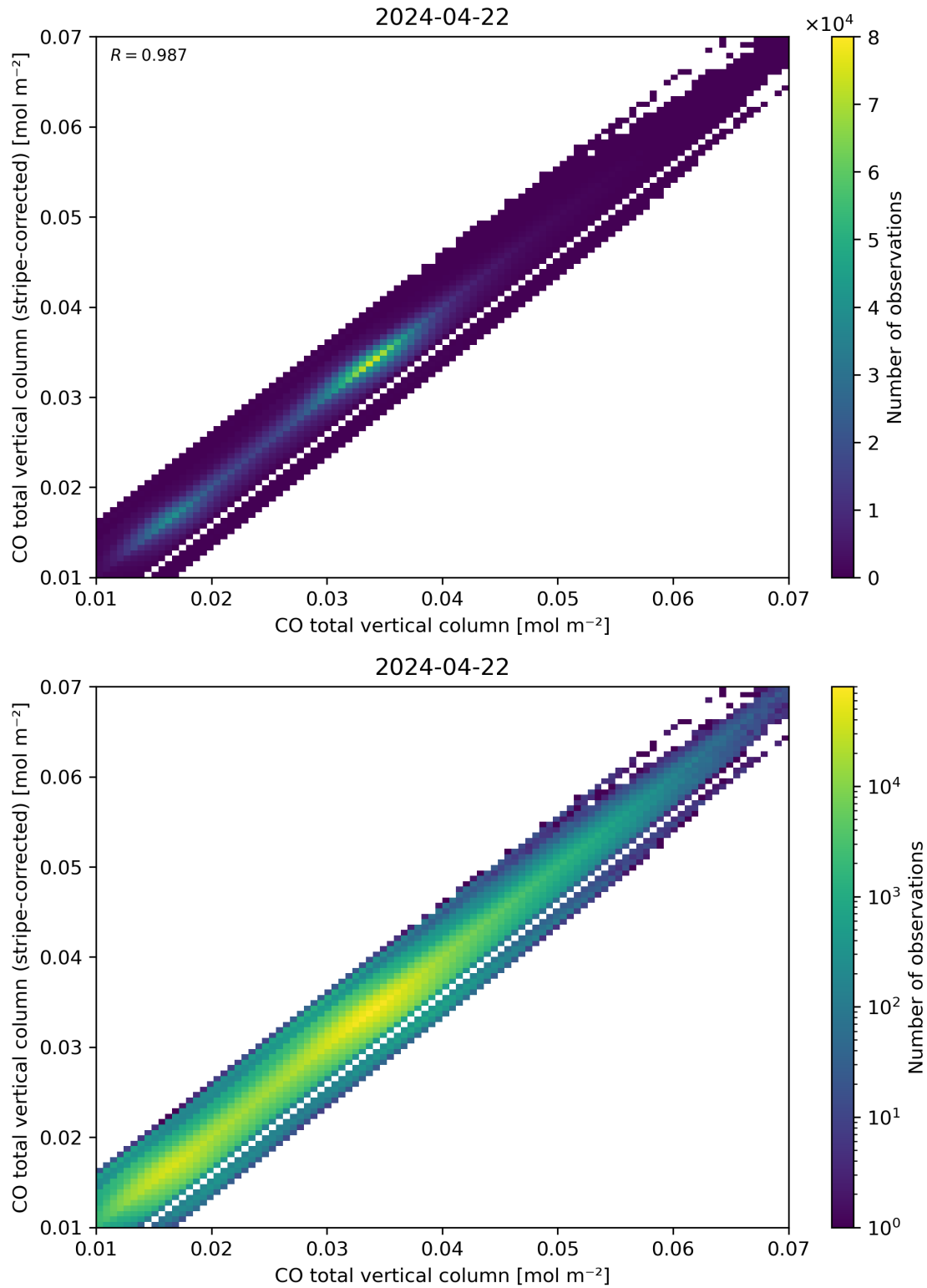
Figure 33: Scatter density plot of “CO total vertical column” against “CO total vertical column (stripe-corrected)” for 2024-04-21 to 2024-04-23.
