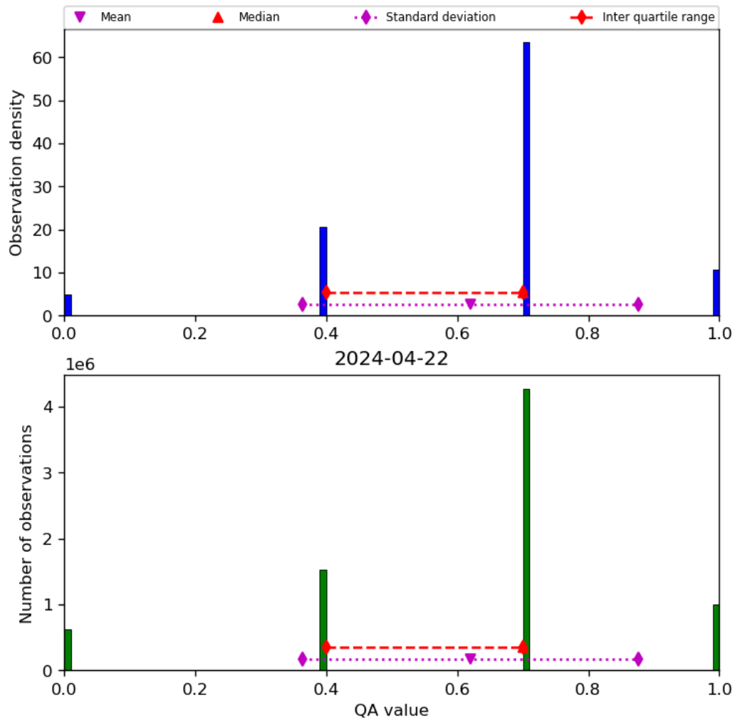
Figure 17: Histogram of “QA value” for 2024-04-21 to 2024-04-23
