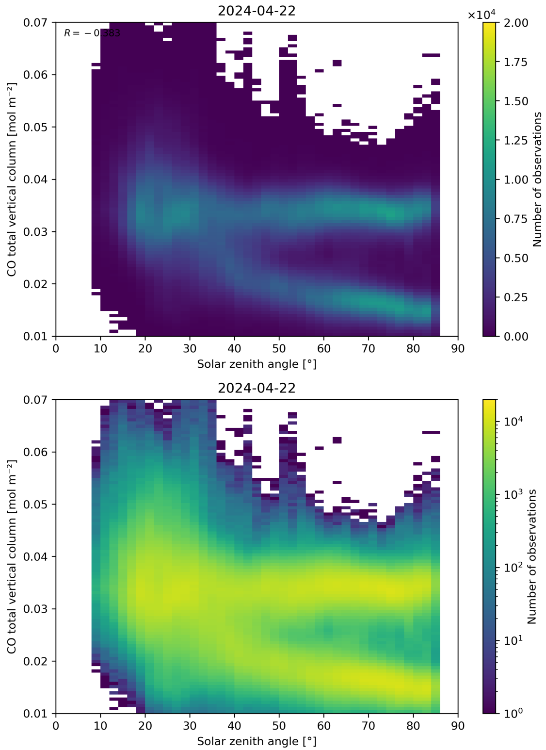
Figure 61: Scatter density plot of “Solar zenith angle” against “CO total vertical column” for 2024-04-21 to 2024-04-23.
