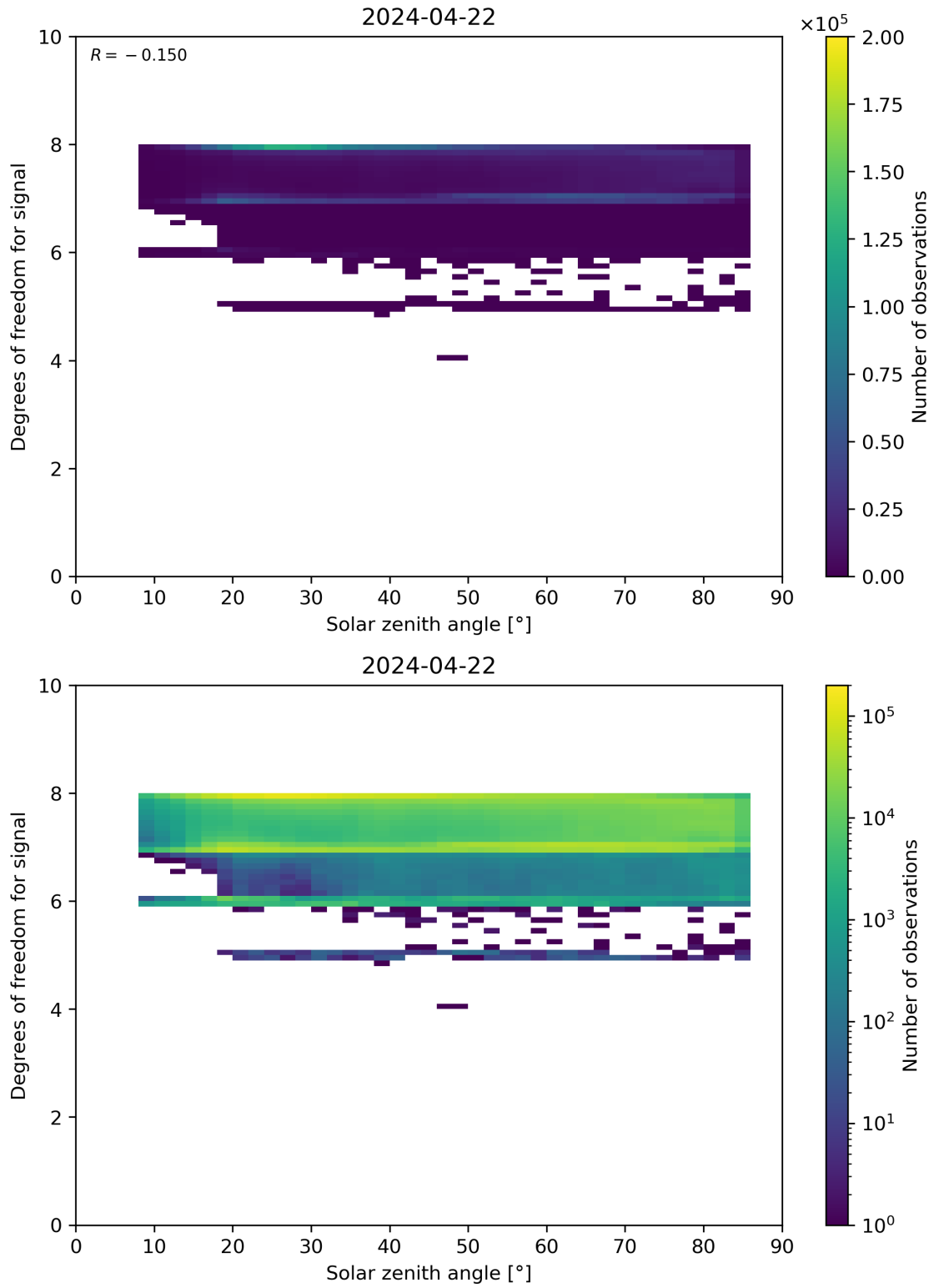
Figure 65: Scatter density plot of “Solar zenith angle” against “Degrees of freedom for signal” for 2024-04-21 to 2024-04-23.
