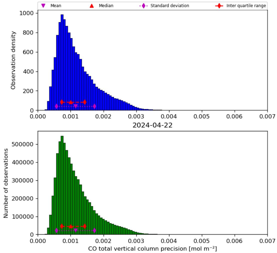
Figure 20: Histogram of “CO total vertical column precision” for 2024-04-21 to 2024-04-23
