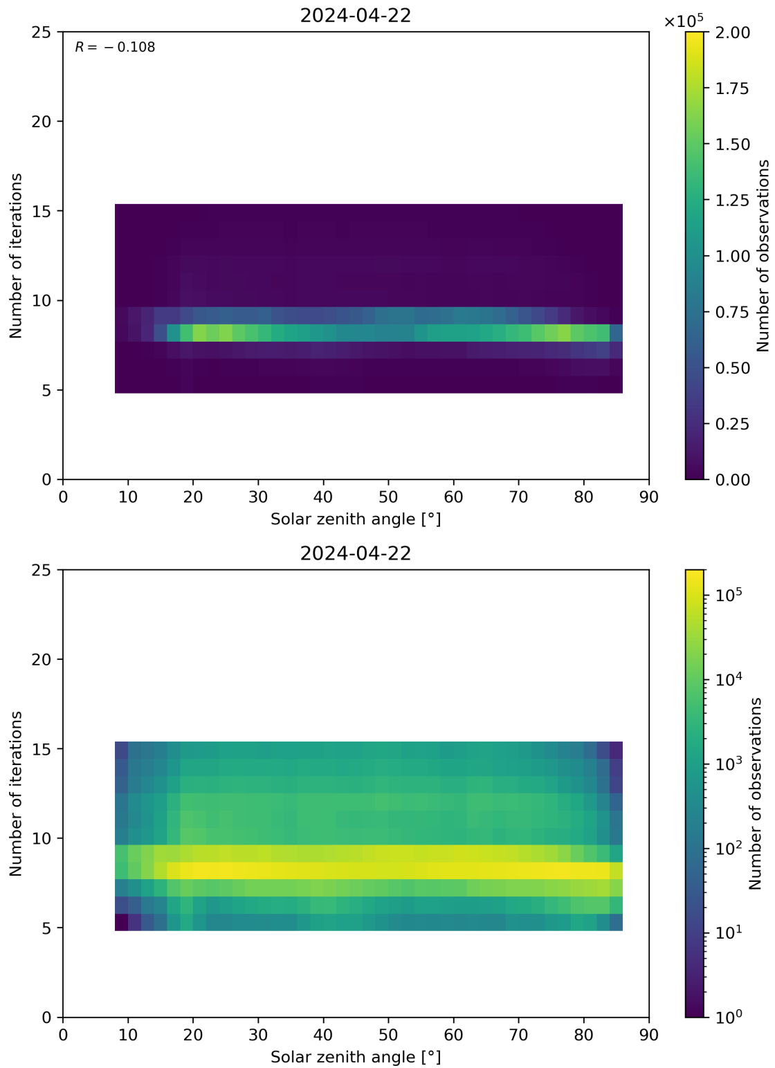
Figure 67: Scatter density plot of “Solar zenith angle” against “Number of iterations” for 2024-04-21 to 2024-04-23.
