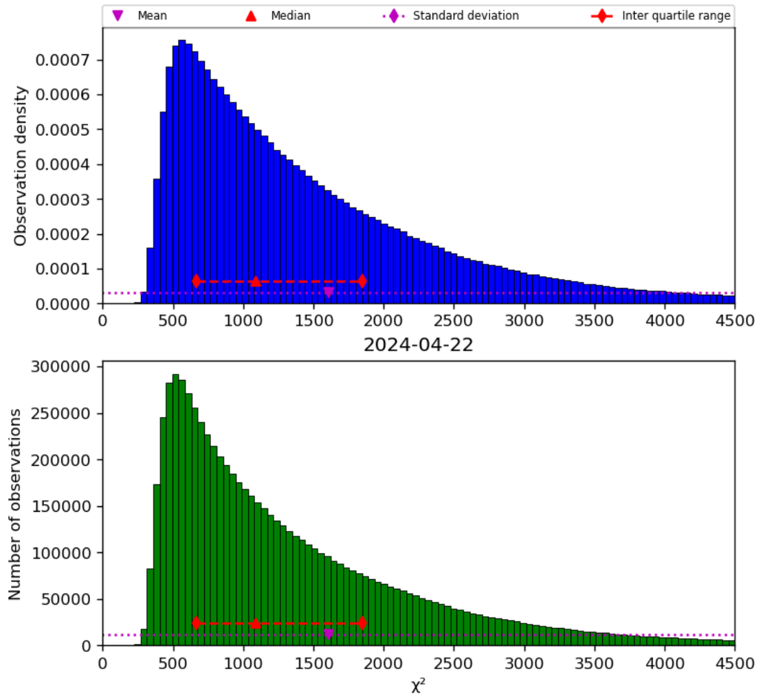
Figure 22: Histogram of “ \chi^2 ” for 2024-04-21 to 2024-04-23
