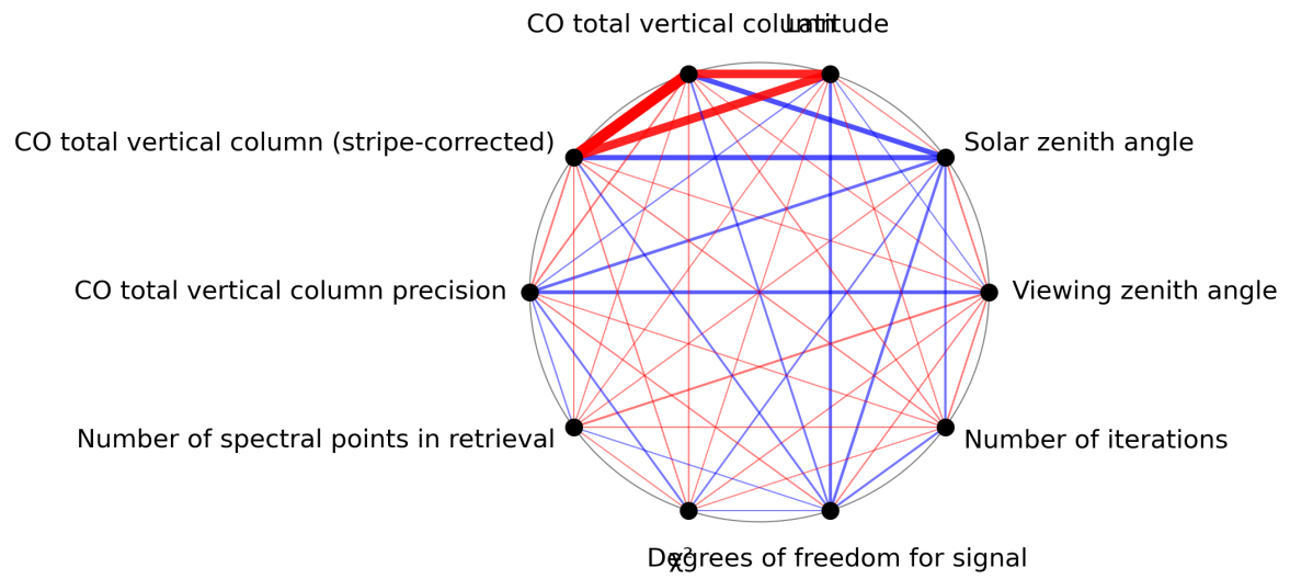
Figure 1: Map of correlation graph for 2024-04-21 to 2024-04-23.
