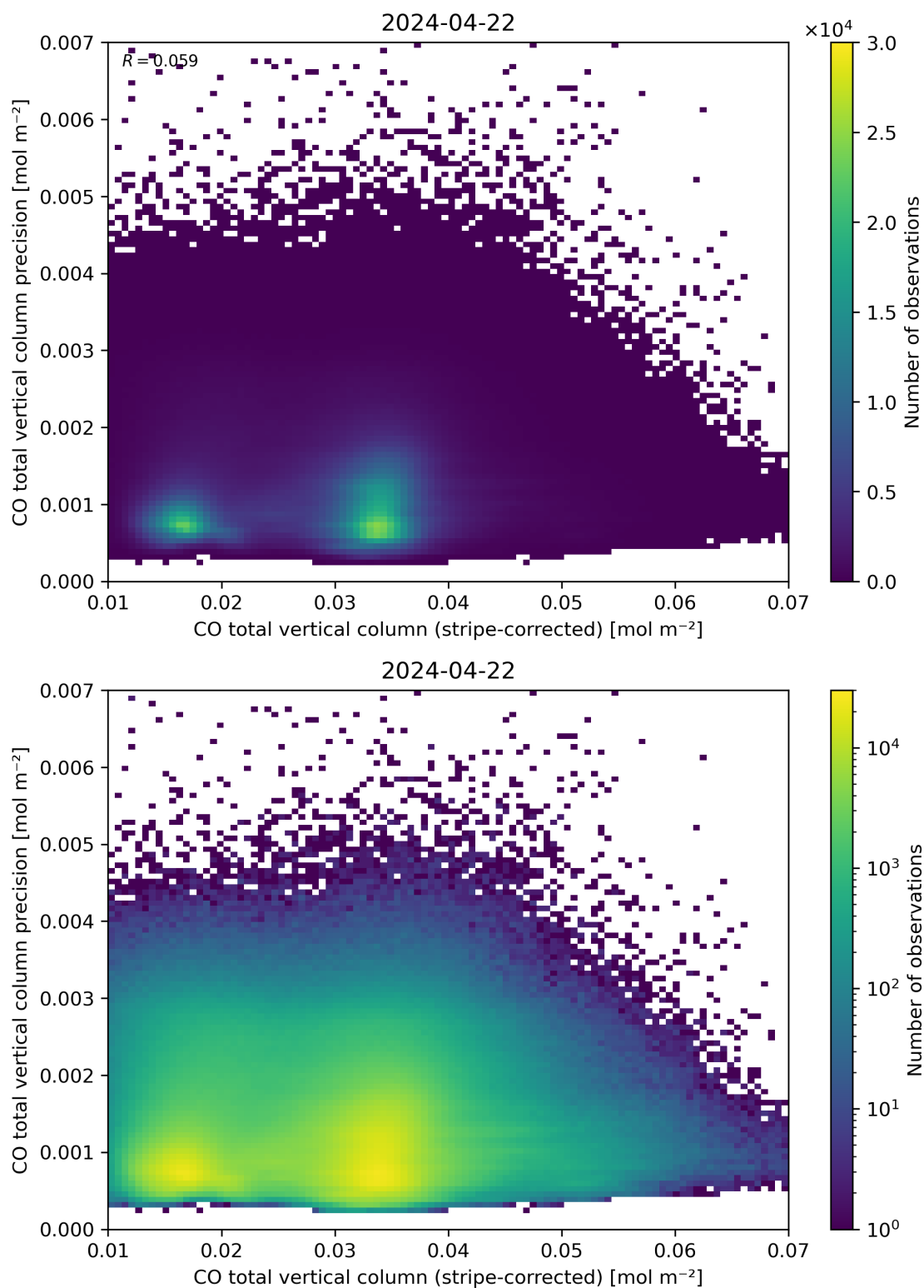
Figure 36: Scatter density plot of “CO total vertical column (stripe-corrected)” against “CO total vertical column precision” for 2024-04-21 to 2024-04-23.
