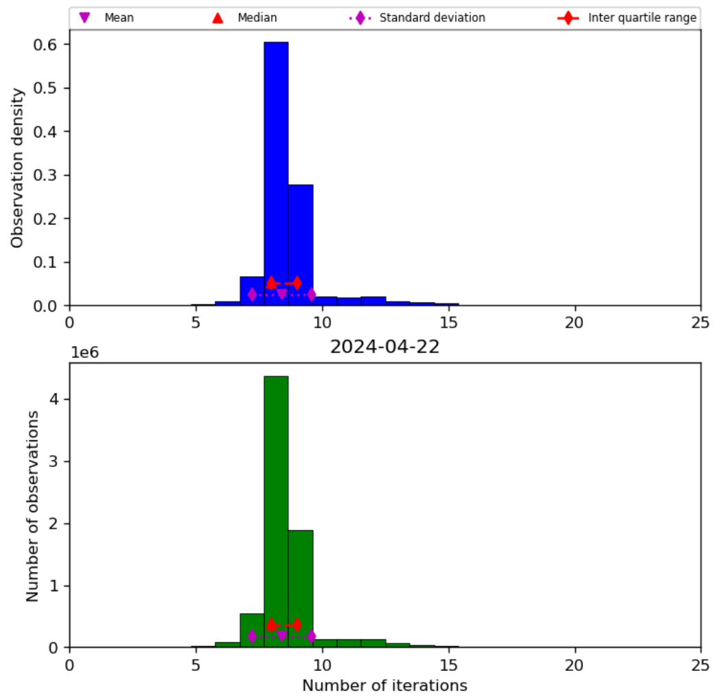
Figure 24: Histogram of “Number of iterations” for 2024-04-21 to 2024-04-23
