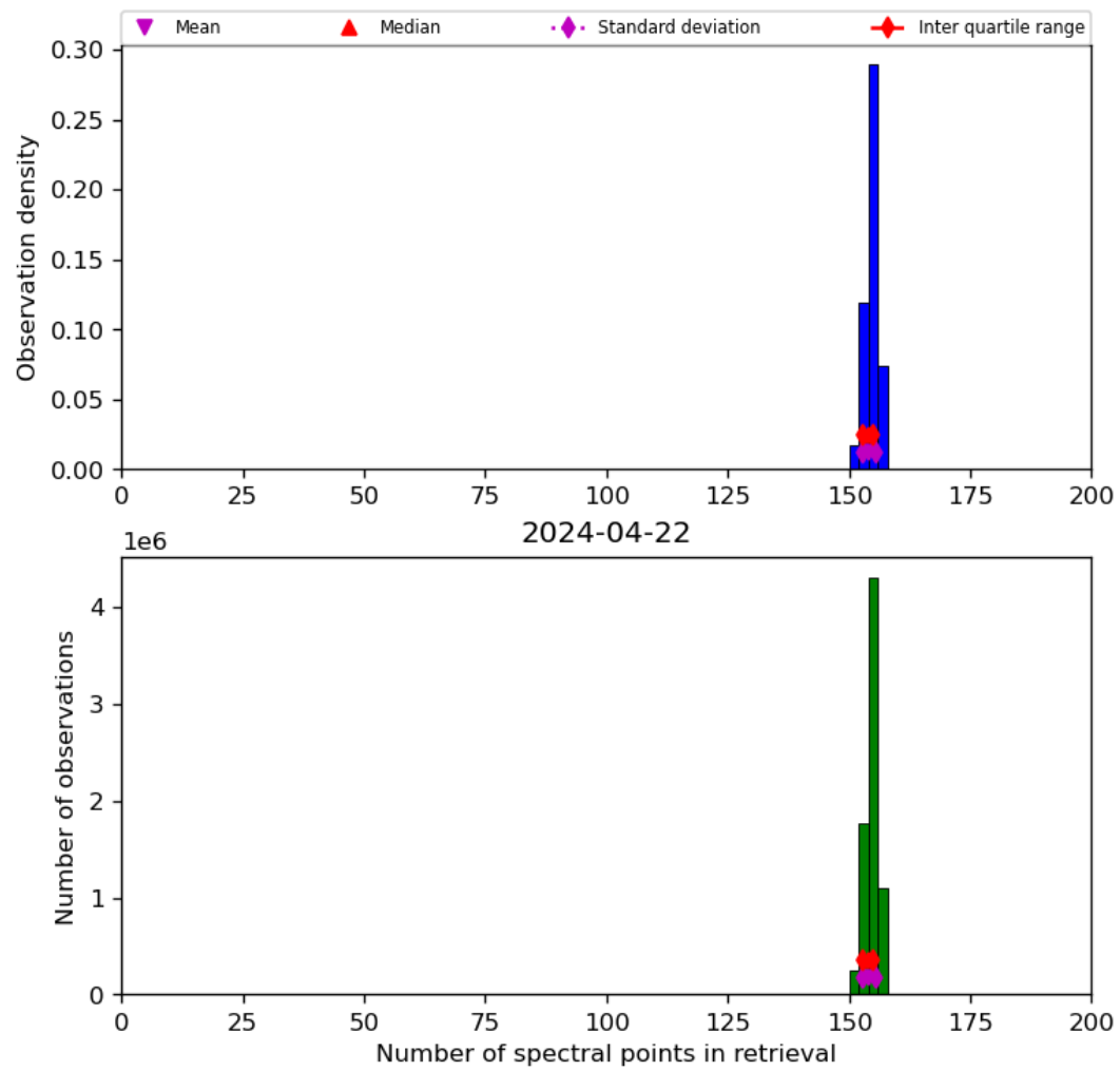
Figure 21: Histogram of “Number of spectral points in retrieval” for 2024-04-21 to 2024-04-23
