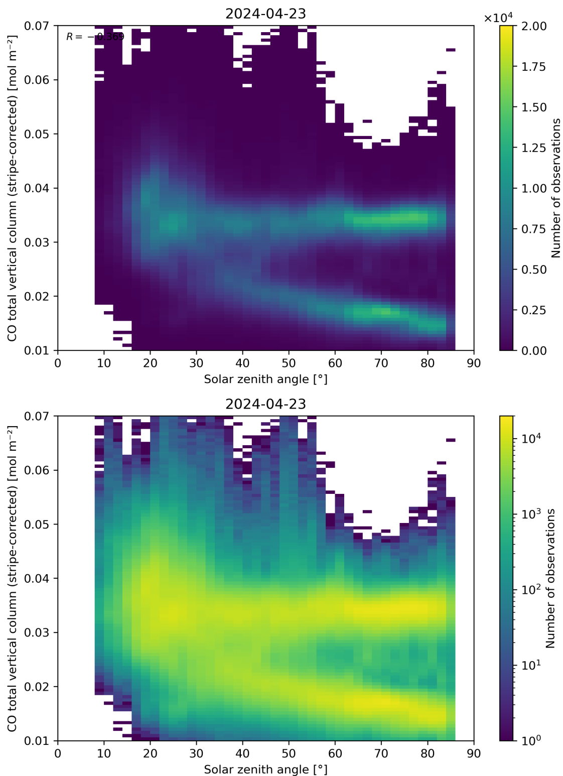
Figure 62: Scatter density plot of “Solar zenith angle” against “CO total vertical column (stripe-corrected)” for 2024-04-22 to 2024-04-24.
