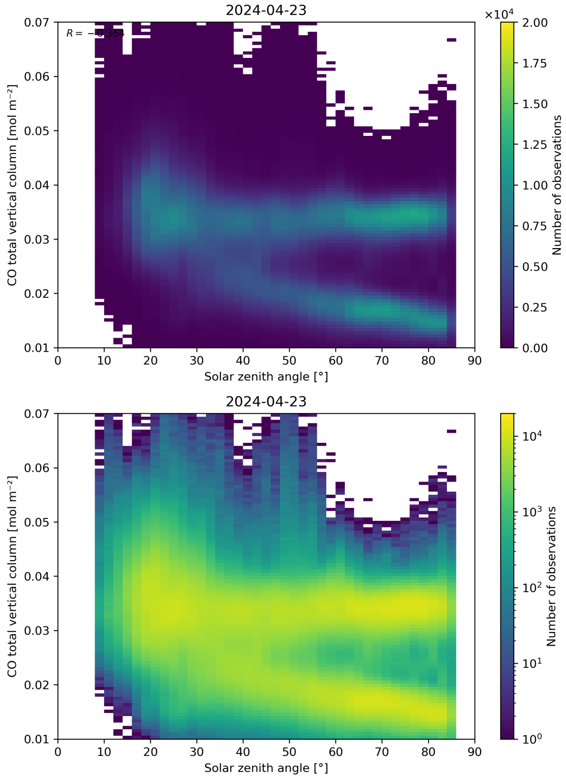
Figure 61: Scatter density plot of “Solar zenith angle” against “CO total vertical column” for 2024-04-22 to 2024-04-24.
