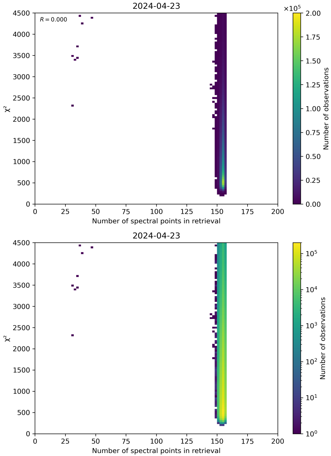
Figure 58: Scatter density plot of “Number of spectral points in retrieval” against “ \chi^2 ” for 2024-04-22 to 2024-04-24.
