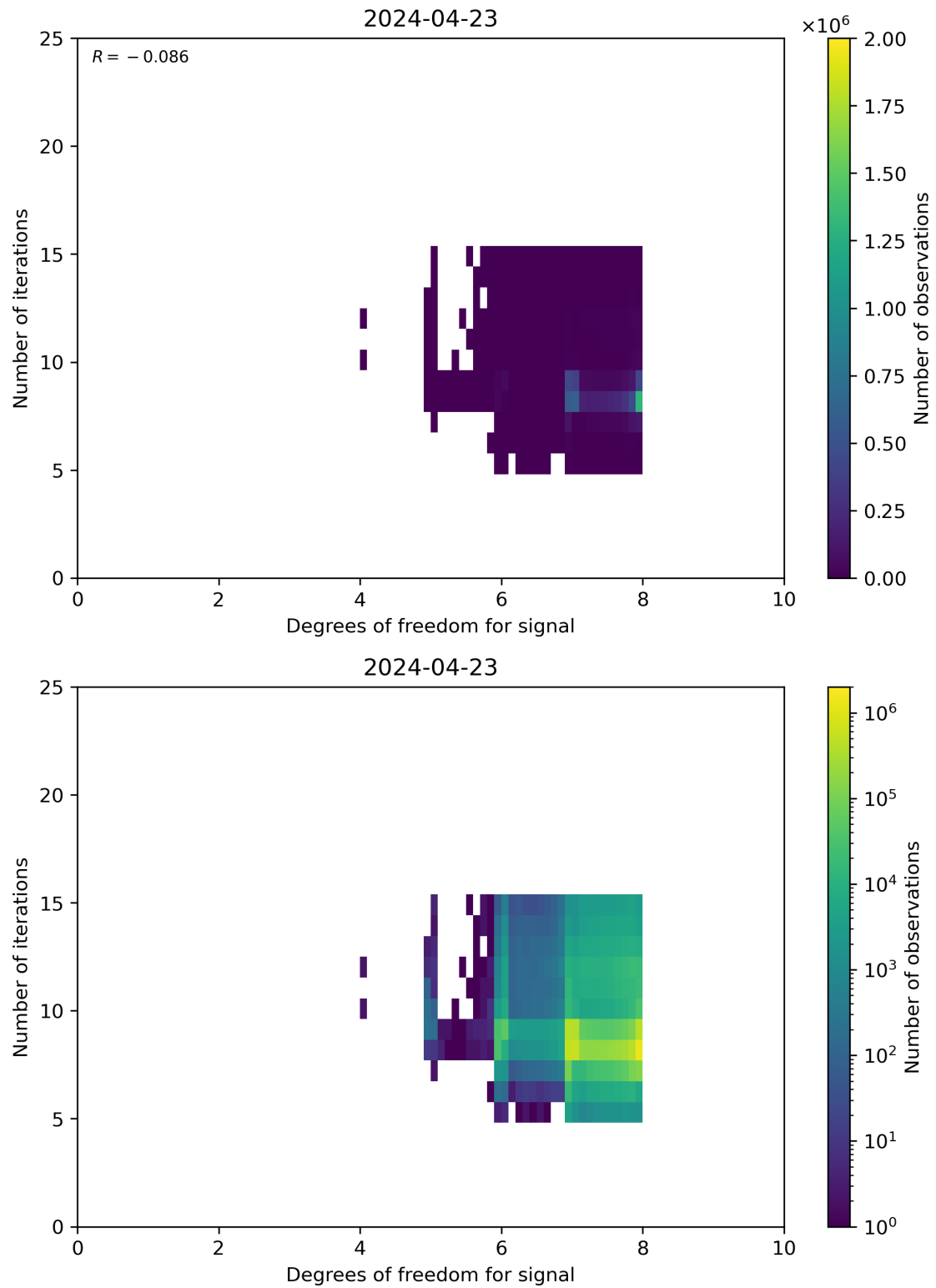
Figure 50: Scatter density plot of “Degrees of freedom for signal” against “Number of iterations” for 2024-04-22 to 2024-04-24.
