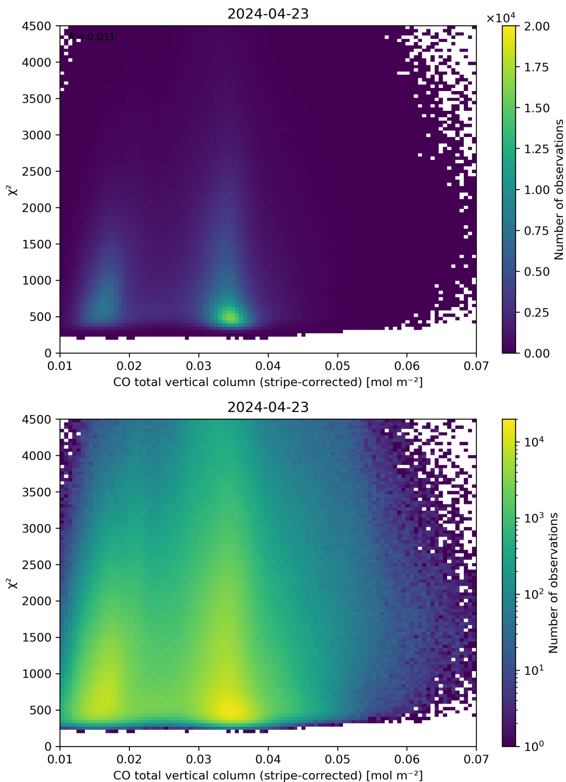
Figure 37: Scatter density plot of “CO total vertical column (stripe-corrected)” against “ \chi^2 ” for 2024-04-22 to 2024-04-24.
