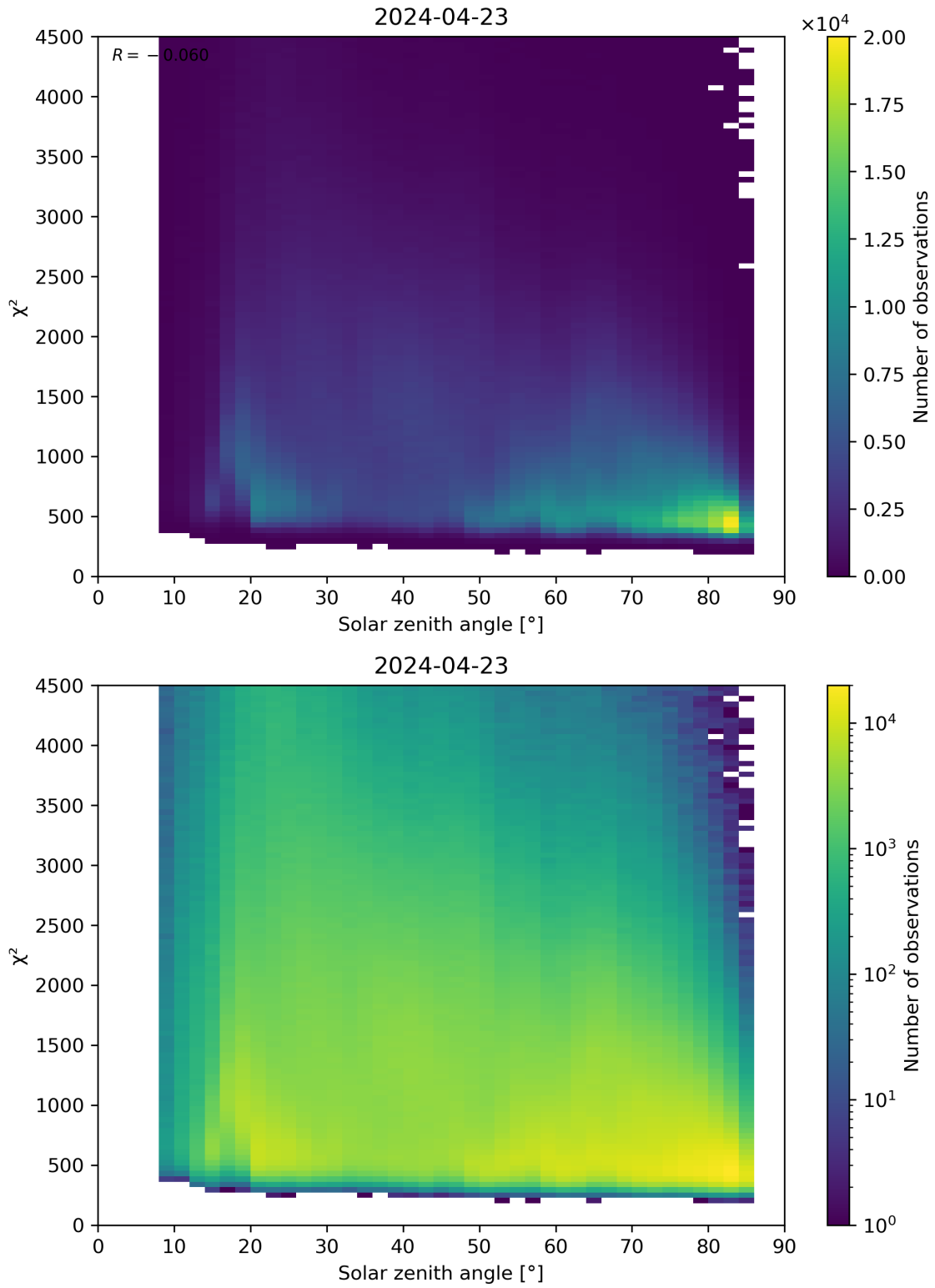
Figure 64: Scatter density plot of “Solar zenith angle” against “ \chi^2 ” for 2024-04-22 to 2024-04-24.
