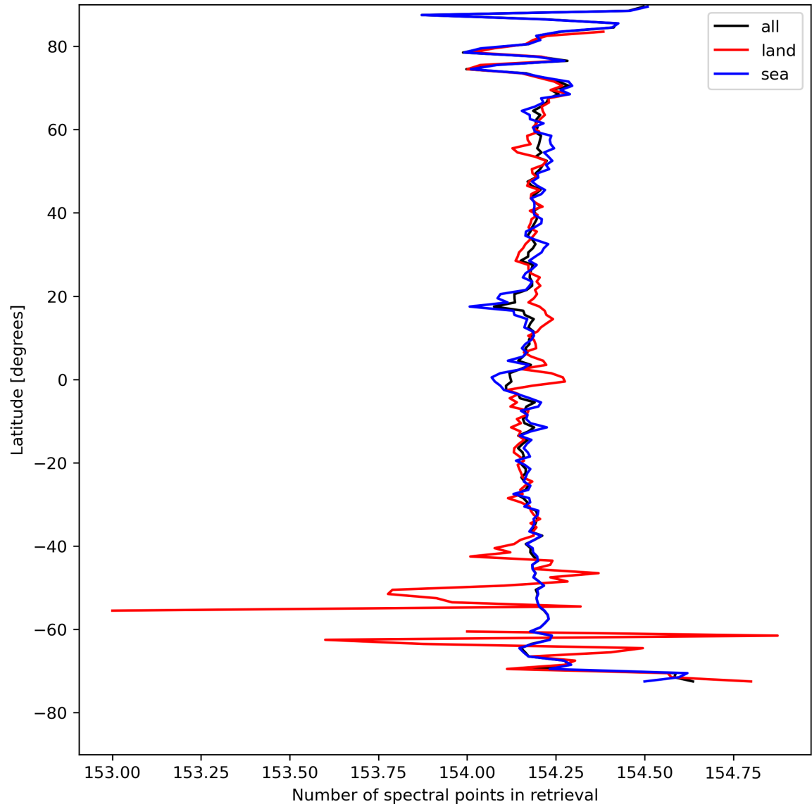
Figure 13: Zonal average of “Number of spectral points in retrieval” for 2024-04-22 to 2024-04-24.
