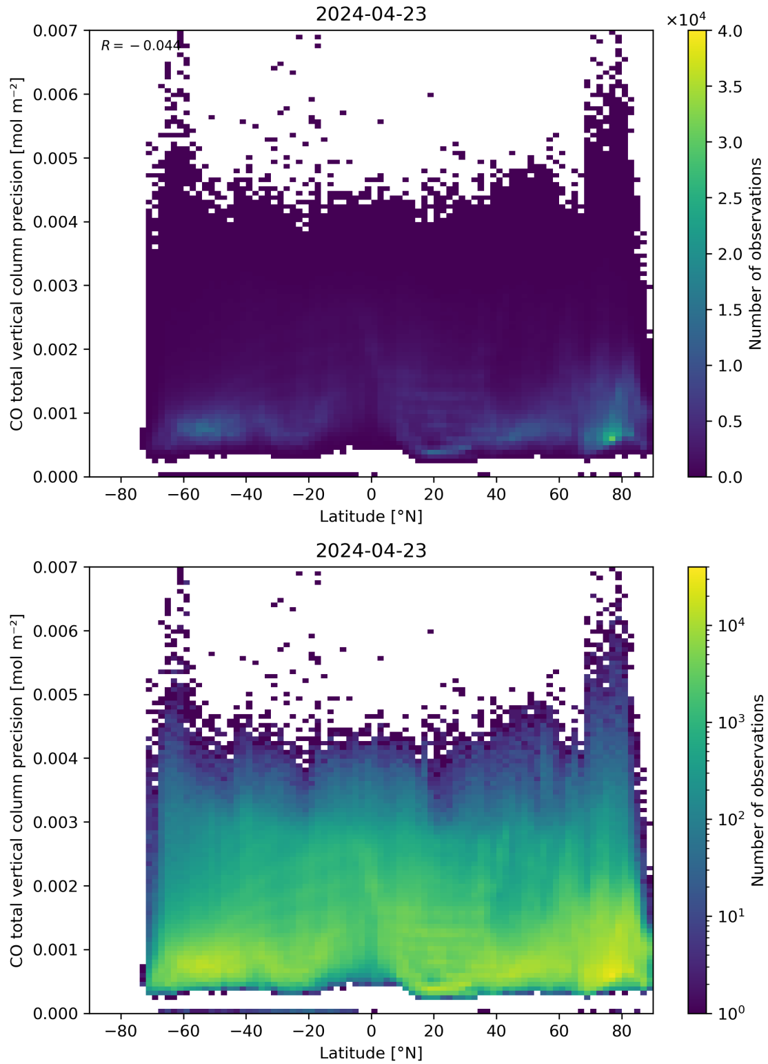
Figure 53: Scatter density plot of “Latitude” against “CO total vertical column precision” for 2024-04-22 to 2024-04-24.
