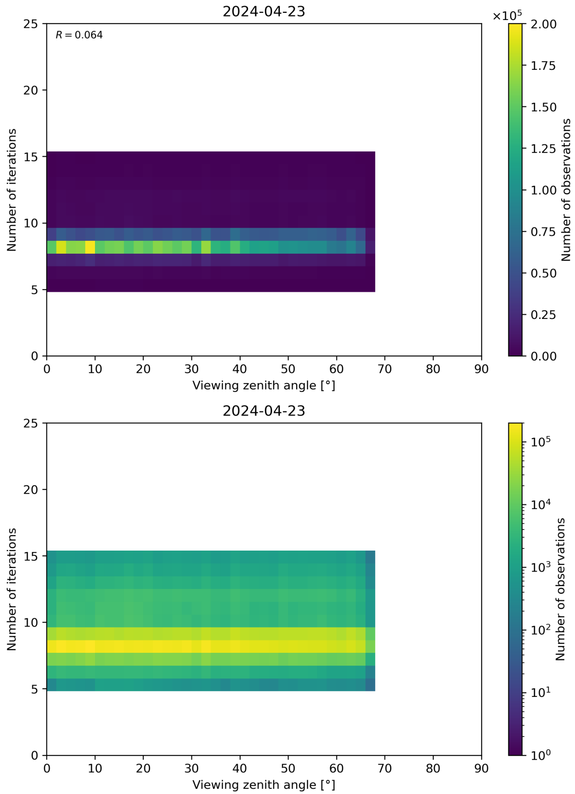
Figure 75: Scatter density plot of “Viewing zenith angle” against “Number of iterations” for 2024-04-22 to 2024-04-24.
