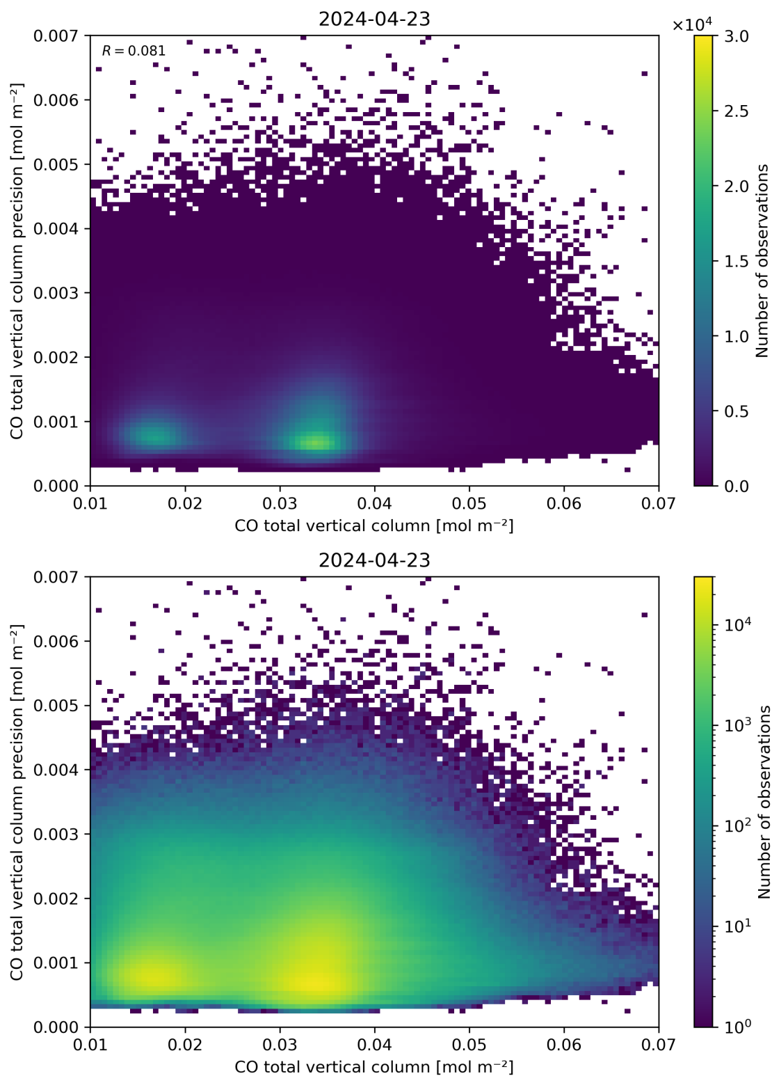
Figure 34: Scatter density plot of “CO total vertical column” against “CO total vertical column precision” for 2024-04-22 to 2024-04-24.
