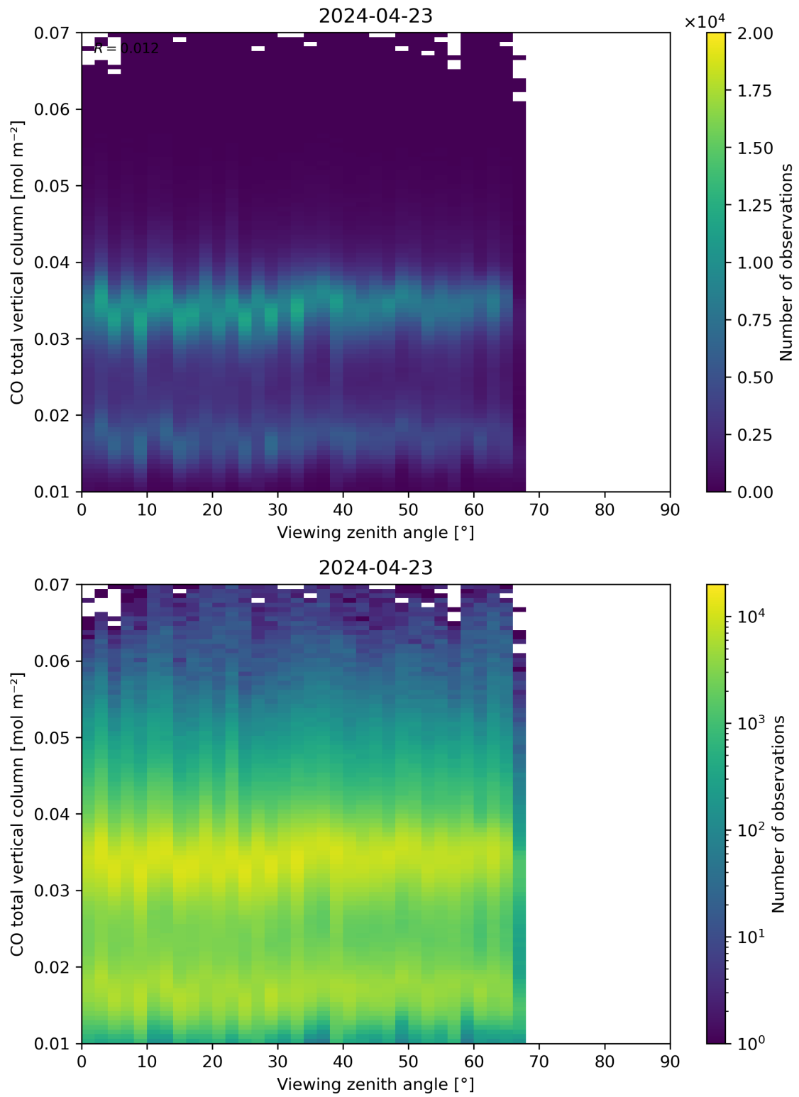
Figure 69: Scatter density plot of “Viewing zenith angle” against “CO total vertical column” for 2024-04-22 to 2024-04-24.
