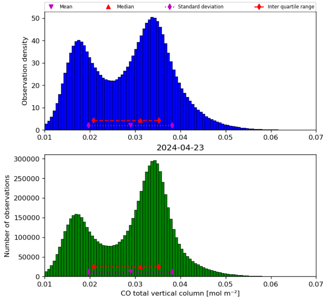
Figure 18: Histogram of “CO total vertical column” for 2024-04-22 to 2024-04-24
