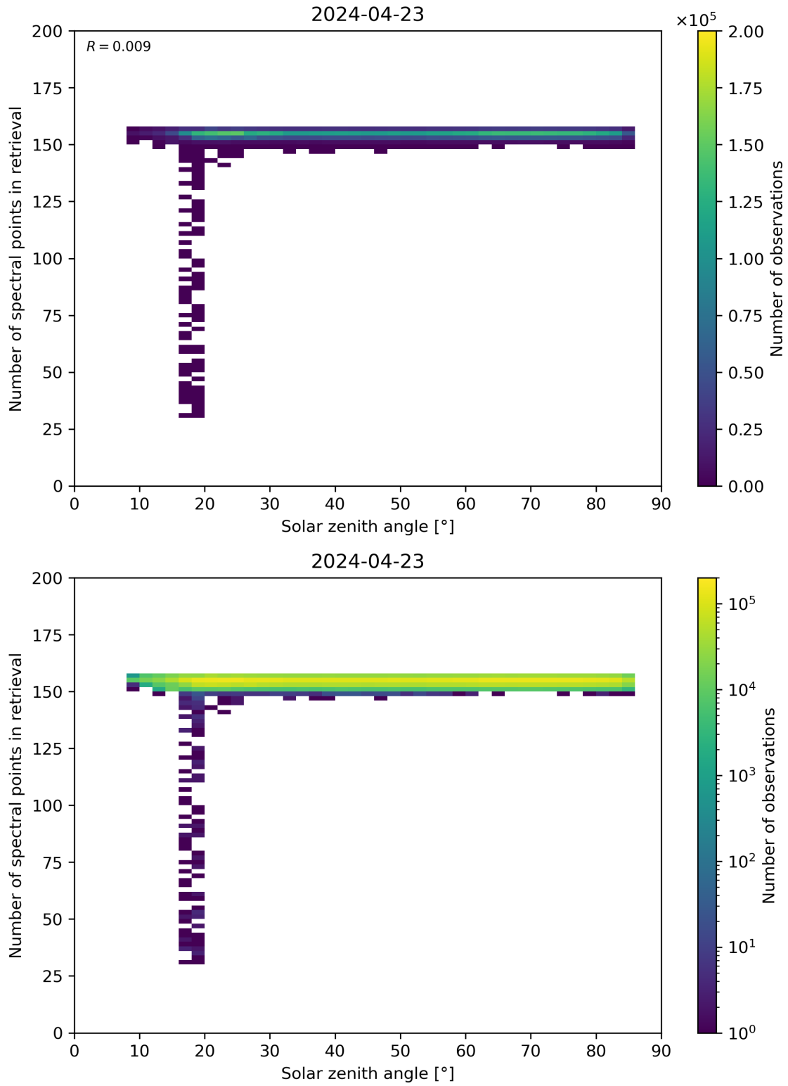
Figure 68: Scatter density plot of “Solar zenith angle” against “Number of spectral points in retrieval” for 2024-04-22 to 2024-04-24.
