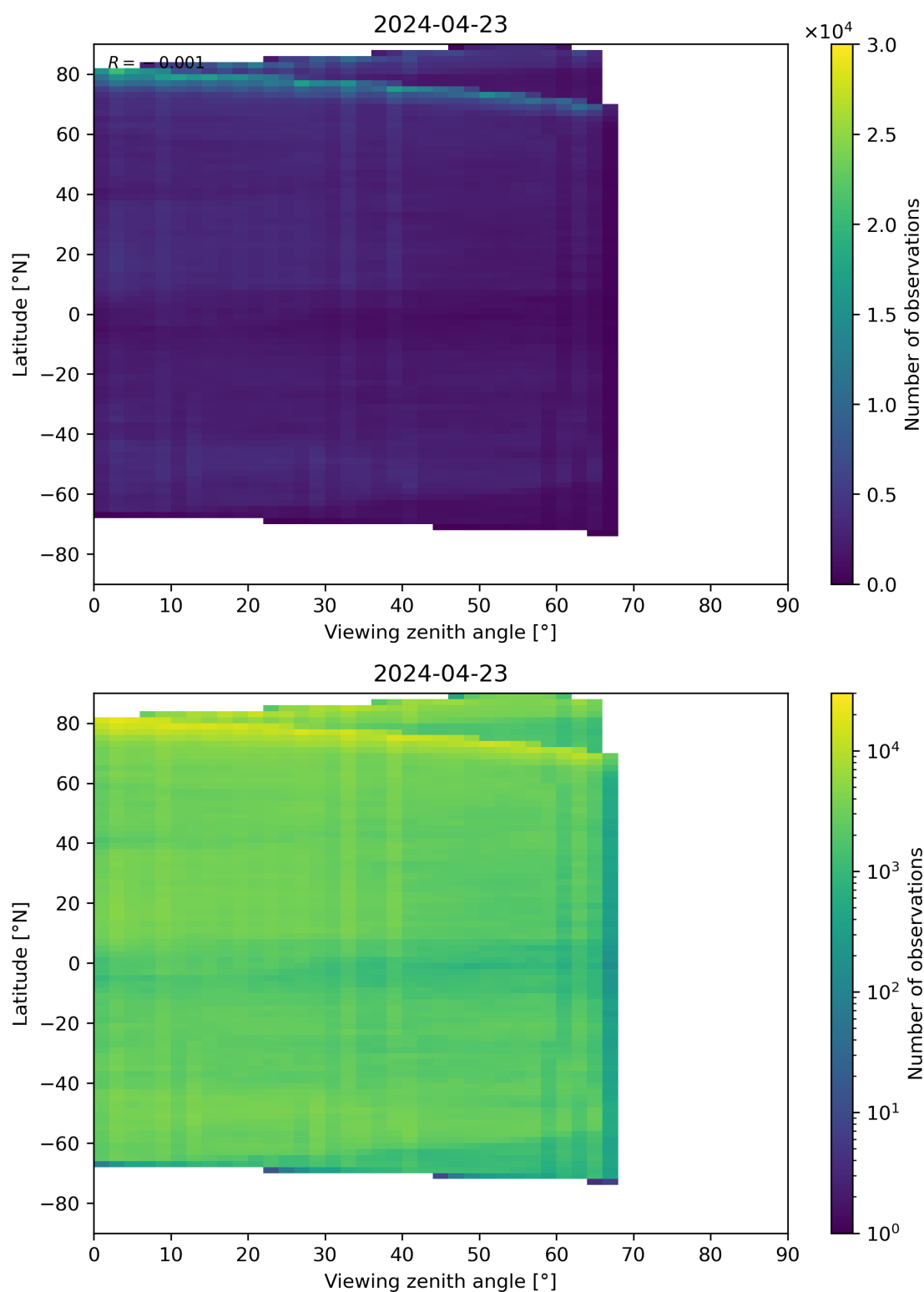
Figure 74: Scatter density plot of “Viewing zenith angle” against “Latitude” for 2024-04-22 to 2024-04-24.
