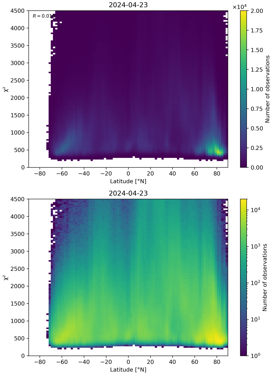
Figure 54: Scatter density plot of “Latitude” against “ \chi^2 ” for 2024-04-22 to 2024-04-24.
