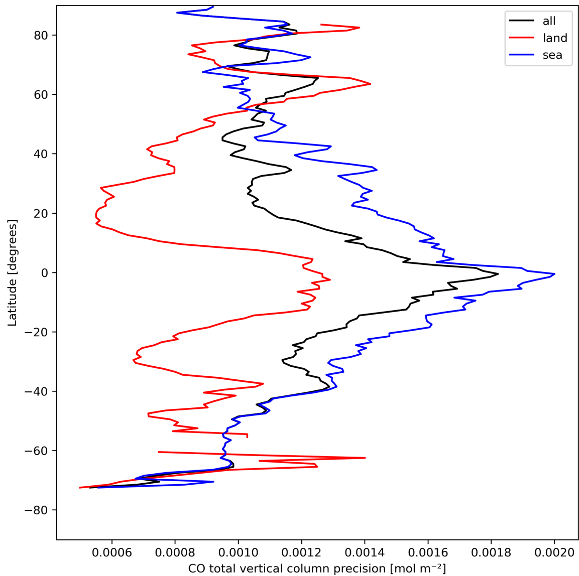
Figure 12: Zonal average of “CO total vertical column precision” for 2024-04-22 to 2024-04-24.
