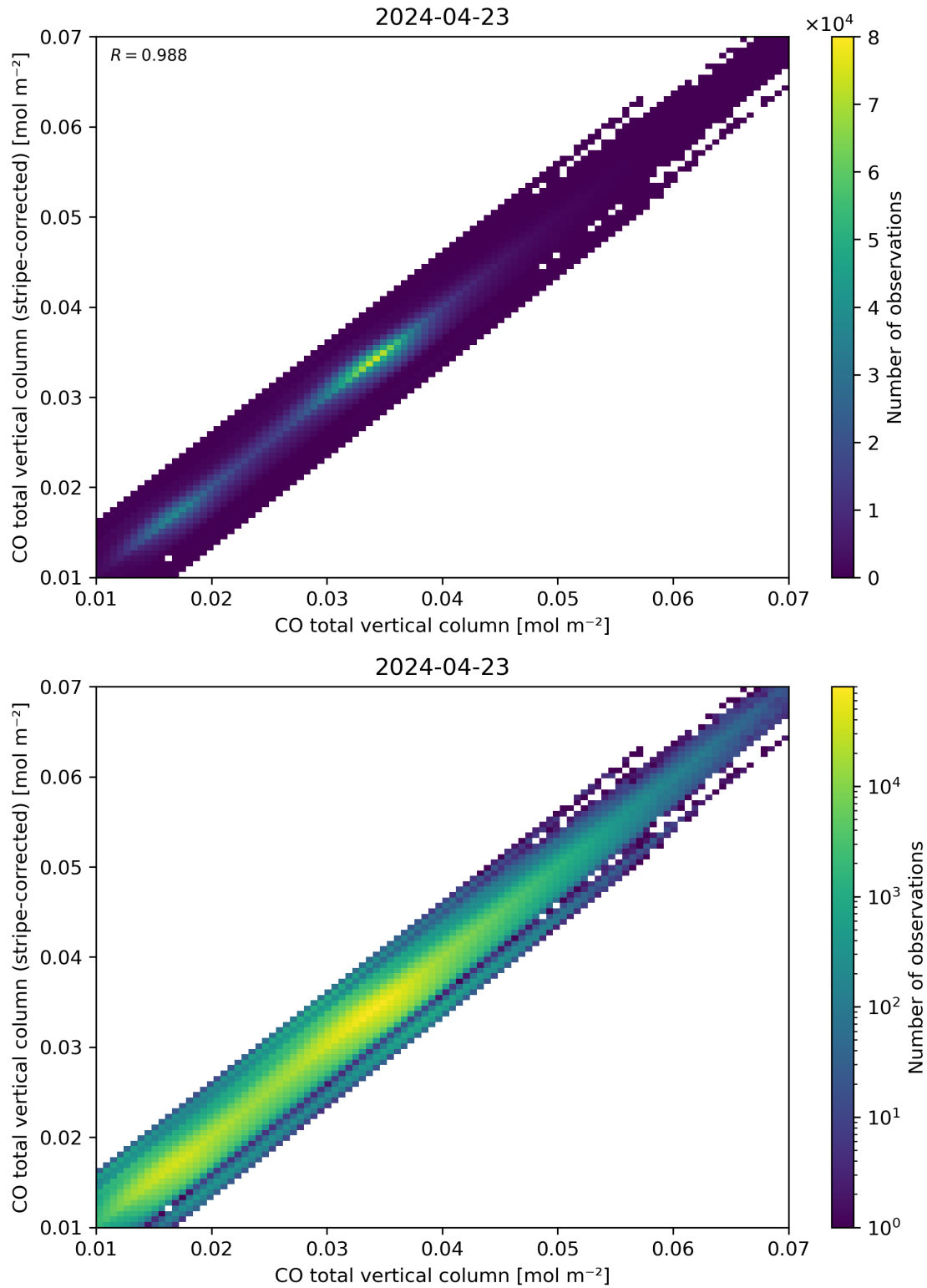
Figure 33: Scatter density plot of “CO total vertical column” against “CO total vertical column (stripe-corrected)” for 2024-04-22 to 2024-04-24.
