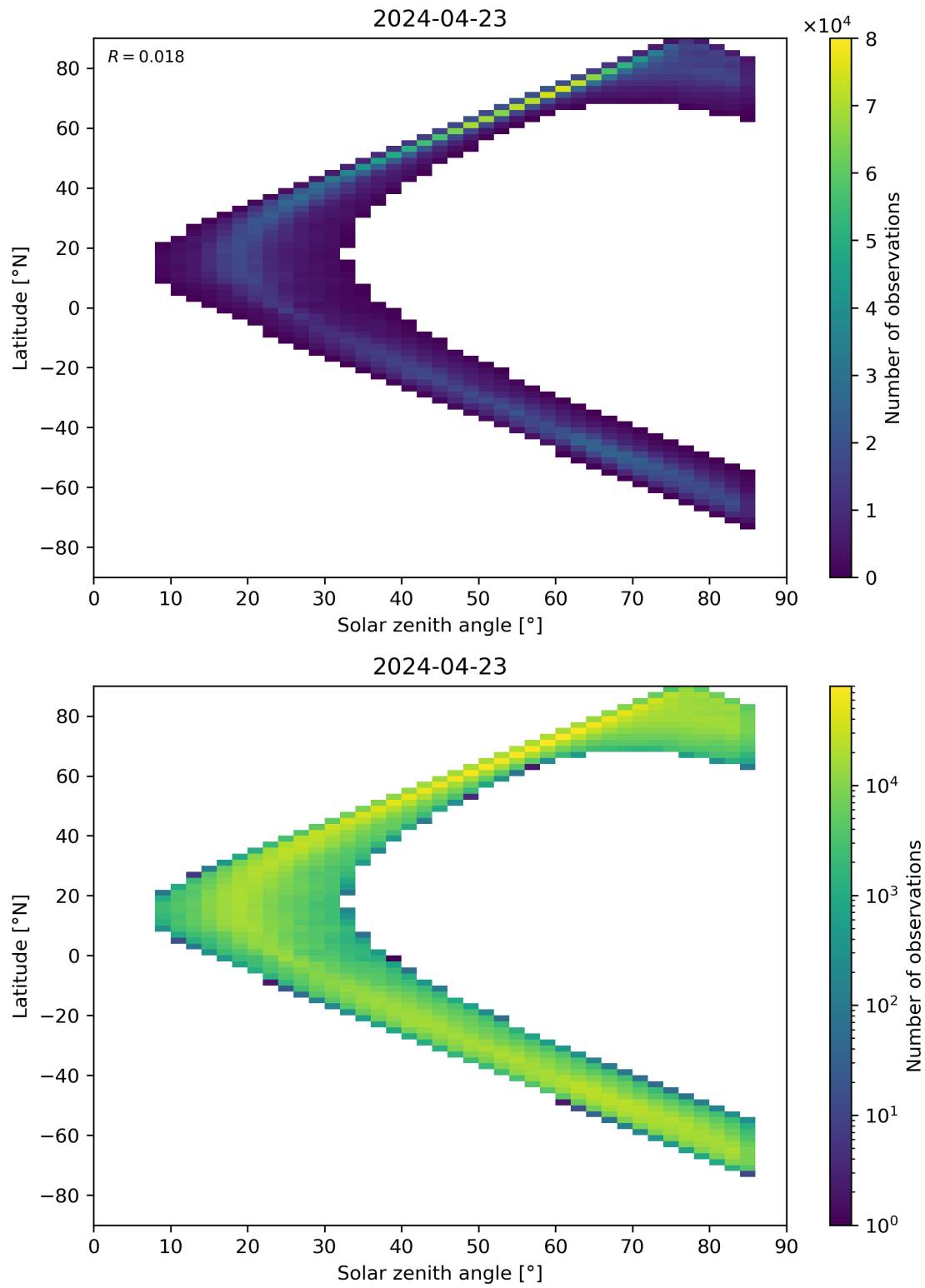
Figure 66: Scatter density plot of “Solar zenith angle” against “Latitude” for 2024-04-22 to 2024-04-24.
