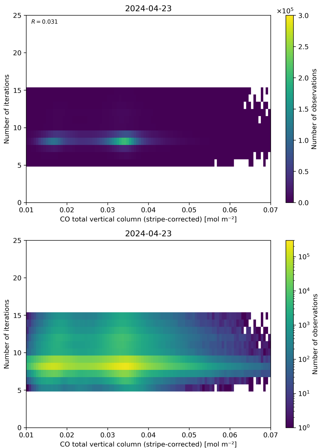
Figure 39: Scatter density plot of “CO total vertical column (stripe-corrected)” against “Number of iterations” for 2024-04-22 to 2024-04-24.
