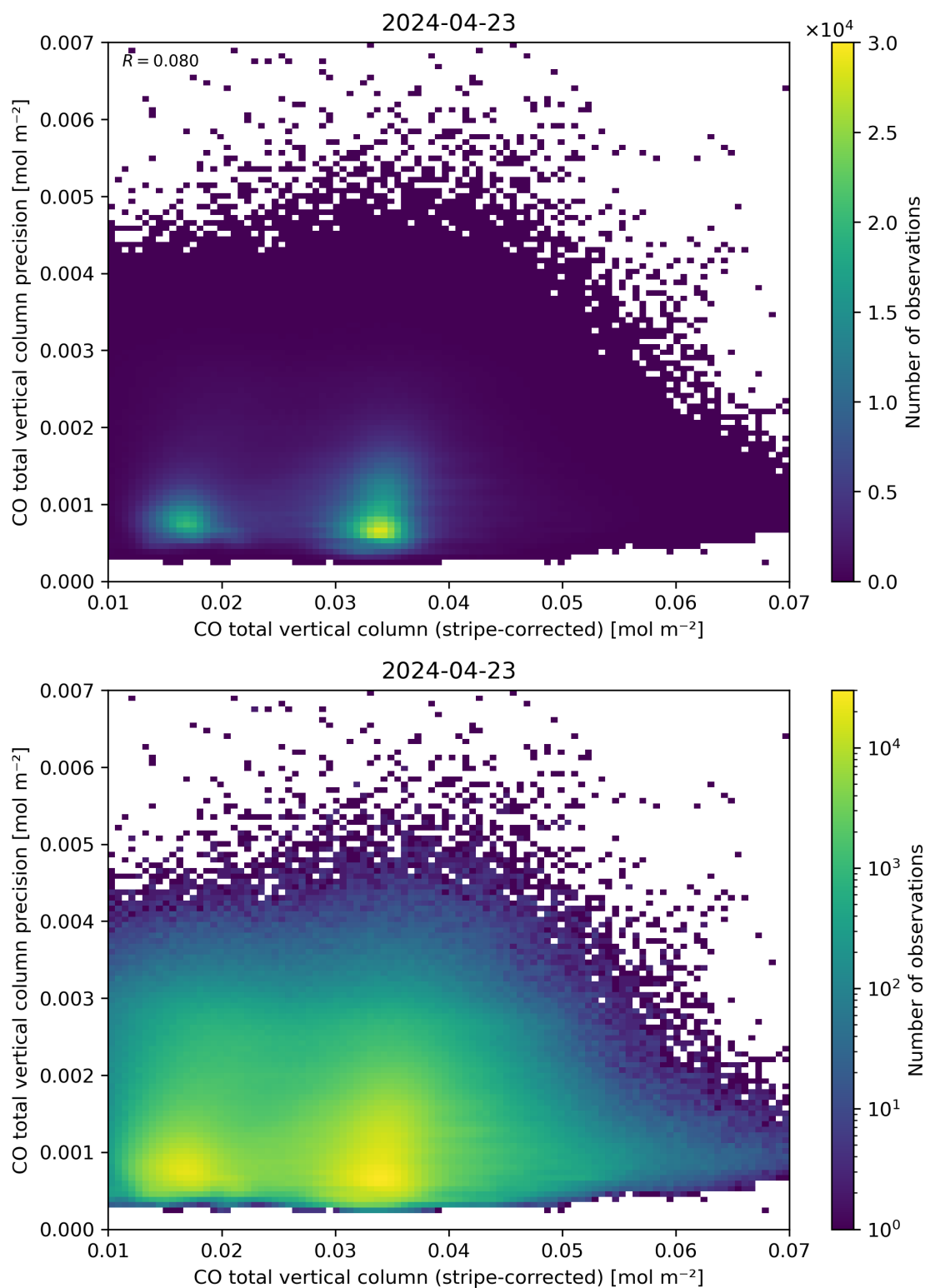
Figure 36: Scatter density plot of “CO total vertical column (stripe-corrected)” against “CO total vertical column precision” for 2024-04-22 to 2024-04-24.
