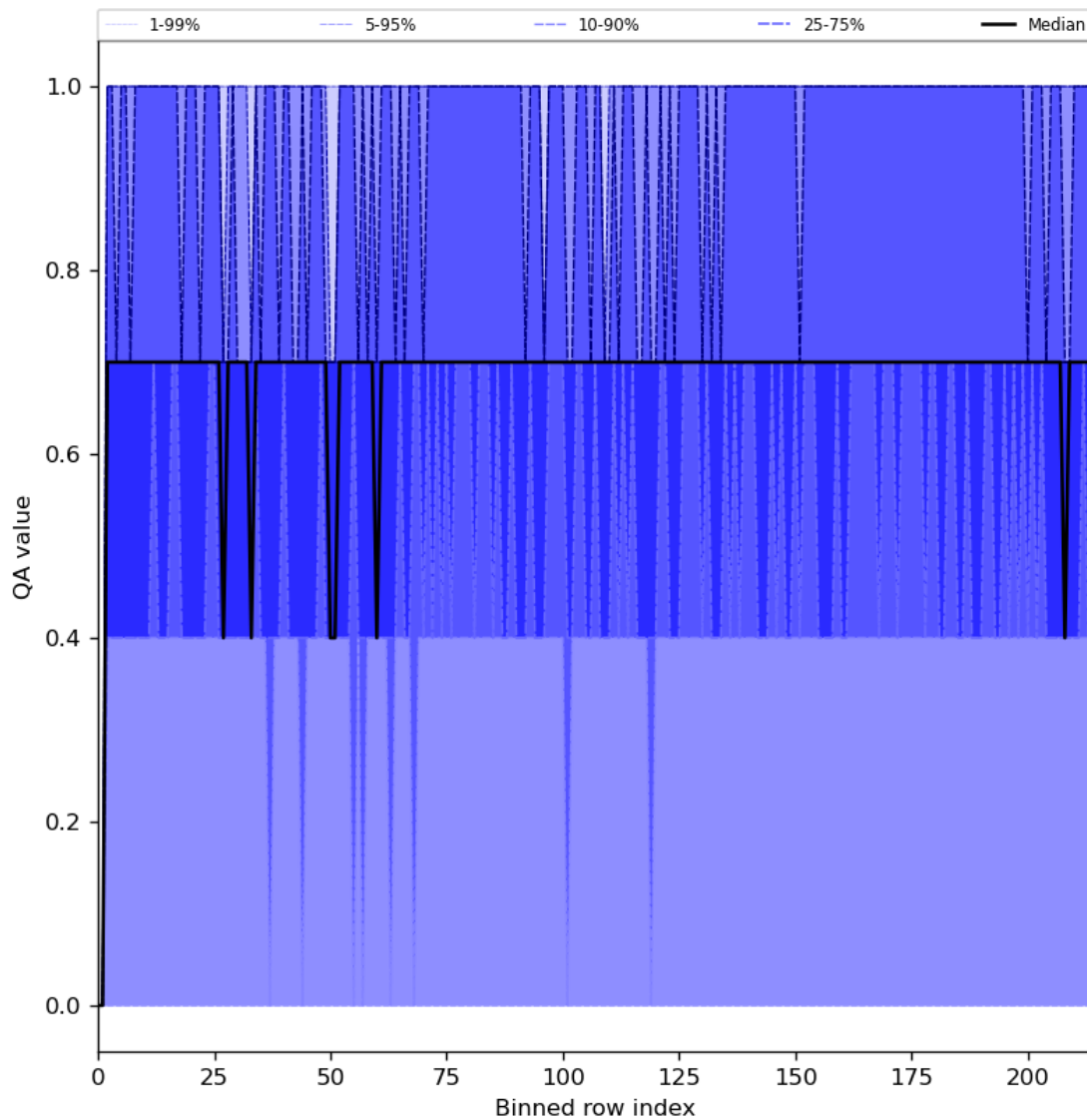
Figure 25: Along track statistics of “QA value” for 2024-04-22 to 2024-04-24
