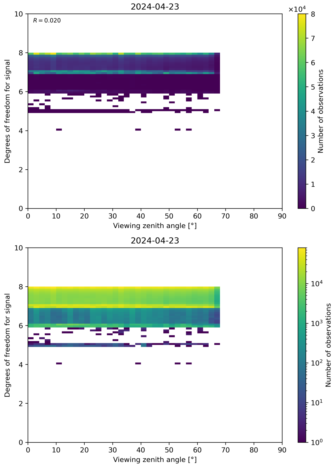
Figure 73: Scatter density plot of “Viewing zenith angle” against “Degrees of freedom for signal” for 2024-04-22 to 2024-04-24.
