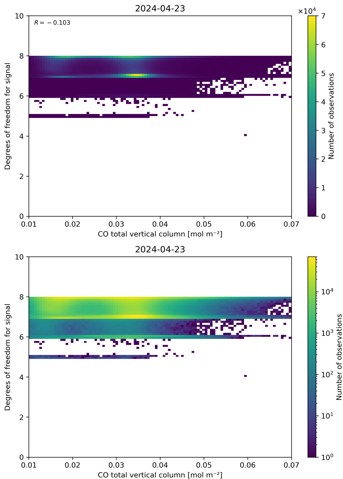
Figure 41: Scatter density plot of “CO total vertical column” against “Degrees of freedom for signal” for 2024-04-22 to 2024-04-24.
