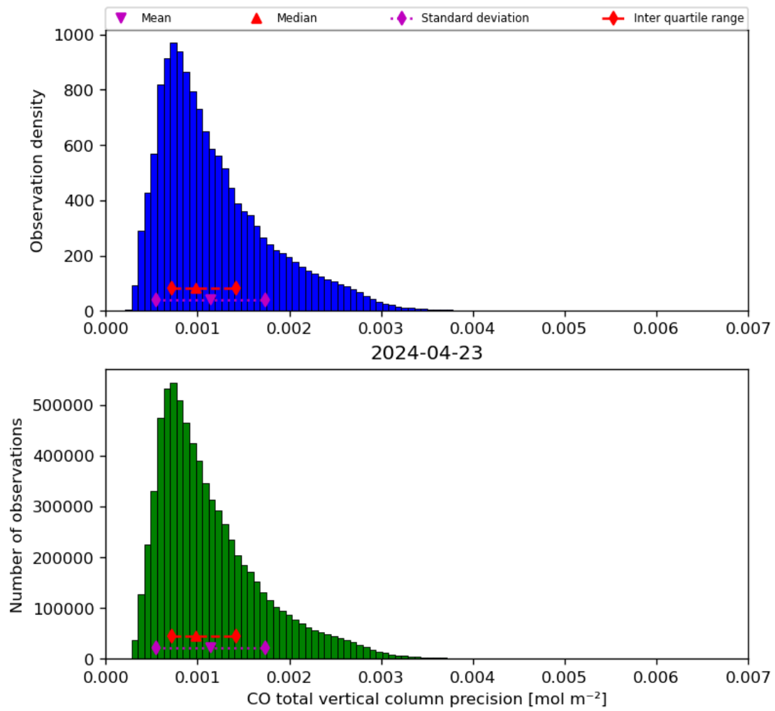
Figure 20: Histogram of “CO total vertical column precision” for 2024-04-22 to 2024-04-24
