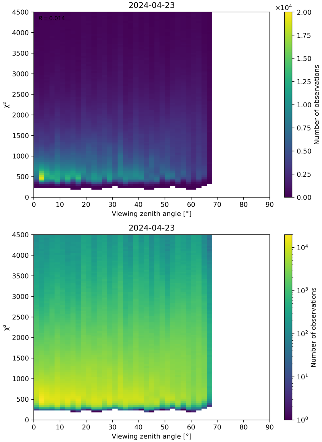
Figure 72: Scatter density plot of “Viewing zenith angle” against “ \chi^2 ” for 2024-04-22 to 2024-04-24.
