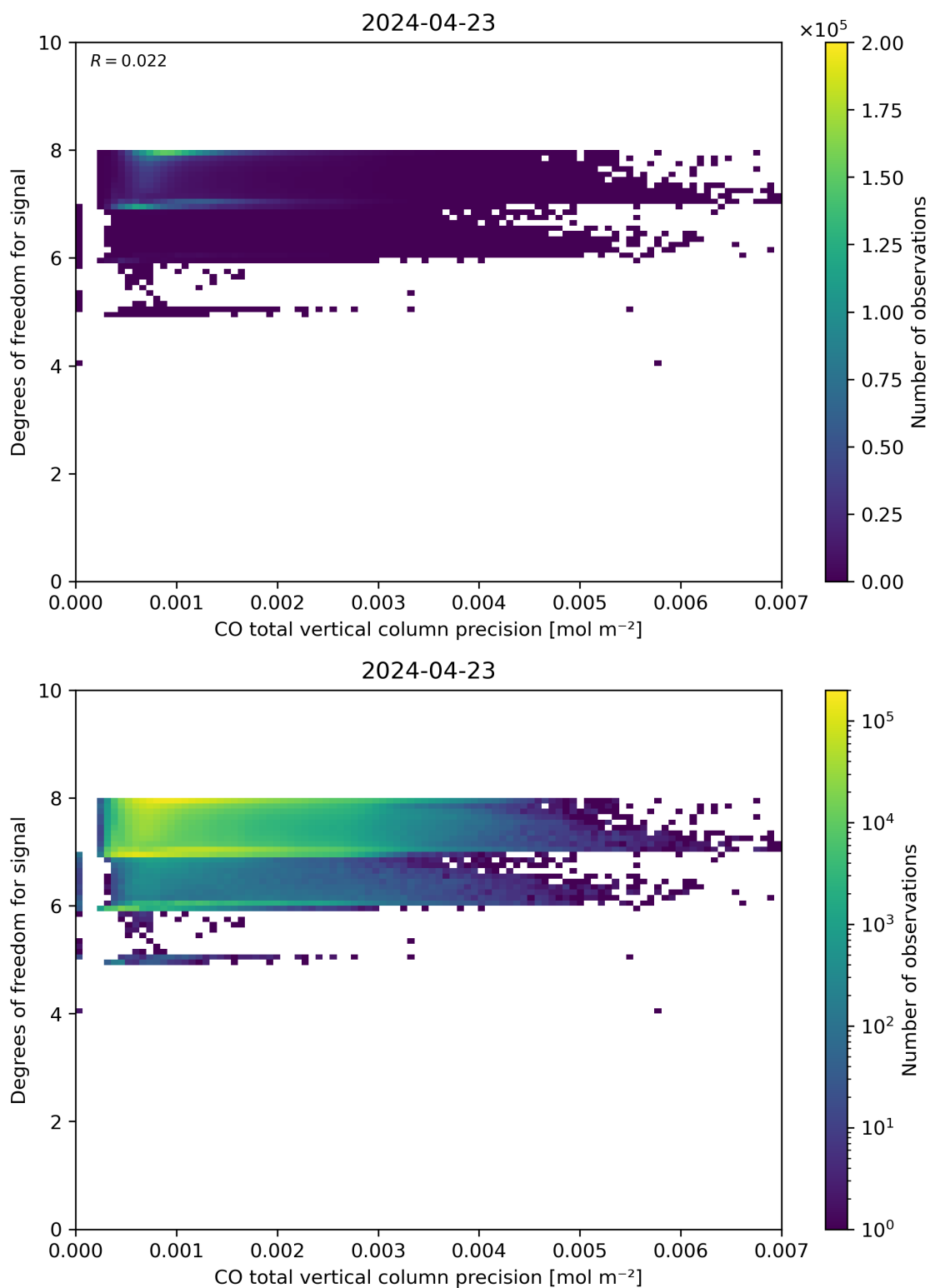
Figure 45: Scatter density plot of “CO total vertical column precision” against “Degrees of freedom for signal” for 2024-04-22 to 2024-04-24.
