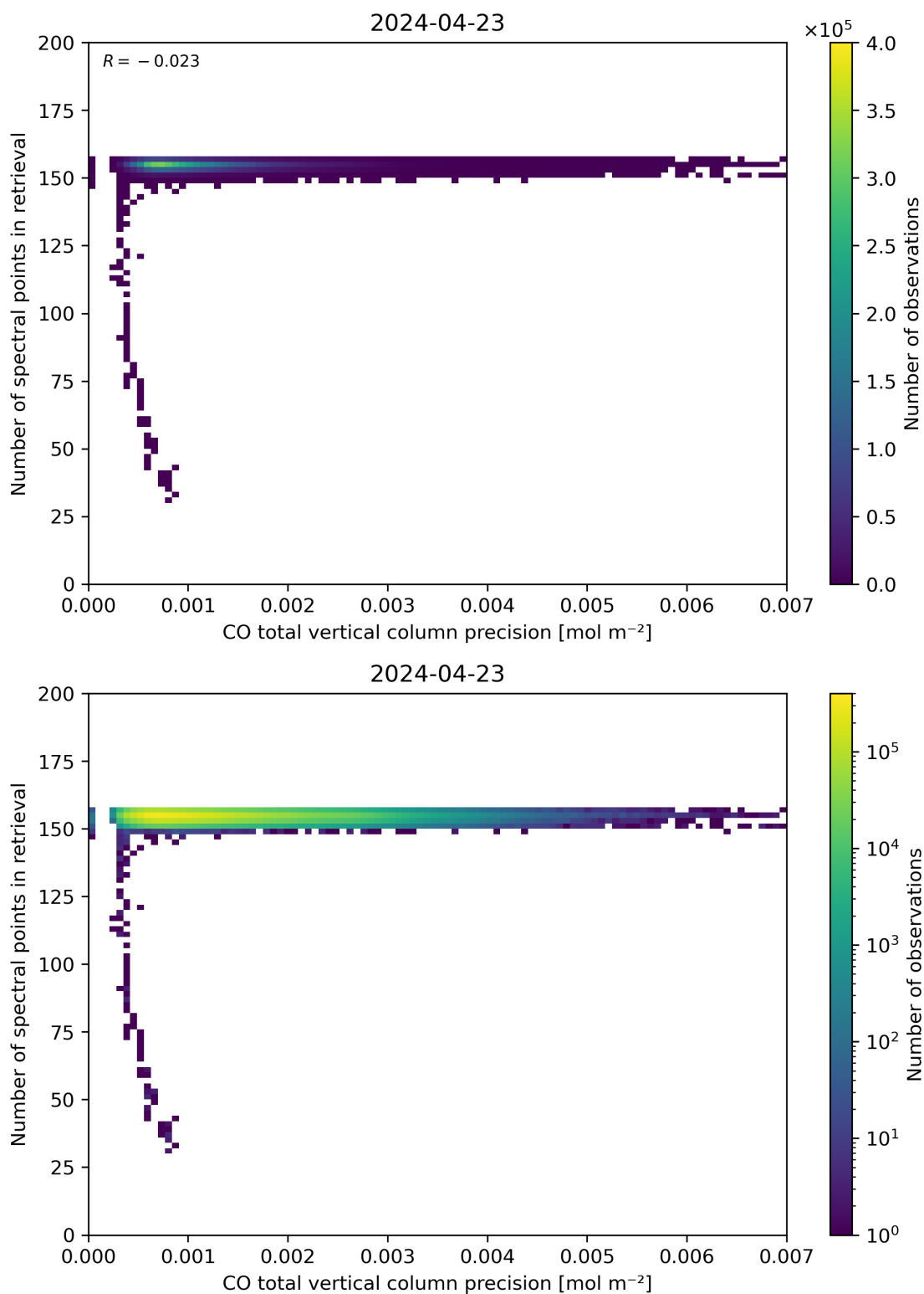
Figure 47: Scatter density plot of “CO total vertical column precision” against “Number of spectral points in retrieval” for 2024-04-22 to 2024-04-24.
