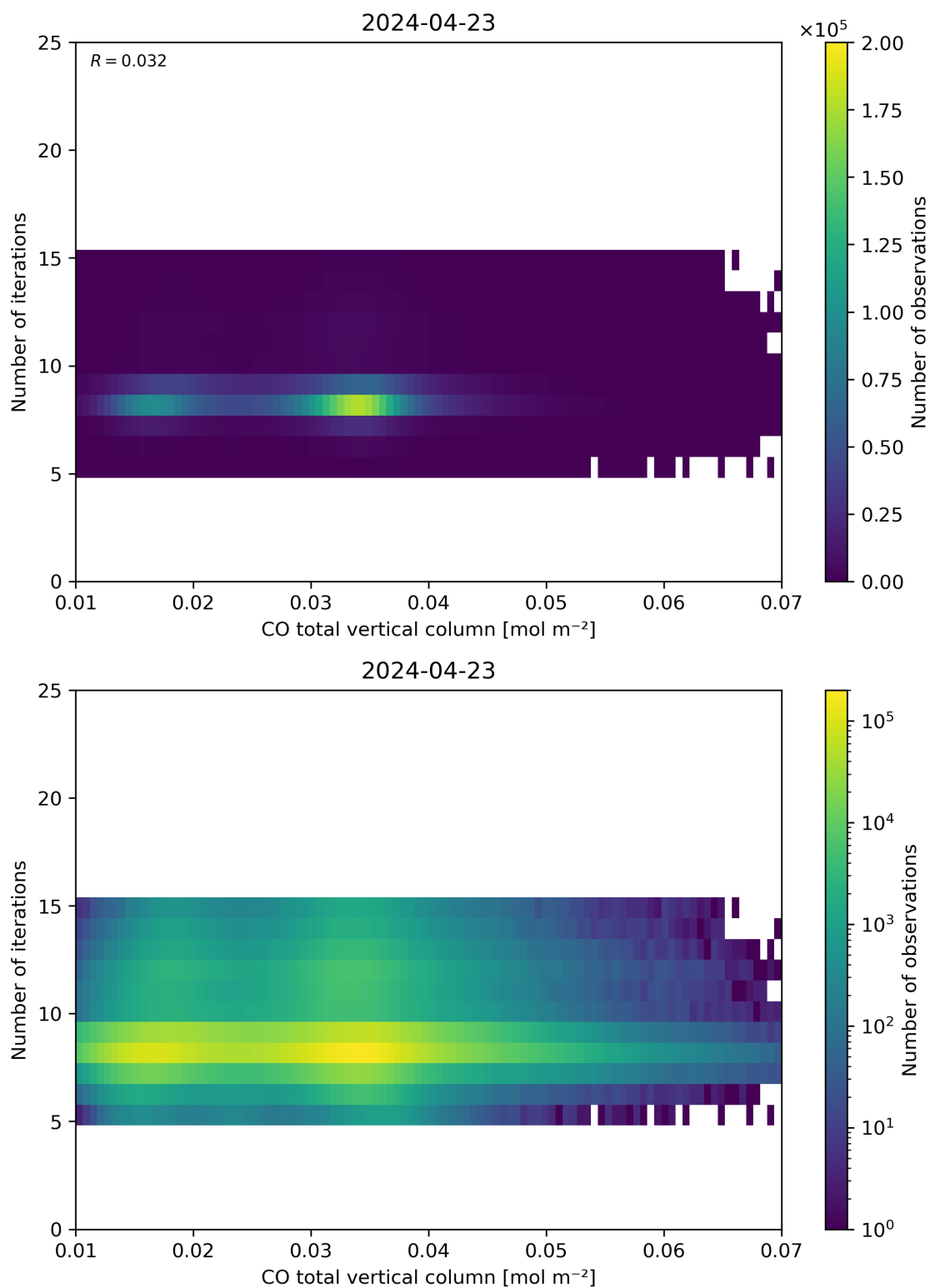
Figure 42: Scatter density plot of “CO total vertical column” against “Number of iterations” for 2024-04-22 to 2024-04-24.
