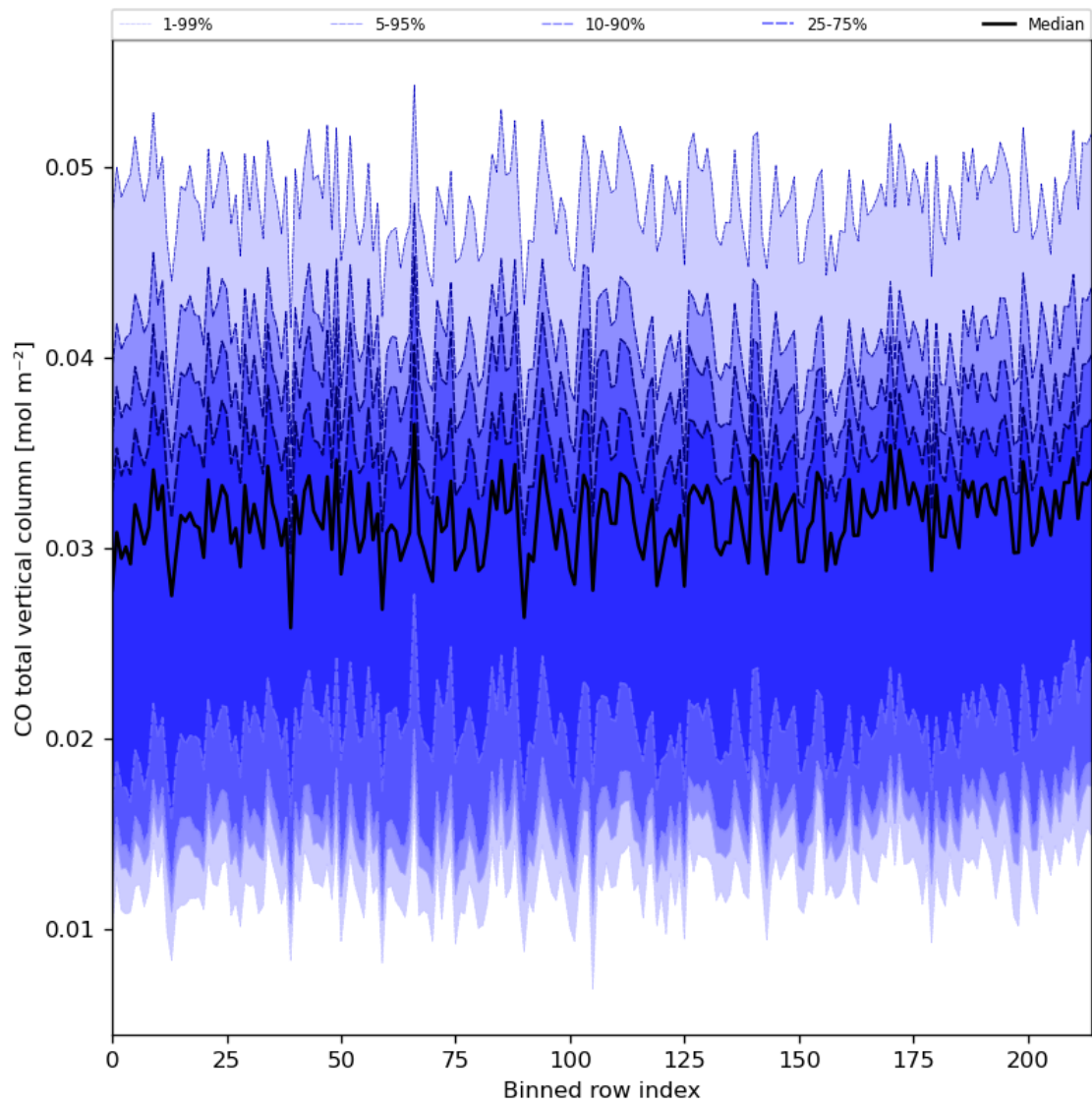
Figure 26: Along track statistics of “CO total vertical column” for 2024-04-22 to 2024-04-24
