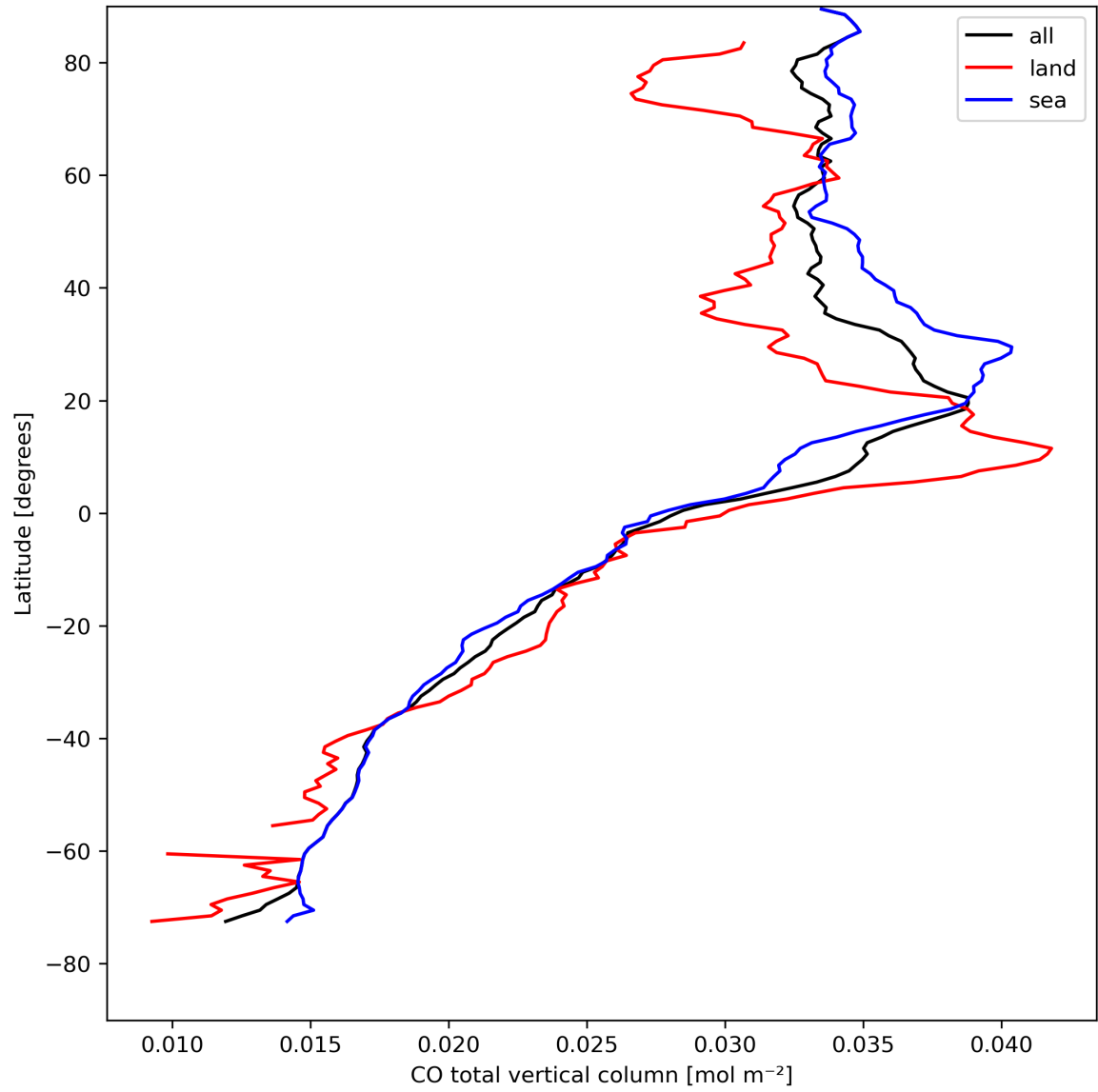
Figure 10: Zonal average of “CO total vertical column” for 2024-04-22 to 2024-04-24.
