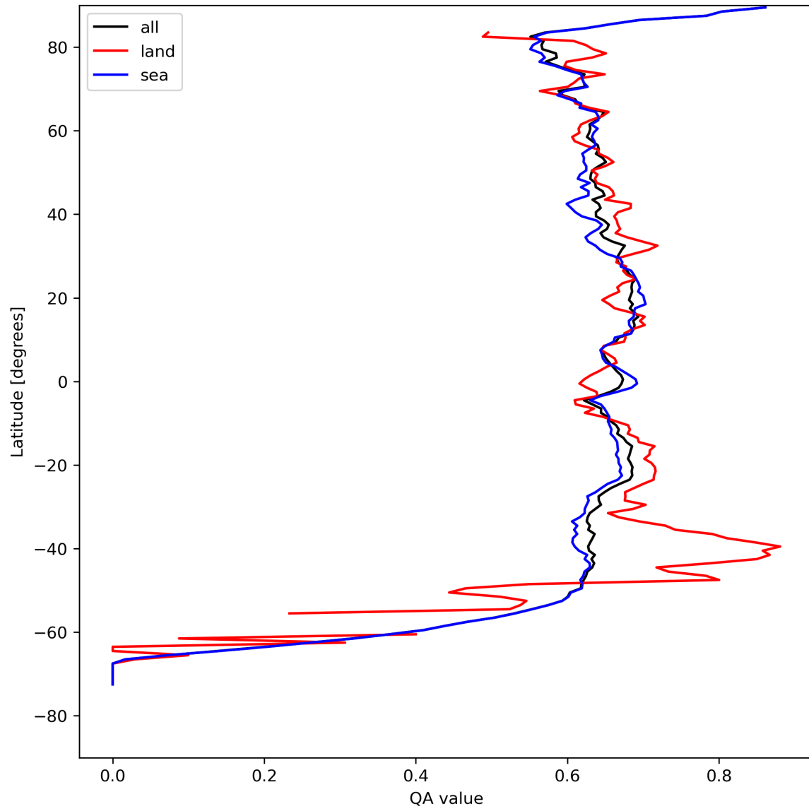
Figure 9: Zonal average of “QA value” for 2024-04-22 to 2024-04-24.
