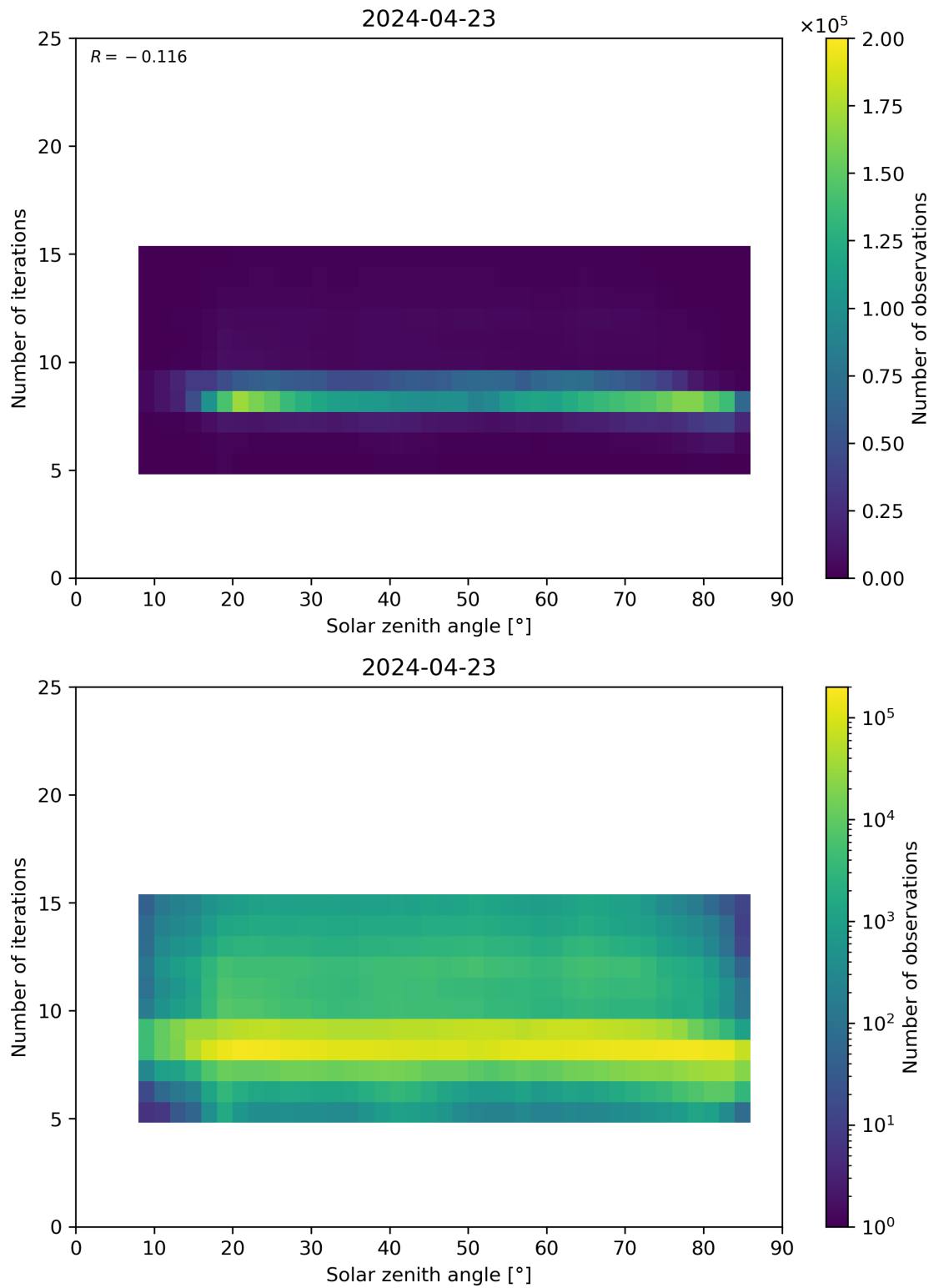
Figure 67: Scatter density plot of “Solar zenith angle” against “Number of iterations” for 2024-04-22 to 2024-04-24.
