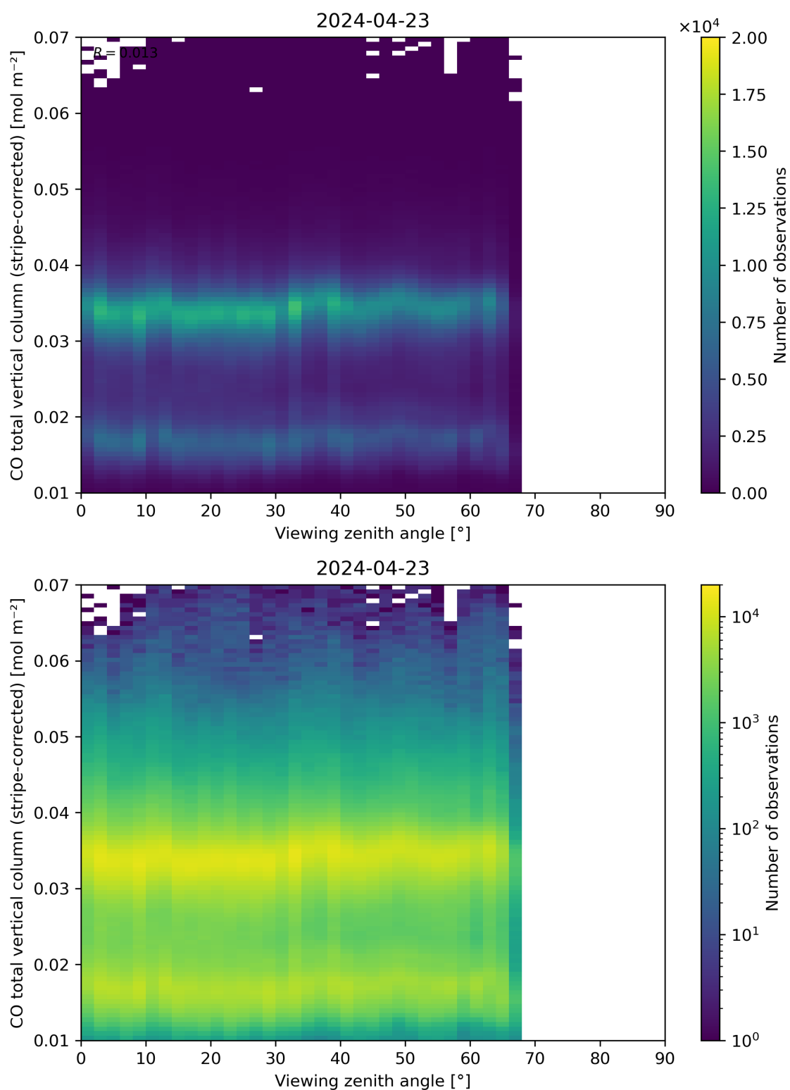
Figure 70: Scatter density plot of “Viewing zenith angle” against “CO total vertical column (stripe-corrected)” for 2024-04-22 to 2024-04-24.
