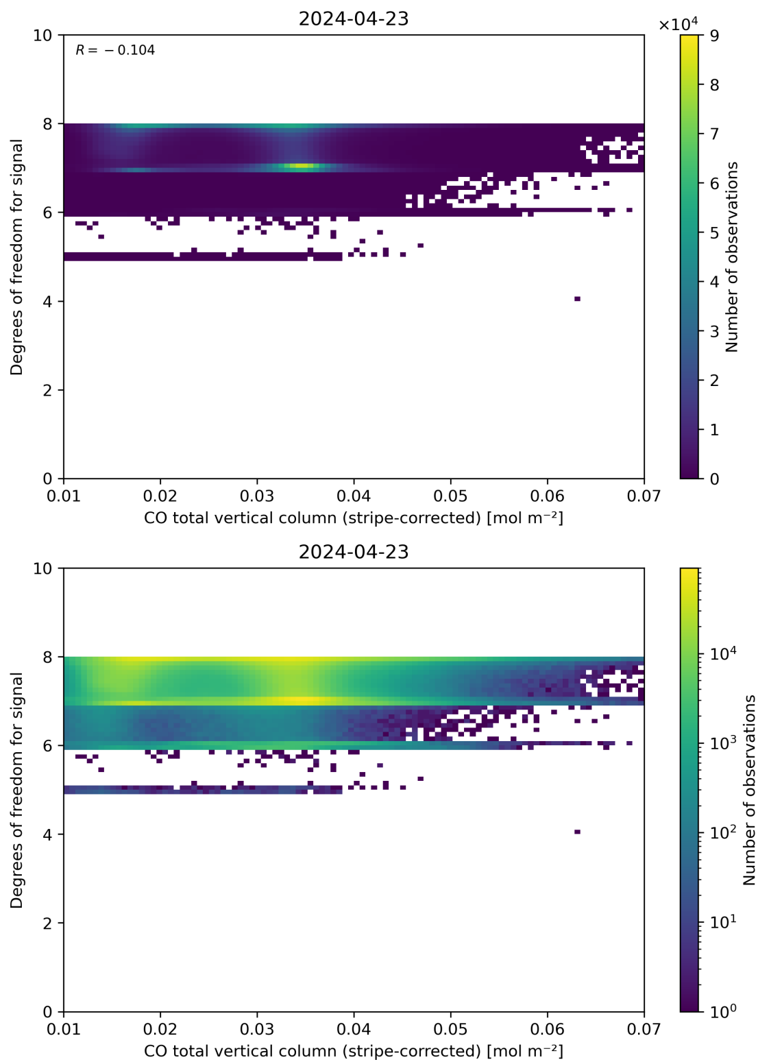
Figure 38: Scatter density plot of “CO total vertical column (stripe-corrected)” against “Degrees of freedom for signal” for 2024-04-22 to 2024-04-24.
