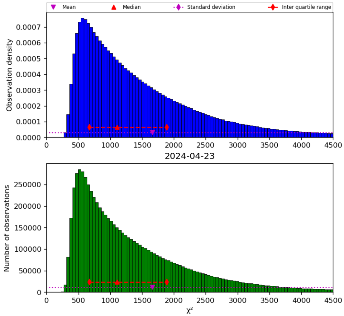
Figure 22: Histogram of “ \chi^2 ” for 2024-04-22 to 2024-04-24
