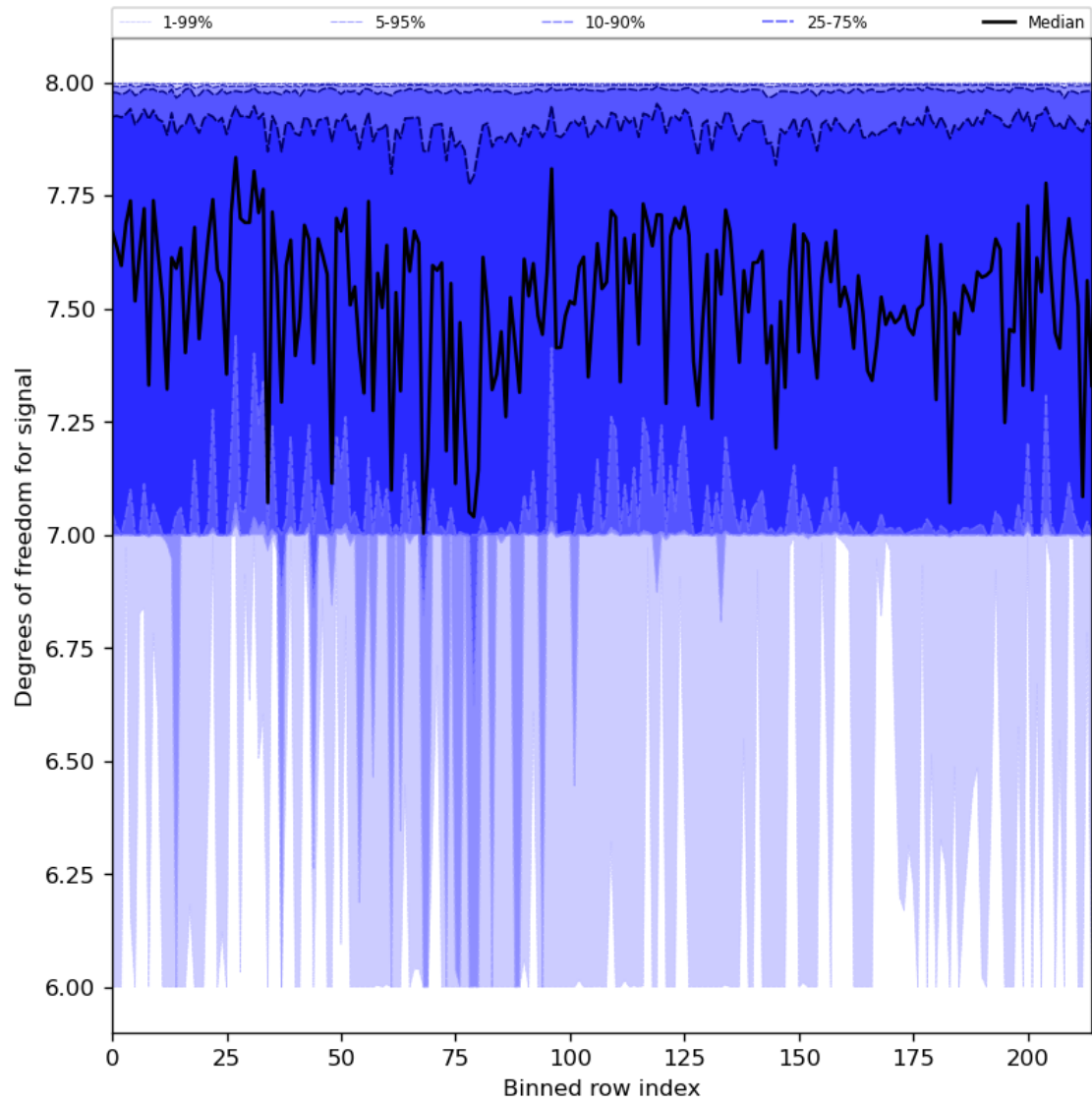
Figure 31: Along track statistics of “Degrees of freedom for signal” for 2024-04-22 to 2024-04-24
