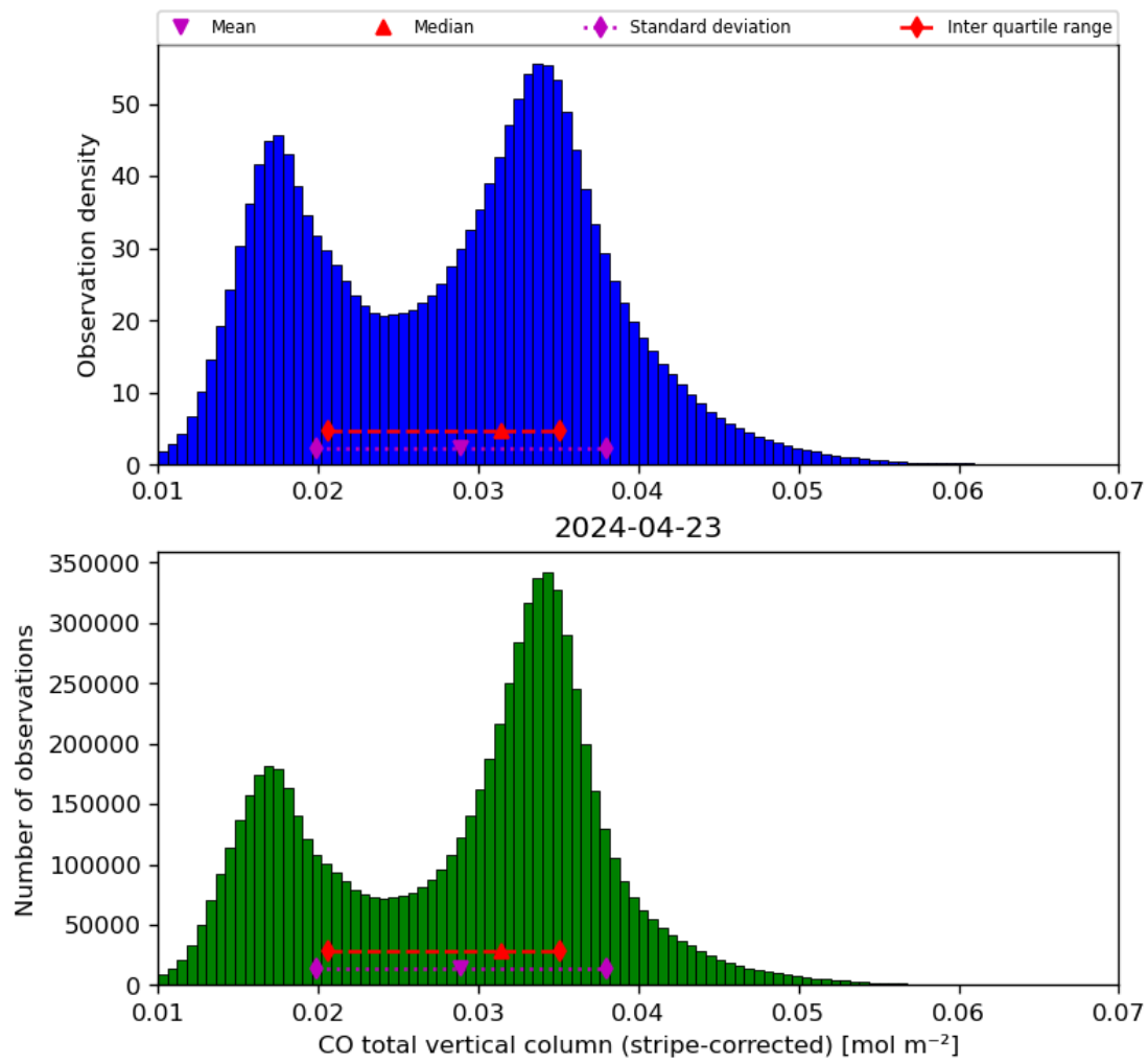
Figure 19: Histogram of “CO total vertical column (stripe-corrected)” for 2024-04-22 to 2024-04-24
