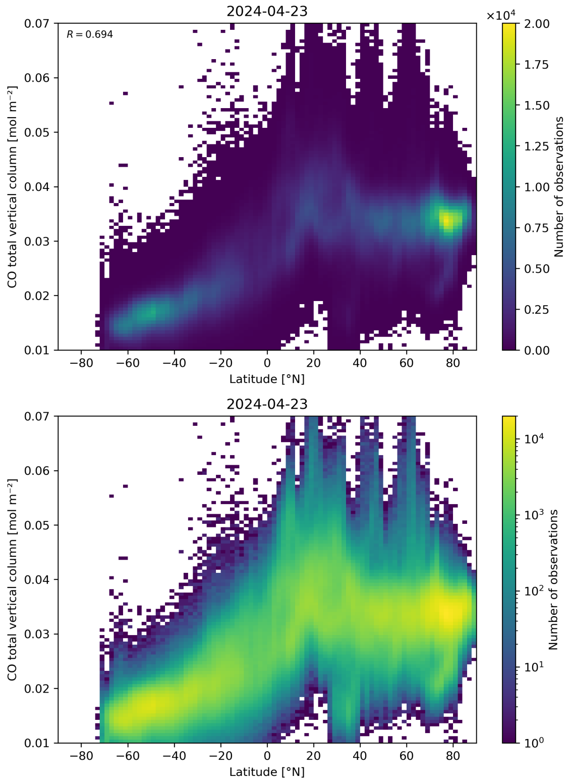
Figure 51: Scatter density plot of “Latitude” against “CO total vertical column” for 2024-04-22 to 2024-04-24.
