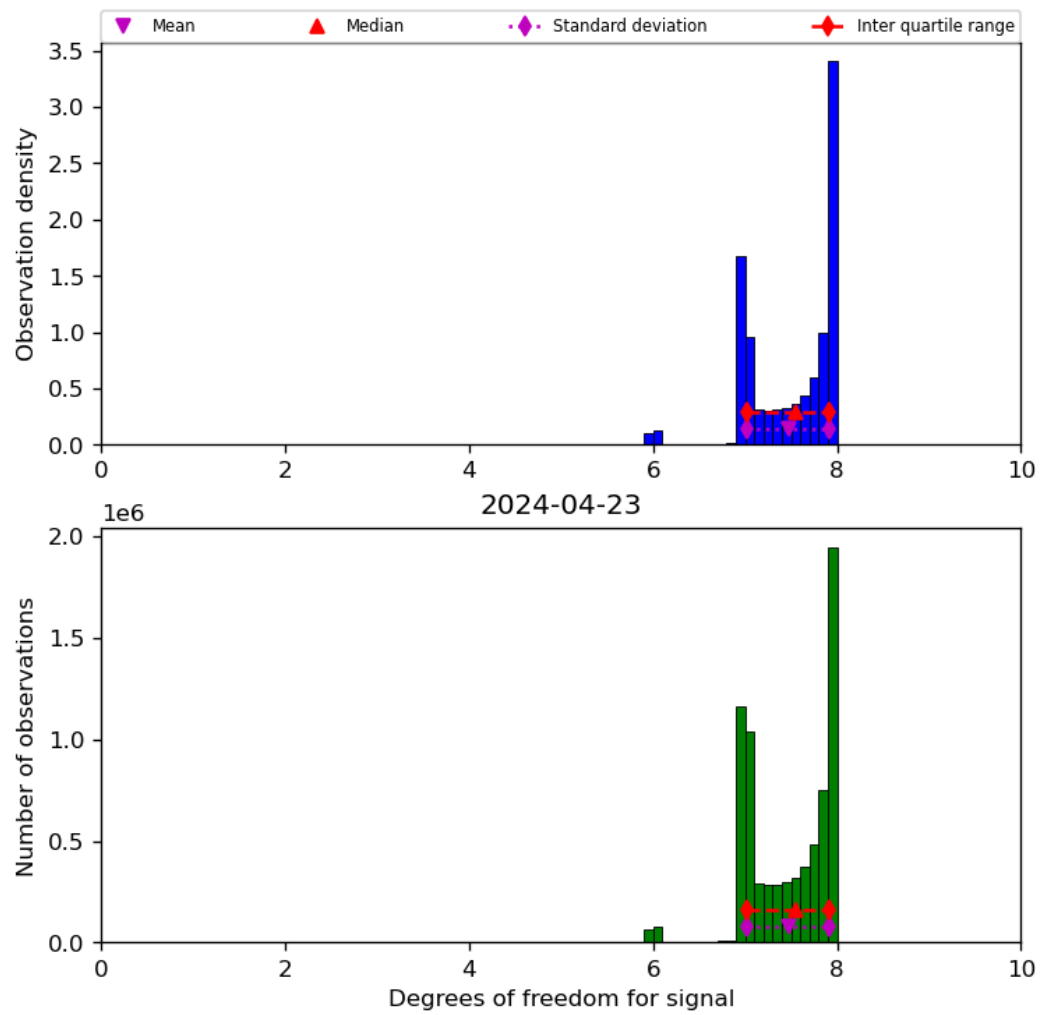
Figure 23: Histogram of “Degrees of freedom for signal” for 2024-04-22 to 2024-04-24
