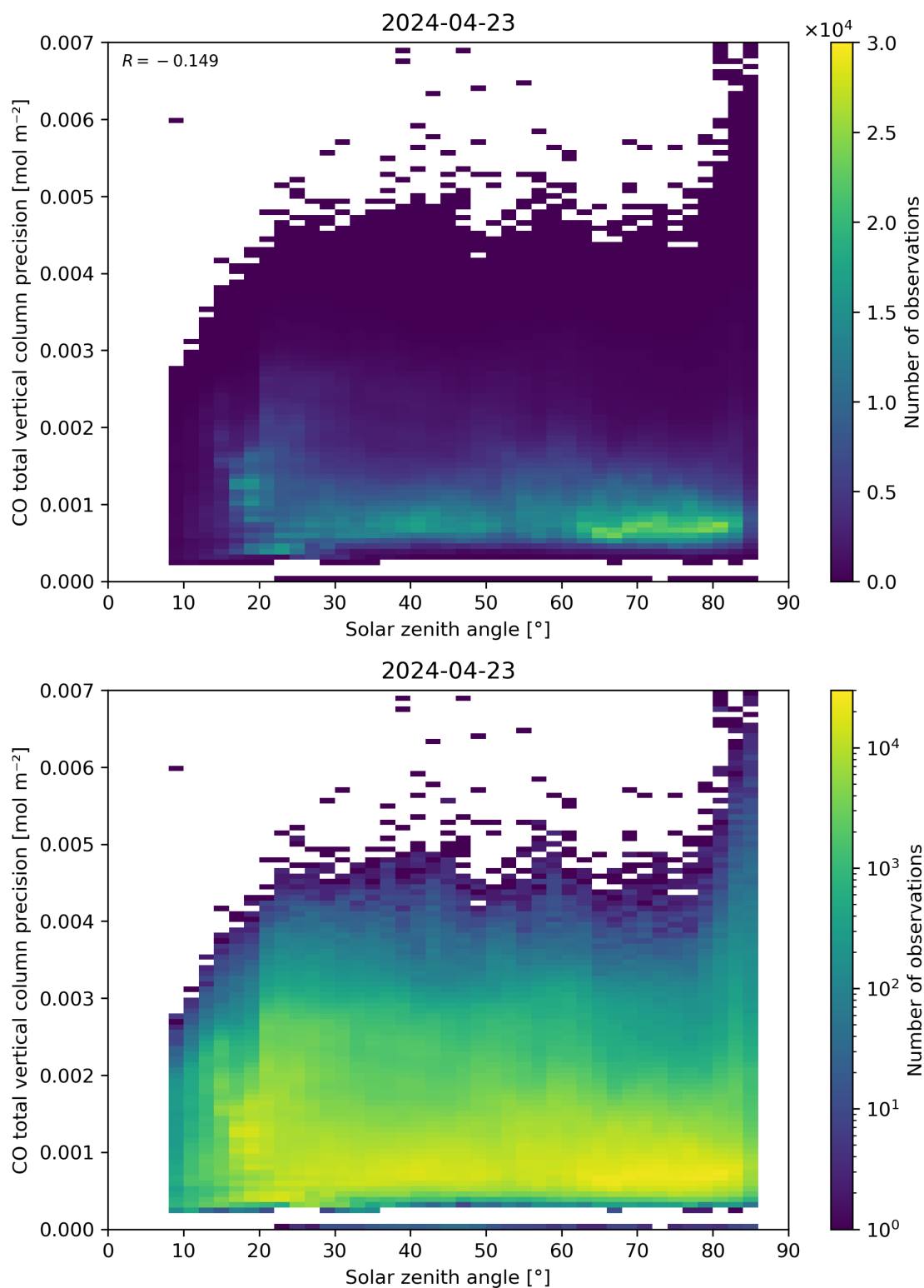
Figure 63: Scatter density plot of “Solar zenith angle” against “CO total vertical column precision” for 2024-04-22 to 2024-04-24.
