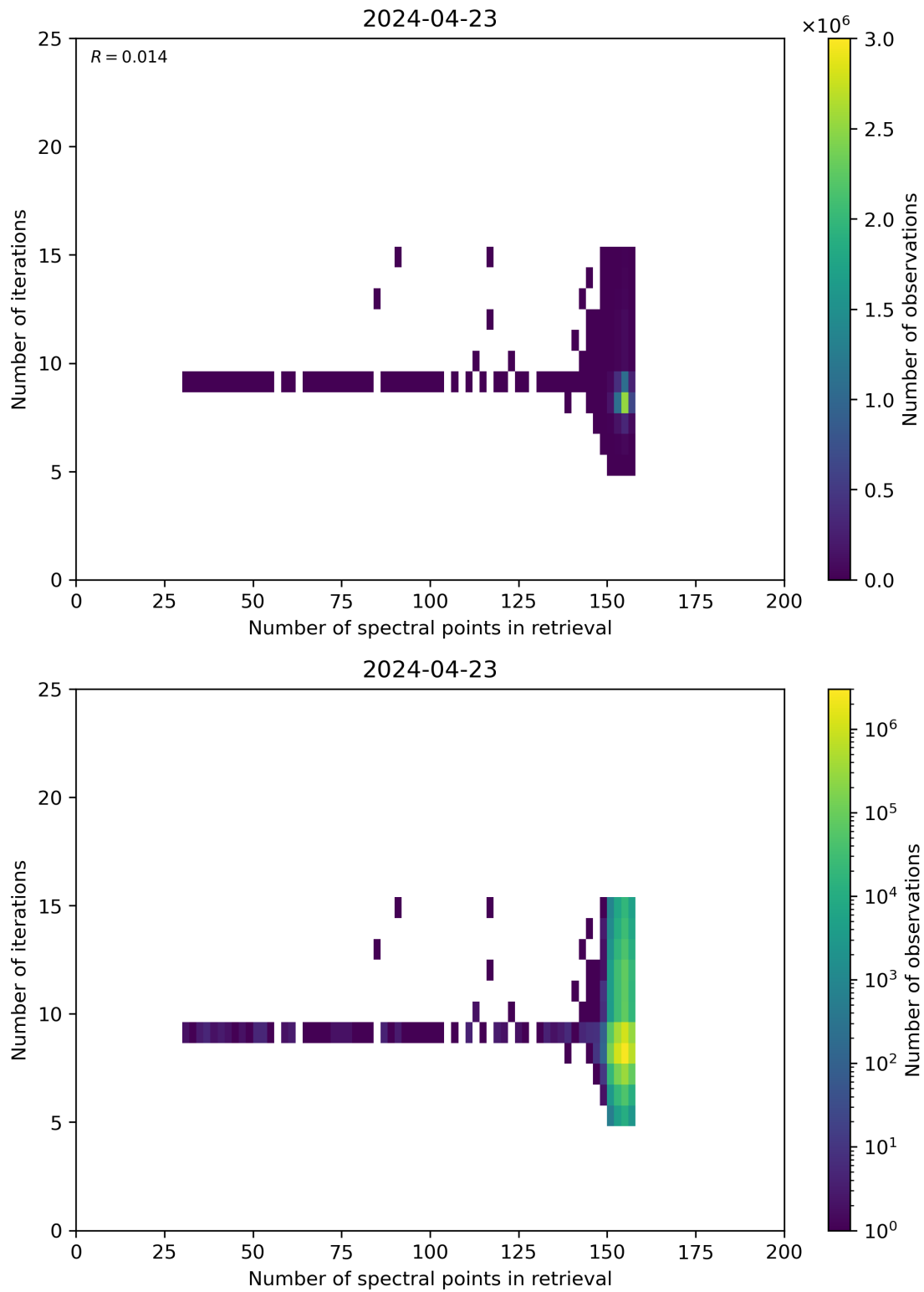
Figure 60: Scatter density plot of “Number of spectral points in retrieval” against “Number of iterations” for 2024-04-22 to 2024-04-24.
