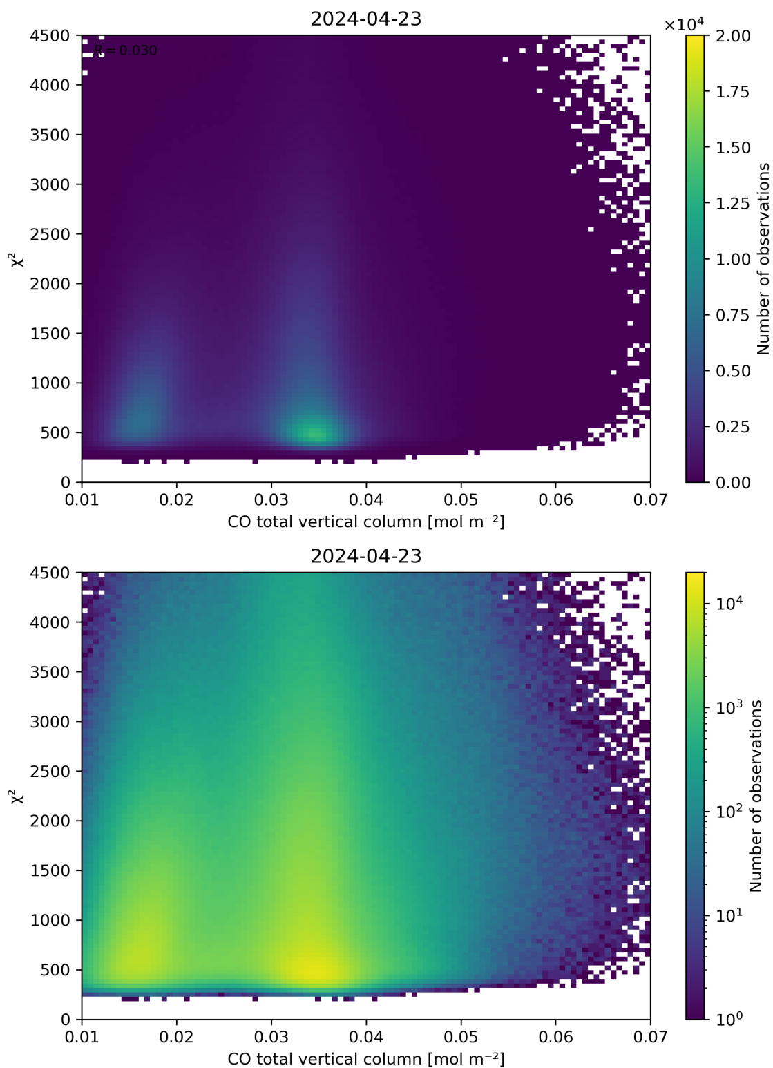
Figure 35: Scatter density plot of “CO total vertical column” against “ \chi^2 ” for 2024-04-22 to 2024-04-24.
