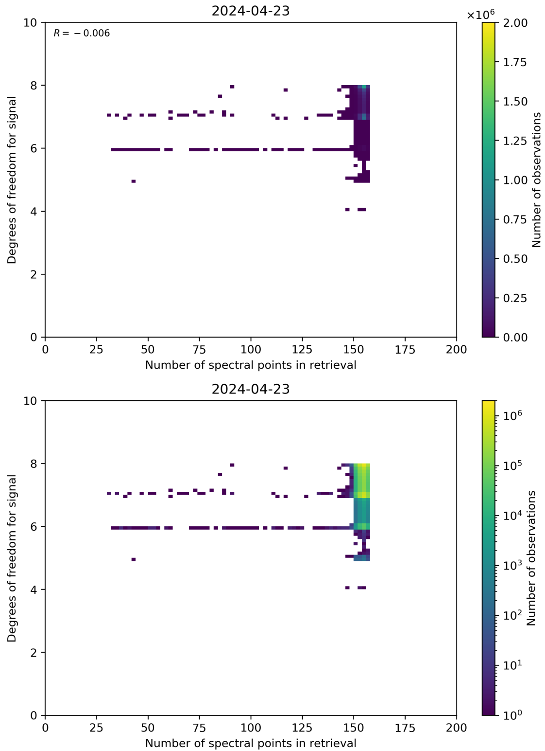
Figure 59: Scatter density plot of “Number of spectral points in retrieval” against “Degrees of freedom for signal” for 2024-04-22 to 2024-04-24.
