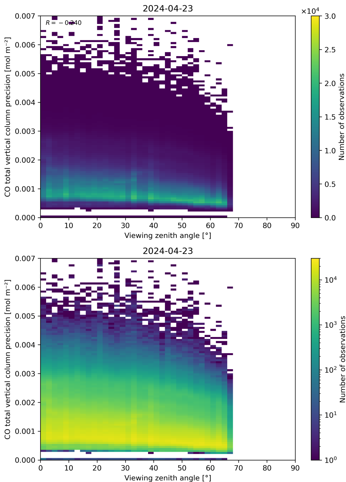
Figure 71: Scatter density plot of “Viewing zenith angle” against “CO total vertical column precision” for 2024-04-22 to 2024-04-24.
