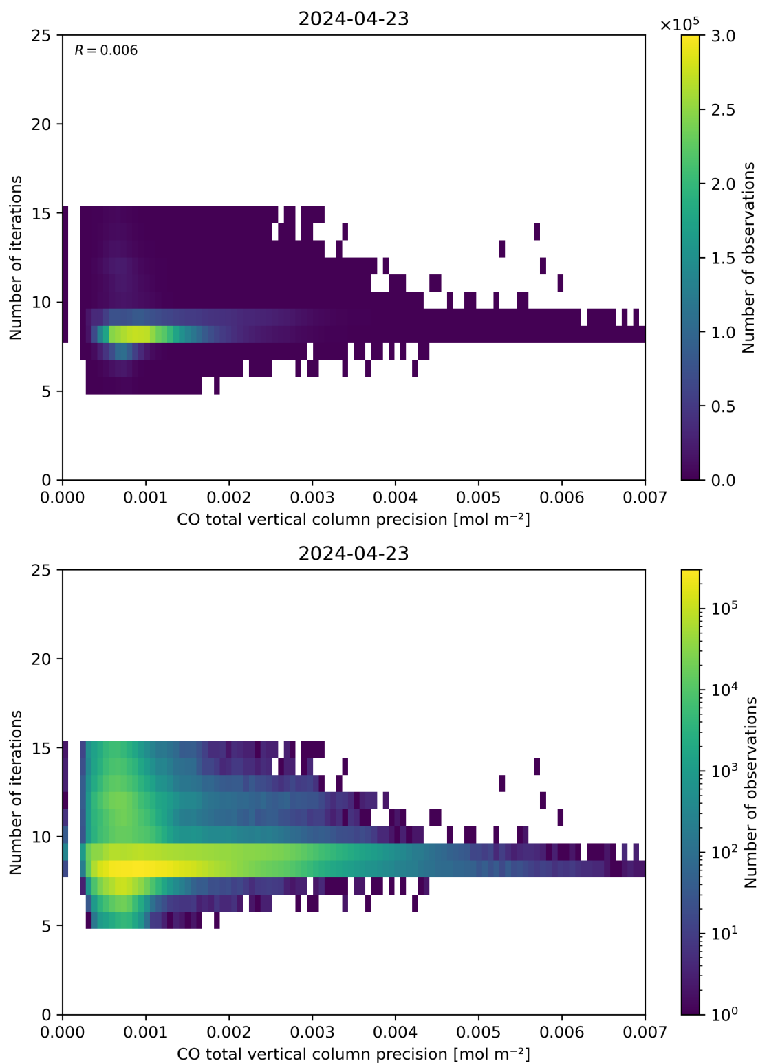
Figure 46: Scatter density plot of “CO total vertical column precision” against “Number of iterations” for 2024-04-22 to 2024-04-24.
