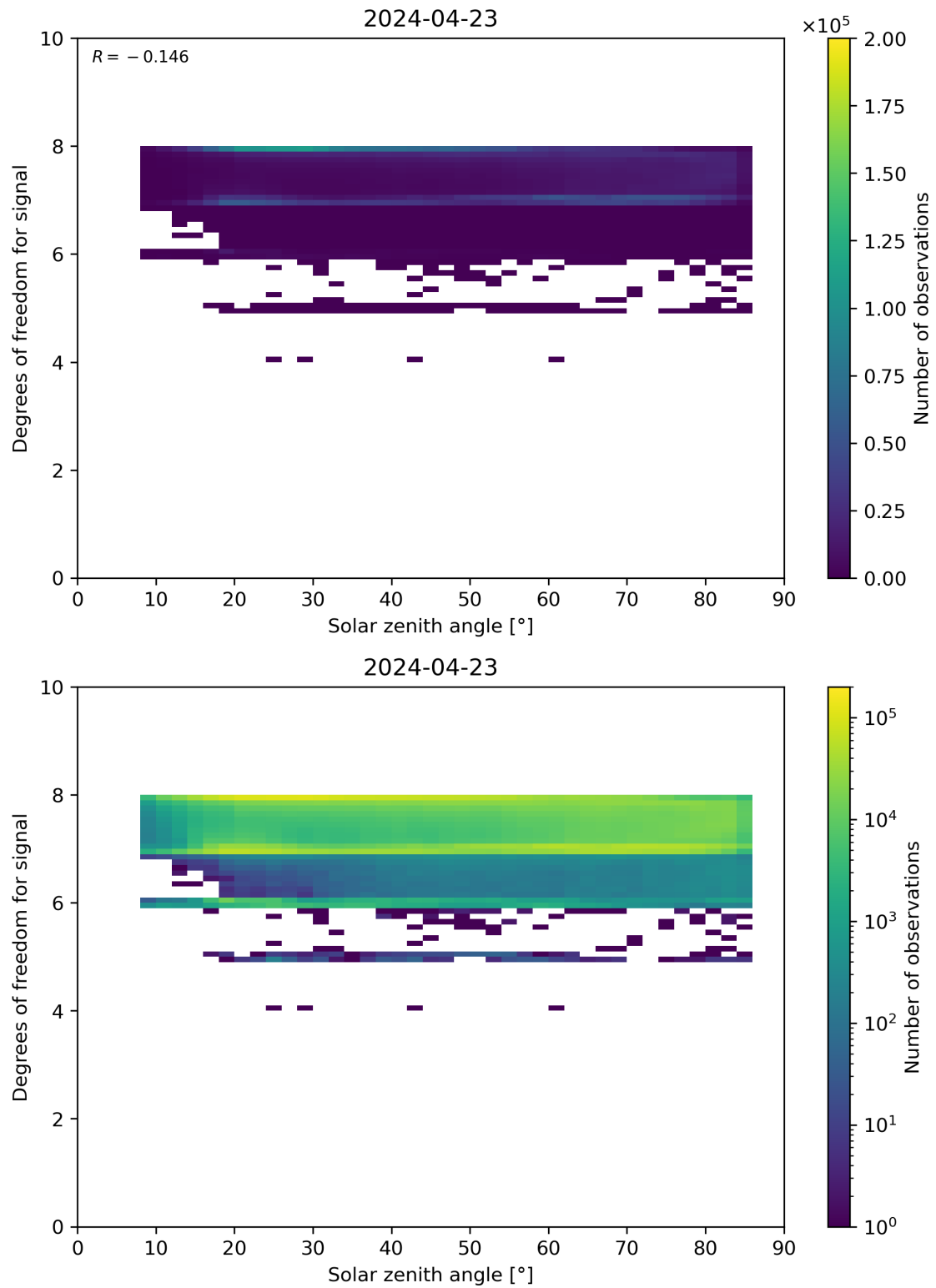
Figure 65: Scatter density plot of “Solar zenith angle” against “Degrees of freedom for signal” for 2024-04-22 to 2024-04-24.
