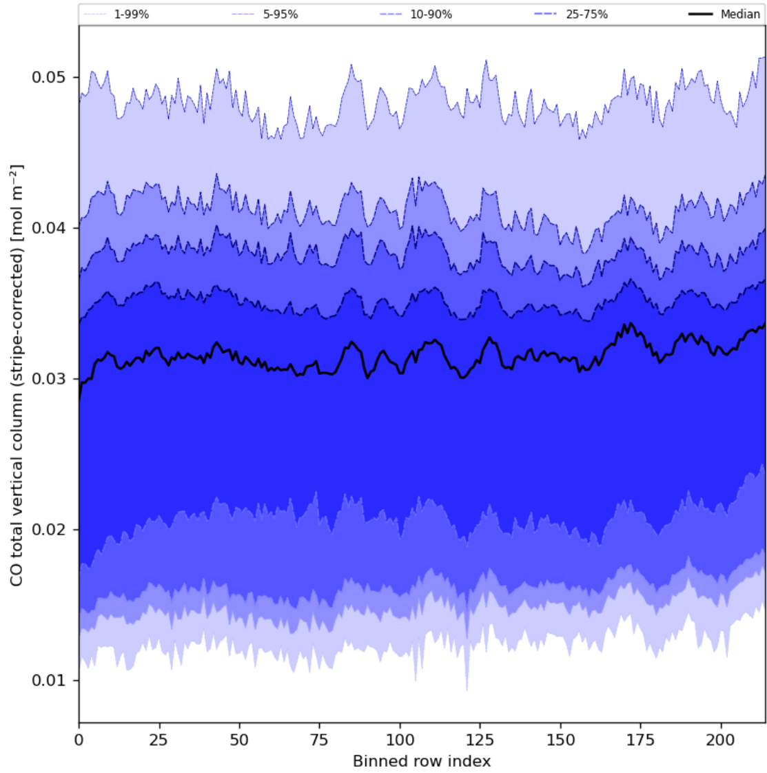
Figure 27: Along track statistics of “CO total vertical column (stripe-corrected)” for 2024-04-22 to 2024-04-24
