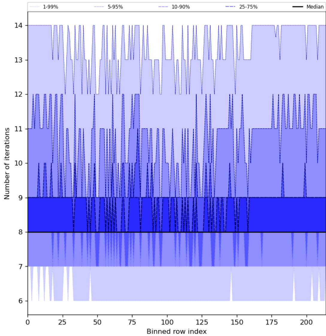
Figure 32: Along track statistics of “Number of iterations” for 2024-04-22 to 2024-04-24
