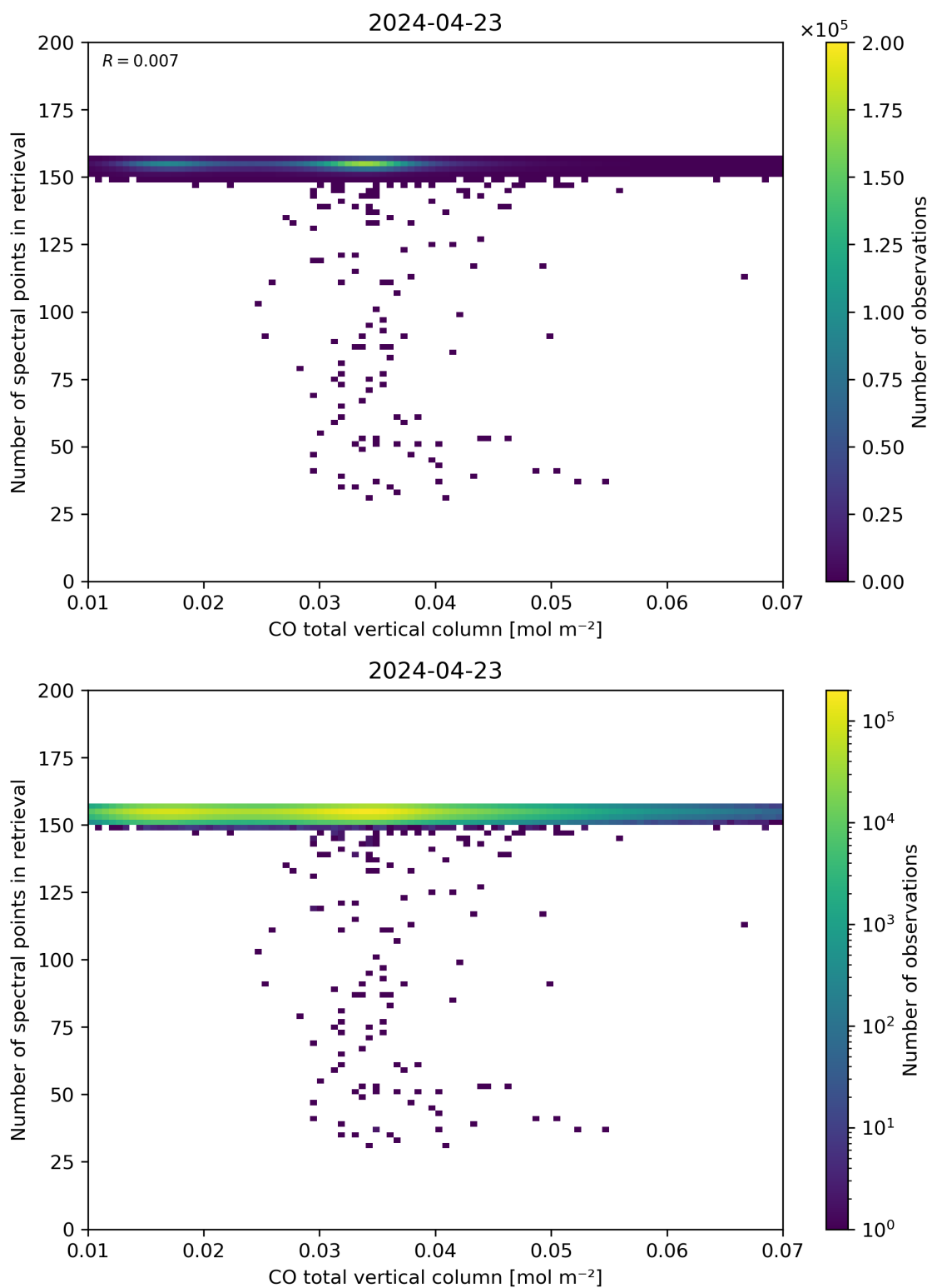
Figure 43: Scatter density plot of “CO total vertical column” against “Number of spectral points in retrieval” for 2024-04-22 to 2024-04-24.
