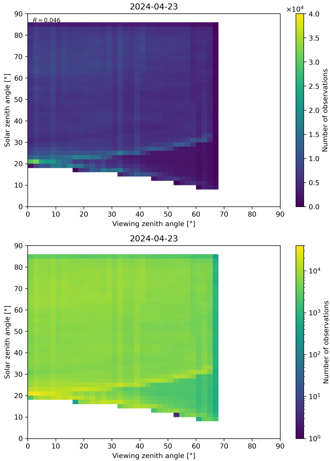
Figure 77: Scatter density plot of “Viewing zenith angle” against “Solar zenith angle” for 2024-04-22 to 2024-04-24.
