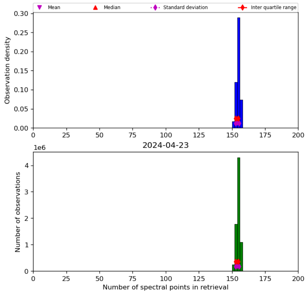
Figure 21: Histogram of “Number of spectral points in retrieval” for 2024-04-22 to 2024-04-24
