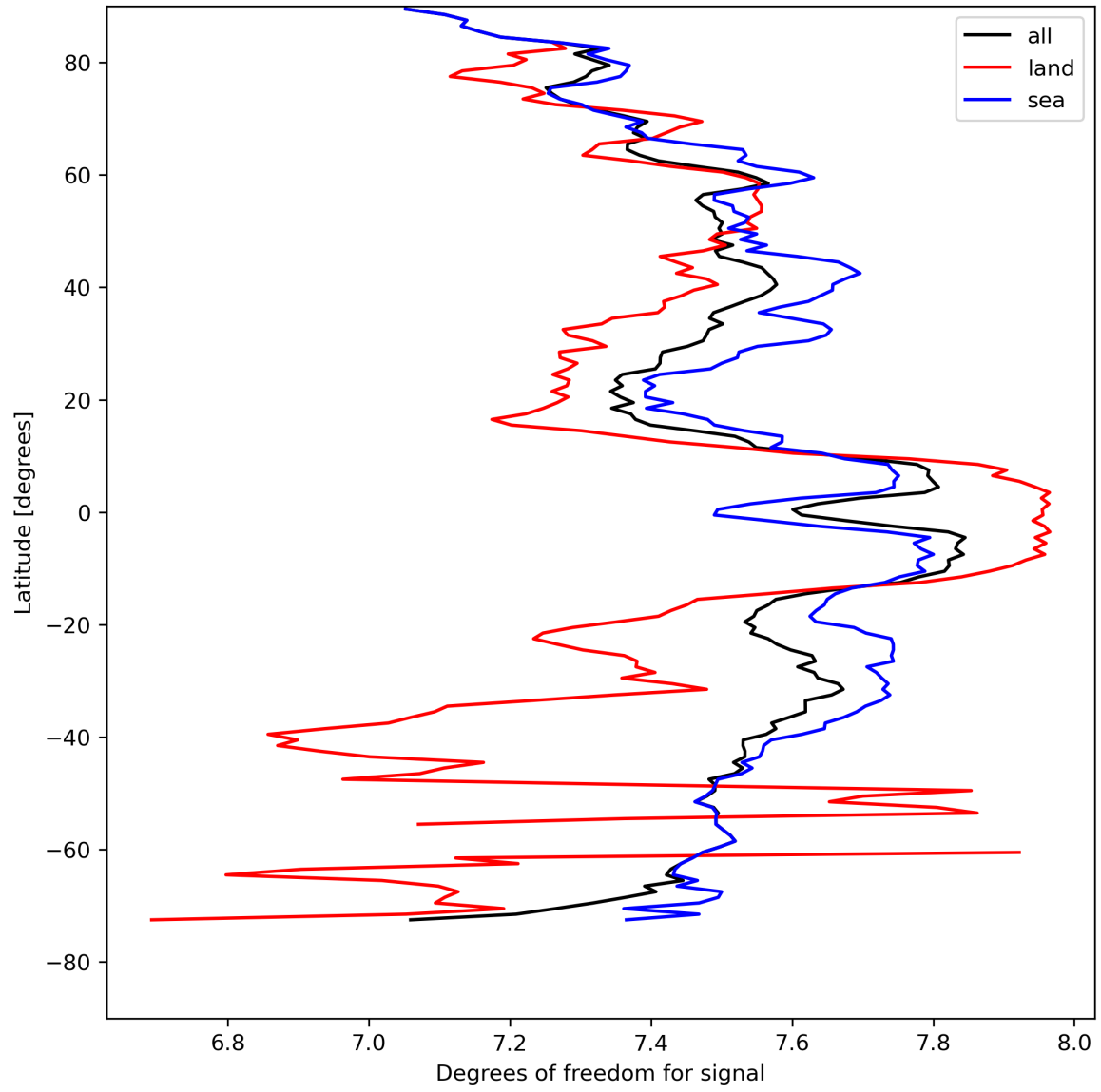
Figure 15: Zonal average of “Degrees of freedom for signal” for 2024-04-22 to 2024-04-24.
