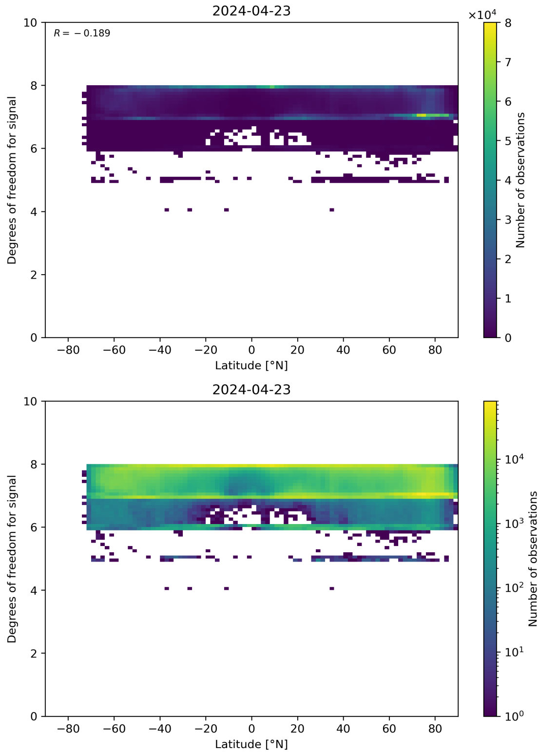
Figure 55: Scatter density plot of “Latitude” against “Degrees of freedom for signal” for 2024-04-22 to 2024-04-24.
