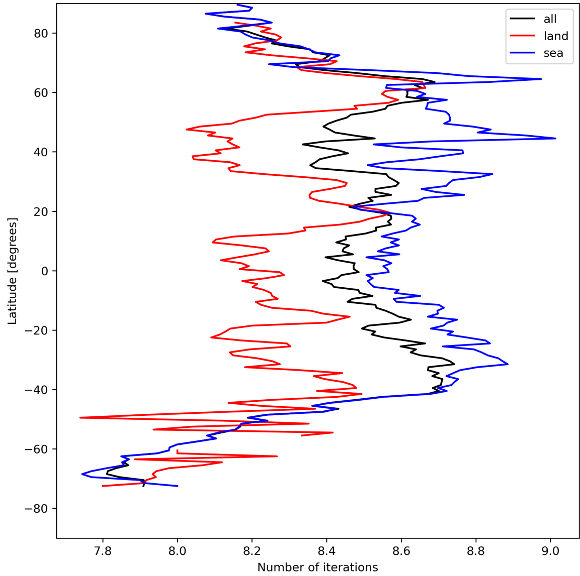
Figure 16: Zonal average of “Number of iterations” for 2024-04-22 to 2024-04-24.
