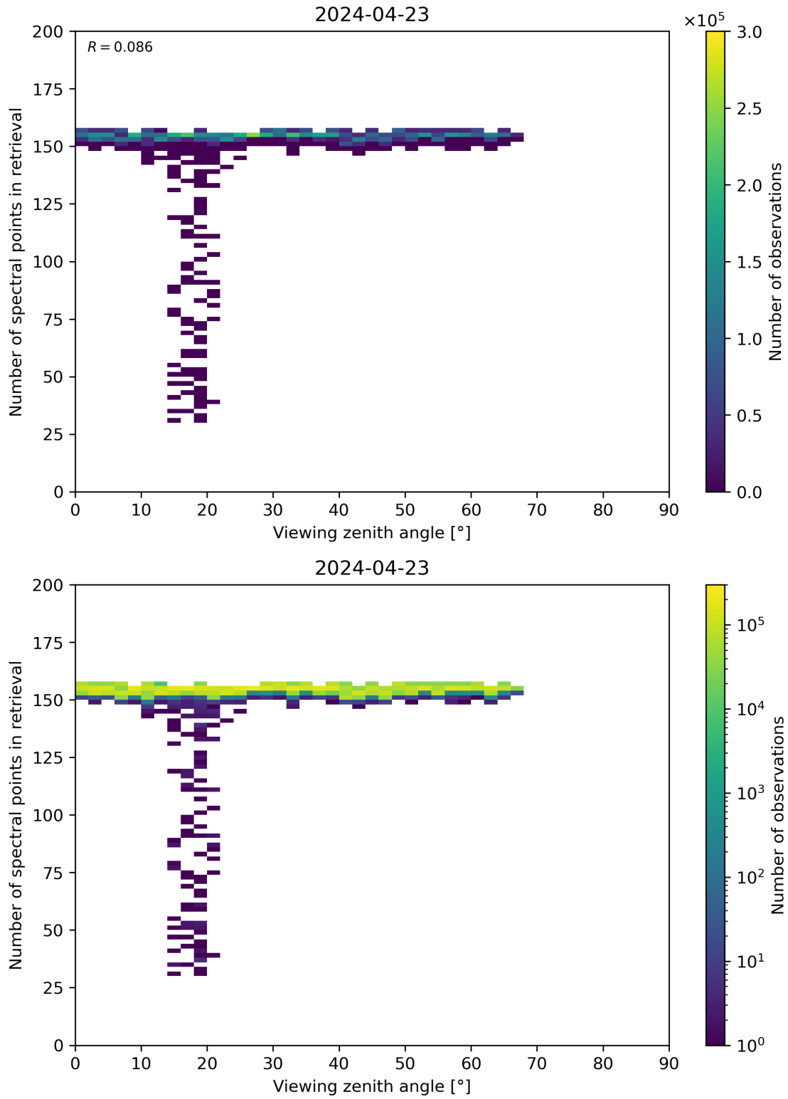
Figure 76: Scatter density plot of “Viewing zenith angle” against “Number of spectral points in retrieval” for 2024-04-22 to 2024-04-24.
