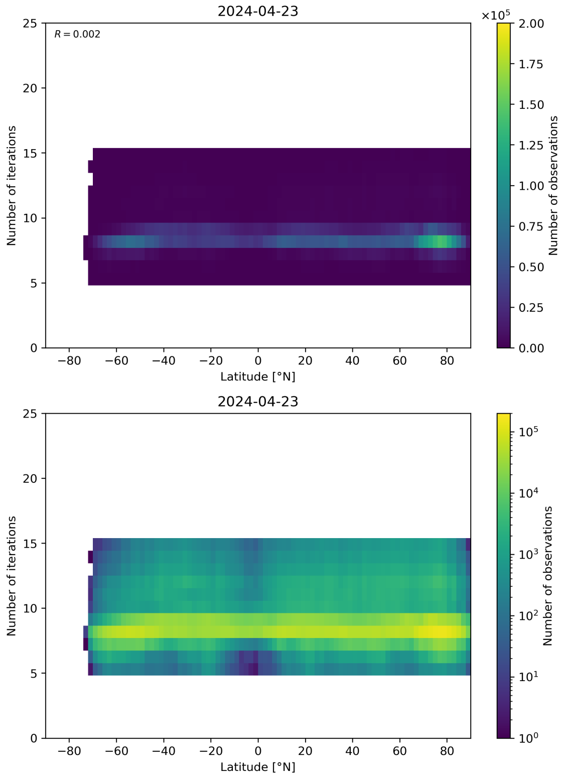
Figure 56: Scatter density plot of “Latitude” against “Number of iterations” for 2024-04-22 to 2024-04-24.
