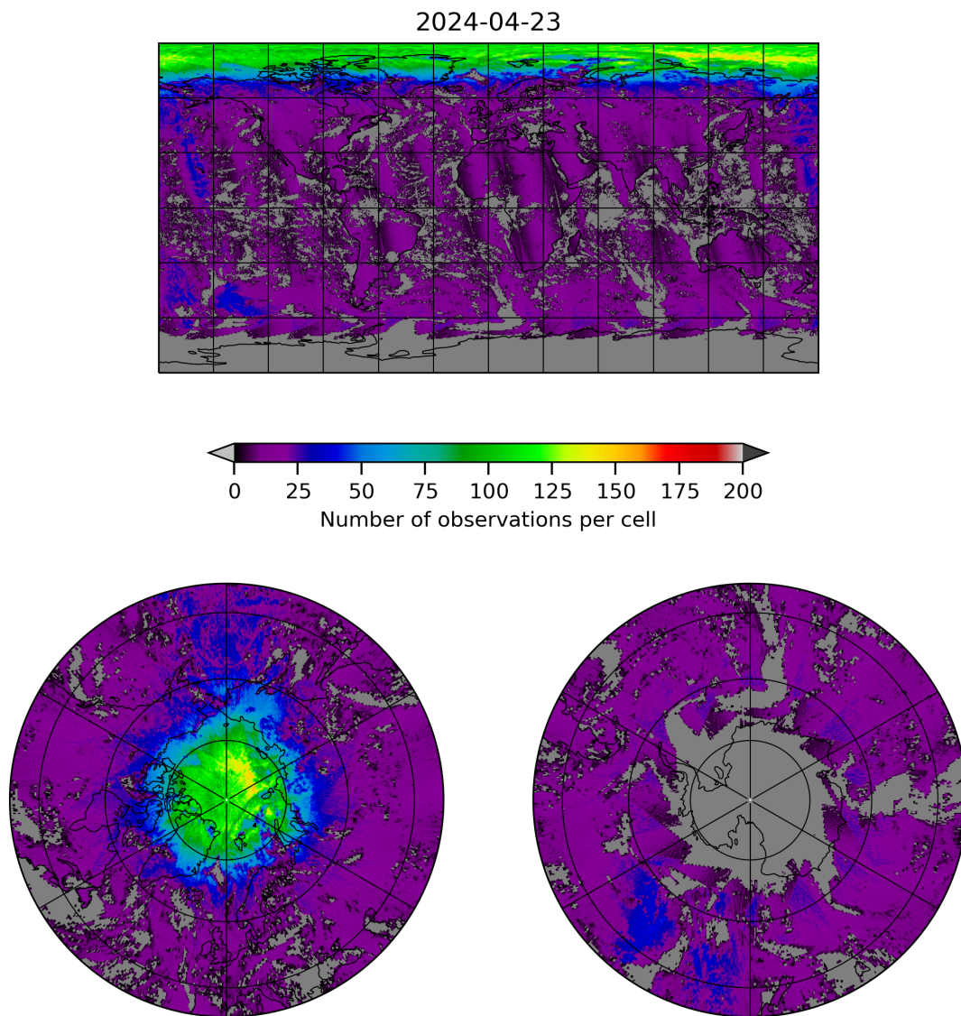
Figure 8: Map of the number of observations for 2024-04-22 to 2024-04-24
