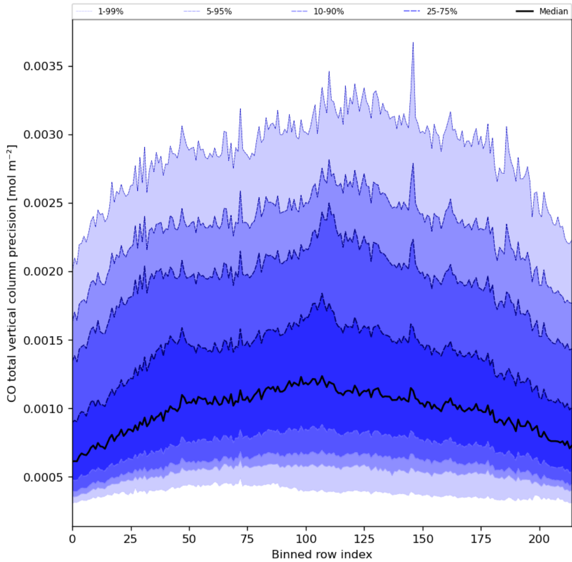
Figure 28: Along track statistics of “CO total vertical column precision” for 2024-04-22 to 2024-04-24
