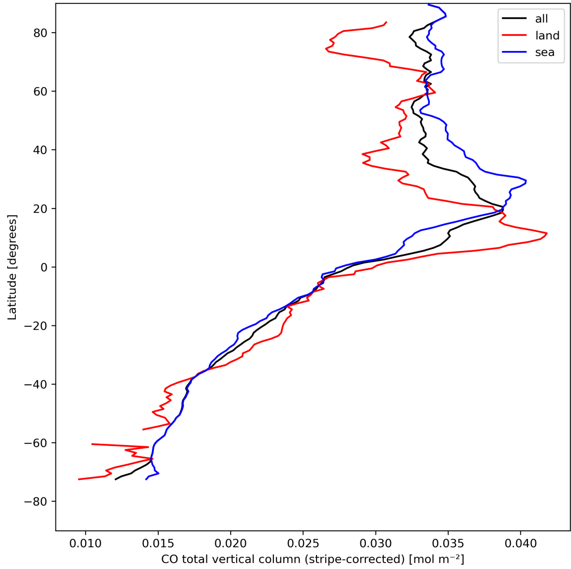
Figure 11: Zonal average of “CO total vertical column (stripe-corrected)” for 2024-04-22 to 2024-04-24.
