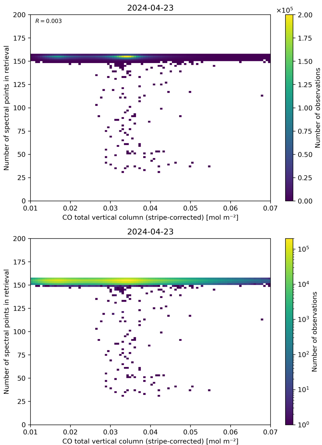
Figure 40: Scatter density plot of “CO total vertical column (stripe-corrected)” against “Number of spectral points in retrieval” for 2024-04-22 to 2024-04-24.
