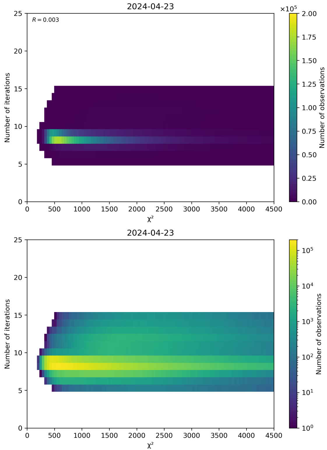
Figure 49: Scatter density plot of “ \chi^2 ” against “Number of iterations” for 2024-04-22 to 2024-04-24.
