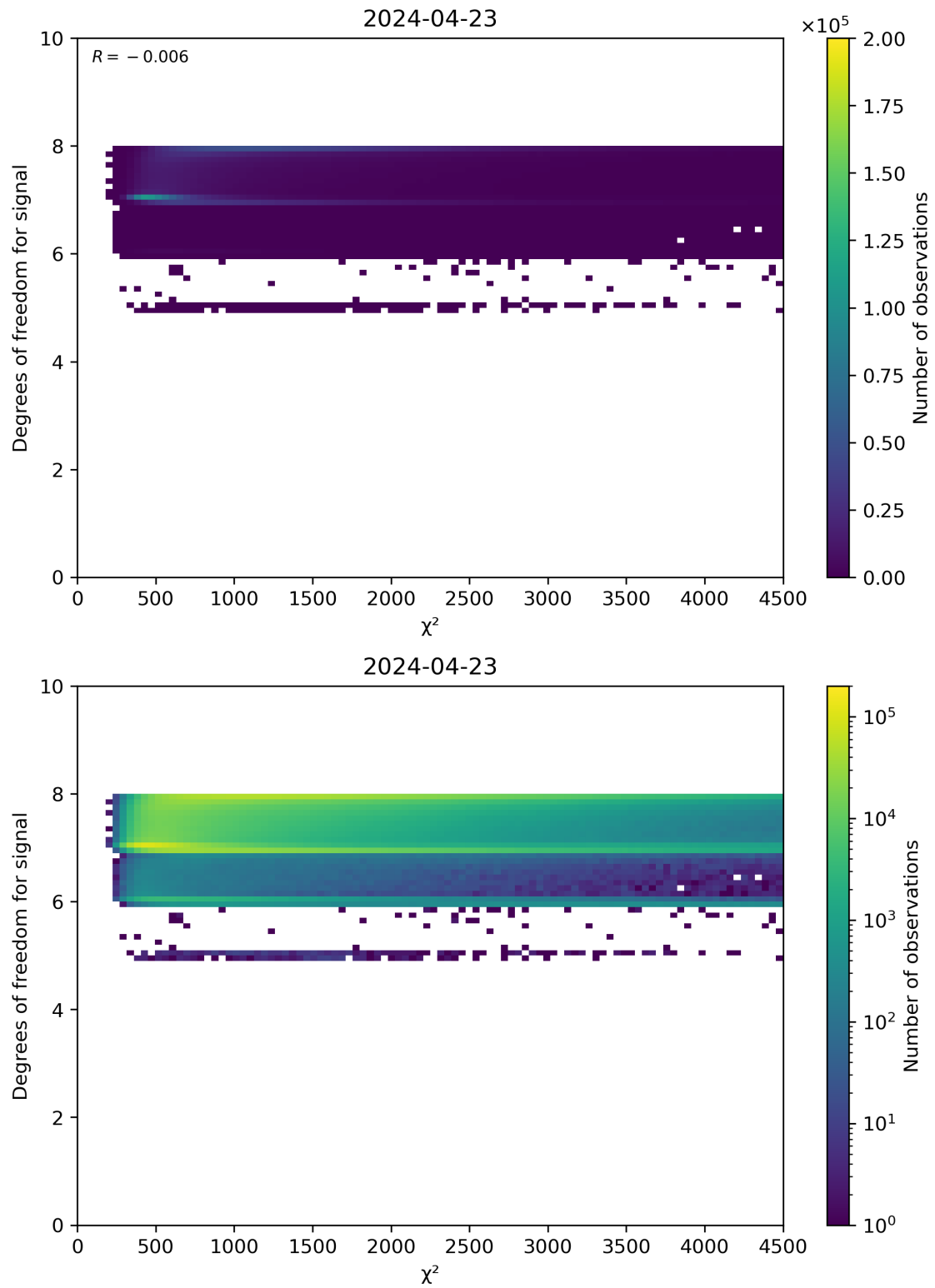
Figure 48: Scatter density plot of “ \chi^2 ” against “Degrees of freedom for signal” for 2024-04-22 to 2024-04-24.
