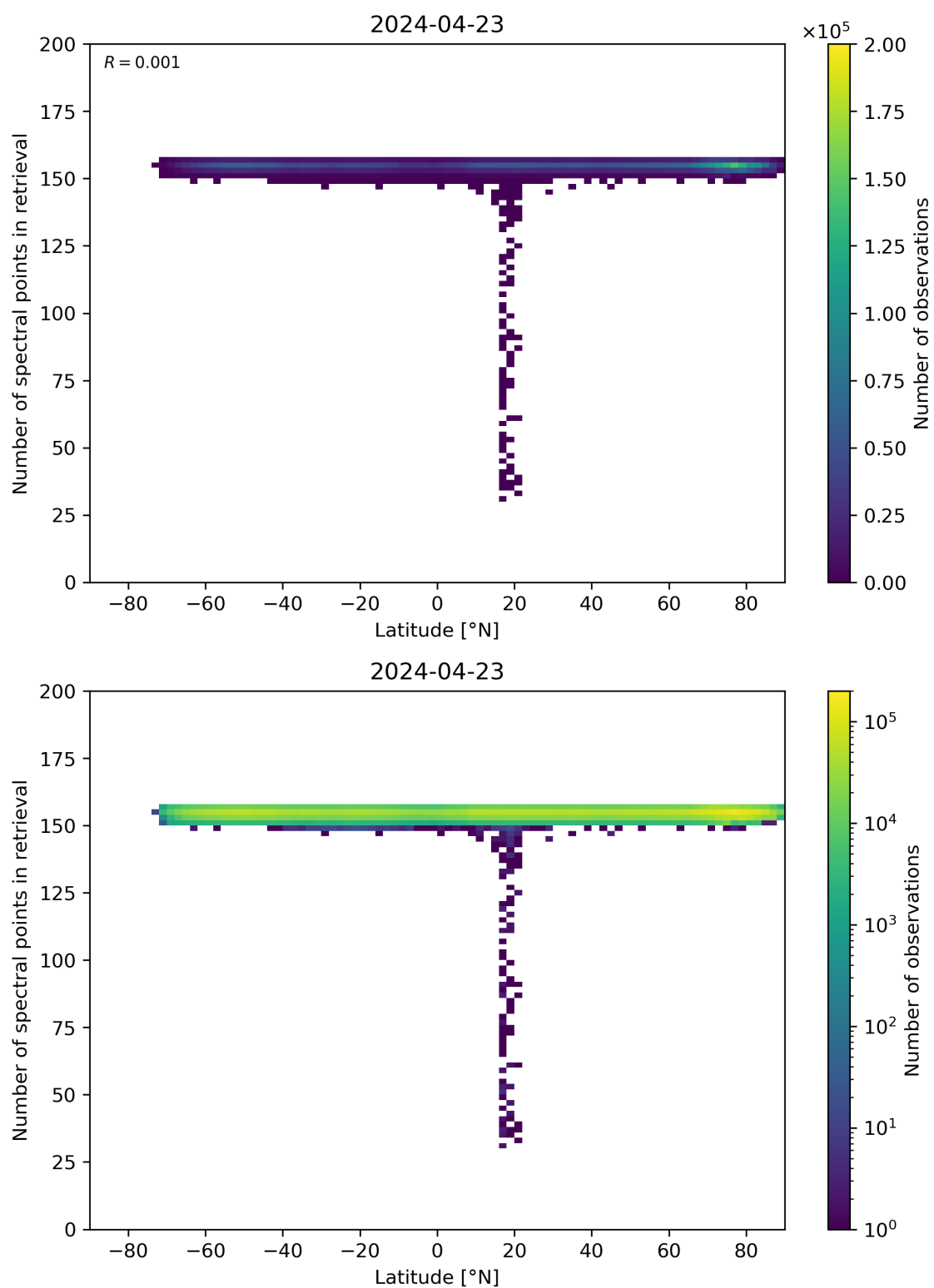
Figure 57: Scatter density plot of “Latitude” against “Number of spectral points in retrieval” for 2024-04-22 to 2024-04-24.
