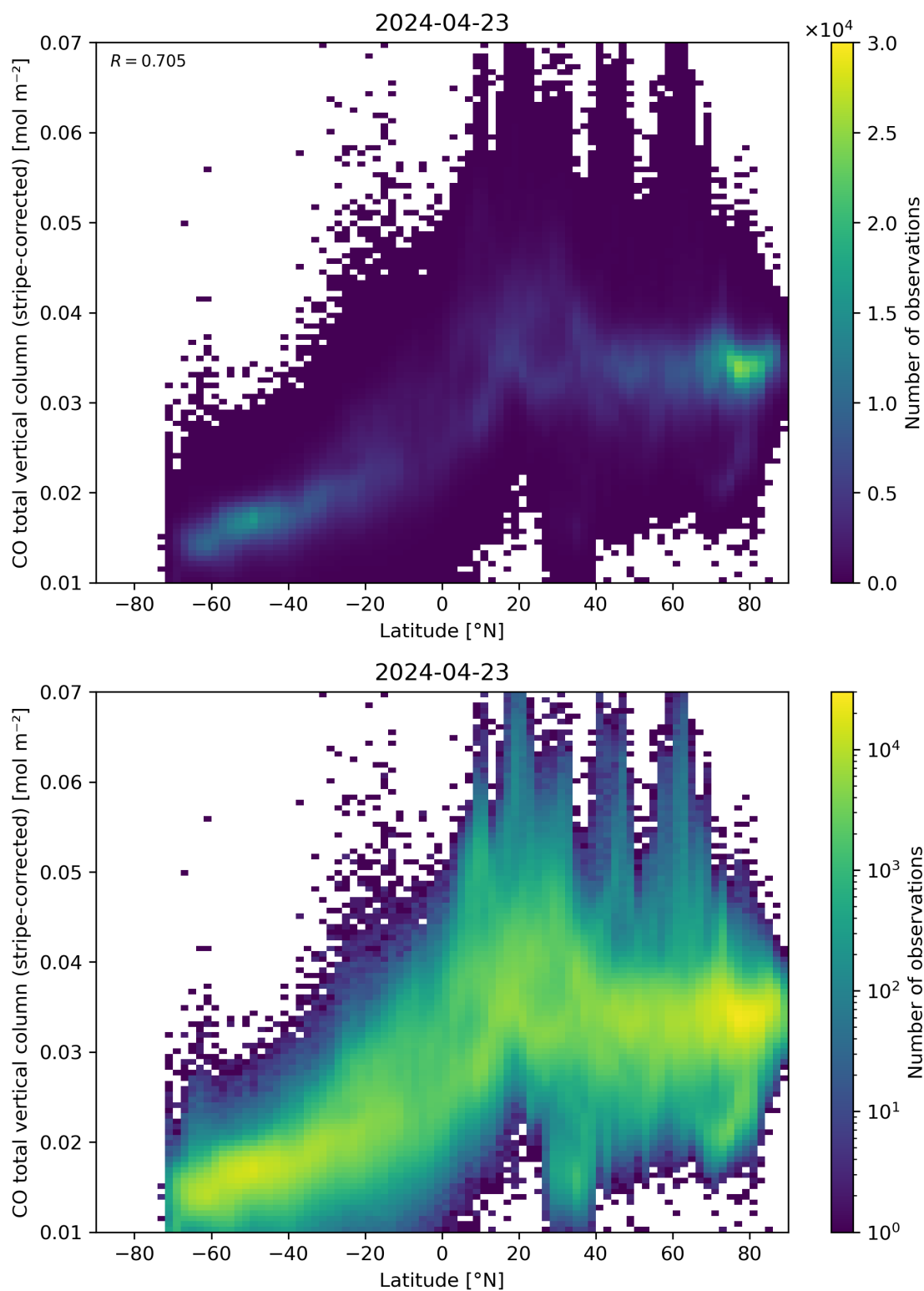
Figure 52: Scatter density plot of “Latitude” against “CO total vertical column (stripe-corrected)” for 2024-04-22 to 2024-04-24.
