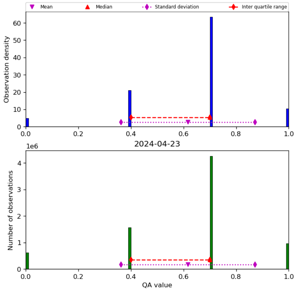
Figure 17: Histogram of “QA value” for 2024-04-22 to 2024-04-24
