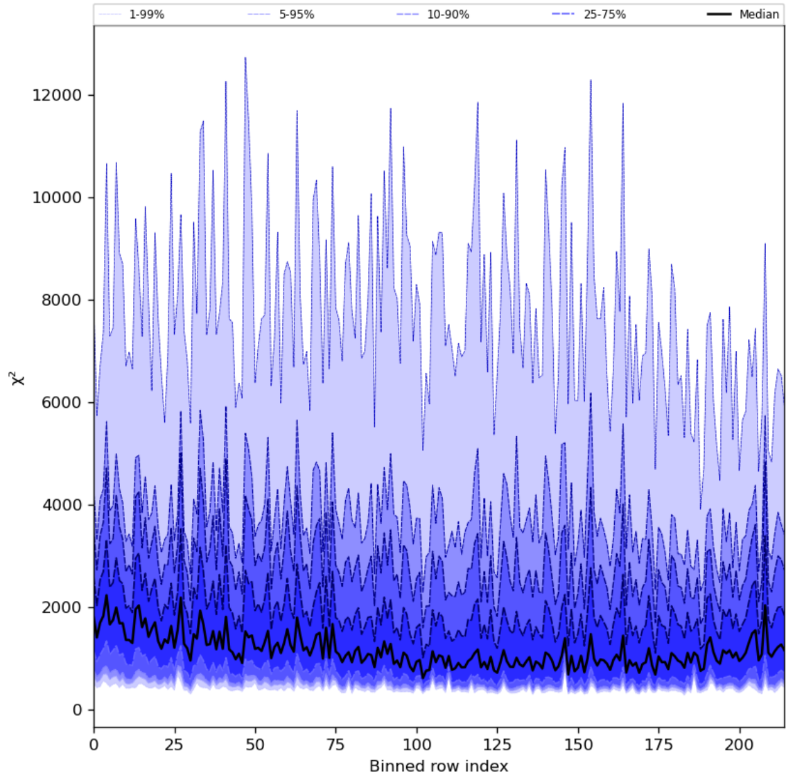
Figure 30: Along track statistics of “ \chi^2 ” for 2024-04-22 to 2024-04-24
