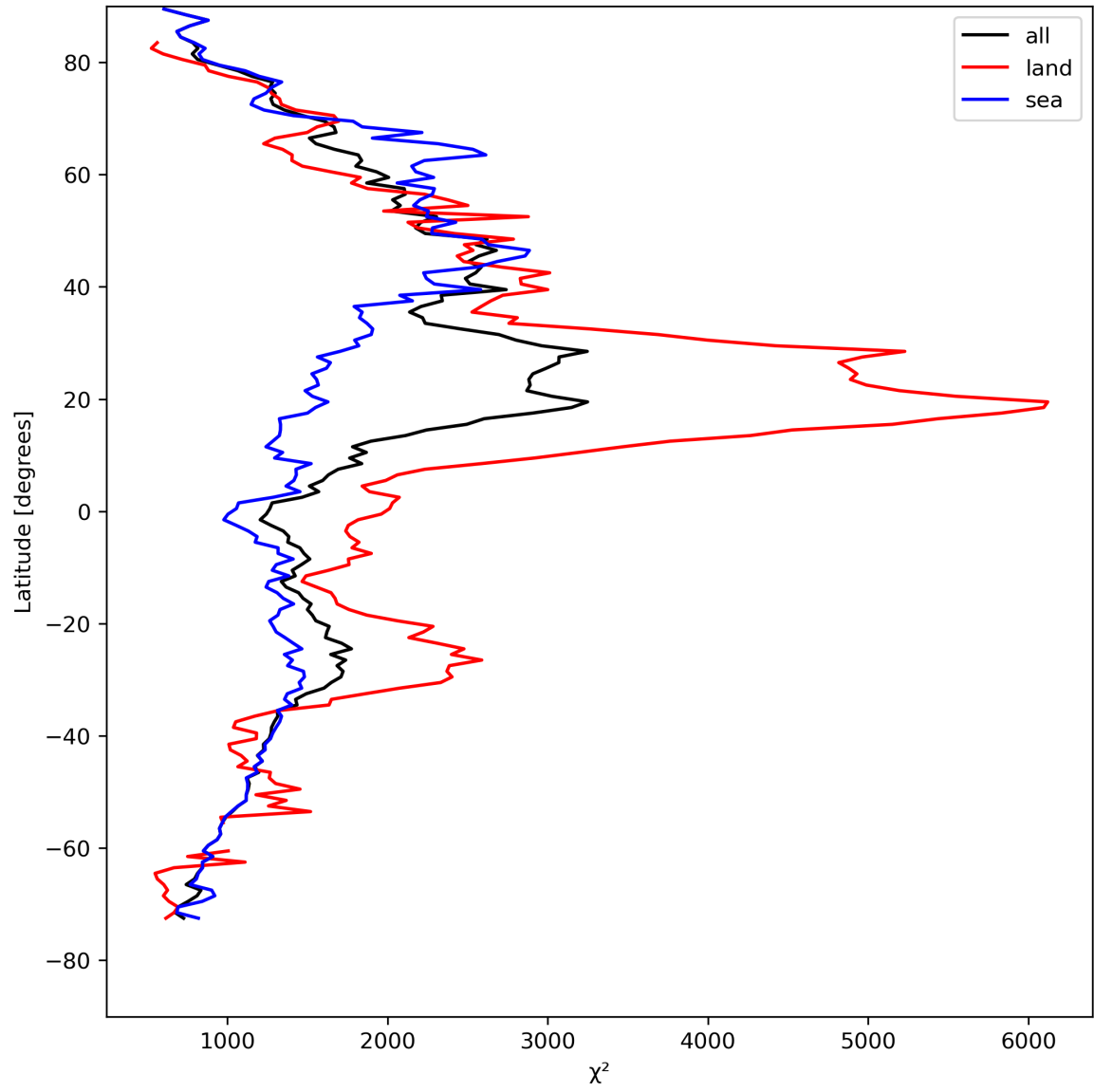
Figure 14: Zonal average of “ \chi^2 ” for 2024-04-22 to 2024-04-24.
