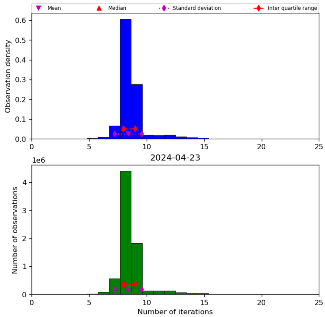
Figure 24: Histogram of “Number of iterations” for 2024-04-22 to 2024-04-24
