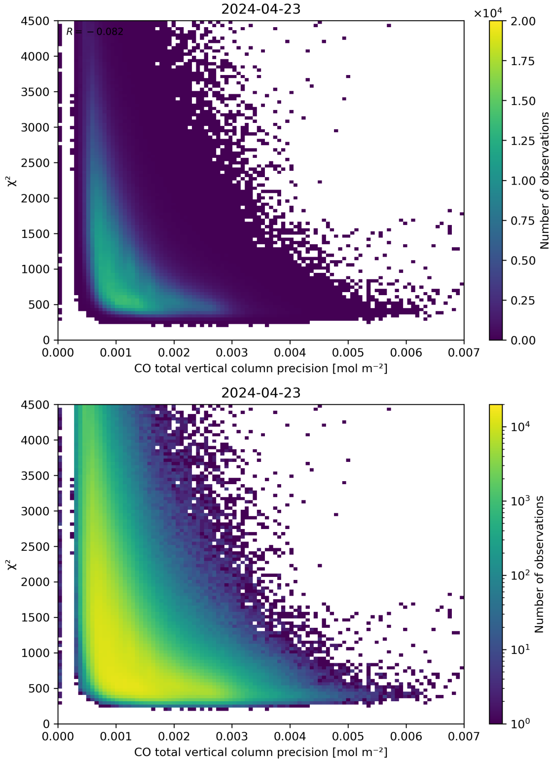
Figure 44: Scatter density plot of “CO total vertical column precision” against “ \chi^2 ” for 2024-04-22 to 2024-04-24.
