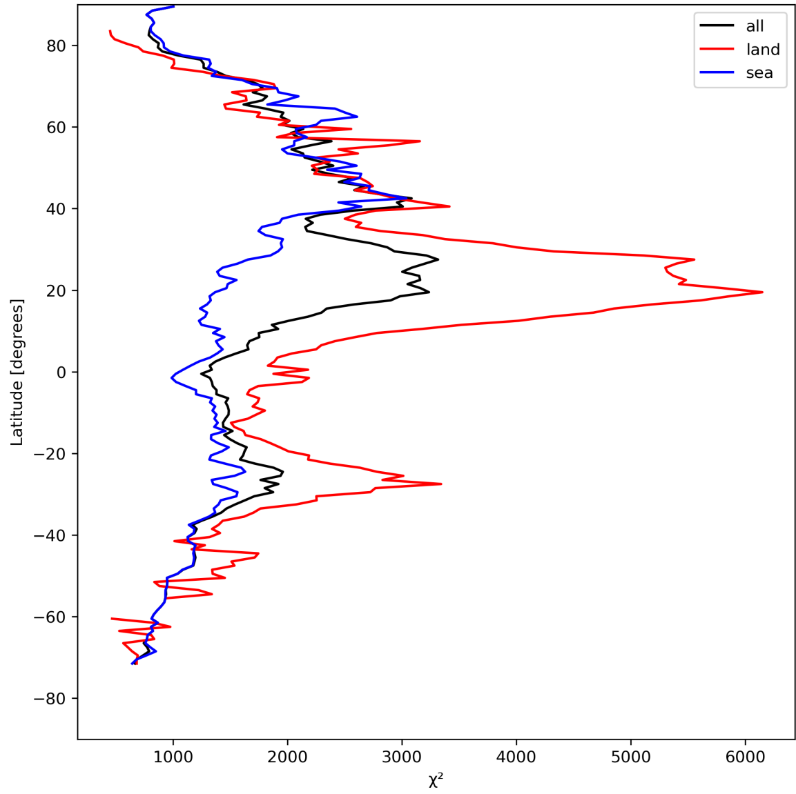
Figure 14: Zonal average of “ \chi^2 ” for 2024-04-23 to 2024-04-25.
