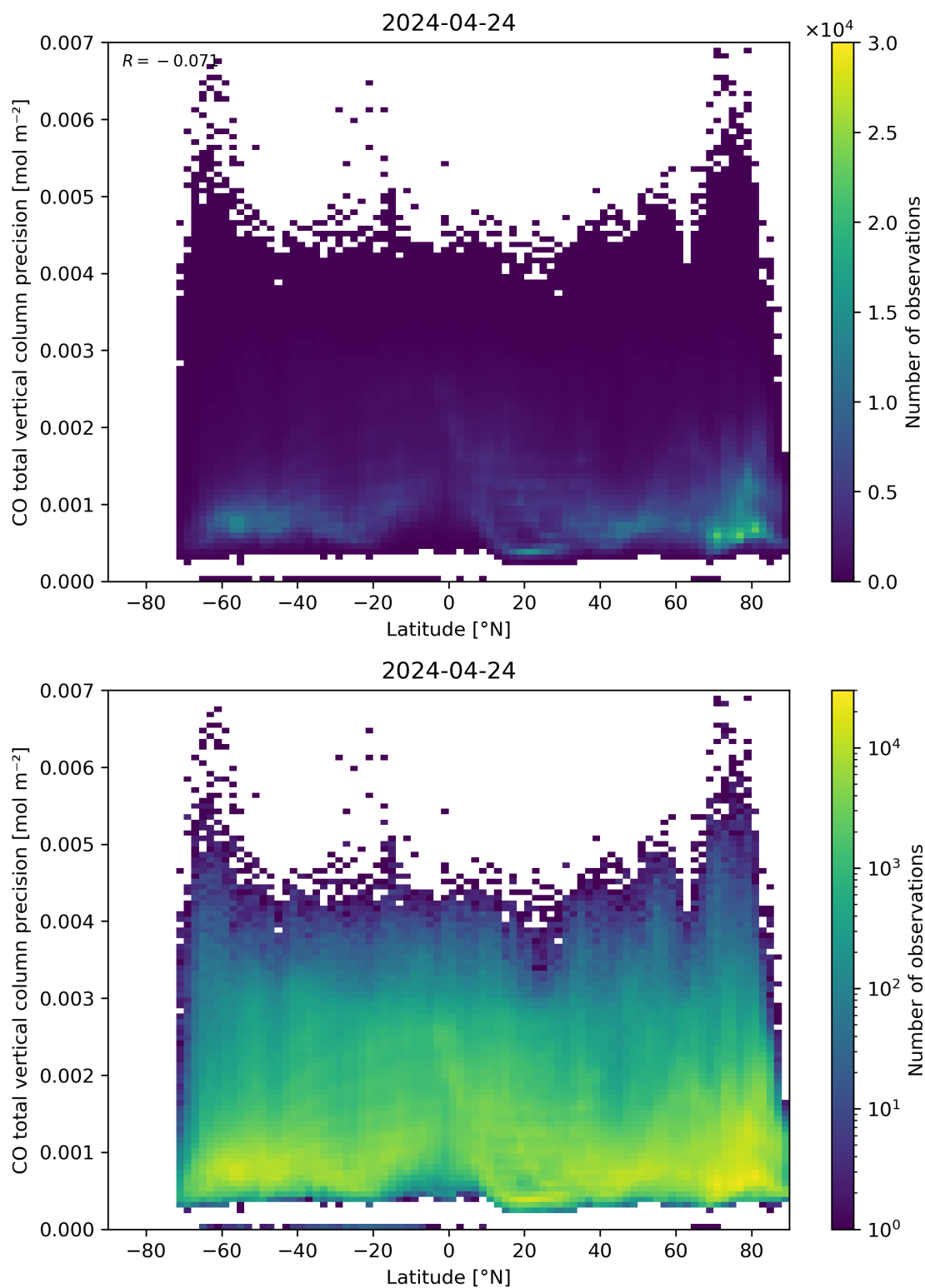
Figure 53: Scatter density plot of “Latitude” against “CO total vertical column precision” for 2024-04-23 to 2024-04-25.
