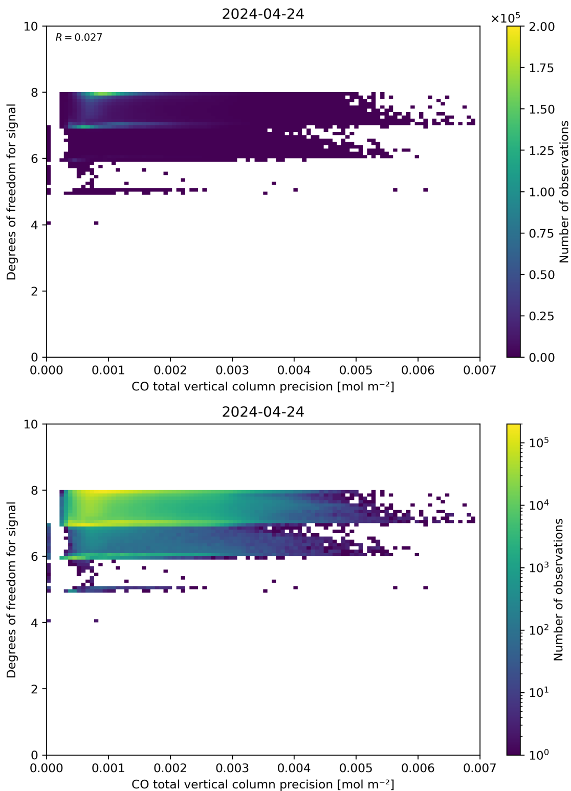
Figure 45: Scatter density plot of “CO total vertical column precision” against “Degrees of freedom for signal” for 2024-04-23 to 2024-04-25.
