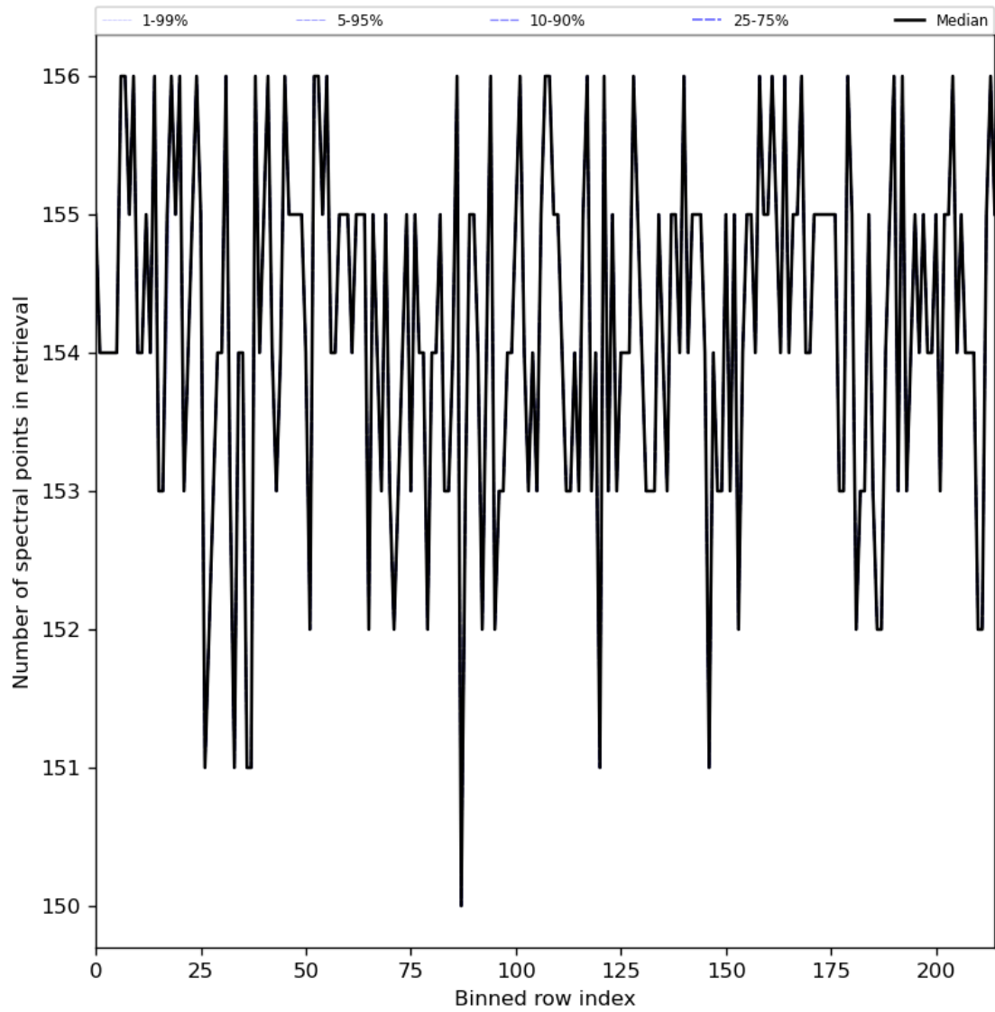
Figure 29: Along track statistics of “Number of spectral points in retrieval” for 2024-04-23 to 2024-04-25
