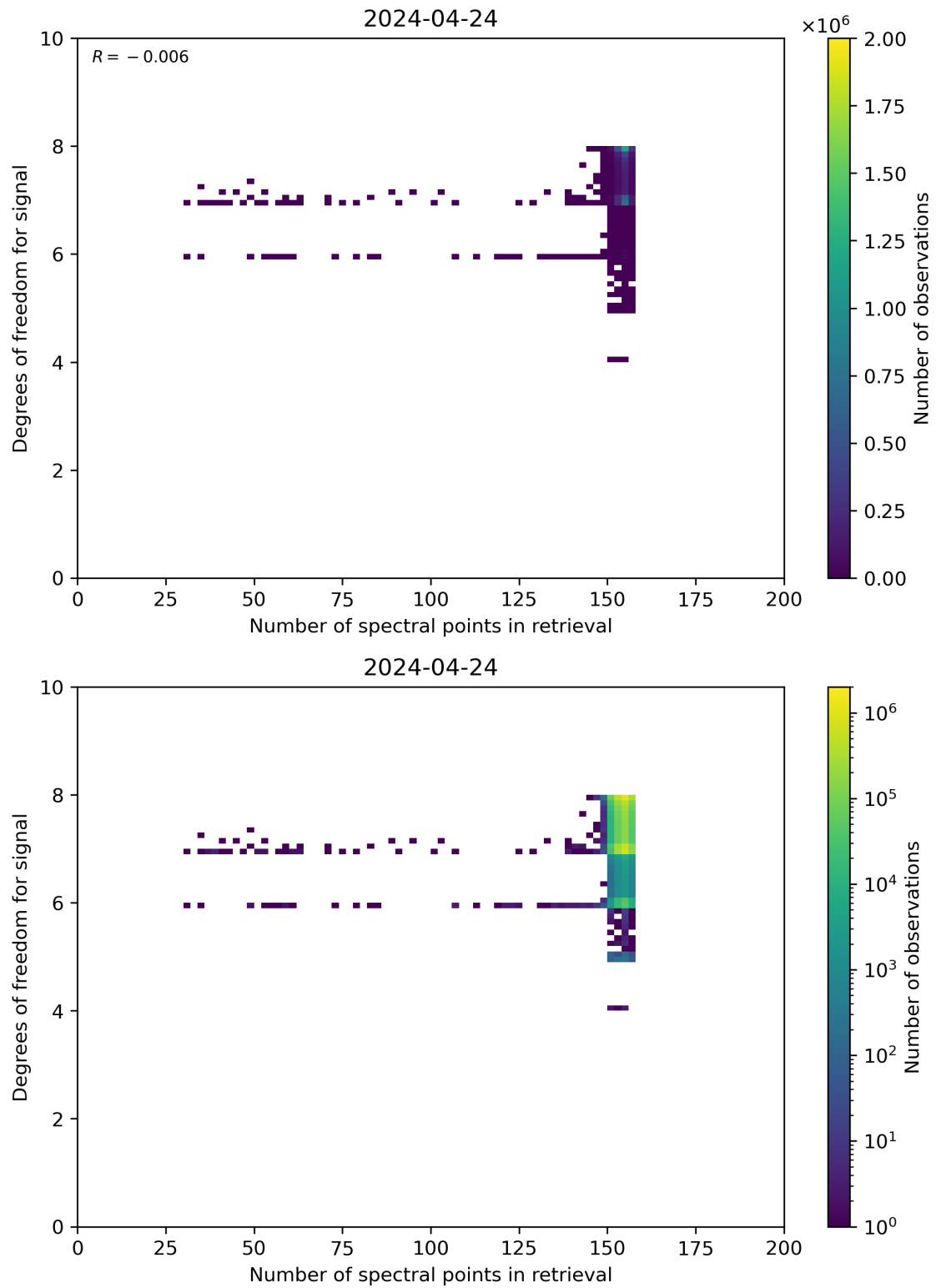
Figure 59: Scatter density plot of “Number of spectral points in retrieval” against “Degrees of freedom for signal” for 2024-04-23 to 2024-04-25.
