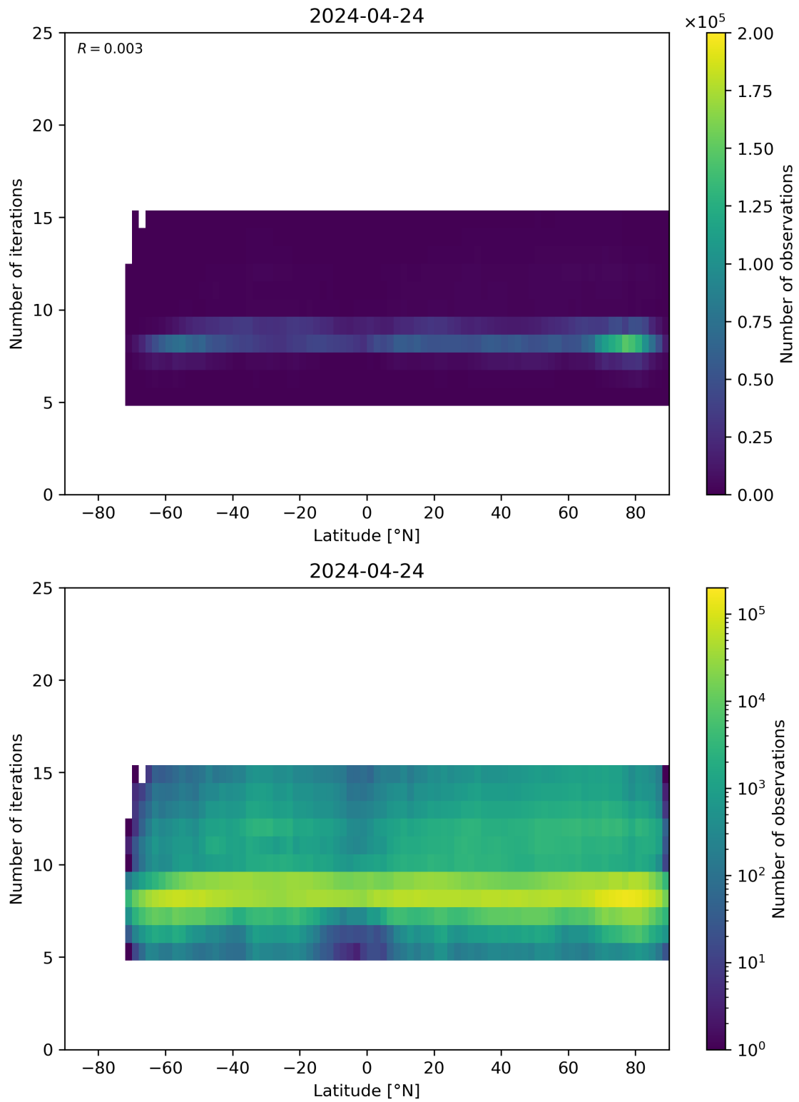
Figure 56: Scatter density plot of “Latitude” against “Number of iterations” for 2024-04-23 to 2024-04-25.
