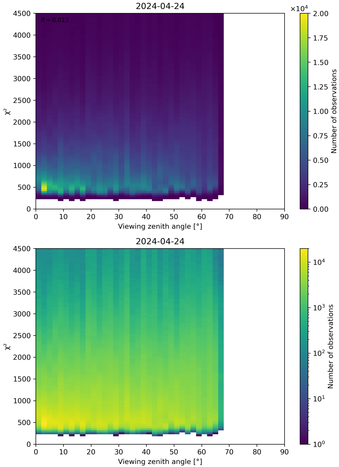
Figure 72: Scatter density plot of “Viewing zenith angle” against “ \chi^2 ” for 2024-04-23 to 2024-04-25.
