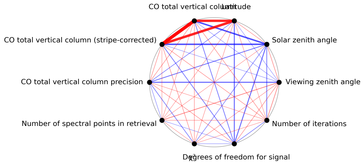
Figure 1: Map of correlation graph for 2024-04-23 to 2024-04-25.
