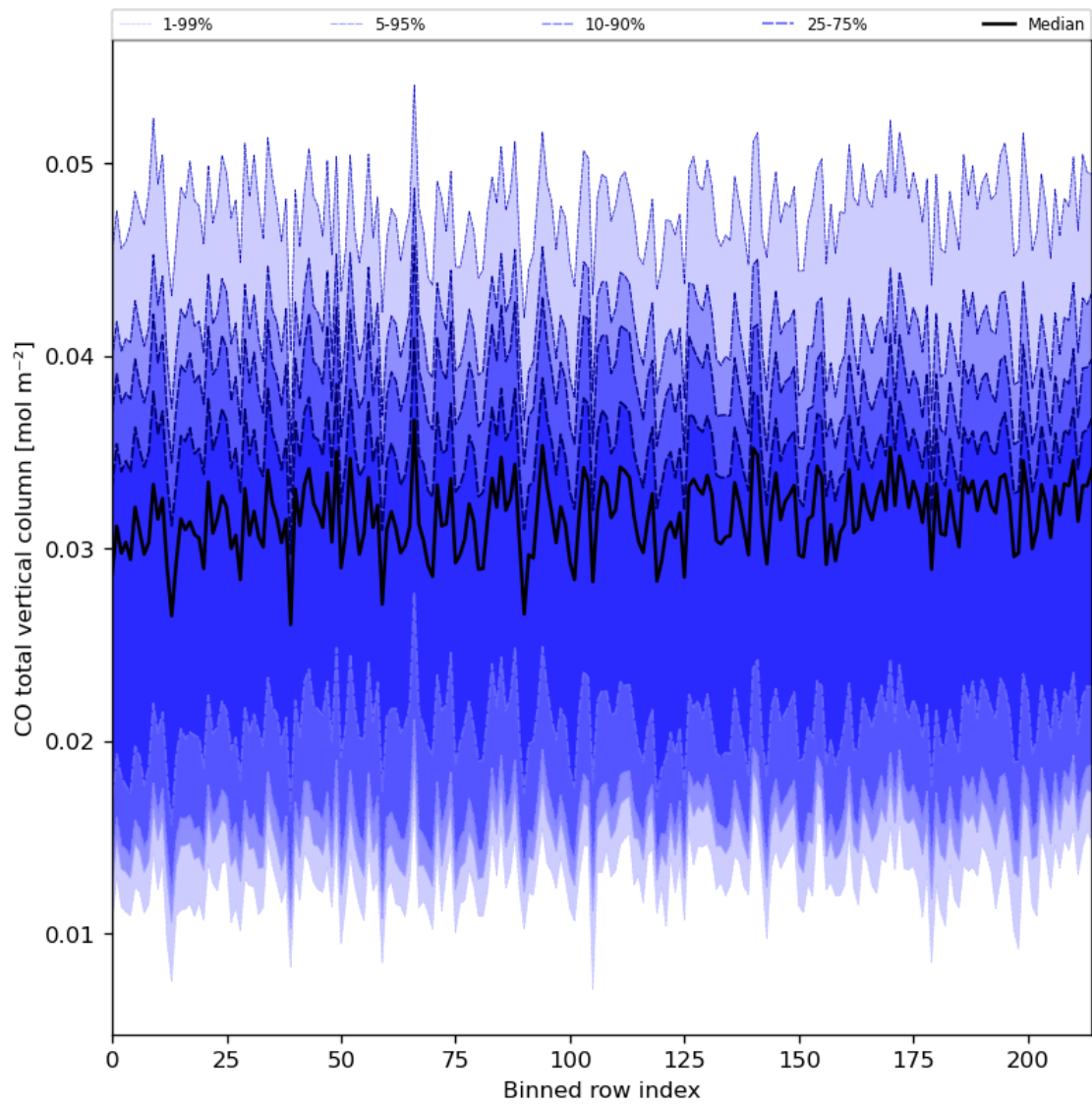
Figure 26: Along track statistics of “CO total vertical column” for 2024-04-23 to 2024-04-25
