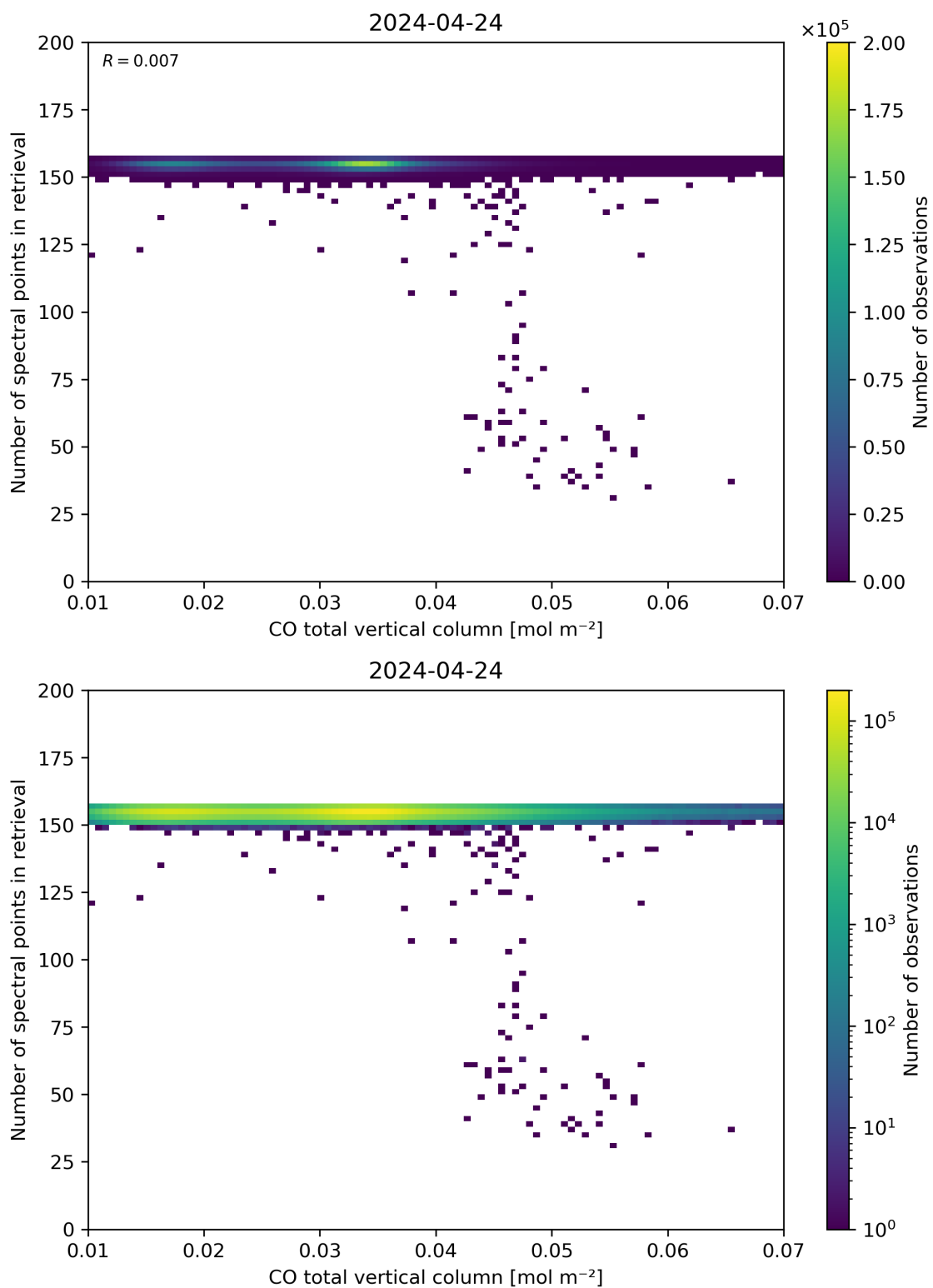
Figure 43: Scatter density plot of “CO total vertical column” against “Number of spectral points in retrieval” for 2024-04-23 to 2024-04-25.
