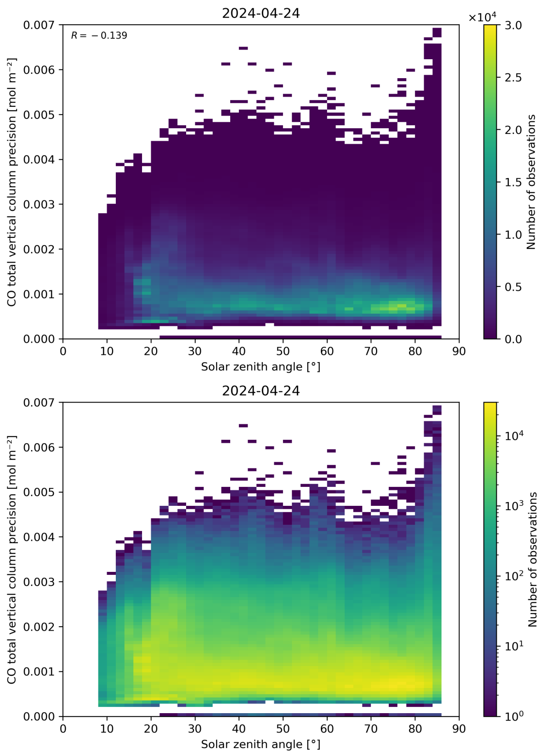
Figure 63: Scatter density plot of “Solar zenith angle” against “CO total vertical column precision” for 2024-04-23 to 2024-04-25.
