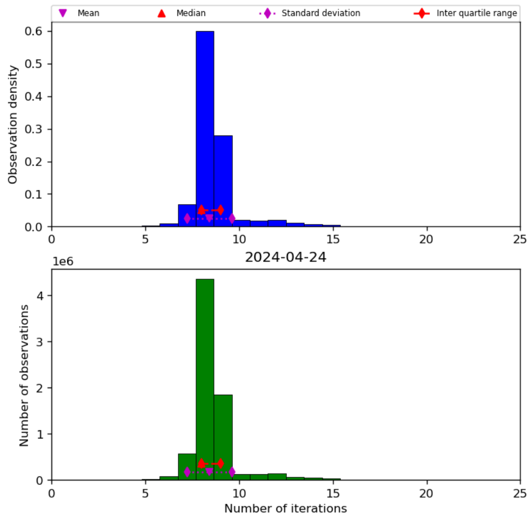
Figure 24: Histogram of “Number of iterations” for 2024-04-23 to 2024-04-25
