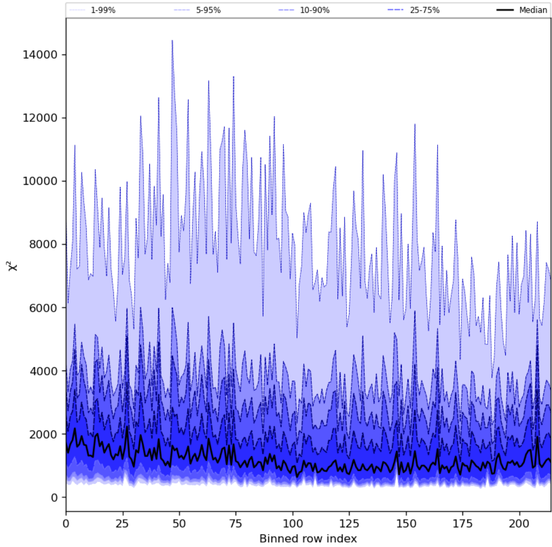
Figure 30: Along track statistics of “ \chi^2 ” for 2024-04-23 to 2024-04-25
