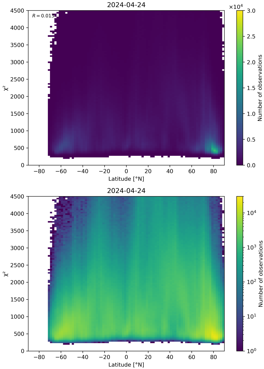
Figure 54: Scatter density plot of “Latitude” against “ \chi^2 ” for 2024-04-23 to 2024-04-25.
