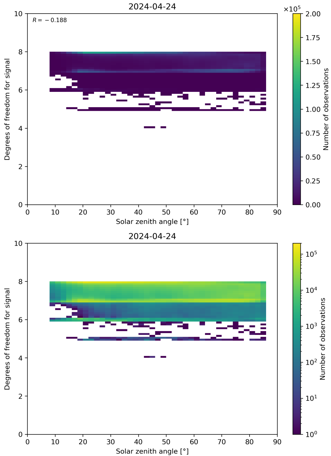
Figure 65: Scatter density plot of “Solar zenith angle” against “Degrees of freedom for signal” for 2024-04-23 to 2024-04-25.
