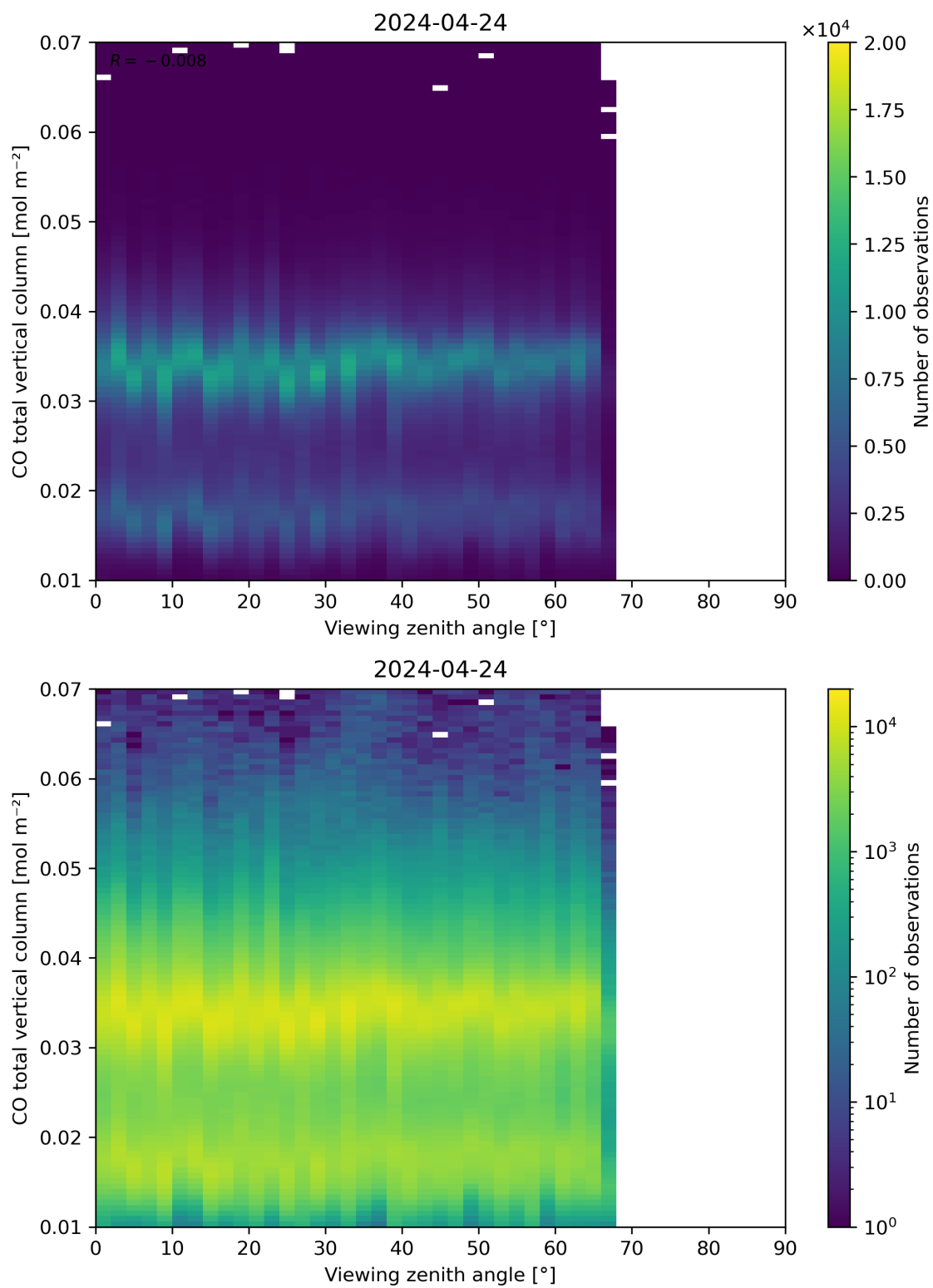
Figure 69: Scatter density plot of “Viewing zenith angle” against “CO total vertical column” for 2024-04-23 to 2024-04-25.
