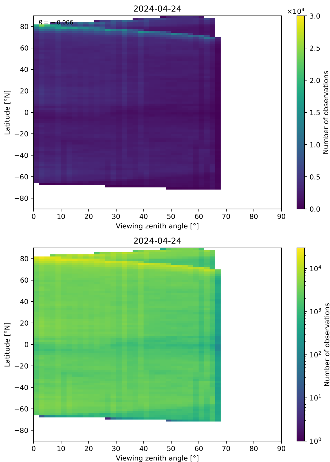
Figure 74: Scatter density plot of “Viewing zenith angle” against “Latitude” for 2024-04-23 to 2024-04-25.
