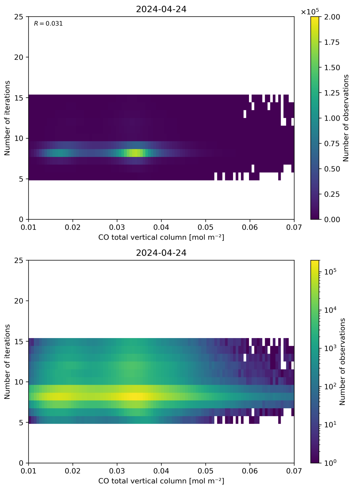
Figure 42: Scatter density plot of “CO total vertical column” against “Number of iterations” for 2024-04-23 to 2024-04-25.
