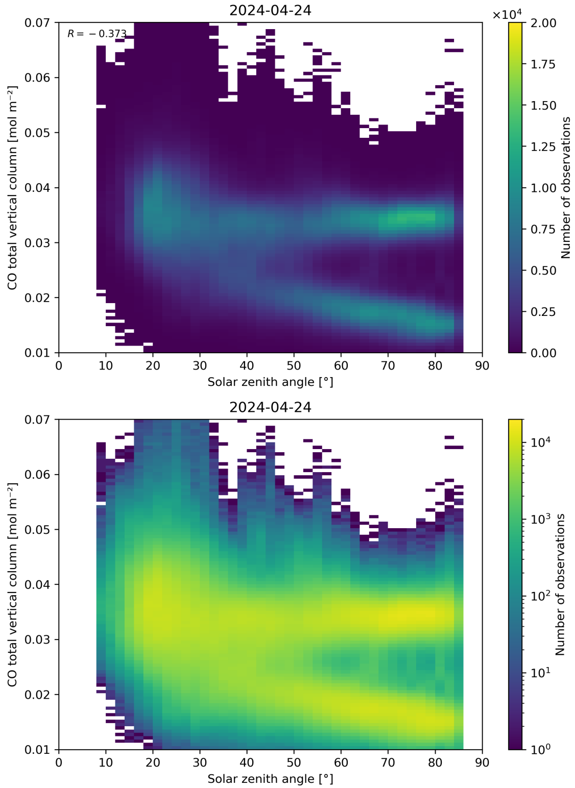
Figure 61: Scatter density plot of “Solar zenith angle” against “CO total vertical column” for 2024-04-23 to 2024-04-25.
