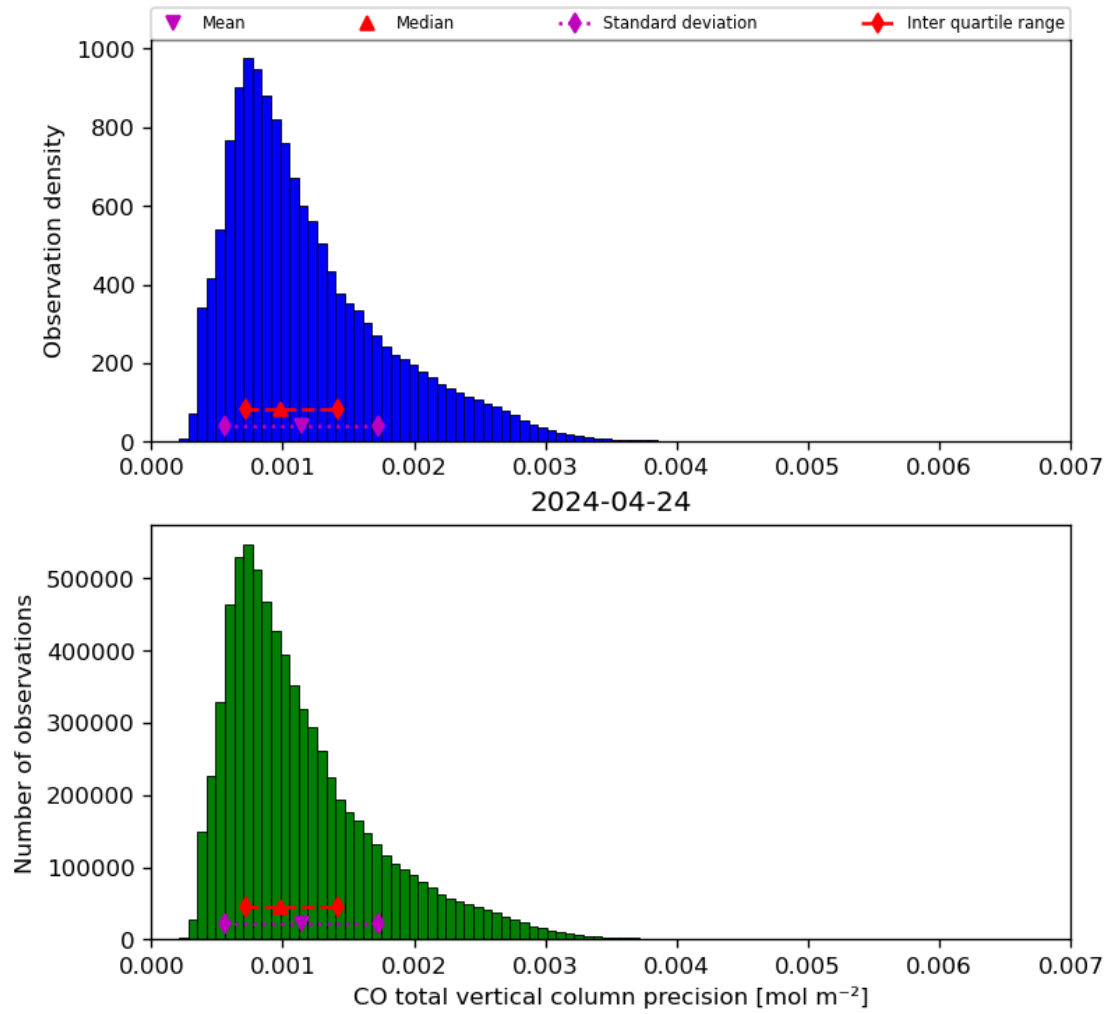
Figure 20: Histogram of “CO total vertical column precision” for 2024-04-23 to 2024-04-25
