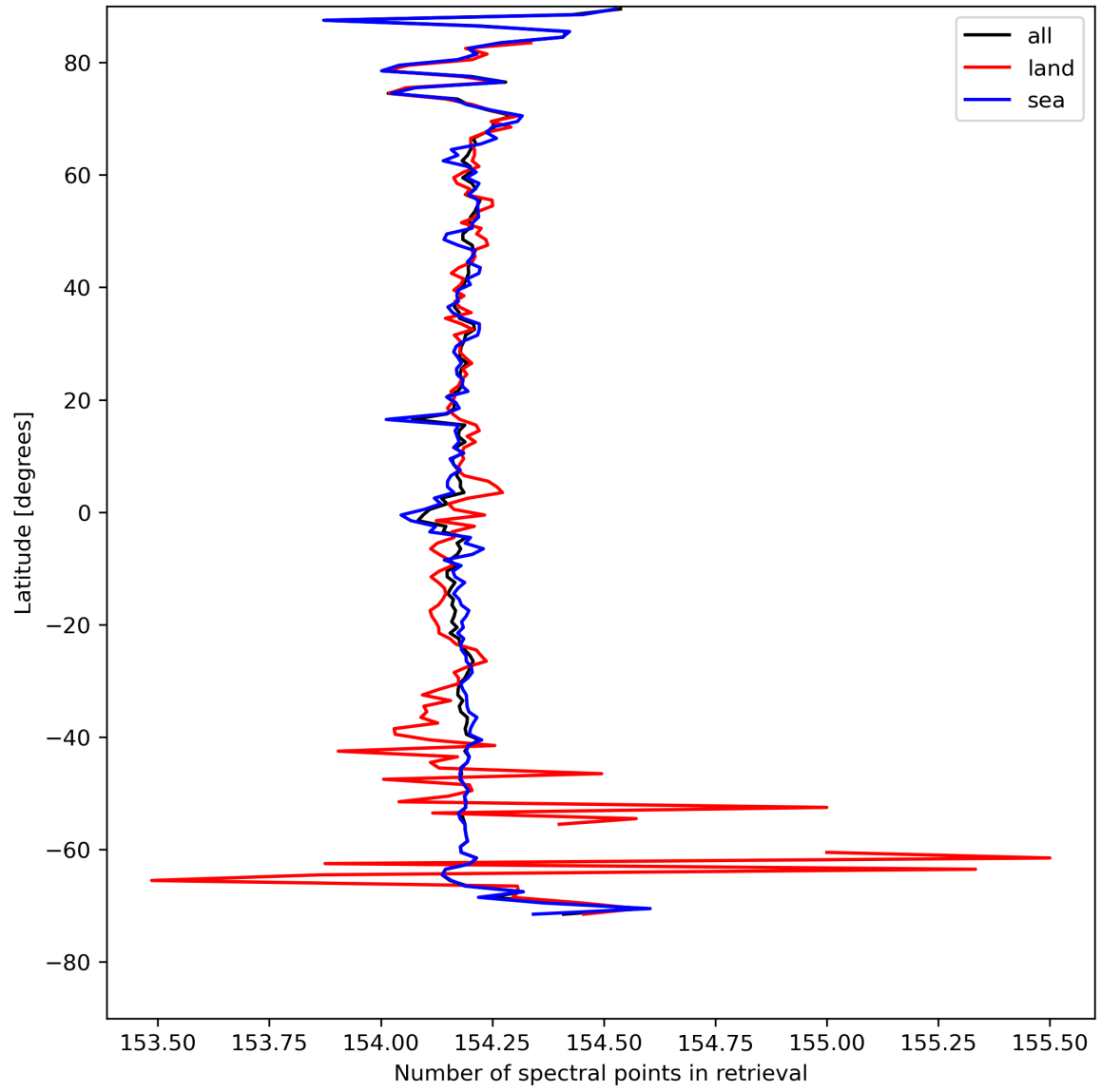
Figure 13: Zonal average of “Number of spectral points in retrieval” for 2024-04-23 to 2024-04-25.
