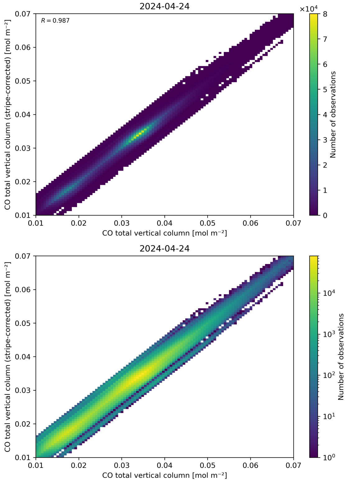
Figure 33: Scatter density plot of “CO total vertical column” against “CO total vertical column (stripe-corrected)” for 2024-04-23 to 2024-04-25.
