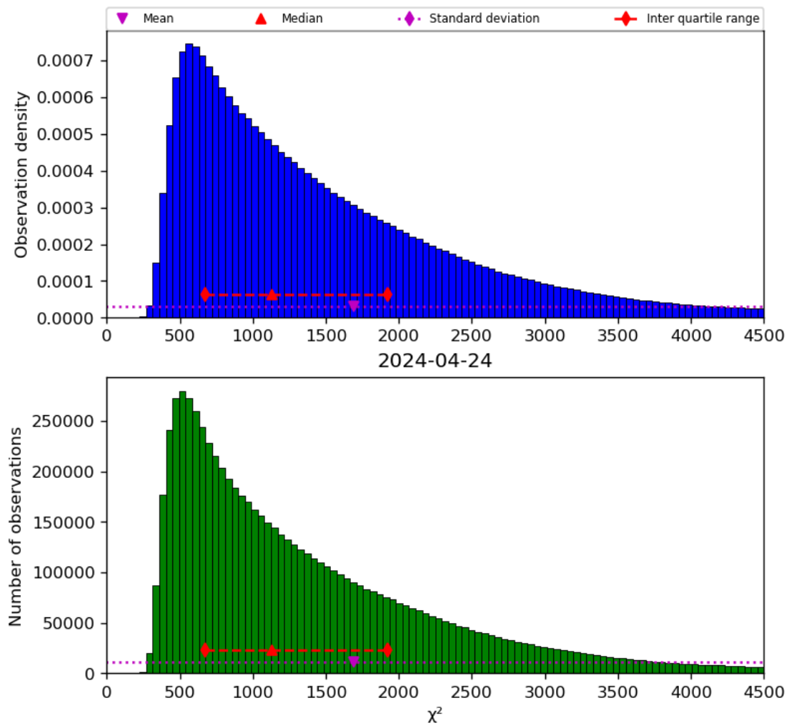
Figure 22: Histogram of “ \chi^2 ” for 2024-04-23 to 2024-04-25
