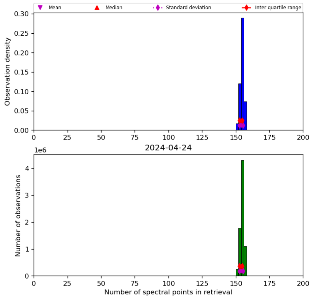
Figure 21: Histogram of “Number of spectral points in retrieval” for 2024-04-23 to 2024-04-25
