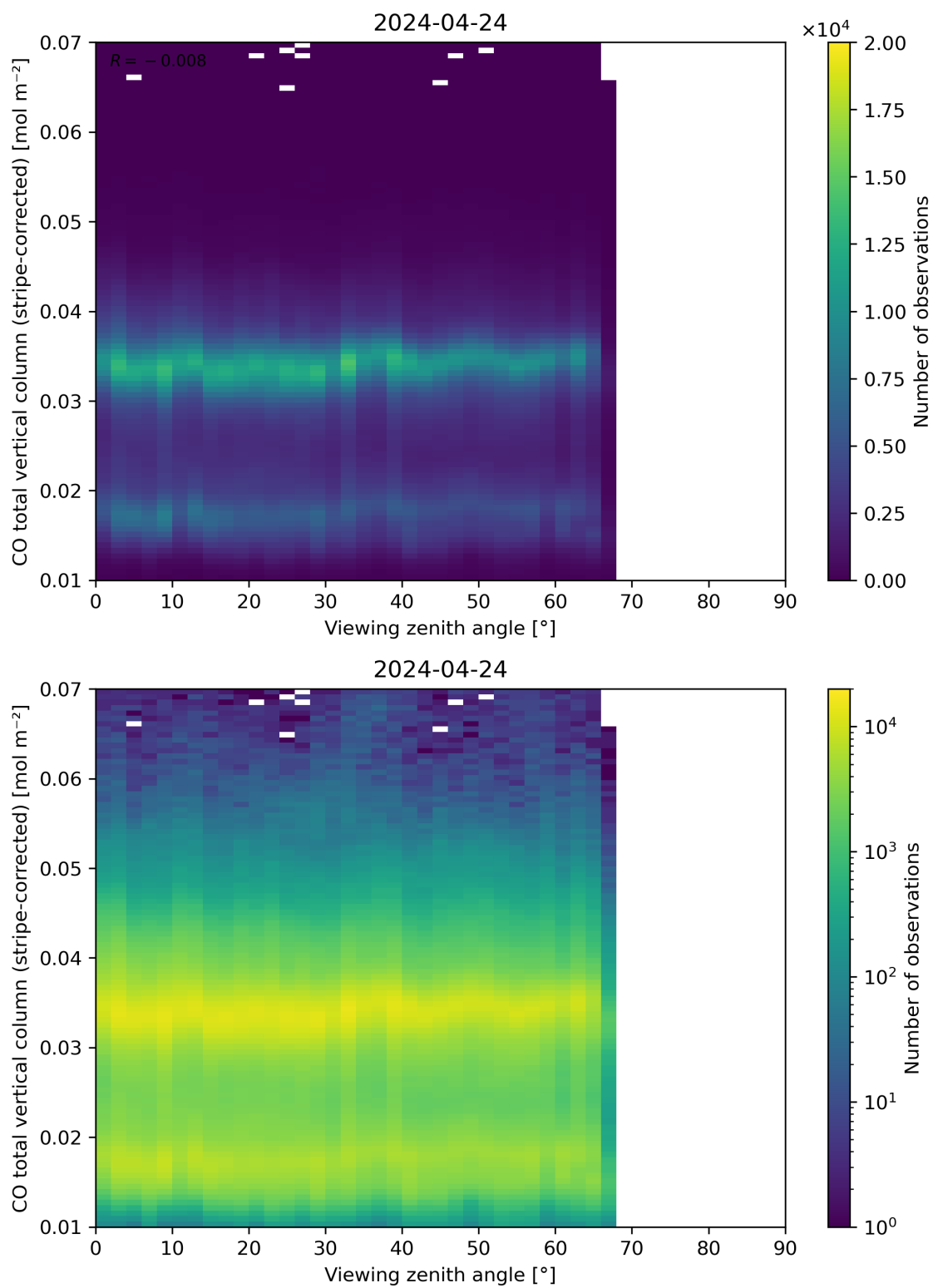
Figure 70: Scatter density plot of “Viewing zenith angle” against “CO total vertical column (stripe-corrected)” for 2024-04-23 to 2024-04-25.
