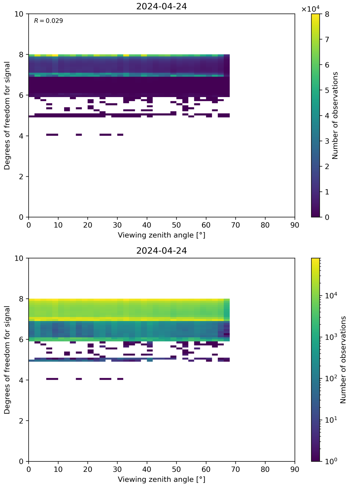
Figure 73: Scatter density plot of “Viewing zenith angle” against “Degrees of freedom for signal” for 2024-04-23 to 2024-04-25.
