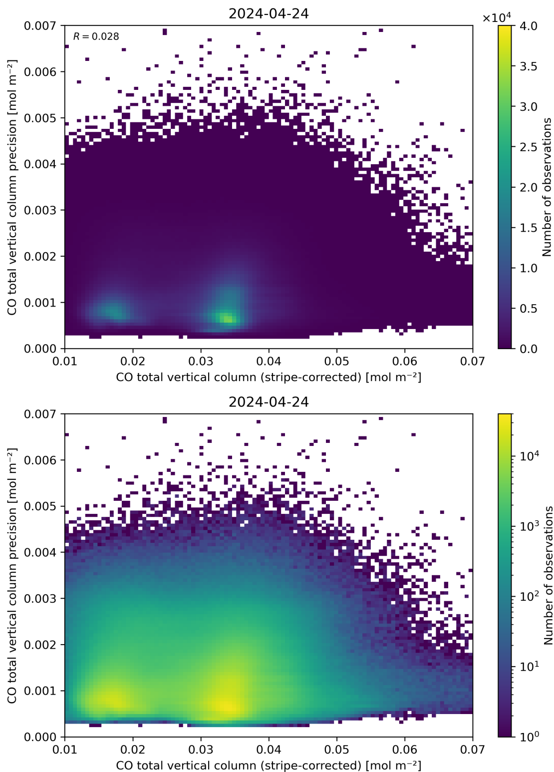
Figure 36: Scatter density plot of “CO total vertical column (stripe-corrected)” against “CO total vertical column precision” for 2024-04-23 to 2024-04-25.
