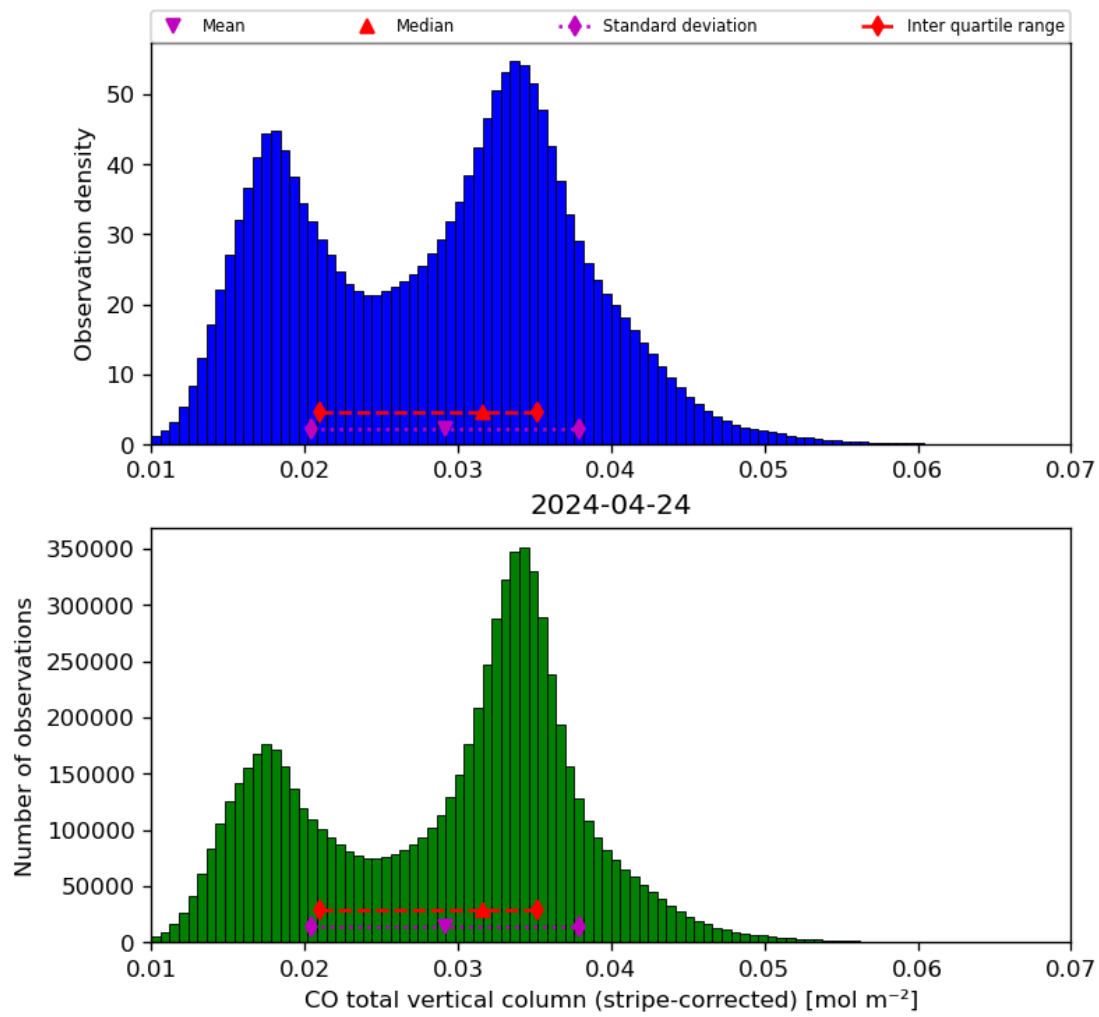
Figure 19: Histogram of “CO total vertical column (stripe-corrected)” for 2024-04-23 to 2024-04-25
