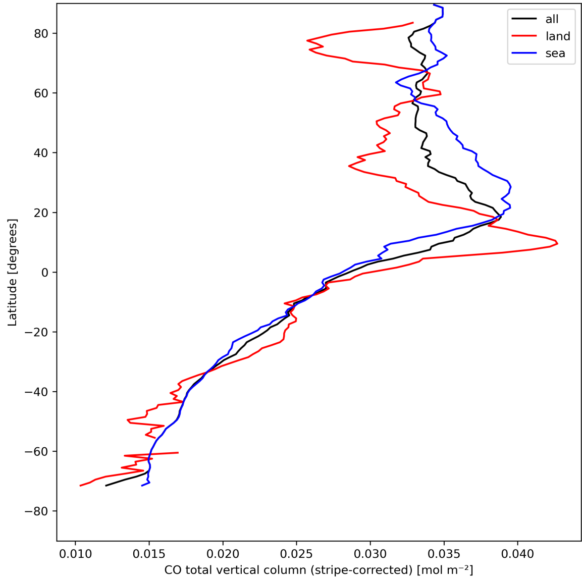
Figure 11: Zonal average of “CO total vertical column (stripe-corrected)” for 2024-04-23 to 2024-04-25.
