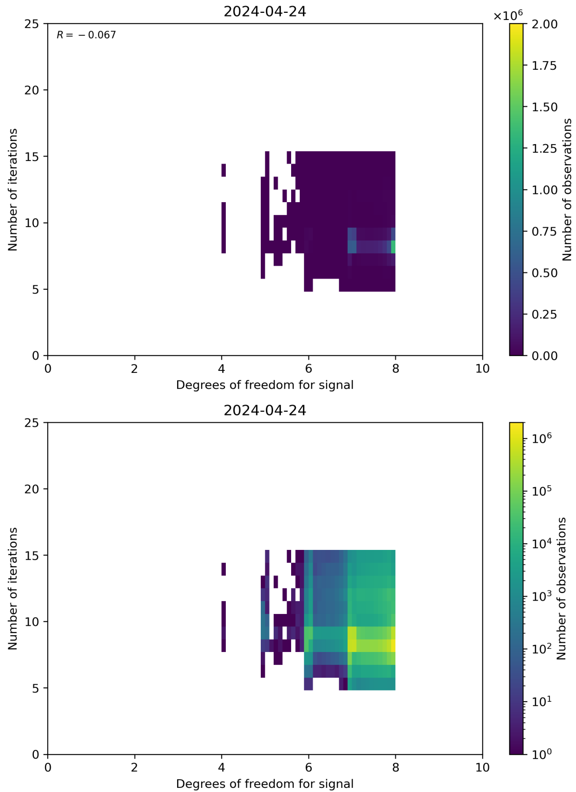
Figure 50: Scatter density plot of “Degrees of freedom for signal” against “Number of iterations” for 2024-04-23 to 2024-04-25.
