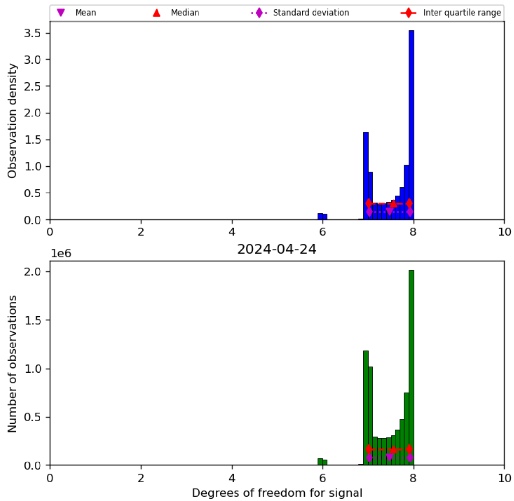
Figure 23: Histogram of “Degrees of freedom for signal” for 2024-04-23 to 2024-04-25
