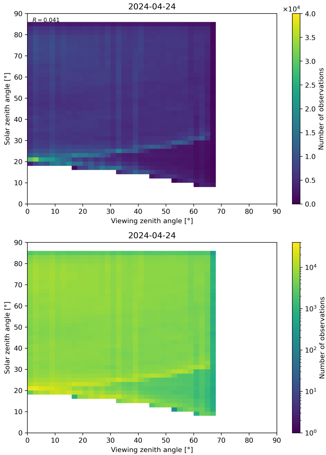
Figure 77: Scatter density plot of “Viewing zenith angle” against “Solar zenith angle” for 2024-04-23 to 2024-04-25.
