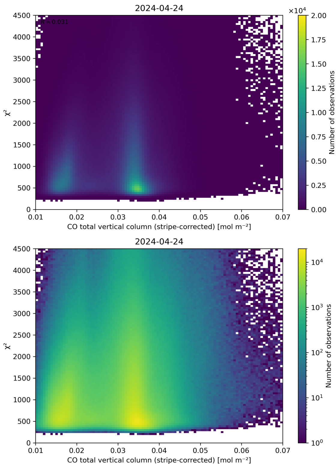
Figure 37: Scatter density plot of “CO total vertical column (stripe-corrected)” against “ \chi^2 ” for 2024-04-23 to 2024-04-25.
