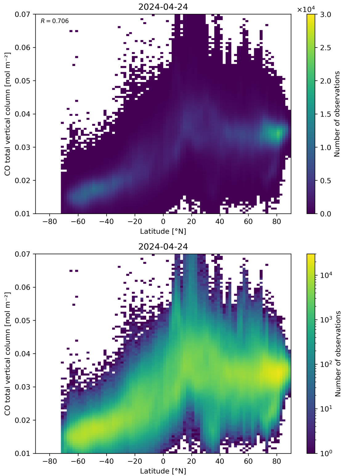
Figure 51: Scatter density plot of “Latitude” against “CO total vertical column” for 2024-04-23 to 2024-04-25.
