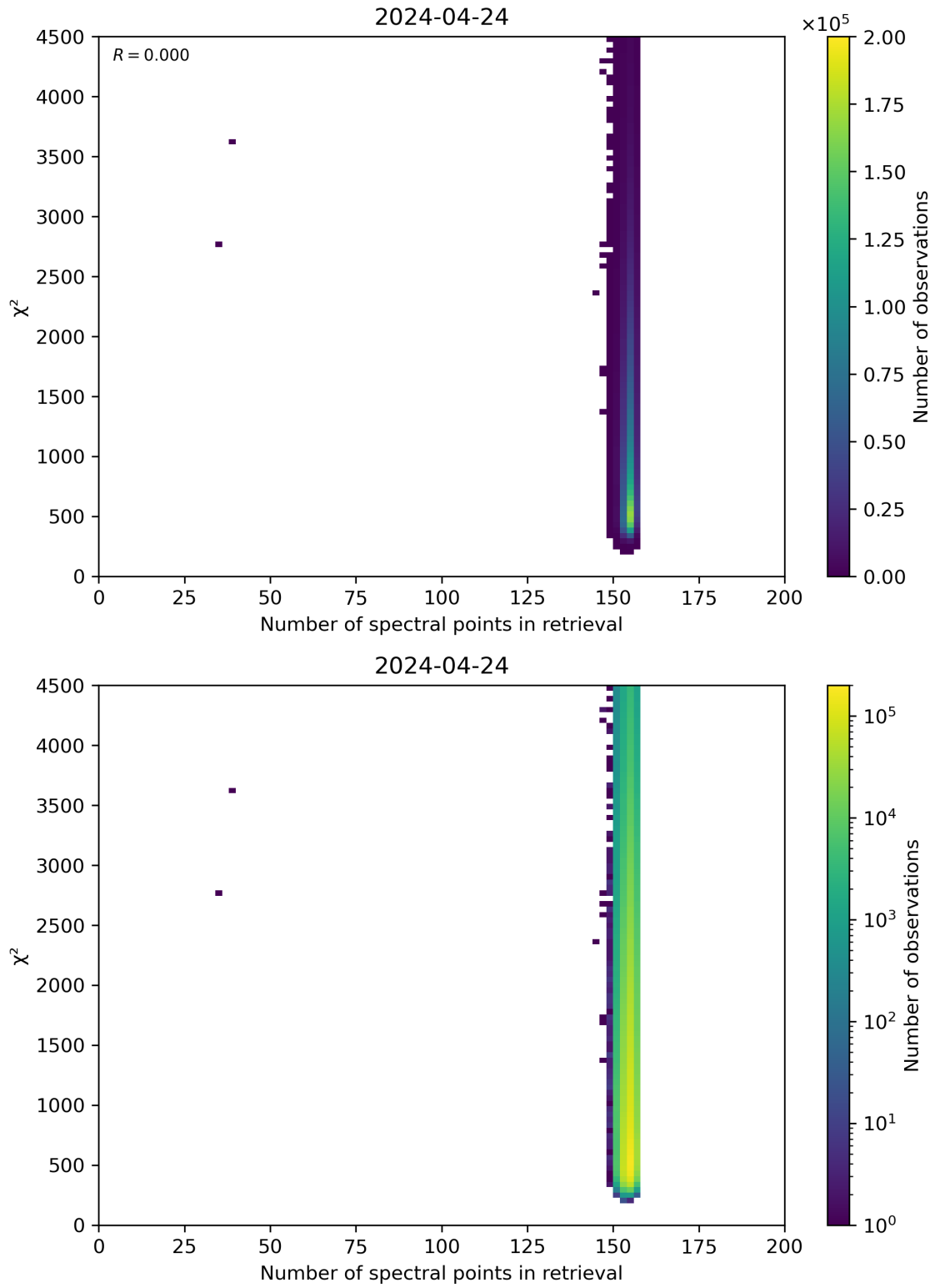
Figure 58: Scatter density plot of “Number of spectral points in retrieval” against “ \chi^2 ” for 2024-04-23 to 2024-04-25.
