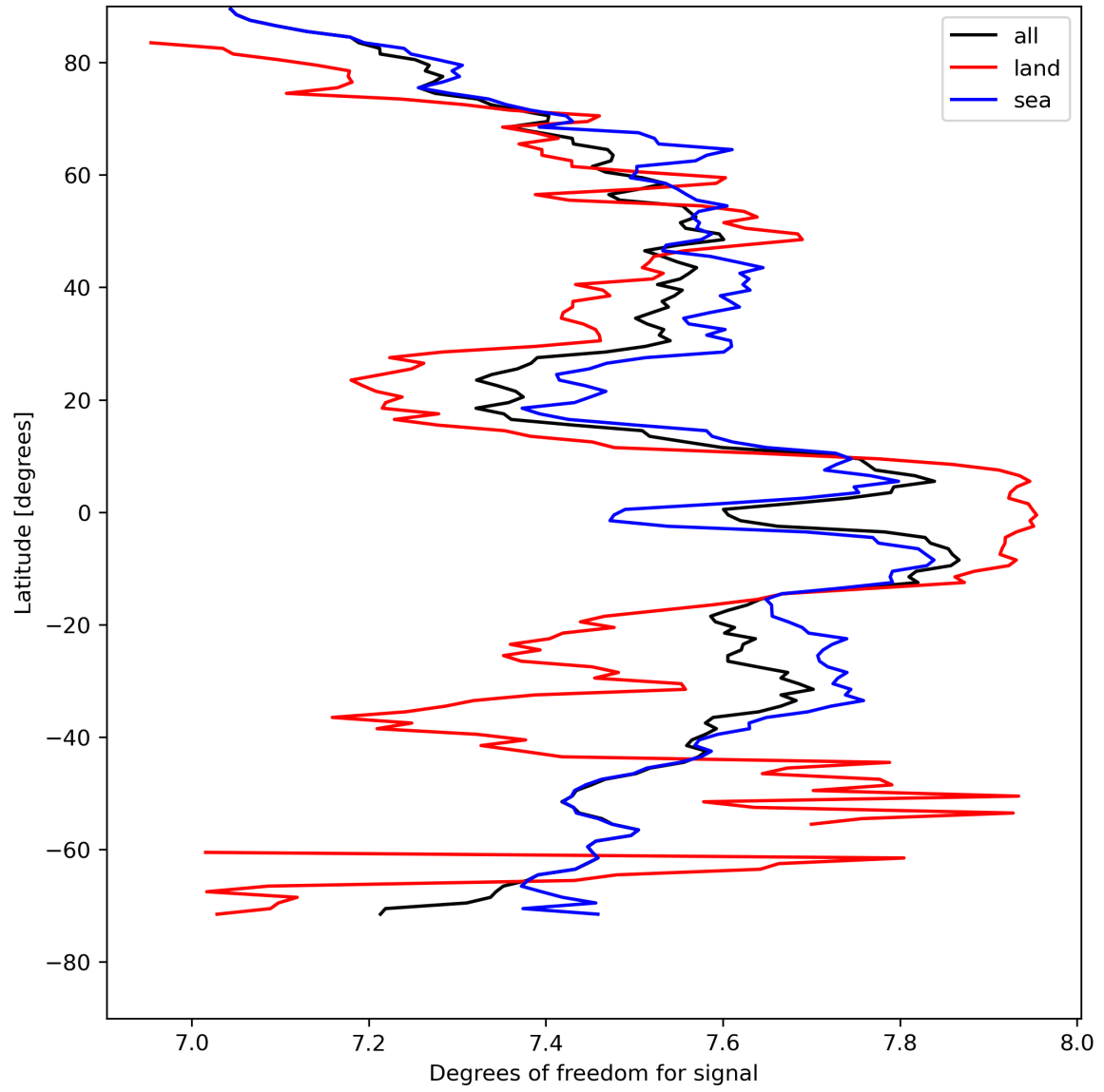
Figure 15: Zonal average of “Degrees of freedom for signal” for 2024-04-23 to 2024-04-25.
