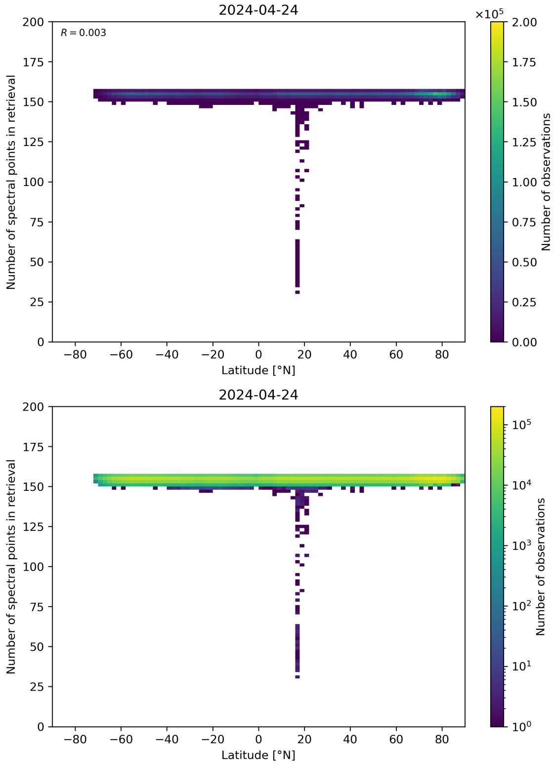
Figure 57: Scatter density plot of “Latitude” against “Number of spectral points in retrieval” for 2024-04-23 to 2024-04-25.
