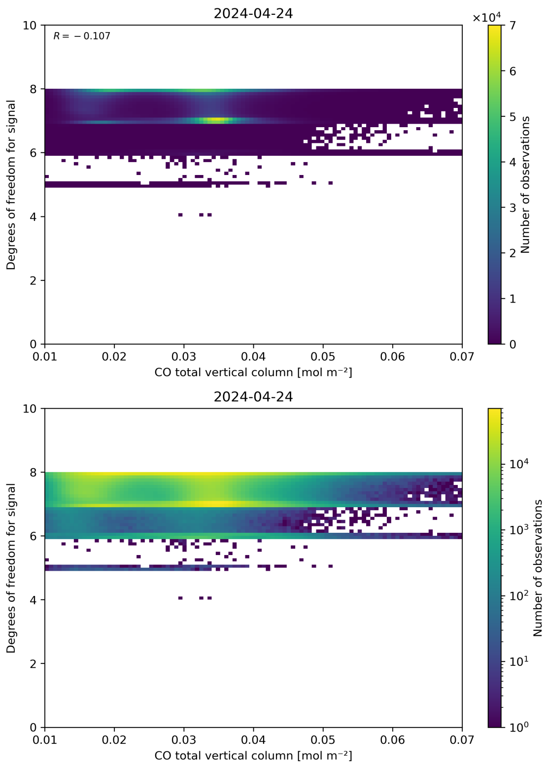
Figure 41: Scatter density plot of “CO total vertical column” against “Degrees of freedom for signal” for 2024-04-23 to 2024-04-25.
