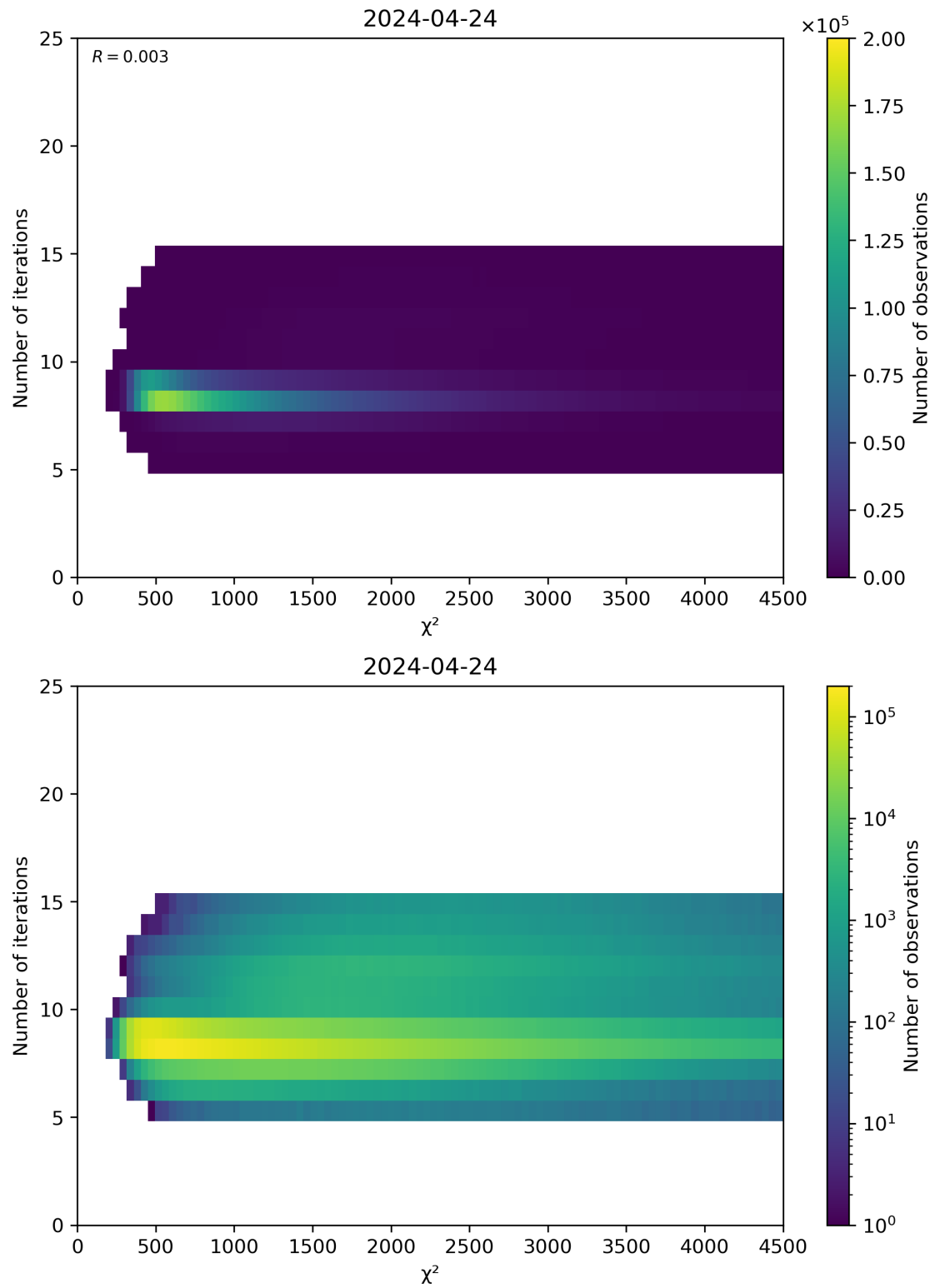
Figure 49: Scatter density plot of “ \chi^2 ” against “Number of iterations” for 2024-04-23 to 2024-04-25.
