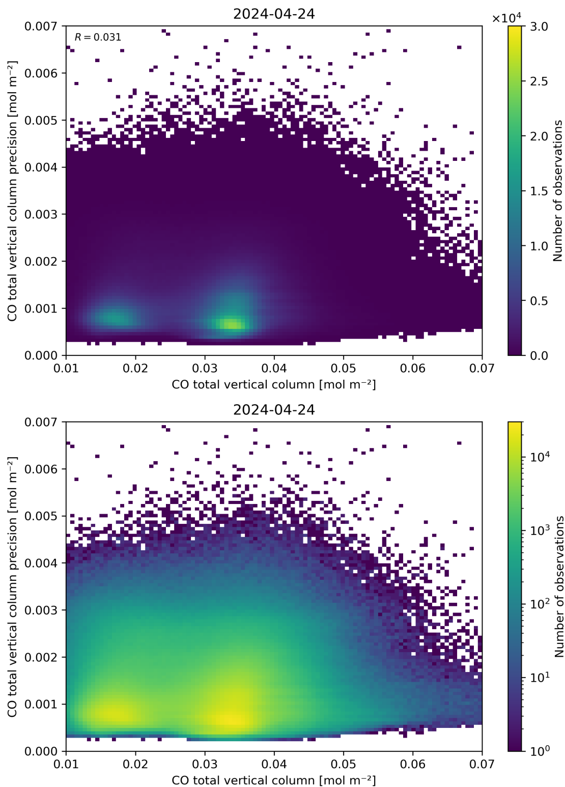
Figure 34: Scatter density plot of “CO total vertical column” against “CO total vertical column precision” for 2024-04-23 to 2024-04-25.
