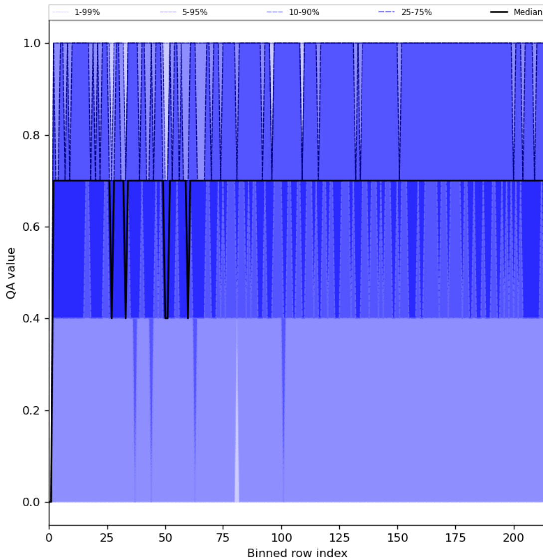
Figure 25: Along track statistics of “QA value” for 2024-04-23 to 2024-04-25
