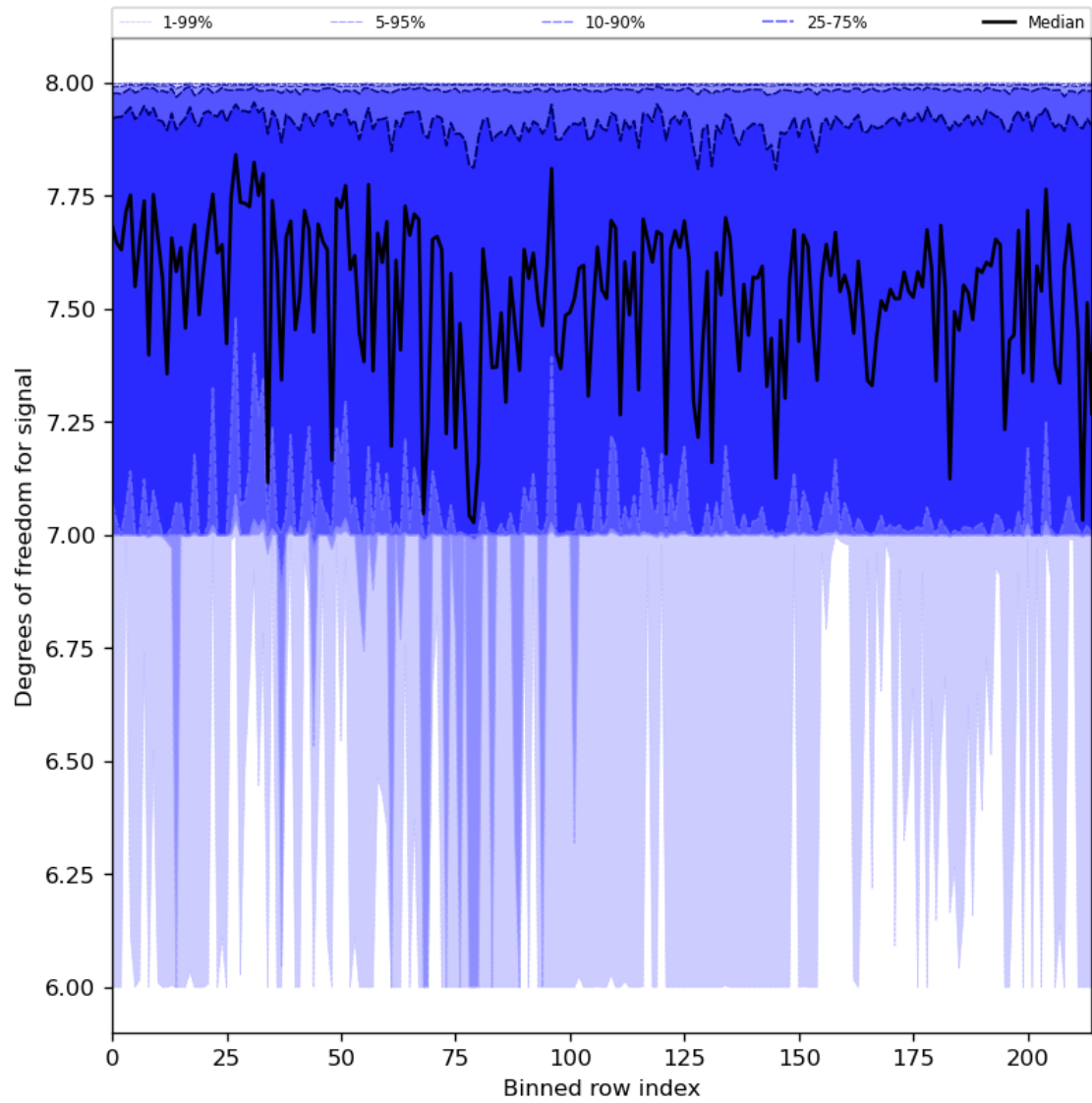
Figure 31: Along track statistics of “Degrees of freedom for signal” for 2024-04-23 to 2024-04-25
