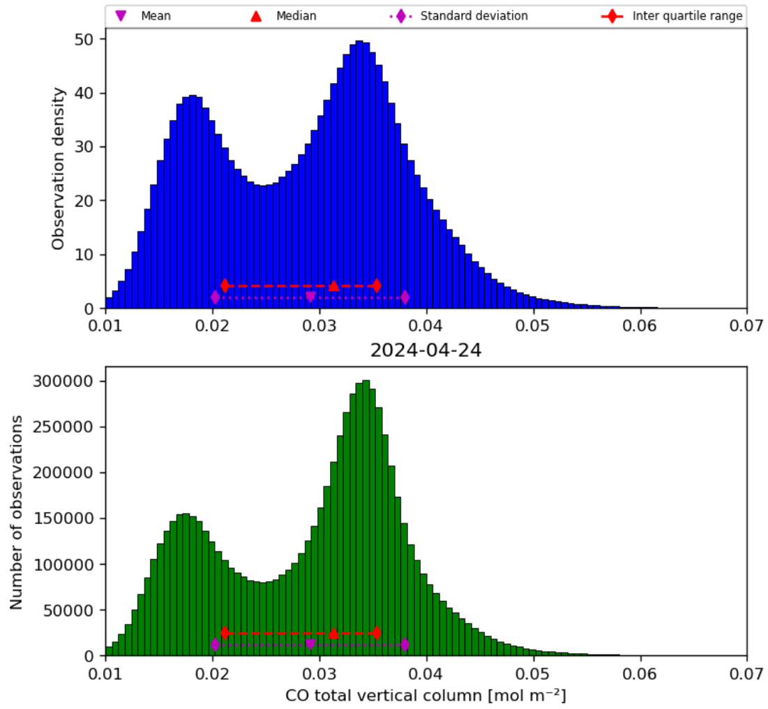
Figure 18: Histogram of “CO total vertical column” for 2024-04-23 to 2024-04-25
