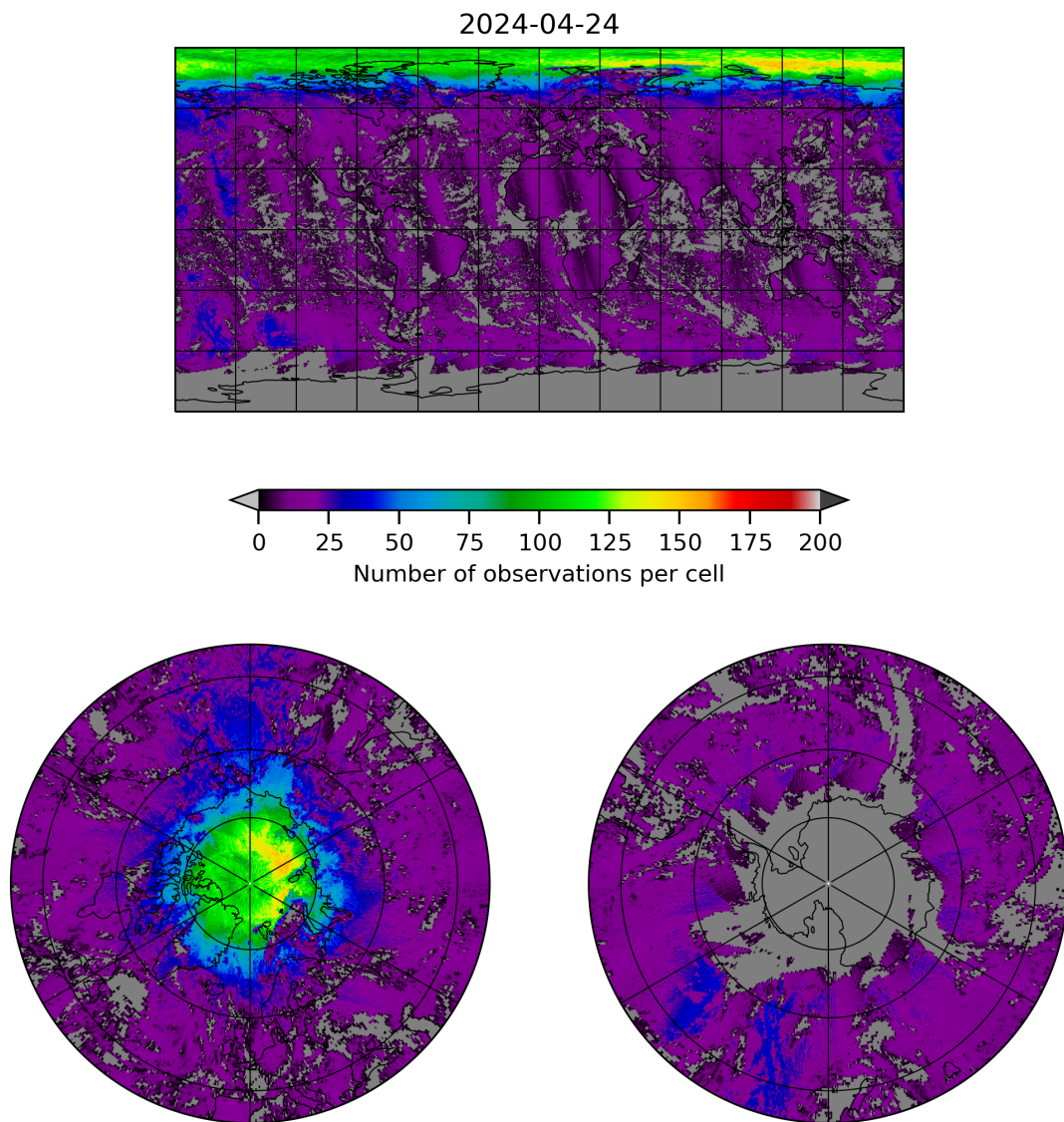
Figure 8: Map of the number of observations for 2024-04-23 to 2024-04-25
