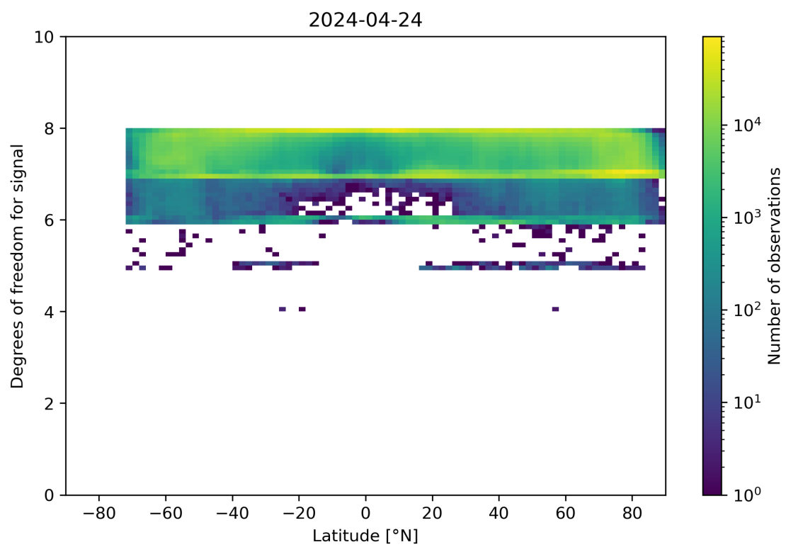
Figure 55: Scatter density plot of “Latitude” against “Degrees of freedom for signal” for 2024-04-23 to 2024-04-25.
