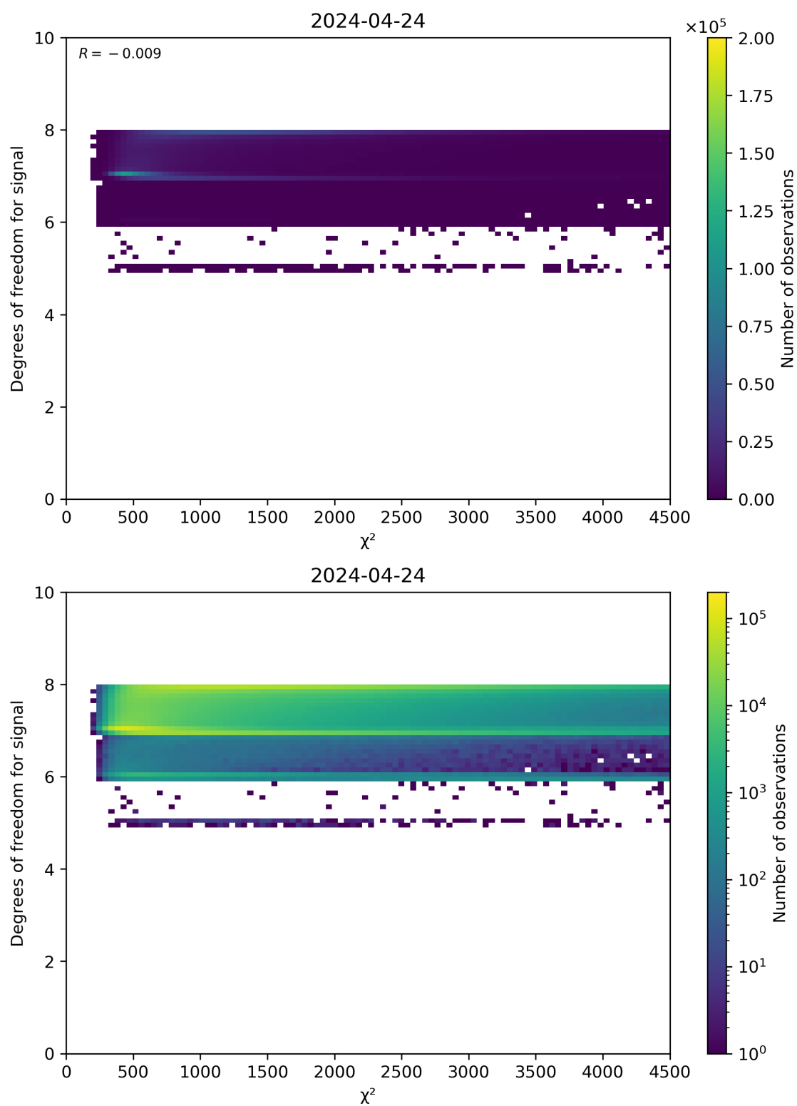
Figure 48: Scatter density plot of “ \chi^2 ” against “Degrees of freedom for signal” for 2024-04-23 to 2024-04-25.
