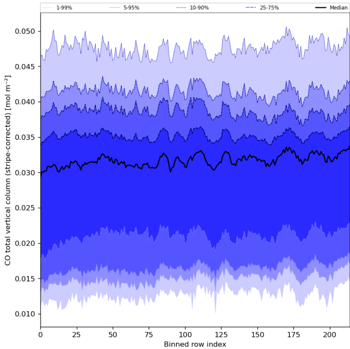
Figure 27: Along track statistics of “CO total vertical column (stripe-corrected)” for 2024-04-23 to 2024-04-25
