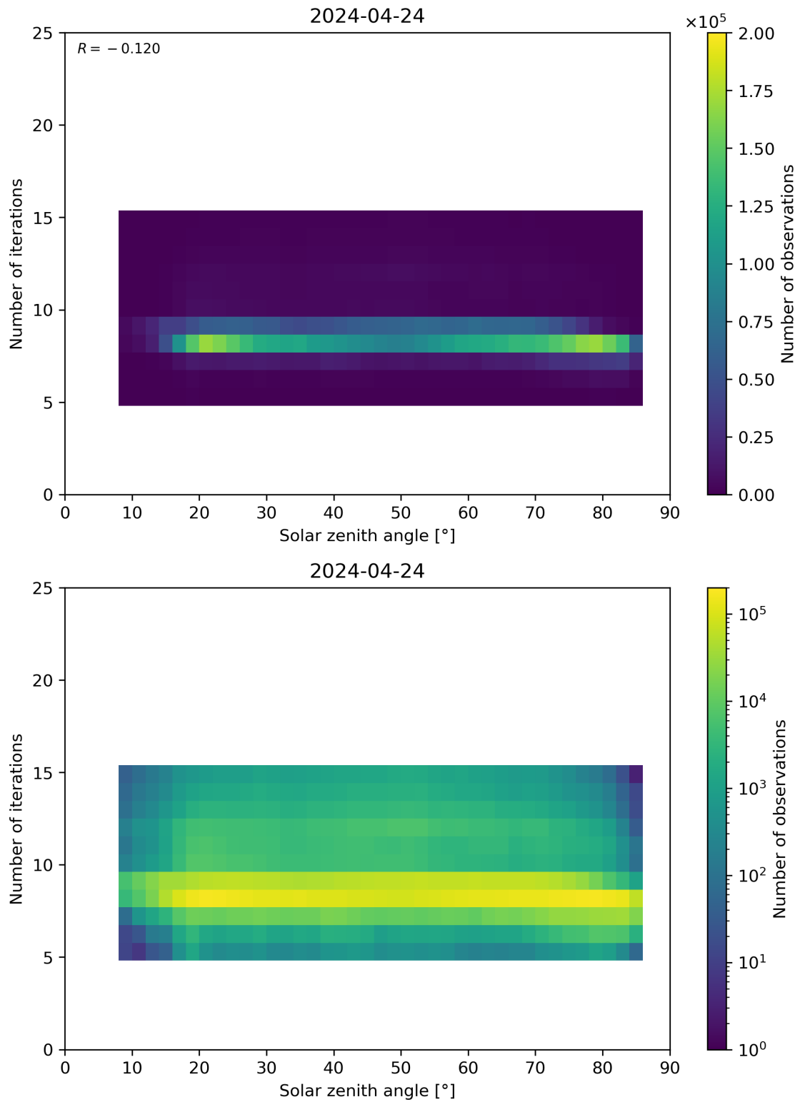
Figure 67: Scatter density plot of “Solar zenith angle” against “Number of iterations” for 2024-04-23 to 2024-04-25.
