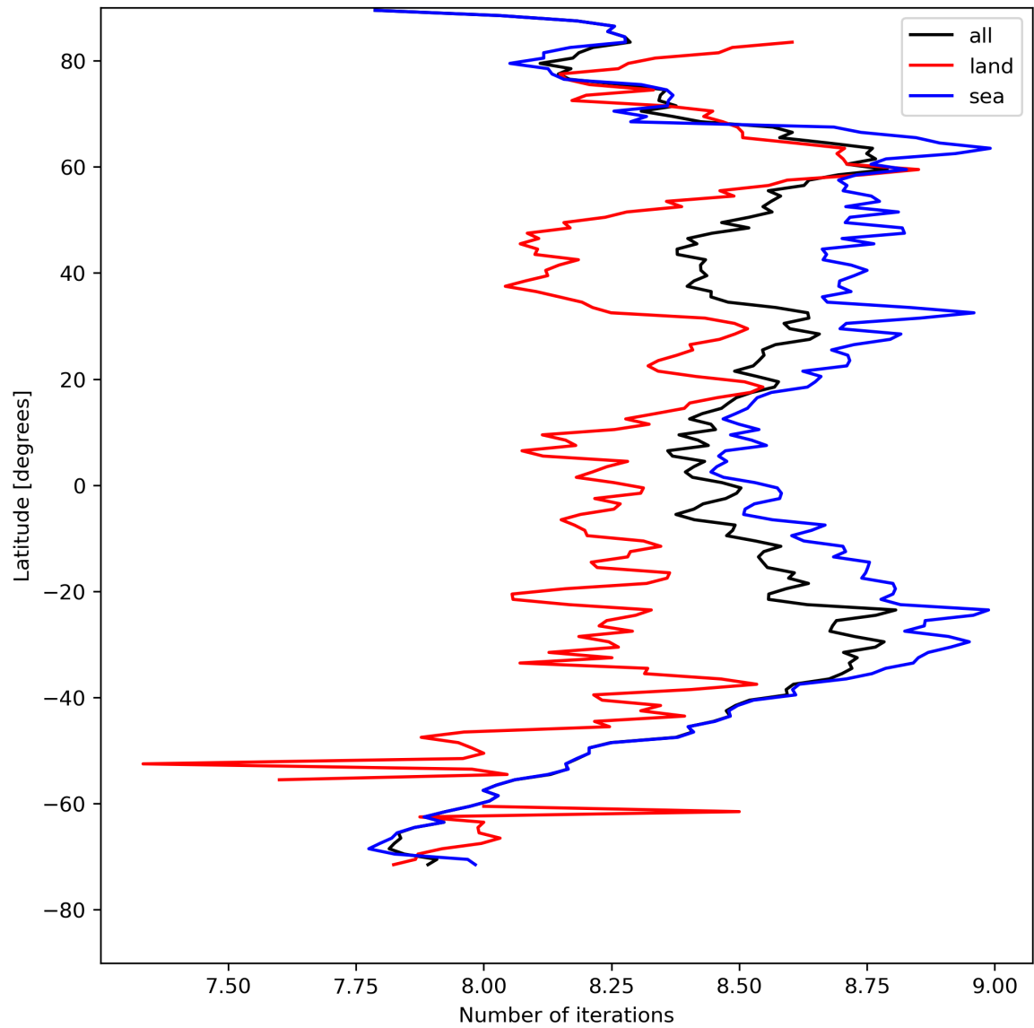
Figure 16: Zonal average of “Number of iterations” for 2024-04-23 to 2024-04-25.
