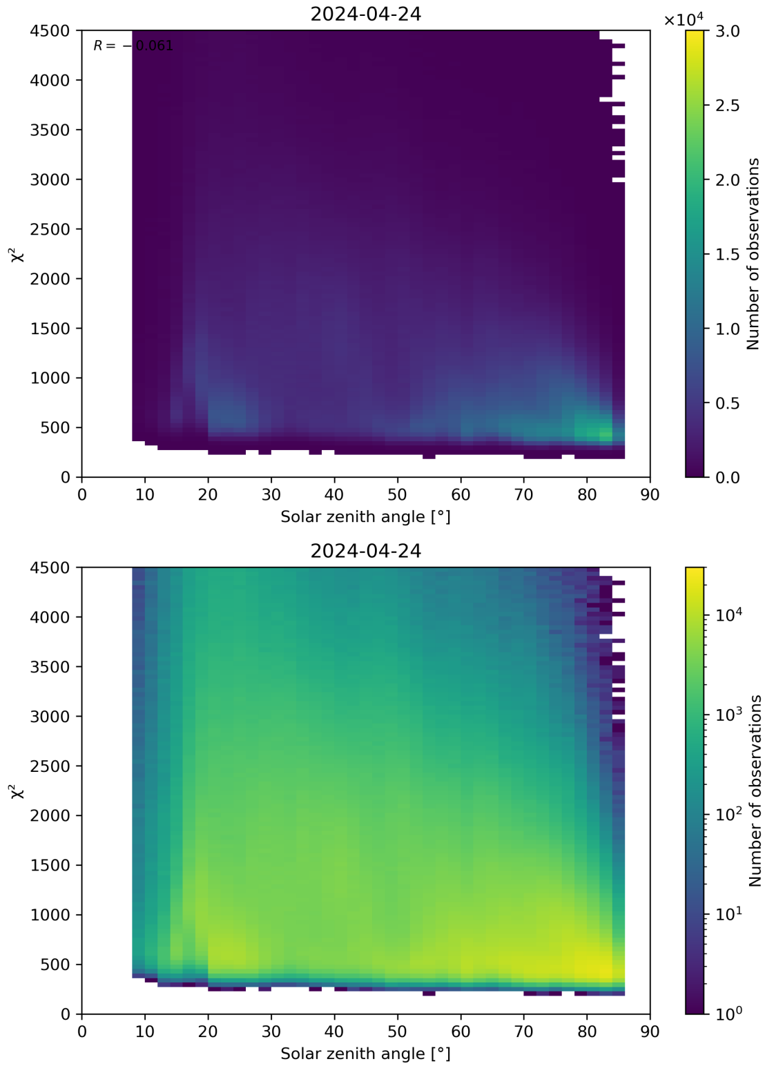
Figure 64: Scatter density plot of “Solar zenith angle” against “ \chi^2 ” for 2024-04-23 to 2024-04-25.
