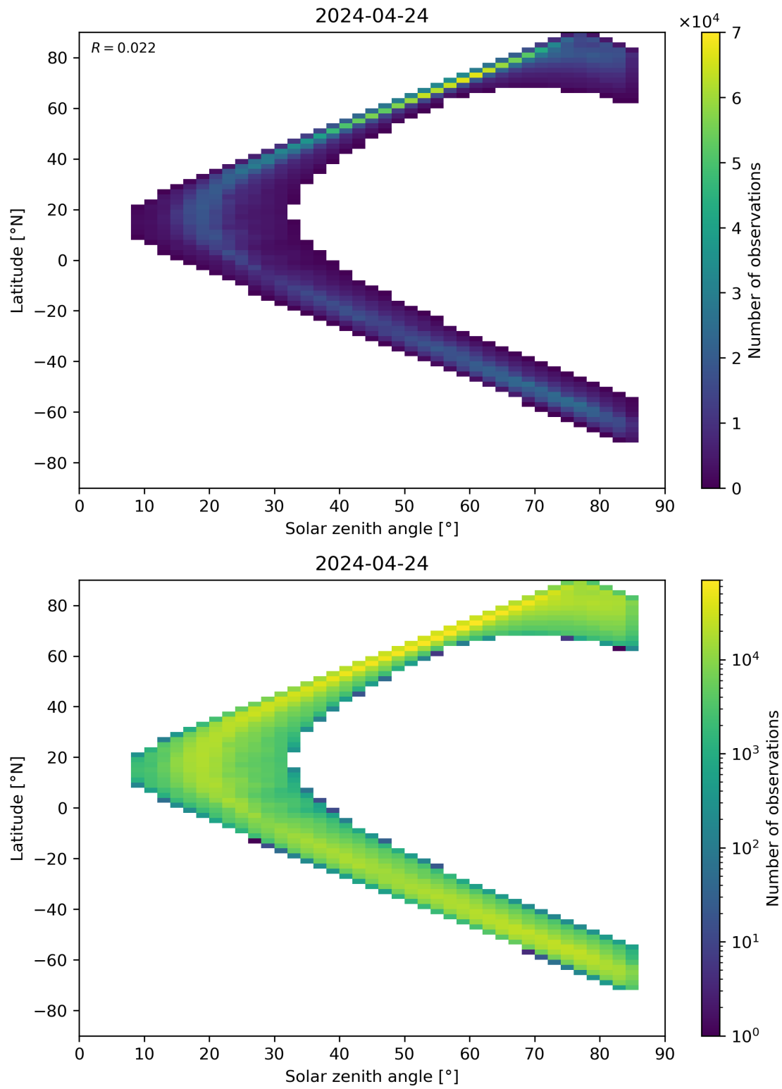
Figure 66: Scatter density plot of “Solar zenith angle” against “Latitude” for 2024-04-23 to 2024-04-25.
