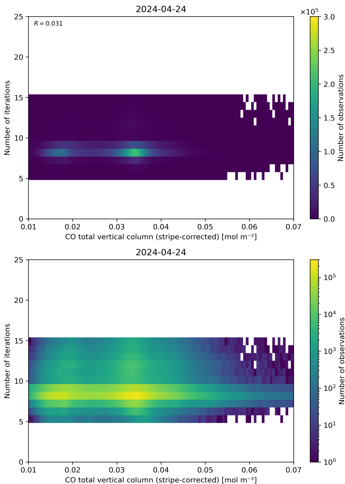
Figure 39: Scatter density plot of “CO total vertical column (stripe-corrected)” against “Number of iterations” for 2024-04-23 to 2024-04-25.
