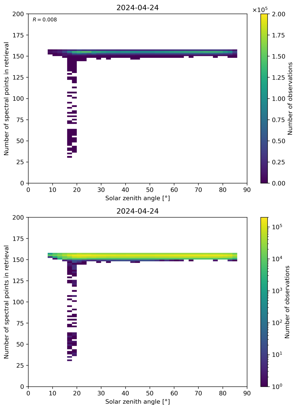
Figure 68: Scatter density plot of “Solar zenith angle” against “Number of spectral points in retrieval” for 2024-04-23 to 2024-04-25.
