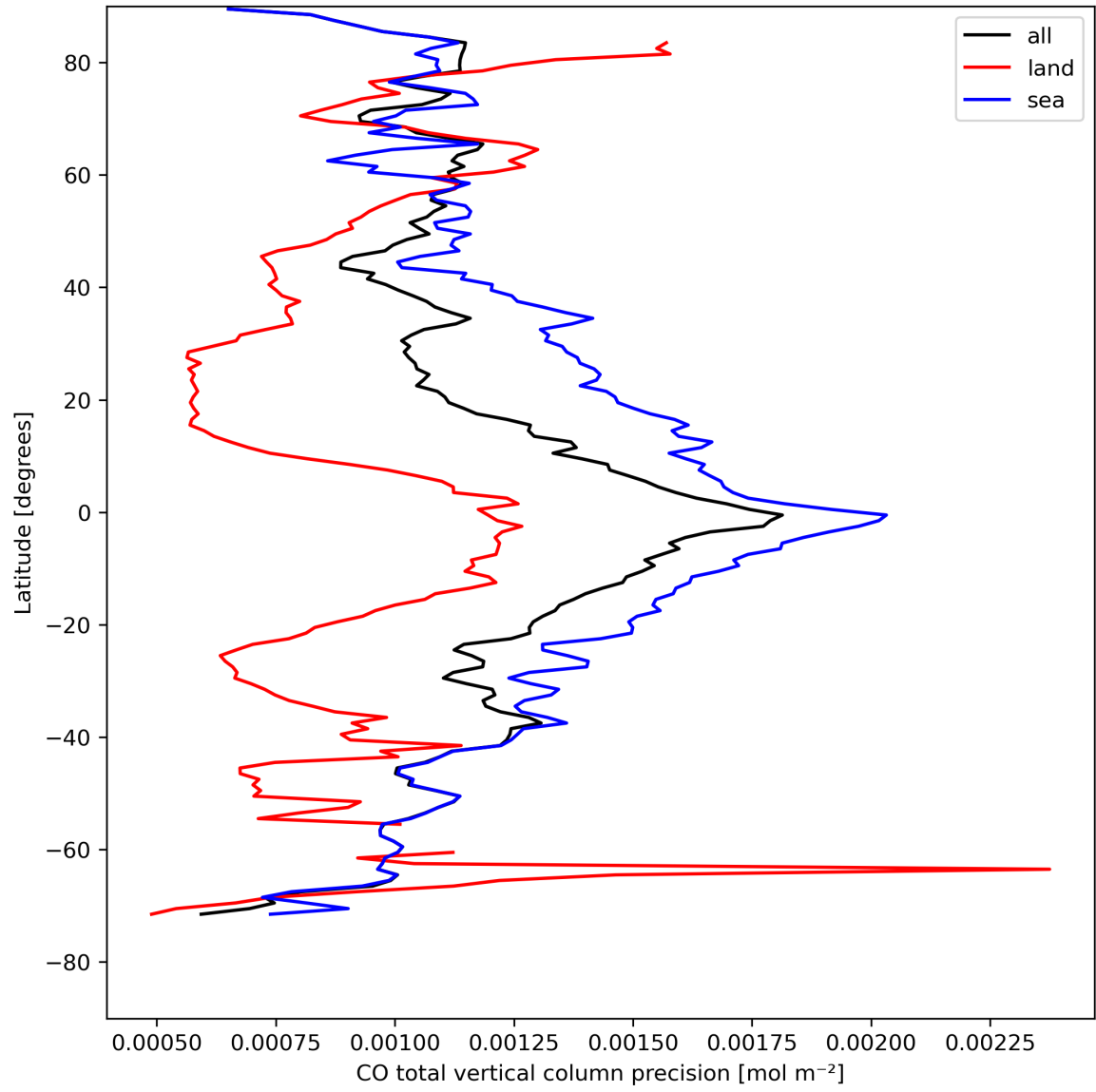
Figure 12: Zonal average of “CO total vertical column precision” for 2024-04-23 to 2024-04-25.
