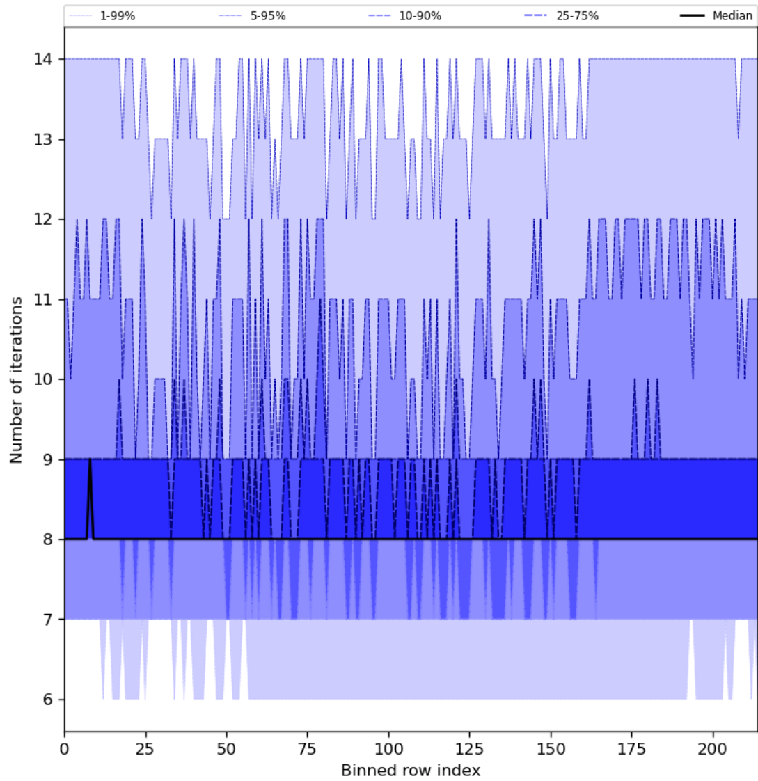
Figure 32: Along track statistics of “Number of iterations” for 2024-04-23 to 2024-04-25
