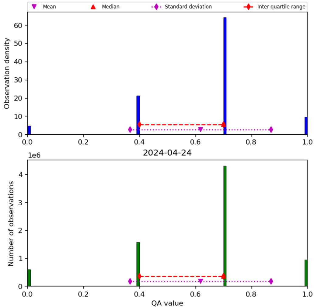
Figure 17: Histogram of “QA value” for 2024-04-23 to 2024-04-25
