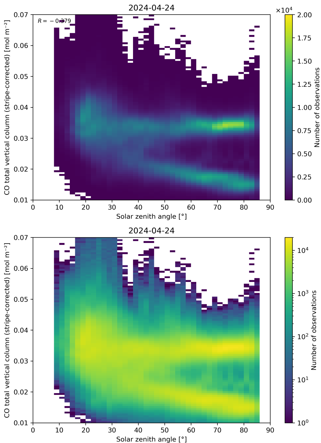
Figure 62: Scatter density plot of “Solar zenith angle” against “CO total vertical column (stripe-corrected)” for 2024-04-23 to 2024-04-25.
