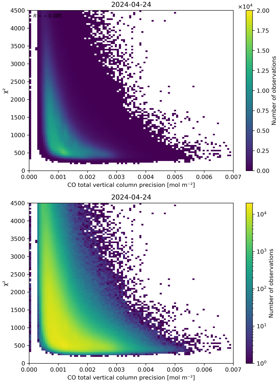
Figure 44: Scatter density plot of “CO total vertical column precision” against “ \chi^2 ” for 2024-04-23 to 2024-04-25.
