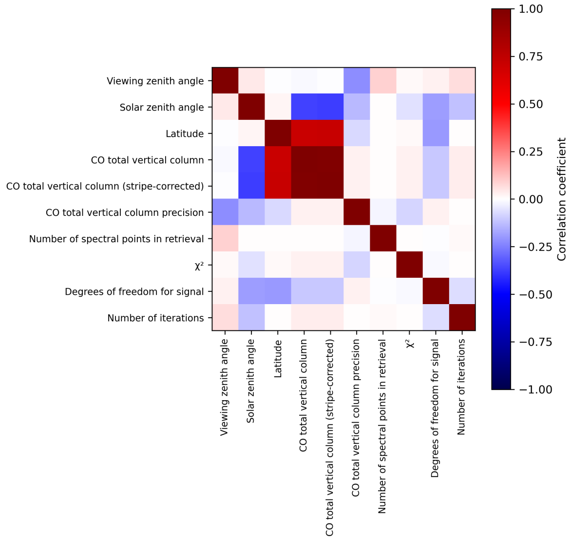
Figure 2: Map of correlation matrix for 2024-04-23 to 2024-04-25.
