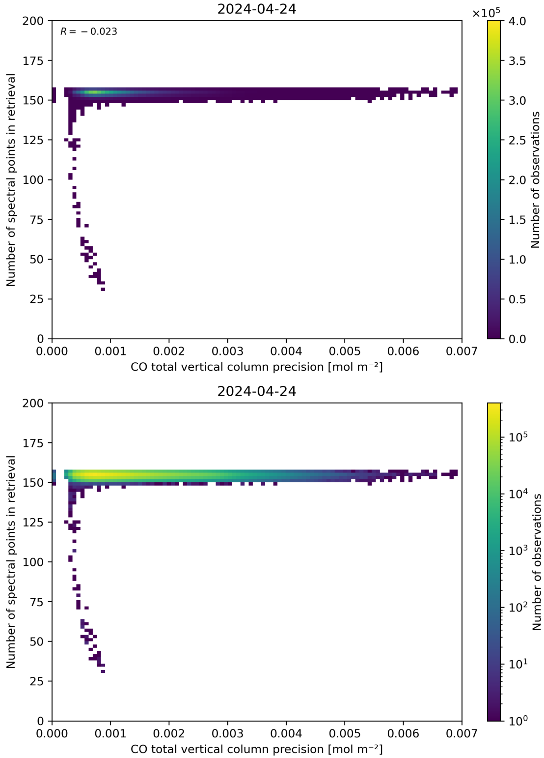
Figure 47: Scatter density plot of “CO total vertical column precision” against “Number of spectral points in retrieval” for 2024-04-23 to 2024-04-25.
