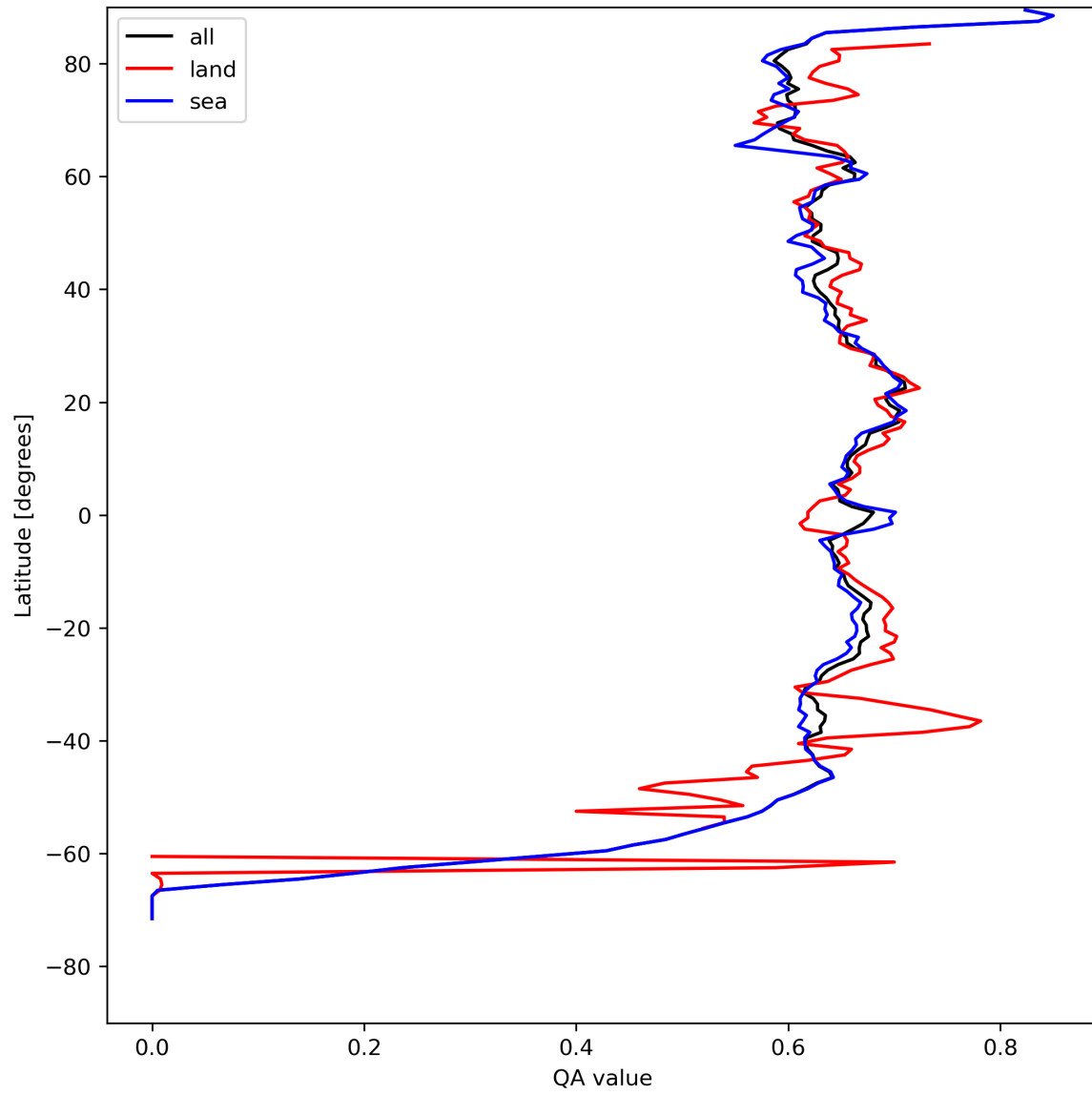
Figure 9: Zonal average of “QA value” for 2024-04-23 to 2024-04-25.
