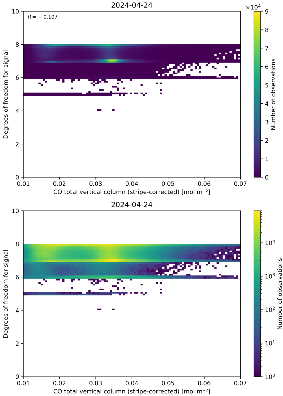
Figure 38: Scatter density plot of “CO total vertical column (stripe-corrected)” against “Degrees of freedom for signal” for 2024-04-23 to 2024-04-25.
