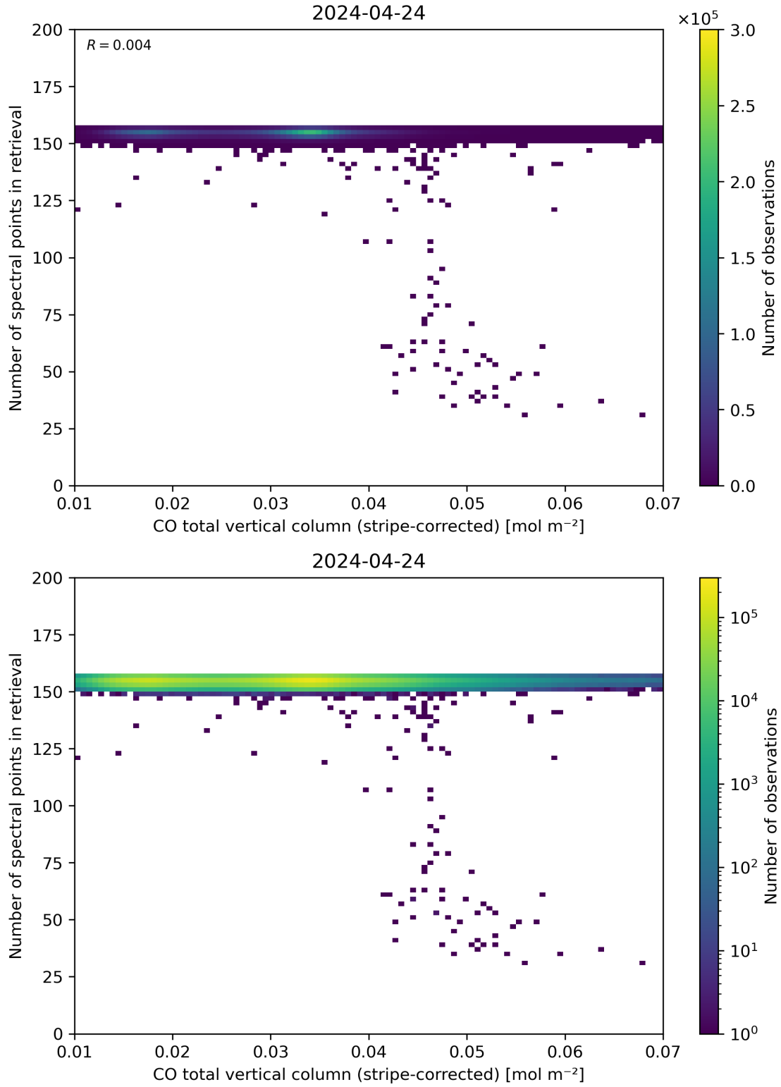
Figure 40: Scatter density plot of “CO total vertical column (stripe-corrected)” against “Number of spectral points in retrieval” for 2024-04-23 to 2024-04-25.
