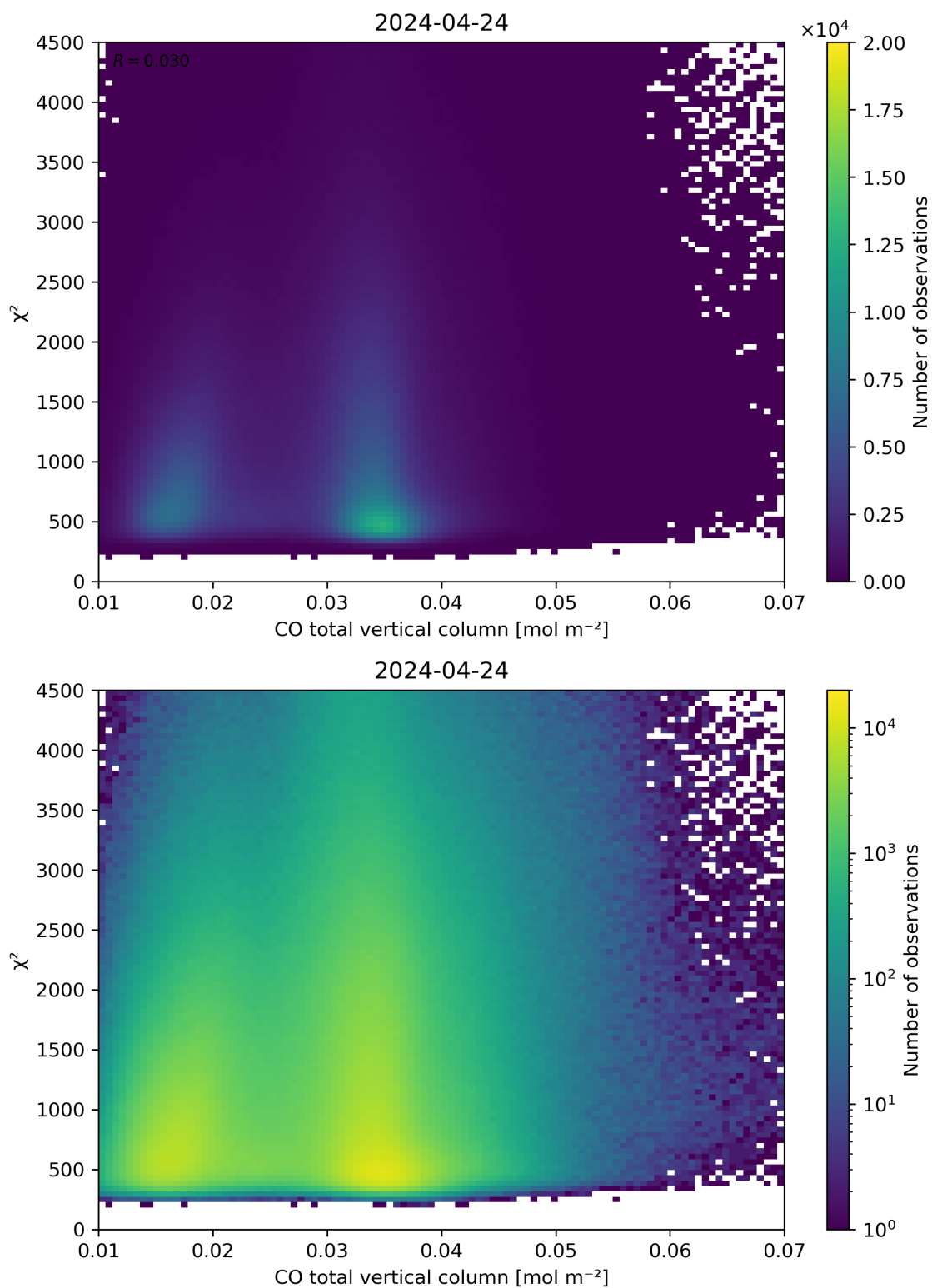
Figure 35: Scatter density plot of “CO total vertical column” against “ \chi^2 ” for 2024-04-23 to 2024-04-25.
