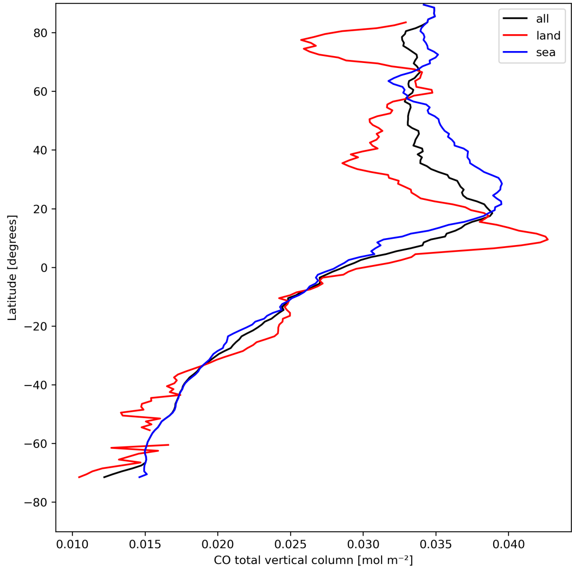
Figure 10: Zonal average of “CO total vertical column” for 2024-04-23 to 2024-04-25.
