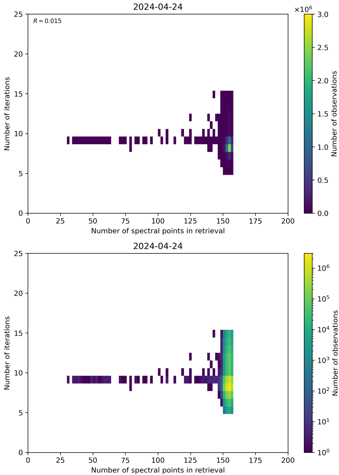
Figure 60: Scatter density plot of “Number of spectral points in retrieval” against “Number of iterations” for 2024-04-23 to 2024-04-25.
