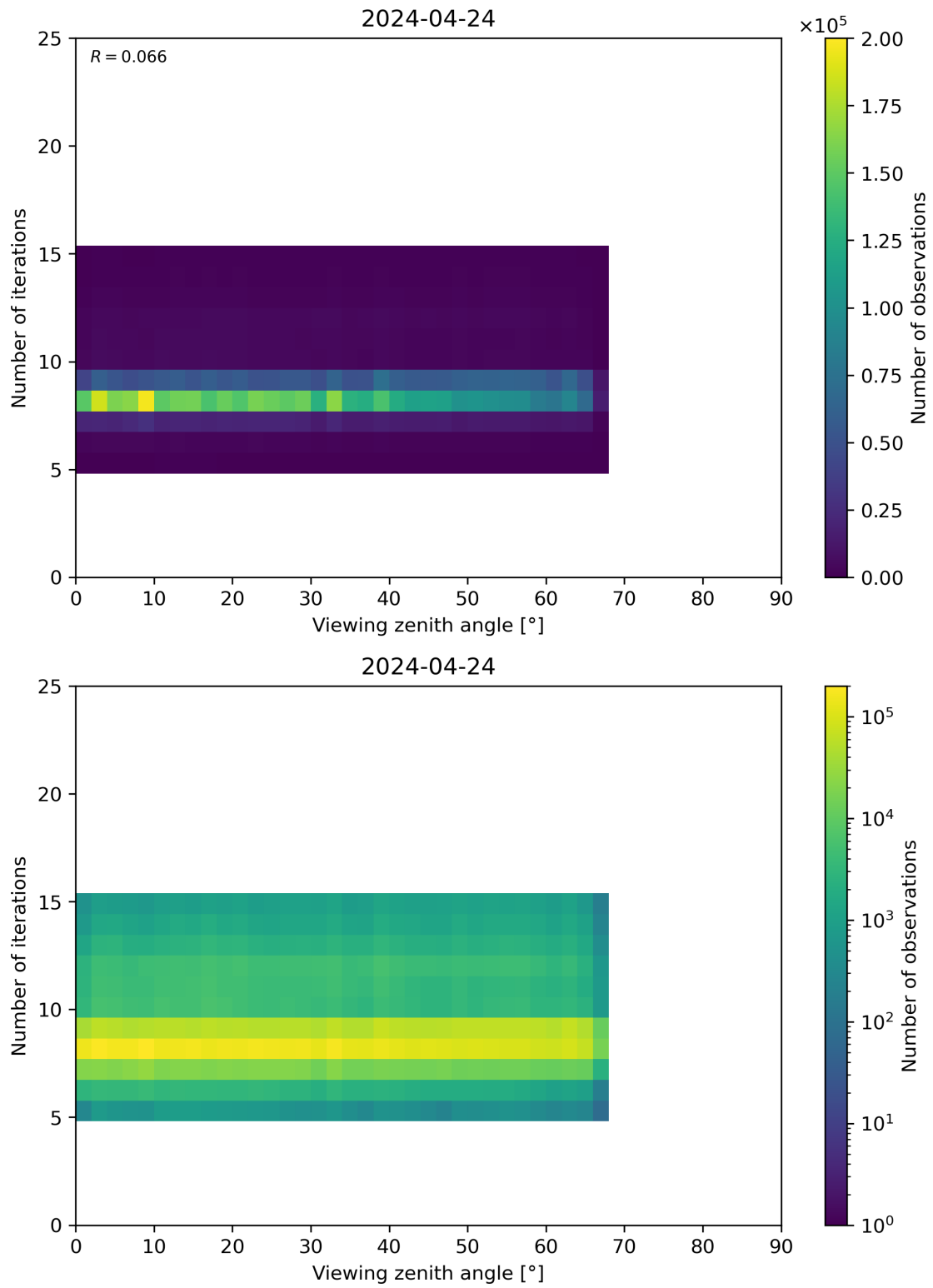
Figure 75: Scatter density plot of “Viewing zenith angle” against “Number of iterations” for 2024-04-23 to 2024-04-25.
