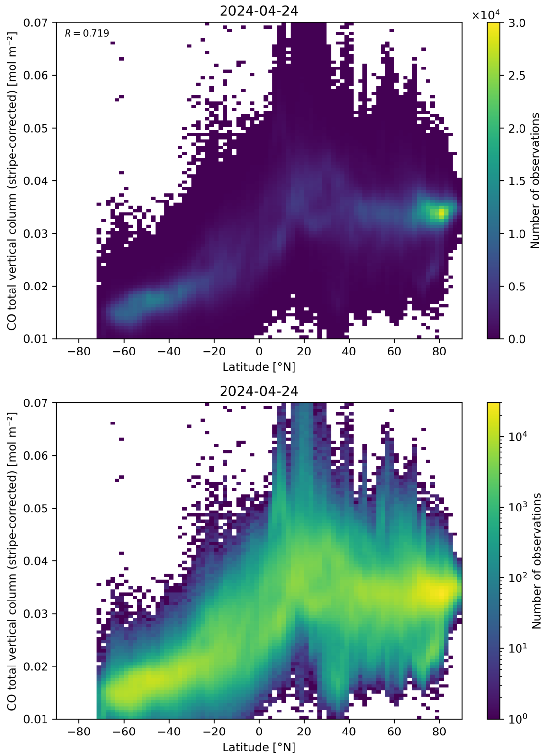
Figure 52: Scatter density plot of “Latitude” against “CO total vertical column (stripe-corrected)” for 2024-04-23 to 2024-04-25.
