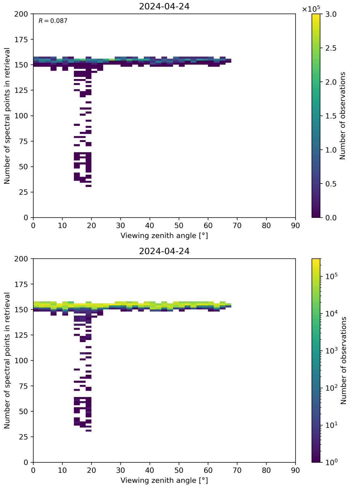
Figure 76: Scatter density plot of “Viewing zenith angle” against “Number of spectral points in retrieval” for 2024-04-23 to 2024-04-25.
