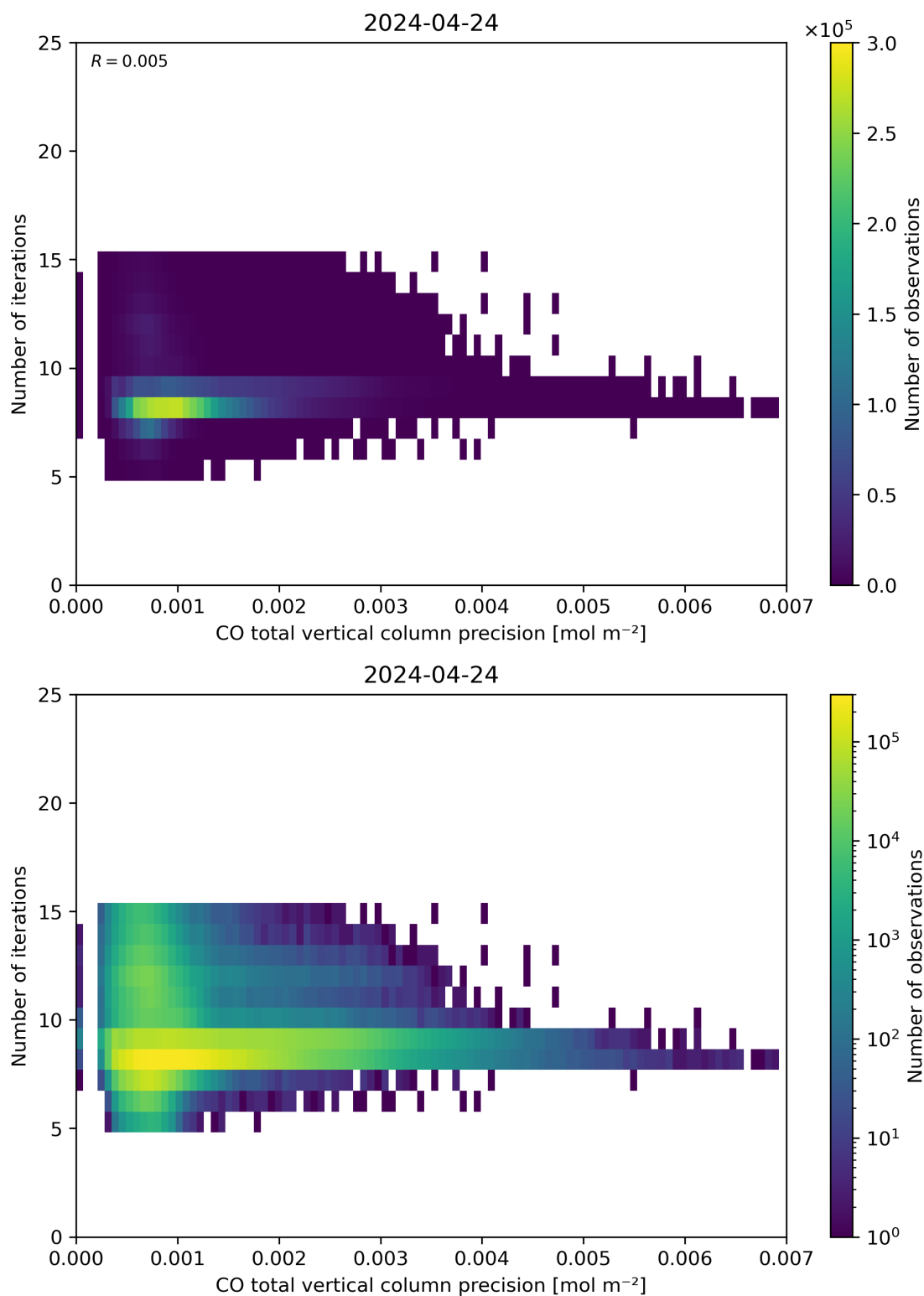
Figure 46: Scatter density plot of “CO total vertical column precision” against “Number of iterations” for 2024-04-23 to 2024-04-25.
