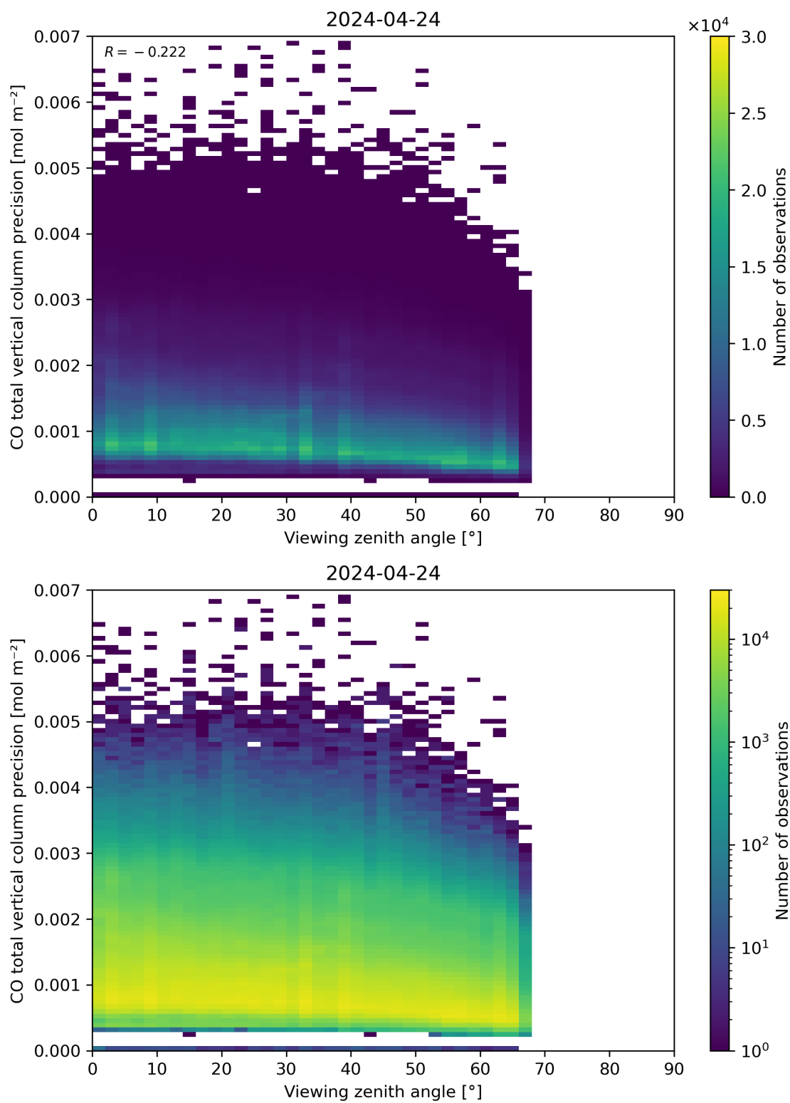
Figure 71: Scatter density plot of “Viewing zenith angle” against “CO total vertical column precision” for 2024-04-23 to 2024-04-25.
