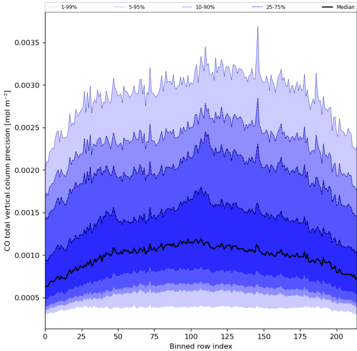
Figure 28: Along track statistics of “CO total vertical column precision” for 2024-04-23 to 2024-04-25
