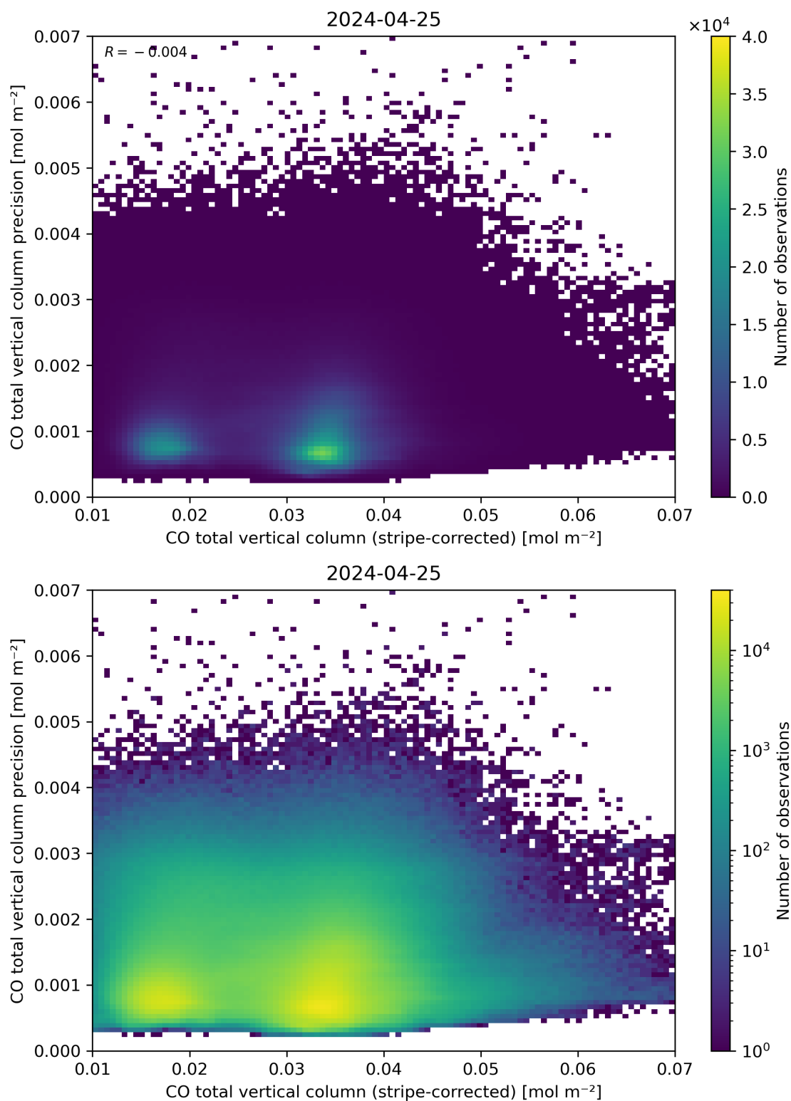
Figure 36: Scatter density plot of “CO total vertical column (stripe-corrected)” against “CO total vertical column precision” for 2024-04-24 to 2024-04-26.
