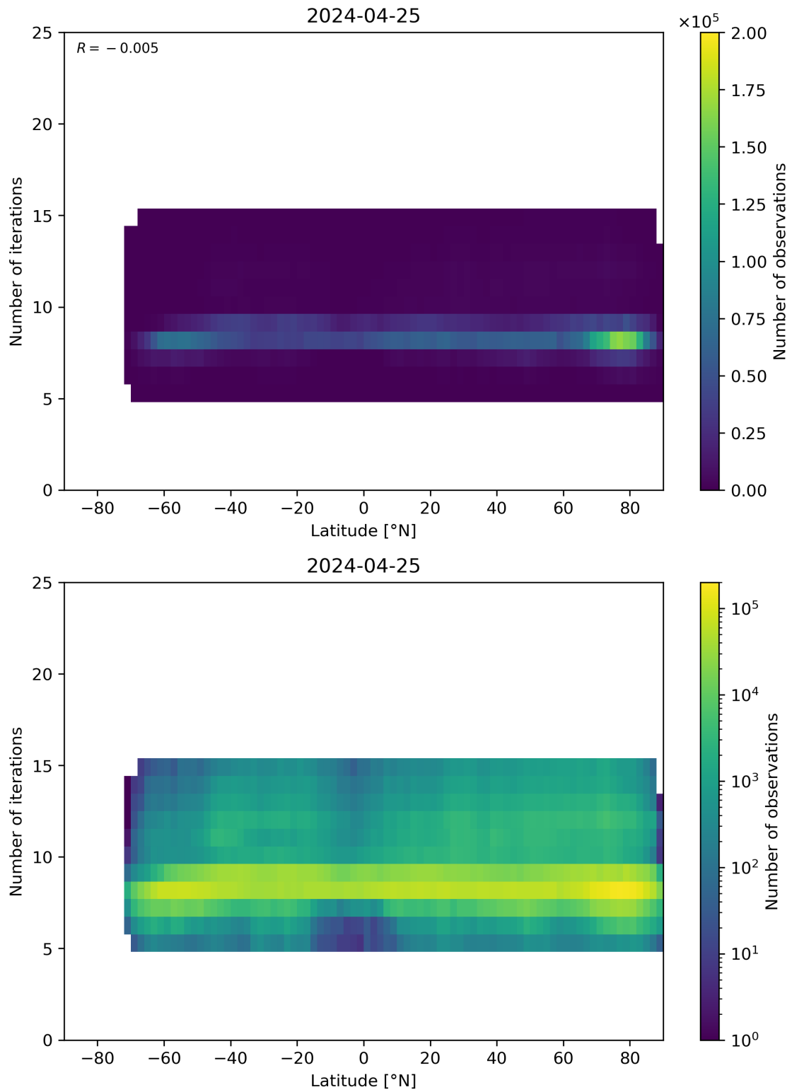
Figure 56: Scatter density plot of “Latitude” against “Number of iterations” for 2024-04-24 to 2024-04-26.
