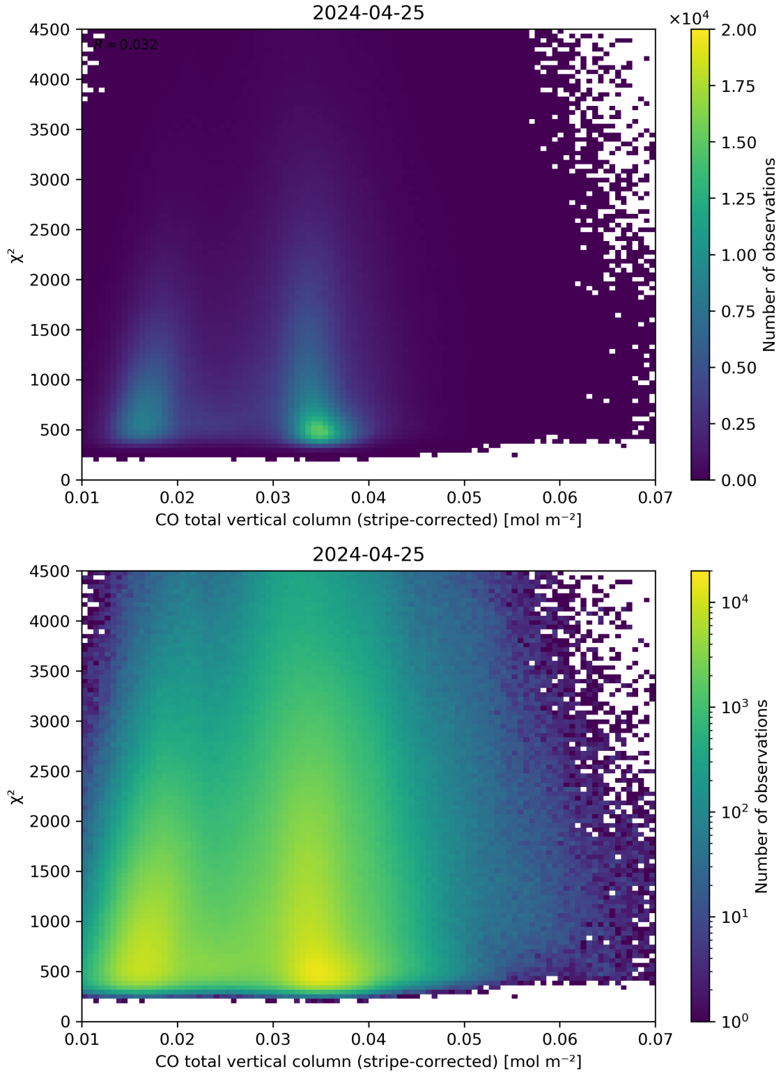
Figure 37: Scatter density plot of “CO total vertical column (stripe-corrected)” against “ \chi^2 ” for 2024-04-24 to 2024-04-26.
