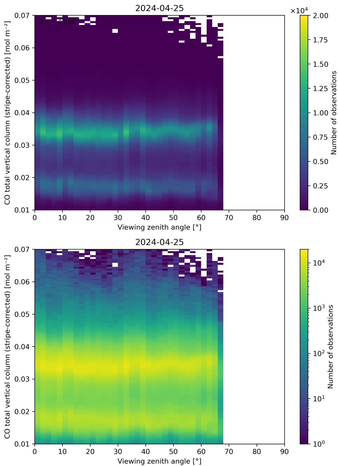
Figure 70: Scatter density plot of “Viewing zenith angle” against “CO total vertical column (stripe-corrected)” for 2024-04-24 to 2024-04-26.
