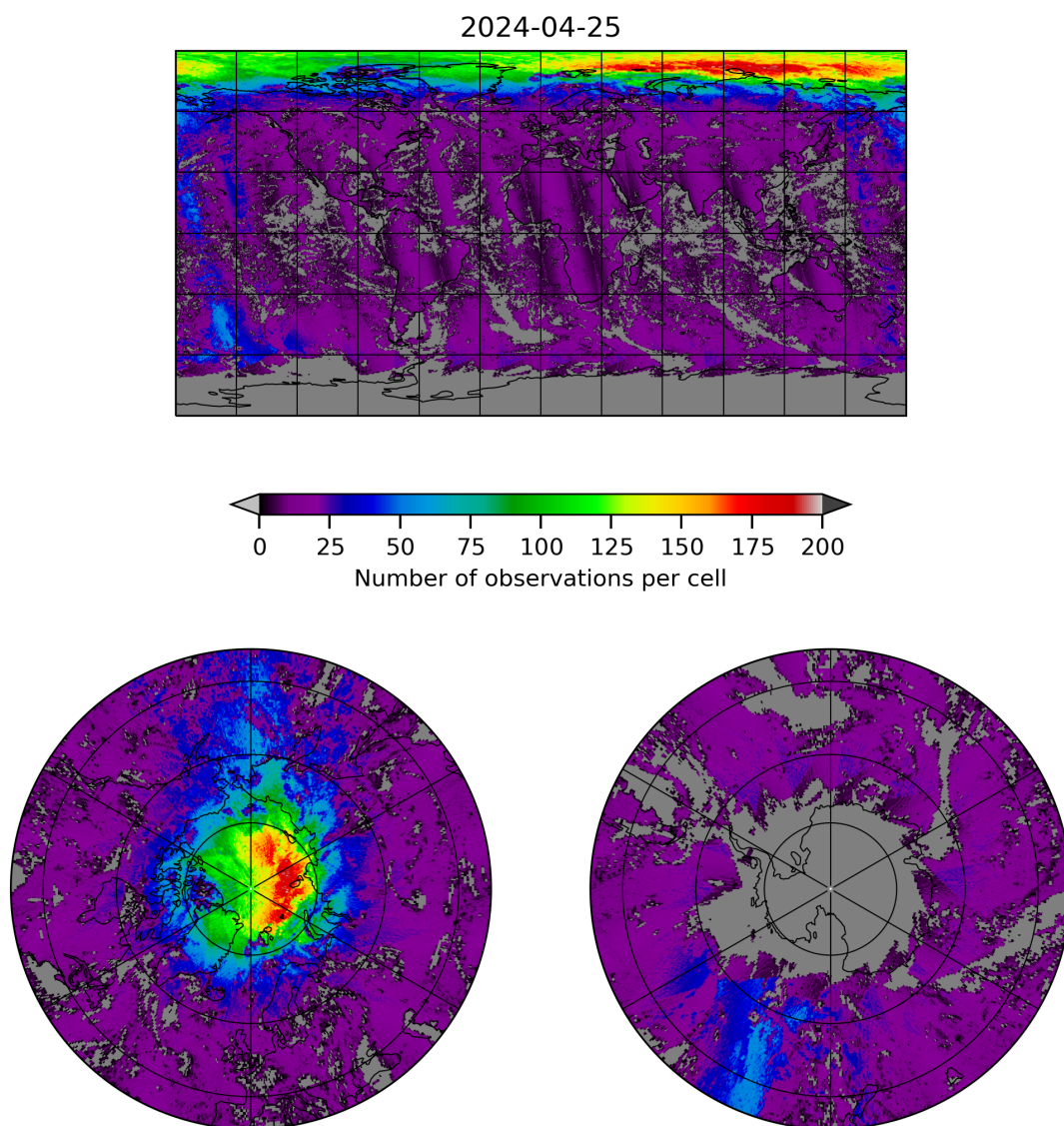
Figure 8: Map of the number of observations for 2024-04-24 to 2024-04-26
