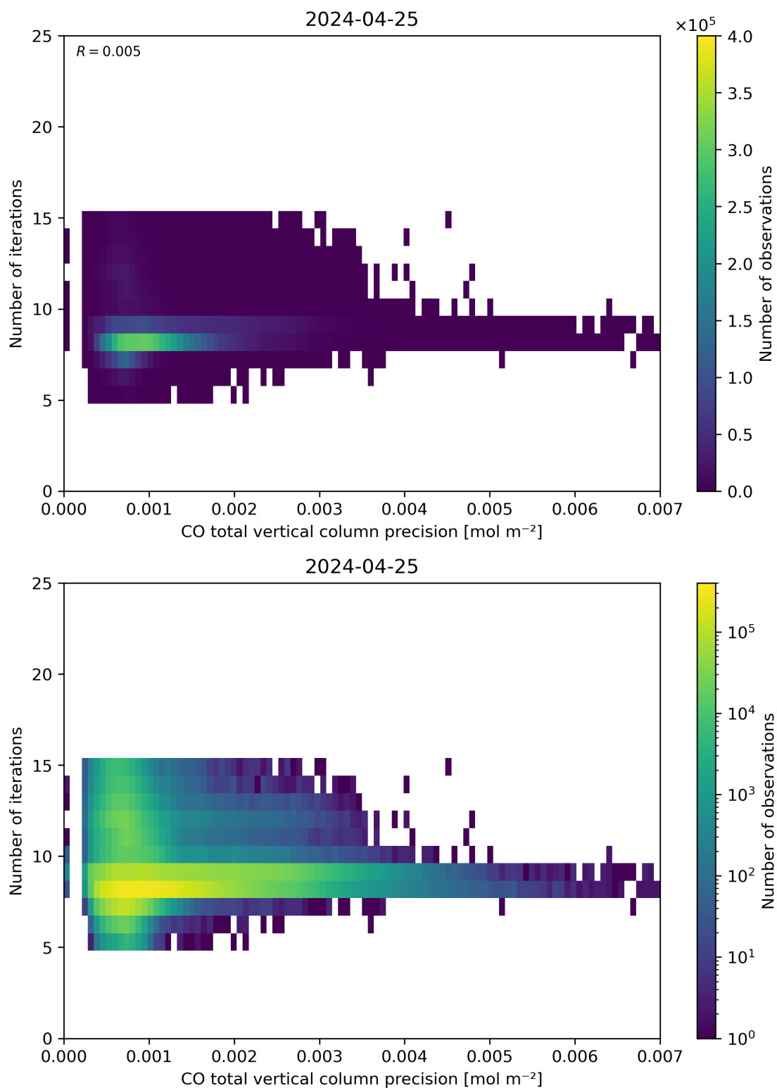
Figure 46: Scatter density plot of “CO total vertical column precision” against “Number of iterations” for 2024-04-24 to 2024-04-26.
