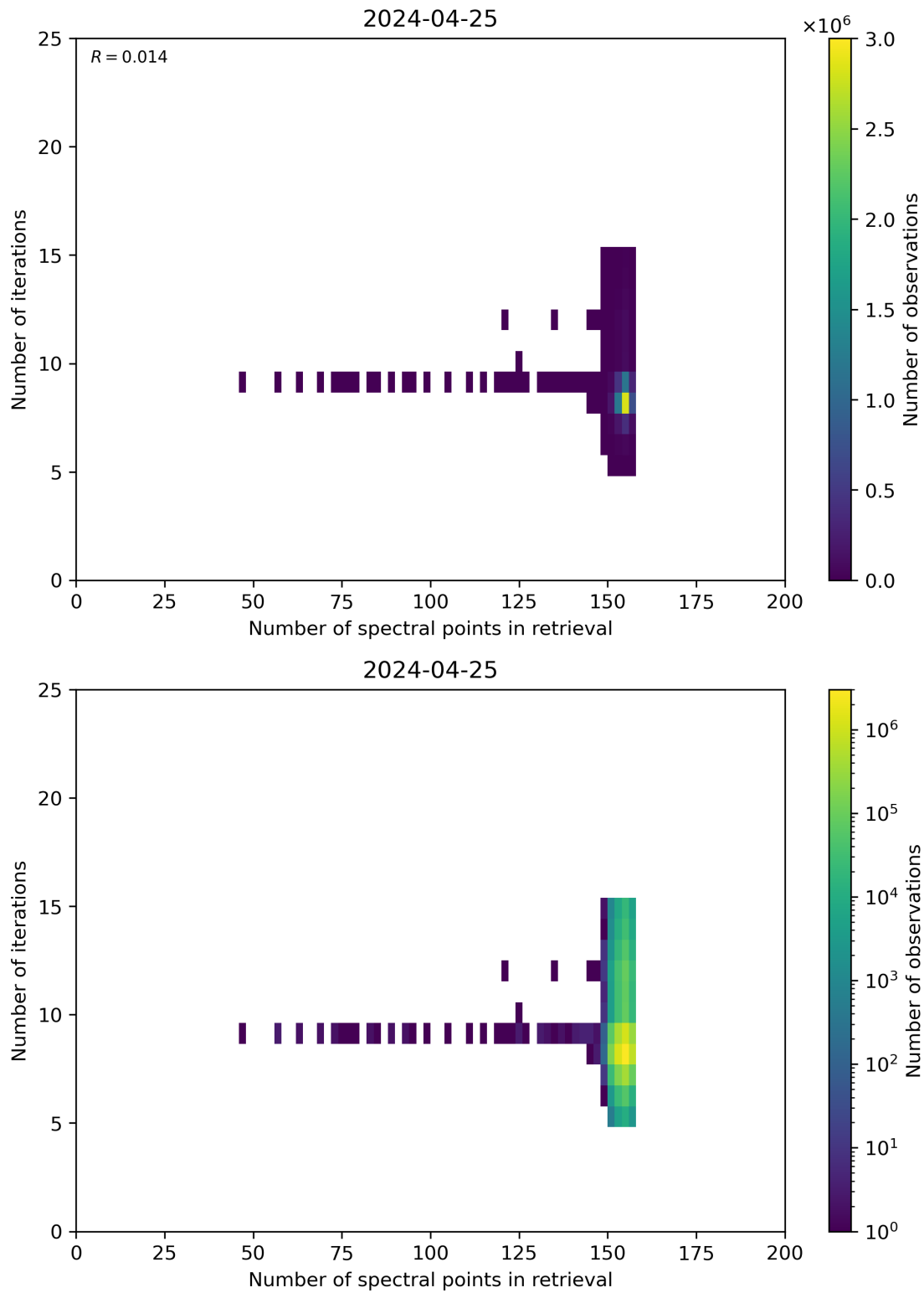
Figure 60: Scatter density plot of “Number of spectral points in retrieval” against “Number of iterations” for 2024-04-24 to 2024-04-26.
