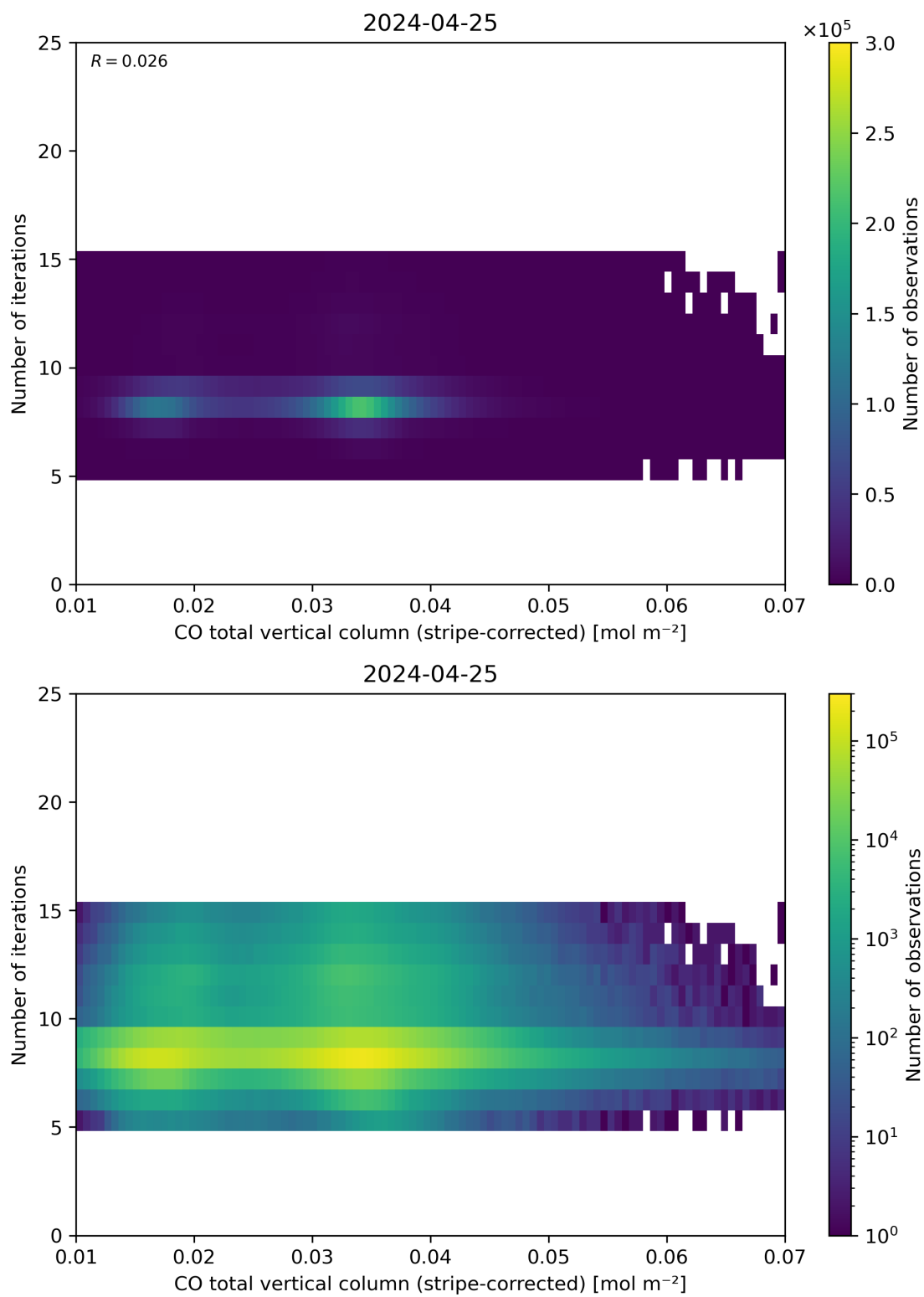
Figure 39: Scatter density plot of “CO total vertical column (stripe-corrected)” against “Number of iterations” for 2024-04-24 to 2024-04-26.
