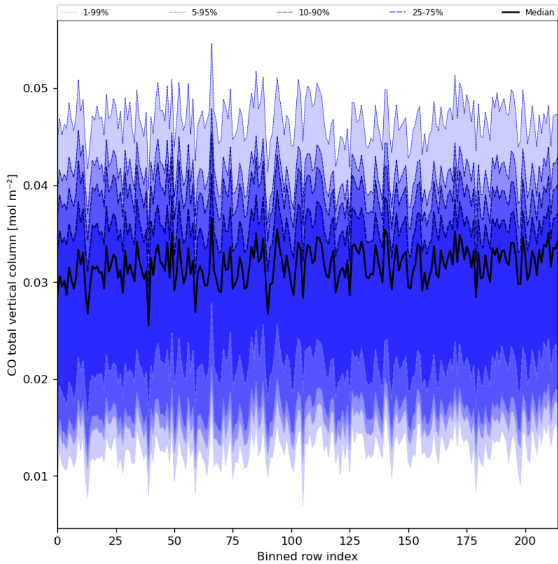
Figure 26: Along track statistics of “CO total vertical column” for 2024-04-24 to 2024-04-26
