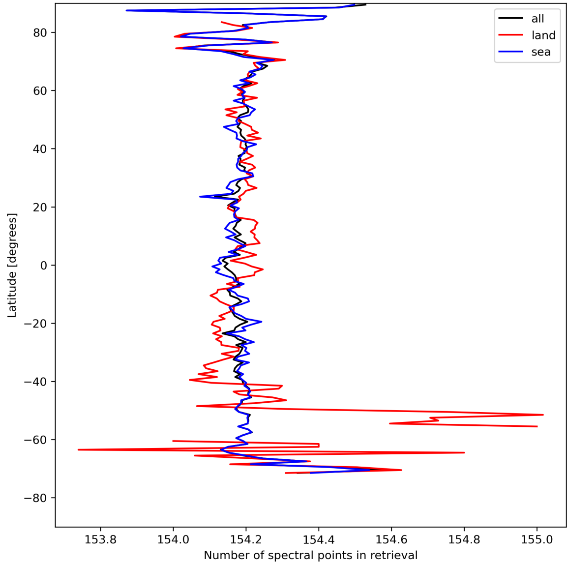
Figure 13: Zonal average of “Number of spectral points in retrieval” for 2024-04-24 to 2024-04-26.
