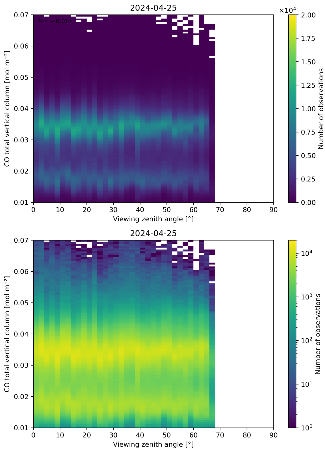
Figure 69: Scatter density plot of “Viewing zenith angle” against “CO total vertical column” for 2024-04-24 to 2024-04-26.
