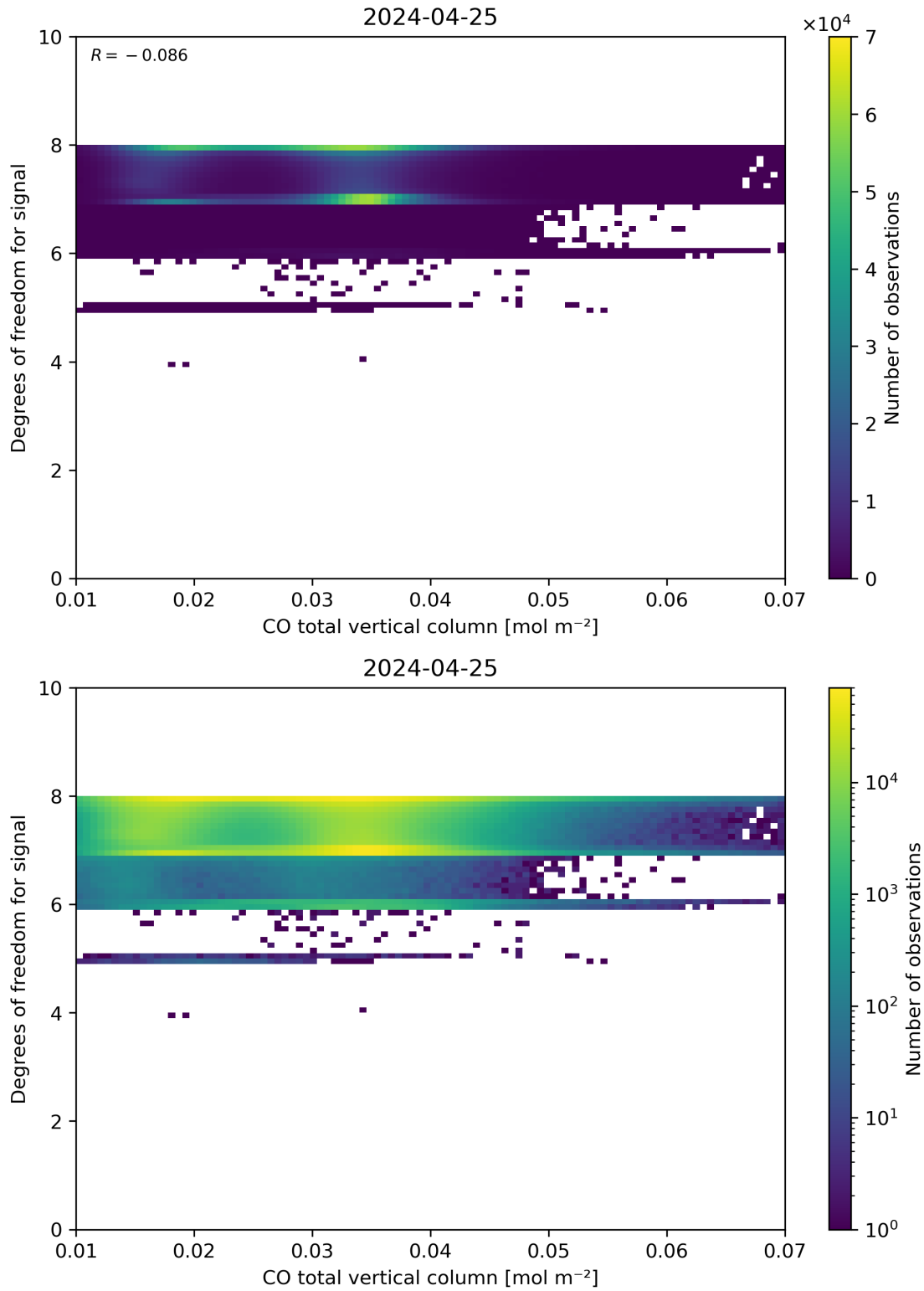
Figure 41: Scatter density plot of “CO total vertical column” against “Degrees of freedom for signal” for 2024-04-24 to 2024-04-26.
