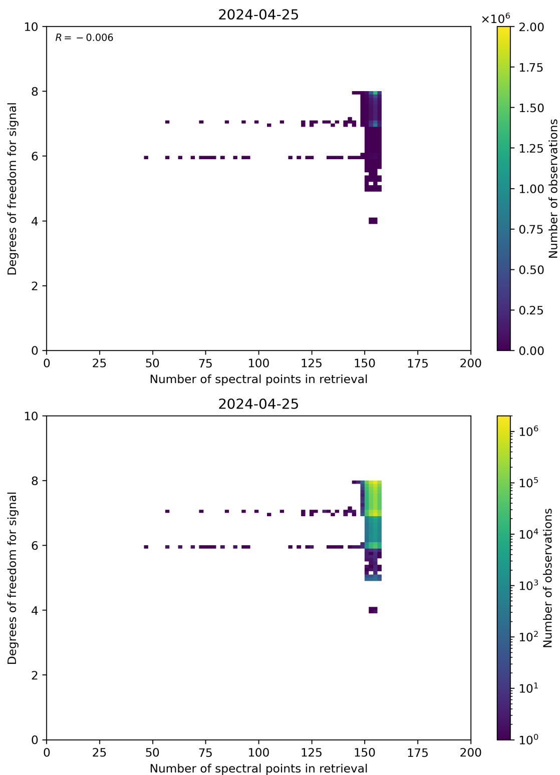
Figure 59: Scatter density plot of “Number of spectral points in retrieval” against “Degrees of freedom for signal” for 2024-04-24 to 2024-04-26.
