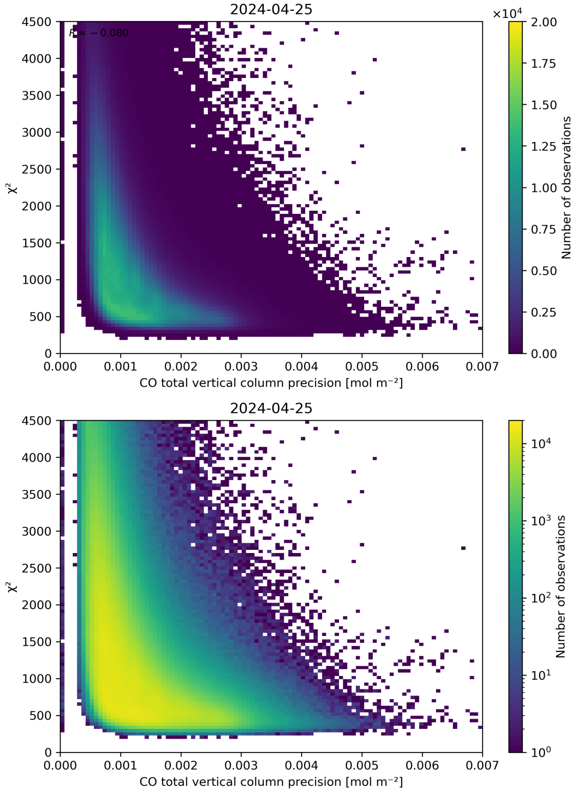
Figure 44: Scatter density plot of “CO total vertical column precision” against “ \chi^2 ” for 2024-04-24 to 2024-04-26.
