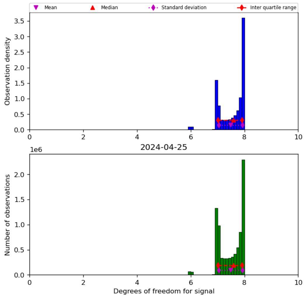
Figure 23: Histogram of “Degrees of freedom for signal” for 2024-04-24 to 2024-04-26
