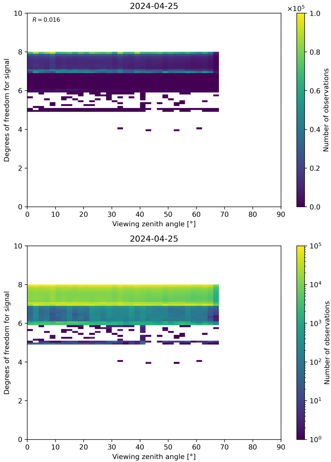
Figure 73: Scatter density plot of “Viewing zenith angle” against “Degrees of freedom for signal” for 2024-04-24 to 2024-04-26.
