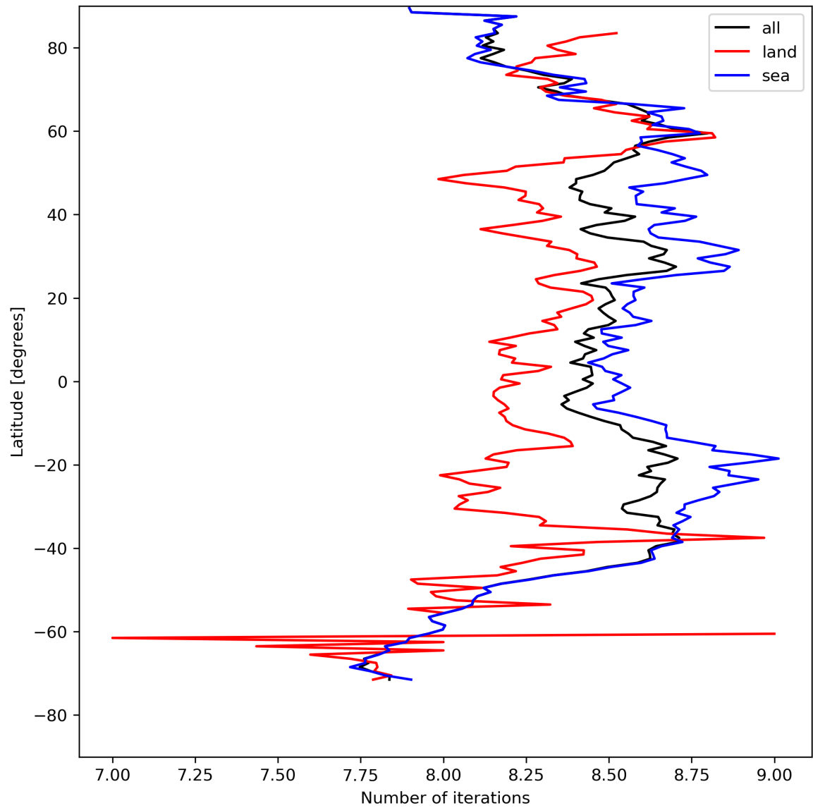
Figure 16: Zonal average of “Number of iterations” for 2024-04-24 to 2024-04-26.
