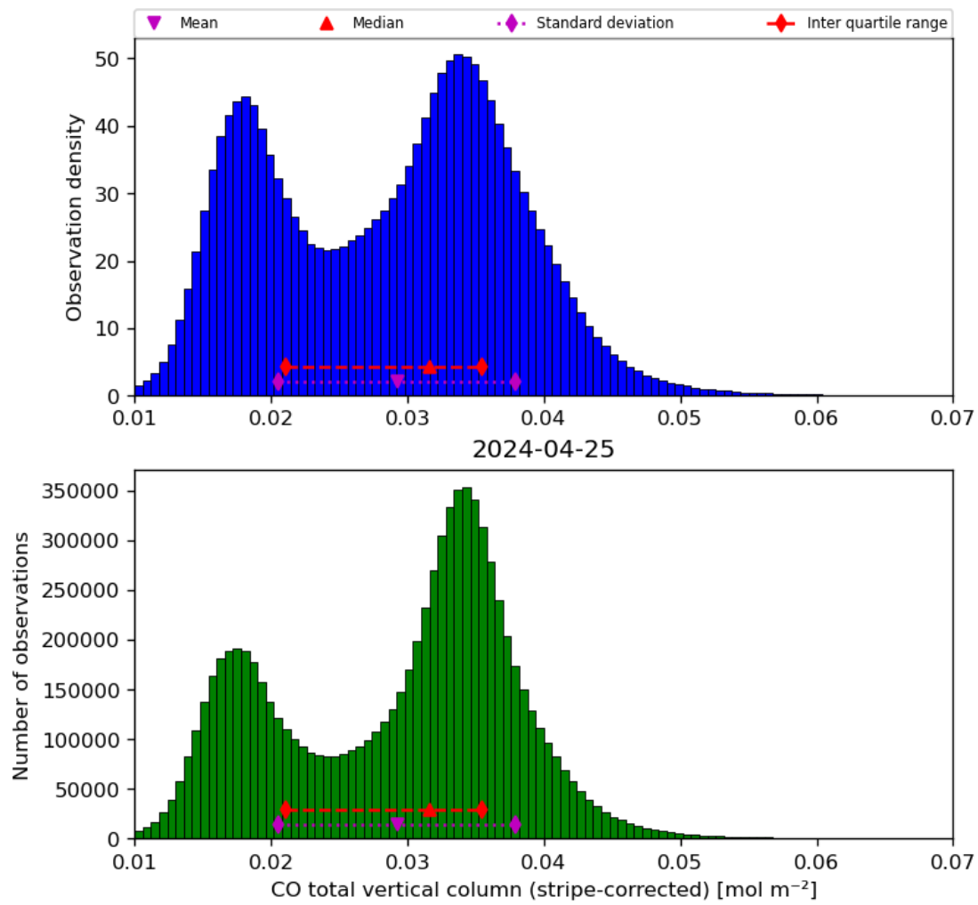
Figure 19: Histogram of “CO total vertical column (stripe-corrected)” for 2024-04-24 to 2024-04-26
