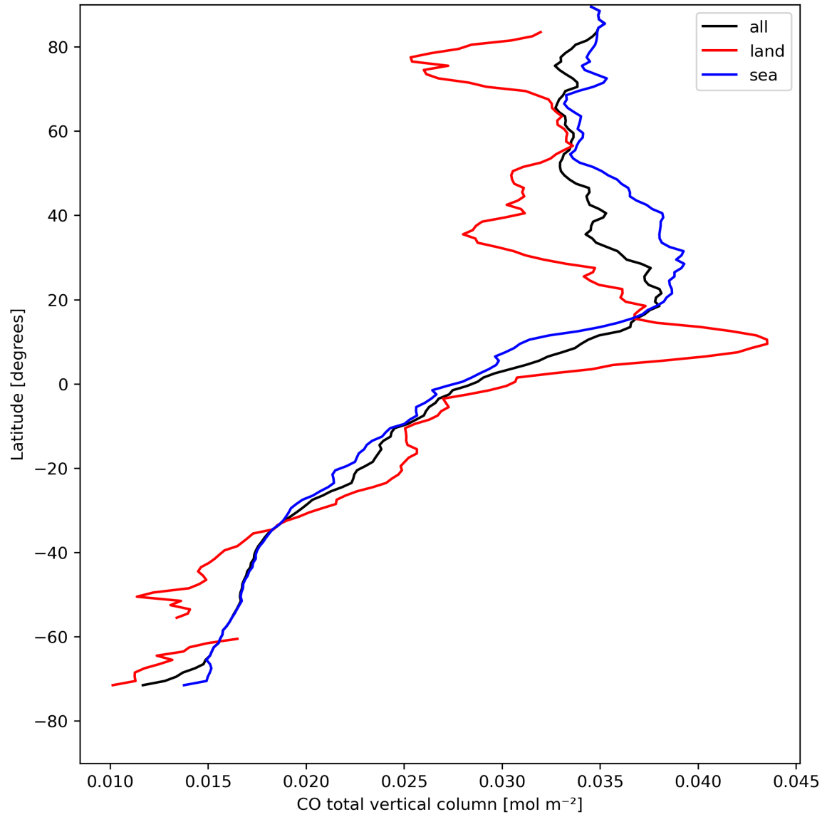
Figure 10: Zonal average of “CO total vertical column” for 2024-04-24 to 2024-04-26.
