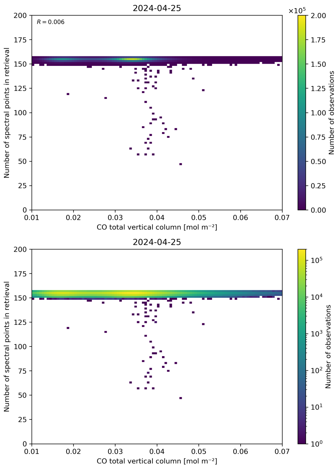
Figure 43: Scatter density plot of “CO total vertical column” against “Number of spectral points in retrieval” for 2024-04-24 to 2024-04-26.
