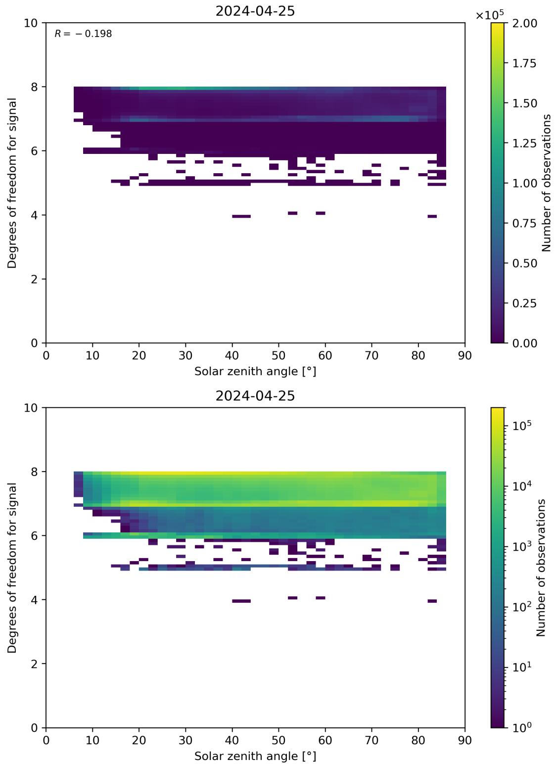
Figure 65: Scatter density plot of “Solar zenith angle” against “Degrees of freedom for signal” for 2024-04-24 to 2024-04-26.
