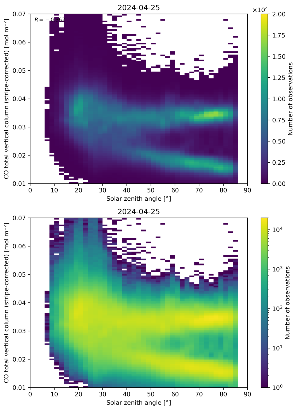
Figure 62: Scatter density plot of “Solar zenith angle” against “CO total vertical column (stripe-corrected)” for 2024-04-24 to 2024-04-26.
