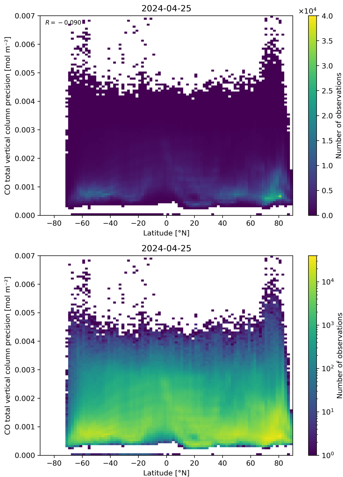
Figure 53: Scatter density plot of “Latitude” against “CO total vertical column precision” for 2024-04-24 to 2024-04-26.
