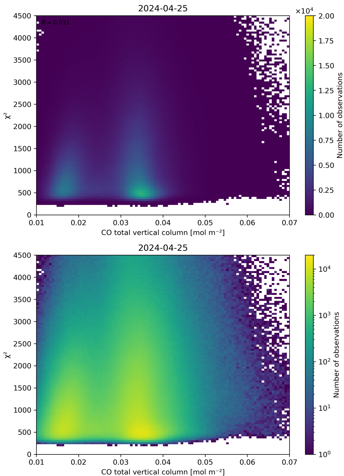
Figure 35: Scatter density plot of “CO total vertical column” against “ \chi^2 ” for 2024-04-24 to 2024-04-26.
