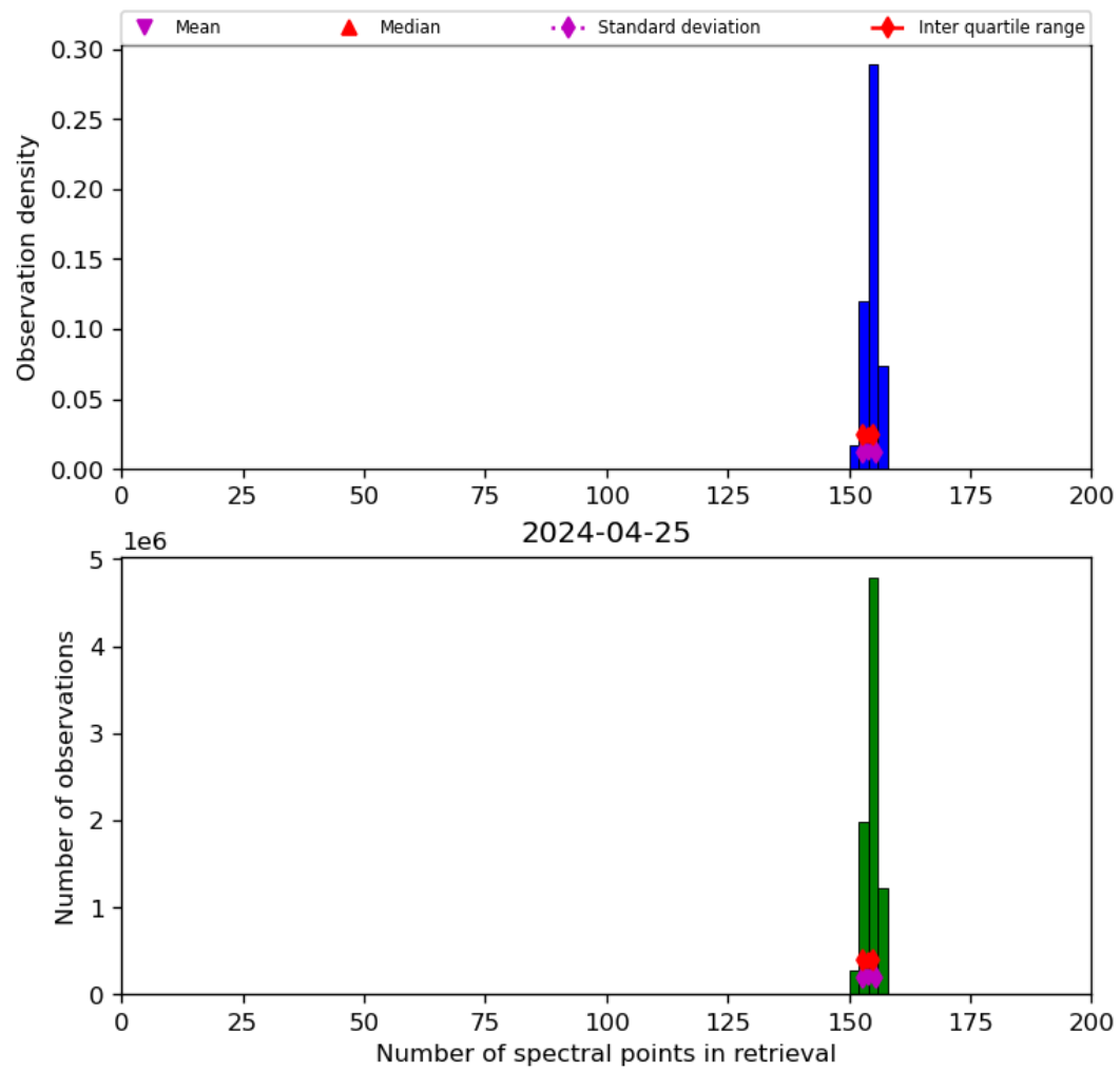
Figure 21: Histogram of “Number of spectral points in retrieval” for 2024-04-24 to 2024-04-26
