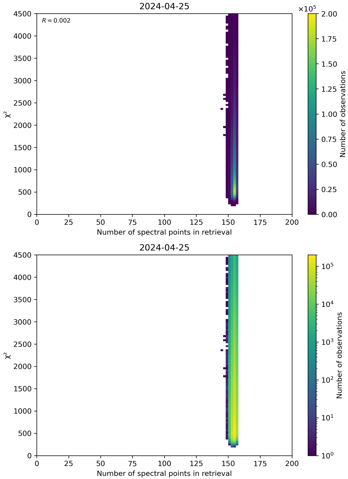
Figure 58: Scatter density plot of “Number of spectral points in retrieval” against “ \chi^2 ” for 2024-04-24 to 2024-04-26.
