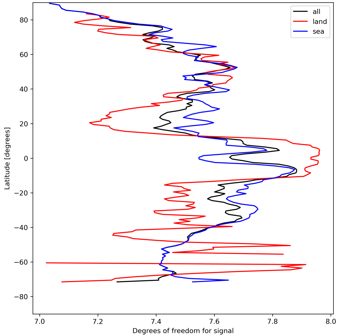
Figure 15: Zonal average of “Degrees of freedom for signal” for 2024-04-24 to 2024-04-26.
