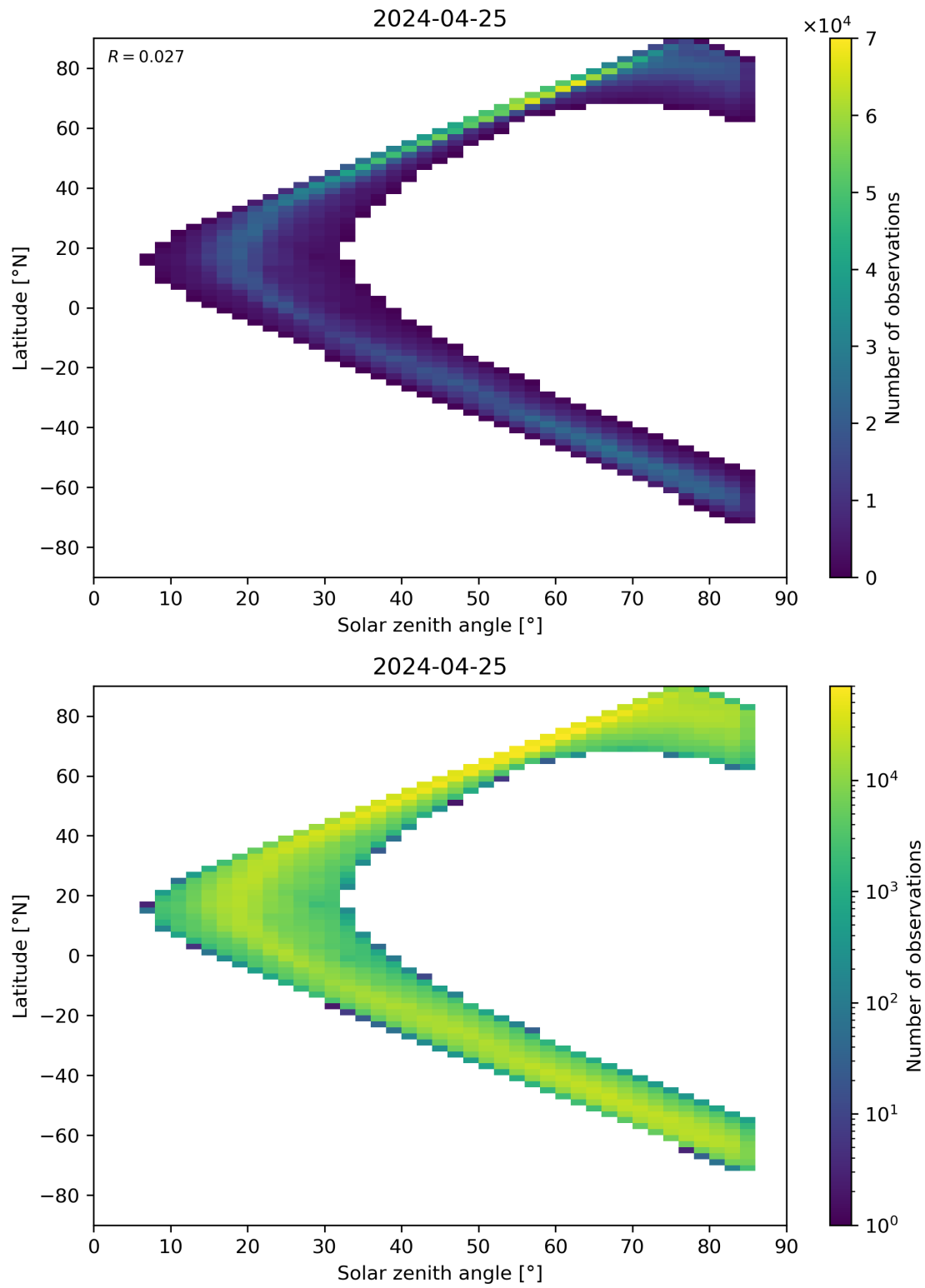
Figure 66: Scatter density plot of “Solar zenith angle” against “Latitude” for 2024-04-24 to 2024-04-26.
