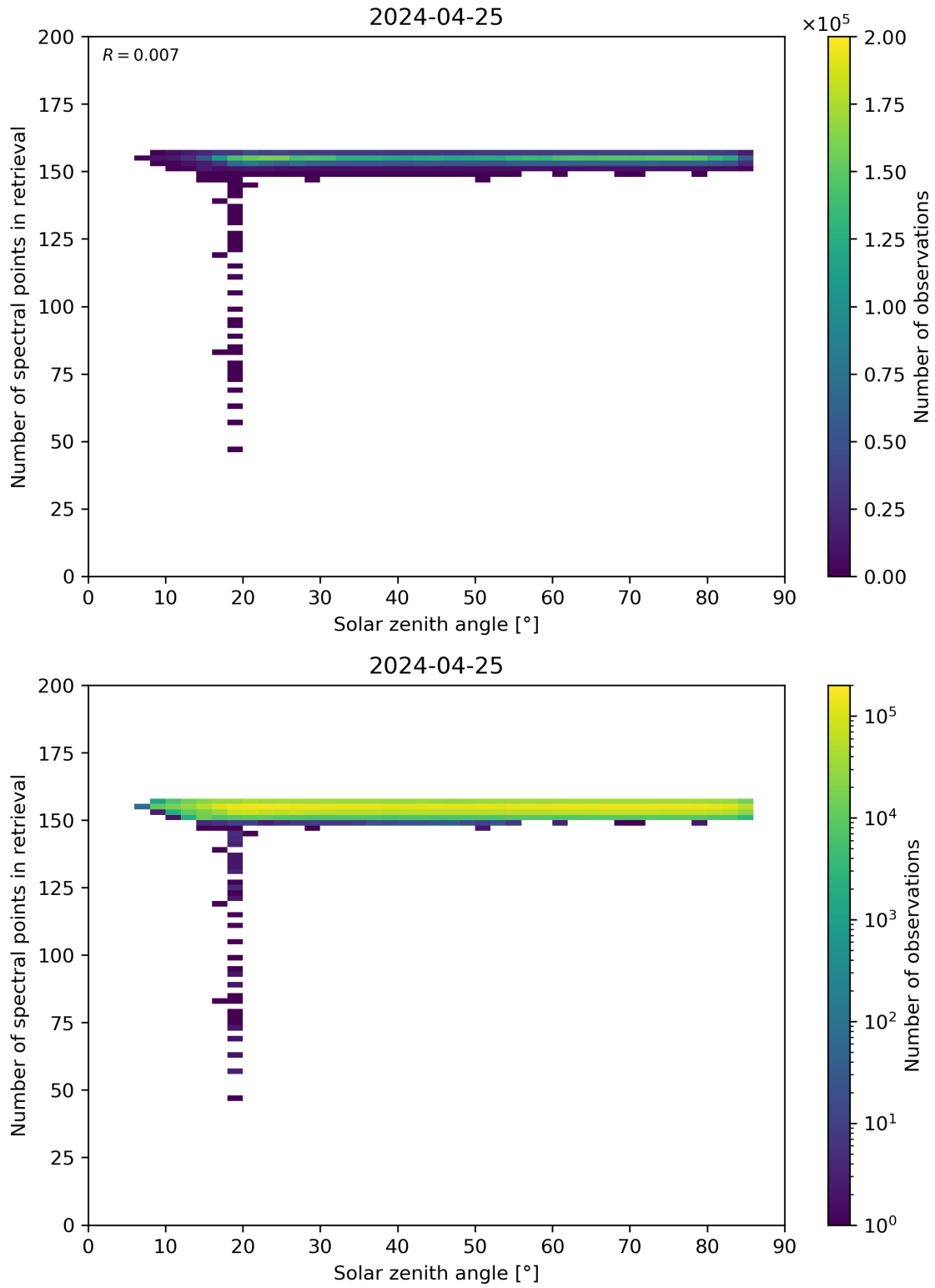
Figure 68: Scatter density plot of “Solar zenith angle” against “Number of spectral points in retrieval” for 2024-04-24 to 2024-04-26.
