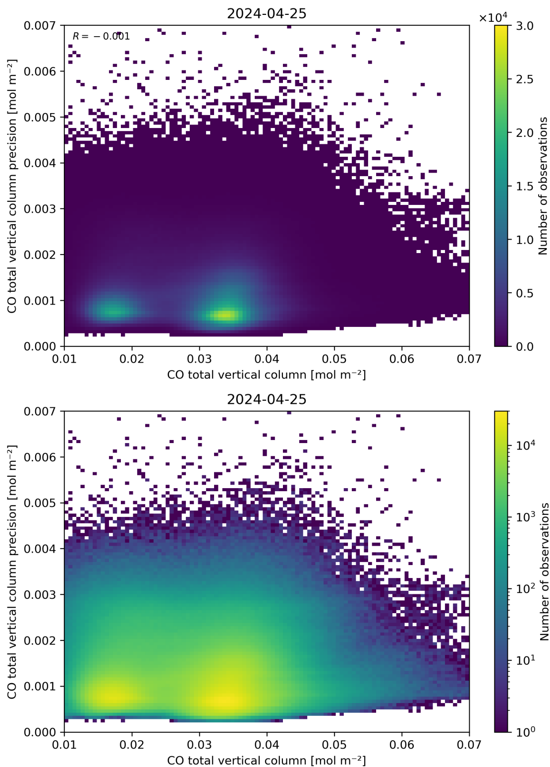
Figure 34: Scatter density plot of “CO total vertical column” against “CO total vertical column precision” for 2024-04-24 to 2024-04-26.
