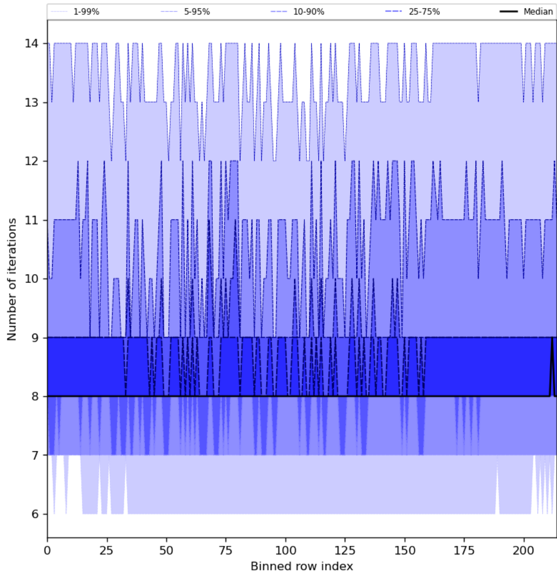
Figure 32: Along track statistics of “Number of iterations” for 2024-04-24 to 2024-04-26
