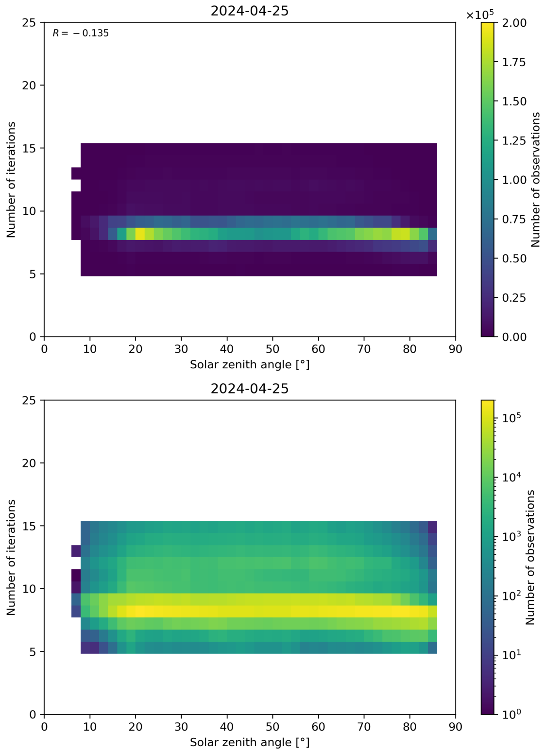
Figure 67: Scatter density plot of “Solar zenith angle” against “Number of iterations” for 2024-04-24 to 2024-04-26.
