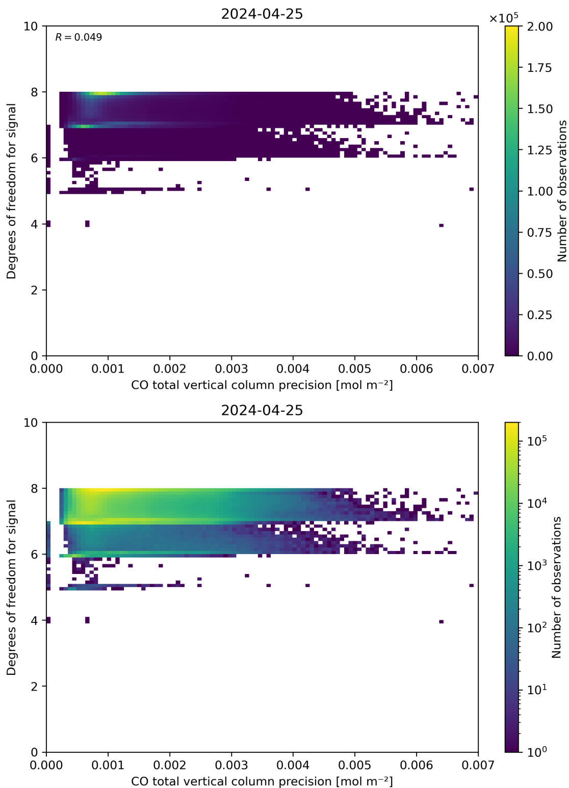
Figure 45: Scatter density plot of “CO total vertical column precision” against “Degrees of freedom for signal” for 2024-04-24 to 2024-04-26.
