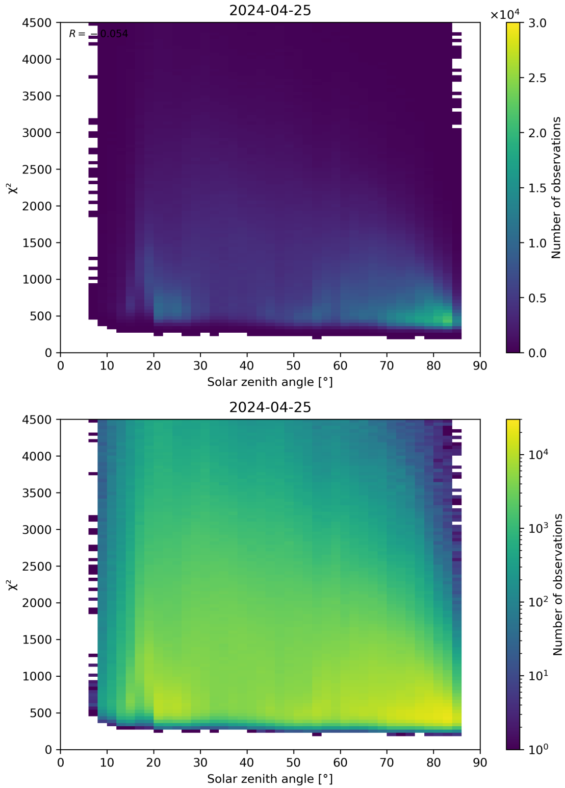
Figure 64: Scatter density plot of “Solar zenith angle” against “ \chi^2 ” for 2024-04-24 to 2024-04-26.
