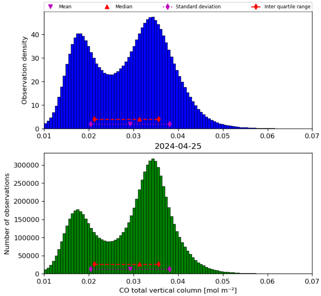
Figure 18: Histogram of “CO total vertical column” for 2024-04-24 to 2024-04-26
