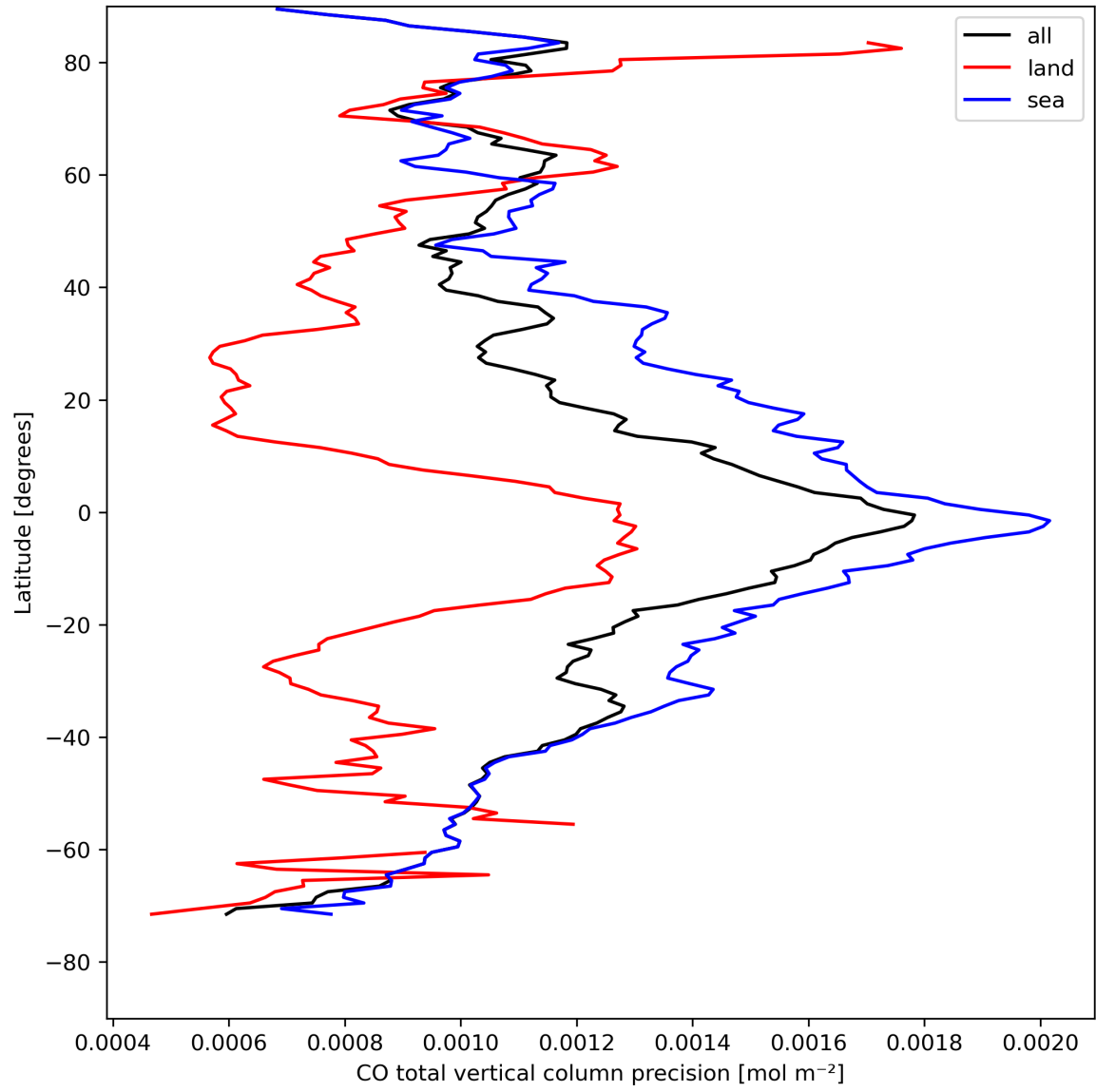
Figure 12: Zonal average of “CO total vertical column precision” for 2024-04-24 to 2024-04-26.
