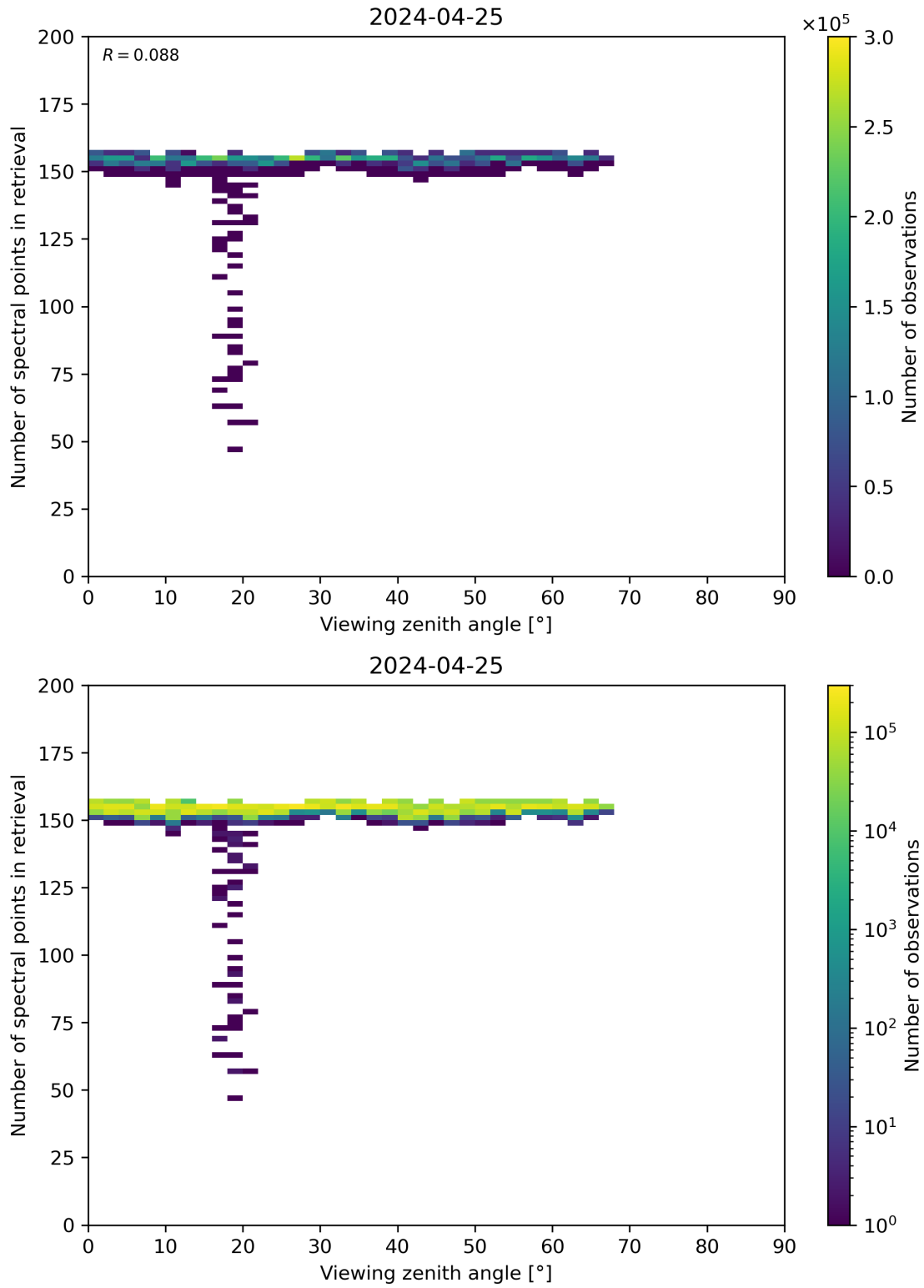
Figure 76: Scatter density plot of “Viewing zenith angle” against “Number of spectral points in retrieval” for 2024-04-24 to 2024-04-26.
