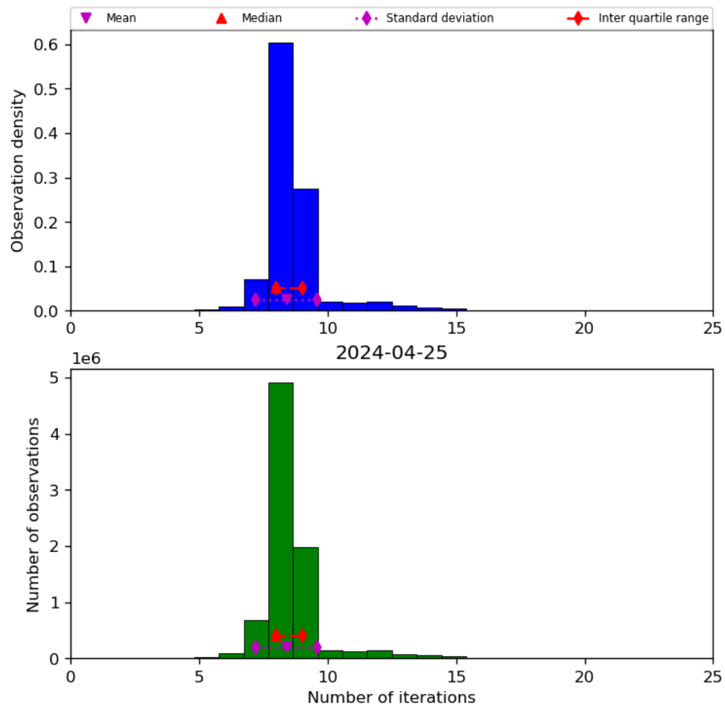
Figure 24: Histogram of “Number of iterations” for 2024-04-24 to 2024-04-26
