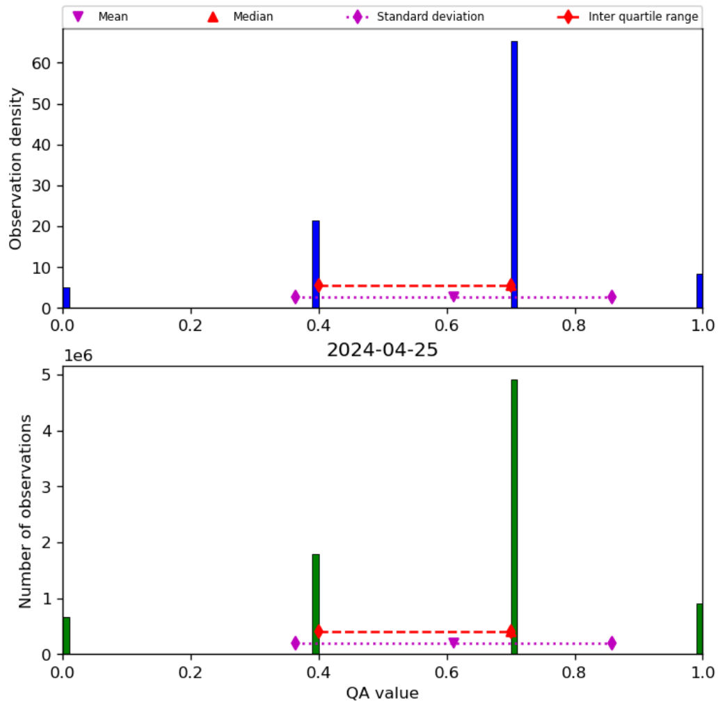
Figure 17: Histogram of “QA value” for 2024-04-24 to 2024-04-26
