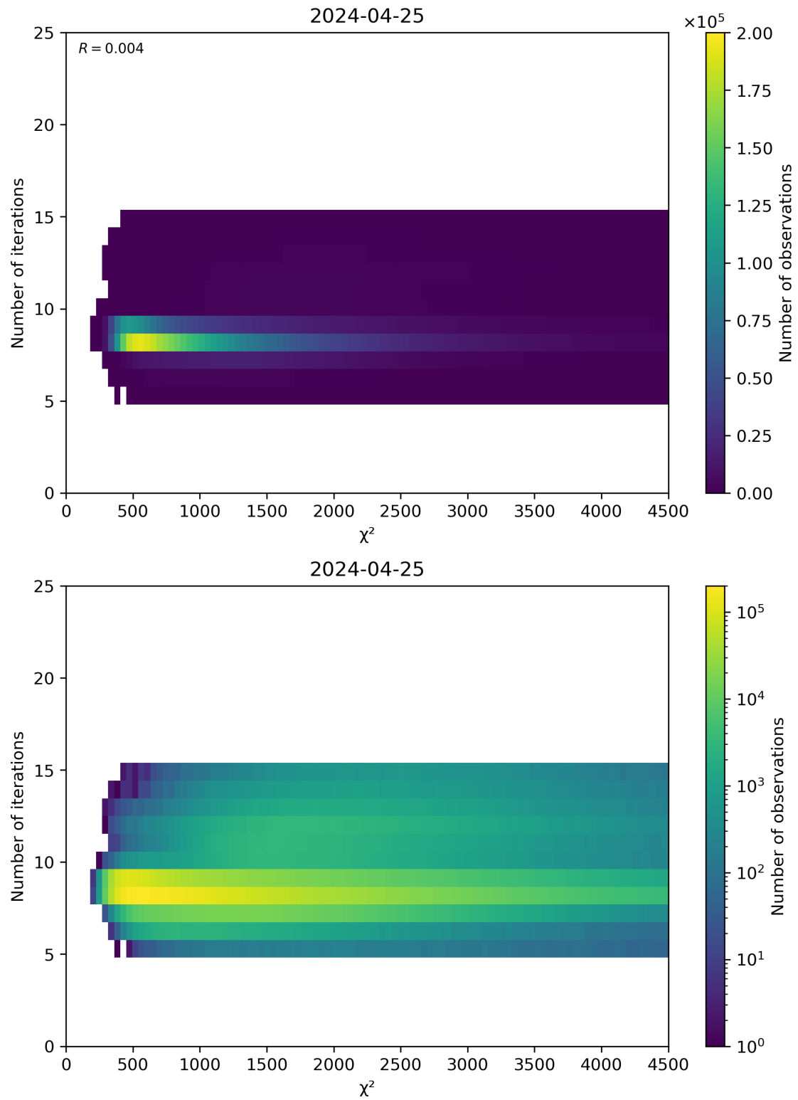
Figure 49: Scatter density plot of “ \chi^2 ” against “Number of iterations” for 2024-04-24 to 2024-04-26.
