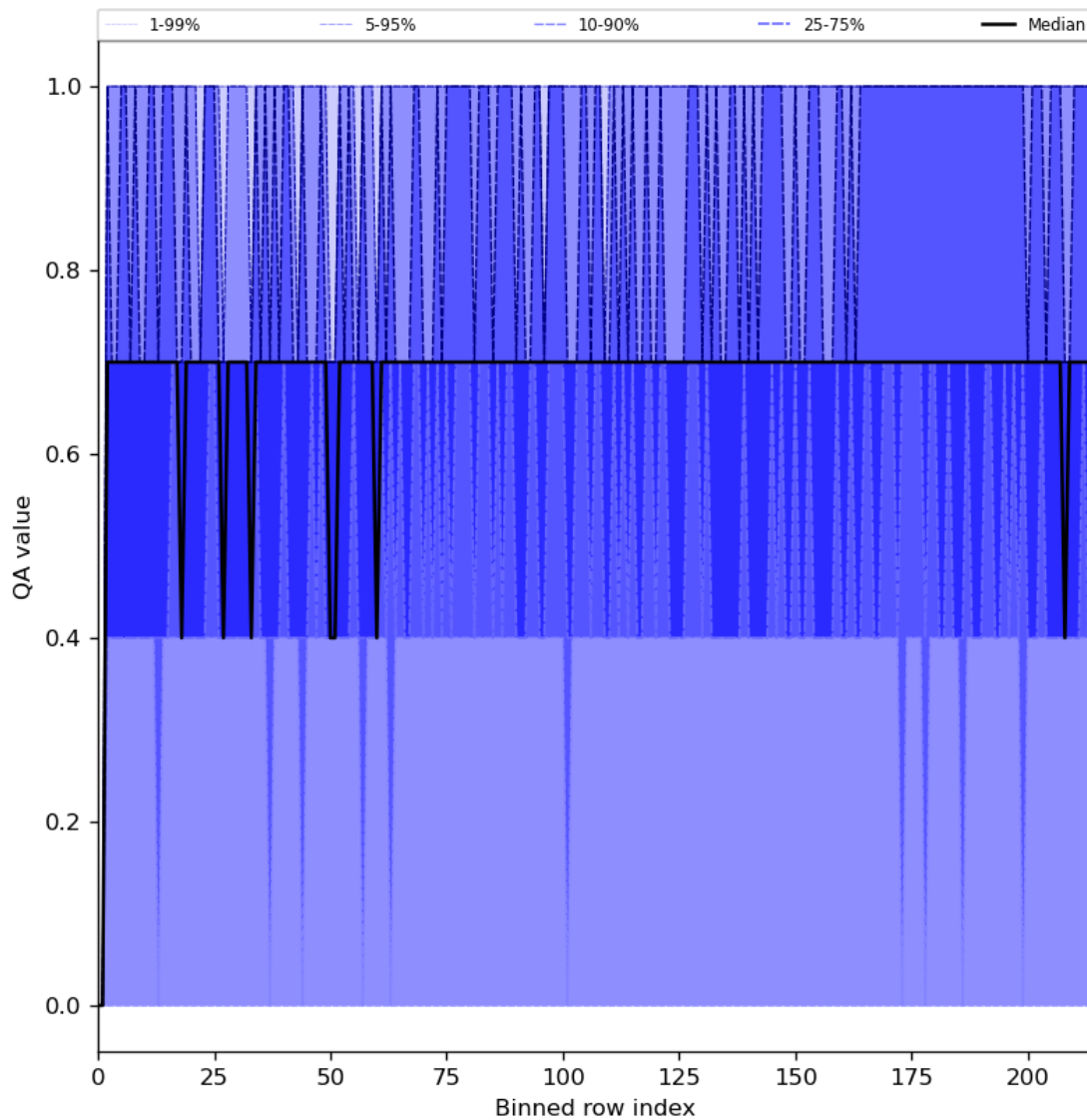
Figure 25: Along track statistics of “QA value” for 2024-04-24 to 2024-04-26
