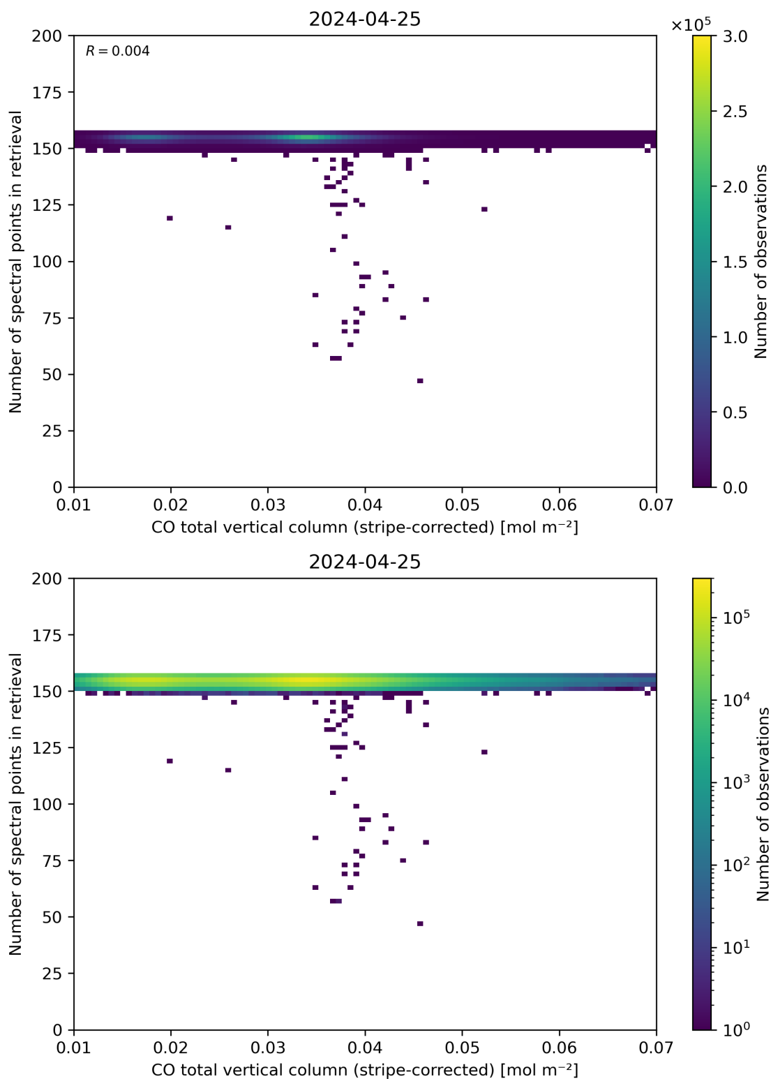
Figure 40: Scatter density plot of “CO total vertical column (stripe-corrected)” against “Number of spectral points in retrieval” for 2024-04-24 to 2024-04-26.
