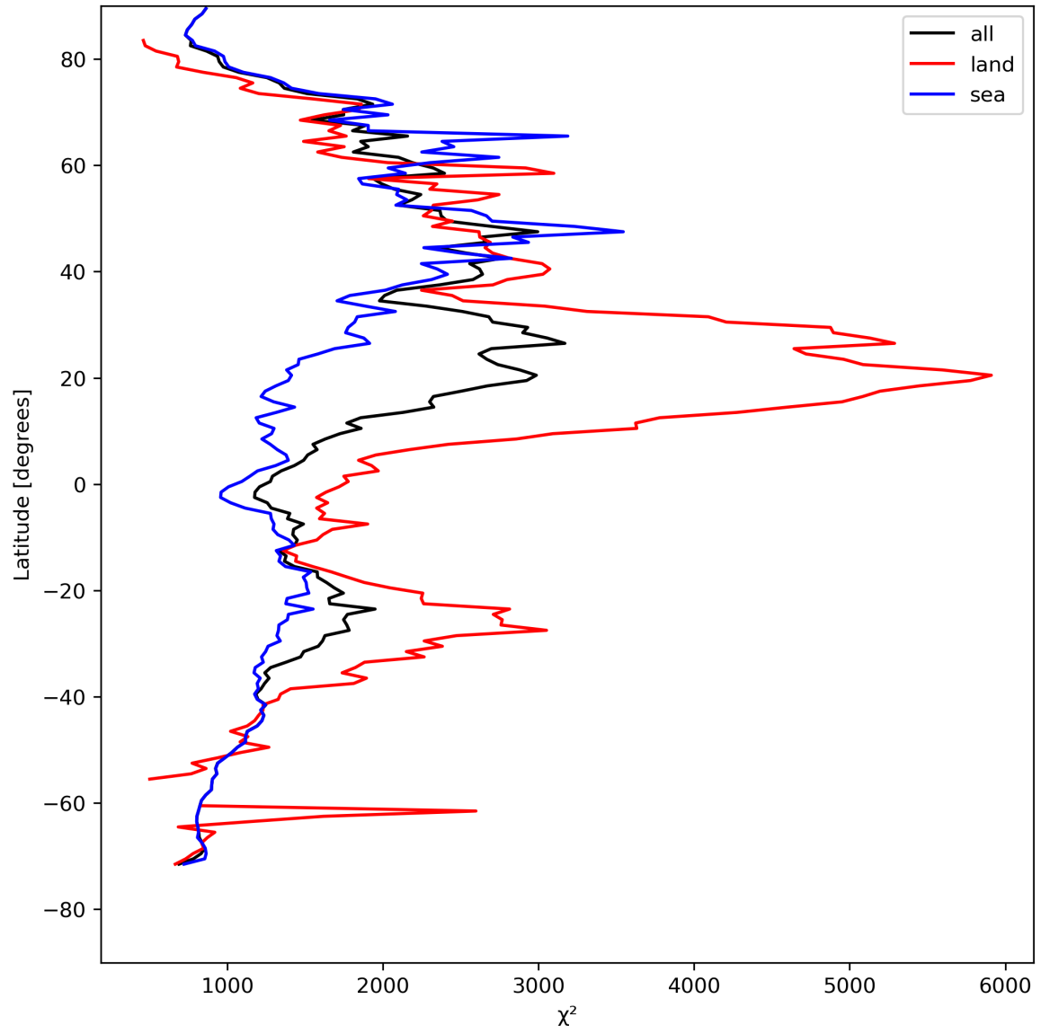
Figure 14: Zonal average of “ \chi^2 ” for 2024-04-24 to 2024-04-26.
