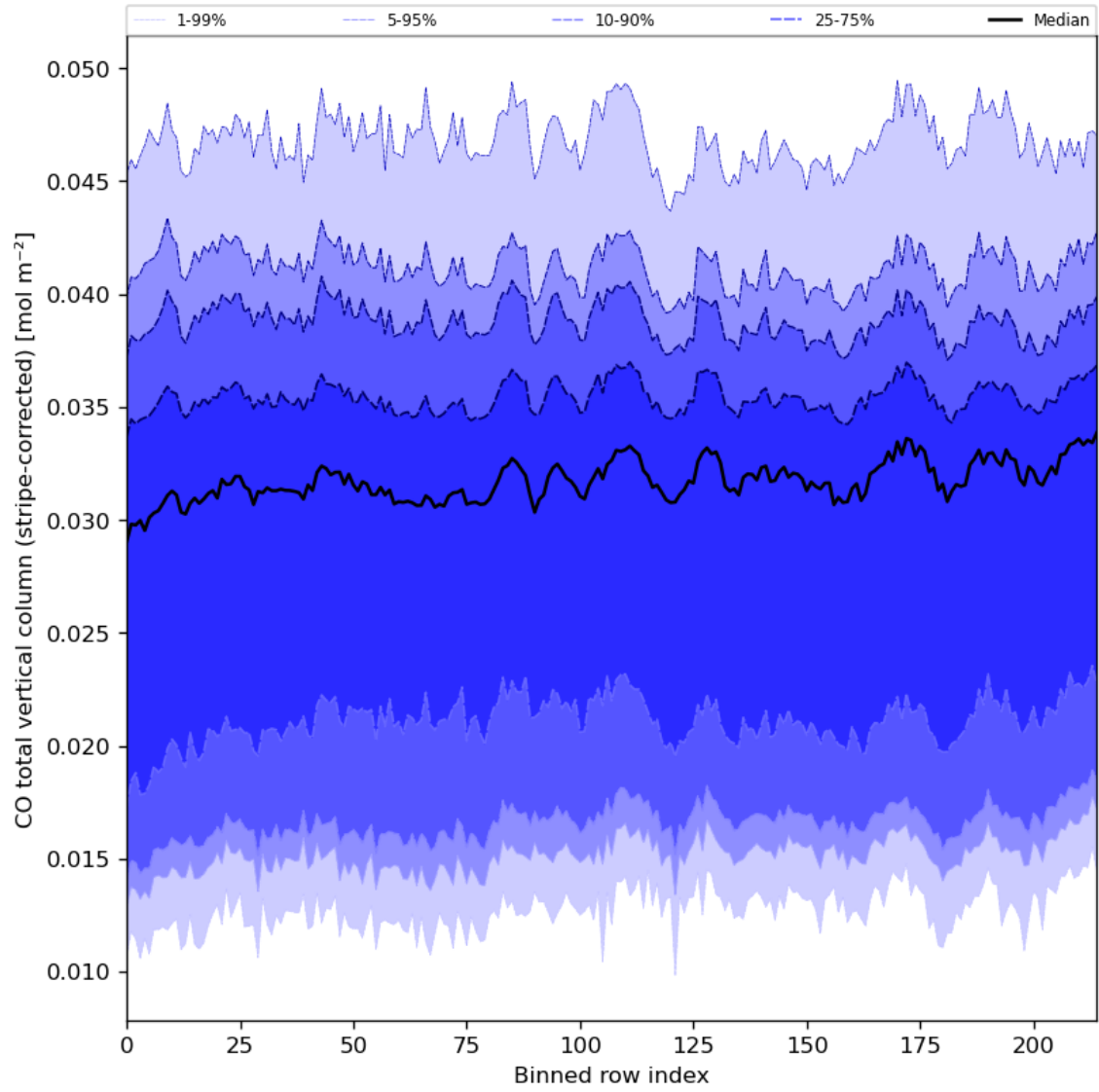
Figure 27: Along track statistics of “CO total vertical column (stripe-corrected)” for 2024-04-24 to 2024-04-26
