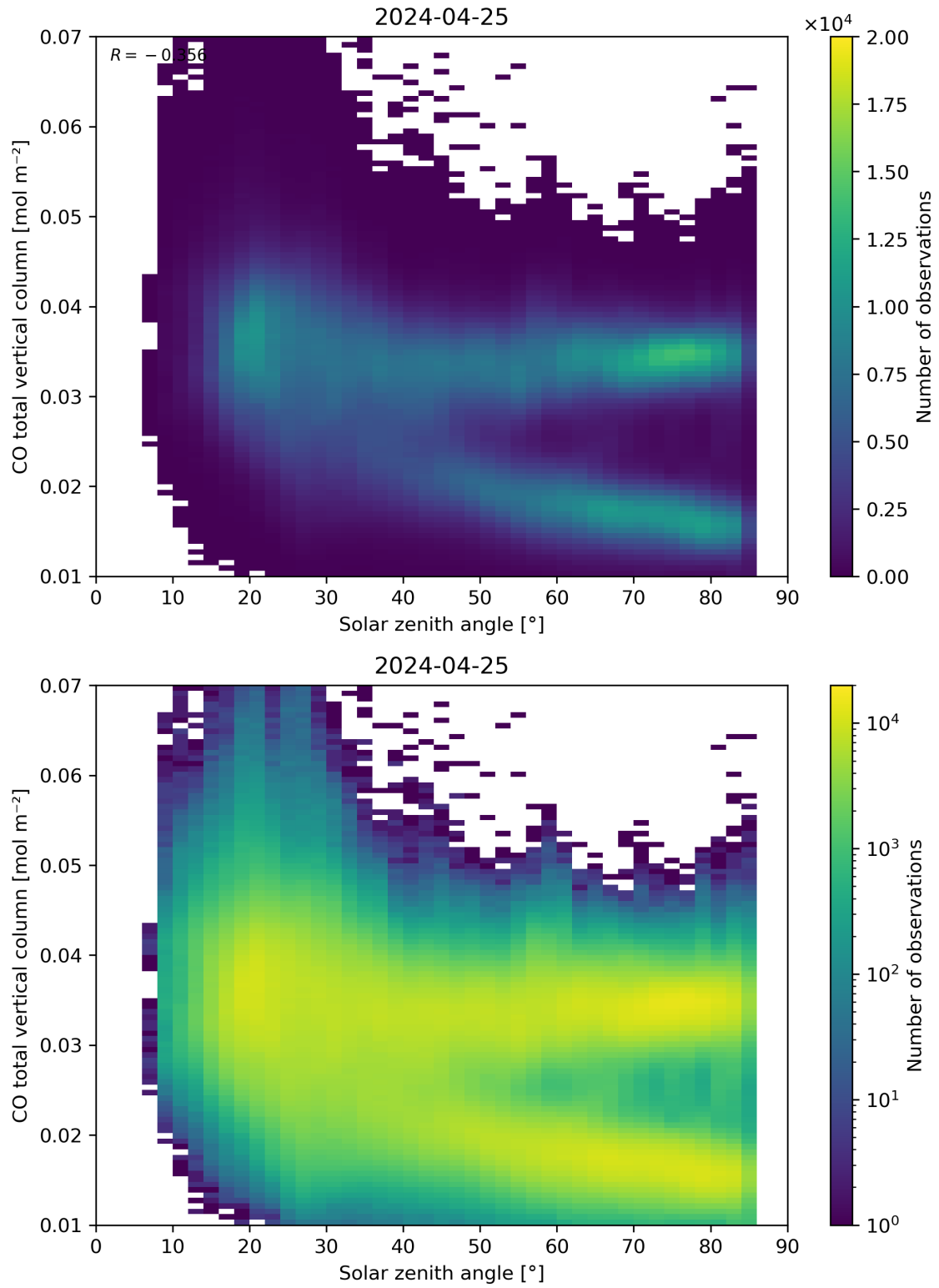
Figure 61: Scatter density plot of “Solar zenith angle” against “CO total vertical column” for 2024-04-24 to 2024-04-26.
