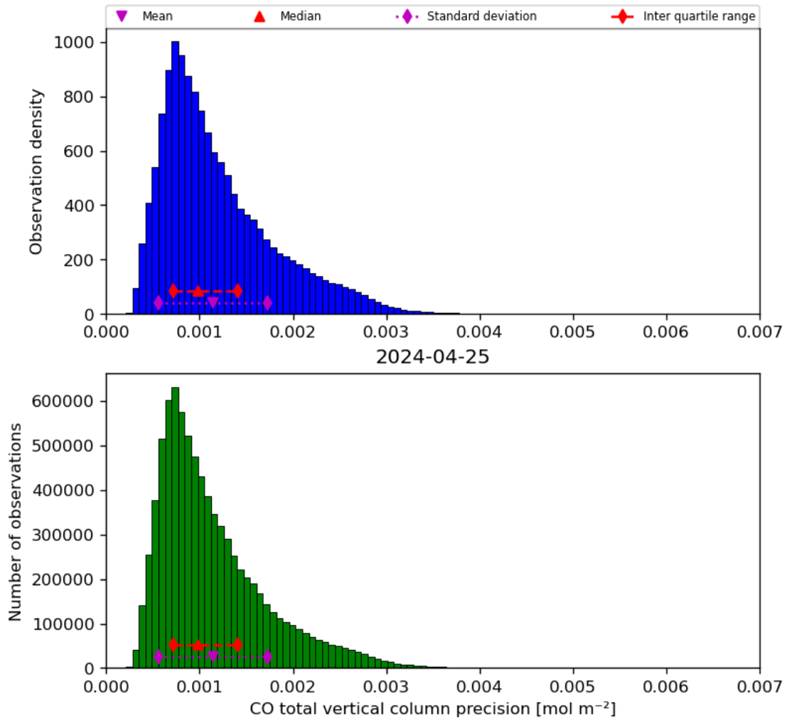
Figure 20: Histogram of “CO total vertical column precision” for 2024-04-24 to 2024-04-26
