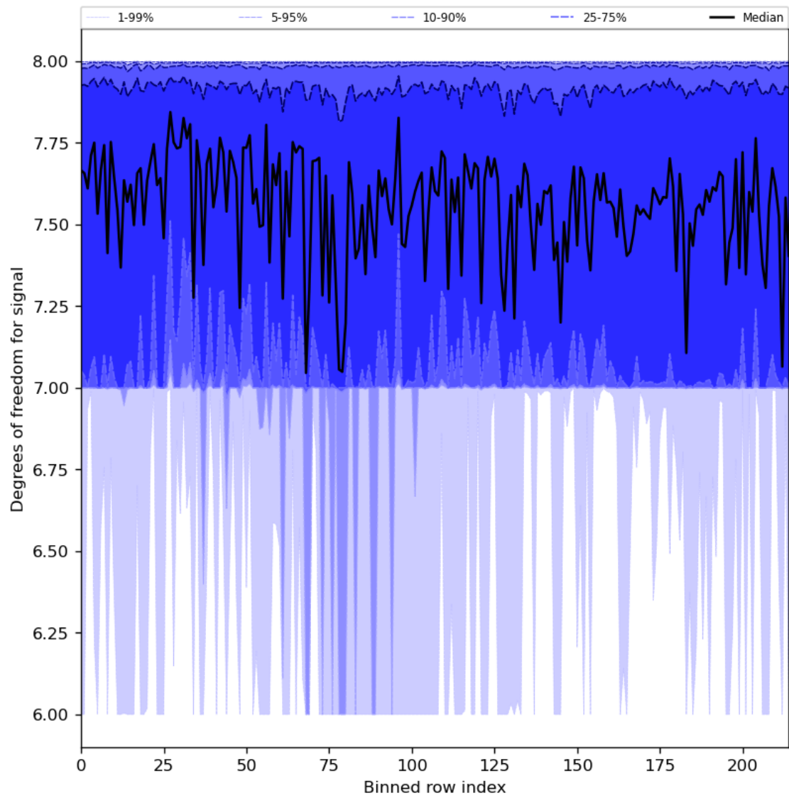
Figure 31: Along track statistics of “Degrees of freedom for signal” for 2024-04-24 to 2024-04-26
