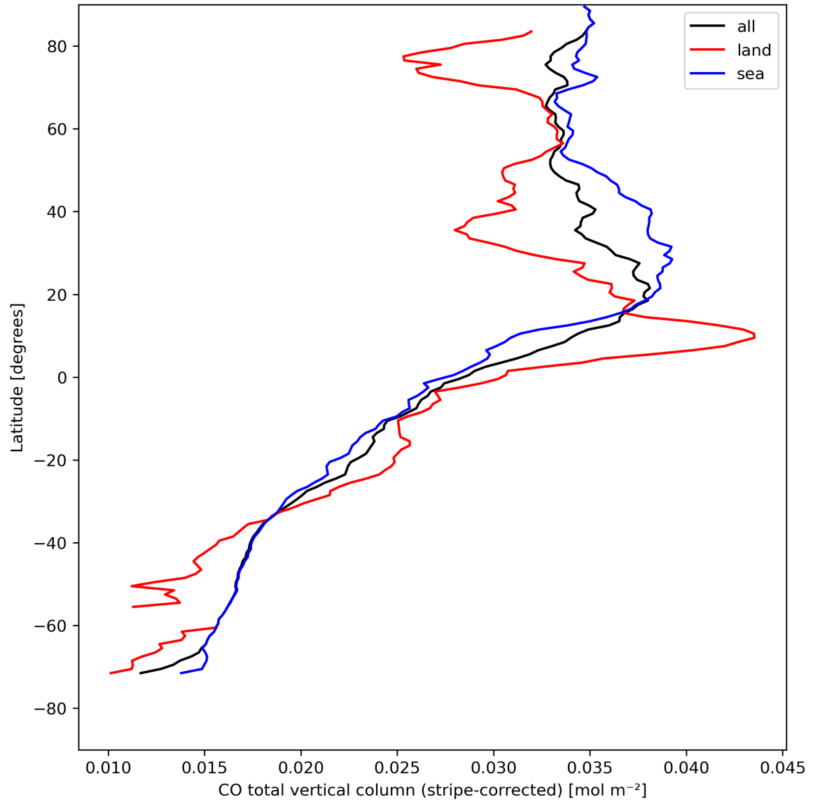
Figure 11: Zonal average of “CO total vertical column (stripe-corrected)” for 2024-04-24 to 2024-04-26.
