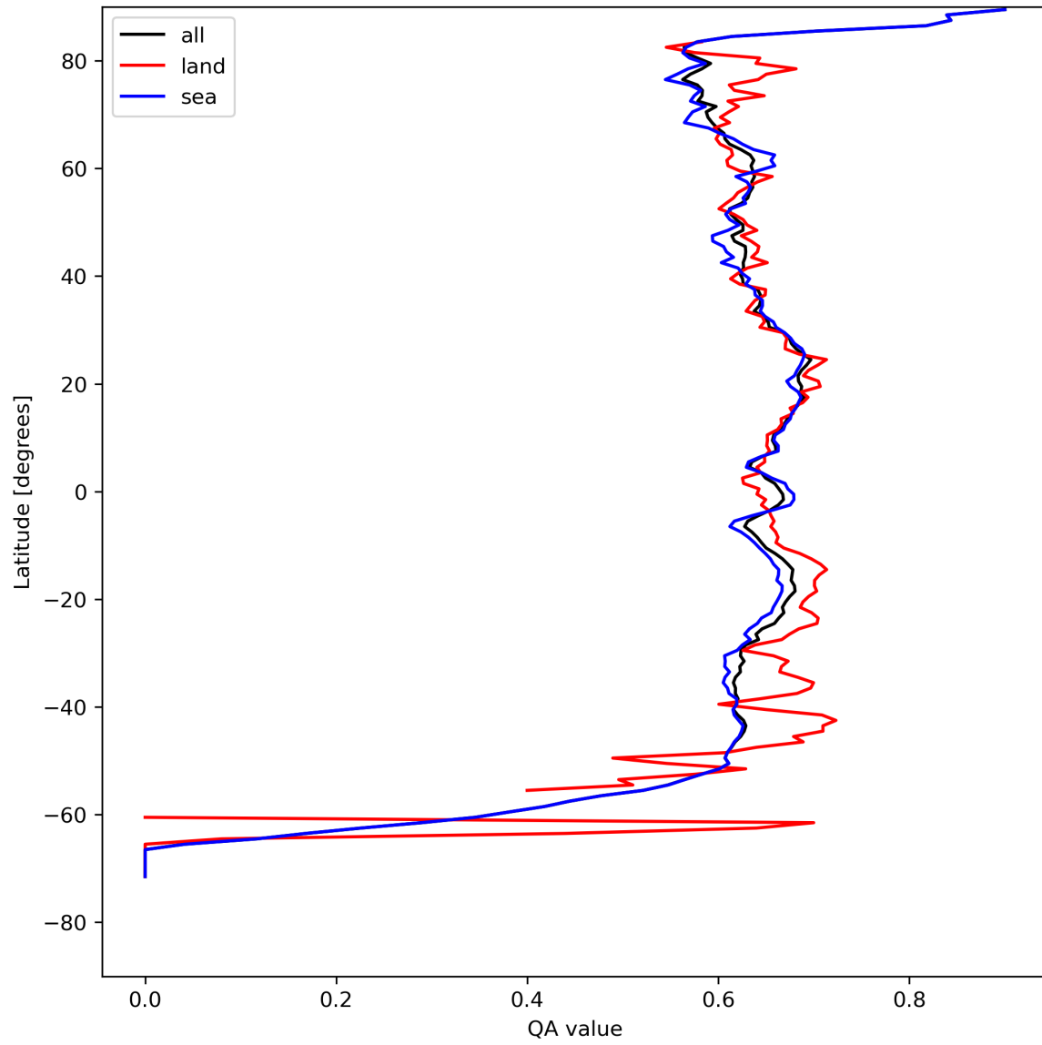
Figure 9: Zonal average of “QA value” for 2024-04-24 to 2024-04-26.
