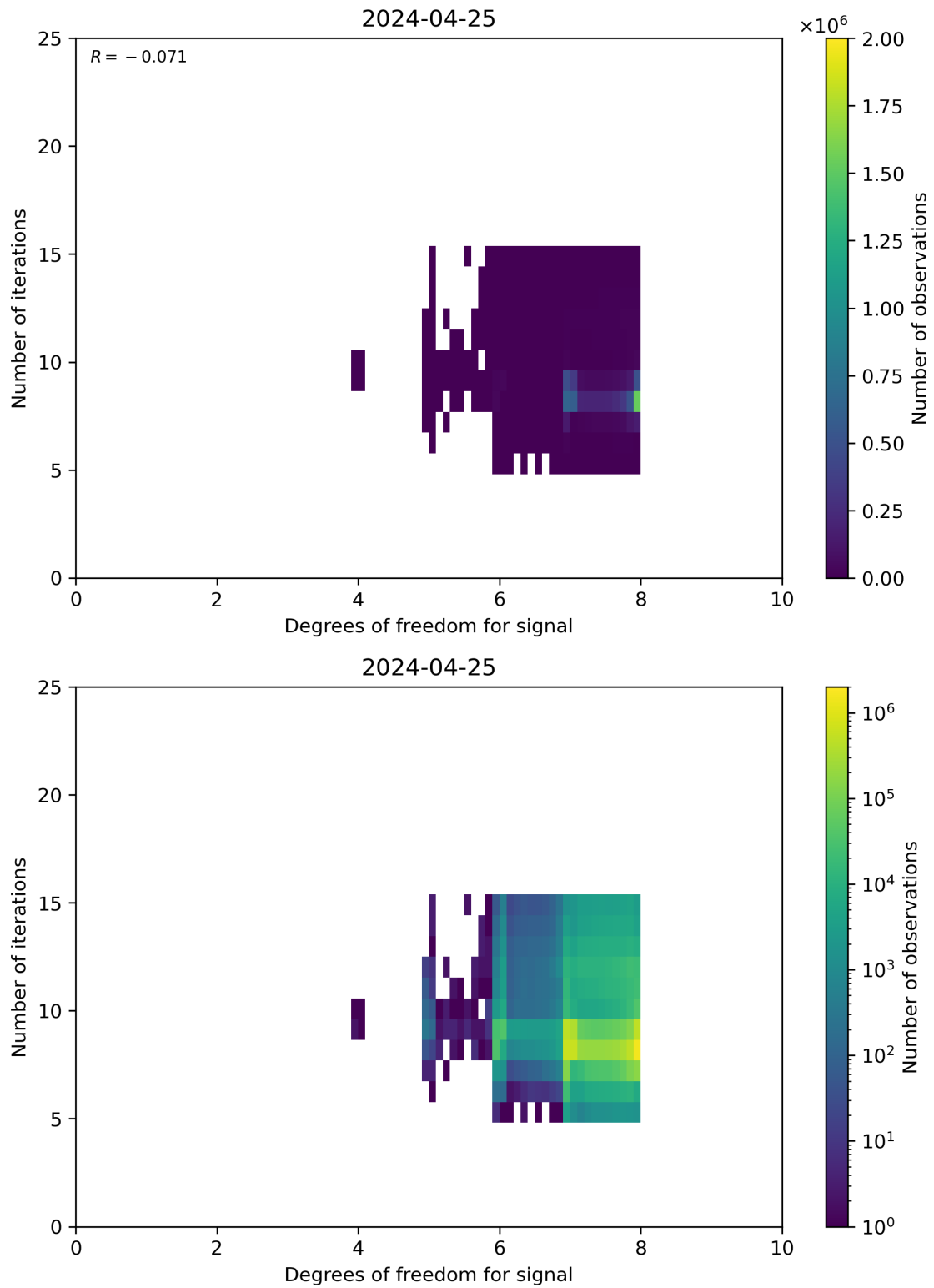
Figure 50: Scatter density plot of “Degrees of freedom for signal” against “Number of iterations” for 2024-04-24 to 2024-04-26.
