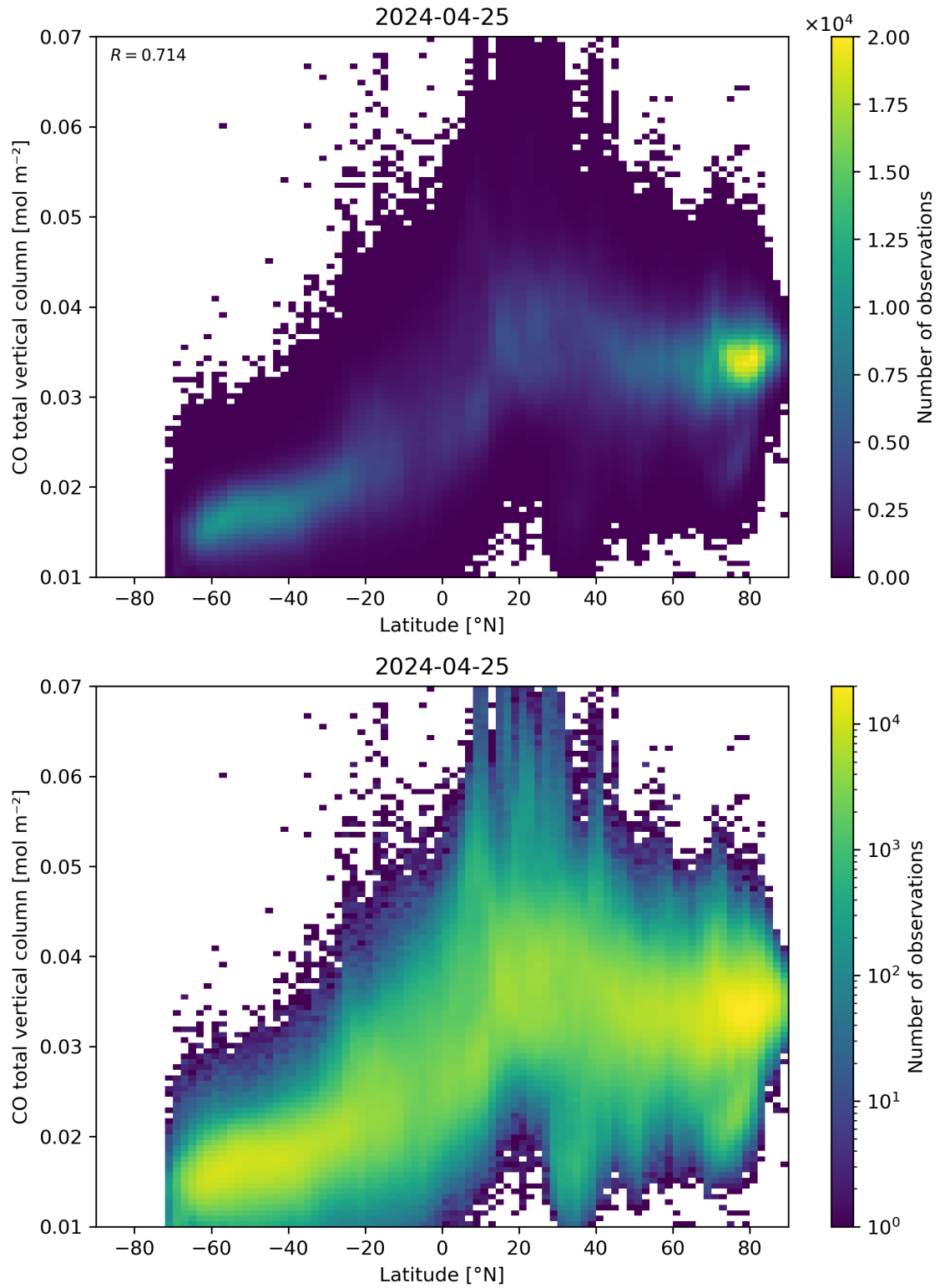
Figure 51: Scatter density plot of “Latitude” against “CO total vertical column” for 2024-04-24 to 2024-04-26.
