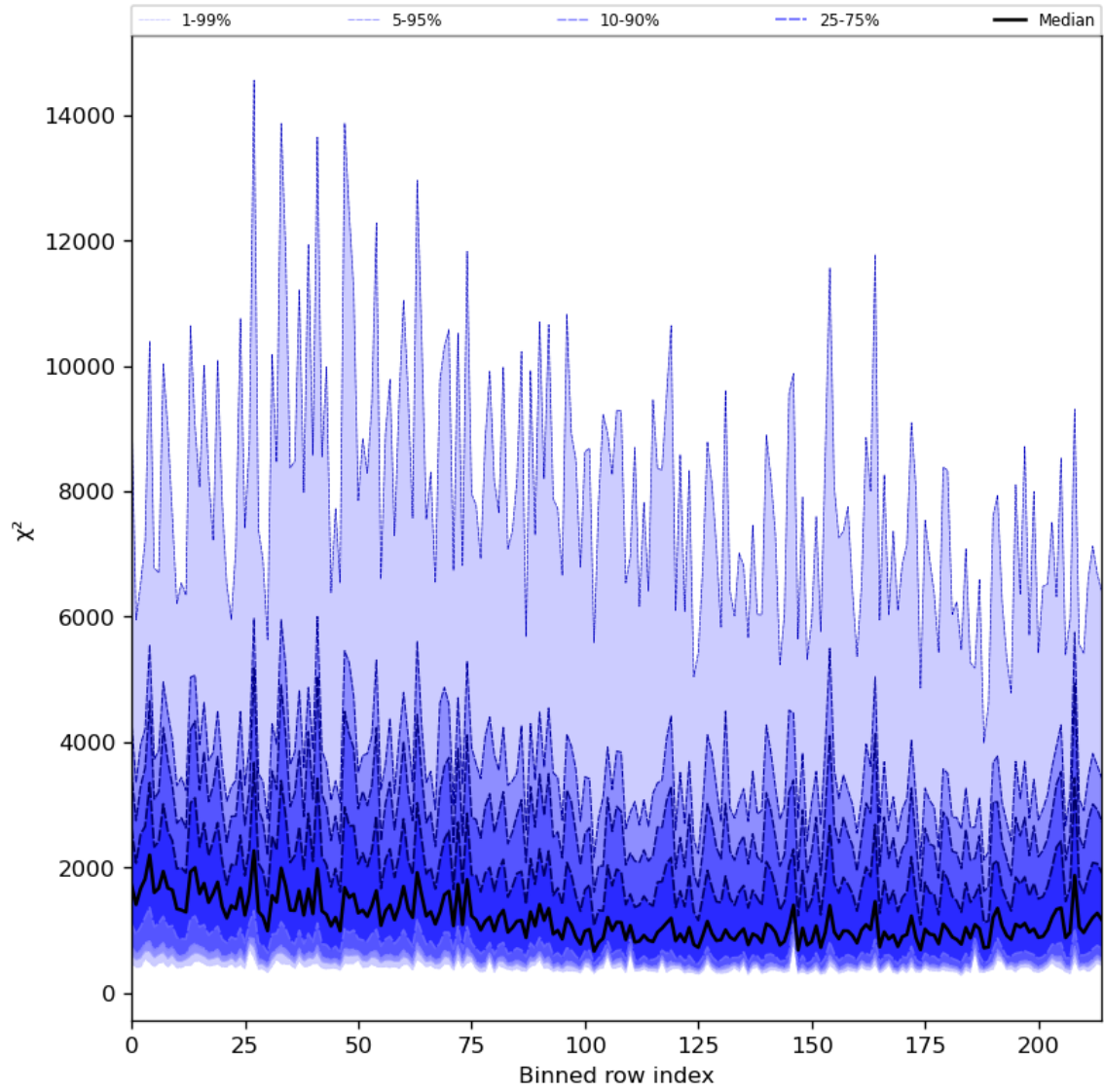
Figure 30: Along track statistics of “ \chi^2 ” for 2024-04-24 to 2024-04-26
