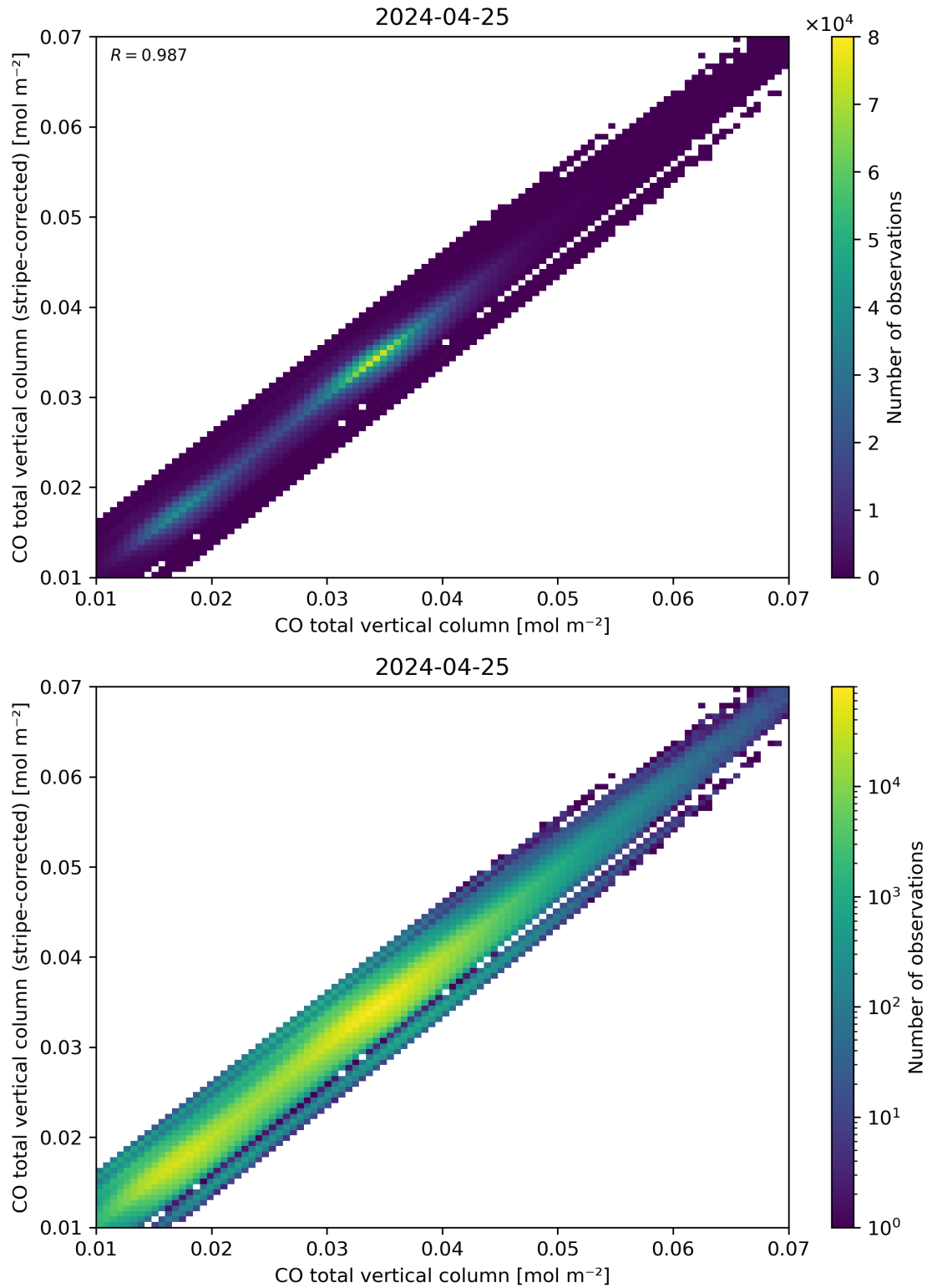
Figure 33: Scatter density plot of “CO total vertical column” against “CO total vertical column (stripe-corrected)” for 2024-04-24 to 2024-04-26.
