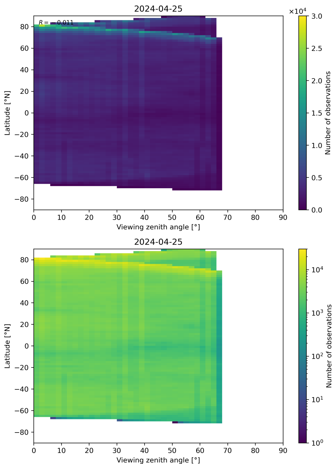
Figure 74: Scatter density plot of “Viewing zenith angle” against “Latitude” for 2024-04-24 to 2024-04-26.
