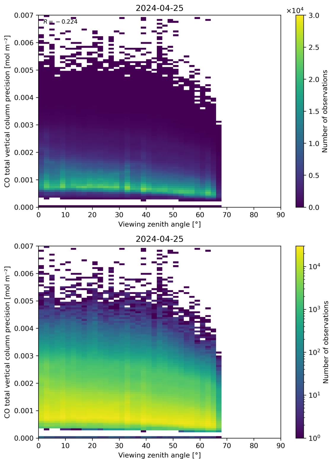
Figure 71: Scatter density plot of “Viewing zenith angle” against “CO total vertical column precision” for 2024-04-24 to 2024-04-26.
