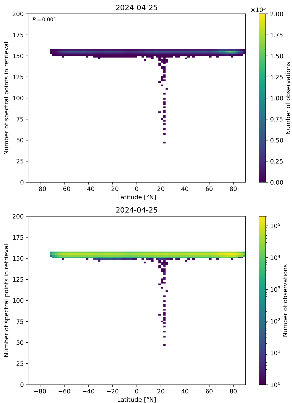
Figure 57: Scatter density plot of “Latitude” against “Number of spectral points in retrieval” for 2024-04-24 to 2024-04-26.
