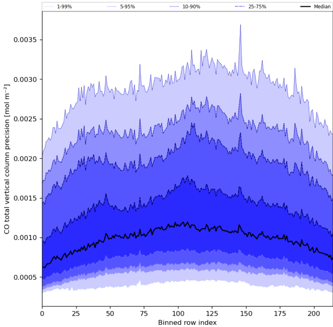
Figure 28: Along track statistics of “CO total vertical column precision” for 2024-04-24 to 2024-04-26
