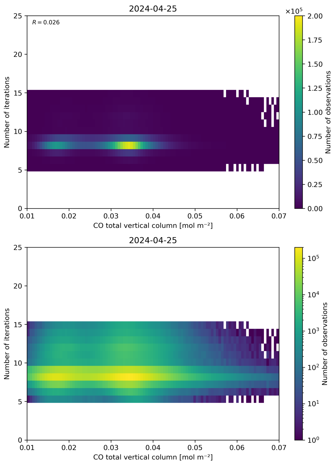
Figure 42: Scatter density plot of “CO total vertical column” against “Number of iterations” for 2024-04-24 to 2024-04-26.
