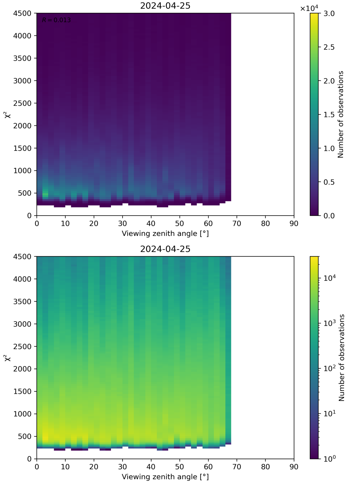
Figure 72: Scatter density plot of “Viewing zenith angle” against “ \chi^2 ” for 2024-04-24 to 2024-04-26.
