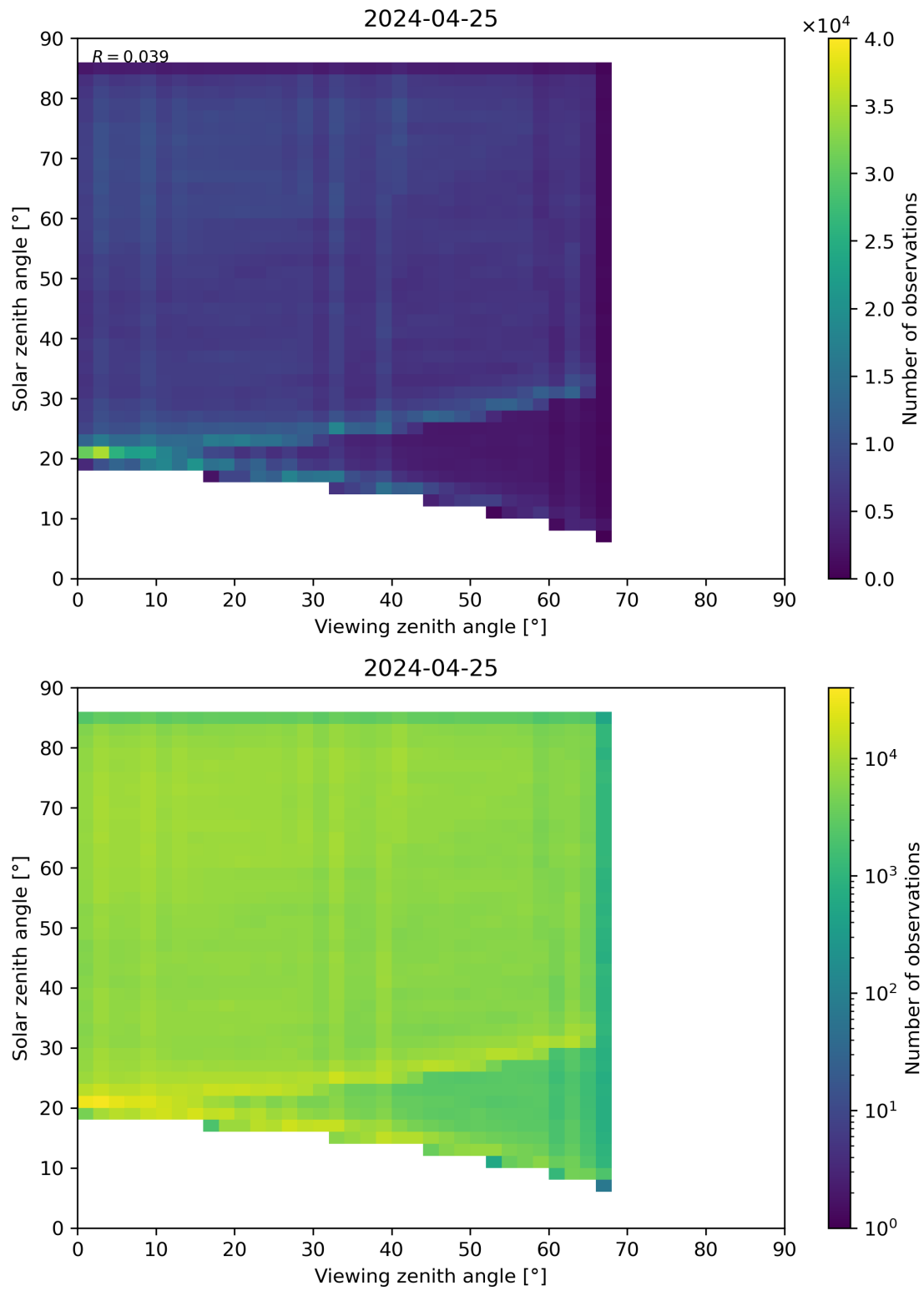
Figure 77: Scatter density plot of “Viewing zenith angle” against “Solar zenith angle” for 2024-04-24 to 2024-04-26.
