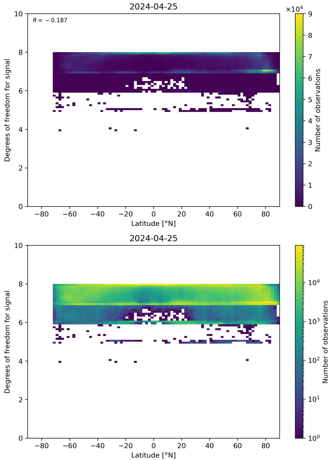
Figure 55: Scatter density plot of “Latitude” against “Degrees of freedom for signal” for 2024-04-24 to 2024-04-26.
