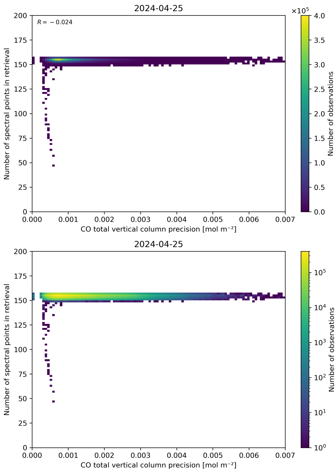
Figure 47: Scatter density plot of “CO total vertical column precision” against “Number of spectral points in retrieval” for 2024-04-24 to 2024-04-26.
