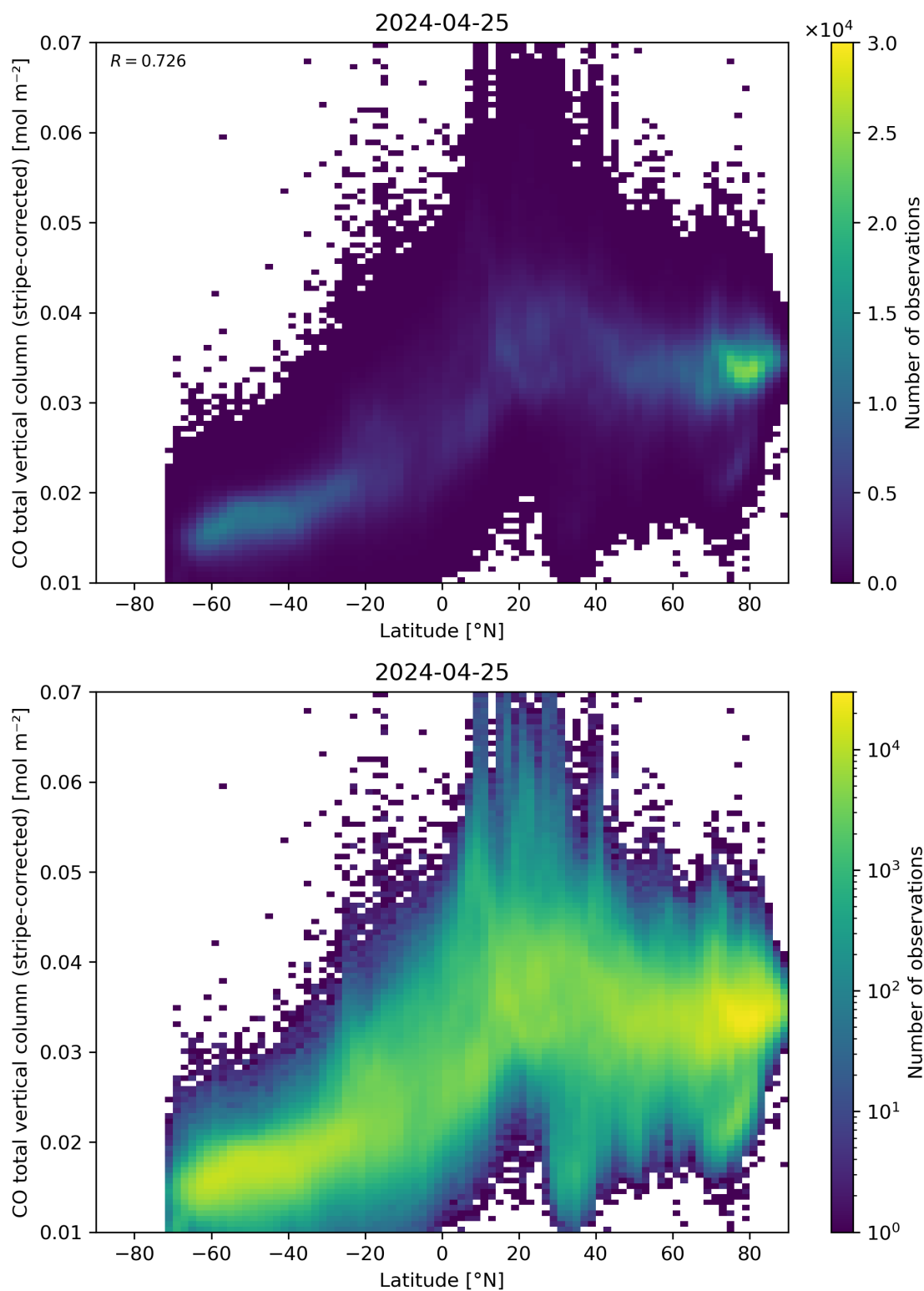
Figure 52: Scatter density plot of “Latitude” against “CO total vertical column (stripe-corrected)” for 2024-04-24 to 2024-04-26.
