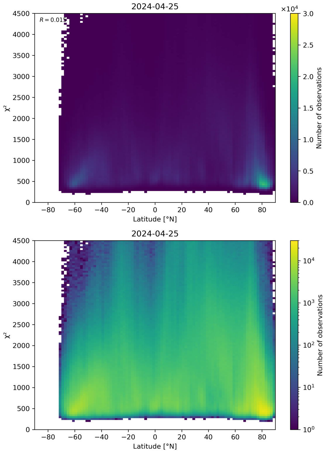
Figure 54: Scatter density plot of “Latitude” against “ \chi^2 ” for 2024-04-24 to 2024-04-26.
