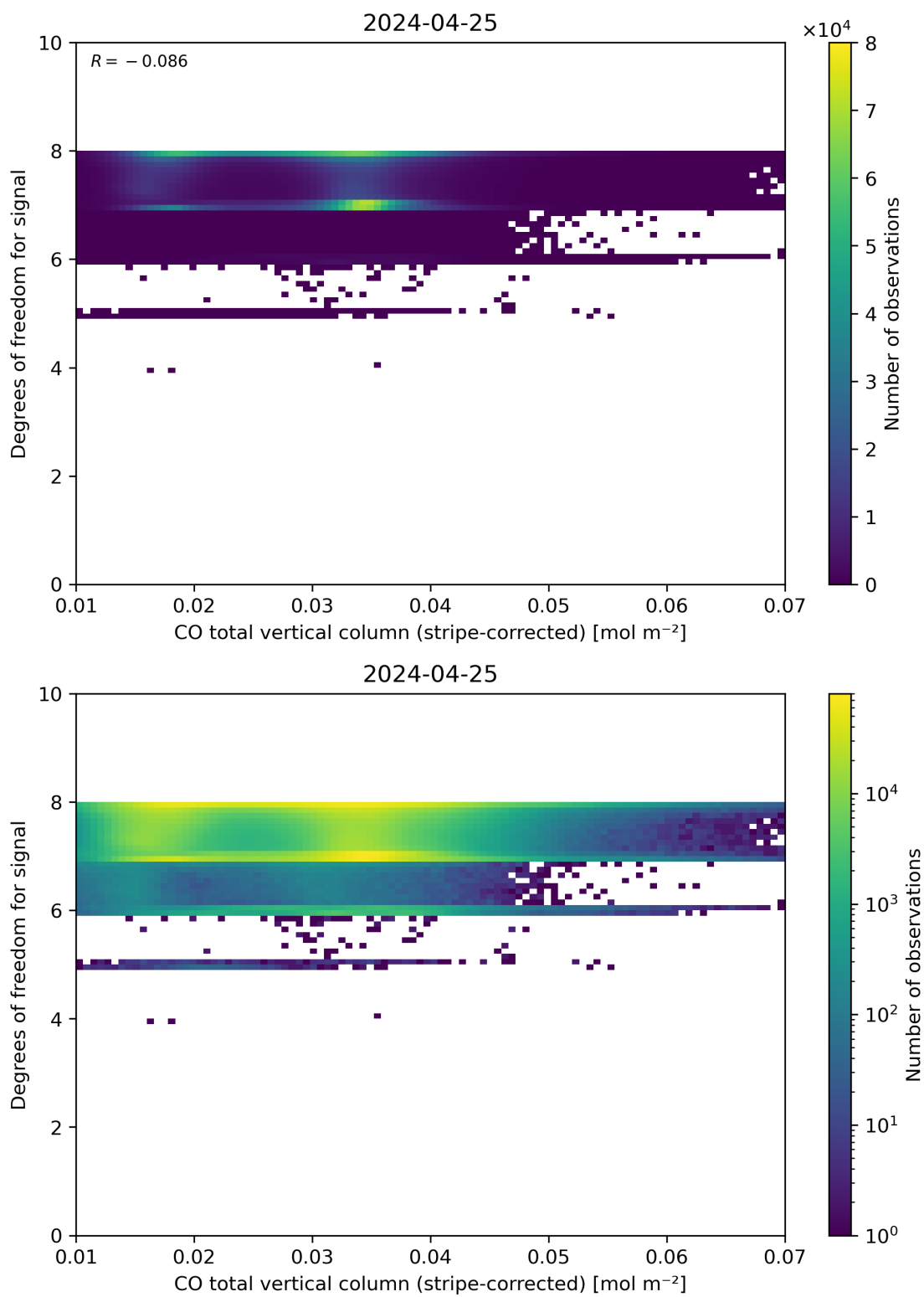
Figure 38: Scatter density plot of “CO total vertical column (stripe-corrected)” against “Degrees of freedom for signal” for 2024-04-24 to 2024-04-26.
