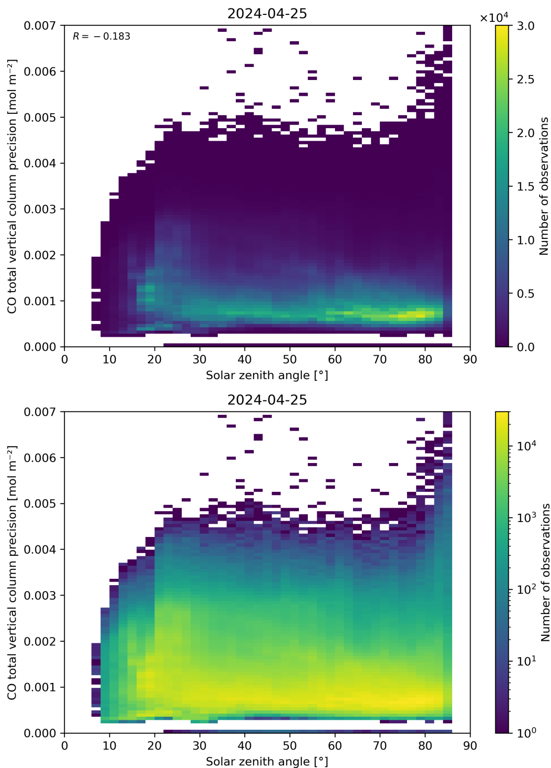
Figure 63: Scatter density plot of “Solar zenith angle” against “CO total vertical column precision” for 2024-04-24 to 2024-04-26.
