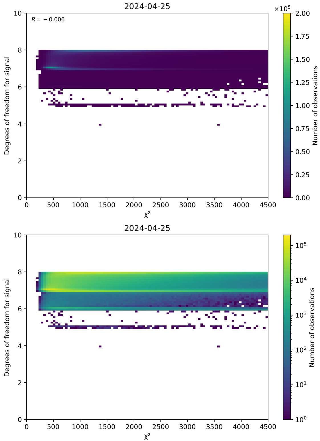
Figure 48: Scatter density plot of “ \chi^2 ” against “Degrees of freedom for signal” for 2024-04-24 to 2024-04-26.
