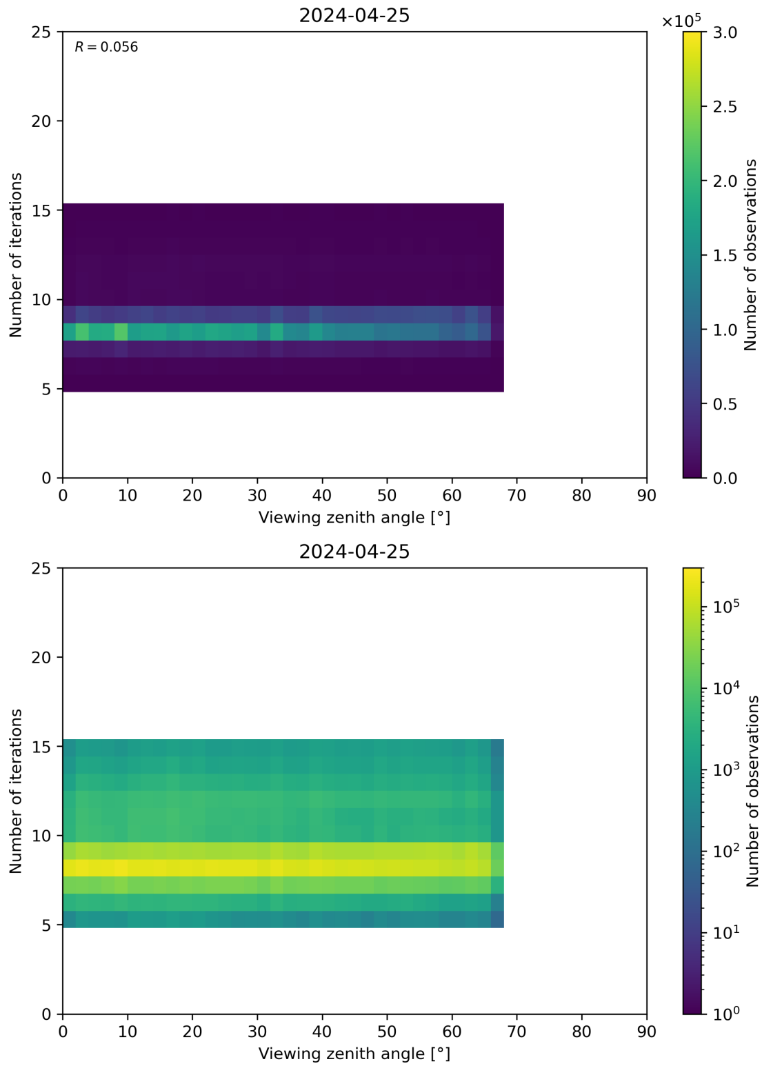
Figure 75: Scatter density plot of “Viewing zenith angle” against “Number of iterations” for 2024-04-24 to 2024-04-26.
