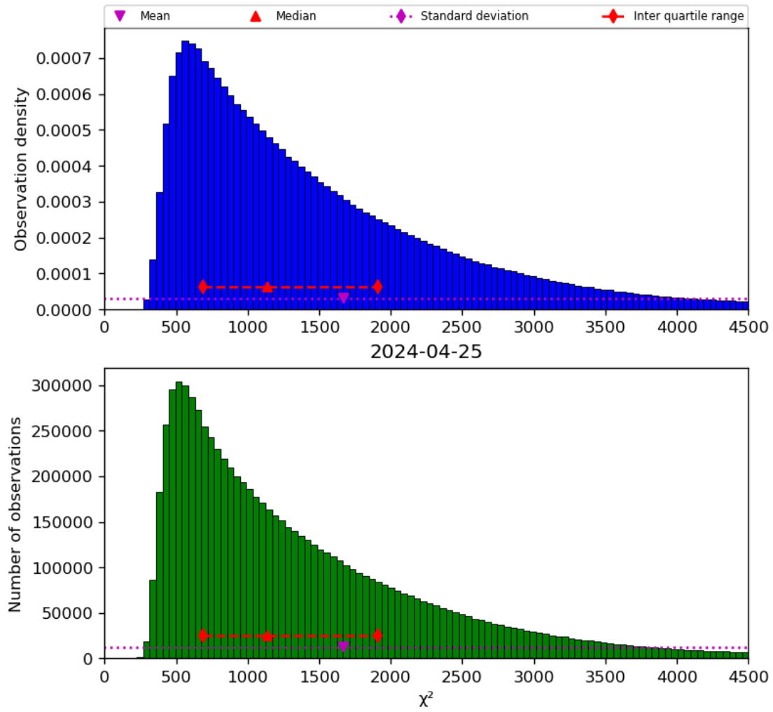
Figure 22: Histogram of “ \chi^2 ” for 2024-04-24 to 2024-04-26
