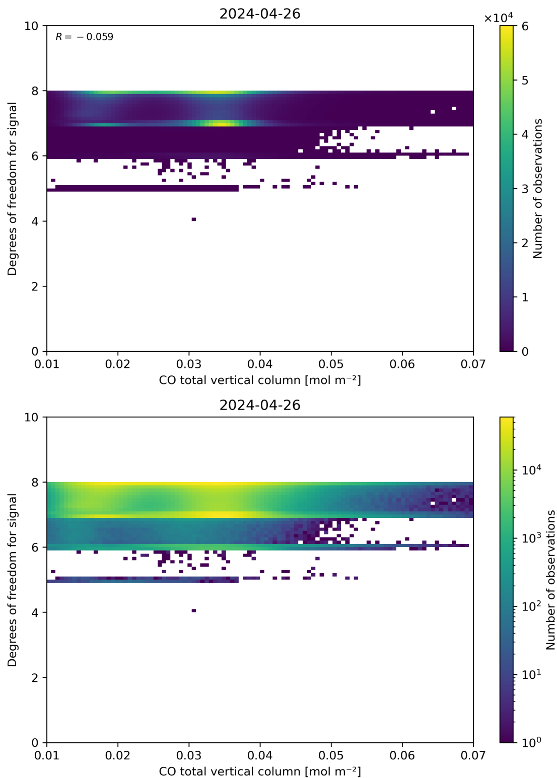
Figure 41: Scatter density plot of “CO total vertical column” against “Degrees of freedom for signal” for 2024-04-26 to 2024-04-27.
