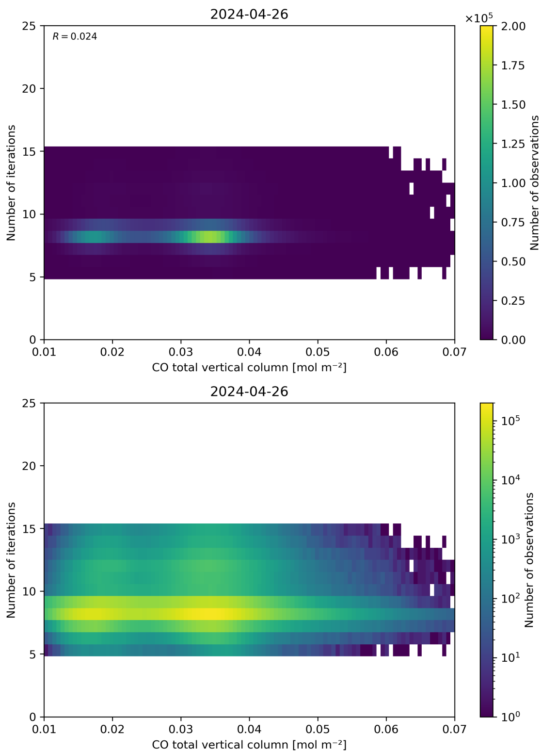
Figure 42: Scatter density plot of “CO total vertical column” against “Number of iterations” for 2024-04-26 to 2024-04-27.
