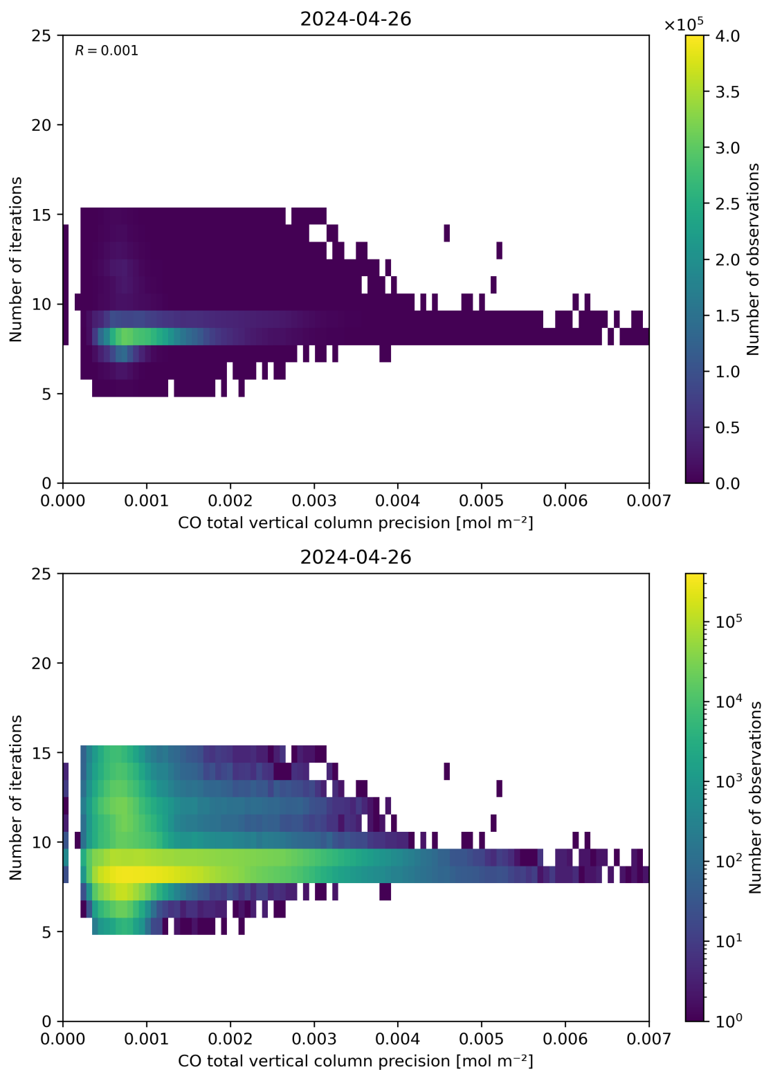
Figure 46: Scatter density plot of “CO total vertical column precision” against “Number of iterations” for 2024-04-26 to 2024-04-27.
