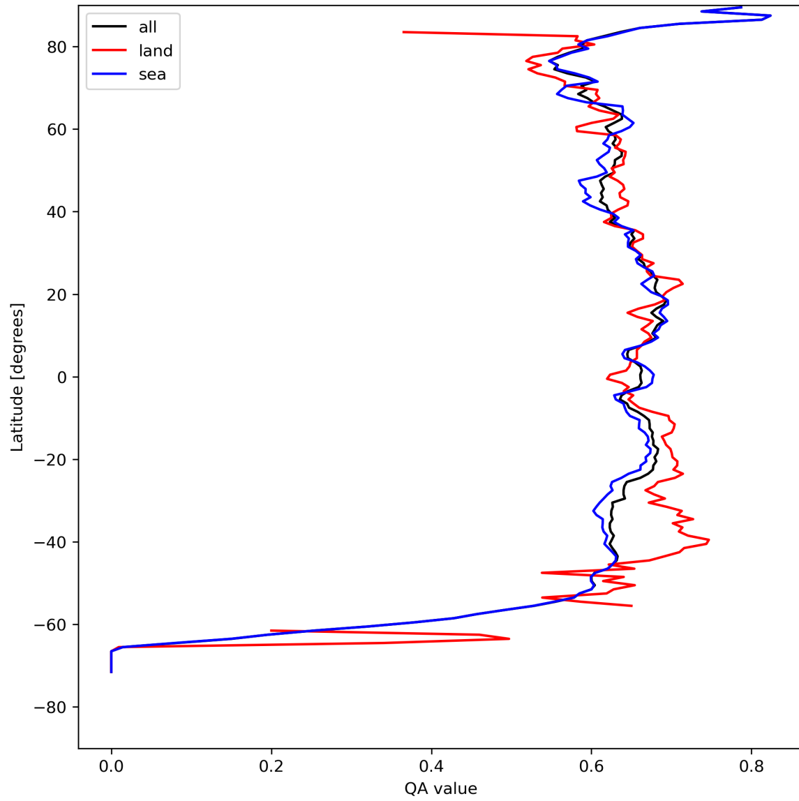
Figure 9: Zonal average of “QA value” for 2024-04-26 to 2024-04-27.
