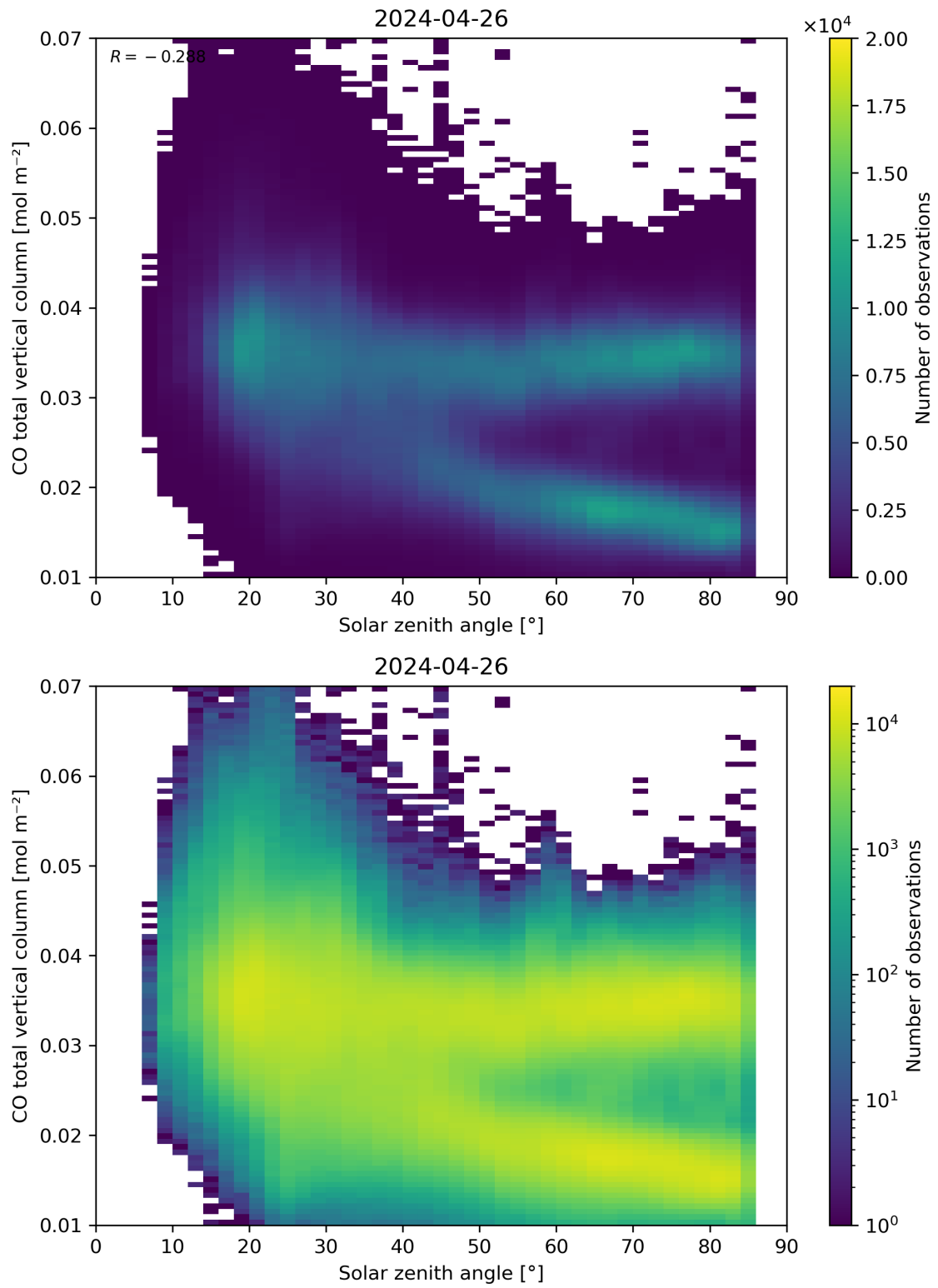
Figure 61: Scatter density plot of “Solar zenith angle” against “CO total vertical column” for 2024-04-26 to 2024-04-27.
