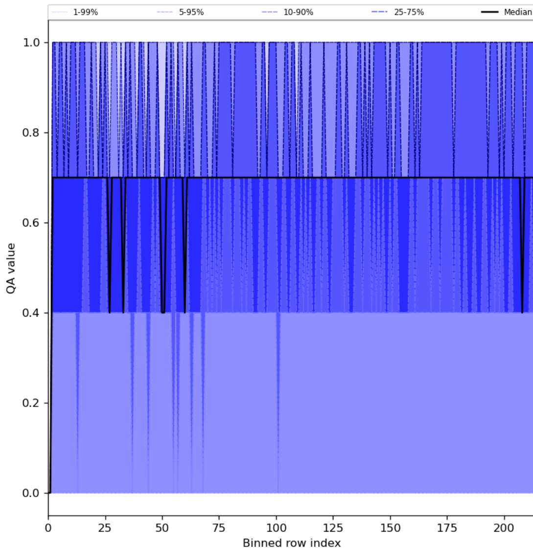
Figure 25: Along track statistics of “QA value” for 2024-04-26 to 2024-04-27
