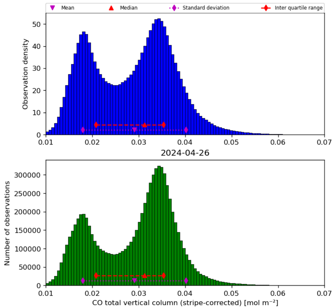
Figure 19: Histogram of “CO total vertical column (stripe-corrected)” for 2024-04-26 to 2024-04-27
