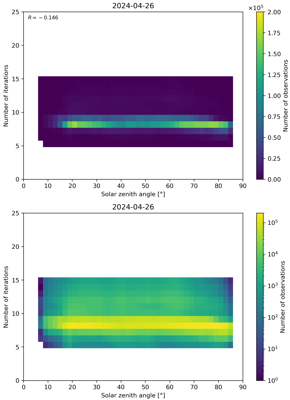
Figure 67: Scatter density plot of “Solar zenith angle” against “Number of iterations” for 2024-04-26 to 2024-04-27.
