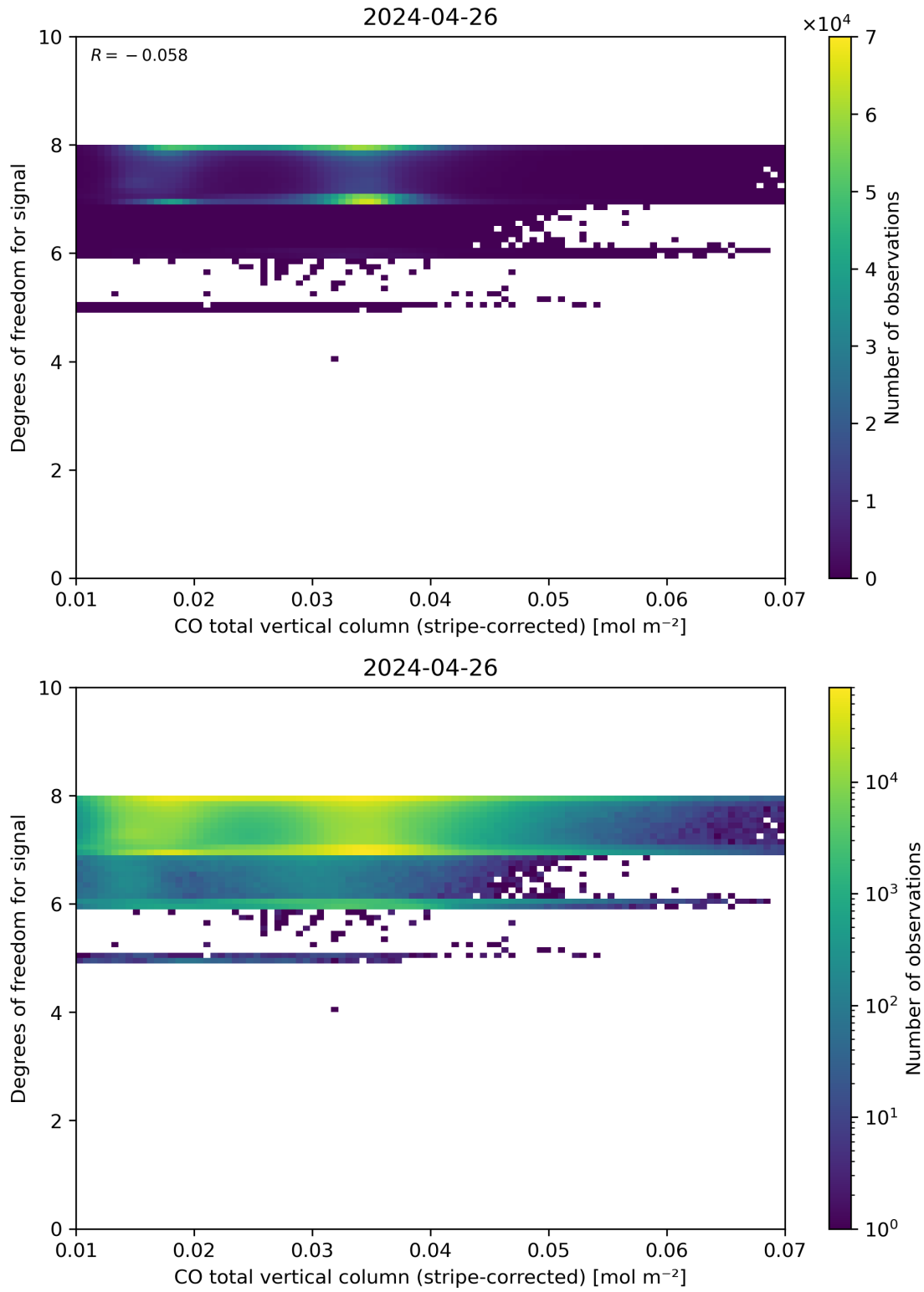
Figure 38: Scatter density plot of “CO total vertical column (stripe-corrected)” against “Degrees of freedom for signal” for 2024-04-26 to 2024-04-27.
