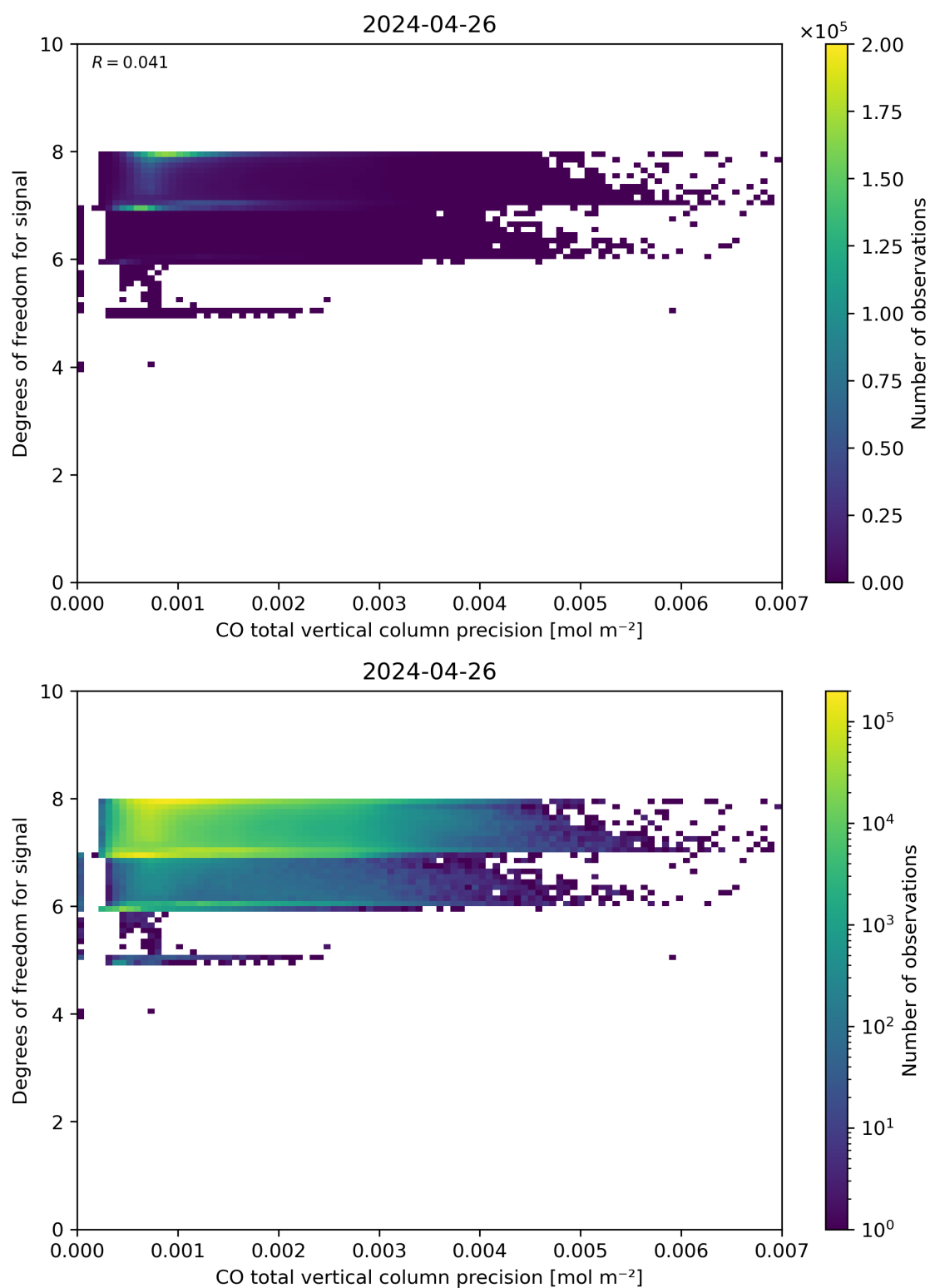
Figure 45: Scatter density plot of “CO total vertical column precision” against “Degrees of freedom for signal” for 2024-04-26 to 2024-04-27.
