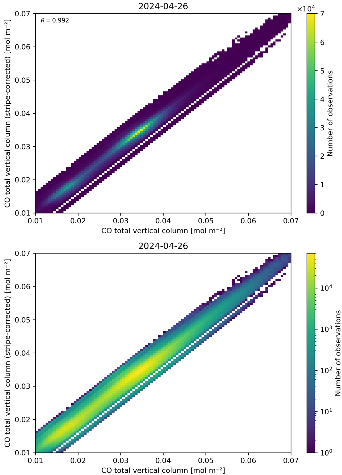
Figure 33: Scatter density plot of “CO total vertical column” against “CO total vertical column (stripe-corrected)” for 2024-04-26 to 2024-04-27.
