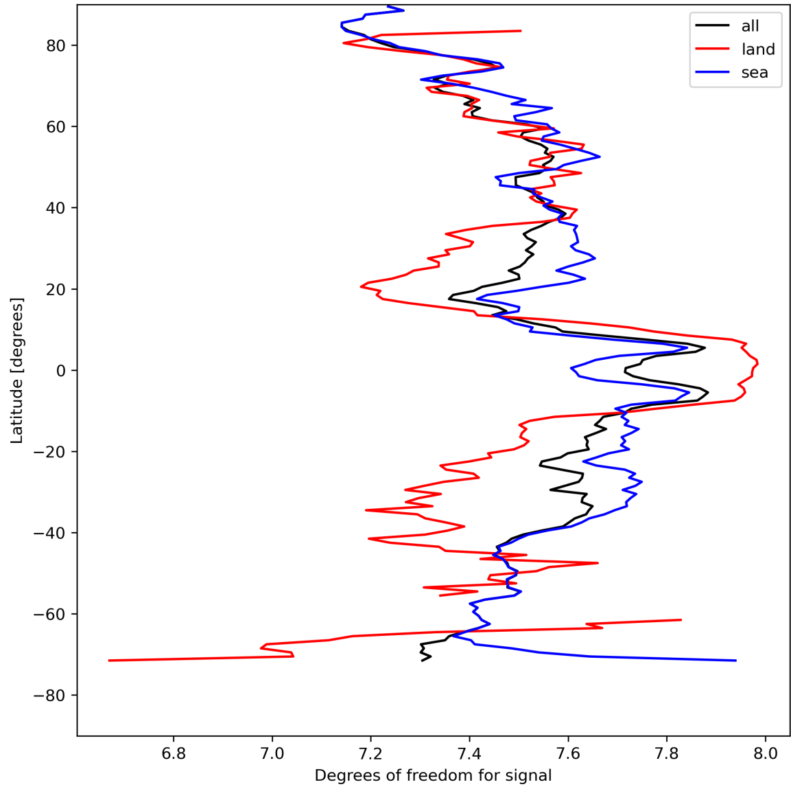
Figure 15: Zonal average of “Degrees of freedom for signal” for 2024-04-26 to 2024-04-27.
