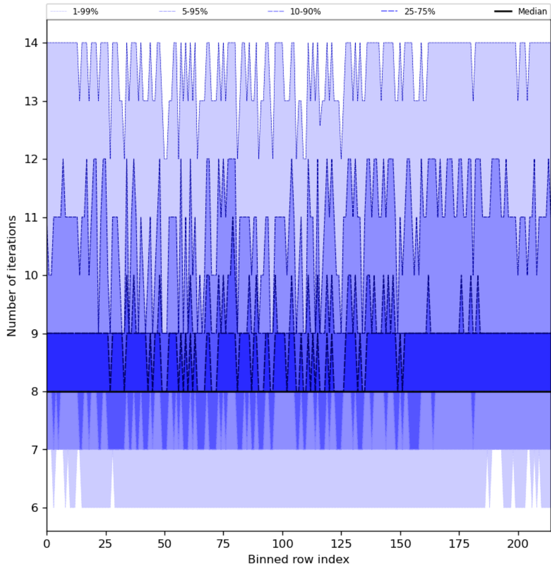
Figure 32: Along track statistics of “Number of iterations” for 2024-04-26 to 2024-04-27
