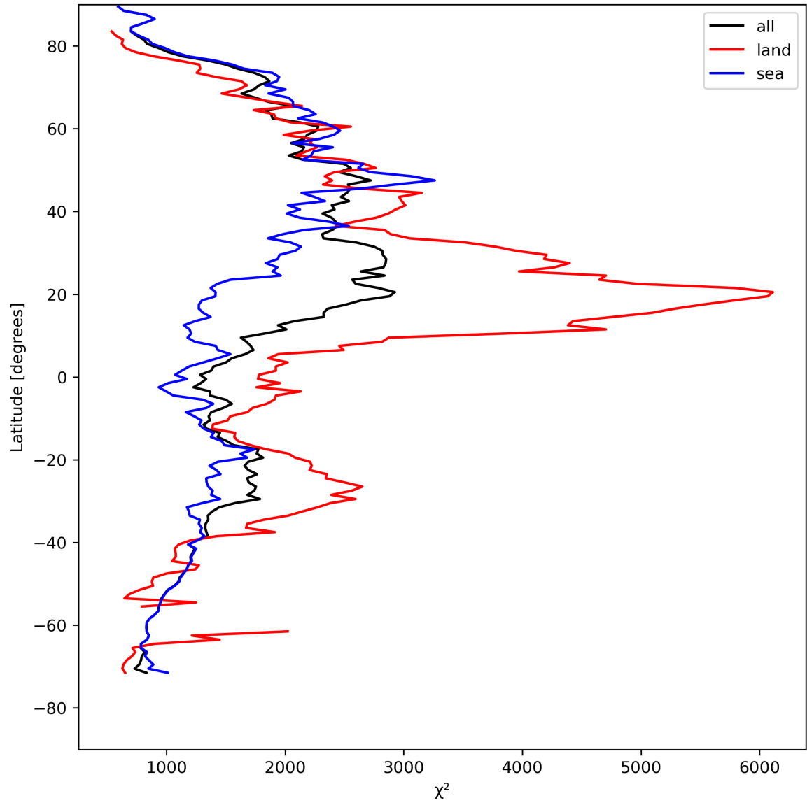
Figure 14: Zonal average of “ \chi^2 ” for 2024-04-26 to 2024-04-27.
