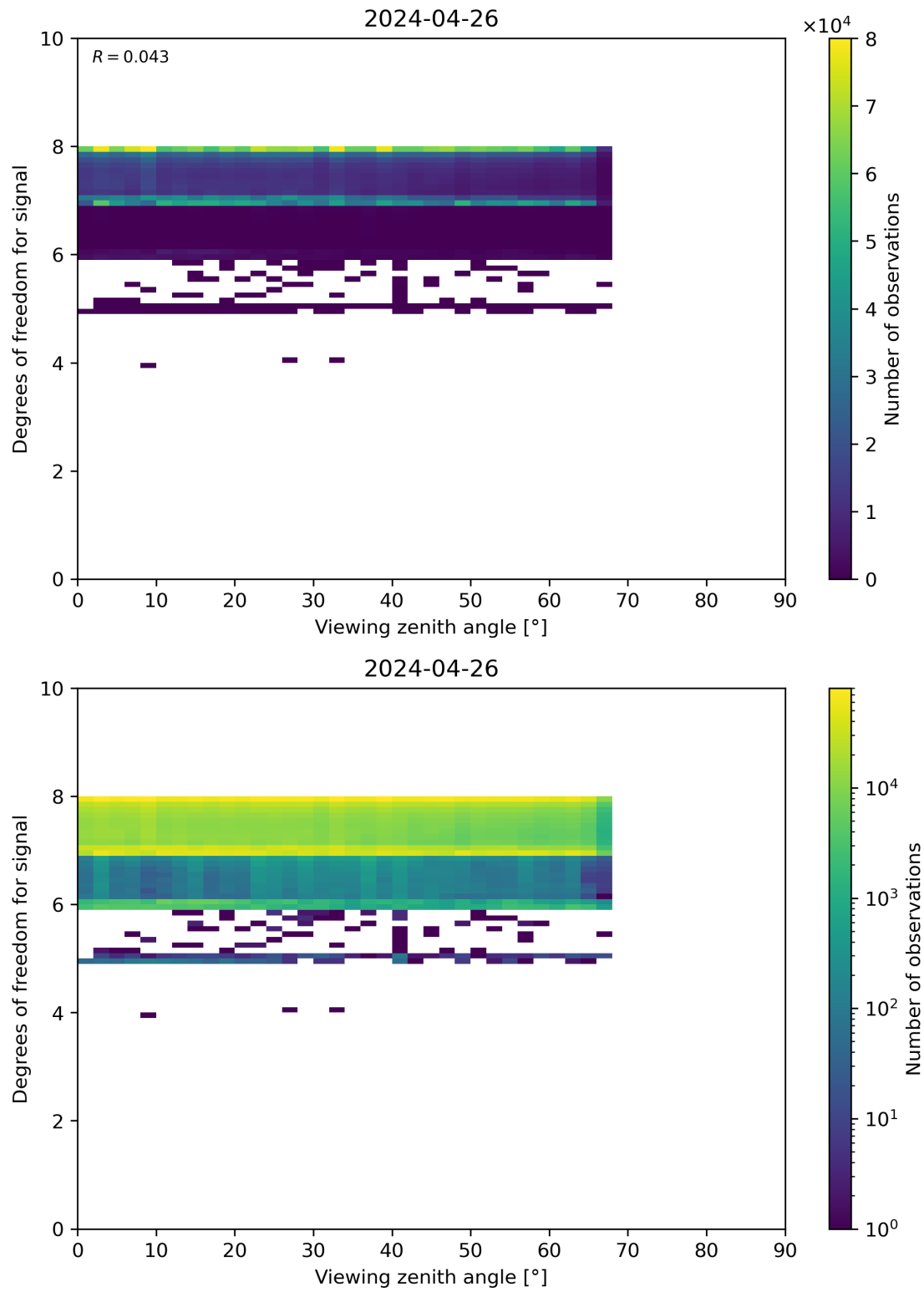
Figure 73: Scatter density plot of “Viewing zenith angle” against “Degrees of freedom for signal” for 2024-04-26 to 2024-04-27.
