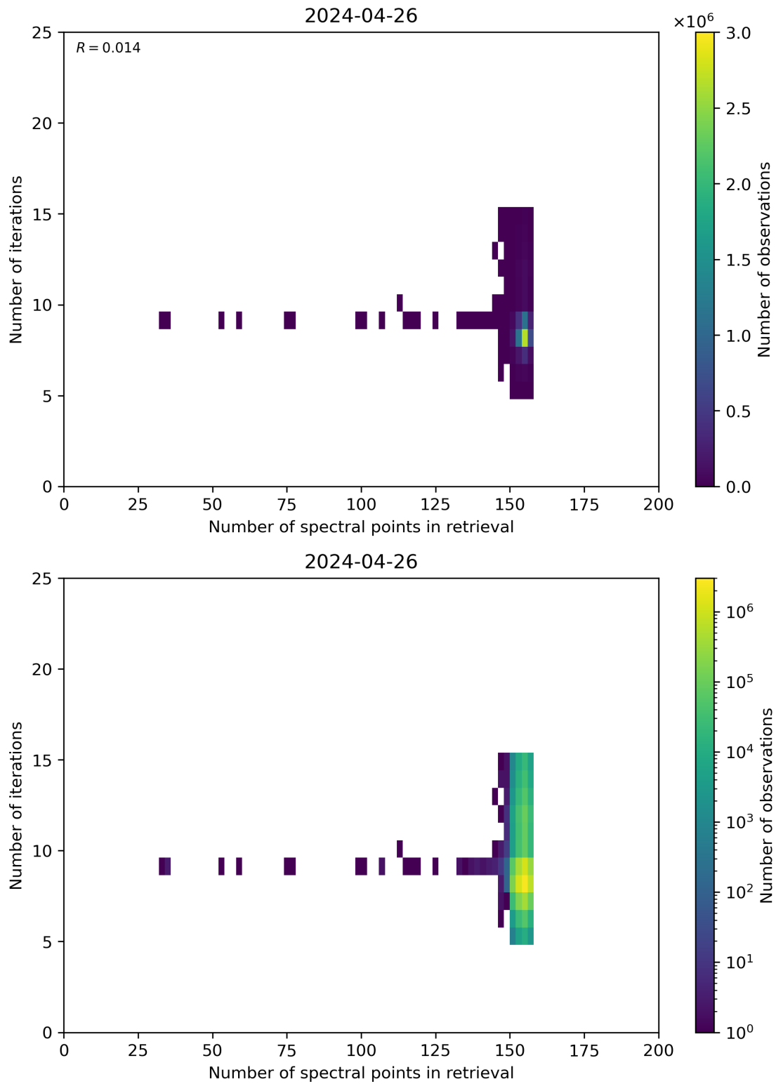
Figure 60: Scatter density plot of “Number of spectral points in retrieval” against “Number of iterations” for 2024-04-26 to 2024-04-27.
