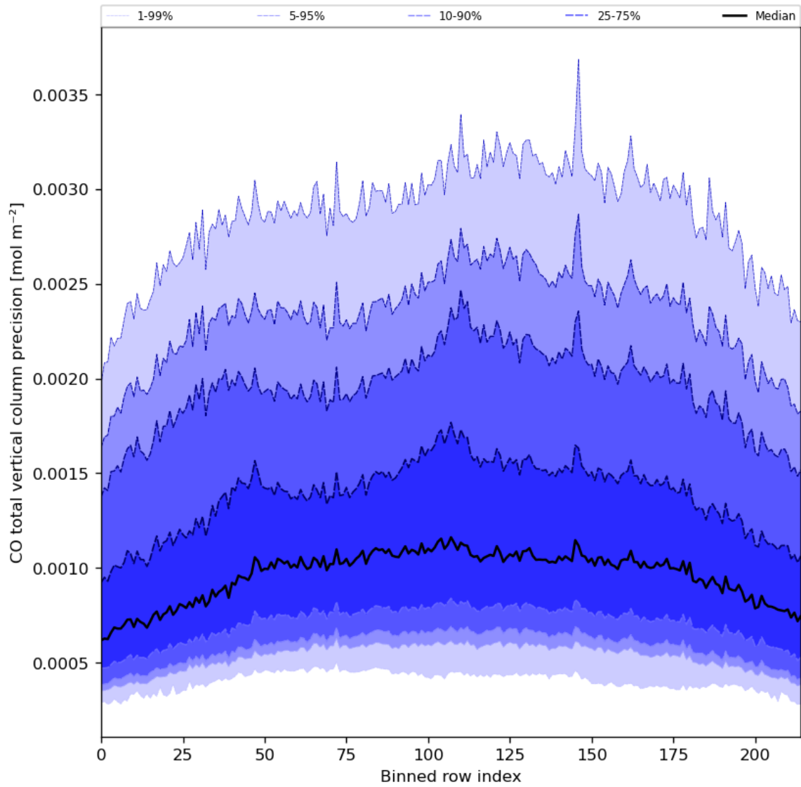
Figure 28: Along track statistics of “CO total vertical column precision” for 2024-04-26 to 2024-04-27
