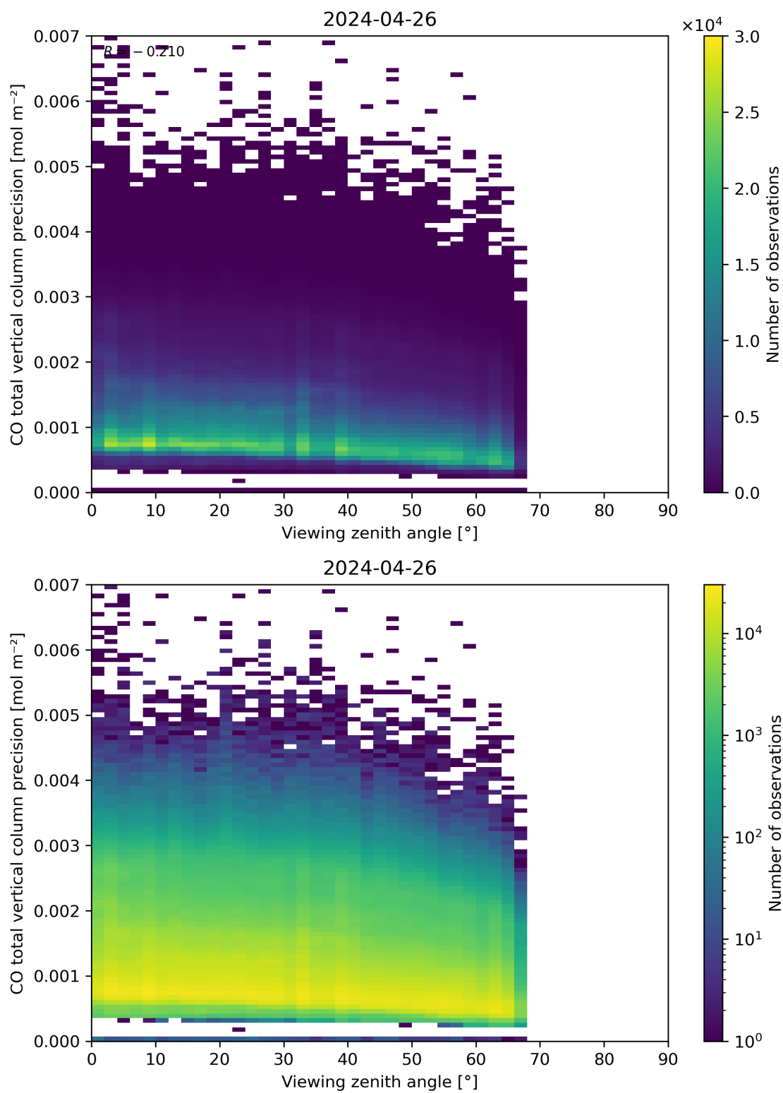
Figure 71: Scatter density plot of “Viewing zenith angle” against “CO total vertical column precision” for 2024-04-26 to 2024-04-27.
