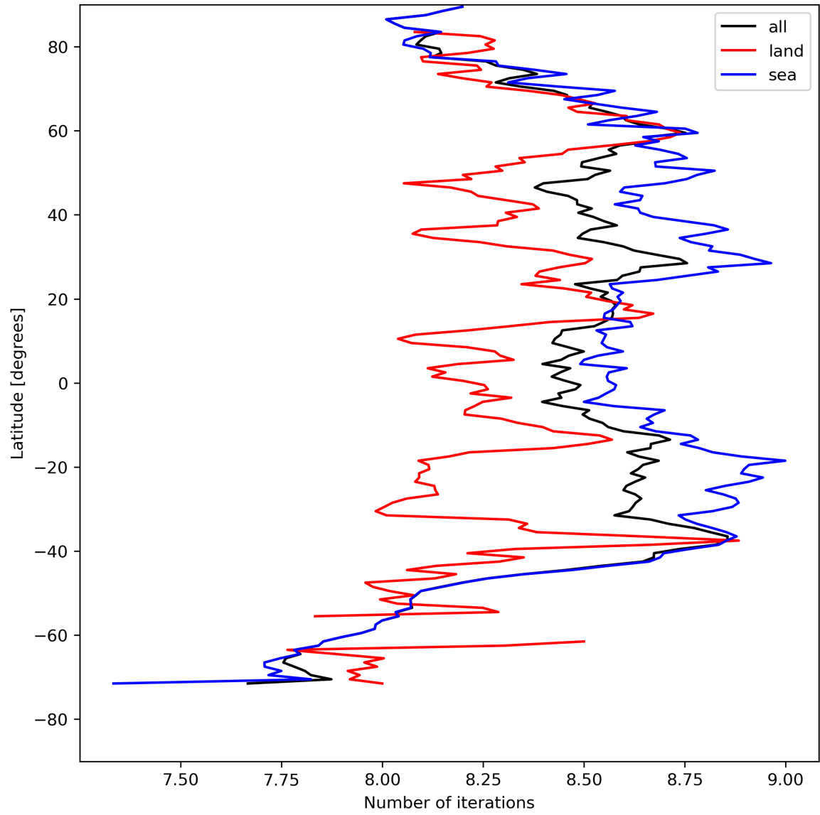
Figure 16: Zonal average of “Number of iterations” for 2024-04-26 to 2024-04-27.
