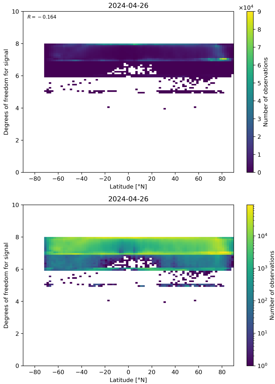
Figure 55: Scatter density plot of “Latitude” against “Degrees of freedom for signal” for 2024-04-26 to 2024-04-27.
