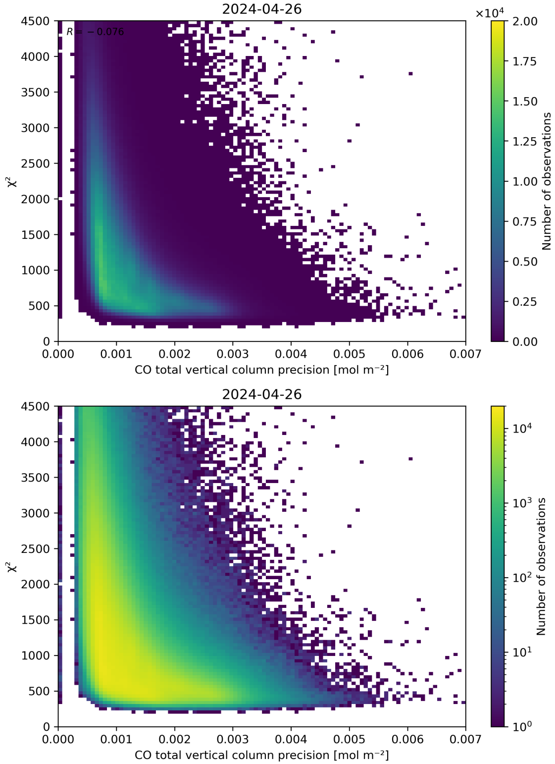
Figure 44: Scatter density plot of “CO total vertical column precision” against “ \chi^2 ” for 2024-04-26 to 2024-04-27.
