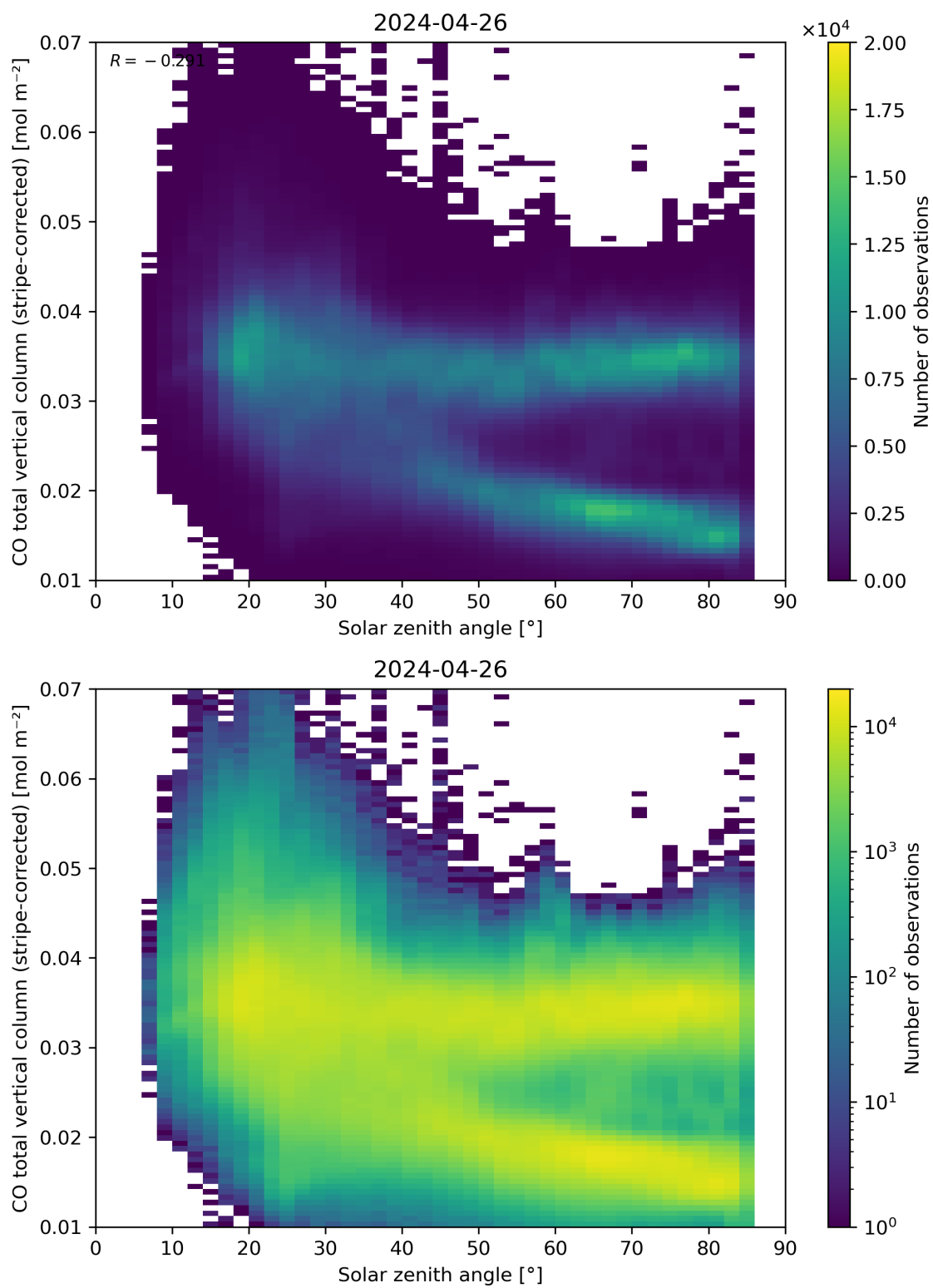
Figure 62: Scatter density plot of “Solar zenith angle” against “CO total vertical column (stripe-corrected)” for 2024-04-26 to 2024-04-27.
