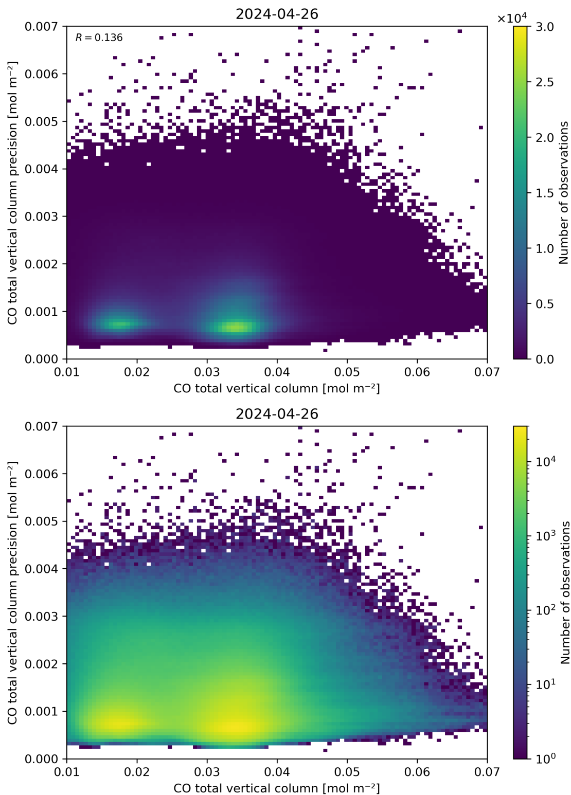
Figure 34: Scatter density plot of “CO total vertical column” against “CO total vertical column precision” for 2024-04-26 to 2024-04-27.
