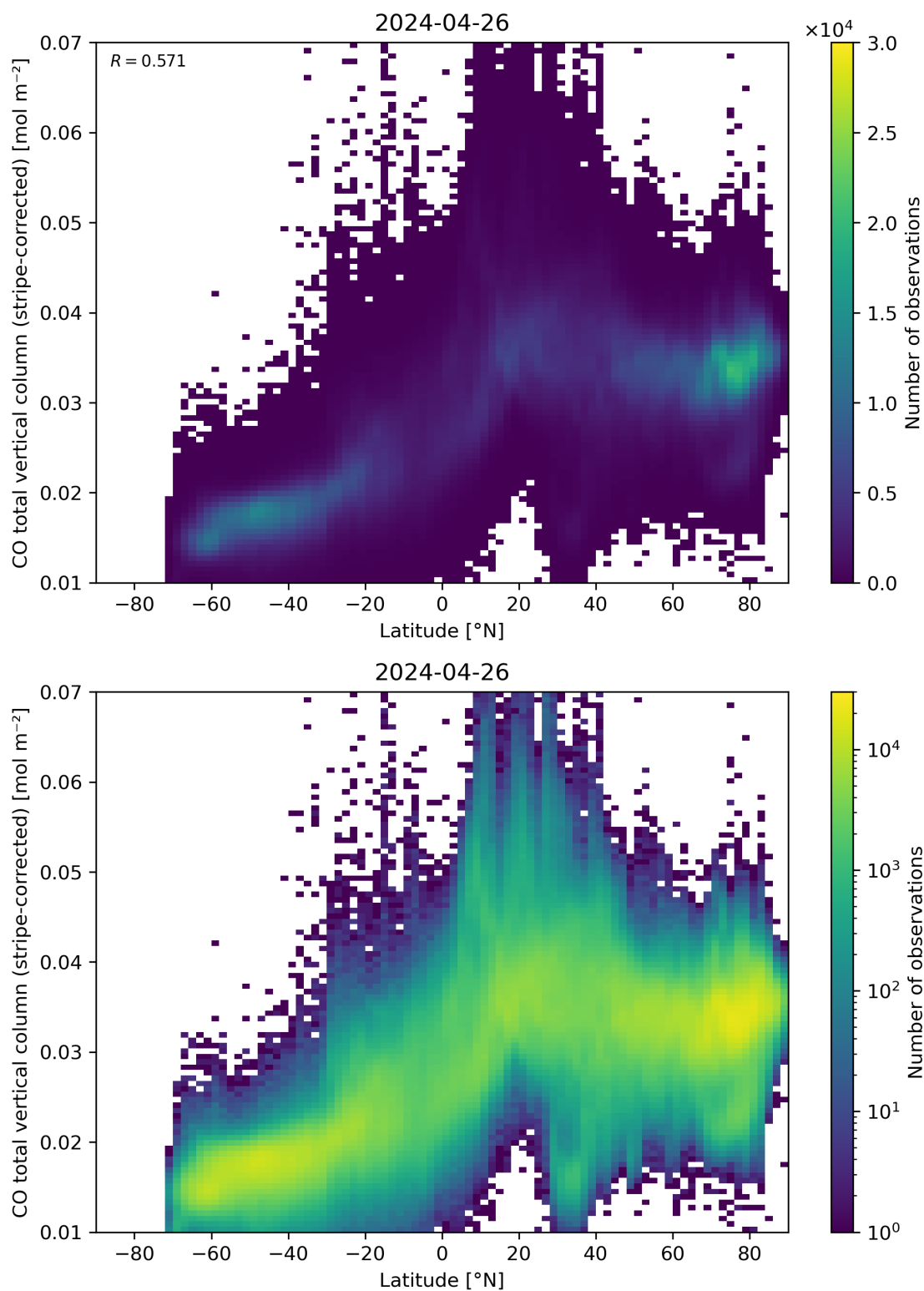
Figure 52: Scatter density plot of “Latitude” against “CO total vertical column (stripe-corrected)” for 2024-04-26 to 2024-04-27.
