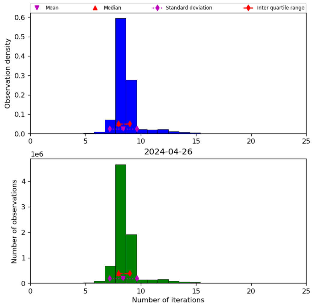
Figure 24: Histogram of “Number of iterations” for 2024-04-26 to 2024-04-27
