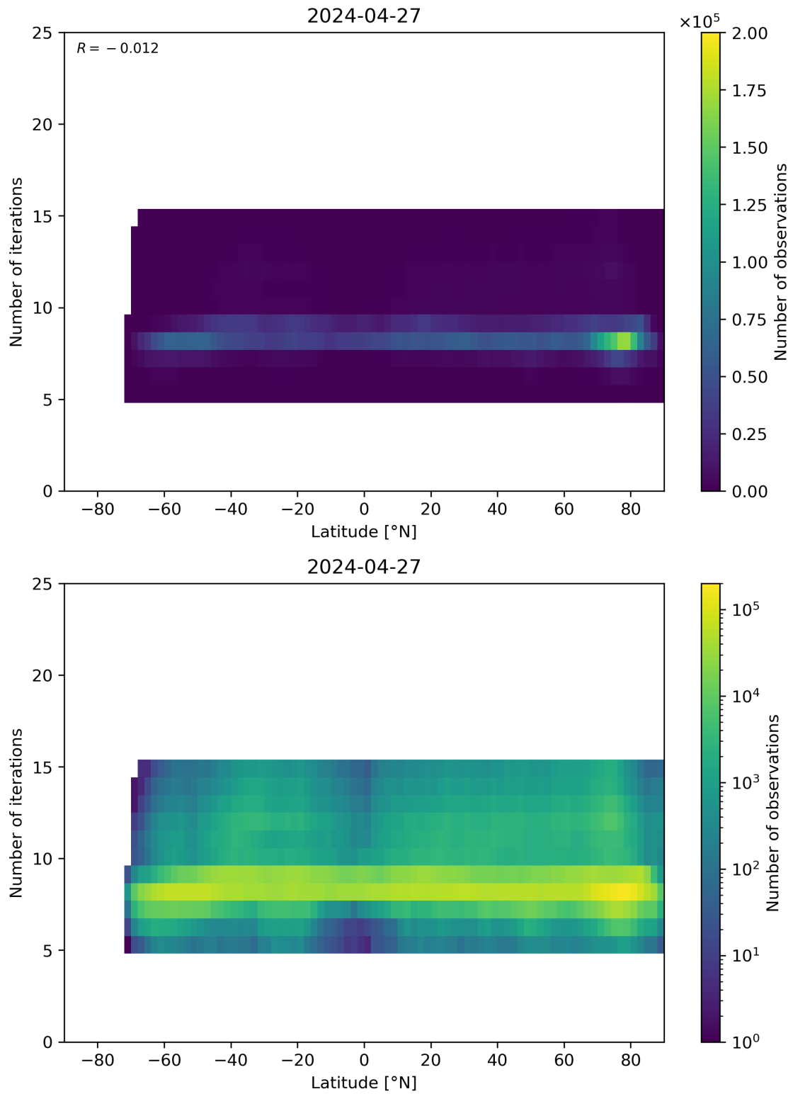
Figure 56: Scatter density plot of “Latitude” against “Number of iterations” for 2024-04-26 to 2024-04-28.
