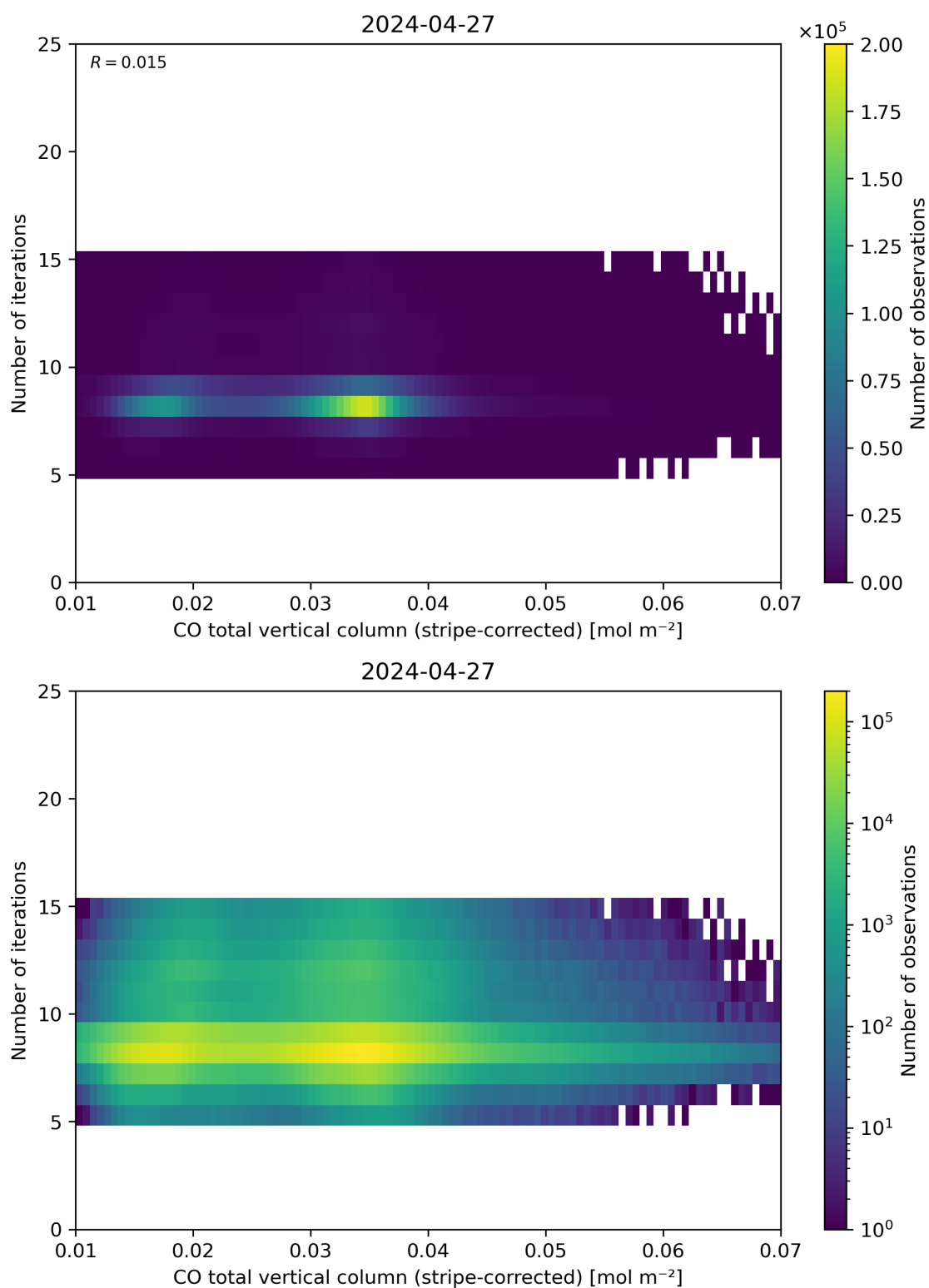
Figure 39: Scatter density plot of “CO total vertical column (stripe-corrected)” against “Number of iterations” for 2024-04-26 to 2024-04-28.
