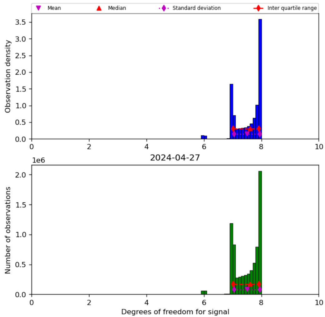
Figure 23: Histogram of “Degrees of freedom for signal” for 2024-04-26 to 2024-04-28
