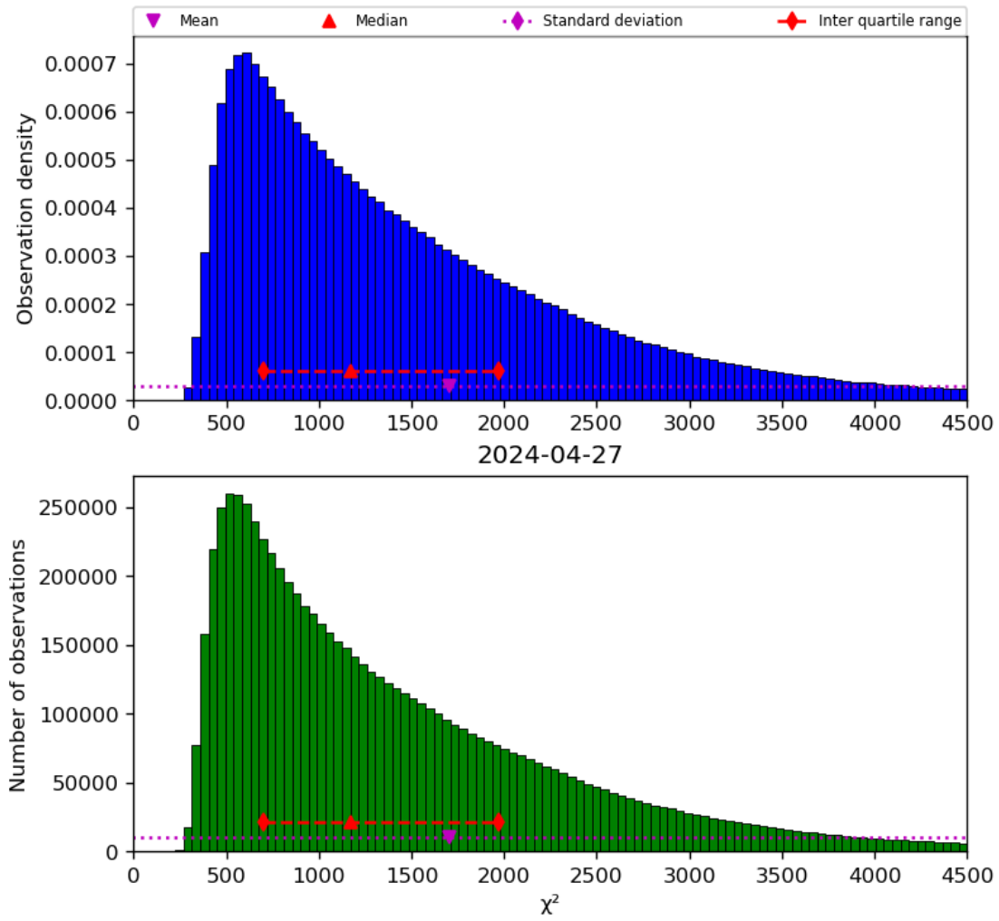
Figure 22: Histogram of “ \chi^2 ” for 2024-04-26 to 2024-04-28
