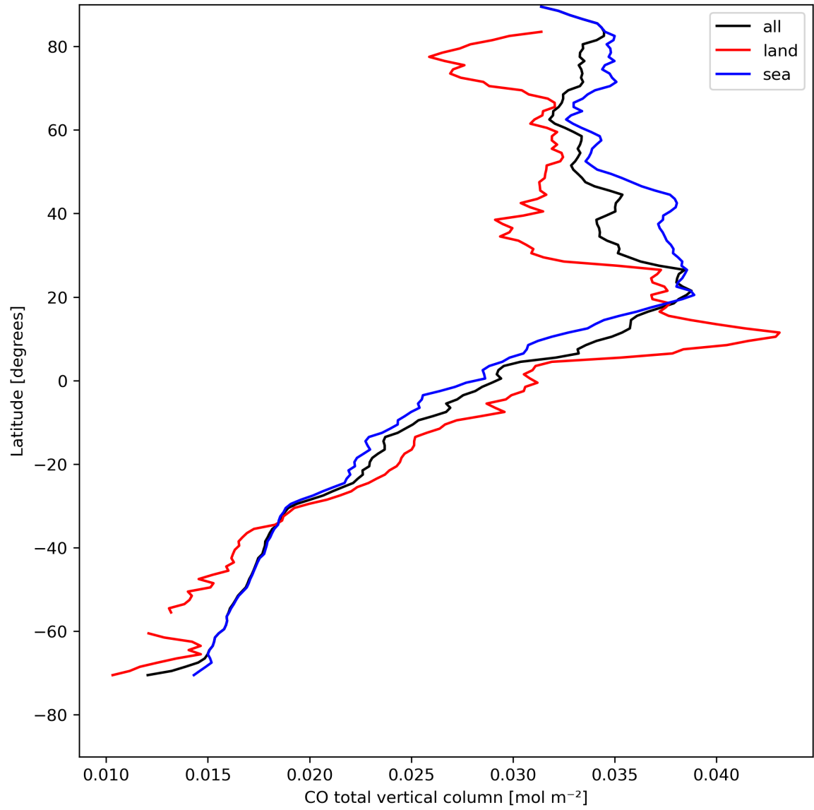
Figure 10: Zonal average of “CO total vertical column” for 2024-04-26 to 2024-04-28.
