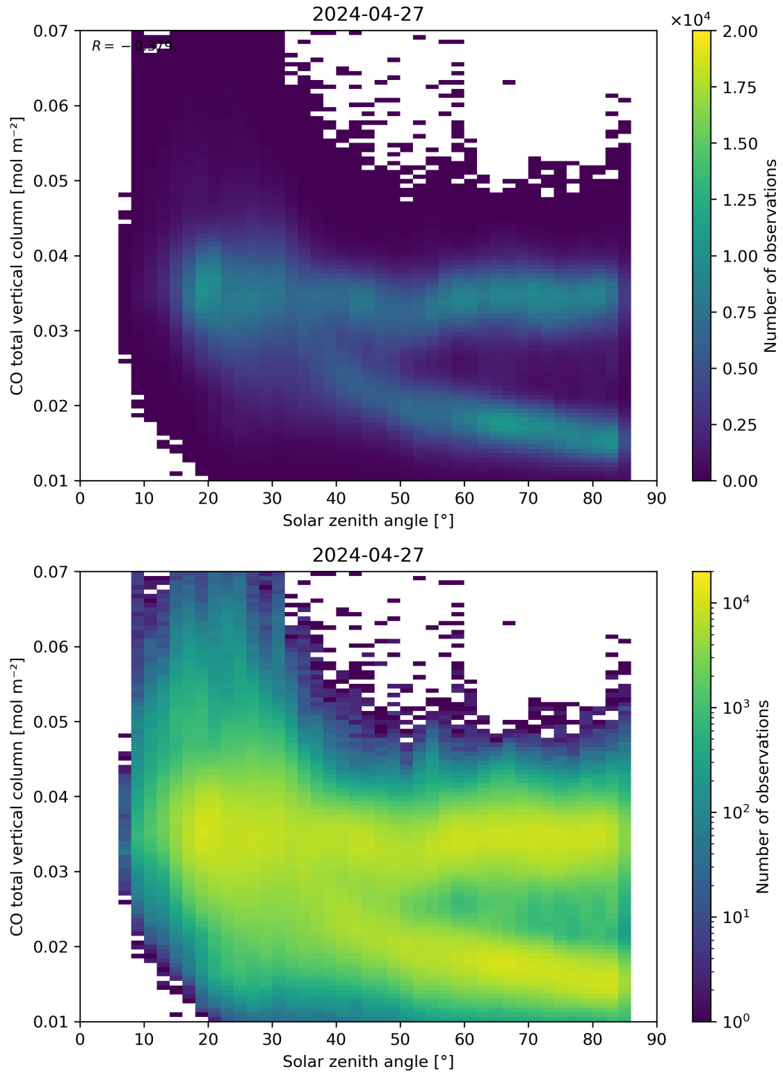
Figure 61: Scatter density plot of “Solar zenith angle” against “CO total vertical column” for 2024-04-26 to 2024-04-28.
