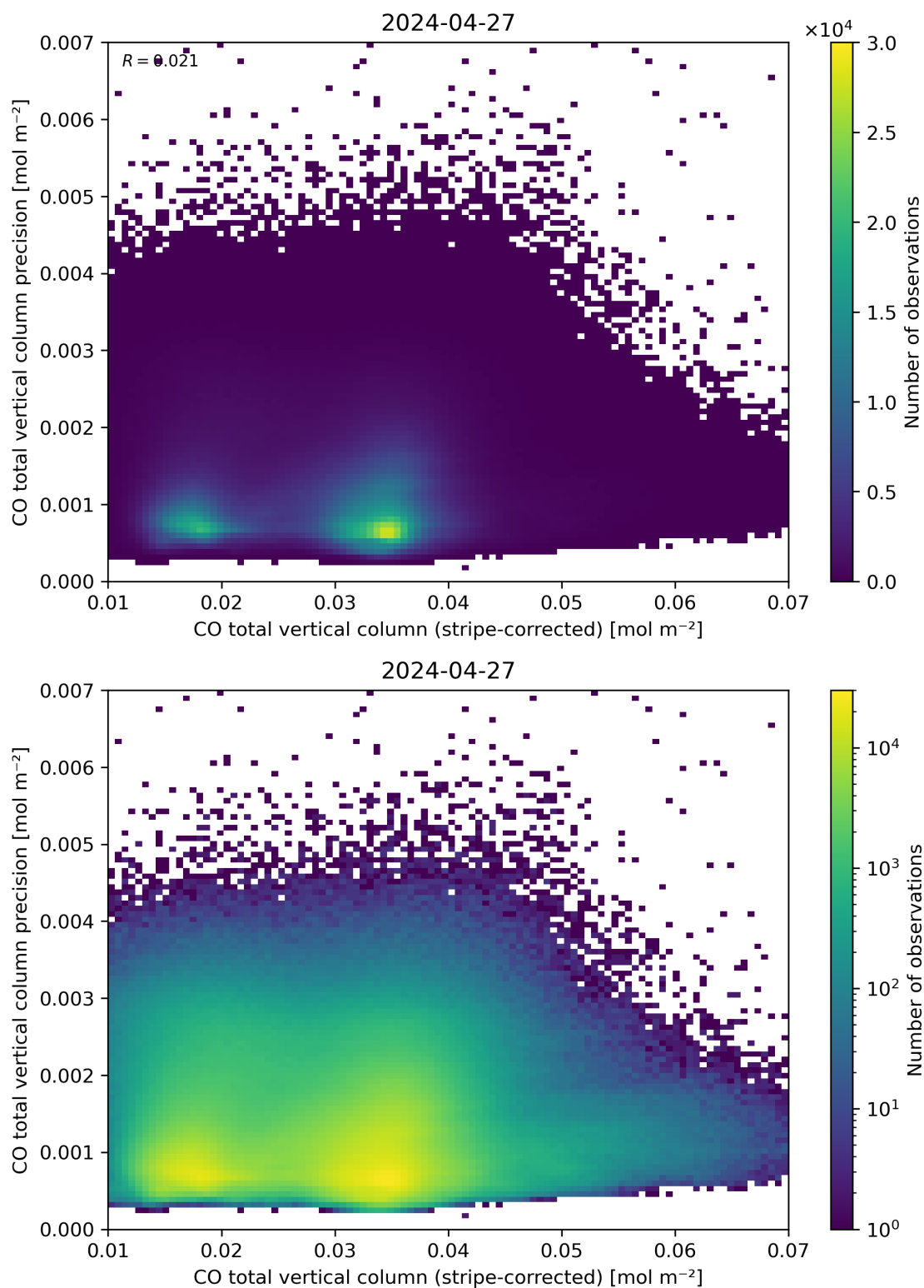
Figure 36: Scatter density plot of “CO total vertical column (stripe-corrected)” against “CO total vertical column precision” for 2024-04-26 to 2024-04-28.
