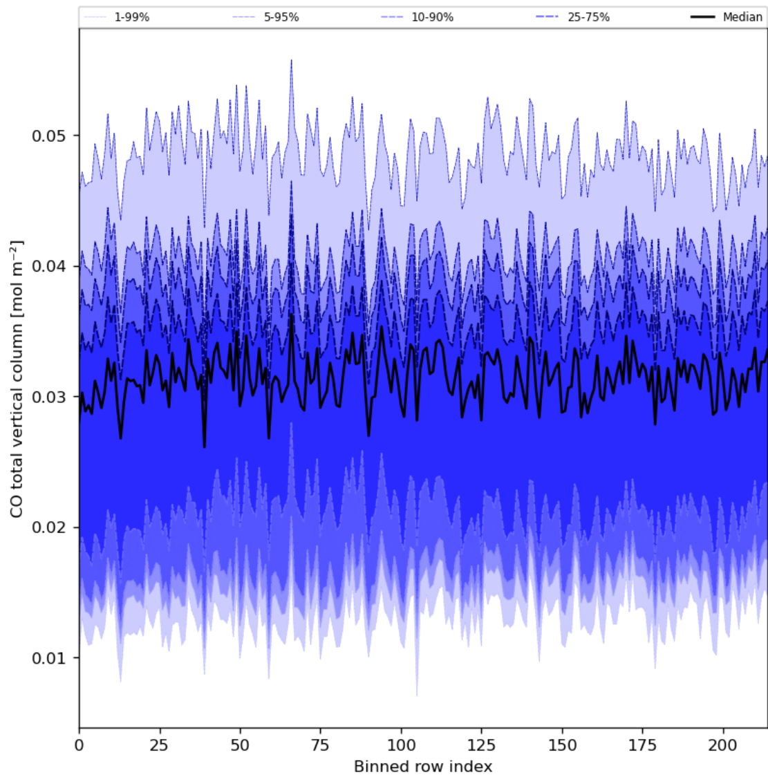
Figure 26: Along track statistics of “CO total vertical column” for 2024-04-26 to 2024-04-28
