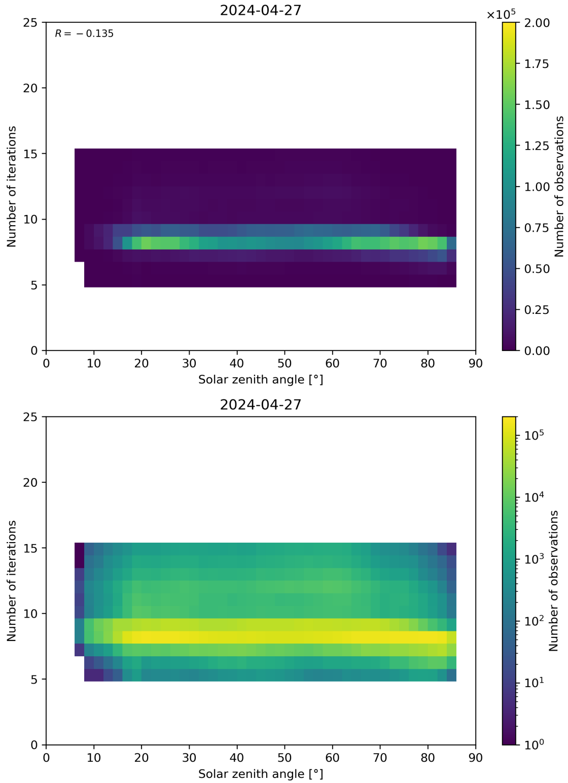
Figure 67: Scatter density plot of “Solar zenith angle” against “Number of iterations” for 2024-04-26 to 2024-04-28.
