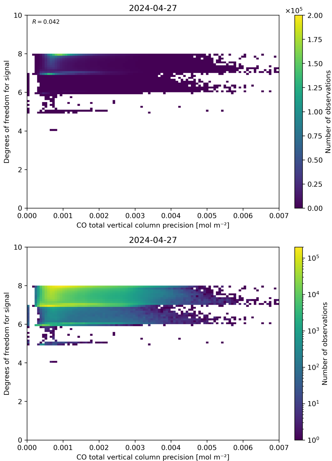
Figure 45: Scatter density plot of “CO total vertical column precision” against “Degrees of freedom for signal” for 2024-04-26 to 2024-04-28.
