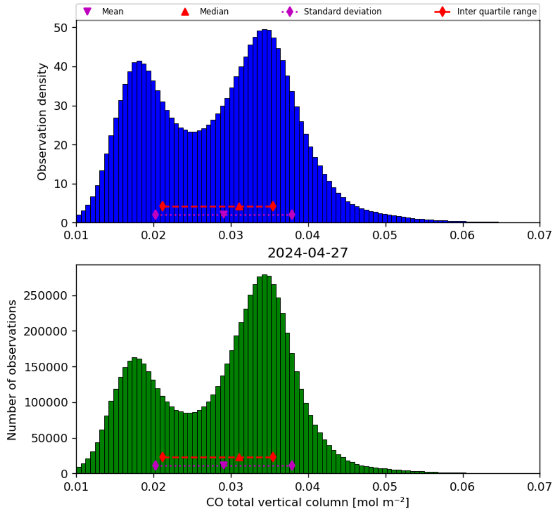
Figure 18: Histogram of “CO total vertical column” for 2024-04-26 to 2024-04-28
