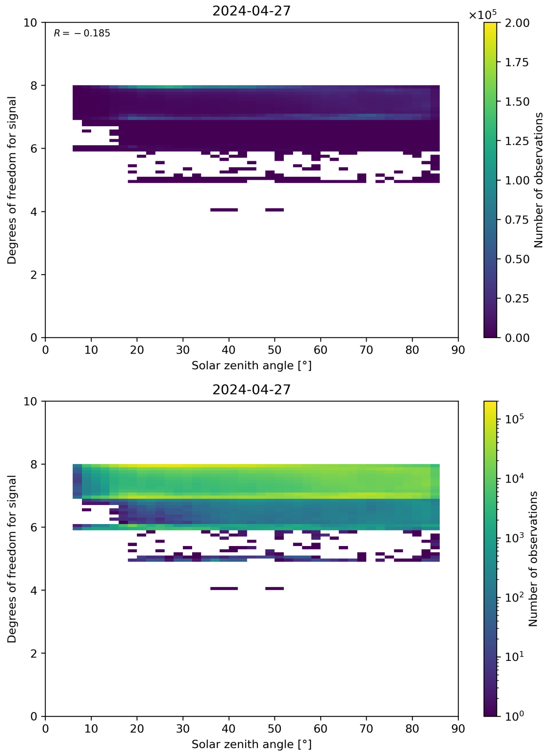
Figure 65: Scatter density plot of “Solar zenith angle” against “Degrees of freedom for signal” for 2024-04-26 to 2024-04-28.
