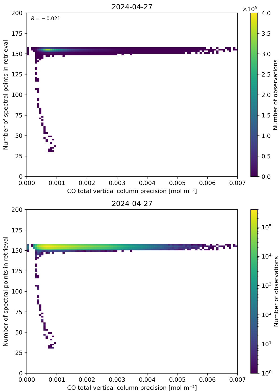
Figure 47: Scatter density plot of “CO total vertical column precision” against “Number of spectral points in retrieval” for 2024-04-26 to 2024-04-28.
