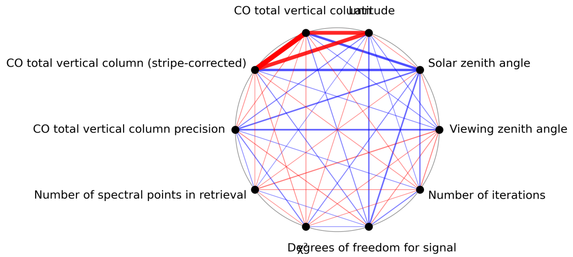
Figure 1: Map of correlation graph for 2024-04-26 to 2024-04-28.
