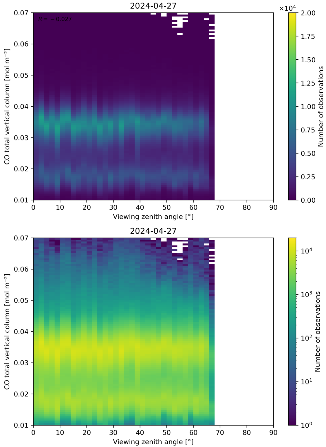
Figure 69: Scatter density plot of “Viewing zenith angle” against “CO total vertical column” for 2024-04-26 to 2024-04-28.
