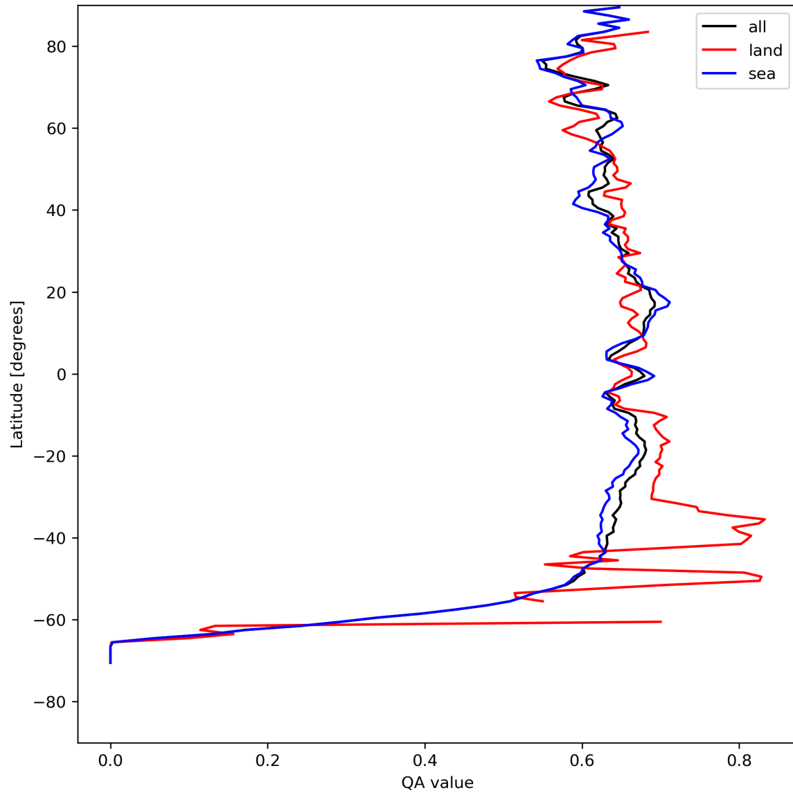
Figure 9: Zonal average of “QA value” for 2024-04-26 to 2024-04-28.
