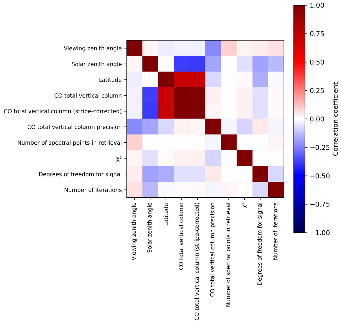
Figure 2: Map of correlation matrix for 2024-04-26 to 2024-04-28.
