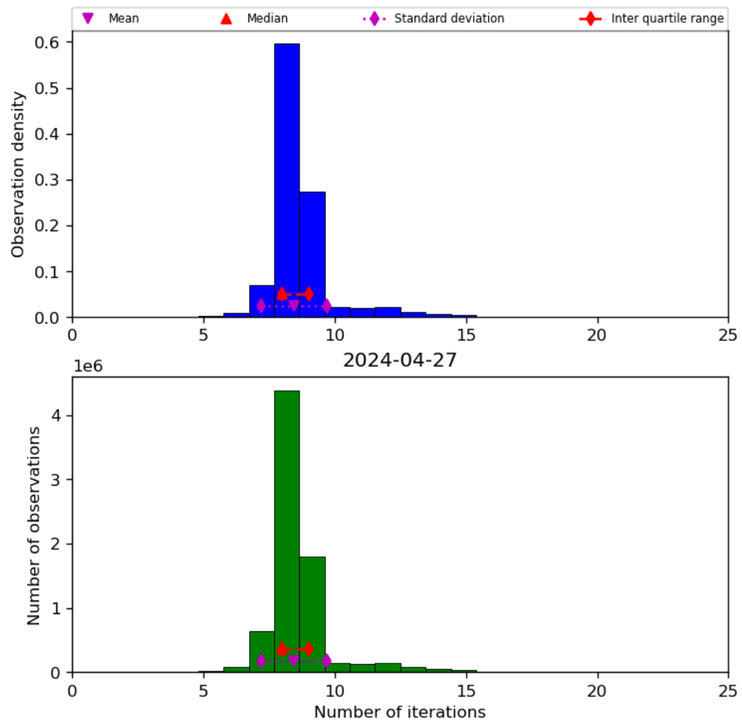
Figure 24: Histogram of “Number of iterations” for 2024-04-26 to 2024-04-28
