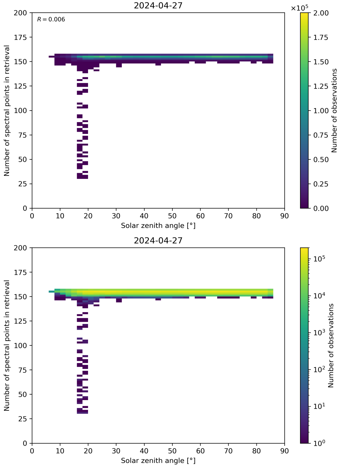
Figure 68: Scatter density plot of “Solar zenith angle” against “Number of spectral points in retrieval” for 2024-04-26 to 2024-04-28.
