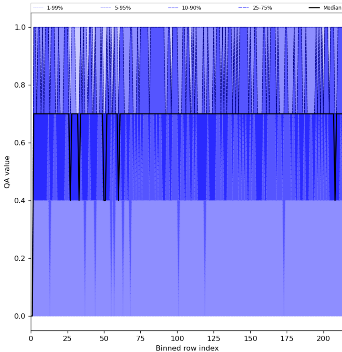
Figure 25: Along track statistics of “QA value” for 2024-04-26 to 2024-04-28
