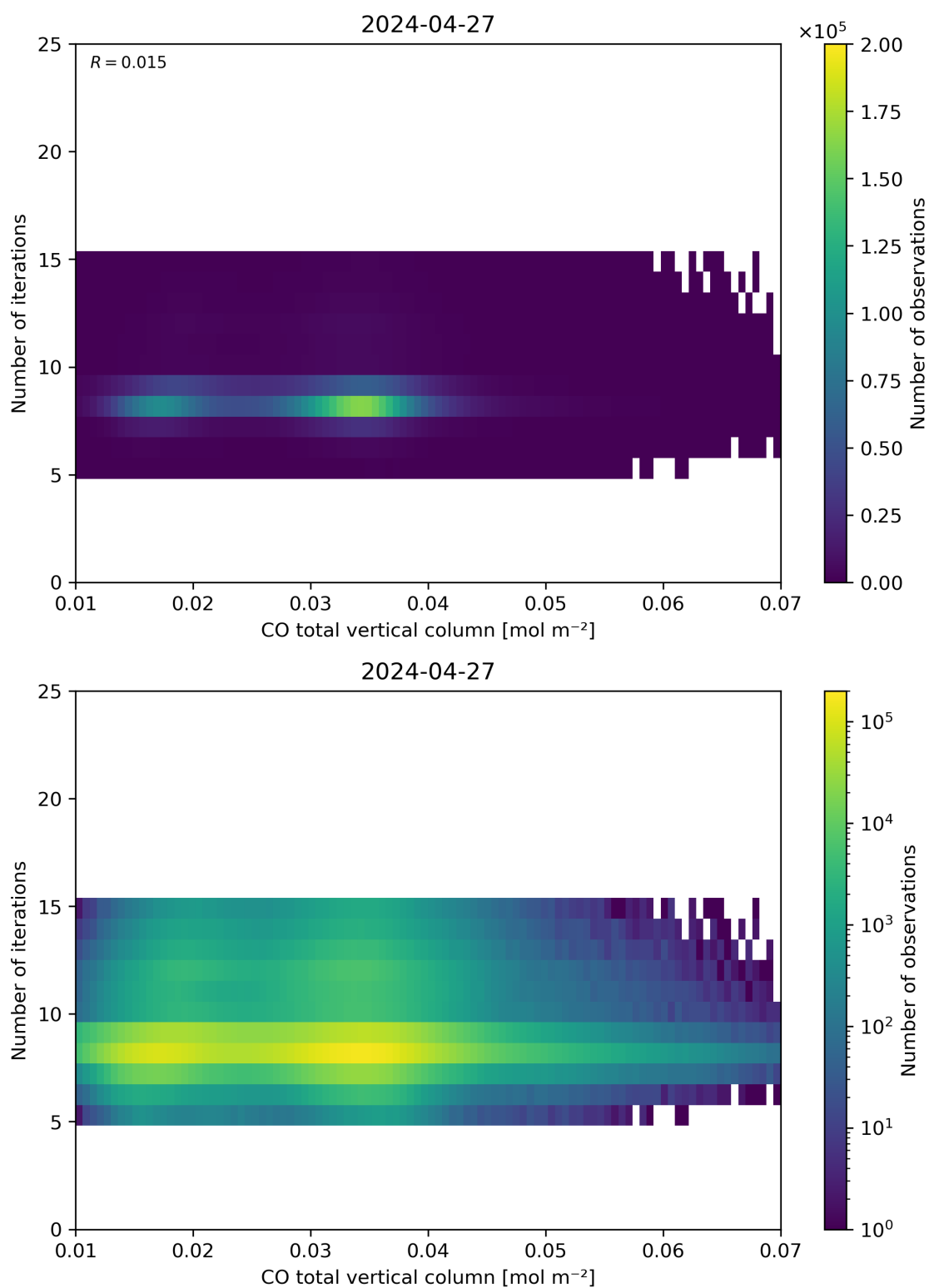
Figure 42: Scatter density plot of “CO total vertical column” against “Number of iterations” for 2024-04-26 to 2024-04-28.
