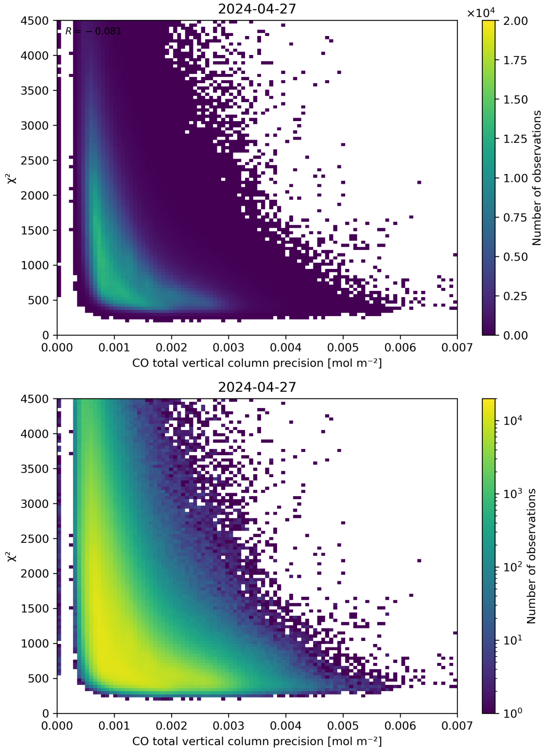
Figure 44: Scatter density plot of “CO total vertical column precision” against “ \chi^2 ” for 2024-04-26 to 2024-04-28.
