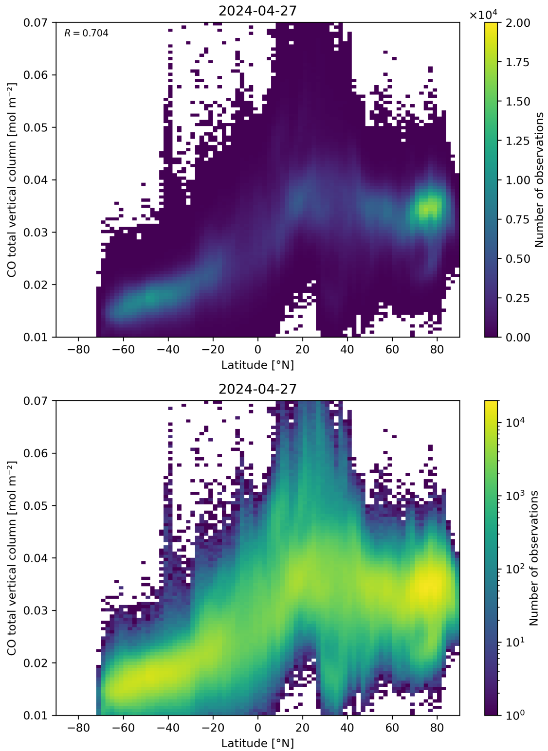
Figure 51: Scatter density plot of “Latitude” against “CO total vertical column” for 2024-04-26 to 2024-04-28.
