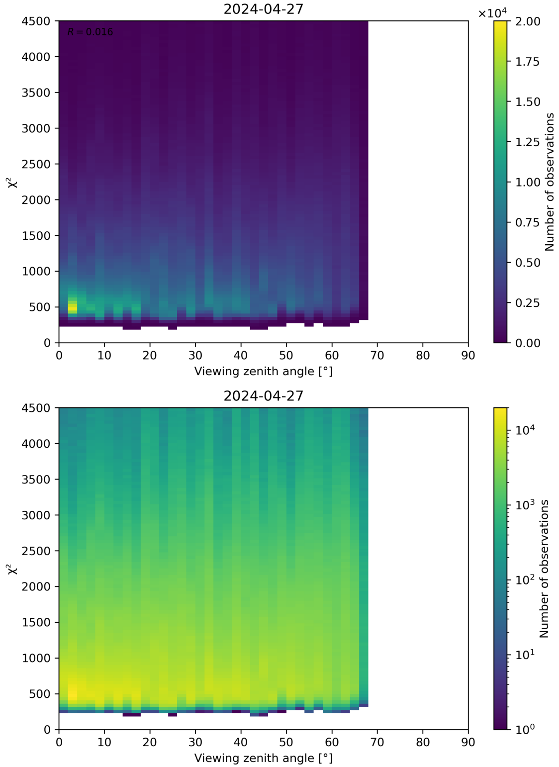
Figure 72: Scatter density plot of “Viewing zenith angle” against “ \chi^2 ” for 2024-04-26 to 2024-04-28.
