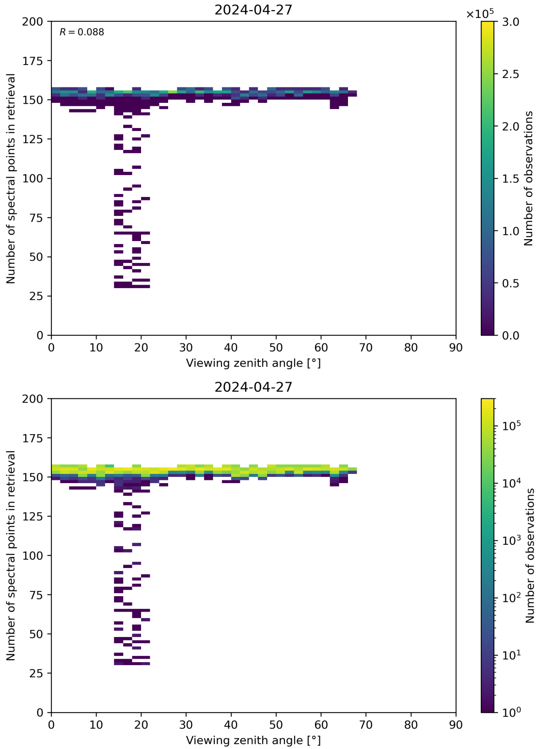
Figure 76: Scatter density plot of “Viewing zenith angle” against “Number of spectral points in retrieval” for 2024-04-26 to 2024-04-28.
