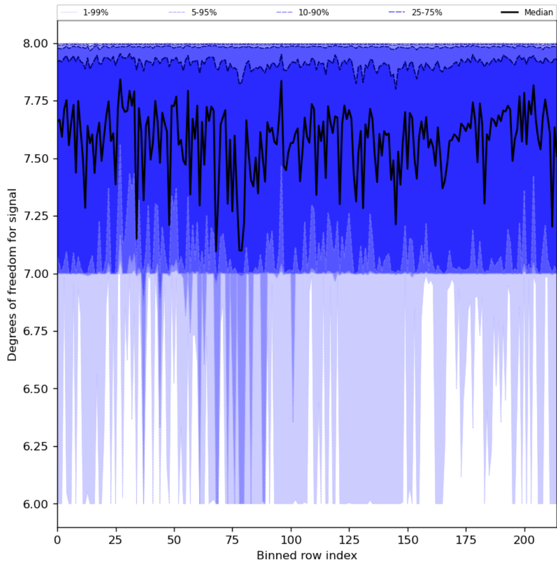
Figure 31: Along track statistics of “Degrees of freedom for signal” for 2024-04-26 to 2024-04-28
