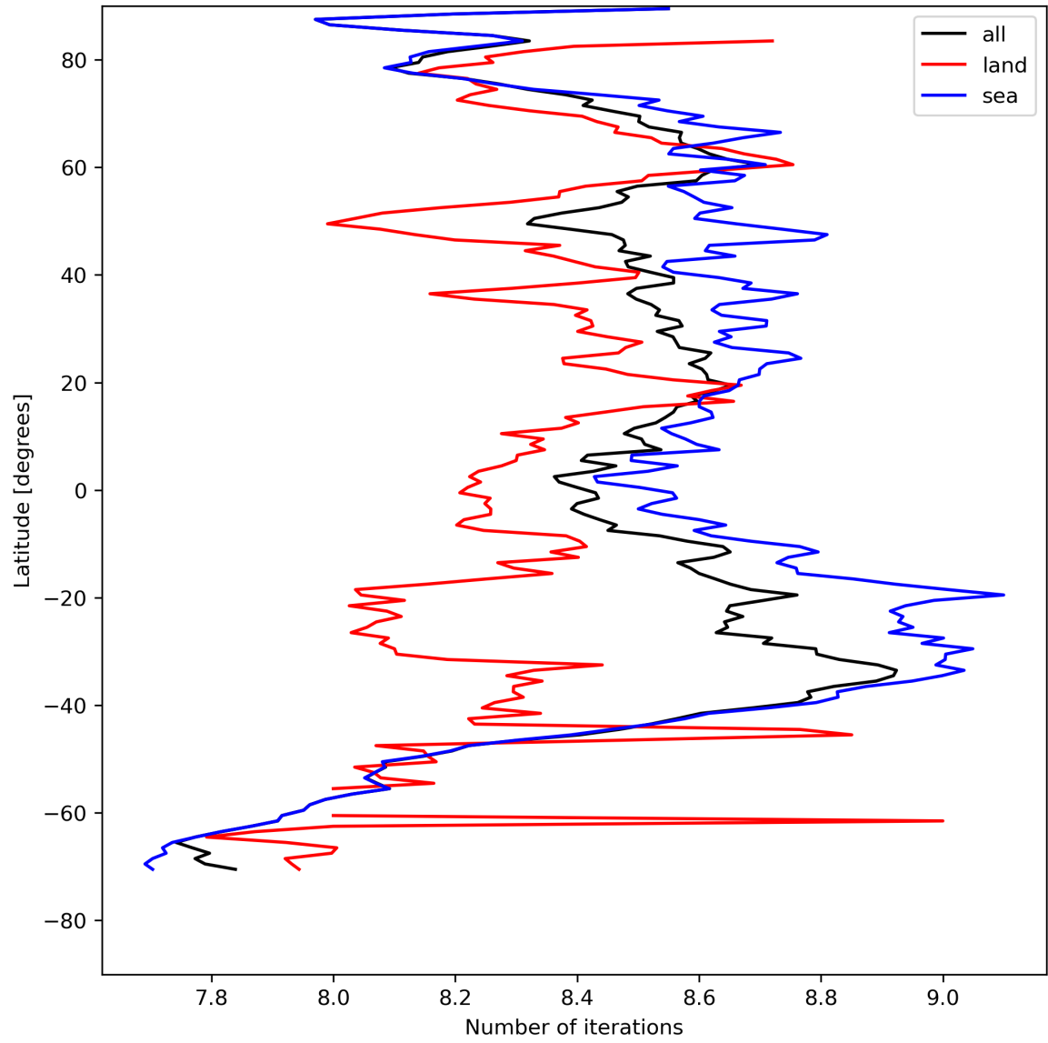
Figure 16: Zonal average of “Number of iterations” for 2024-04-26 to 2024-04-28.
