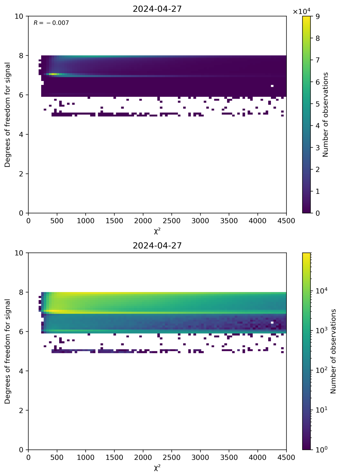
Figure 48: Scatter density plot of “ \chi^2 ” against “Degrees of freedom for signal” for 2024-04-26 to 2024-04-28.
