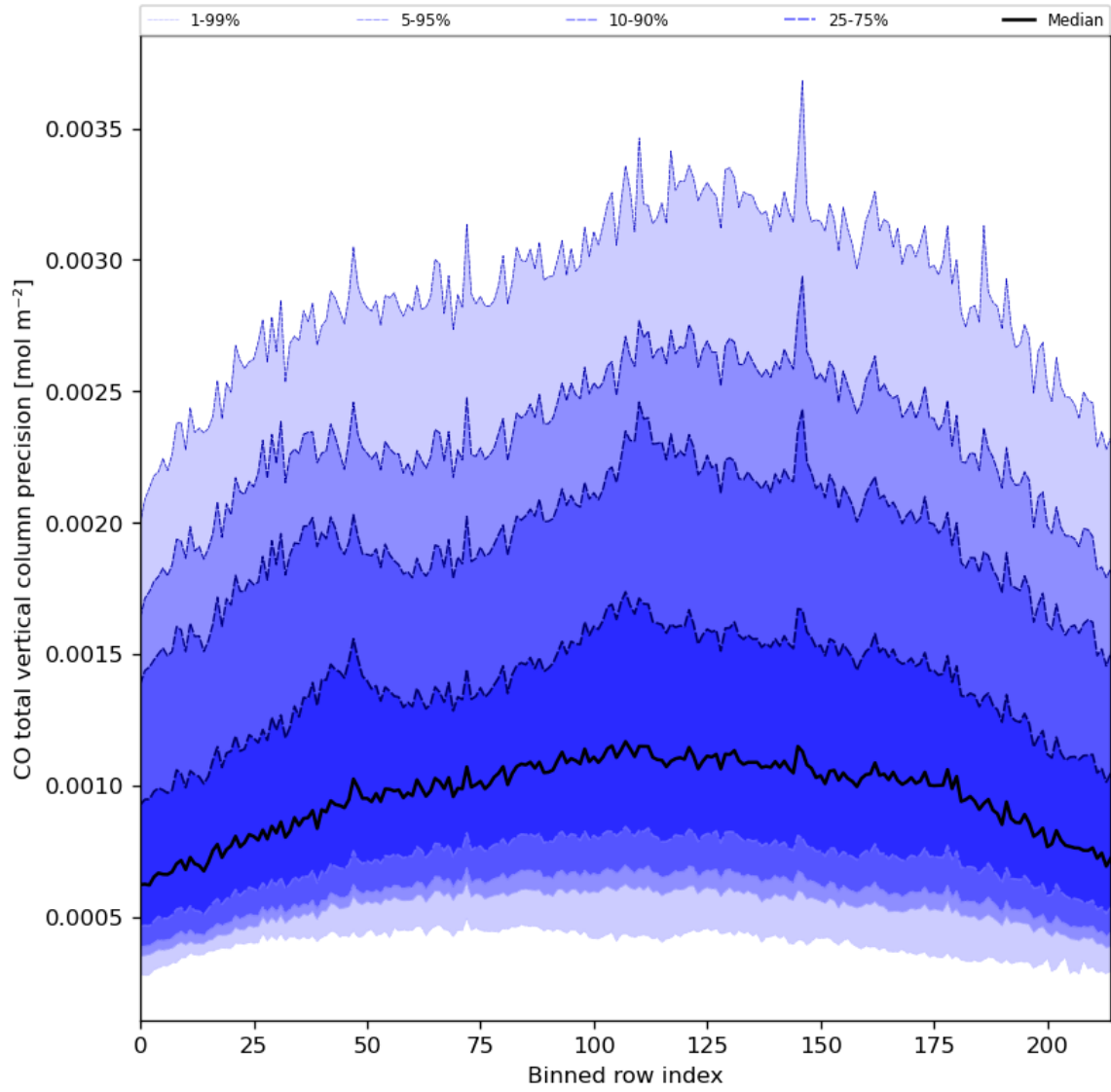
Figure 28: Along track statistics of “CO total vertical column precision” for 2024-04-26 to 2024-04-28
