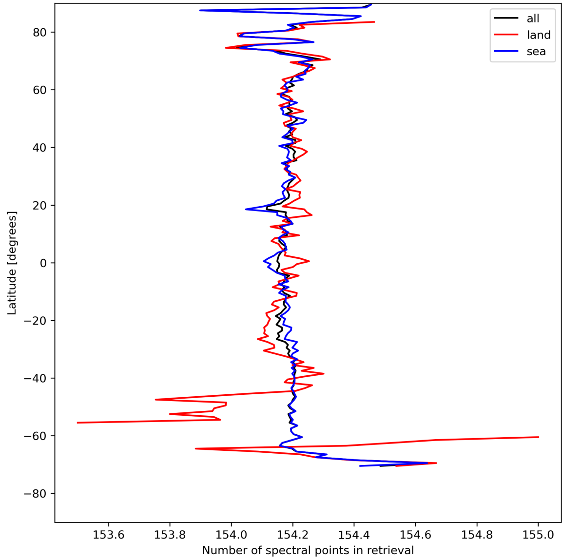
Figure 13: Zonal average of “Number of spectral points in retrieval” for 2024-04-26 to 2024-04-28.
