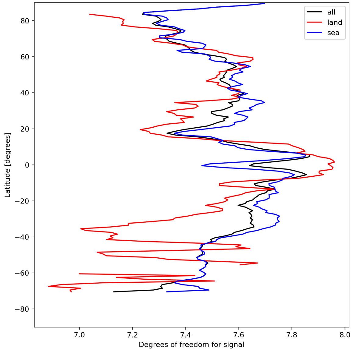
Figure 15: Zonal average of “Degrees of freedom for signal” for 2024-04-26 to 2024-04-28.
