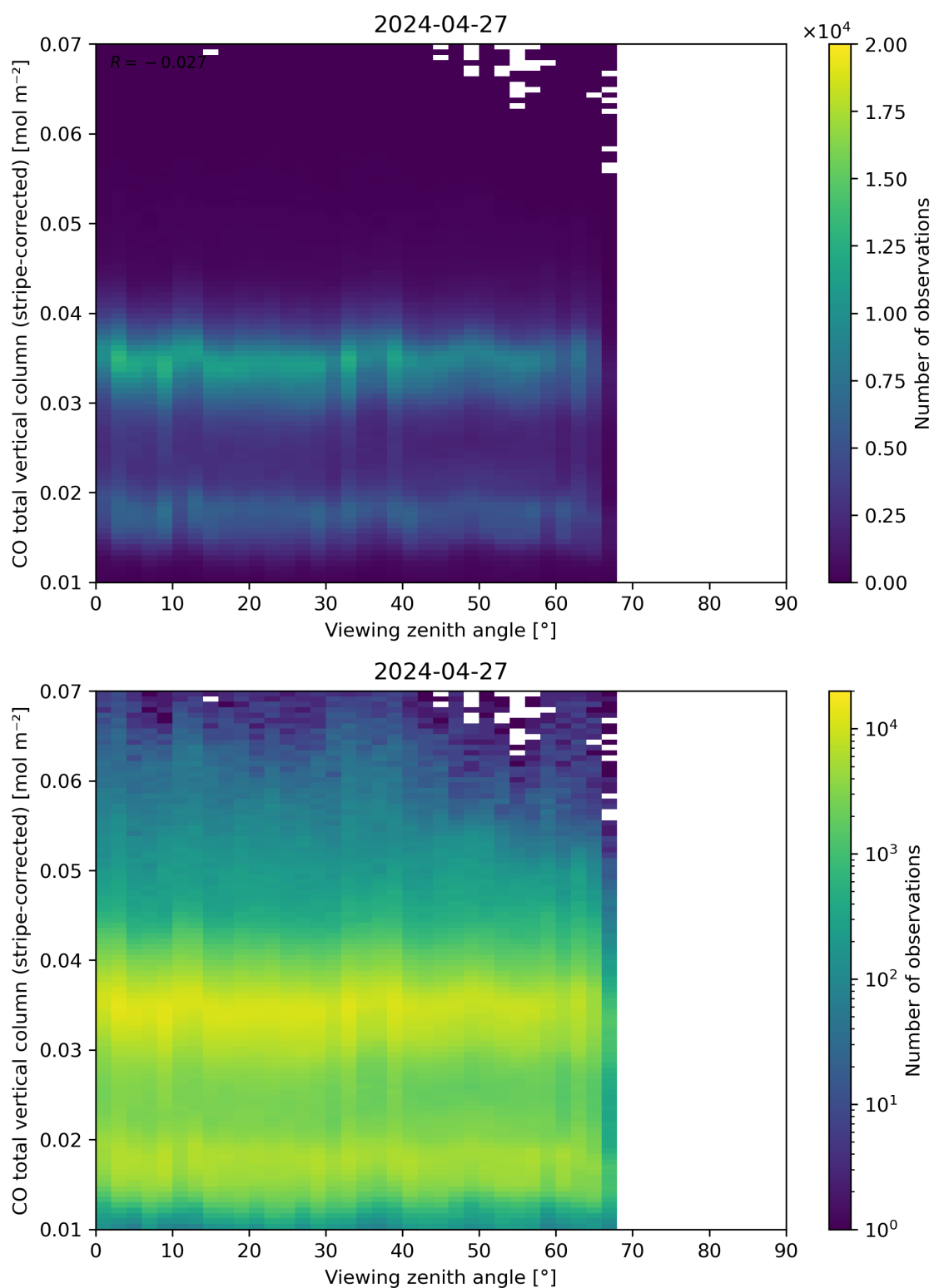
Figure 70: Scatter density plot of “Viewing zenith angle” against “CO total vertical column (stripe-corrected)” for 2024-04-26 to 2024-04-28.
