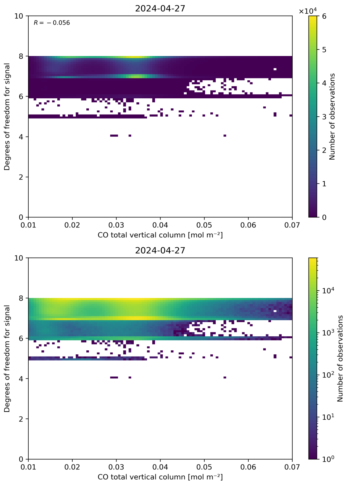
Figure 41: Scatter density plot of “CO total vertical column” against “Degrees of freedom for signal” for 2024-04-26 to 2024-04-28.
