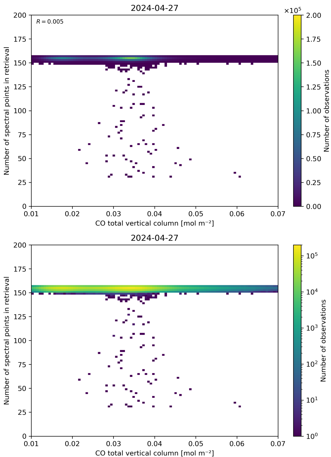
Figure 43: Scatter density plot of “CO total vertical column” against “Number of spectral points in retrieval” for 2024-04-26 to 2024-04-28.
