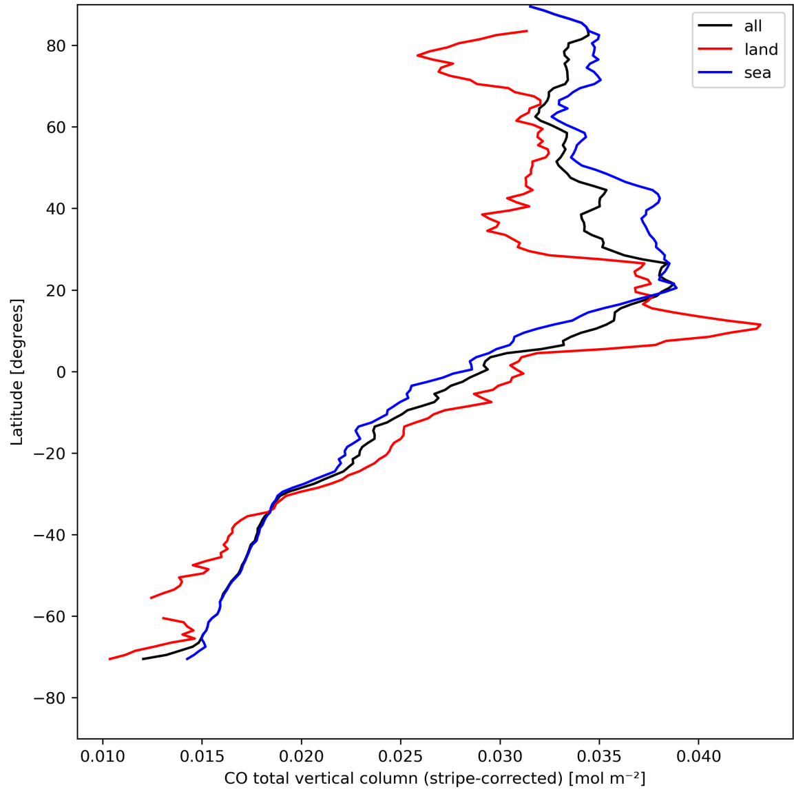
Figure 11: Zonal average of “CO total vertical column (stripe-corrected)” for 2024-04-26 to 2024-04-28.
