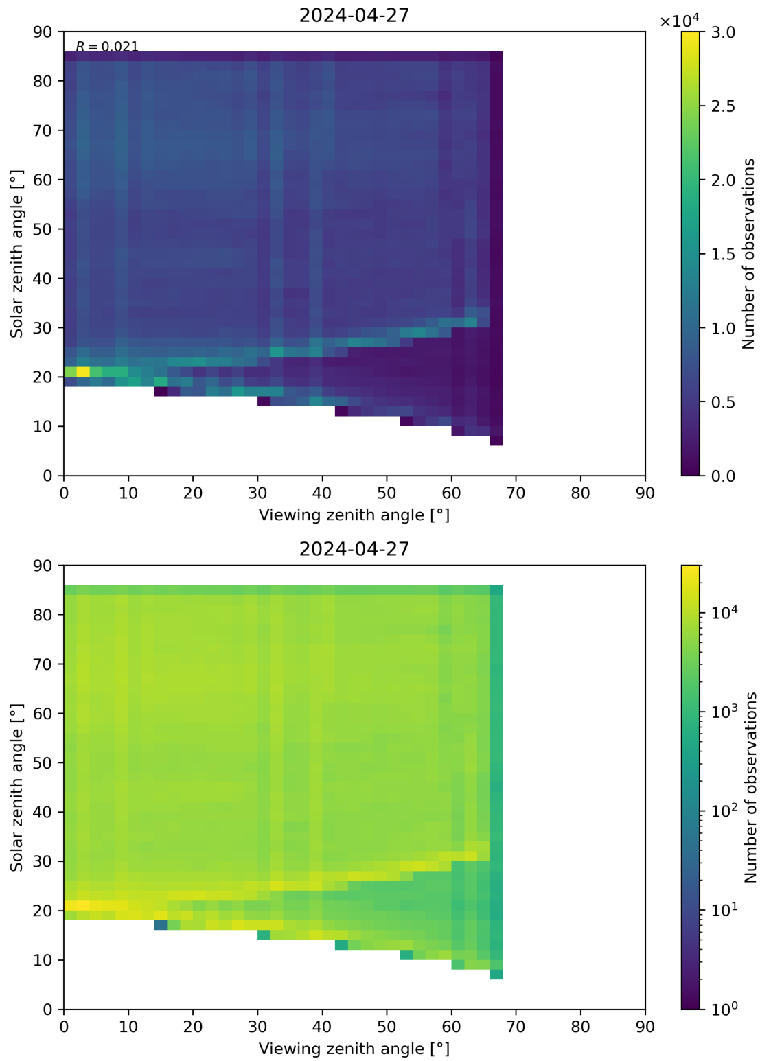
Figure 77: Scatter density plot of “Viewing zenith angle” against “Solar zenith angle” for 2024-04-26 to 2024-04-28.
