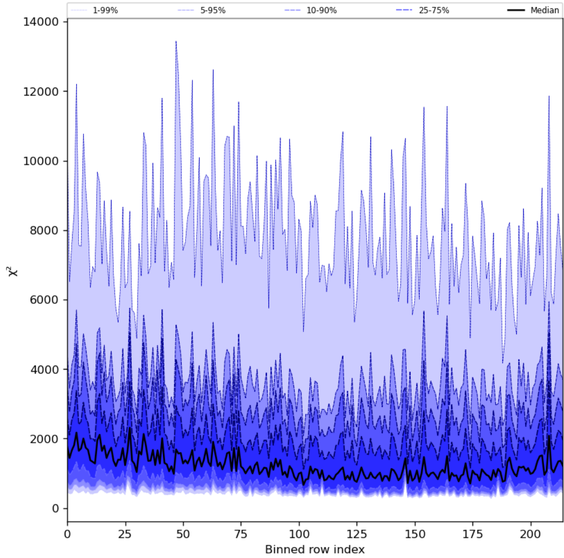
Figure 30: Along track statistics of “ \chi^2 ” for 2024-04-26 to 2024-04-28
