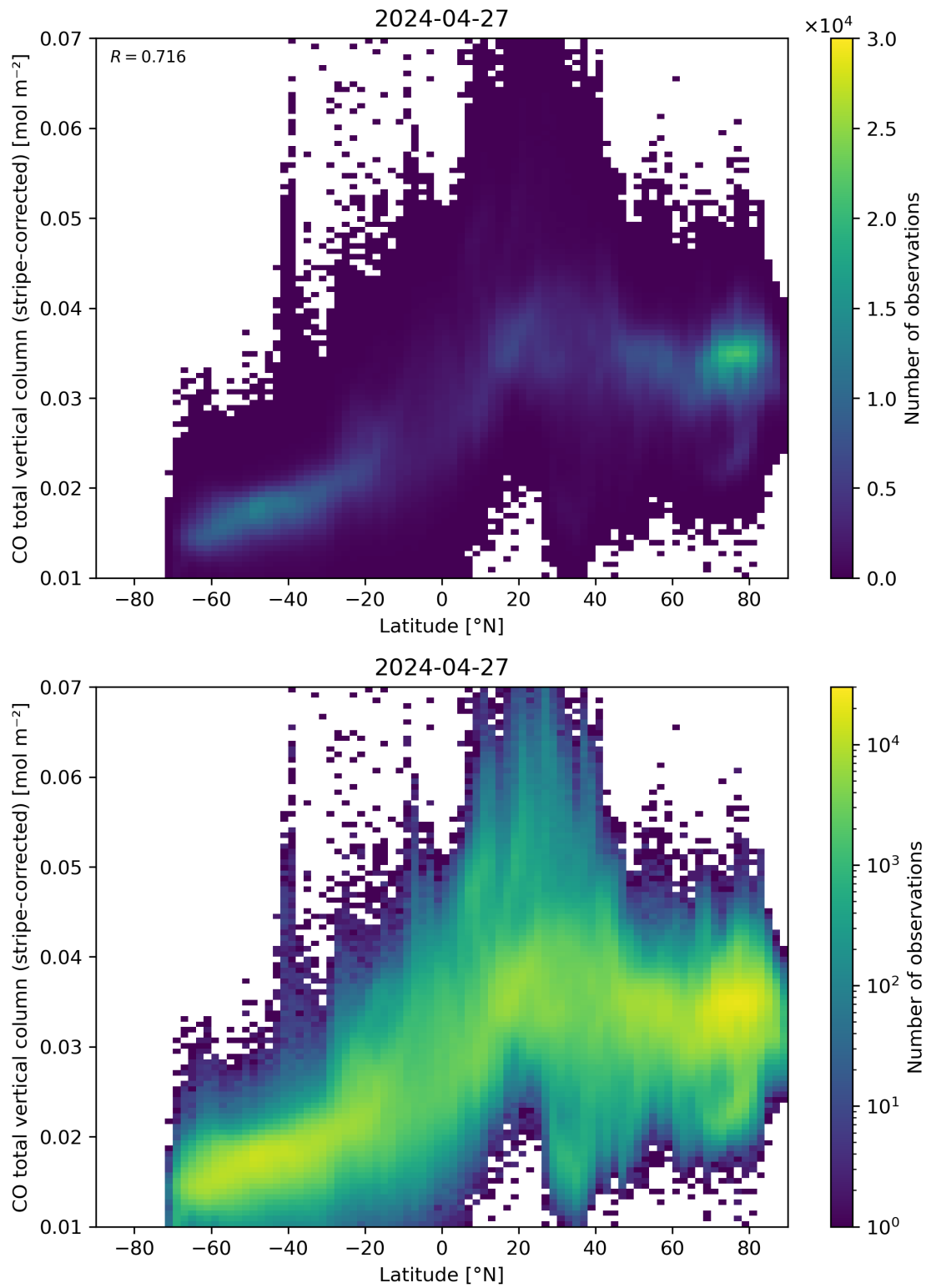
Figure 52: Scatter density plot of “Latitude” against “CO total vertical column (stripe-corrected)” for 2024-04-26 to 2024-04-28.
