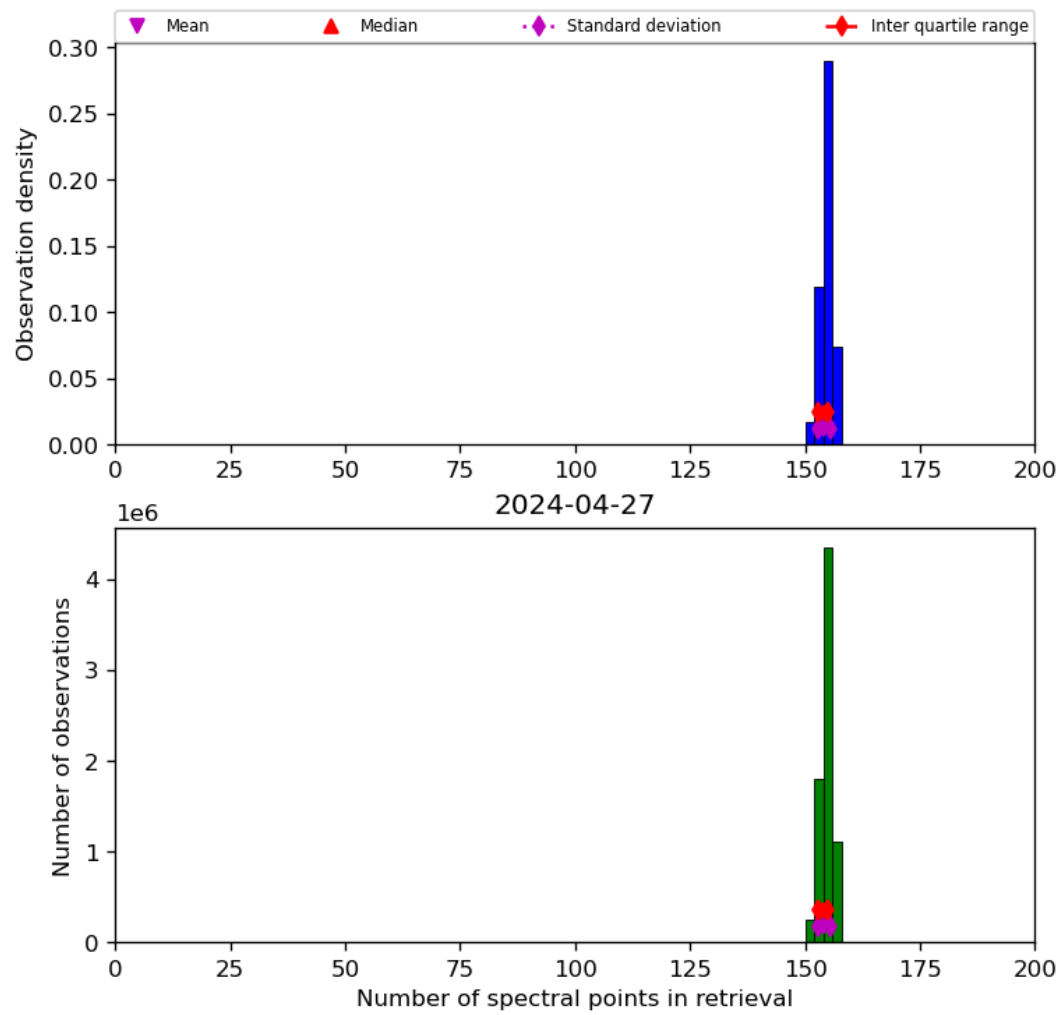
Figure 21: Histogram of “Number of spectral points in retrieval” for 2024-04-26 to 2024-04-28
