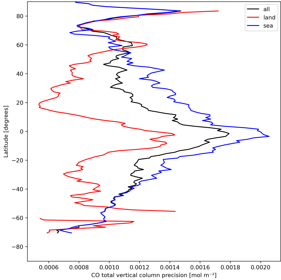
Figure 12: Zonal average of “CO total vertical column precision” for 2024-04-26 to 2024-04-28.
