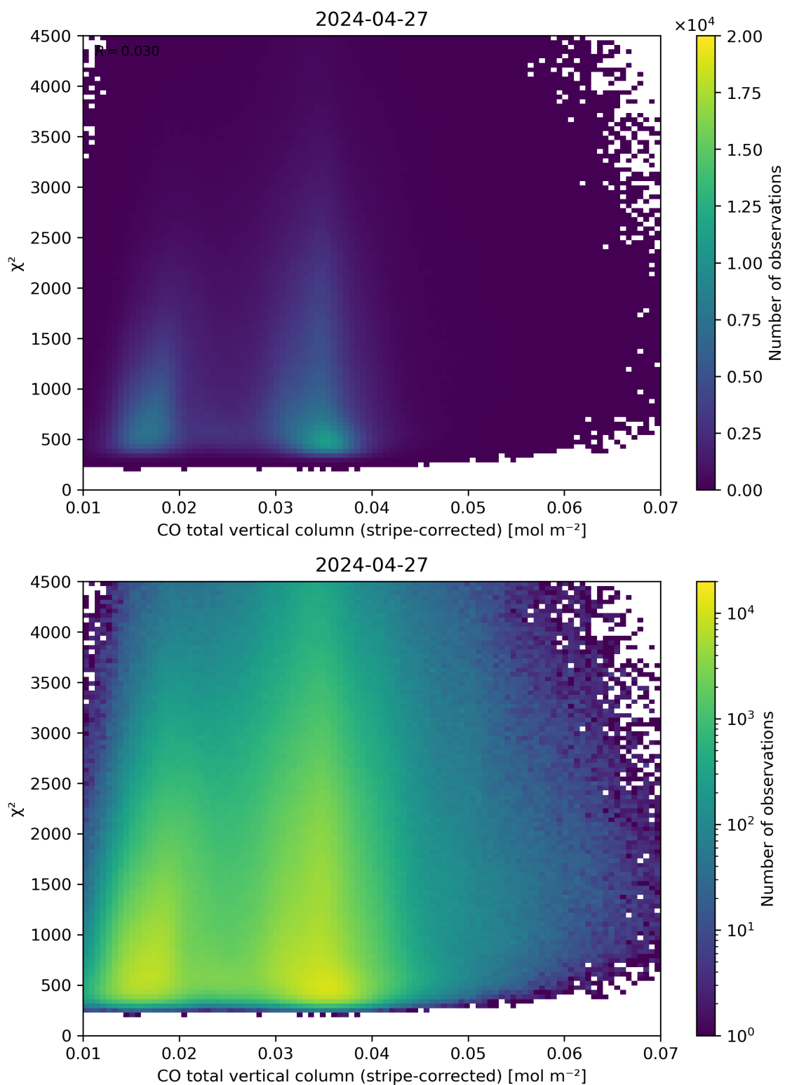
Figure 37: Scatter density plot of “CO total vertical column (stripe-corrected)” against “ \chi^2 ” for 2024-04-26 to 2024-04-28.
