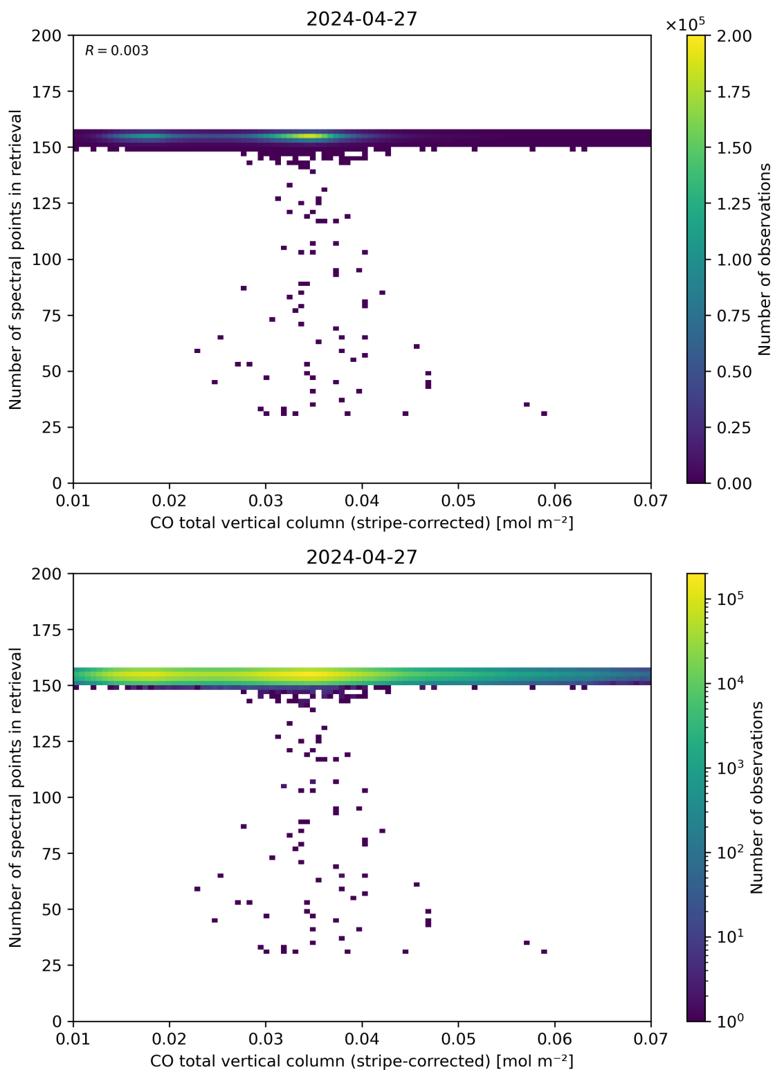
Figure 40: Scatter density plot of “CO total vertical column (stripe-corrected)” against “Number of spectral points in retrieval” for 2024-04-26 to 2024-04-28.
