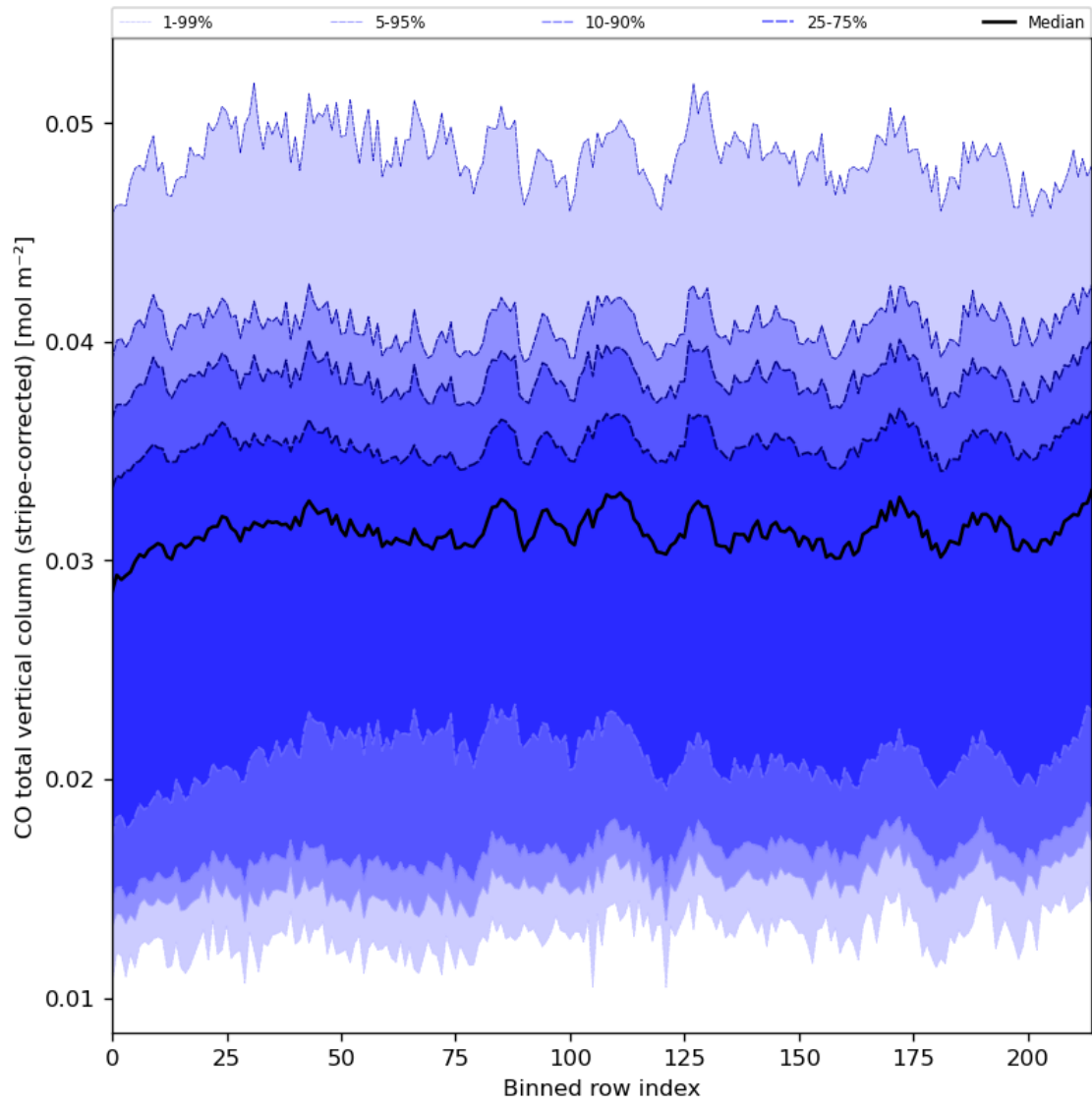
Figure 27: Along track statistics of “CO total vertical column (stripe-corrected)” for 2024-04-26 to 2024-04-28
