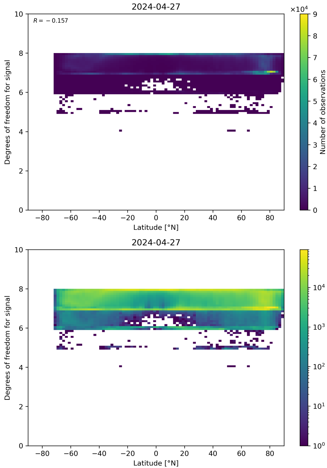
Figure 55: Scatter density plot of “Latitude” against “Degrees of freedom for signal” for 2024-04-26 to 2024-04-28.
