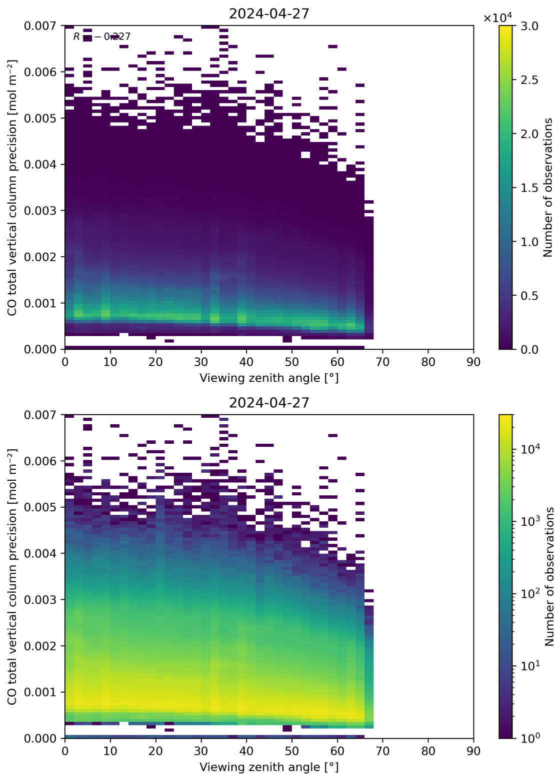
Figure 71: Scatter density plot of “Viewing zenith angle” against “CO total vertical column precision” for 2024-04-26 to 2024-04-28.
