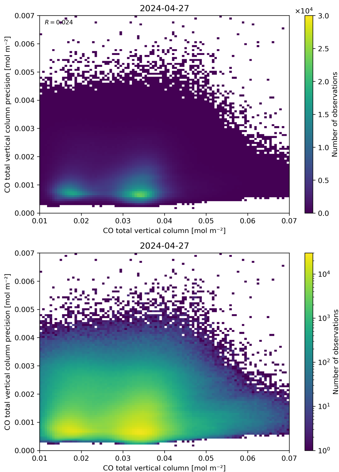
Figure 34: Scatter density plot of “CO total vertical column” against “CO total vertical column precision” for 2024-04-26 to 2024-04-28.
