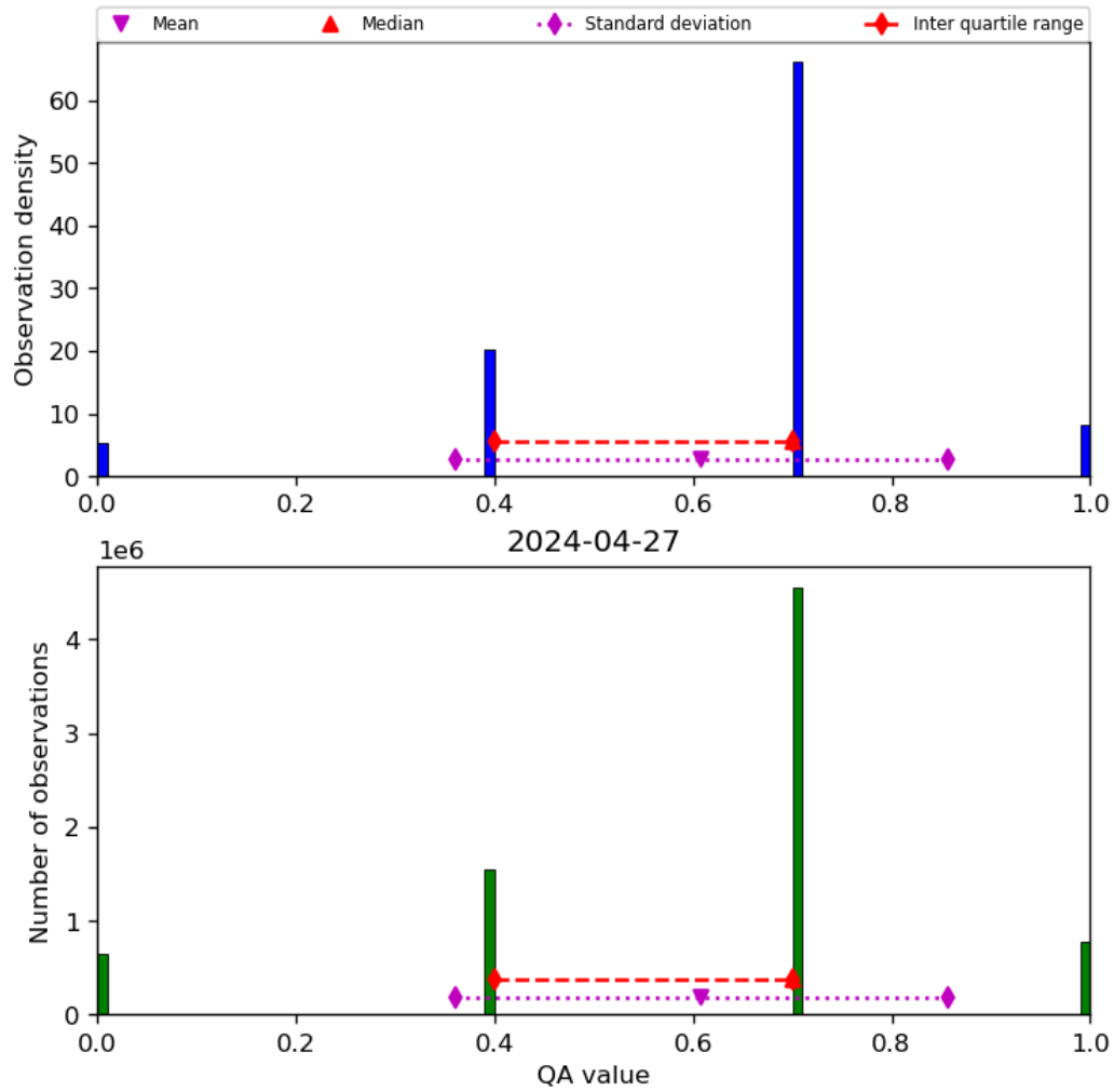
Figure 17: Histogram of “QA value” for 2024-04-26 to 2024-04-28
