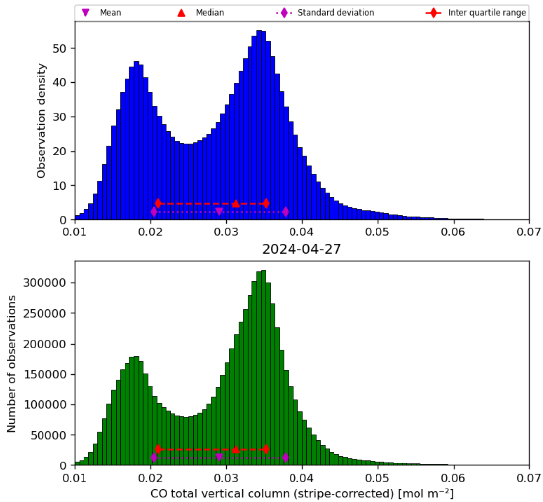
Figure 19: Histogram of “CO total vertical column (stripe-corrected)” for 2024-04-26 to 2024-04-28
