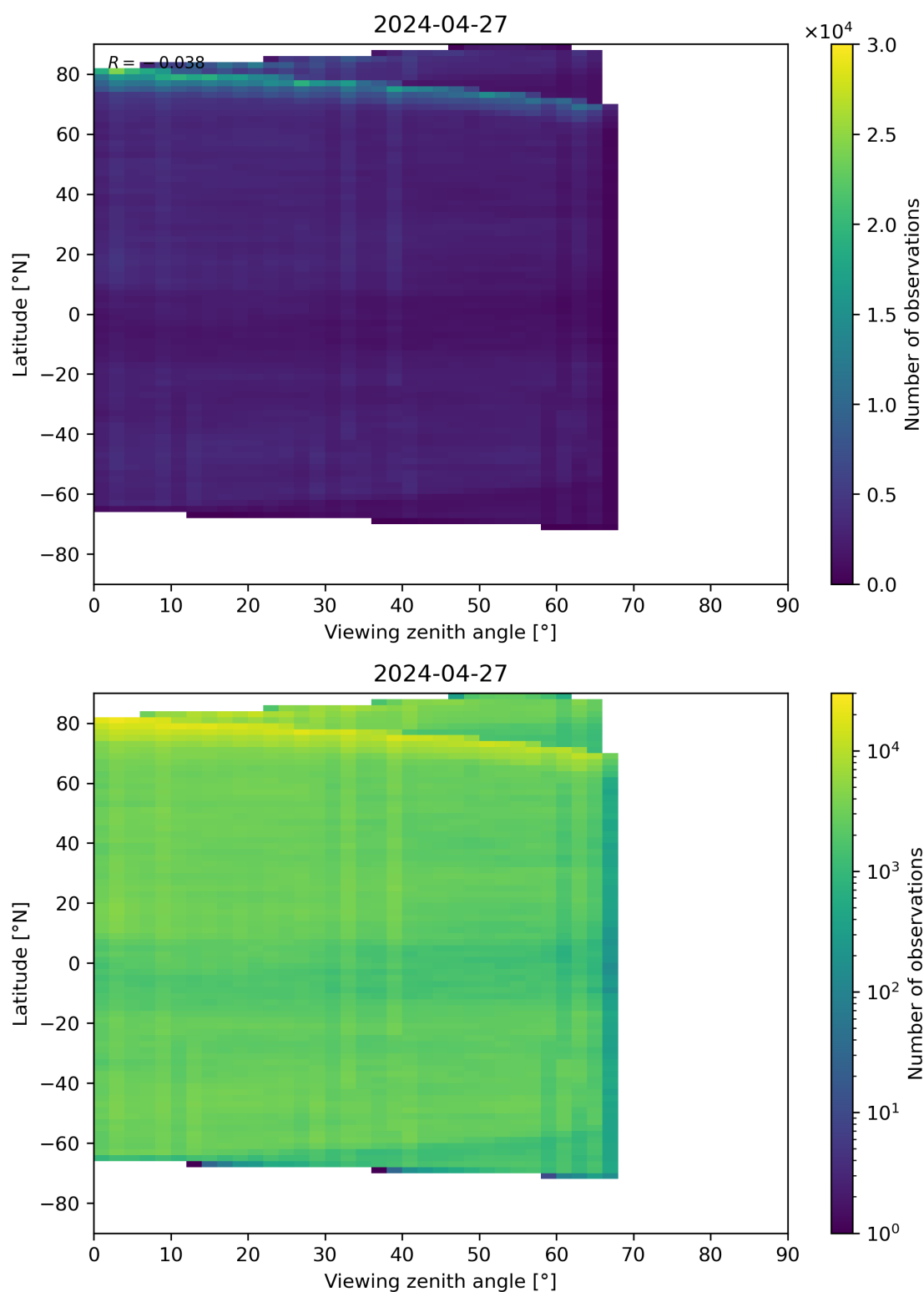
Figure 74: Scatter density plot of “Viewing zenith angle” against “Latitude” for 2024-04-26 to 2024-04-28.
