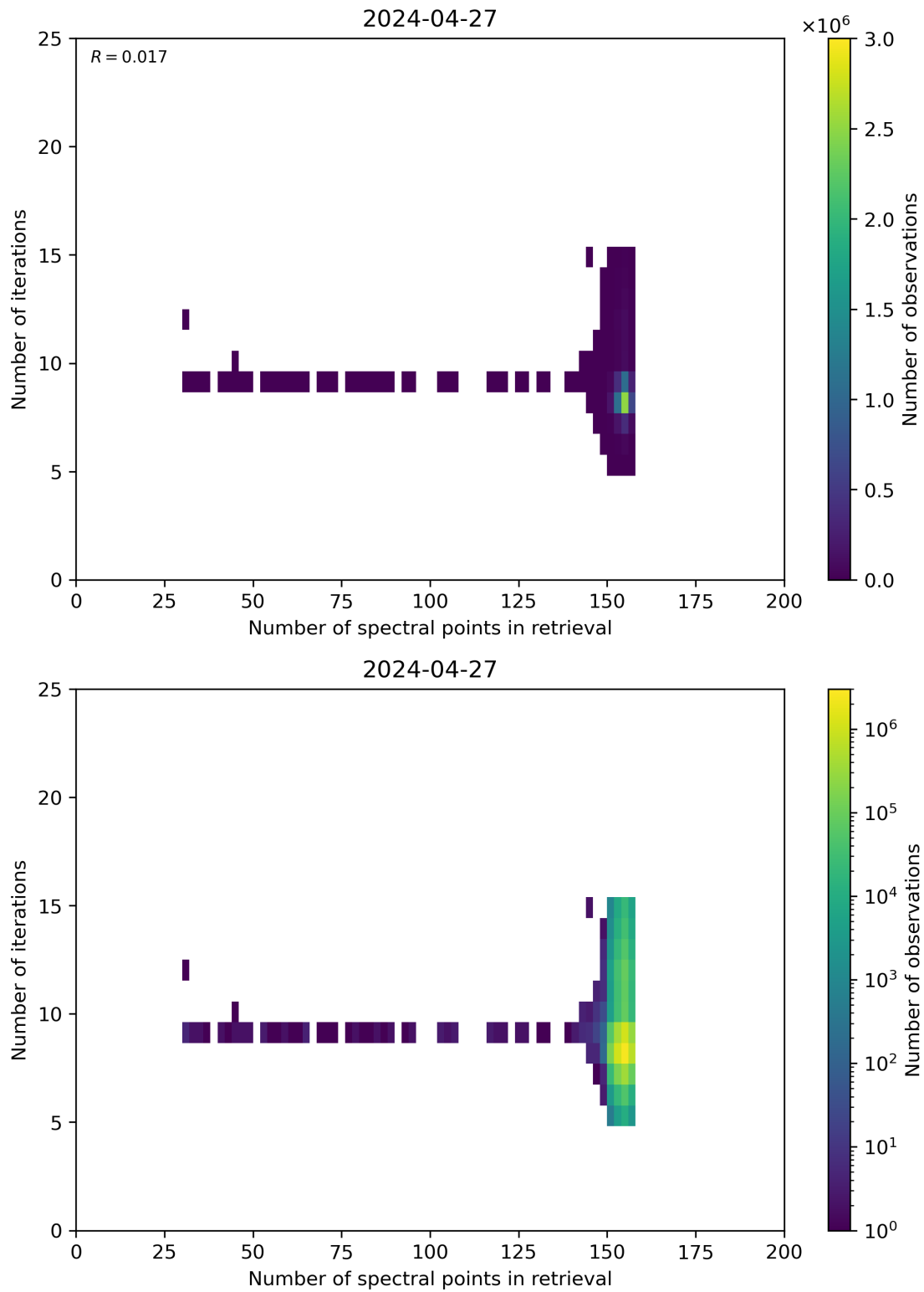
Figure 60: Scatter density plot of “Number of spectral points in retrieval” against “Number of iterations” for 2024-04-26 to 2024-04-28.
