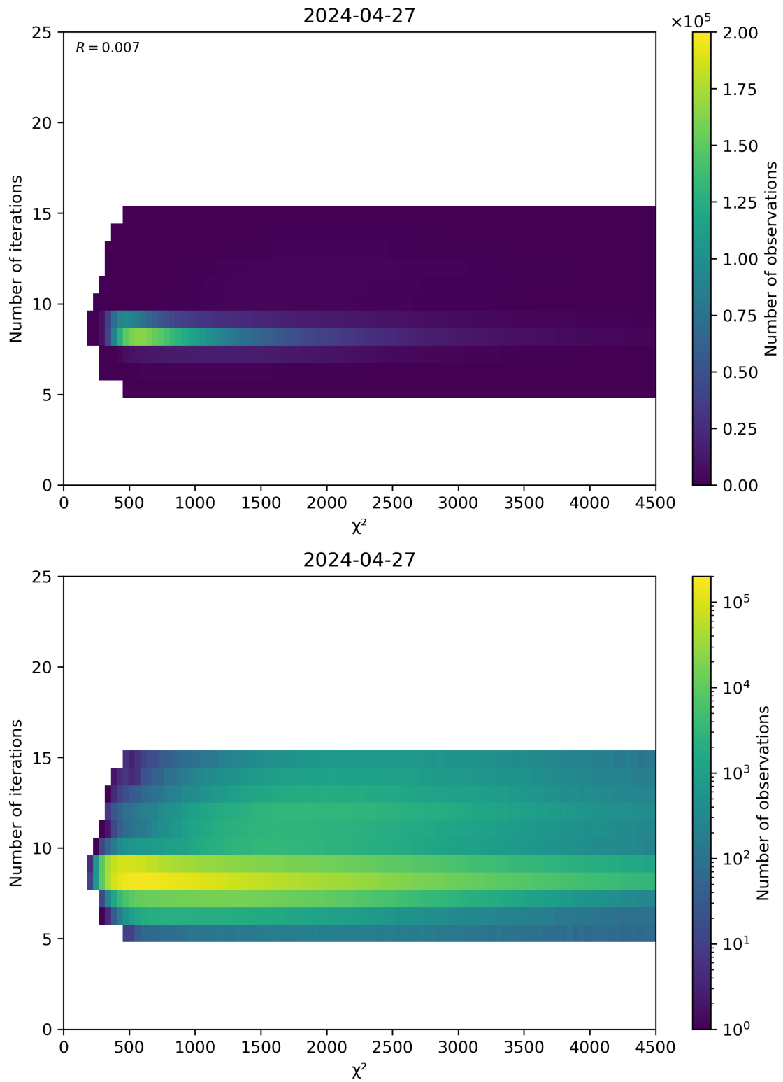
Figure 49: Scatter density plot of “ \chi^2 ” against “Number of iterations” for 2024-04-26 to 2024-04-28.
