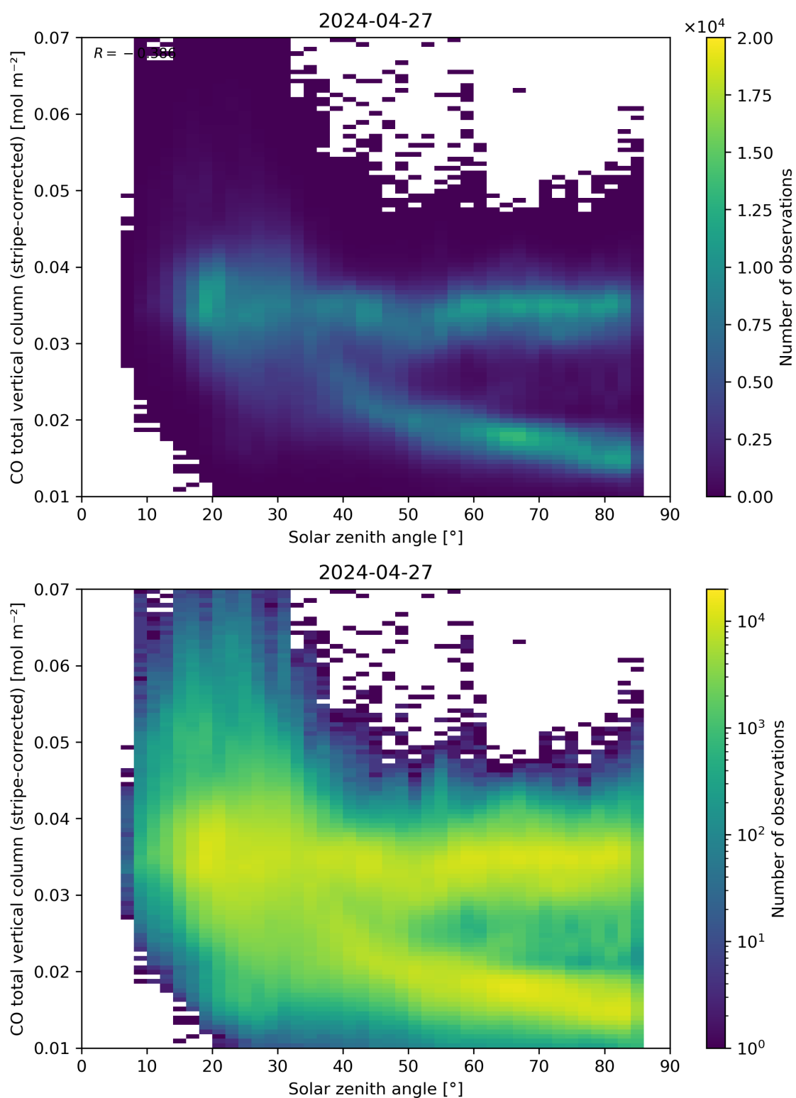
Figure 62: Scatter density plot of “Solar zenith angle” against “CO total vertical column (stripe-corrected)” for 2024-04-26 to 2024-04-28.
