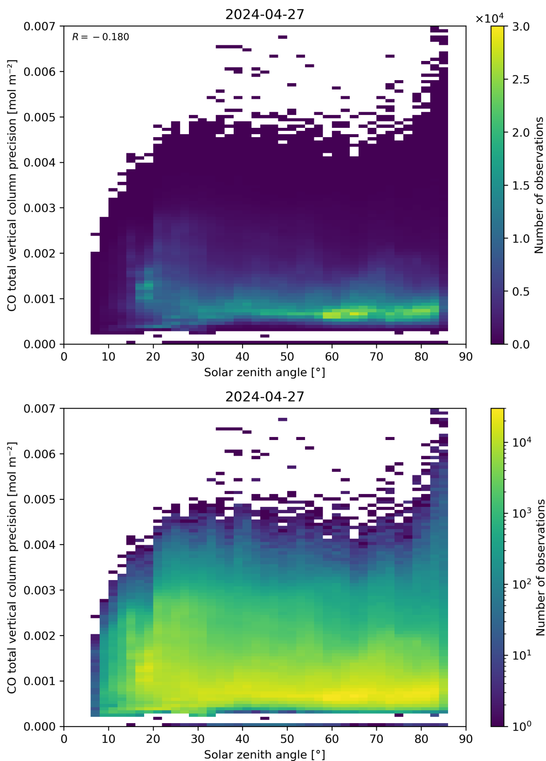
Figure 63: Scatter density plot of “Solar zenith angle” against “CO total vertical column precision” for 2024-04-26 to 2024-04-28.
