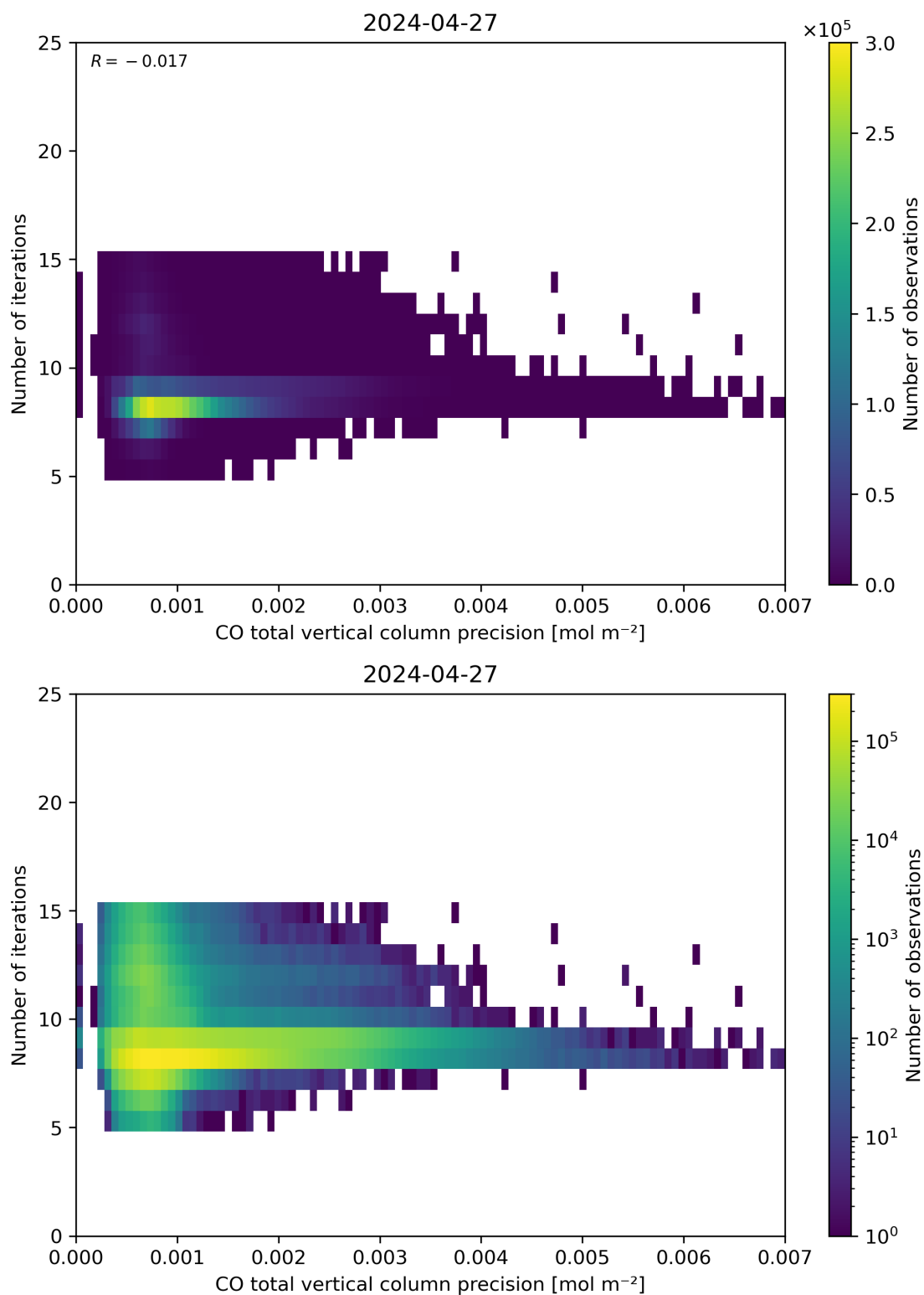
Figure 46: Scatter density plot of “CO total vertical column precision” against “Number of iterations” for 2024-04-26 to 2024-04-28.
