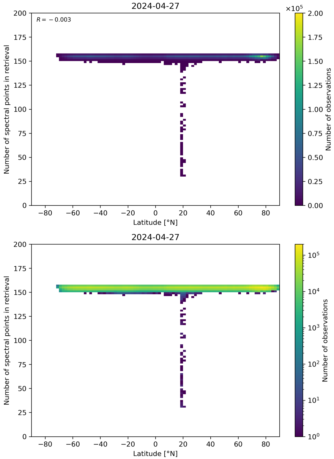
Figure 57: Scatter density plot of “Latitude” against “Number of spectral points in retrieval” for 2024-04-26 to 2024-04-28.
