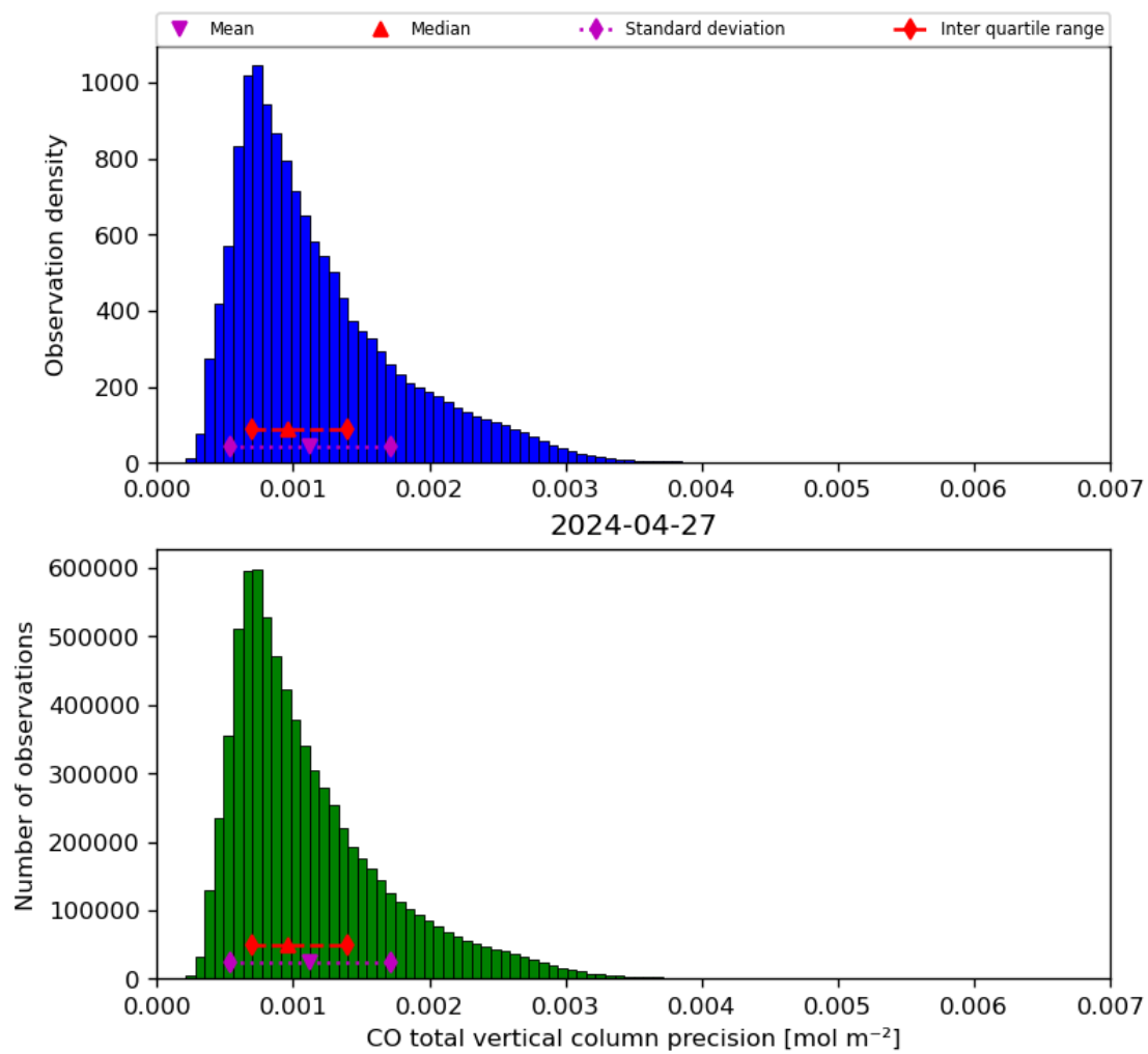
Figure 20: Histogram of “CO total vertical column precision” for 2024-04-26 to 2024-04-28
