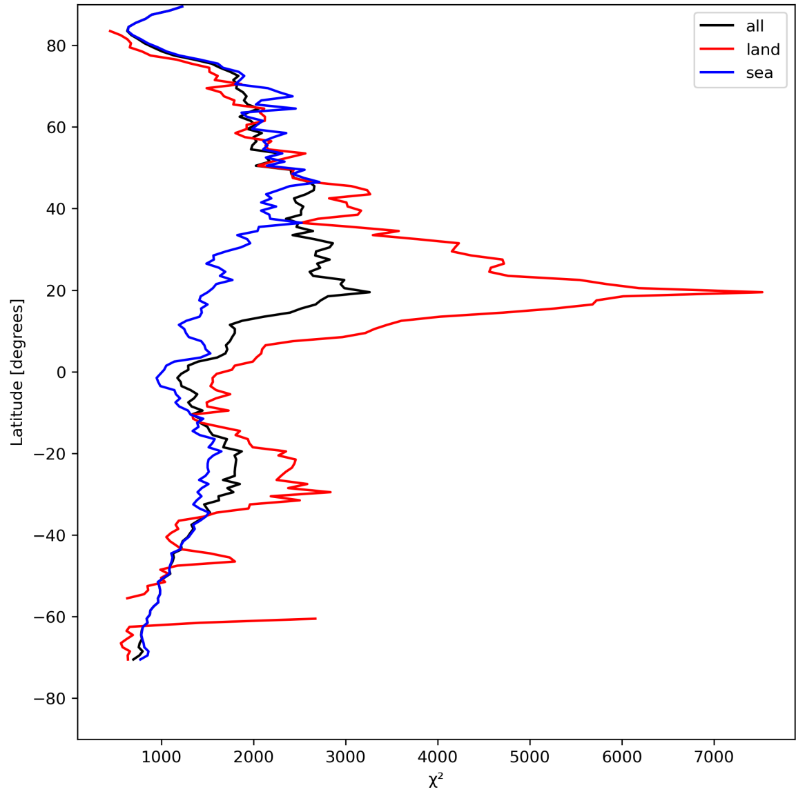
Figure 14: Zonal average of “ \chi^2 ” for 2024-04-26 to 2024-04-28.
