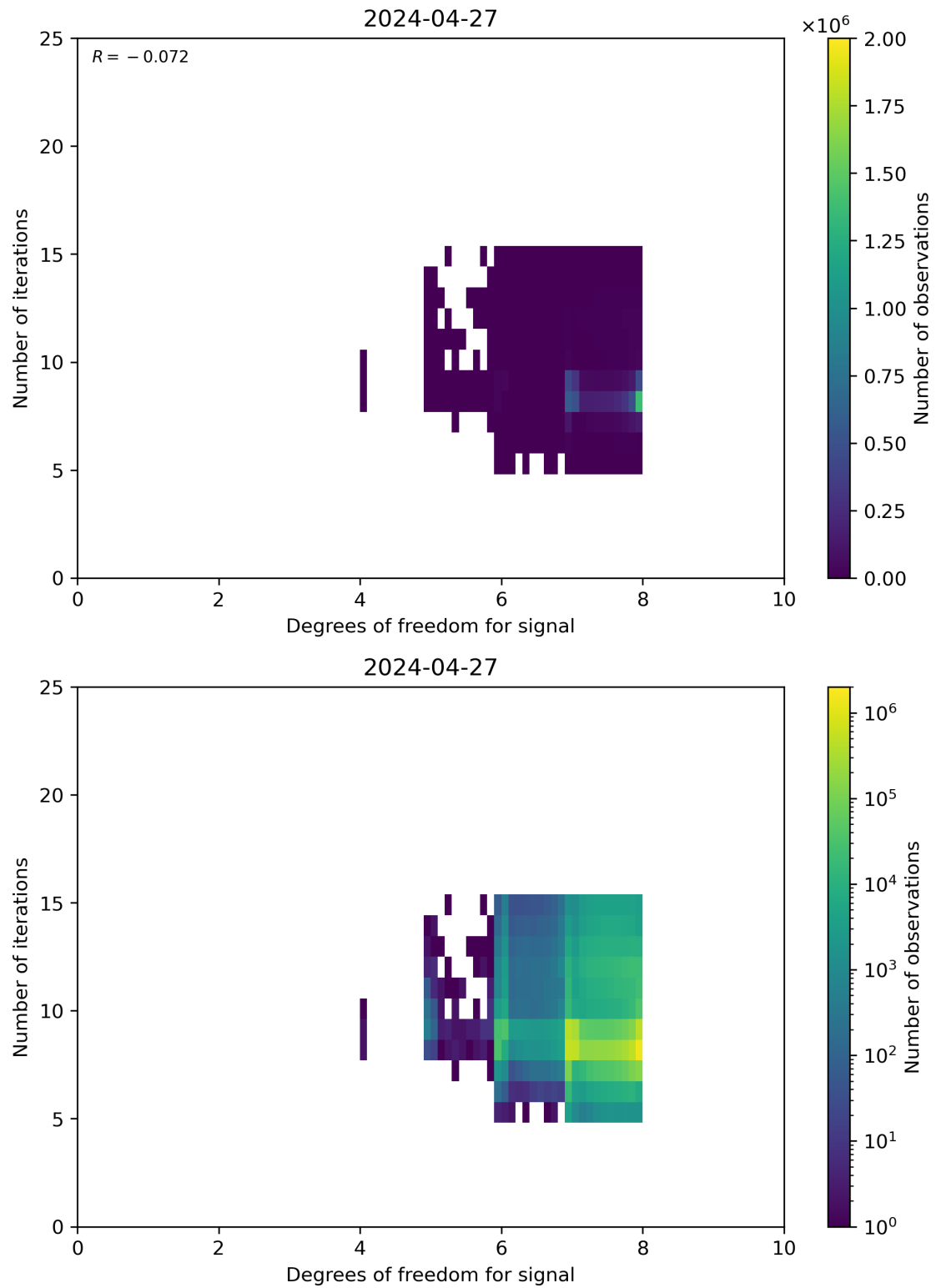
Figure 50: Scatter density plot of “Degrees of freedom for signal” against “Number of iterations” for 2024-04-26 to 2024-04-28.
