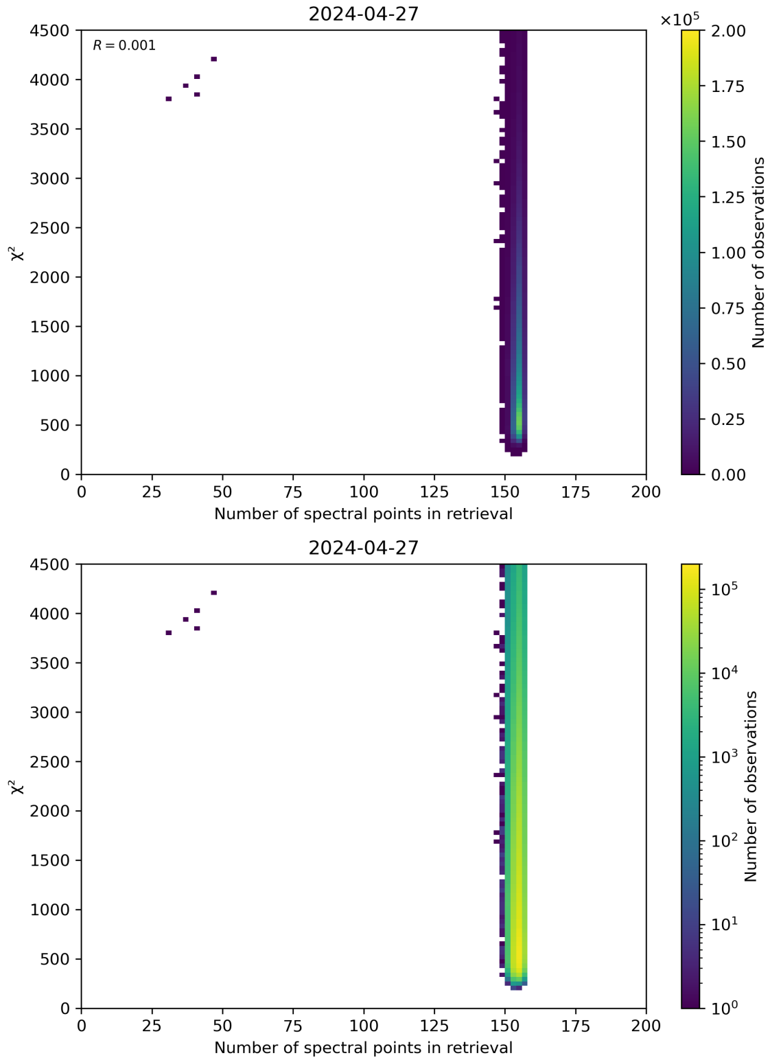
Figure 58: Scatter density plot of “Number of spectral points in retrieval” against “ \chi^2 ” for 2024-04-26 to 2024-04-28.
