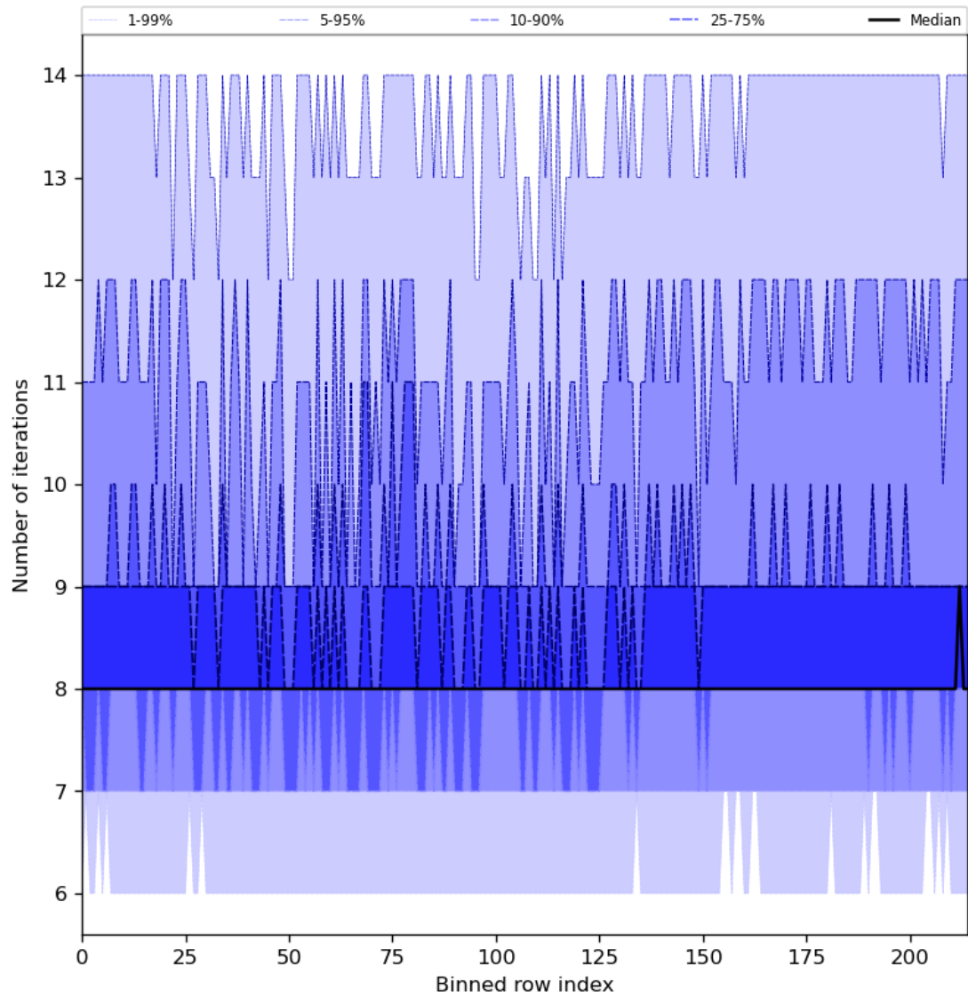
Figure 32: Along track statistics of “Number of iterations” for 2024-04-26 to 2024-04-28
