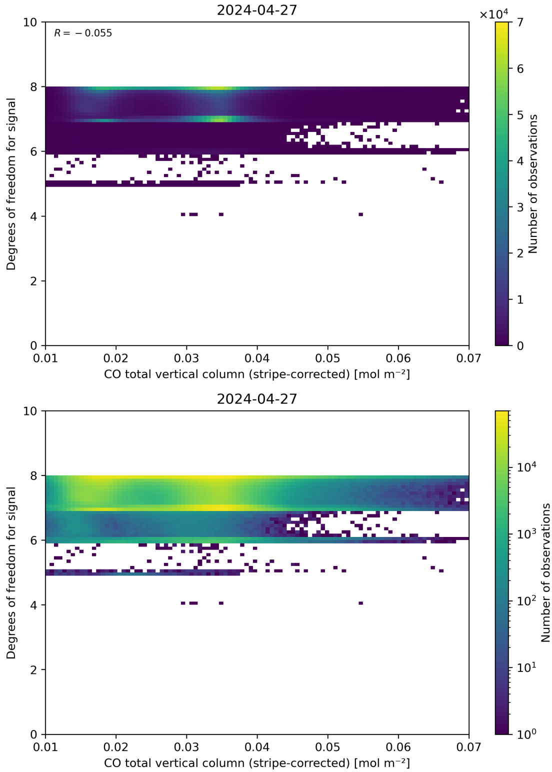
Figure 38: Scatter density plot of “CO total vertical column (stripe-corrected)” against “Degrees of freedom for signal” for 2024-04-26 to 2024-04-28.
