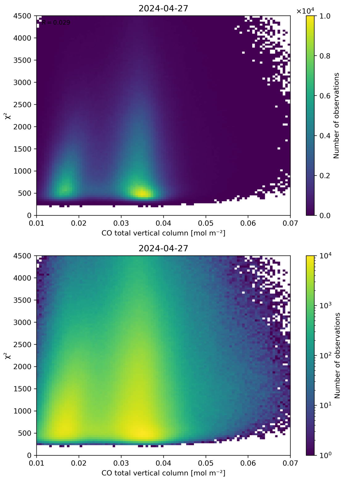
Figure 35: Scatter density plot of “CO total vertical column” against “ \chi^2 ” for 2024-04-26 to 2024-04-28.
