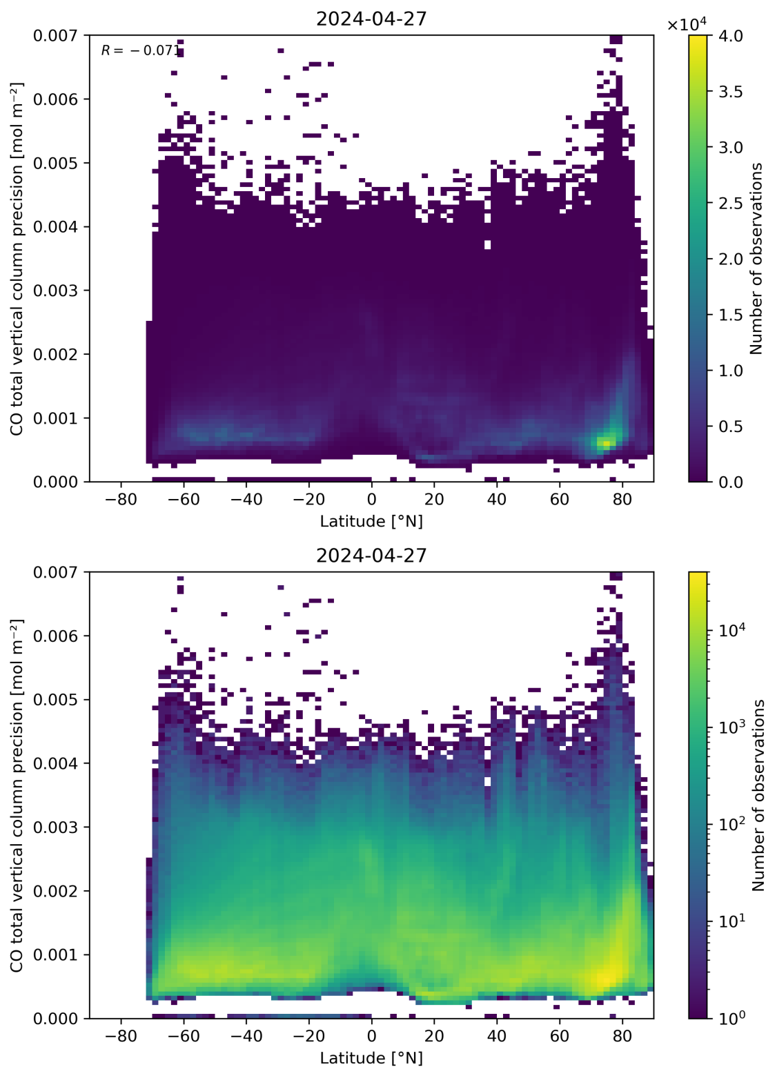
Figure 53: Scatter density plot of “Latitude” against “CO total vertical column precision” for 2024-04-26 to 2024-04-28.
