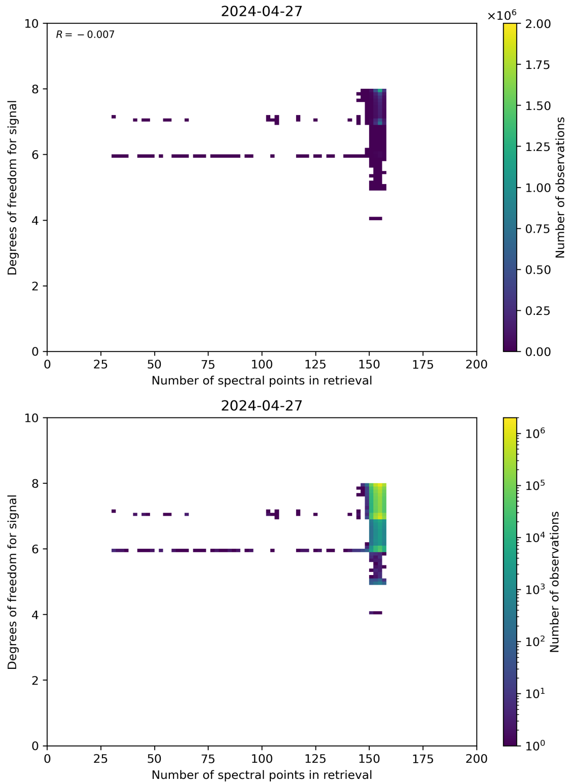
Figure 59: Scatter density plot of “Number of spectral points in retrieval” against “Degrees of freedom for signal” for 2024-04-26 to 2024-04-28.
