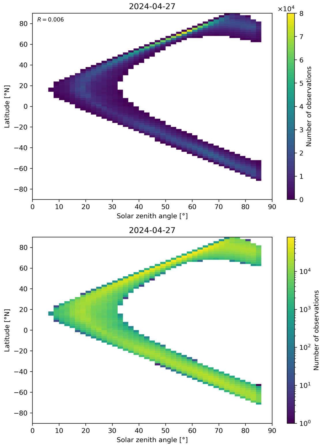
Figure 66: Scatter density plot of “Solar zenith angle” against “Latitude” for 2024-04-26 to 2024-04-28.
