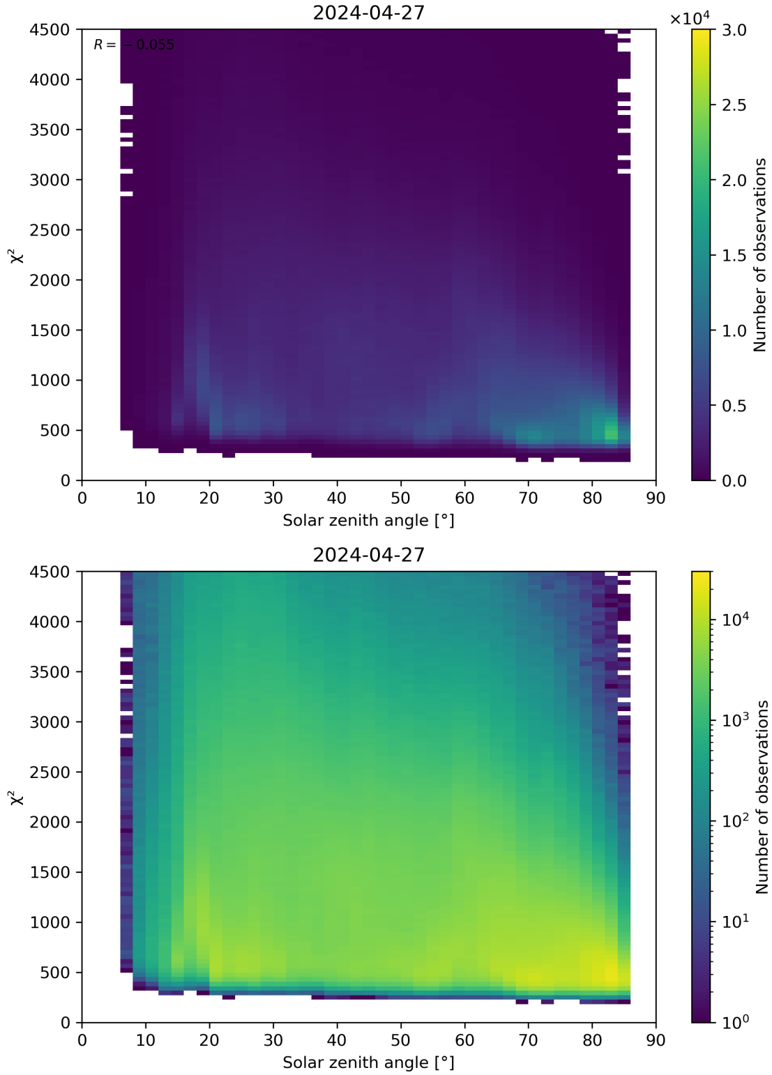
Figure 64: Scatter density plot of “Solar zenith angle” against “ \chi^2 ” for 2024-04-26 to 2024-04-28.
