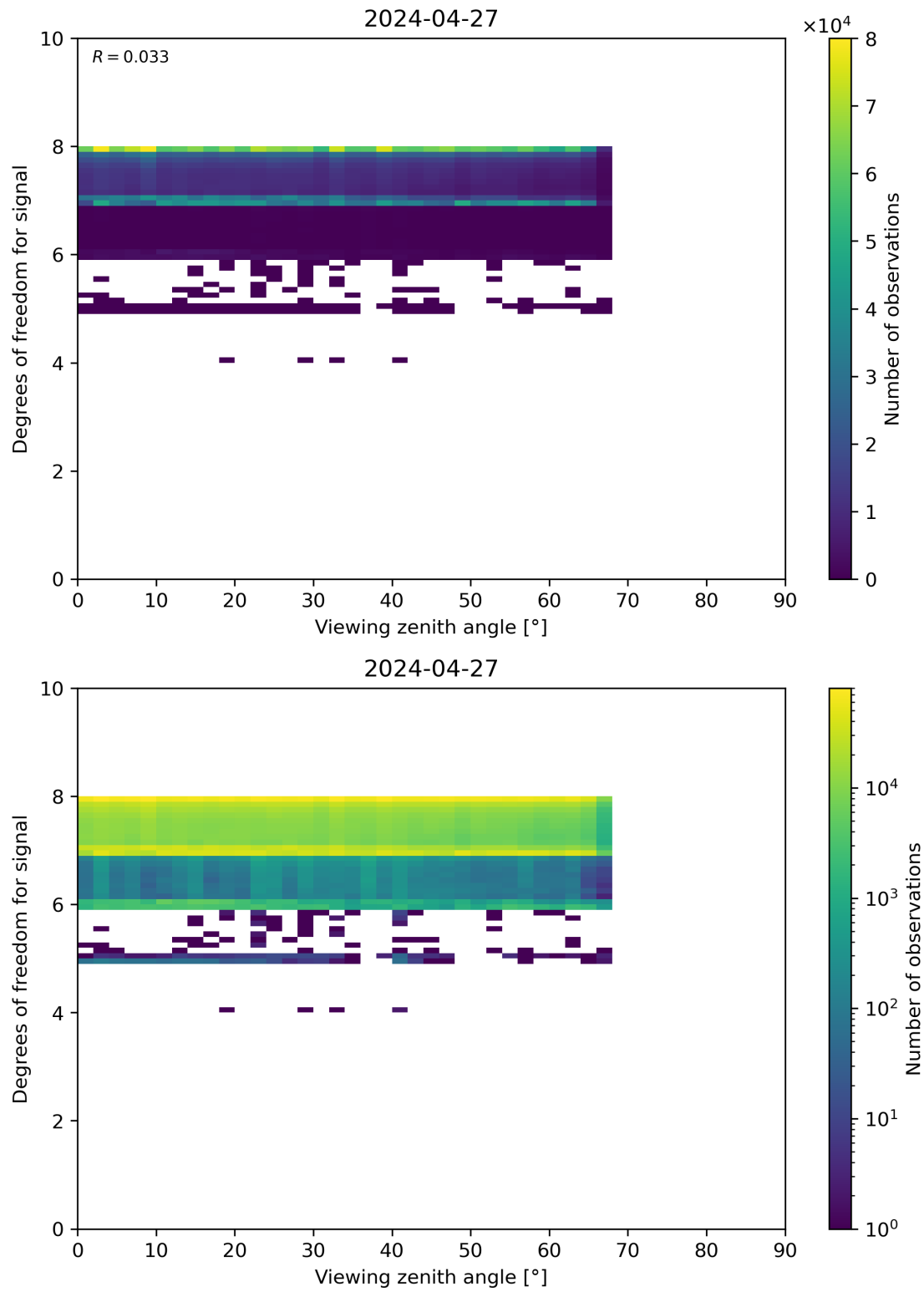
Figure 73: Scatter density plot of “Viewing zenith angle” against “Degrees of freedom for signal” for 2024-04-26 to 2024-04-28.
