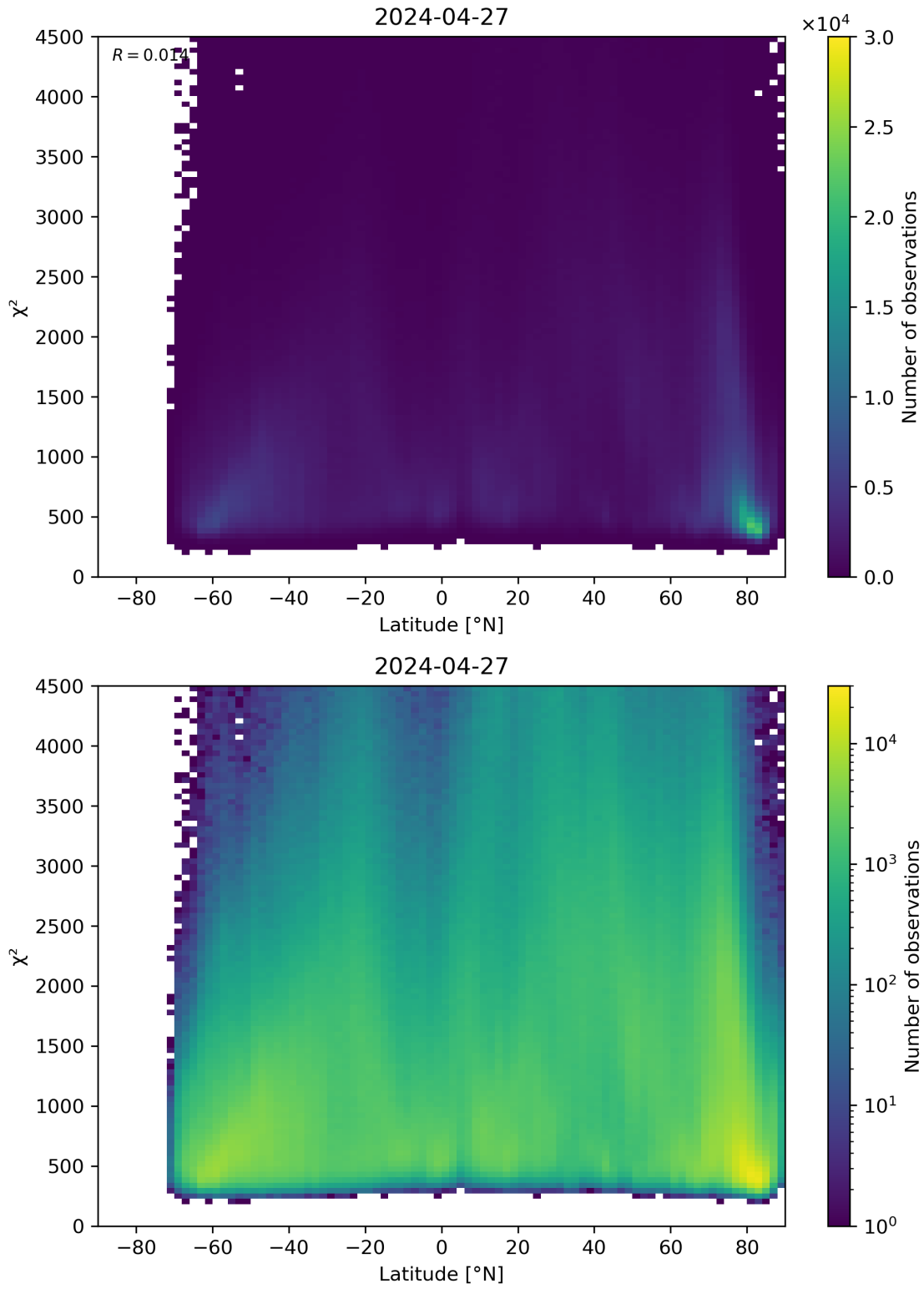
Figure 54: Scatter density plot of “Latitude” against “ \chi^2 ” for 2024-04-26 to 2024-04-28.
