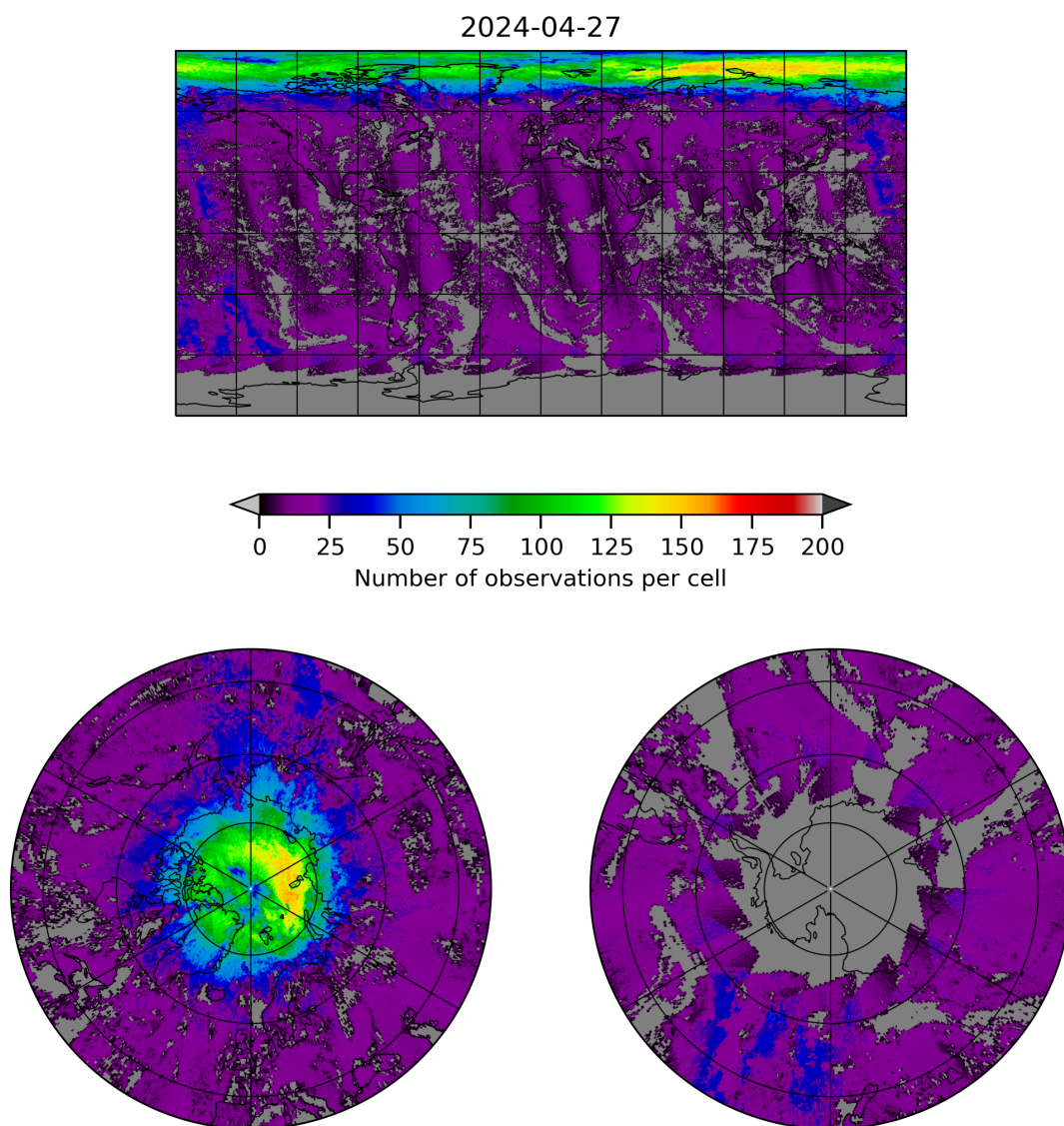
Figure 8: Map of the number of observations for 2024-04-26 to 2024-04-28
