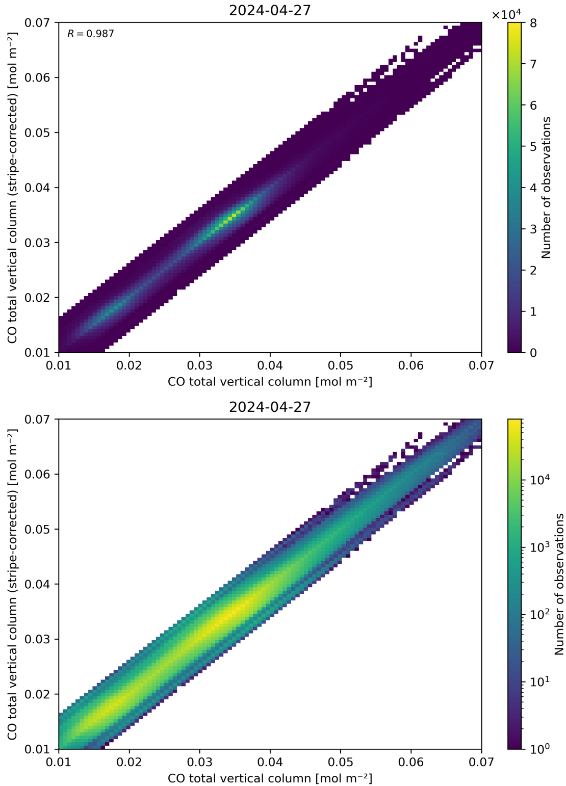
Figure 33: Scatter density plot of “CO total vertical column” against “CO total vertical column (stripe-corrected)” for 2024-04-26 to 2024-04-28.
