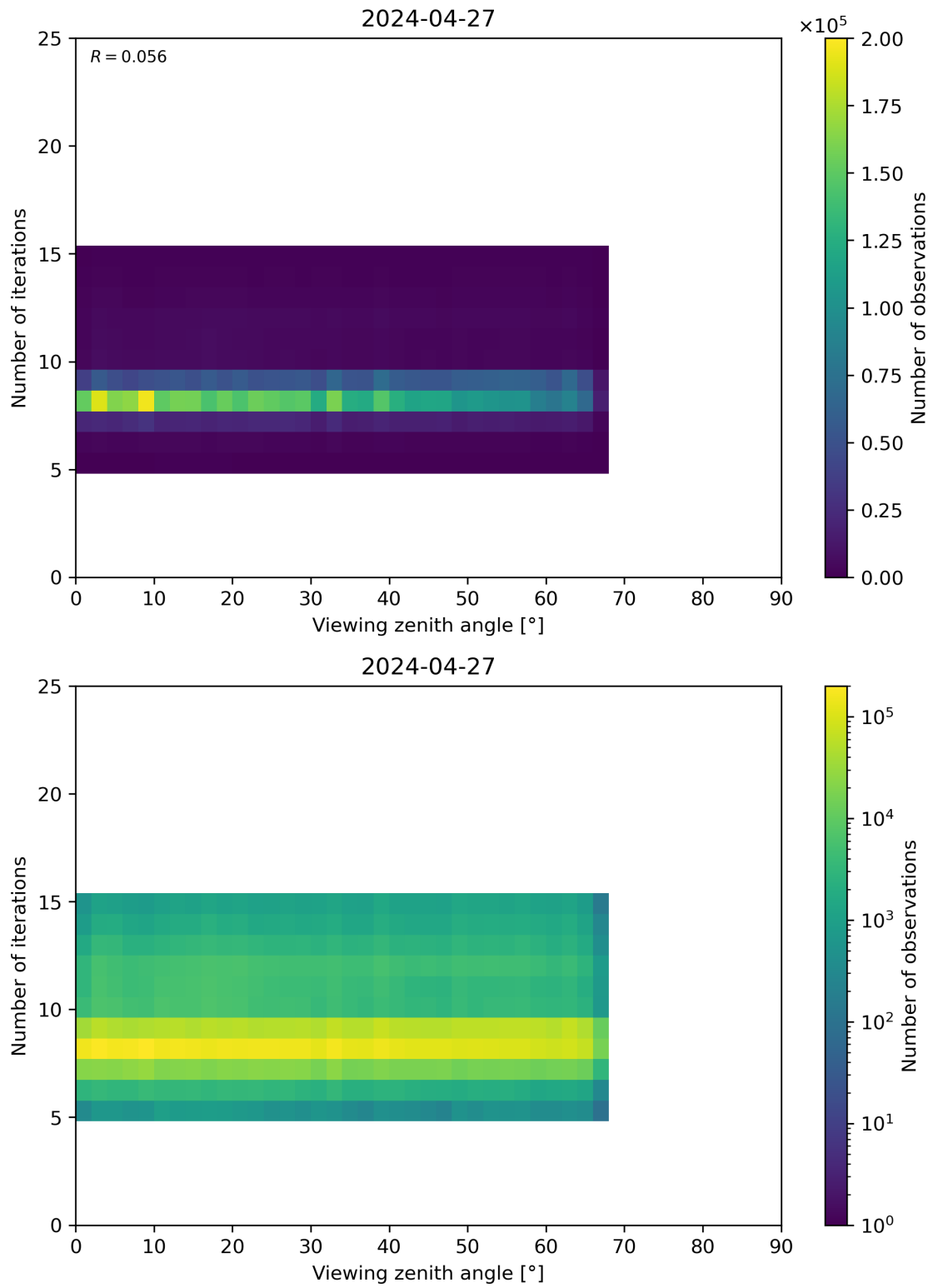
Figure 75: Scatter density plot of “Viewing zenith angle” against “Number of iterations” for 2024-04-26 to 2024-04-28.
