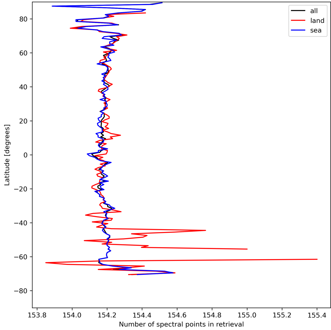
Figure 13: Zonal average of “Number of spectral points in retrieval” for 2024-04-27 to 2024-04-29.
