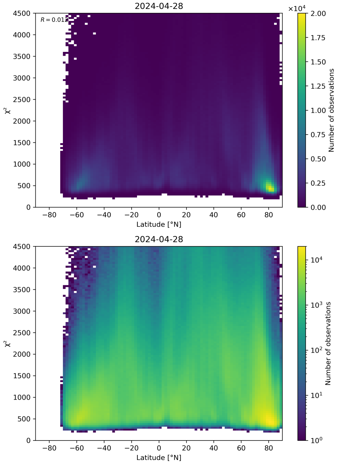
Figure 54: Scatter density plot of “Latitude” against “ \chi^2 ” for 2024-04-27 to 2024-04-29.
