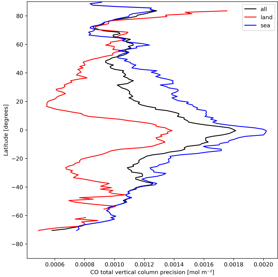
Figure 12: Zonal average of “CO total vertical column precision” for 2024-04-27 to 2024-04-29.
