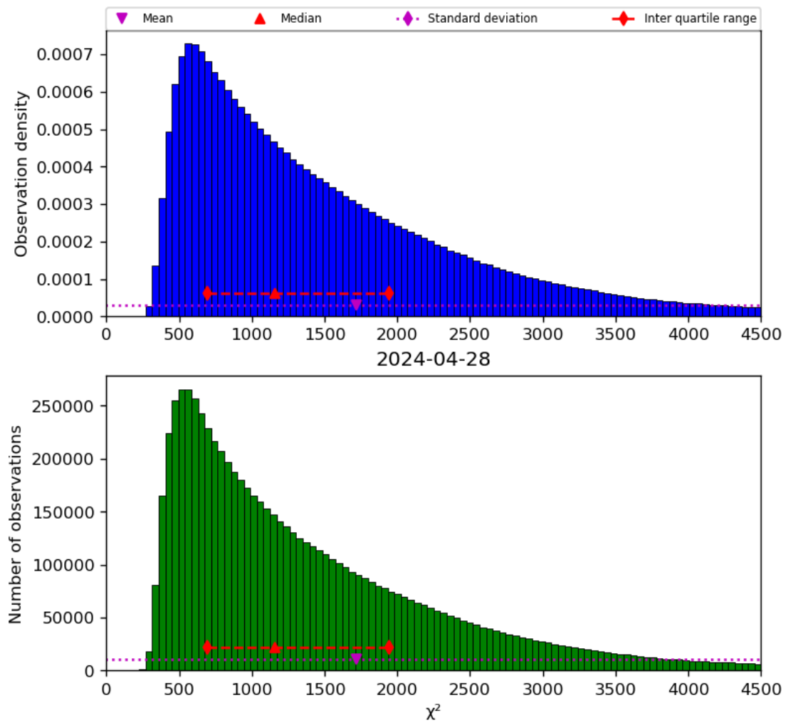
Figure 22: Histogram of “ \chi^2 ” for 2024-04-27 to 2024-04-29
