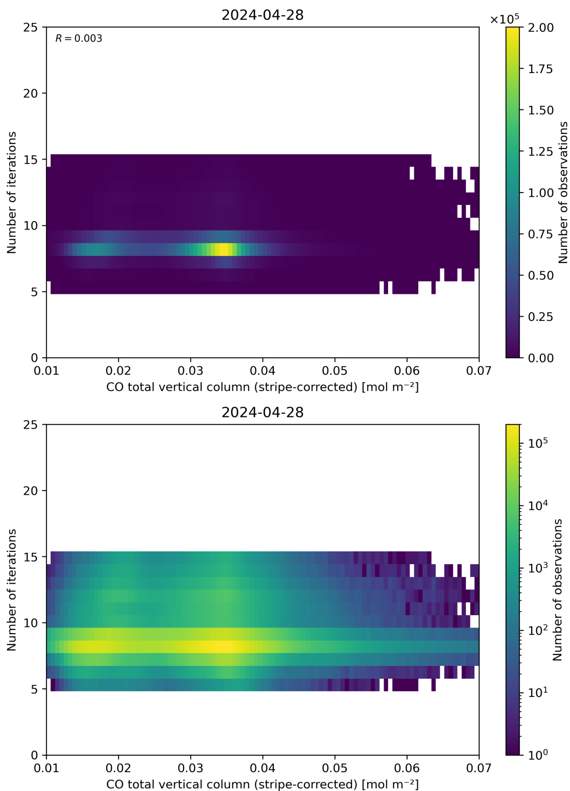
Figure 39: Scatter density plot of “CO total vertical column (stripe-corrected)” against “Number of iterations” for 2024-04-27 to 2024-04-29.
