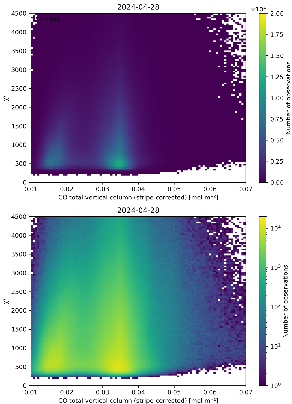
Figure 37: Scatter density plot of “CO total vertical column (stripe-corrected)” against “ \chi^2 ” for 2024-04-27 to 2024-04-29.
