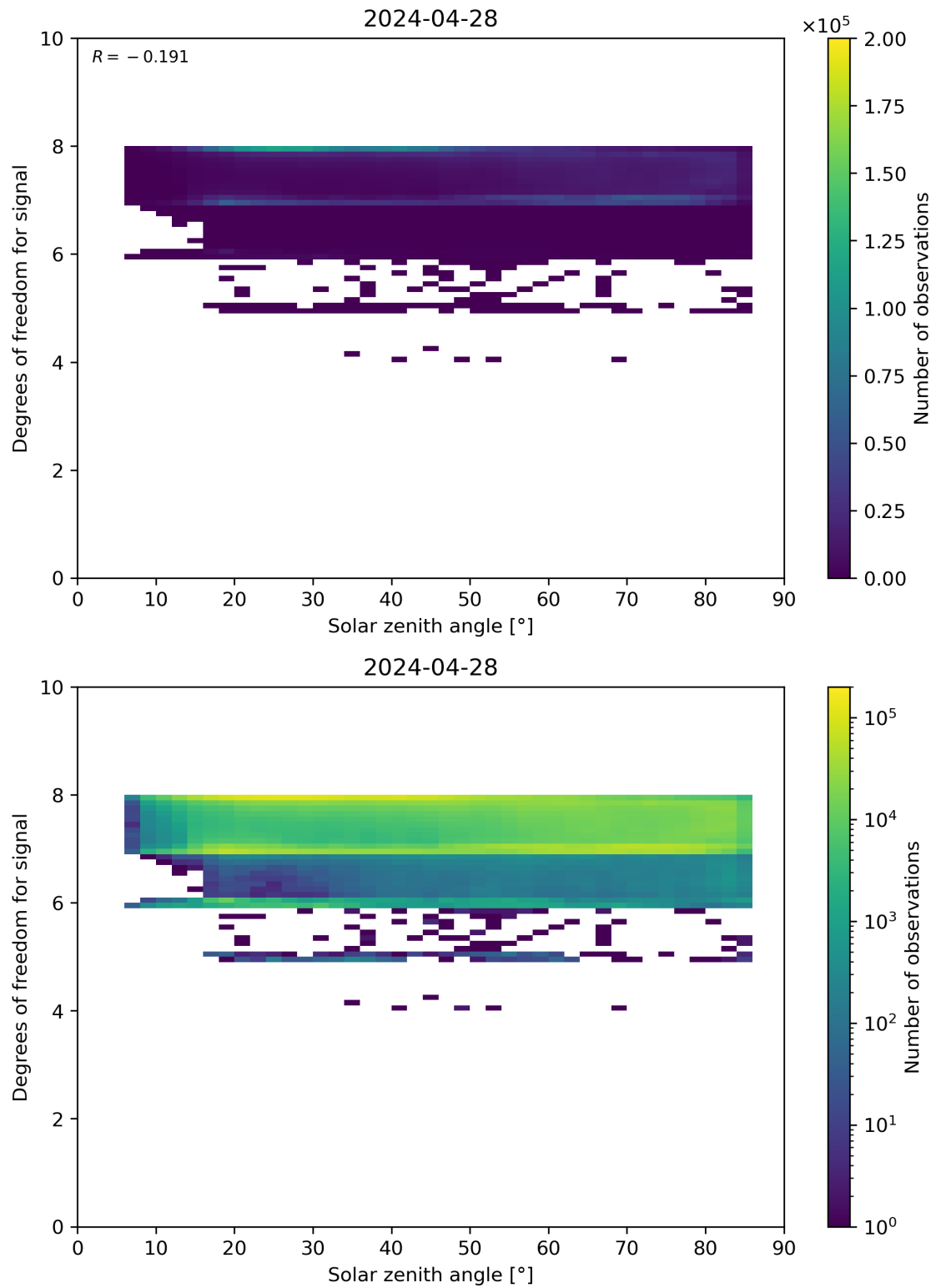
Figure 65: Scatter density plot of “Solar zenith angle” against “Degrees of freedom for signal” for 2024-04-27 to 2024-04-29.
