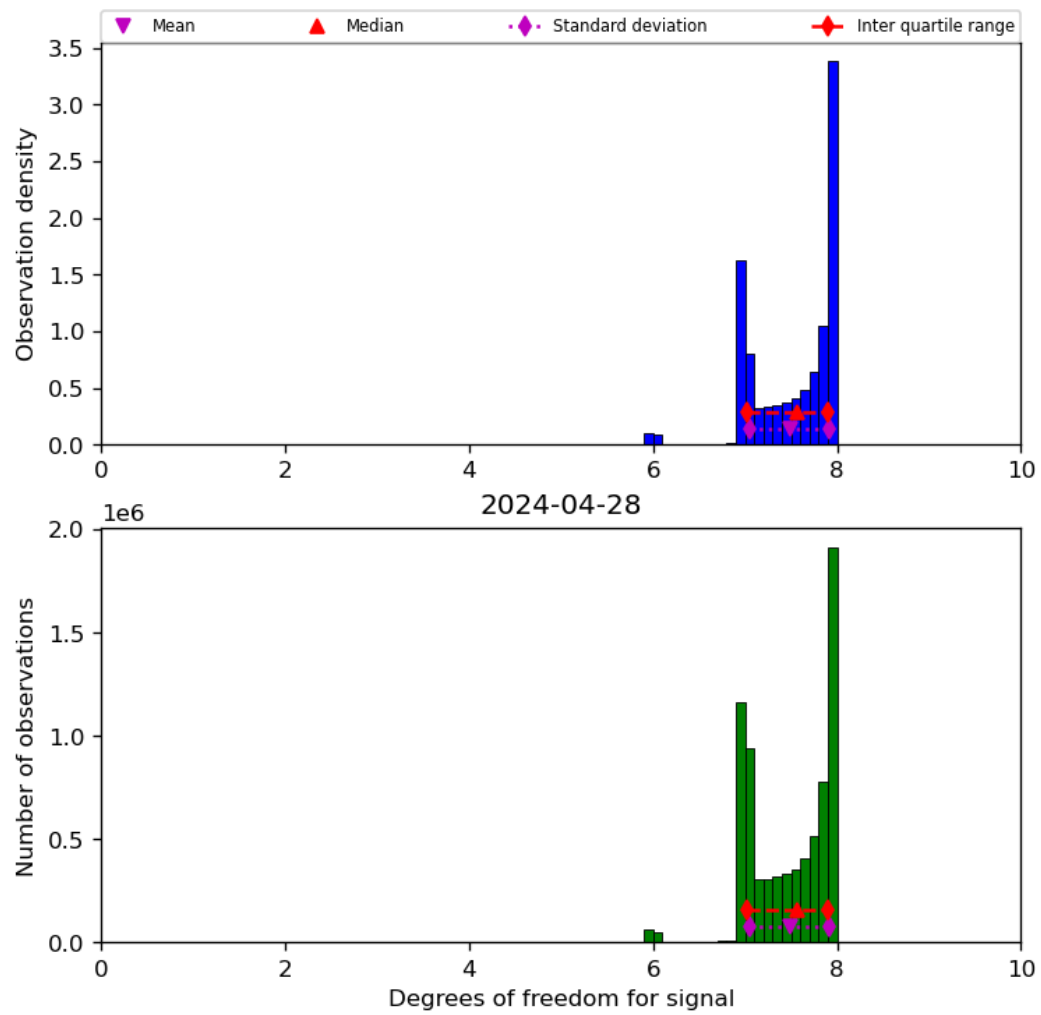
Figure 23: Histogram of “Degrees of freedom for signal” for 2024-04-27 to 2024-04-29
