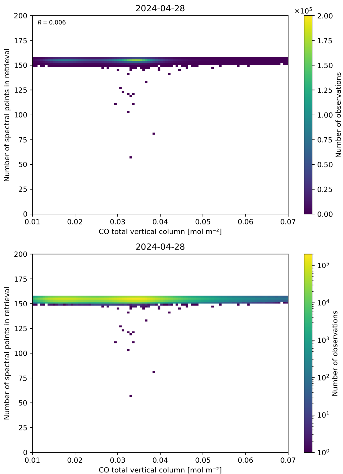
Figure 43: Scatter density plot of “CO total vertical column” against “Number of spectral points in retrieval” for 2024-04-27 to 2024-04-29.
