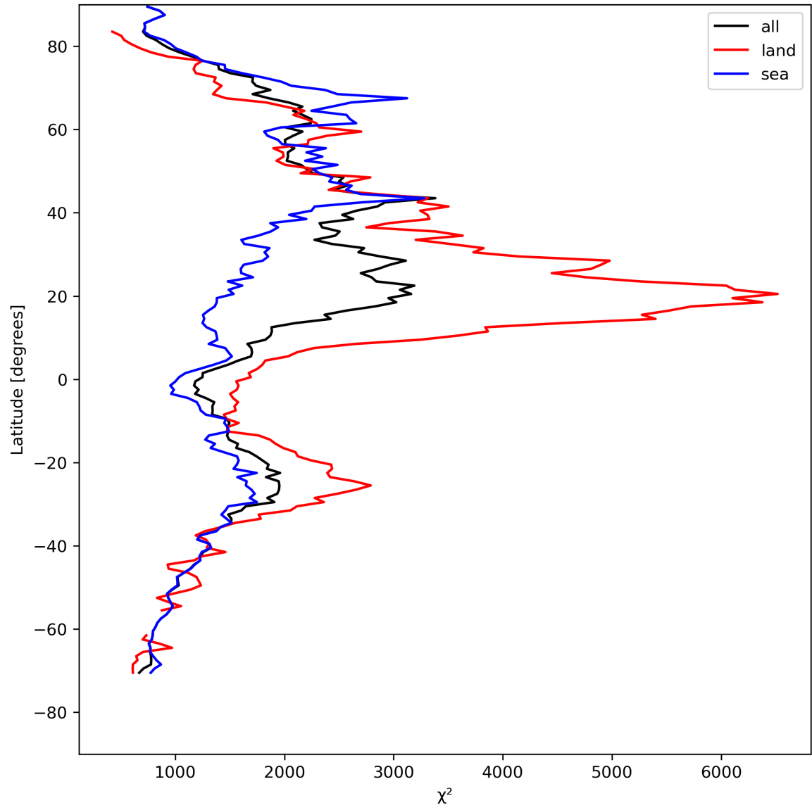
Figure 14: Zonal average of “ \chi^2 ” for 2024-04-27 to 2024-04-29.
