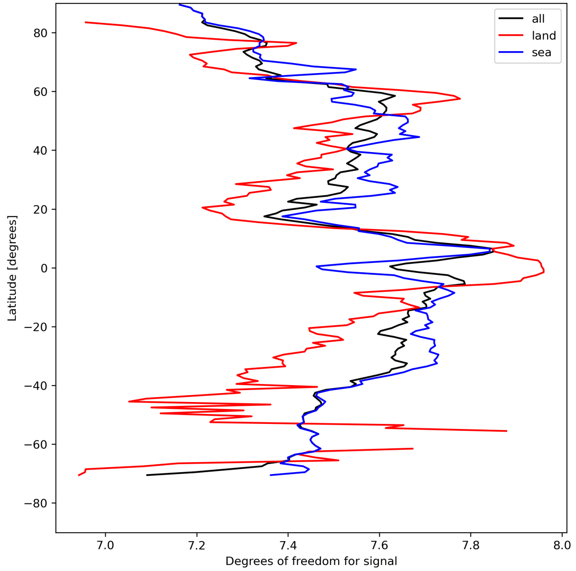
Figure 15: Zonal average of “Degrees of freedom for signal” for 2024-04-27 to 2024-04-29.
