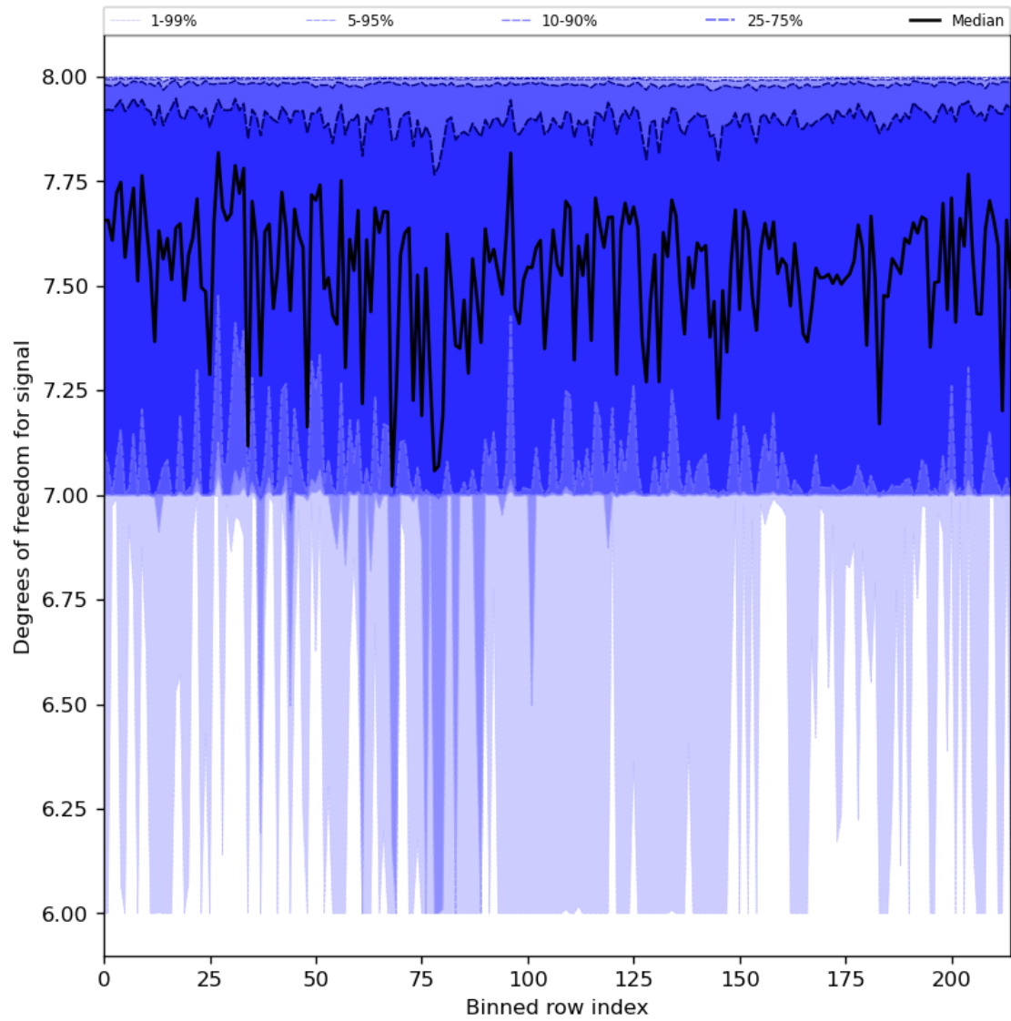
Figure 31: Along track statistics of “Degrees of freedom for signal” for 2024-04-27 to 2024-04-29
