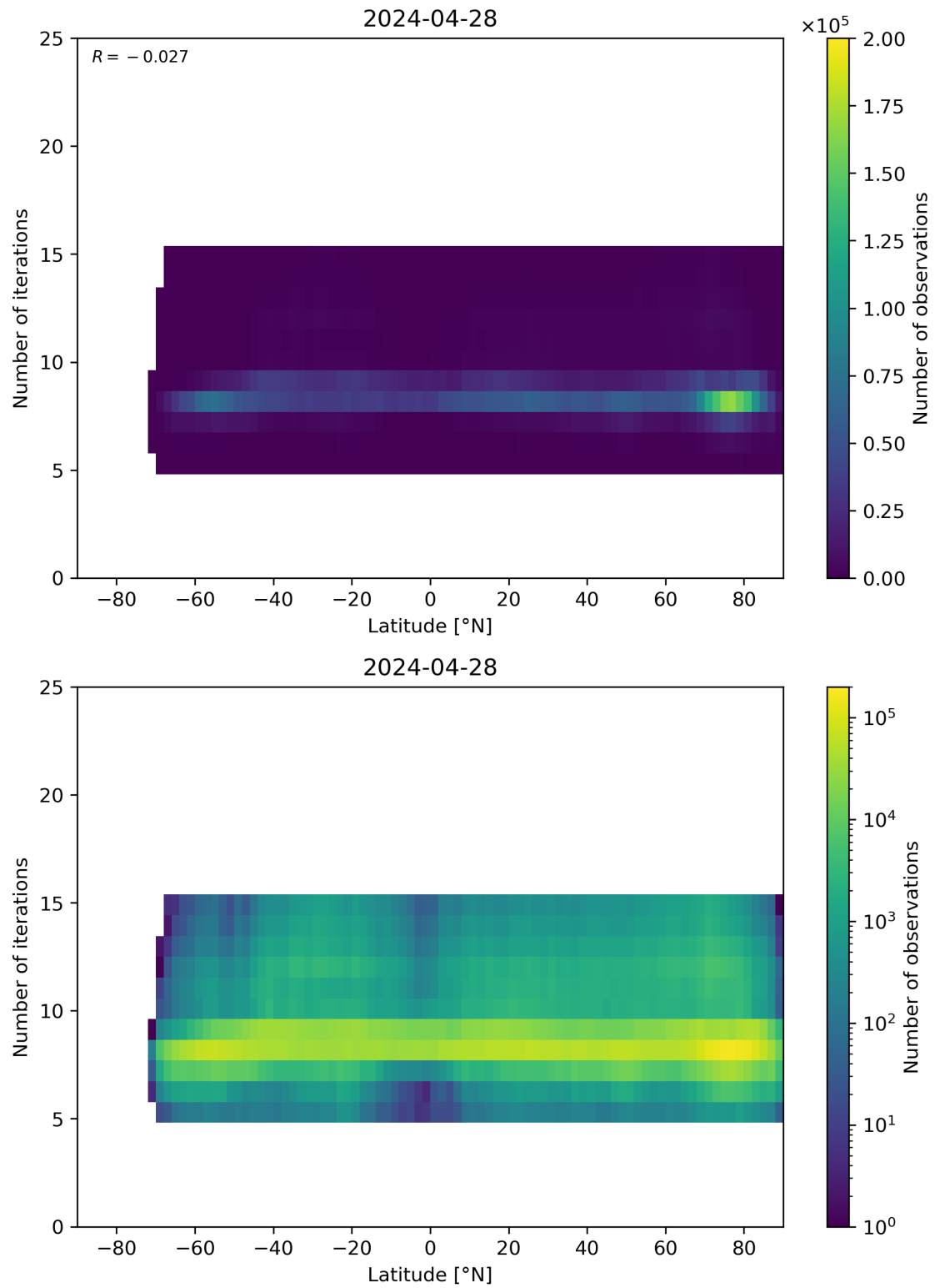
Figure 56: Scatter density plot of “Latitude” against “Number of iterations” for 2024-04-27 to 2024-04-29.
