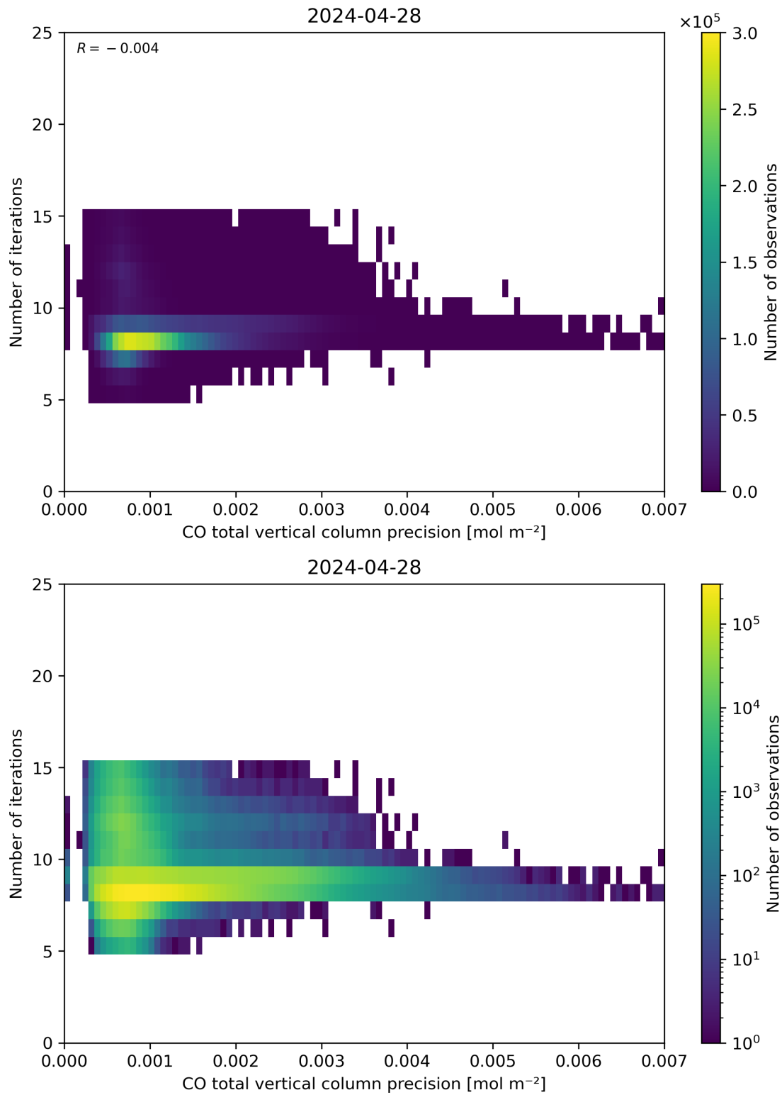
Figure 46: Scatter density plot of “CO total vertical column precision” against “Number of iterations” for 2024-04-27 to 2024-04-29.
