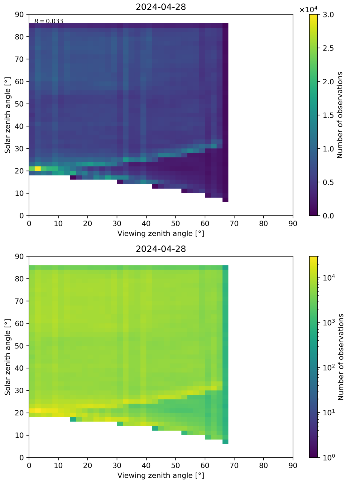
Figure 77: Scatter density plot of “Viewing zenith angle” against “Solar zenith angle” for 2024-04-27 to 2024-04-29.
