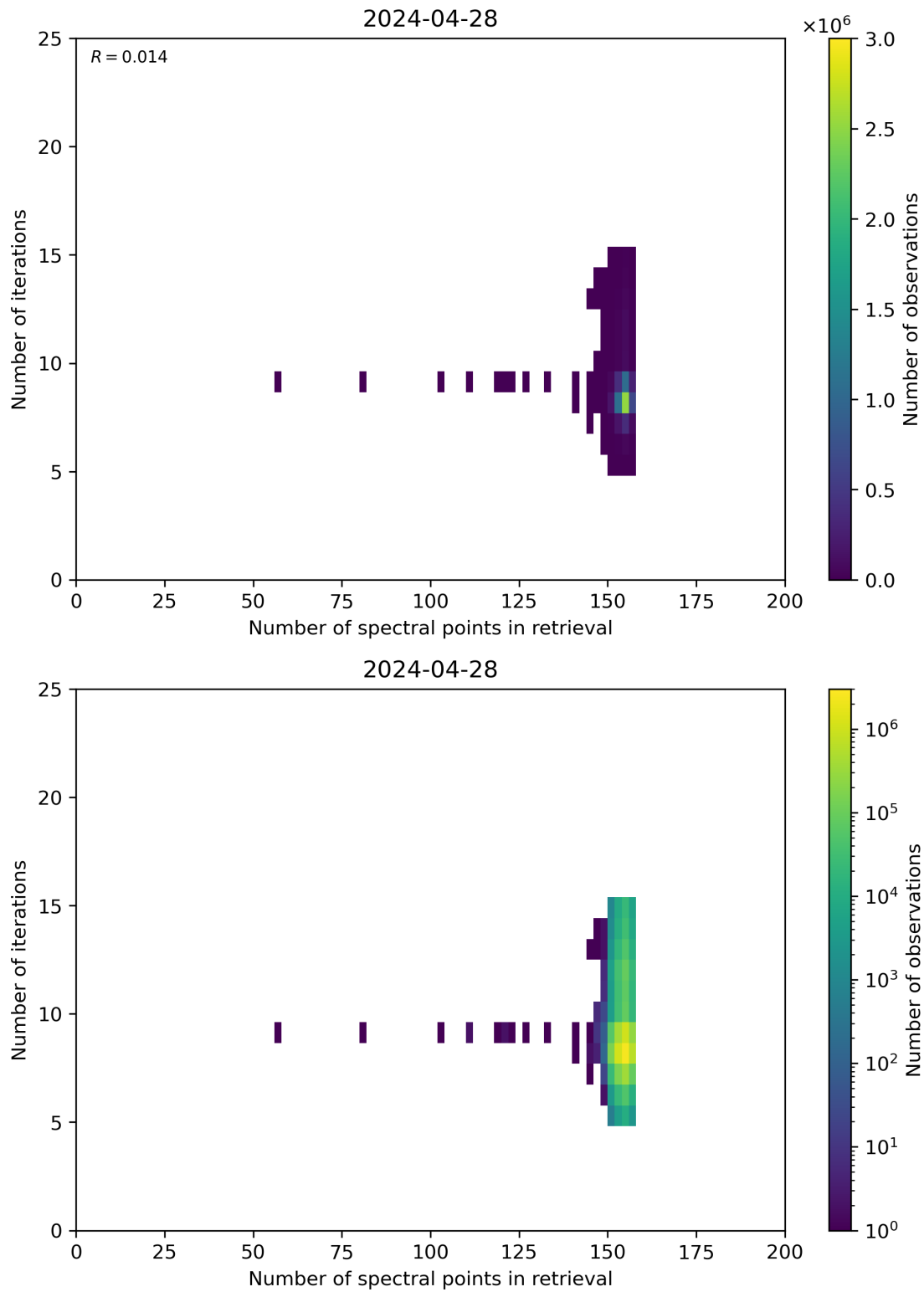
Figure 60: Scatter density plot of “Number of spectral points in retrieval” against “Number of iterations” for 2024-04-27 to 2024-04-29.
