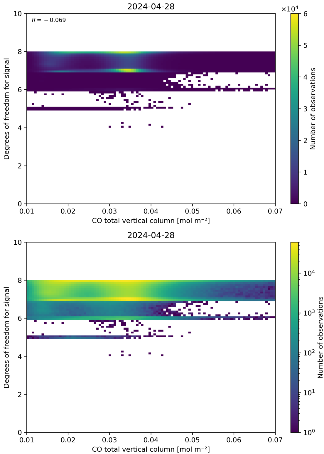
Figure 41: Scatter density plot of “CO total vertical column” against “Degrees of freedom for signal” for 2024-04-27 to 2024-04-29.
