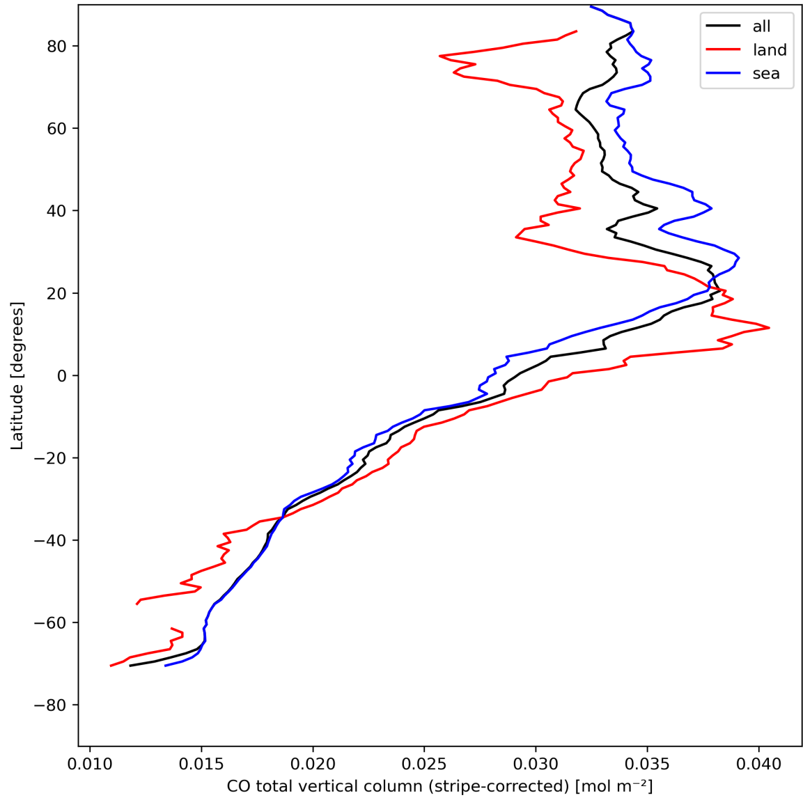
Figure 11: Zonal average of “CO total vertical column (stripe-corrected)” for 2024-04-27 to 2024-04-29.
