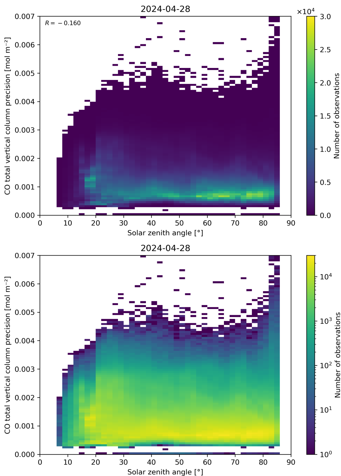
Figure 63: Scatter density plot of “Solar zenith angle” against “CO total vertical column precision” for 2024-04-27 to 2024-04-29.
