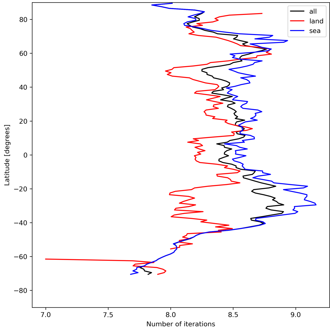
Figure 16: Zonal average of “Number of iterations” for 2024-04-27 to 2024-04-29.
