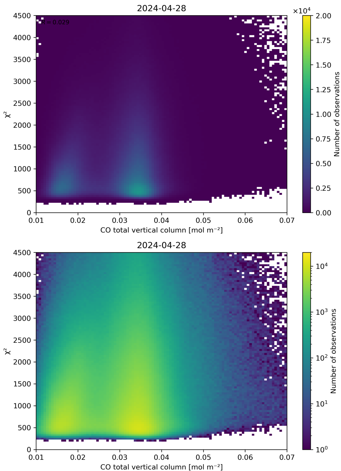
Figure 35: Scatter density plot of “CO total vertical column” against “ \chi^2 ” for 2024-04-27 to 2024-04-29.
