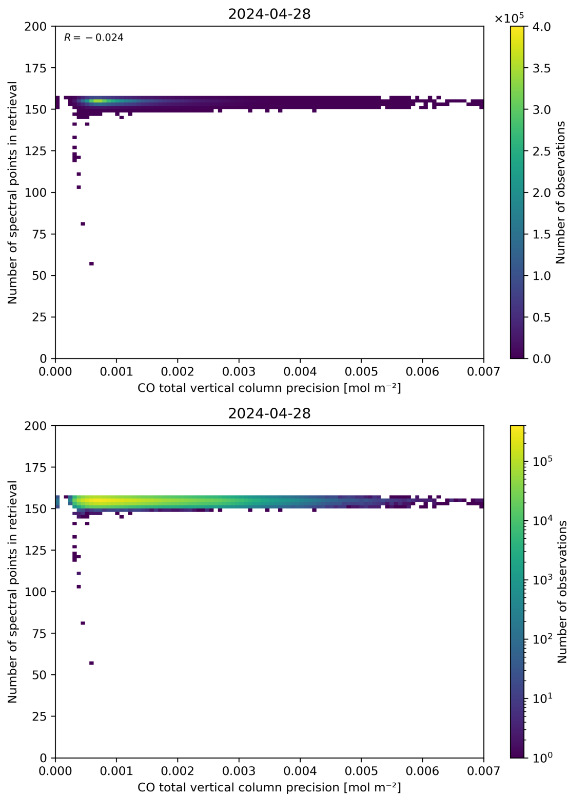
Figure 47: Scatter density plot of “CO total vertical column precision” against “Number of spectral points in retrieval” for 2024-04-27 to 2024-04-29.
