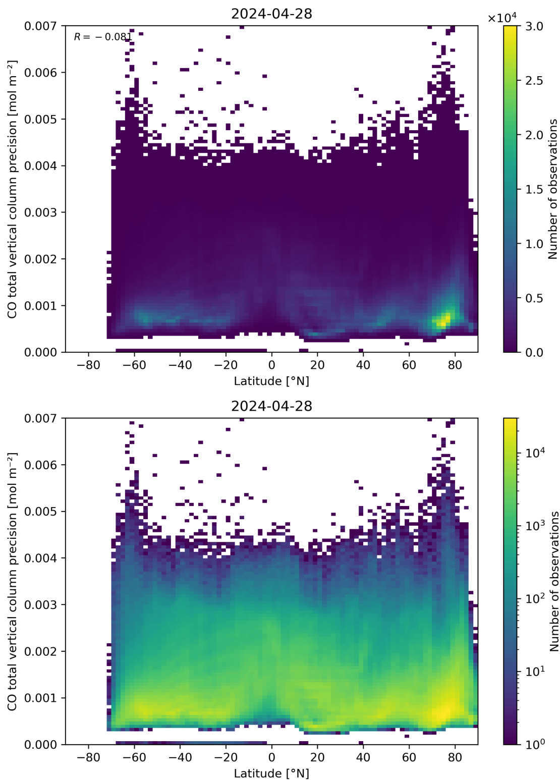
Figure 53: Scatter density plot of “Latitude” against “CO total vertical column precision” for 2024-04-27 to 2024-04-29.
