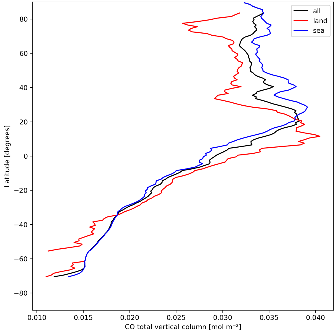
Figure 10: Zonal average of “CO total vertical column” for 2024-04-27 to 2024-04-29.
