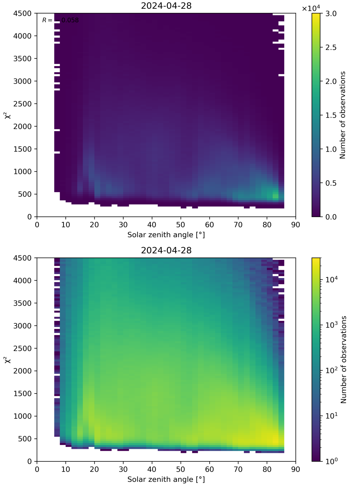
Figure 64: Scatter density plot of “Solar zenith angle” against “ \chi^2 ” for 2024-04-27 to 2024-04-29.
