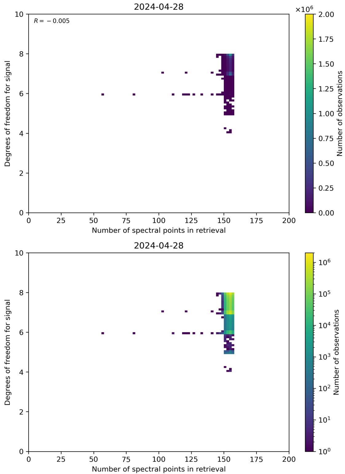
Figure 59: Scatter density plot of “Number of spectral points in retrieval” against “Degrees of freedom for signal” for 2024-04-27 to 2024-04-29.
