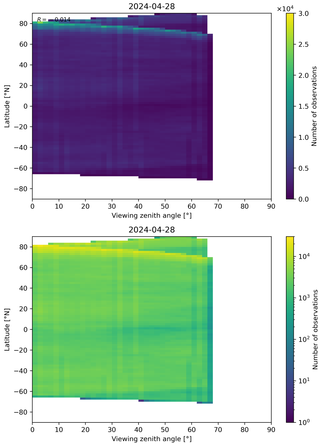
Figure 74: Scatter density plot of “Viewing zenith angle” against “Latitude” for 2024-04-27 to 2024-04-29.
