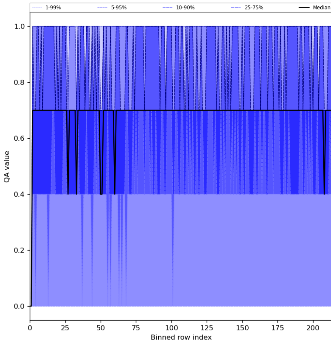
Figure 25: Along track statistics of “QA value” for 2024-04-27 to 2024-04-29
