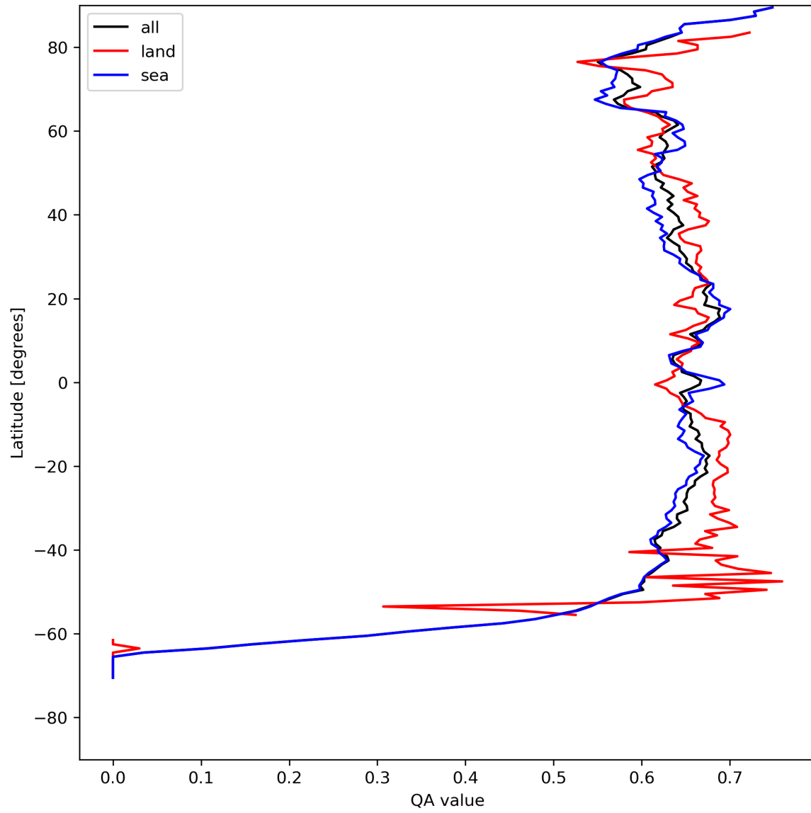
Figure 9: Zonal average of “QA value” for 2024-04-27 to 2024-04-29.
