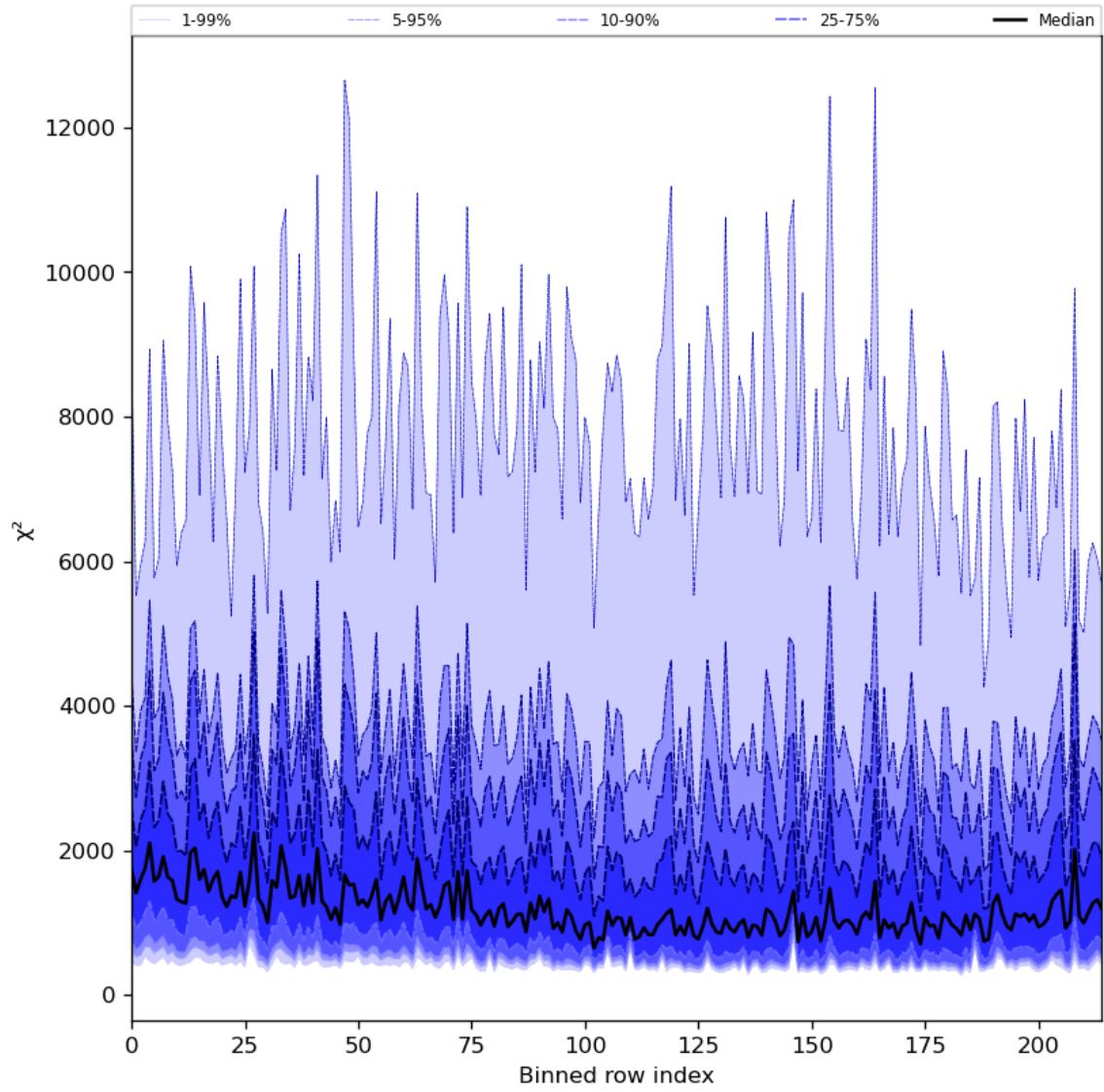
Figure 30: Along track statistics of “ \chi^2 ” for 2024-04-27 to 2024-04-29
