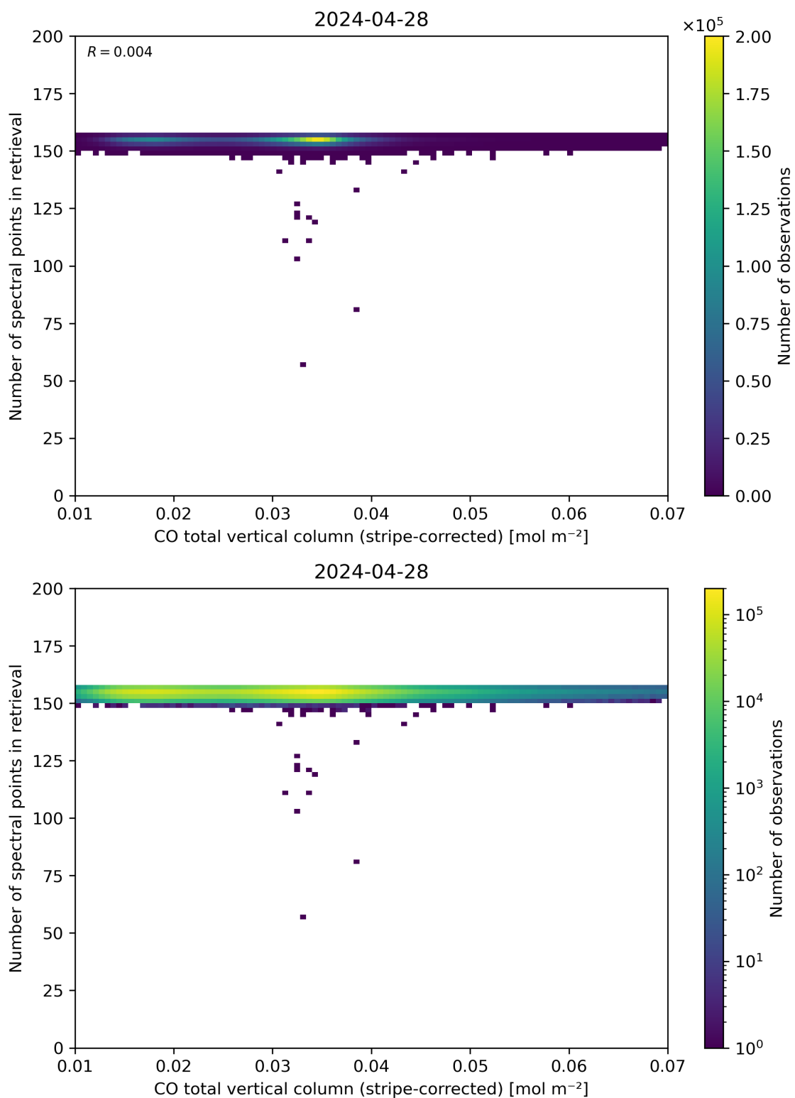
Figure 40: Scatter density plot of “CO total vertical column (stripe-corrected)” against “Number of spectral points in retrieval” for 2024-04-27 to 2024-04-29.
