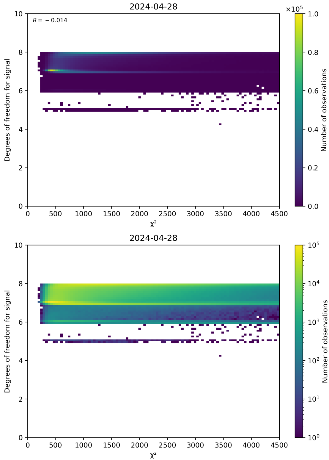
Figure 48: Scatter density plot of “ \chi^2 ” against “Degrees of freedom for signal” for 2024-04-27 to 2024-04-29.
