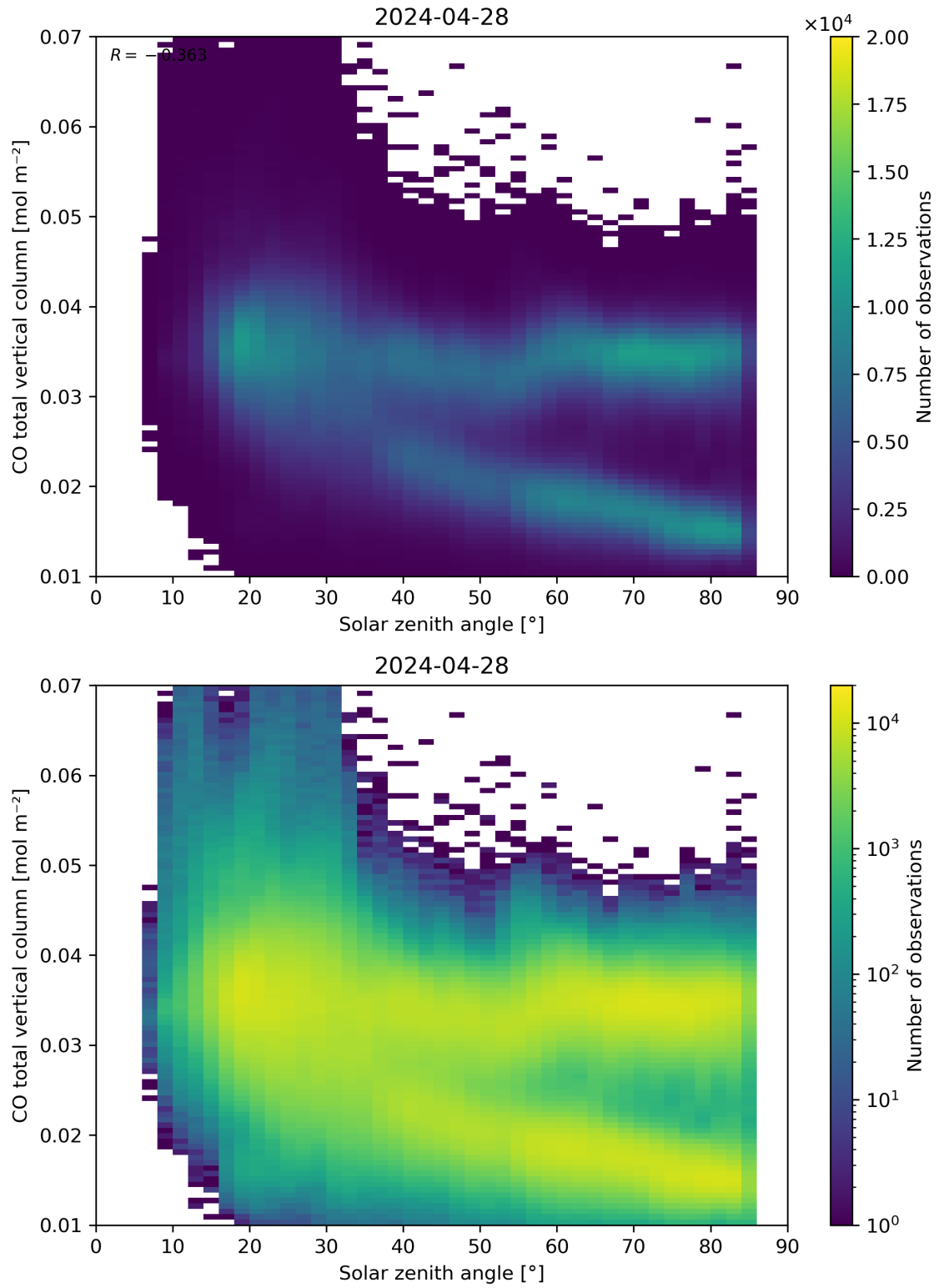
Figure 61: Scatter density plot of “Solar zenith angle” against “CO total vertical column” for 2024-04-27 to 2024-04-29.
