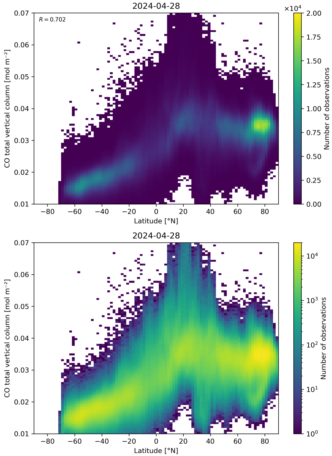
Figure 51: Scatter density plot of “Latitude” against “CO total vertical column” for 2024-04-27 to 2024-04-29.
