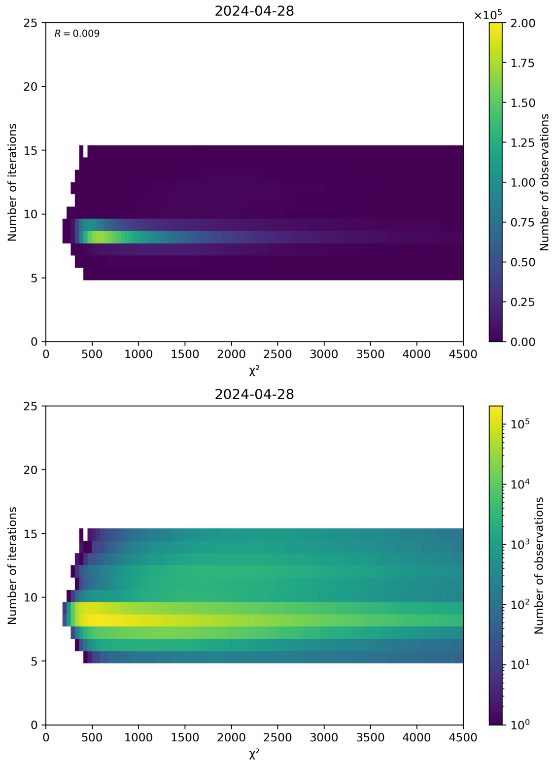
Figure 49: Scatter density plot of “ \chi^2 ” against “Number of iterations” for 2024-04-27 to 2024-04-29.
