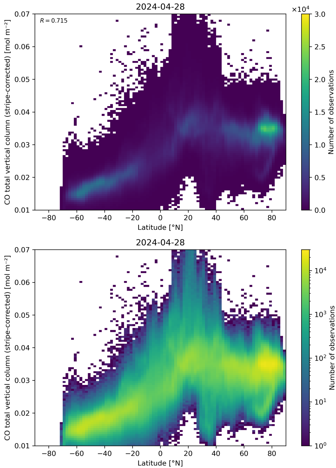
Figure 52: Scatter density plot of “Latitude” against “CO total vertical column (stripe-corrected)” for 2024-04-27 to 2024-04-29.
