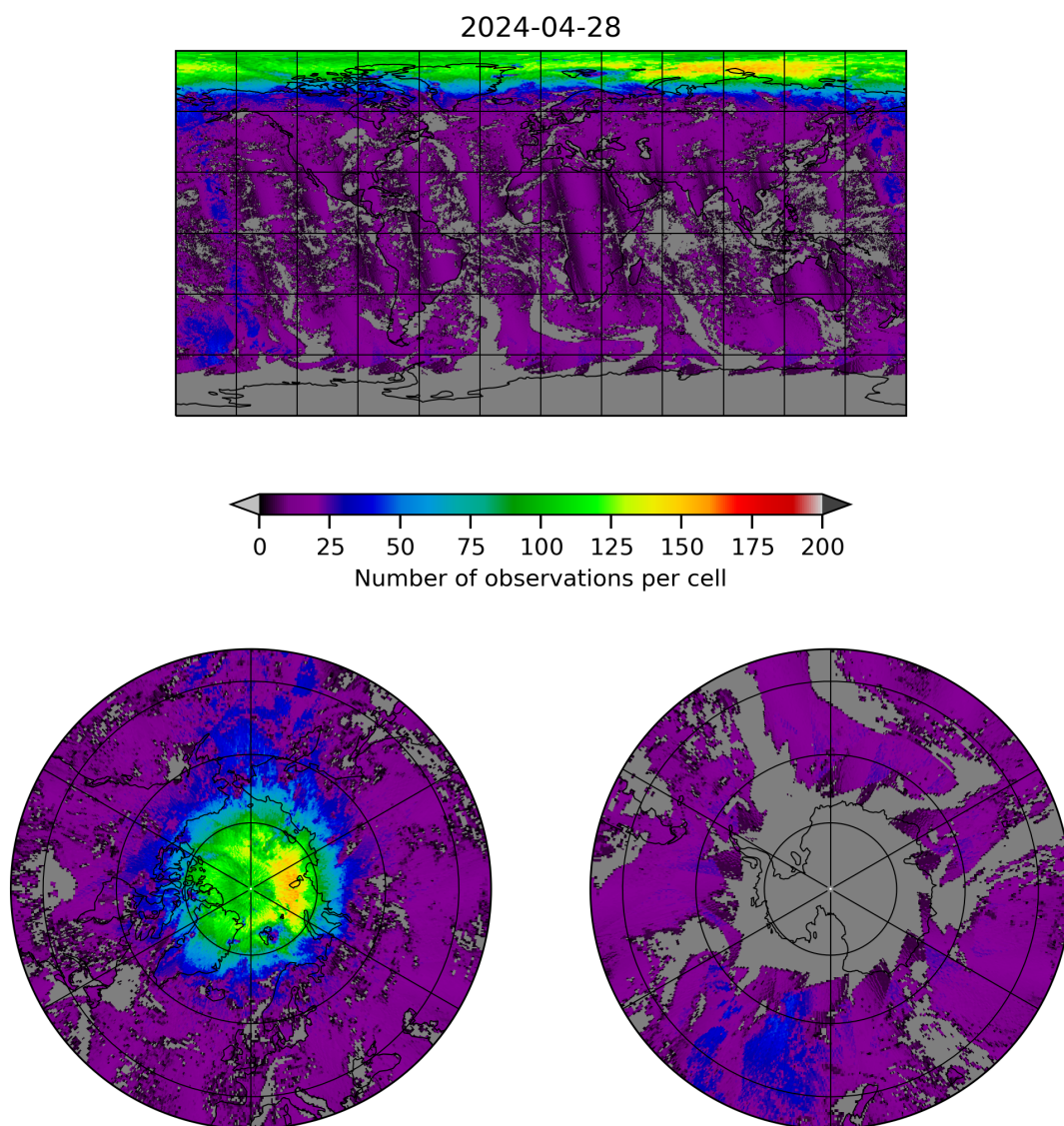
Figure 8: Map of the number of observations for 2024-04-27 to 2024-04-29
