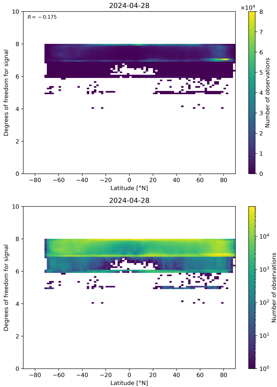
Figure 55: Scatter density plot of “Latitude” against “Degrees of freedom for signal” for 2024-04-27 to 2024-04-29.
