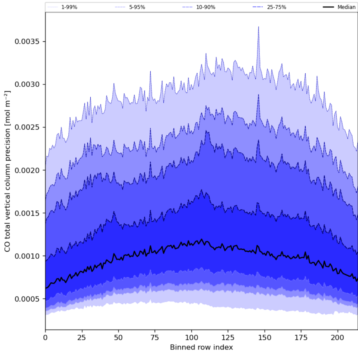
Figure 28: Along track statistics of “CO total vertical column precision” for 2024-04-27 to 2024-04-29
