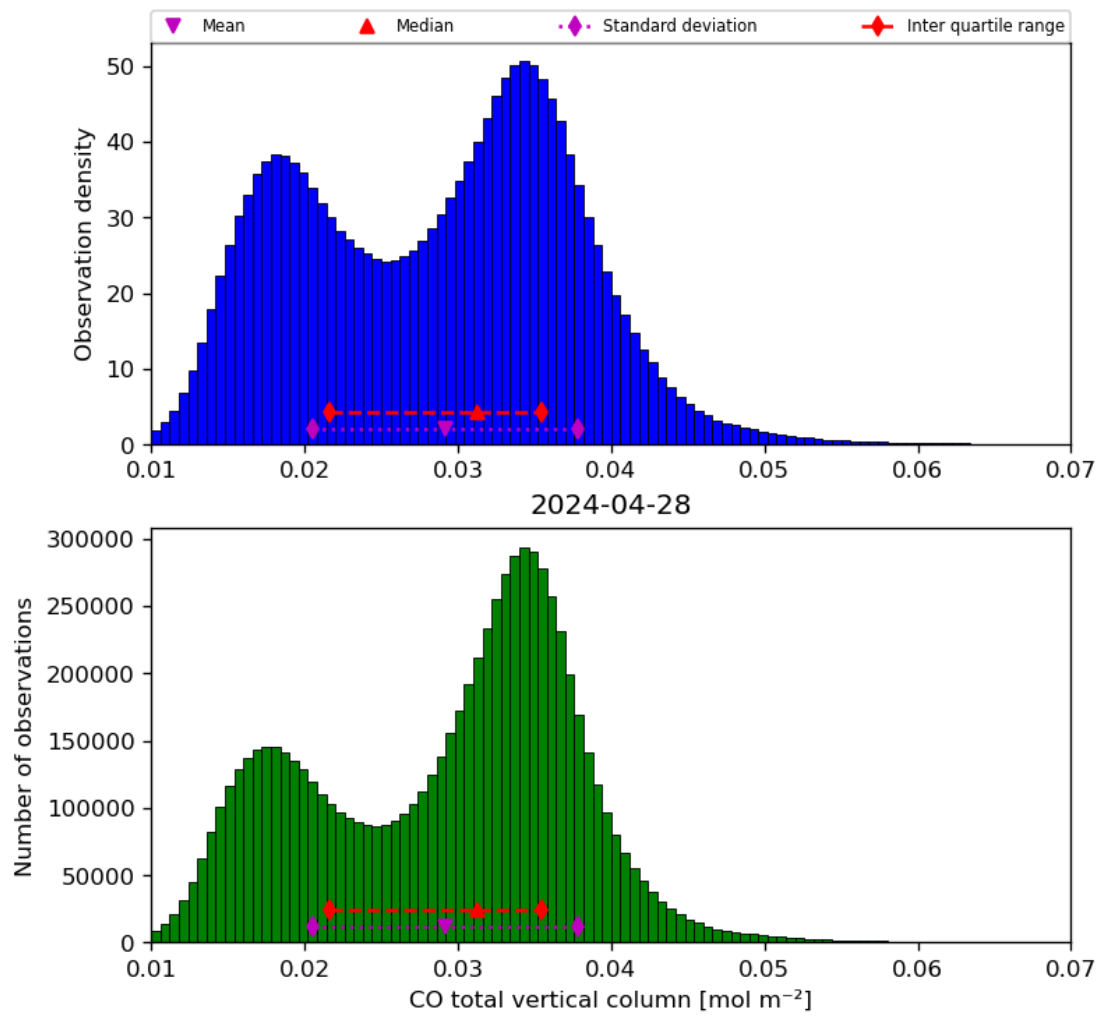
Figure 18: Histogram of “CO total vertical column” for 2024-04-27 to 2024-04-29
