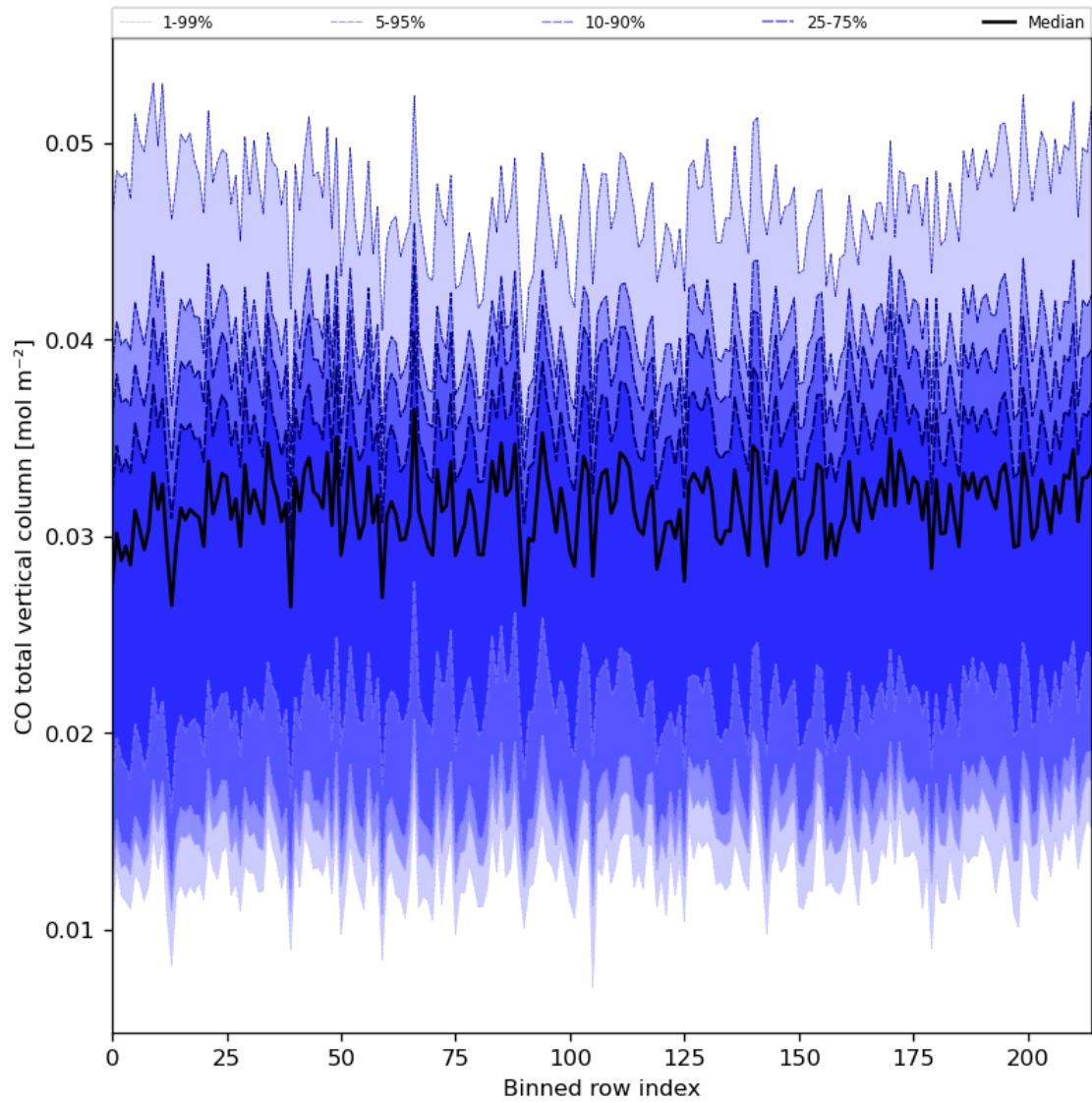
Figure 26: Along track statistics of “CO total vertical column” for 2024-04-27 to 2024-04-29
