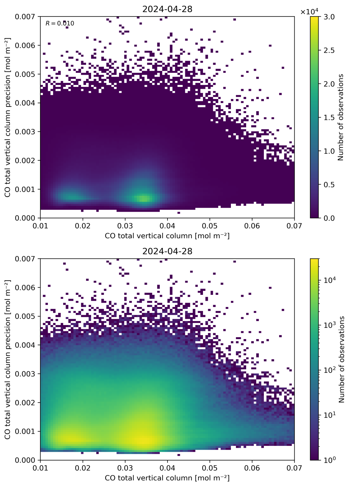
Figure 34: Scatter density plot of “CO total vertical column” against “CO total vertical column precision” for 2024-04-27 to 2024-04-29.
