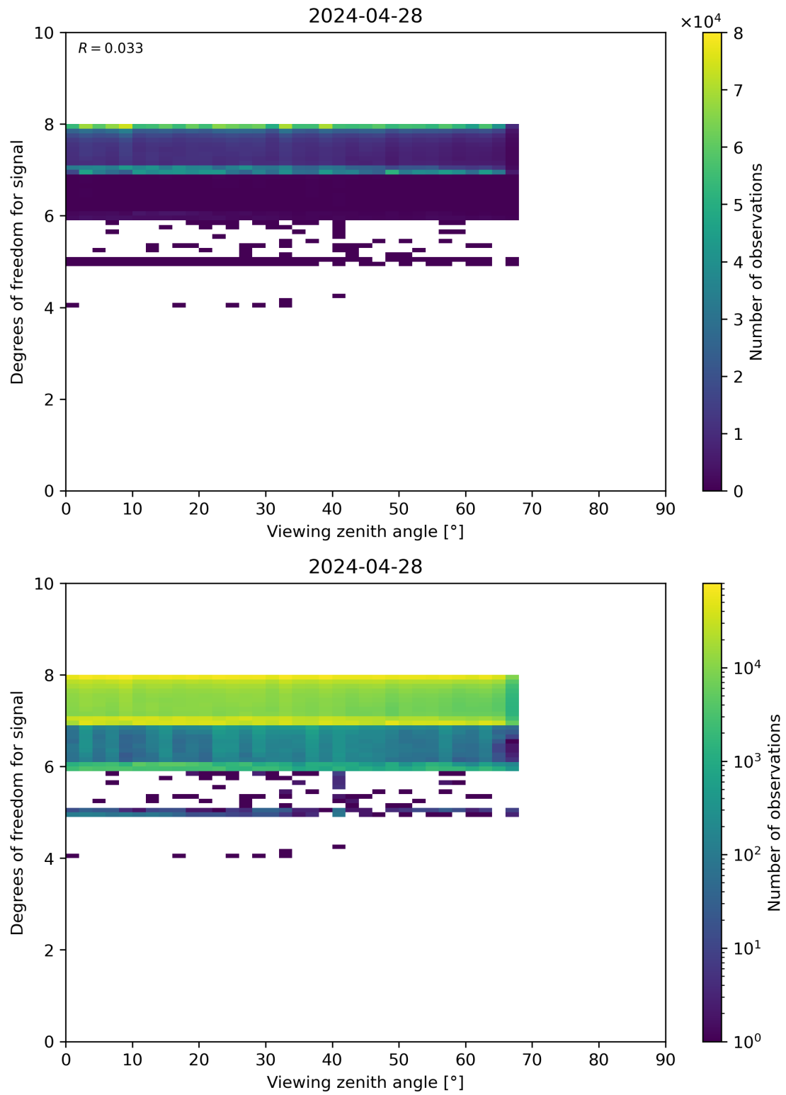
Figure 73: Scatter density plot of “Viewing zenith angle” against “Degrees of freedom for signal” for 2024-04-27 to 2024-04-29.
