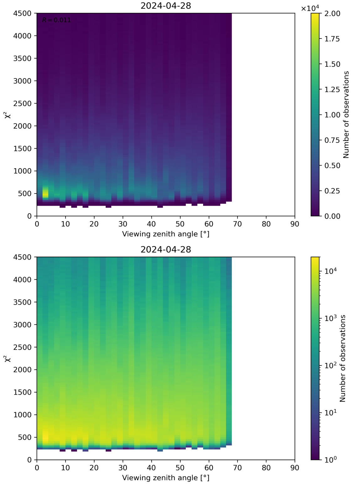
Figure 72: Scatter density plot of “Viewing zenith angle” against “ \chi^2 ” for 2024-04-27 to 2024-04-29.
