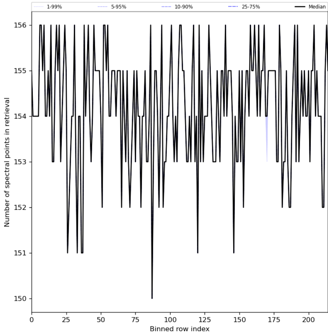
Figure 29: Along track statistics of “Number of spectral points in retrieval” for 2024-04-27 to 2024-04-29
