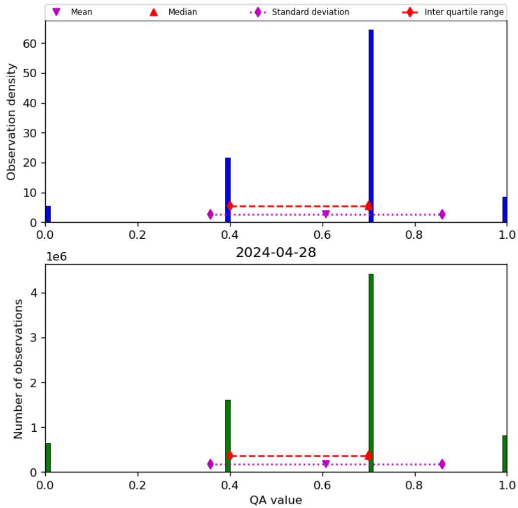
Figure 17: Histogram of “QA value” for 2024-04-27 to 2024-04-29
