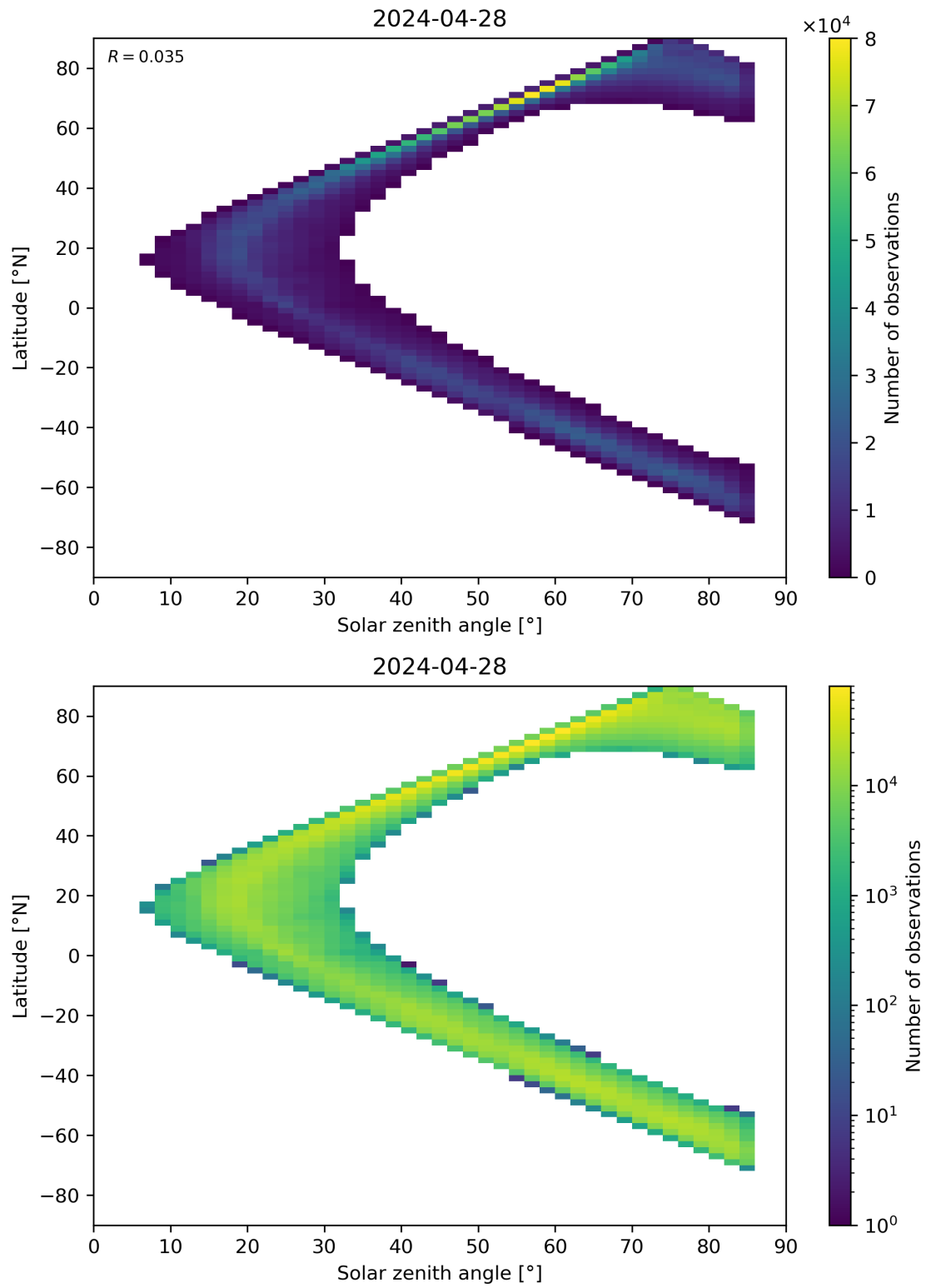
Figure 66: Scatter density plot of “Solar zenith angle” against “Latitude” for 2024-04-27 to 2024-04-29.
