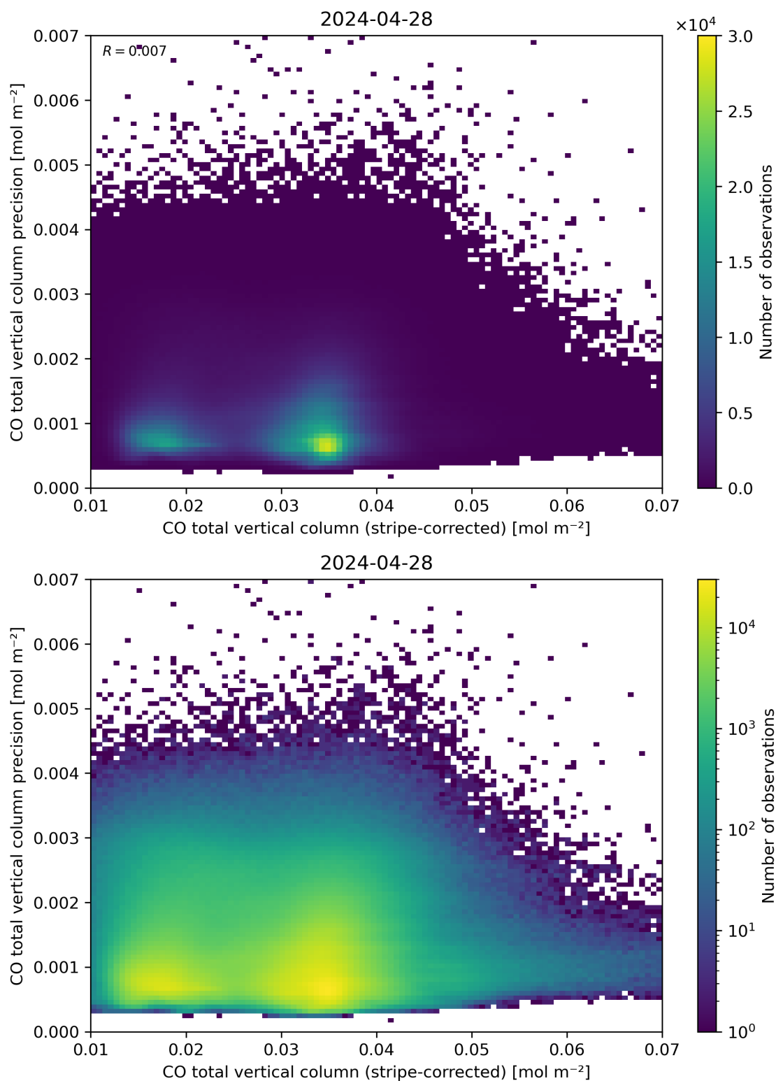
Figure 36: Scatter density plot of “CO total vertical column (stripe-corrected)” against “CO total vertical column precision” for 2024-04-27 to 2024-04-29.
