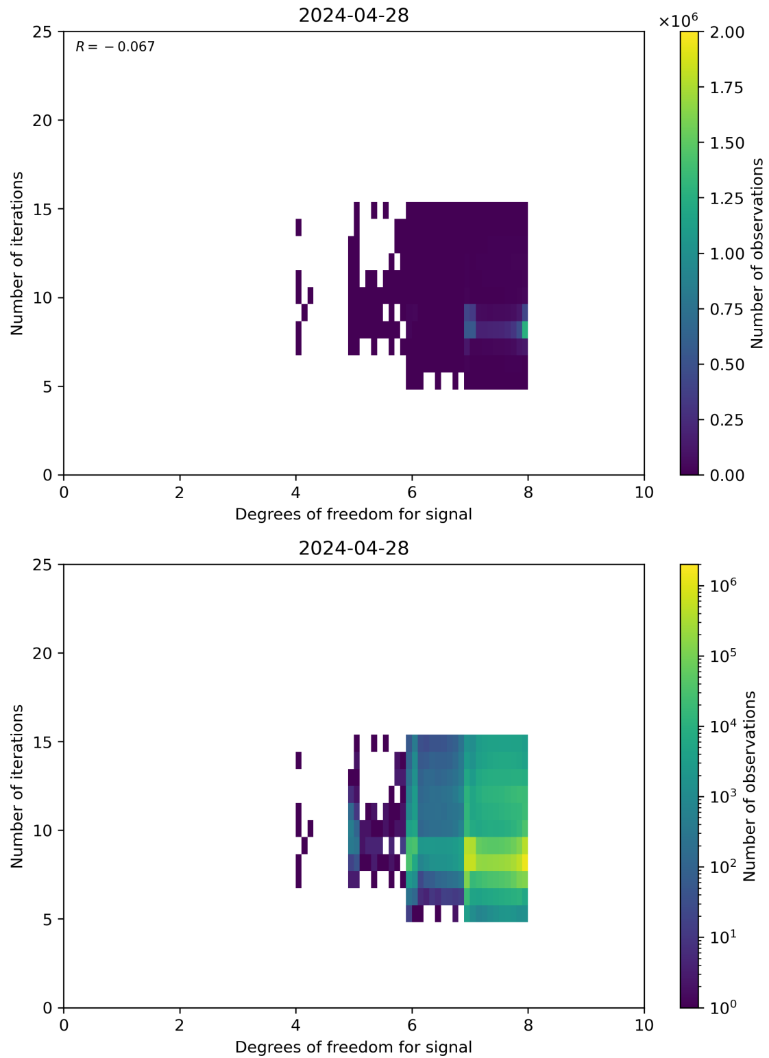
Figure 50: Scatter density plot of “Degrees of freedom for signal” against “Number of iterations” for 2024-04-27 to 2024-04-29.
