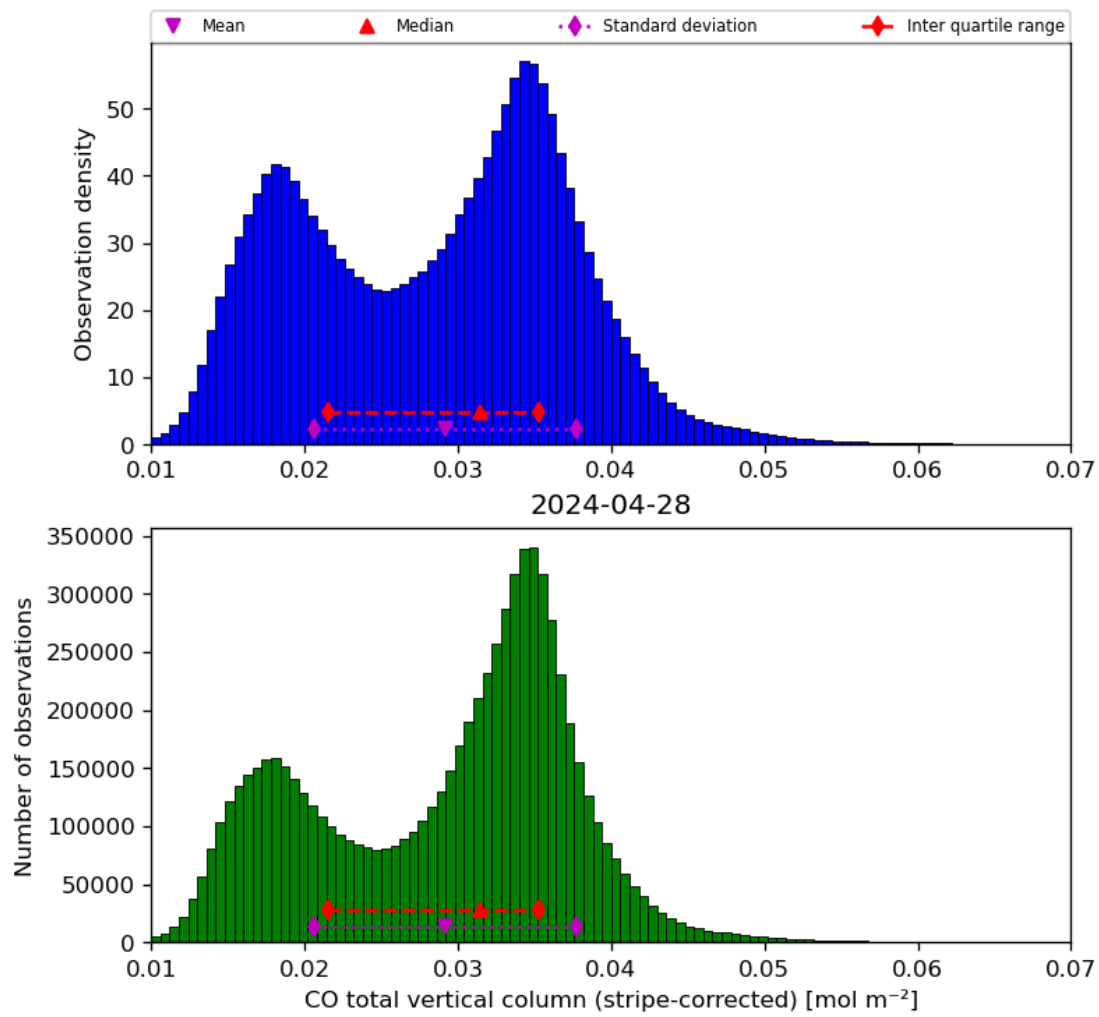
Figure 19: Histogram of “CO total vertical column (stripe-corrected)” for 2024-04-27 to 2024-04-29
