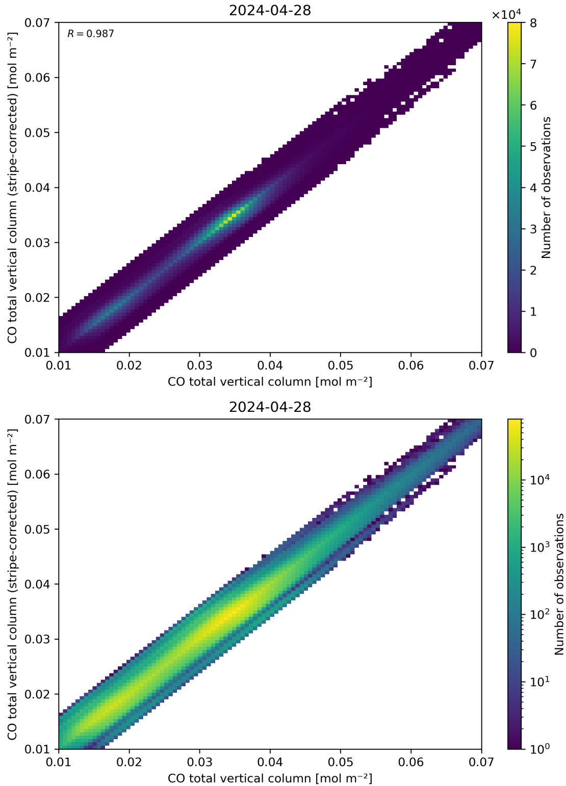
Figure 33: Scatter density plot of “CO total vertical column” against “CO total vertical column (stripe-corrected)” for 2024-04-27 to 2024-04-29.
