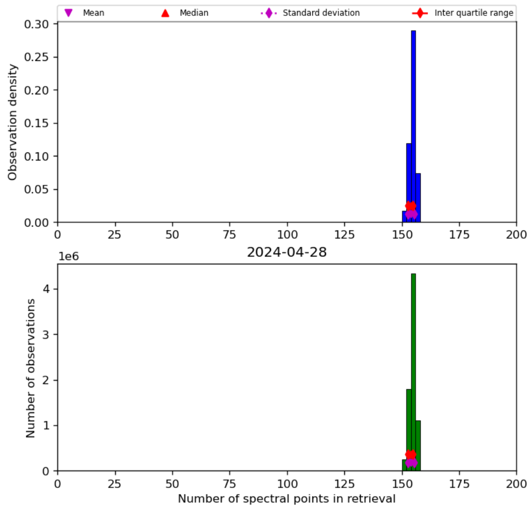
Figure 21: Histogram of “Number of spectral points in retrieval” for 2024-04-27 to 2024-04-29
