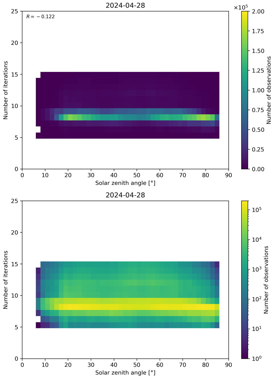
Figure 67: Scatter density plot of “Solar zenith angle” against “Number of iterations” for 2024-04-27 to 2024-04-29.
