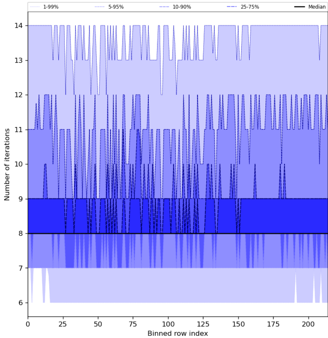
Figure 32: Along track statistics of “Number of iterations” for 2024-04-27 to 2024-04-29
