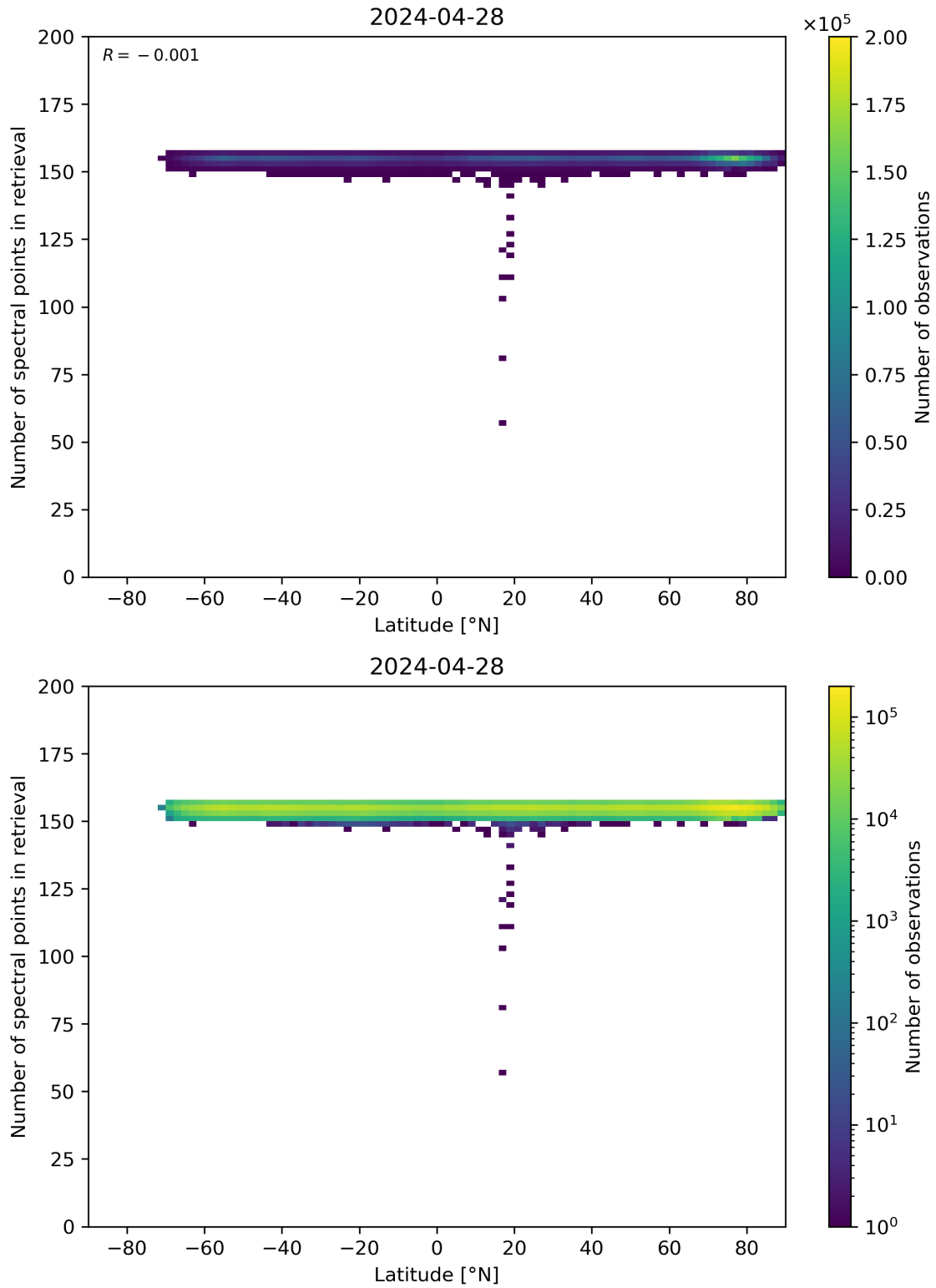
Figure 57: Scatter density plot of “Latitude” against “Number of spectral points in retrieval” for 2024-04-27 to 2024-04-29.
