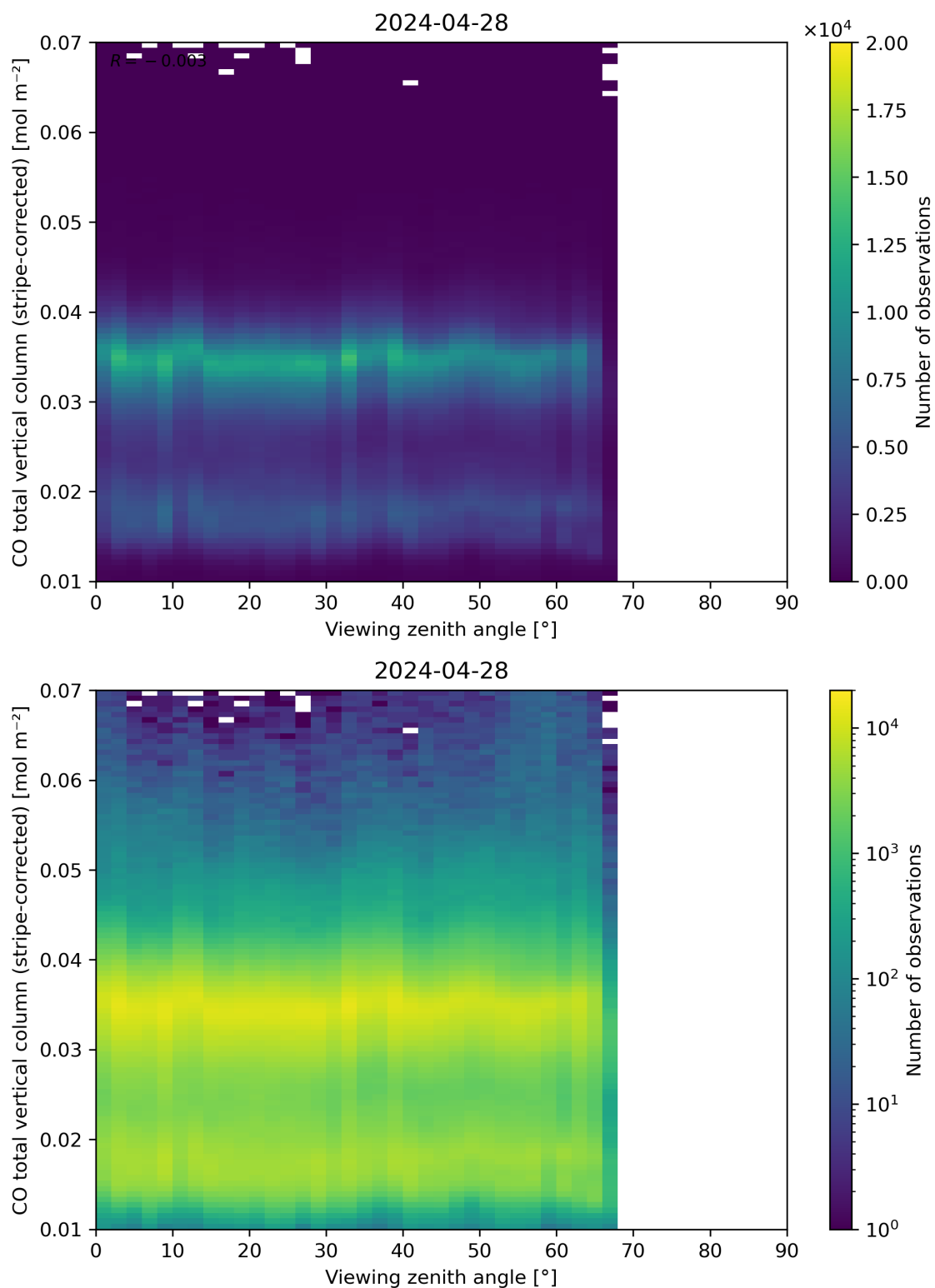
Figure 70: Scatter density plot of “Viewing zenith angle” against “CO total vertical column (stripe-corrected)” for 2024-04-27 to 2024-04-29.
