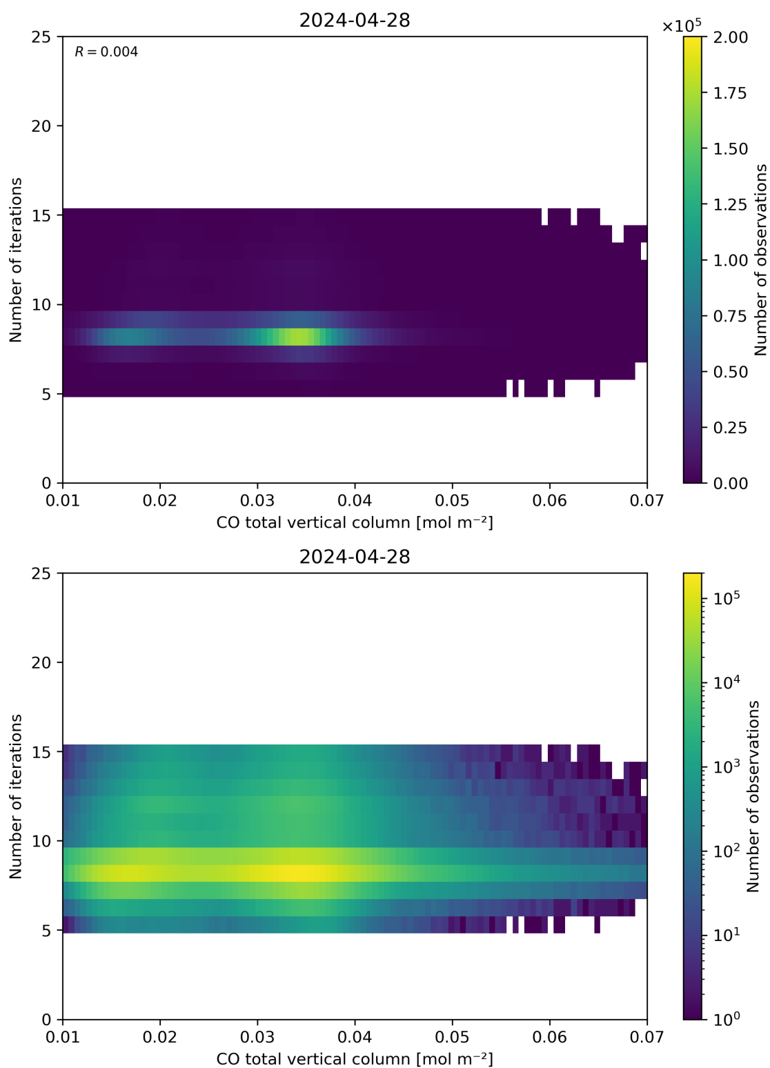
Figure 42: Scatter density plot of “CO total vertical column” against “Number of iterations” for 2024-04-27 to 2024-04-29.
