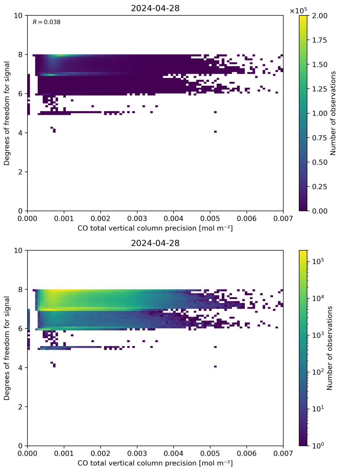
Figure 45: Scatter density plot of “CO total vertical column precision” against “Degrees of freedom for signal” for 2024-04-27 to 2024-04-29.
