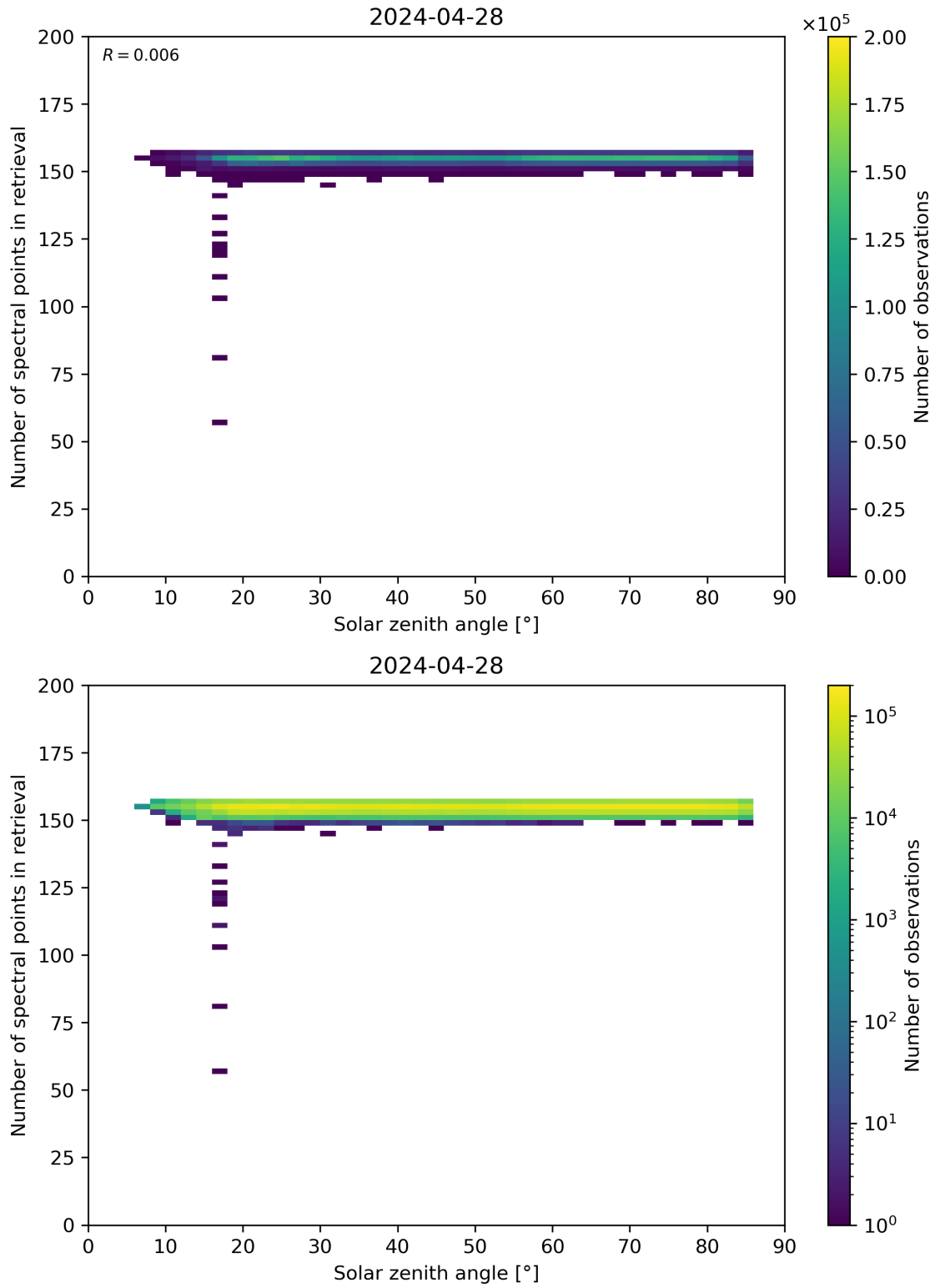
Figure 68: Scatter density plot of “Solar zenith angle” against “Number of spectral points in retrieval” for 2024-04-27 to 2024-04-29.
