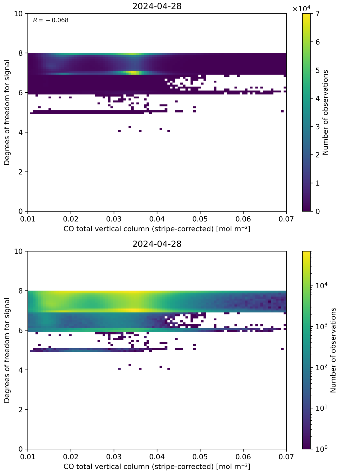
Figure 38: Scatter density plot of “CO total vertical column (stripe-corrected)” against “Degrees of freedom for signal” for 2024-04-27 to 2024-04-29.
