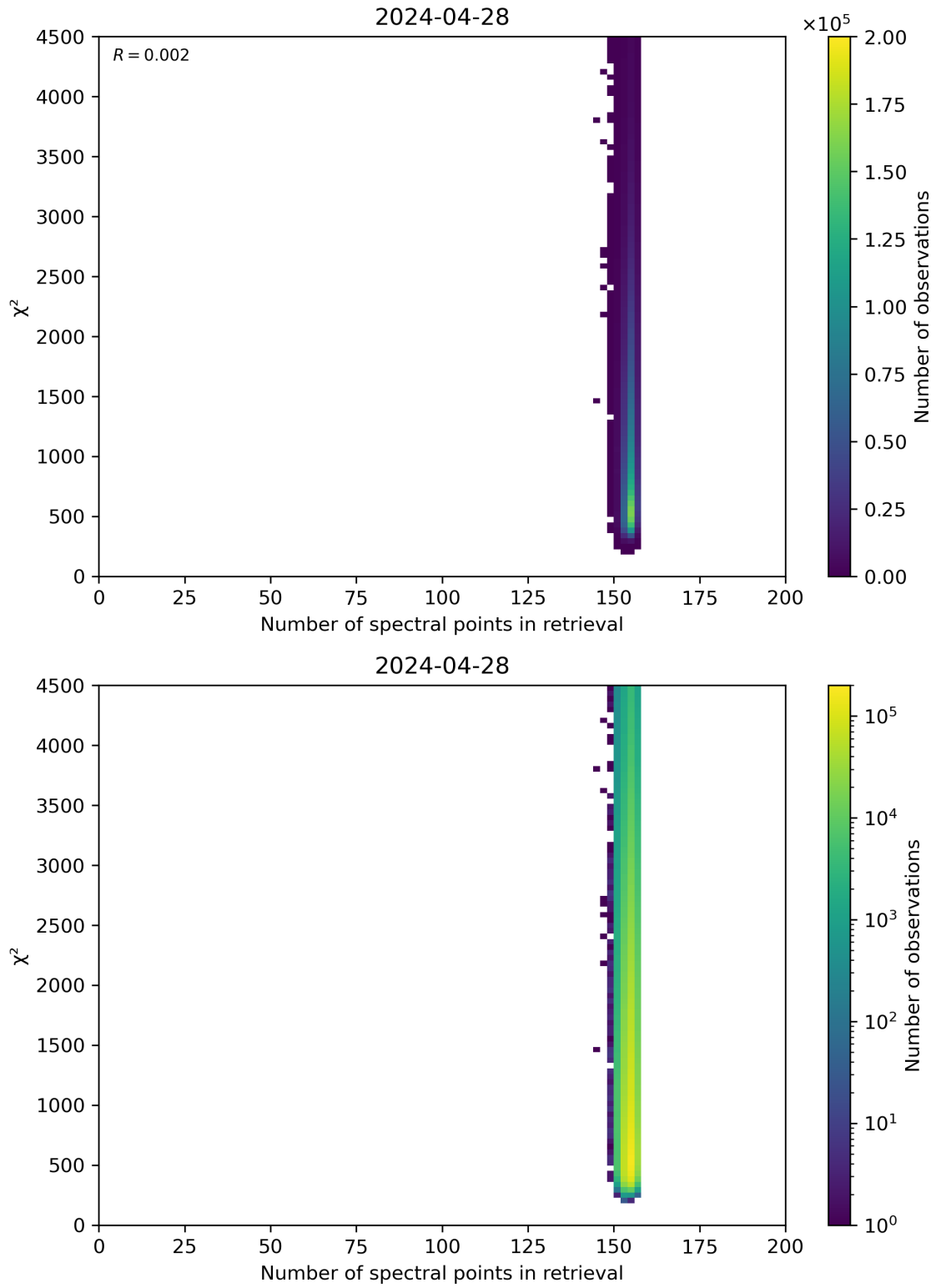
Figure 58: Scatter density plot of “Number of spectral points in retrieval” against “ \chi^2 ” for 2024-04-27 to 2024-04-29.
