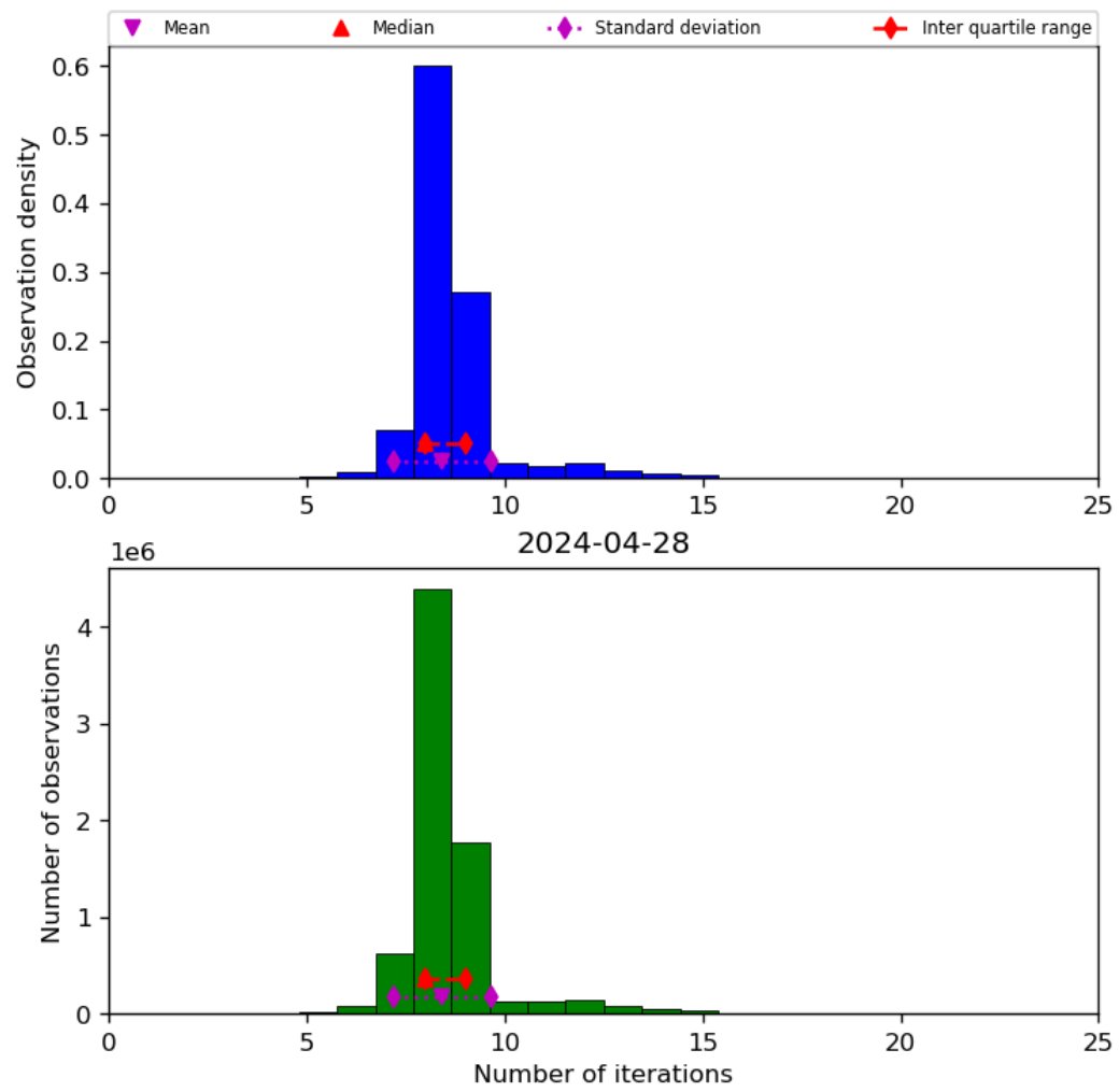
Figure 24: Histogram of “Number of iterations” for 2024-04-27 to 2024-04-29
