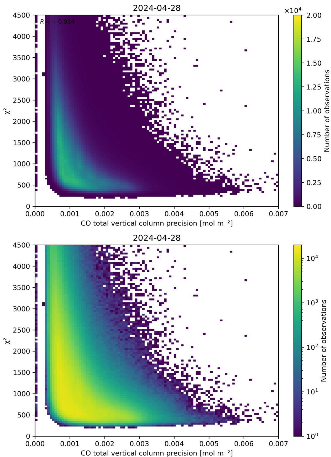
Figure 44: Scatter density plot of “CO total vertical column precision” against “ \chi^2 ” for 2024-04-27 to 2024-04-29.
