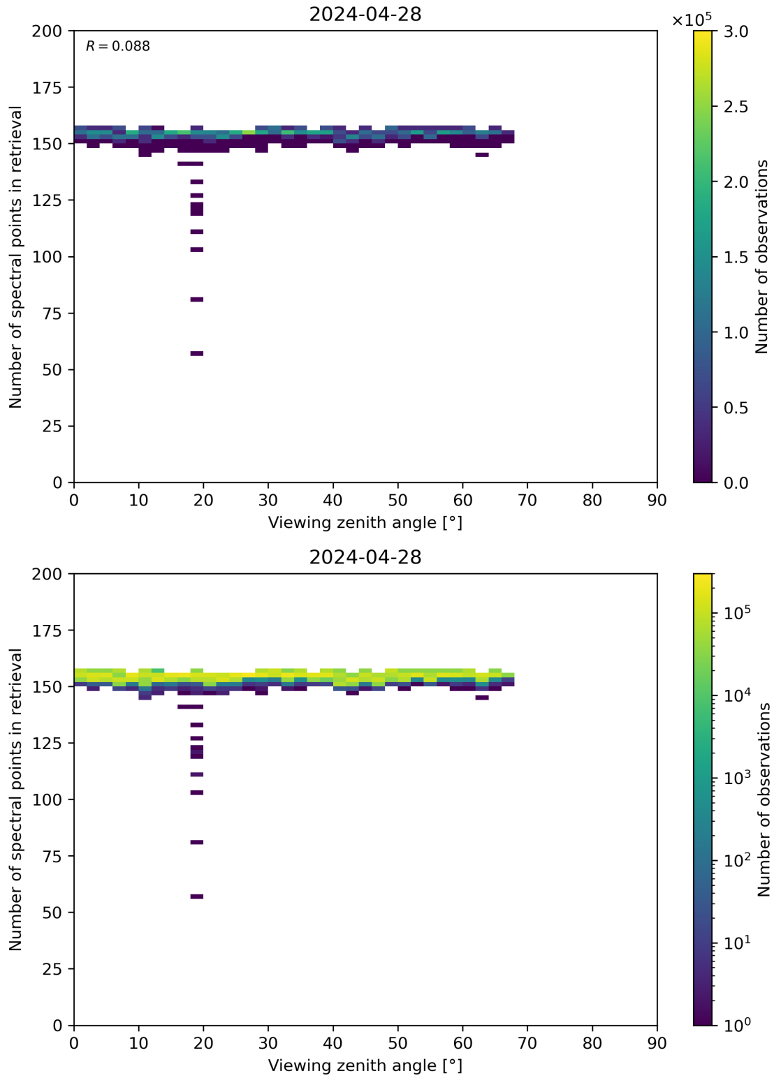
Figure 76: Scatter density plot of “Viewing zenith angle” against “Number of spectral points in retrieval” for 2024-04-27 to 2024-04-29.
