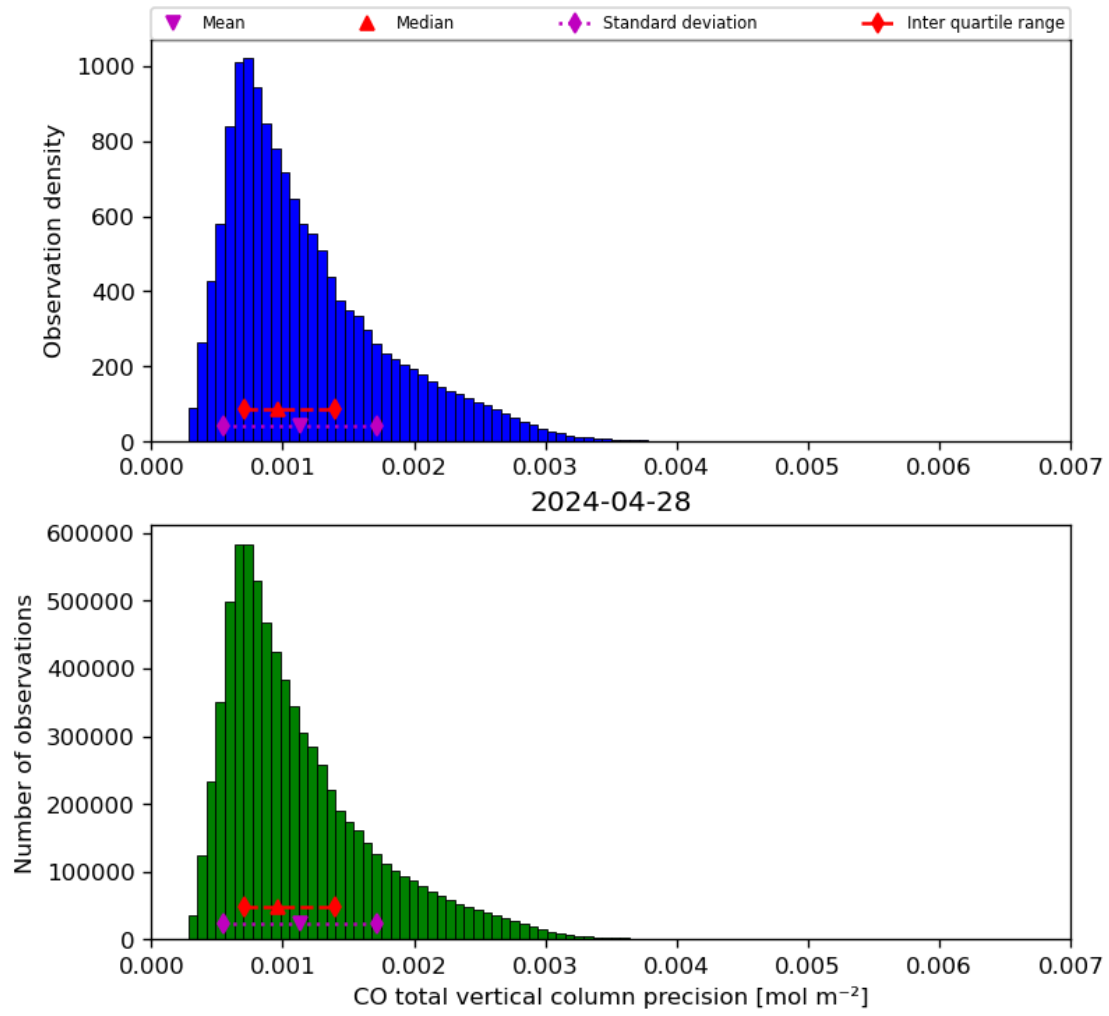
Figure 20: Histogram of “CO total vertical column precision” for 2024-04-27 to 2024-04-29
