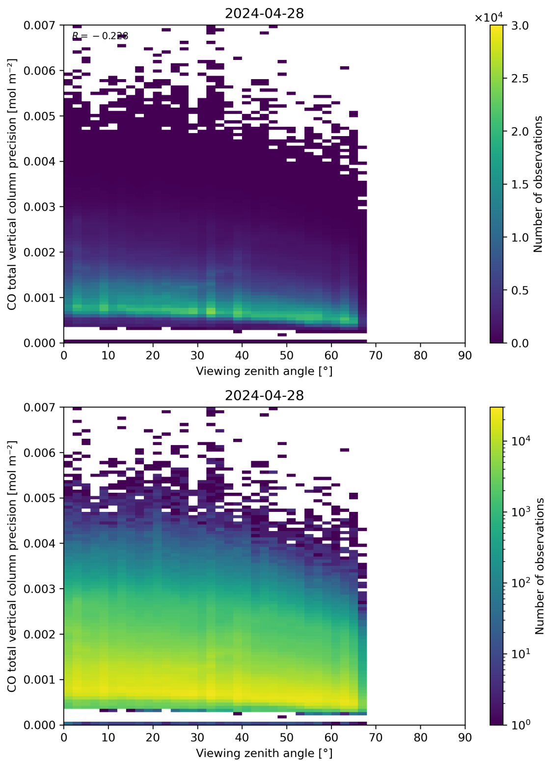
Figure 71: Scatter density plot of “Viewing zenith angle” against “CO total vertical column precision” for 2024-04-27 to 2024-04-29.
