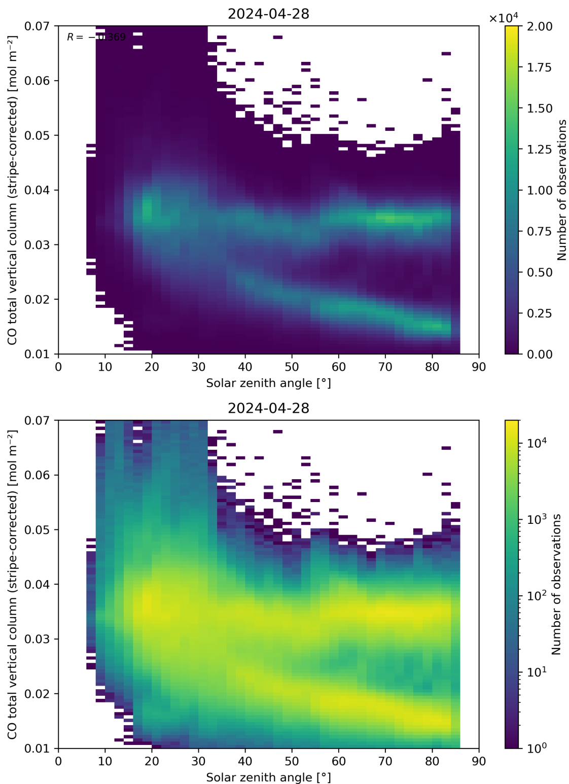
Figure 62: Scatter density plot of “Solar zenith angle” against “CO total vertical column (stripe-corrected)” for 2024-04-27 to 2024-04-29.
