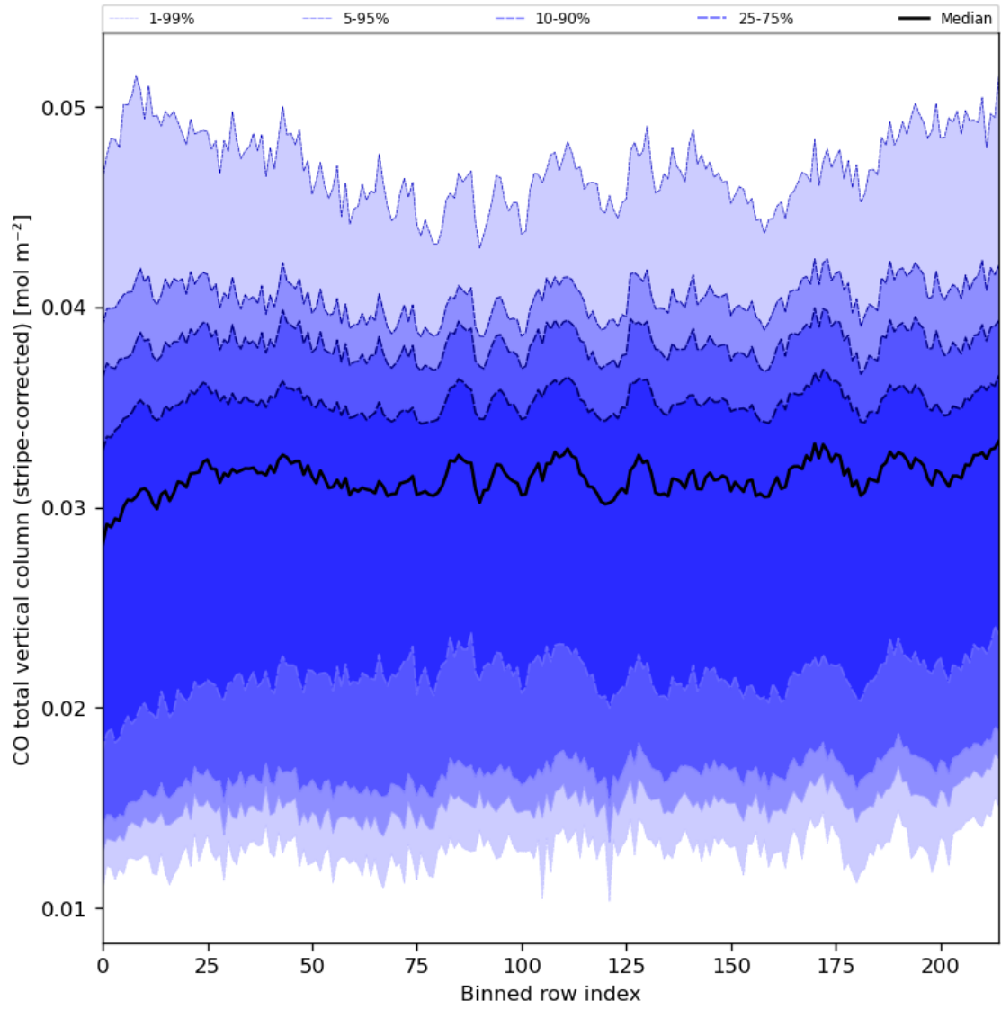
Figure 27: Along track statistics of “CO total vertical column (stripe-corrected)” for 2024-04-27 to 2024-04-29
