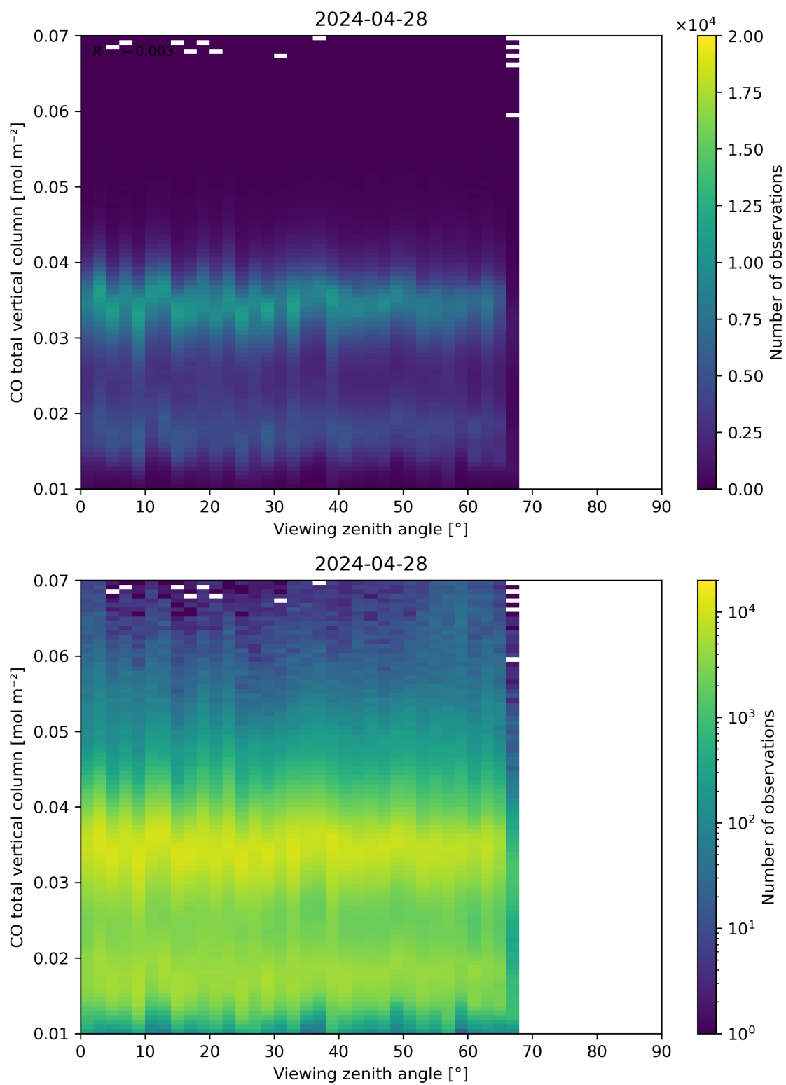
Figure 69: Scatter density plot of “Viewing zenith angle” against “CO total vertical column” for 2024-04-27 to 2024-04-29.
