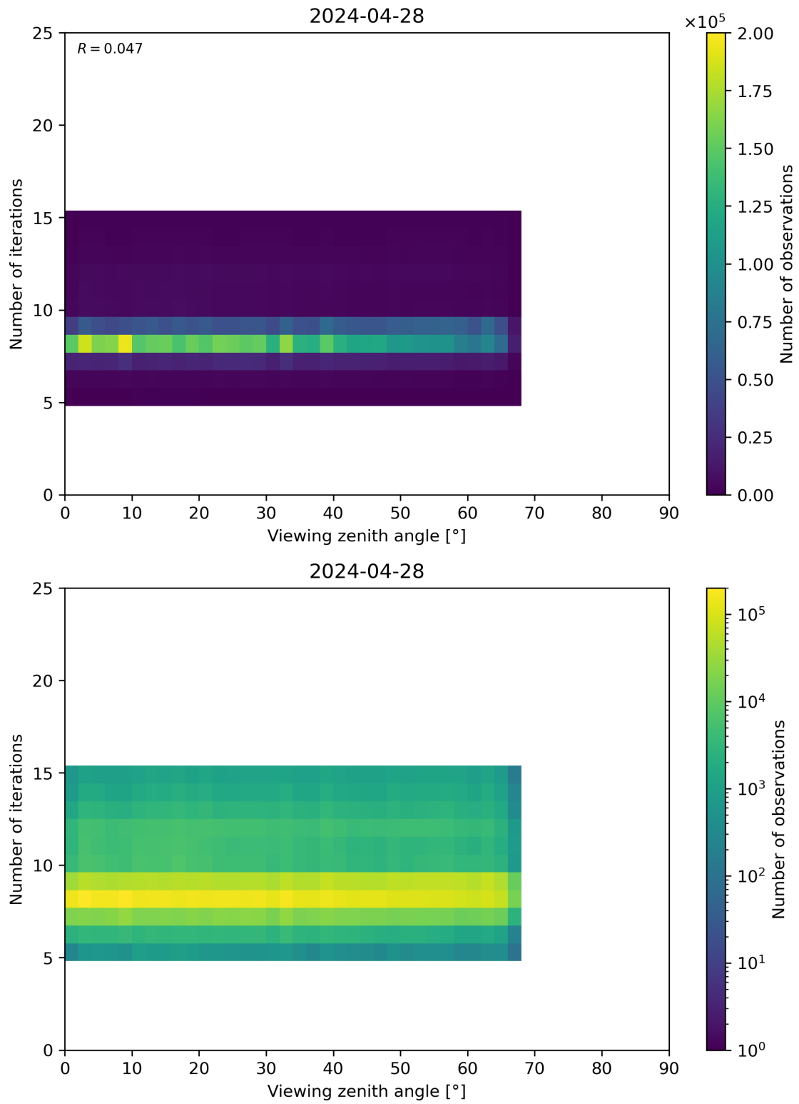
Figure 75: Scatter density plot of “Viewing zenith angle” against “Number of iterations” for 2024-04-27 to 2024-04-29.
