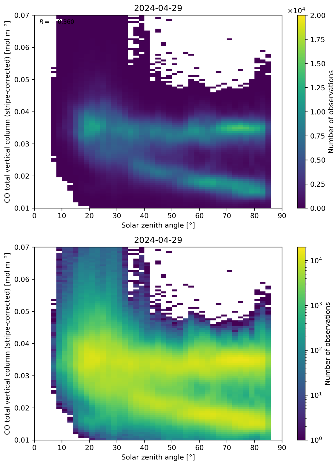
Figure 62: Scatter density plot of “Solar zenith angle” against “CO total vertical column (stripe-corrected)” for 2024-04-28 to 2024-04-30.
