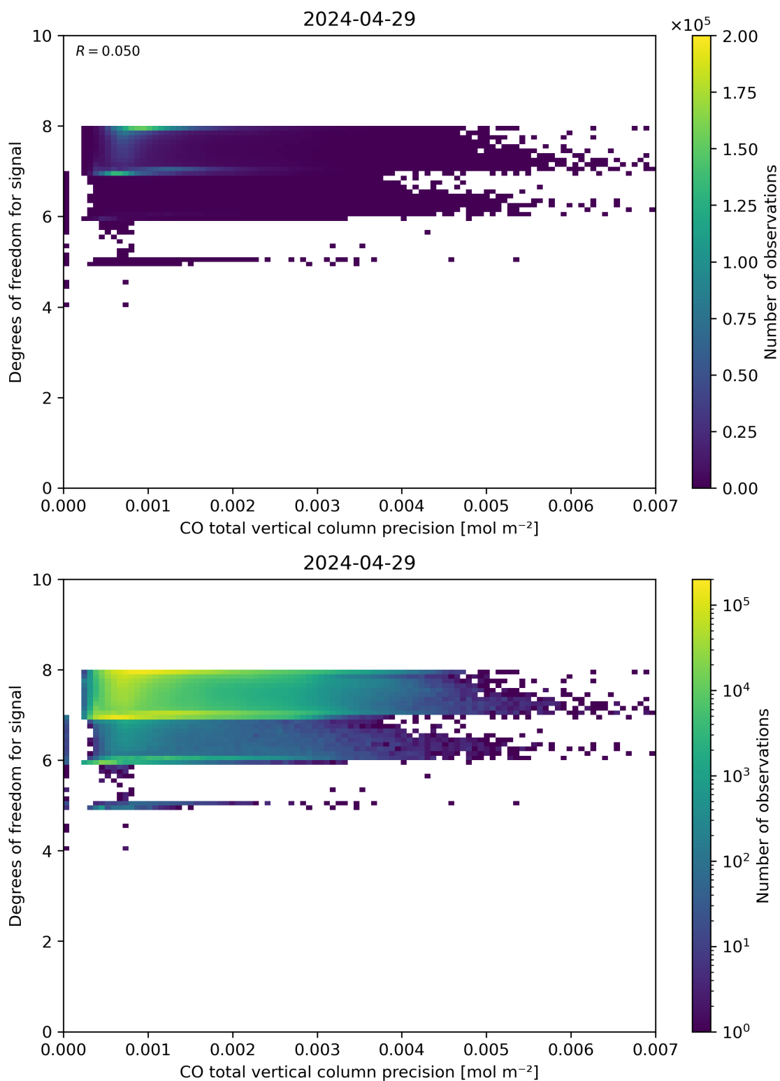
Figure 45: Scatter density plot of “CO total vertical column precision” against “Degrees of freedom for signal” for 2024-04-28 to 2024-04-30.
