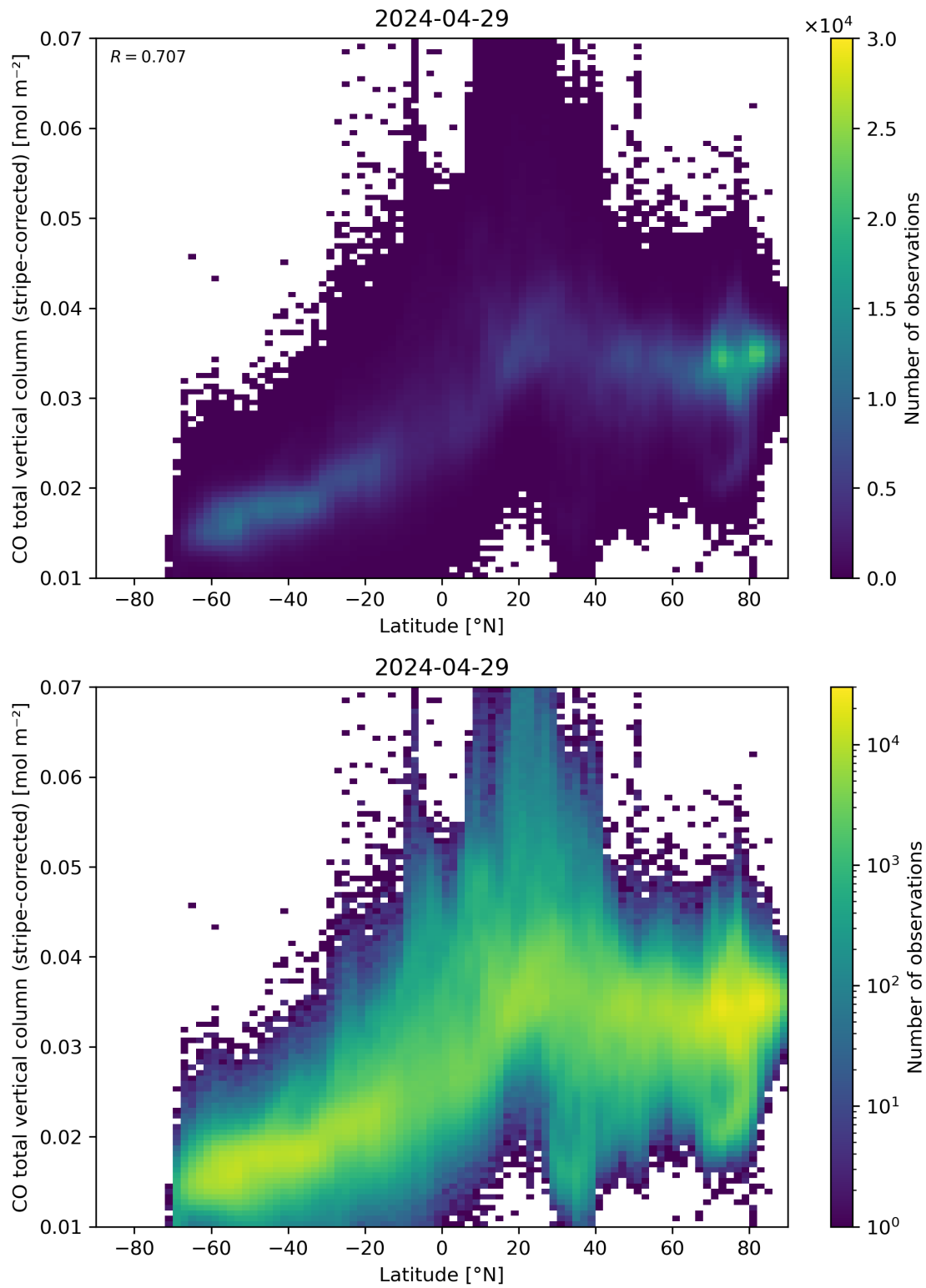
Figure 52: Scatter density plot of “Latitude” against “CO total vertical column (stripe-corrected)” for 2024-04-28 to 2024-04-30.
