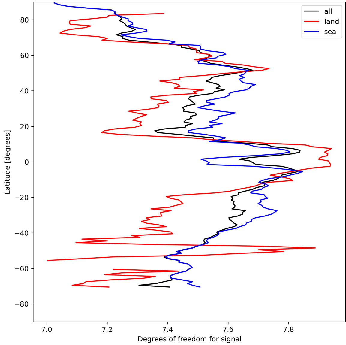
Figure 15: Zonal average of “Degrees of freedom for signal” for 2024-04-28 to 2024-04-30.
