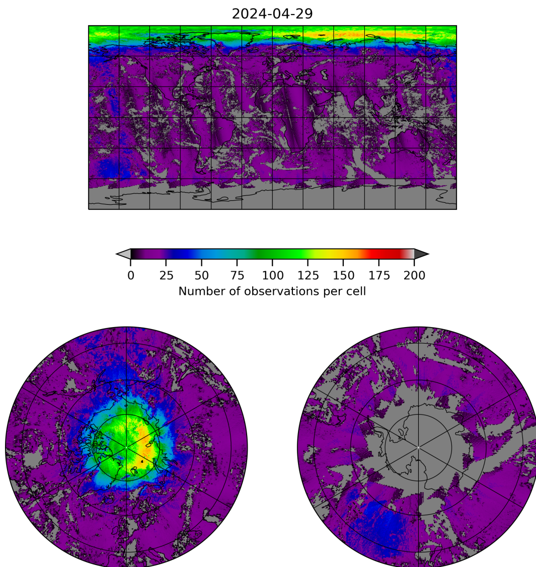
Figure 8: Map of the number of observations for 2024-04-28 to 2024-04-30
