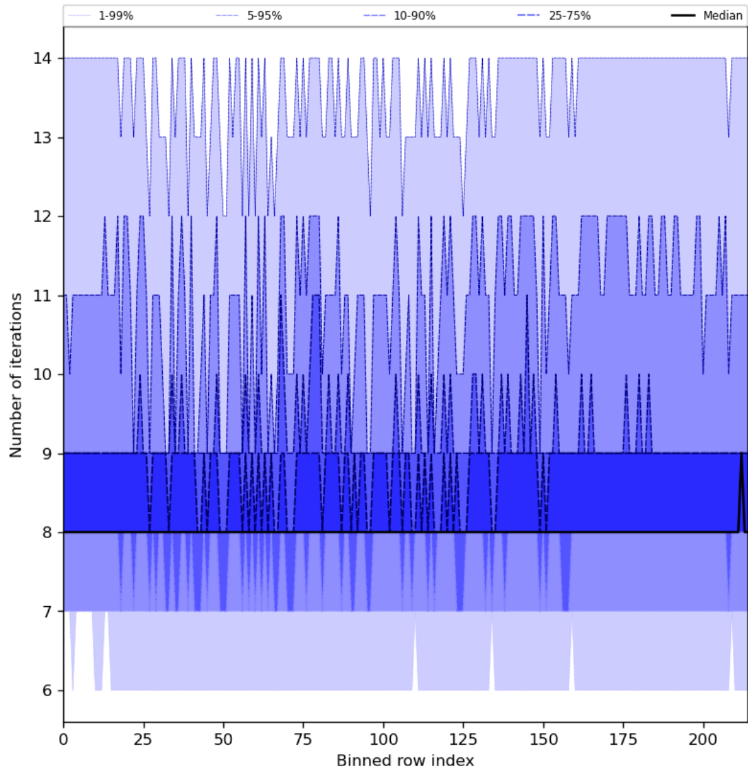
Figure 32: Along track statistics of “Number of iterations” for 2024-04-28 to 2024-04-30
