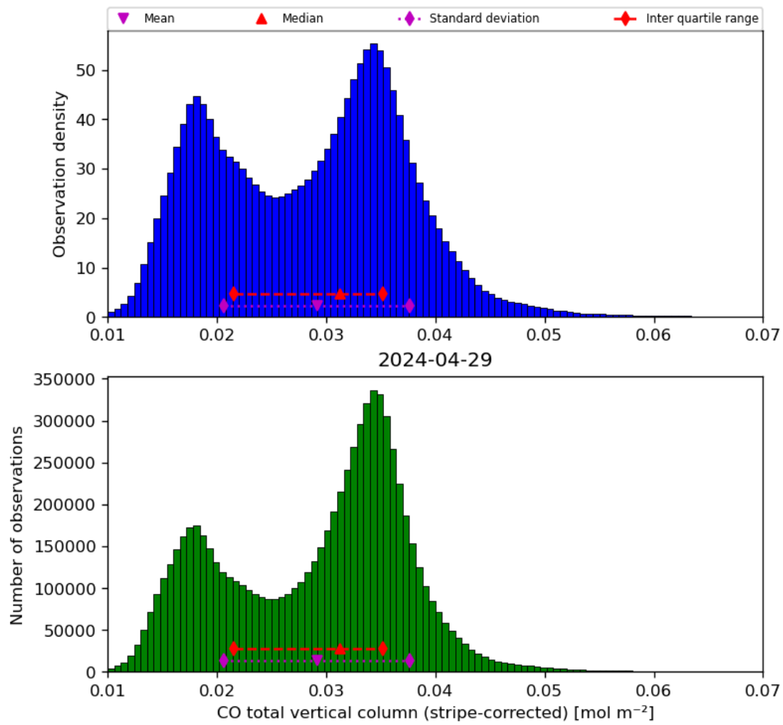
Figure 19: Histogram of “CO total vertical column (stripe-corrected)” for 2024-04-28 to 2024-04-30
