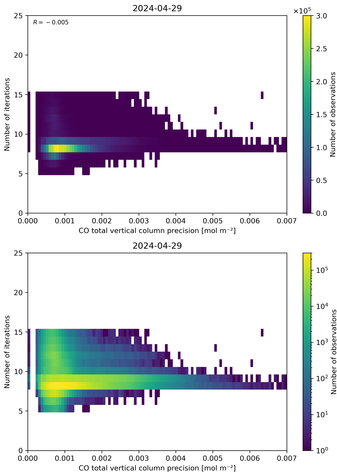
Figure 46: Scatter density plot of “CO total vertical column precision” against “Number of iterations” for 2024-04-28 to 2024-04-30.
