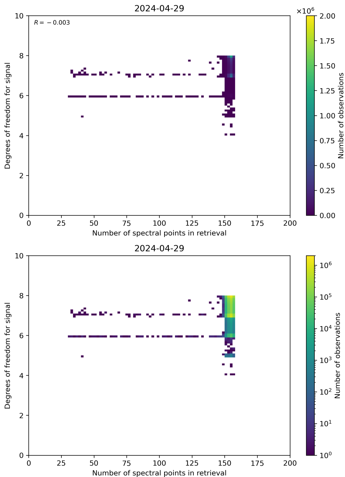
Figure 59: Scatter density plot of “Number of spectral points in retrieval” against “Degrees of freedom for signal” for 2024-04-28 to 2024-04-30.
