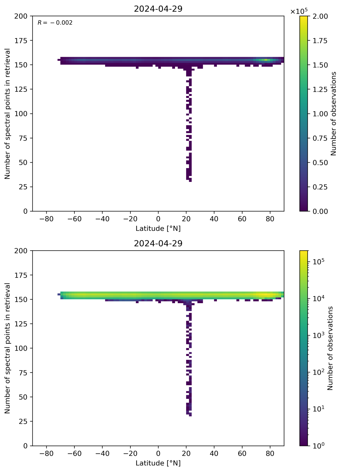
Figure 57: Scatter density plot of “Latitude” against “Number of spectral points in retrieval” for 2024-04-28 to 2024-04-30.
