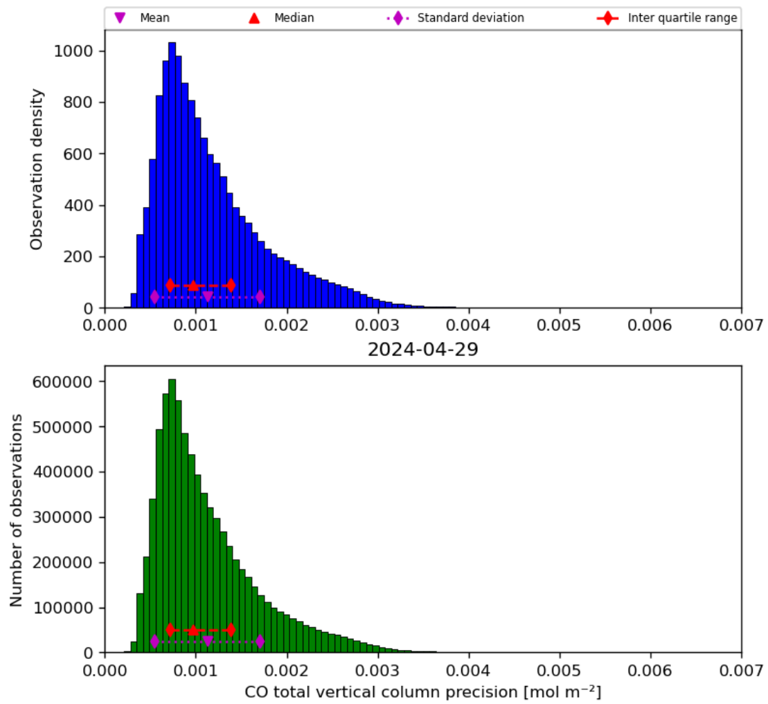
Figure 20: Histogram of “CO total vertical column precision” for 2024-04-28 to 2024-04-30
