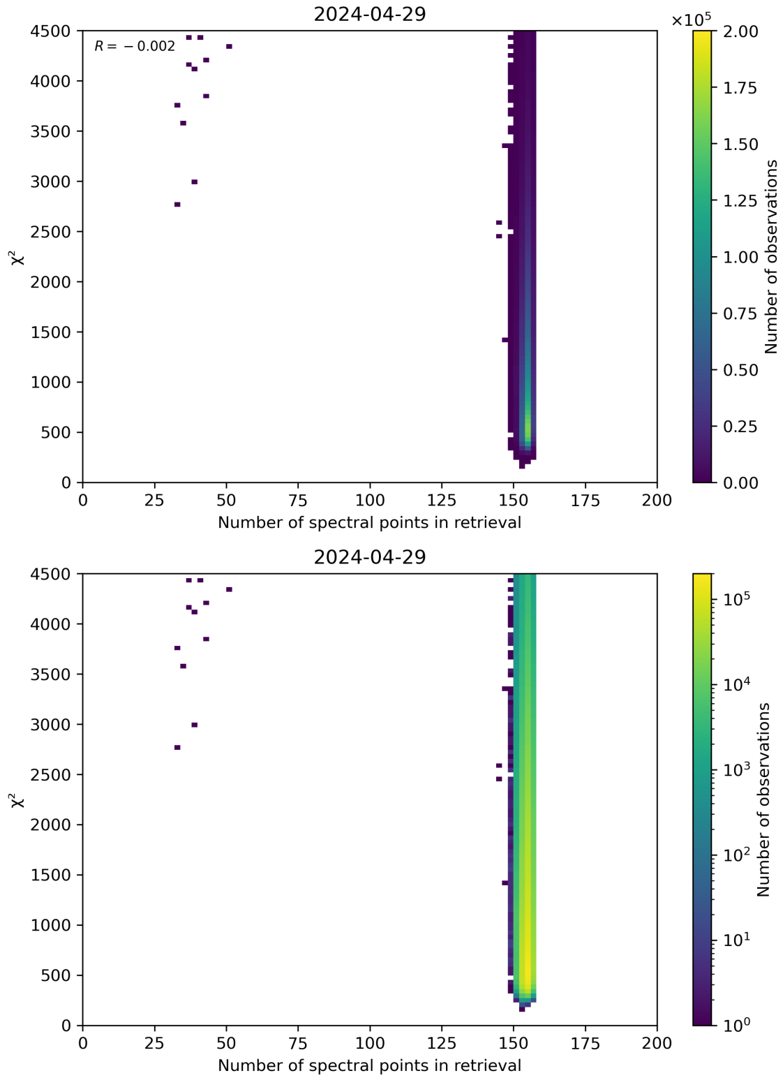
Figure 58: Scatter density plot of “Number of spectral points in retrieval” against “ \chi^2 ” for 2024-04-28 to 2024-04-30.
