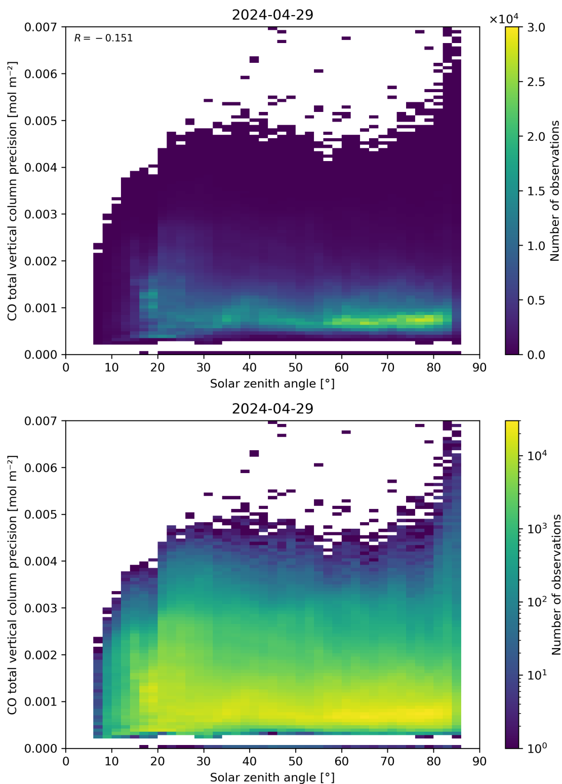
Figure 63: Scatter density plot of “Solar zenith angle” against “CO total vertical column precision” for 2024-04-28 to 2024-04-30.
