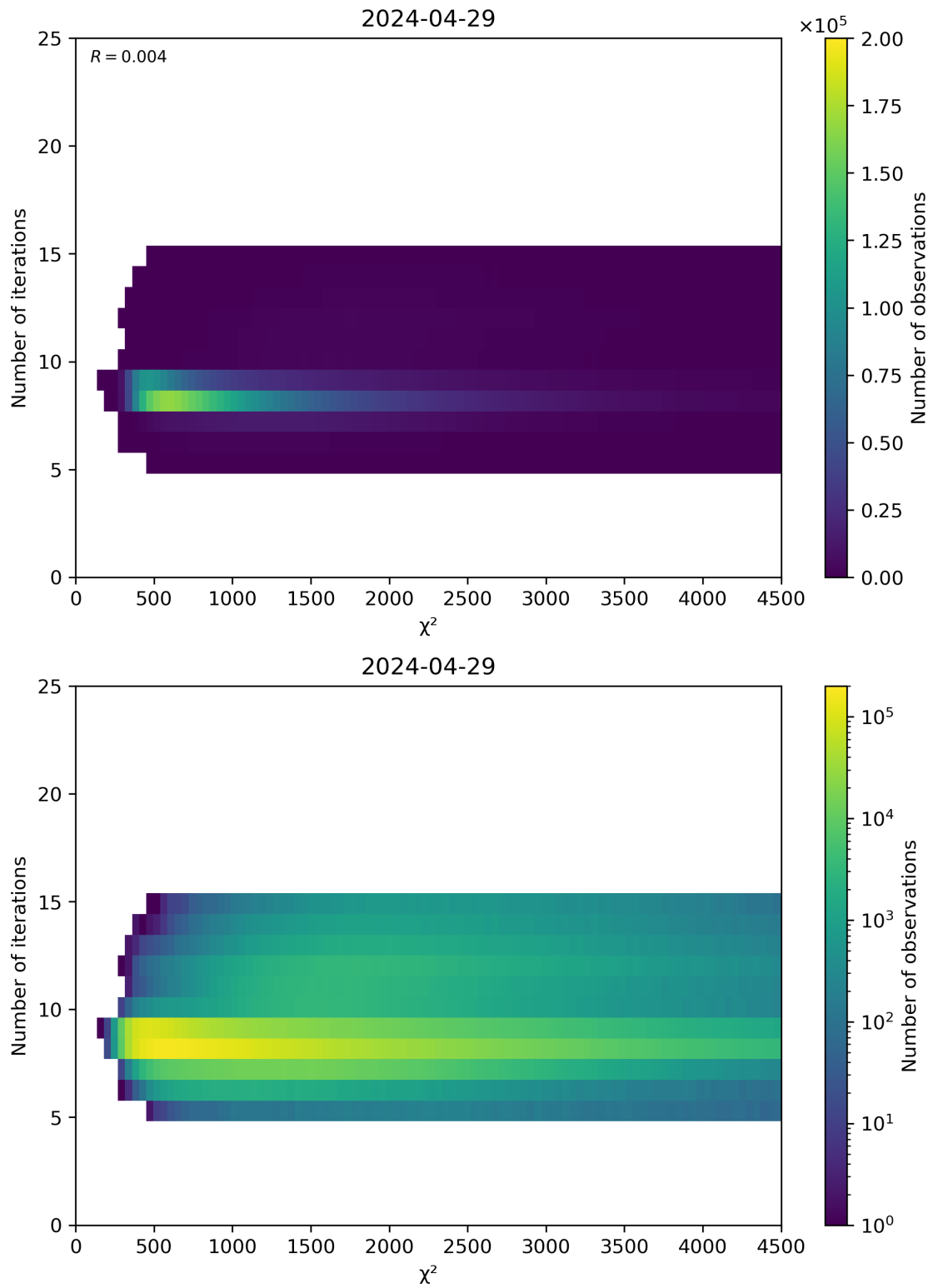
Figure 49: Scatter density plot of “ \chi^2 ” against “Number of iterations” for 2024-04-28 to 2024-04-30.
