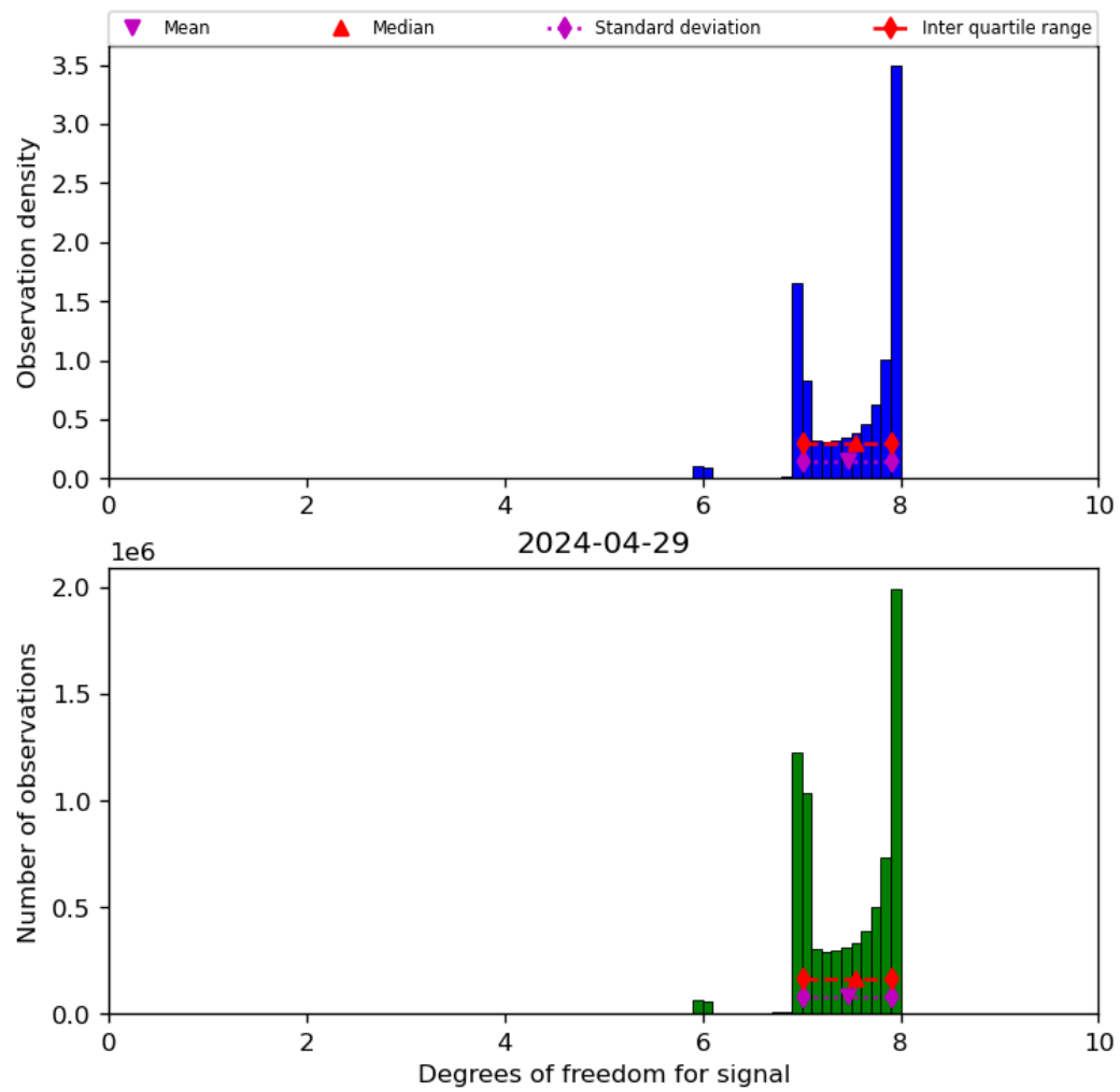
Figure 23: Histogram of “Degrees of freedom for signal” for 2024-04-28 to 2024-04-30
