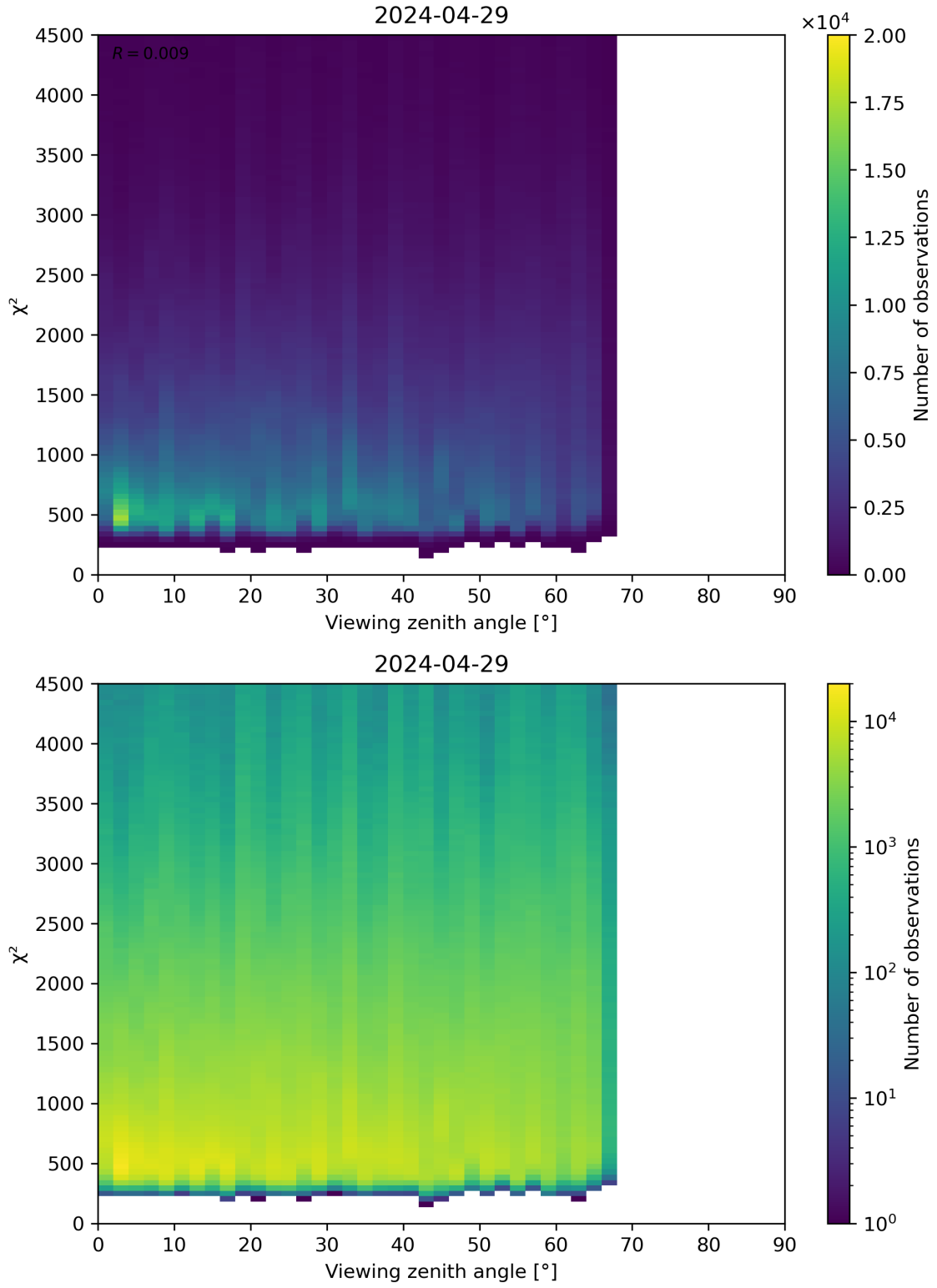
Figure 72: Scatter density plot of “Viewing zenith angle” against “ \chi^2 ” for 2024-04-28 to 2024-04-30.
