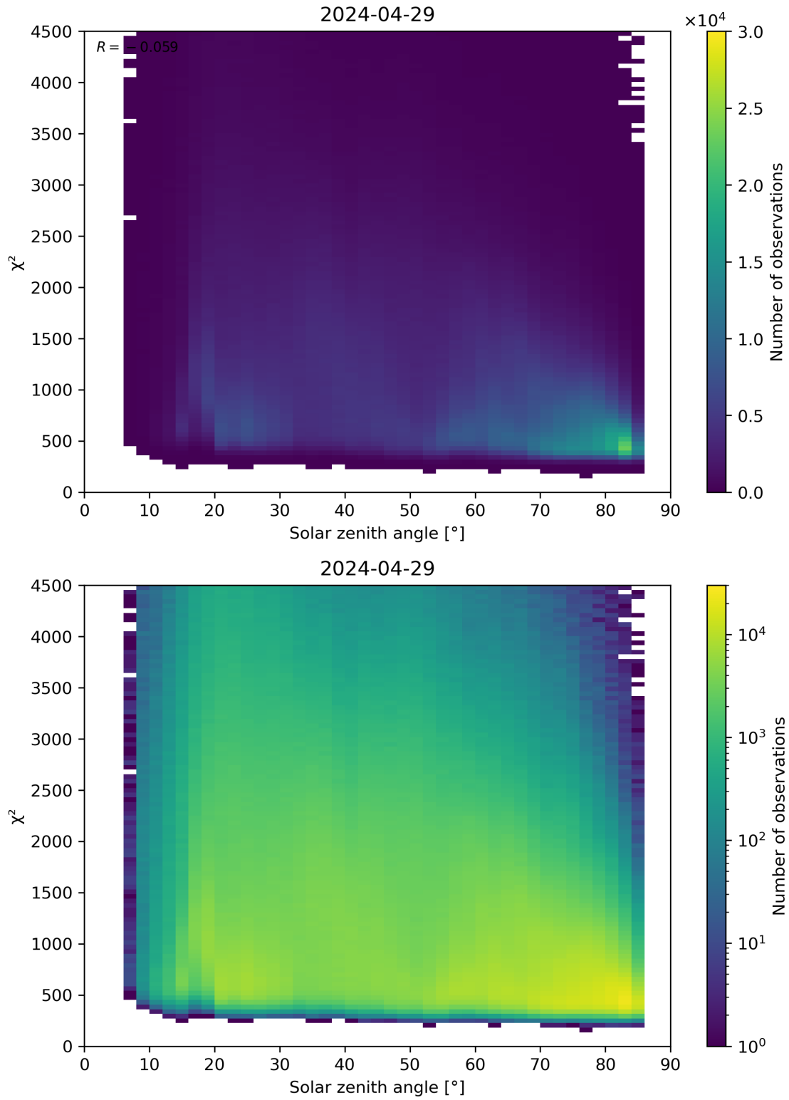
Figure 64: Scatter density plot of “Solar zenith angle” against “ \chi^2 ” for 2024-04-28 to 2024-04-30.
