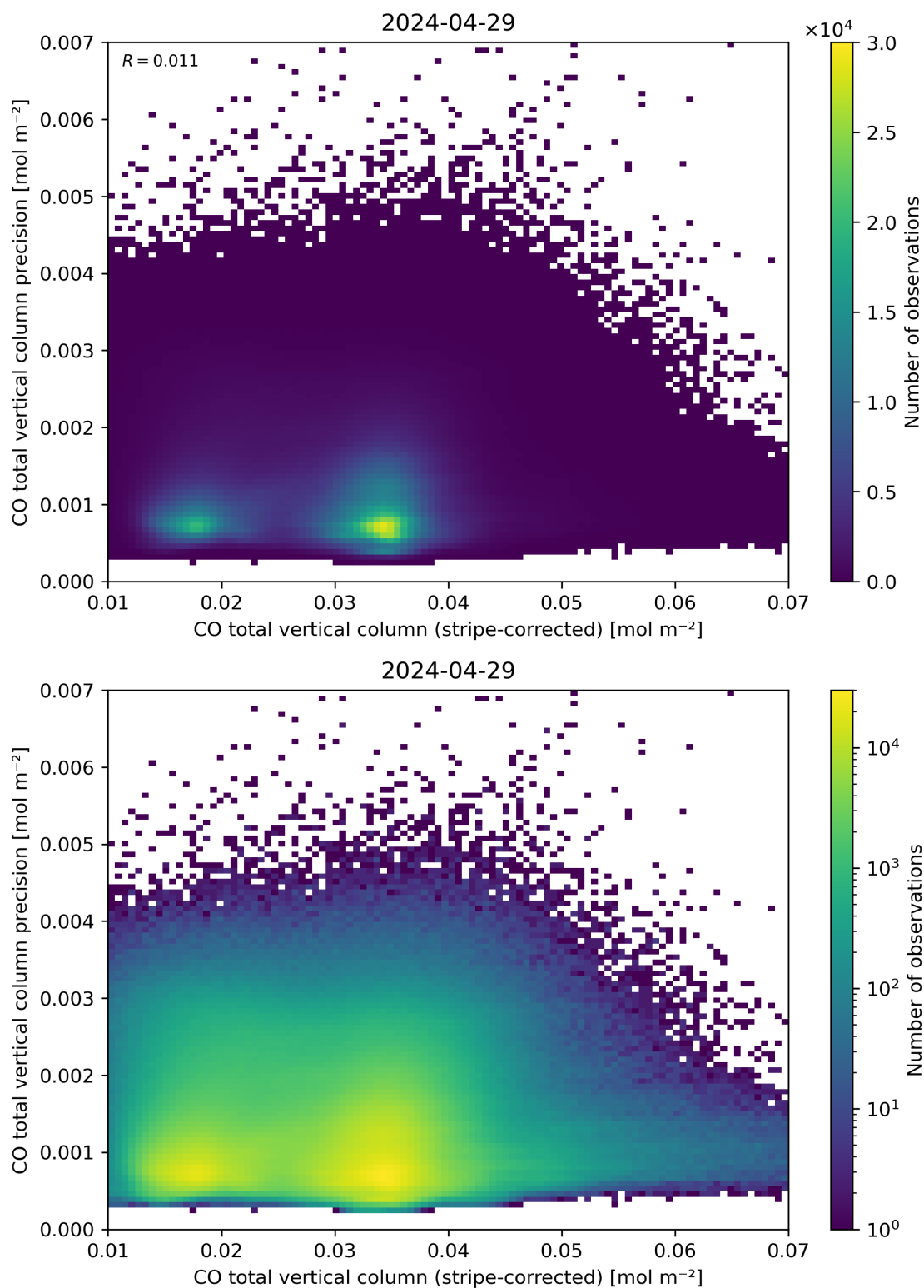
Figure 36: Scatter density plot of “CO total vertical column (stripe-corrected)” against “CO total vertical column precision” for 2024-04-28 to 2024-04-30.
