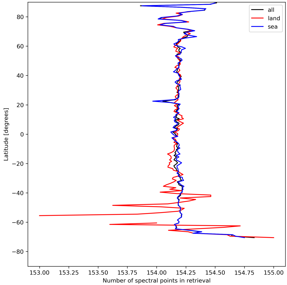
Figure 13: Zonal average of “Number of spectral points in retrieval” for 2024-04-28 to 2024-04-30.
