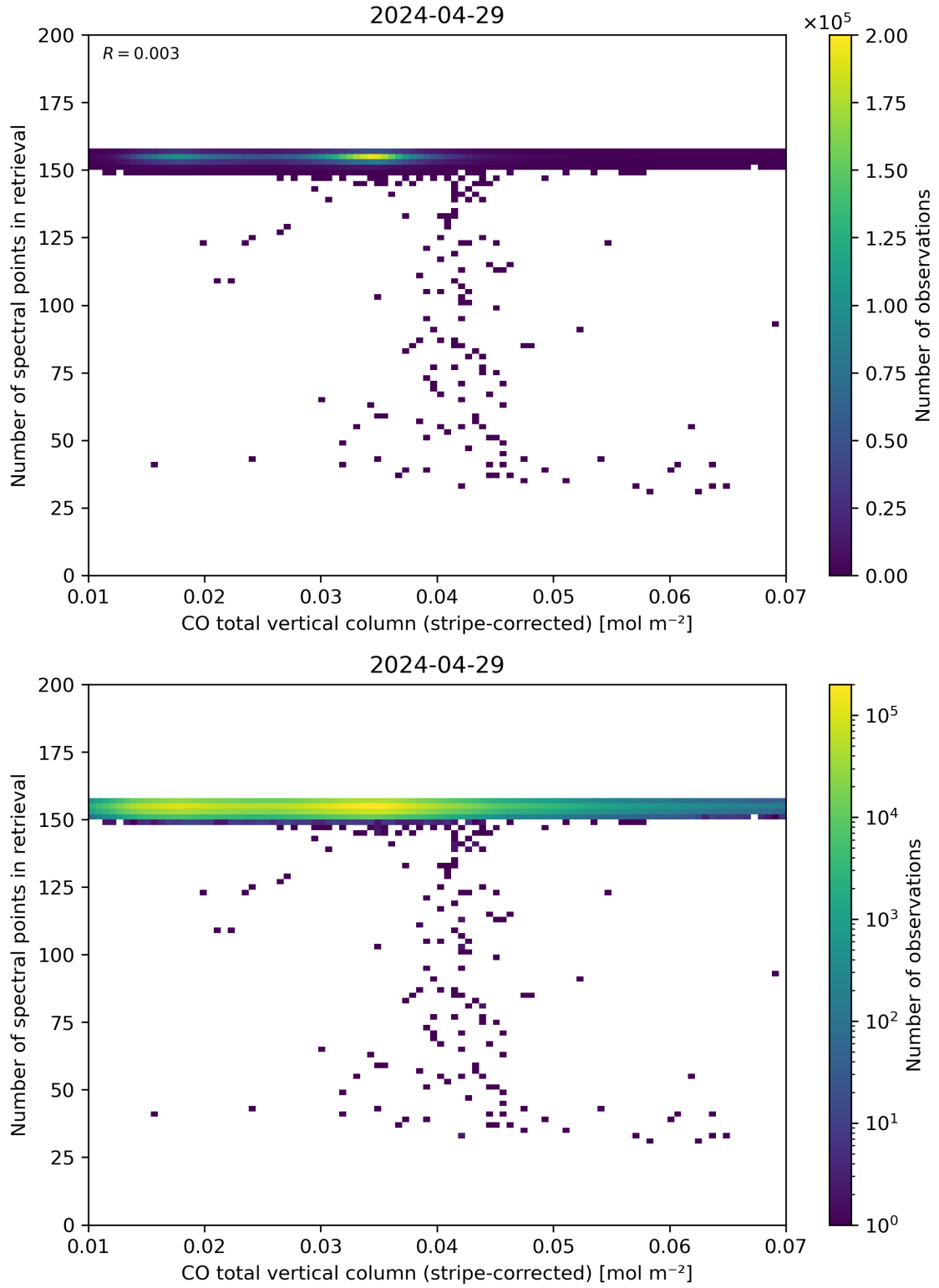
Figure 40: Scatter density plot of “CO total vertical column (stripe-corrected)” against “Number of spectral points in retrieval” for 2024-04-28 to 2024-04-30.
