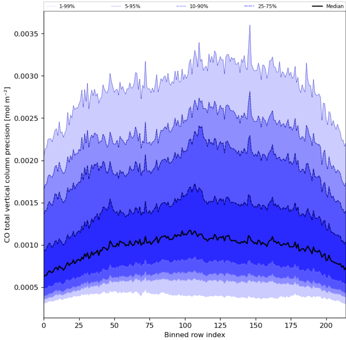
Figure 28: Along track statistics of “CO total vertical column precision” for 2024-04-28 to 2024-04-30
