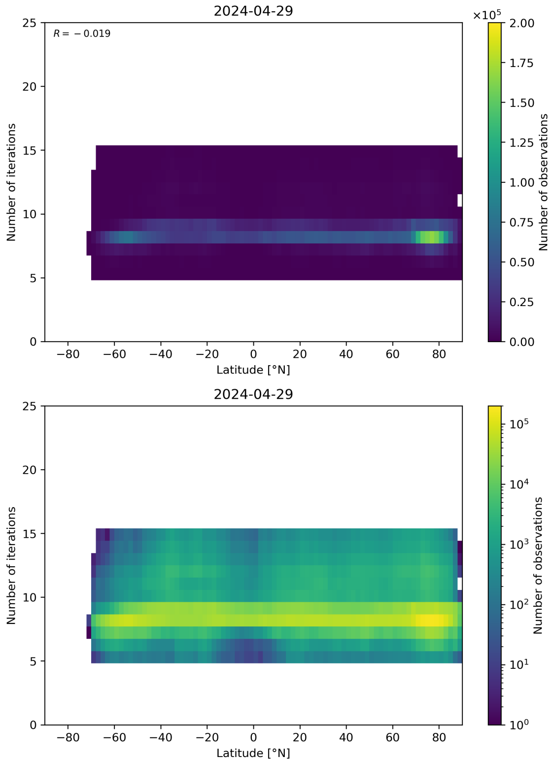
Figure 56: Scatter density plot of “Latitude” against “Number of iterations” for 2024-04-28 to 2024-04-30.
