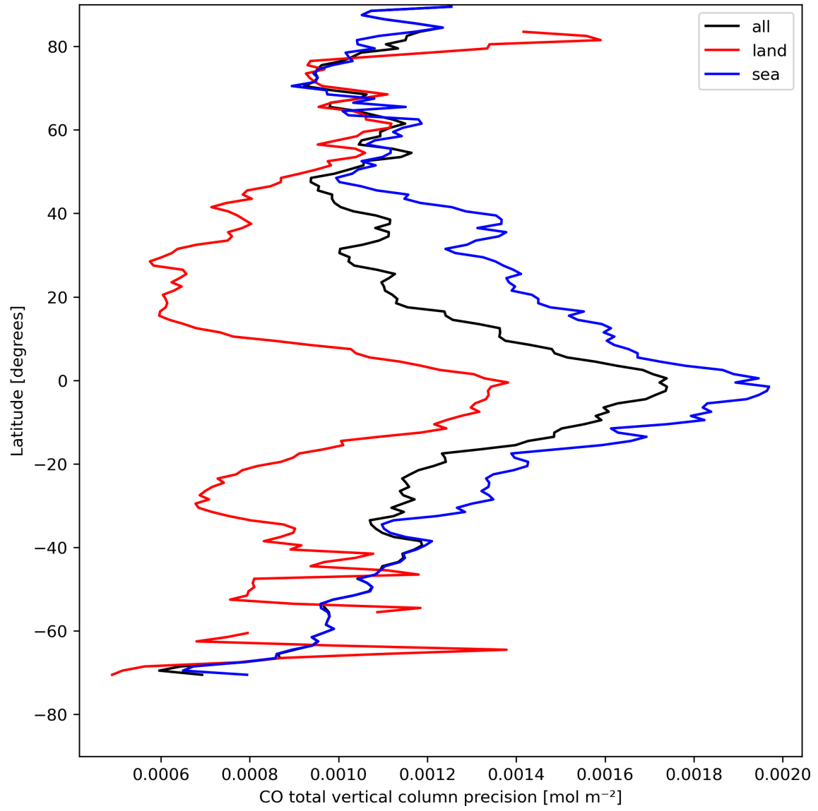
Figure 12: Zonal average of “CO total vertical column precision” for 2024-04-28 to 2024-04-30.
