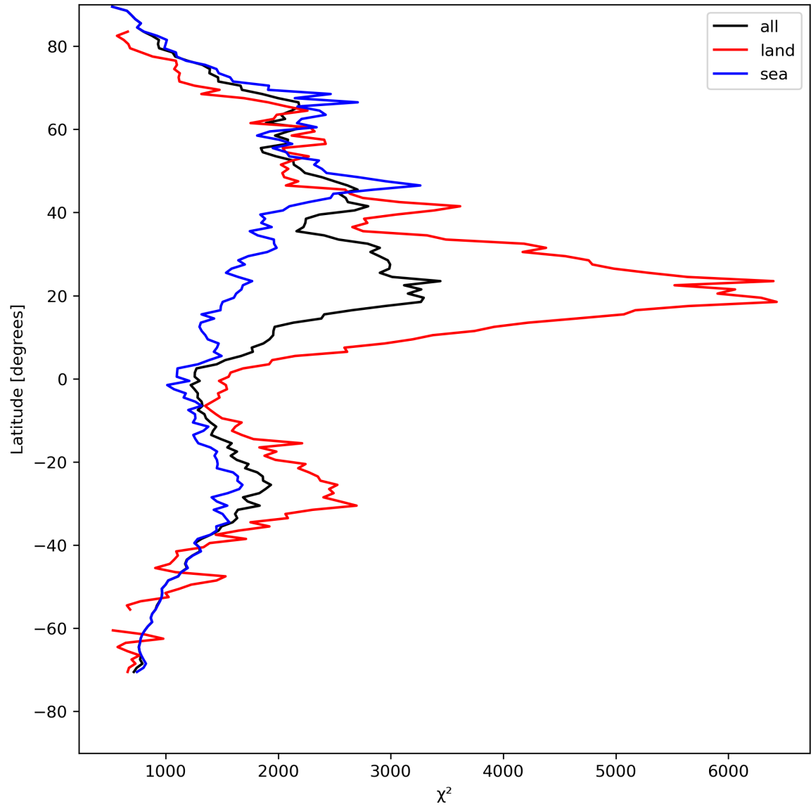
Figure 14: Zonal average of “ \chi^2 ” for 2024-04-28 to 2024-04-30.
