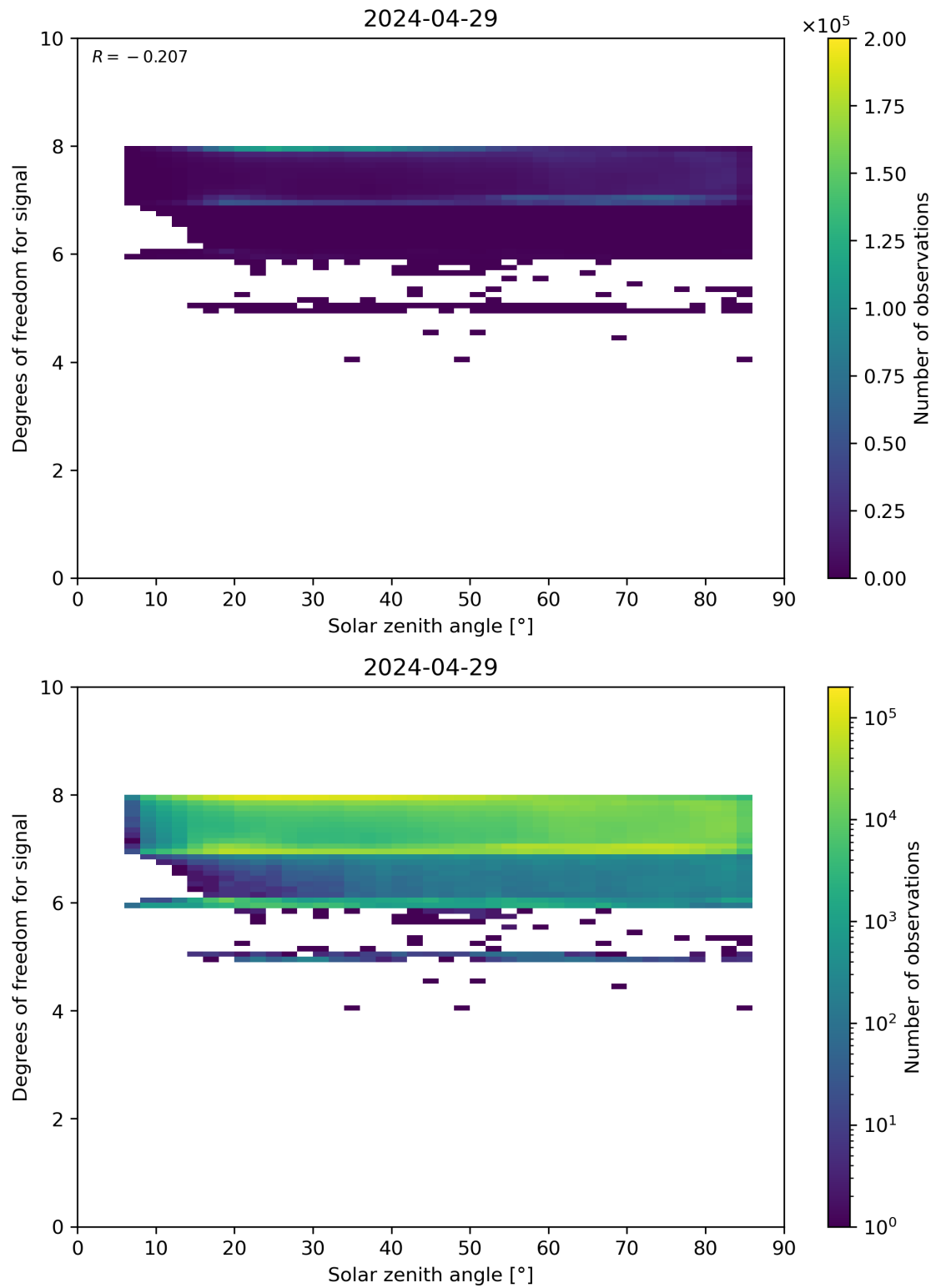
Figure 65: Scatter density plot of “Solar zenith angle” against “Degrees of freedom for signal” for 2024-04-28 to 2024-04-30.
