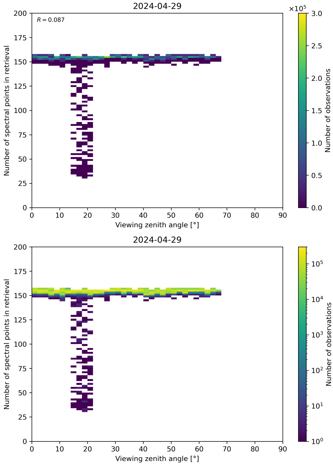
Figure 76: Scatter density plot of “Viewing zenith angle” against “Number of spectral points in retrieval” for 2024-04-28 to 2024-04-30.
