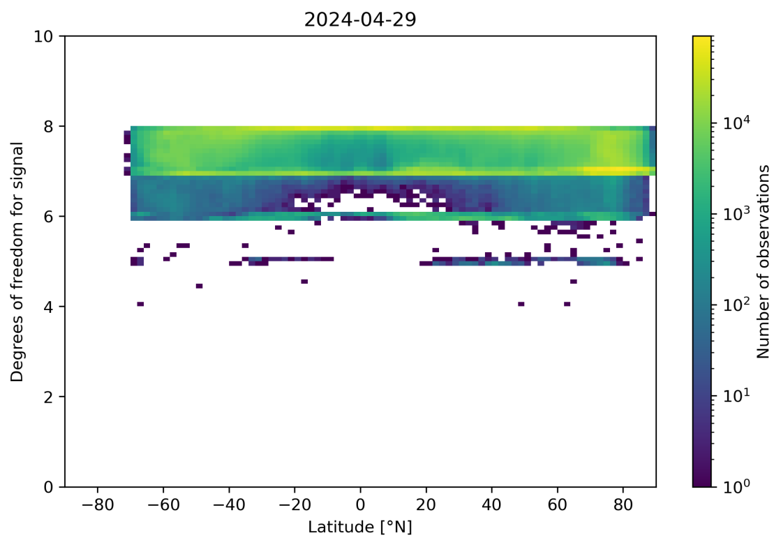
Figure 55: Scatter density plot of “Latitude” against “Degrees of freedom for signal” for 2024-04-28 to 2024-04-30.
