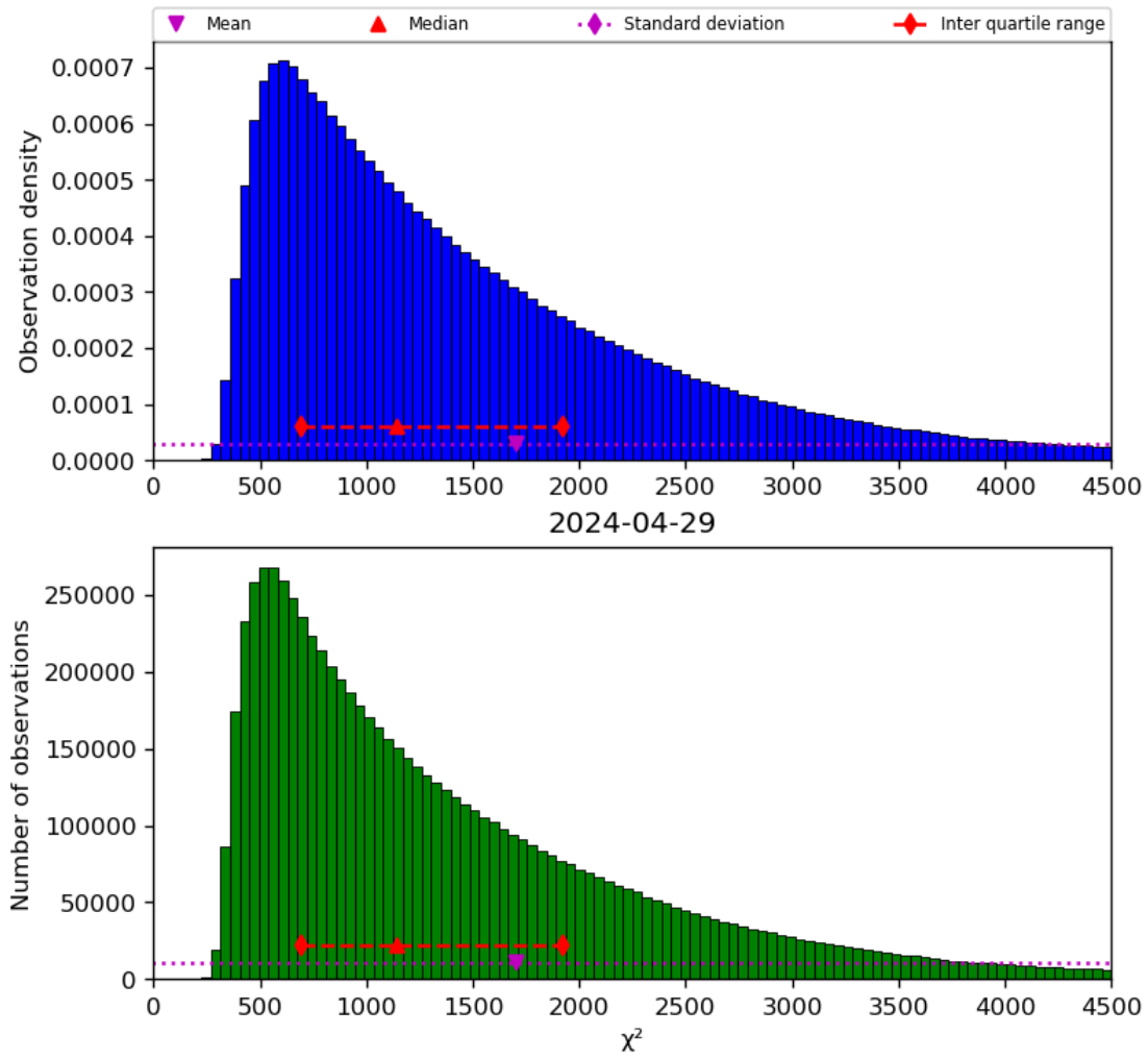
Figure 22: Histogram of “ \chi^2 ” for 2024-04-28 to 2024-04-30
