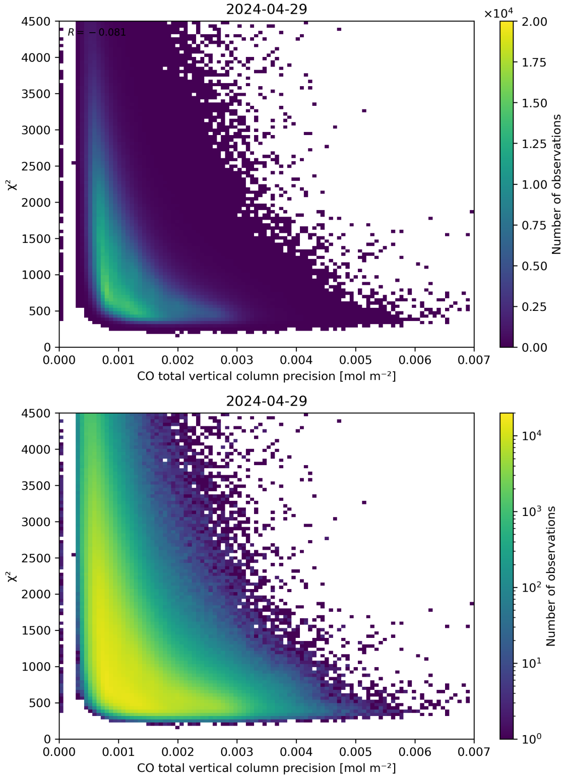
Figure 44: Scatter density plot of “CO total vertical column precision” against “ \chi^2 ” for 2024-04-28 to 2024-04-30.
