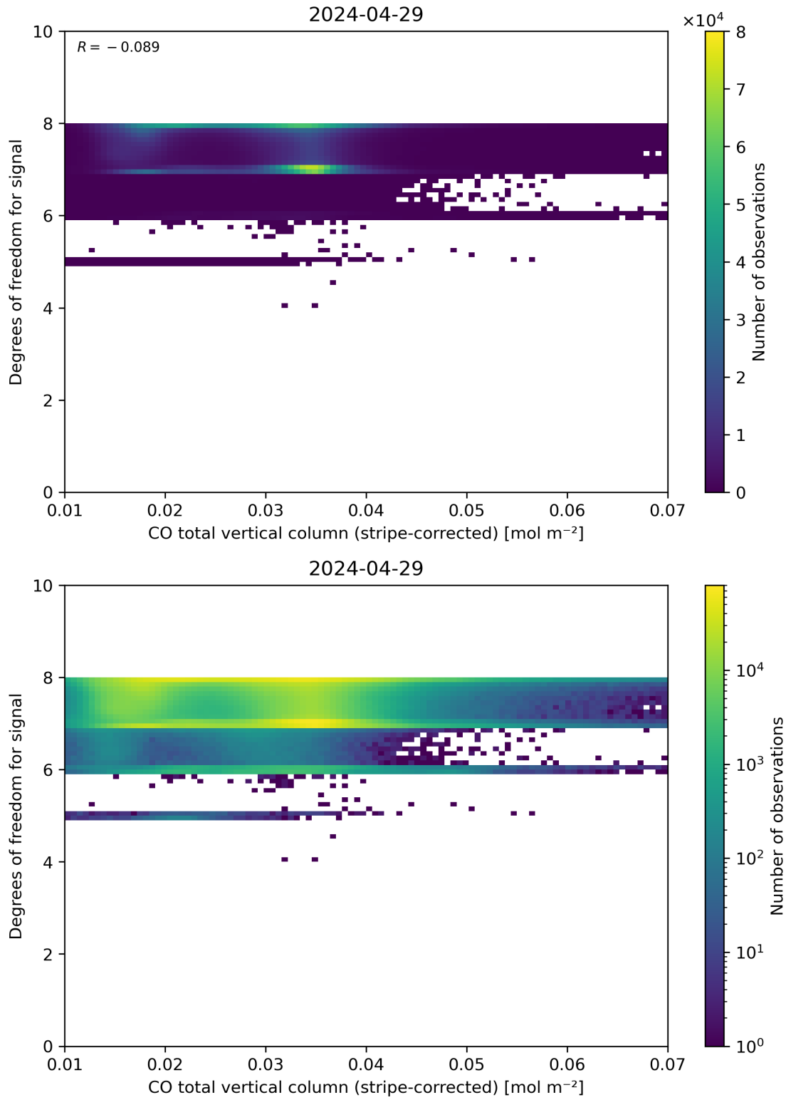
Figure 38: Scatter density plot of “CO total vertical column (stripe-corrected)” against “Degrees of freedom for signal” for 2024-04-28 to 2024-04-30.
