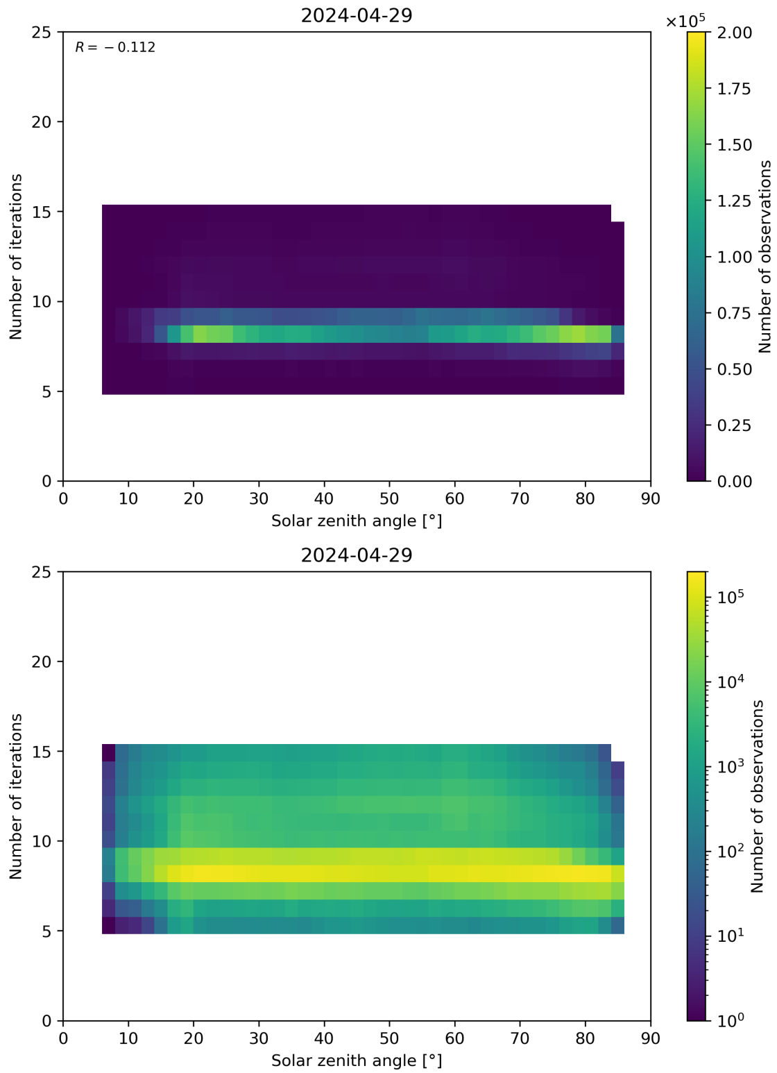
Figure 67: Scatter density plot of “Solar zenith angle” against “Number of iterations” for 2024-04-28 to 2024-04-30.
