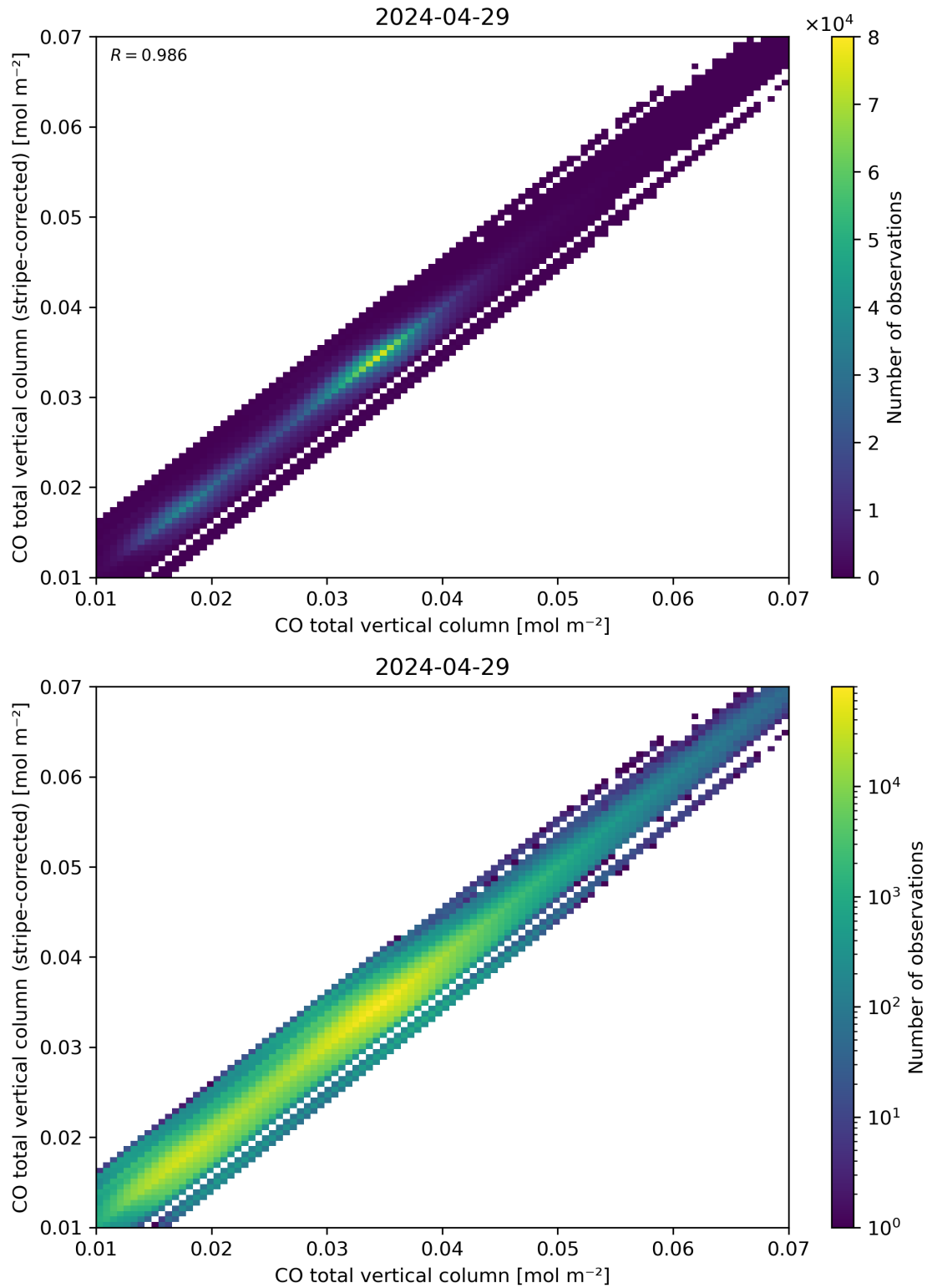
Figure 33: Scatter density plot of “CO total vertical column” against “CO total vertical column (stripe-corrected)” for 2024-04-28 to 2024-04-30.
