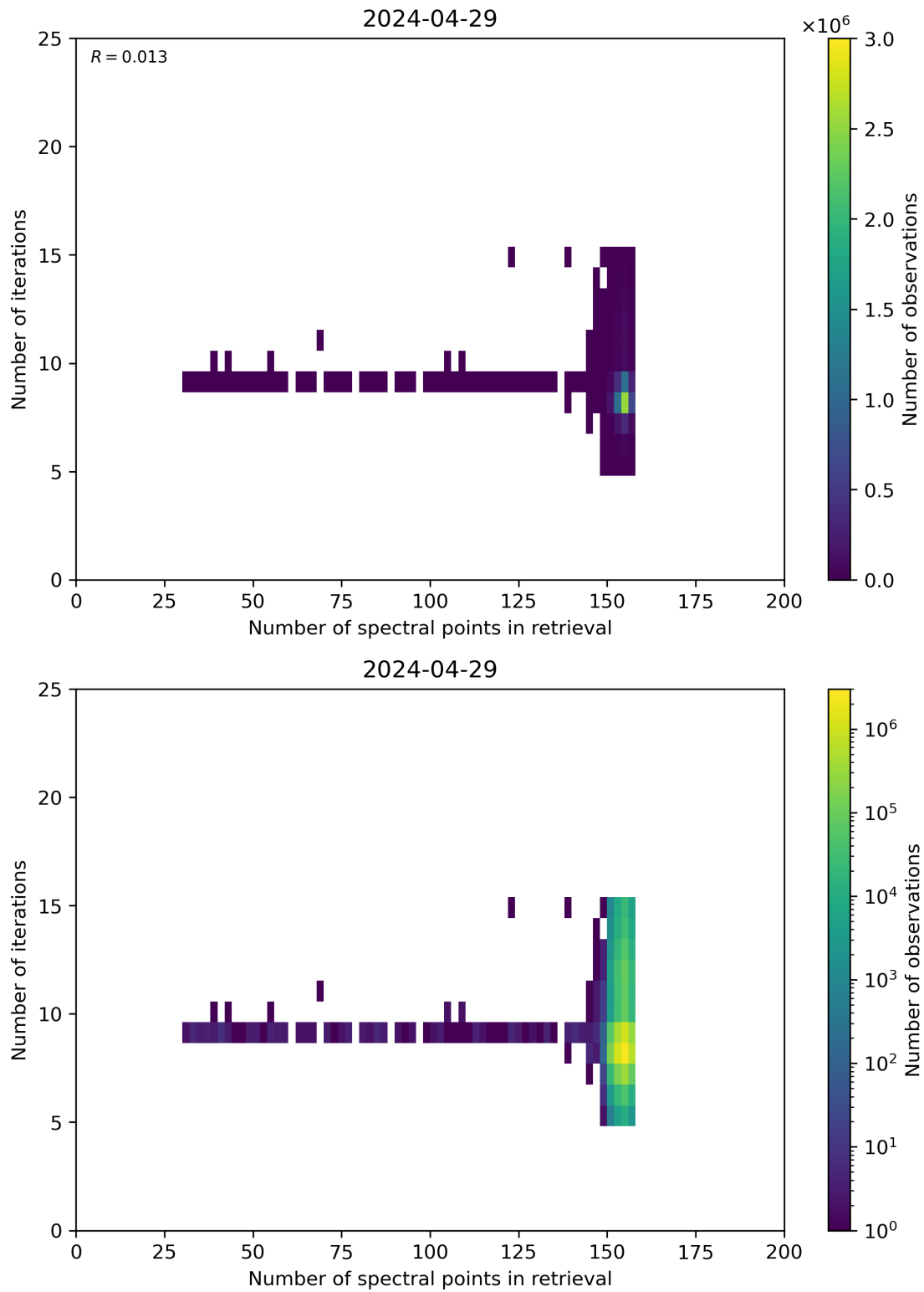
Figure 60: Scatter density plot of “Number of spectral points in retrieval” against “Number of iterations” for 2024-04-28 to 2024-04-30.
