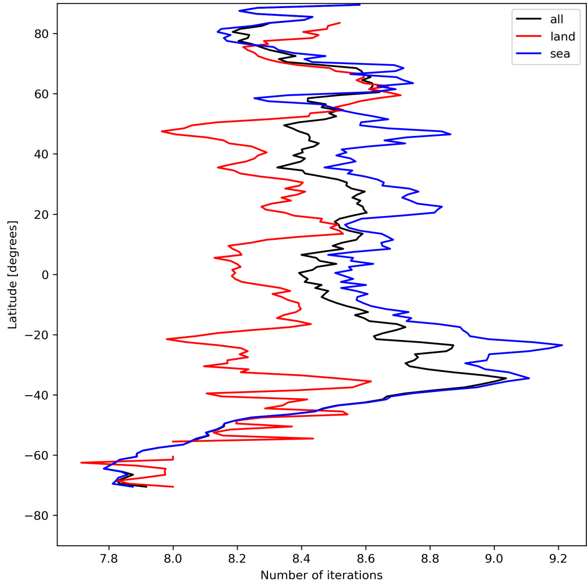
Figure 16: Zonal average of “Number of iterations” for 2024-04-28 to 2024-04-30.
