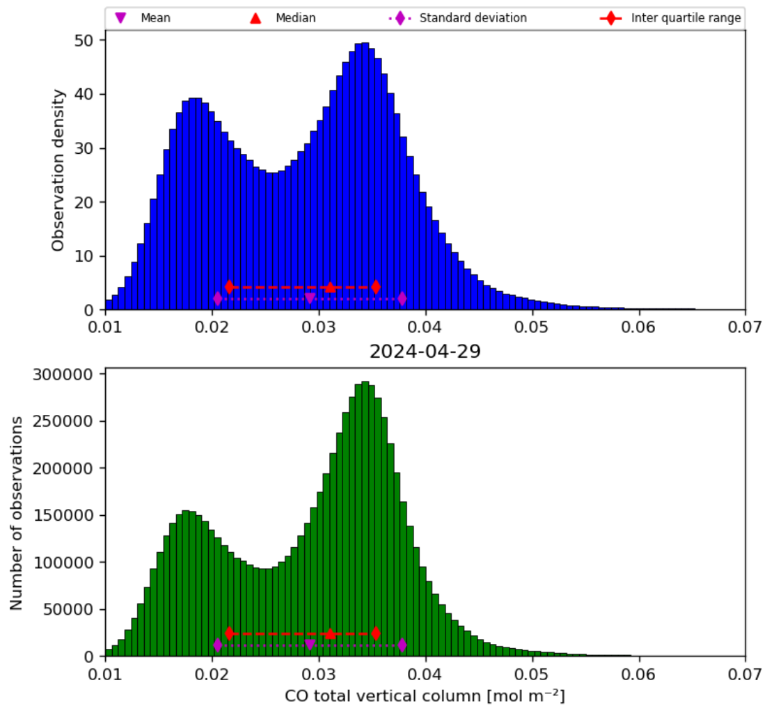
Figure 18: Histogram of “CO total vertical column” for 2024-04-28 to 2024-04-30
