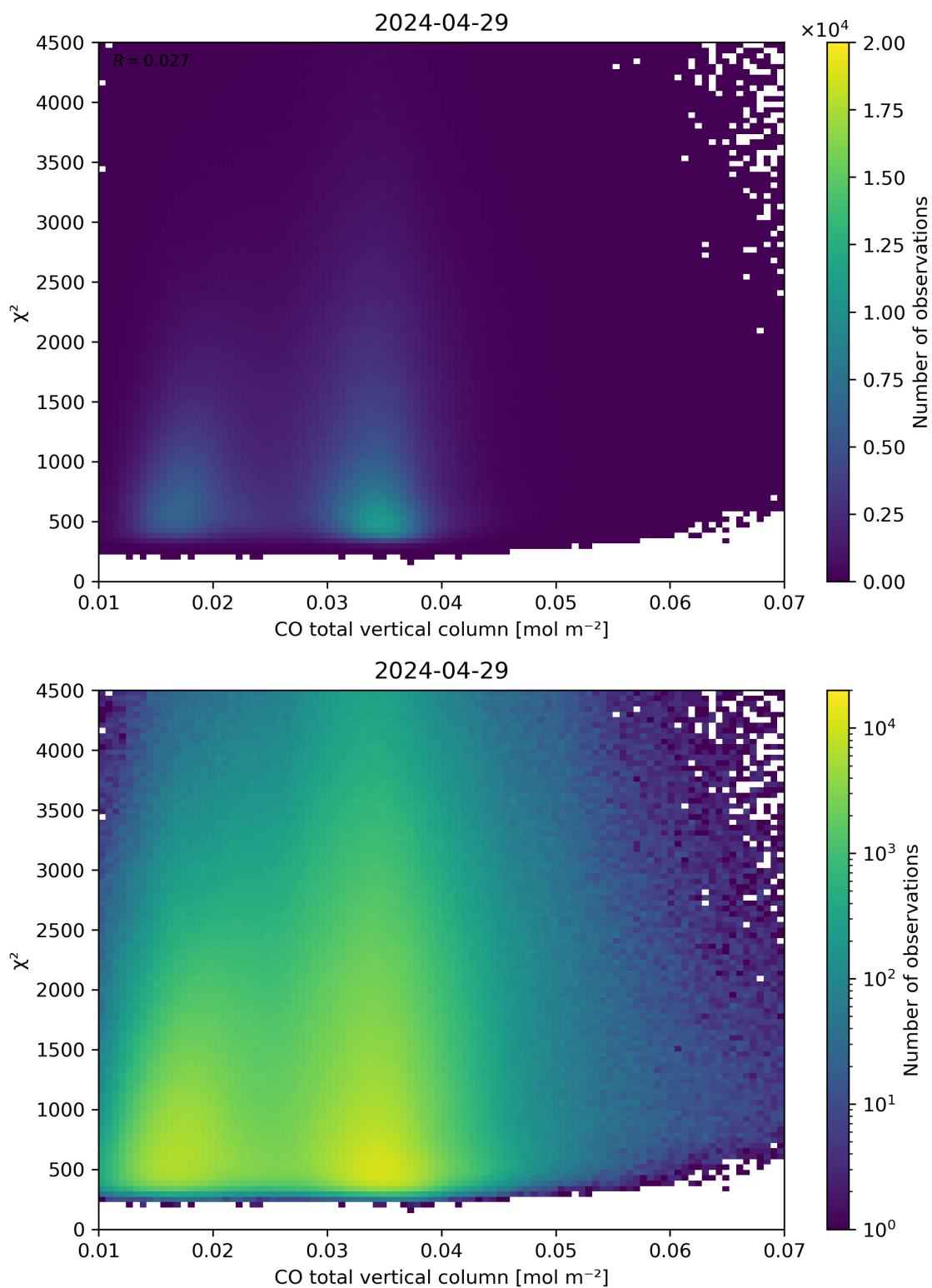
Figure 35: Scatter density plot of “CO total vertical column” against “ \chi^2 ” for 2024-04-28 to 2024-04-30.
