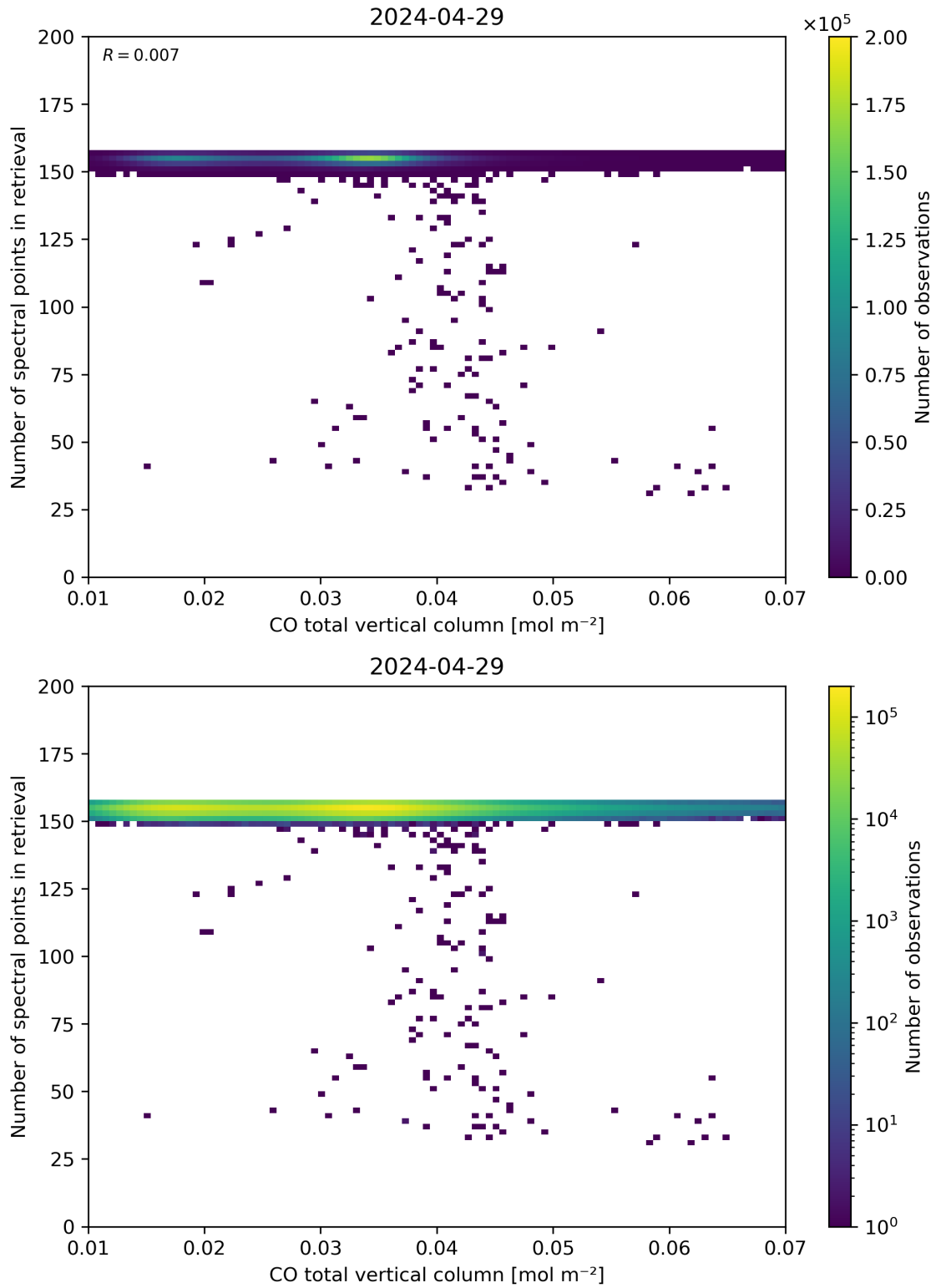
Figure 43: Scatter density plot of “CO total vertical column” against “Number of spectral points in retrieval” for 2024-04-28 to 2024-04-30.
