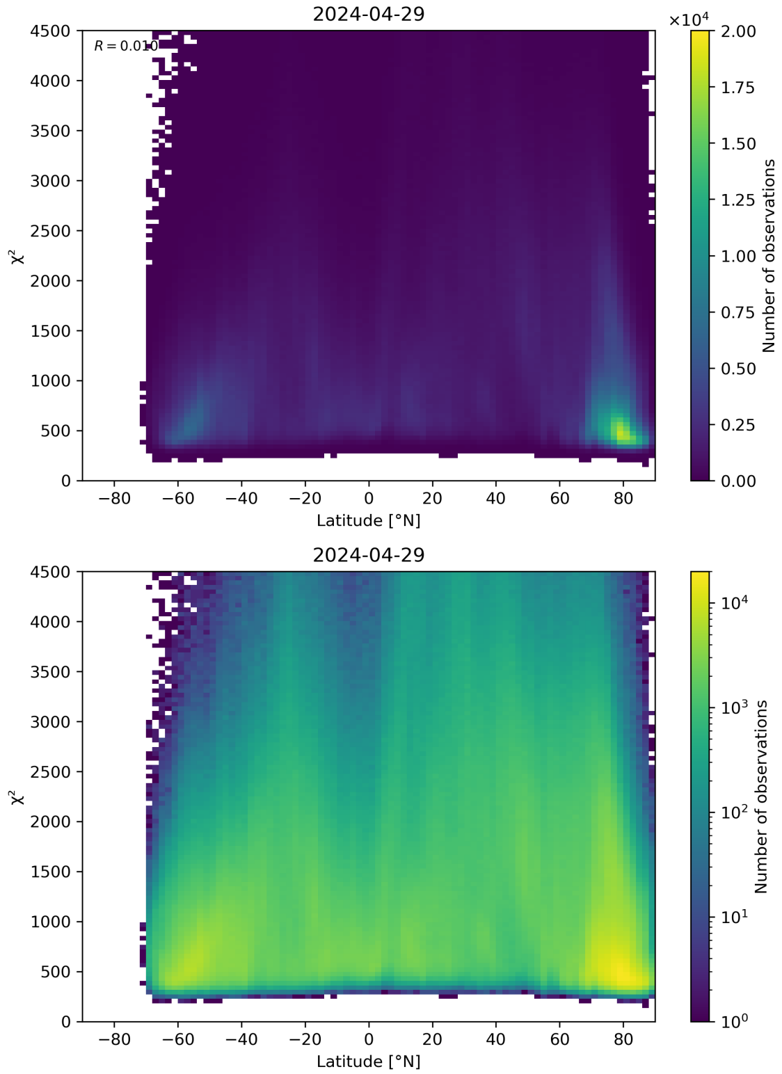
Figure 54: Scatter density plot of “Latitude” against “ \chi^2 ” for 2024-04-28 to 2024-04-30.
