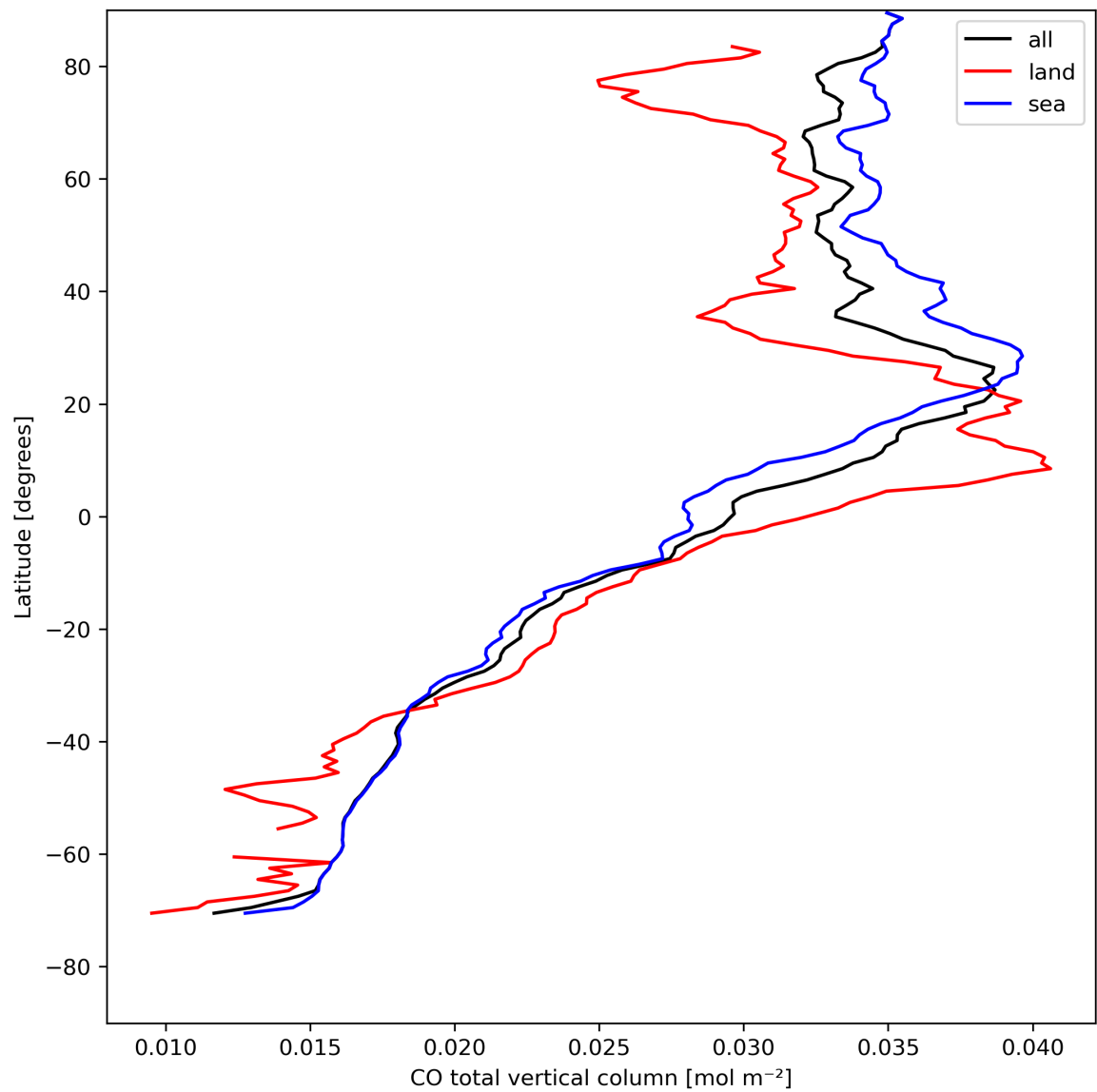
Figure 10: Zonal average of “CO total vertical column” for 2024-04-28 to 2024-04-30.
