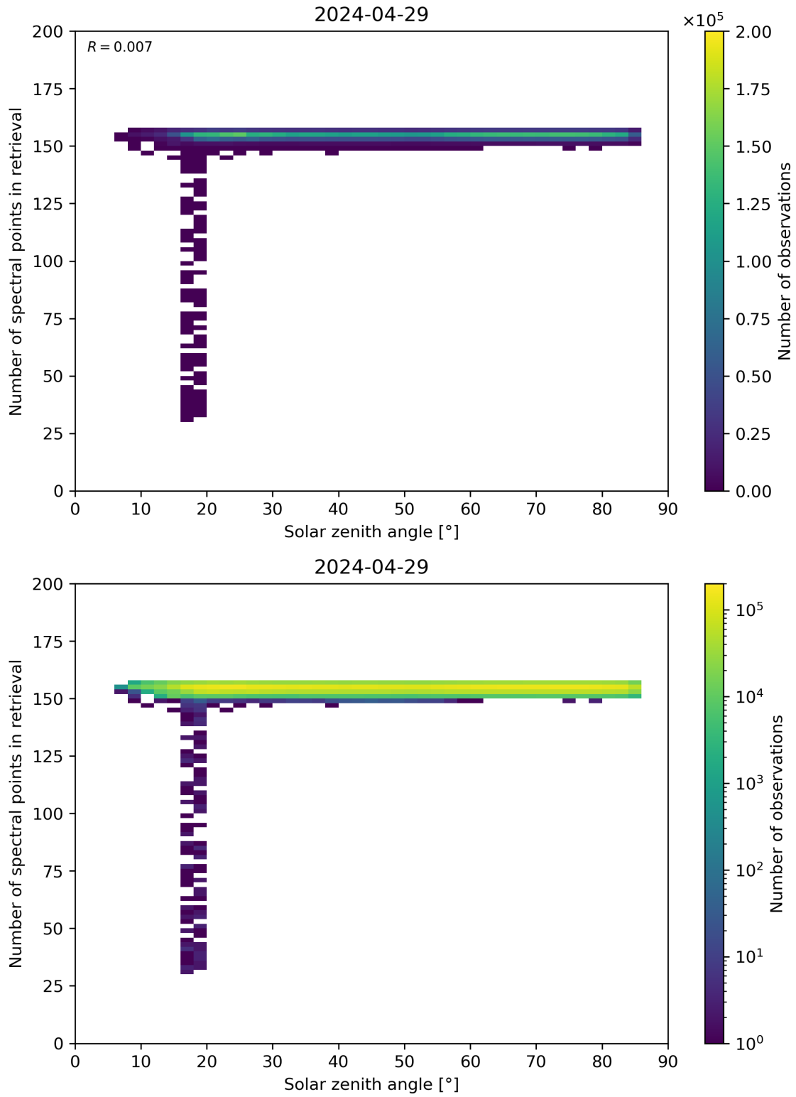
Figure 68: Scatter density plot of “Solar zenith angle” against “Number of spectral points in retrieval” for 2024-04-28 to 2024-04-30.
