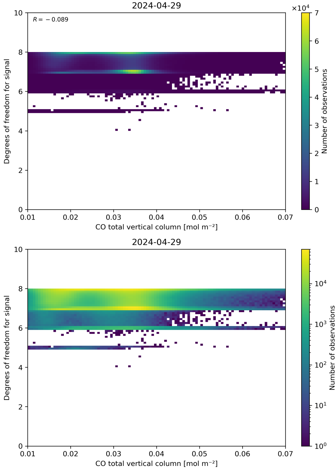
Figure 41: Scatter density plot of “CO total vertical column” against “Degrees of freedom for signal” for 2024-04-28 to 2024-04-30.
