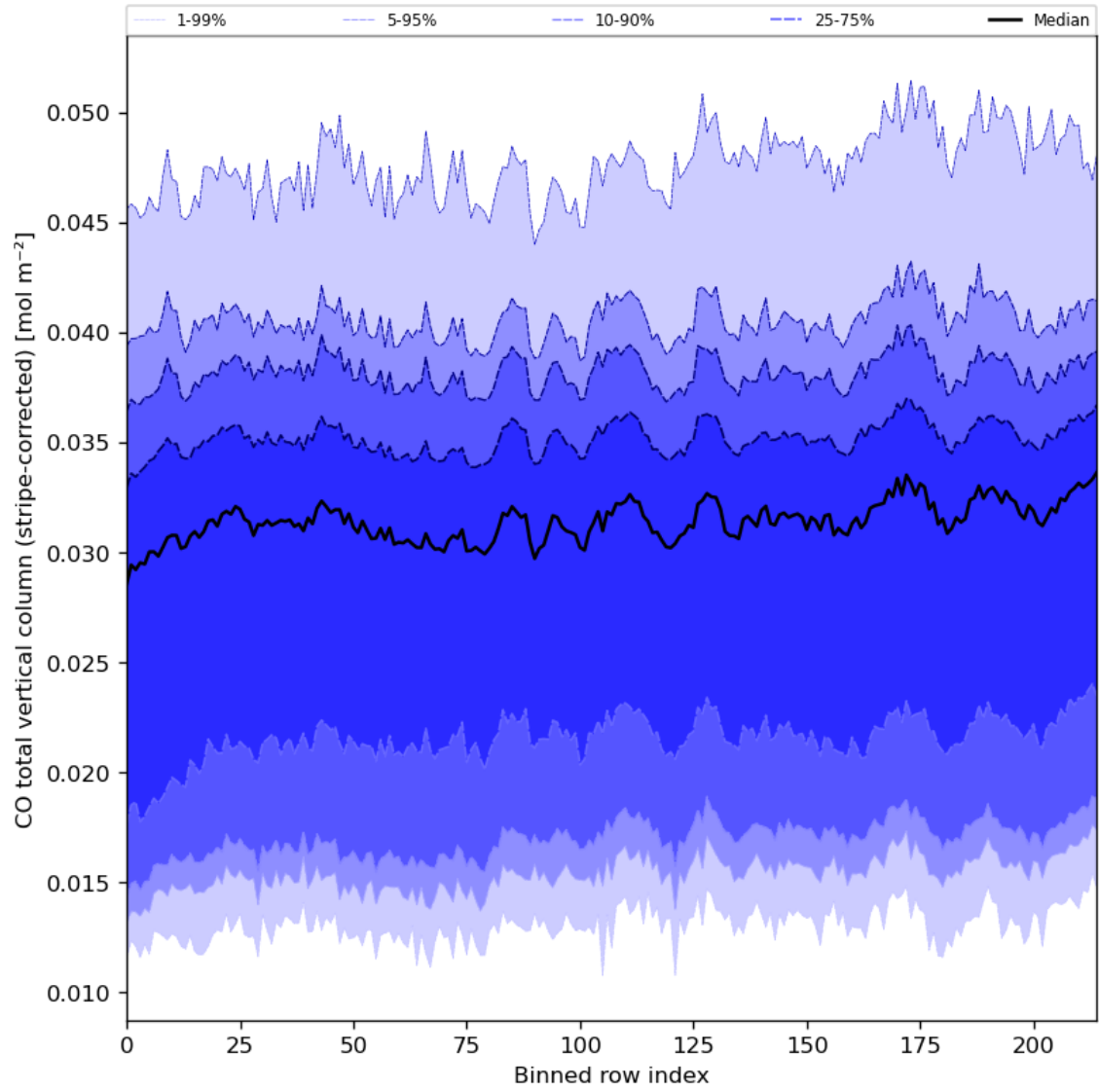
Figure 27: Along track statistics of “CO total vertical column (stripe-corrected)” for 2024-04-28 to 2024-04-30
