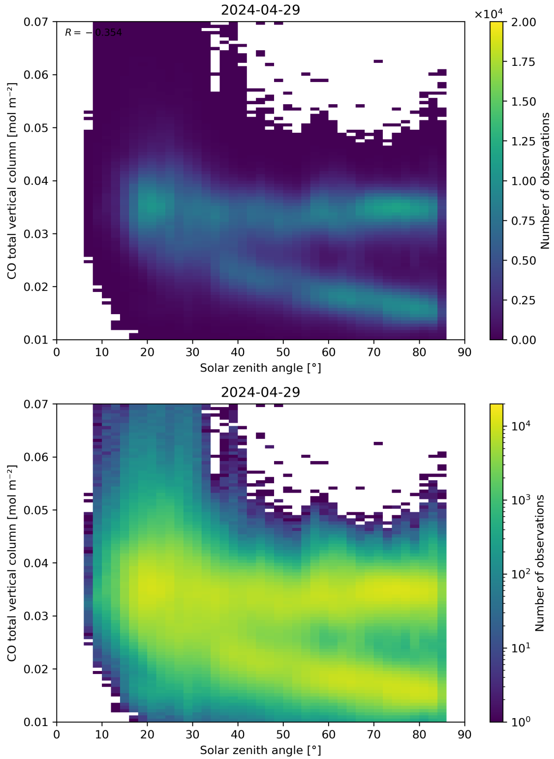
Figure 61: Scatter density plot of “Solar zenith angle” against “CO total vertical column” for 2024-04-28 to 2024-04-30.
