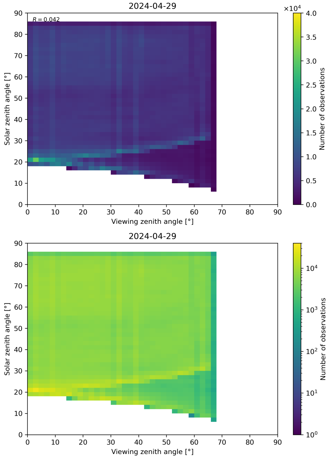
Figure 77: Scatter density plot of “Viewing zenith angle” against “Solar zenith angle” for 2024-04-28 to 2024-04-30.
