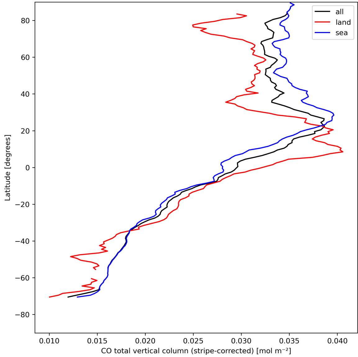
Figure 11: Zonal average of “CO total vertical column (stripe-corrected)” for 2024-04-28 to 2024-04-30.
