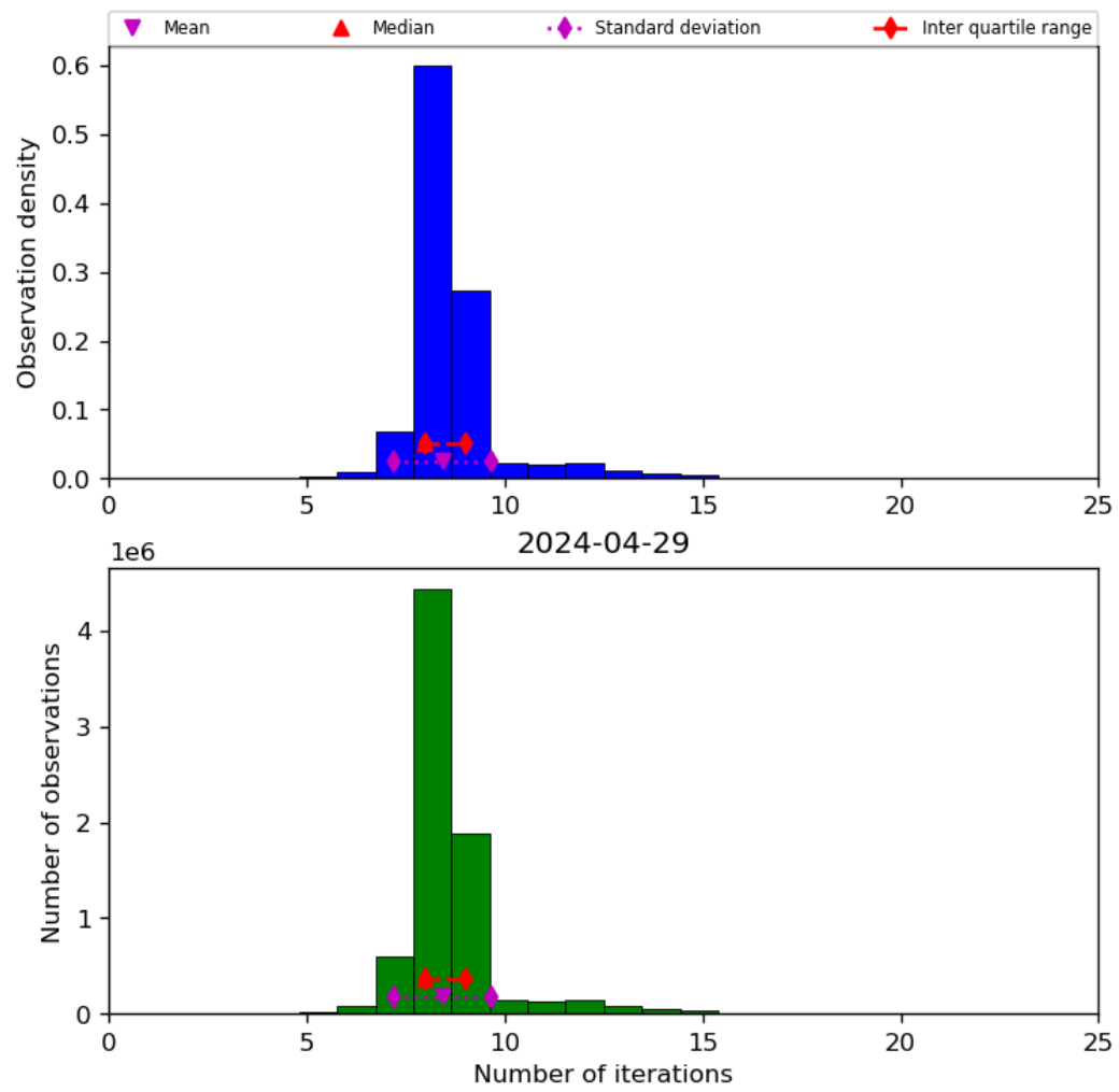
Figure 24: Histogram of “Number of iterations” for 2024-04-28 to 2024-04-30
