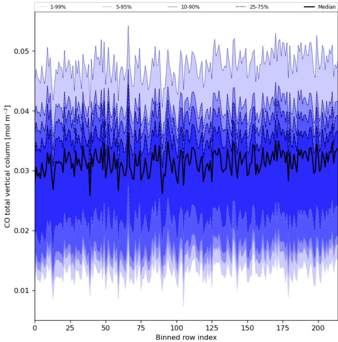
Figure 26: Along track statistics of “CO total vertical column” for 2024-04-28 to 2024-04-30
