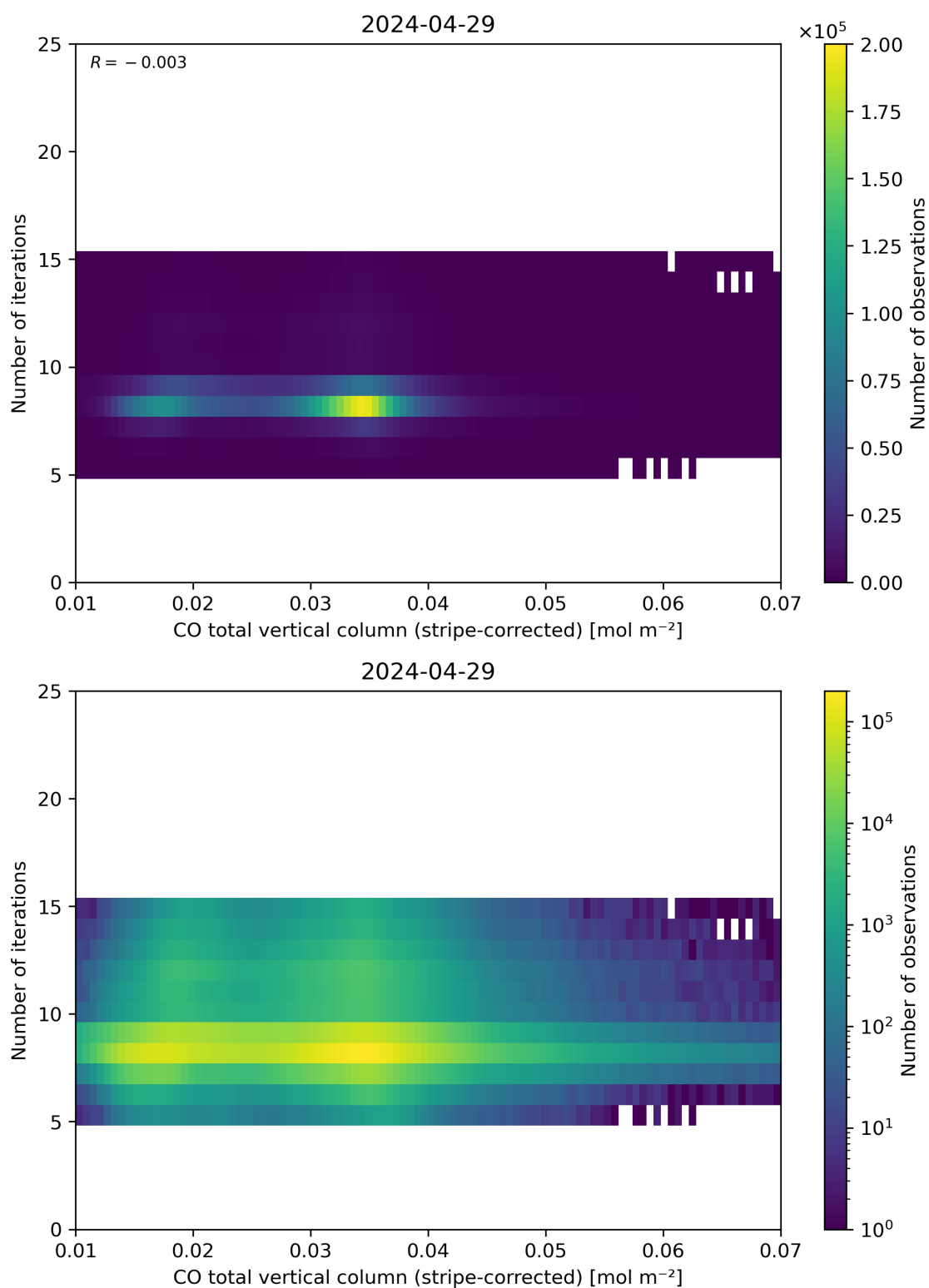
Figure 39: Scatter density plot of “CO total vertical column (stripe-corrected)” against “Number of iterations” for 2024-04-28 to 2024-04-30.
