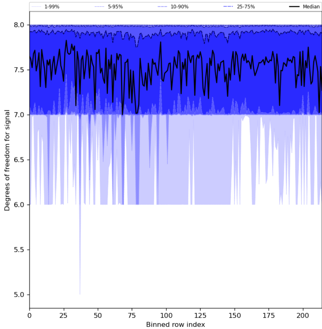
Figure 31: Along track statistics of “Degrees of freedom for signal” for 2024-04-28 to 2024-04-30
