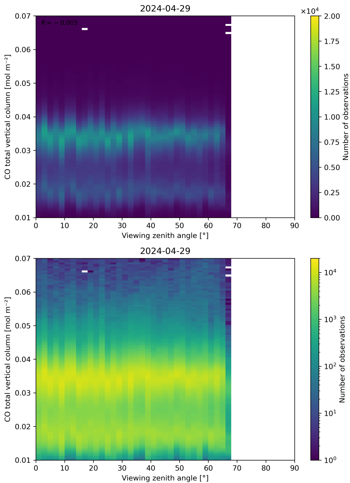
Figure 69: Scatter density plot of “Viewing zenith angle” against “CO total vertical column” for 2024-04-28 to 2024-04-30.
