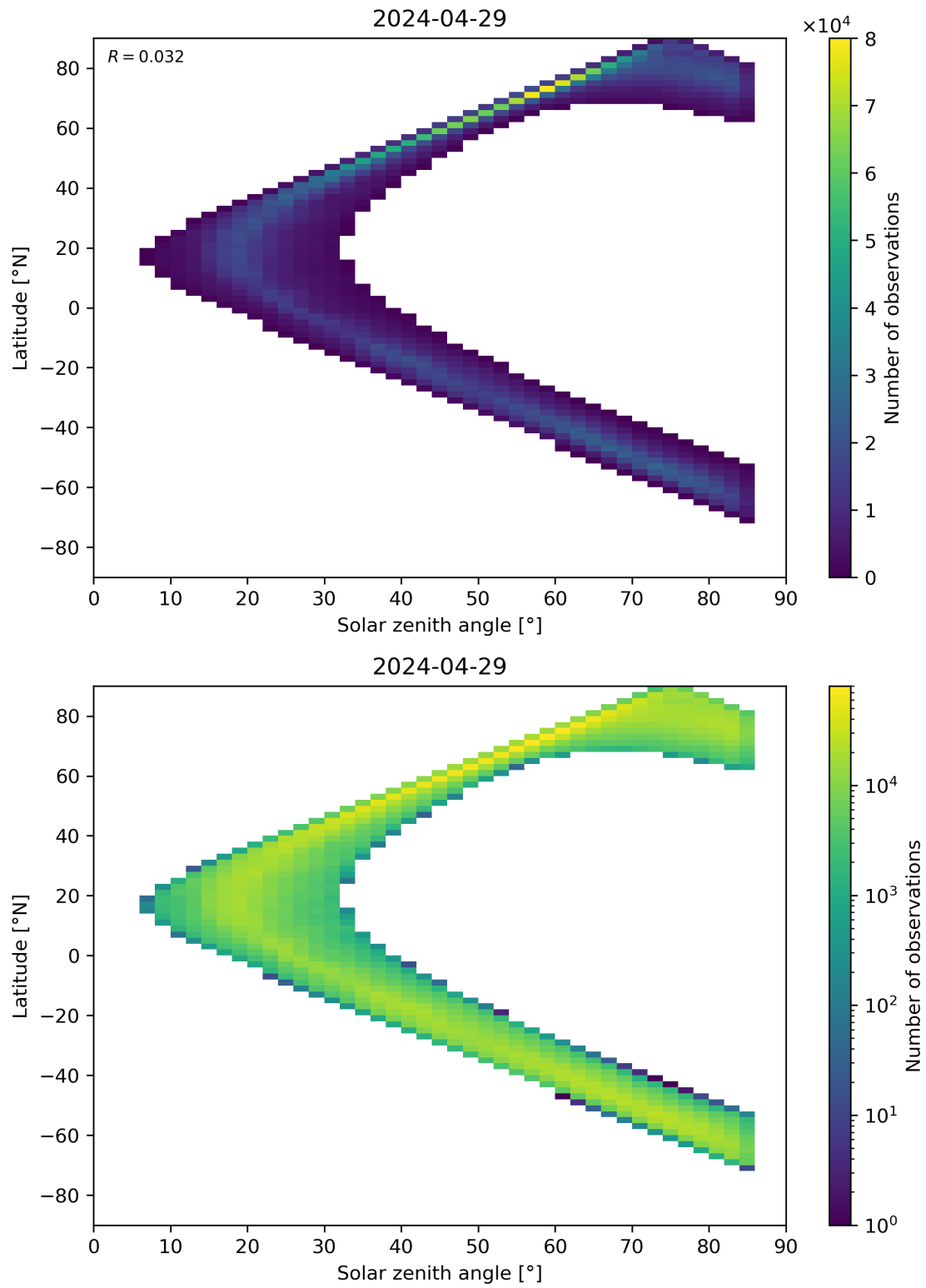
Figure 66: Scatter density plot of “Solar zenith angle” against “Latitude” for 2024-04-28 to 2024-04-30.
