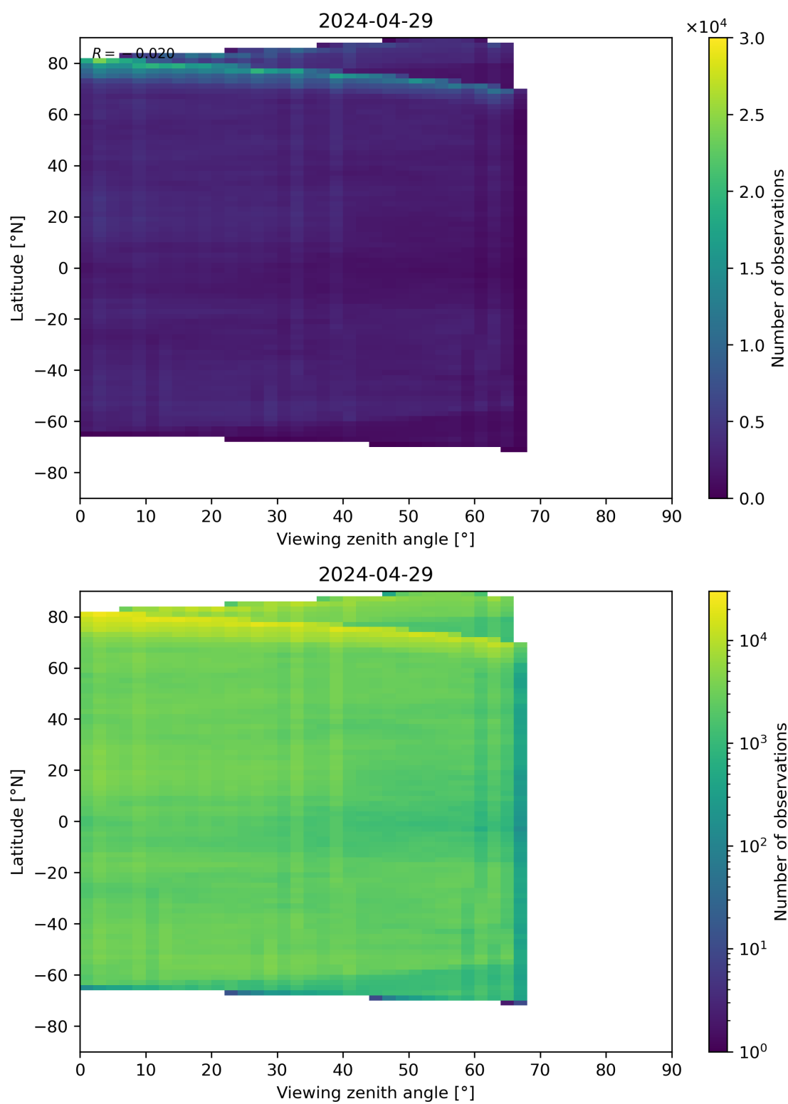
Figure 74: Scatter density plot of “Viewing zenith angle” against “Latitude” for 2024-04-28 to 2024-04-30.
