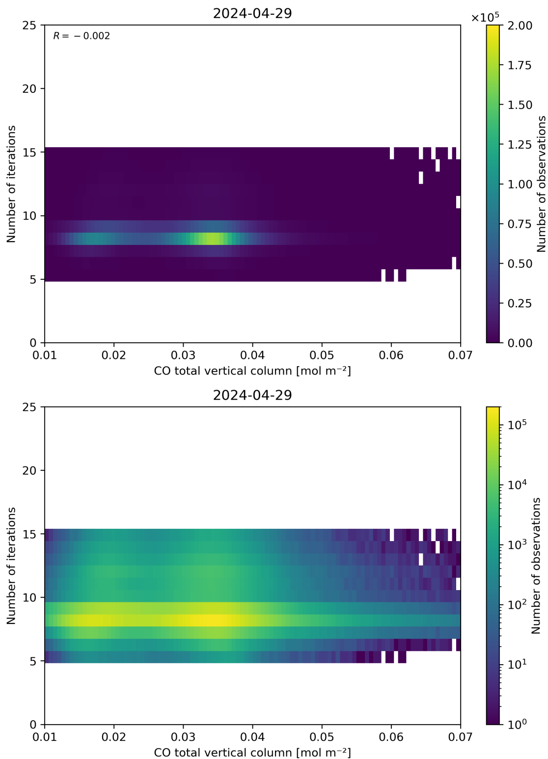
Figure 42: Scatter density plot of “CO total vertical column” against “Number of iterations” for 2024-04-28 to 2024-04-30.
