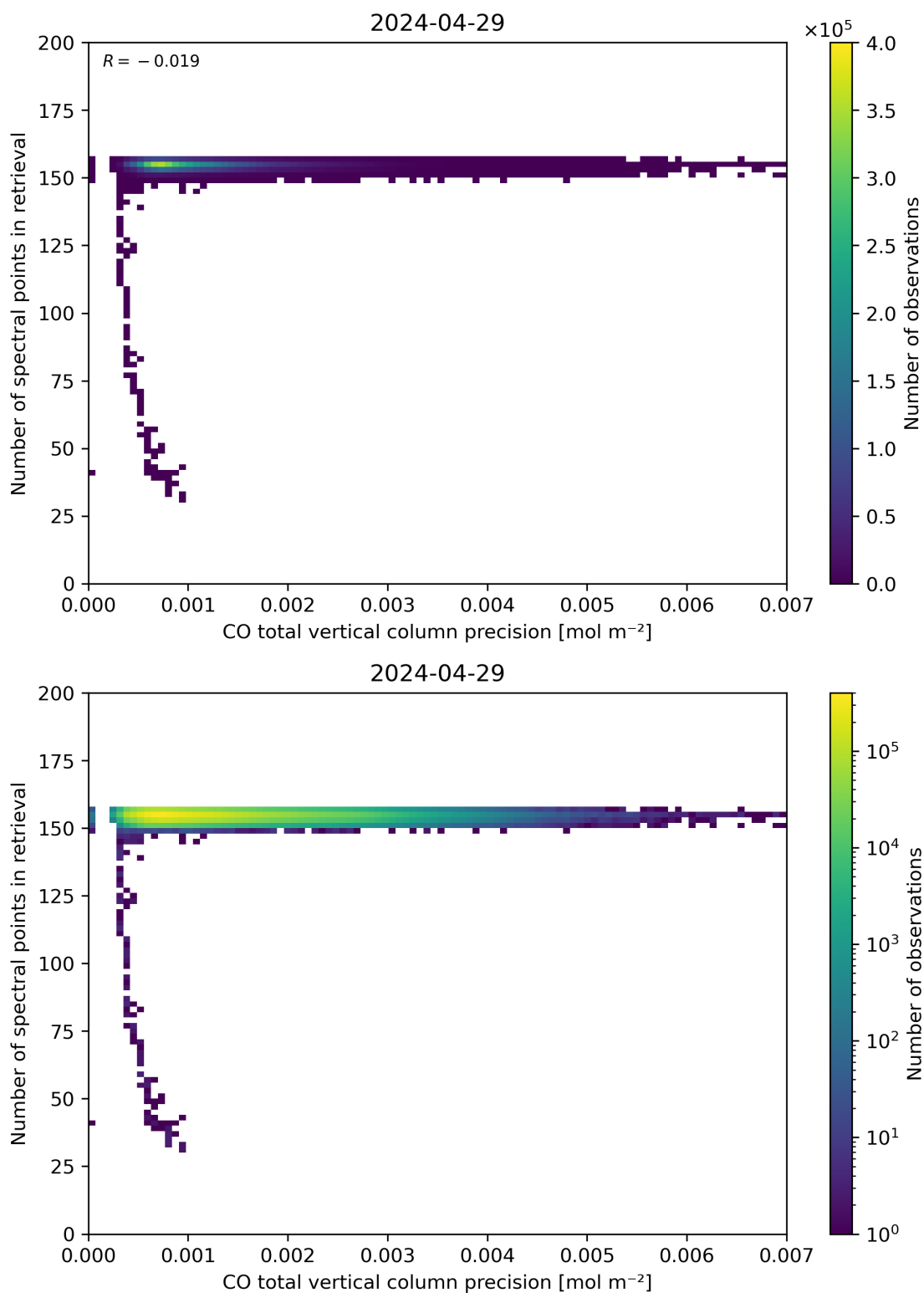
Figure 47: Scatter density plot of “CO total vertical column precision” against “Number of spectral points in retrieval” for 2024-04-28 to 2024-04-30.
