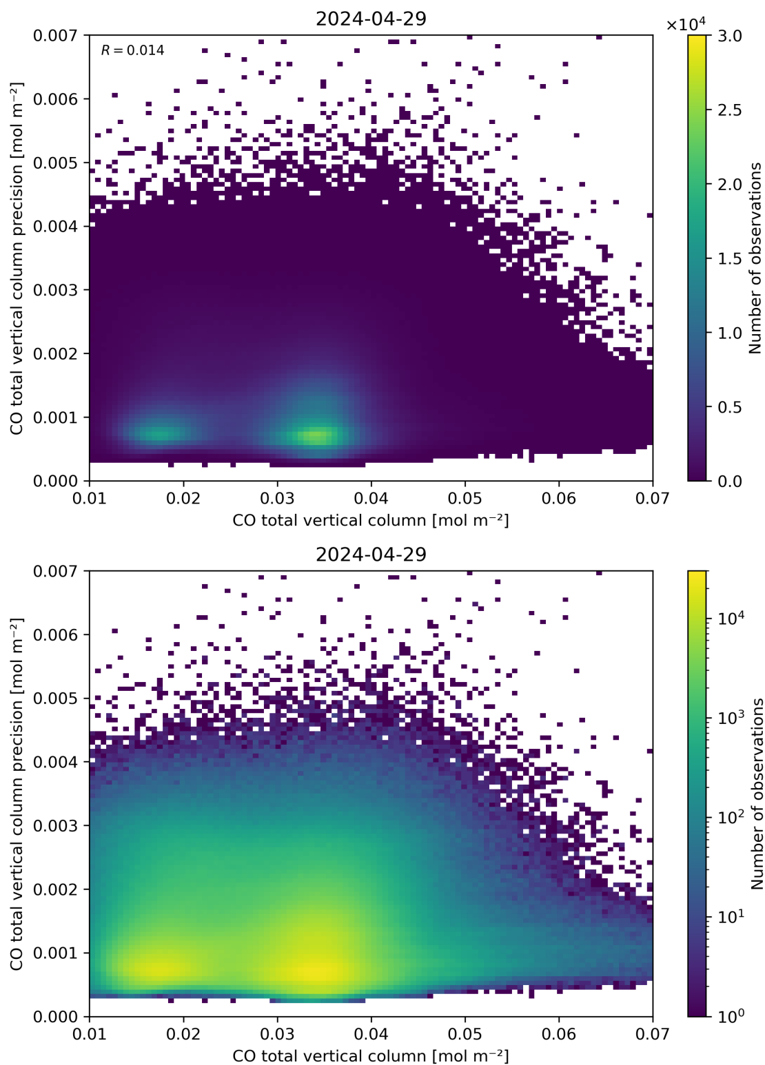
Figure 34: Scatter density plot of “CO total vertical column” against “CO total vertical column precision” for 2024-04-28 to 2024-04-30.
