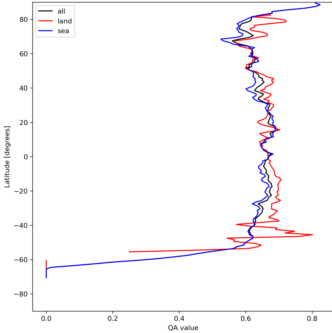
Figure 9: Zonal average of “QA value” for 2024-04-28 to 2024-04-30.
