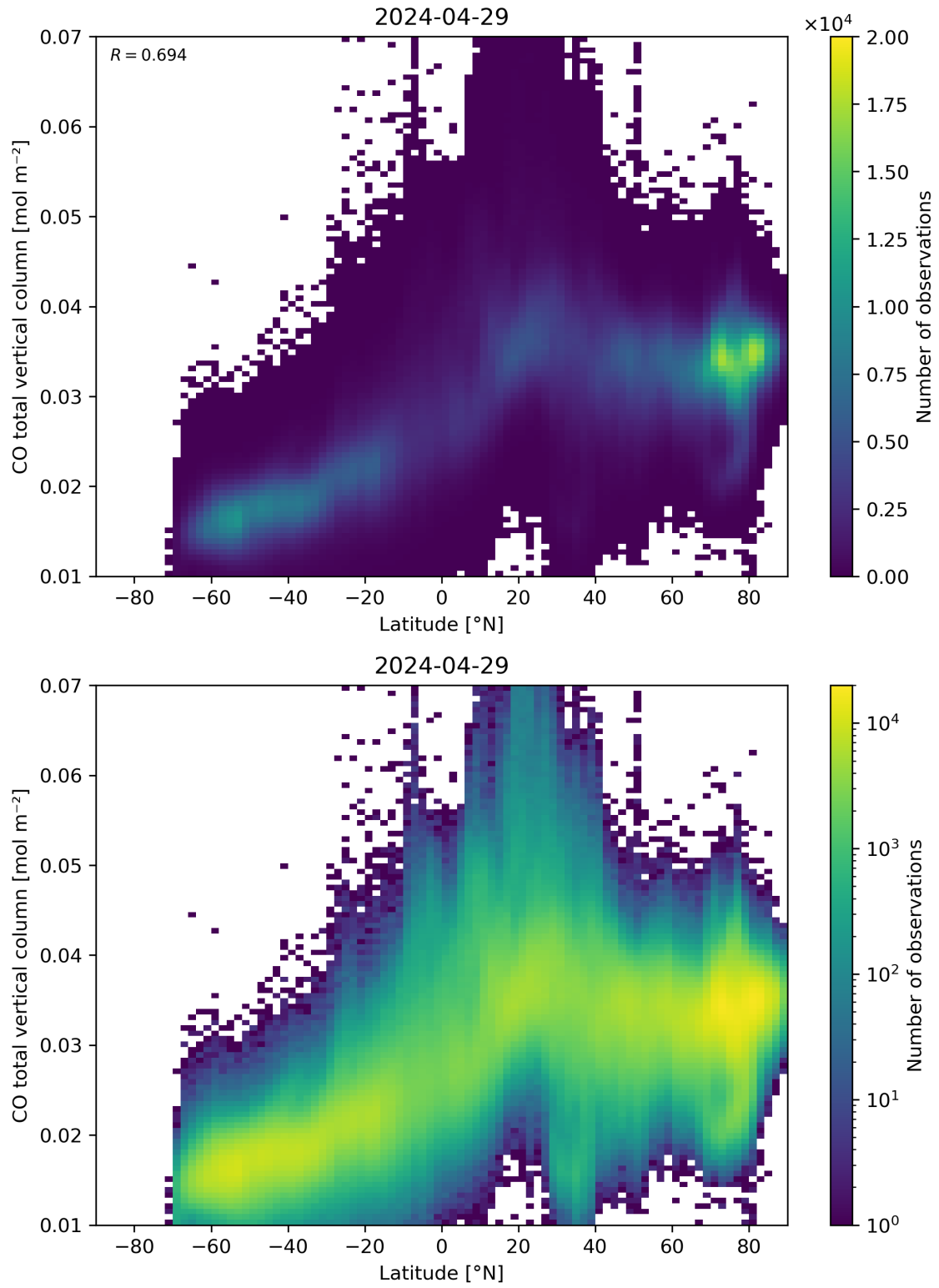
Figure 51: Scatter density plot of “Latitude” against “CO total vertical column” for 2024-04-28 to 2024-04-30.
