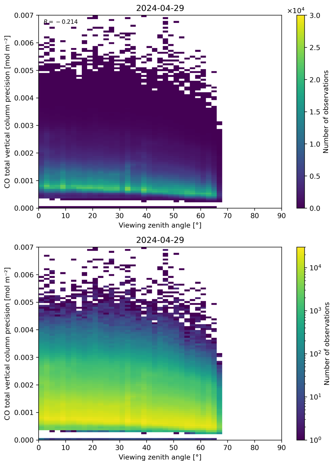
Figure 71: Scatter density plot of “Viewing zenith angle” against “CO total vertical column precision” for 2024-04-28 to 2024-04-30.
