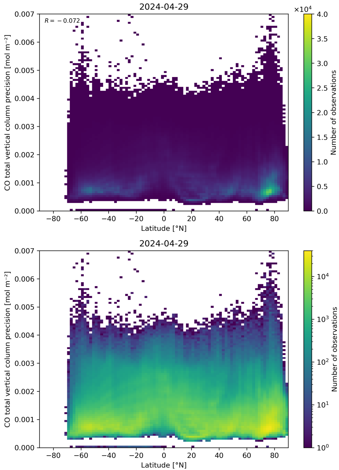
Figure 53: Scatter density plot of “Latitude” against “CO total vertical column precision” for 2024-04-28 to 2024-04-30.
