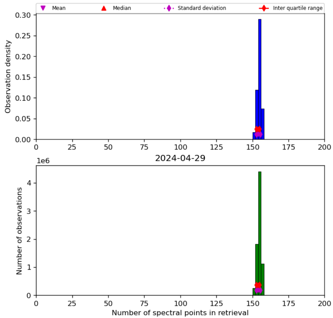
Figure 21: Histogram of “Number of spectral points in retrieval” for 2024-04-28 to 2024-04-30
