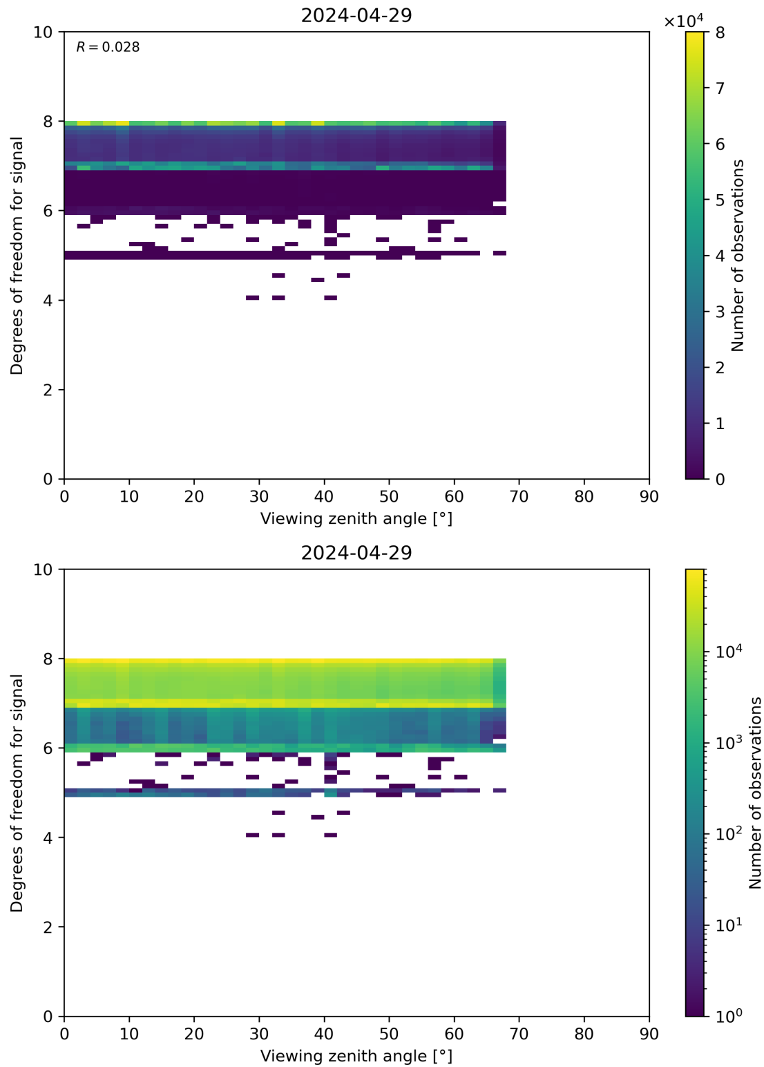
Figure 73: Scatter density plot of “Viewing zenith angle” against “Degrees of freedom for signal” for 2024-04-28 to 2024-04-30.
