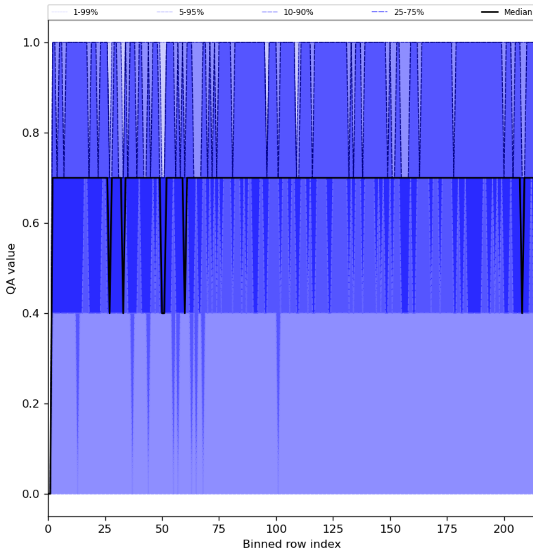
Figure 25: Along track statistics of “QA value” for 2024-04-28 to 2024-04-30
