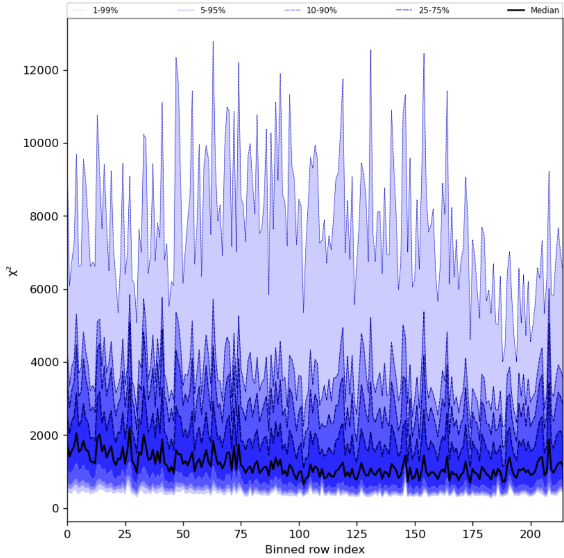
Figure 30: Along track statistics of “ \chi^2 ” for 2024-04-28 to 2024-04-30
