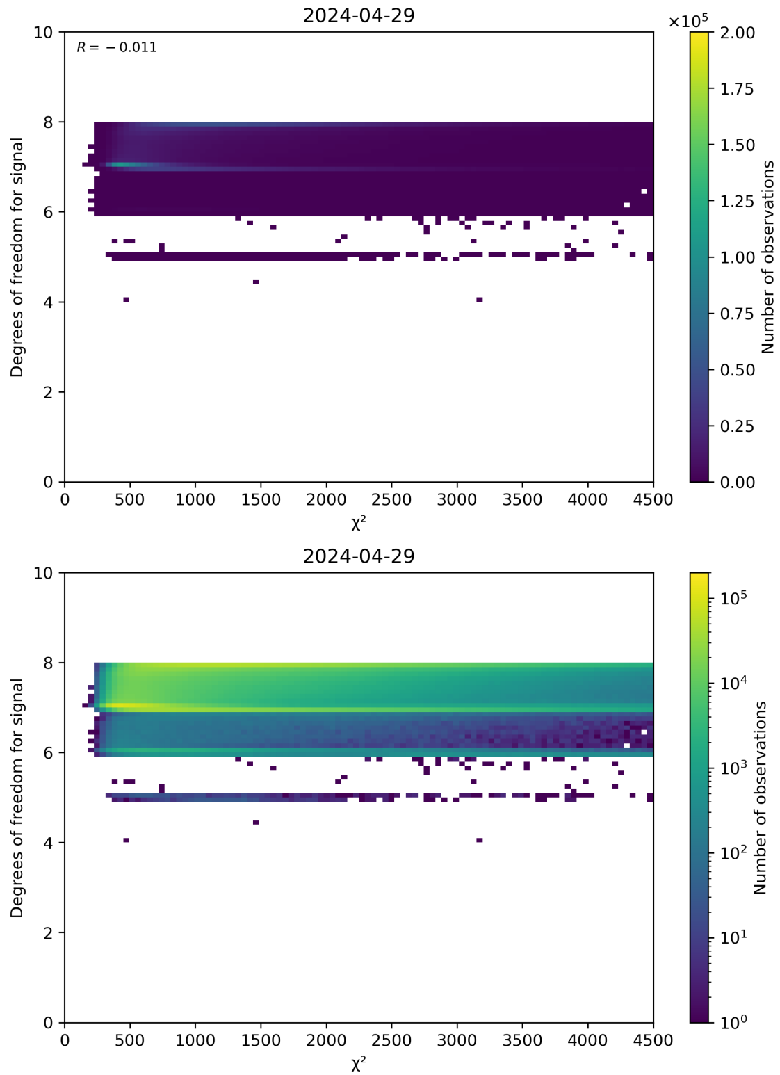
Figure 48: Scatter density plot of “ \chi^2 ” against “Degrees of freedom for signal” for 2024-04-28 to 2024-04-30.
