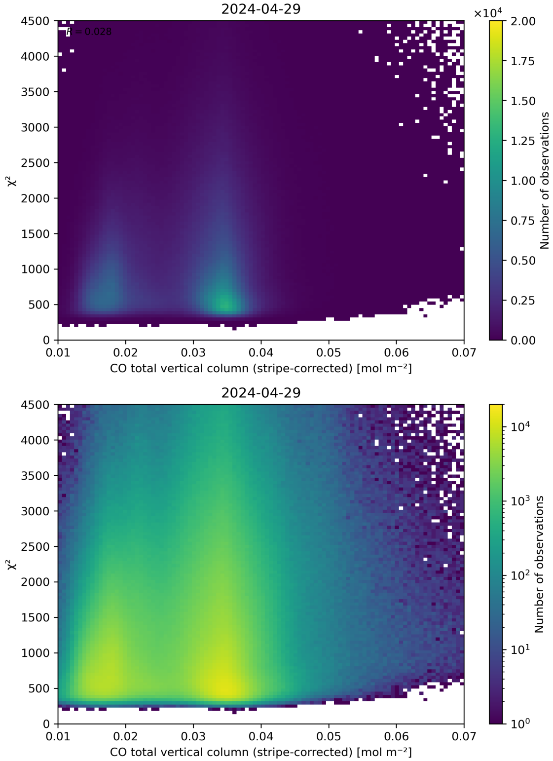
Figure 37: Scatter density plot of “CO total vertical column (stripe-corrected)” against “ \chi^2 ” for 2024-04-28 to 2024-04-30.
