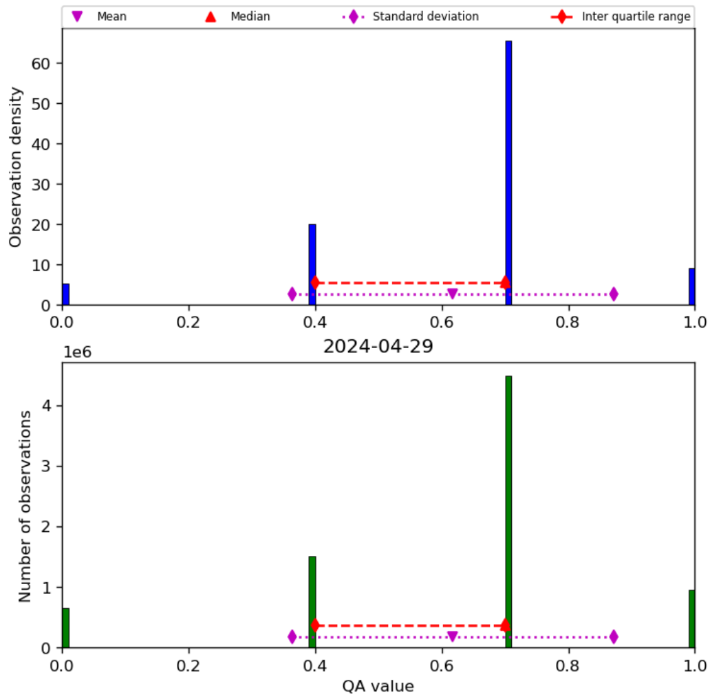
Figure 17: Histogram of “QA value” for 2024-04-28 to 2024-04-30
