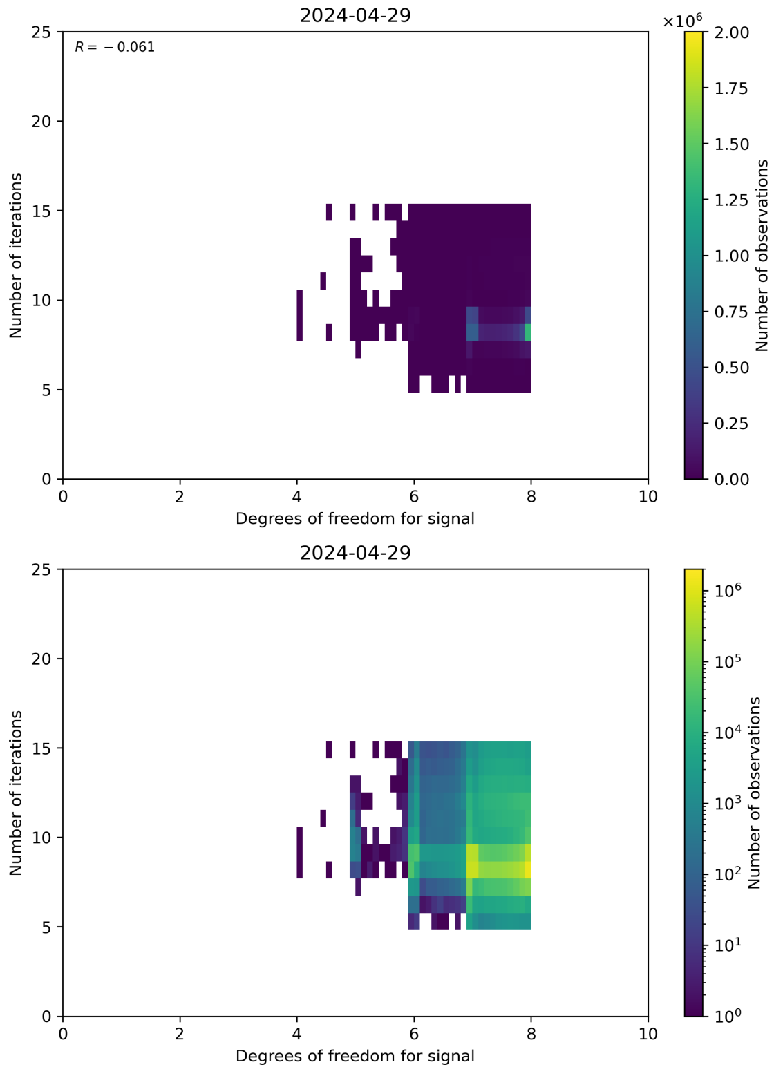
Figure 50: Scatter density plot of “Degrees of freedom for signal” against “Number of iterations” for 2024-04-28 to 2024-04-30.
