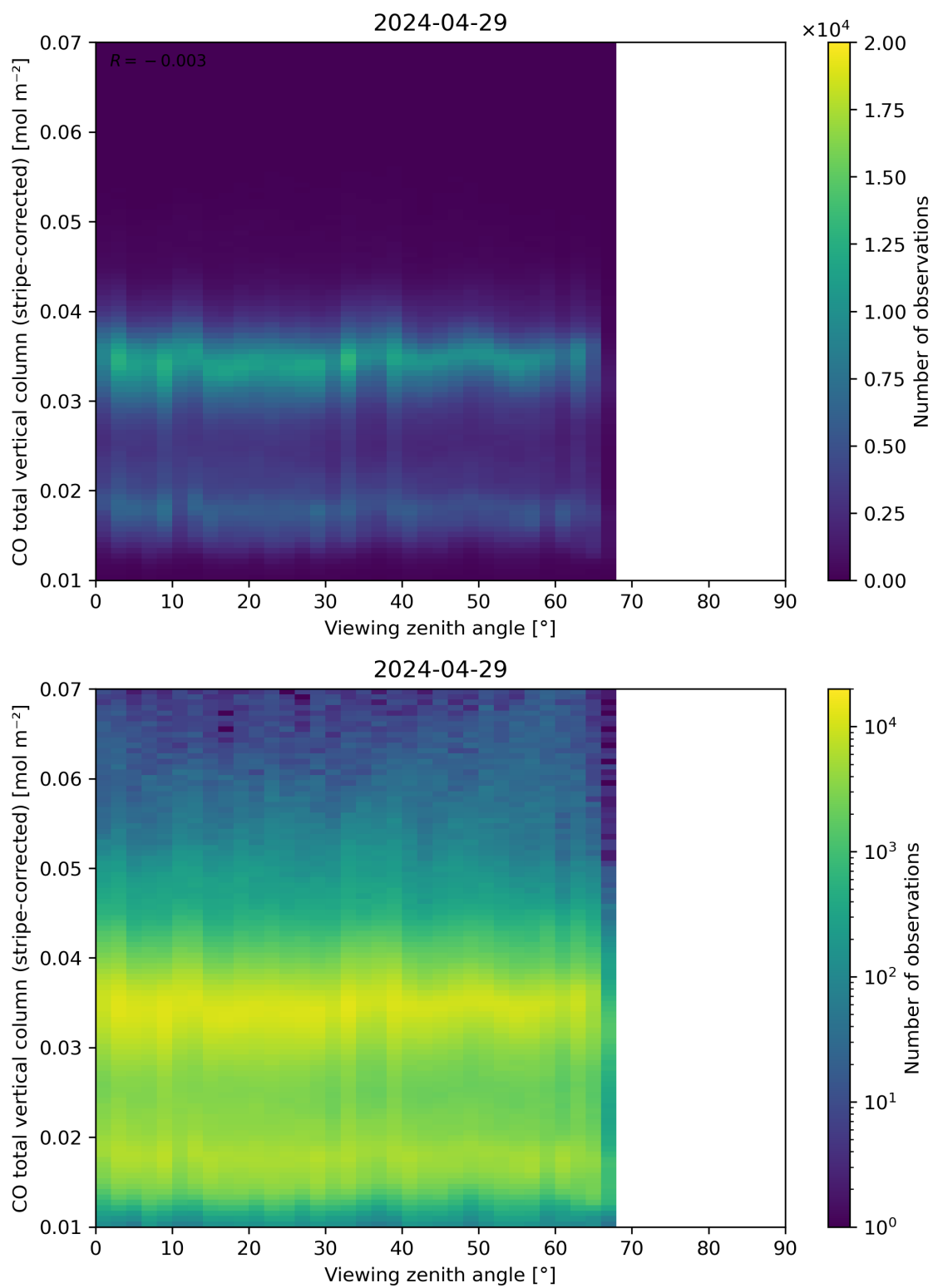
Figure 70: Scatter density plot of “Viewing zenith angle” against “CO total vertical column (stripe-corrected)” for 2024-04-28 to 2024-04-30.
