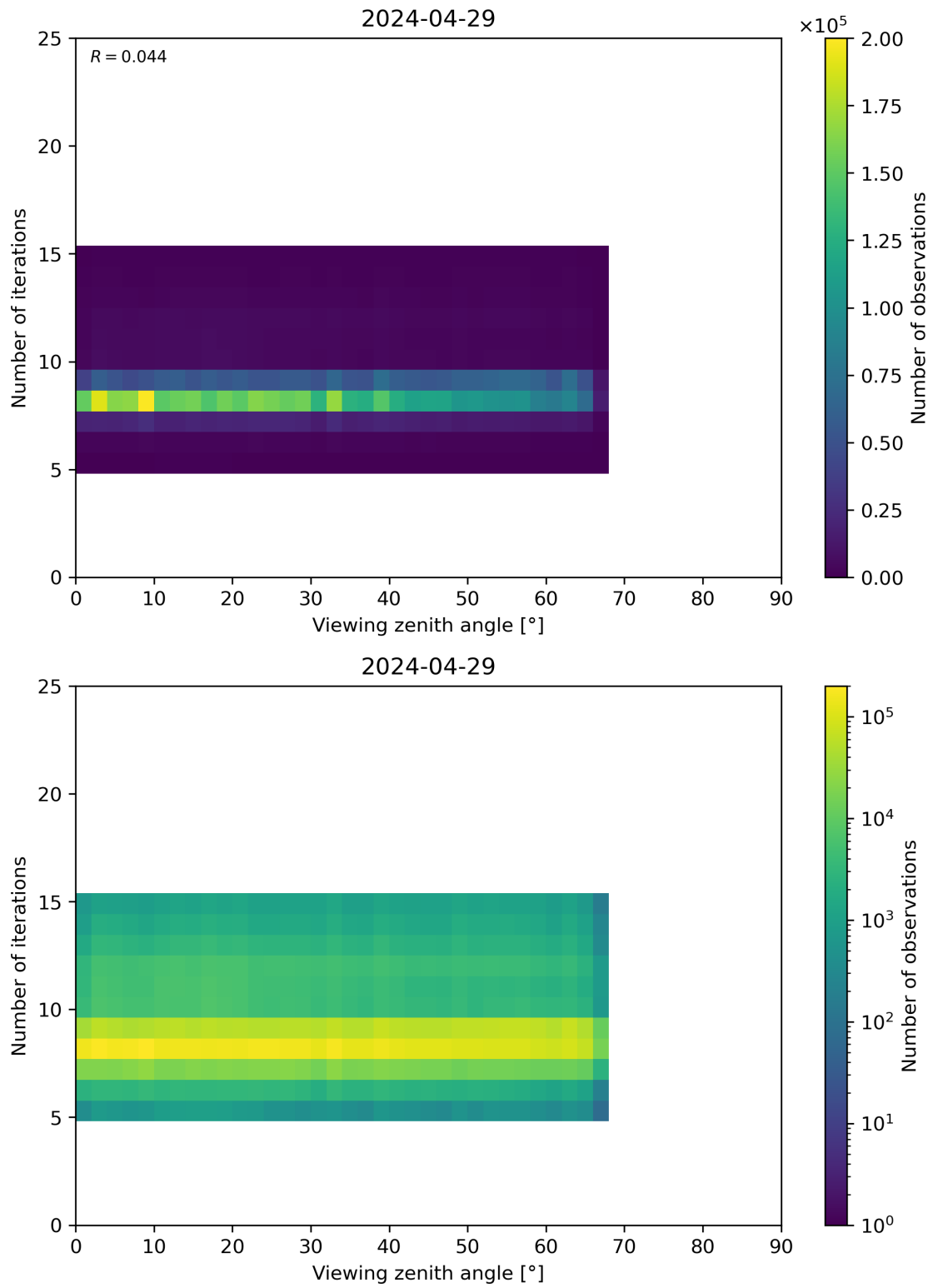
Figure 75: Scatter density plot of “Viewing zenith angle” against “Number of iterations” for 2024-04-28 to 2024-04-30.
