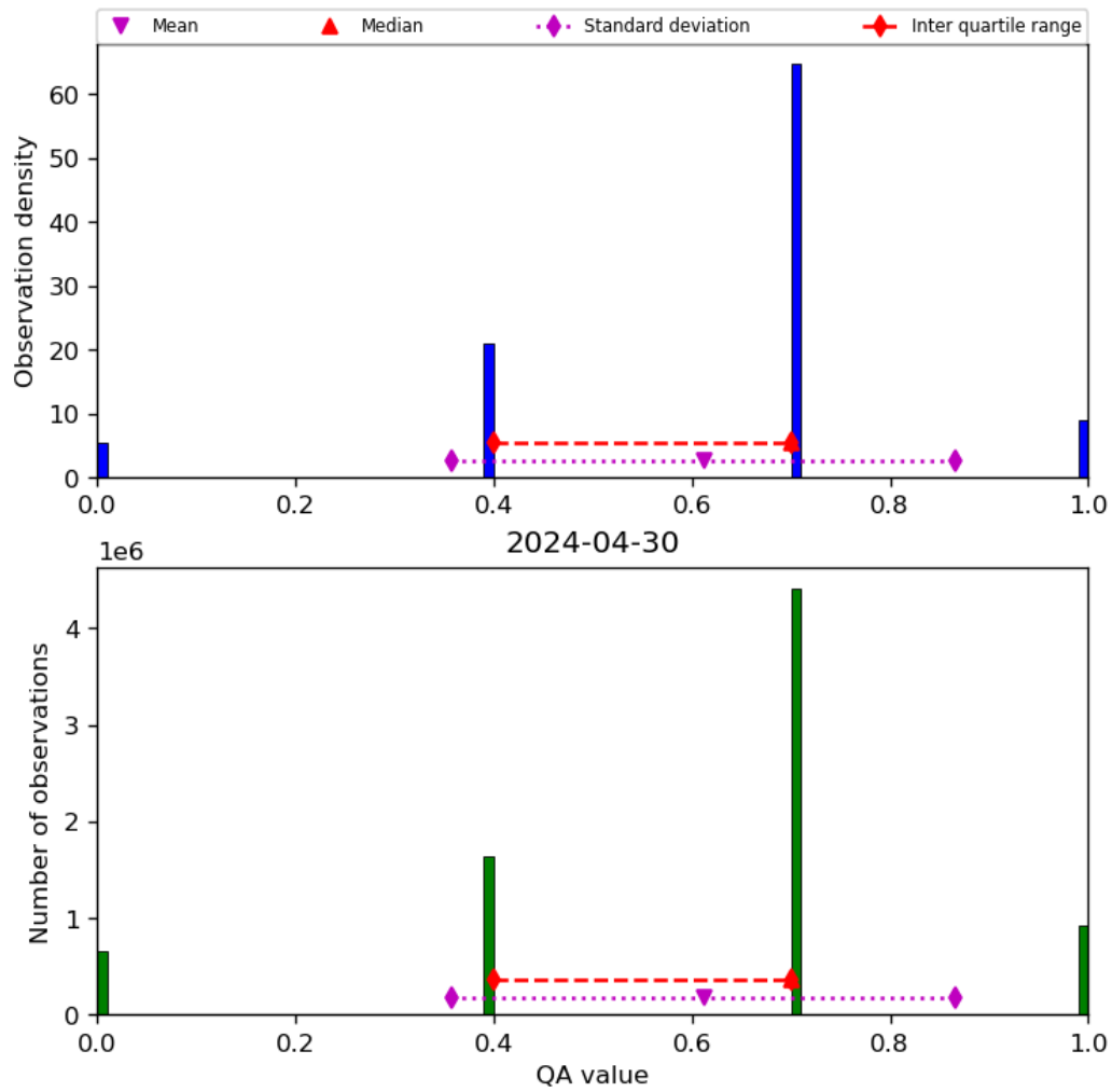
Figure 17: Histogram of “QA value” for 2024-04-29 to 2024-05-01
