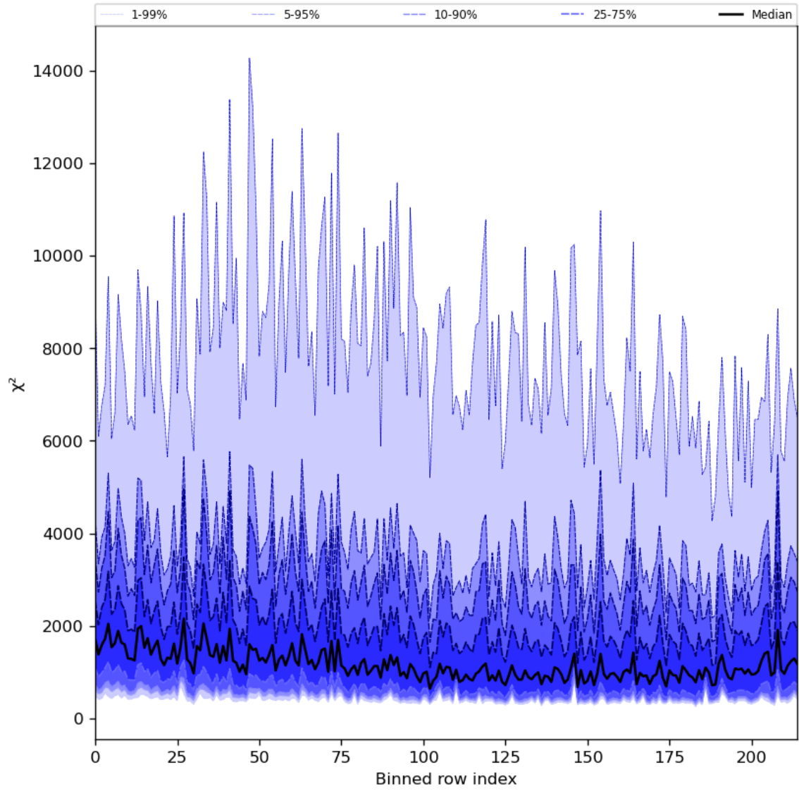
Figure 30: Along track statistics of “ \chi^2 ” for 2024-04-29 to 2024-05-01
