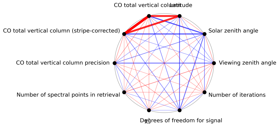
Figure 1: Map of correlation graph for 2024-04-29 to 2024-05-01.
