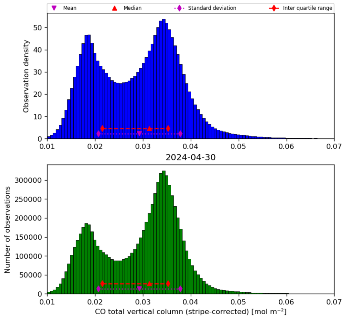
Figure 19: Histogram of “CO total vertical column (stripe-corrected)” for 2024-04-29 to 2024-05-01
