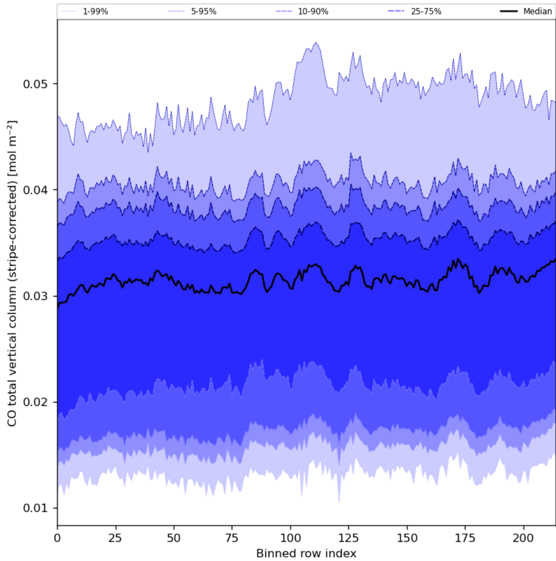
Figure 27: Along track statistics of “CO total vertical column (stripe-corrected)” for 2024-04-29 to 2024-05-01
