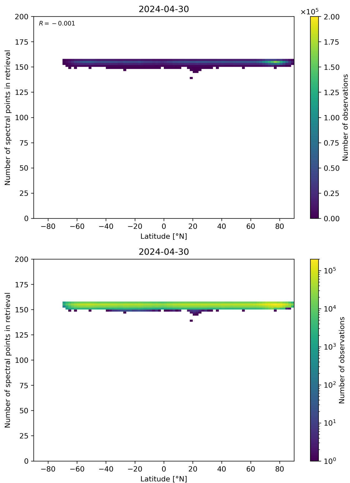
Figure 57: Scatter density plot of “Latitude” against “Number of spectral points in retrieval” for 2024-04-29 to 2024-05-01.
