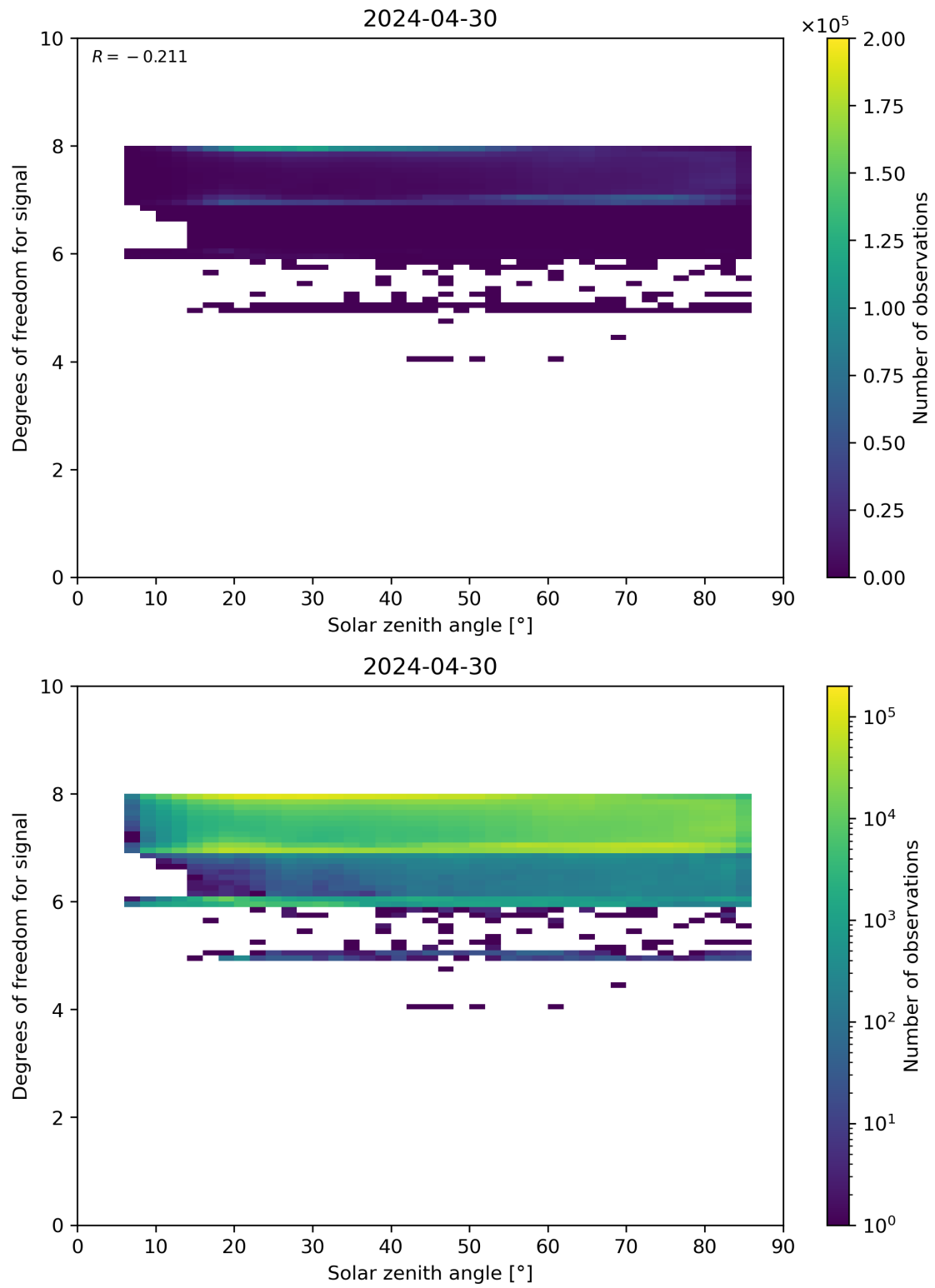
Figure 65: Scatter density plot of “Solar zenith angle” against “Degrees of freedom for signal” for 2024-04-29 to 2024-05-01.
