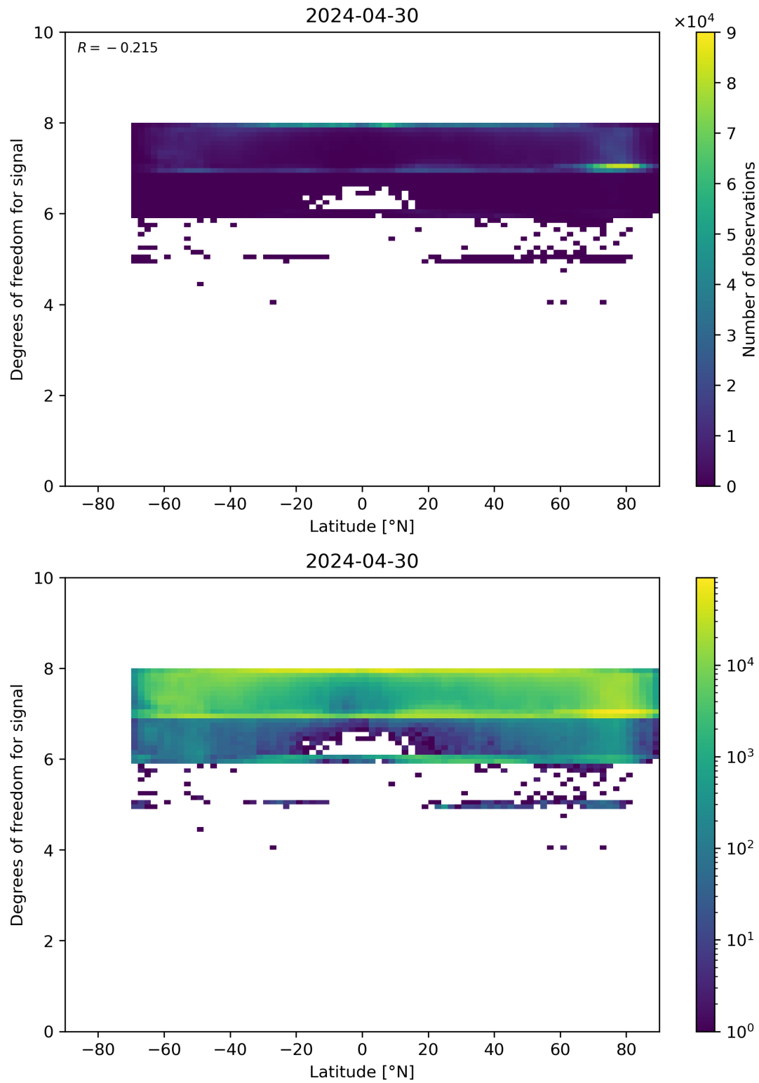
Figure 55: Scatter density plot of “Latitude” against “Degrees of freedom for signal” for 2024-04-29 to 2024-05-01.
