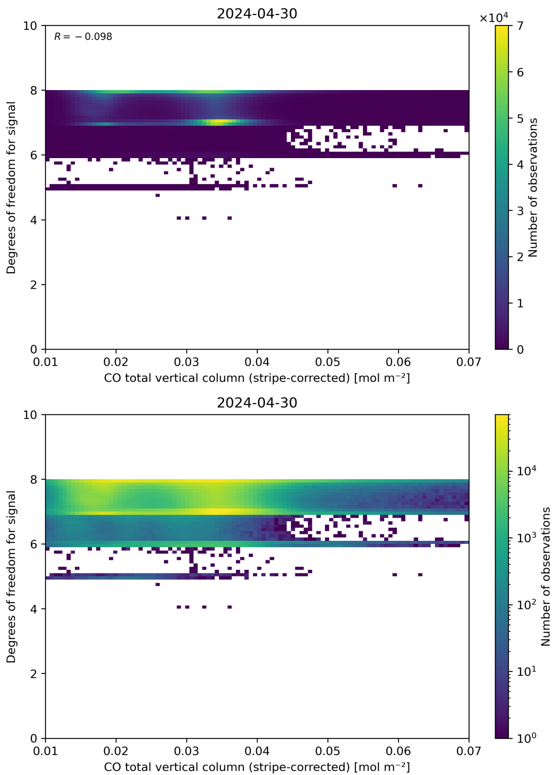
Figure 38: Scatter density plot of “CO total vertical column (stripe-corrected)” against “Degrees of freedom for signal” for 2024-04-29 to 2024-05-01.
