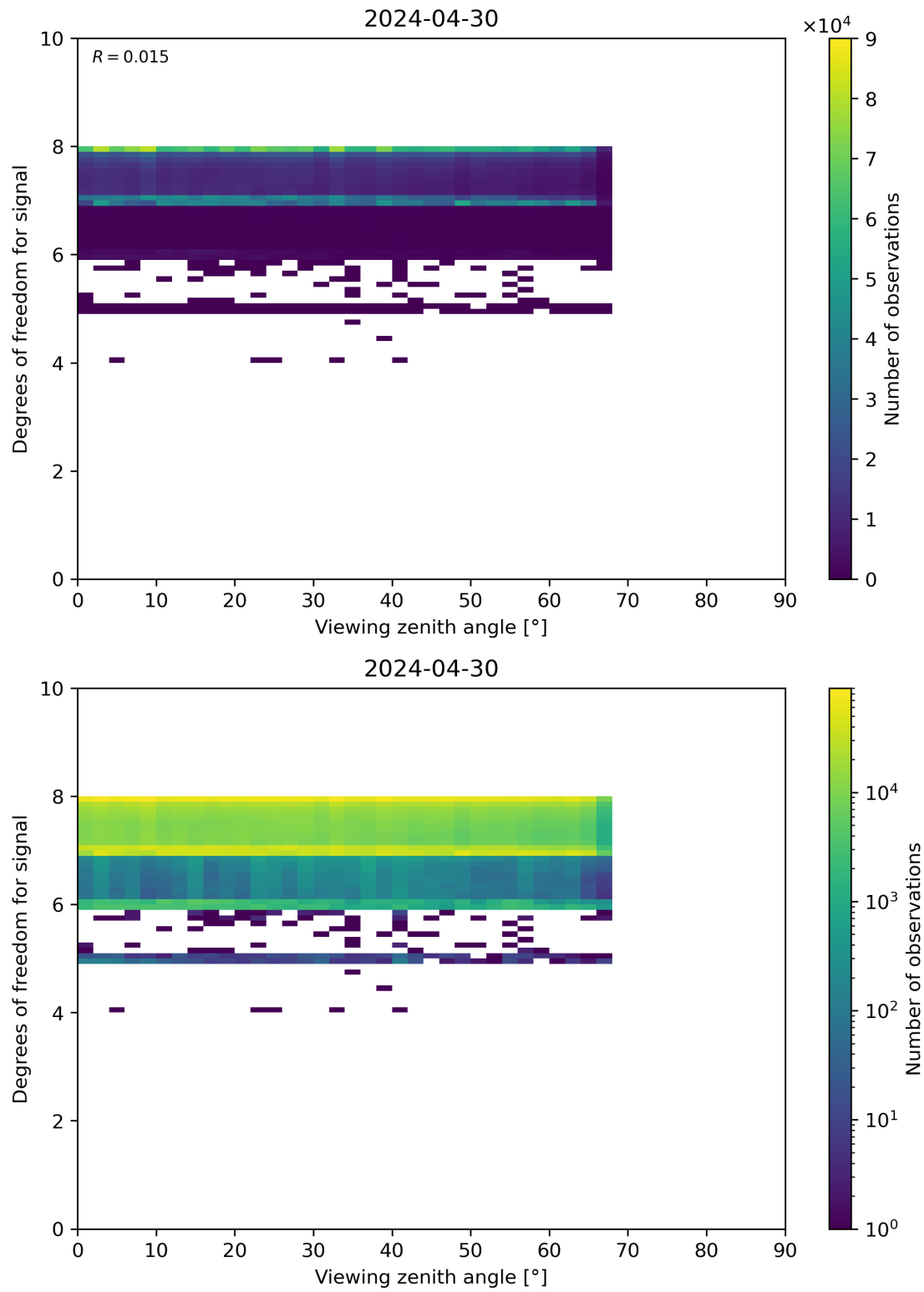
Figure 73: Scatter density plot of “Viewing zenith angle” against “Degrees of freedom for signal” for 2024-04-29 to 2024-05-01.
