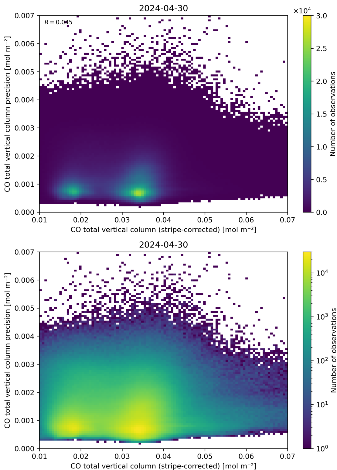
Figure 36: Scatter density plot of “CO total vertical column (stripe-corrected)” against “CO total vertical column precision” for 2024-04-29 to 2024-05-01.
