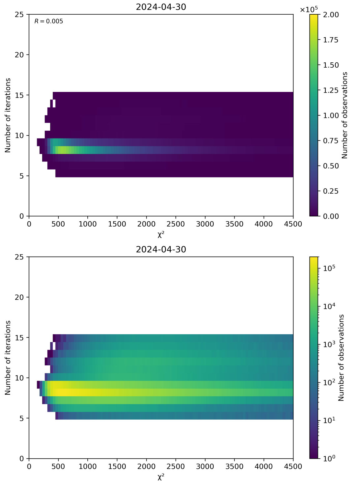
Figure 49: Scatter density plot of “ \chi^2 ” against “Number of iterations” for 2024-04-29 to 2024-05-01.
