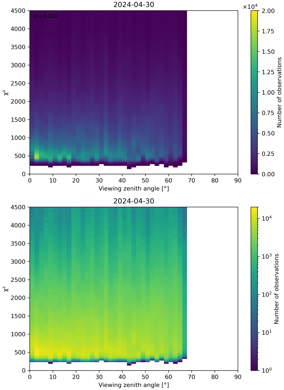
Figure 72: Scatter density plot of “Viewing zenith angle” against “ \chi^2 ” for 2024-04-29 to 2024-05-01.
