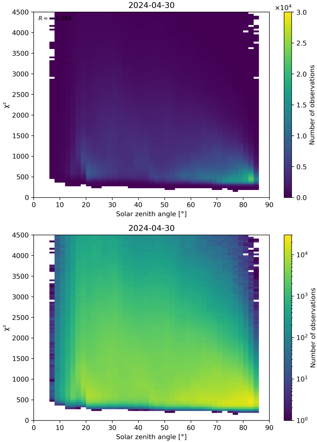
Figure 64: Scatter density plot of “Solar zenith angle” against “ \chi^2 ” for 2024-04-29 to 2024-05-01.
