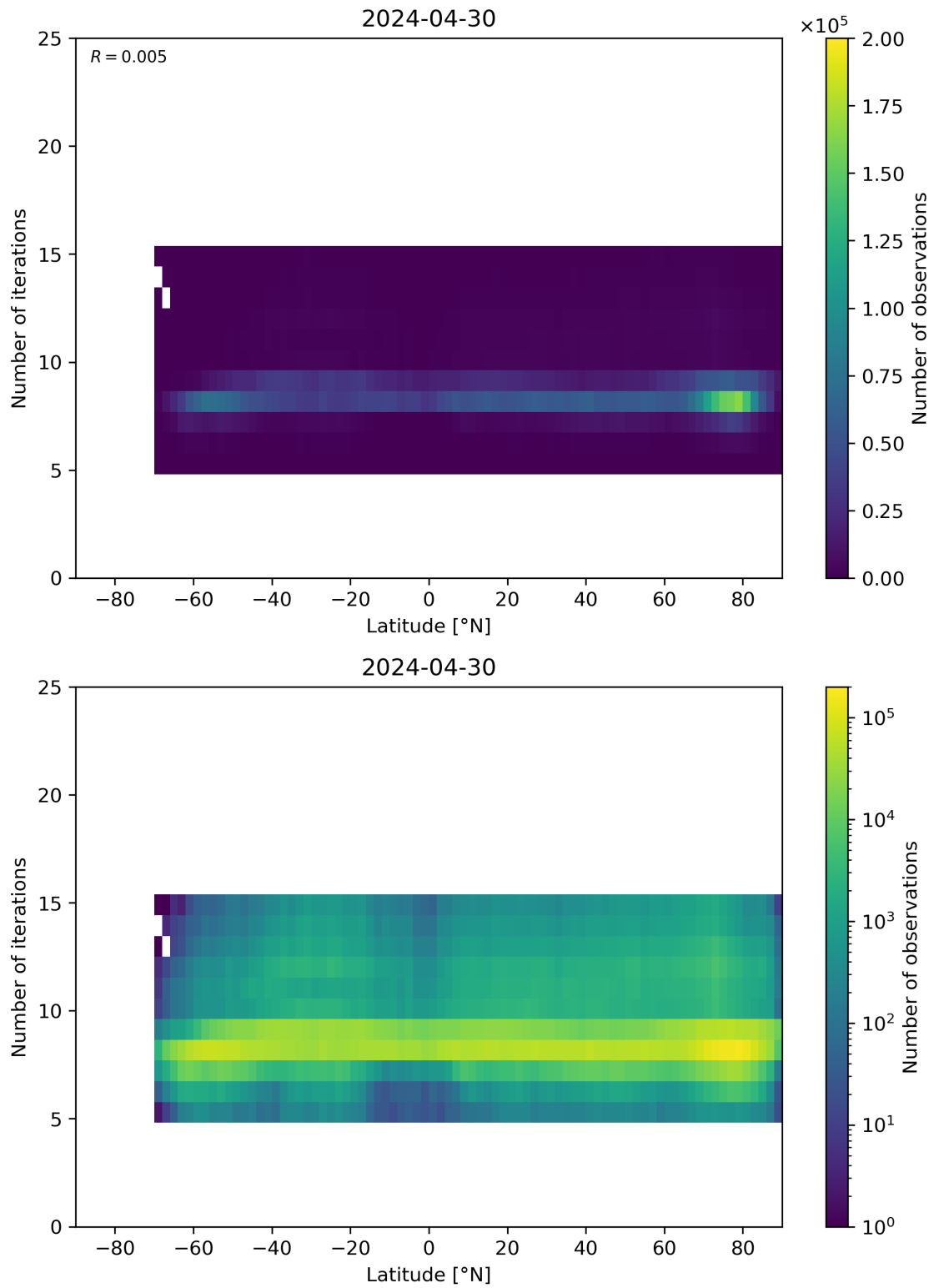
Figure 56: Scatter density plot of “Latitude” against “Number of iterations” for 2024-04-29 to 2024-05-01.
