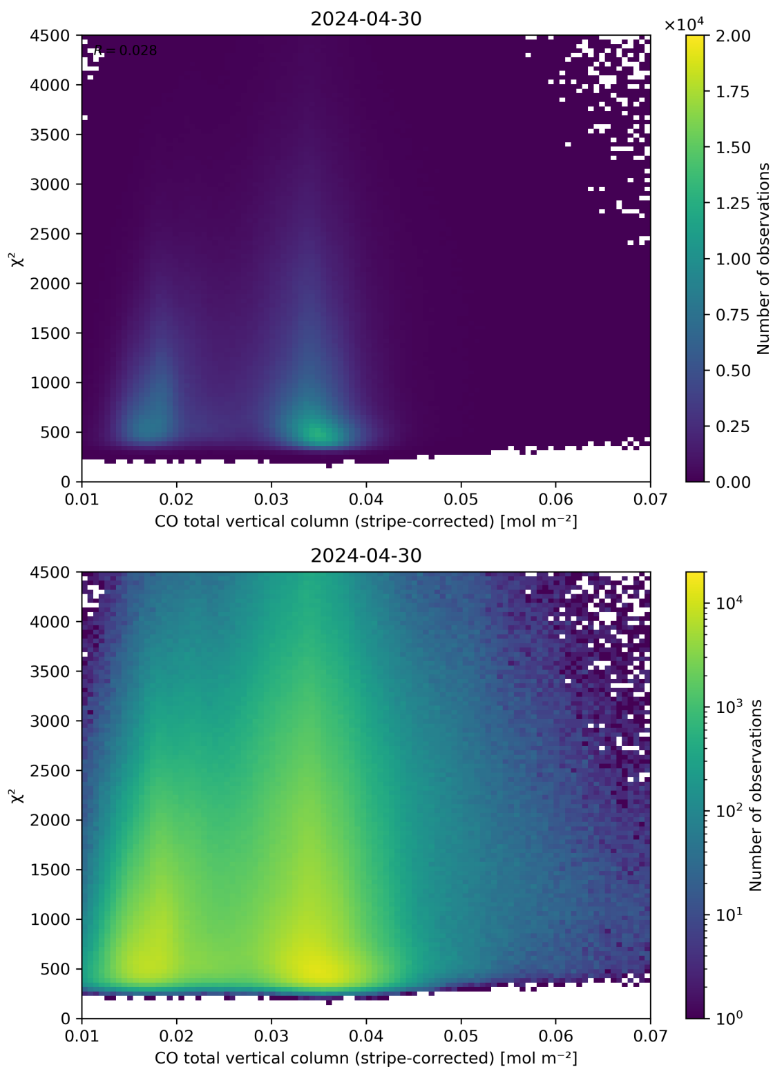
Figure 37: Scatter density plot of “CO total vertical column (stripe-corrected)” against “ \chi^2 ” for 2024-04-29 to 2024-05-01.
