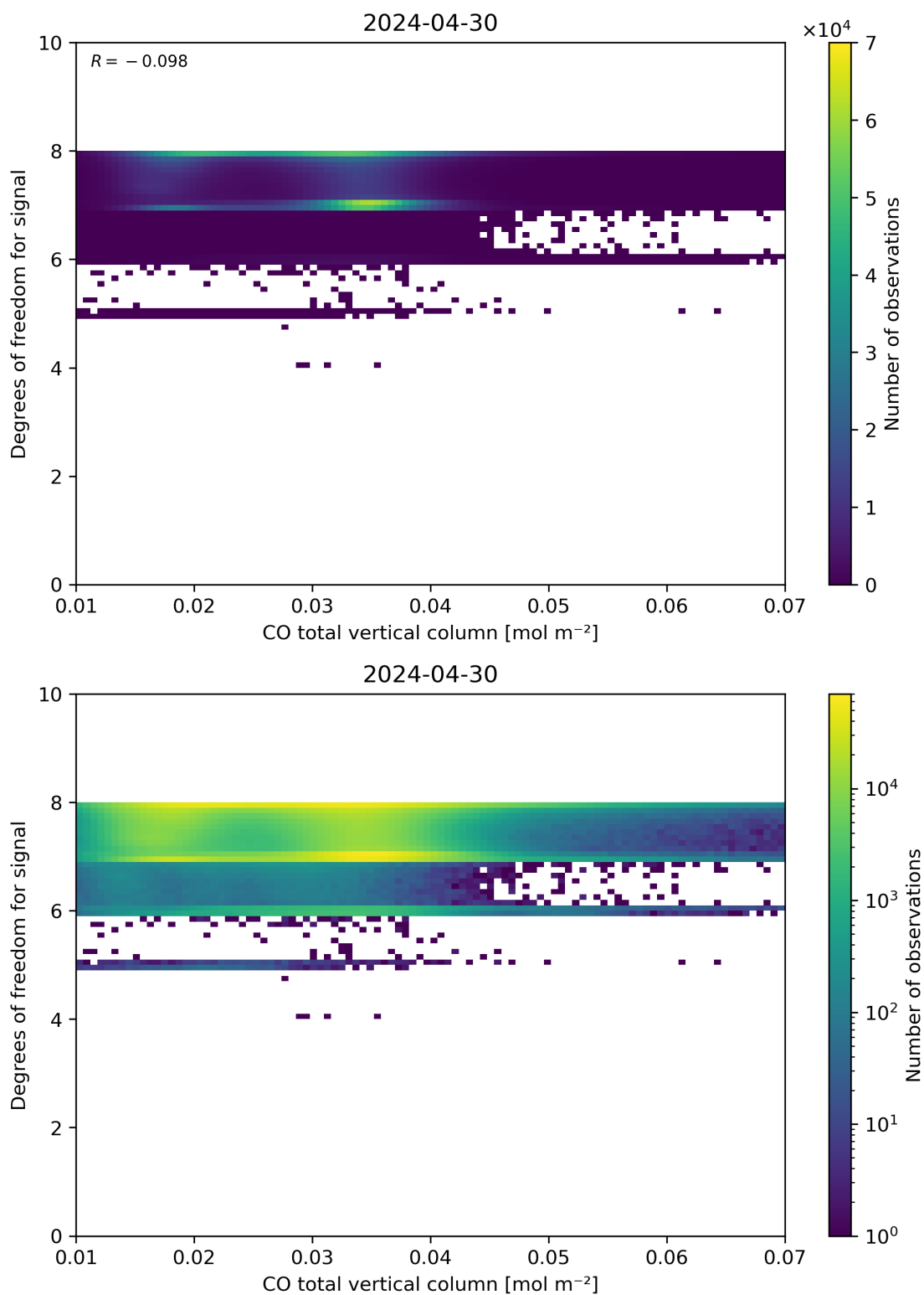
Figure 41: Scatter density plot of “CO total vertical column” against “Degrees of freedom for signal” for 2024-04-29 to 2024-05-01.
