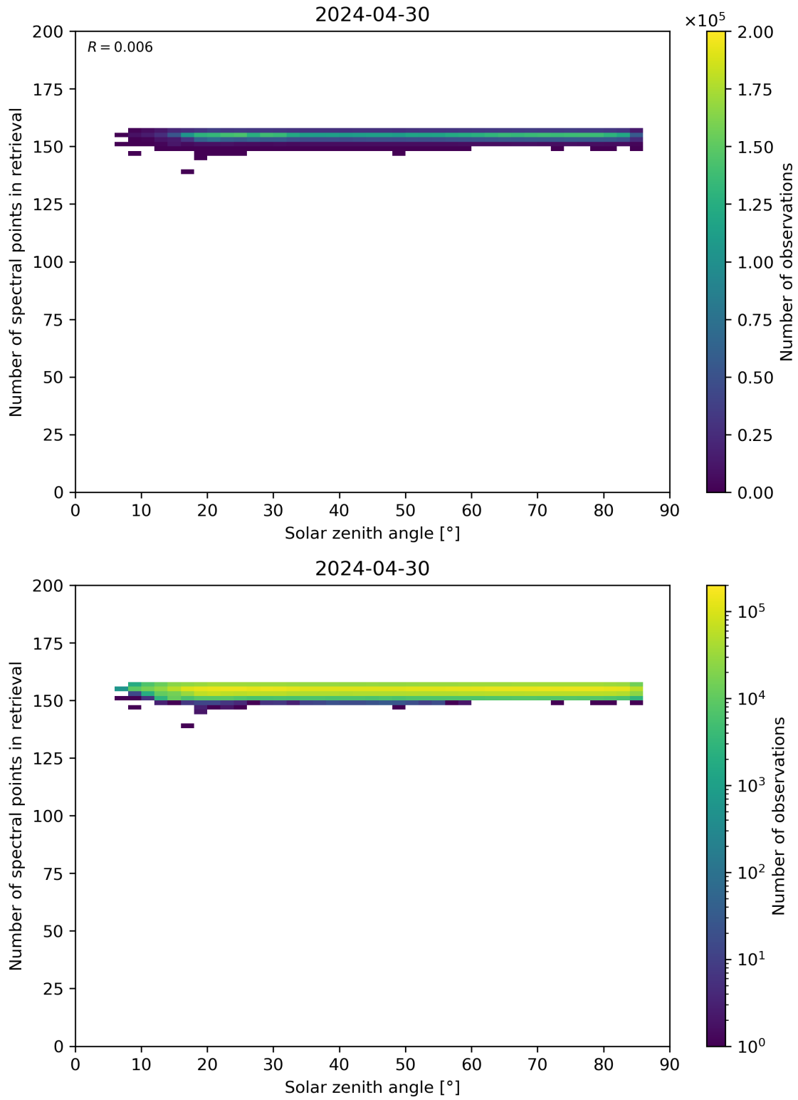
Figure 68: Scatter density plot of “Solar zenith angle” against “Number of spectral points in retrieval” for 2024-04-29 to 2024-05-01.
