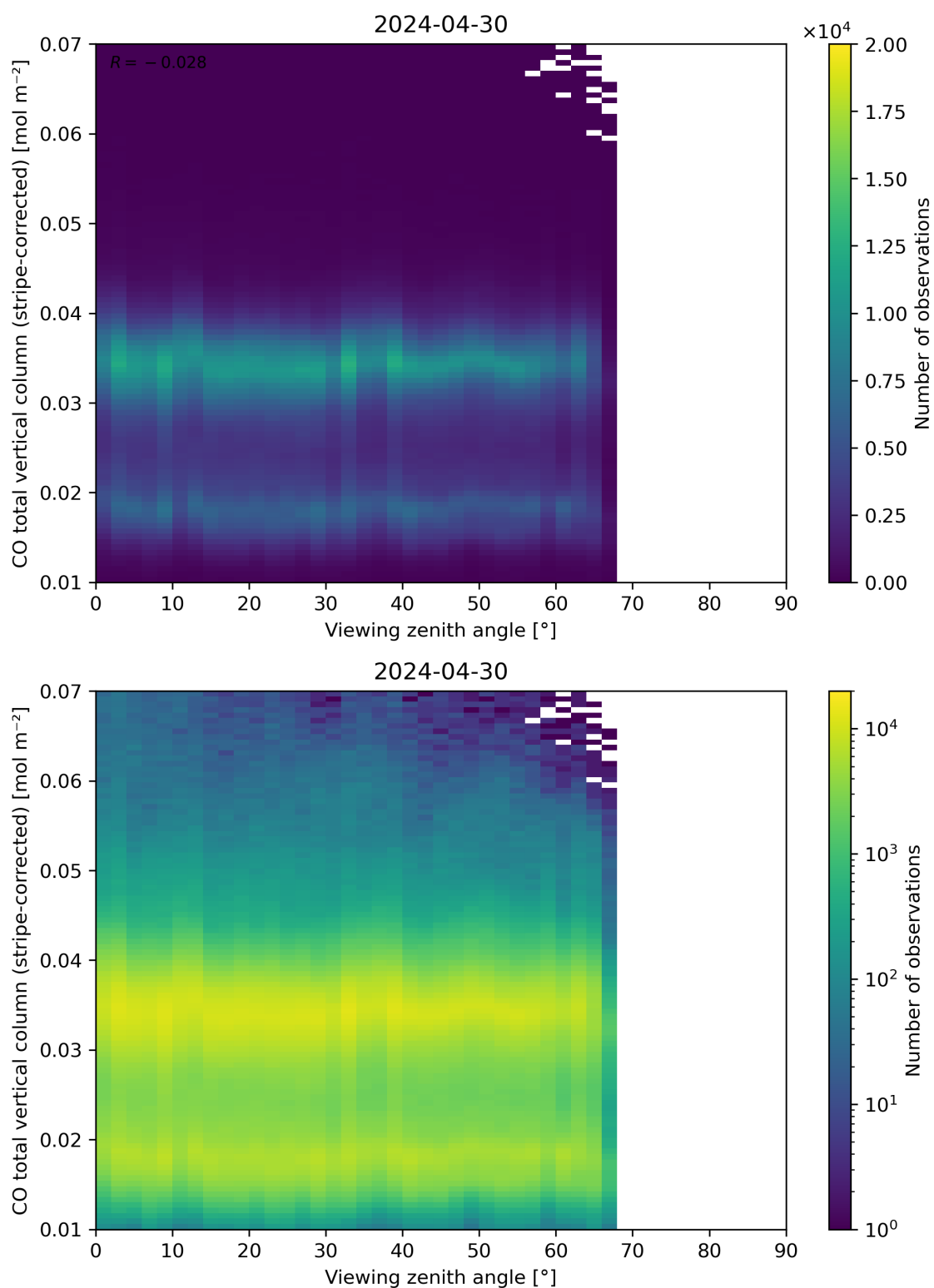
Figure 70: Scatter density plot of “Viewing zenith angle” against “CO total vertical column (stripe-corrected)” for 2024-04-29 to 2024-05-01.
