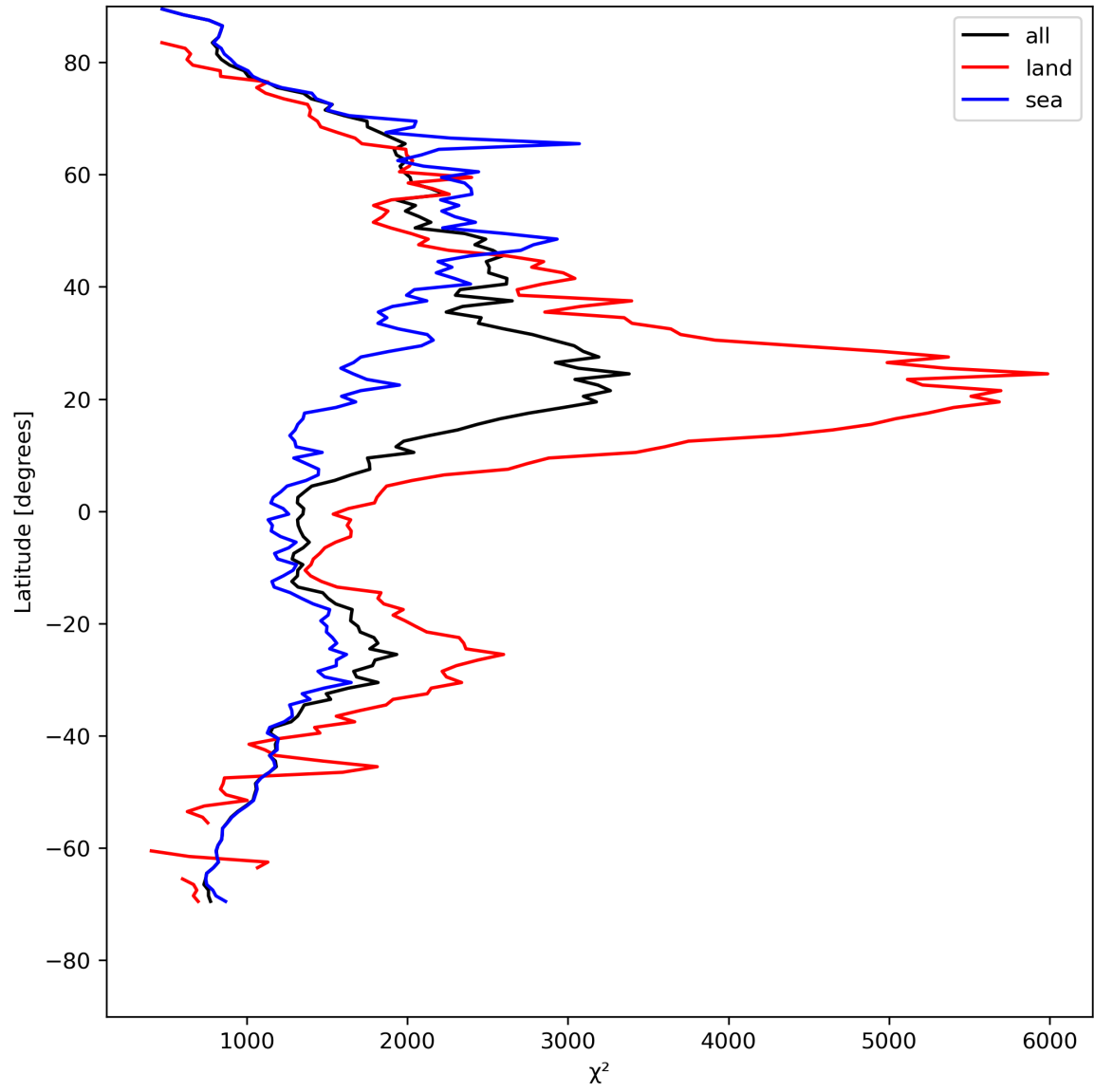
Figure 14: Zonal average of “ \chi^2 ” for 2024-04-29 to 2024-05-01.
