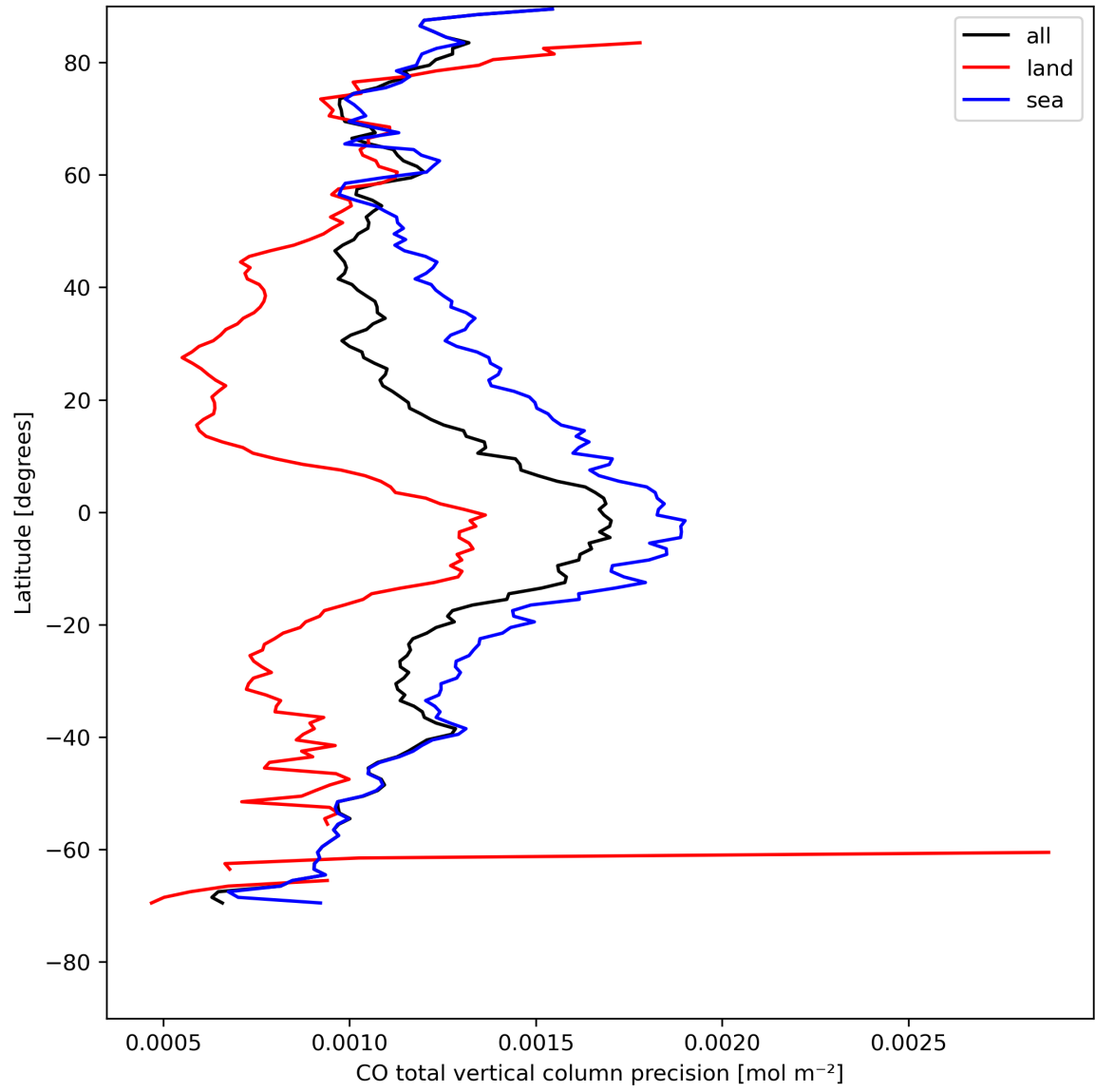
Figure 12: Zonal average of “CO total vertical column precision” for 2024-04-29 to 2024-05-01.
