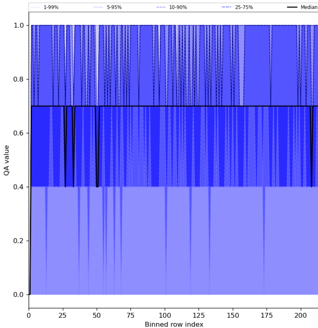
Figure 25: Along track statistics of “QA value” for 2024-04-29 to 2024-05-01
