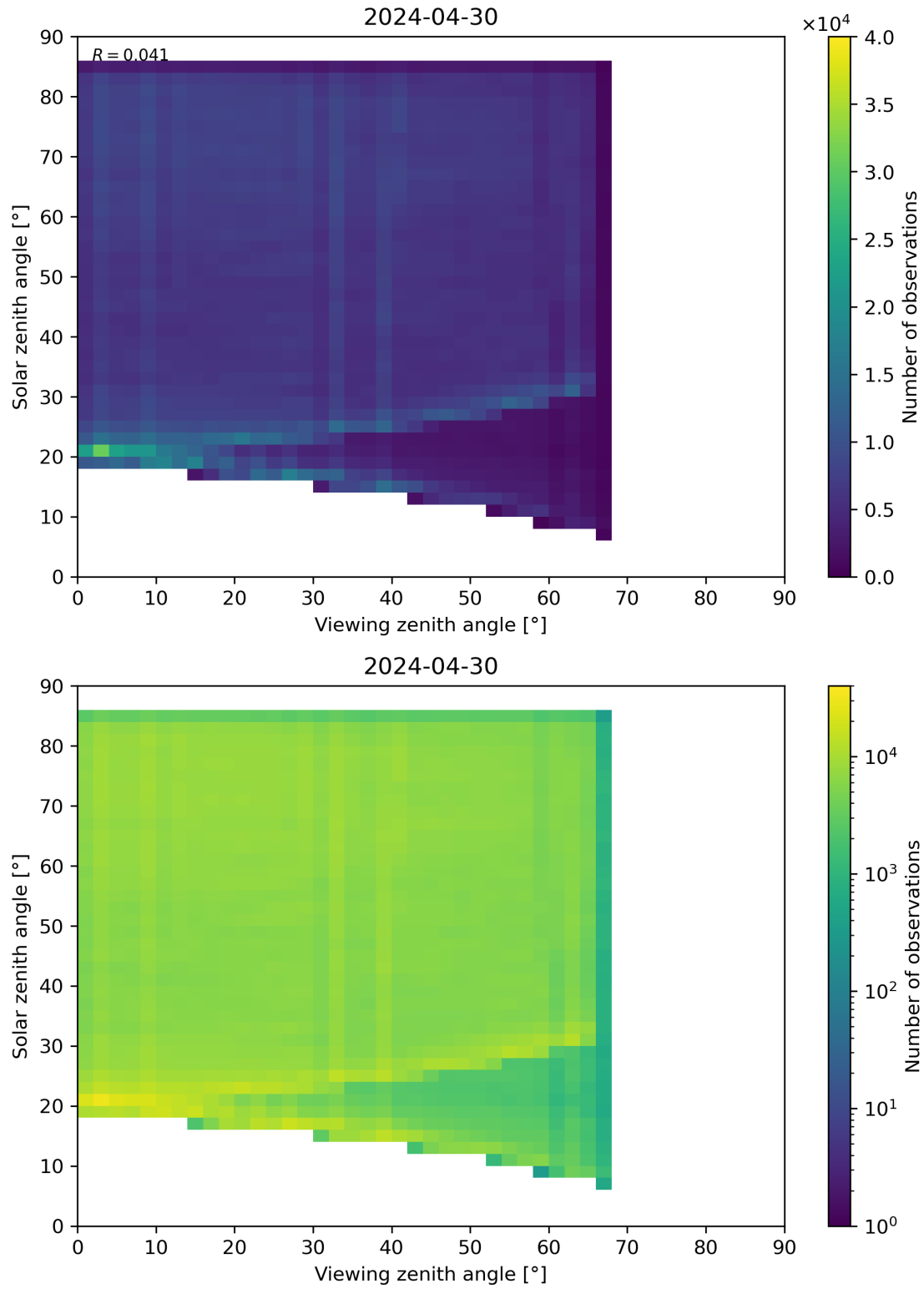
Figure 77: Scatter density plot of “Viewing zenith angle” against “Solar zenith angle” for 2024-04-29 to 2024-05-01.
