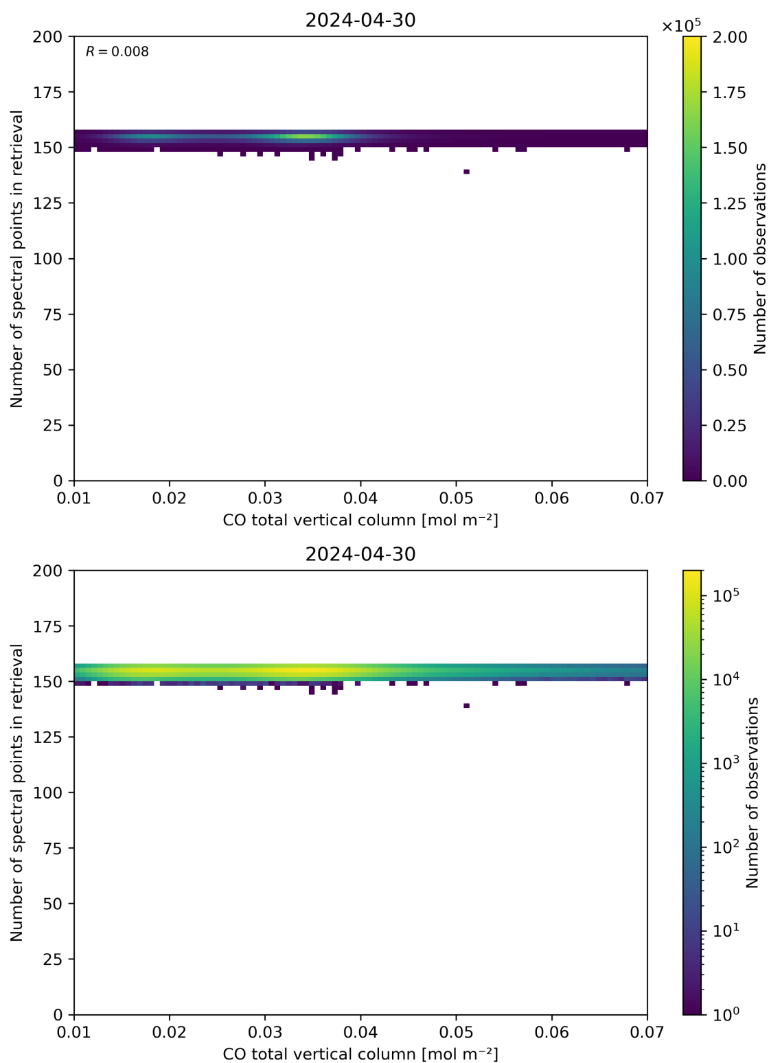
Figure 43: Scatter density plot of “CO total vertical column” against “Number of spectral points in retrieval” for 2024-04-29 to 2024-05-01.
