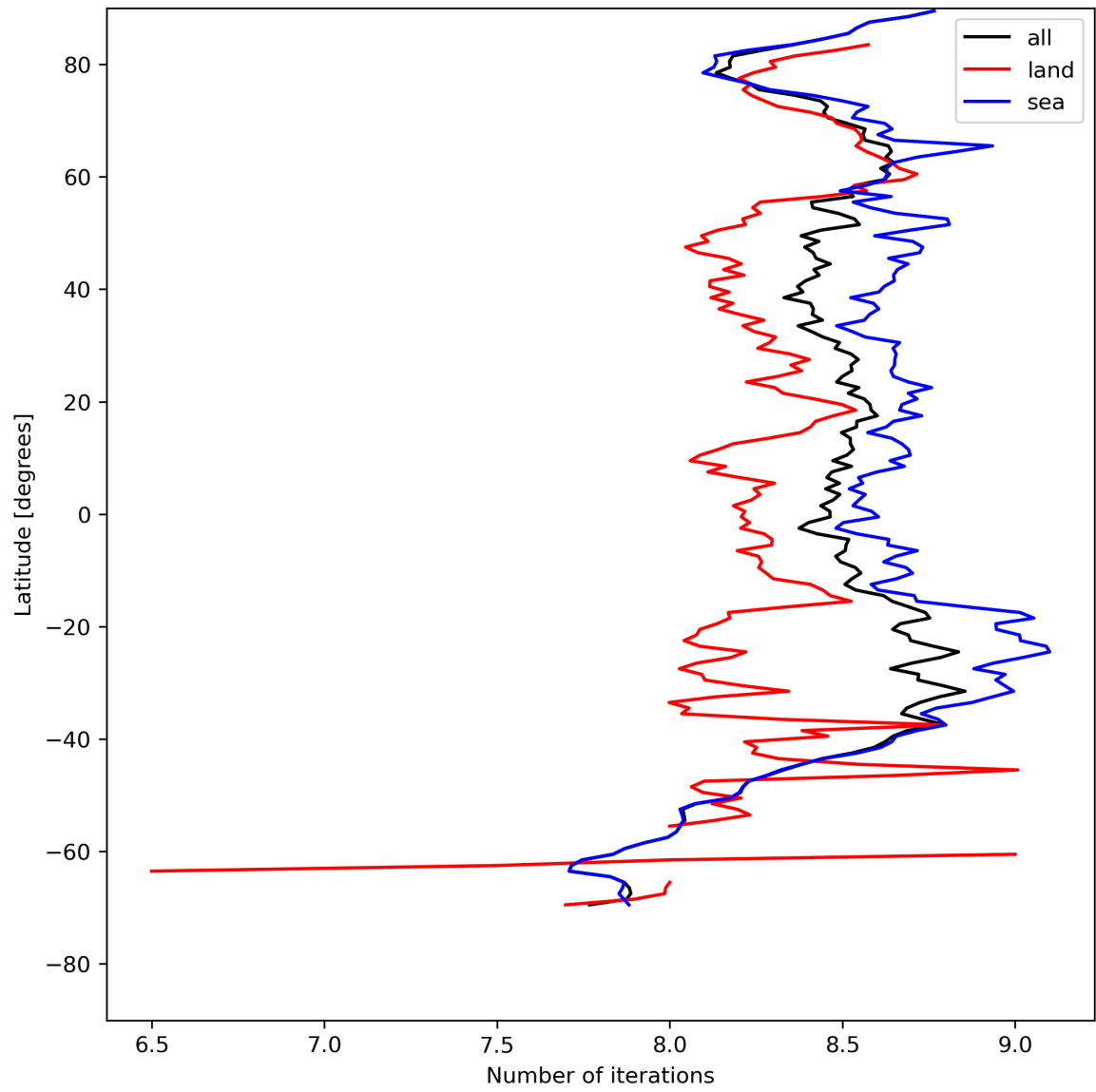
Figure 16: Zonal average of “Number of iterations” for 2024-04-29 to 2024-05-01.
