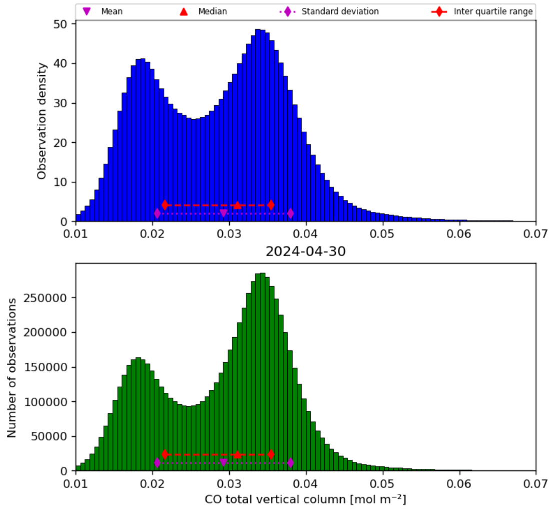
Figure 18: Histogram of “CO total vertical column” for 2024-04-29 to 2024-05-01
