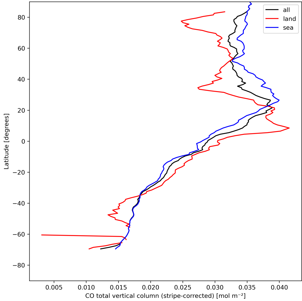
Figure 11: Zonal average of “CO total vertical column (stripe-corrected)” for 2024-04-29 to 2024-05-01.
