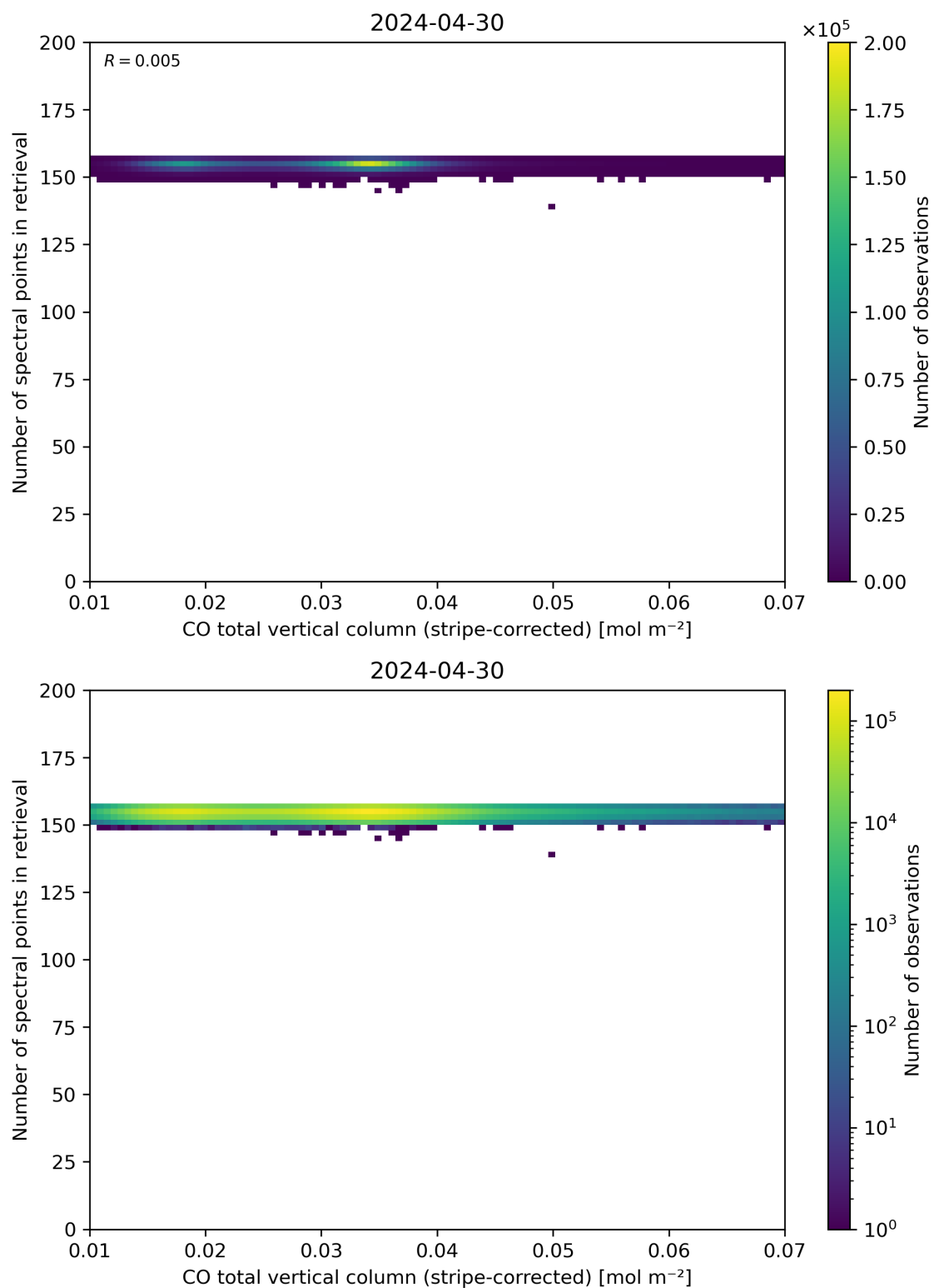
Figure 40: Scatter density plot of “CO total vertical column (stripe-corrected)” against “Number of spectral points in retrieval” for 2024-04-29 to 2024-05-01.
