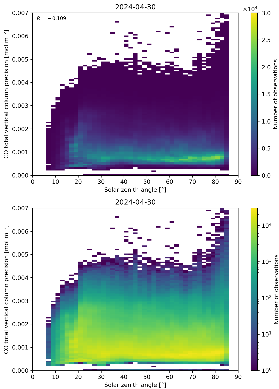
Figure 63: Scatter density plot of “Solar zenith angle” against “CO total vertical column precision” for 2024-04-29 to 2024-05-01.
