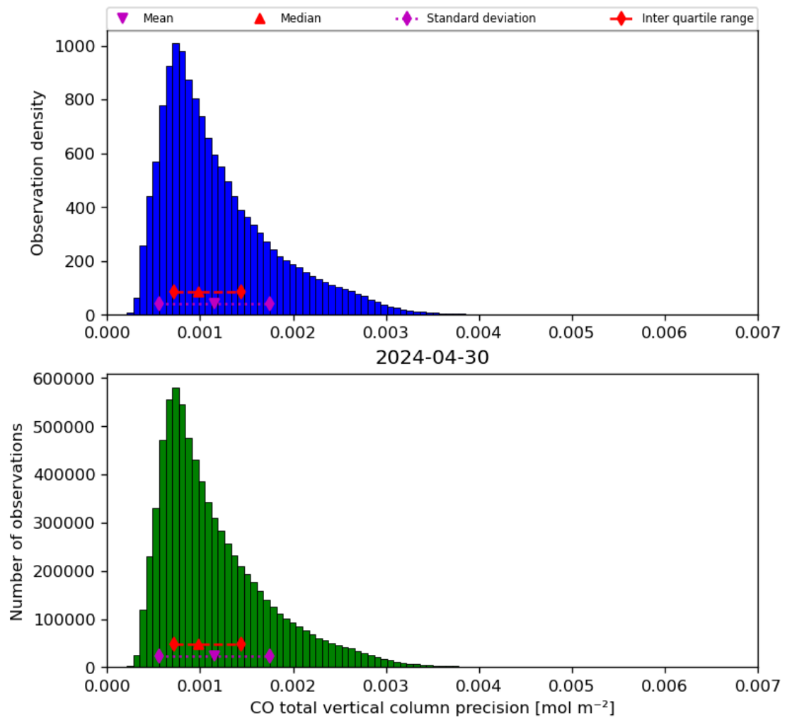
Figure 20: Histogram of “CO total vertical column precision” for 2024-04-29 to 2024-05-01
