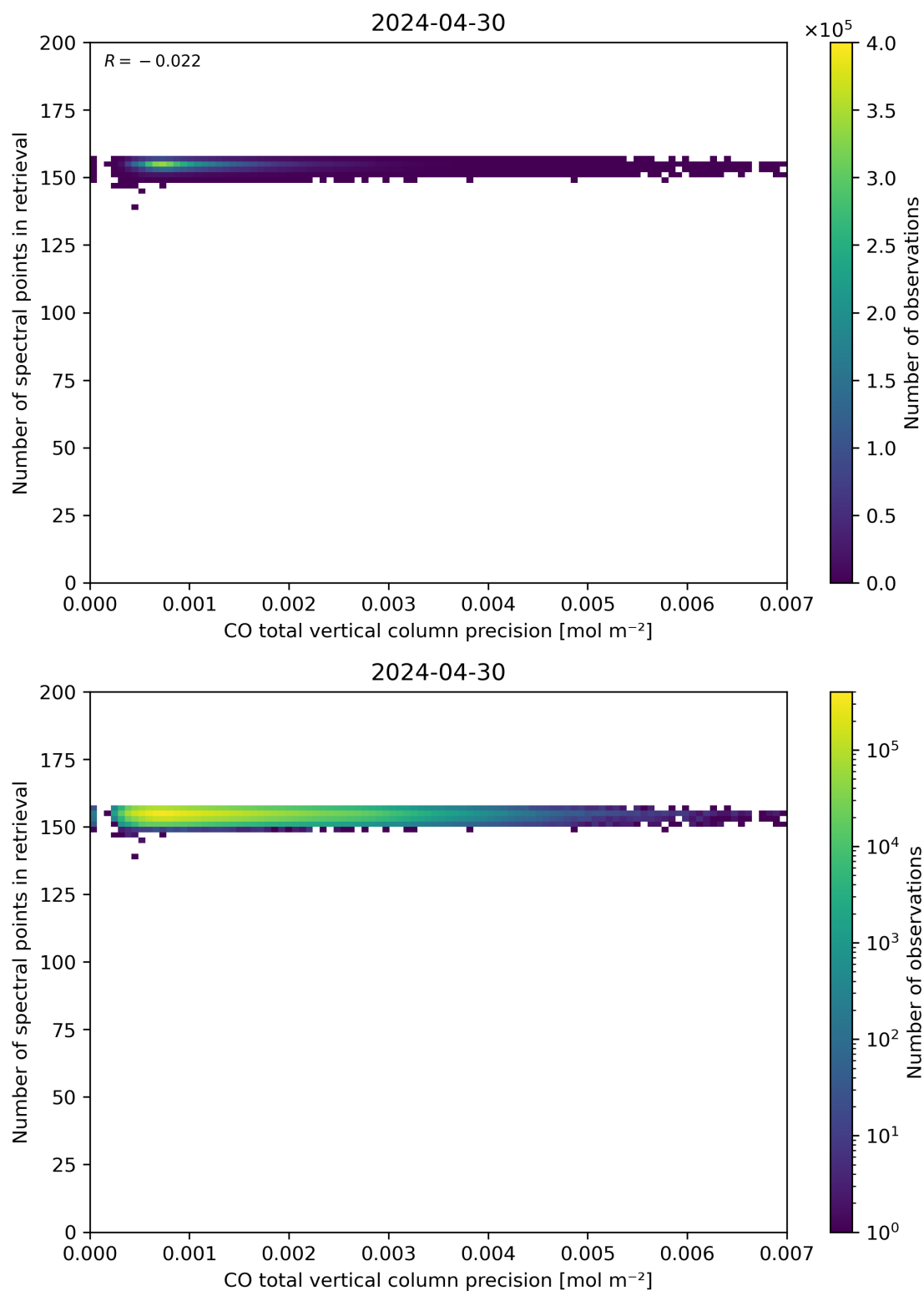
Figure 47: Scatter density plot of “CO total vertical column precision” against “Number of spectral points in retrieval” for 2024-04-29 to 2024-05-01.
