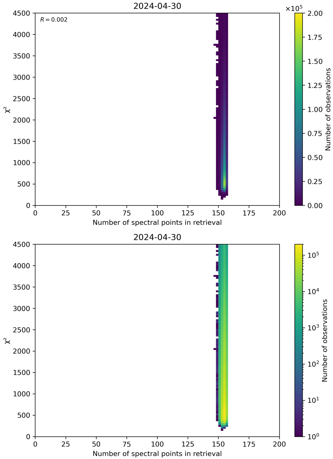
Figure 58: Scatter density plot of “Number of spectral points in retrieval” against “ \chi^2 ” for 2024-04-29 to 2024-05-01.
