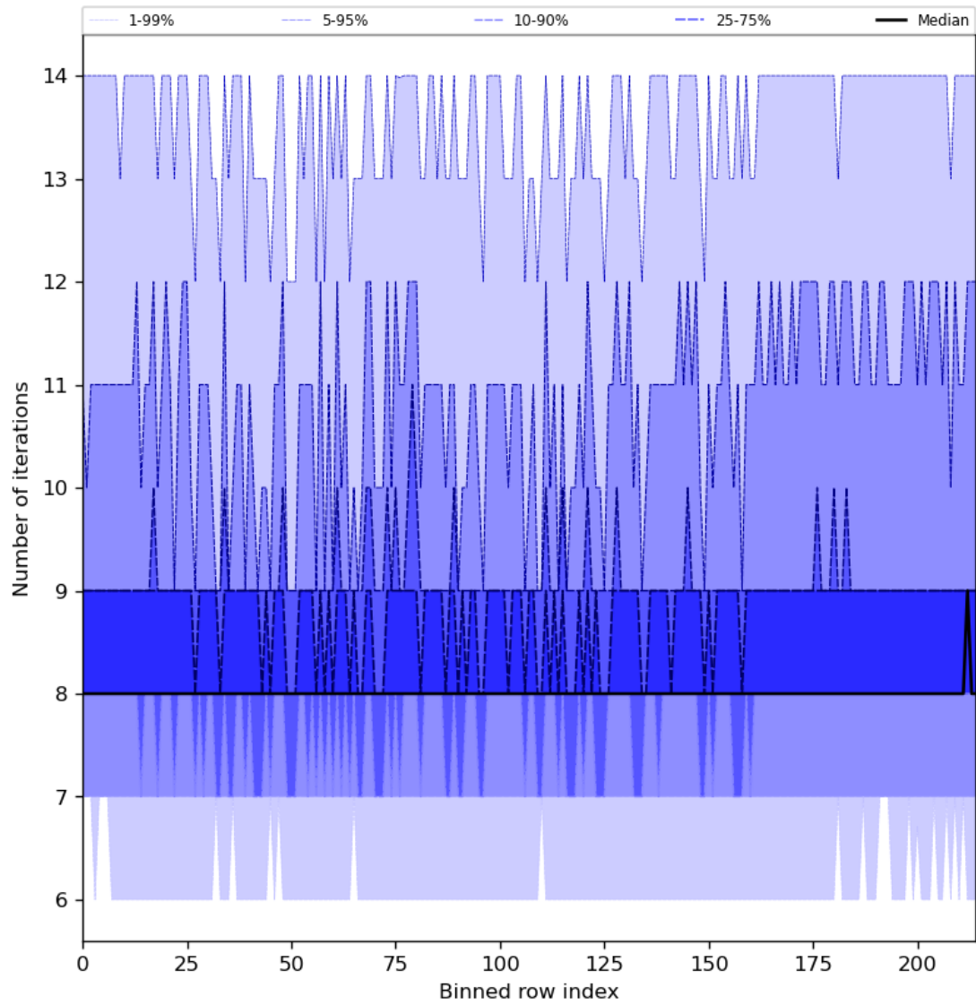
Figure 32: Along track statistics of “Number of iterations” for 2024-04-29 to 2024-05-01
