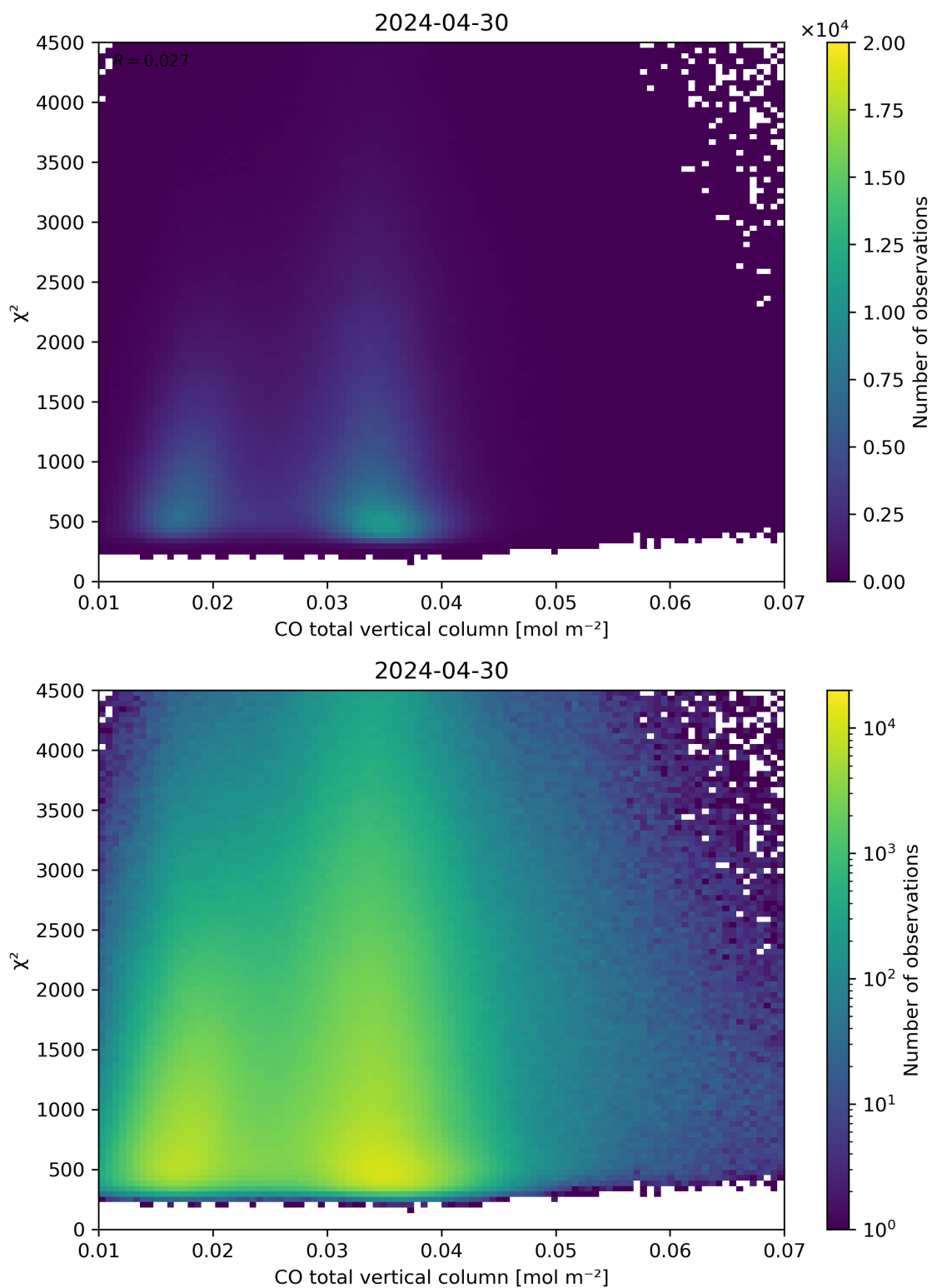
Figure 35: Scatter density plot of “CO total vertical column” against “ \chi^2 ” for 2024-04-29 to 2024-05-01.
