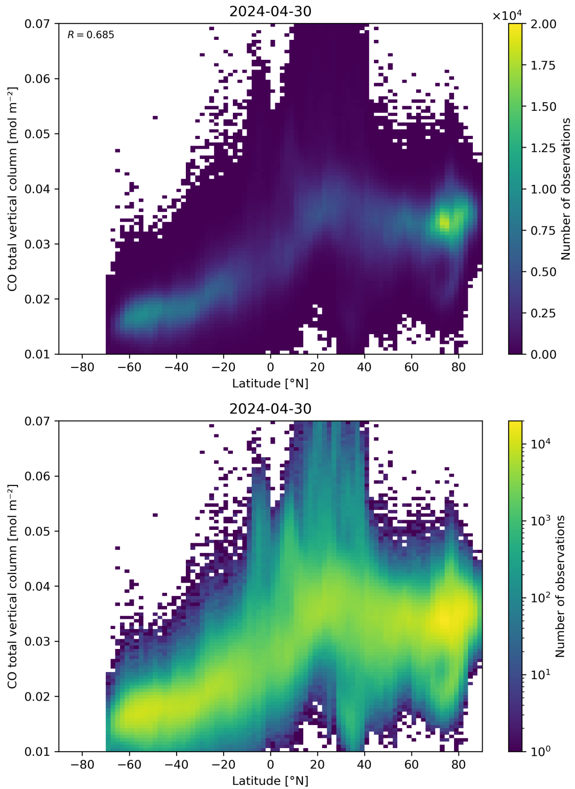
Figure 51: Scatter density plot of “Latitude” against “CO total vertical column” for 2024-04-29 to 2024-05-01.
