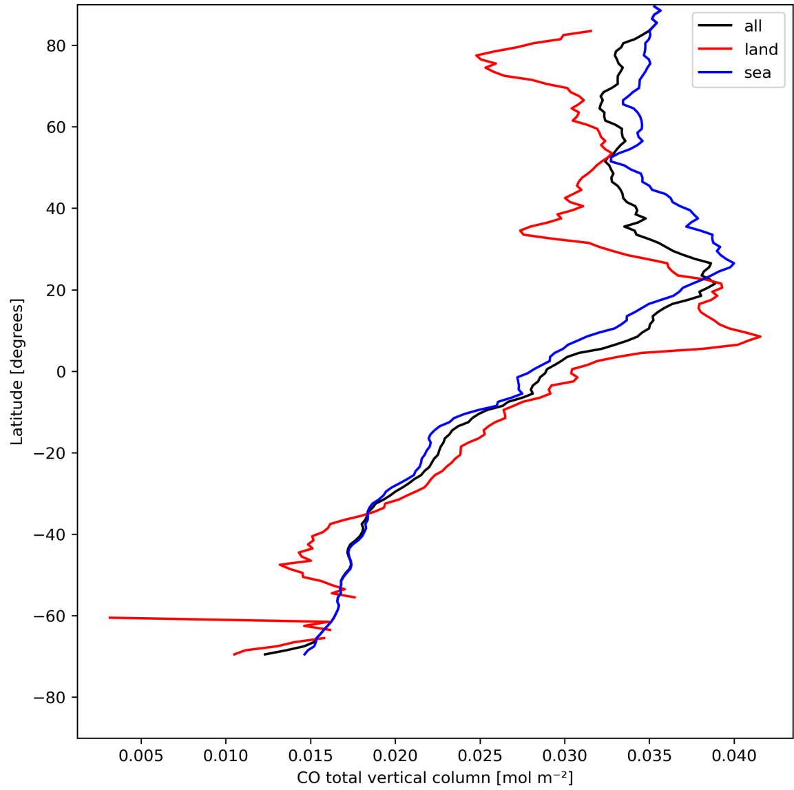
Figure 10: Zonal average of “CO total vertical column” for 2024-04-29 to 2024-05-01.
