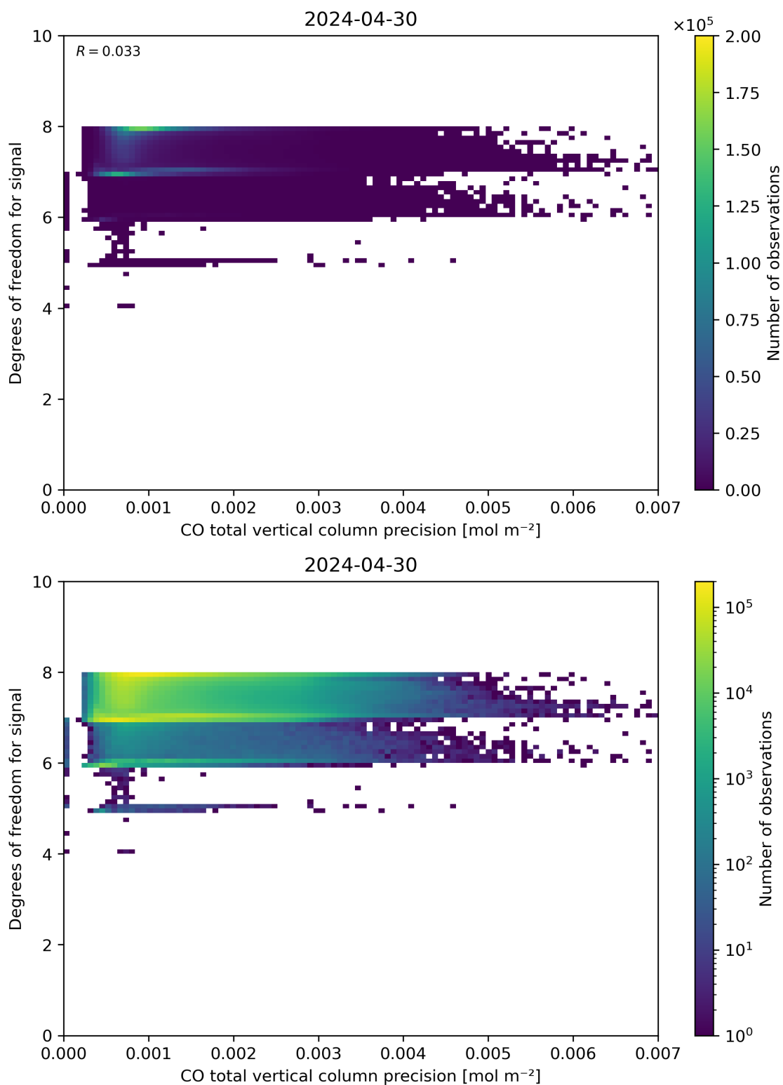
Figure 45: Scatter density plot of “CO total vertical column precision” against “Degrees of freedom for signal” for 2024-04-29 to 2024-05-01.
