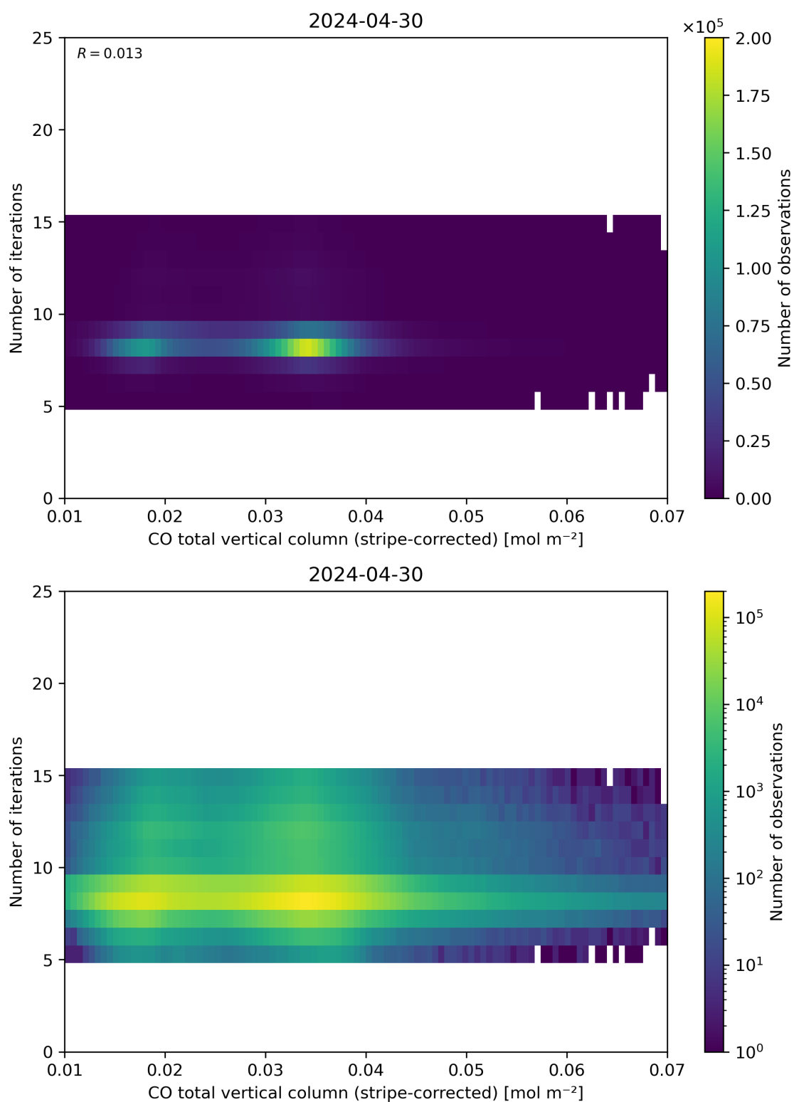
Figure 39: Scatter density plot of “CO total vertical column (stripe-corrected)” against “Number of iterations” for 2024-04-29 to 2024-05-01.
