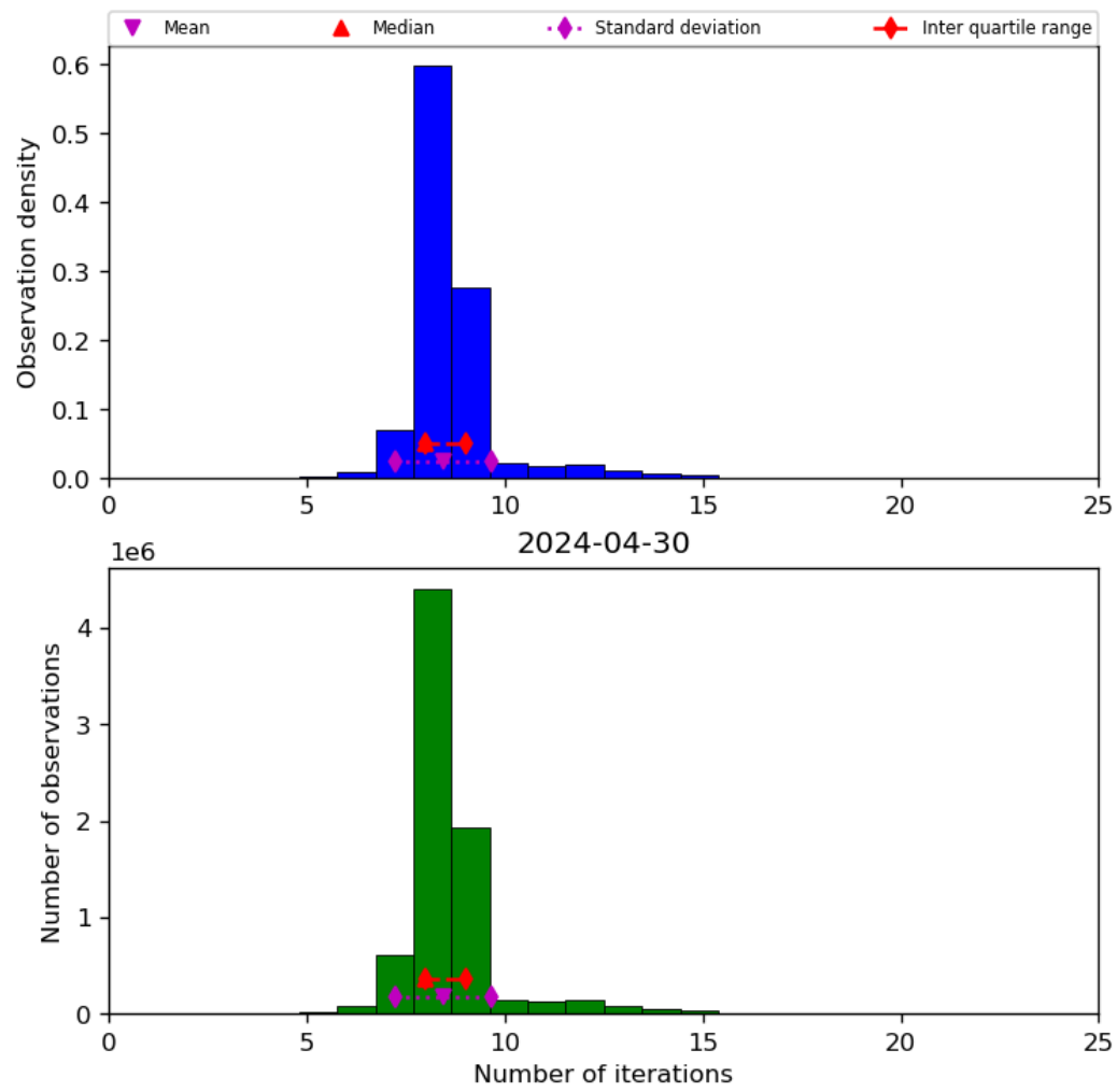
Figure 24: Histogram of “Number of iterations” for 2024-04-29 to 2024-05-01
