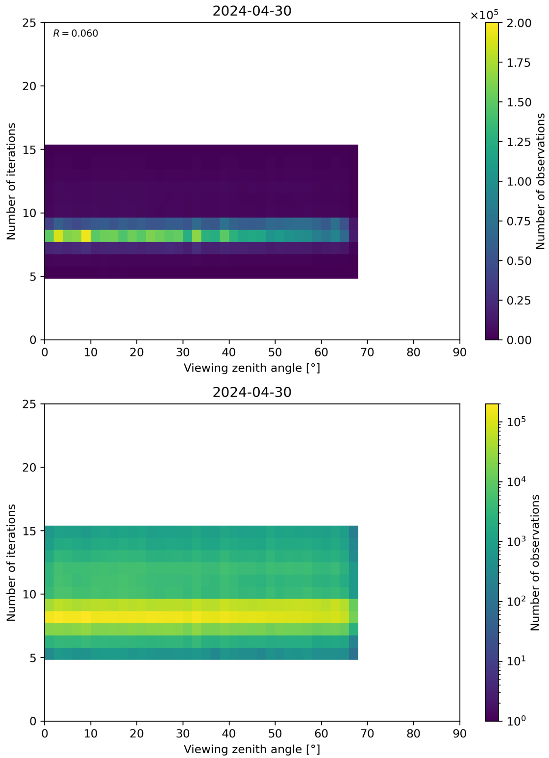
Figure 75: Scatter density plot of “Viewing zenith angle” against “Number of iterations” for 2024-04-29 to 2024-05-01.
