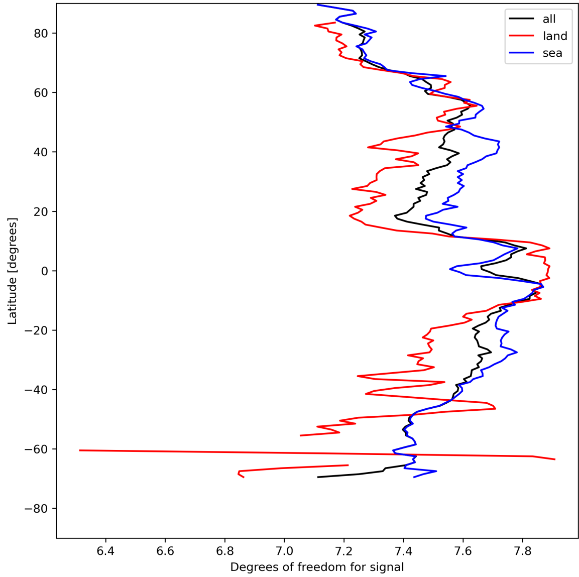
Figure 15: Zonal average of “Degrees of freedom for signal” for 2024-04-29 to 2024-05-01.
