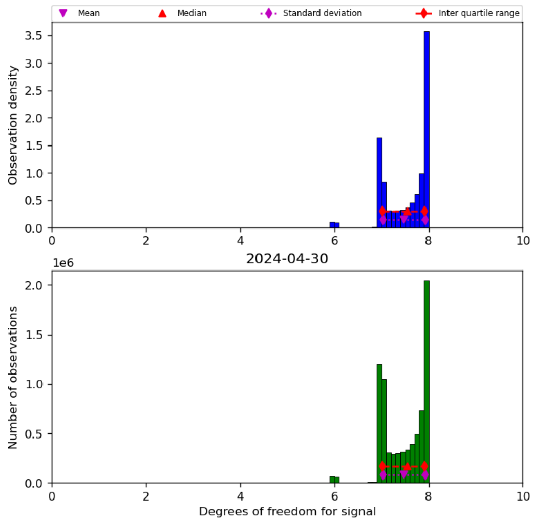
Figure 23: Histogram of “Degrees of freedom for signal” for 2024-04-29 to 2024-05-01
