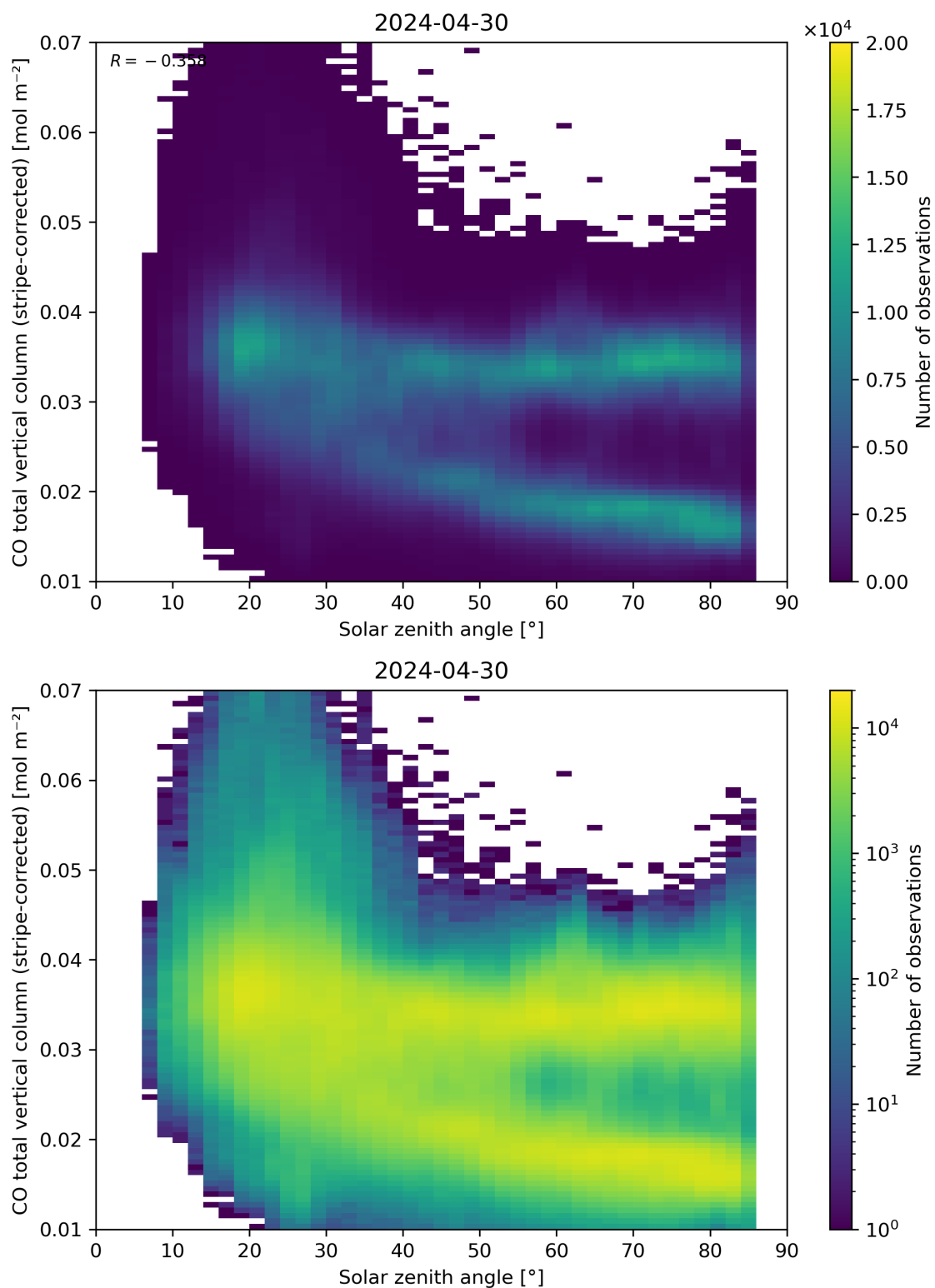
Figure 62: Scatter density plot of “Solar zenith angle” against “CO total vertical column (stripe-corrected)” for 2024-04-29 to 2024-05-01.
