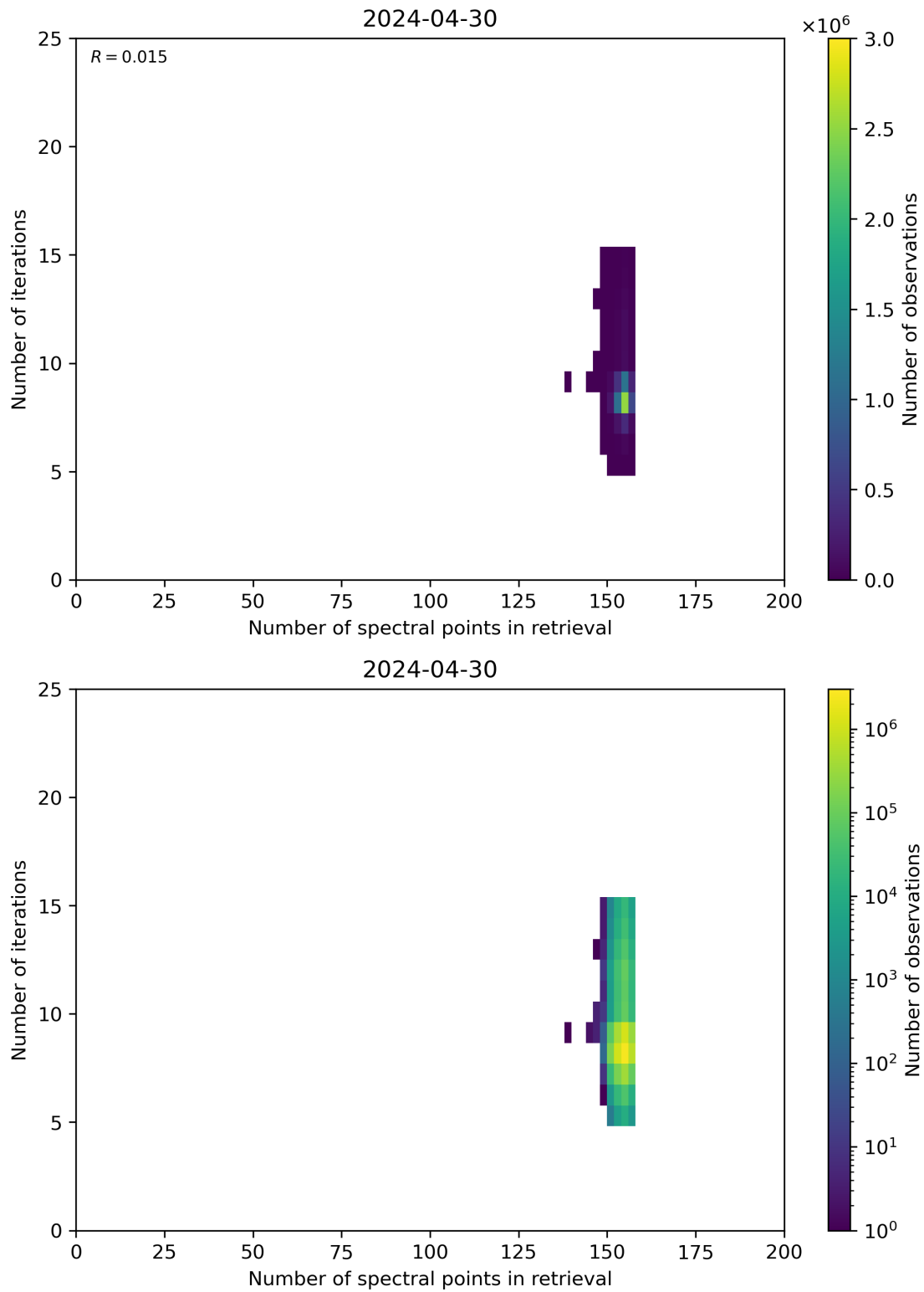
Figure 60: Scatter density plot of “Number of spectral points in retrieval” against “Number of iterations” for 2024-04-29 to 2024-05-01.
