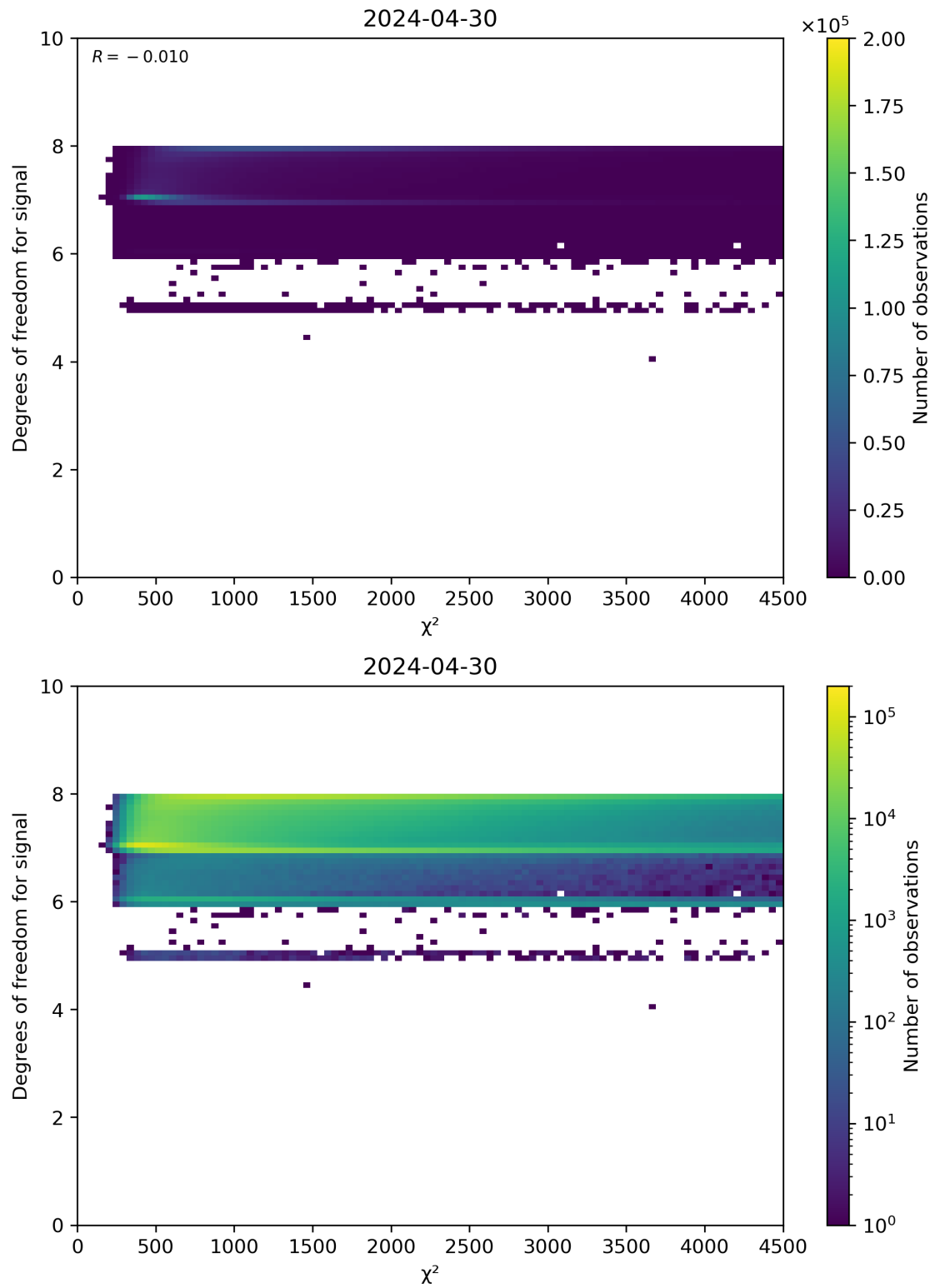
Figure 48: Scatter density plot of “ \chi^2 ” against “Degrees of freedom for signal” for 2024-04-29 to 2024-05-01.
