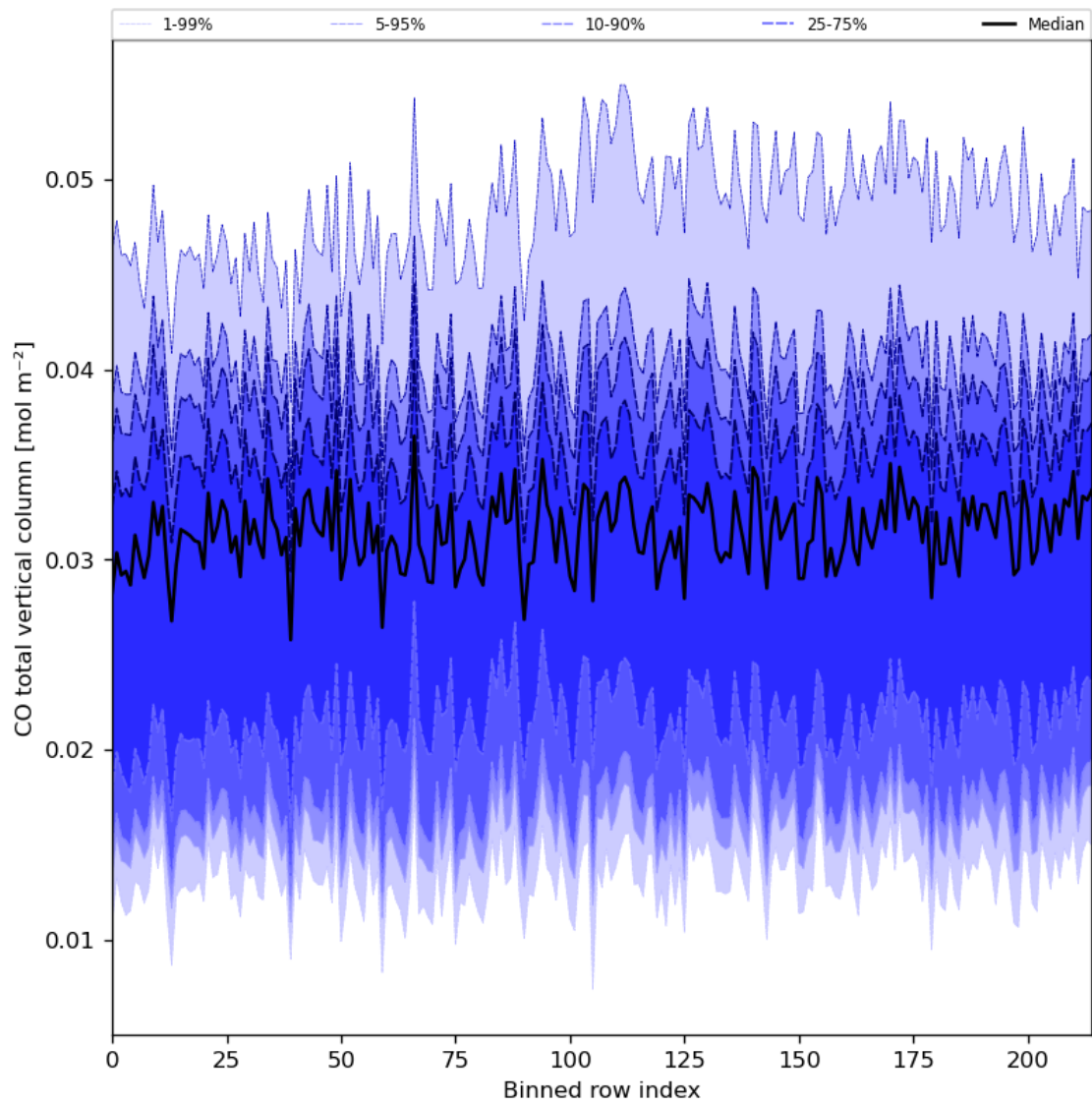
Figure 26: Along track statistics of “CO total vertical column” for 2024-04-29 to 2024-05-01
