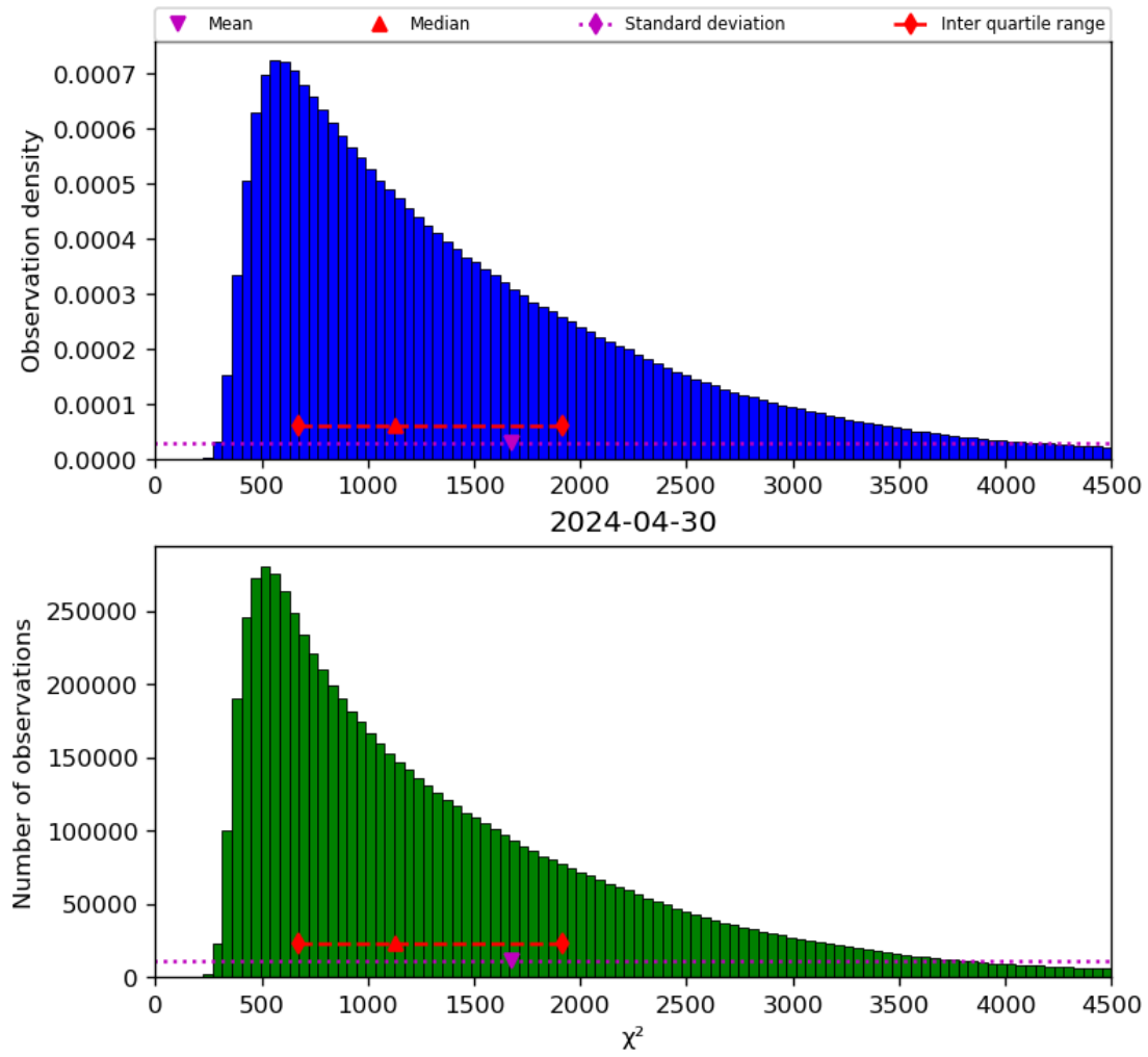
Figure 22: Histogram of “ \chi^2 ” for 2024-04-29 to 2024-05-01
