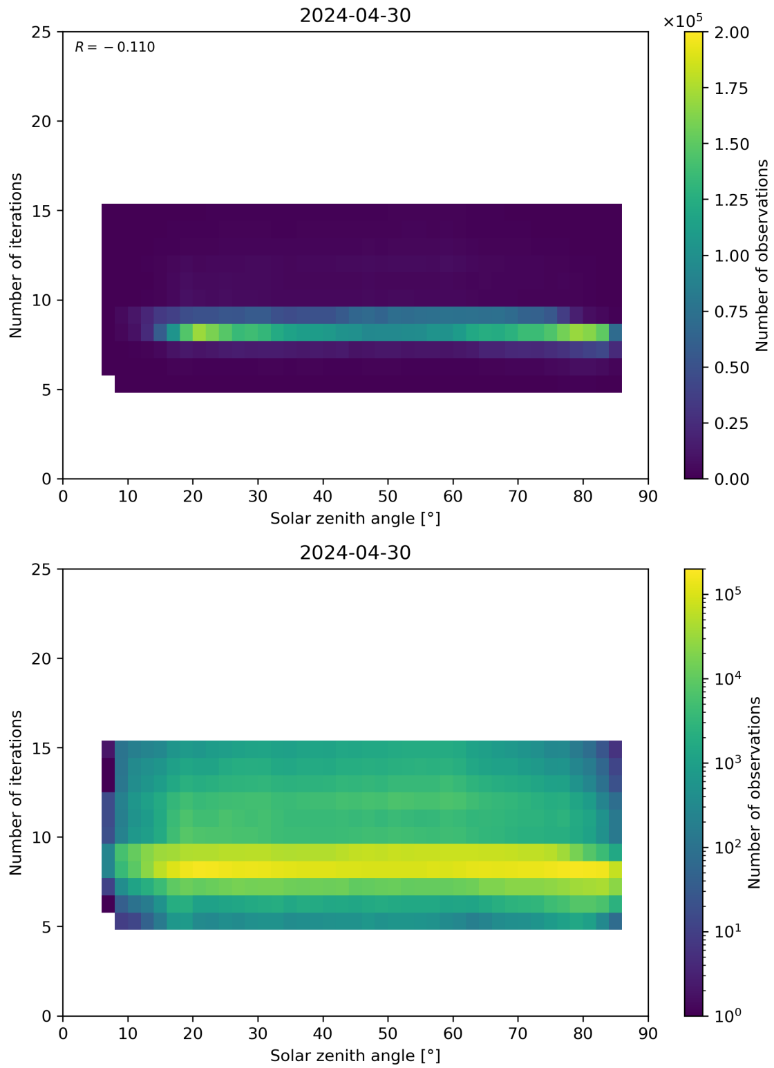
Figure 67: Scatter density plot of “Solar zenith angle” against “Number of iterations” for 2024-04-29 to 2024-05-01.
