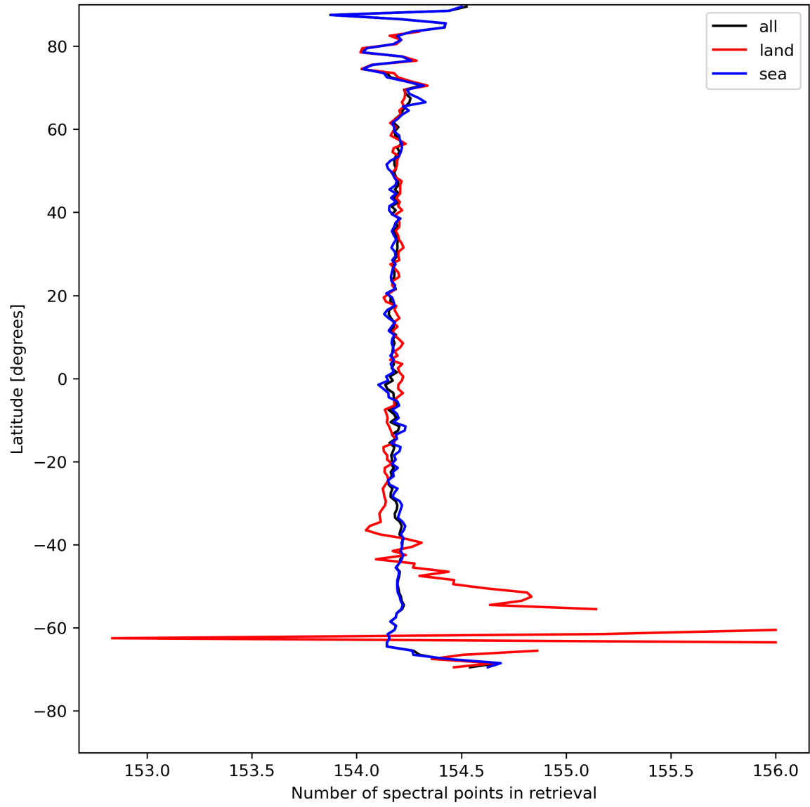
Figure 13: Zonal average of “Number of spectral points in retrieval” for 2024-04-29 to 2024-05-01.
