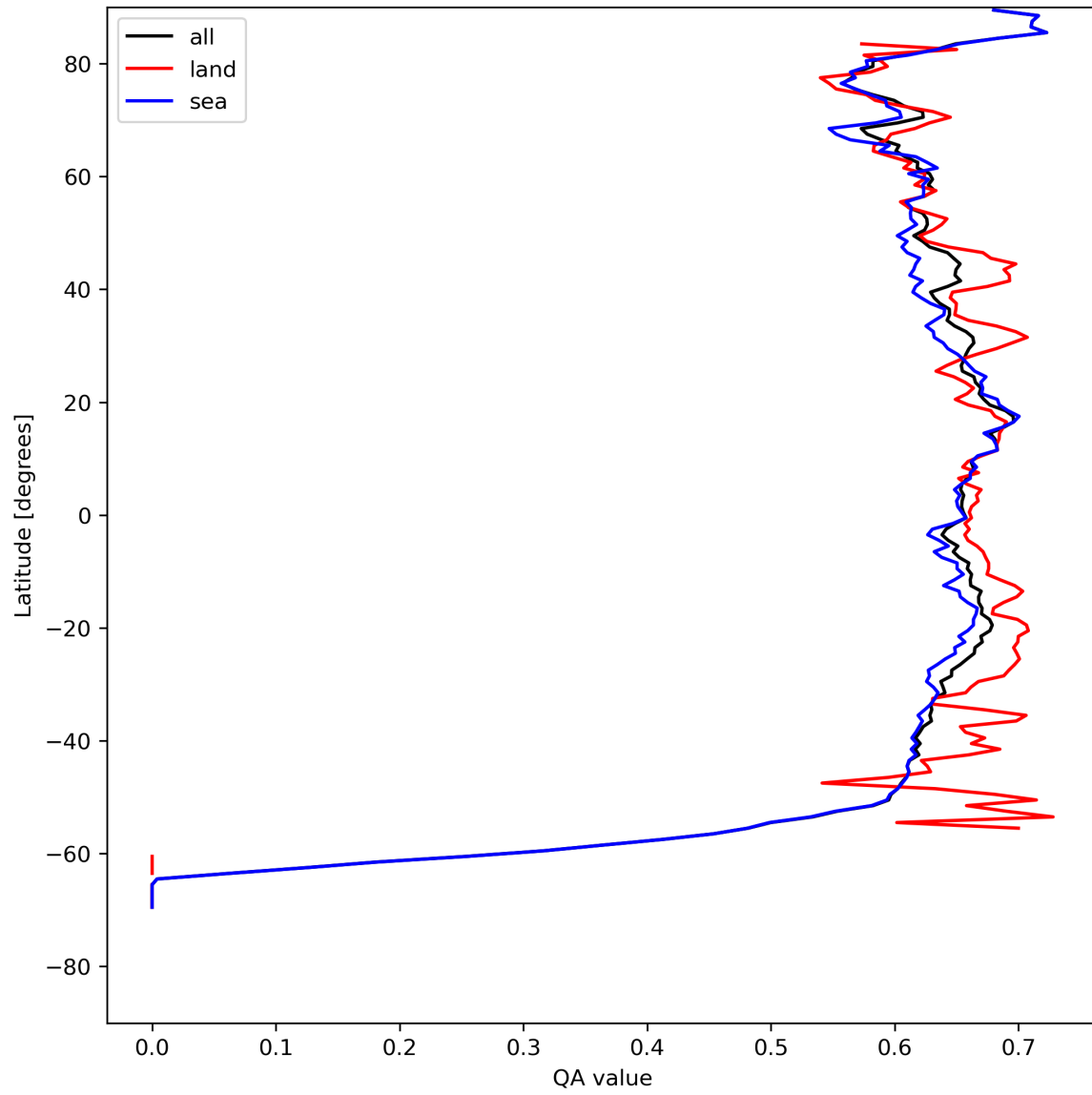
Figure 9: Zonal average of “QA value” for 2024-04-29 to 2024-05-01.
