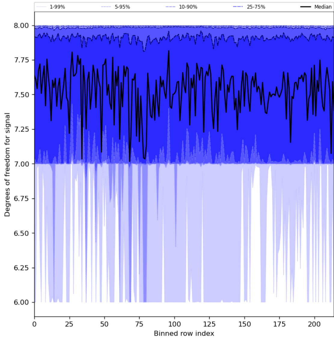
Figure 31: Along track statistics of “Degrees of freedom for signal” for 2024-04-29 to 2024-05-01
