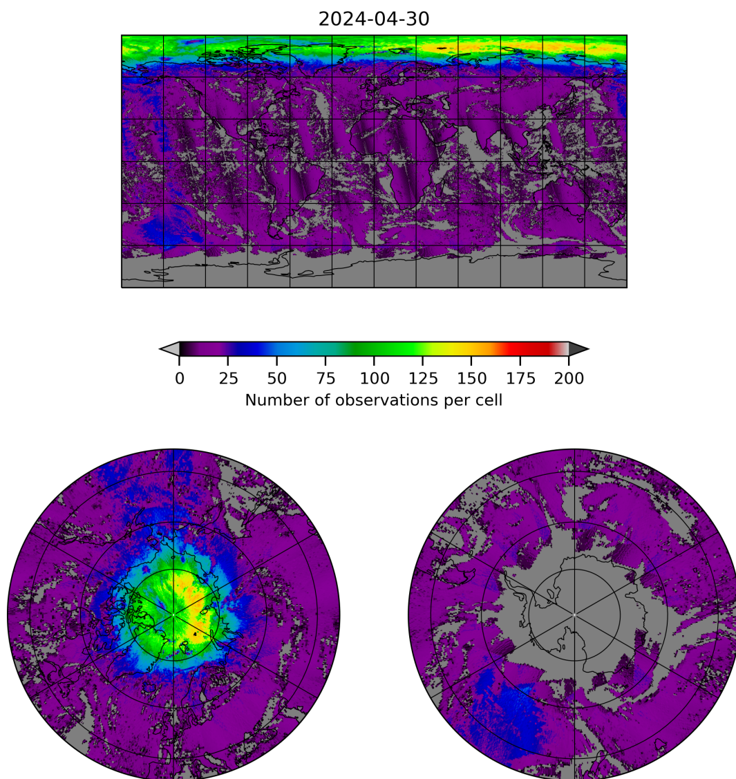
Figure 8: Map of the number of observations for 2024-04-29 to 2024-05-01
