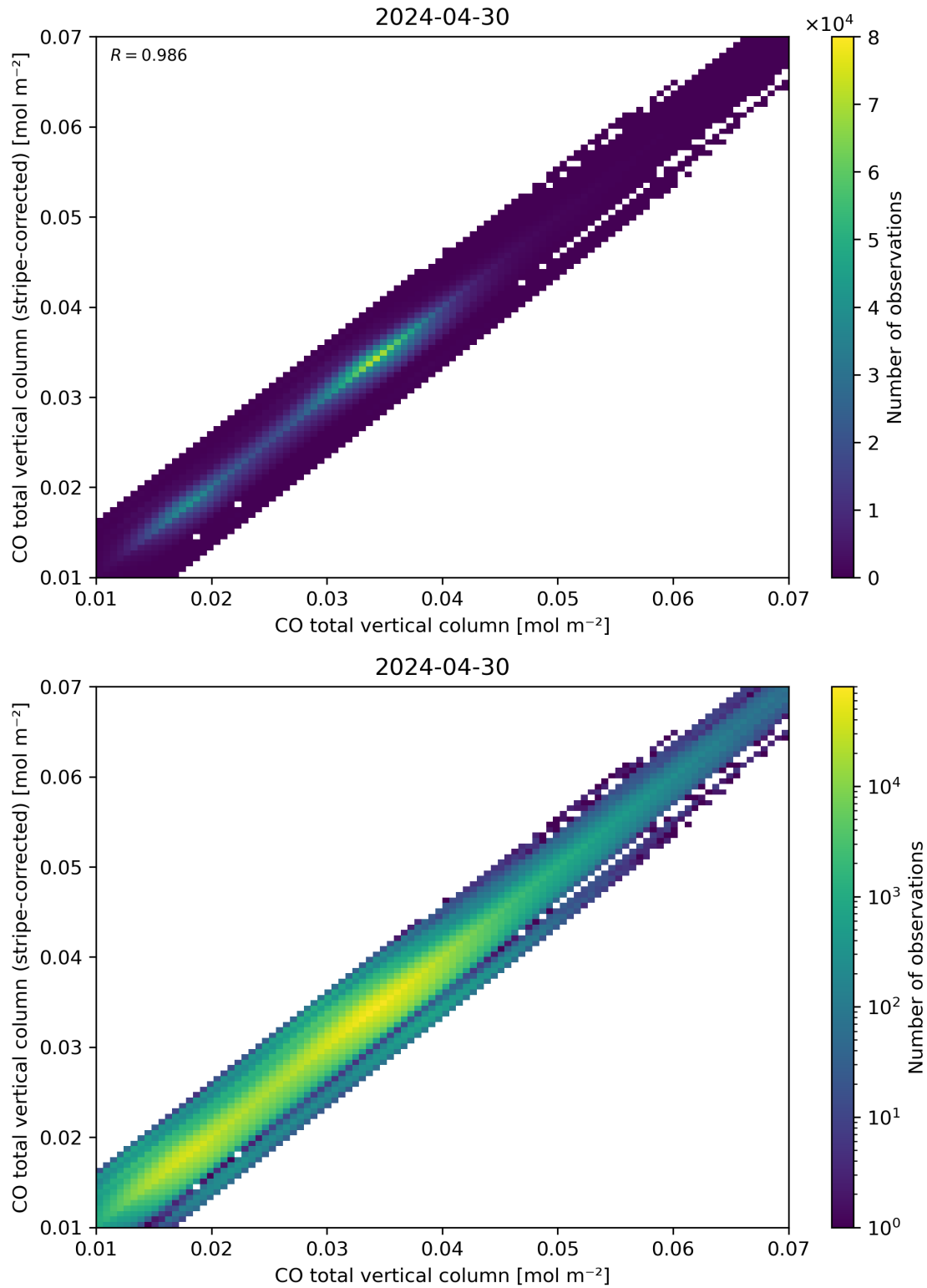
Figure 33: Scatter density plot of “CO total vertical column” against “CO total vertical column (stripe-corrected)” for 2024-04-29 to 2024-05-01.
