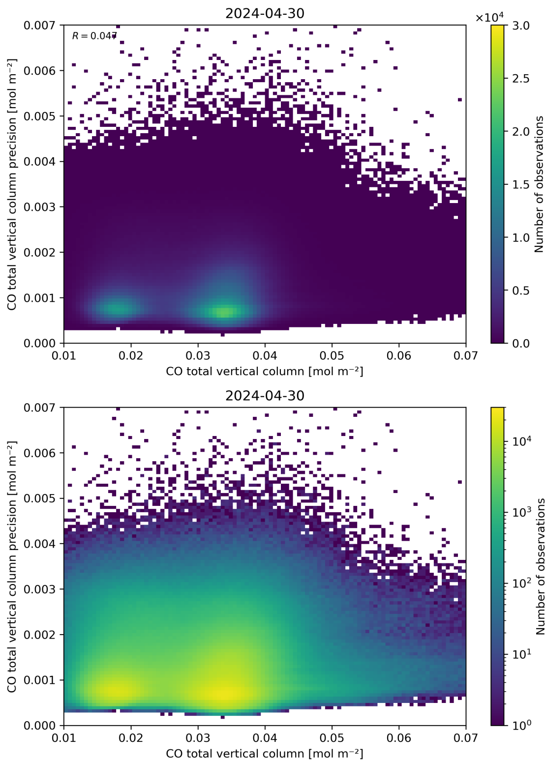
Figure 34: Scatter density plot of “CO total vertical column” against “CO total vertical column precision” for 2024-04-29 to 2024-05-01.
