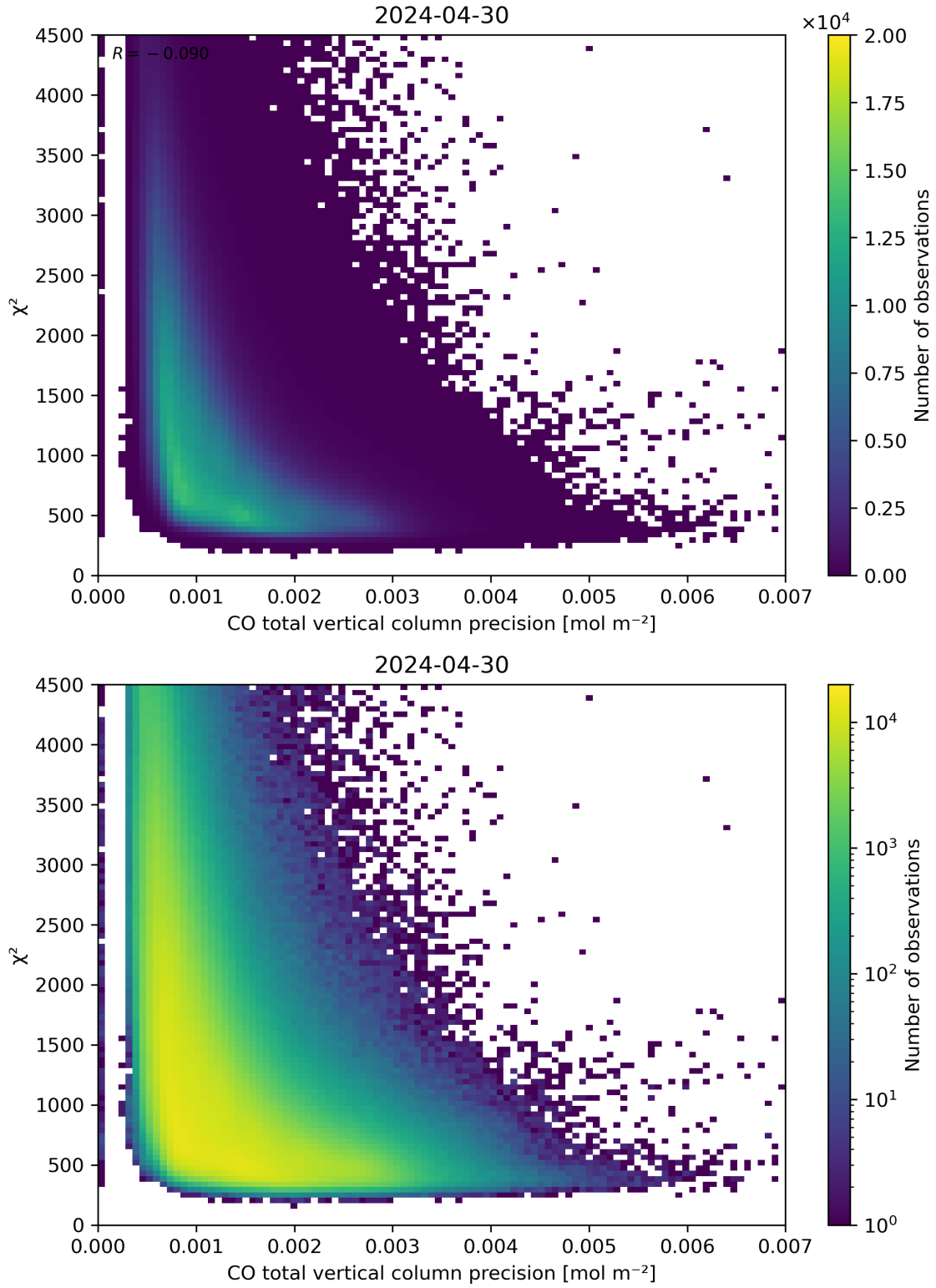
Figure 44: Scatter density plot of “CO total vertical column precision” against “ \chi^2 ” for 2024-04-29 to 2024-05-01.
