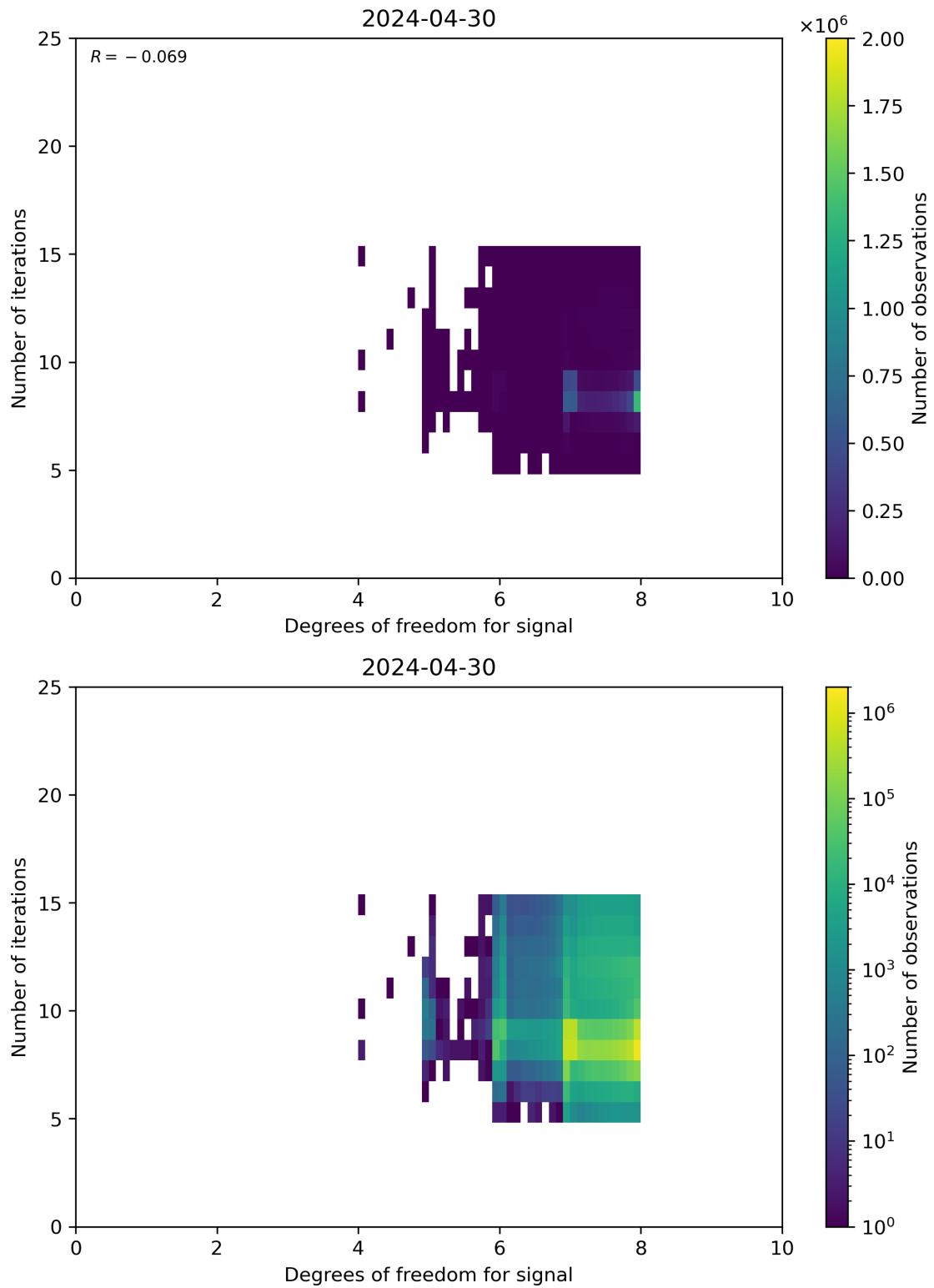
Figure 50: Scatter density plot of “Degrees of freedom for signal” against “Number of iterations” for 2024-04-29 to 2024-05-01.
