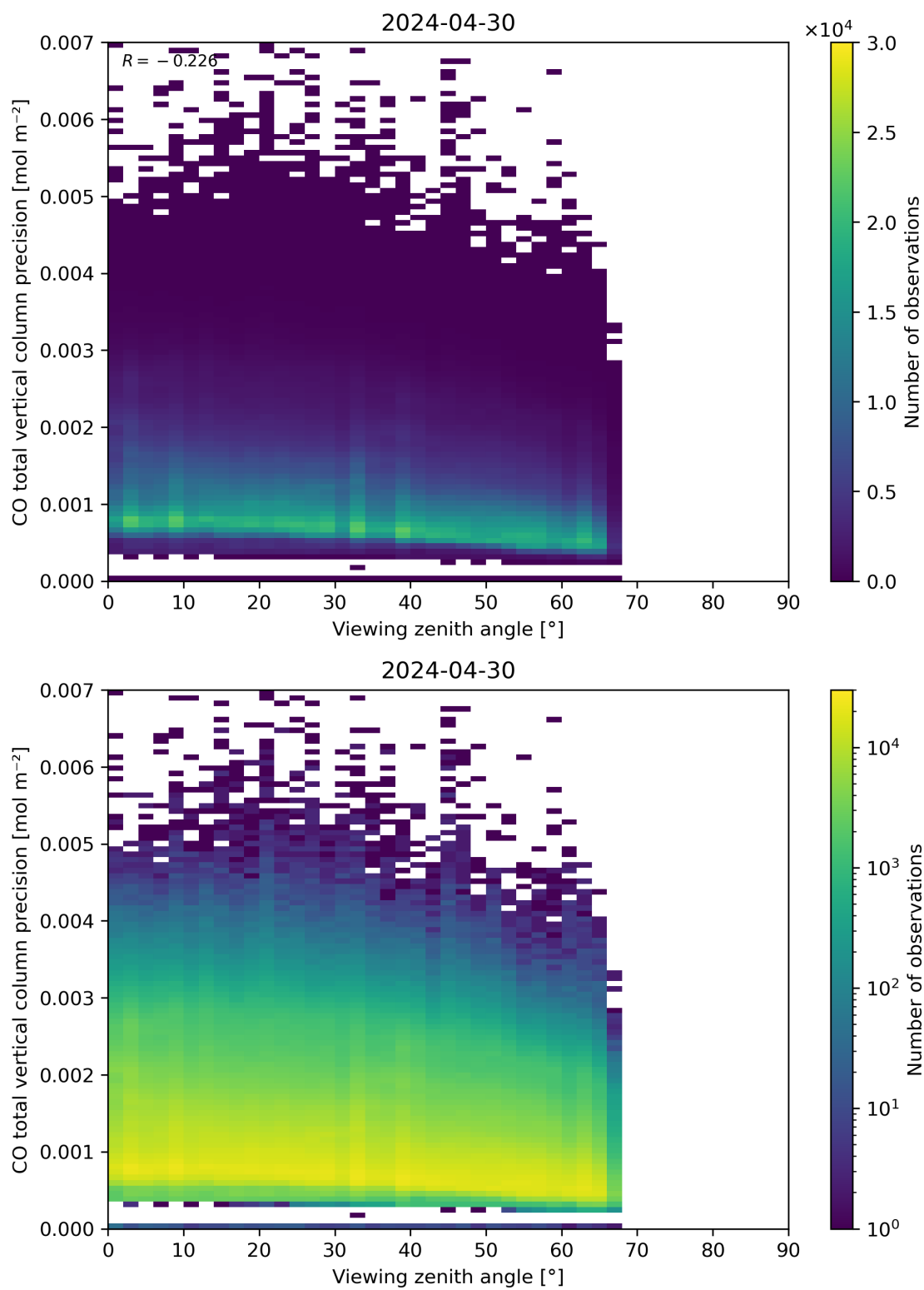
Figure 71: Scatter density plot of “Viewing zenith angle” against “CO total vertical column precision” for 2024-04-29 to 2024-05-01.
