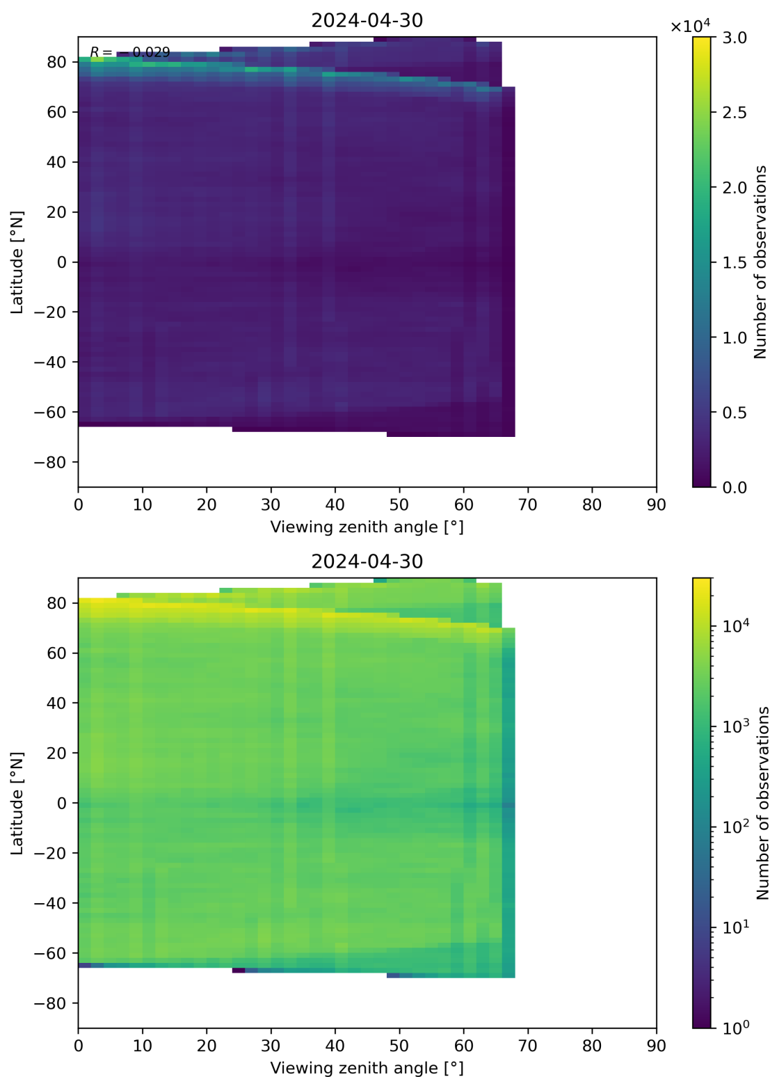
Figure 74: Scatter density plot of “Viewing zenith angle” against “Latitude” for 2024-04-29 to 2024-05-01.
