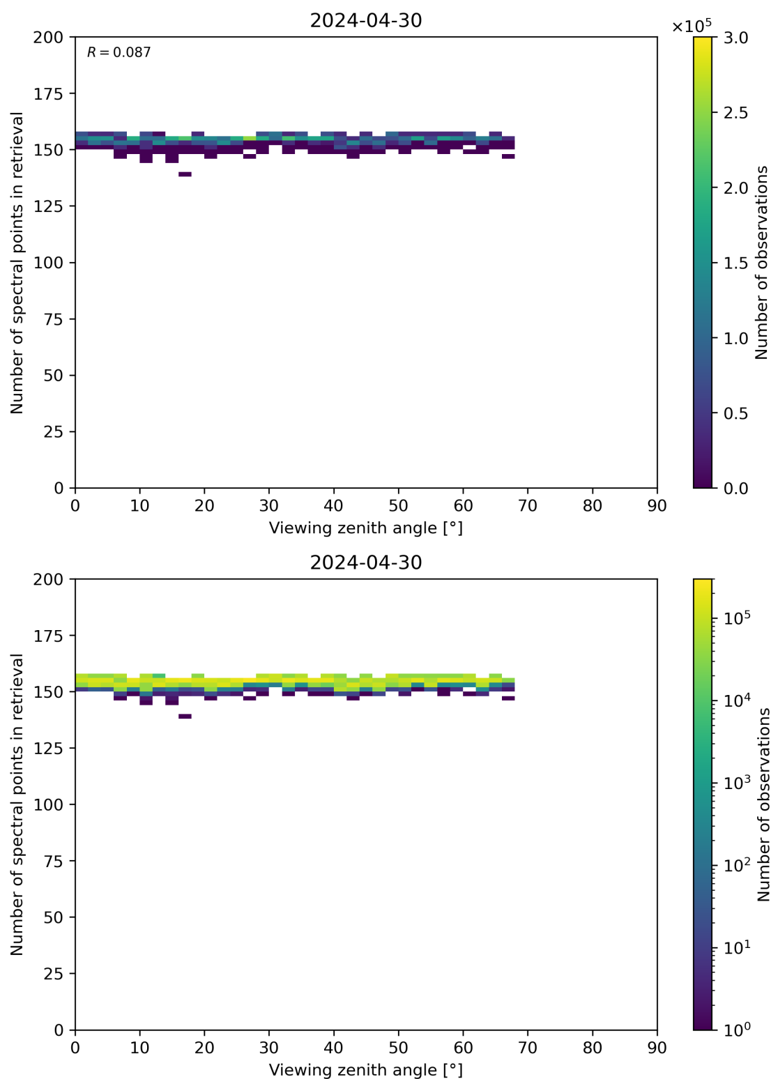
Figure 76: Scatter density plot of “Viewing zenith angle” against “Number of spectral points in retrieval” for 2024-04-29 to 2024-05-01.
