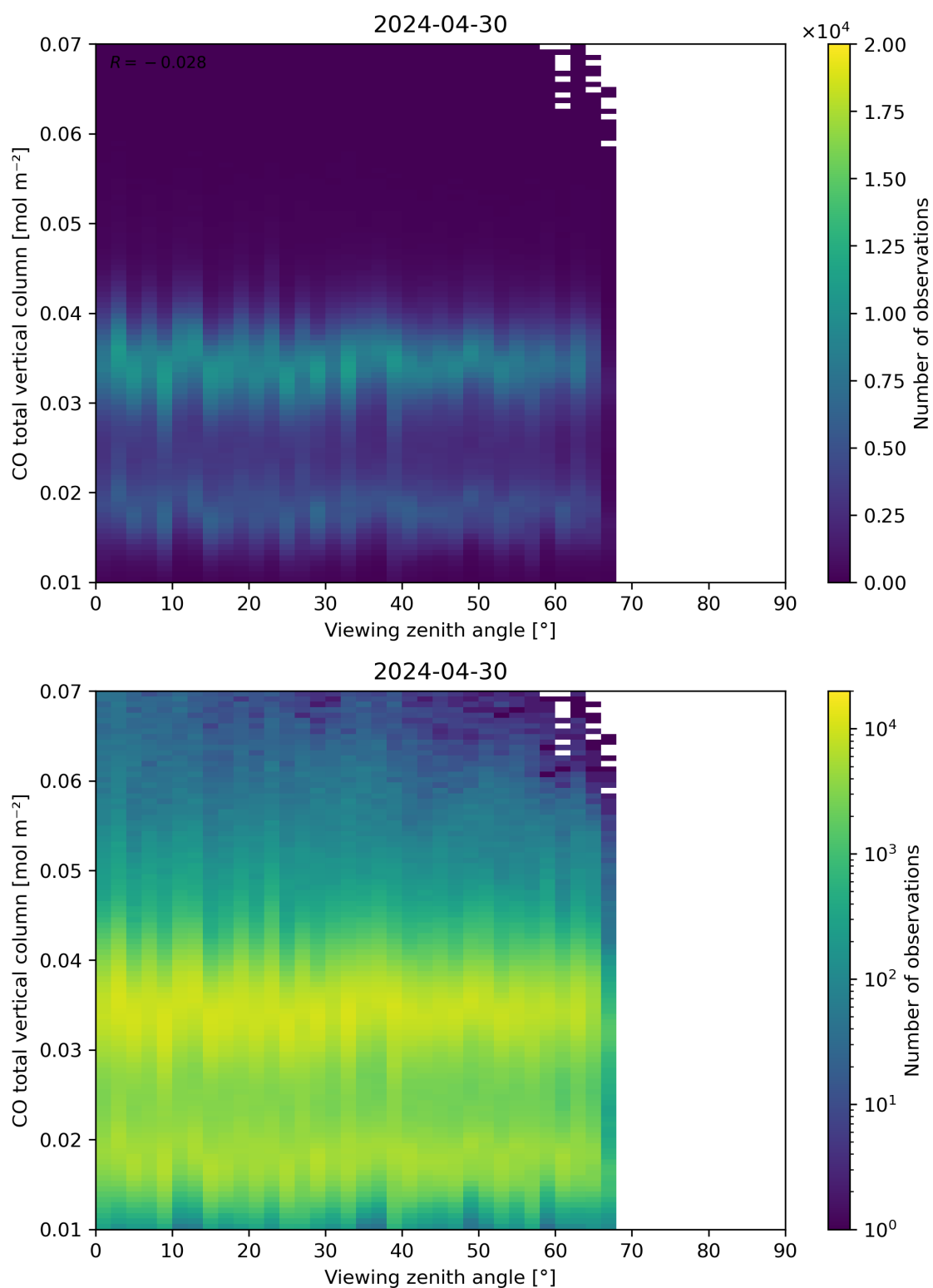
Figure 69: Scatter density plot of “Viewing zenith angle” against “CO total vertical column” for 2024-04-29 to 2024-05-01.
