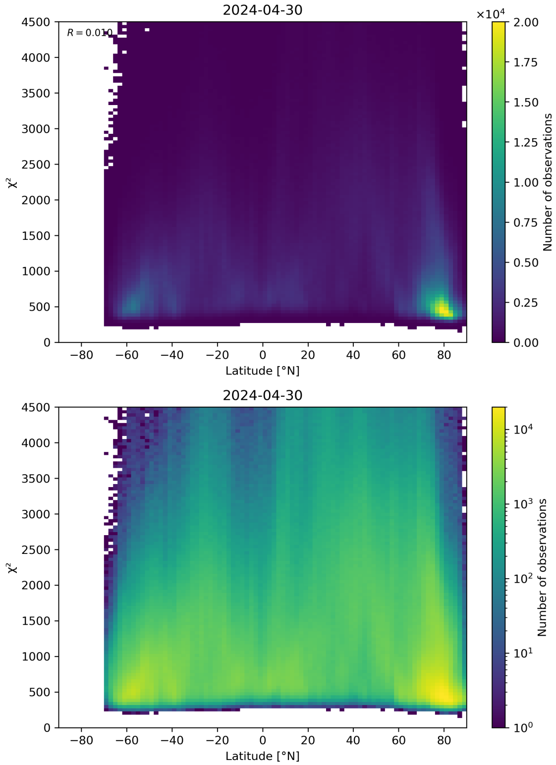
Figure 54: Scatter density plot of “Latitude” against “ \chi^2 ” for 2024-04-29 to 2024-05-01.
