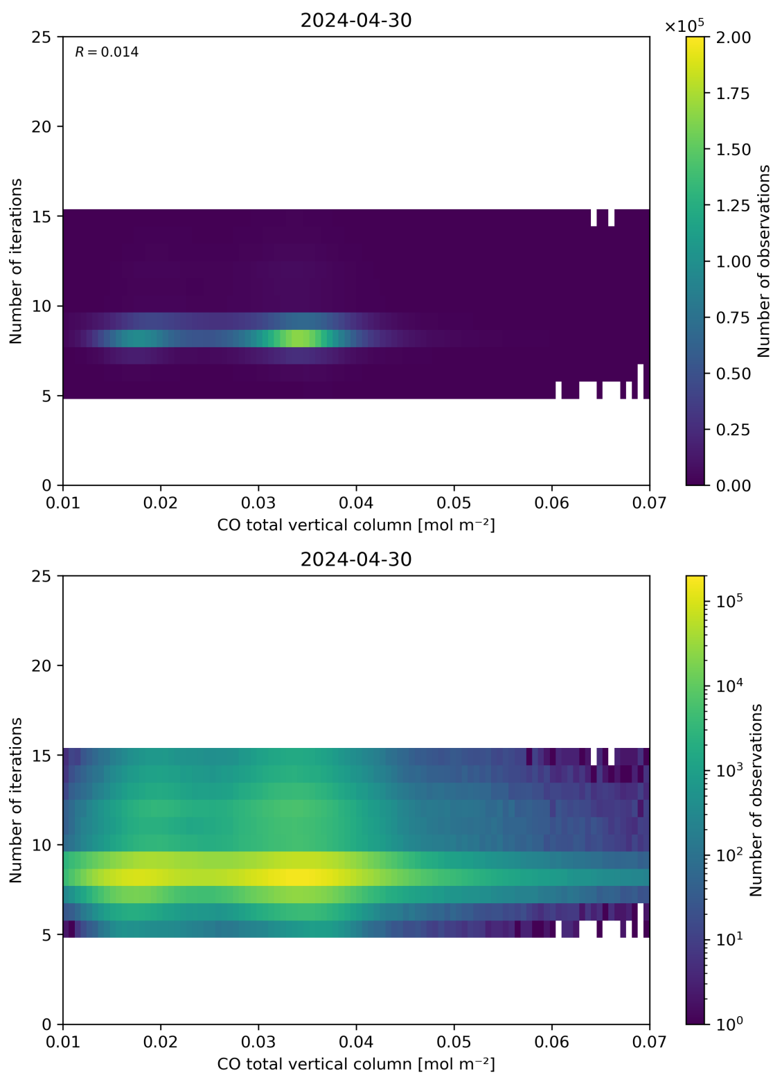
Figure 42: Scatter density plot of “CO total vertical column” against “Number of iterations” for 2024-04-29 to 2024-05-01.
