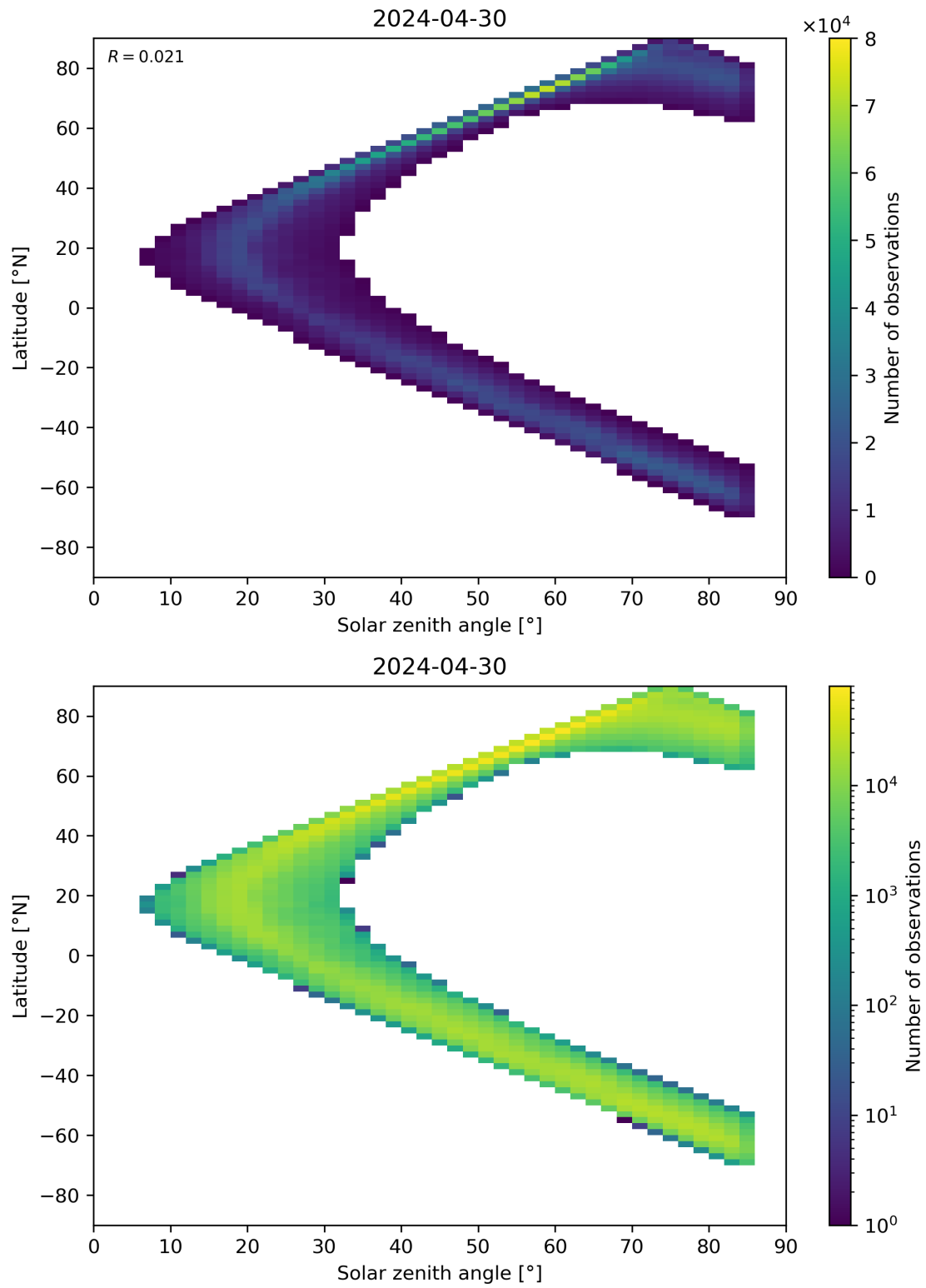
Figure 66: Scatter density plot of “Solar zenith angle” against “Latitude” for 2024-04-29 to 2024-05-01.
