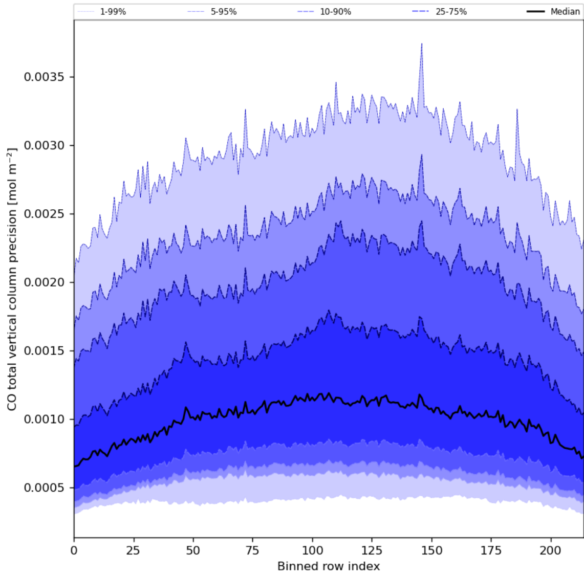
Figure 28: Along track statistics of “CO total vertical column precision” for 2024-04-29 to 2024-05-01
