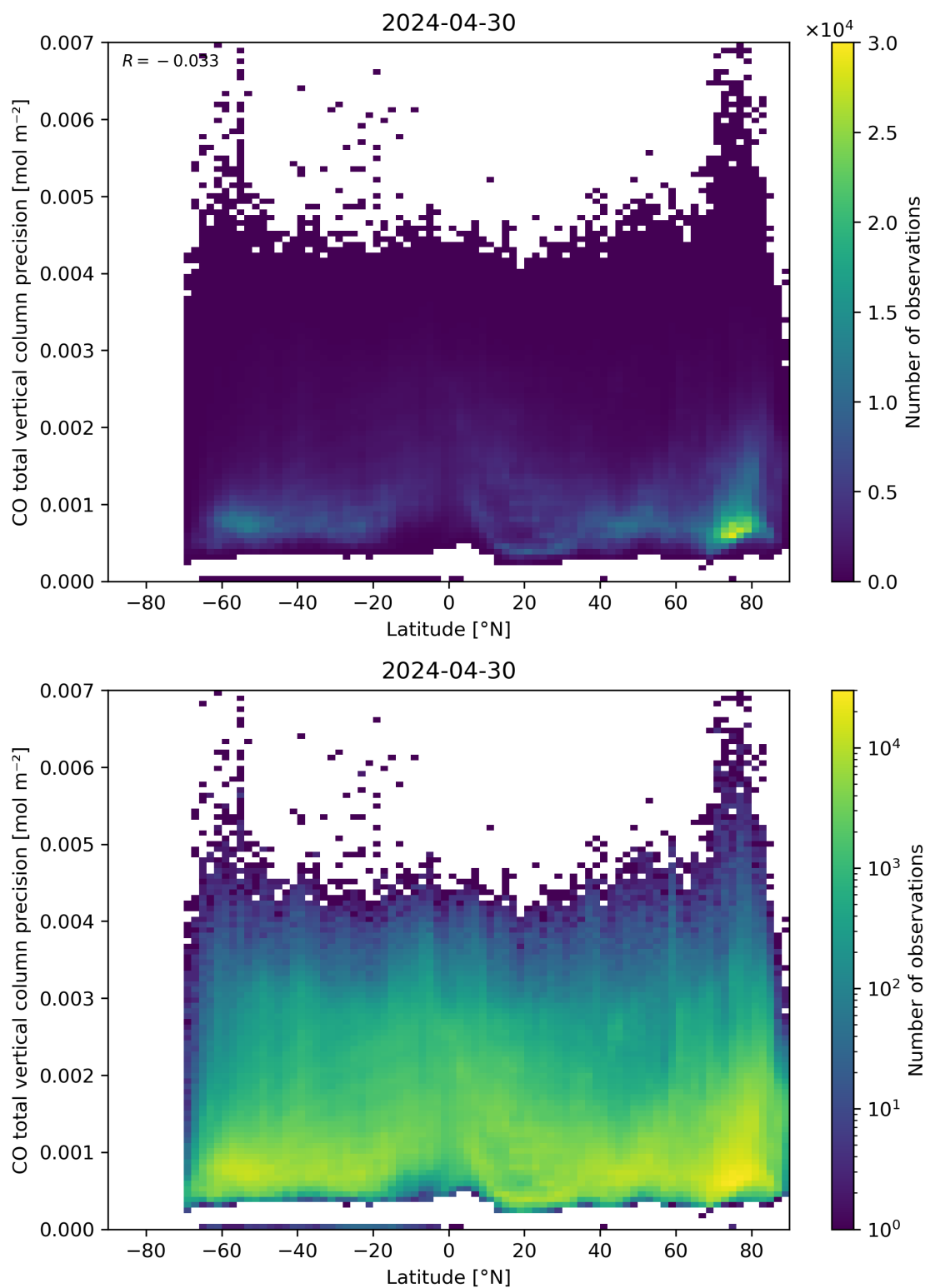
Figure 53: Scatter density plot of “Latitude” against “CO total vertical column precision” for 2024-04-29 to 2024-05-01.
