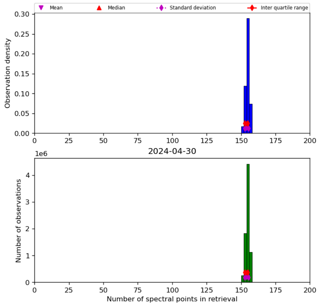
Figure 21: Histogram of “Number of spectral points in retrieval” for 2024-04-29 to 2024-05-01
