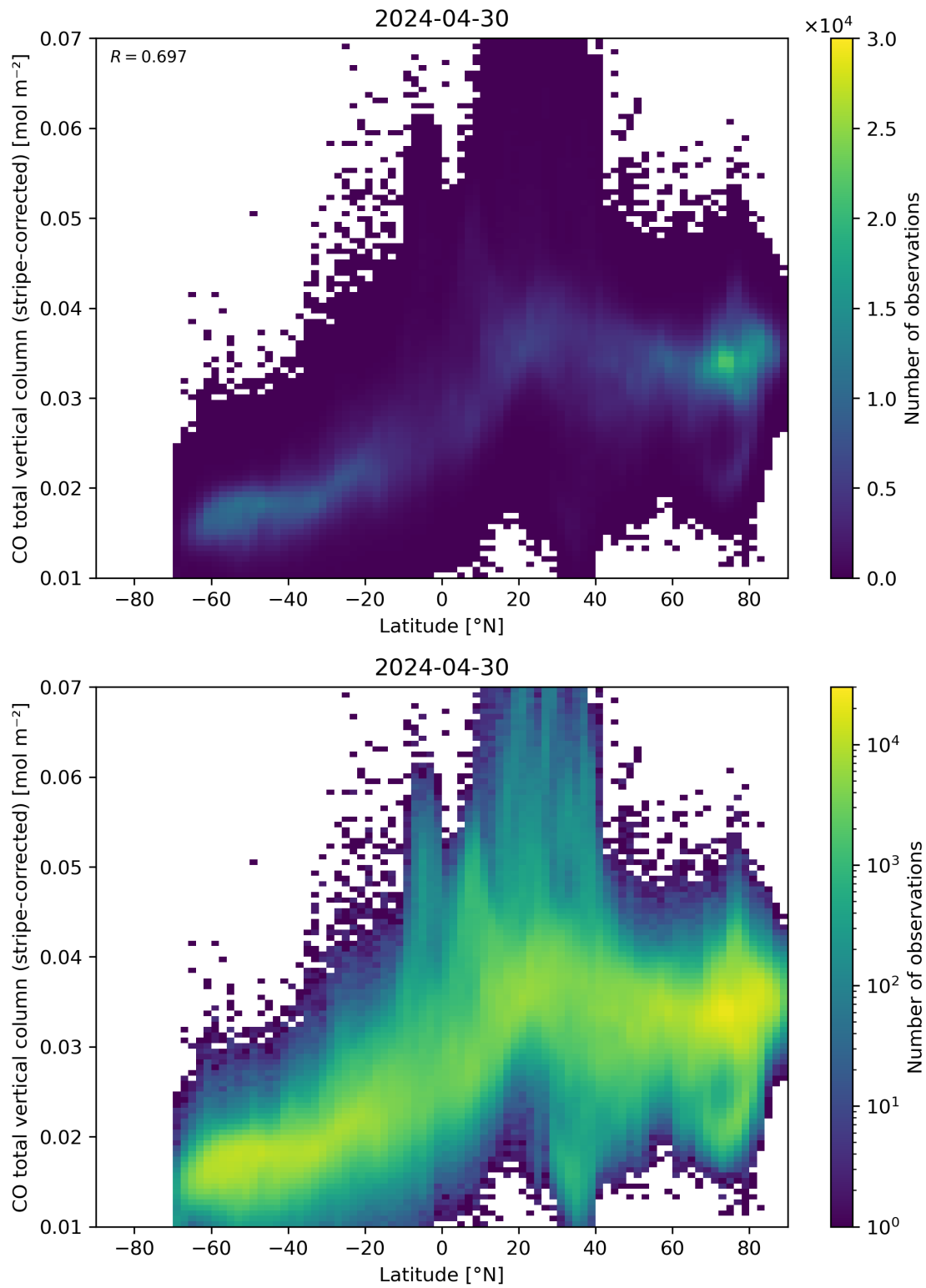
Figure 52: Scatter density plot of “Latitude” against “CO total vertical column (stripe-corrected)” for 2024-04-29 to 2024-05-01.
