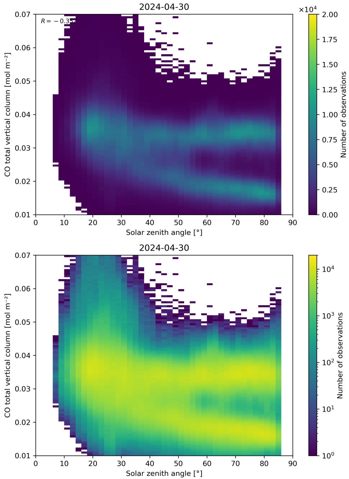
Figure 61: Scatter density plot of “Solar zenith angle” against “CO total vertical column” for 2024-04-29 to 2024-05-01.
