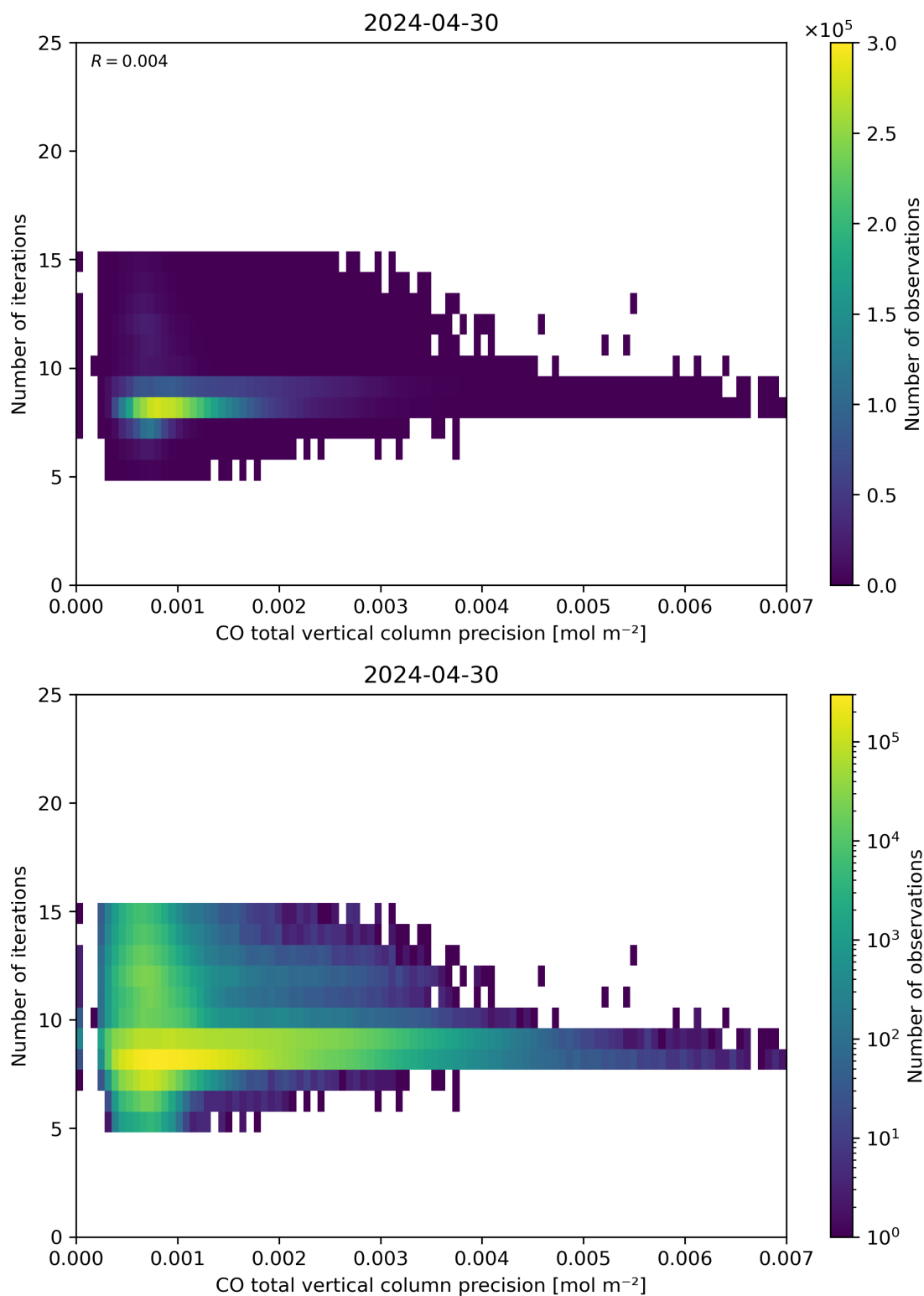
Figure 46: Scatter density plot of “CO total vertical column precision” against “Number of iterations” for 2024-04-29 to 2024-05-01.
