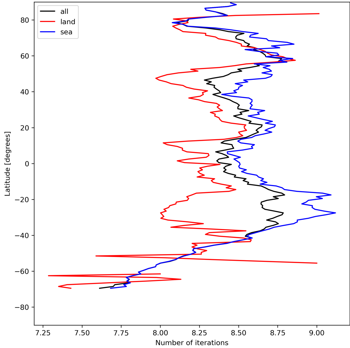
Figure 16: Zonal average of “Number of iterations” for 2024-04-30 to 2024-05-02.
