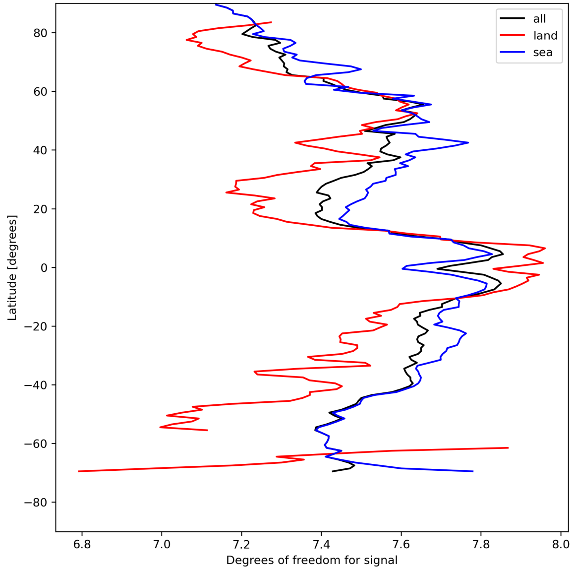
Figure 15: Zonal average of “Degrees of freedom for signal” for 2024-04-30 to 2024-05-02.
