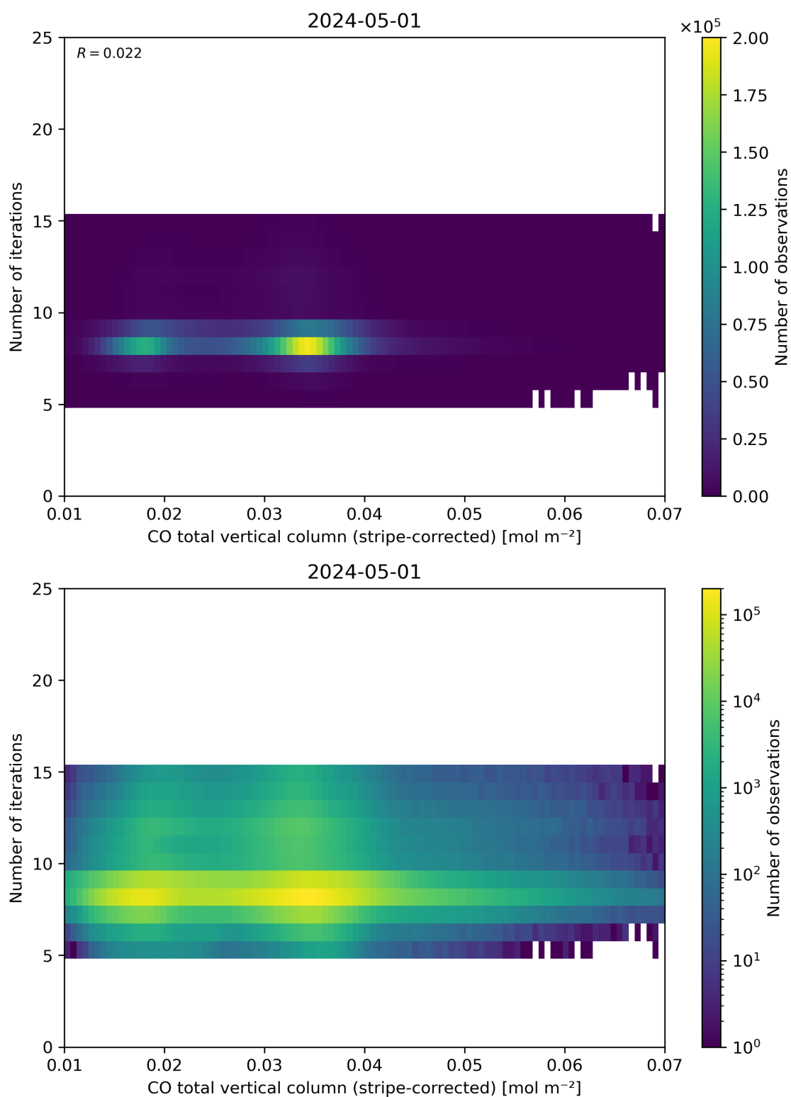
Figure 39: Scatter density plot of “CO total vertical column (stripe-corrected)” against “Number of iterations” for 2024-04-30 to 2024-05-02.
