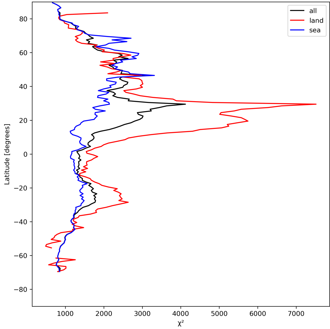
Figure 14: Zonal average of “ \chi^2 ” for 2024-04-30 to 2024-05-02.
