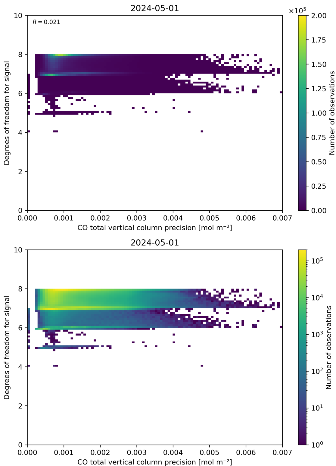
Figure 45: Scatter density plot of “CO total vertical column precision” against “Degrees of freedom for signal” for 2024-04-30 to 2024-05-02.
