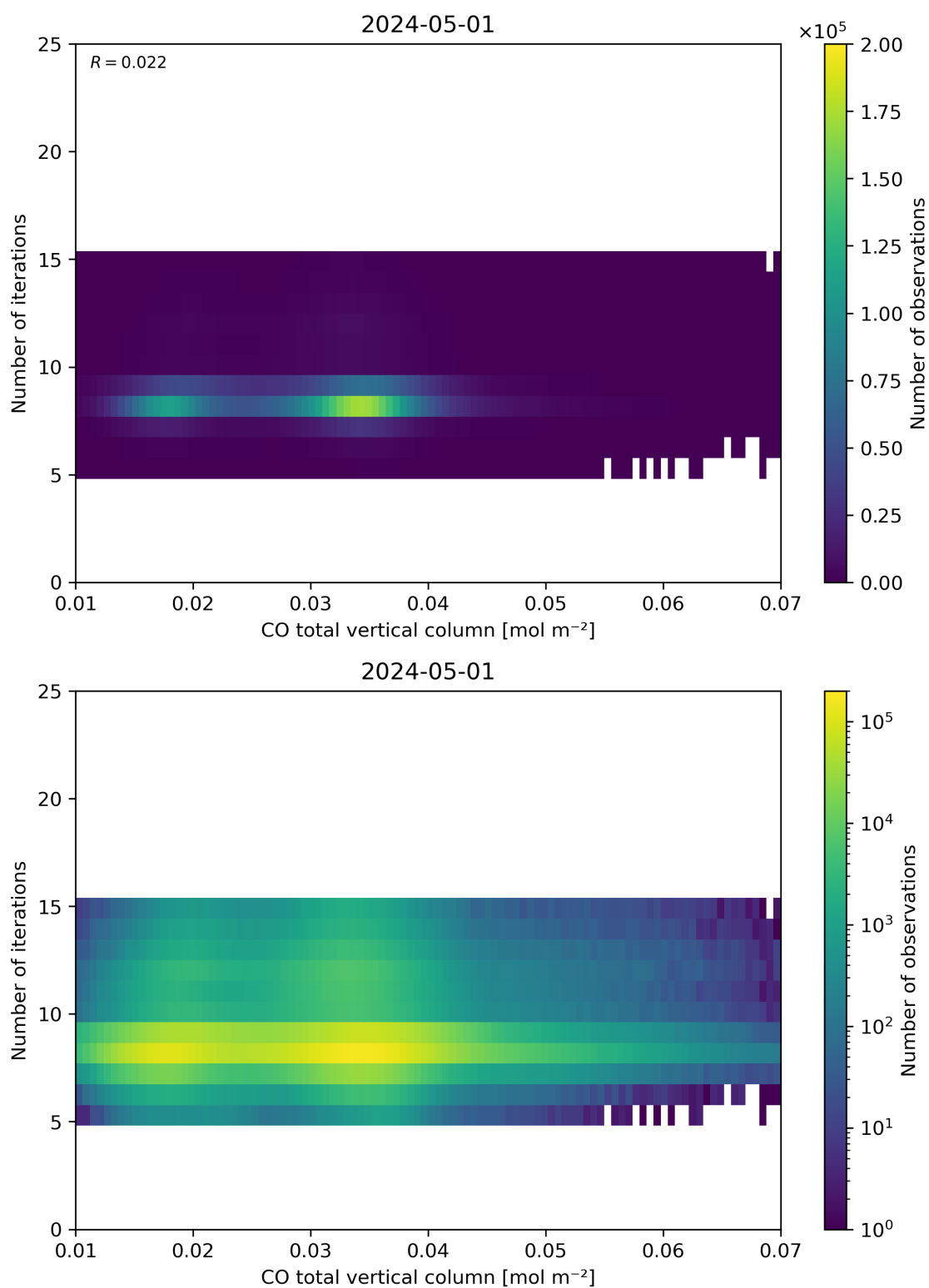
Figure 42: Scatter density plot of “CO total vertical column” against “Number of iterations” for 2024-04-30 to 2024-05-02.
