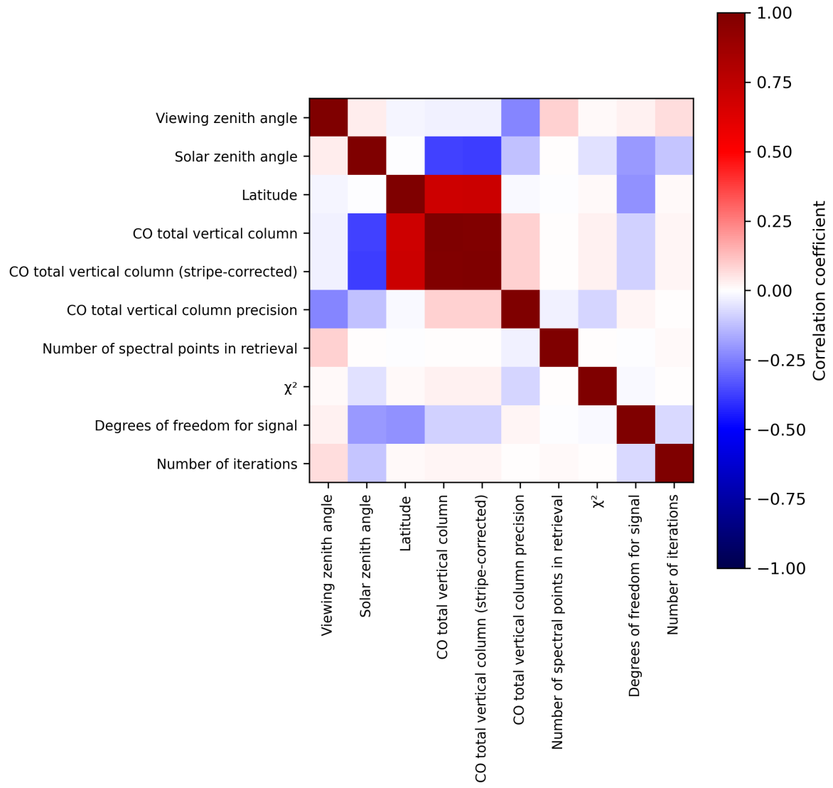
Figure 2: Map of correlation matrix for 2024-04-30 to 2024-05-02.
