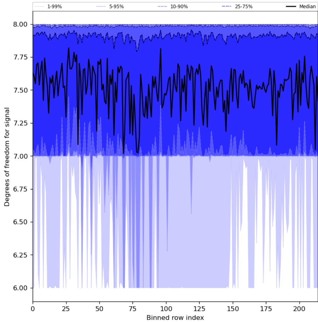
Figure 31: Along track statistics of “Degrees of freedom for signal” for 2024-04-30 to 2024-05-02
