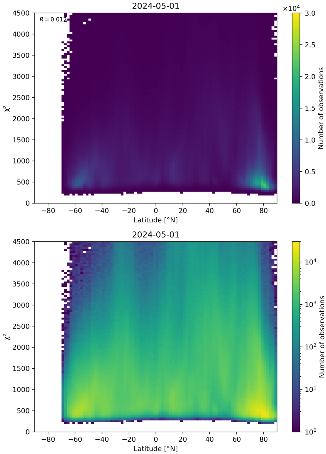
Figure 54: Scatter density plot of “Latitude” against “ \chi^2 ” for 2024-04-30 to 2024-05-02.
