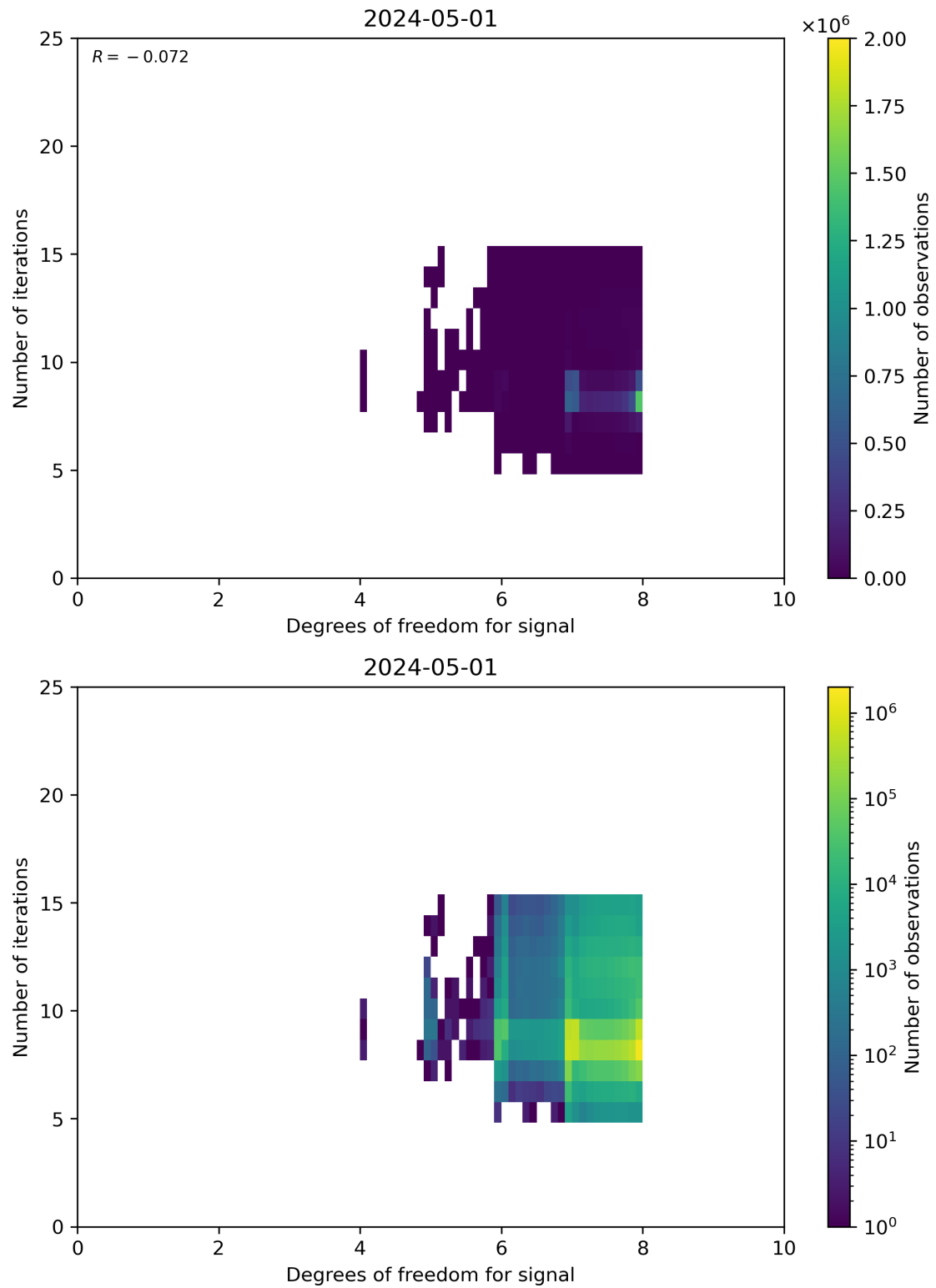
Figure 50: Scatter density plot of “Degrees of freedom for signal” against “Number of iterations” for 2024-04-30 to 2024-05-02.
