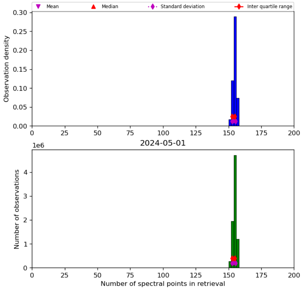
Figure 21: Histogram of “Number of spectral points in retrieval” for 2024-04-30 to 2024-05-02
