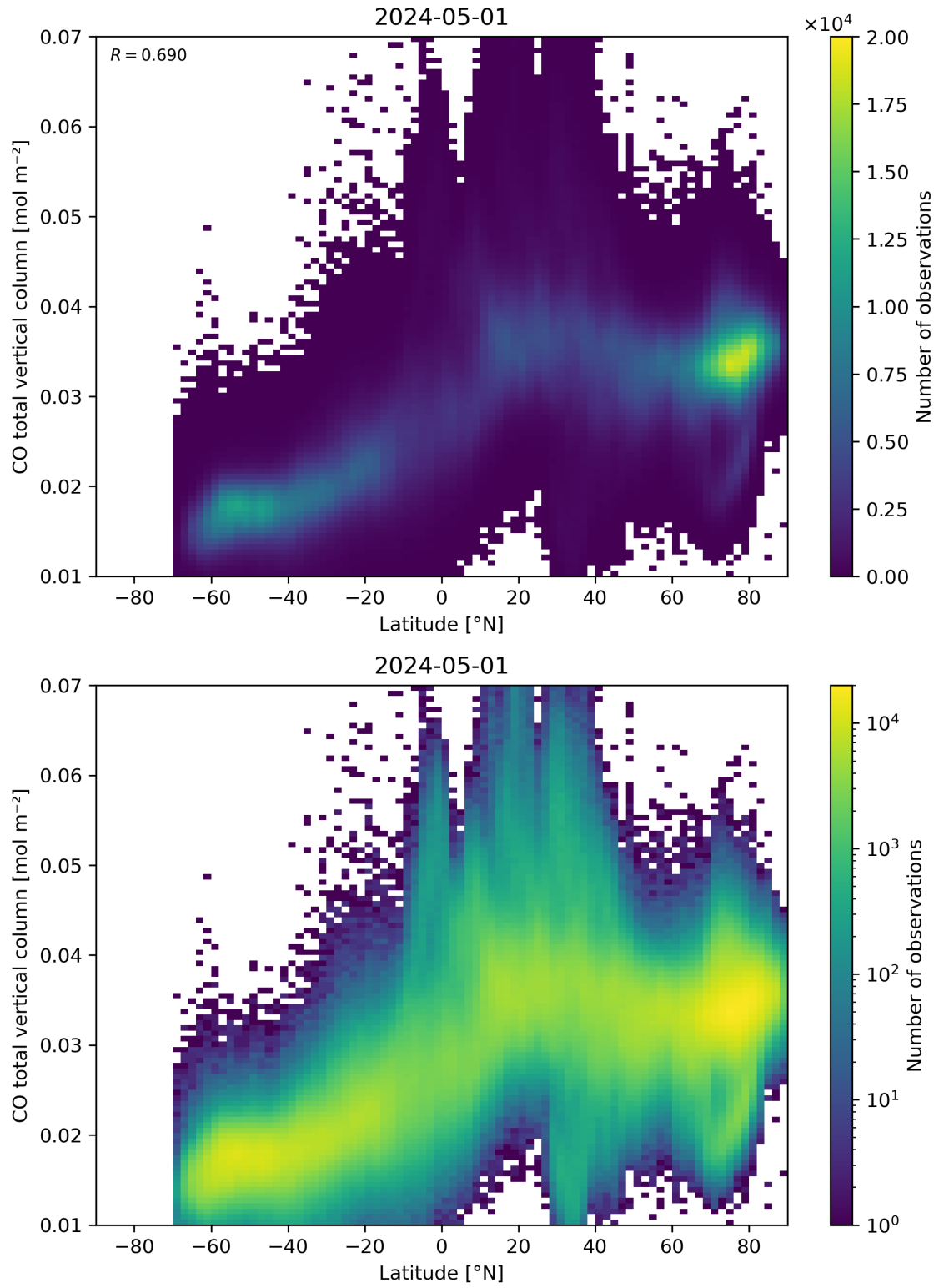
Figure 51: Scatter density plot of “Latitude” against “CO total vertical column” for 2024-04-30 to 2024-05-02.
