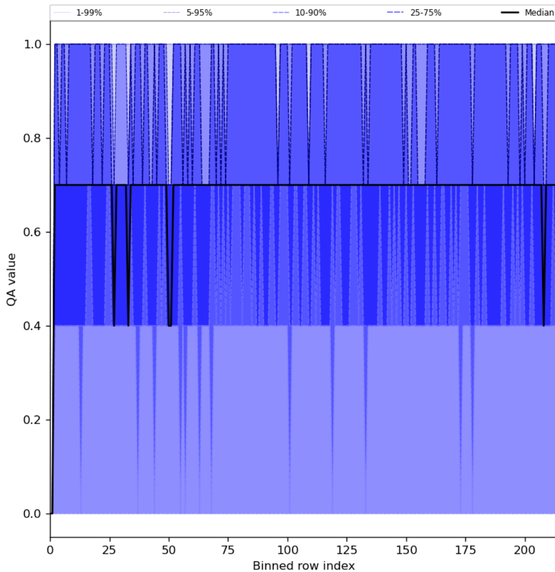
Figure 25: Along track statistics of “QA value” for 2024-04-30 to 2024-05-02
