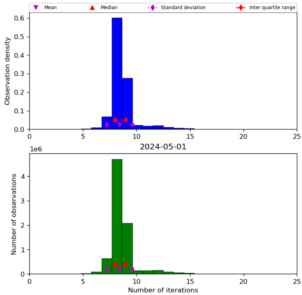
Figure 24: Histogram of “Number of iterations” for 2024-04-30 to 2024-05-02
