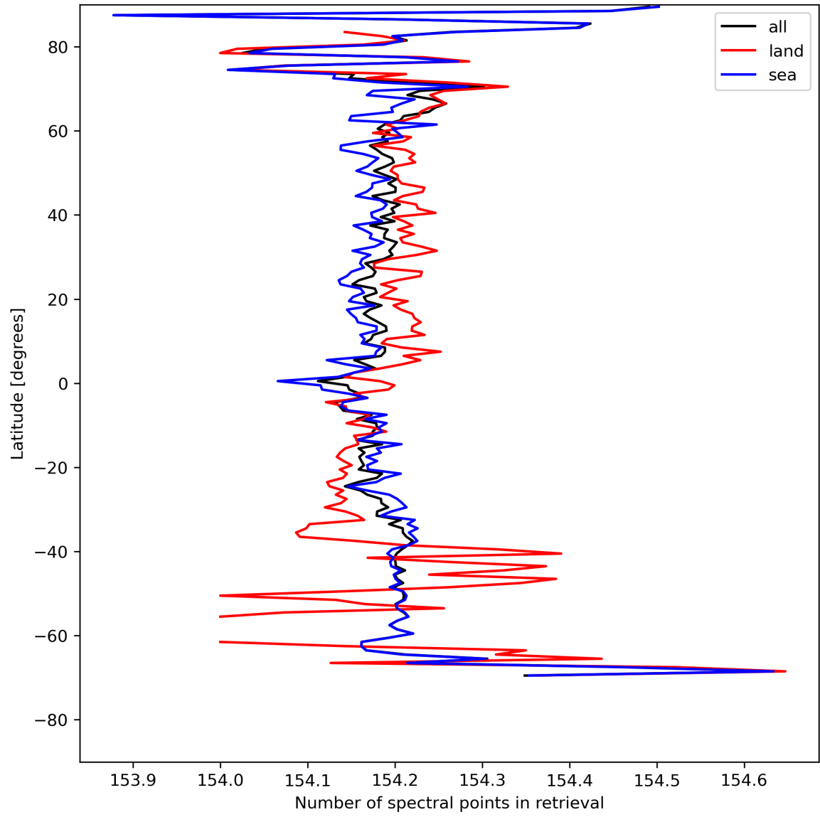
Figure 13: Zonal average of “Number of spectral points in retrieval” for 2024-04-30 to 2024-05-02.
