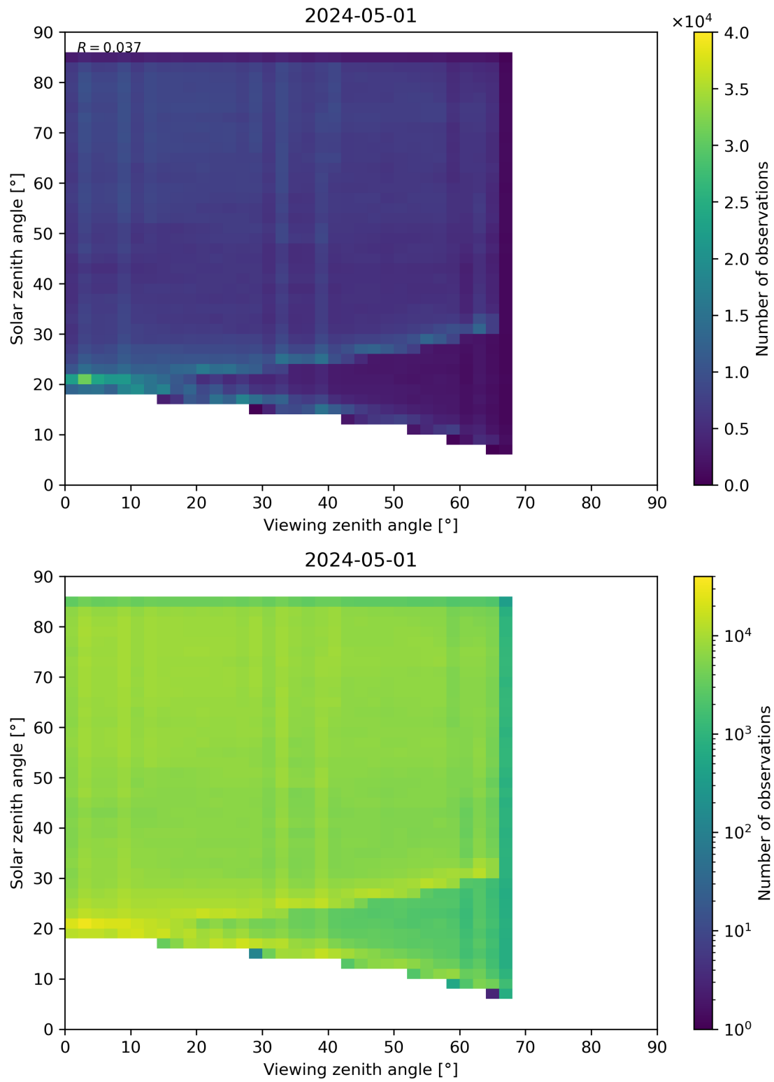
Figure 77: Scatter density plot of “Viewing zenith angle” against “Solar zenith angle” for 2024-04-30 to 2024-05-02.
