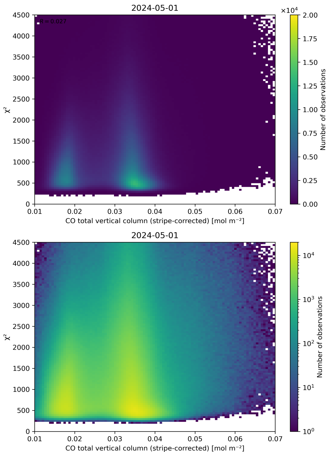
Figure 37: Scatter density plot of “CO total vertical column (stripe-corrected)” against “ \chi^2 ” for 2024-04-30 to 2024-05-02.
