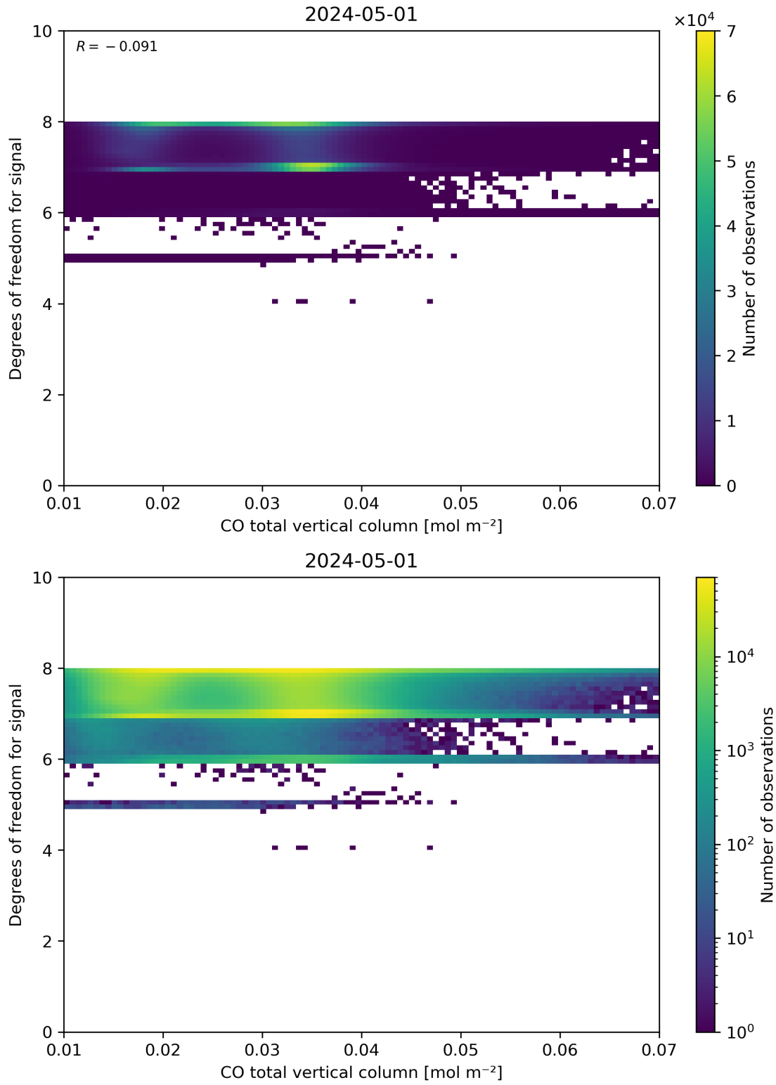
Figure 41: Scatter density plot of “CO total vertical column” against “Degrees of freedom for signal” for 2024-04-30 to 2024-05-02.
