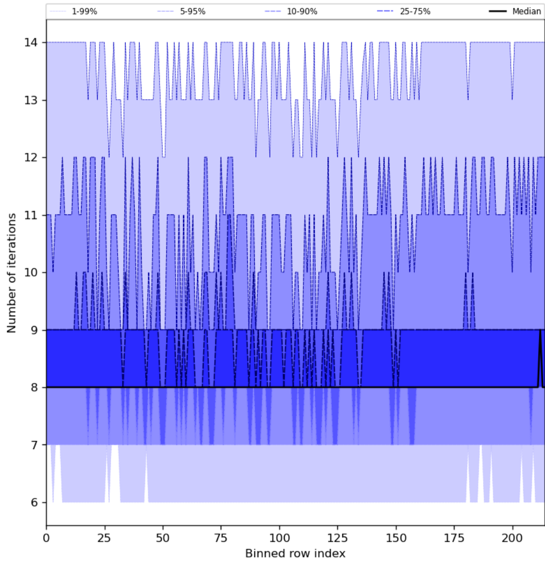
Figure 32: Along track statistics of “Number of iterations” for 2024-04-30 to 2024-05-02
