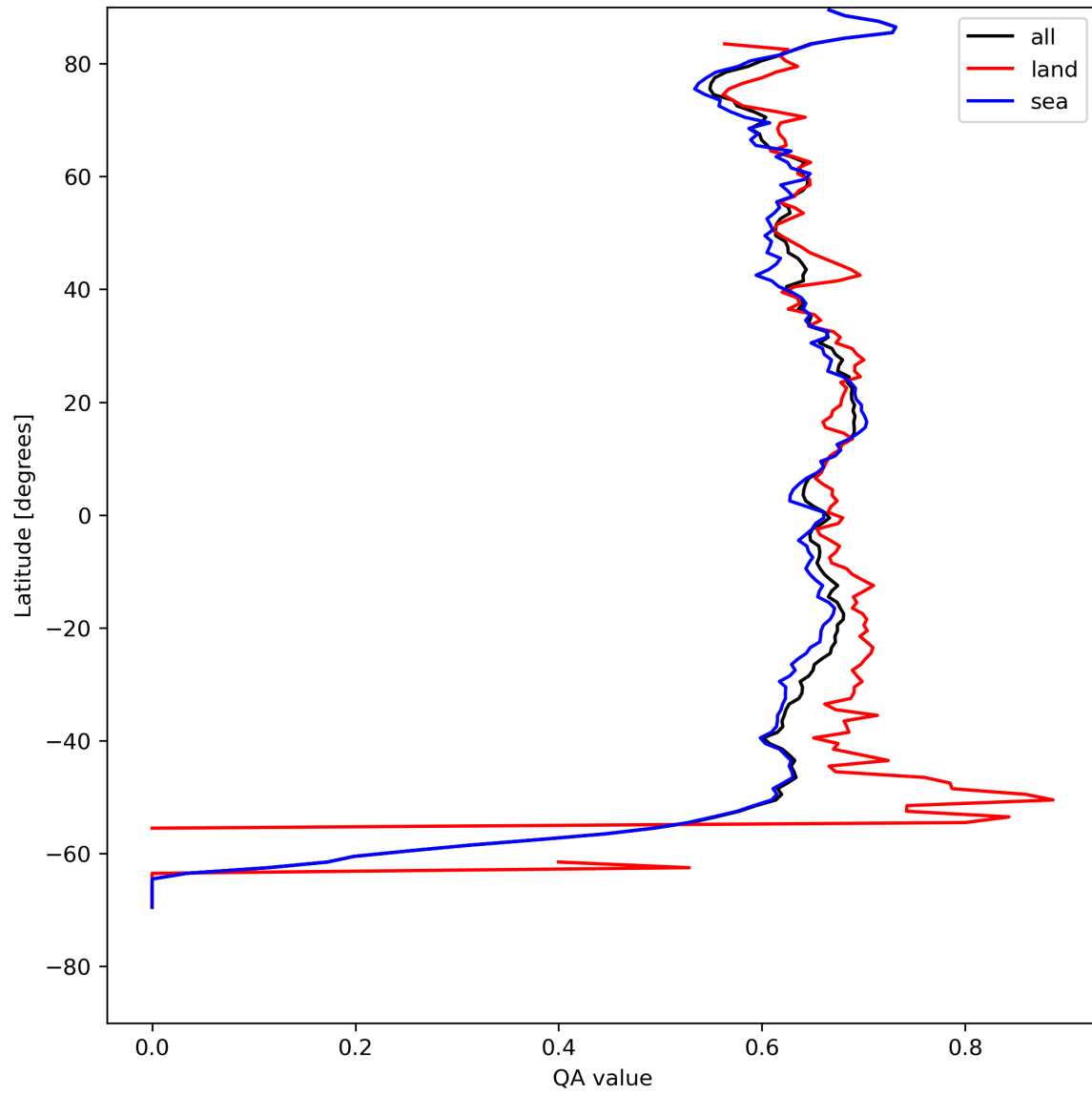
Figure 9: Zonal average of “QA value” for 2024-04-30 to 2024-05-02.
