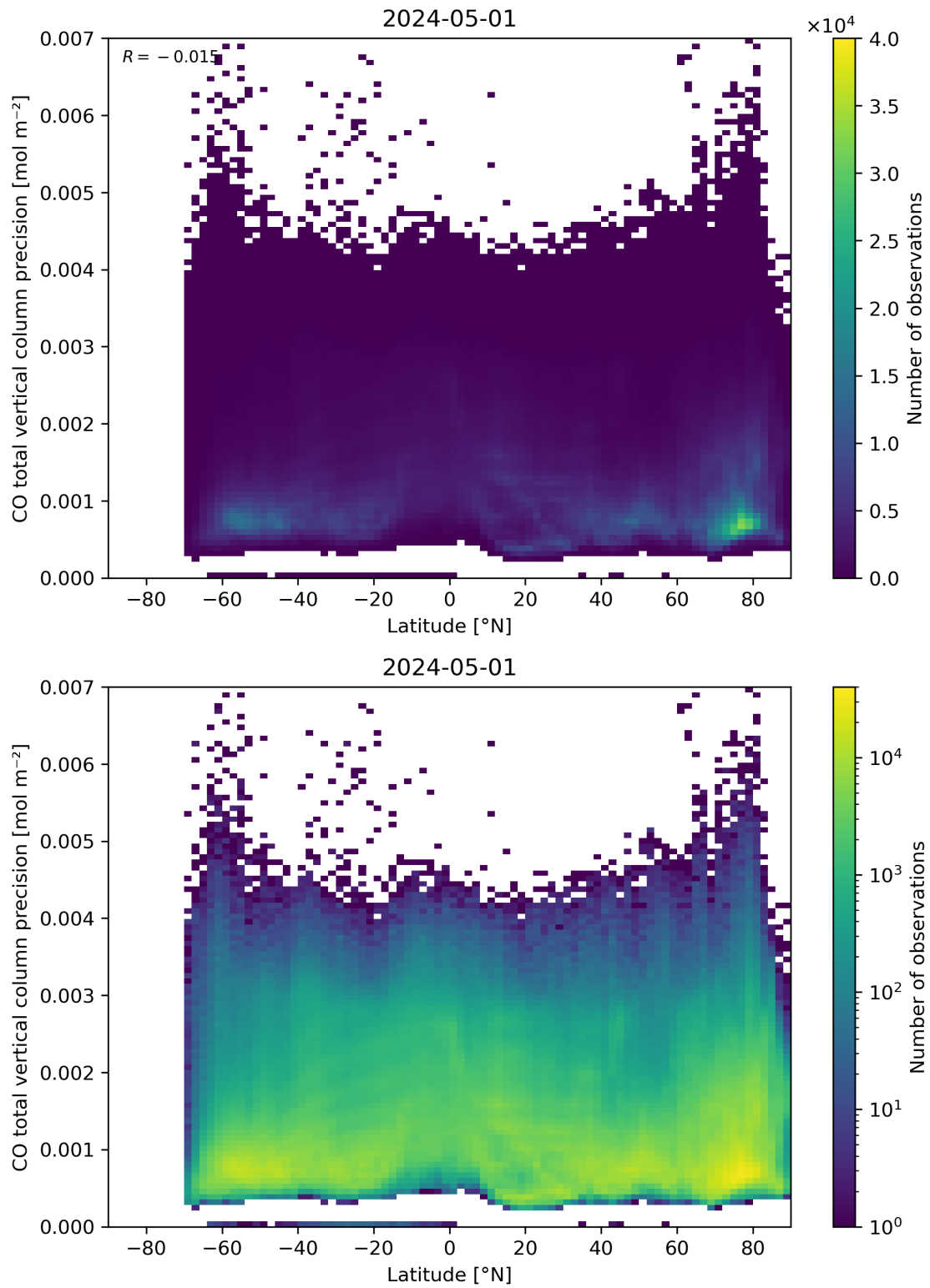
Figure 53: Scatter density plot of “Latitude” against “CO total vertical column precision” for 2024-04-30 to 2024-05-02.
