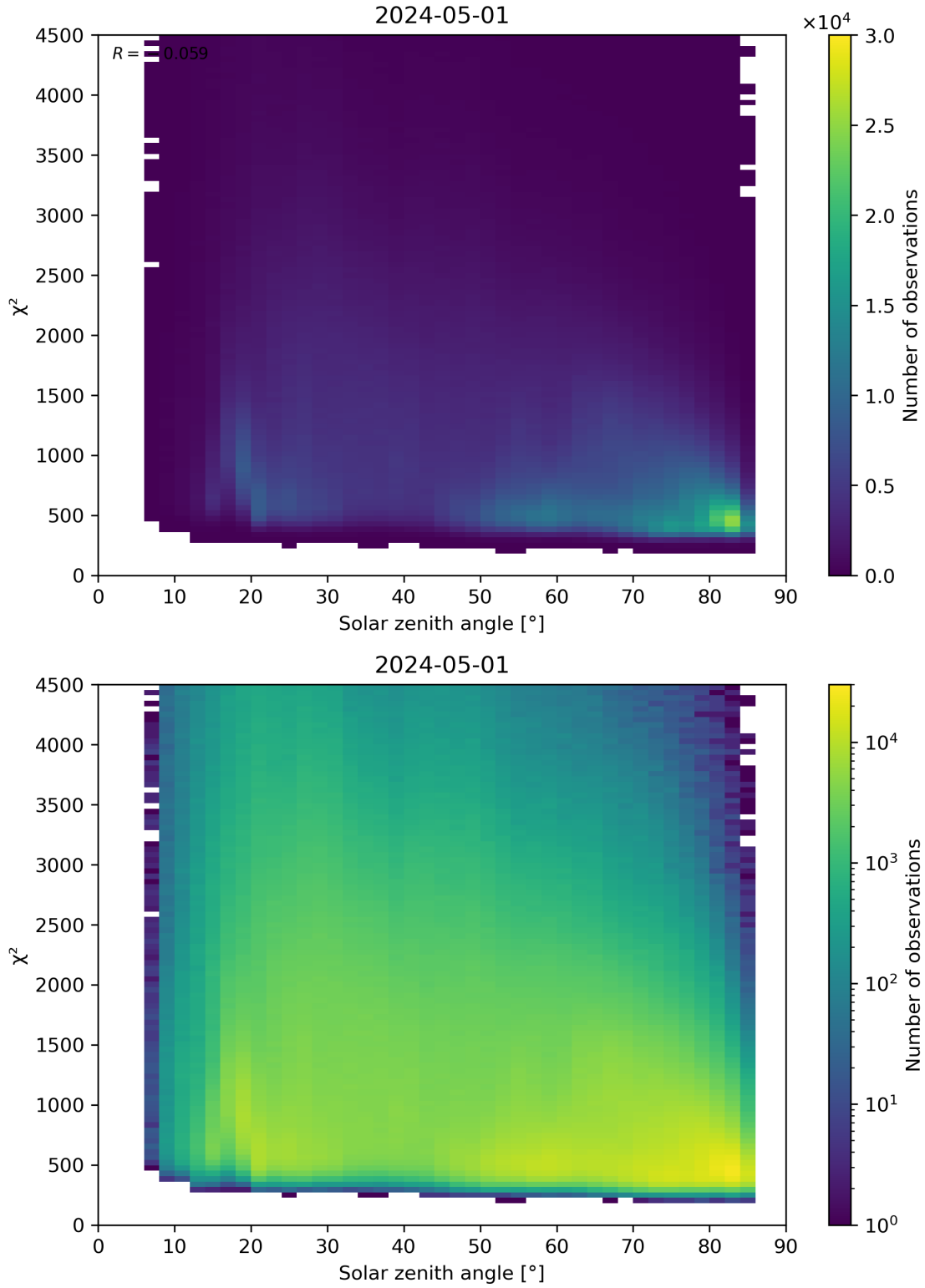
Figure 64: Scatter density plot of “Solar zenith angle” against “ \chi^2 ” for 2024-04-30 to 2024-05-02.
