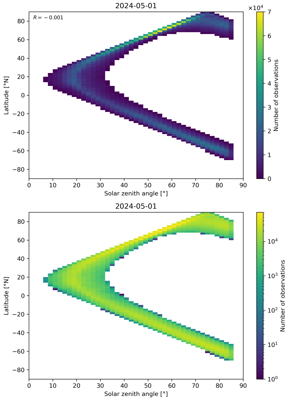
Figure 66: Scatter density plot of “Solar zenith angle” against “Latitude” for 2024-04-30 to 2024-05-02.
