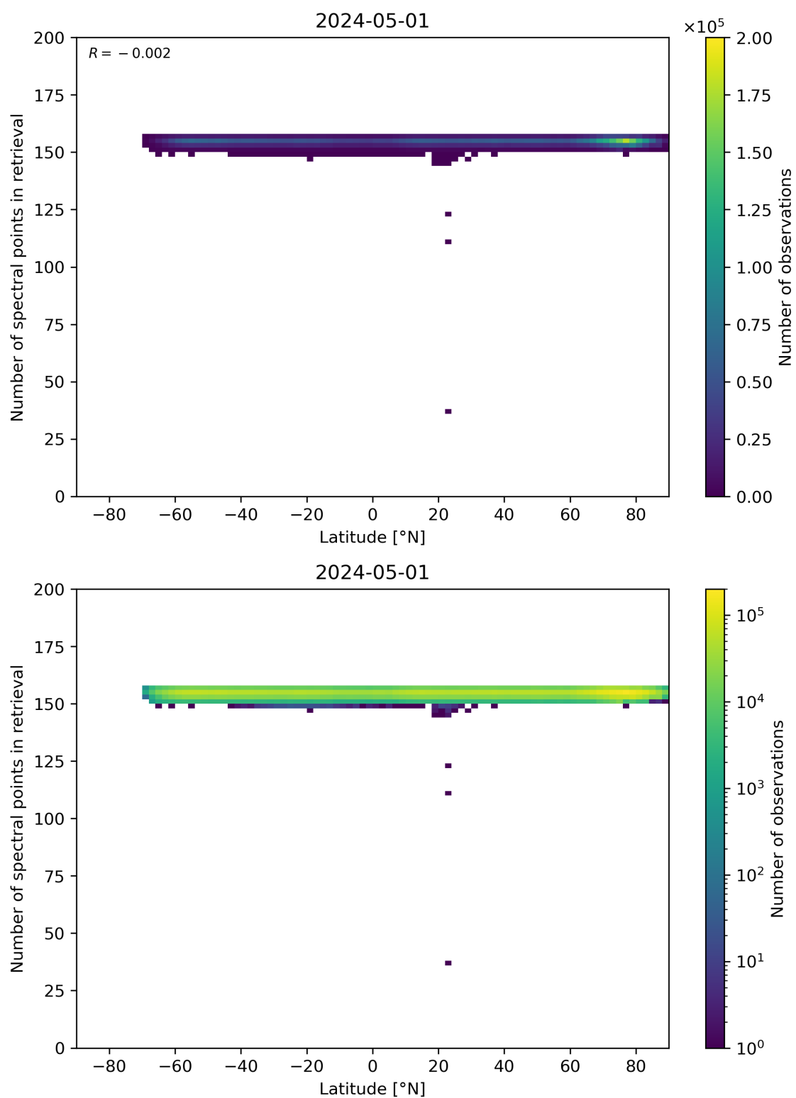
Figure 57: Scatter density plot of “Latitude” against “Number of spectral points in retrieval” for 2024-04-30 to 2024-05-02.
