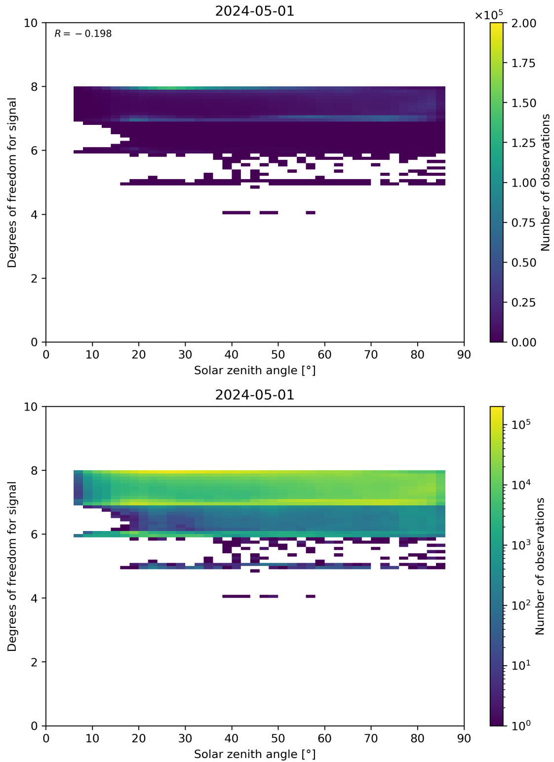
Figure 65: Scatter density plot of “Solar zenith angle” against “Degrees of freedom for signal” for 2024-04-30 to 2024-05-02.
