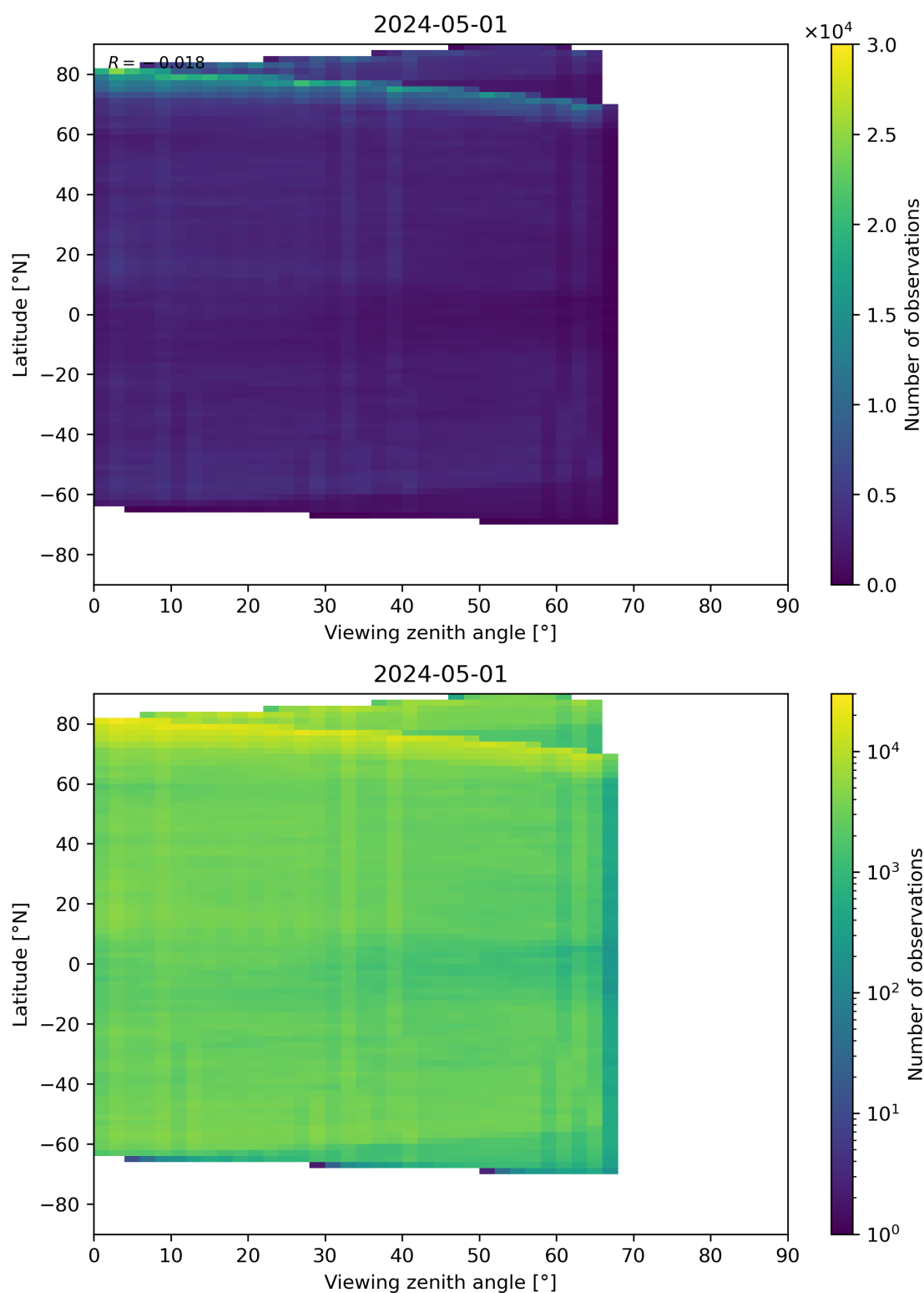
Figure 74: Scatter density plot of “Viewing zenith angle” against “Latitude” for 2024-04-30 to 2024-05-02.
