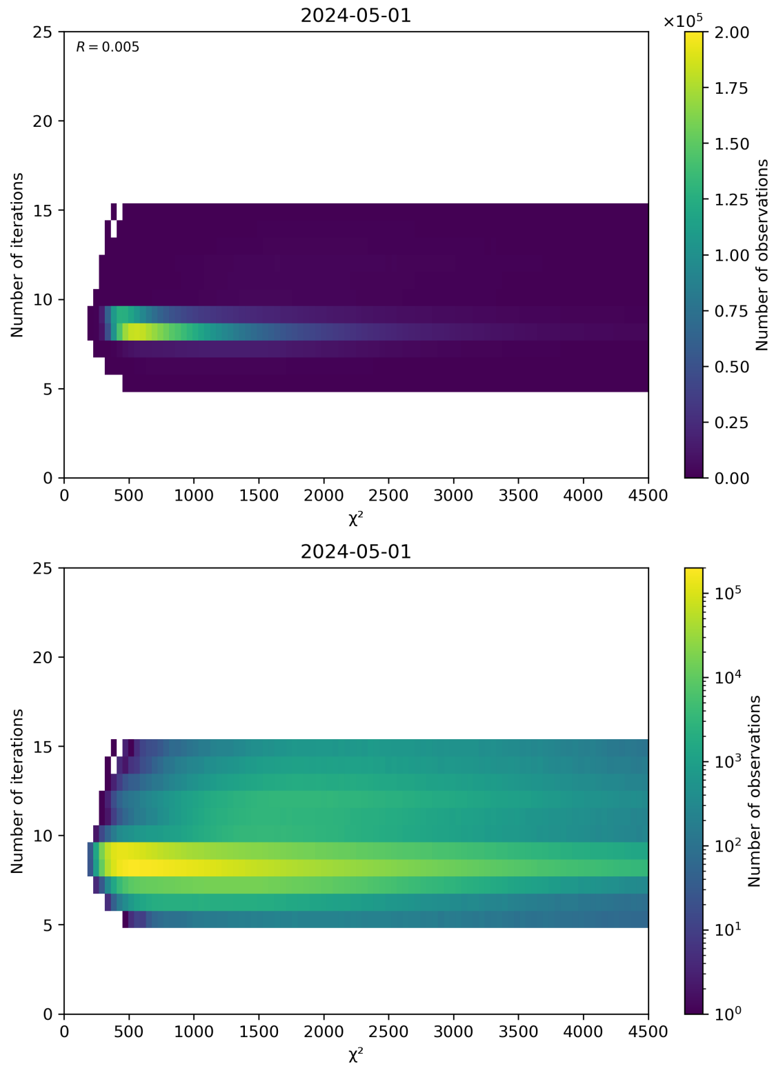
Figure 49: Scatter density plot of “ \chi^2 ” against “Number of iterations” for 2024-04-30 to 2024-05-02.
