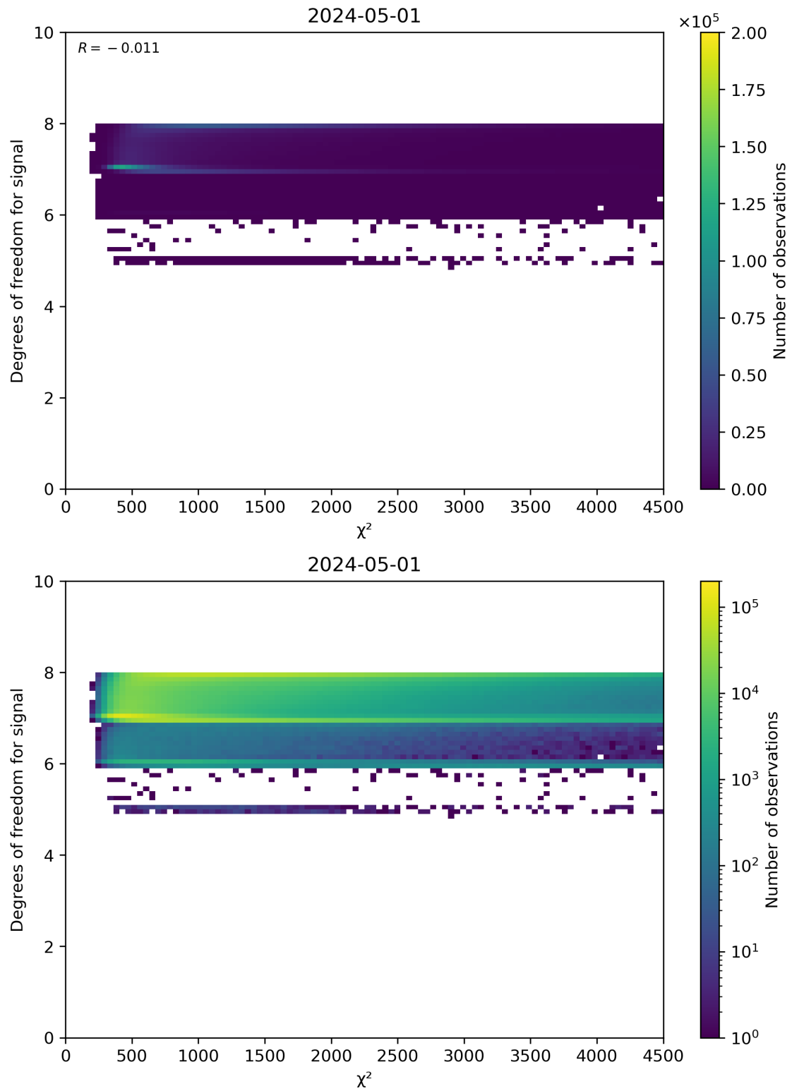
Figure 48: Scatter density plot of “ \chi^2 ” against “Degrees of freedom for signal” for 2024-04-30 to 2024-05-02.
