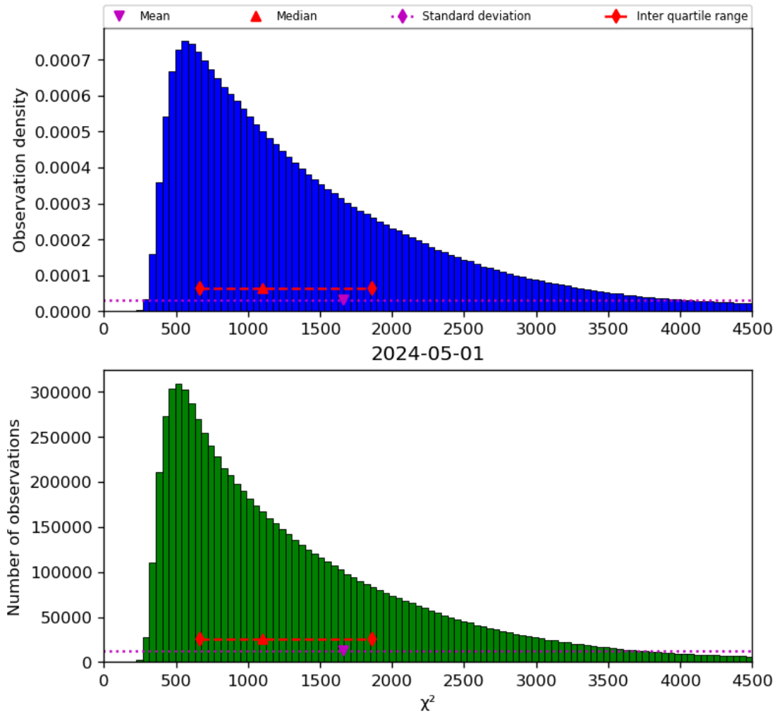
Figure 22: Histogram of “ \chi^2 ” for 2024-04-30 to 2024-05-02
