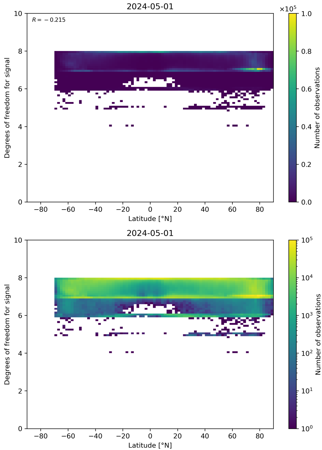
Figure 55: Scatter density plot of “Latitude” against “Degrees of freedom for signal” for 2024-04-30 to 2024-05-02.
