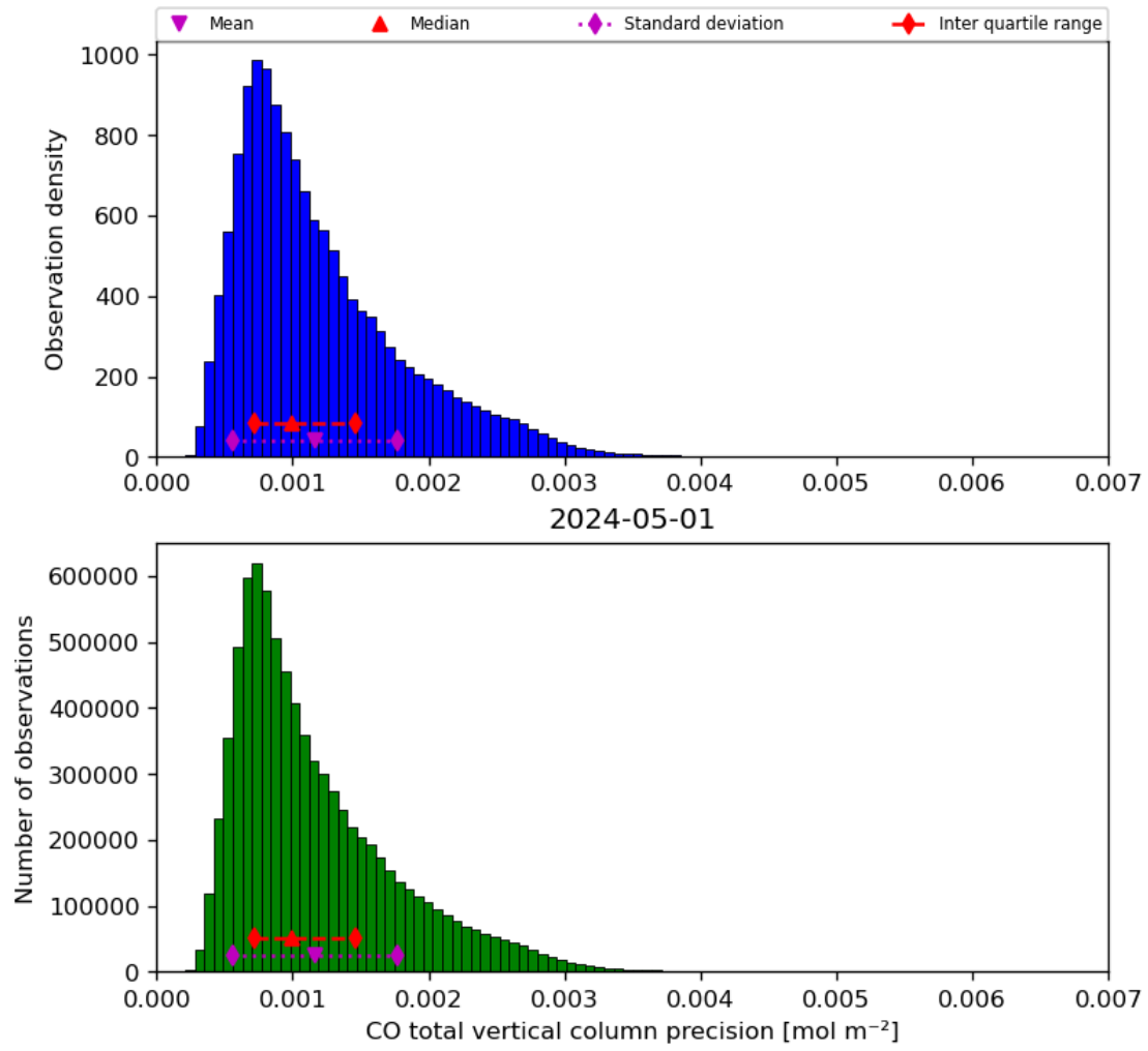
Figure 20: Histogram of “CO total vertical column precision” for 2024-04-30 to 2024-05-02
