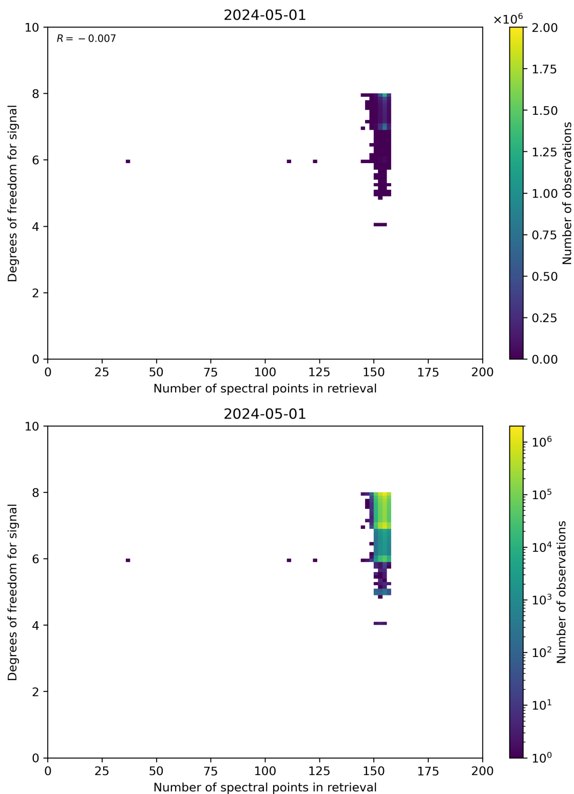
Figure 59: Scatter density plot of “Number of spectral points in retrieval” against “Degrees of freedom for signal” for 2024-04-30 to 2024-05-02.
