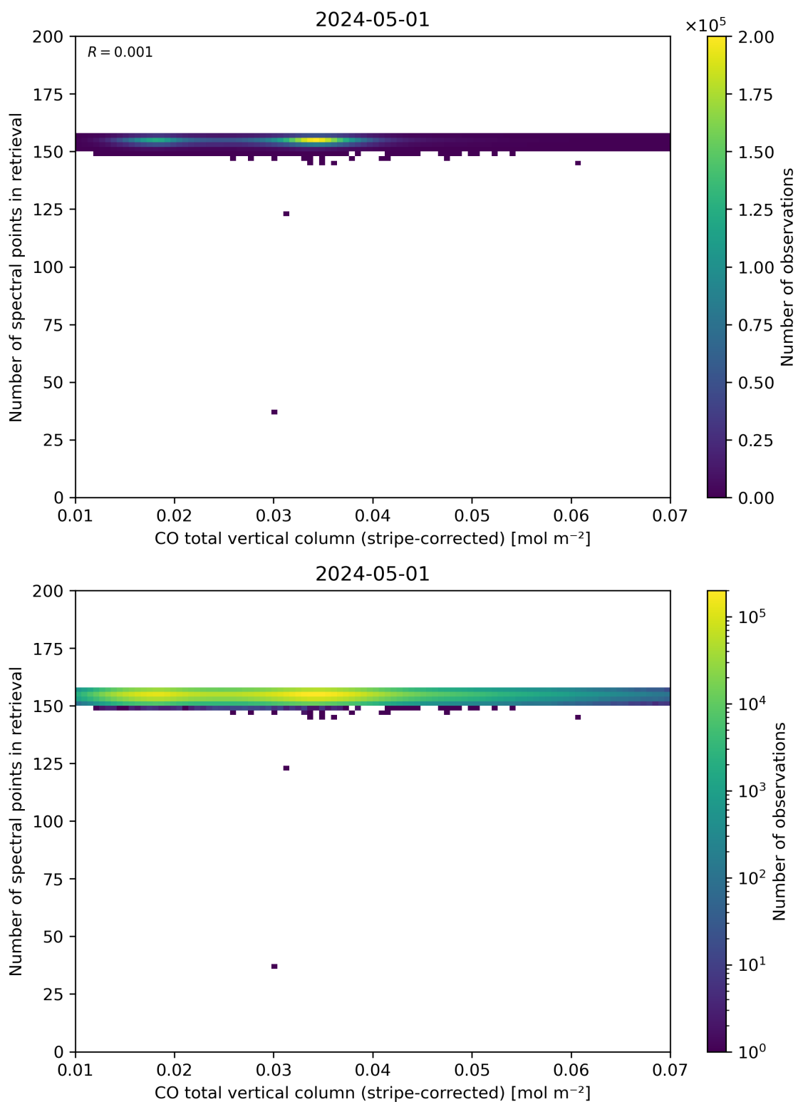
Figure 40: Scatter density plot of “CO total vertical column (stripe-corrected)” against “Number of spectral points in retrieval” for 2024-04-30 to 2024-05-02.
