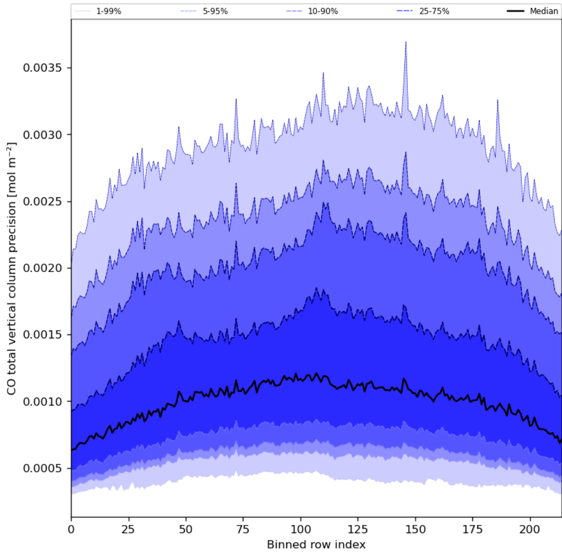
Figure 28: Along track statistics of “CO total vertical column precision” for 2024-04-30 to 2024-05-02
