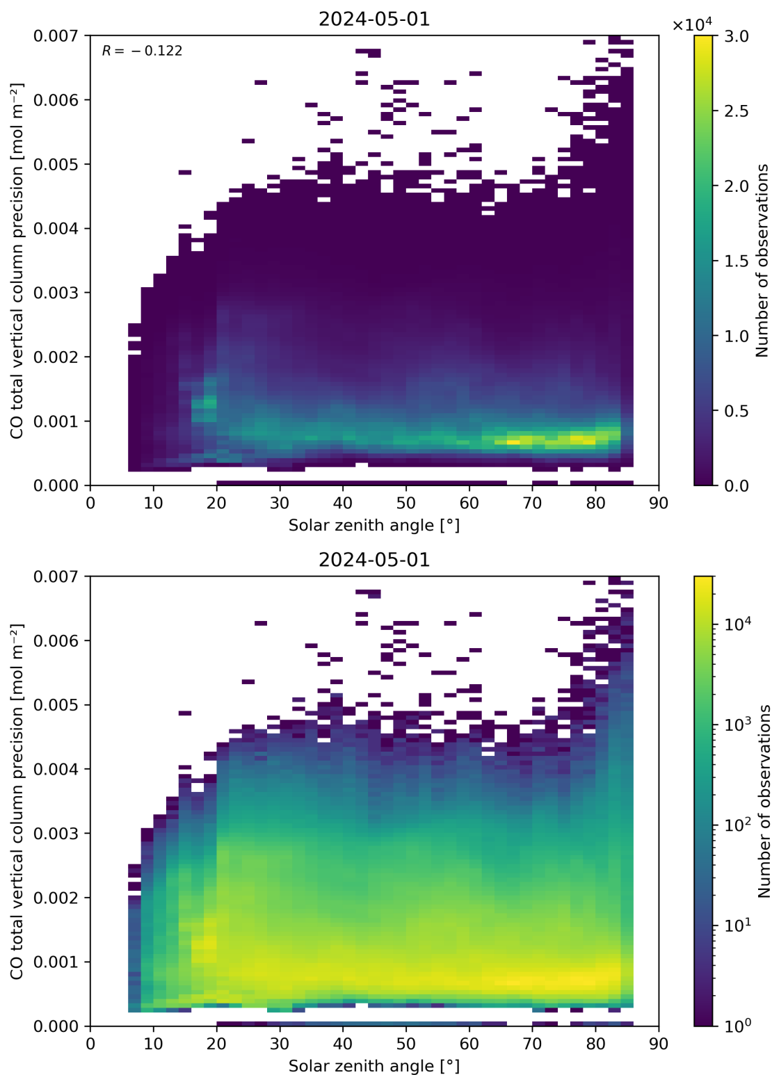
Figure 63: Scatter density plot of “Solar zenith angle” against “CO total vertical column precision” for 2024-04-30 to 2024-05-02.
