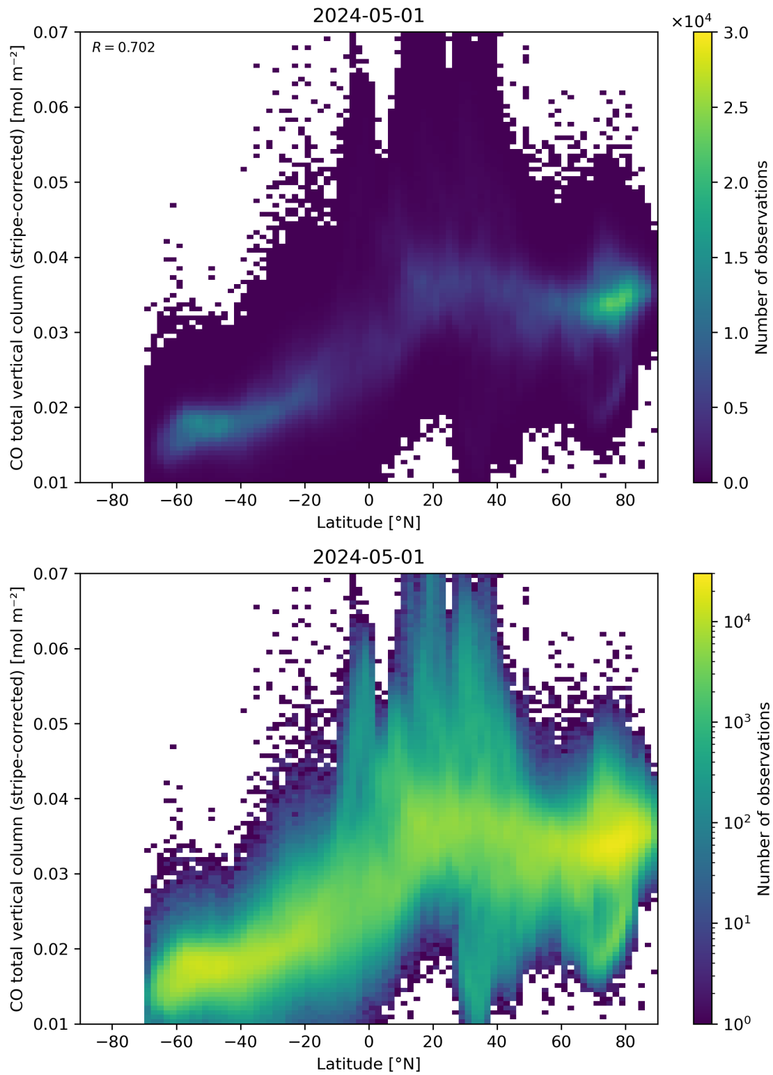
Figure 52: Scatter density plot of “Latitude” against “CO total vertical column (stripe-corrected)” for 2024-04-30 to 2024-05-02.
