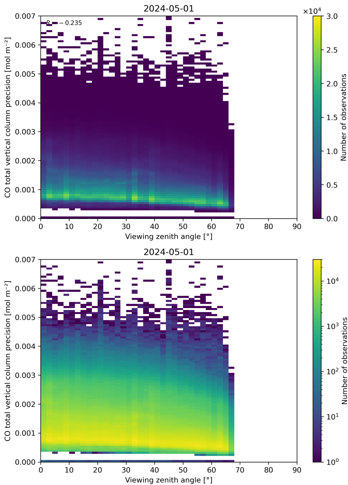
Figure 71: Scatter density plot of “Viewing zenith angle” against “CO total vertical column precision” for 2024-04-30 to 2024-05-02.
