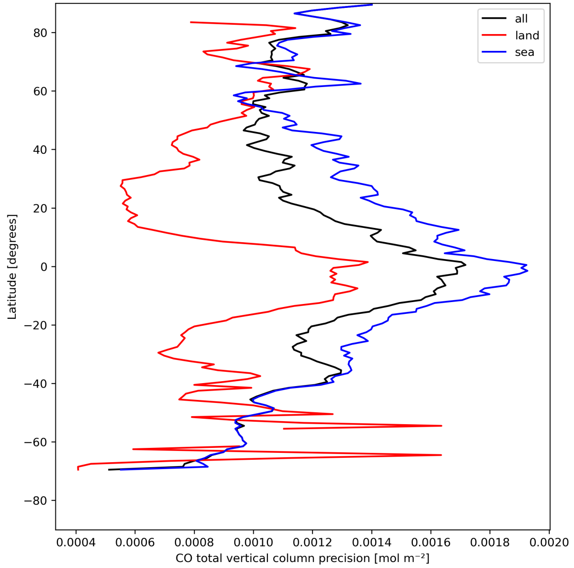
Figure 12: Zonal average of “CO total vertical column precision” for 2024-04-30 to 2024-05-02.
