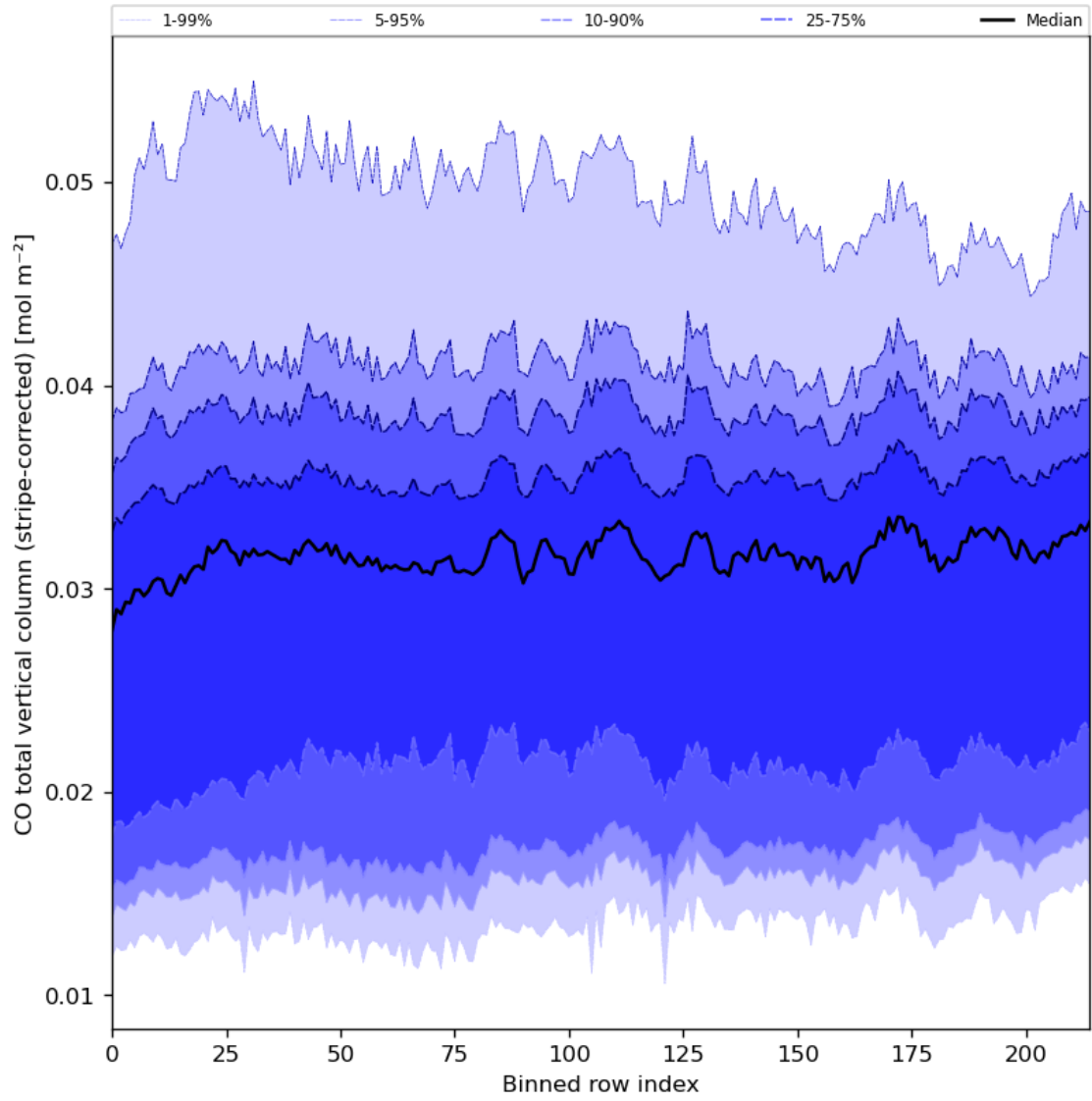
Figure 27: Along track statistics of “CO total vertical column (stripe-corrected)” for 2024-04-30 to 2024-05-02
