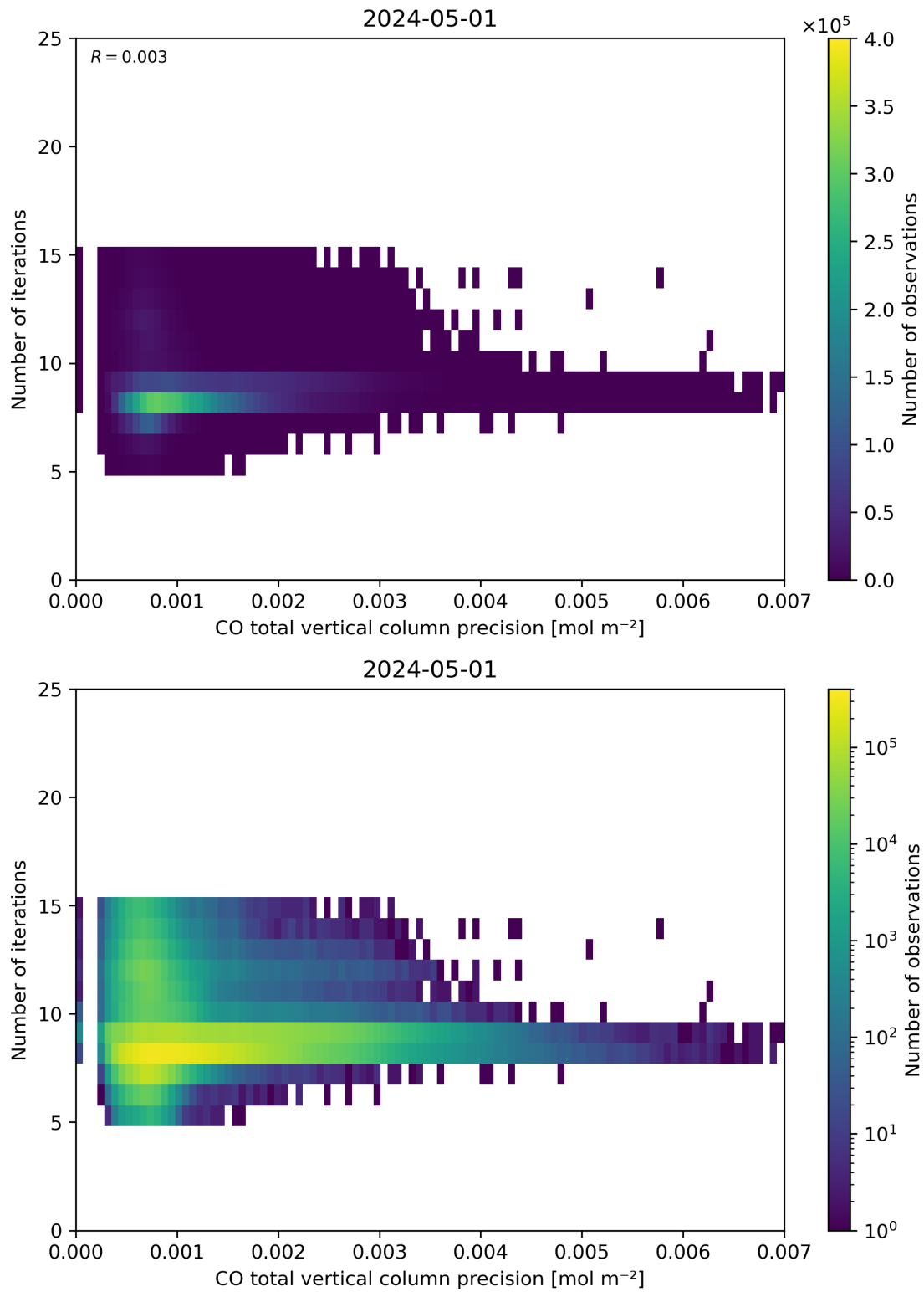
Figure 46: Scatter density plot of “CO total vertical column precision” against “Number of iterations” for 2024-04-30 to 2024-05-02.
