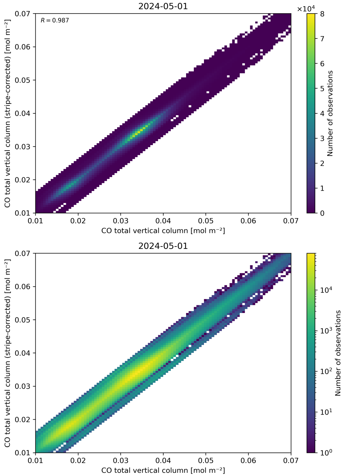
Figure 33: Scatter density plot of “CO total vertical column” against “CO total vertical column (stripe-corrected)” for 2024-04-30 to 2024-05-02.
