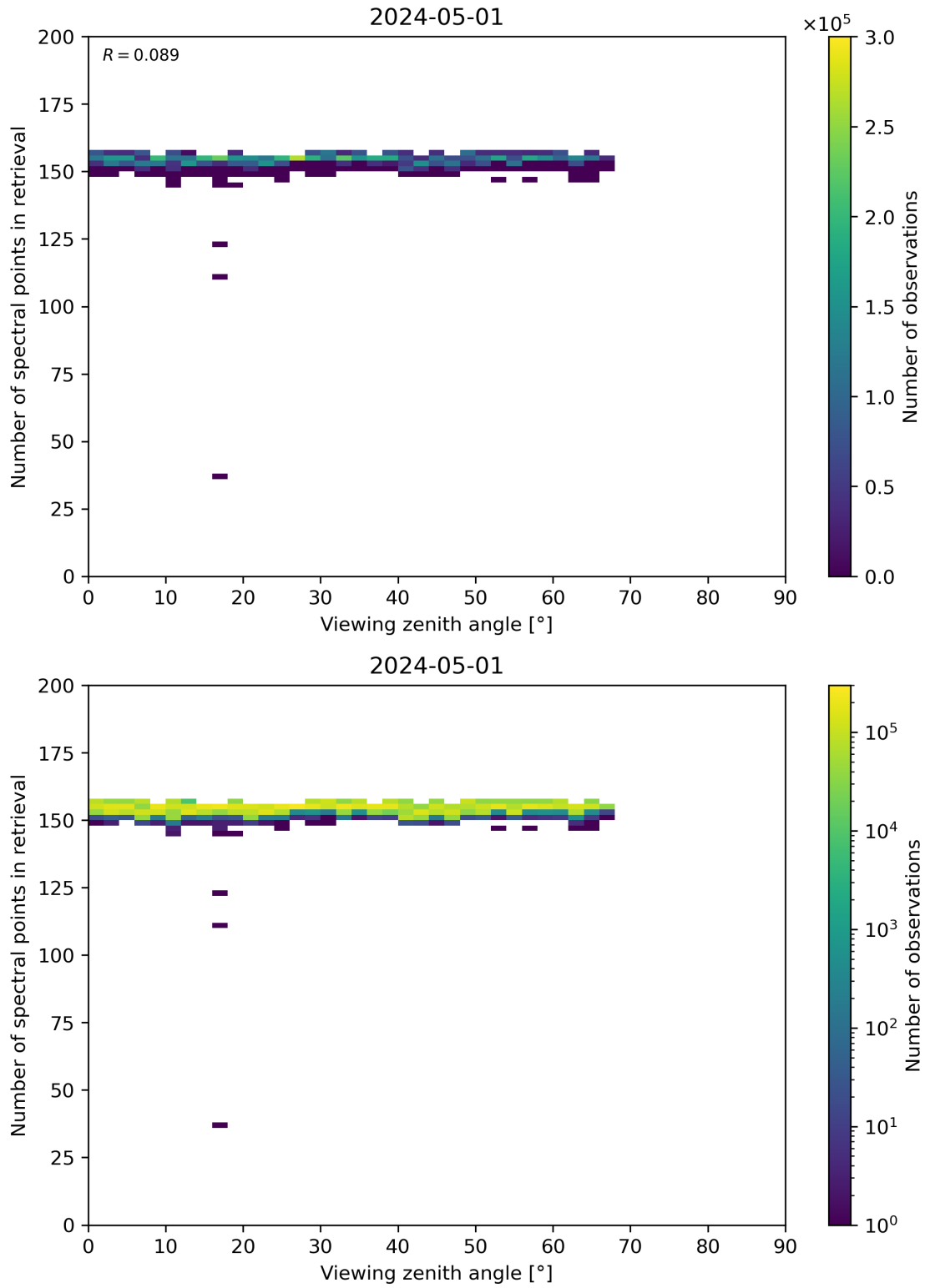
Figure 76: Scatter density plot of “Viewing zenith angle” against “Number of spectral points in retrieval” for 2024-04-30 to 2024-05-02.
