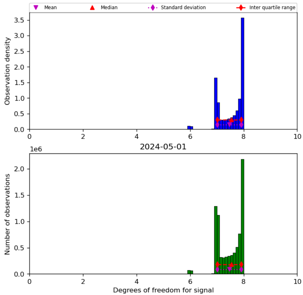
Figure 23: Histogram of “Degrees of freedom for signal” for 2024-04-30 to 2024-05-02
