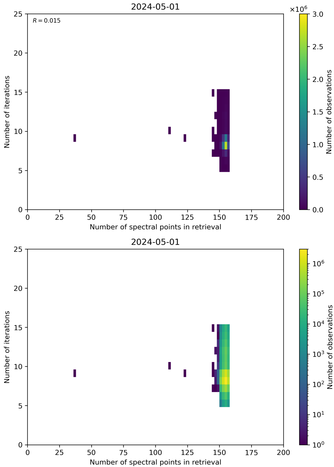
Figure 60: Scatter density plot of “Number of spectral points in retrieval” against “Number of iterations” for 2024-04-30 to 2024-05-02.
