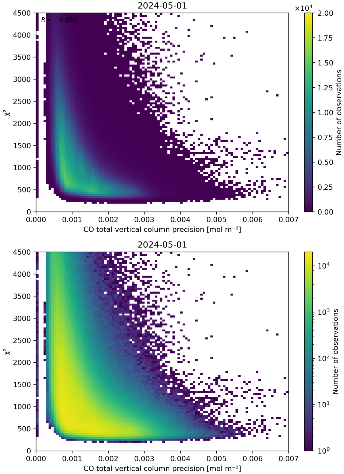
Figure 44: Scatter density plot of “CO total vertical column precision” against “ \chi^2 ” for 2024-04-30 to 2024-05-02.
