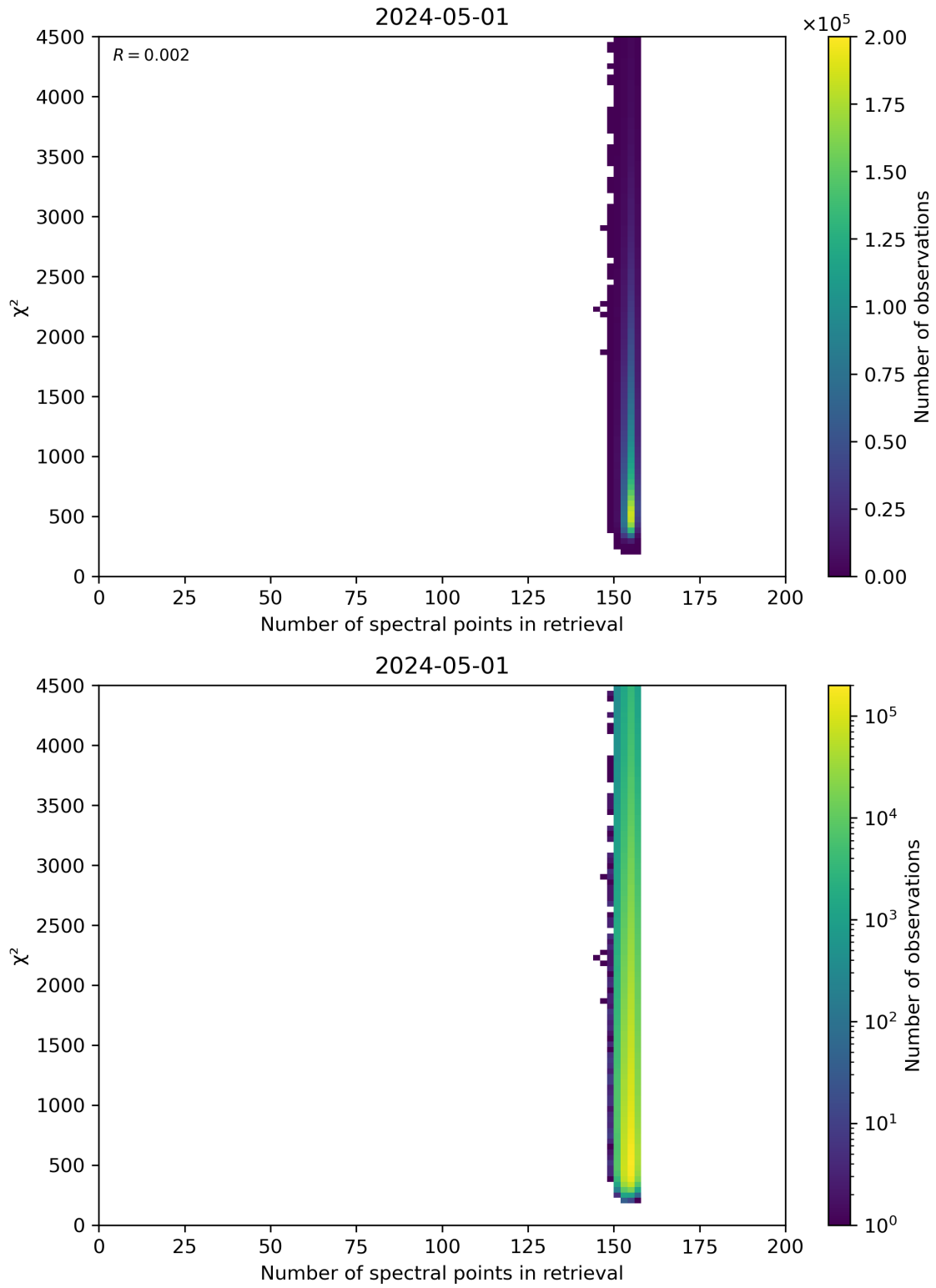
Figure 58: Scatter density plot of “Number of spectral points in retrieval” against “ \chi^2 ” for 2024-04-30 to 2024-05-02.
