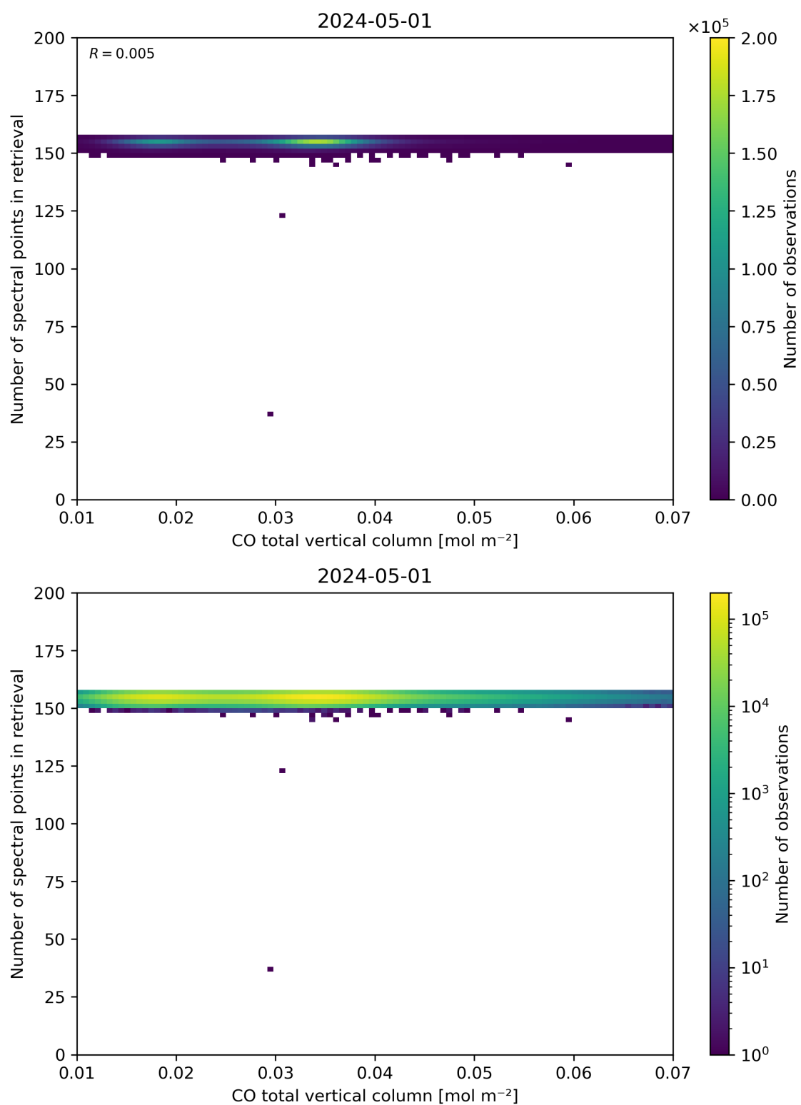
Figure 43: Scatter density plot of “CO total vertical column” against “Number of spectral points in retrieval” for 2024-04-30 to 2024-05-02.
