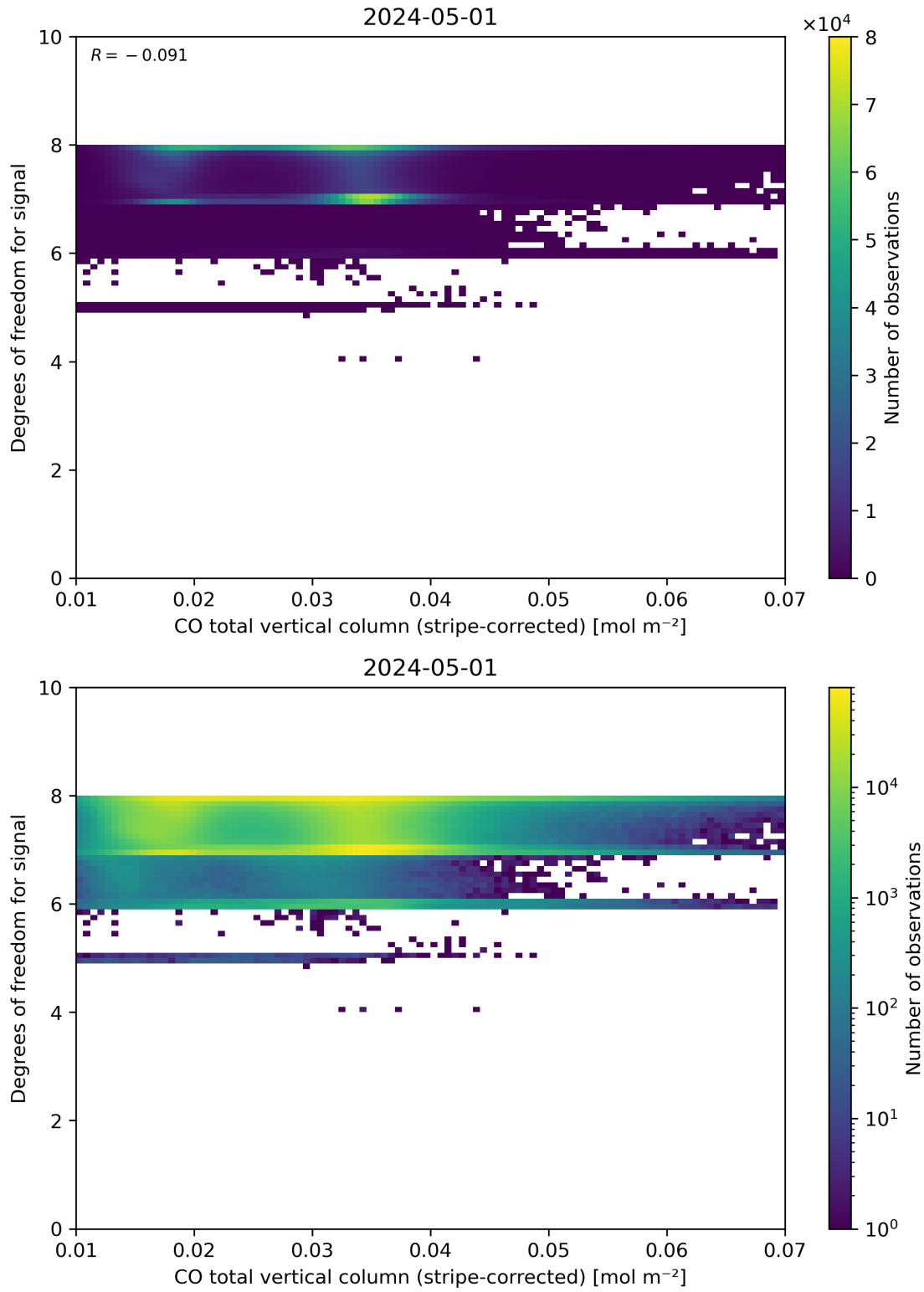
Figure 38: Scatter density plot of “CO total vertical column (stripe-corrected)” against “Degrees of freedom for signal” for 2024-04-30 to 2024-05-02.
