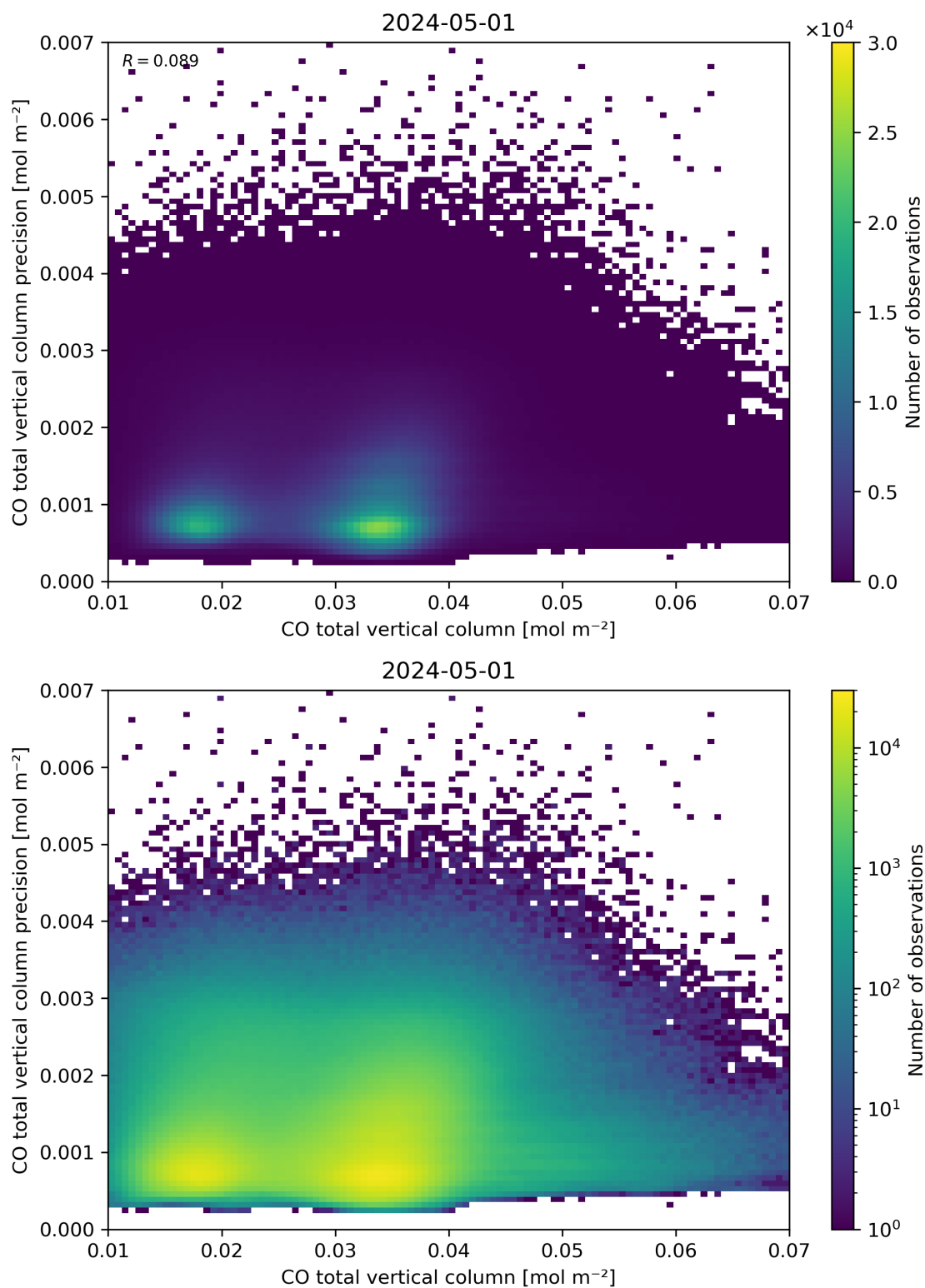
Figure 34: Scatter density plot of “CO total vertical column” against “CO total vertical column precision” for 2024-04-30 to 2024-05-02.
