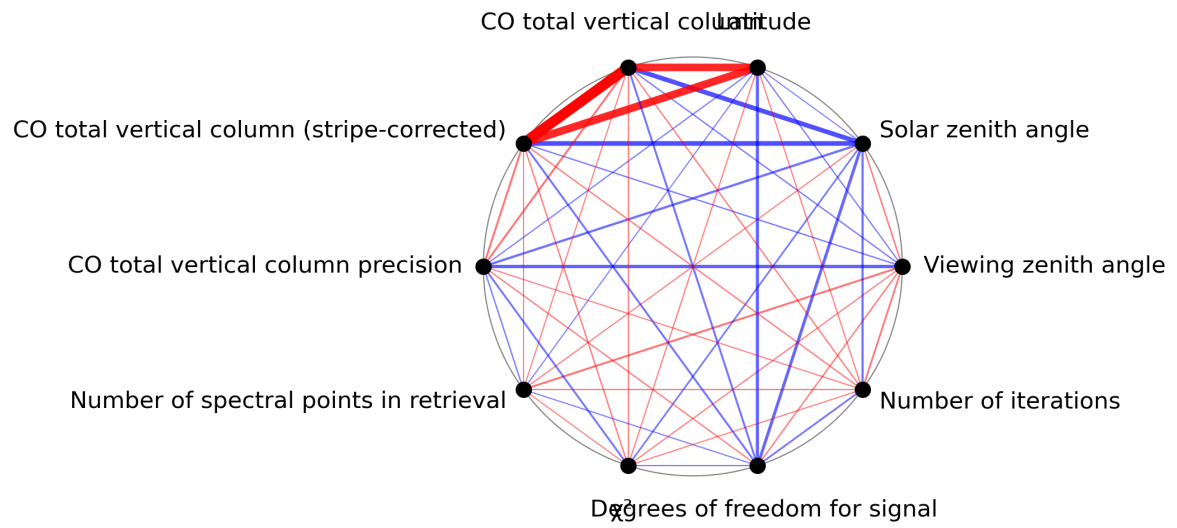
Figure 1: Map of correlation graph for 2024-04-30 to 2024-05-02.
