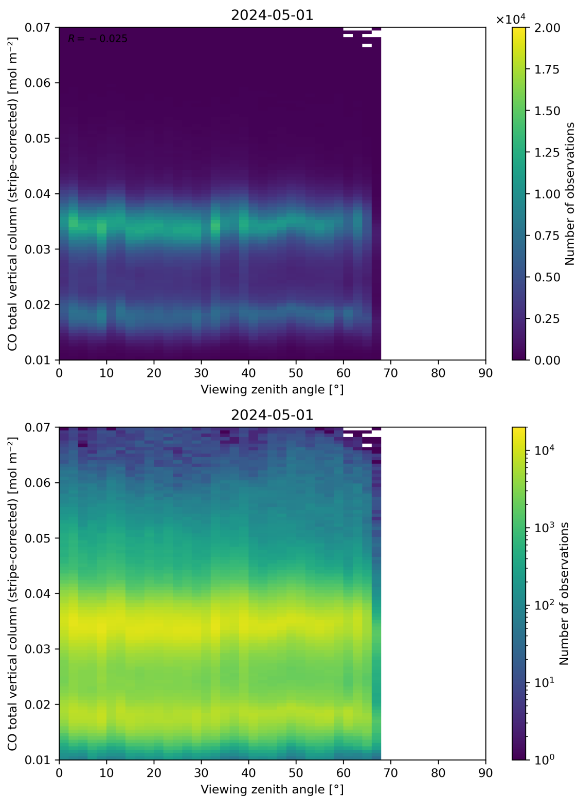
Figure 70: Scatter density plot of “Viewing zenith angle” against “CO total vertical column (stripe-corrected)” for 2024-04-30 to 2024-05-02.
