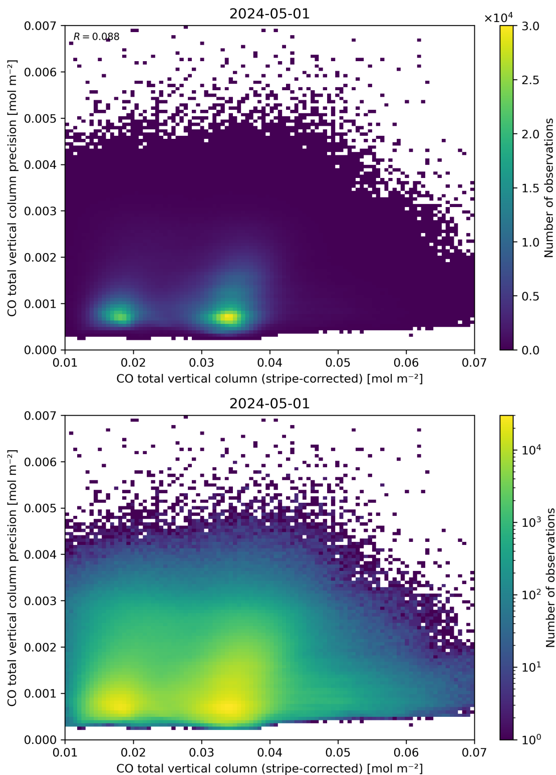
Figure 36: Scatter density plot of “CO total vertical column (stripe-corrected)” against “CO total vertical column precision” for 2024-04-30 to 2024-05-02.
