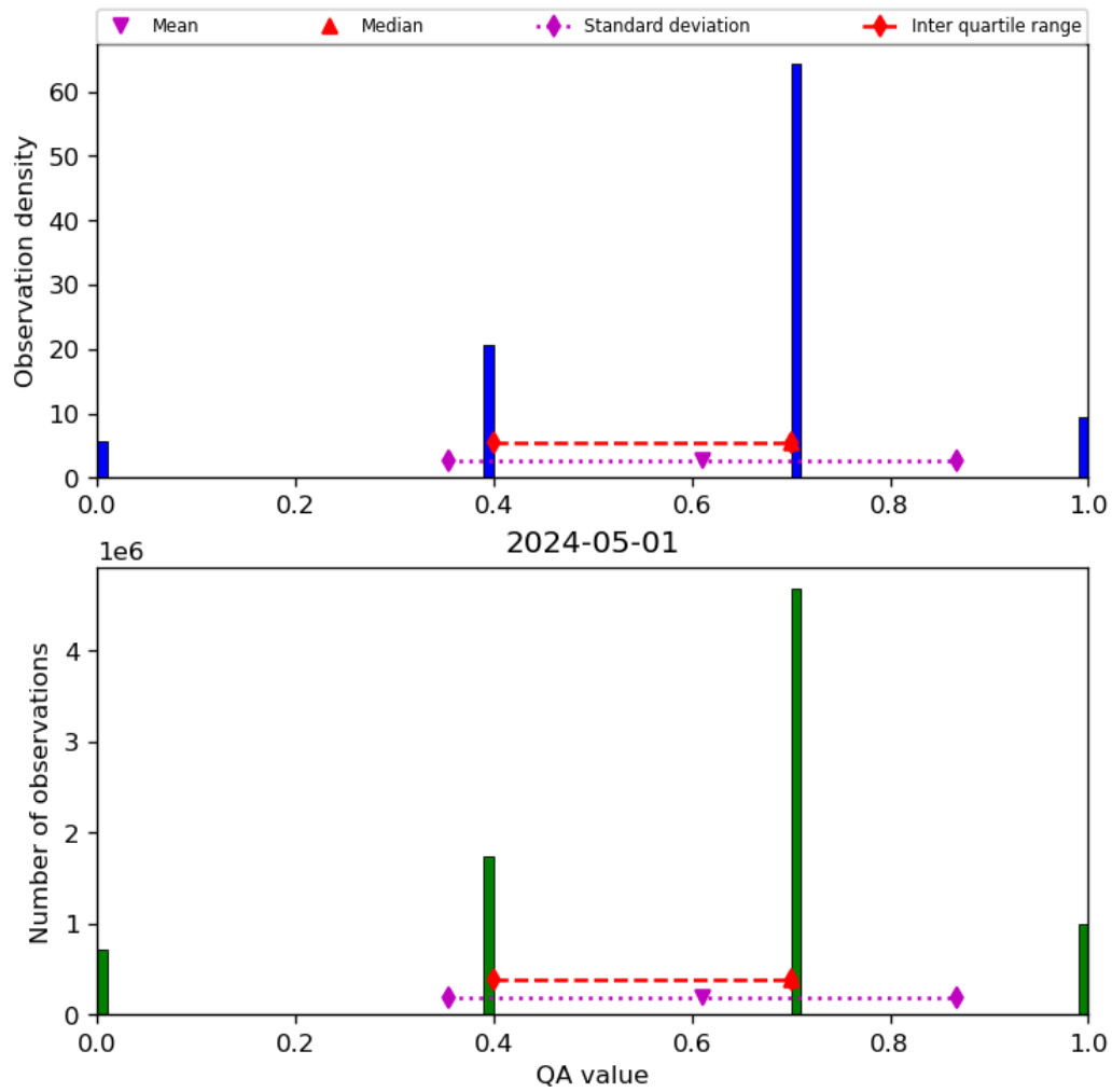
Figure 17: Histogram of “QA value” for 2024-04-30 to 2024-05-02
