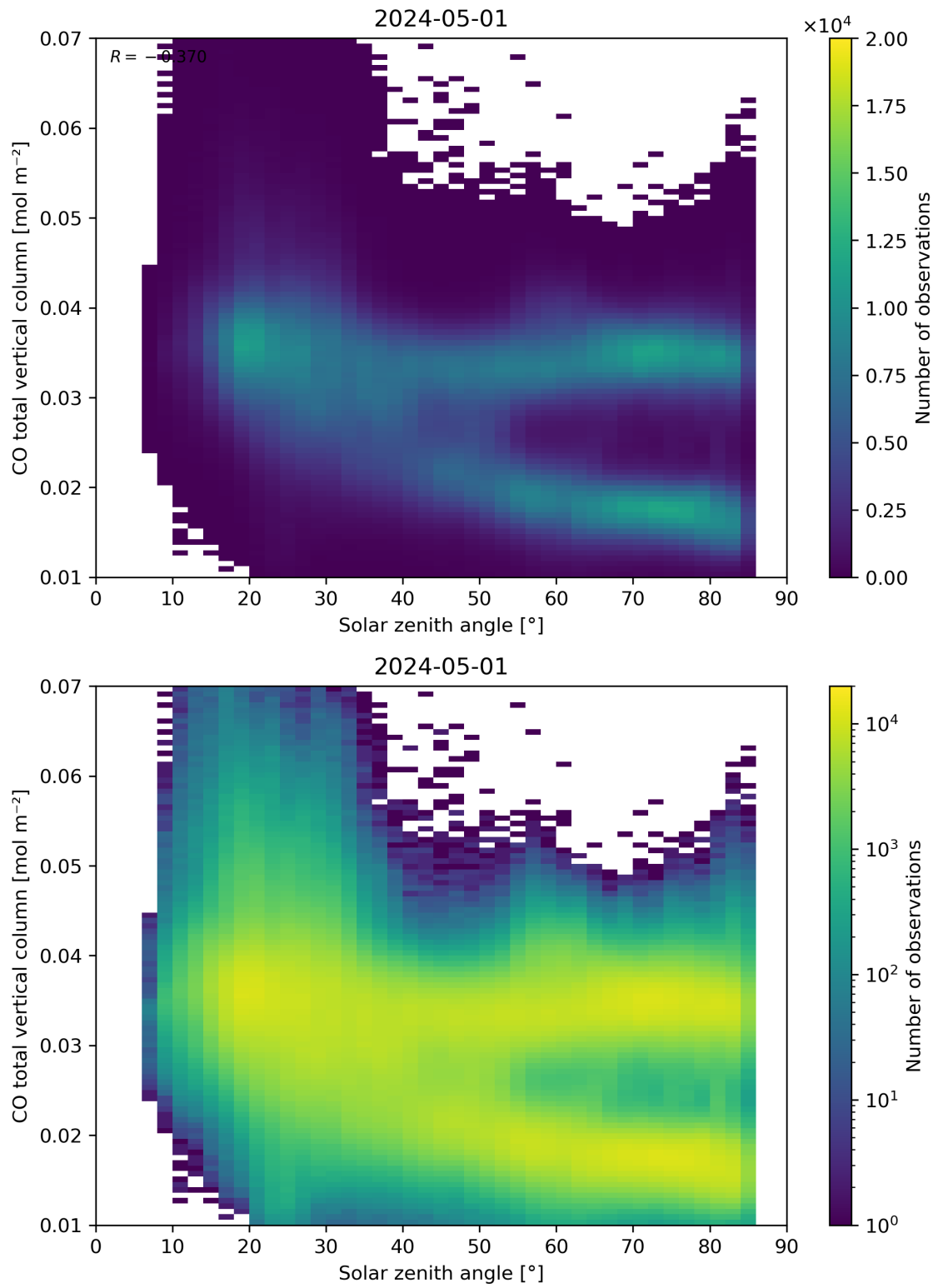
Figure 61: Scatter density plot of “Solar zenith angle” against “CO total vertical column” for 2024-04-30 to 2024-05-02.
