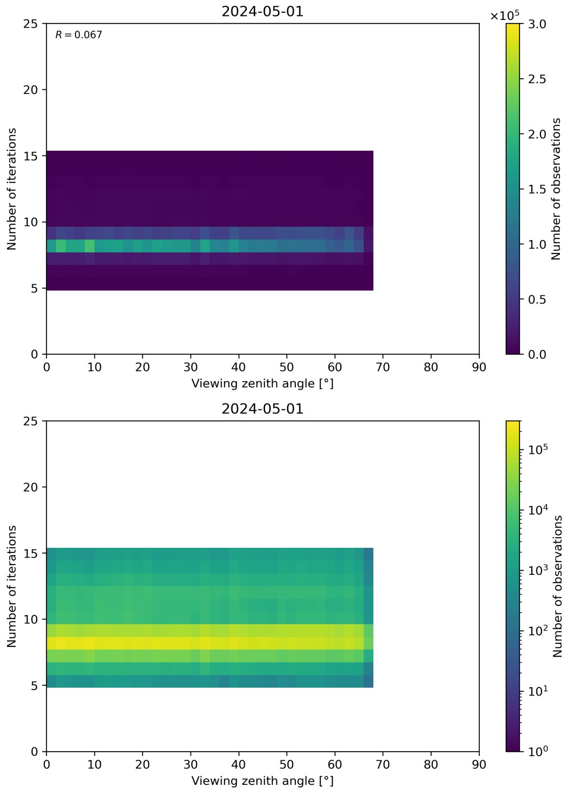
Figure 75: Scatter density plot of “Viewing zenith angle” against “Number of iterations” for 2024-04-30 to 2024-05-02.
