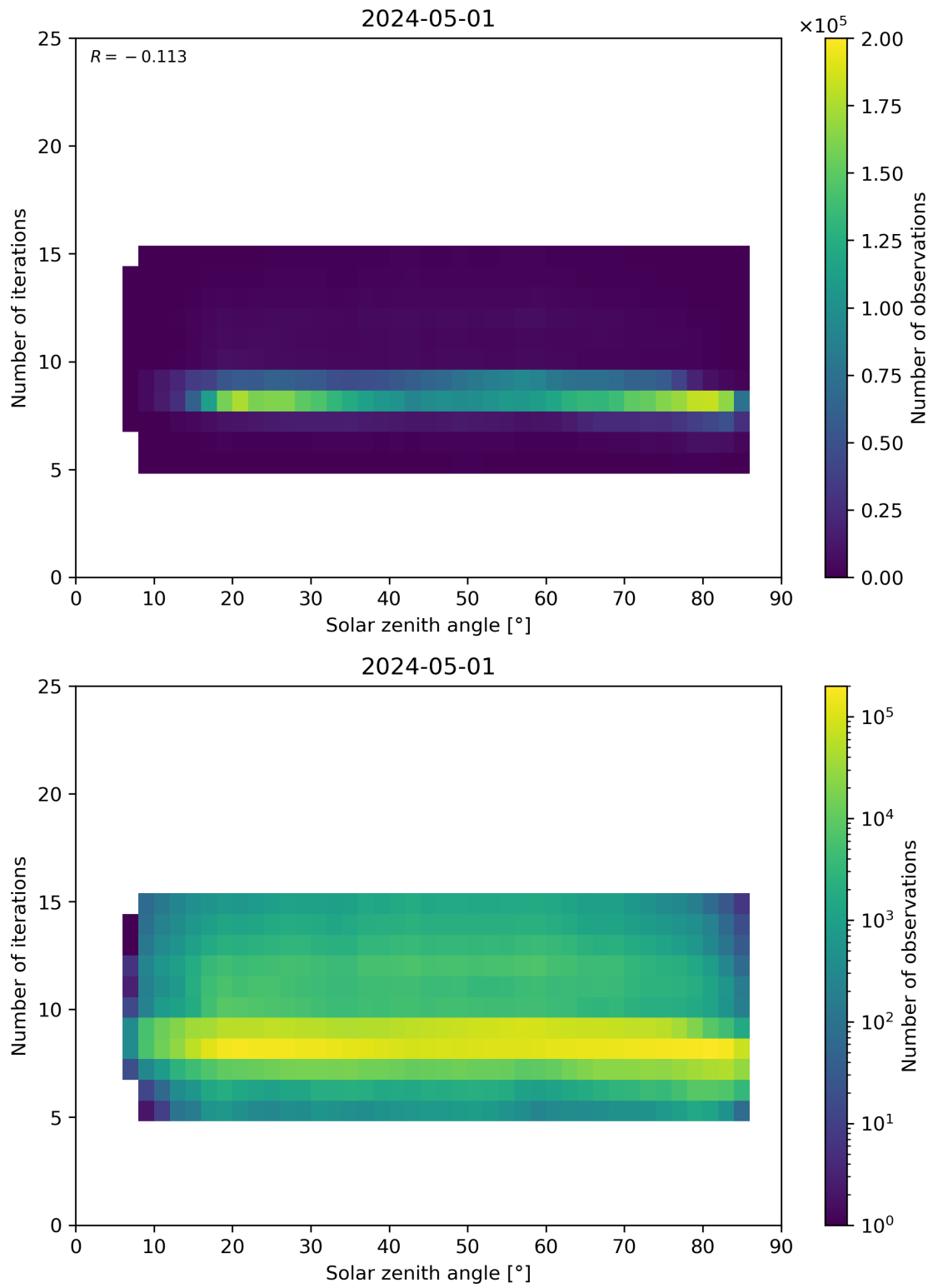
Figure 67: Scatter density plot of “Solar zenith angle” against “Number of iterations” for 2024-04-30 to 2024-05-02.
