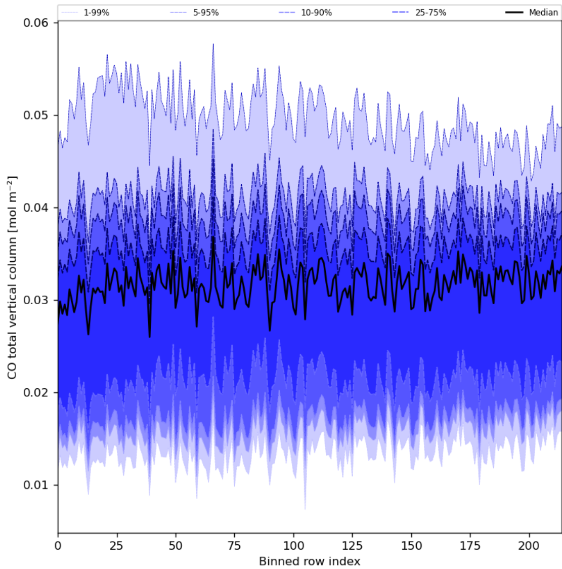
Figure 26: Along track statistics of “CO total vertical column” for 2024-04-30 to 2024-05-02
