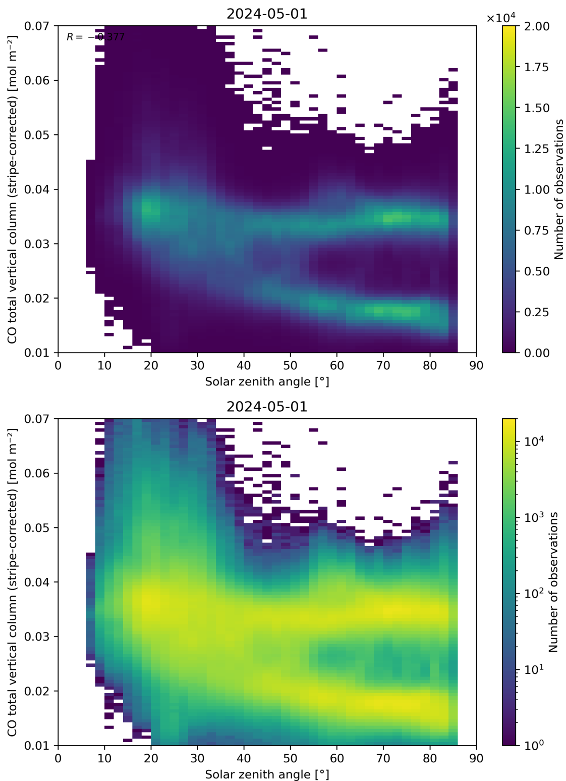
Figure 62: Scatter density plot of “Solar zenith angle” against “CO total vertical column (stripe-corrected)” for 2024-04-30 to 2024-05-02.
