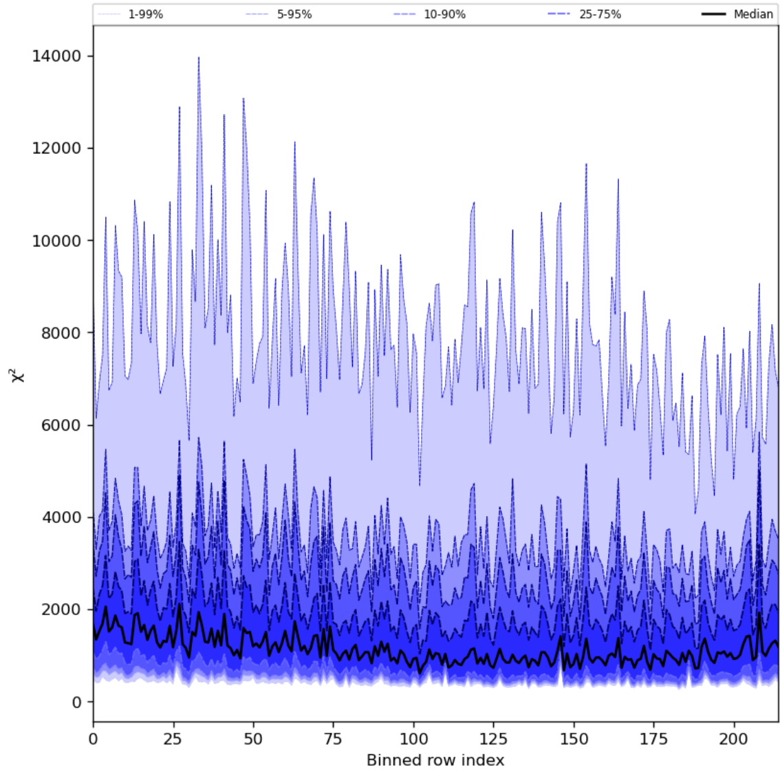
Figure 30: Along track statistics of “ \chi^2 ” for 2024-04-30 to 2024-05-02
