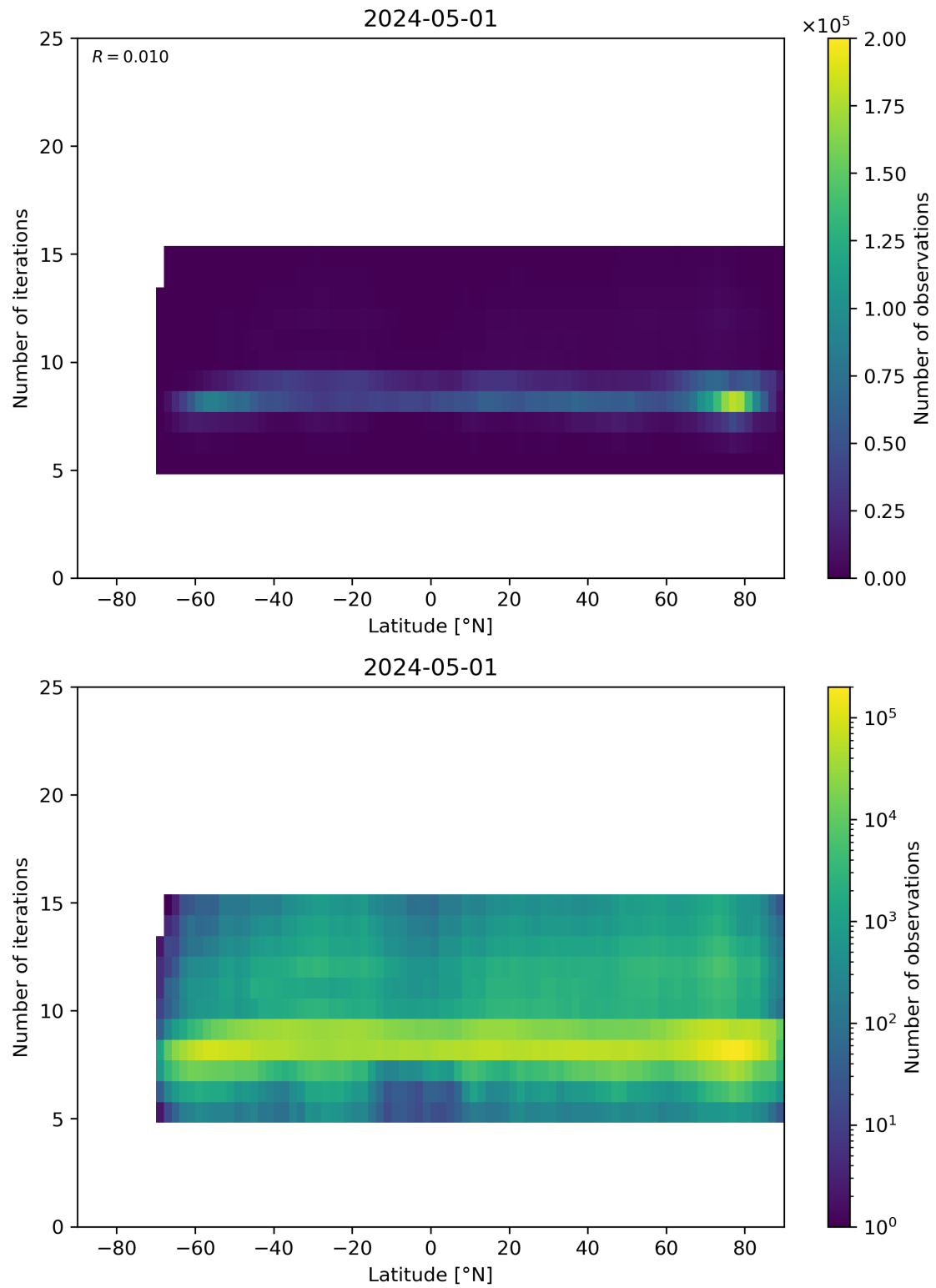
Figure 56: Scatter density plot of “Latitude” against “Number of iterations” for 2024-04-30 to 2024-05-02.
