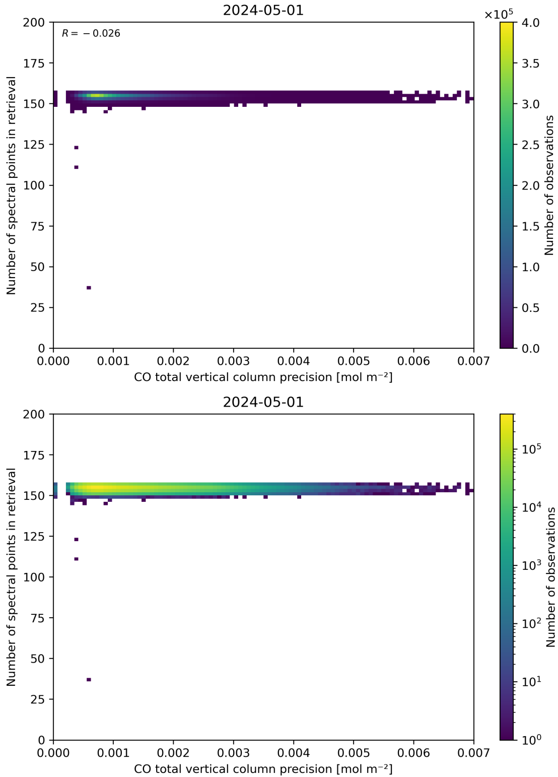
Figure 47: Scatter density plot of “CO total vertical column precision” against “Number of spectral points in retrieval” for 2024-04-30 to 2024-05-02.
