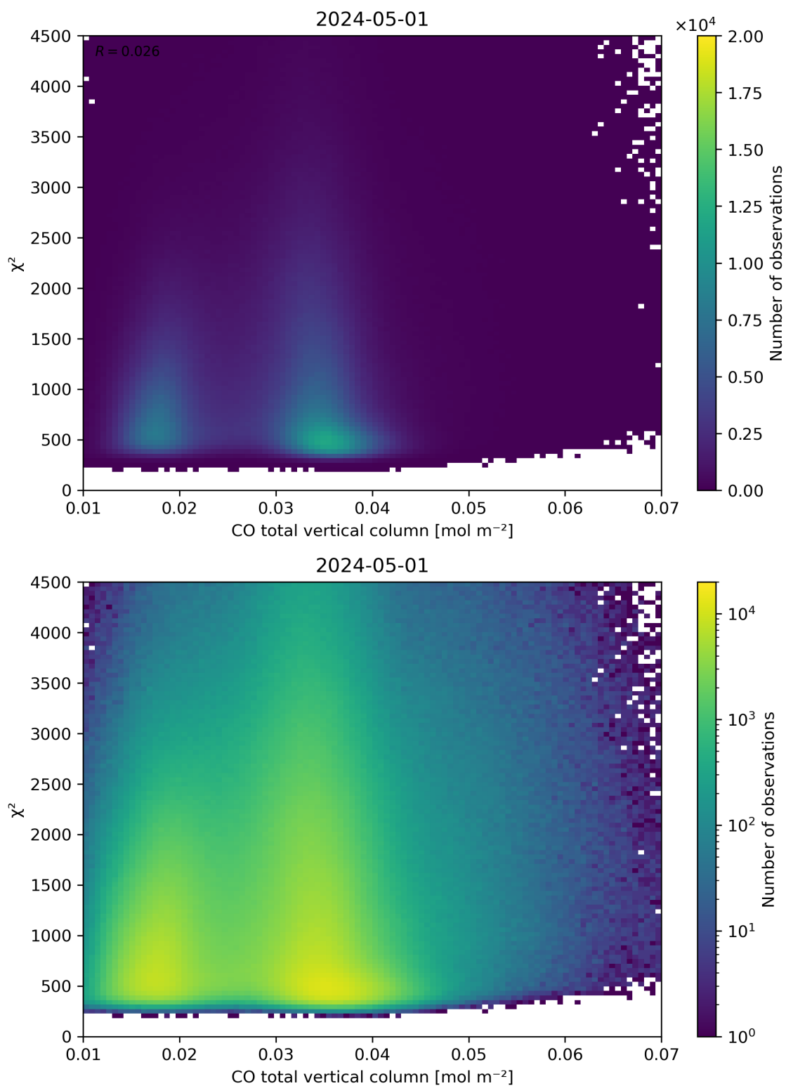
Figure 35: Scatter density plot of “CO total vertical column” against “ \chi^2 ” for 2024-04-30 to 2024-05-02.
