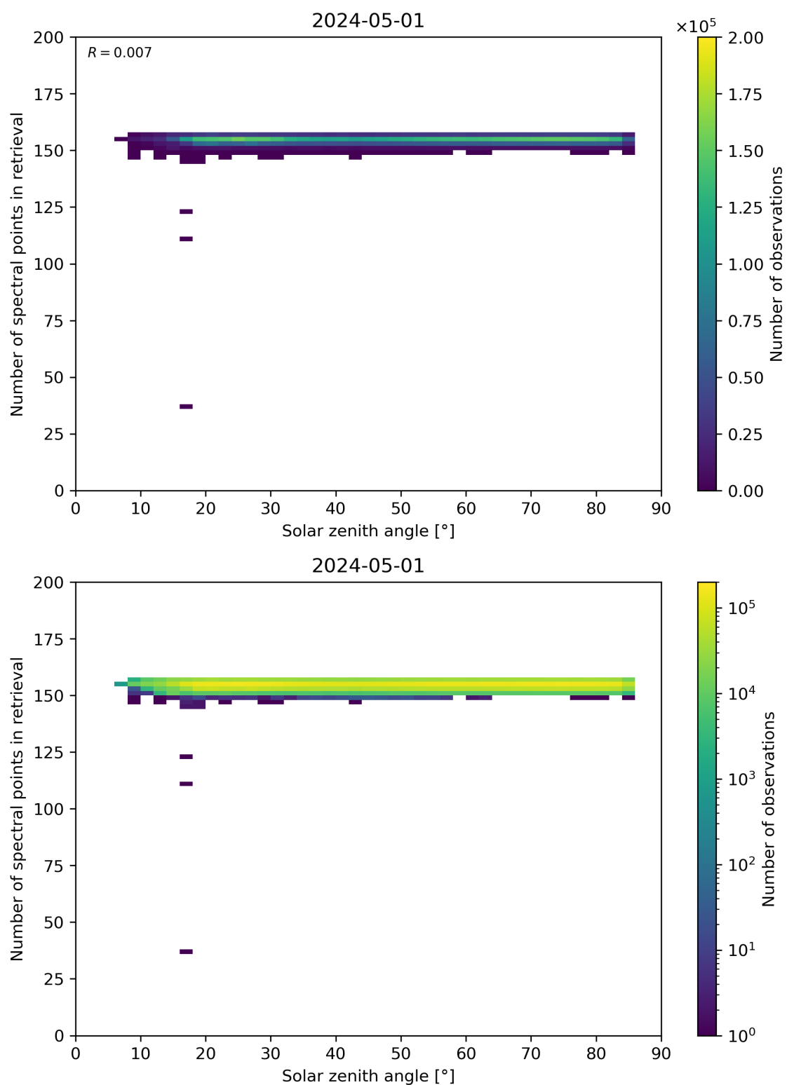
Figure 68: Scatter density plot of “Solar zenith angle” against “Number of spectral points in retrieval” for 2024-04-30 to 2024-05-02.
