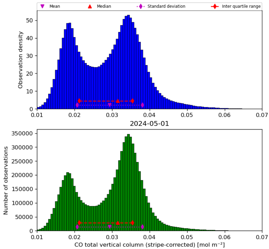
Figure 19: Histogram of “CO total vertical column (stripe-corrected)” for 2024-04-30 to 2024-05-02
