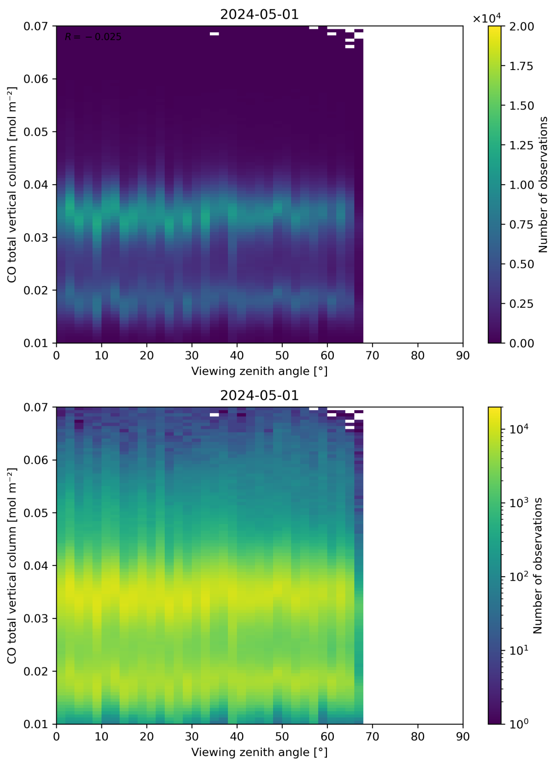
Figure 69: Scatter density plot of “Viewing zenith angle” against “CO total vertical column” for 2024-04-30 to 2024-05-02.
