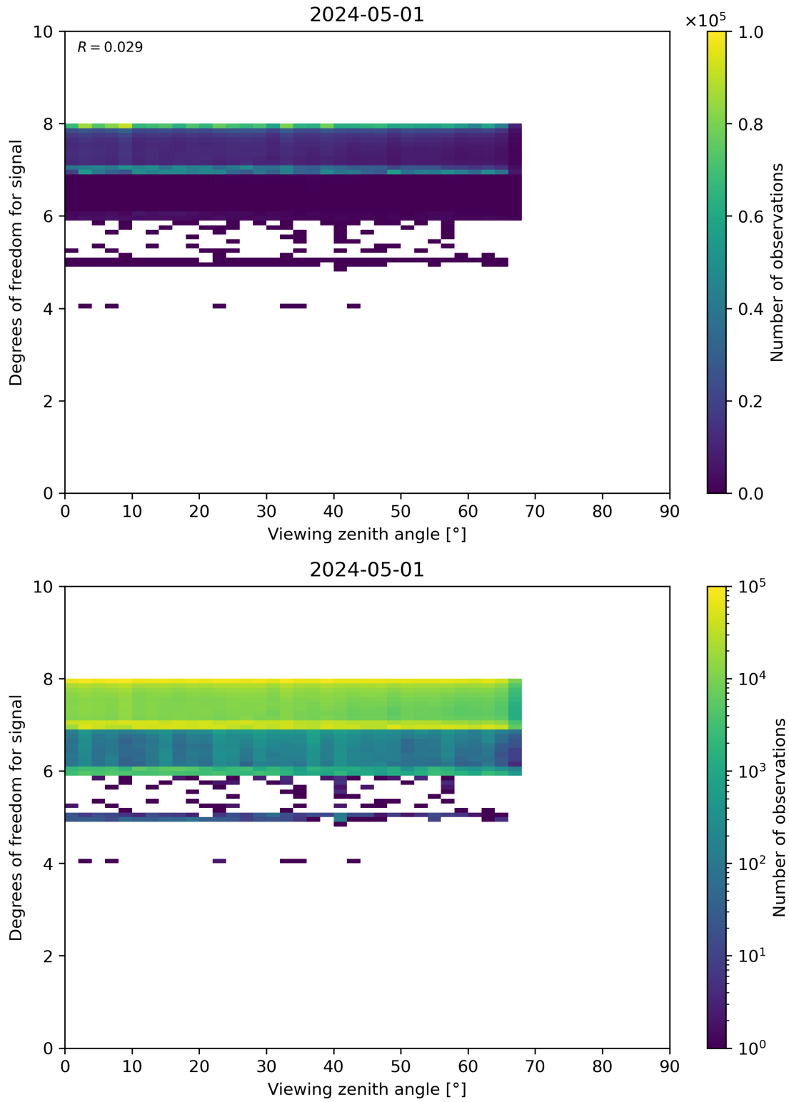
Figure 73: Scatter density plot of “Viewing zenith angle” against “Degrees of freedom for signal” for 2024-04-30 to 2024-05-02.
