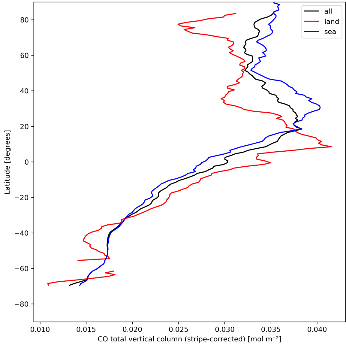
Figure 11: Zonal average of “CO total vertical column (stripe-corrected)” for 2024-04-30 to 2024-05-02.
