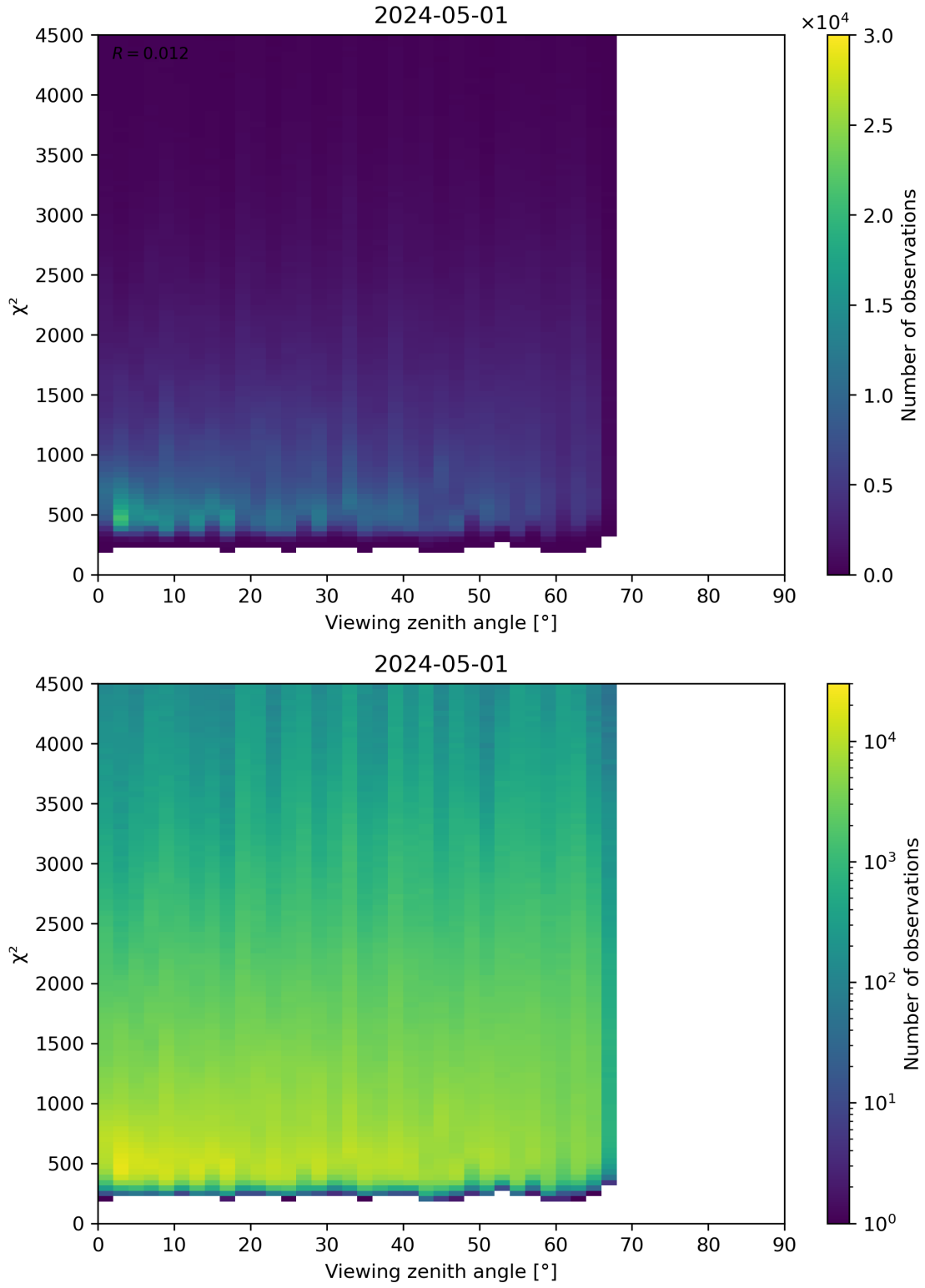
Figure 72: Scatter density plot of “Viewing zenith angle” against “ \chi^2 ” for 2024-04-30 to 2024-05-02.
