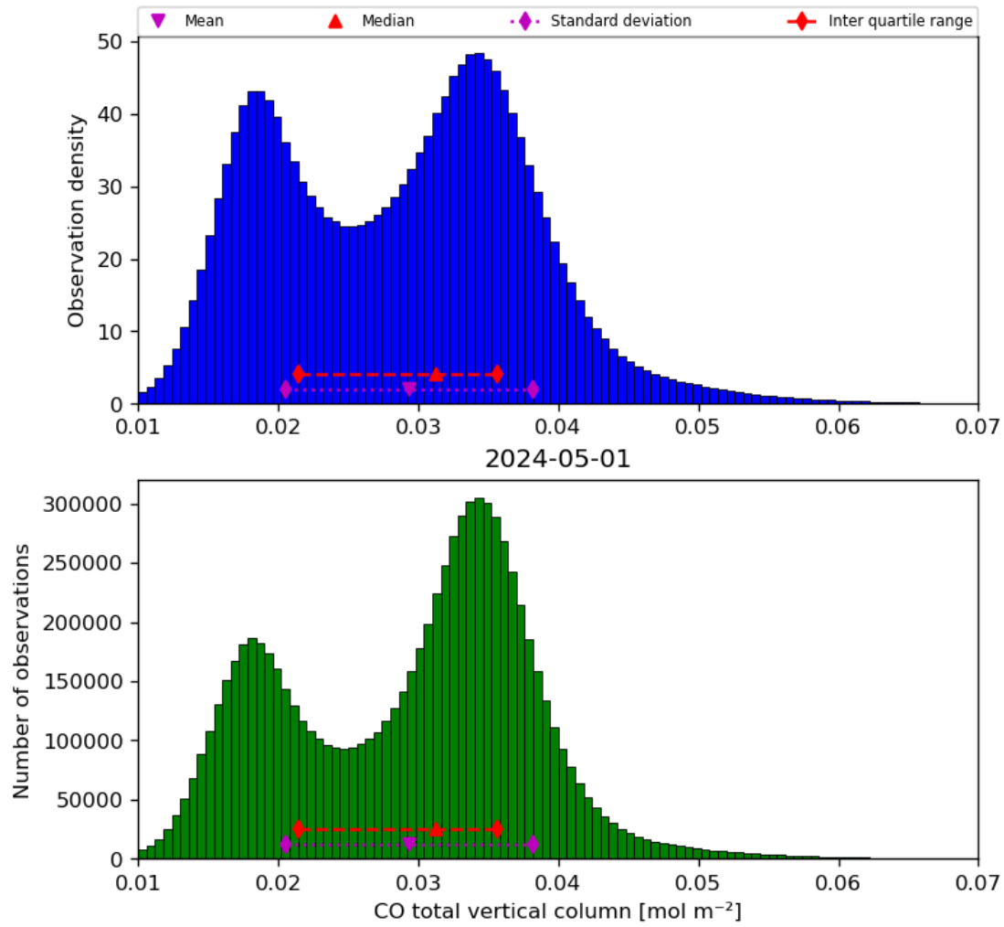
Figure 18: Histogram of “CO total vertical column” for 2024-04-30 to 2024-05-02
