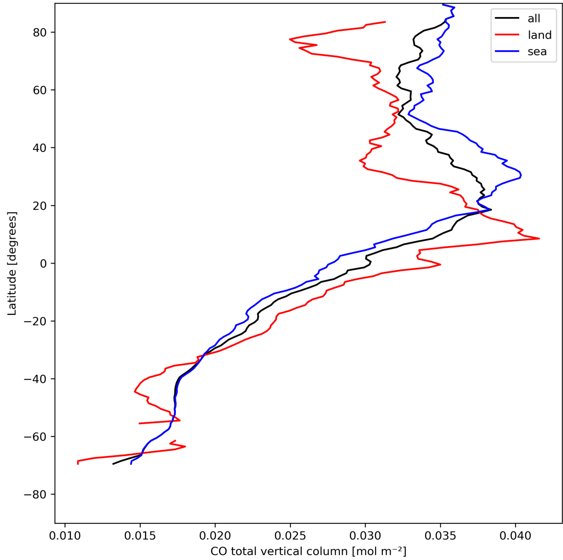
Figure 10: Zonal average of “CO total vertical column” for 2024-04-30 to 2024-05-02.
