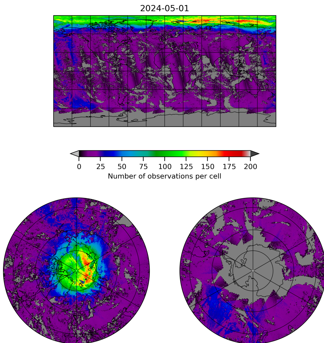
Figure 8: Map of the number of observations for 2024-04-30 to 2024-05-02
