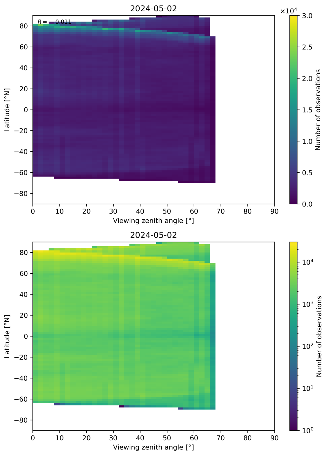
Figure 74: Scatter density plot of “Viewing zenith angle” against “Latitude” for 2024-05-02 to 2024-05-03.
