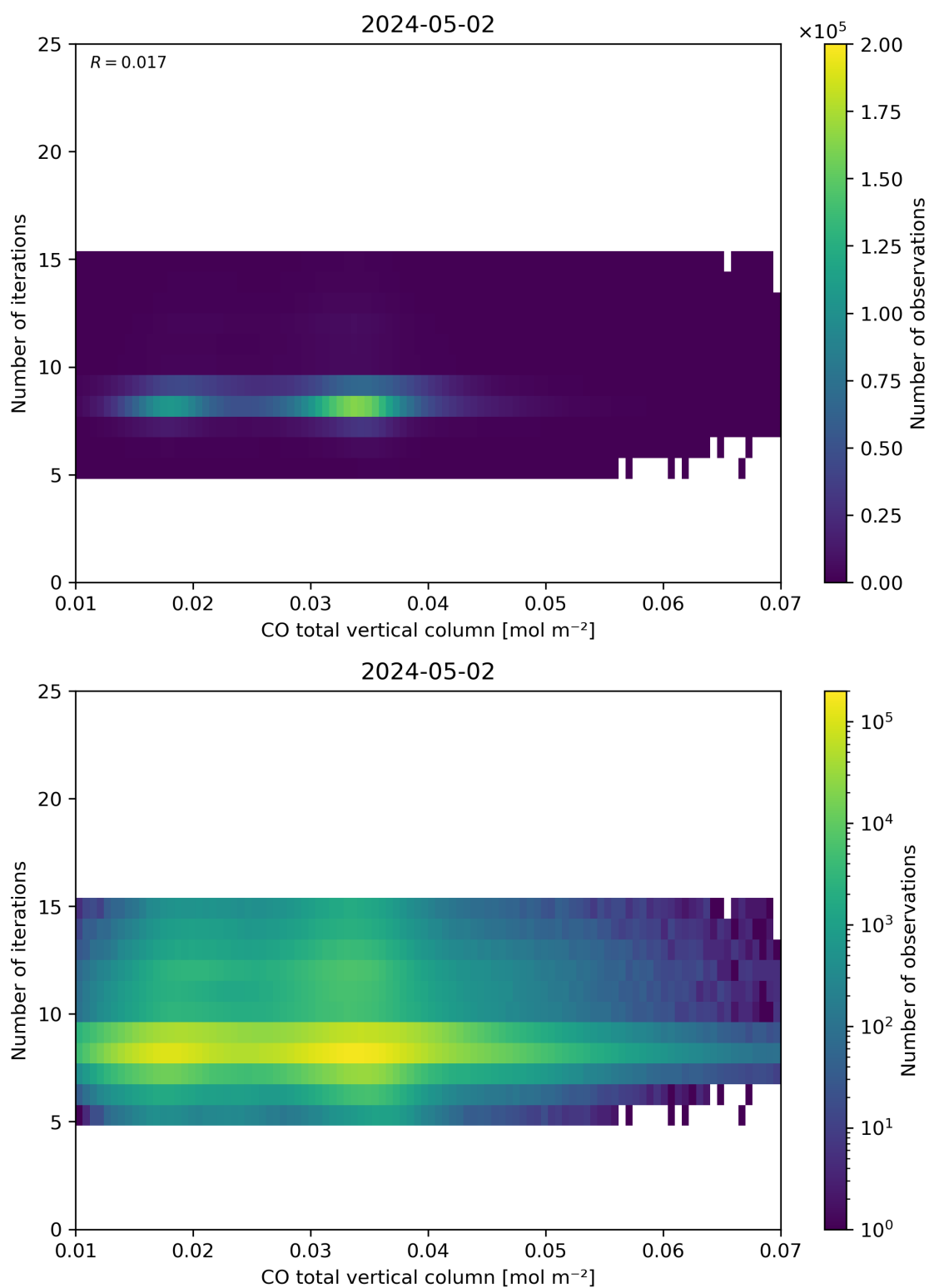
Figure 42: Scatter density plot of “CO total vertical column” against “Number of iterations” for 2024-05-02 to 2024-05-03.
