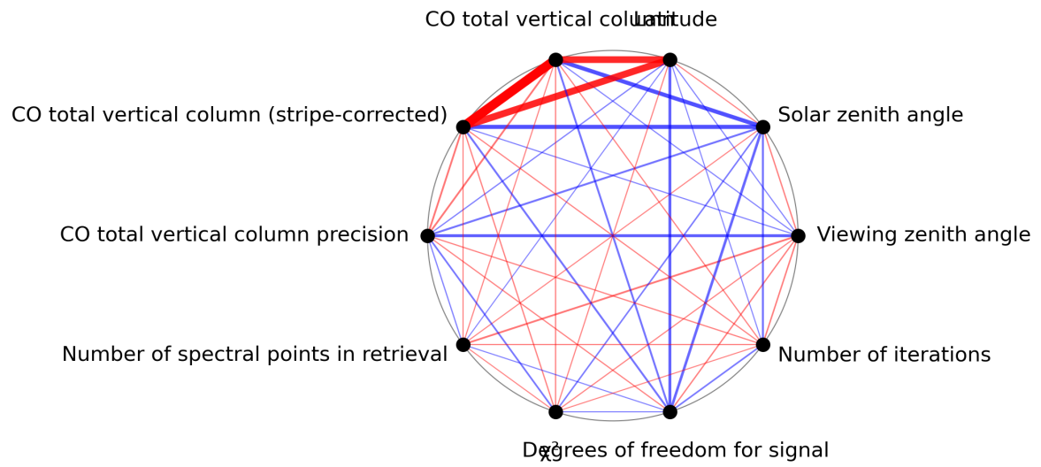
Figure 1: Map of correlation graph for 2024-05-02 to 2024-05-03.
