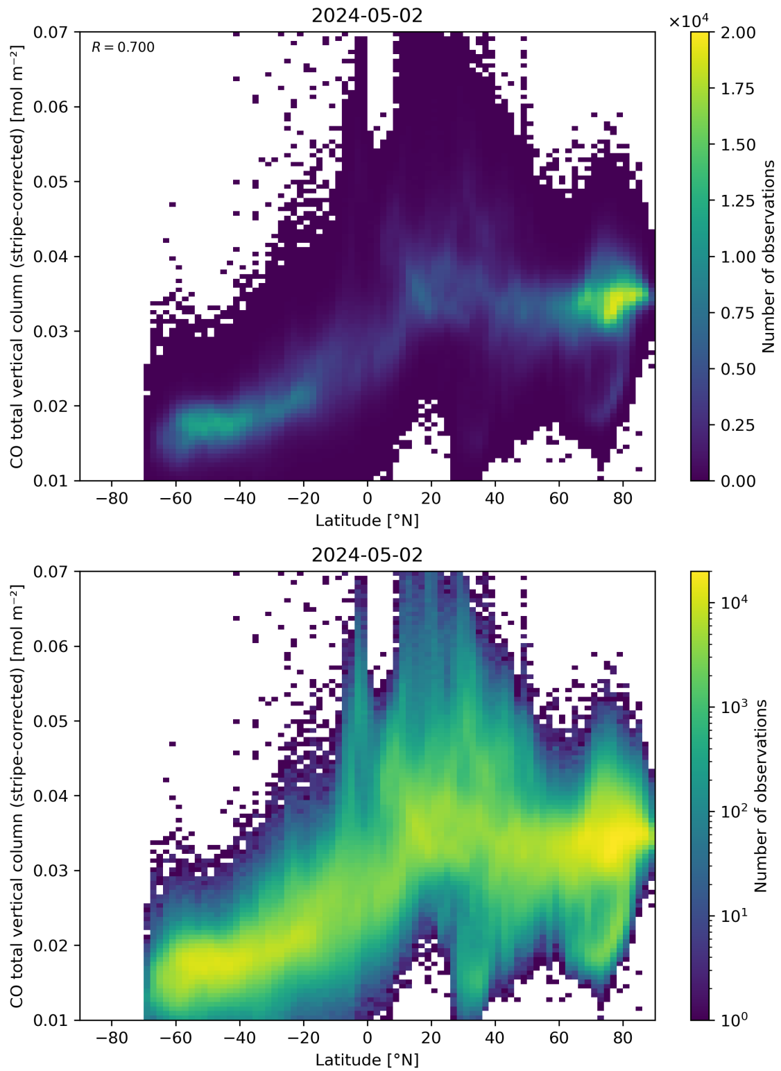
Figure 52: Scatter density plot of “Latitude” against “CO total vertical column (stripe-corrected)” for 2024-05-02 to 2024-05-03.
