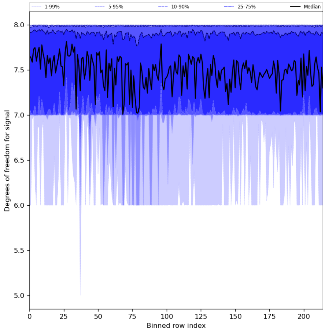
Figure 31: Along track statistics of “Degrees of freedom for signal” for 2024-05-02 to 2024-05-03
