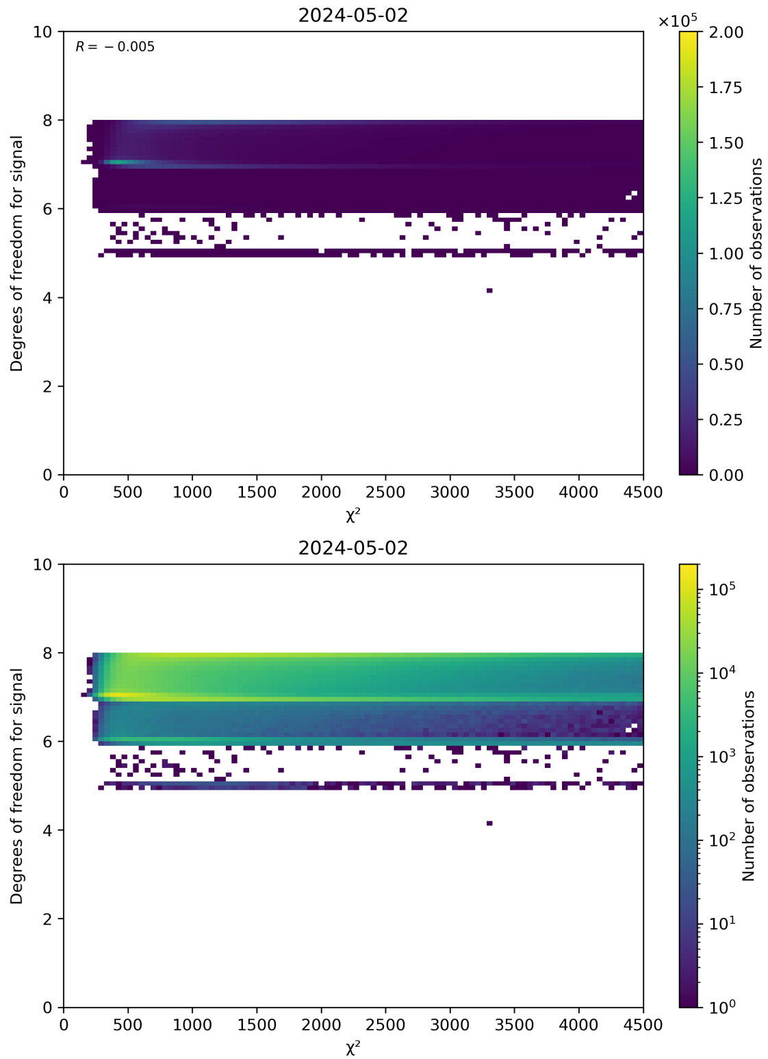
Figure 48: Scatter density plot of " \chi^2 " against "Degrees of freedom for signal" for 2024-05-02 to 2024-05-03.
