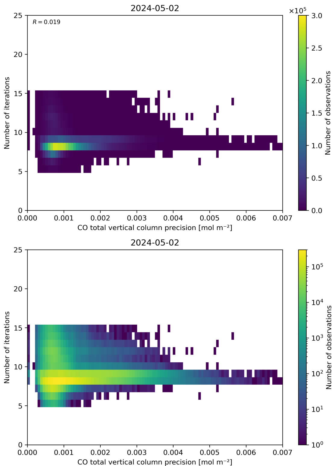
Figure 46: Scatter density plot of “CO total vertical column precision” against “Number of iterations” for 2024-05-02 to 2024-05-03.
