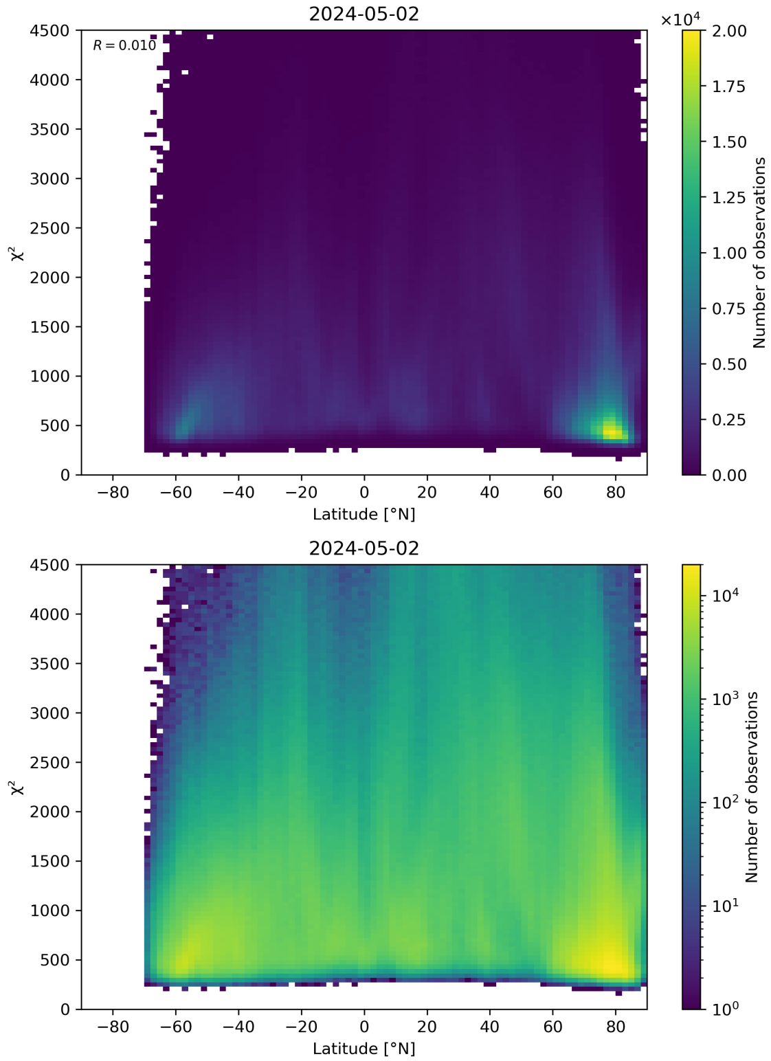
Figure 54: Scatter density plot of “Latitude” against “ \chi^2 ” for 2024-05-02 to 2024-05-03.
