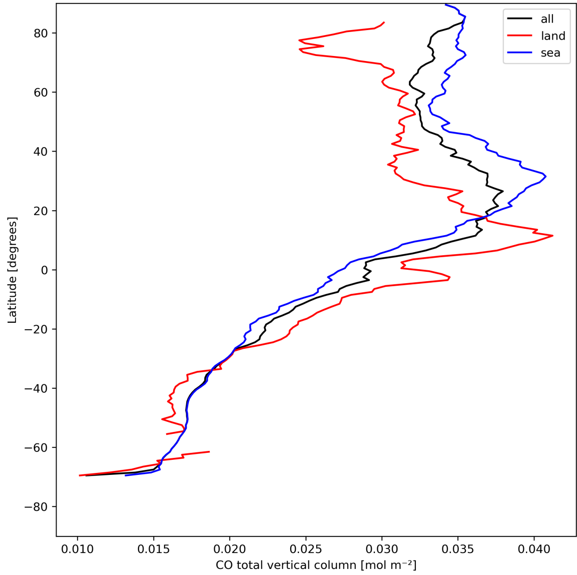
Figure 10: Zonal average of “CO total vertical column” for 2024-05-02 to 2024-05-03.
