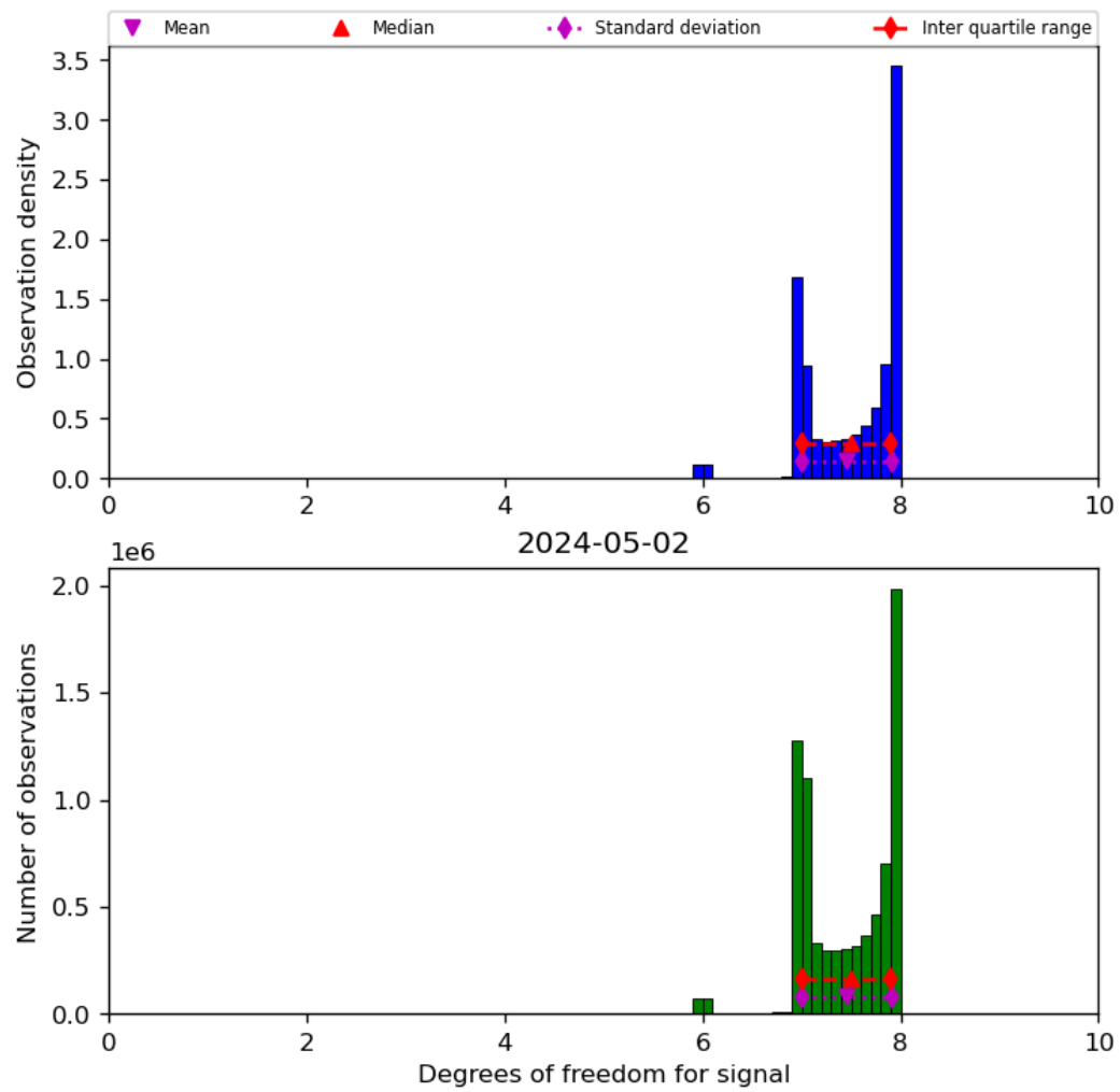
Figure 23: Histogram of “Degrees of freedom for signal” for 2024-05-02 to 2024-05-03
