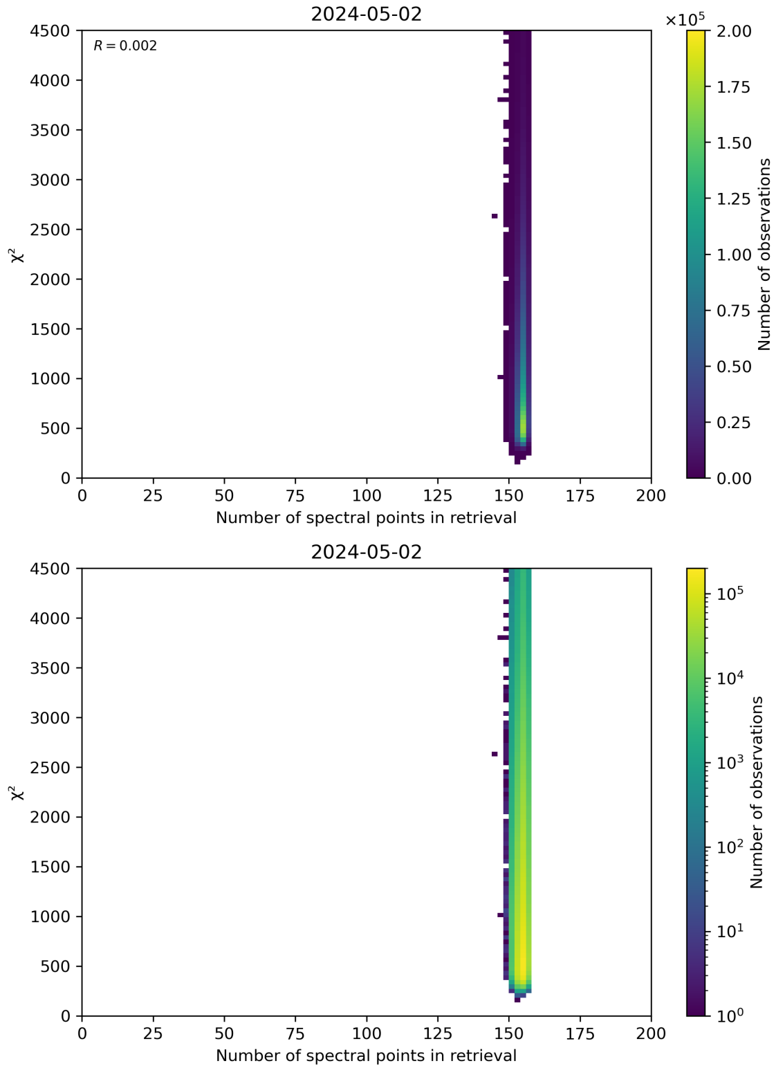
Figure 58: Scatter density plot of “Number of spectral points in retrieval” against “ \chi^2 ” for 2024-05-02 to 2024-05-03.
