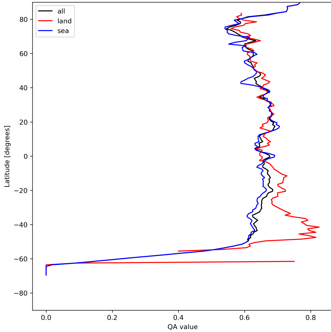
Figure 9: Zonal average of “QA value” for 2024-05-02 to 2024-05-03.
