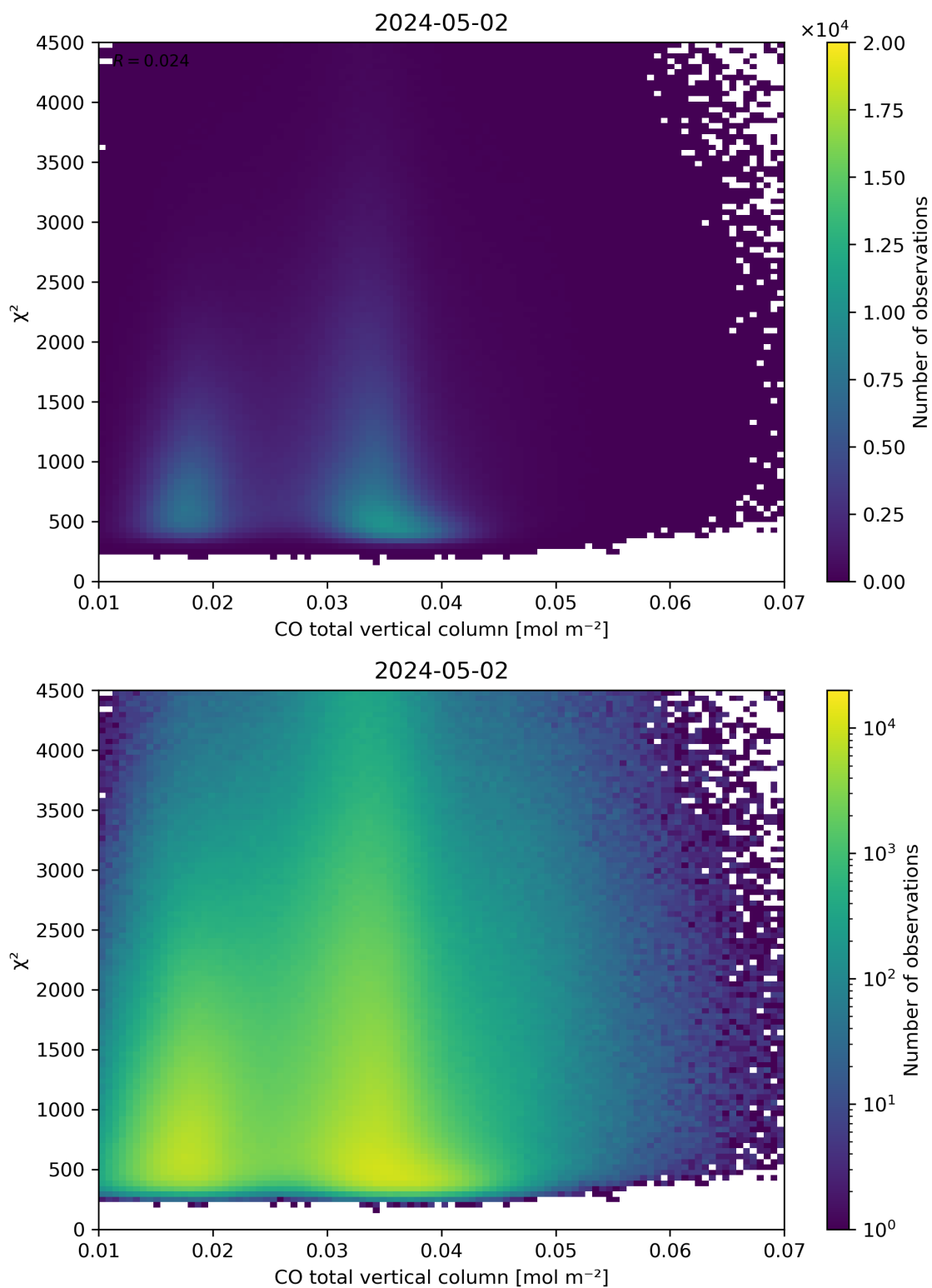
Figure 35: Scatter density plot of “CO total vertical column” against “ \chi^2 ” for 2024-05-02 to 2024-05-03.
