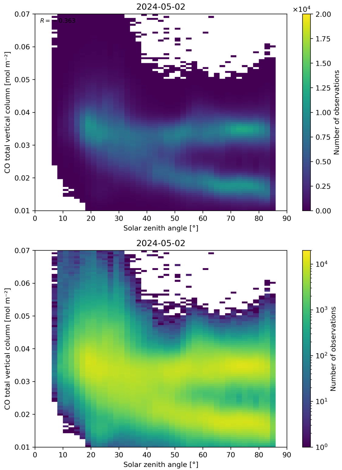
Figure 61: Scatter density plot of “Solar zenith angle” against “CO total vertical column” for 2024-05-02 to 2024-05-03.
