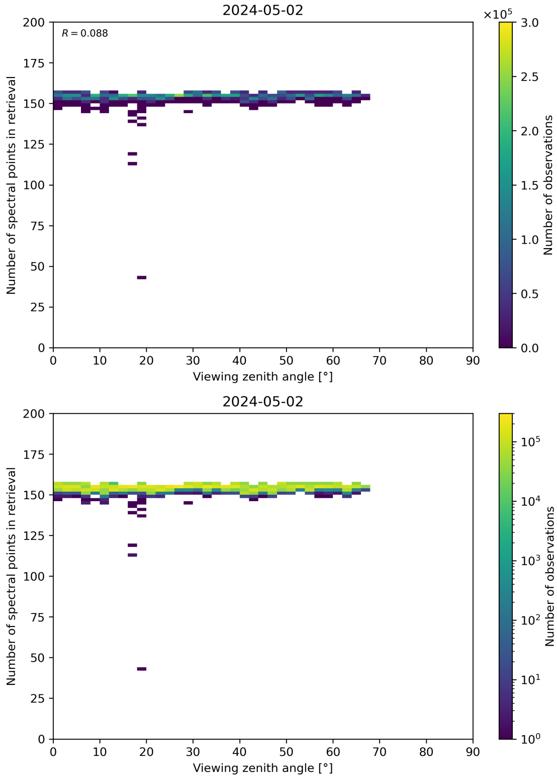
Figure 76: Scatter density plot of “Viewing zenith angle” against “Number of spectral points in retrieval” for 2024-05-02 to 2024-05-03.
