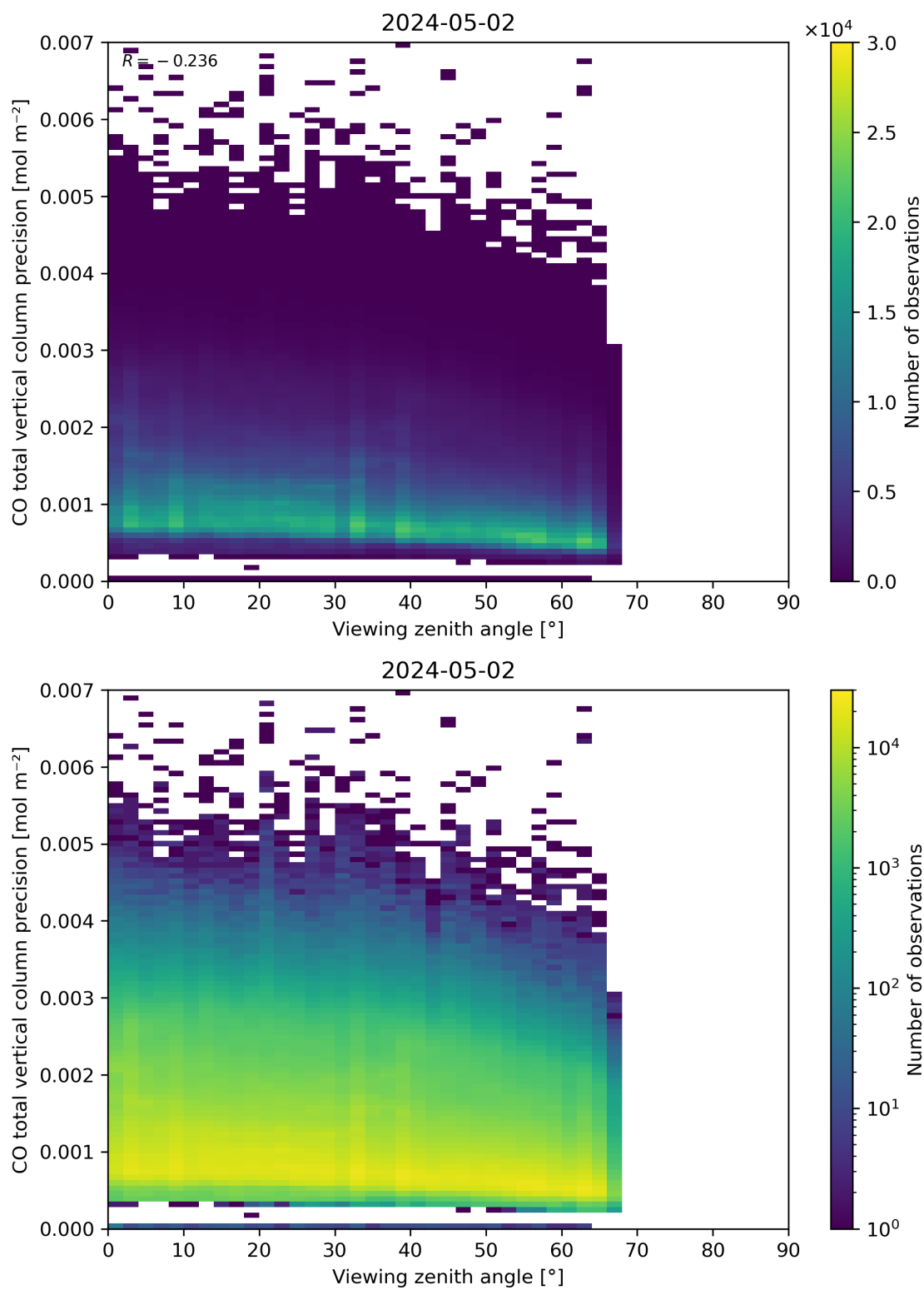
Figure 71: Scatter density plot of “Viewing zenith angle” against “CO total vertical column precision” for 2024-05-02 to 2024-05-03.
