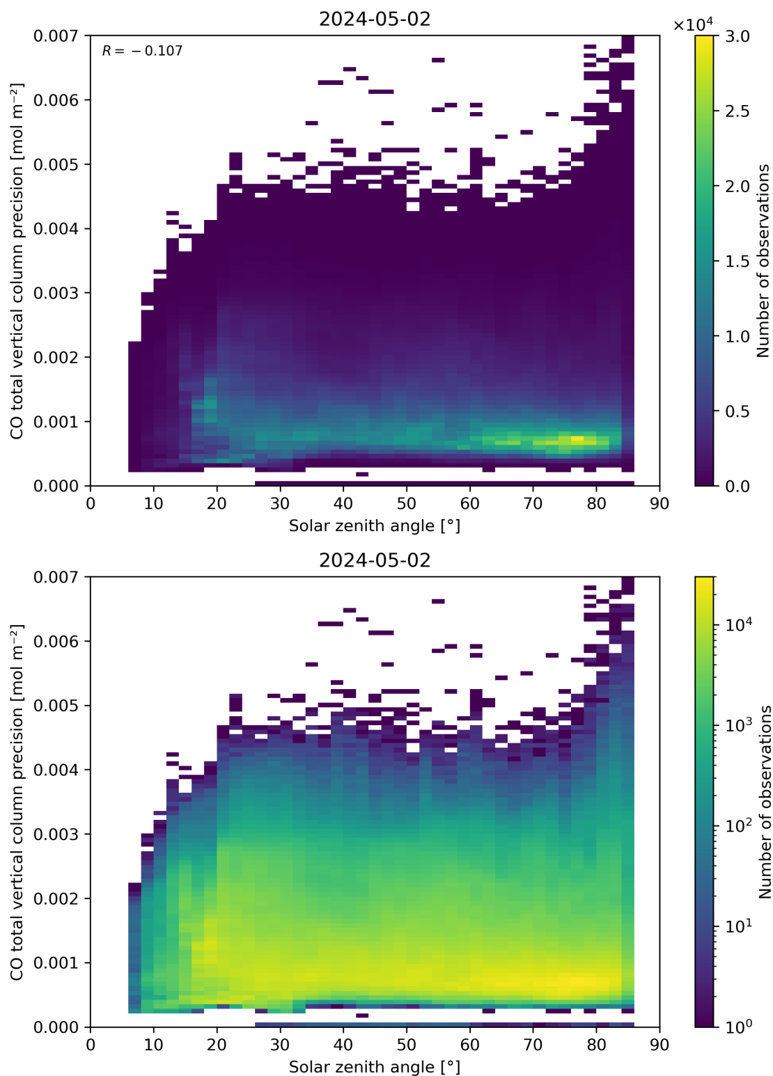
Figure 63: Scatter density plot of “Solar zenith angle” against “CO total vertical column precision” for 2024-05-02 to 2024-05-03.
