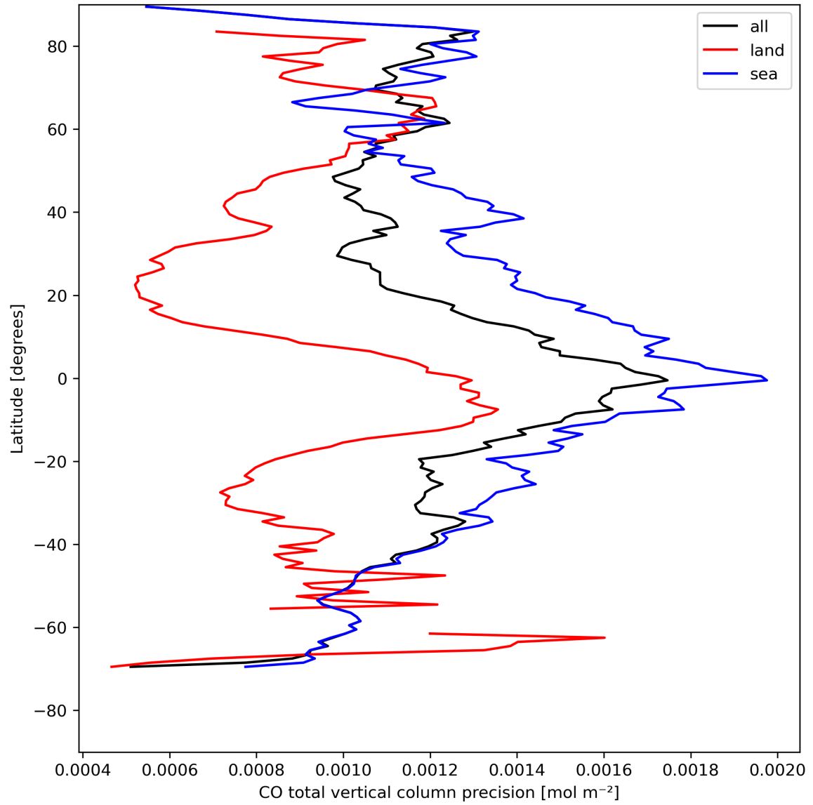
Figure 12: Zonal average of “CO total vertical column precision” for 2024-05-02 to 2024-05-03.
