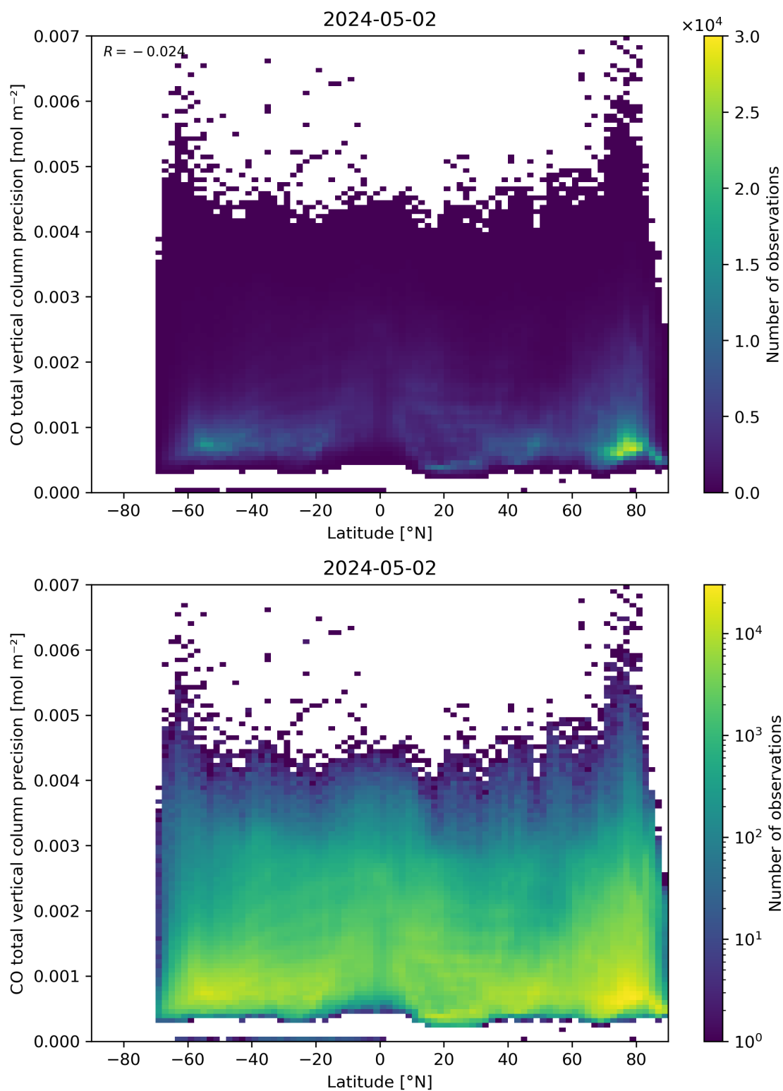
Figure 53: Scatter density plot of “Latitude” against “CO total vertical column precision” for 2024-05-02 to 2024-05-03.
