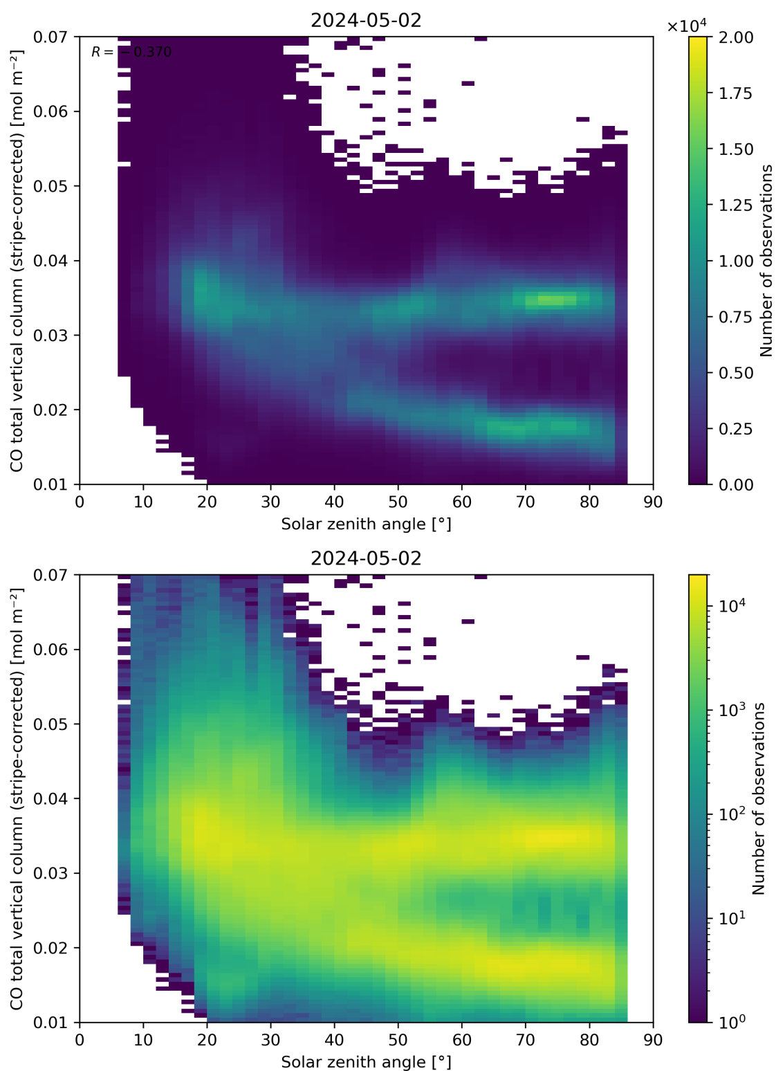
Figure 62: Scatter density plot of “Solar zenith angle” against “CO total vertical column (stripe-corrected)” for 2024-05-02 to 2024-05-03.
