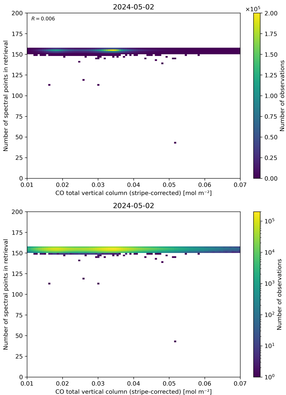
Figure 40: Scatter density plot of “CO total vertical column (stripe-corrected)” against “Number of spectral points in retrieval” for 2024-05-02 to 2024-05-03.
