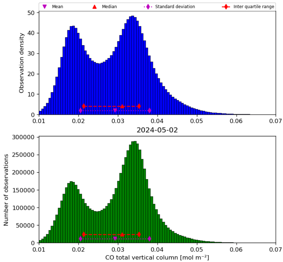
Figure 18: Histogram of “CO total vertical column” for 2024-05-02 to 2024-05-03
