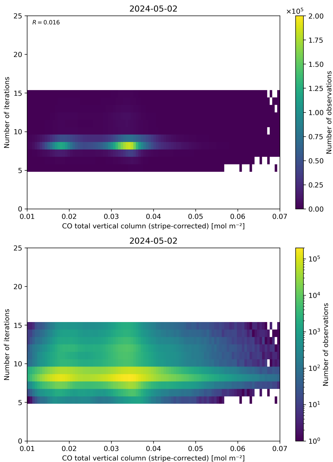
Figure 39: Scatter density plot of “CO total vertical column (stripe-corrected)” against “Number of iterations” for 2024-05-02 to 2024-05-03.
