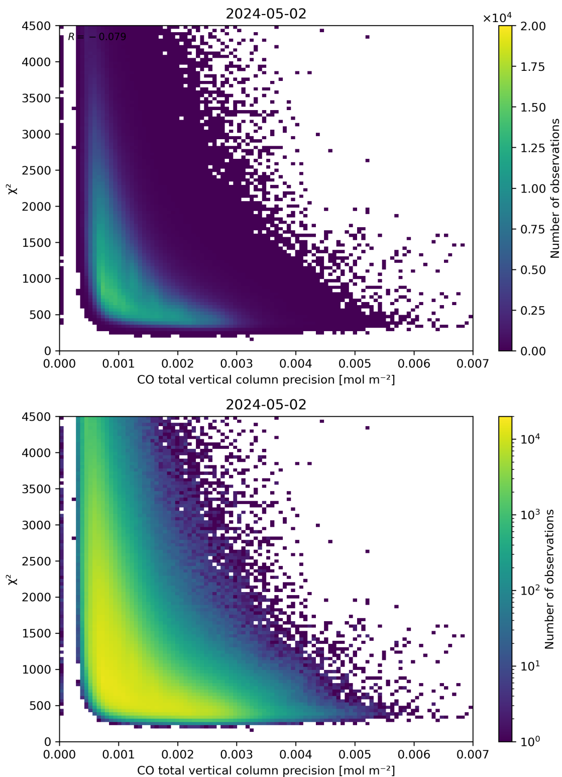
Figure 44: Scatter density plot of “CO total vertical column precision” against “ \chi^2 ” for 2024-05-02 to 2024-05-03.
