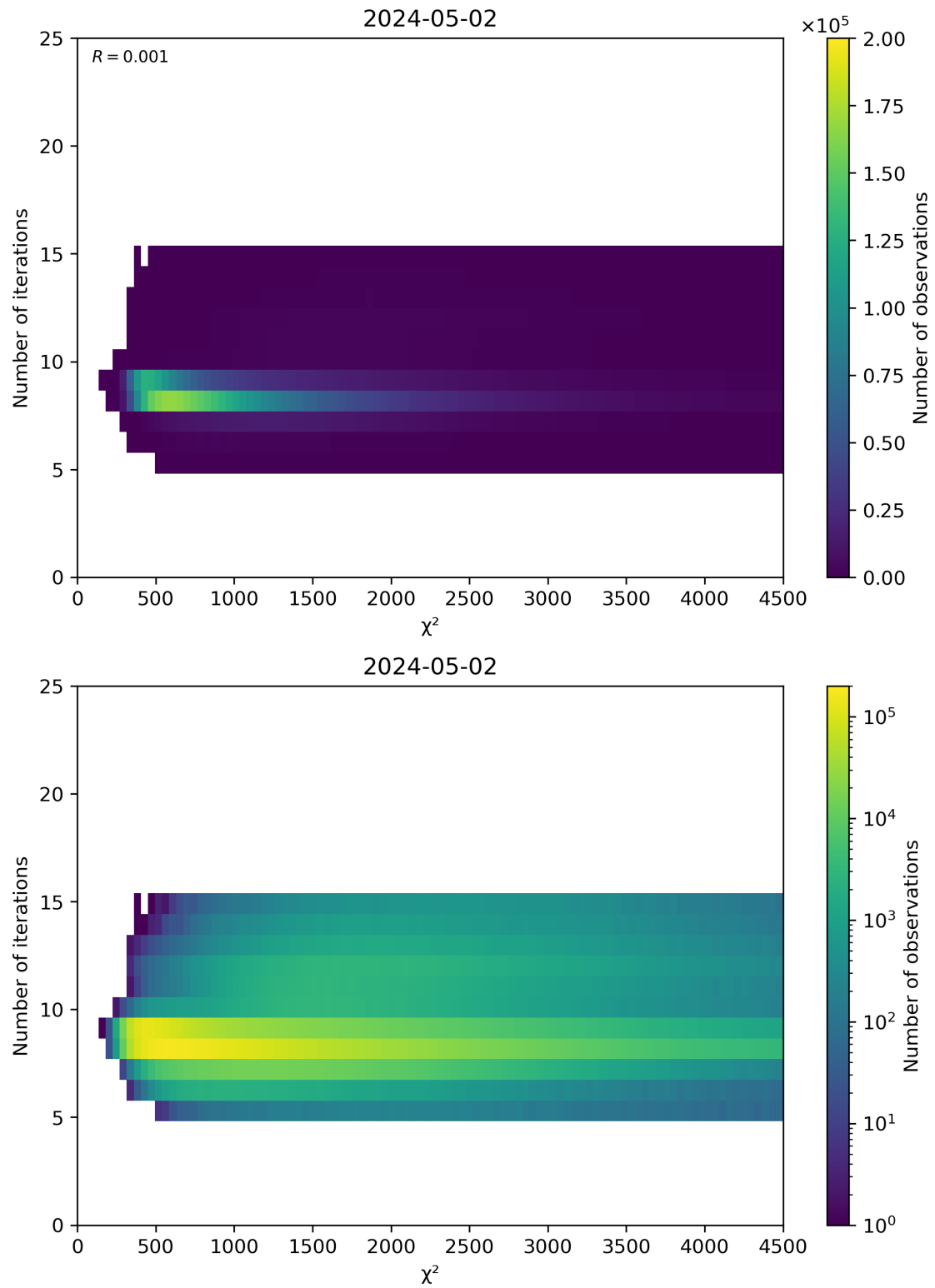
Figure 49: Scatter density plot of “ \chi^2 ” against “Number of iterations” for 2024-05-02 to 2024-05-03.
