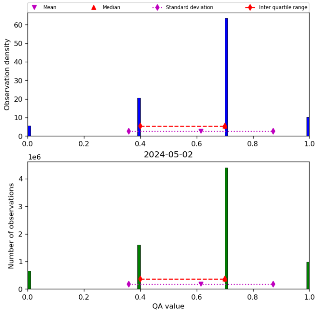
Figure 17: Histogram of “QA value” for 2024-05-02 to 2024-05-03
