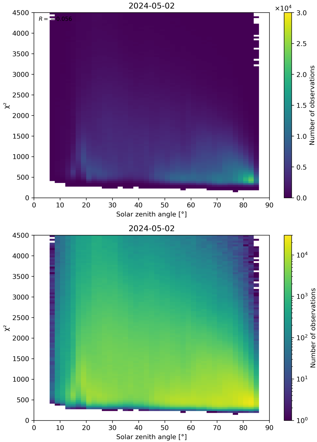
Figure 64: Scatter density plot of “Solar zenith angle” against “ \chi^2 ” for 2024-05-02 to 2024-05-03.
