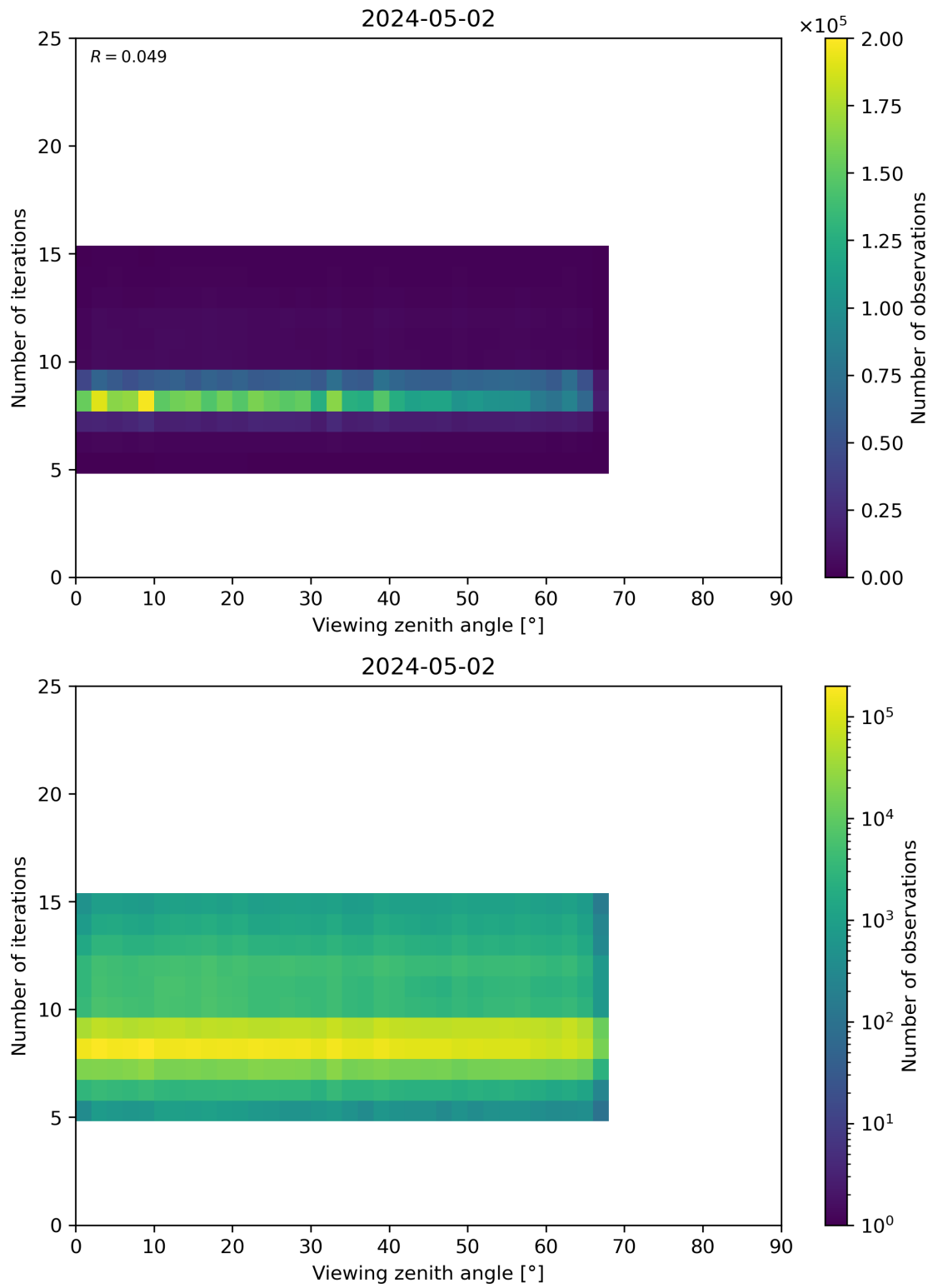
Figure 75: Scatter density plot of “Viewing zenith angle” against “Number of iterations” for 2024-05-02 to 2024-05-03.
