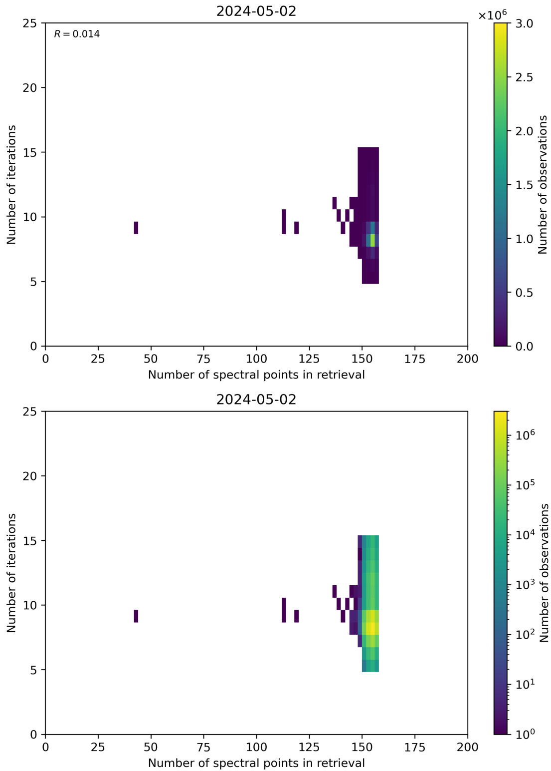
Figure 60: Scatter density plot of “Number of spectral points in retrieval” against “Number of iterations” for 2024-05-02 to 2024-05-03.
