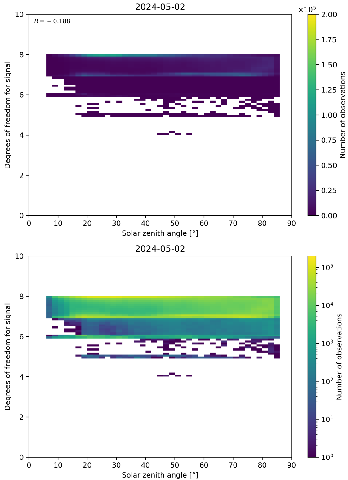
Figure 65: Scatter density plot of “Solar zenith angle” against “Degrees of freedom for signal” for 2024-05-02 to 2024-05-03.
