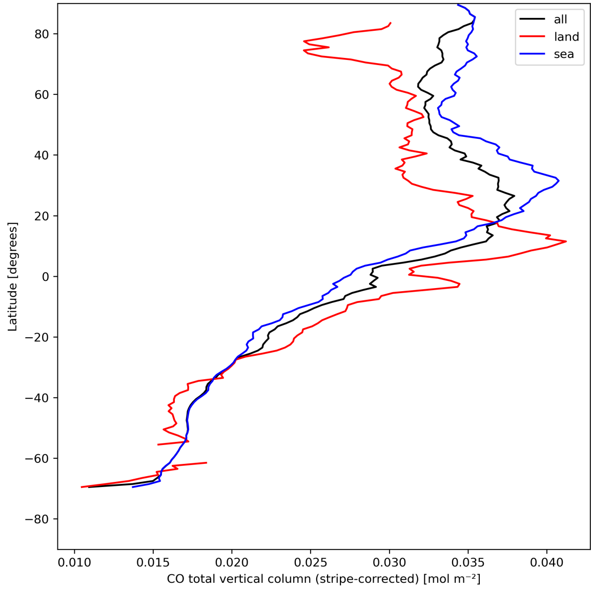
Figure 11: Zonal average of “CO total vertical column (stripe-corrected)” for 2024-05-02 to 2024-05-03.
