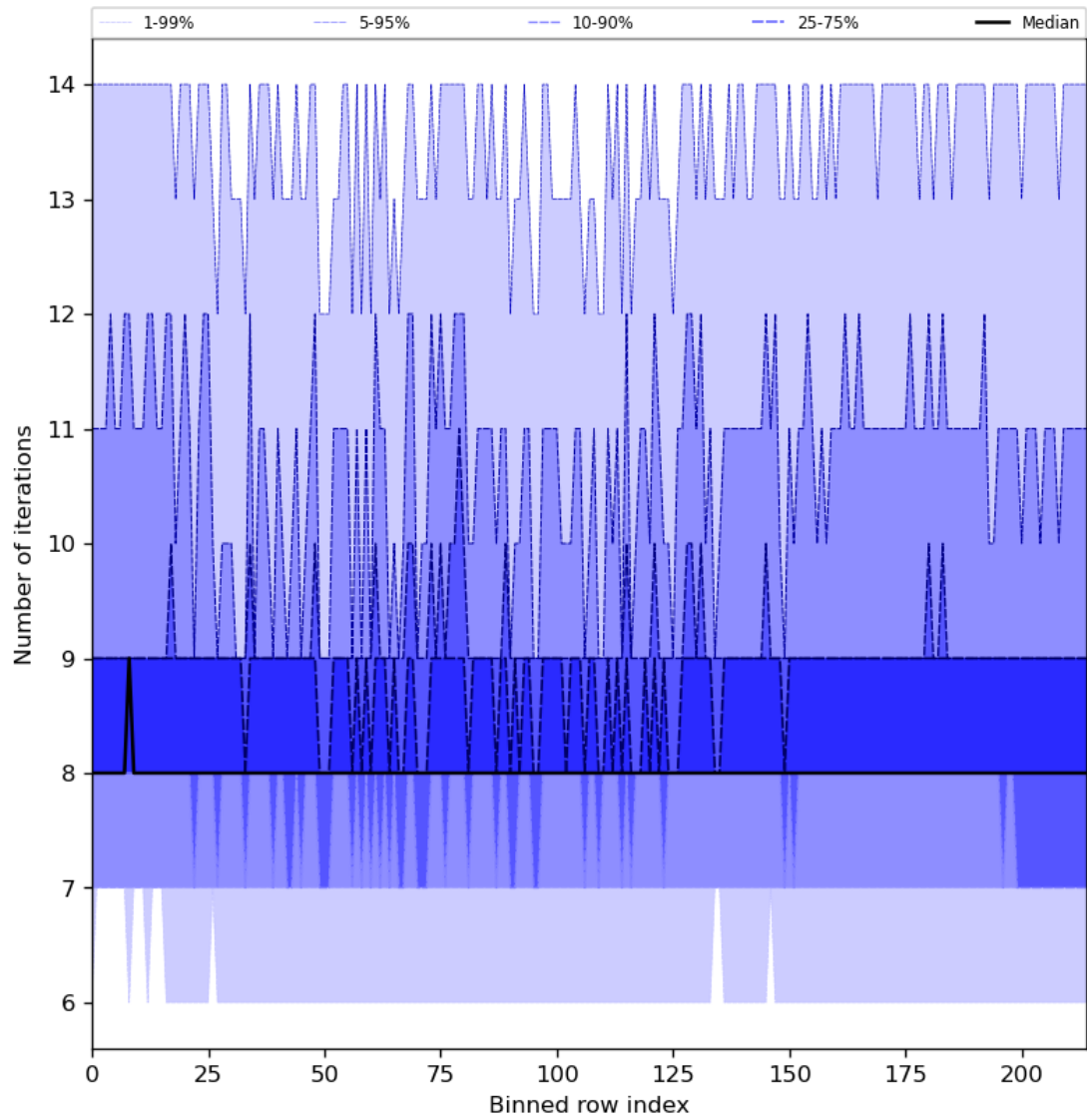
Figure 32: Along track statistics of “Number of iterations” for 2024-05-02 to 2024-05-03
