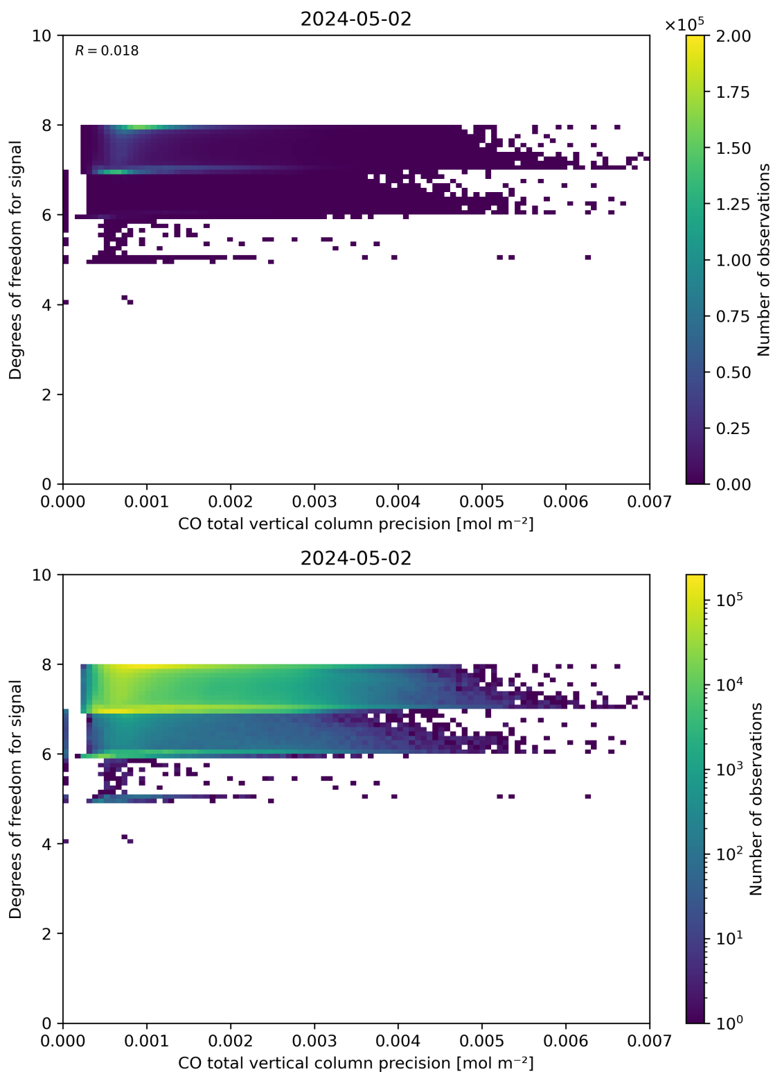
Figure 45: Scatter density plot of “CO total vertical column precision” against “Degrees of freedom for signal” for 2024-05-02 to 2024-05-03.
