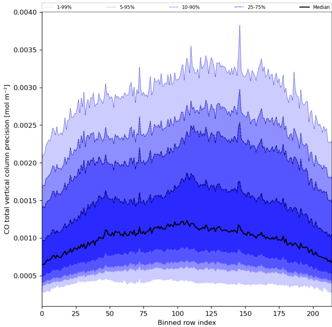
Figure 28: Along track statistics of “CO total vertical column precision” for 2024-05-02 to 2024-05-03
