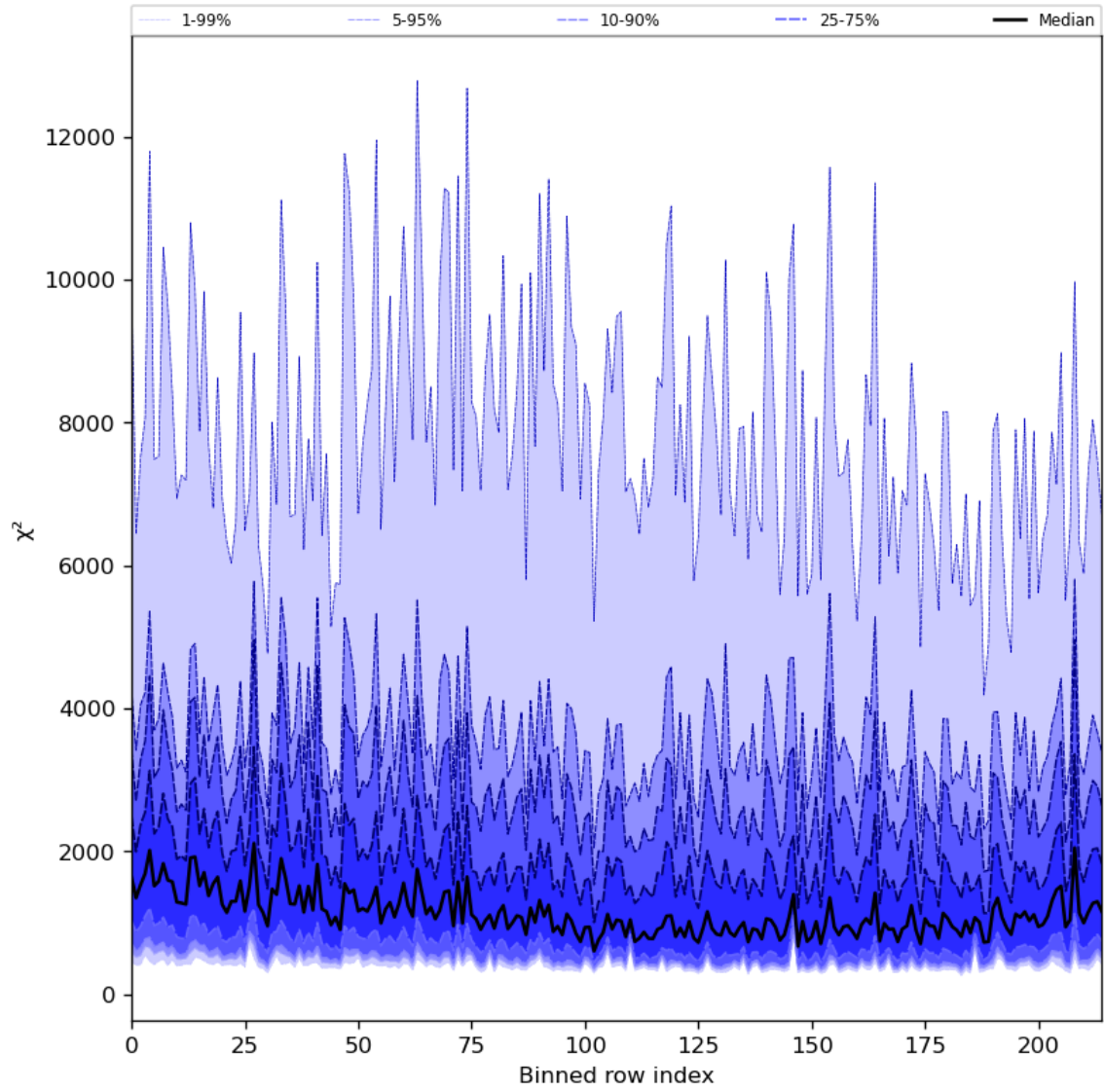
Figure 30: Along track statistics of “ \chi^2 ” for 2024-05-02 to 2024-05-03
