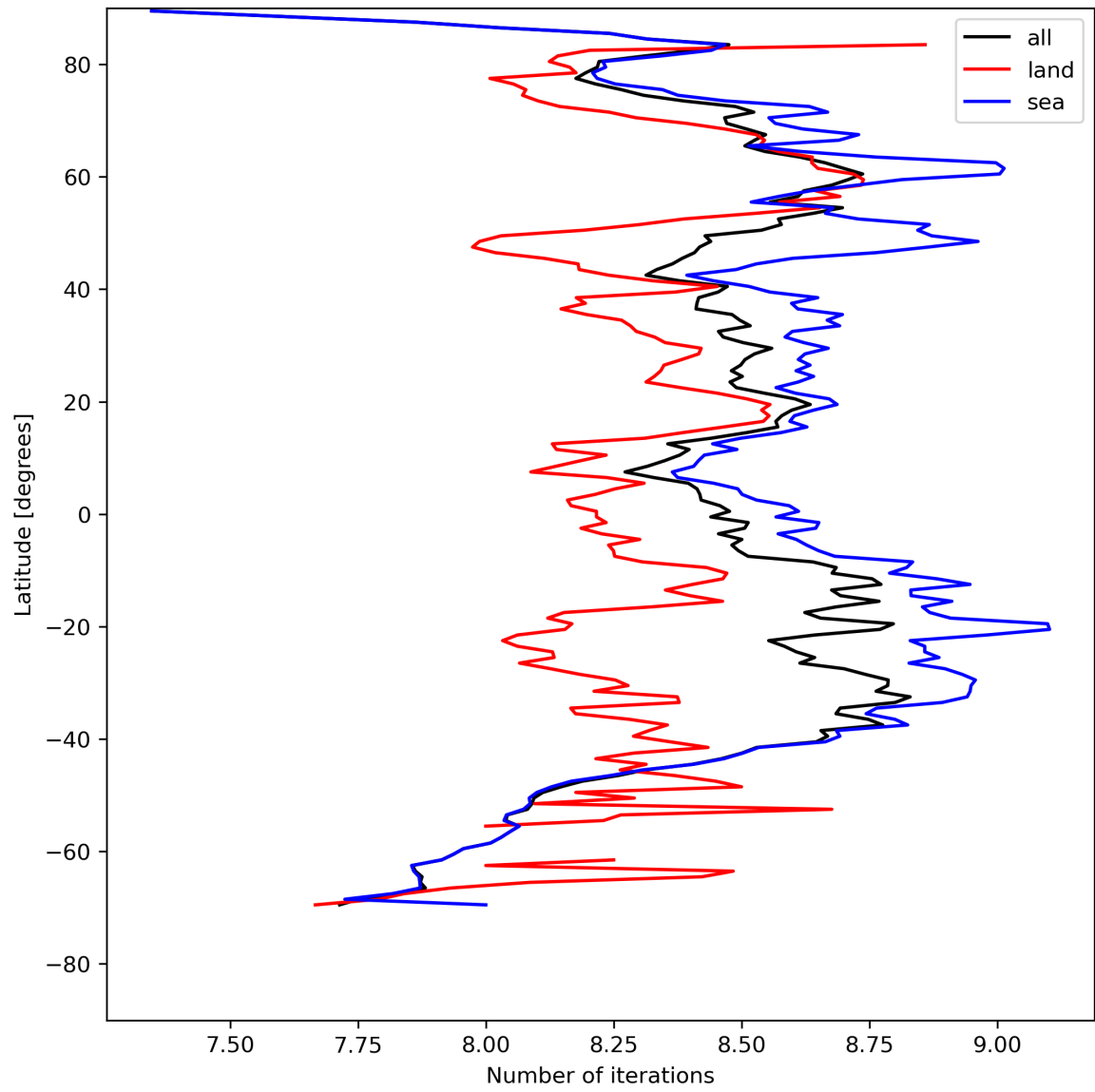
Figure 16: Zonal average of “Number of iterations” for 2024-05-02 to 2024-05-03.
