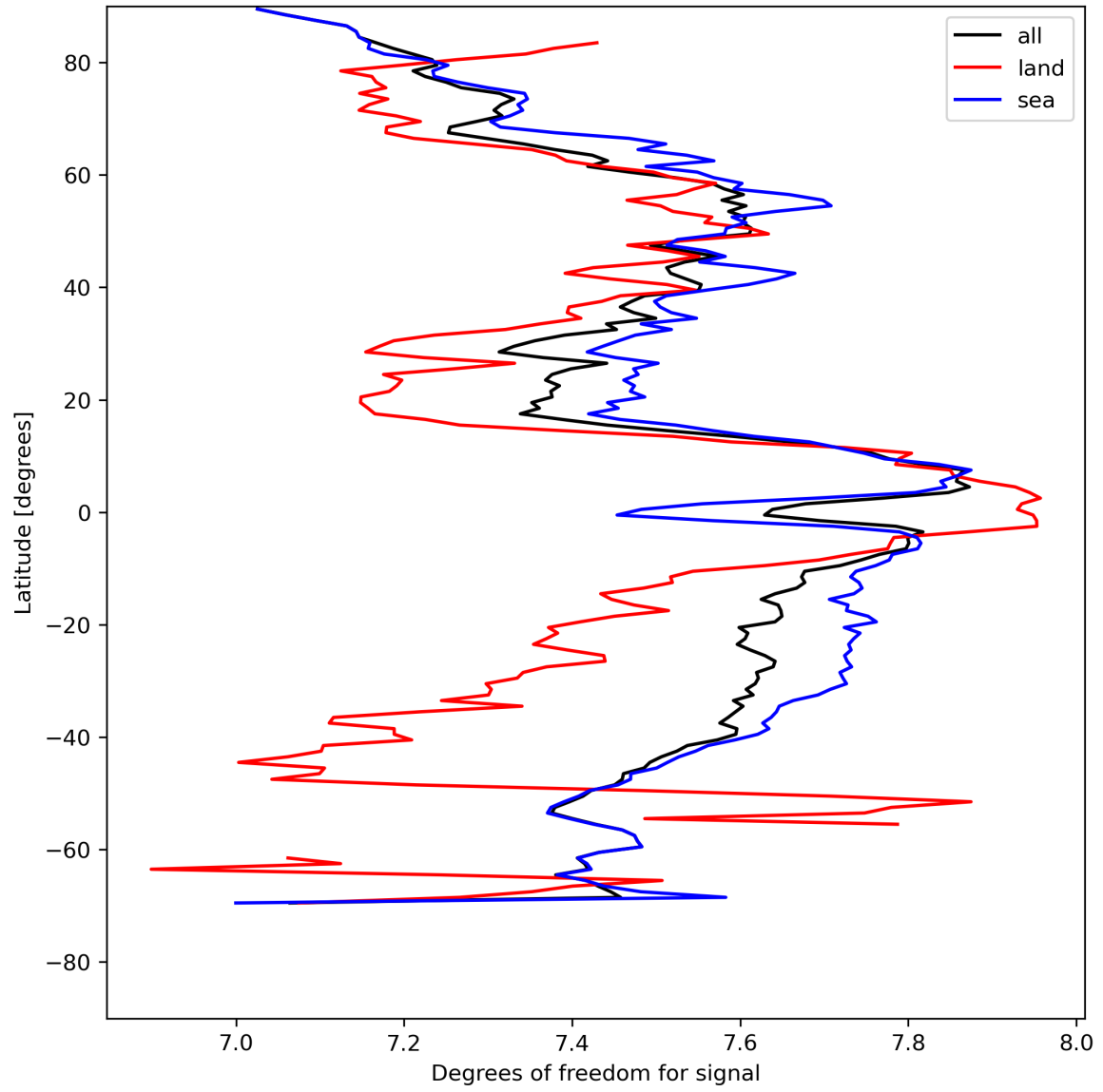
Figure 15: Zonal average of “Degrees of freedom for signal” for 2024-05-02 to 2024-05-03.
