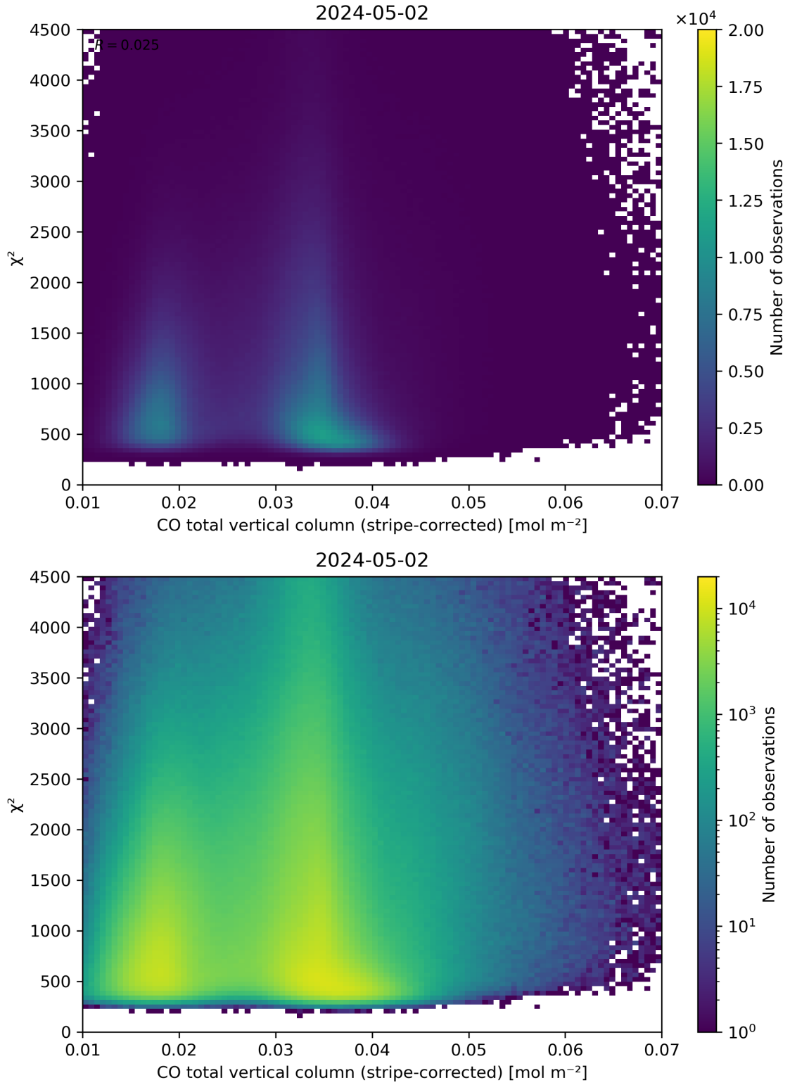
Figure 37: Scatter density plot of “CO total vertical column (stripe-corrected)” against “ \chi^2 ” for 2024-05-02 to 2024-05-03.
