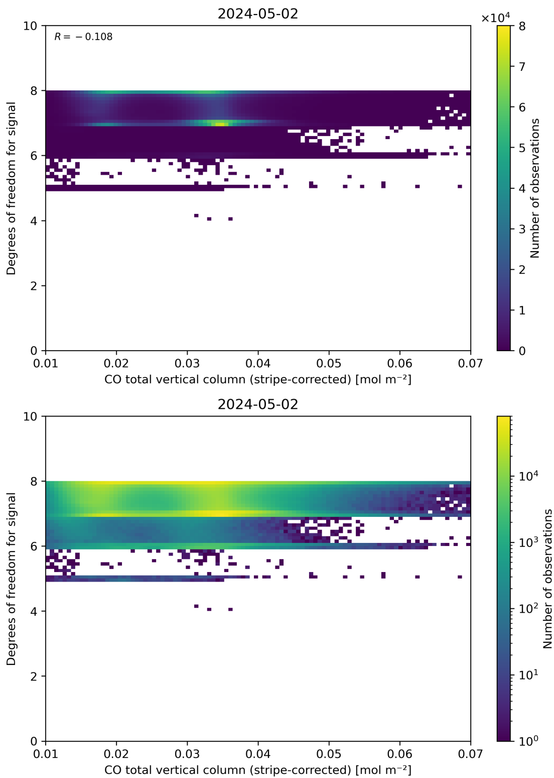
Figure 38: Scatter density plot of “CO total vertical column (stripe-corrected)” against “Degrees of freedom for signal” for 2024-05-02 to 2024-05-03.
