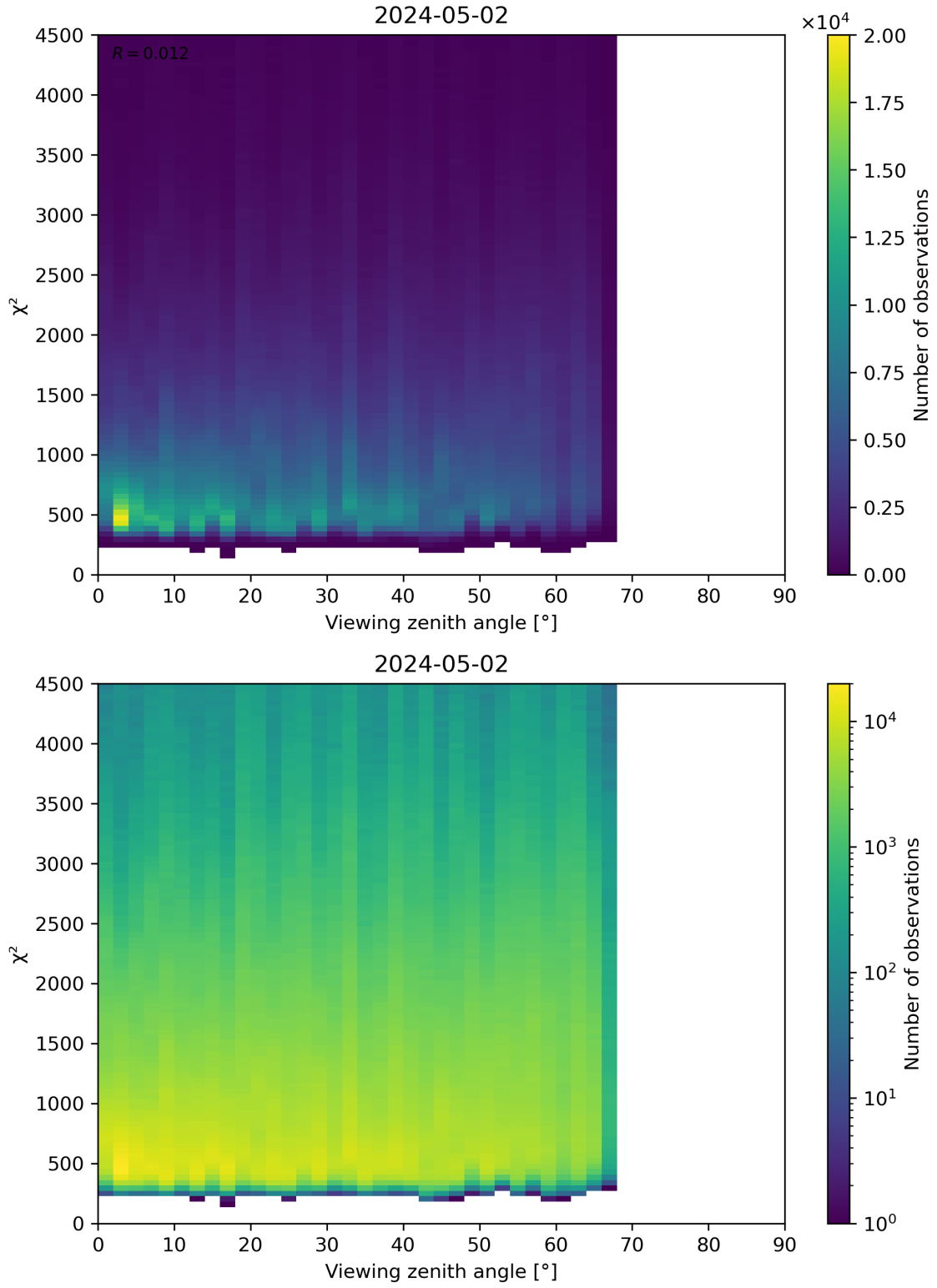
Figure 72: Scatter density plot of “Viewing zenith angle” against “ \chi^2 ” for 2024-05-02 to 2024-05-03.
