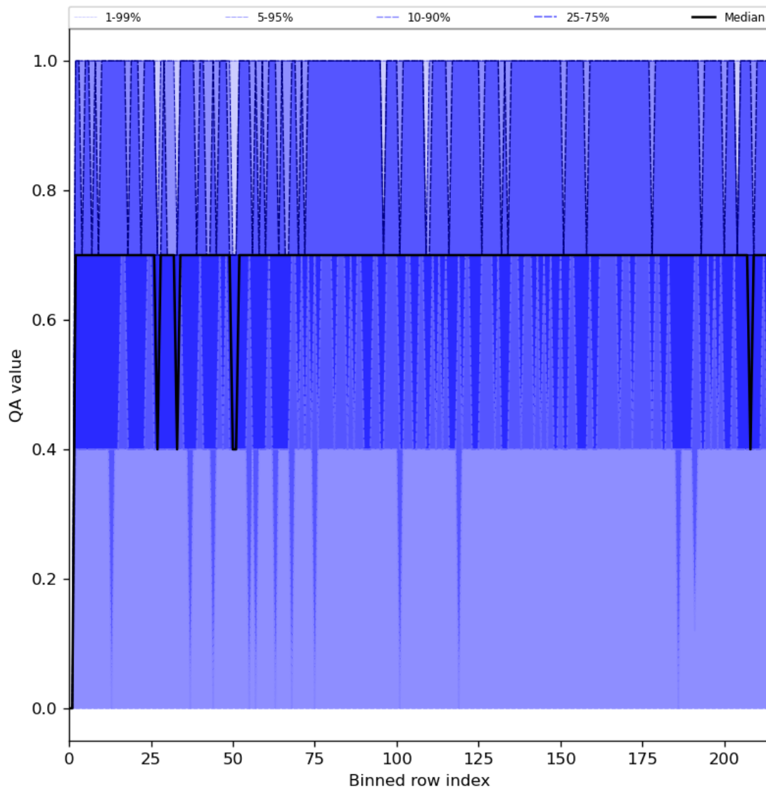
Figure 25: Along track statistics of “QA value” for 2024-05-02 to 2024-05-03
