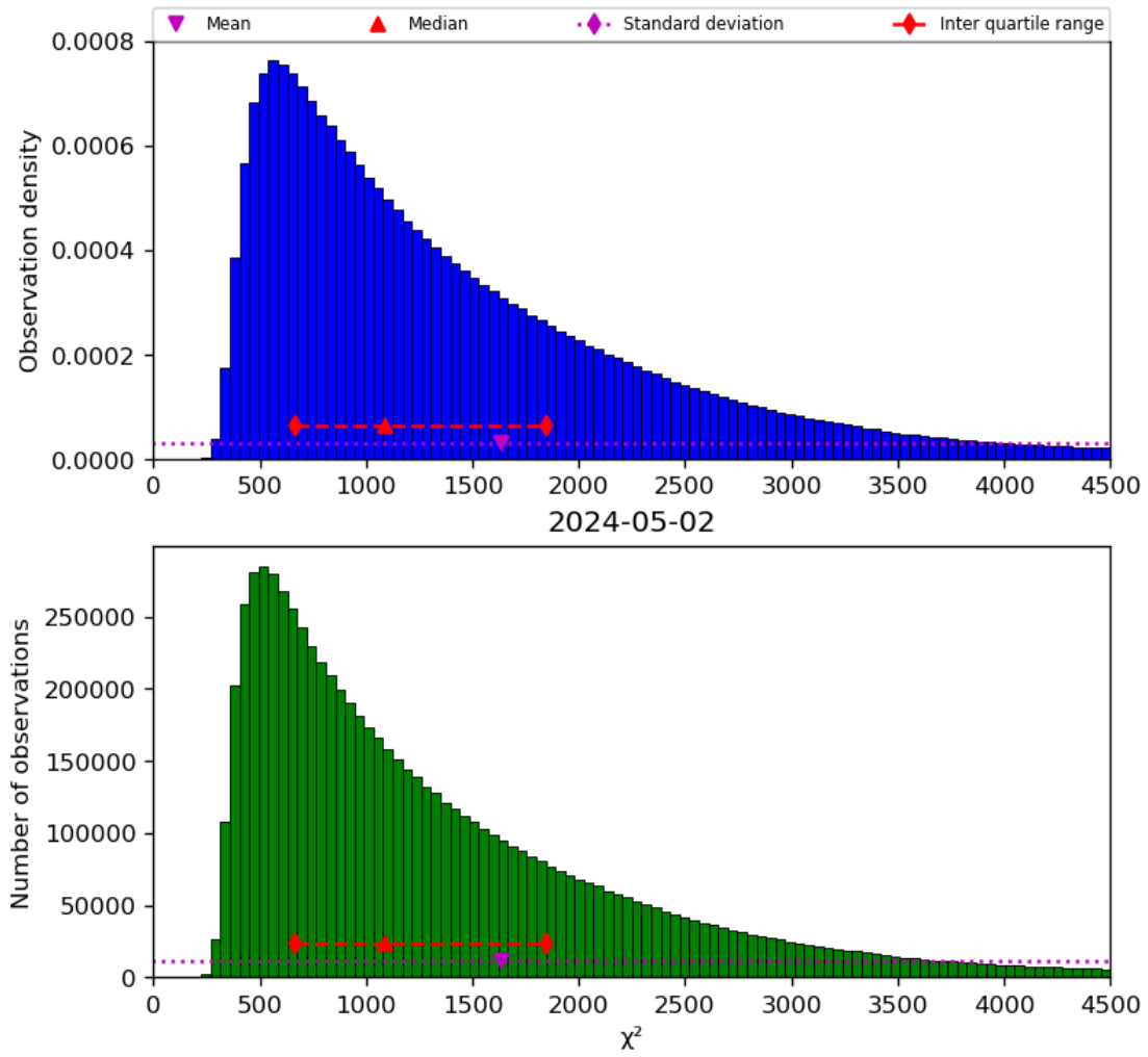
Figure 22: Histogram of “ \chi^2 ” for 2024-05-02 to 2024-05-03
