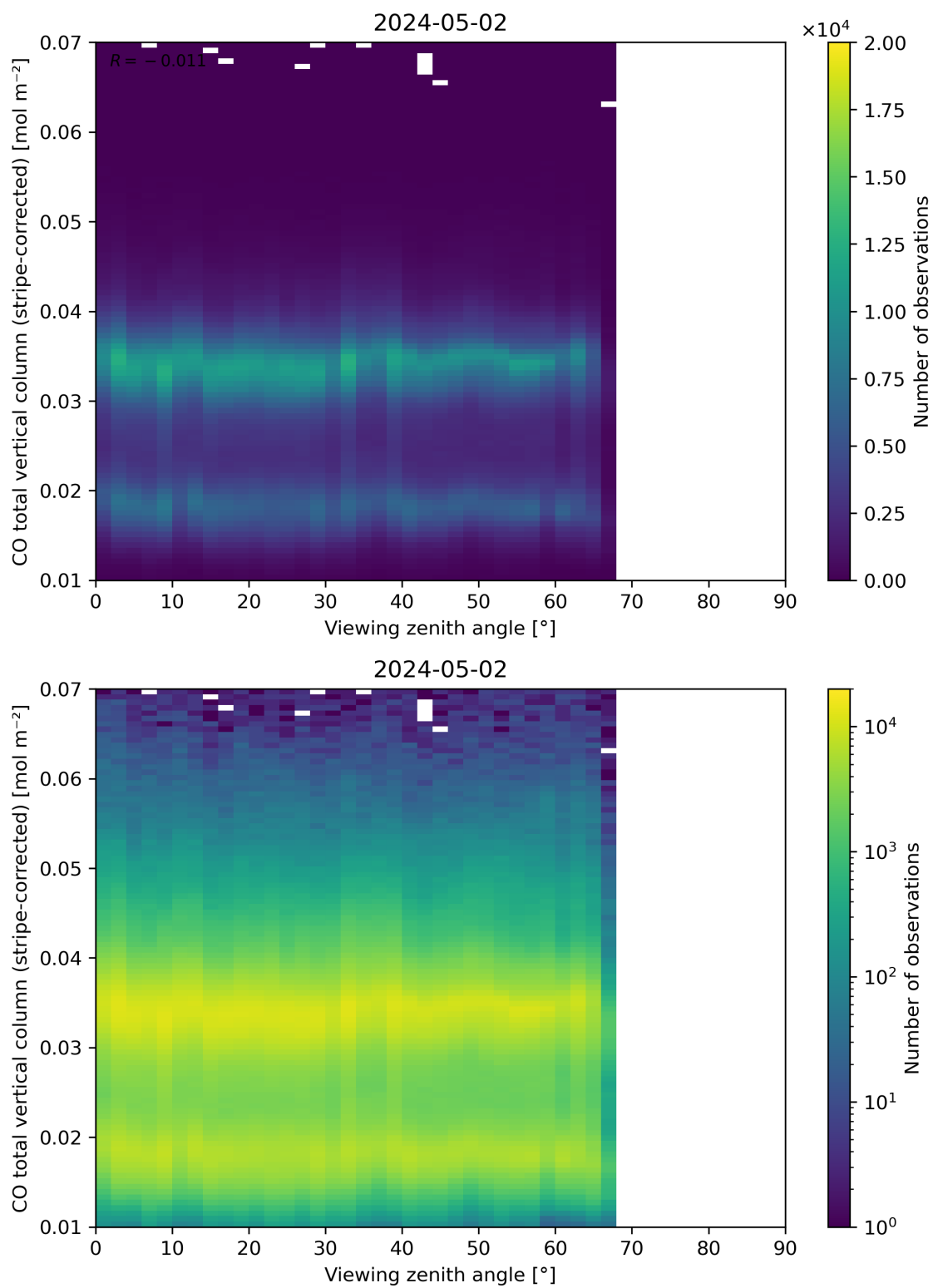
Figure 70: Scatter density plot of “Viewing zenith angle” against “CO total vertical column (stripe-corrected)” for 2024-05-02 to 2024-05-03.
