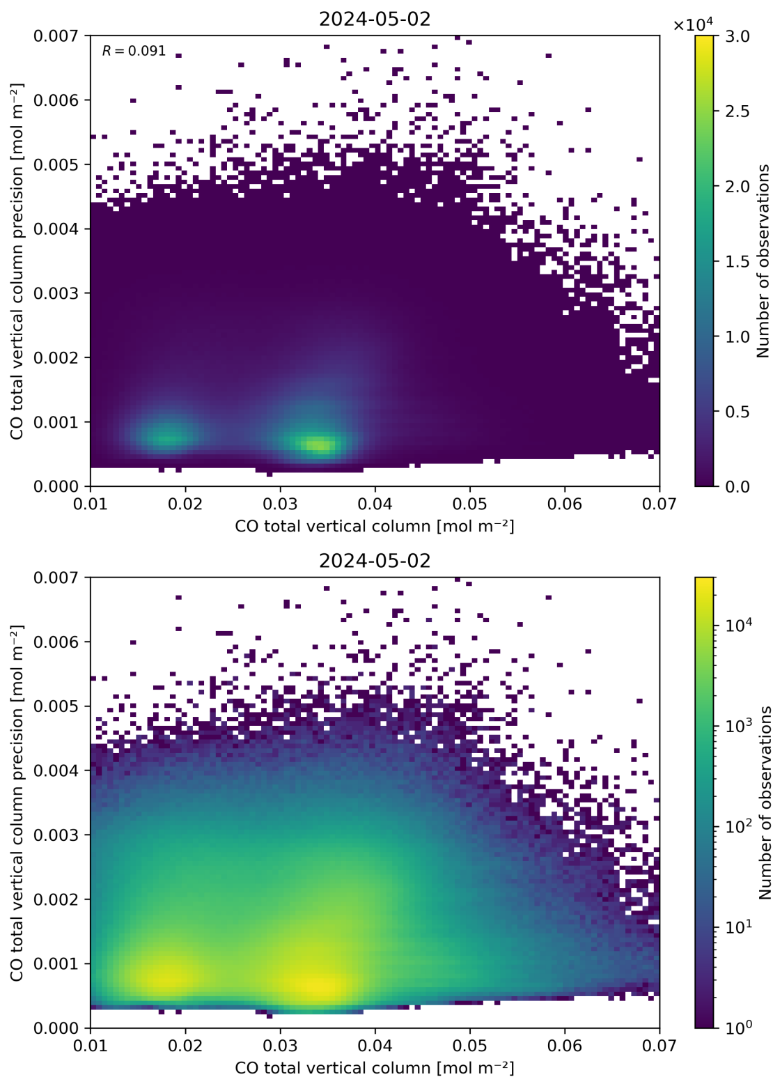
Figure 34: Scatter density plot of “CO total vertical column” against “CO total vertical column precision” for 2024-05-02 to 2024-05-03.
