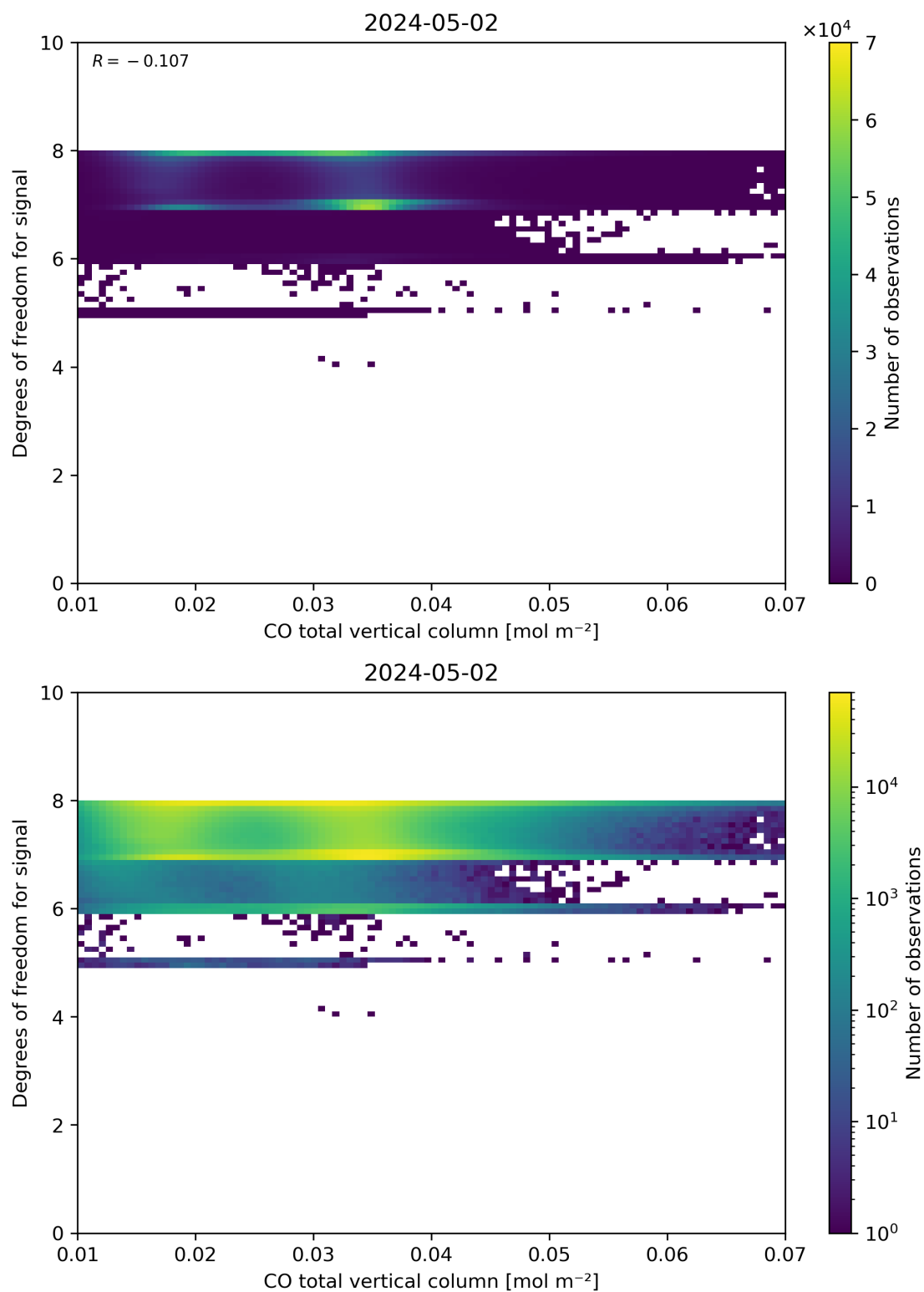
Figure 41: Scatter density plot of “CO total vertical column” against “Degrees of freedom for signal” for 2024-05-02 to 2024-05-03.
