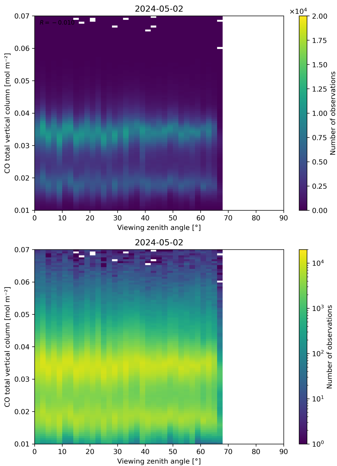
Figure 69: Scatter density plot of “Viewing zenith angle” against “CO total vertical column” for 2024-05-02 to 2024-05-03.
