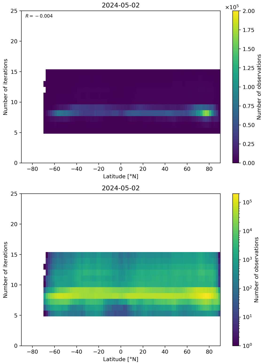
Figure 56: Scatter density plot of “Latitude” against “Number of iterations” for 2024-05-02 to 2024-05-03.
