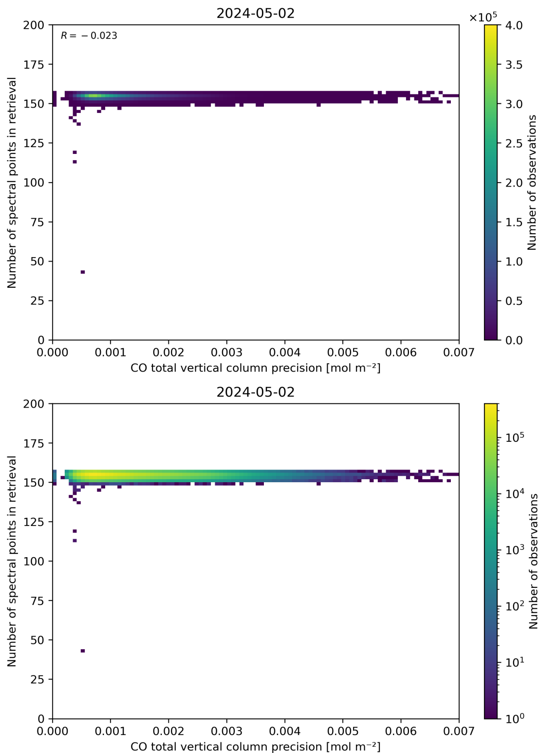
Figure 47: Scatter density plot of “CO total vertical column precision” against “Number of spectral points in retrieval” for 2024-05-02 to 2024-05-03.
