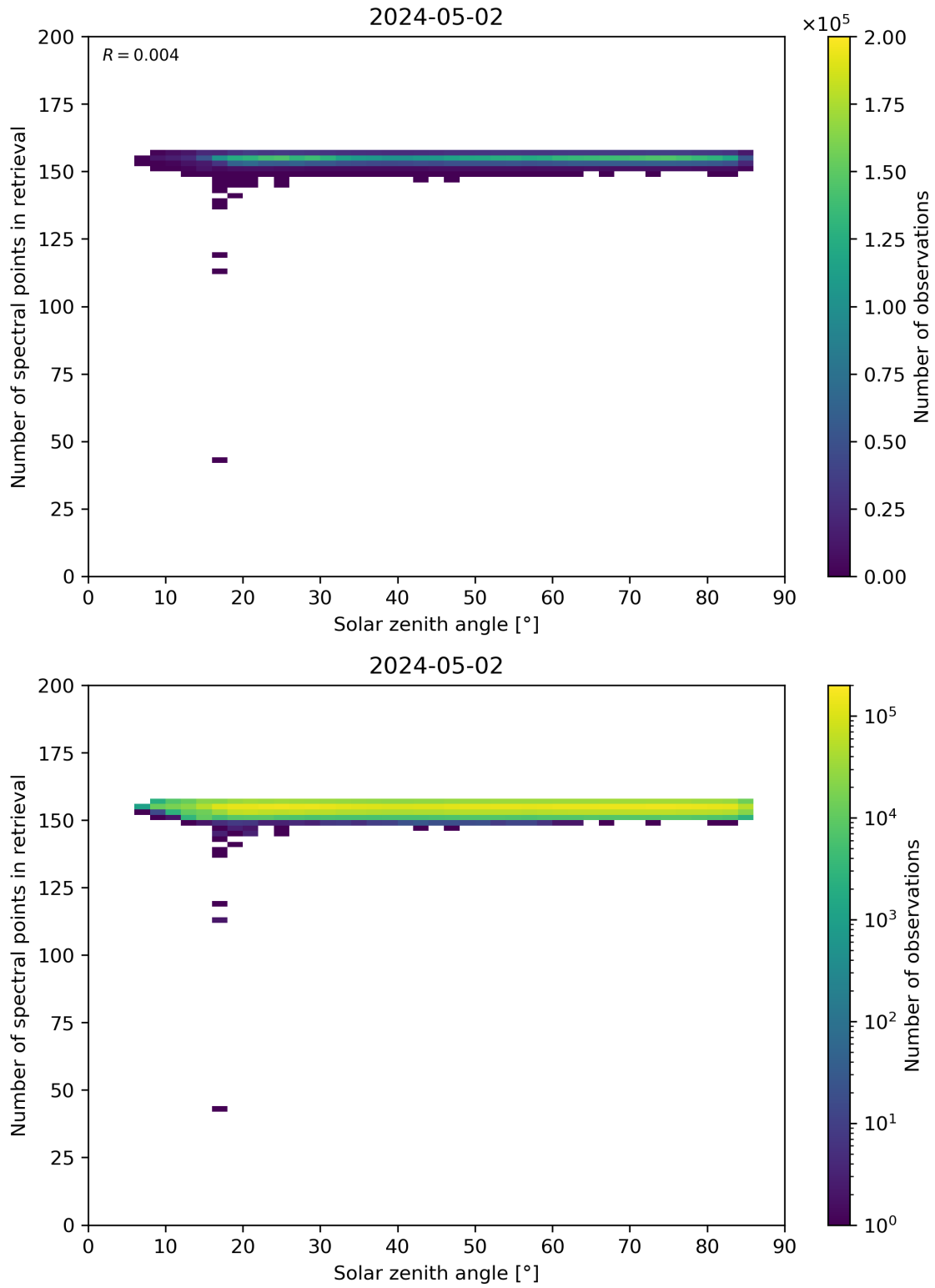
Figure 68: Scatter density plot of “Solar zenith angle” against “Number of spectral points in retrieval” for 2024-05-02 to 2024-05-03.
