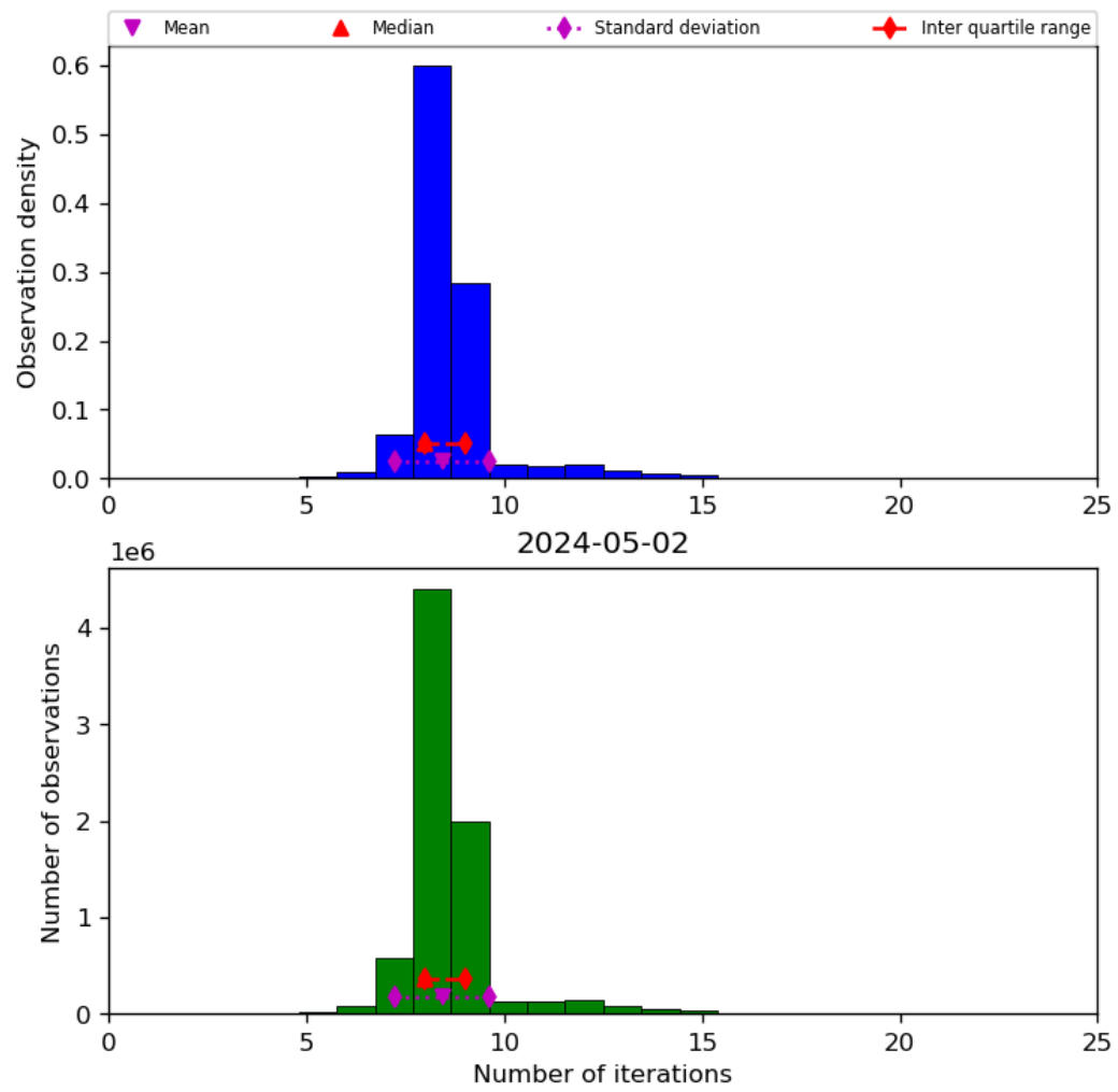
Figure 24: Histogram of “Number of iterations” for 2024-05-02 to 2024-05-03
