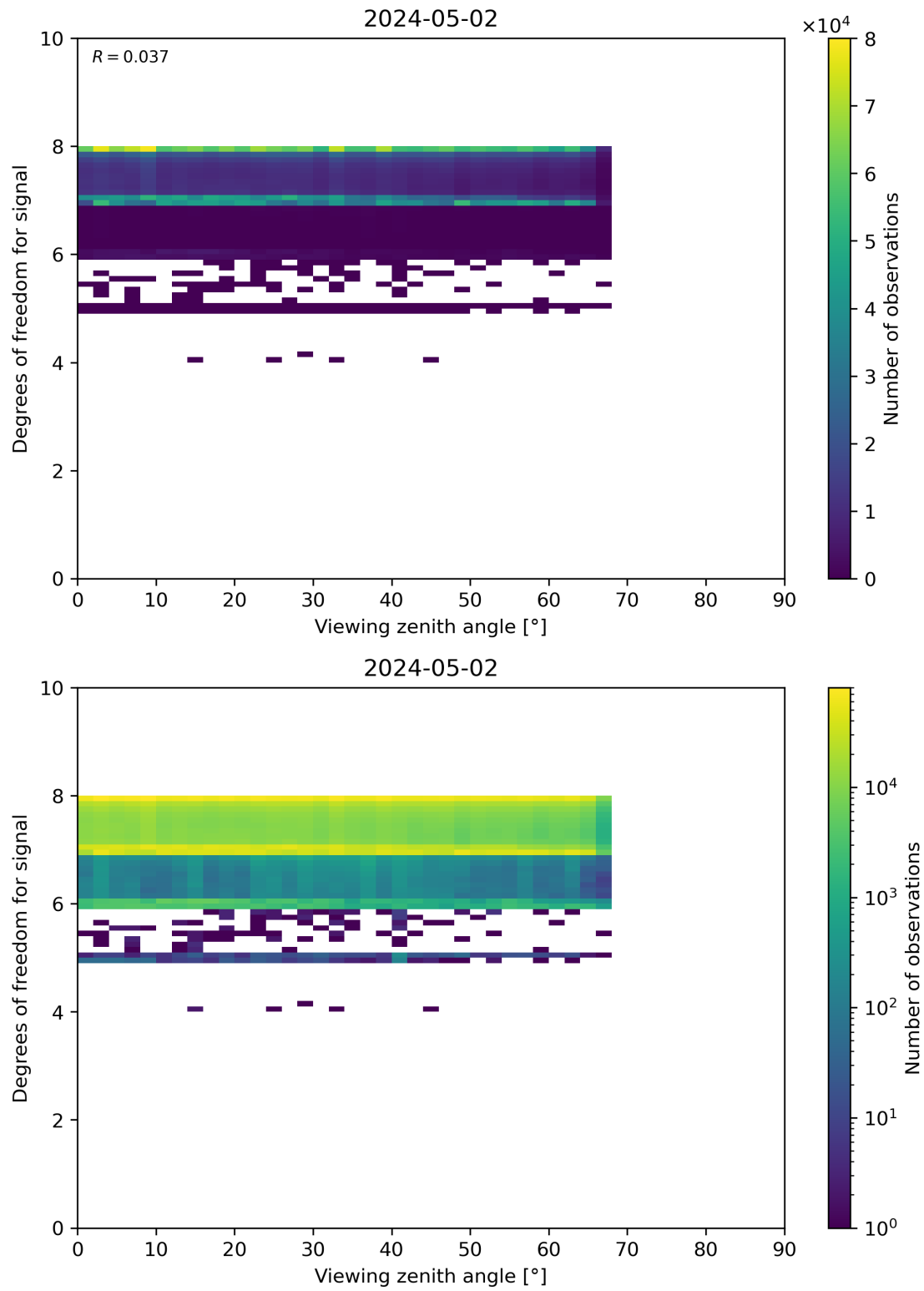
Figure 73: Scatter density plot of “Viewing zenith angle” against “Degrees of freedom for signal” for 2024-05-02 to 2024-05-03.
