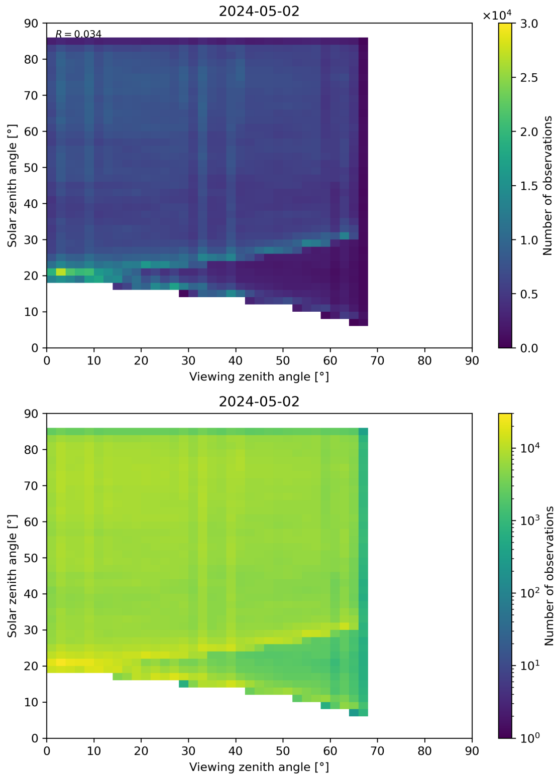
Figure 77: Scatter density plot of “Viewing zenith angle” against “Solar zenith angle” for 2024-05-02 to 2024-05-03.
