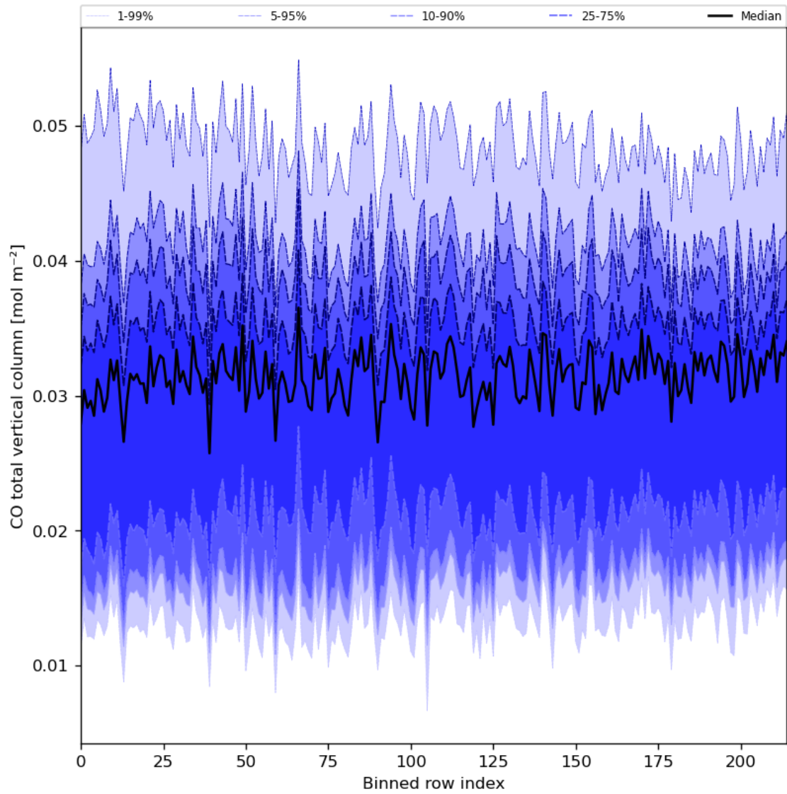
Figure 26: Along track statistics of “CO total vertical column” for 2024-05-02 to 2024-05-03
