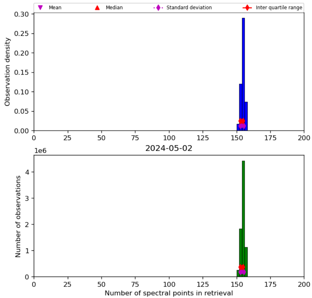
Figure 21: Histogram of “Number of spectral points in retrieval” for 2024-05-02 to 2024-05-03
