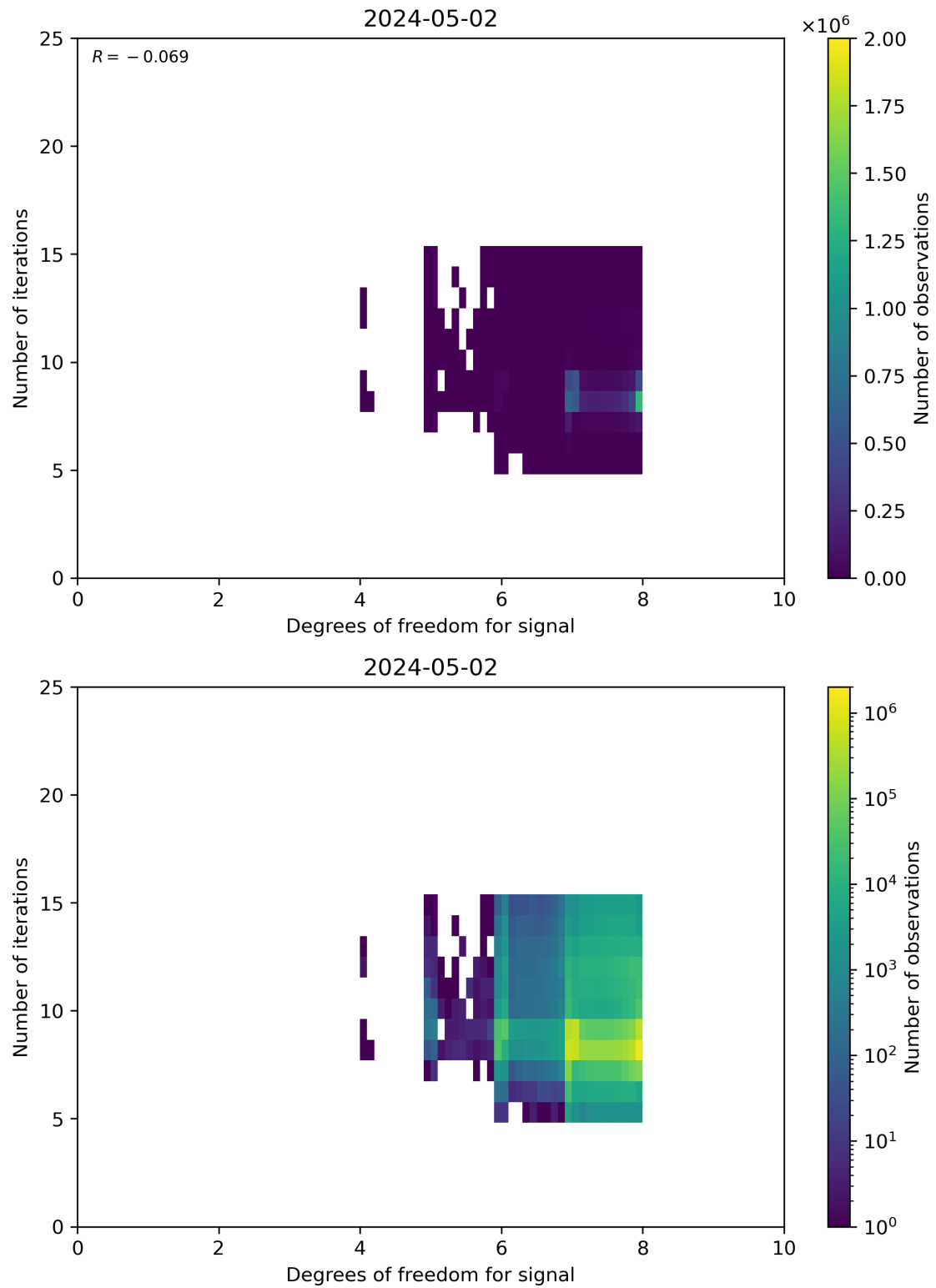
Figure 50: Scatter density plot of “Degrees of freedom for signal” against “Number of iterations” for 2024-05-02 to 2024-05-03.
