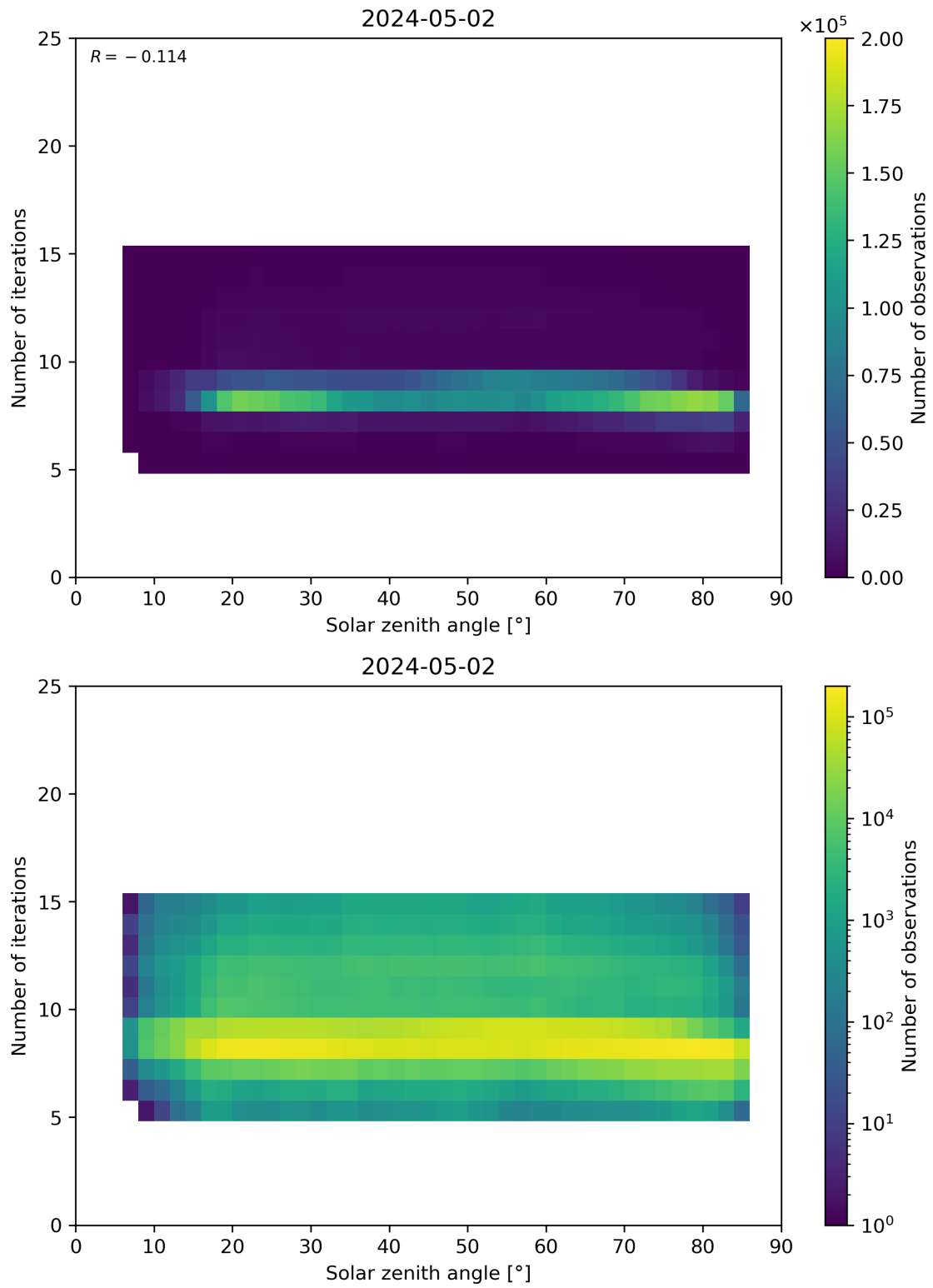
Figure 67: Scatter density plot of “Solar zenith angle” against “Number of iterations” for 2024-05-02 to 2024-05-03.
