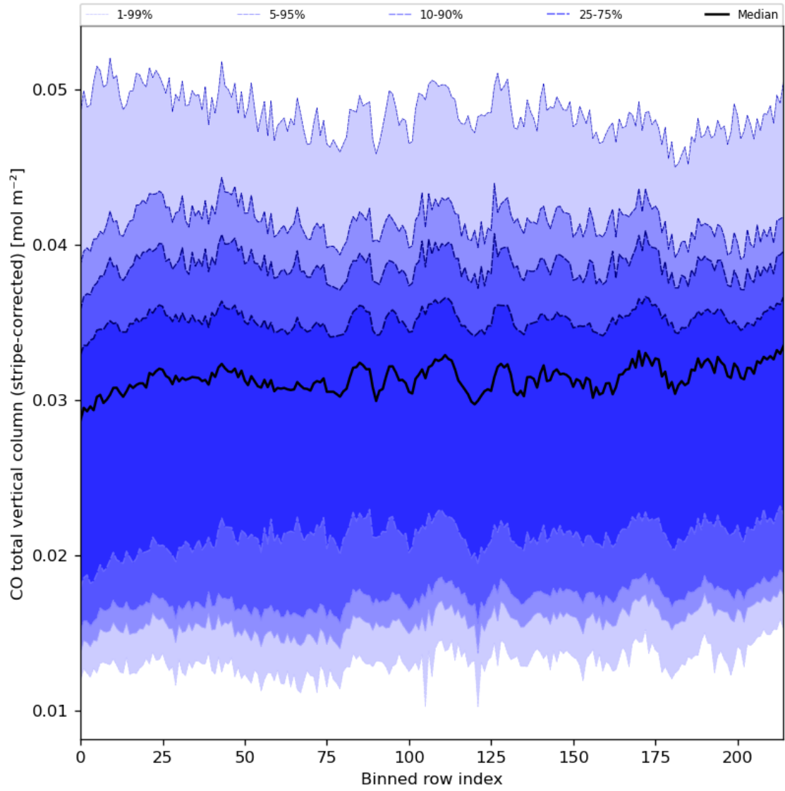
Figure 27: Along track statistics of “CO total vertical column (stripe-corrected)” for 2024-05-02 to 2024-05-03
