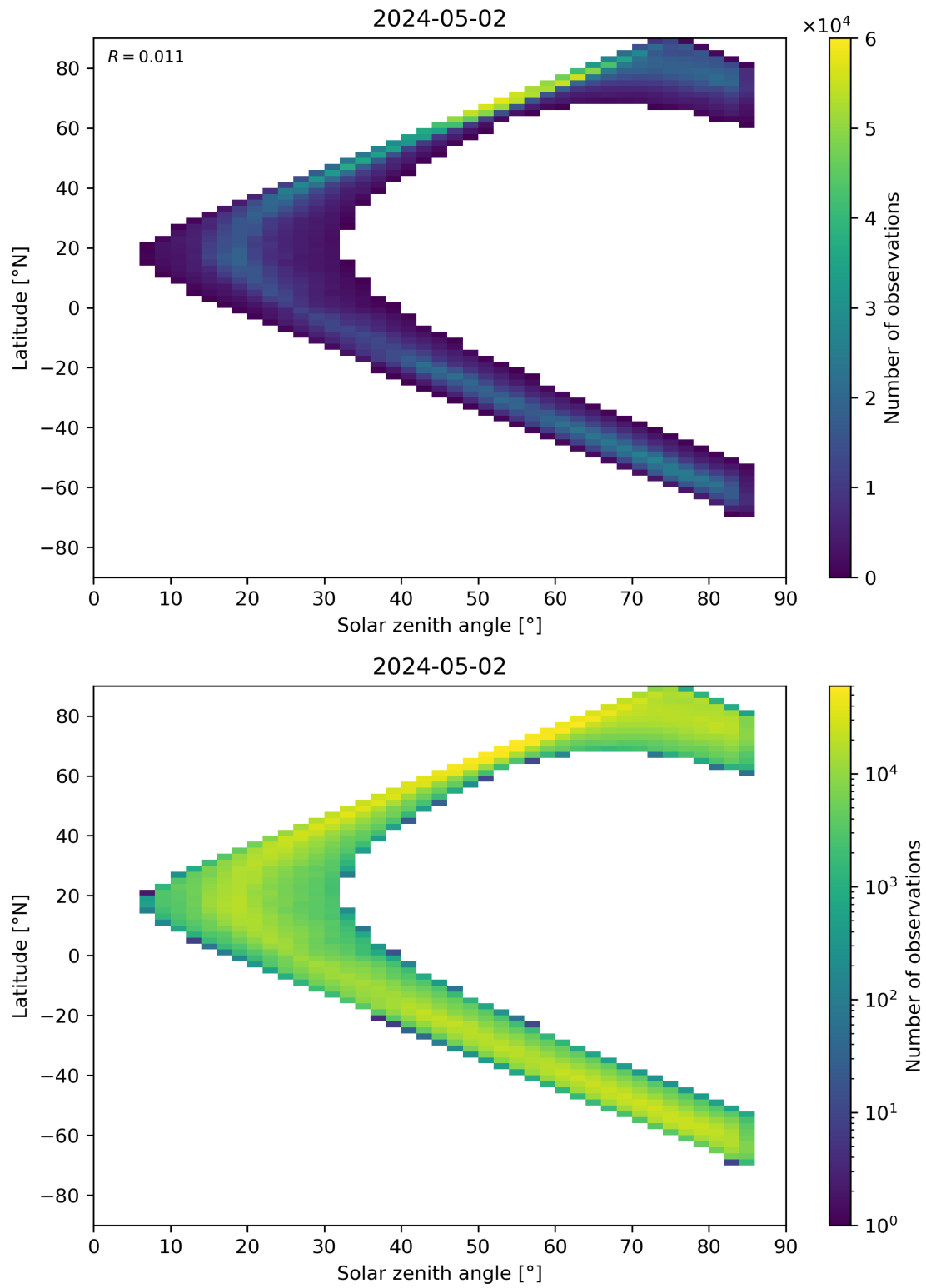
Figure 66: Scatter density plot of “Solar zenith angle” against “Latitude” for 2024-05-02 to 2024-05-03.
