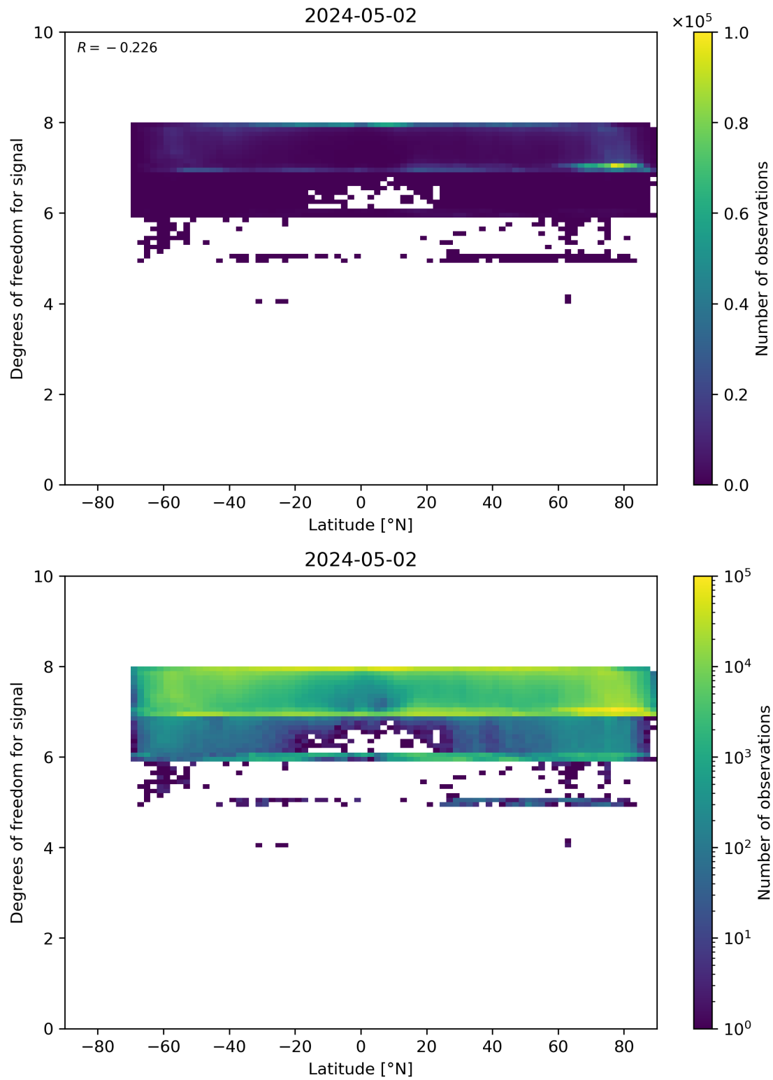
Figure 55: Scatter density plot of “Latitude” against “Degrees of freedom for signal” for 2024-05-02 to 2024-05-03.
