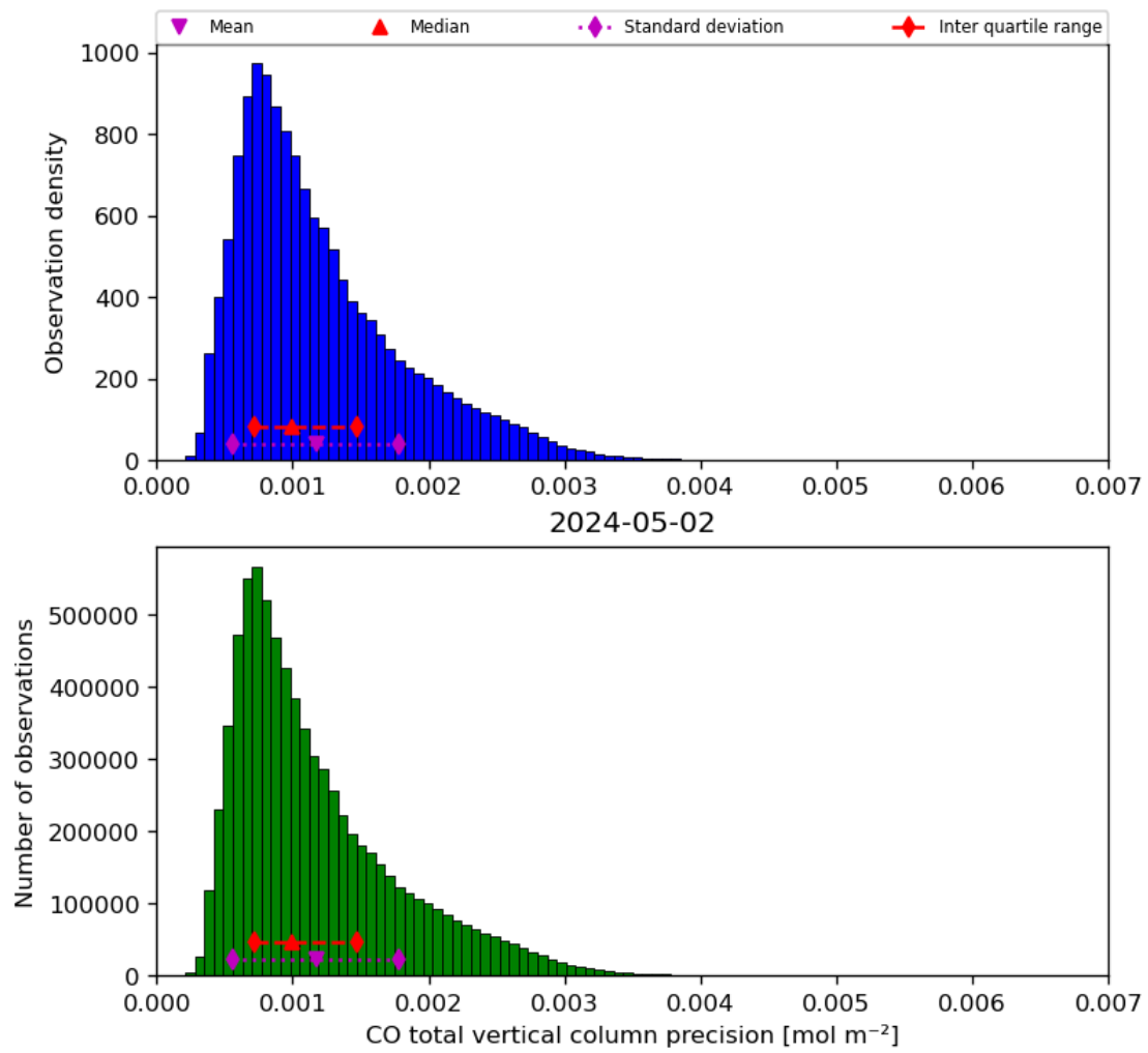
Figure 20: Histogram of “CO total vertical column precision” for 2024-05-02 to 2024-05-03
