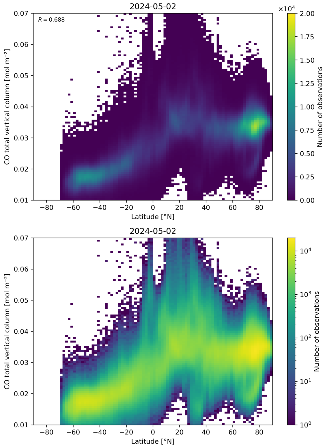
Figure 51: Scatter density plot of “Latitude” against “CO total vertical column” for 2024-05-02 to 2024-05-03.
