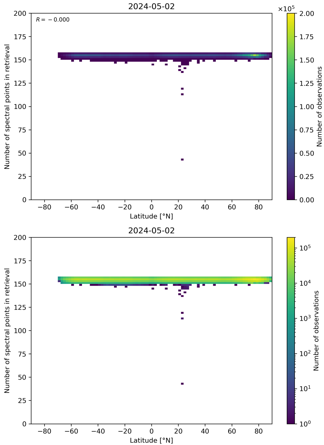
Figure 57: Scatter density plot of “Latitude” against “Number of spectral points in retrieval” for 2024-05-02 to 2024-05-03.
