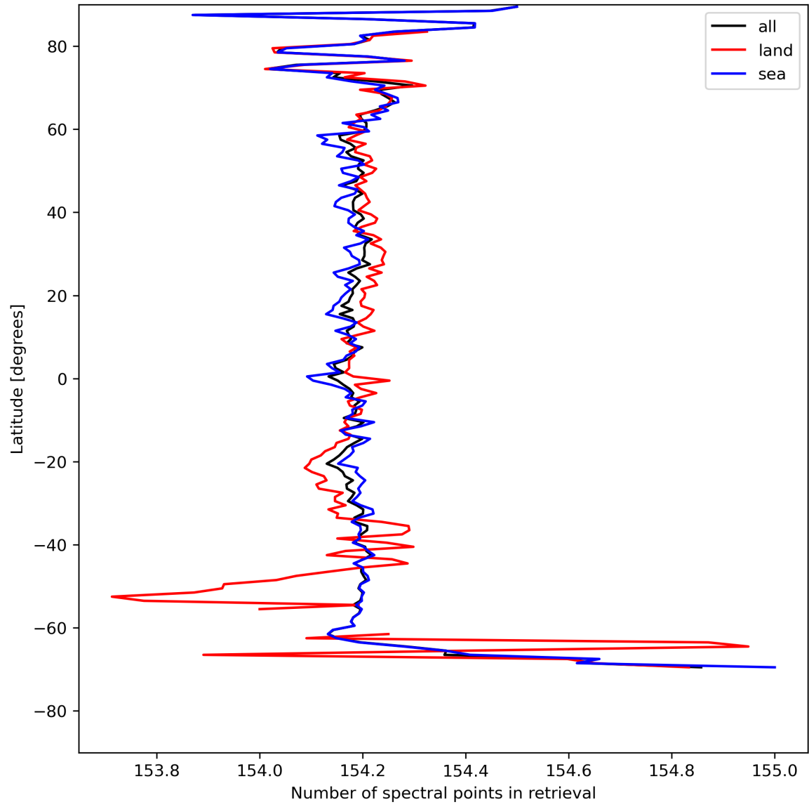
Figure 13: Zonal average of “Number of spectral points in retrieval” for 2024-05-02 to 2024-05-03.
