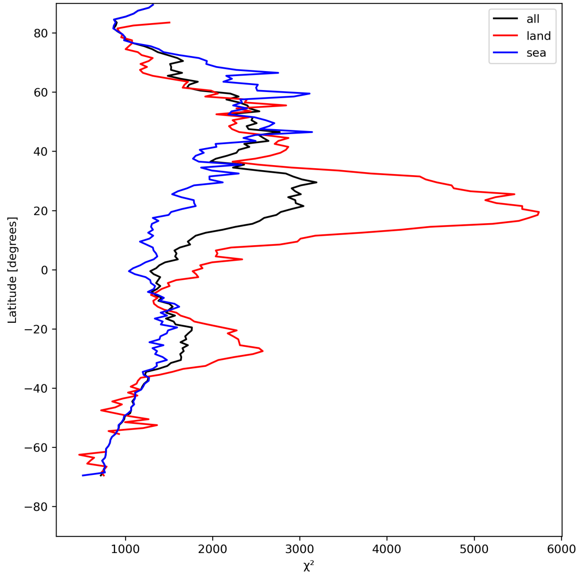
Figure 14: Zonal average of “ \chi^2 ” for 2024-05-02 to 2024-05-03.
