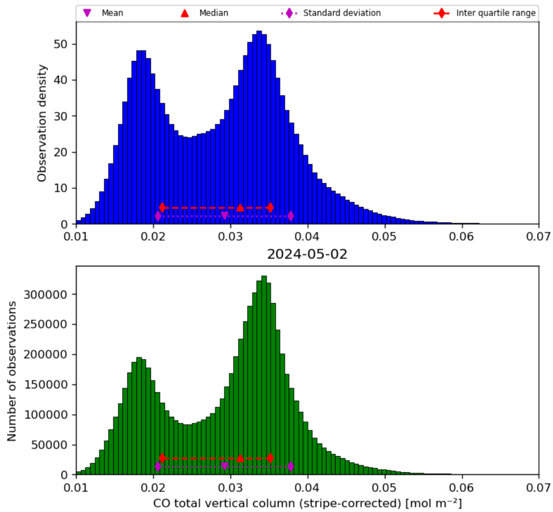
Figure 19: Histogram of “CO total vertical column (stripe-corrected)” for 2024-05-02 to 2024-05-03
