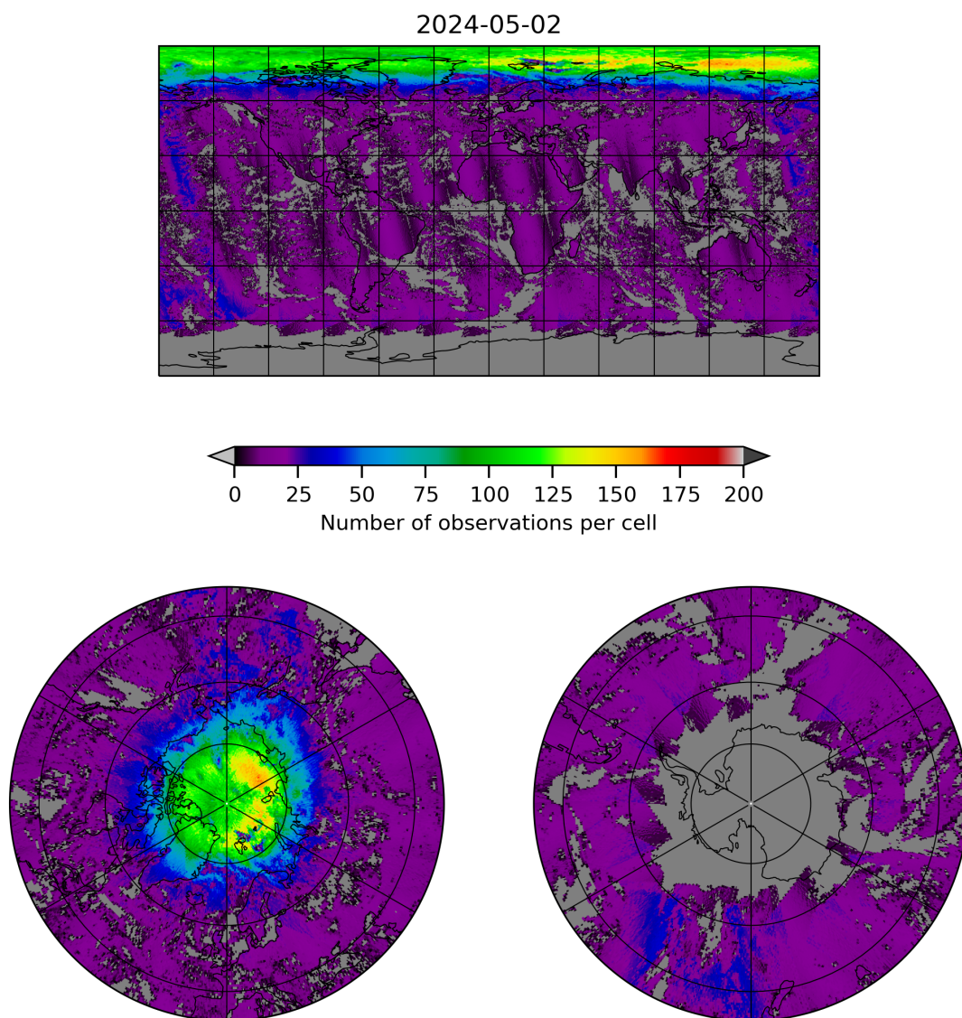
Figure 8: Map of the number of observations for 2024-05-02 to 2024-05-03
