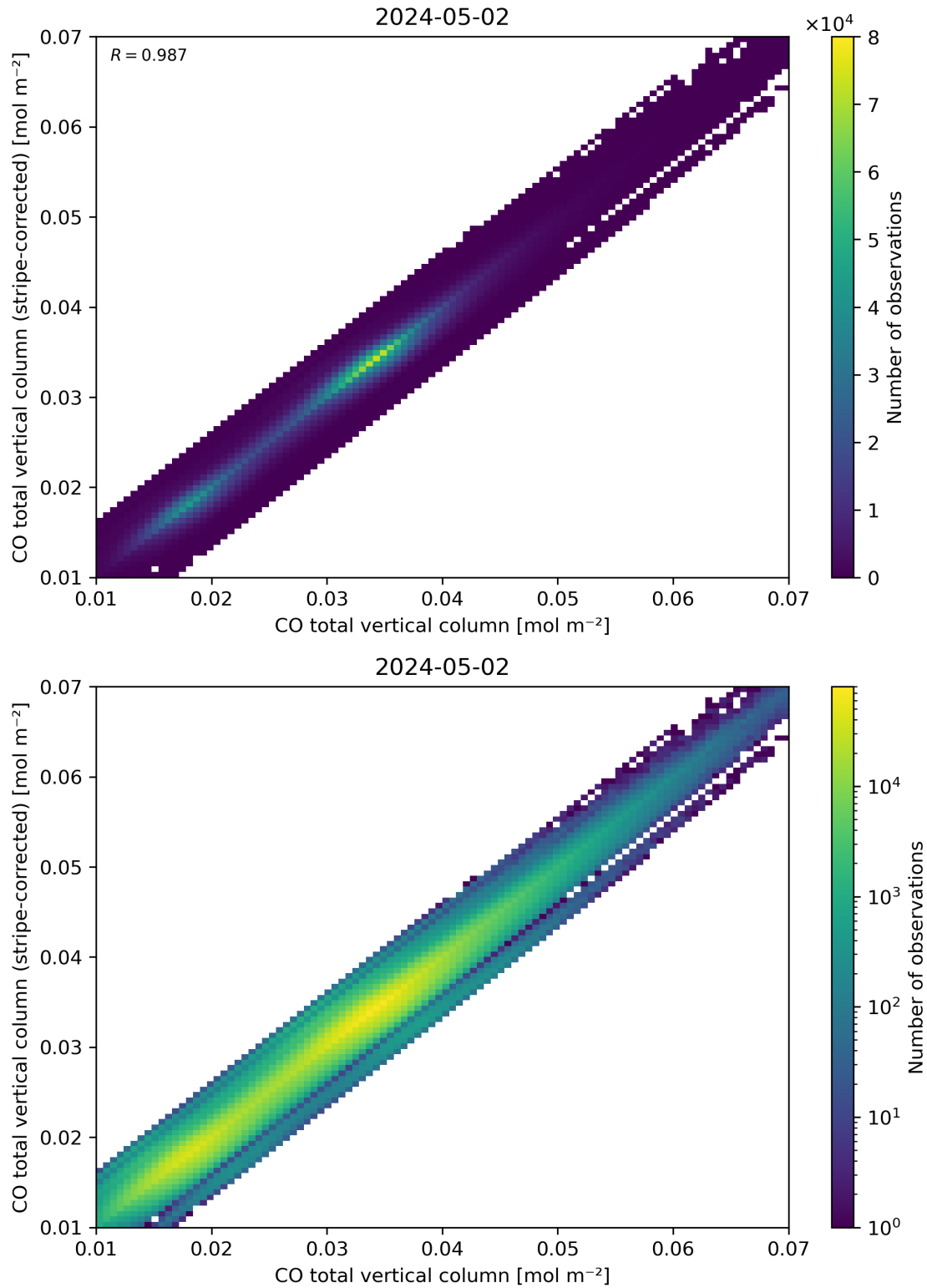
Figure 33: Scatter density plot of “CO total vertical column” against “CO total vertical column (stripe-corrected)” for 2024-05-02 to 2024-05-03.
