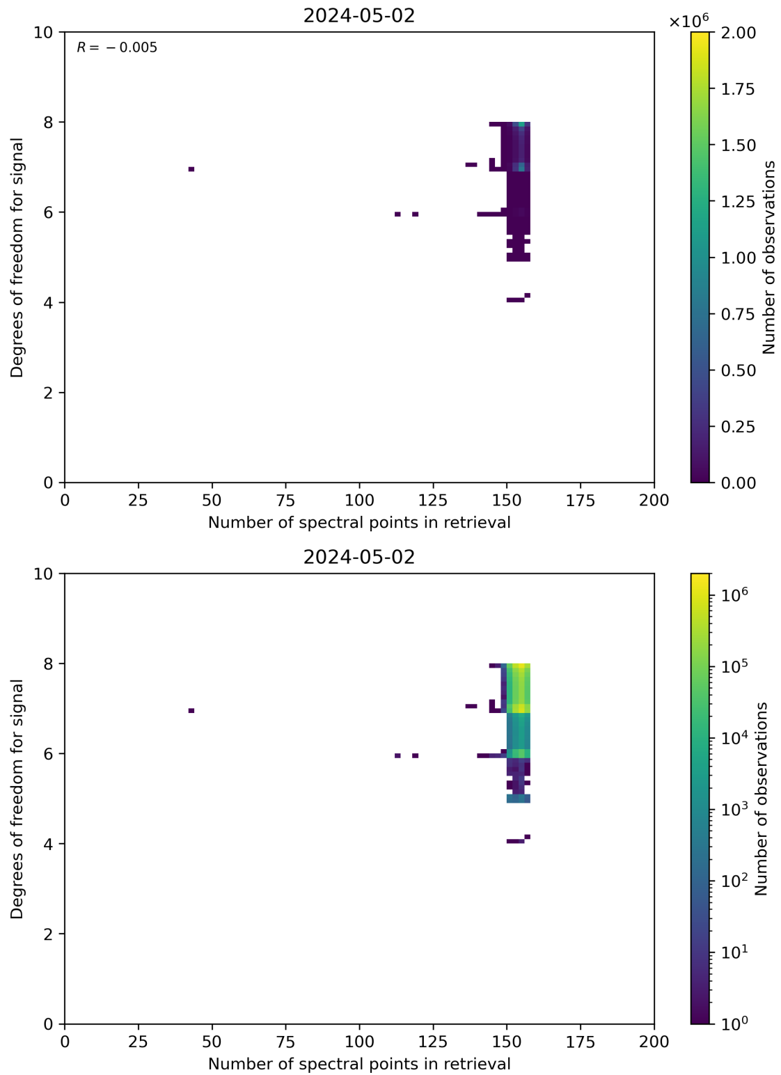
Figure 59: Scatter density plot of “Number of spectral points in retrieval” against “Degrees of freedom for signal” for 2024-05-02 to 2024-05-03.
