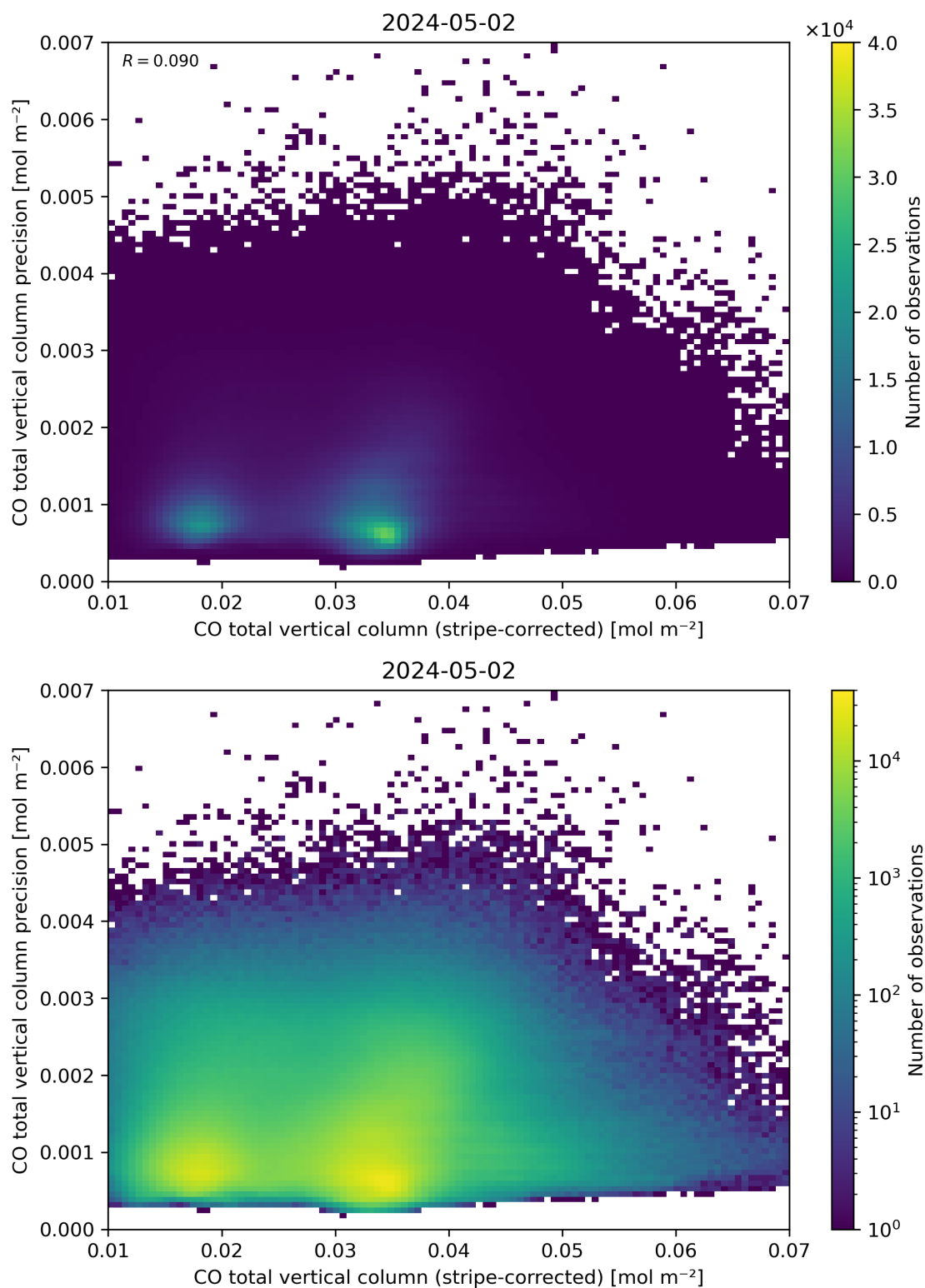
Figure 36: Scatter density plot of “CO total vertical column (stripe-corrected)” against “CO total vertical column precision” for 2024-05-02 to 2024-05-03.
