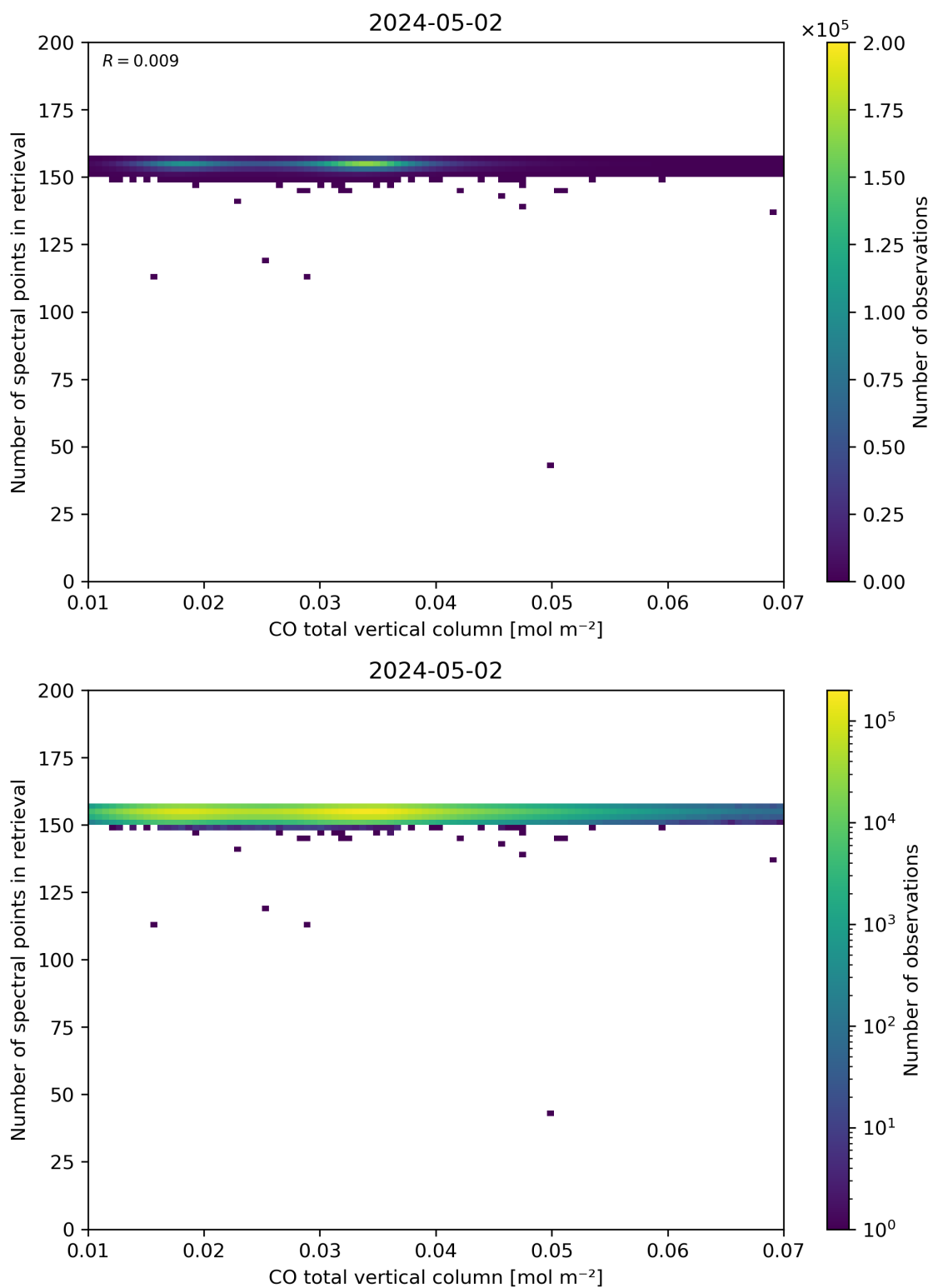
Figure 43: Scatter density plot of “CO total vertical column” against “Number of spectral points in retrieval” for 2024-05-02 to 2024-05-03.
