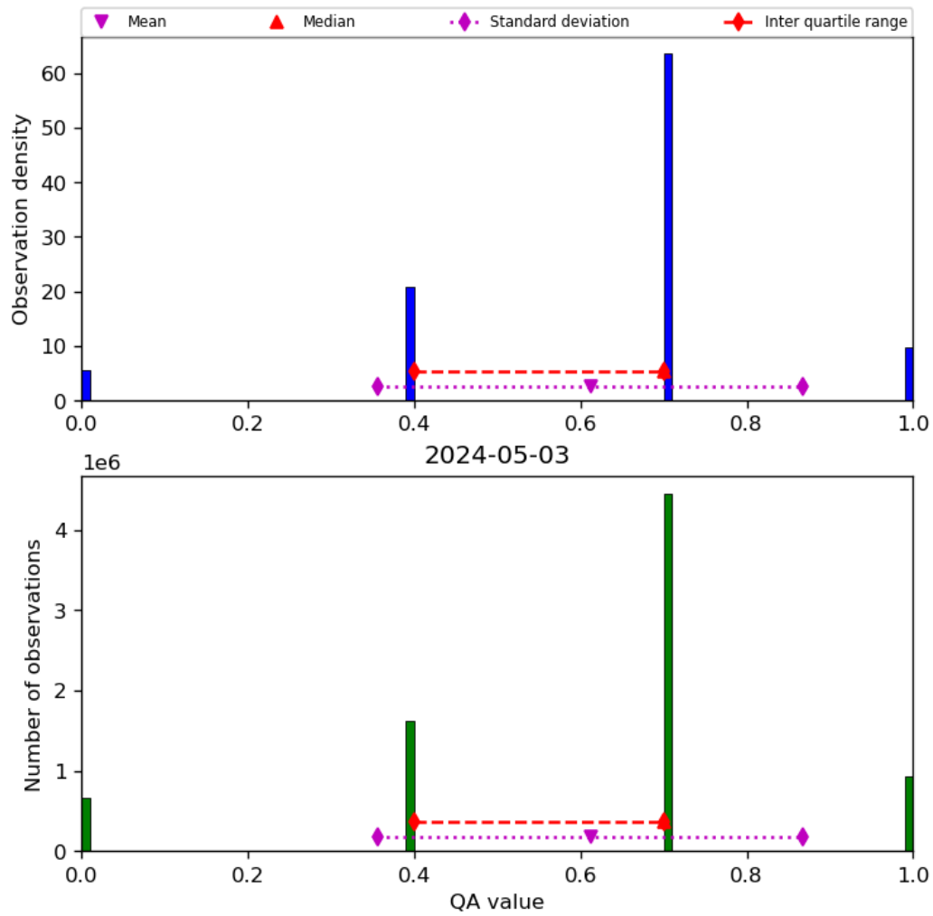
Figure 17: Histogram of “QA value” for 2024-05-02 to 2024-05-04
