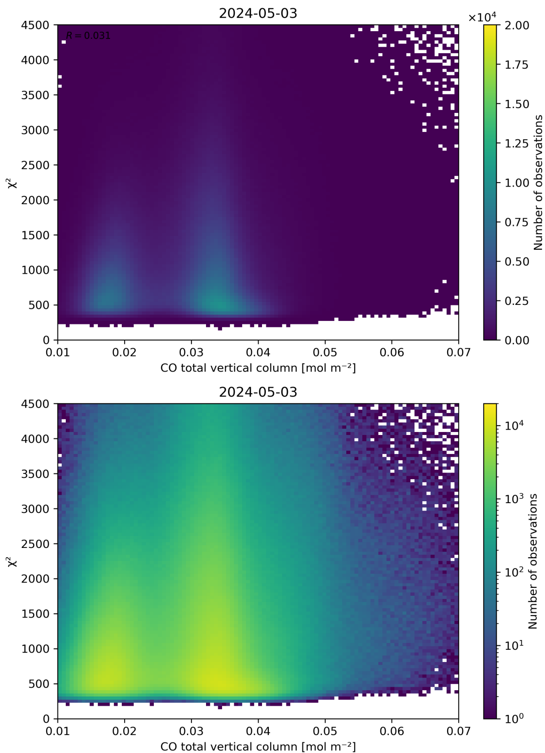
Figure 35: Scatter density plot of “CO total vertical column” against “ \chi^2 ” for 2024-05-02 to 2024-05-04.
