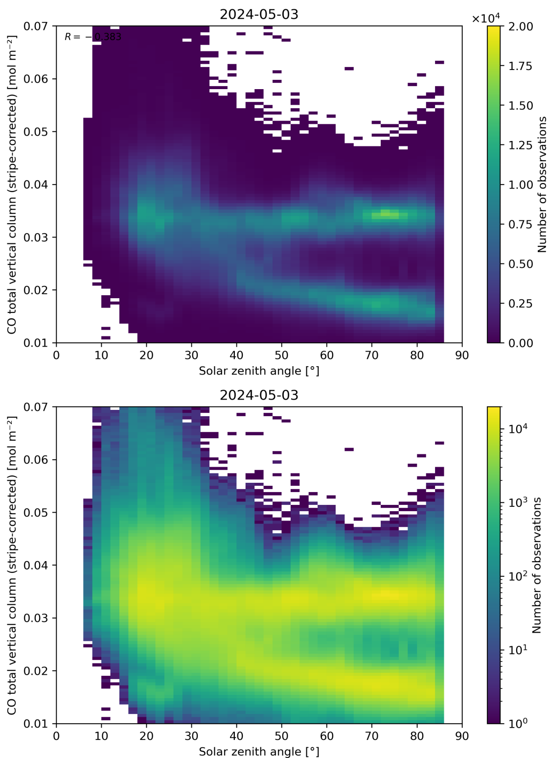
Figure 62: Scatter density plot of “Solar zenith angle” against “CO total vertical column (stripe-corrected)” for 2024-05-02 to 2024-05-04.
