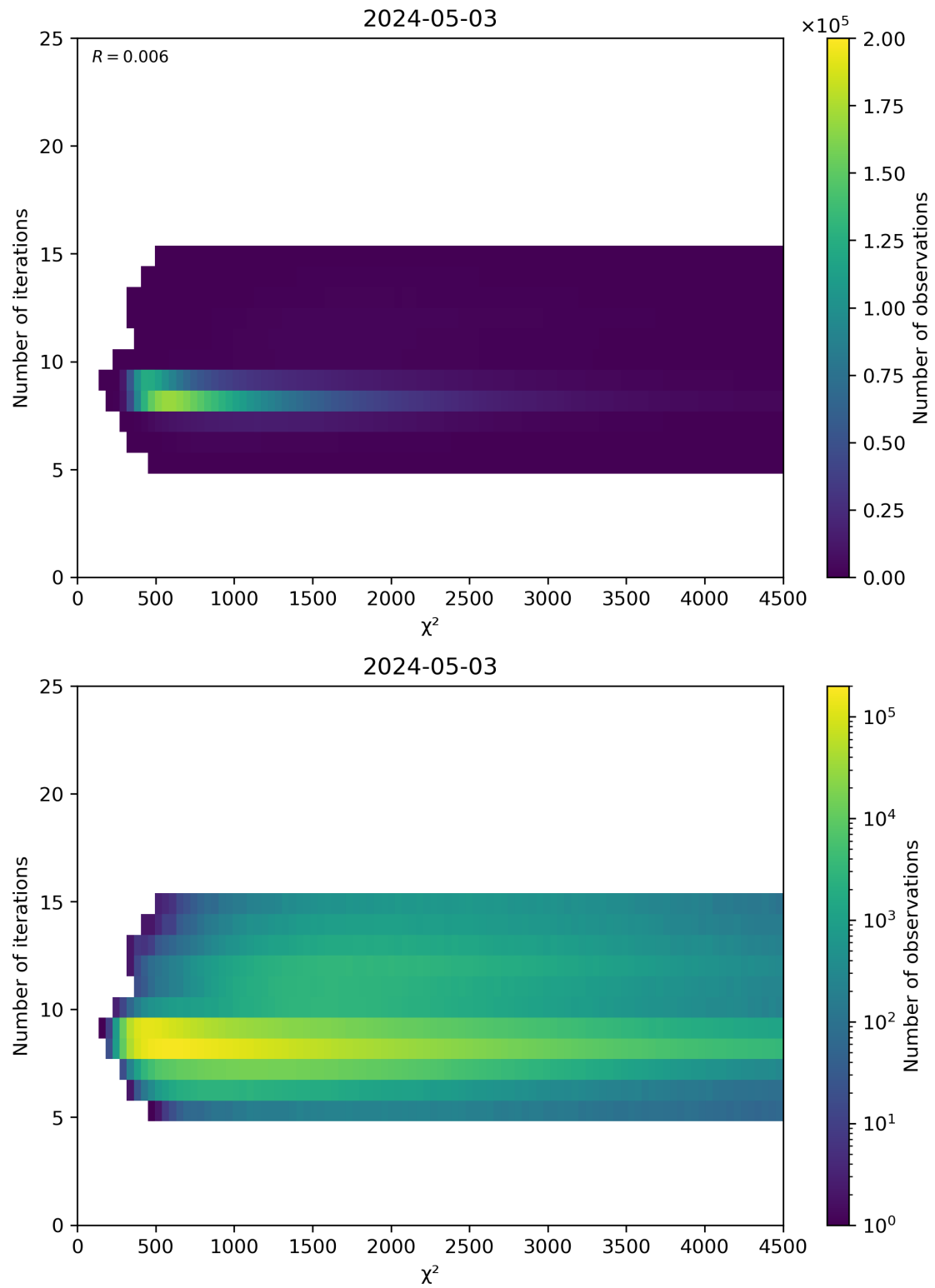
Figure 49: Scatter density plot of " \chi^2 " against "Number of iterations" for 2024-05-02 to 2024-05-04.
