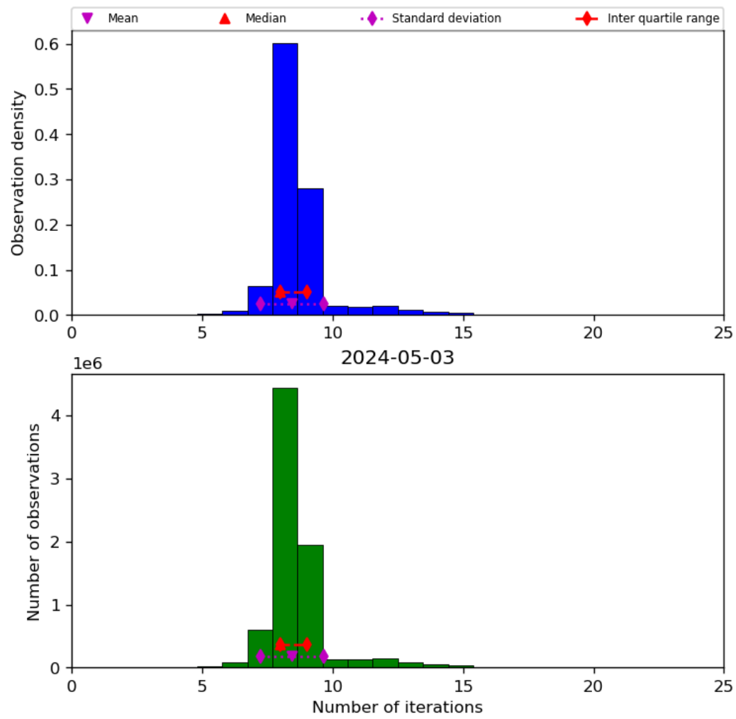
Figure 24: Histogram of “Number of iterations” for 2024-05-02 to 2024-05-04
