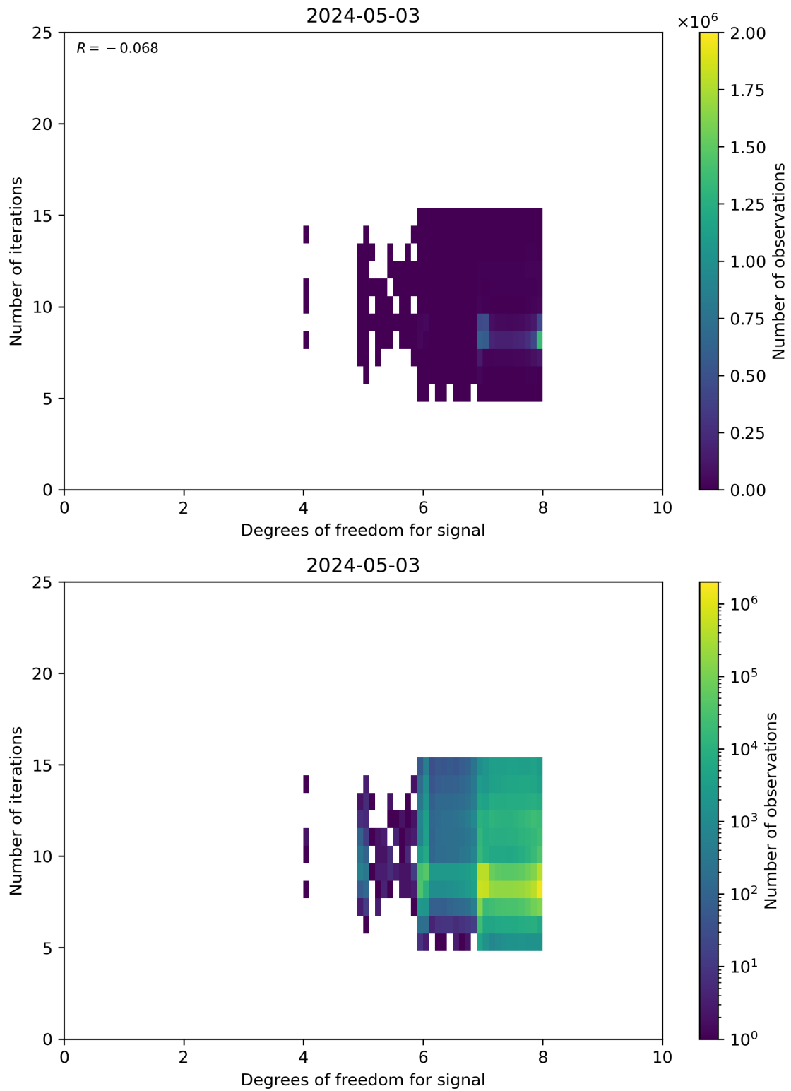
Figure 50: Scatter density plot of “Degrees of freedom for signal” against “Number of iterations” for 2024-05-02 to 2024-05-04.
