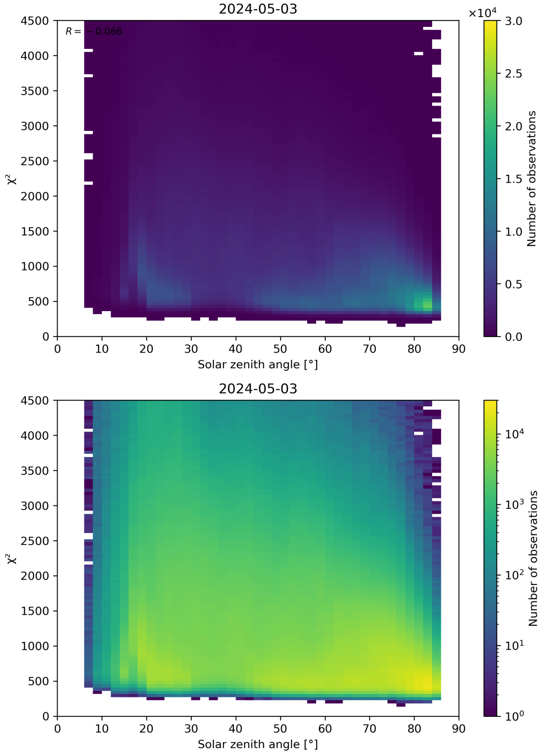
Figure 64: Scatter density plot of “Solar zenith angle” against “ \chi^2 ” for 2024-05-02 to 2024-05-04.
