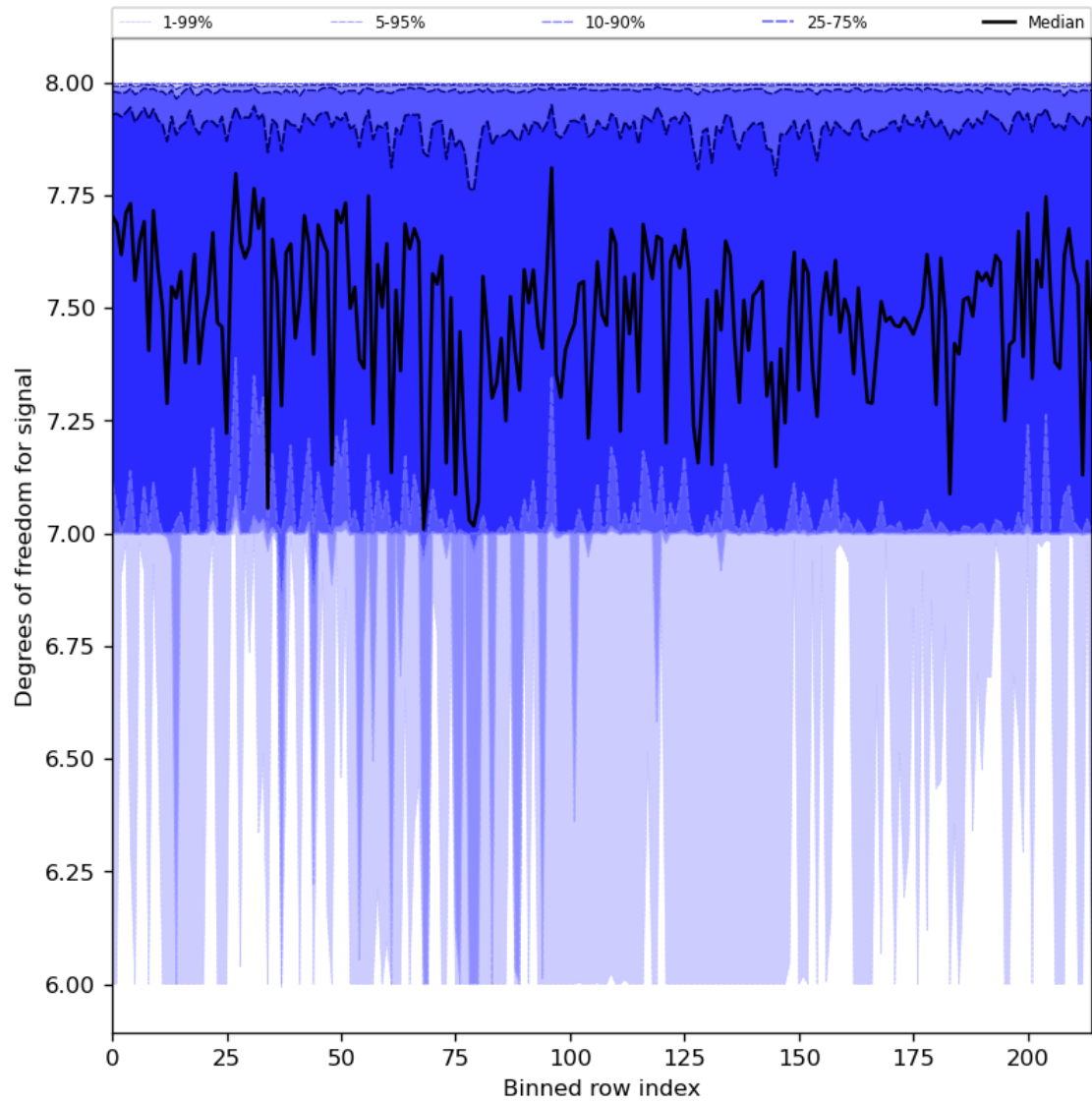
Figure 31: Along track statistics of “Degrees of freedom for signal” for 2024-05-02 to 2024-05-04
