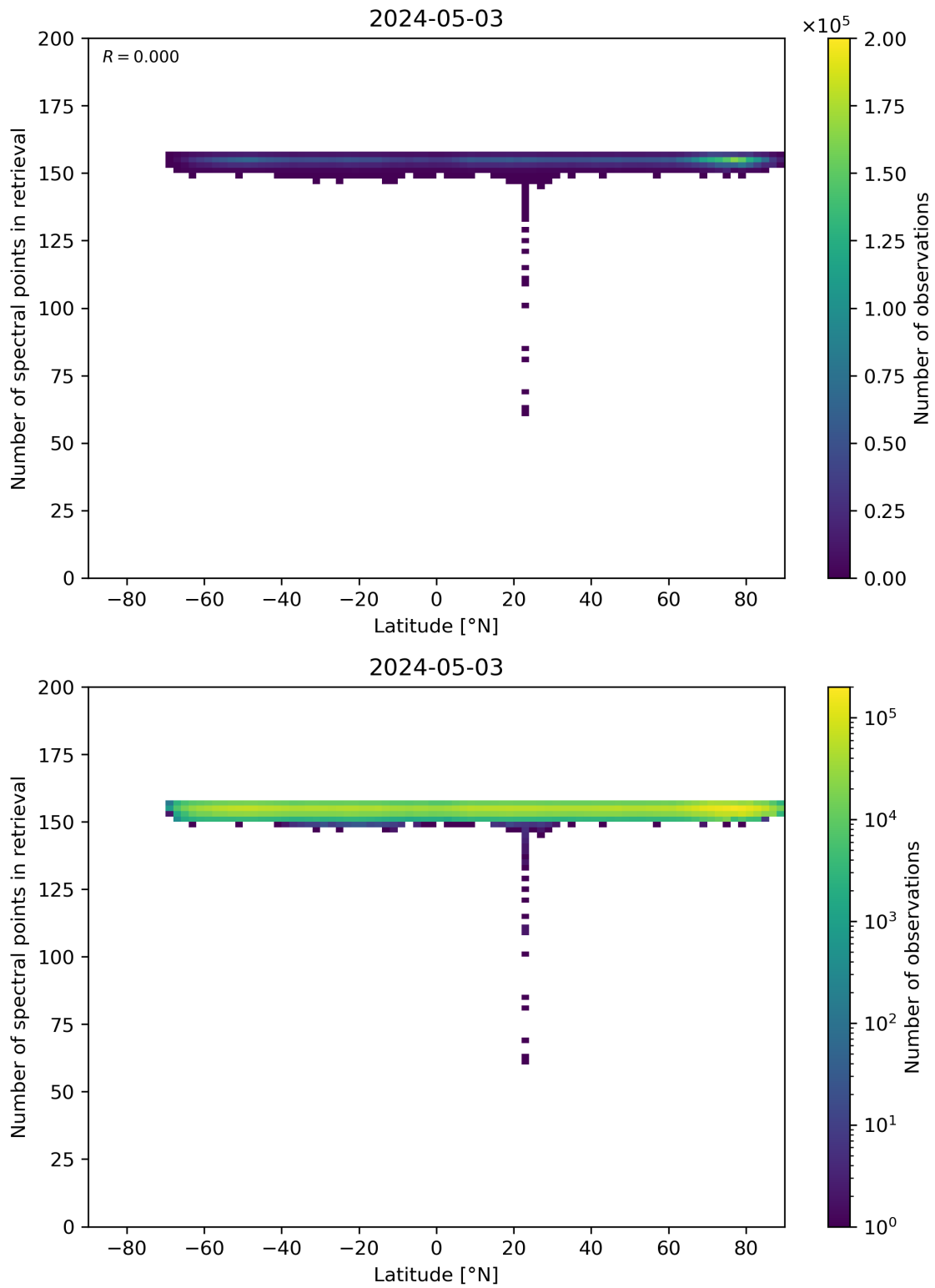
Figure 57: Scatter density plot of “Latitude” against “Number of spectral points in retrieval” for 2024-05-02 to 2024-05-04.
