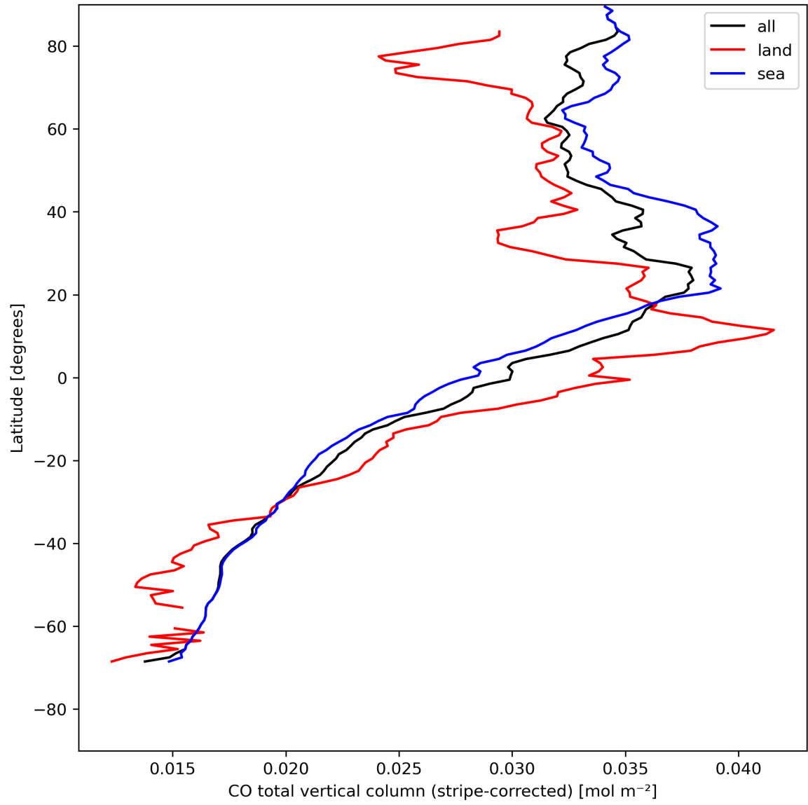
Figure 11: Zonal average of “CO total vertical column (stripe-corrected)” for 2024-05-02 to 2024-05-04.
