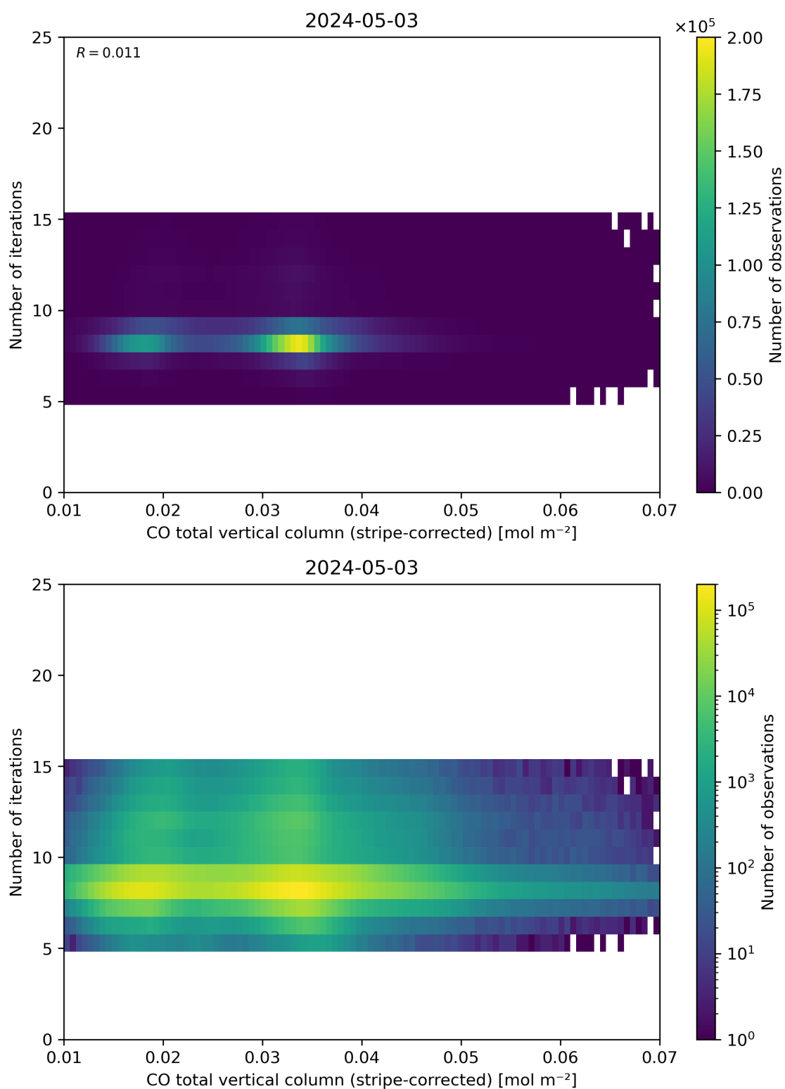
Figure 39: Scatter density plot of “CO total vertical column (stripe-corrected)” against “Number of iterations” for 2024-05-02 to 2024-05-04.
