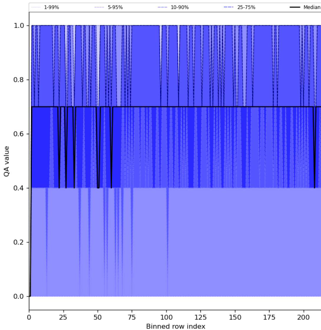
Figure 25: Along track statistics of “QA value” for 2024-05-02 to 2024-05-04
