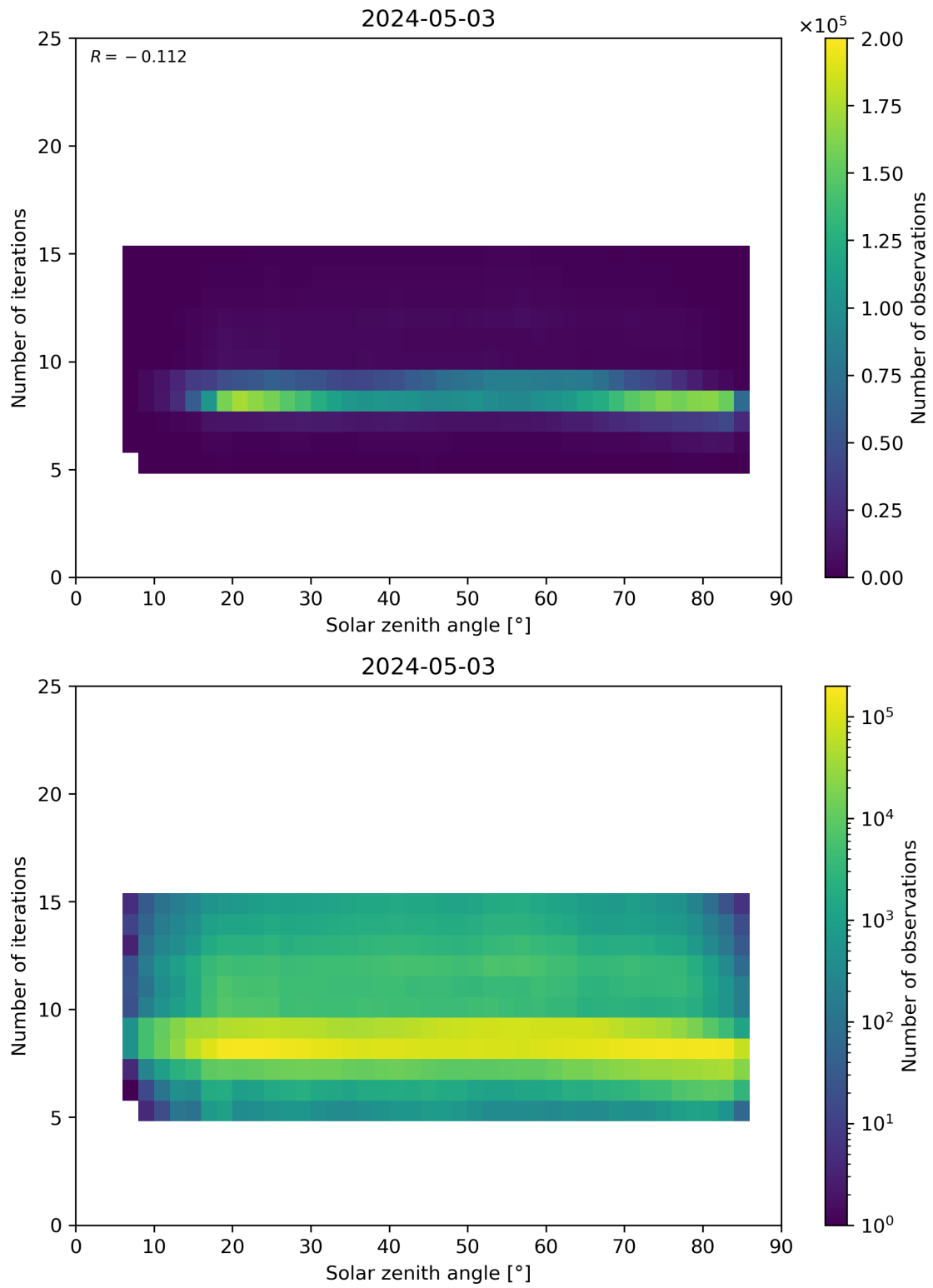
Figure 67: Scatter density plot of “Solar zenith angle” against “Number of iterations” for 2024-05-02 to 2024-05-04.
