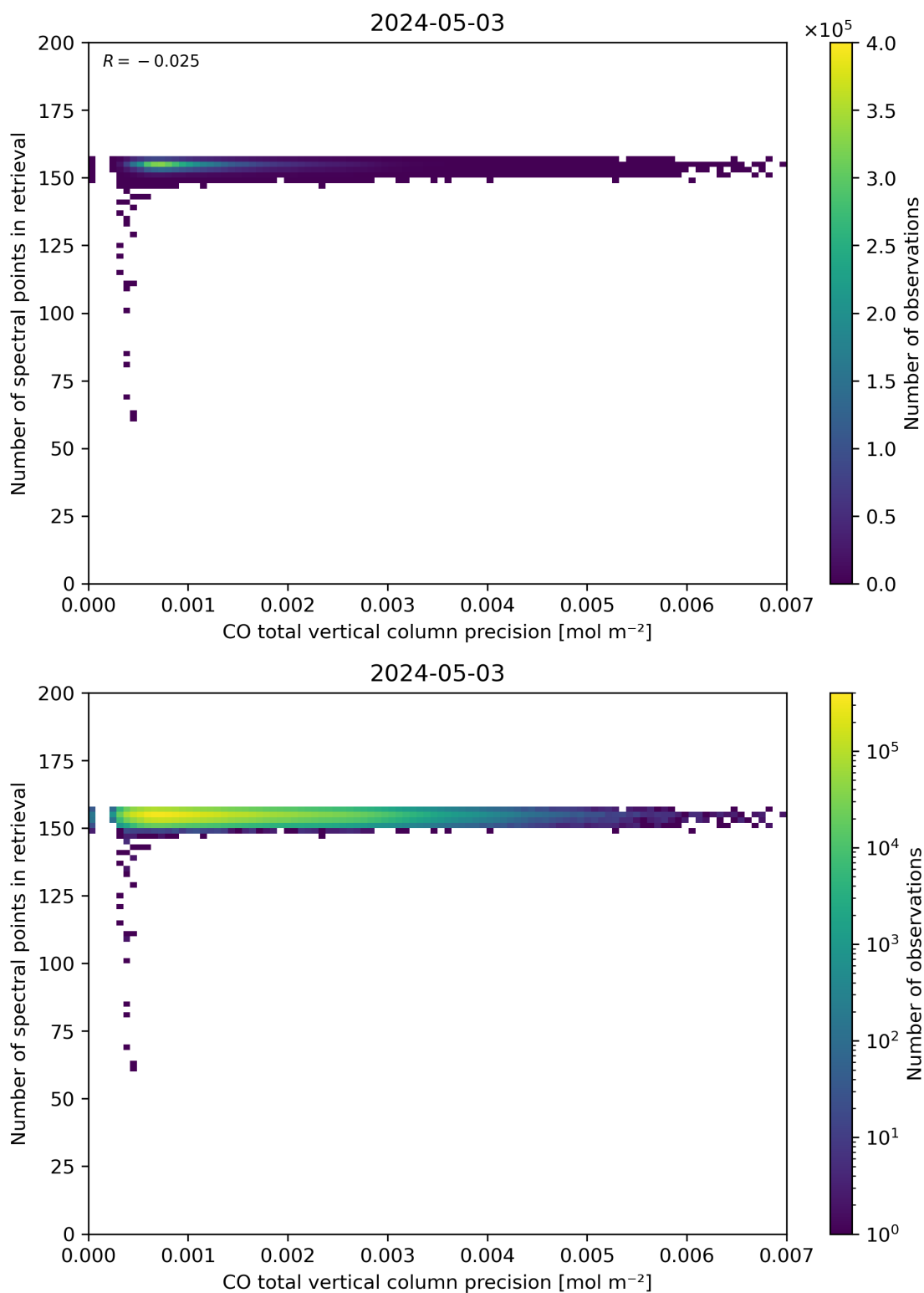
Figure 47: Scatter density plot of “CO total vertical column precision” against “Number of spectral points in retrieval” for 2024-05-02 to 2024-05-04.
