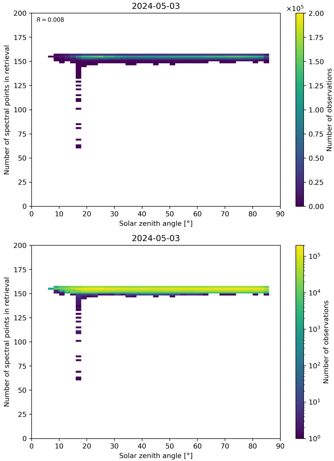
Figure 68: Scatter density plot of “Solar zenith angle” against “Number of spectral points in retrieval” for 2024-05-02 to 2024-05-04.
