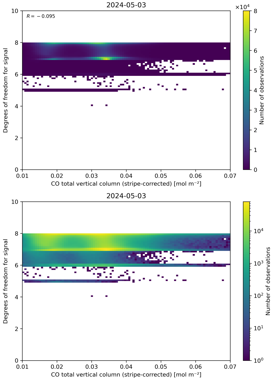
Figure 38: Scatter density plot of “CO total vertical column (stripe-corrected)” against “Degrees of freedom for signal” for 2024-05-02 to 2024-05-04.
