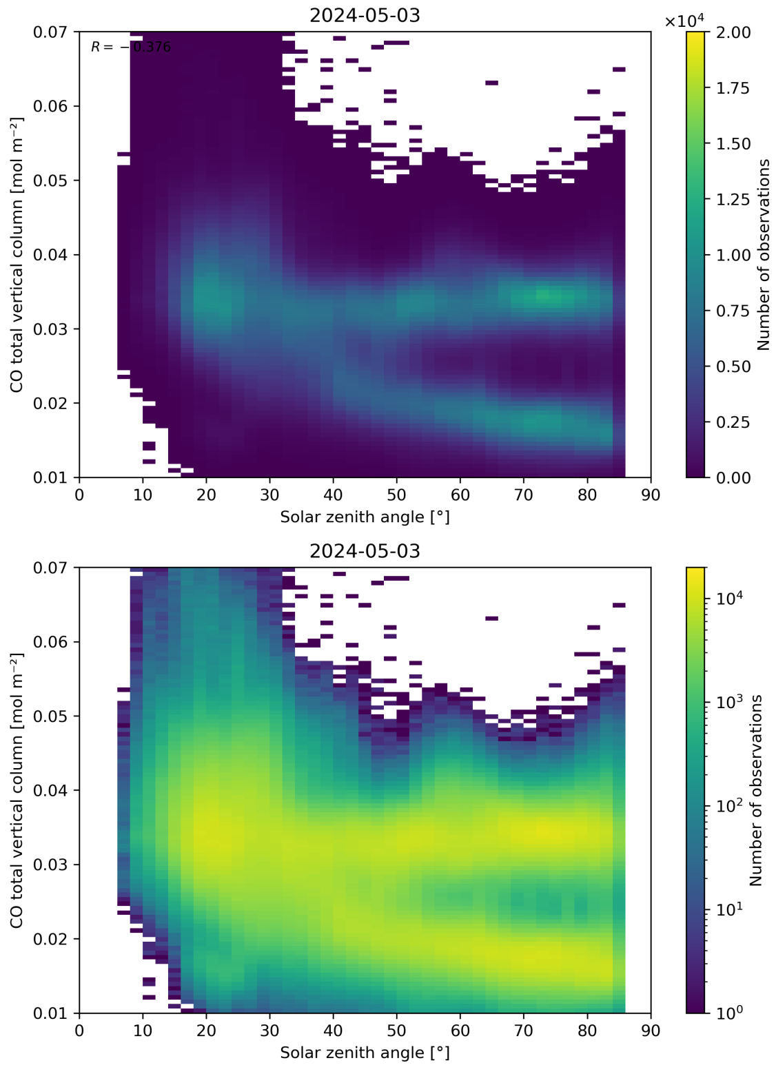
Figure 61: Scatter density plot of “Solar zenith angle” against “CO total vertical column” for 2024-05-02 to 2024-05-04.
