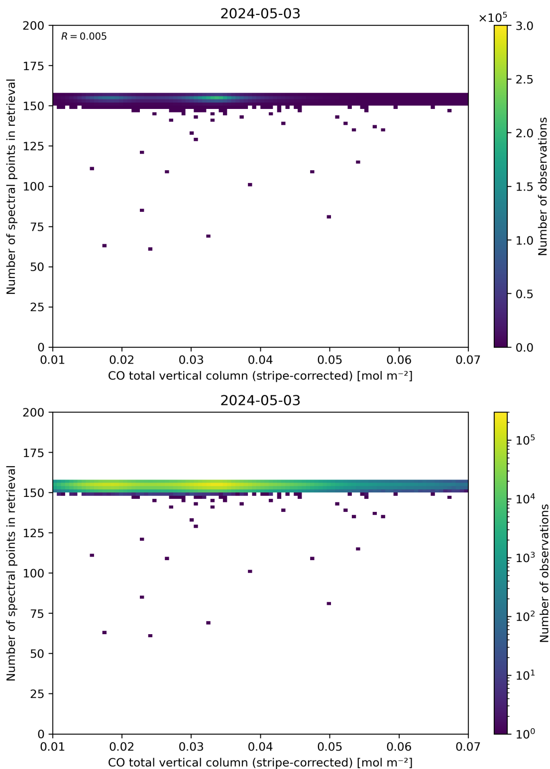
Figure 40: Scatter density plot of “CO total vertical column (stripe-corrected)” against “Number of spectral points in retrieval” for 2024-05-02 to 2024-05-04.
