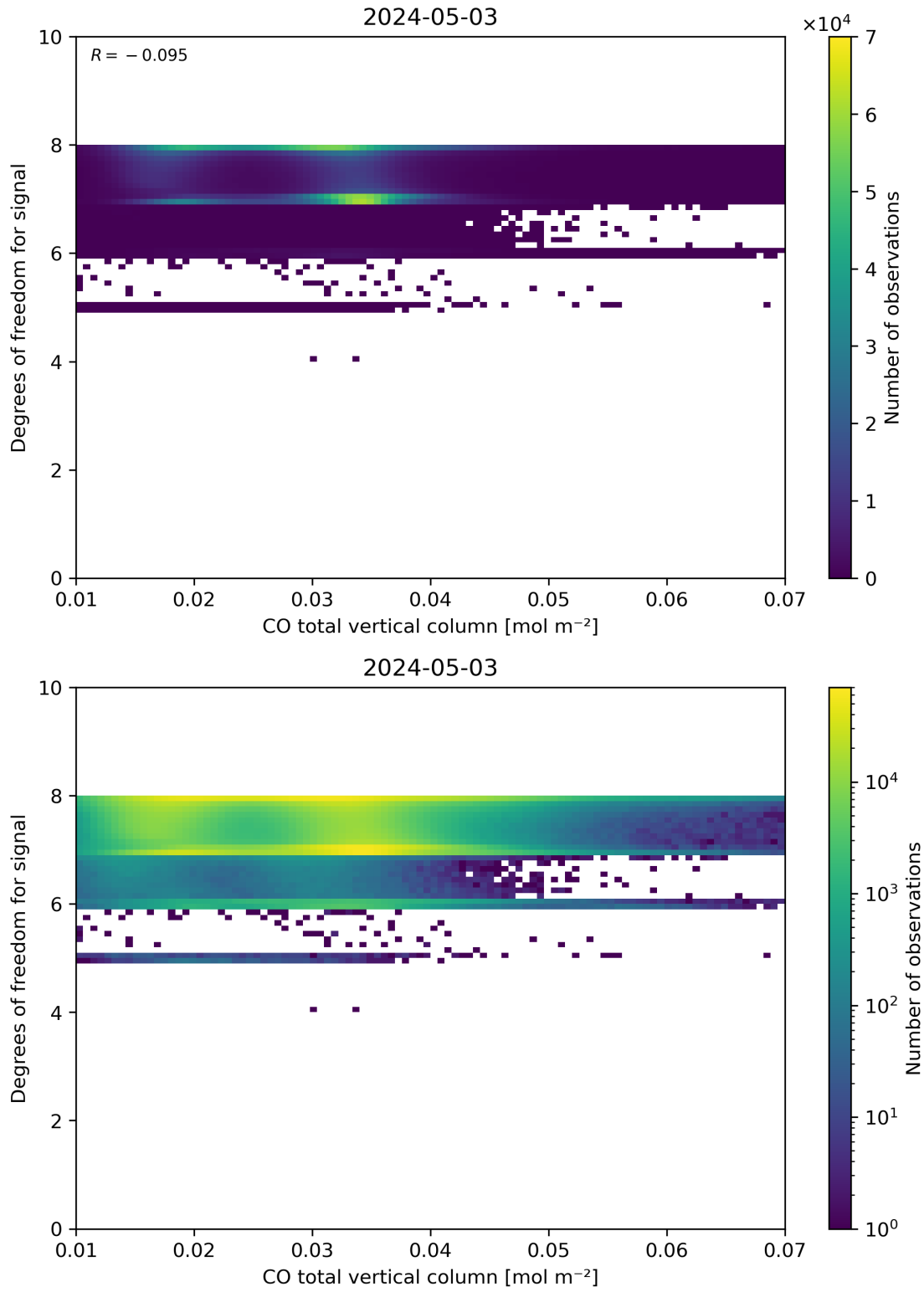
Figure 41: Scatter density plot of “CO total vertical column” against “Degrees of freedom for signal” for 2024-05-02 to 2024-05-04.
