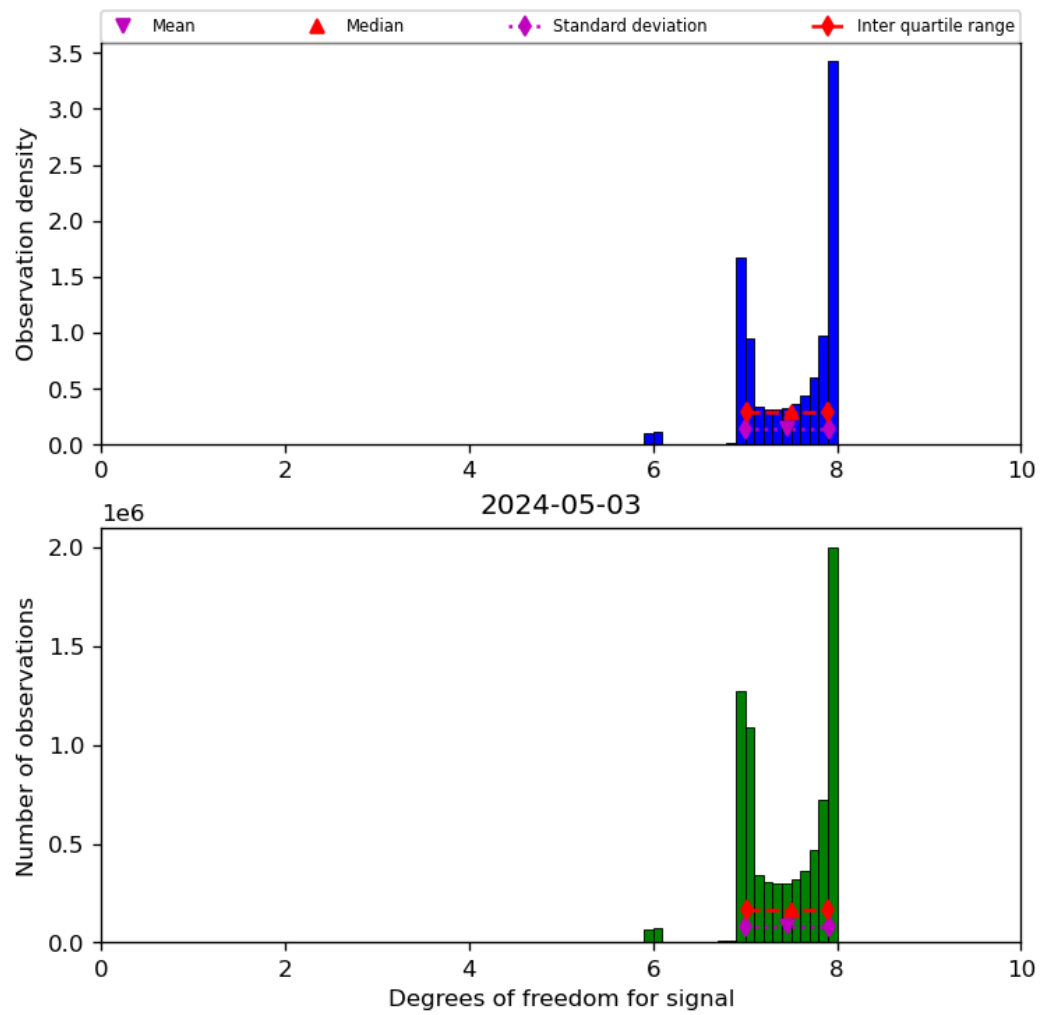
Figure 23: Histogram of “Degrees of freedom for signal” for 2024-05-02 to 2024-05-04
