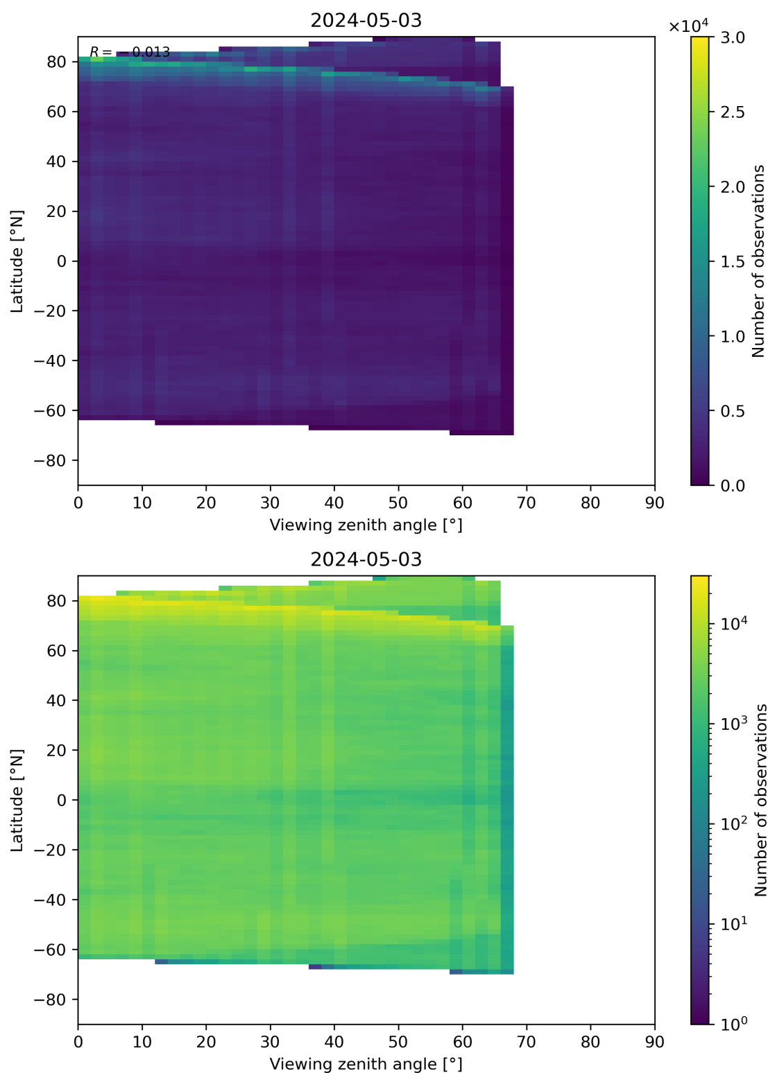
Figure 74: Scatter density plot of “Viewing zenith angle” against “Latitude” for 2024-05-02 to 2024-05-04.
