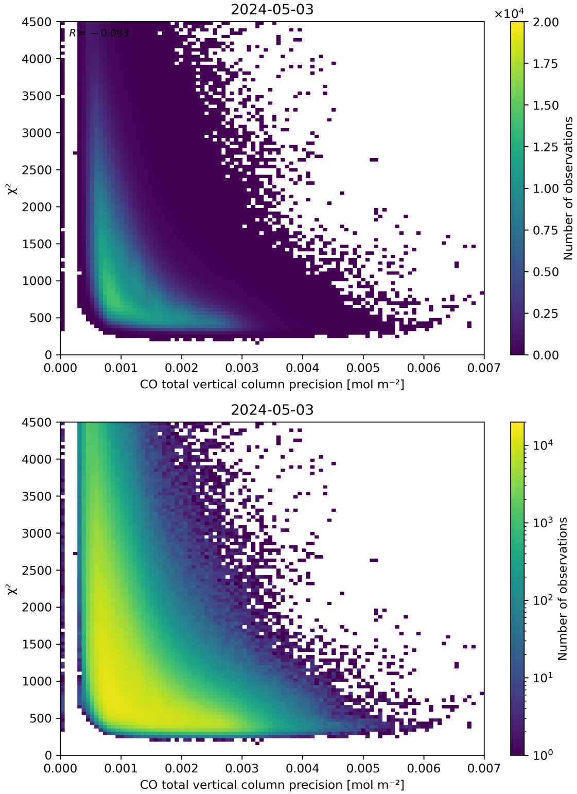
Figure 44: Scatter density plot of “CO total vertical column precision” against “ \chi^2 ” for 2024-05-02 to 2024-05-04.
