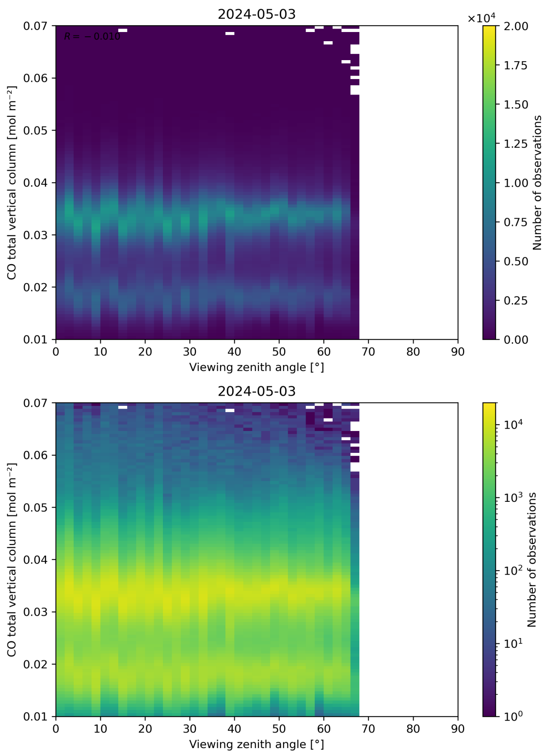
Figure 69: Scatter density plot of “Viewing zenith angle” against “CO total vertical column” for 2024-05-02 to 2024-05-04.
