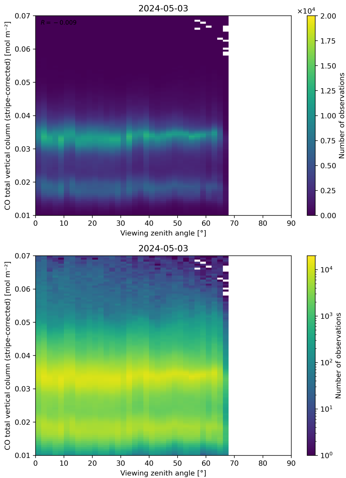
Figure 70: Scatter density plot of “Viewing zenith angle” against “CO total vertical column (stripe-corrected)” for 2024-05-02 to 2024-05-04.
