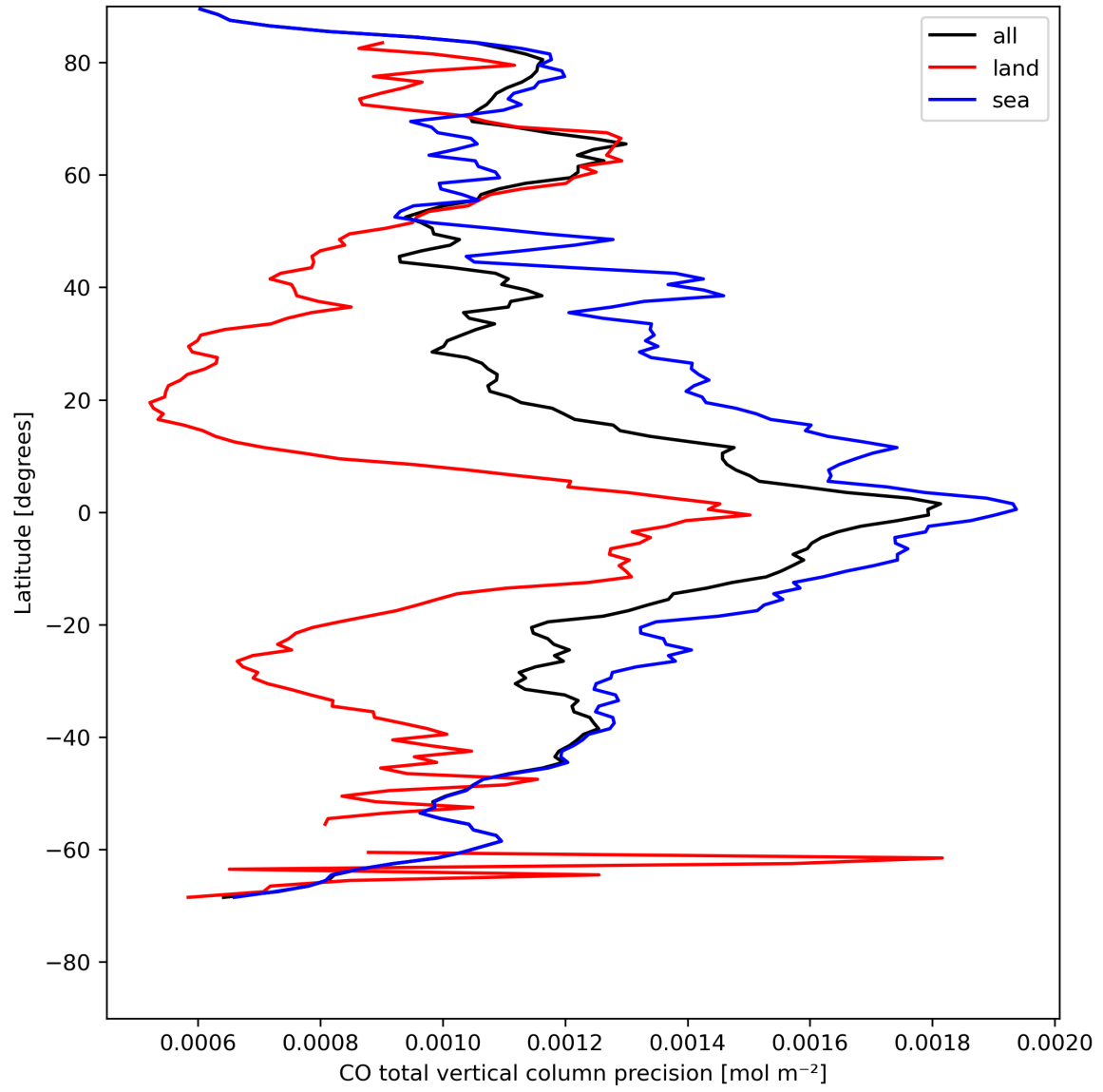
Figure 12: Zonal average of “CO total vertical column precision” for 2024-05-02 to 2024-05-04.
