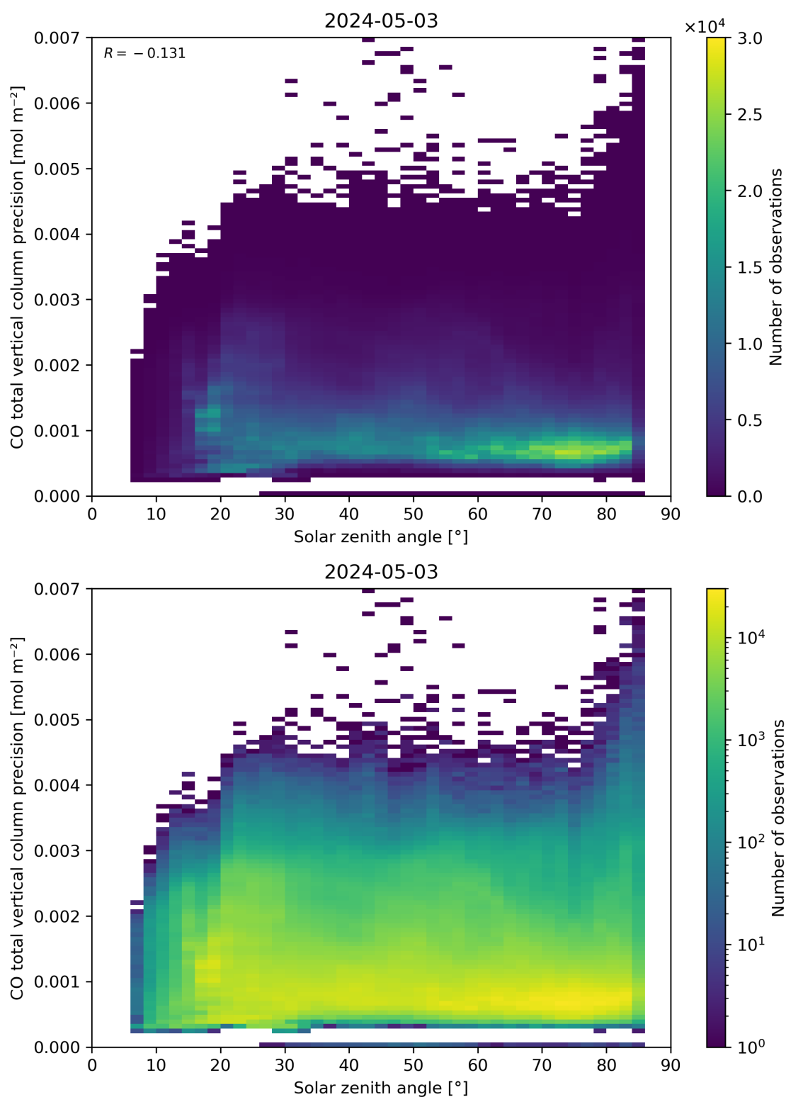
Figure 63: Scatter density plot of “Solar zenith angle” against “CO total vertical column precision” for 2024-05-02 to 2024-05-04.
