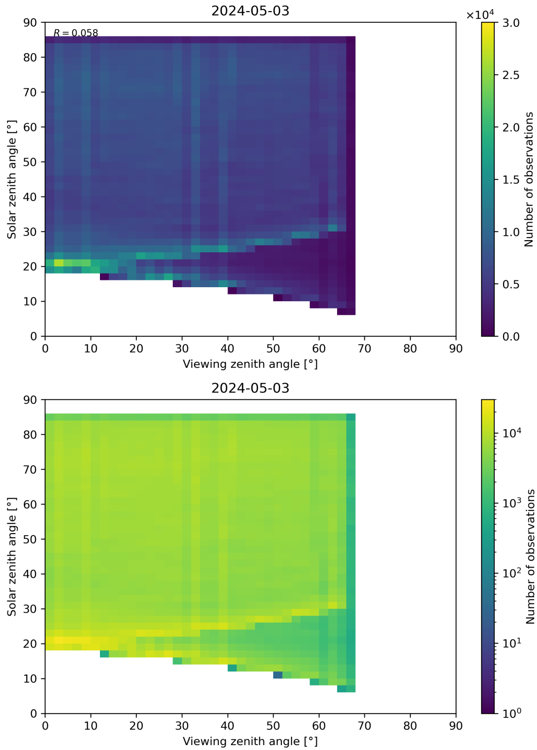
Figure 77: Scatter density plot of “Viewing zenith angle” against “Solar zenith angle” for 2024-05-02 to 2024-05-04.
