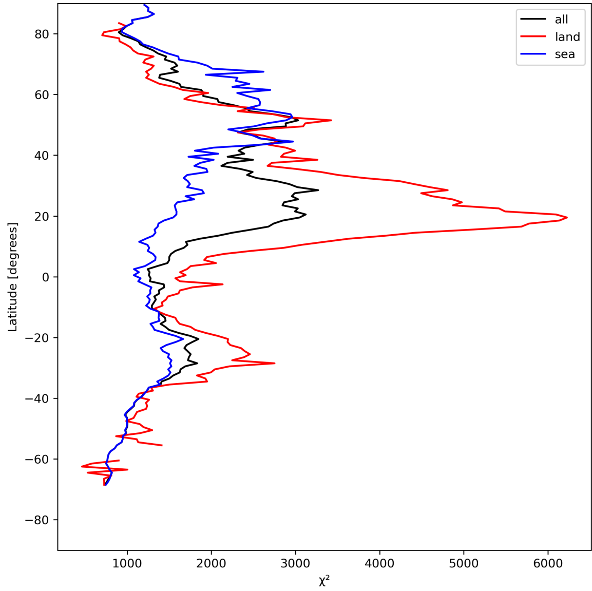
Figure 14: Zonal average of “ \chi^2 ” for 2024-05-02 to 2024-05-04.
