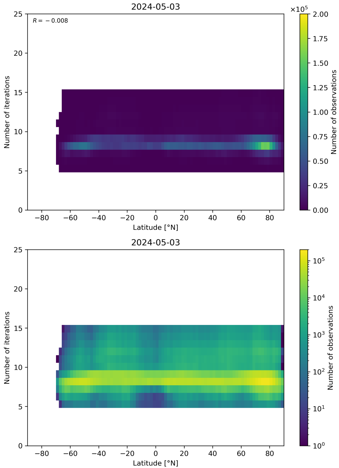
Figure 56: Scatter density plot of “Latitude” against “Number of iterations” for 2024-05-02 to 2024-05-04.
