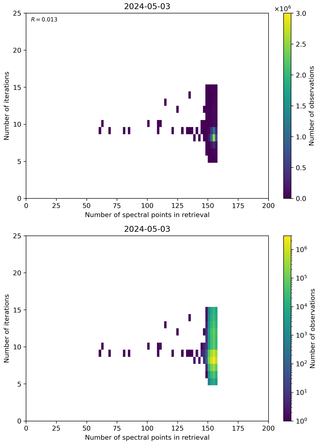
Figure 60: Scatter density plot of “Number of spectral points in retrieval” against “Number of iterations” for 2024-05-02 to 2024-05-04.
