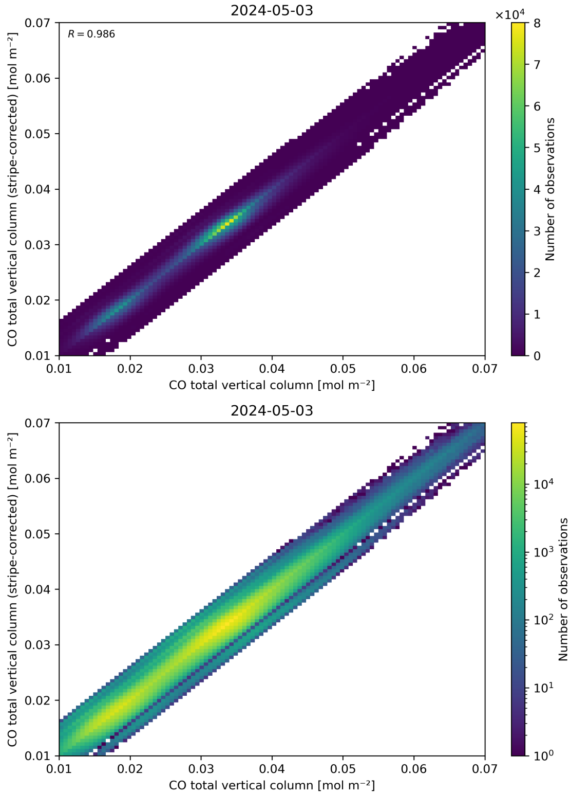
Figure 33: Scatter density plot of “CO total vertical column” against “CO total vertical column (stripe-corrected)” for 2024-05-02 to 2024-05-04.
