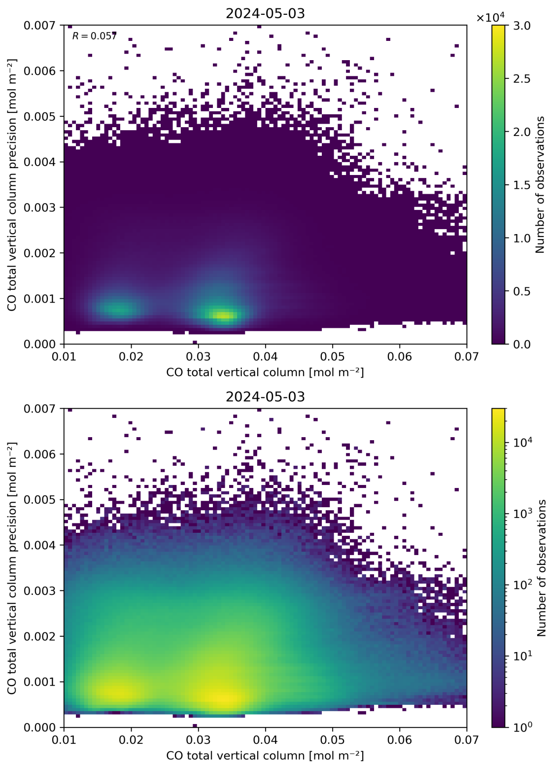
Figure 34: Scatter density plot of “CO total vertical column” against “CO total vertical column precision” for 2024-05-02 to 2024-05-04.
