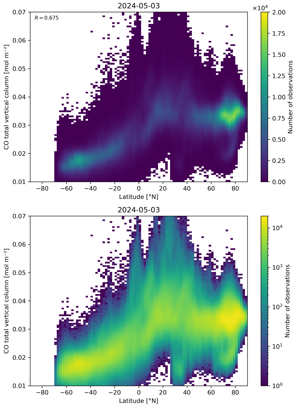
Figure 51: Scatter density plot of “Latitude” against “CO total vertical column” for 2024-05-02 to 2024-05-04.
