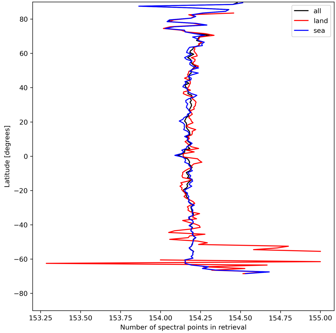
Figure 13: Zonal average of “Number of spectral points in retrieval” for 2024-05-02 to 2024-05-04.
