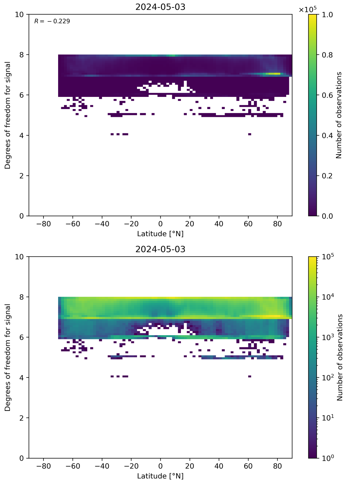
Figure 55: Scatter density plot of “Latitude” against “Degrees of freedom for signal” for 2024-05-02 to 2024-05-04.
