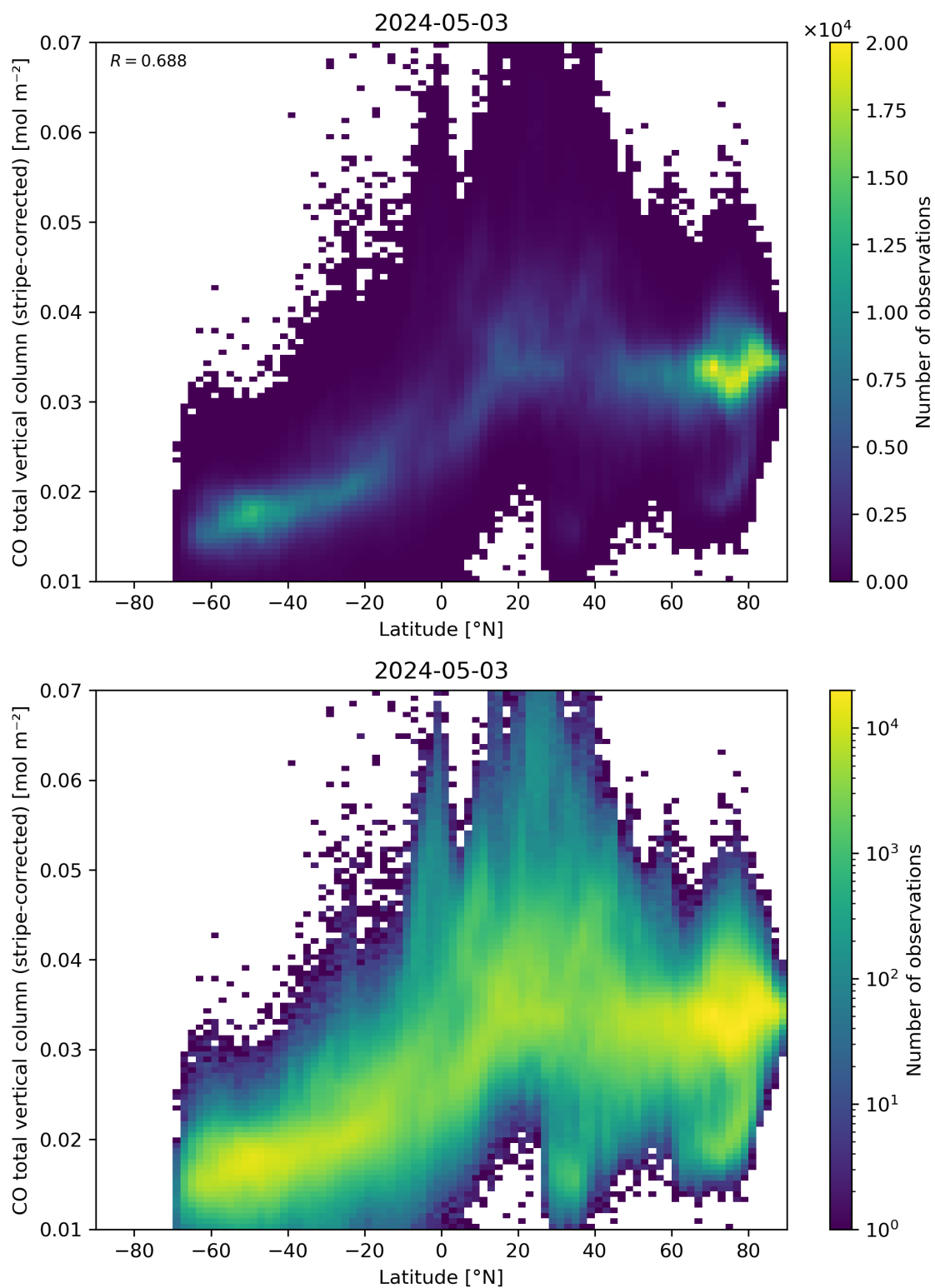
Figure 52: Scatter density plot of “Latitude” against “CO total vertical column (stripe-corrected)” for 2024-05-02 to 2024-05-04.
