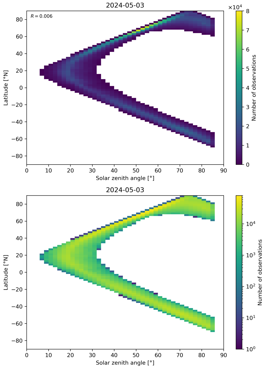
Figure 66: Scatter density plot of “Solar zenith angle” against “Latitude” for 2024-05-02 to 2024-05-04.
