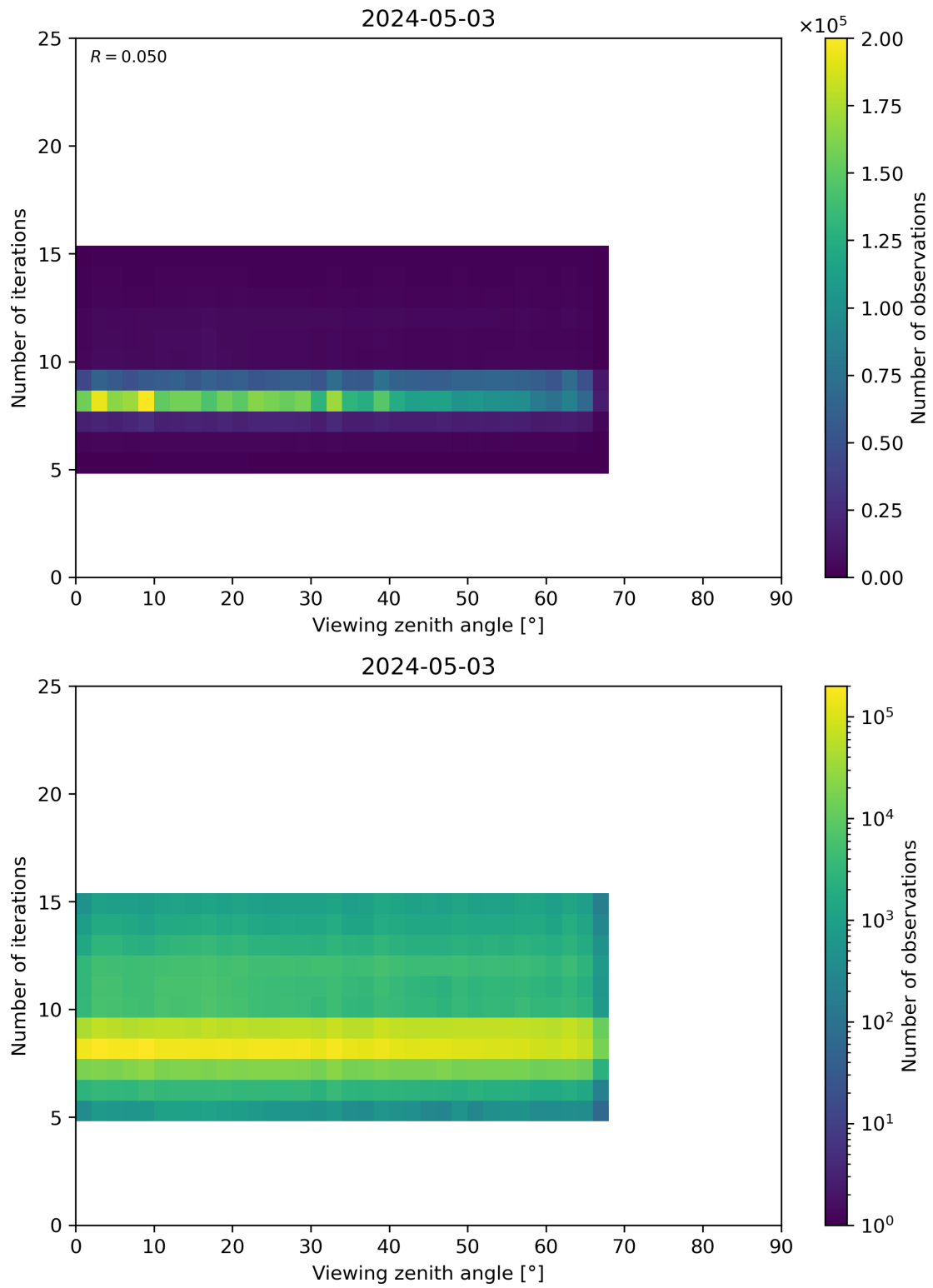
Figure 75: Scatter density plot of “Viewing zenith angle” against “Number of iterations” for 2024-05-02 to 2024-05-04.
