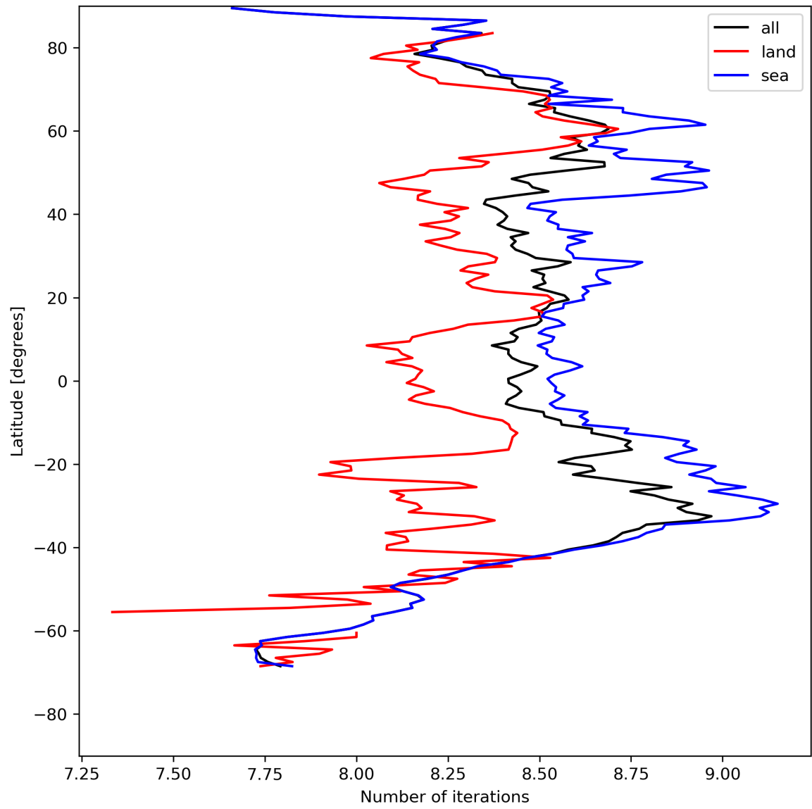
Figure 16: Zonal average of “Number of iterations” for 2024-05-02 to 2024-05-04.
