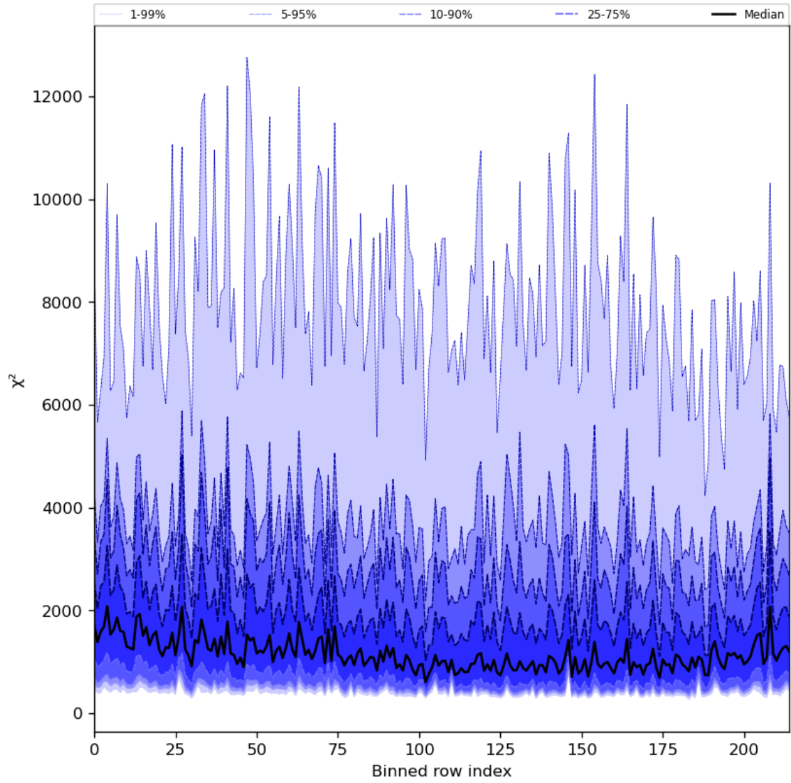
Figure 30: Along track statistics of “ \chi^2 ” for 2024-05-02 to 2024-05-04
