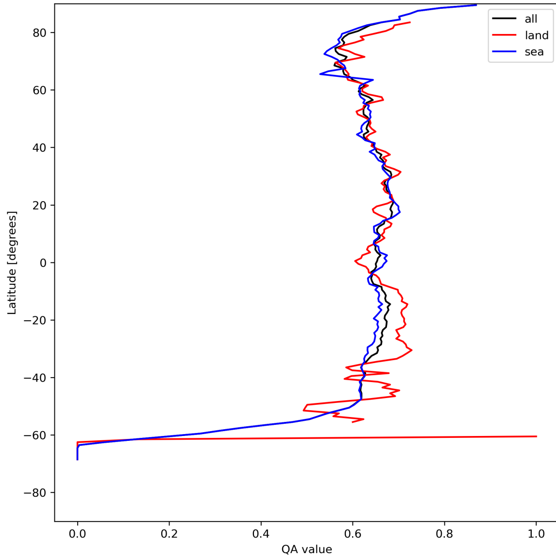
Figure 9: Zonal average of “QA value” for 2024-05-02 to 2024-05-04.
