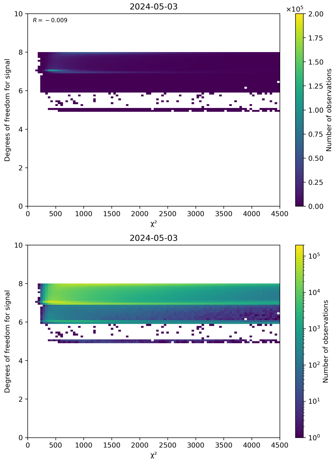
Figure 48: Scatter density plot of “ \chi^2 ” against “Degrees of freedom for signal” for 2024-05-02 to 2024-05-04.
