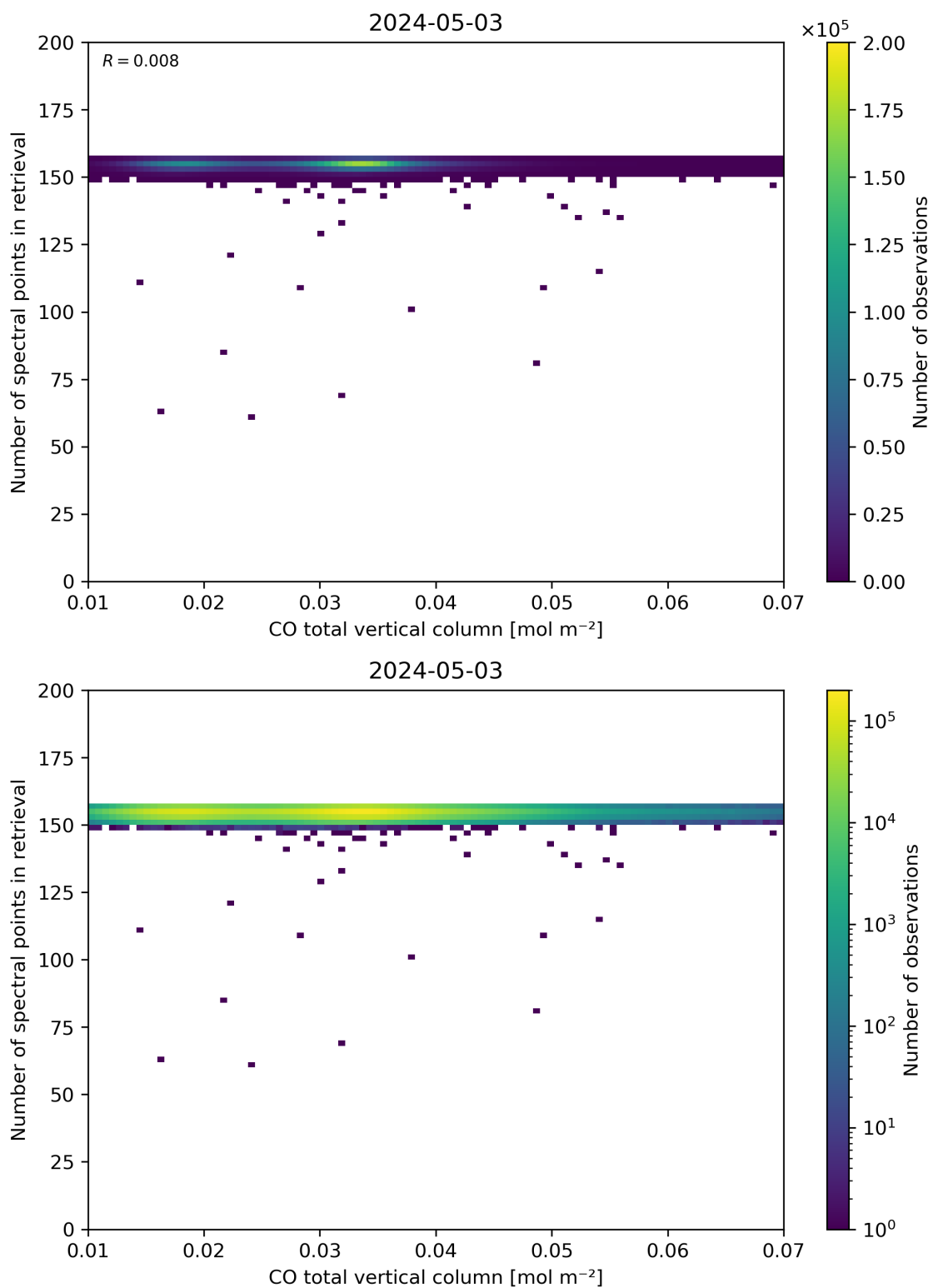
Figure 43: Scatter density plot of “CO total vertical column” against “Number of spectral points in retrieval” for 2024-05-02 to 2024-05-04.
