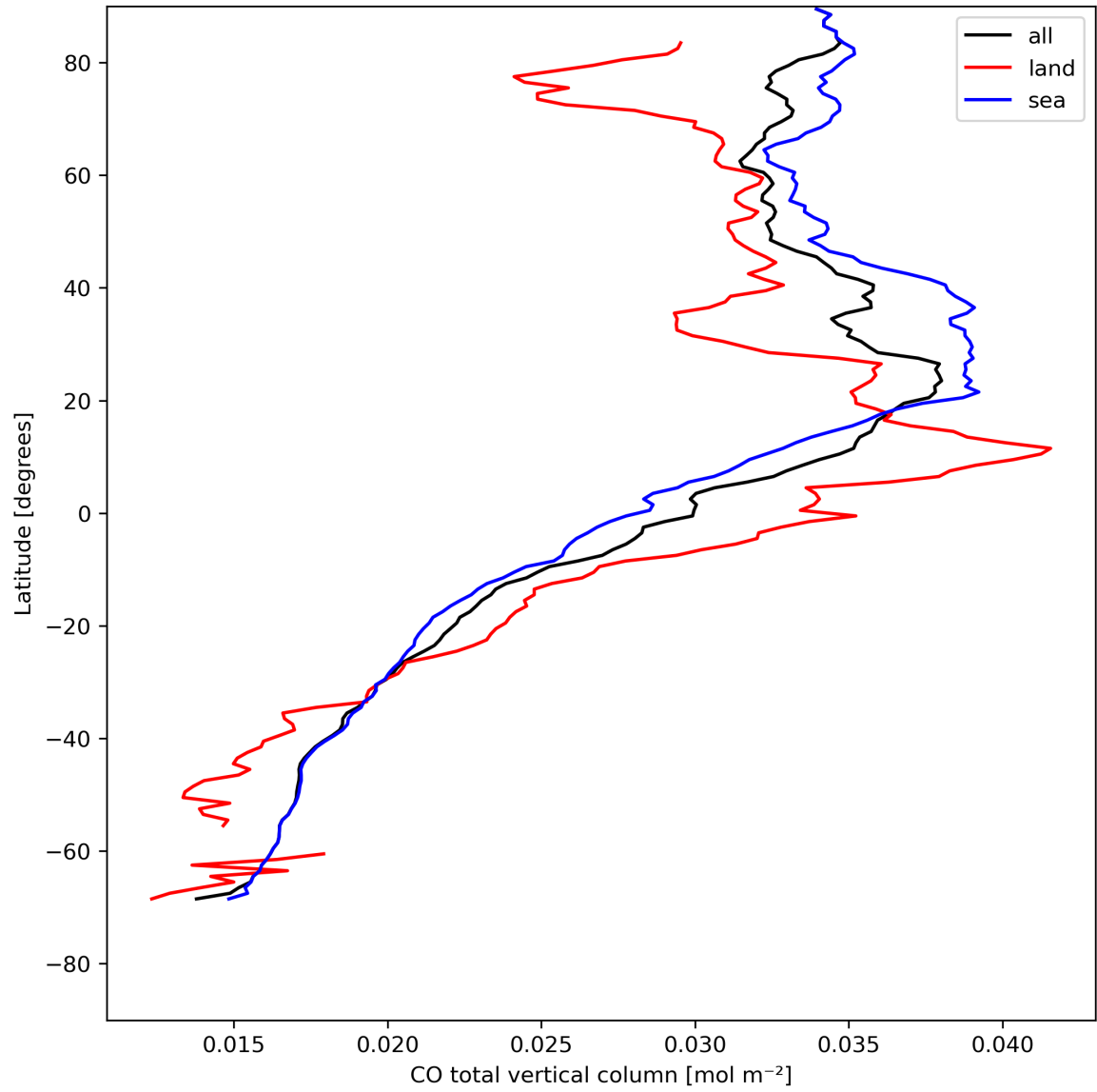
Figure 10: Zonal average of “CO total vertical column” for 2024-05-02 to 2024-05-04.
