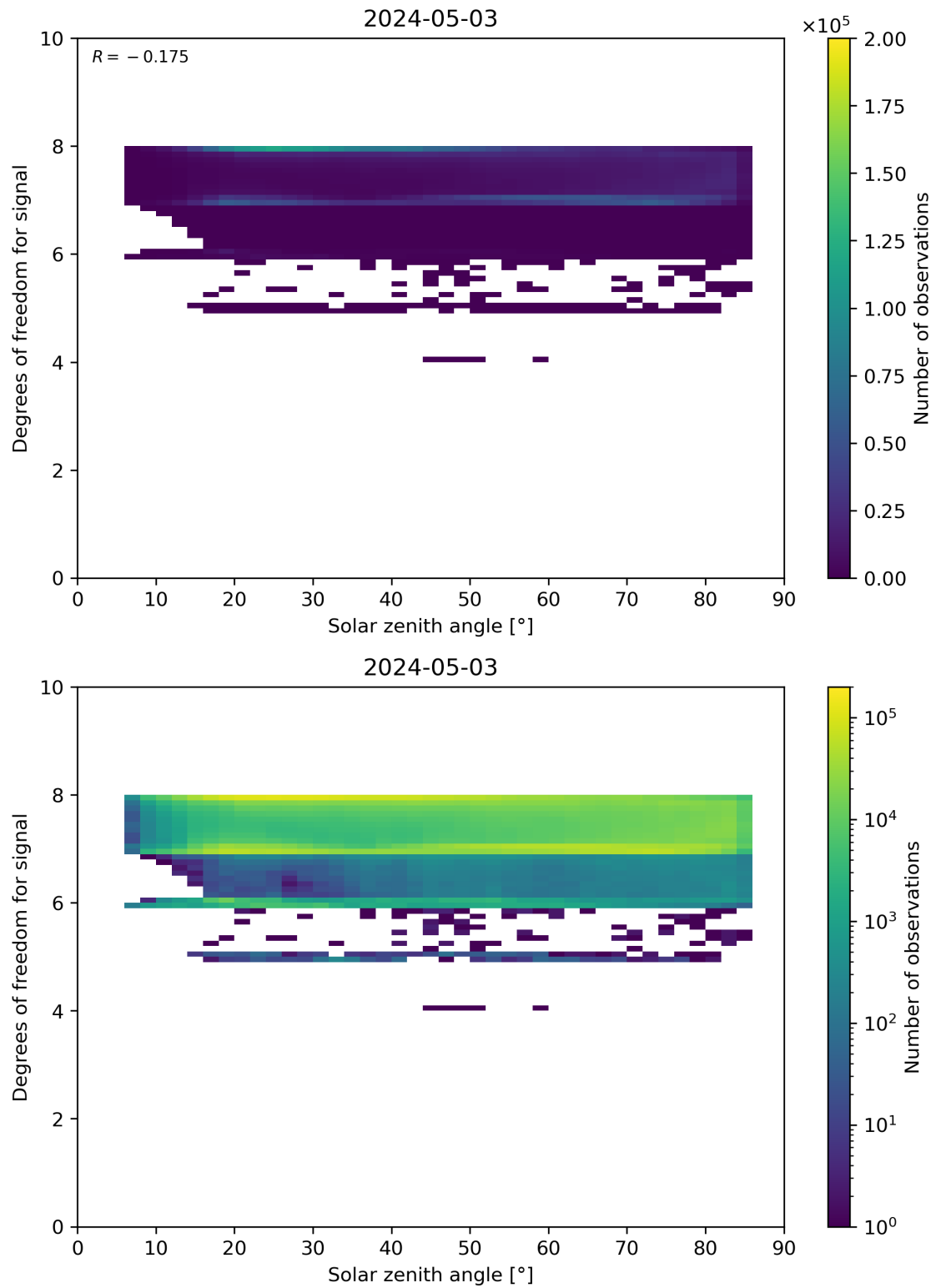
Figure 65: Scatter density plot of “Solar zenith angle” against “Degrees of freedom for signal” for 2024-05-02 to 2024-05-04.
