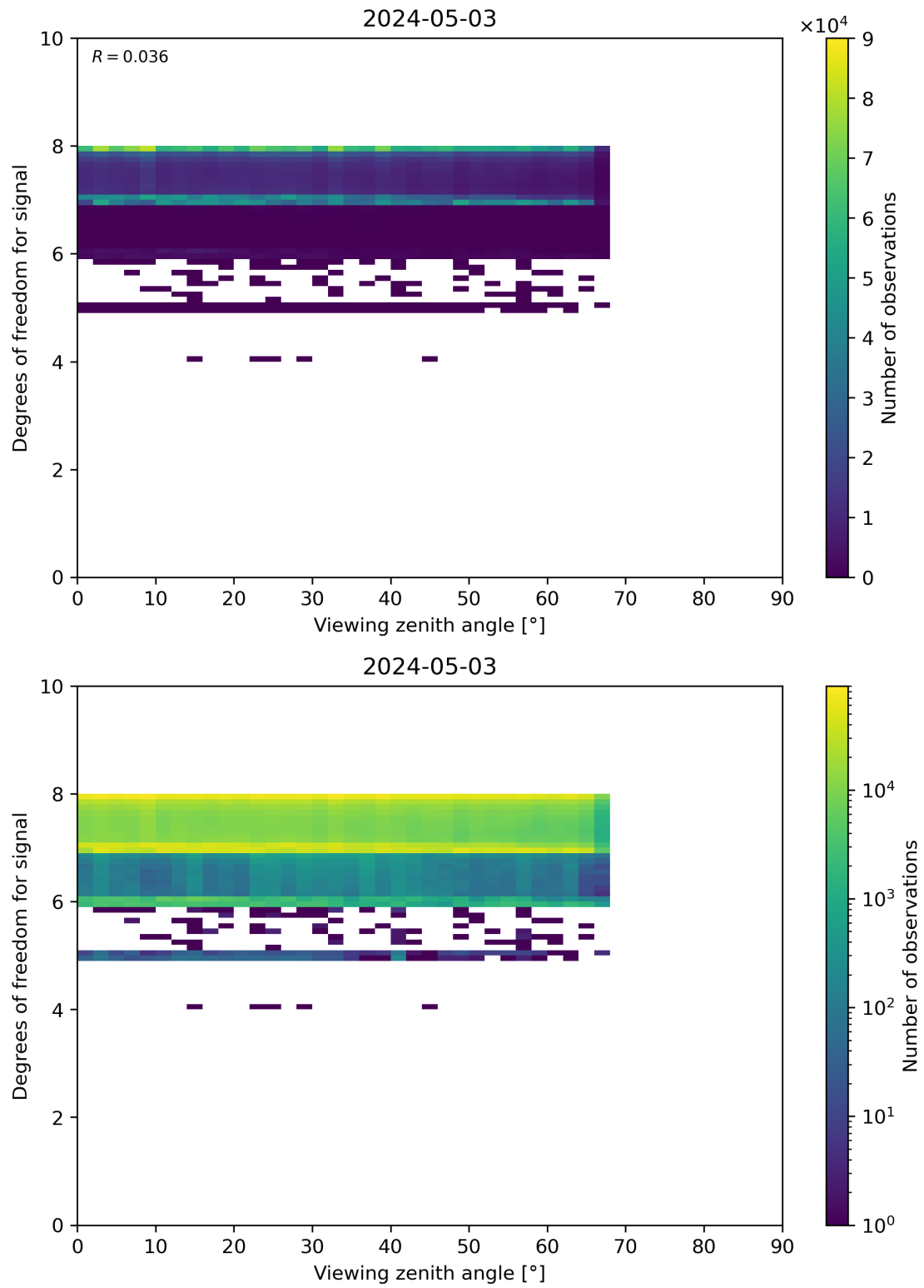
Figure 73: Scatter density plot of “Viewing zenith angle” against “Degrees of freedom for signal” for 2024-05-02 to 2024-05-04.
