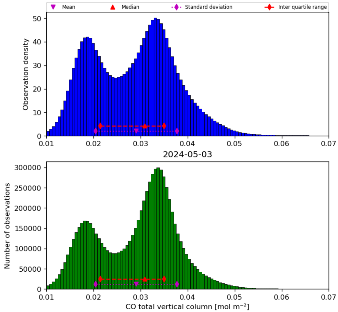
Figure 18: Histogram of “CO total vertical column” for 2024-05-02 to 2024-05-04
