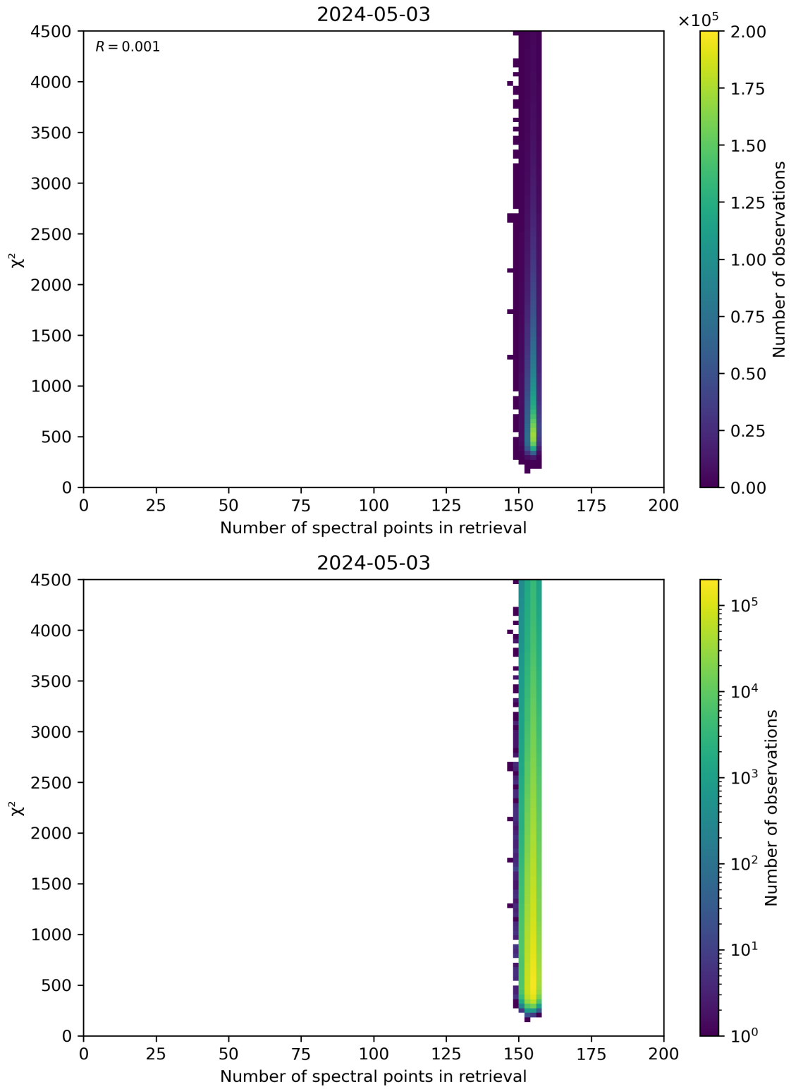
Figure 58: Scatter density plot of “Number of spectral points in retrieval” against “ \chi^2 ” for 2024-05-02 to 2024-05-04.
