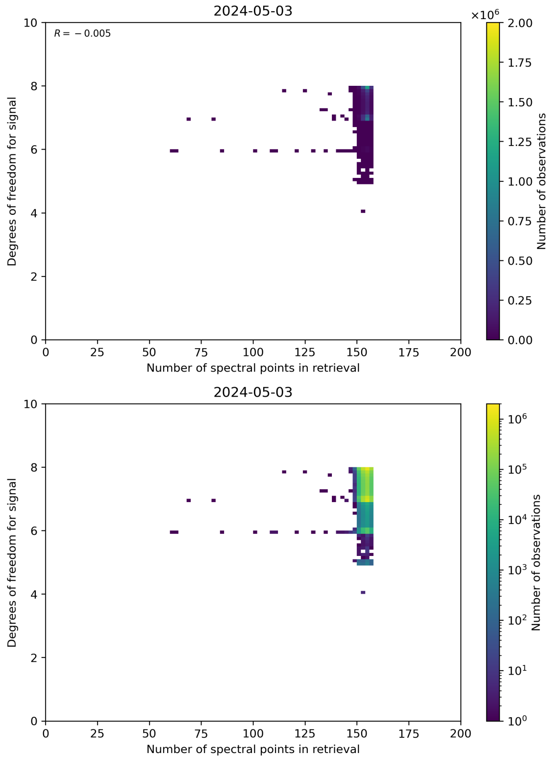
Figure 59: Scatter density plot of “Number of spectral points in retrieval” against “Degrees of freedom for signal” for 2024-05-02 to 2024-05-04.
