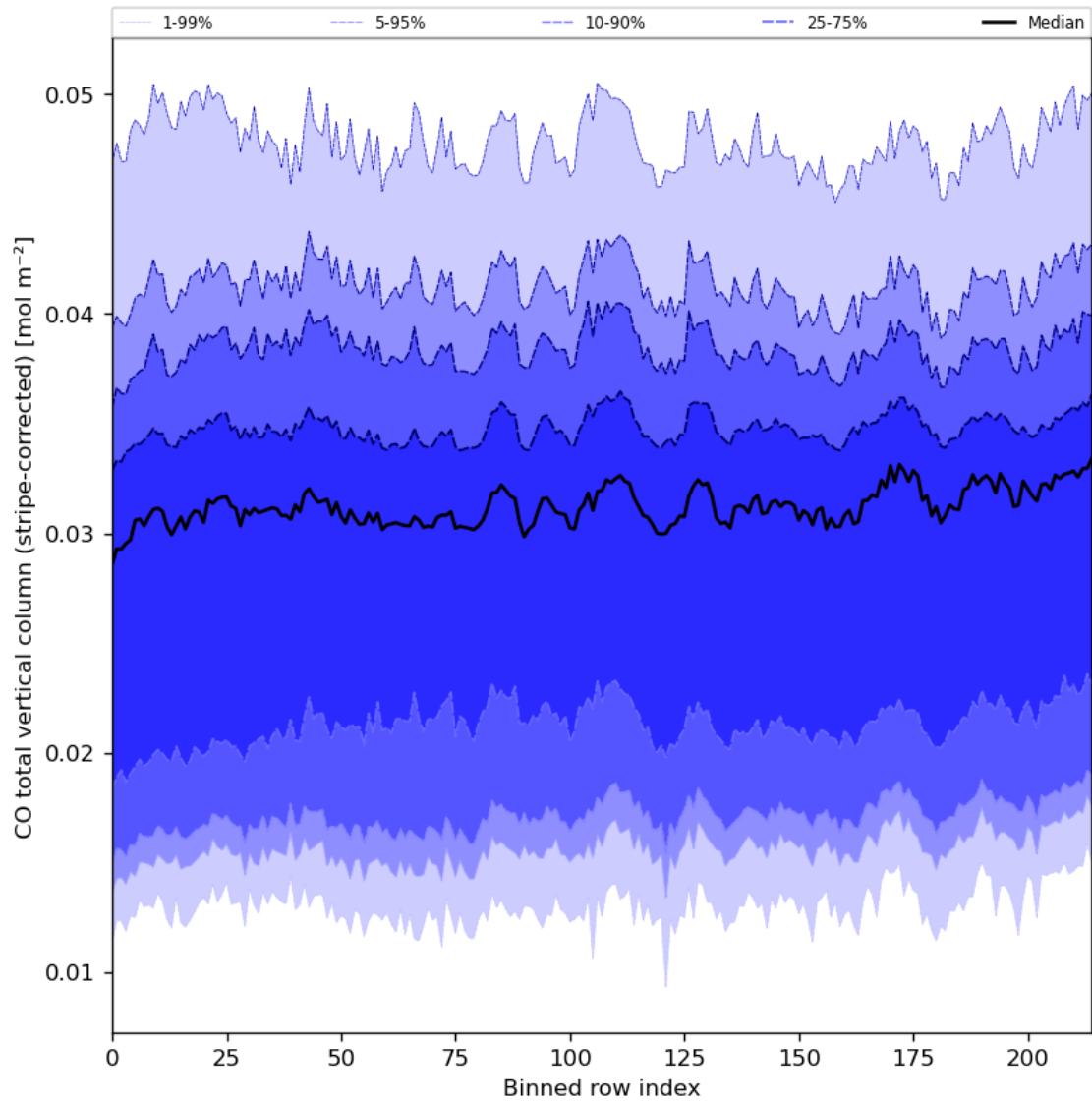
Figure 27: Along track statistics of “CO total vertical column (stripe-corrected)” for 2024-05-02 to 2024-05-04
