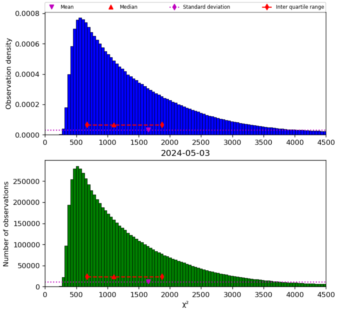
Figure 22: Histogram of “ \chi^2 ” for 2024-05-02 to 2024-05-04
