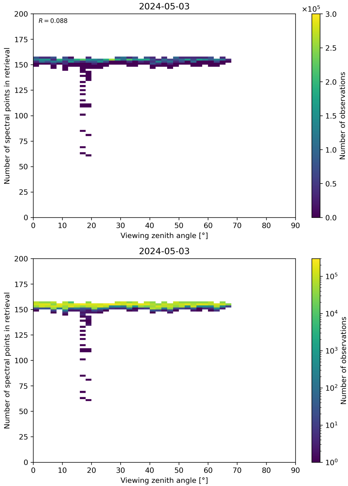
Figure 76: Scatter density plot of “Viewing zenith angle” against “Number of spectral points in retrieval” for 2024-05-02 to 2024-05-04.
