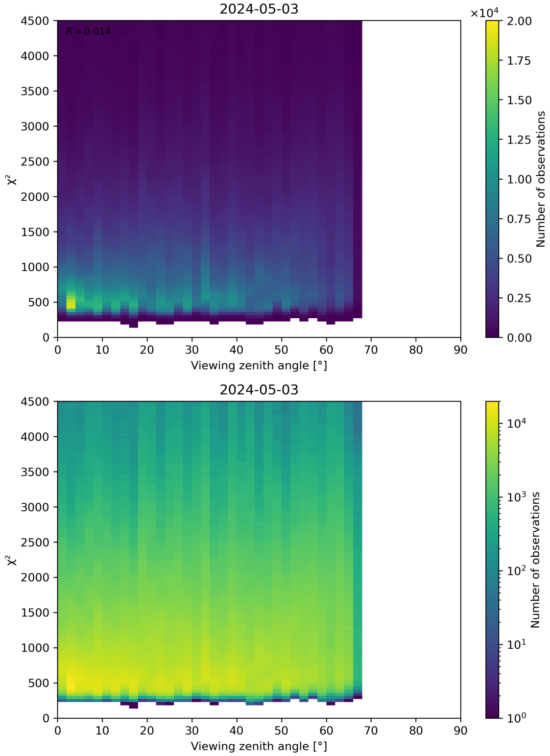
Figure 72: Scatter density plot of “Viewing zenith angle” against “ \chi^2 ” for 2024-05-02 to 2024-05-04.
