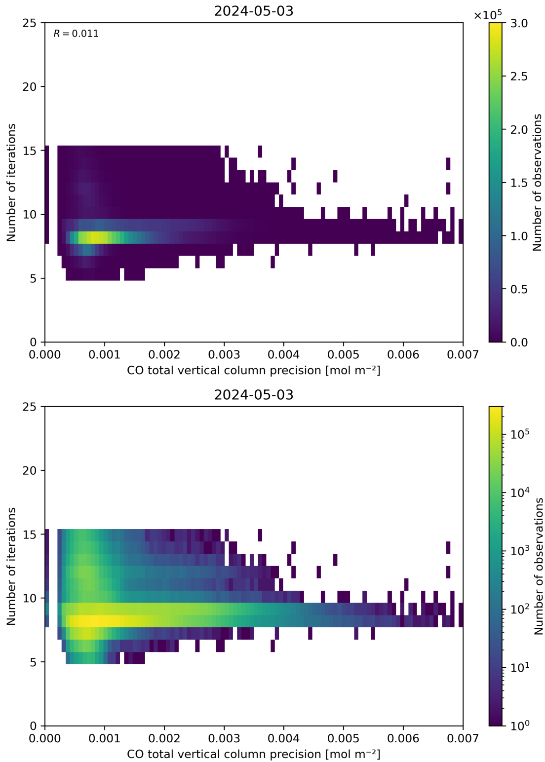
Figure 46: Scatter density plot of “CO total vertical column precision” against “Number of iterations” for 2024-05-02 to 2024-05-04.
