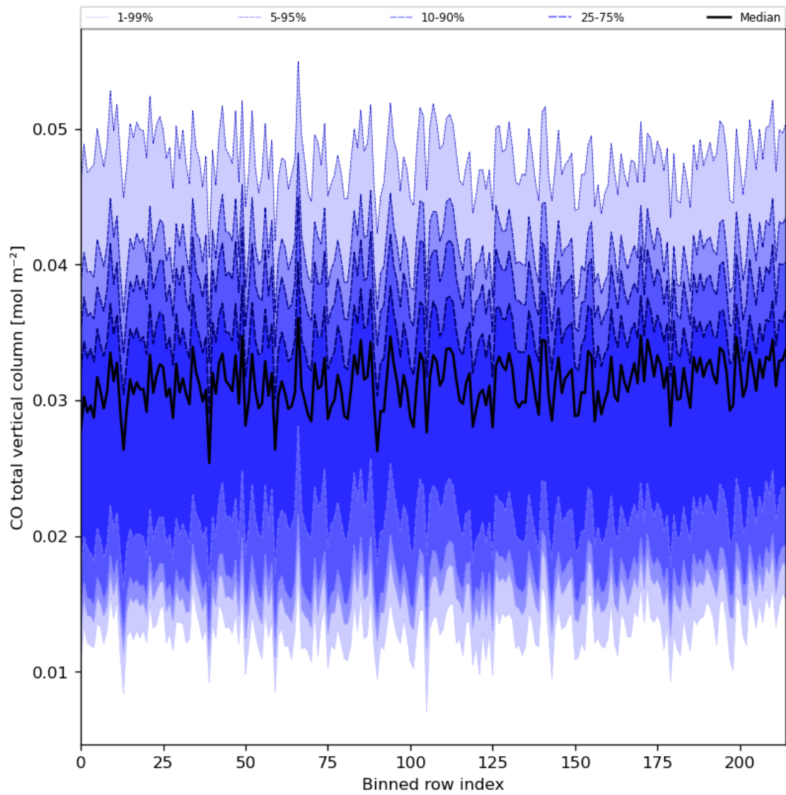
Figure 26: Along track statistics of "CO total vertical column" for 2024-05-02 to 2024-05-04
