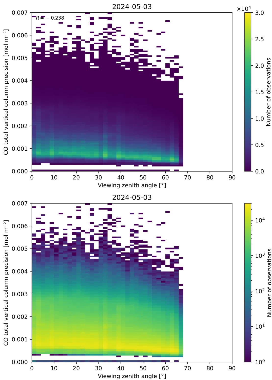
Figure 71: Scatter density plot of “Viewing zenith angle” against “CO total vertical column precision” for 2024-05-02 to 2024-05-04.
