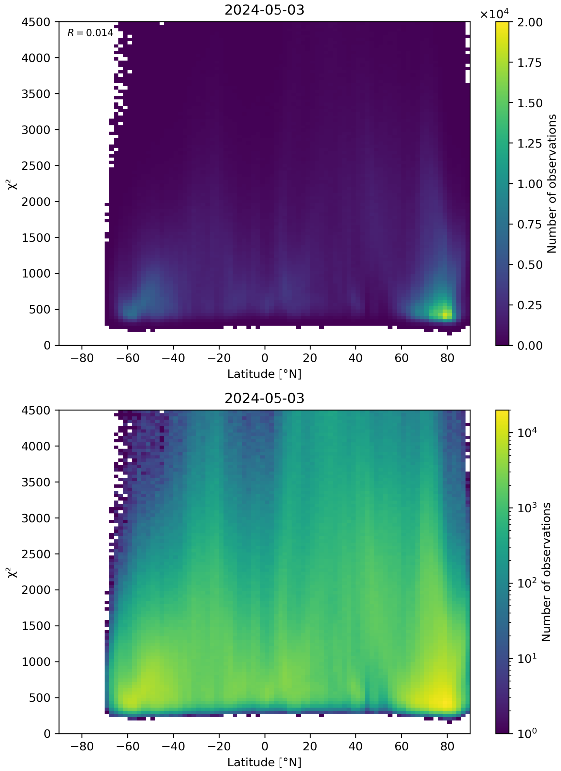
Figure 54: Scatter density plot of “Latitude” against “ \chi^2 ” for 2024-05-02 to 2024-05-04.
