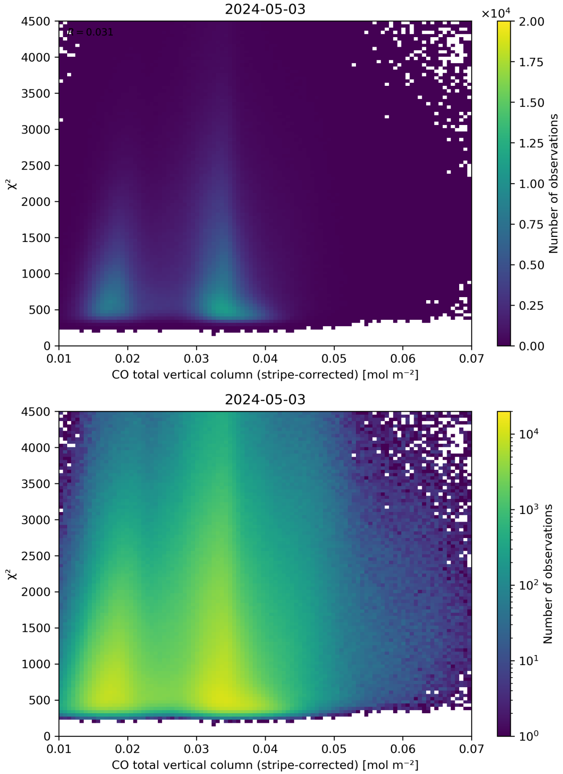
Figure 37: Scatter density plot of “CO total vertical column (stripe-corrected)” against “ \chi^2 ” for 2024-05-02 to 2024-05-04.
