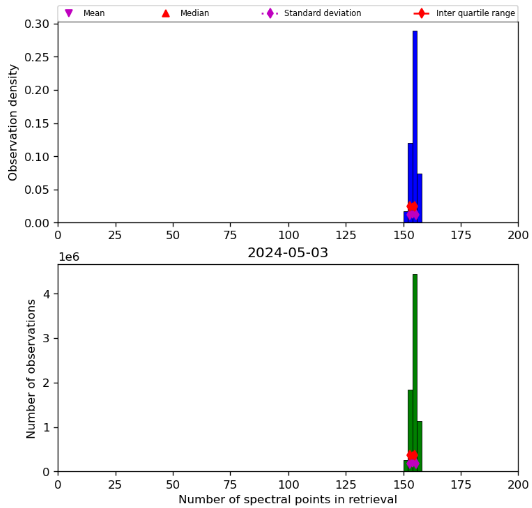
Figure 21: Histogram of “Number of spectral points in retrieval” for 2024-05-02 to 2024-05-04
