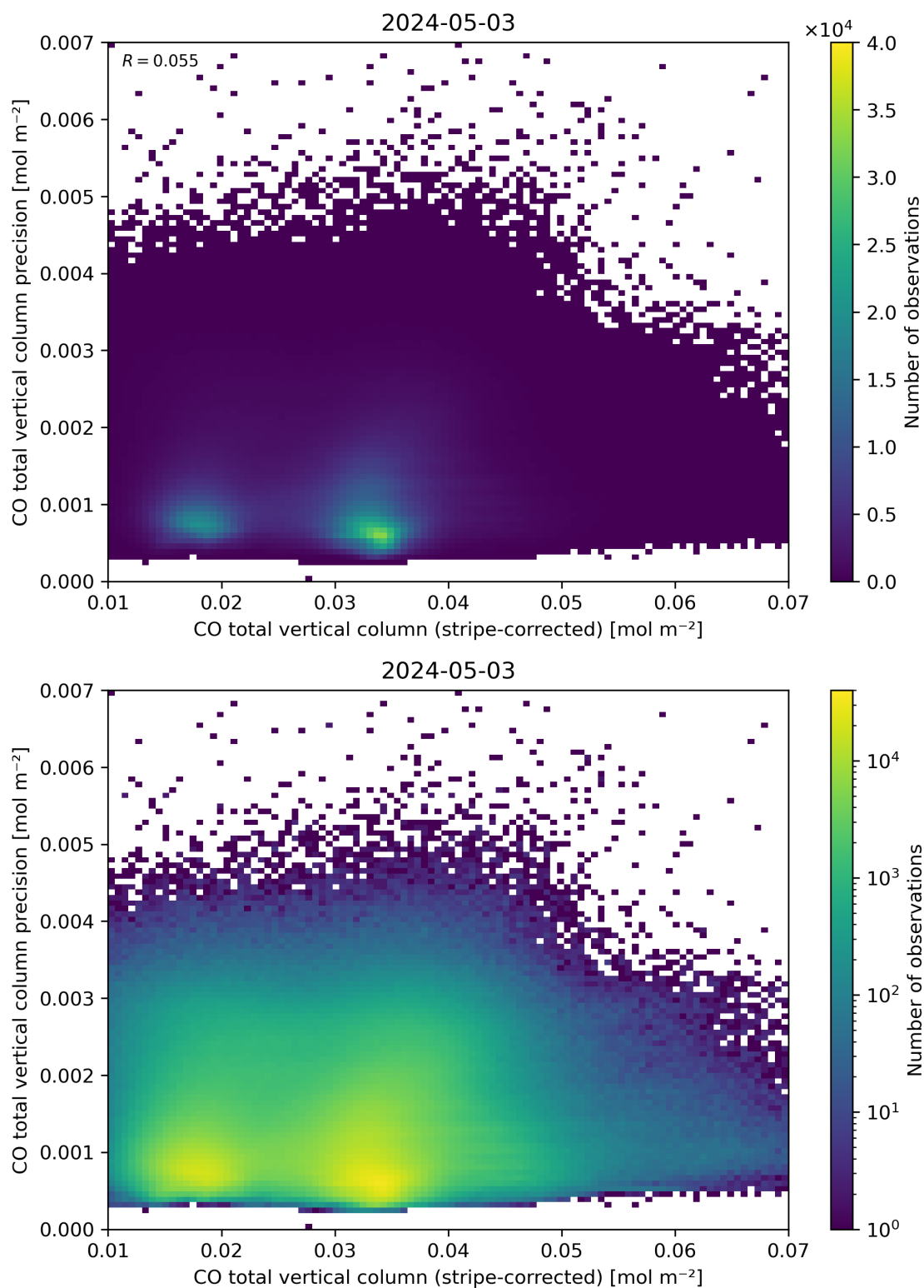
Figure 36: Scatter density plot of “CO total vertical column (stripe-corrected)” against “CO total vertical column precision” for 2024-05-02 to 2024-05-04.
