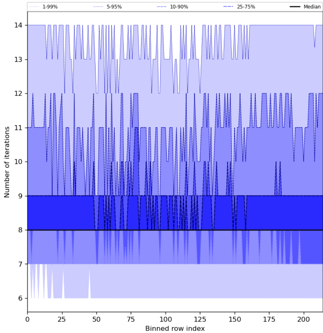
Figure 32: Along track statistics of “Number of iterations” for 2024-05-02 to 2024-05-04
