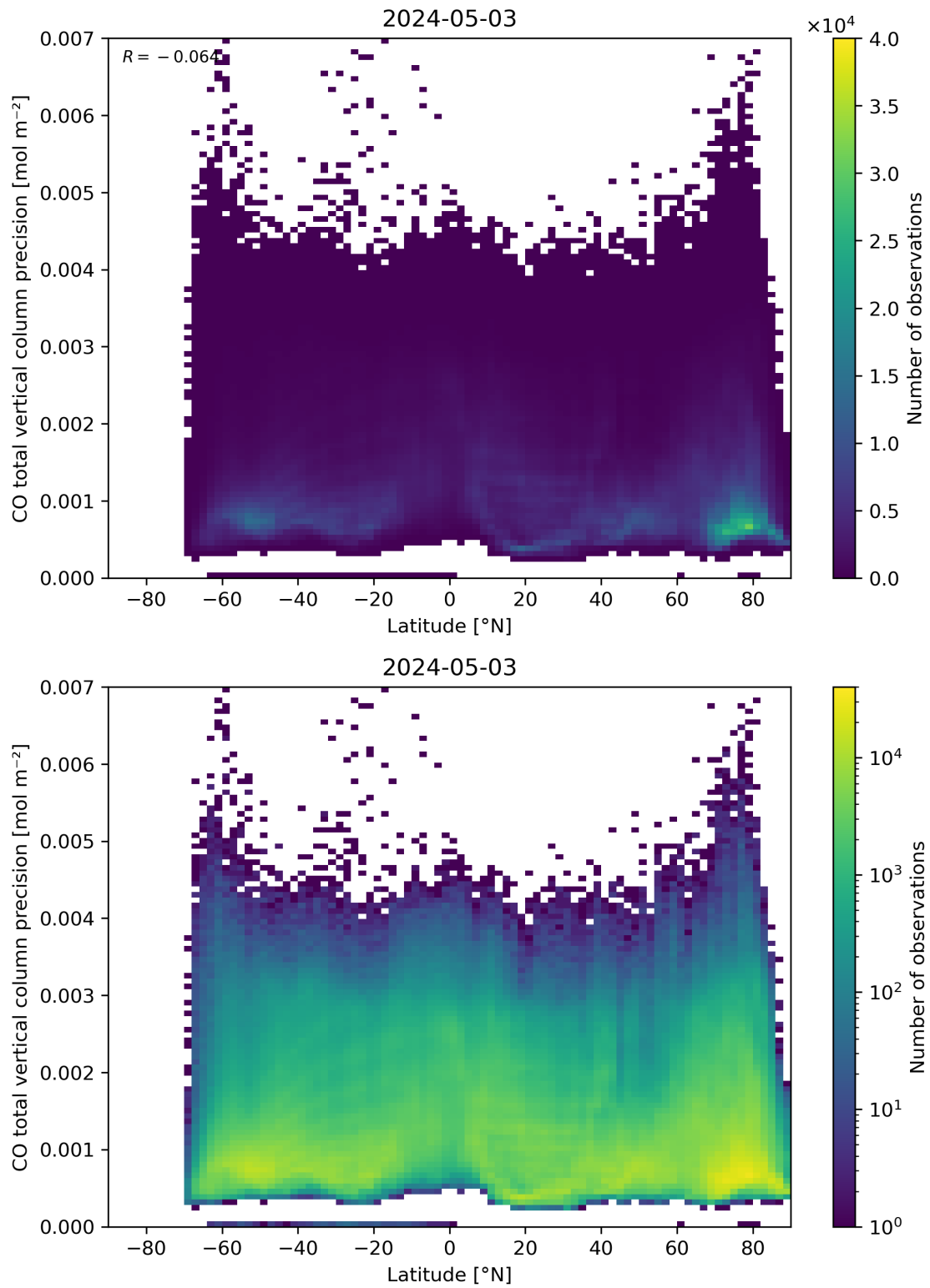
Figure 53: Scatter density plot of “Latitude” against “CO total vertical column precision” for 2024-05-02 to 2024-05-04.
