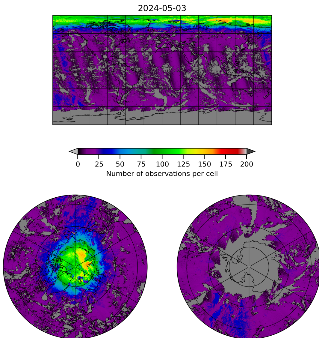
Figure 8: Map of the number of observations for 2024-05-02 to 2024-05-04
