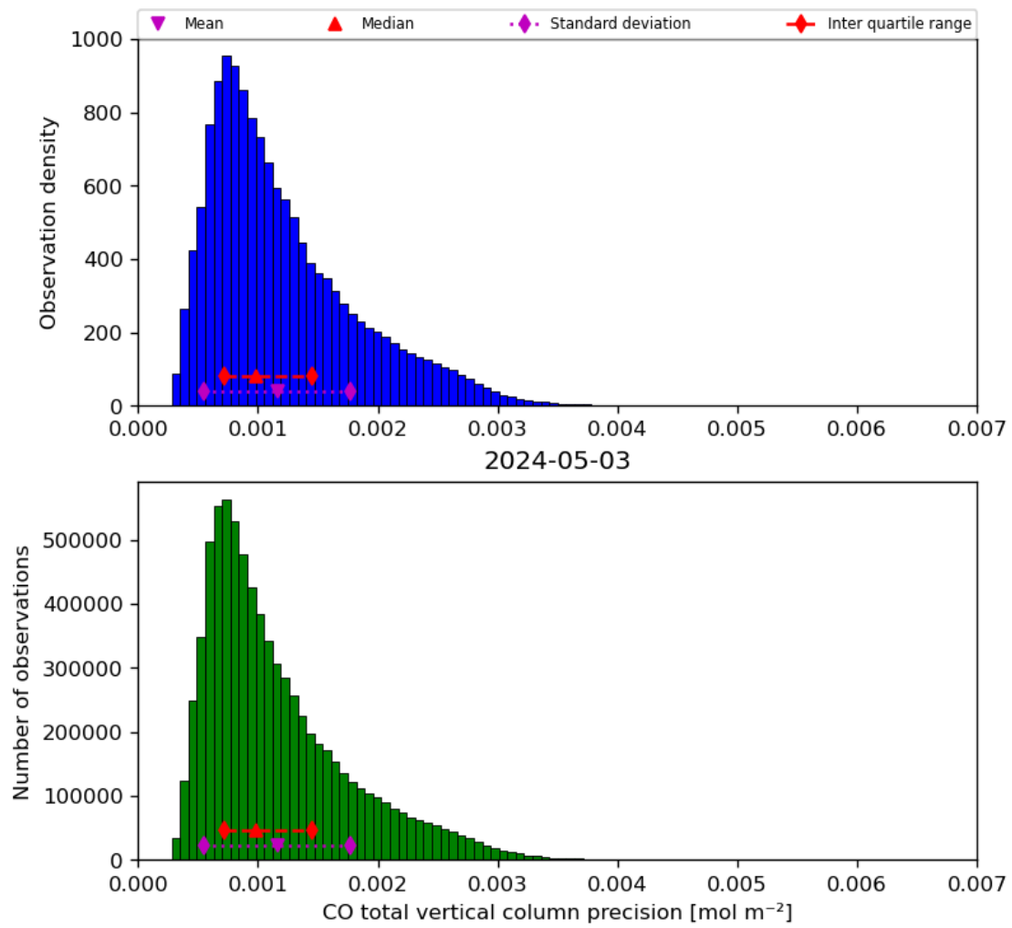
Figure 20: Histogram of “CO total vertical column precision” for 2024-05-02 to 2024-05-04
