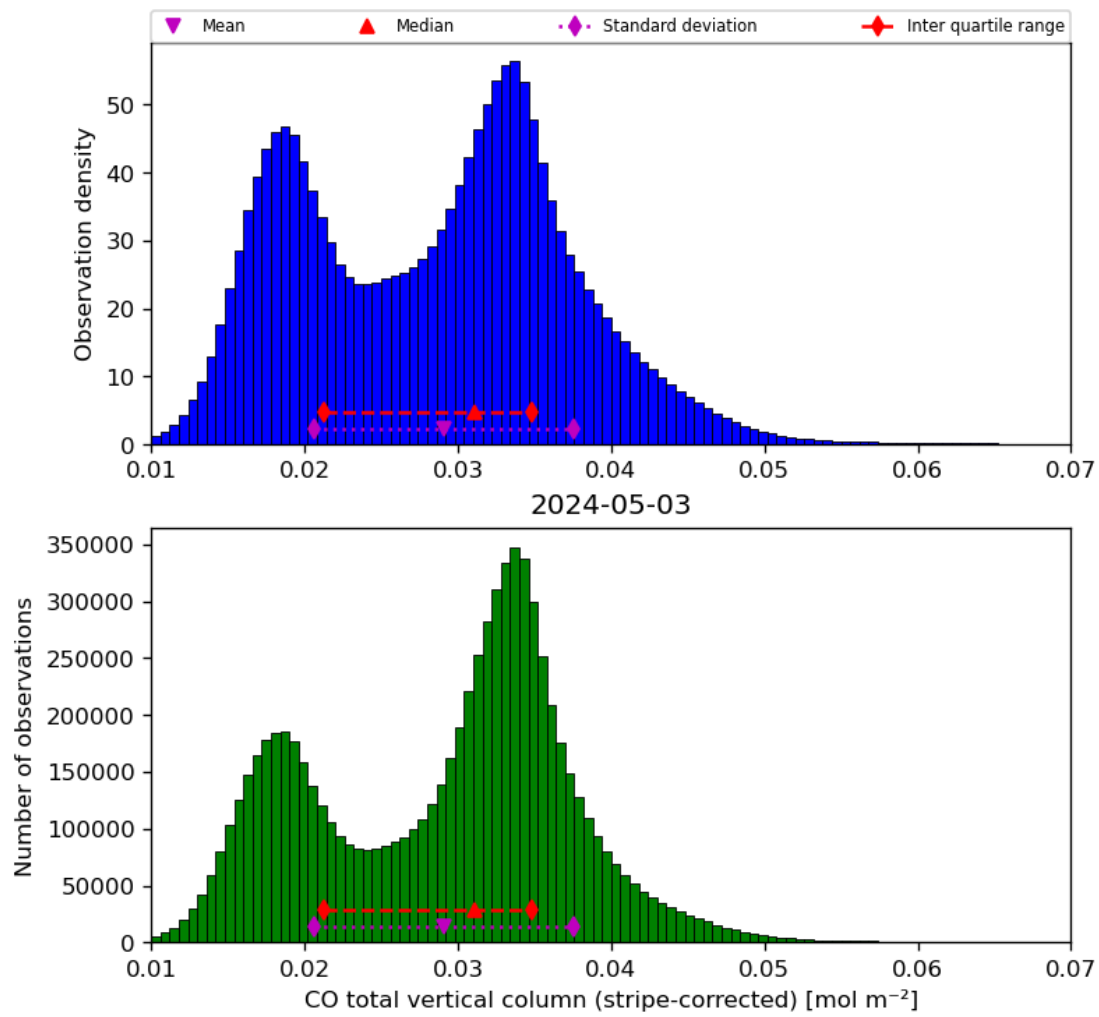
Figure 19: Histogram of “CO total vertical column (stripe-corrected)” for 2024-05-02 to 2024-05-04
