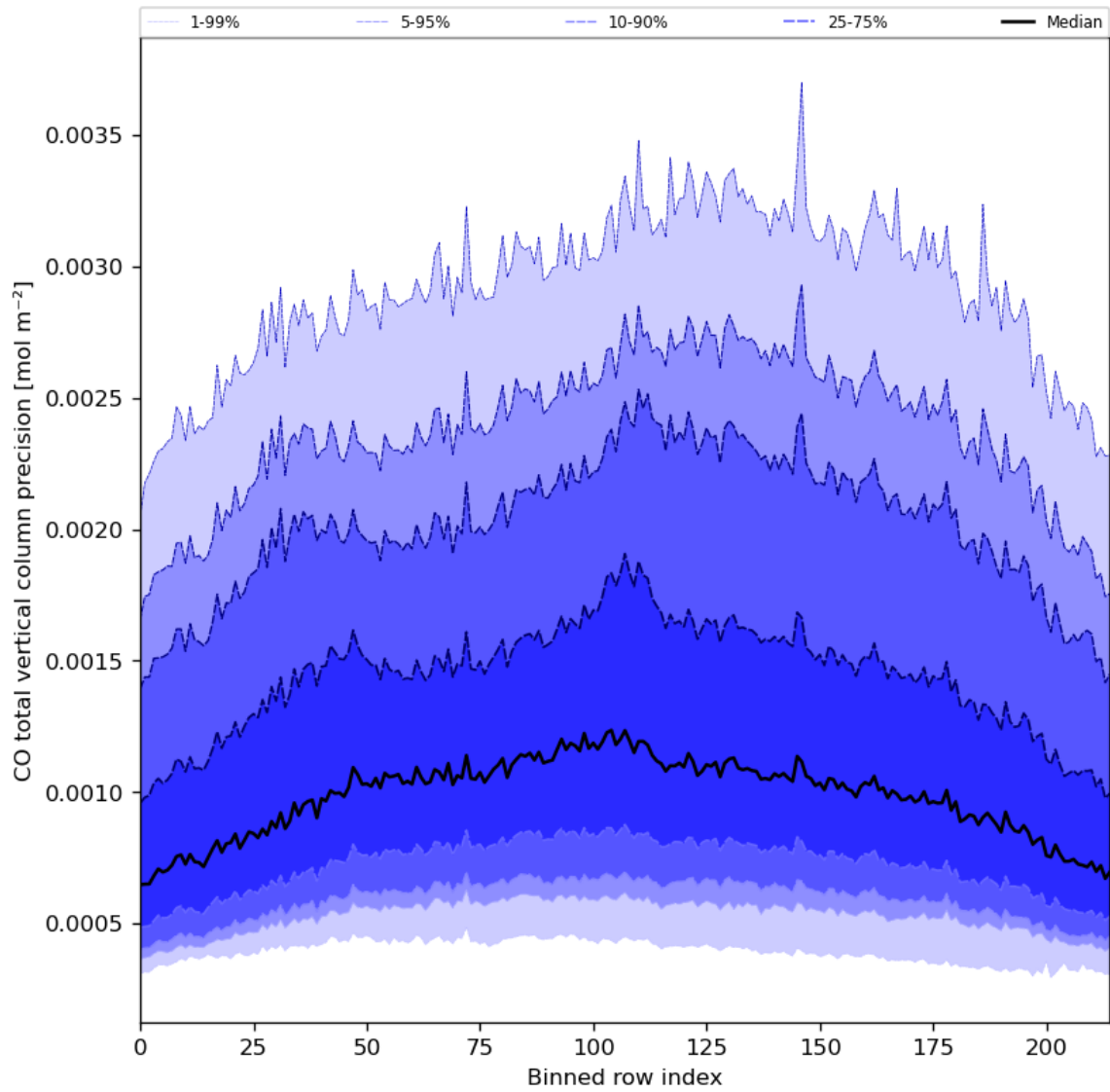
Figure 28: Along track statistics of “CO total vertical column precision” for 2024-05-02 to 2024-05-04
