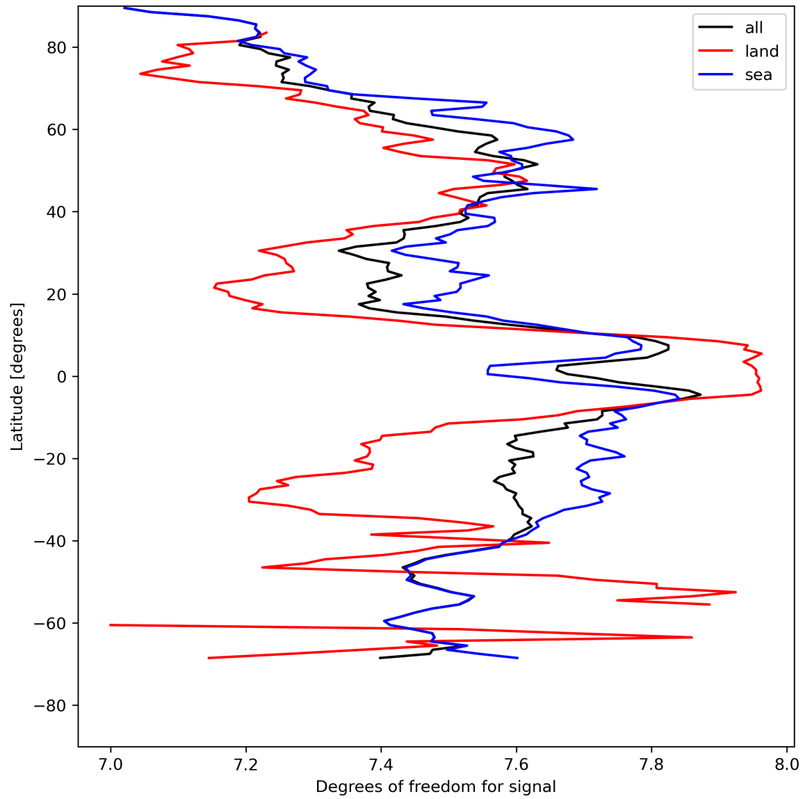
Figure 15: Zonal average of “Degrees of freedom for signal” for 2024-05-02 to 2024-05-04.
