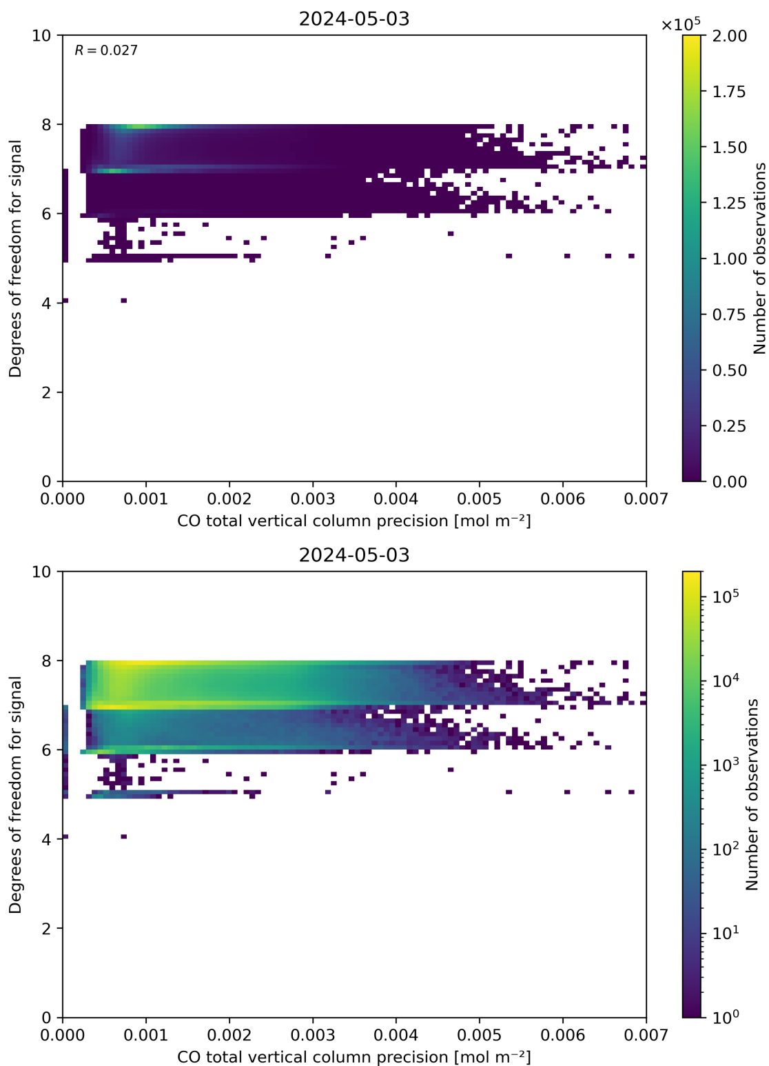
Figure 45: Scatter density plot of “CO total vertical column precision” against “Degrees of freedom for signal” for 2024-05-02 to 2024-05-04.
