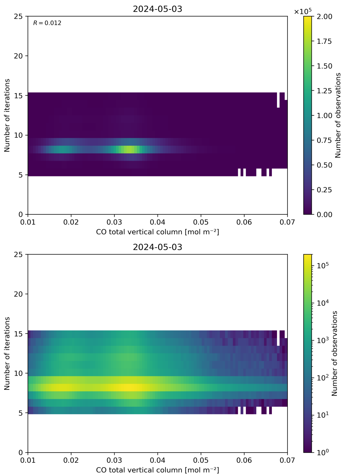
Figure 42: Scatter density plot of “CO total vertical column” against “Number of iterations” for 2024-05-02 to 2024-05-04.
