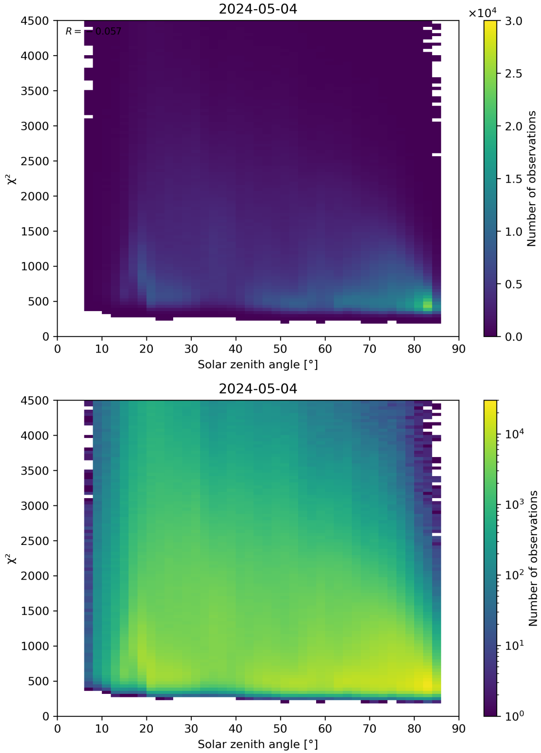
Figure 64: Scatter density plot of “Solar zenith angle” against “ \chi^2 ” for 2024-05-03 to 2024-05-05.
