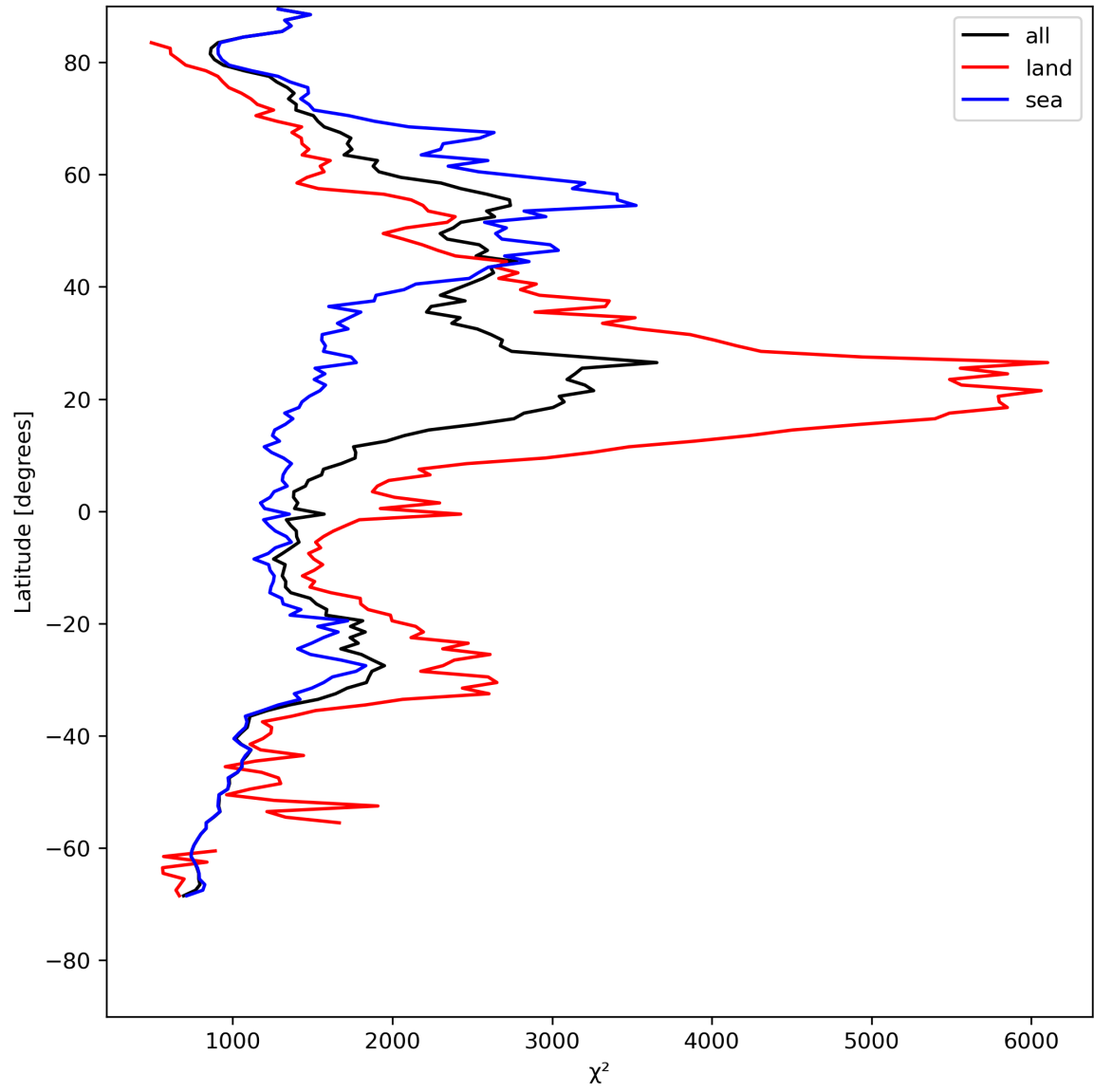
Figure 14: Zonal average of “ \chi^2 ” for 2024-05-03 to 2024-05-05.
