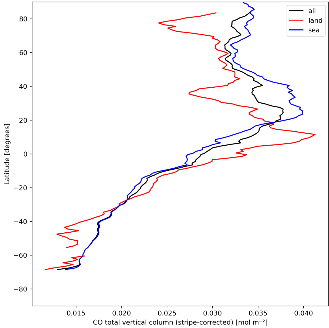
Figure 11: Zonal average of “CO total vertical column (stripe-corrected)” for 2024-05-03 to 2024-05-05.
