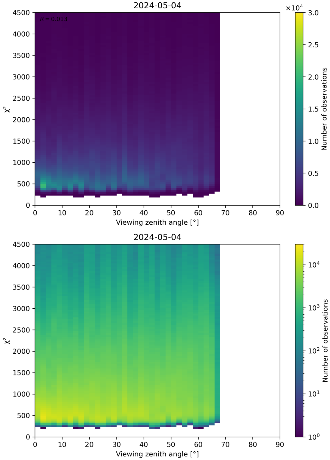
Figure 72: Scatter density plot of “Viewing zenith angle” against “ \chi^2 ” for 2024-05-03 to 2024-05-05.
