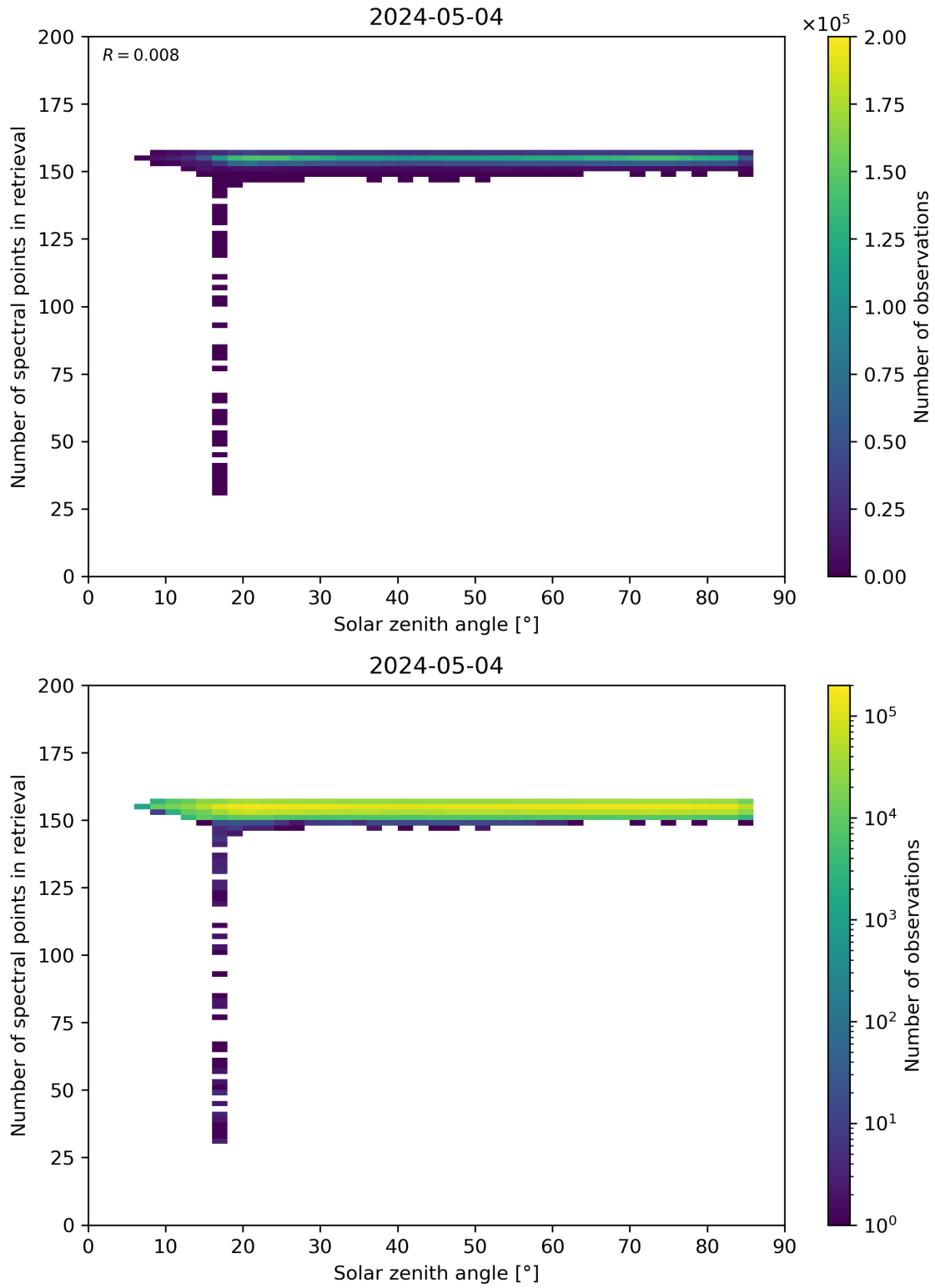
Figure 68: Scatter density plot of “Solar zenith angle” against “Number of spectral points in retrieval” for 2024-05-03 to 2024-05-05.
