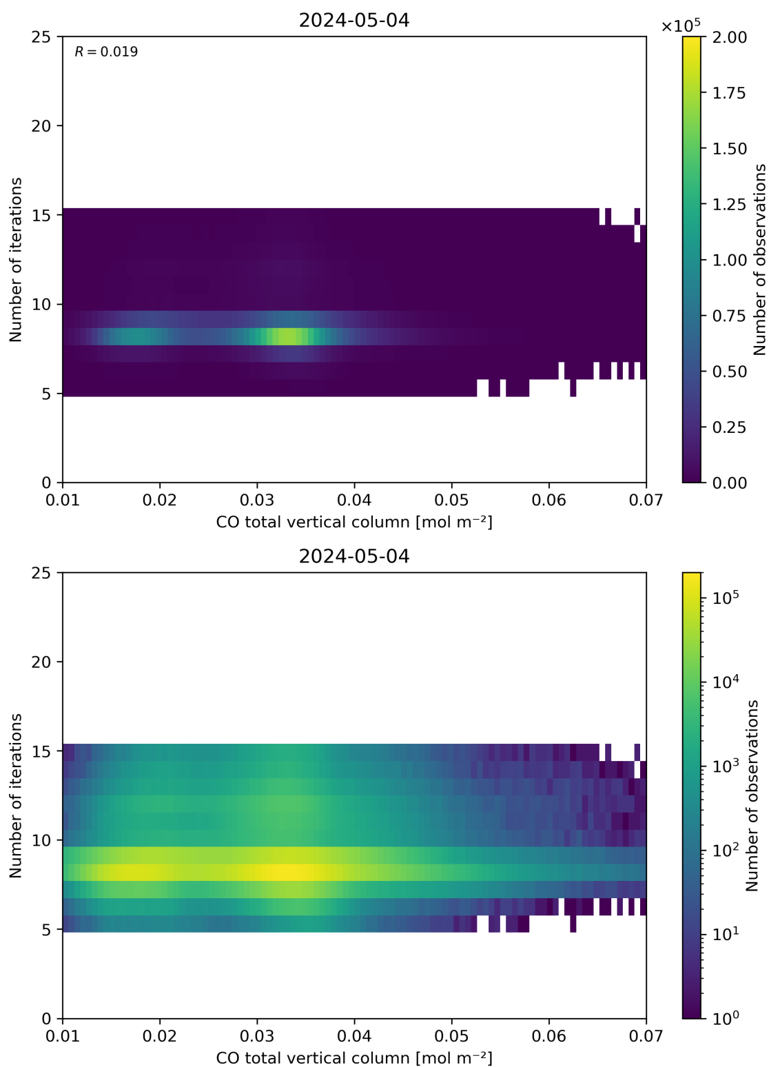
Figure 42: Scatter density plot of “CO total vertical column” against “Number of iterations” for 2024-05-03 to 2024-05-05.
