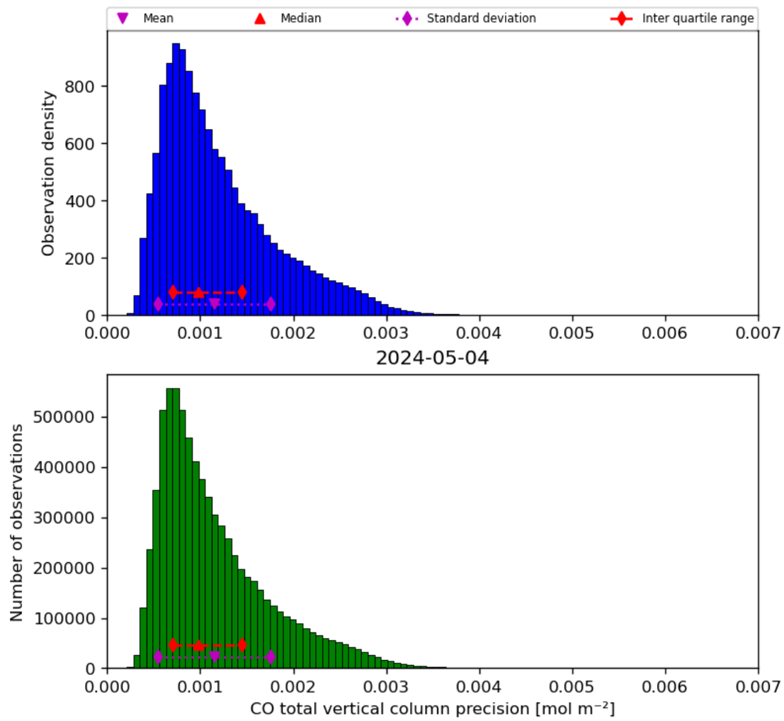
Figure 20: Histogram of “CO total vertical column precision” for 2024-05-03 to 2024-05-05
