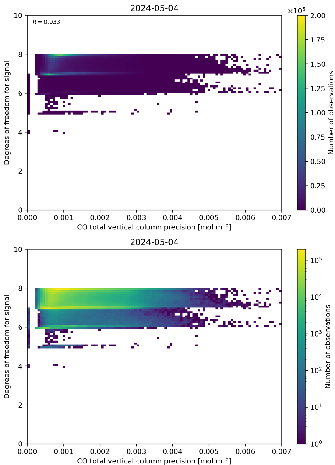
Figure 45: Scatter density plot of “CO total vertical column precision” against “Degrees of freedom for signal” for 2024-05-03 to 2024-05-05.
