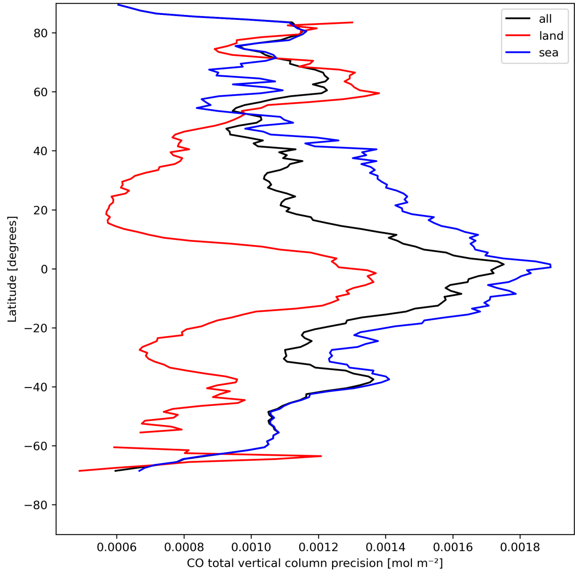
Figure 12: Zonal average of “CO total vertical column precision” for 2024-05-03 to 2024-05-05.
