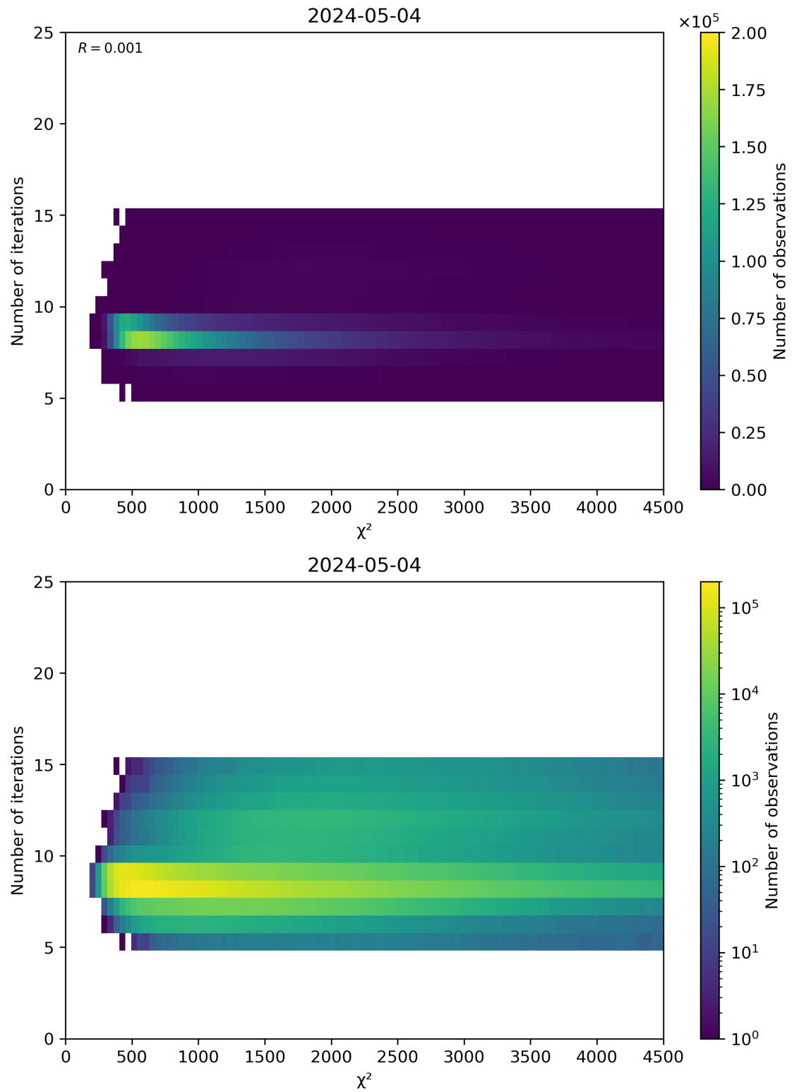
Figure 49: Scatter density plot of “ \chi^2 ” against “Number of iterations” for 2024-05-03 to 2024-05-05.
