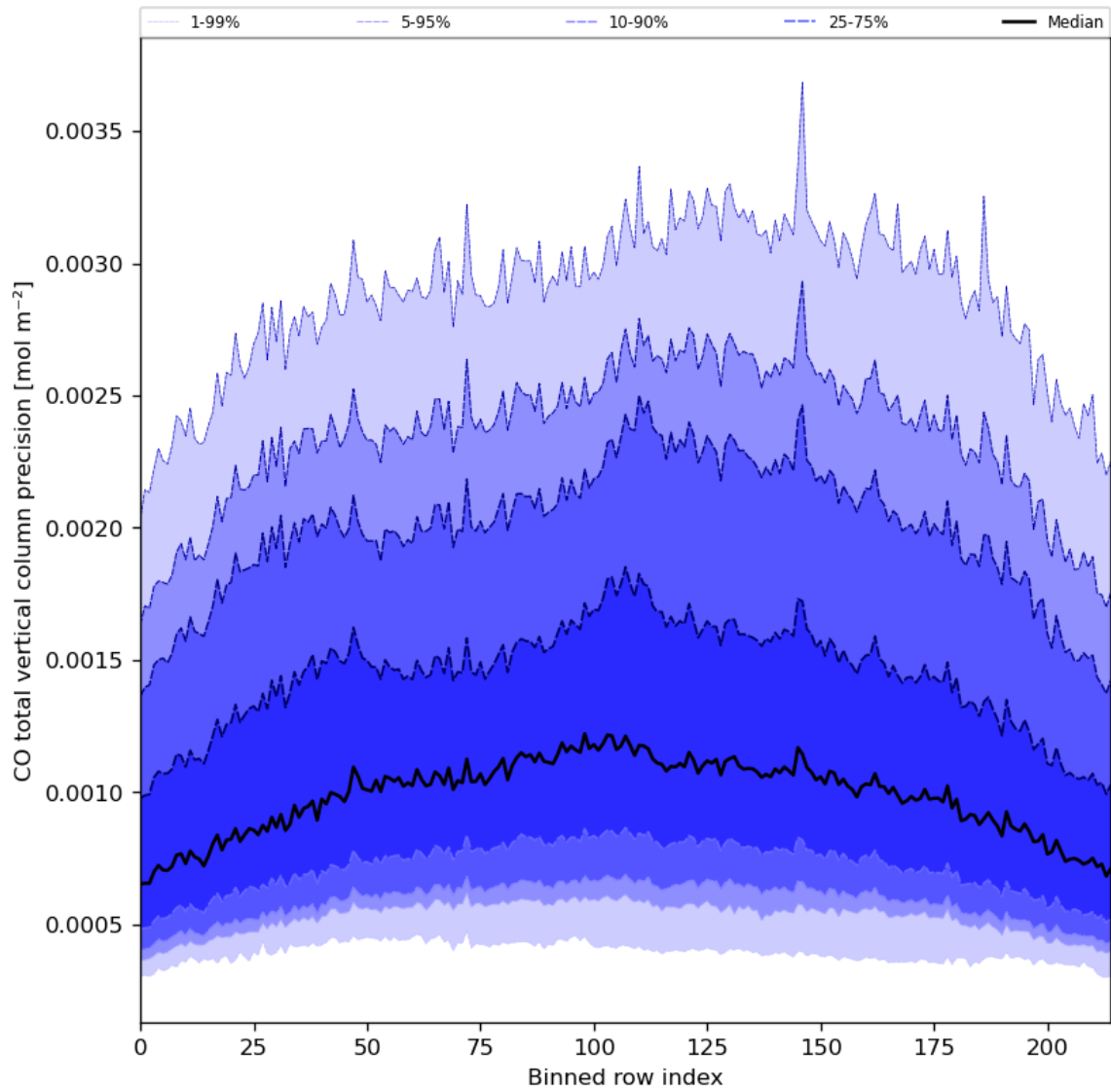
Figure 28: Along track statistics of “CO total vertical column precision” for 2024-05-03 to 2024-05-05
