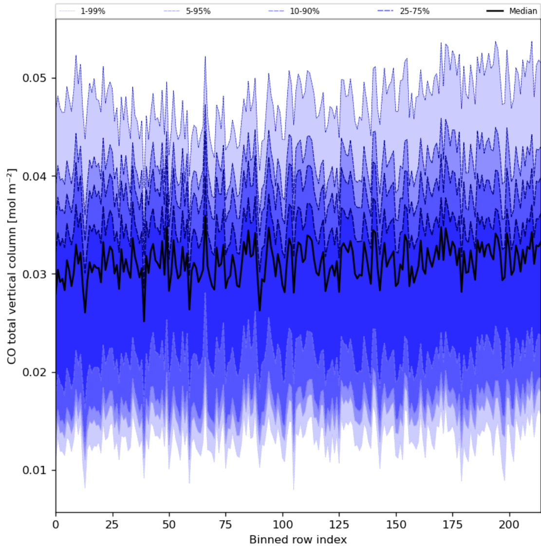
Figure 26: Along track statistics of “CO total vertical column” for 2024-05-03 to 2024-05-05
