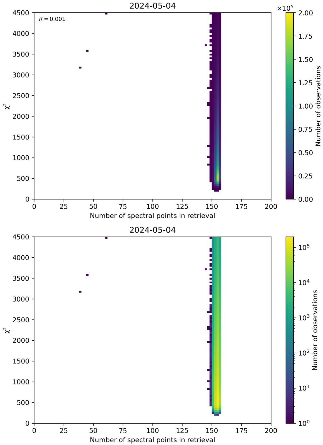
Figure 58: Scatter density plot of “Number of spectral points in retrieval” against “ \chi^2 ” for 2024-05-03 to 2024-05-05.
