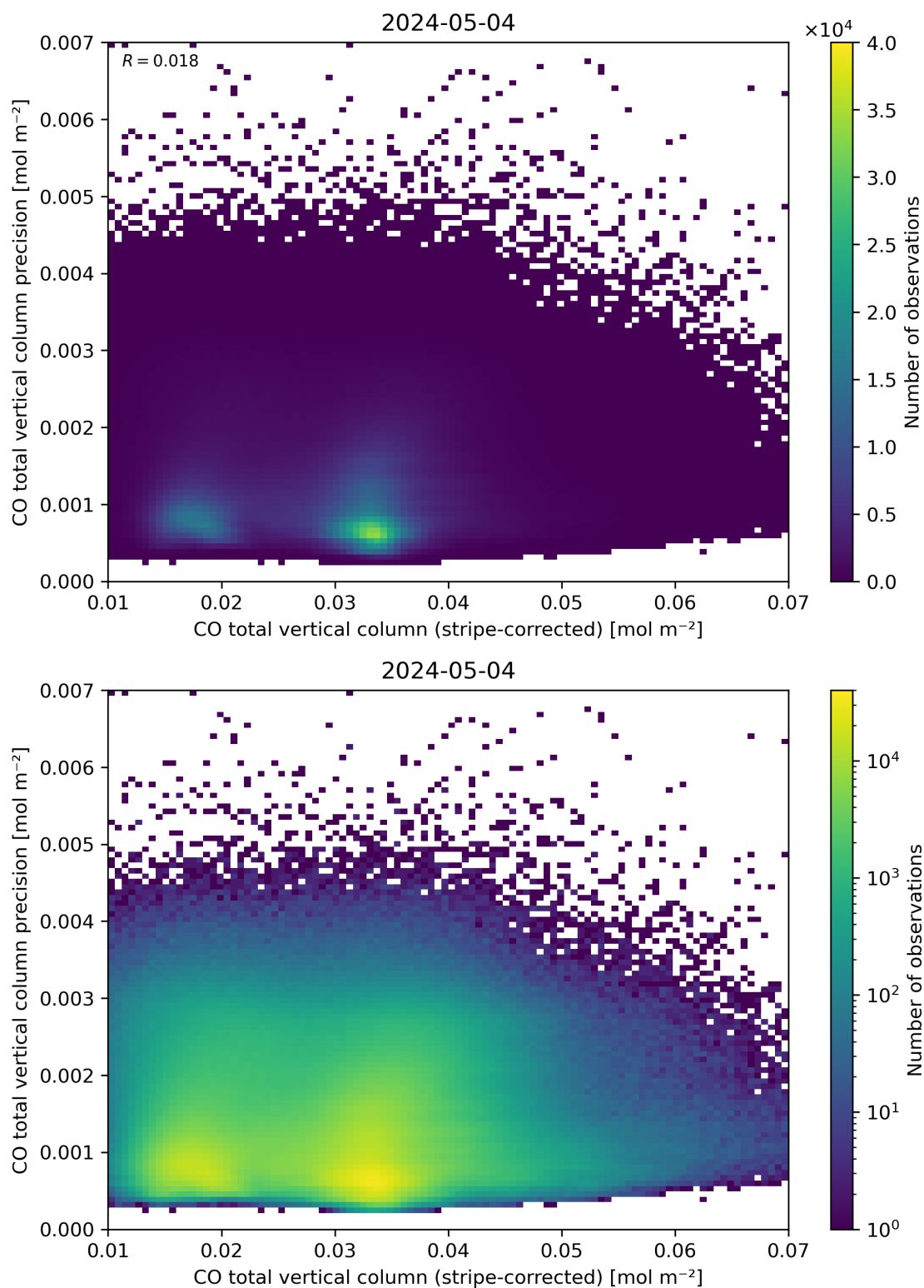
Figure 36: Scatter density plot of “CO total vertical column (stripe-corrected)” against “CO total vertical column precision” for 2024-05-03 to 2024-05-05.
