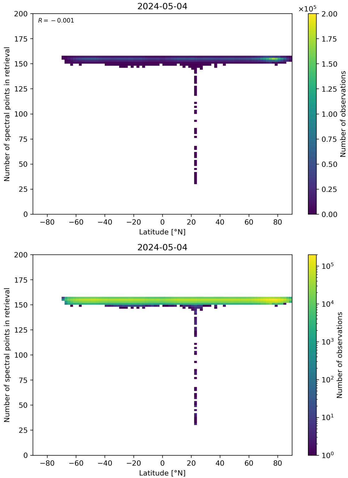
Figure 57: Scatter density plot of “Latitude” against “Number of spectral points in retrieval” for 2024-05-03 to 2024-05-05.
