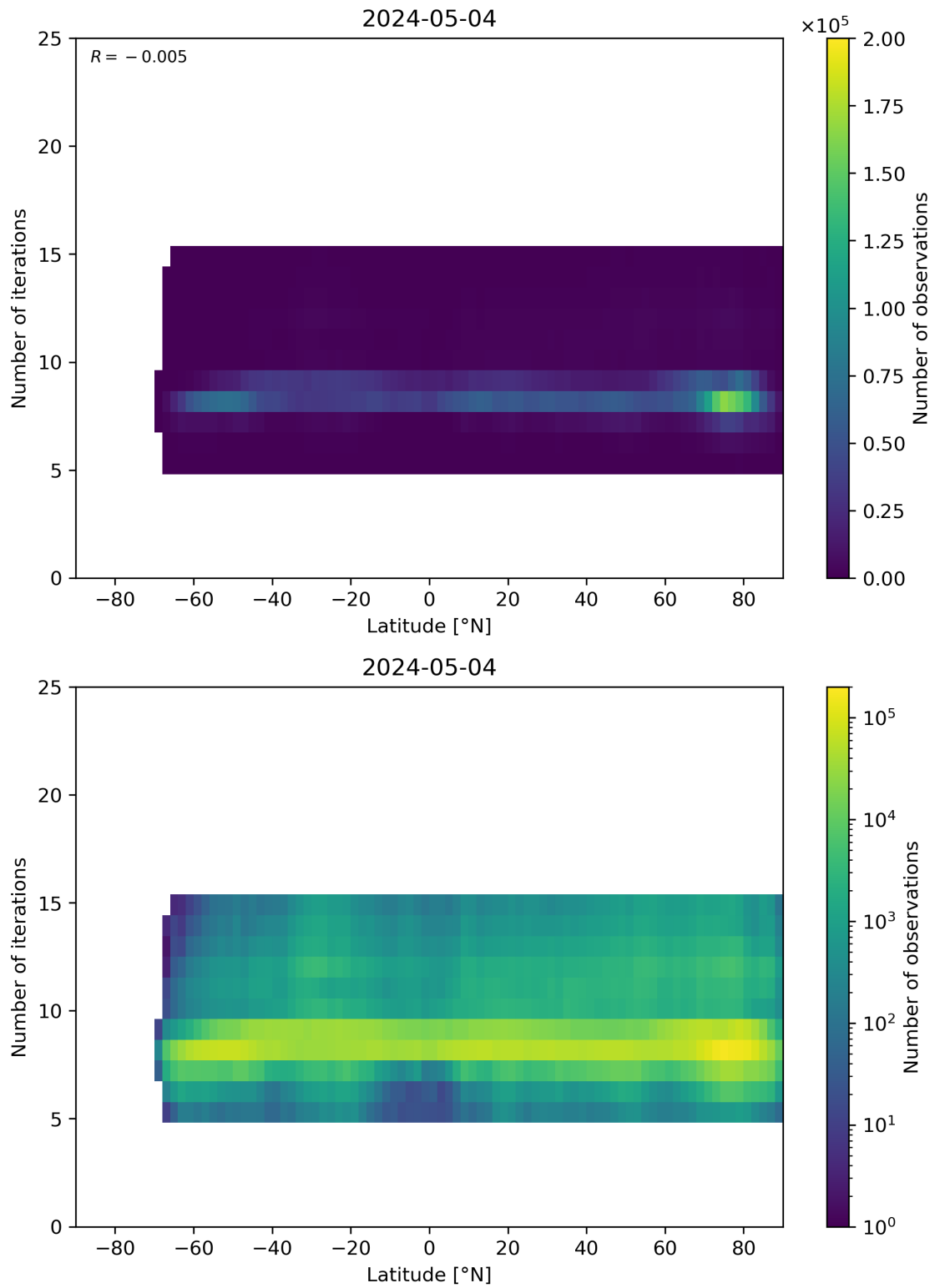
Figure 56: Scatter density plot of “Latitude” against “Number of iterations” for 2024-05-03 to 2024-05-05.
