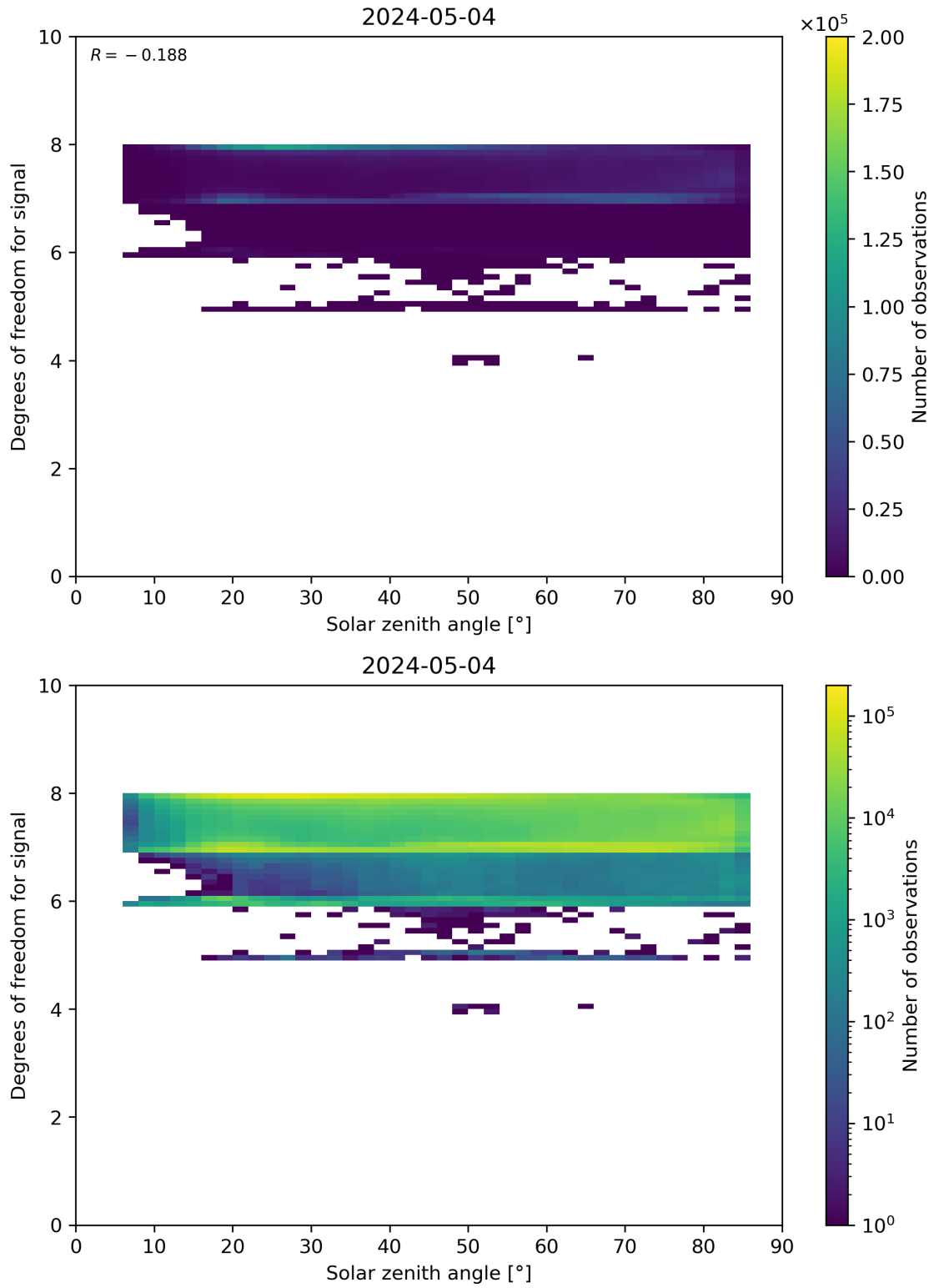
Figure 65: Scatter density plot of “Solar zenith angle” against “Degrees of freedom for signal” for 2024-05-03 to 2024-05-05.
