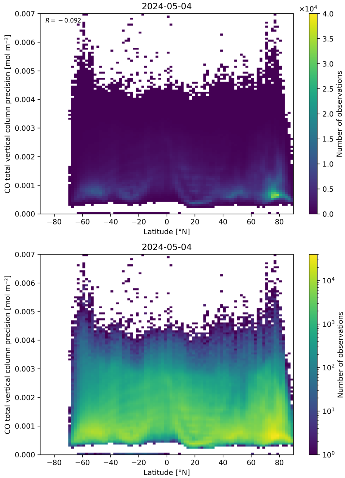
Figure 53: Scatter density plot of “Latitude” against “CO total vertical column precision” for 2024-05-03 to 2024-05-05.
