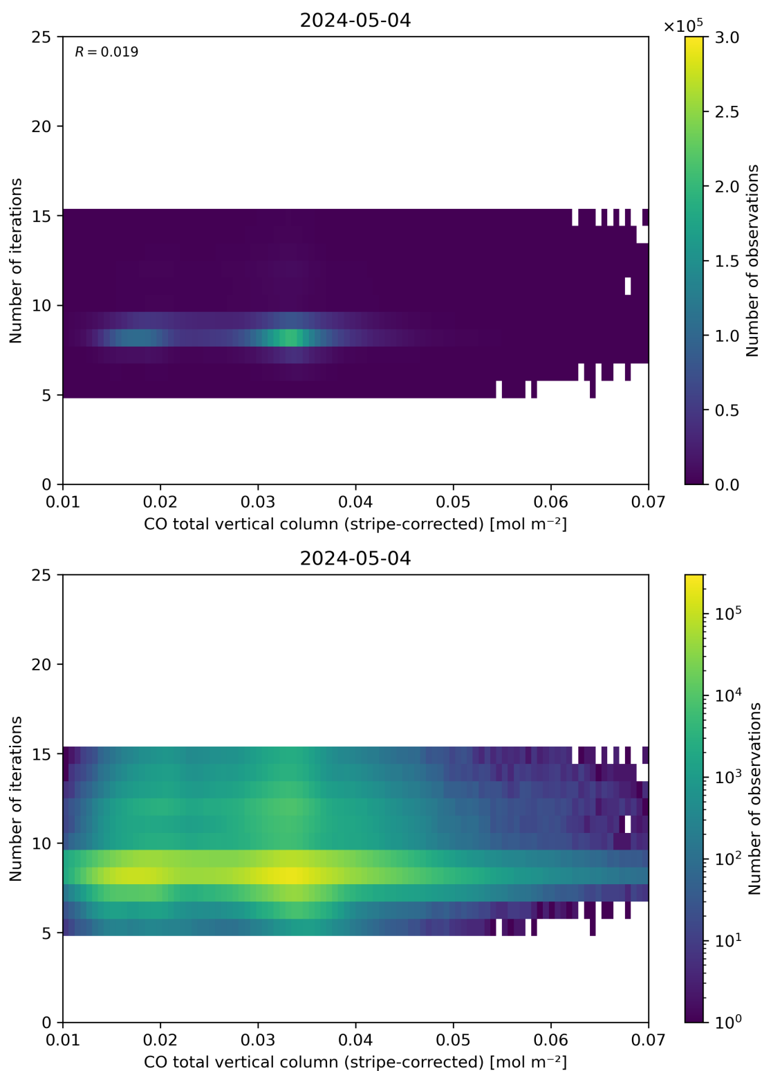
Figure 39: Scatter density plot of “CO total vertical column (stripe-corrected)” against “Number of iterations” for 2024-05-03 to 2024-05-05.
