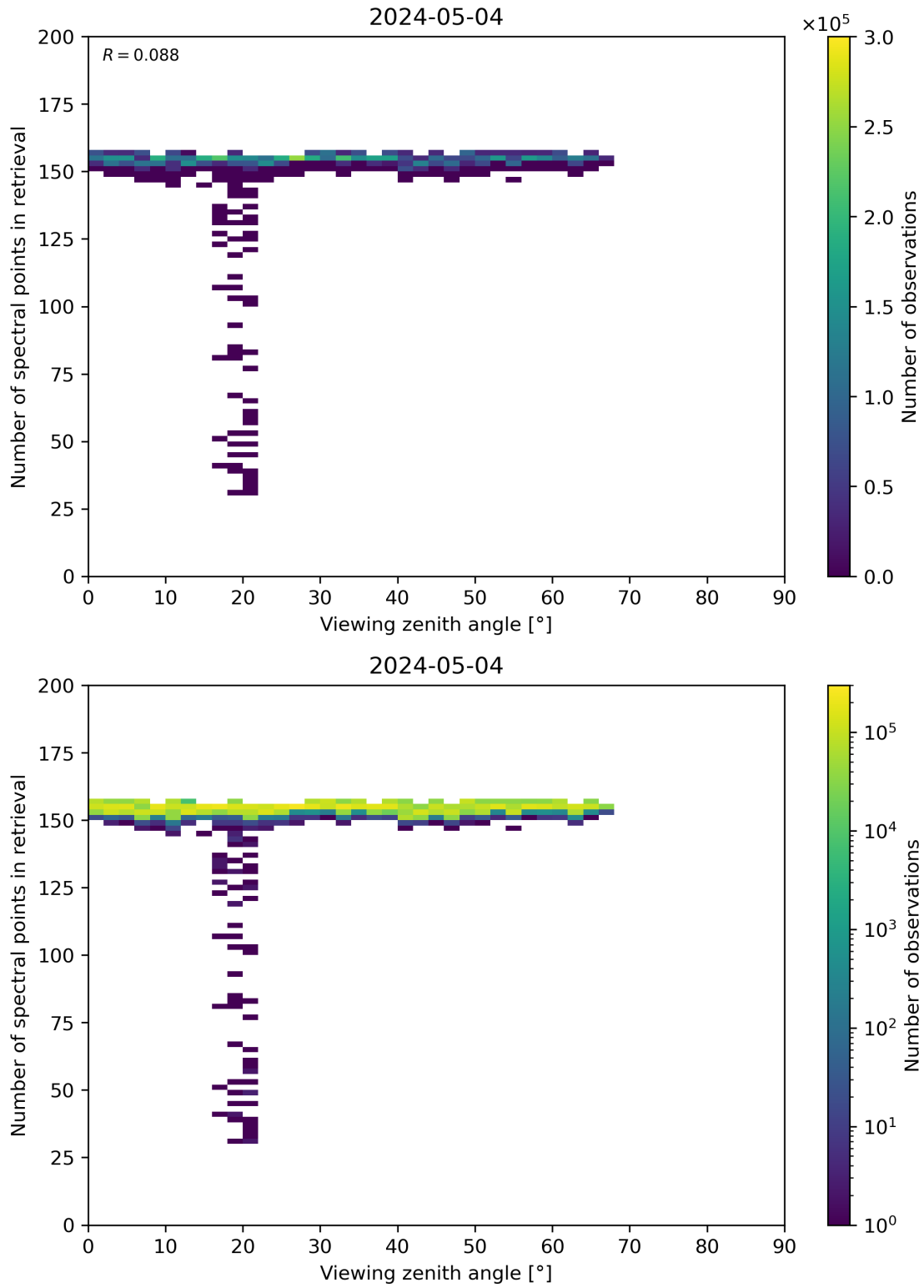
Figure 76: Scatter density plot of “Viewing zenith angle” against “Number of spectral points in retrieval” for 2024-05-03 to 2024-05-05.
