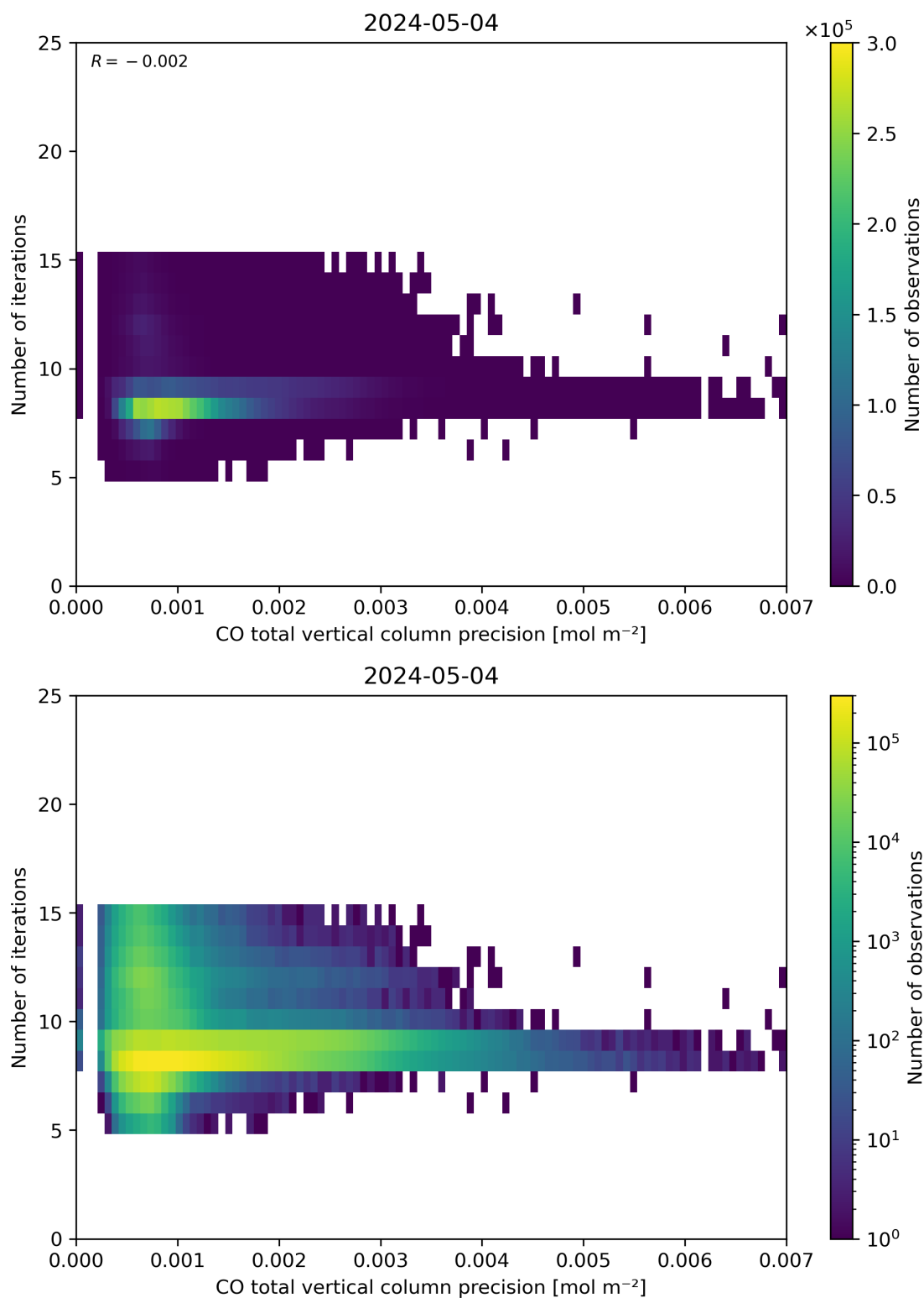
Figure 46: Scatter density plot of “CO total vertical column precision” against “Number of iterations” for 2024-05-03 to 2024-05-05.
