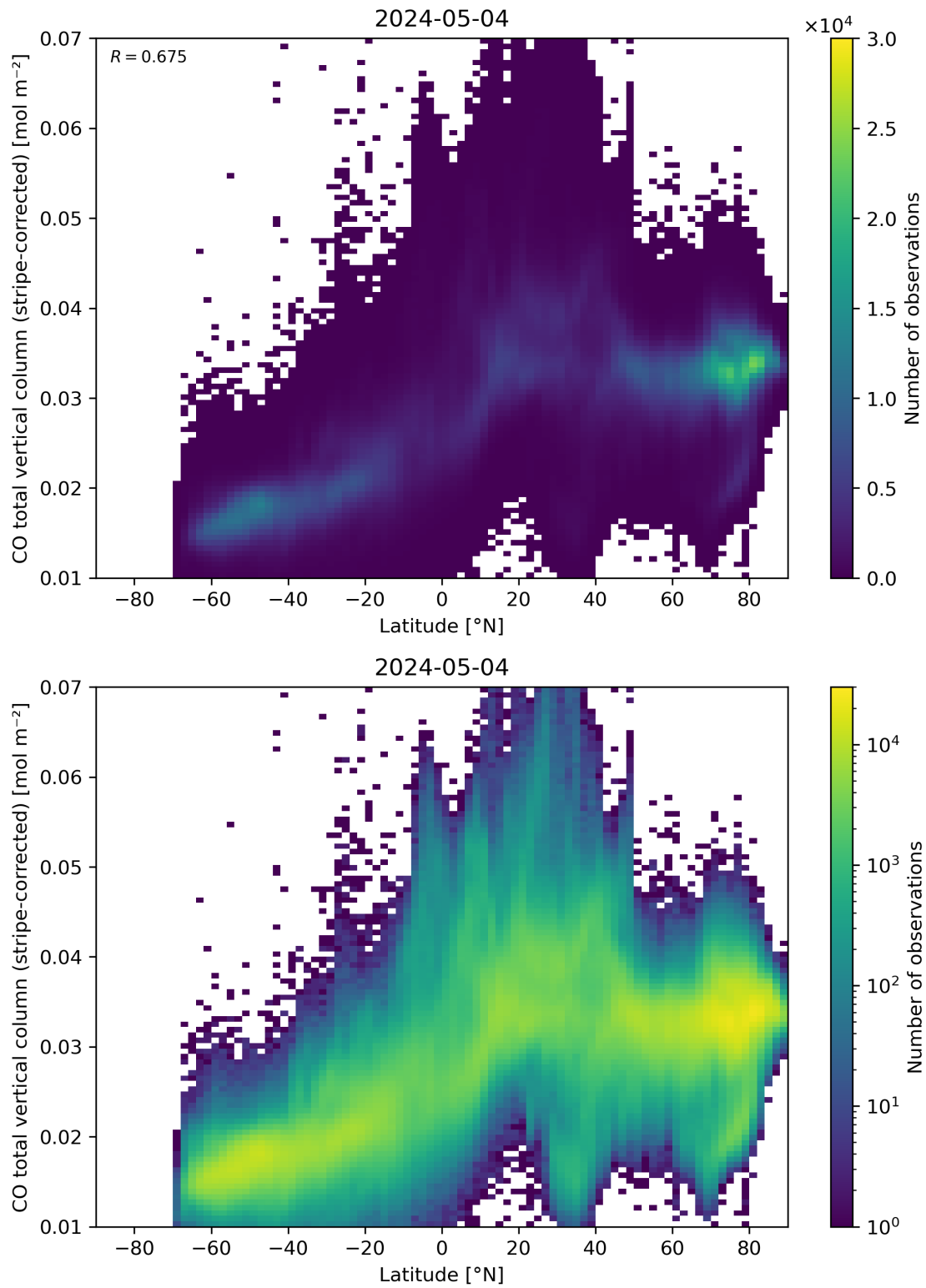
Figure 52: Scatter density plot of “Latitude” against “CO total vertical column (stripe-corrected)” for 2024-05-03 to 2024-05-05.
