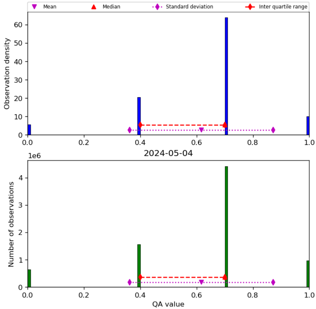
Figure 17: Histogram of “QA value” for 2024-05-03 to 2024-05-05
