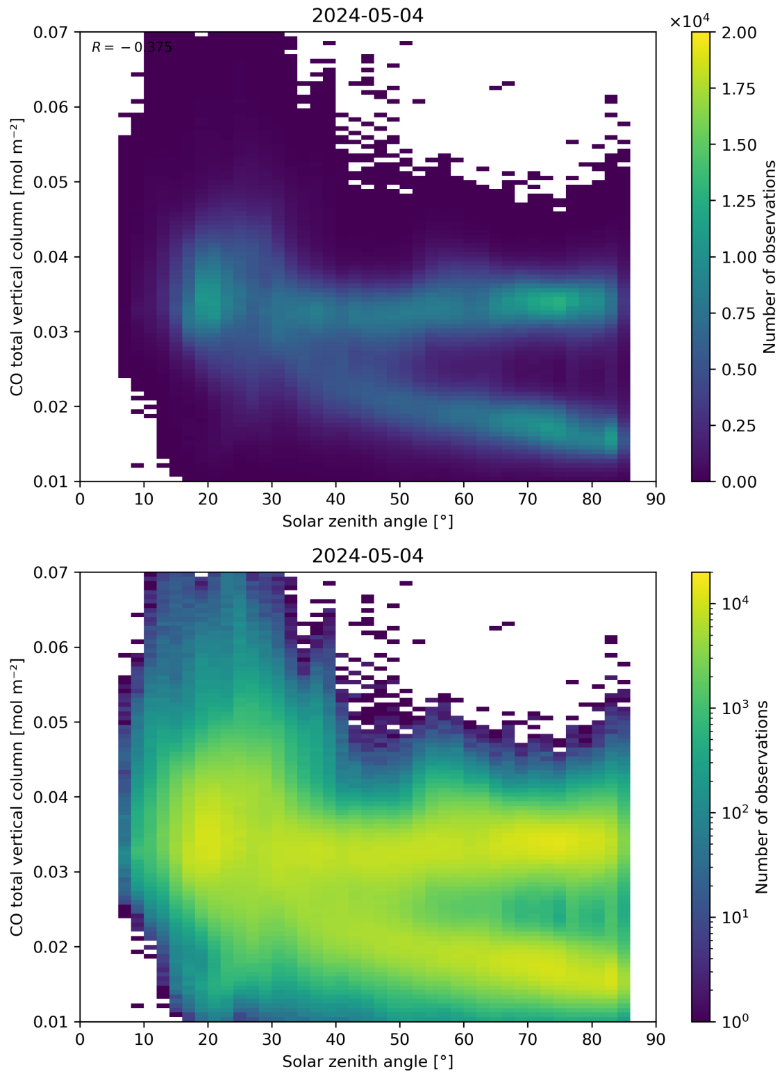
Figure 61: Scatter density plot of “Solar zenith angle” against “CO total vertical column” for 2024-05-03 to 2024-05-05.
