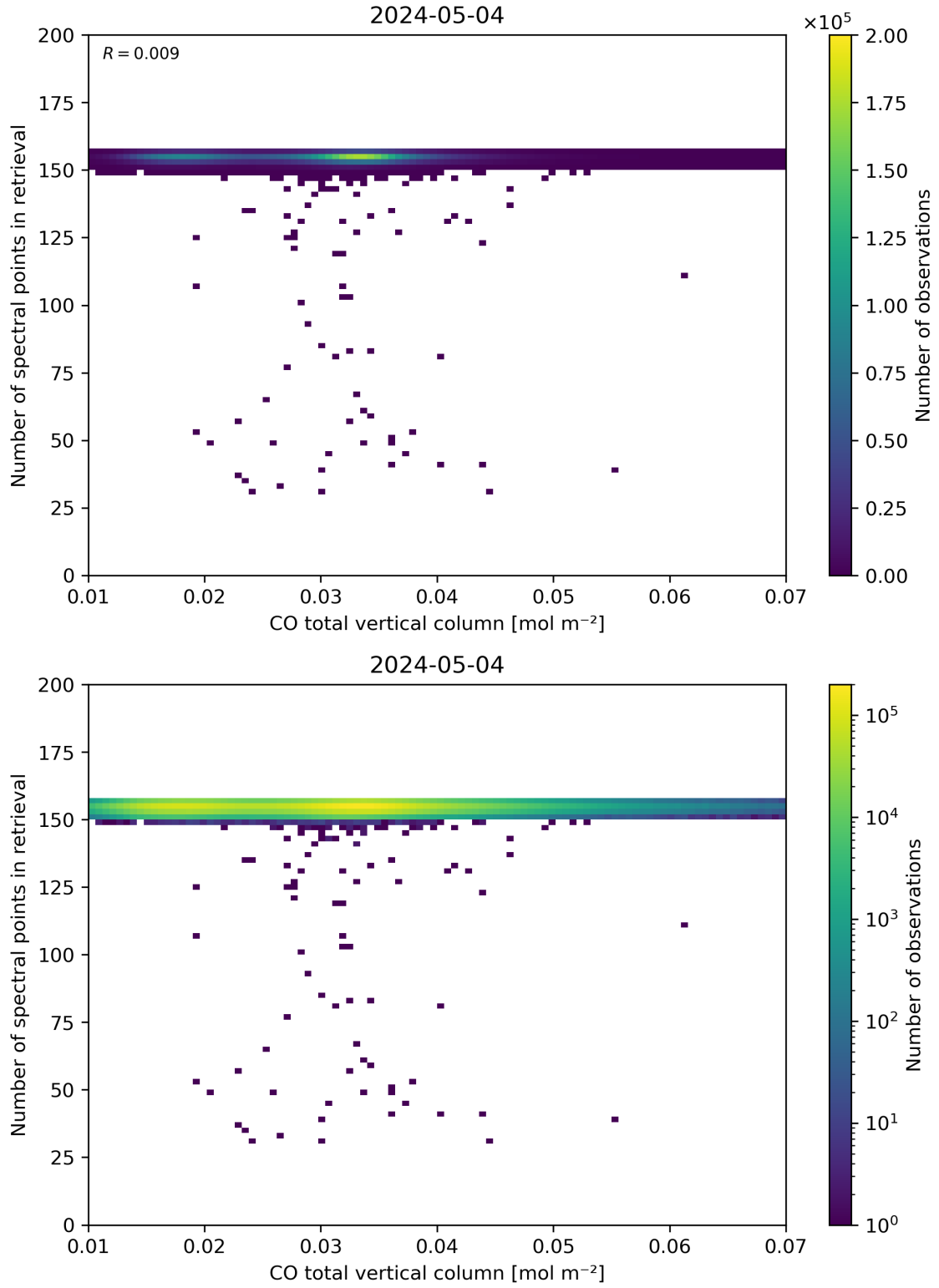
Figure 43: Scatter density plot of “CO total vertical column” against “Number of spectral points in retrieval” for 2024-05-03 to 2024-05-05.
