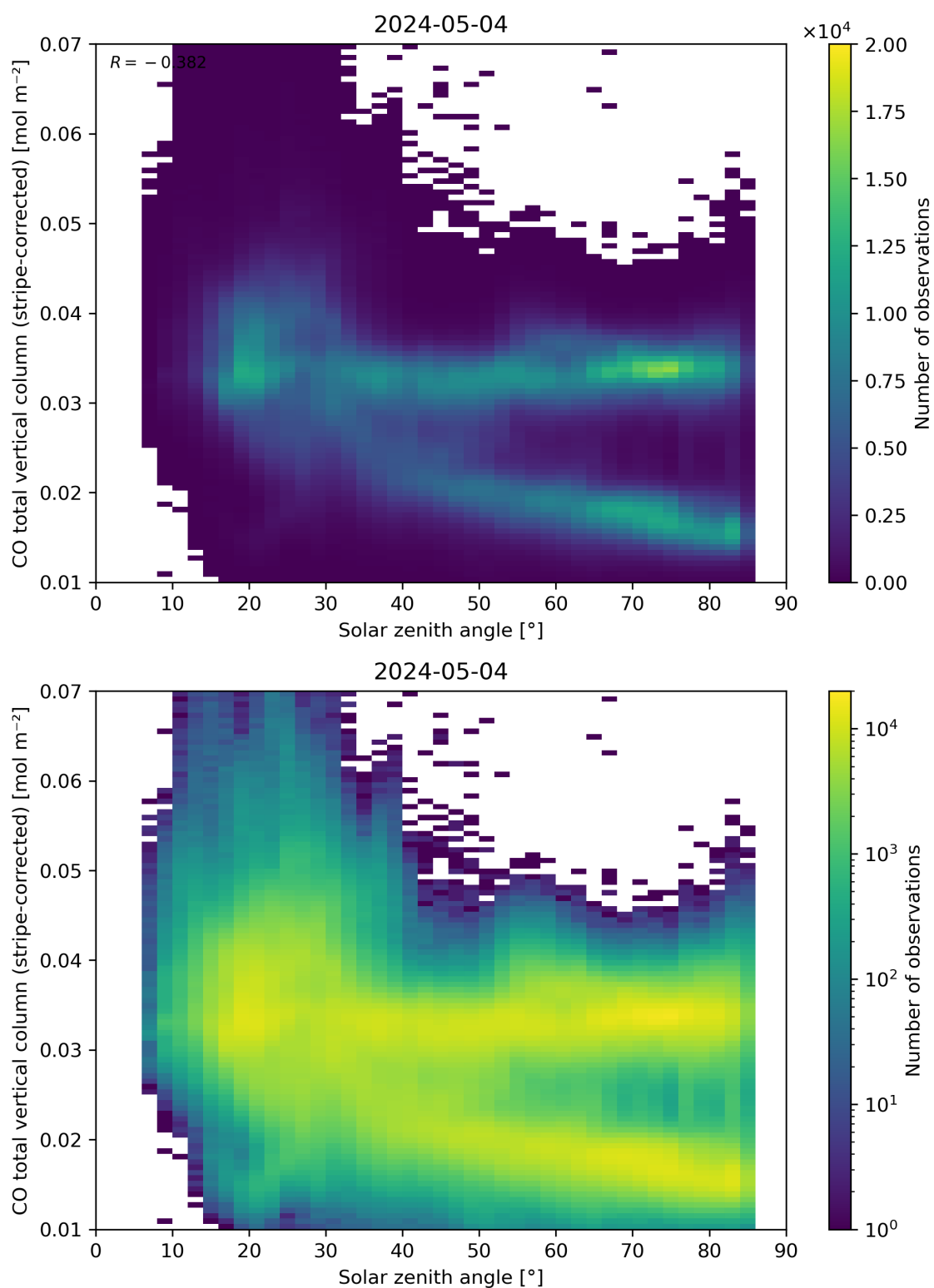
Figure 62: Scatter density plot of “Solar zenith angle” against “CO total vertical column (stripe-corrected)” for 2024-05-03 to 2024-05-05.
