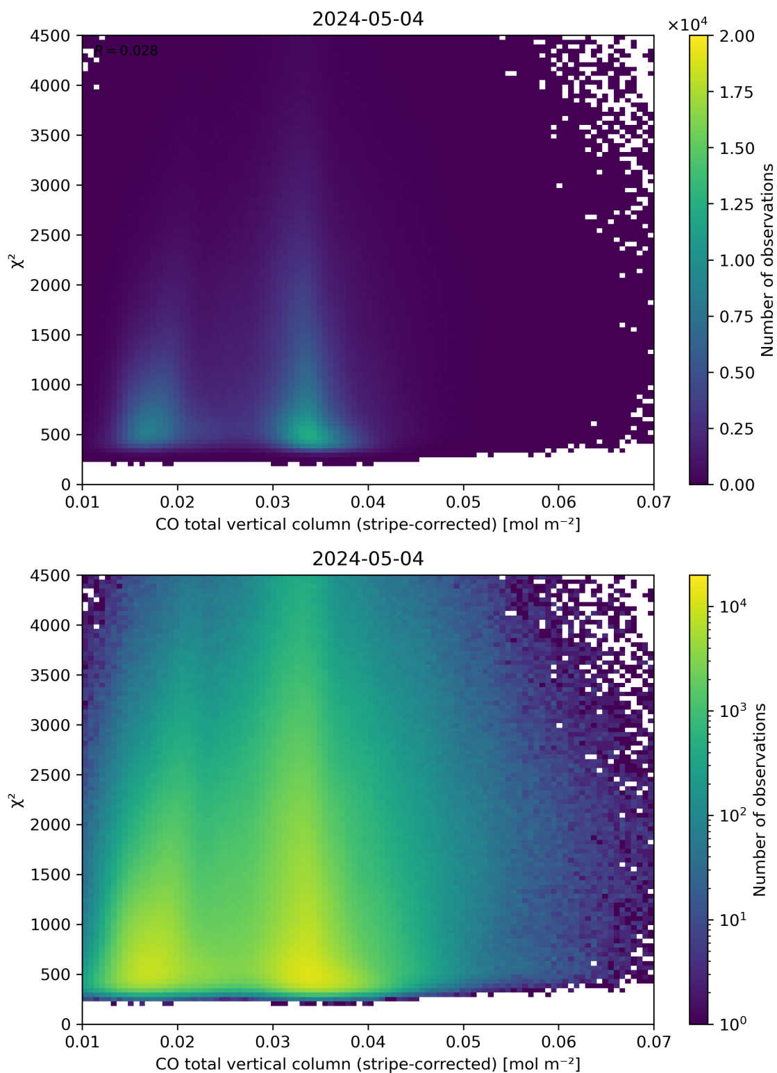
Figure 37: Scatter density plot of “CO total vertical column (stripe-corrected)” against “ \chi^2 ” for 2024-05-03 to 2024-05-05.
