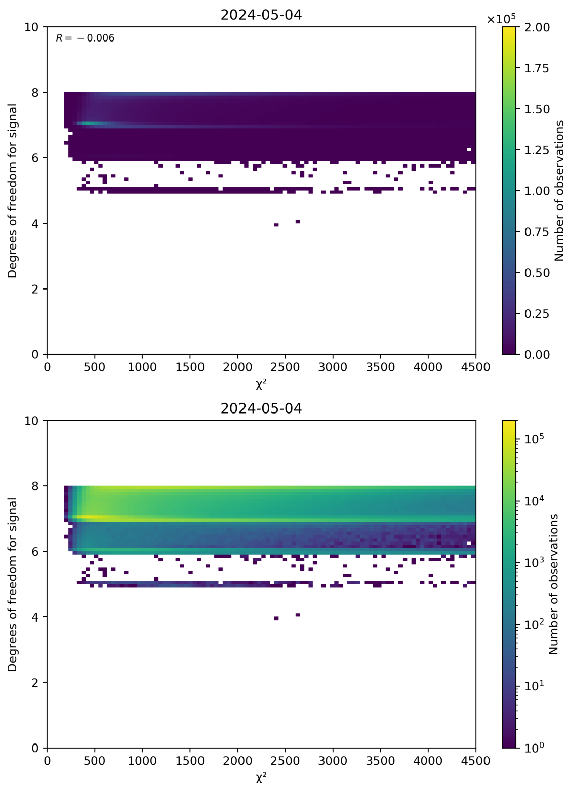
Figure 48: Scatter density plot of “ \chi^2 ” against “Degrees of freedom for signal” for 2024-05-03 to 2024-05-05.
