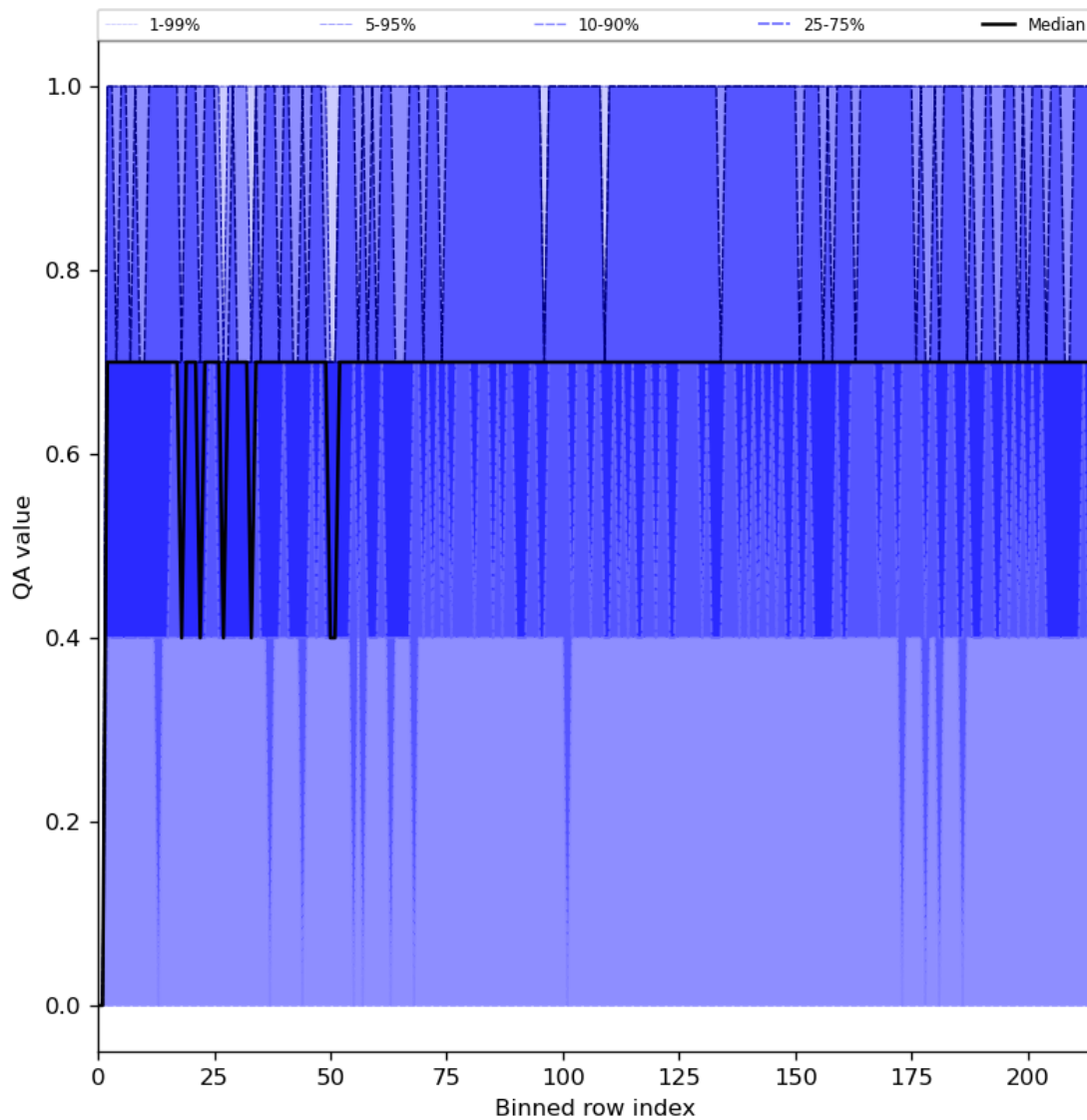
Figure 25: Along track statistics of “QA value” for 2024-05-03 to 2024-05-05
