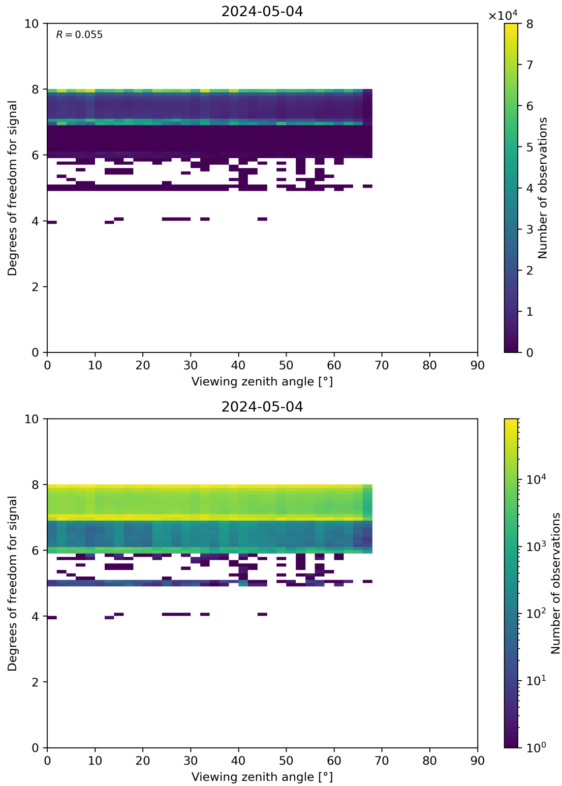
Figure 73: Scatter density plot of “Viewing zenith angle” against “Degrees of freedom for signal” for 2024-05-03 to 2024-05-05.
