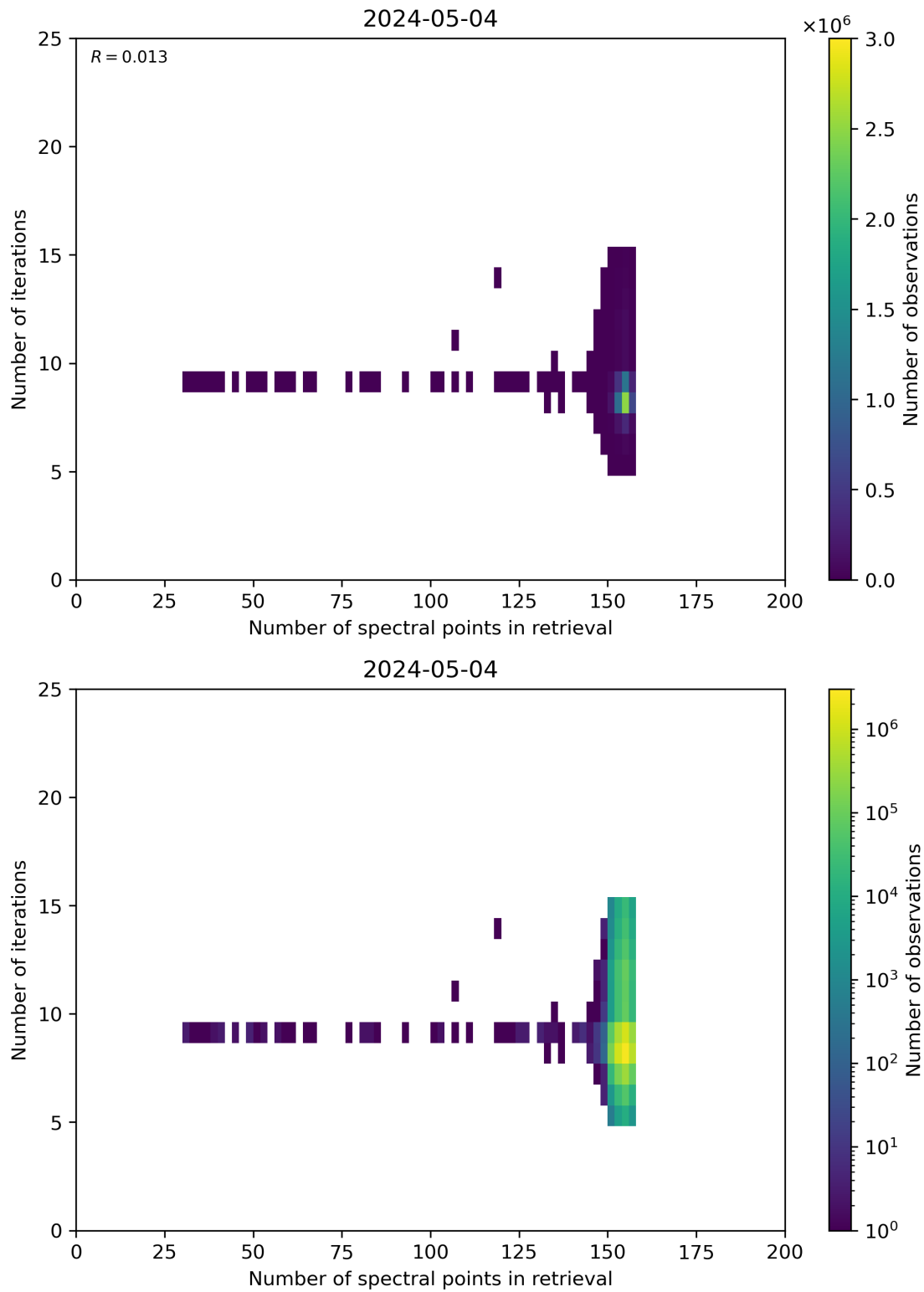
Figure 60: Scatter density plot of “Number of spectral points in retrieval” against “Number of iterations” for 2024-05-03 to 2024-05-05.
