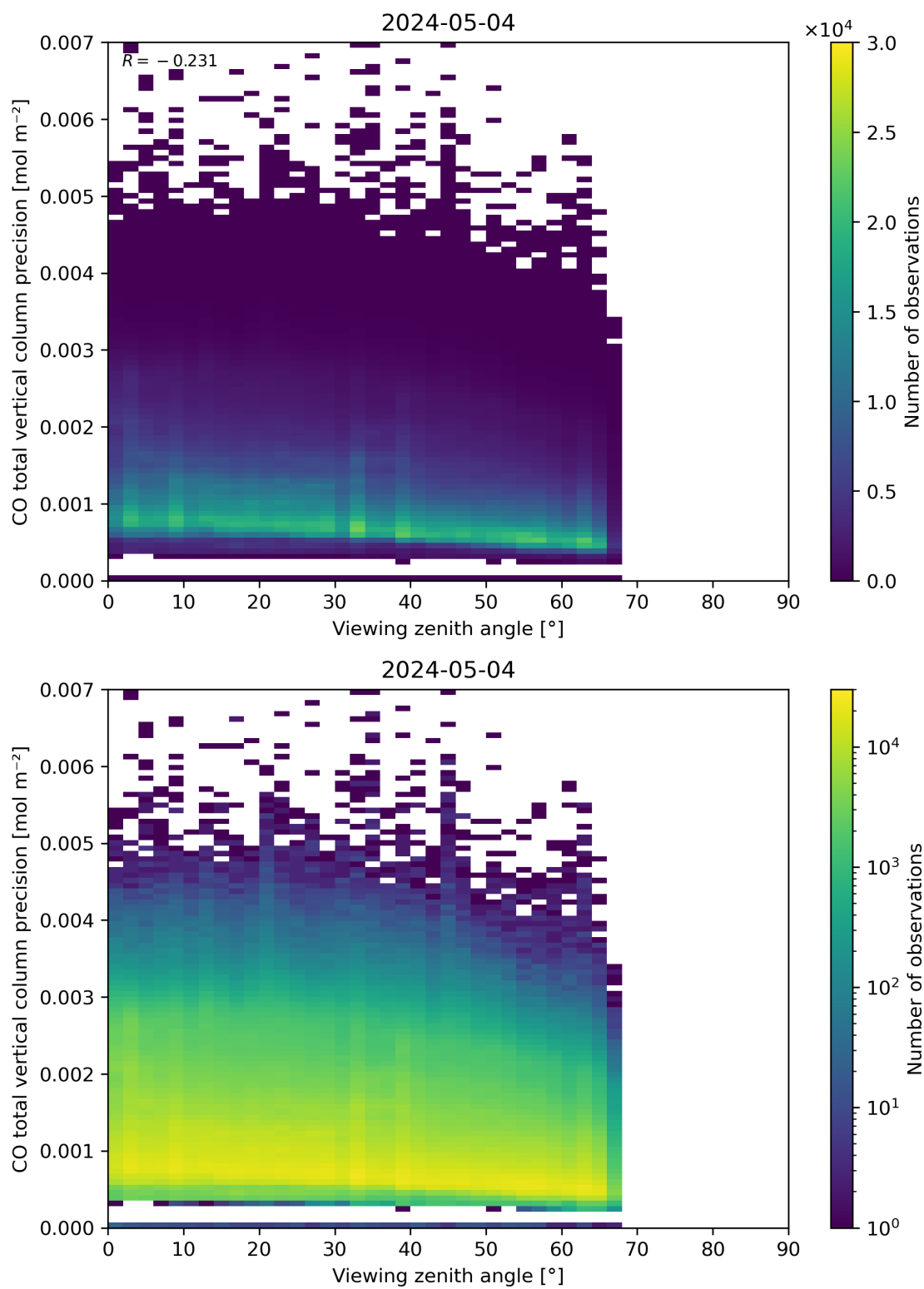
Figure 71: Scatter density plot of “Viewing zenith angle” against “CO total vertical column precision” for 2024-05-03 to 2024-05-05.
