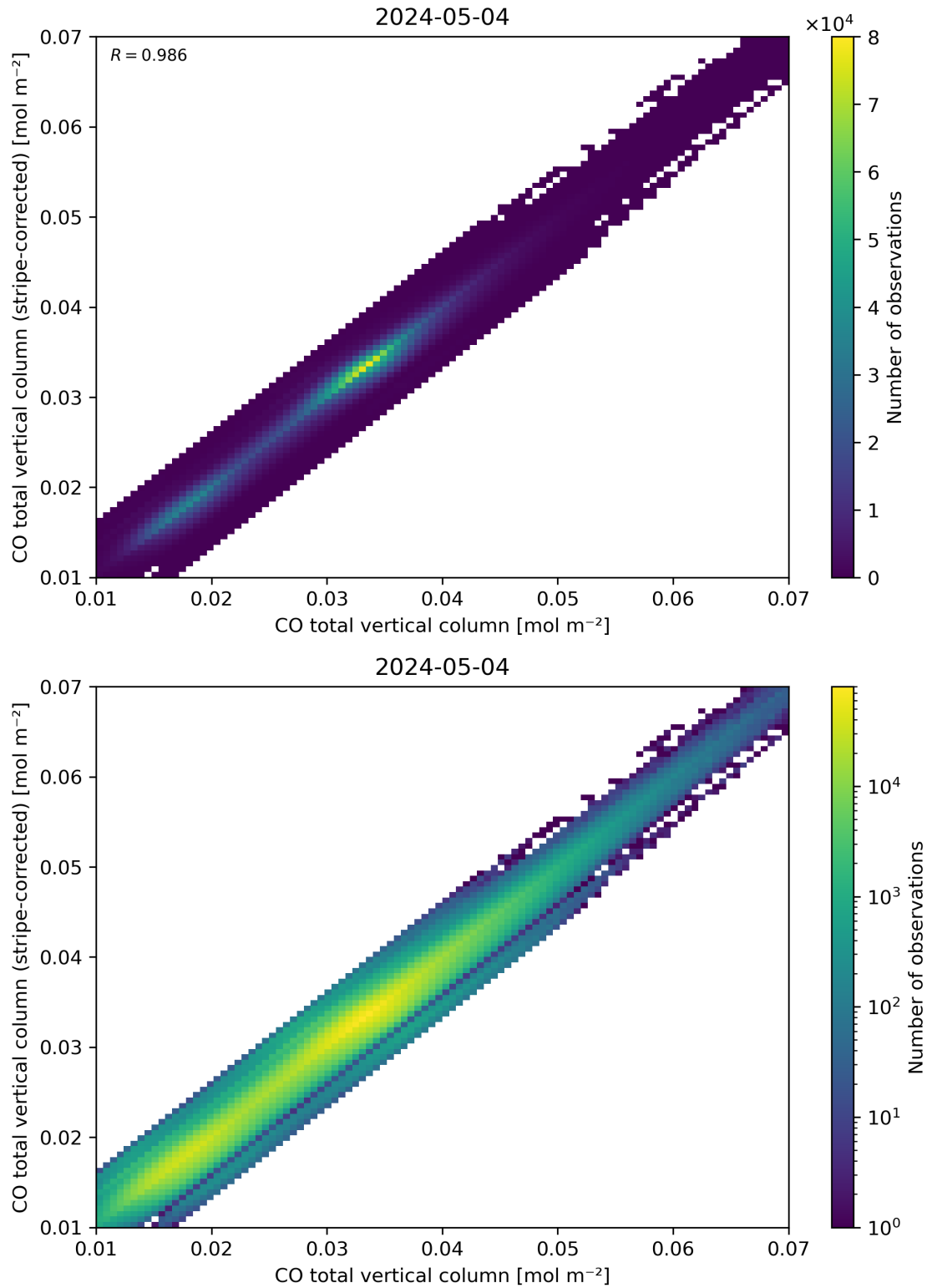
Figure 33: Scatter density plot of “CO total vertical column” against “CO total vertical column (stripe-corrected)” for 2024-05-03 to 2024-05-05.
