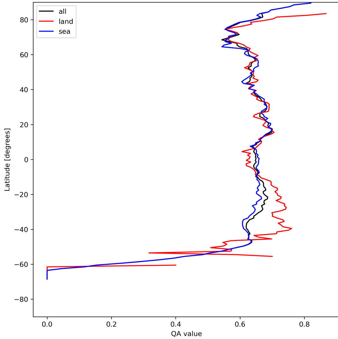
Figure 9: Zonal average of “QA value” for 2024-05-03 to 2024-05-05.
