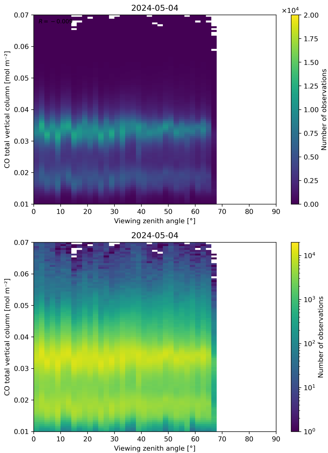
Figure 69: Scatter density plot of “Viewing zenith angle” against “CO total vertical column” for 2024-05-03 to 2024-05-05.
