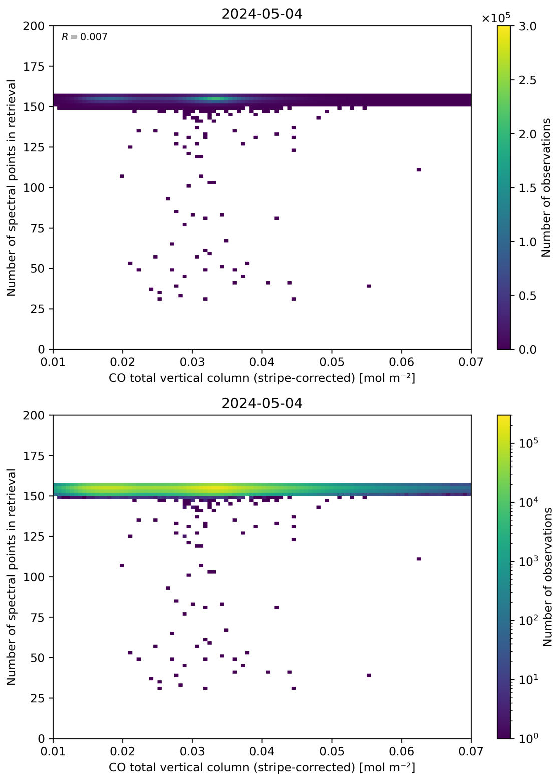
Figure 40: Scatter density plot of “CO total vertical column (stripe-corrected)” against “Number of spectral points in retrieval” for 2024-05-03 to 2024-05-05.
