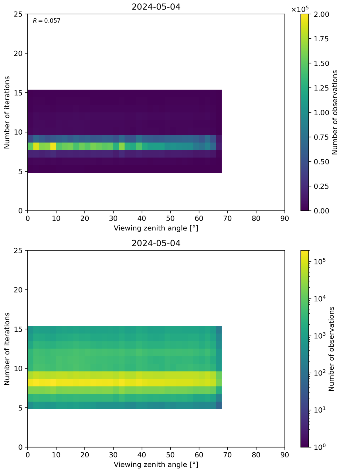
Figure 75: Scatter density plot of “Viewing zenith angle” against “Number of iterations” for 2024-05-03 to 2024-05-05.
