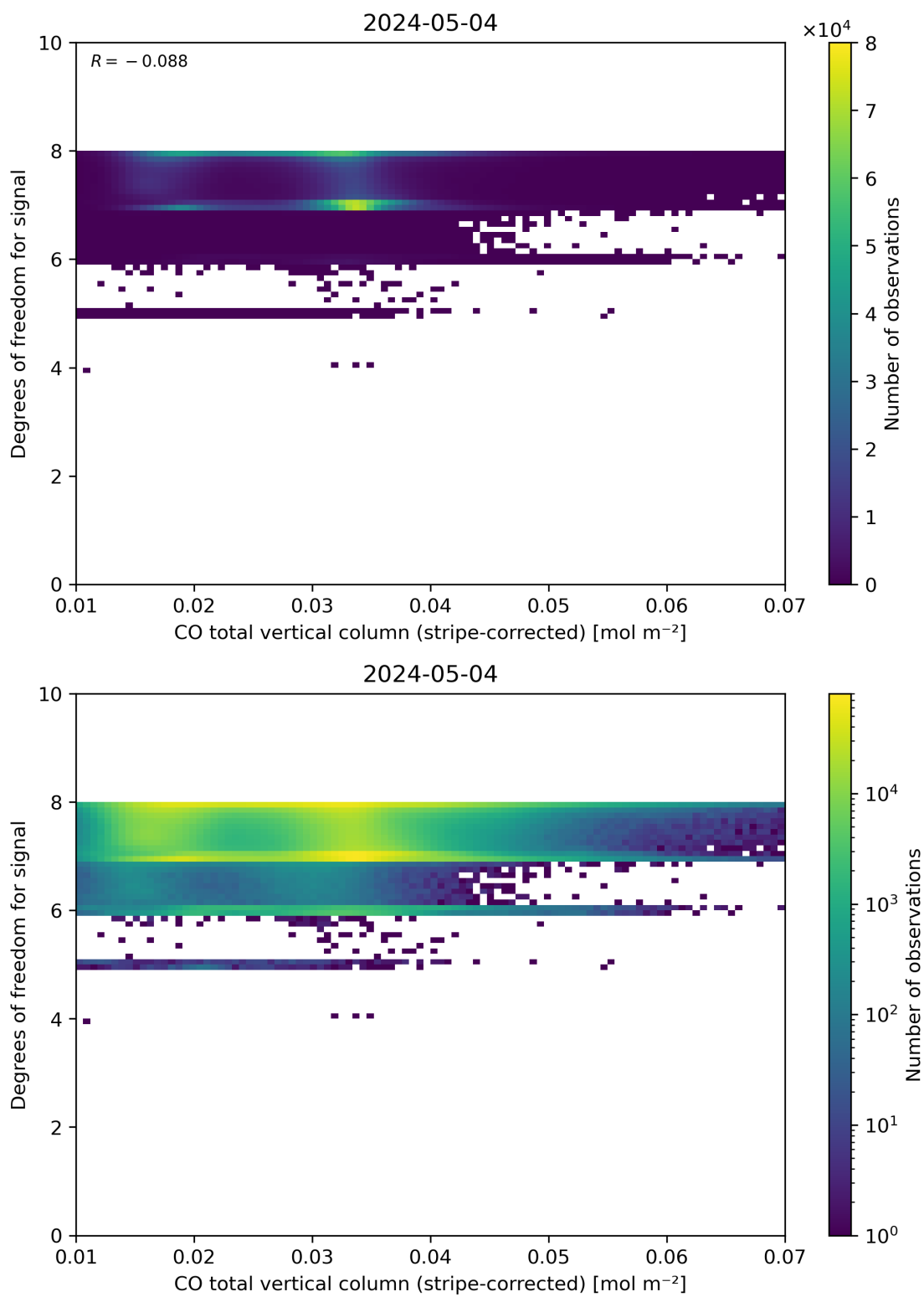
Figure 38: Scatter density plot of “CO total vertical column (stripe-corrected)” against “Degrees of freedom for signal” for 2024-05-03 to 2024-05-05.
