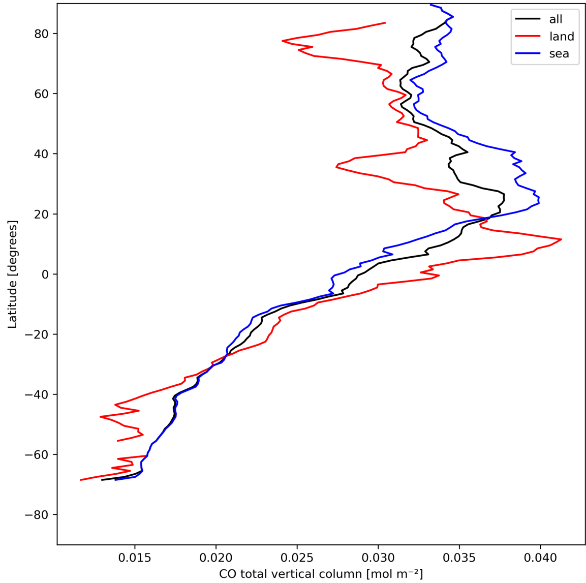
Figure 10: Zonal average of “CO total vertical column” for 2024-05-03 to 2024-05-05.
