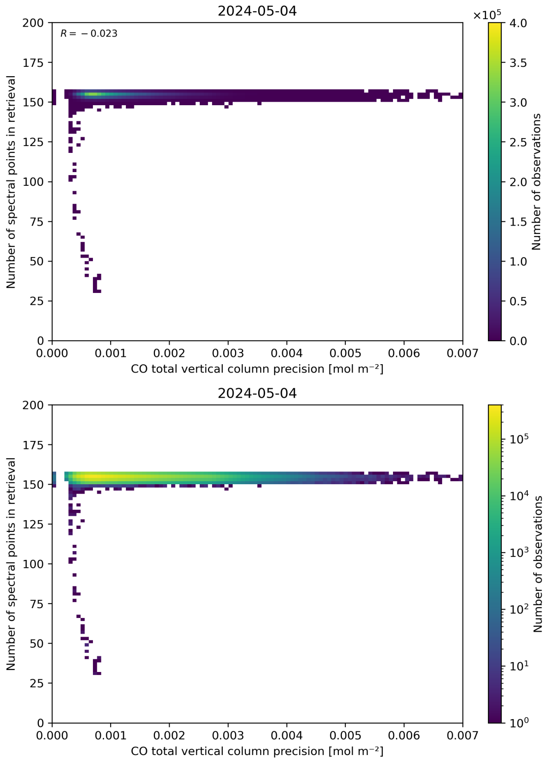
Figure 47: Scatter density plot of “CO total vertical column precision” against “Number of spectral points in retrieval” for 2024-05-03 to 2024-05-05.
