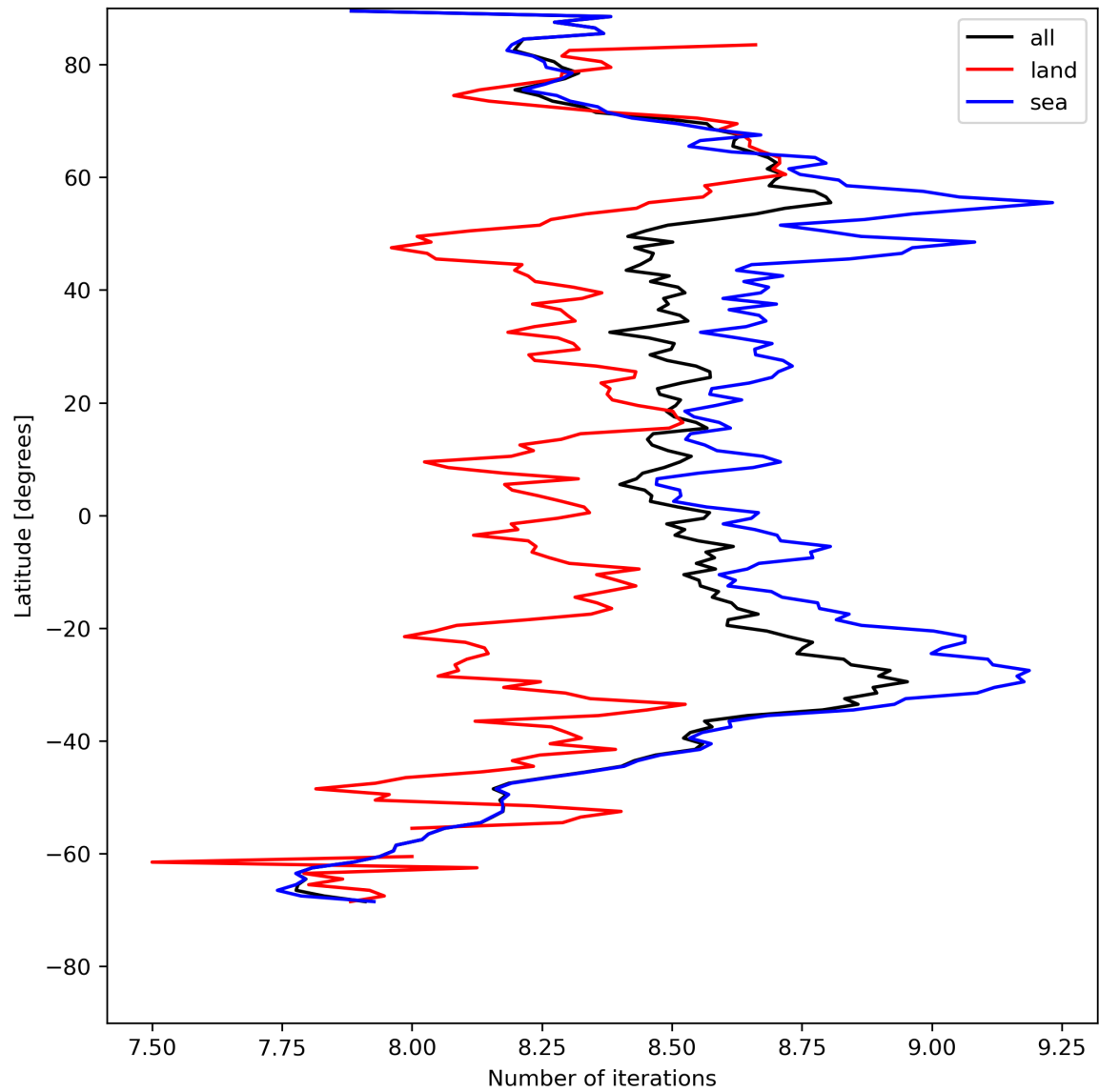
Figure 16: Zonal average of “Number of iterations” for 2024-05-03 to 2024-05-05.
