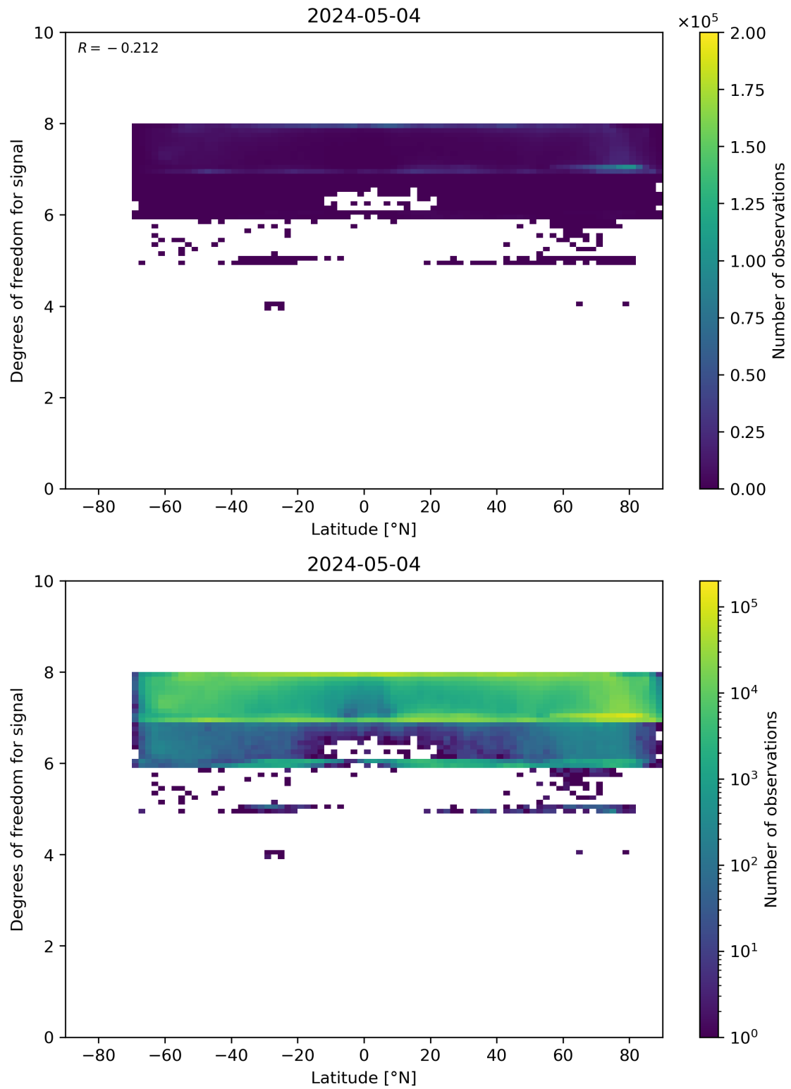
Figure 55: Scatter density plot of “Latitude” against “Degrees of freedom for signal” for 2024-05-03 to 2024-05-05.
