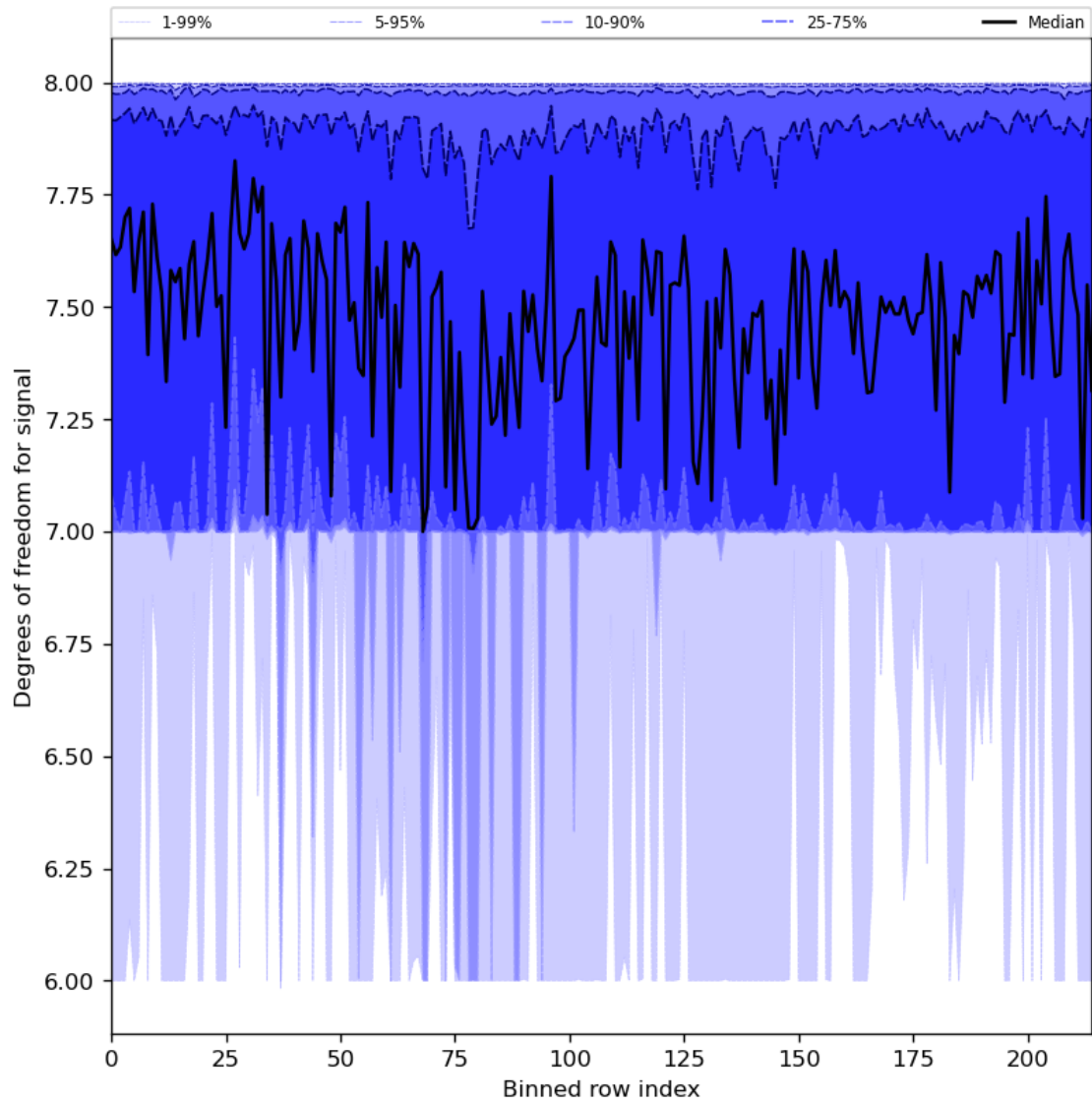
Figure 31: Along track statistics of “Degrees of freedom for signal” for 2024-05-03 to 2024-05-05
