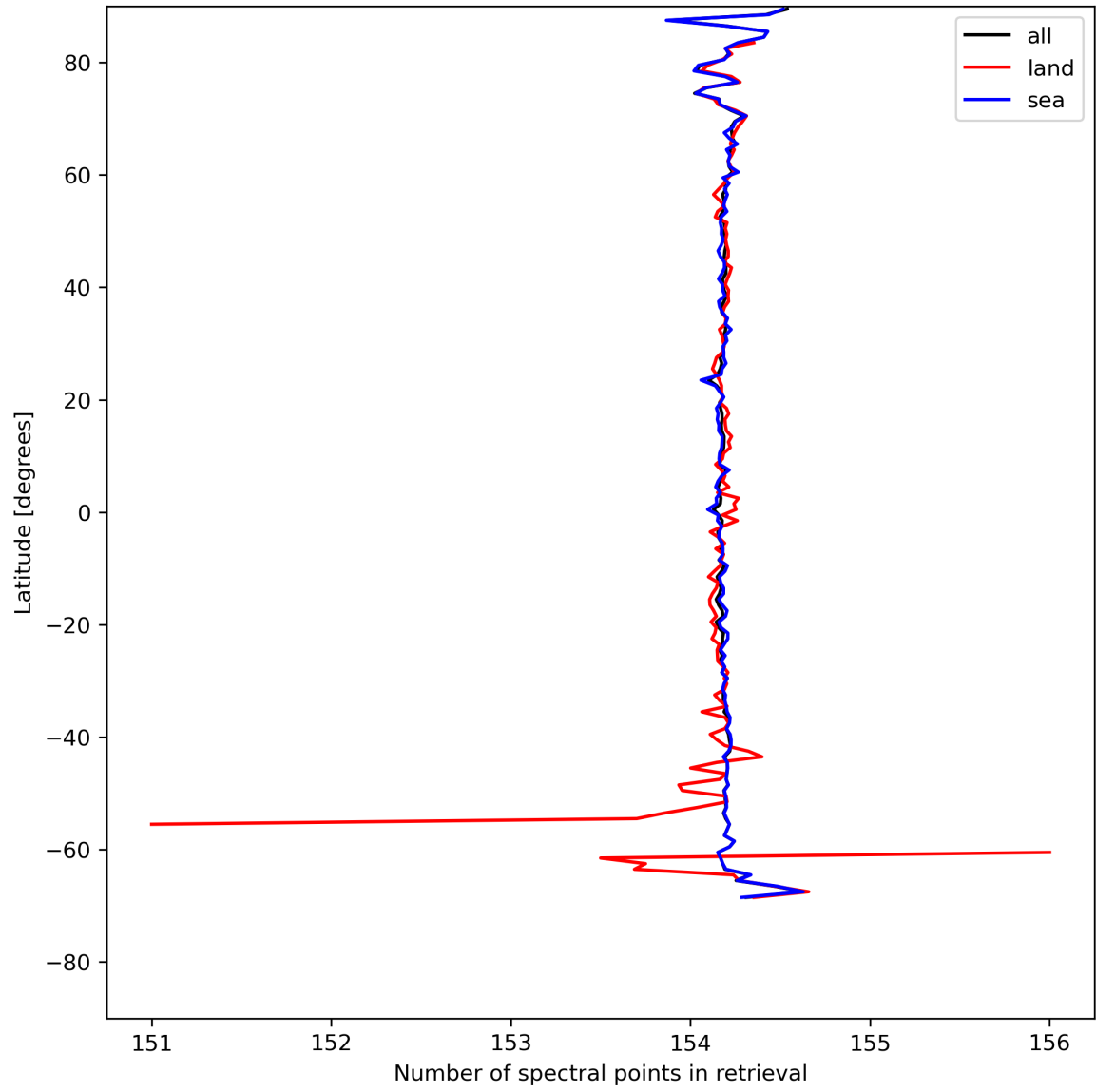
Figure 13: Zonal average of “Number of spectral points in retrieval” for 2024-05-03 to 2024-05-05.
