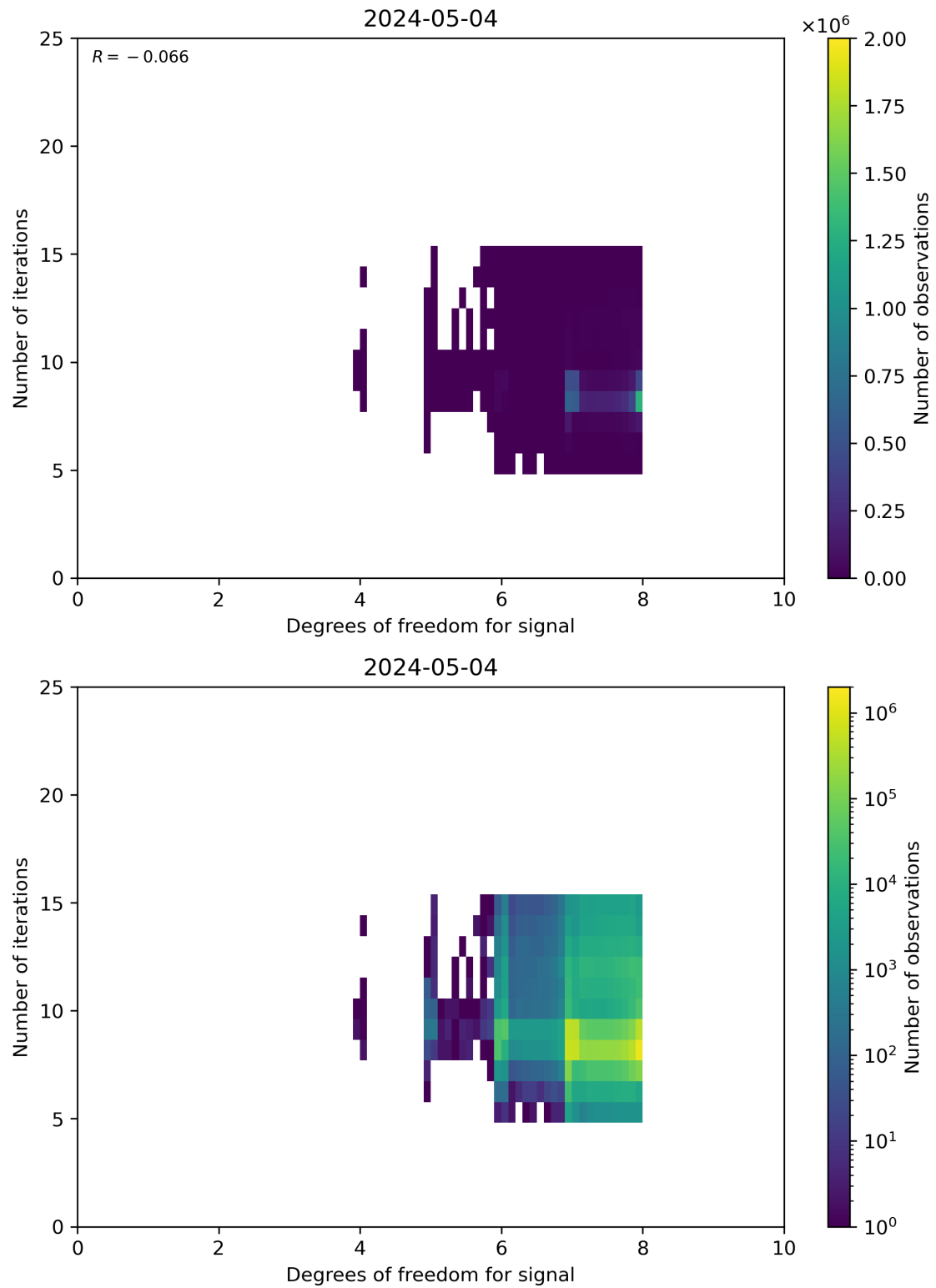
Figure 50: Scatter density plot of “Degrees of freedom for signal” against “Number of iterations” for 2024-05-03 to 2024-05-05.
