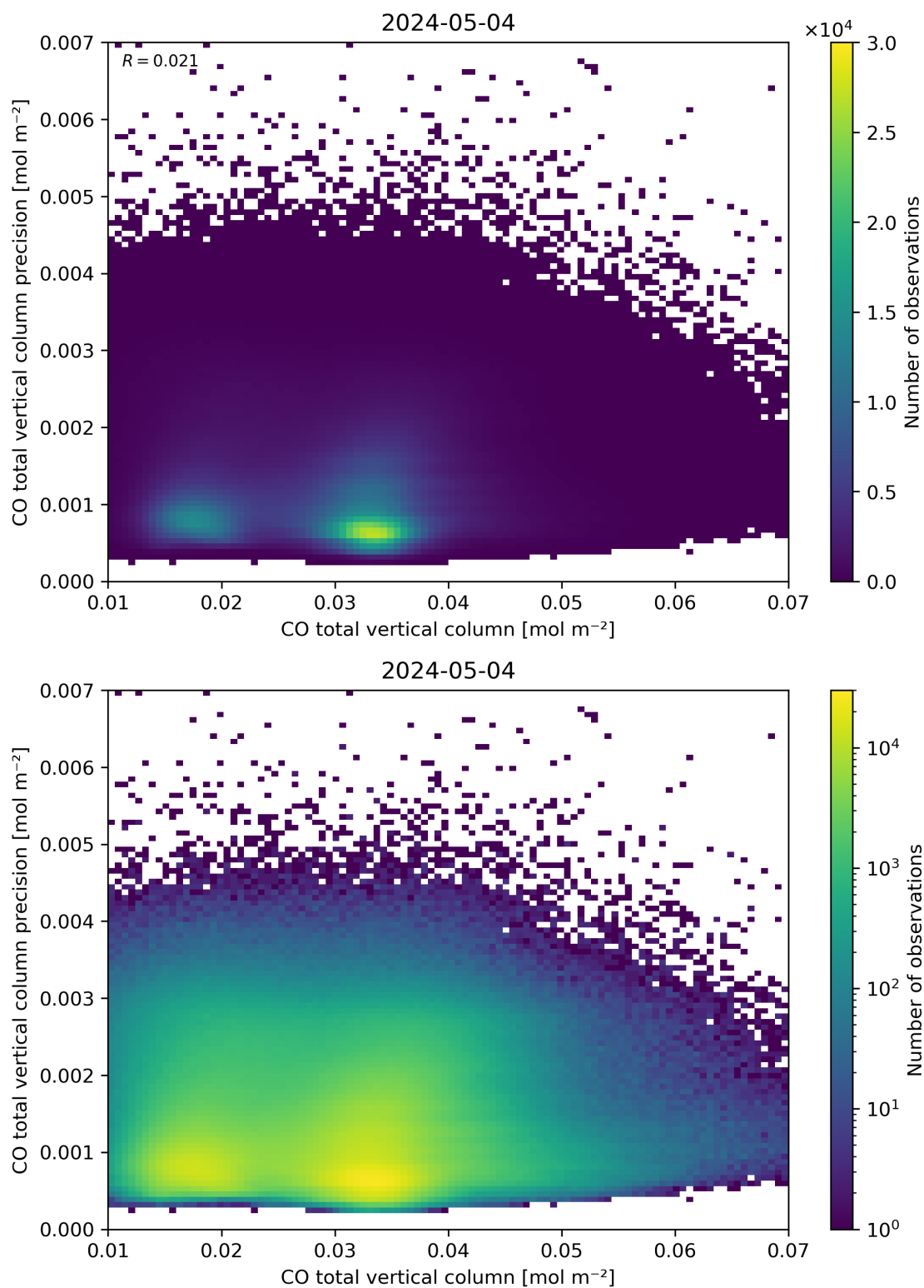
Figure 34: Scatter density plot of “CO total vertical column” against “CO total vertical column precision” for 2024-05-03 to 2024-05-05.
