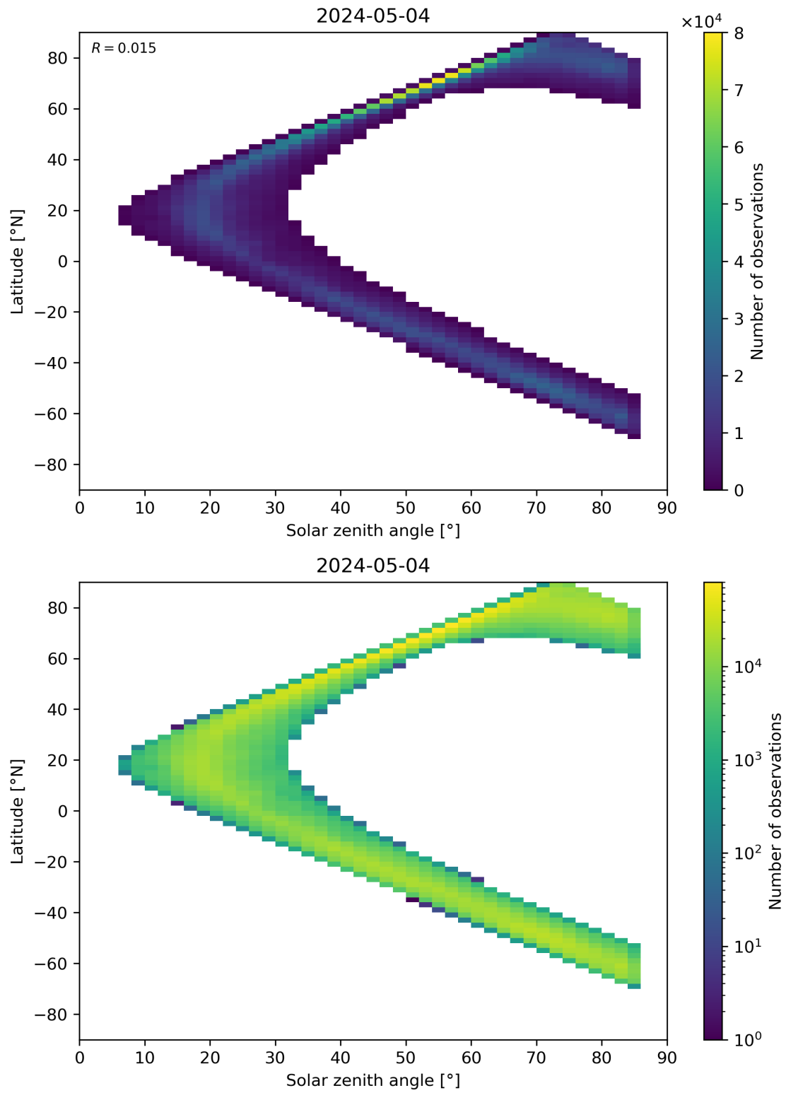
Figure 66: Scatter density plot of “Solar zenith angle” against “Latitude” for 2024-05-03 to 2024-05-05.
