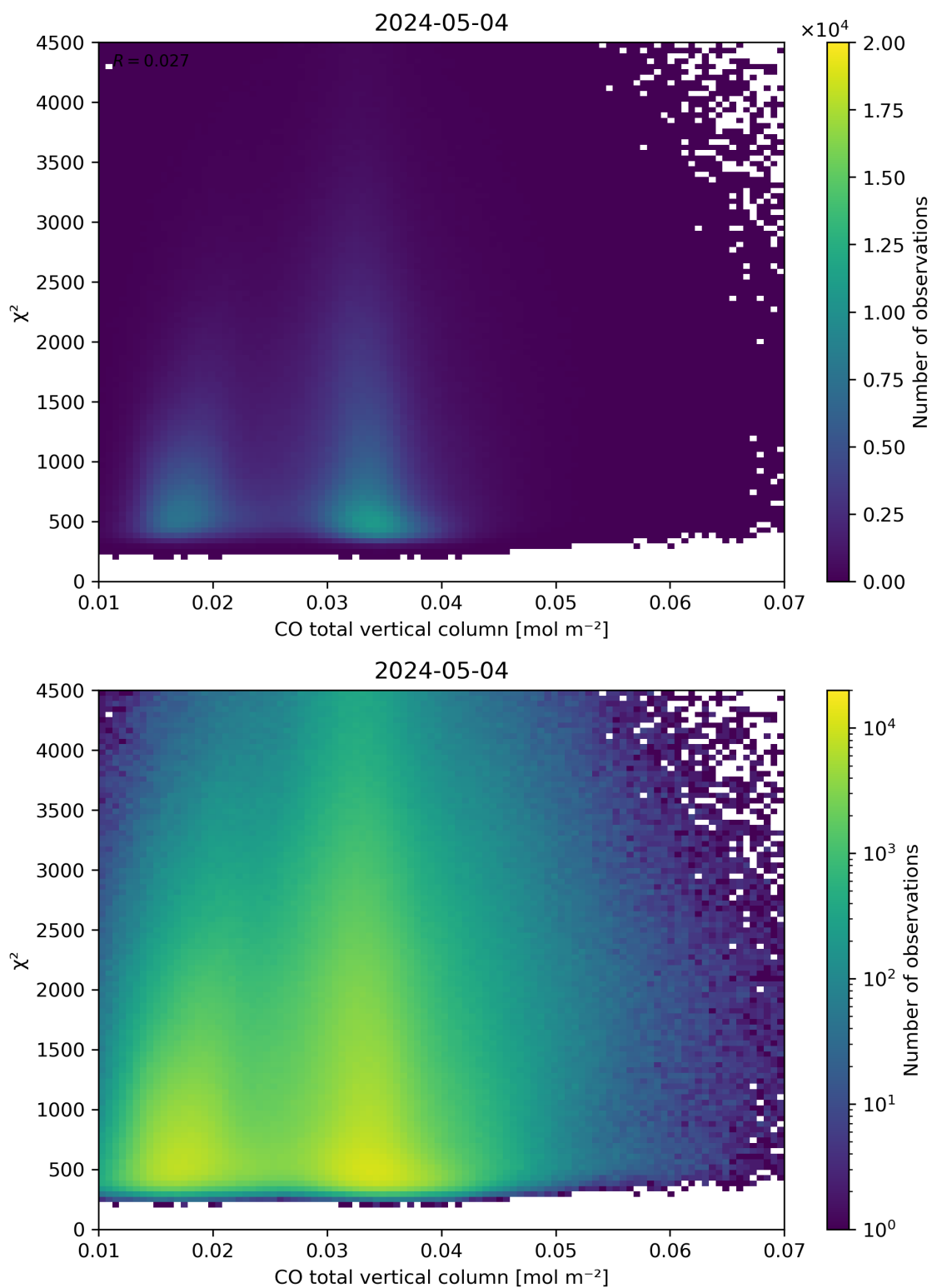
Figure 35: Scatter density plot of “CO total vertical column” against “ \chi^2 ” for 2024-05-03 to 2024-05-05.
