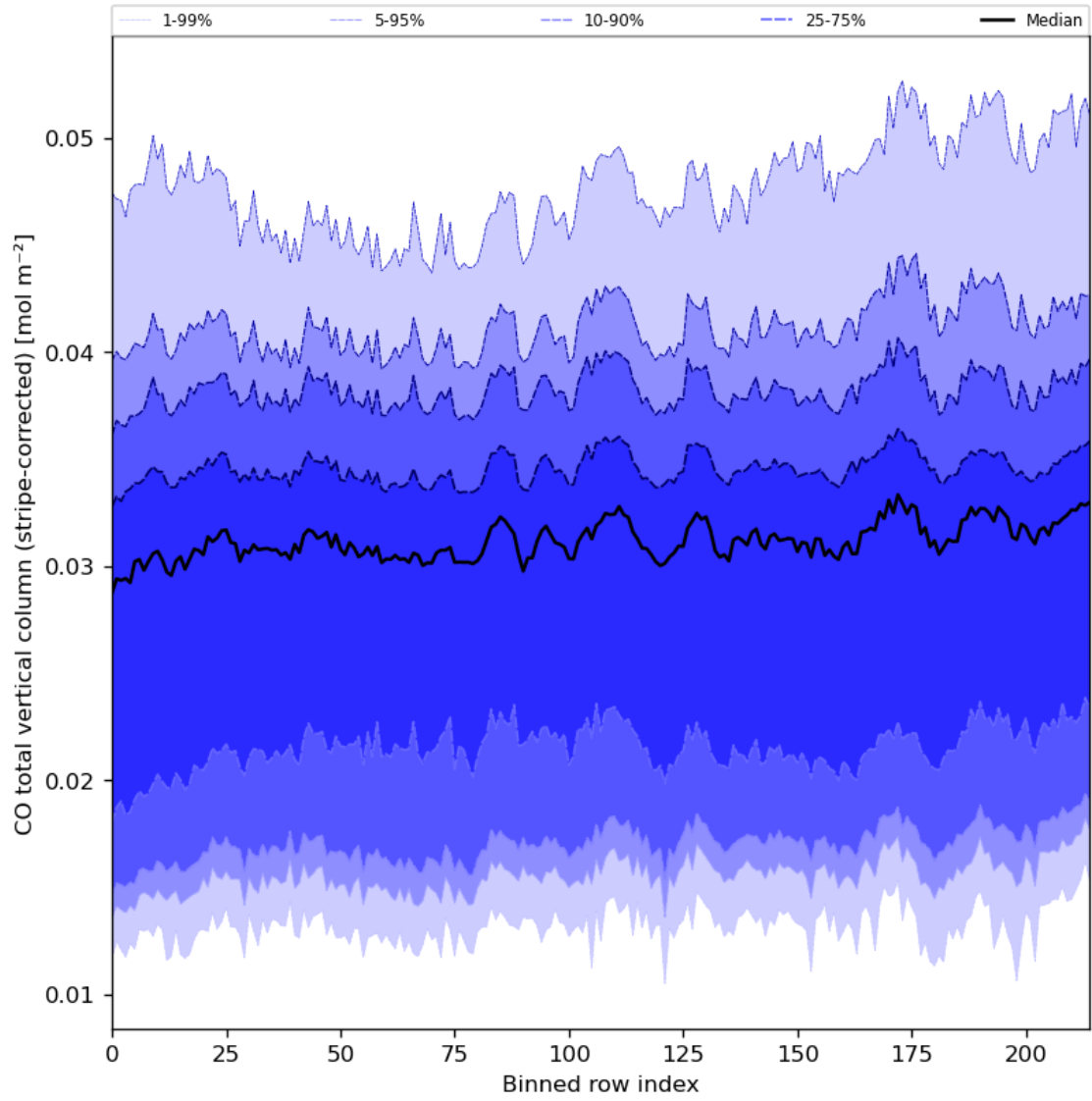
Figure 27: Along track statistics of “CO total vertical column (stripe-corrected)” for 2024-05-03 to 2024-05-05
