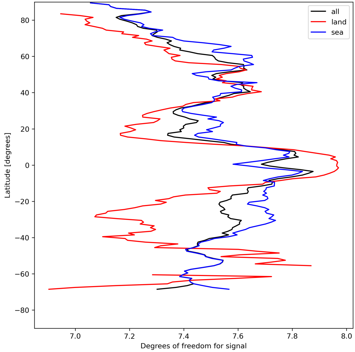
Figure 15: Zonal average of “Degrees of freedom for signal” for 2024-05-03 to 2024-05-05.
