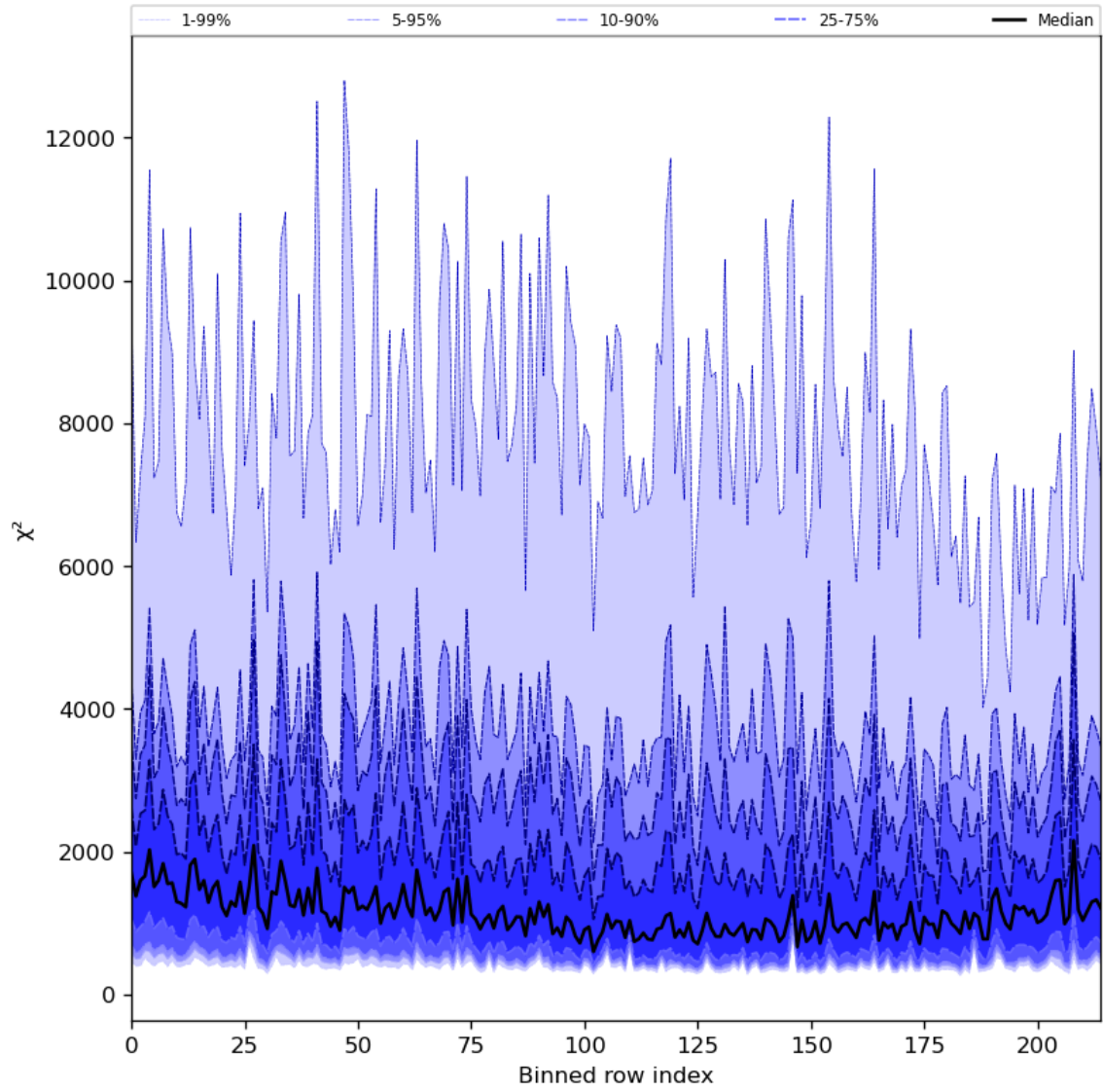
Figure 30: Along track statistics of “ \chi^2 ” for 2024-05-03 to 2024-05-05
