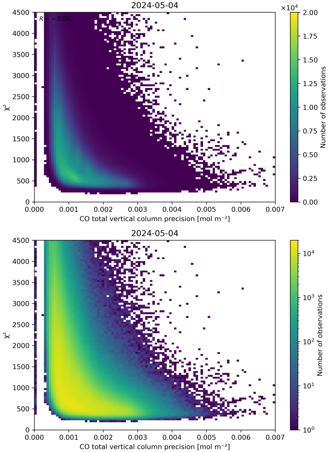
Figure 44: Scatter density plot of “CO total vertical column precision” against “ \chi^2 ” for 2024-05-03 to 2024-05-05.
