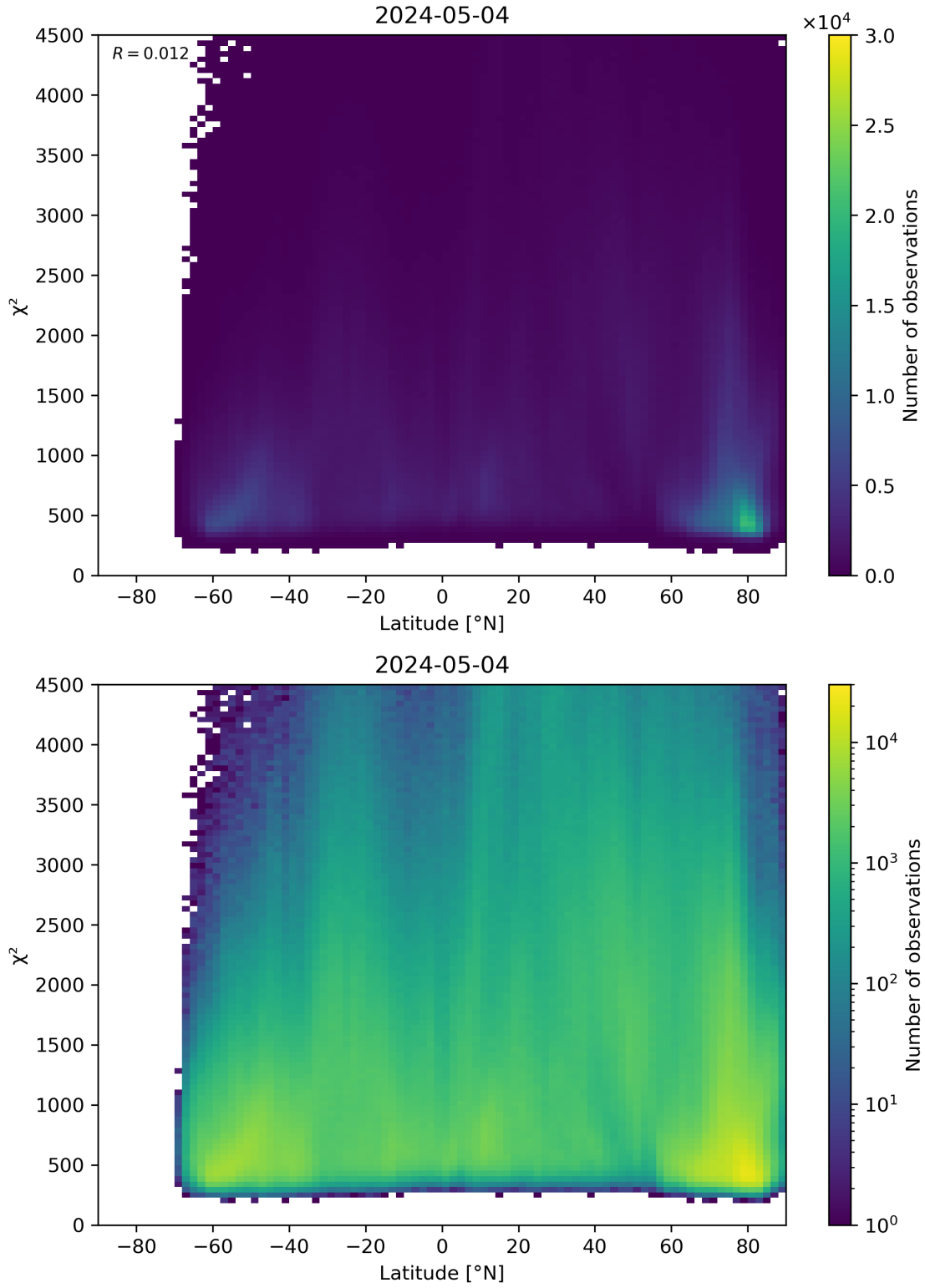
Figure 54: Scatter density plot of “Latitude” against “ \chi^2 ” for 2024-05-03 to 2024-05-05.
