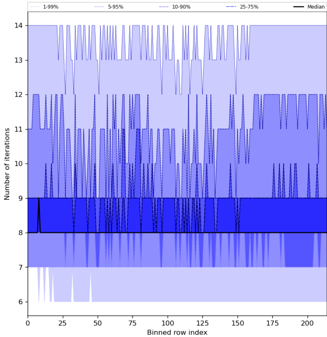
Figure 32: Along track statistics of “Number of iterations” for 2024-05-03 to 2024-05-05
