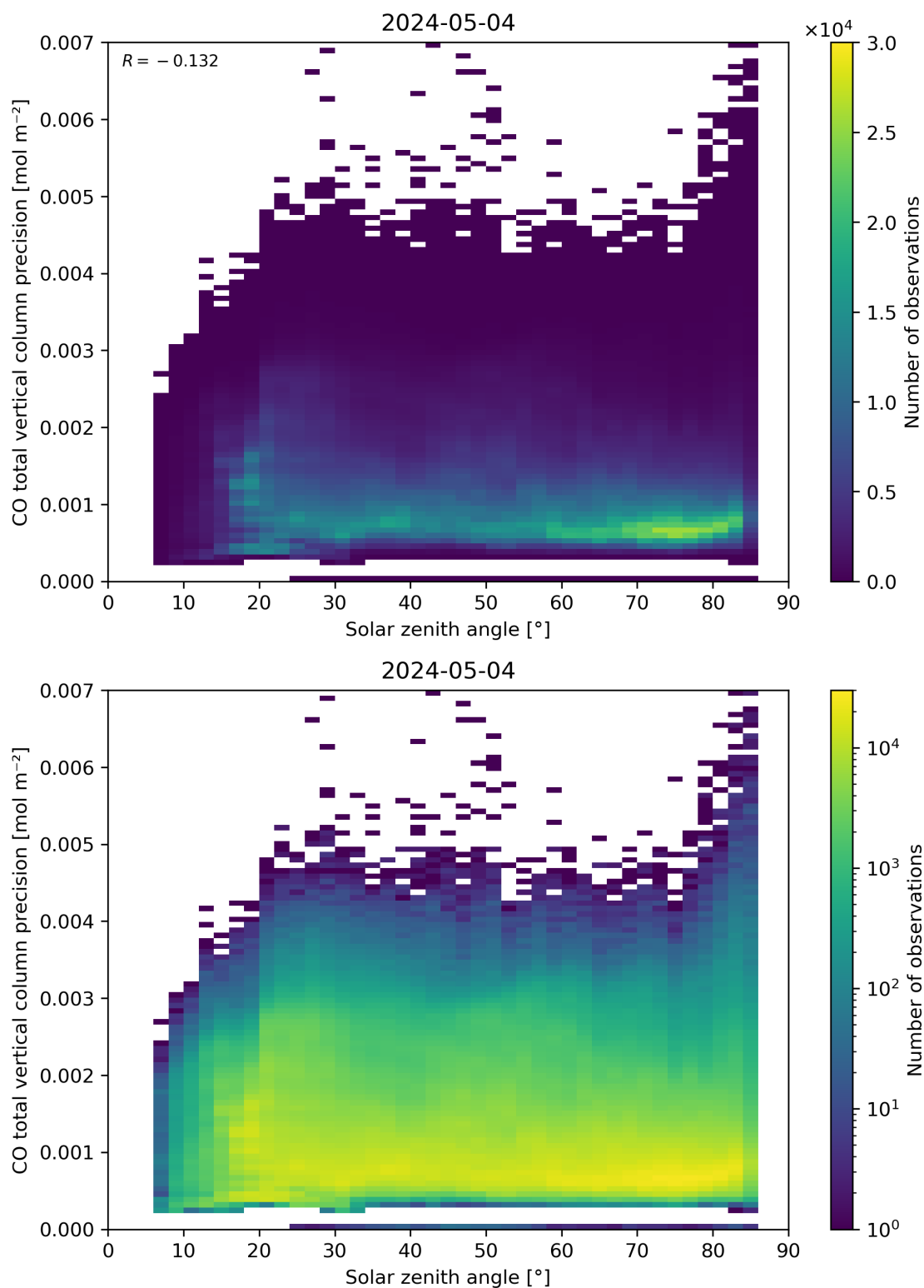
Figure 63: Scatter density plot of “Solar zenith angle” against “CO total vertical column precision” for 2024-05-03 to 2024-05-05.
