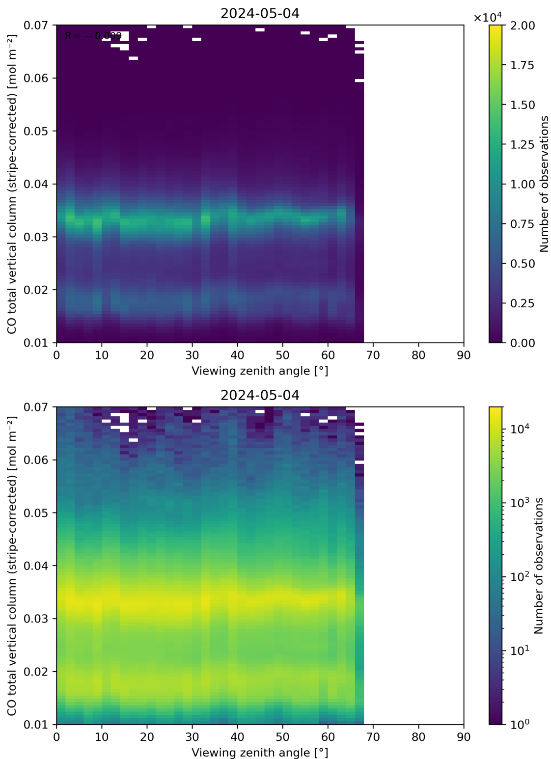
Figure 70: Scatter density plot of “Viewing zenith angle” against “CO total vertical column (stripe-corrected)” for 2024-05-03 to 2024-05-05.
