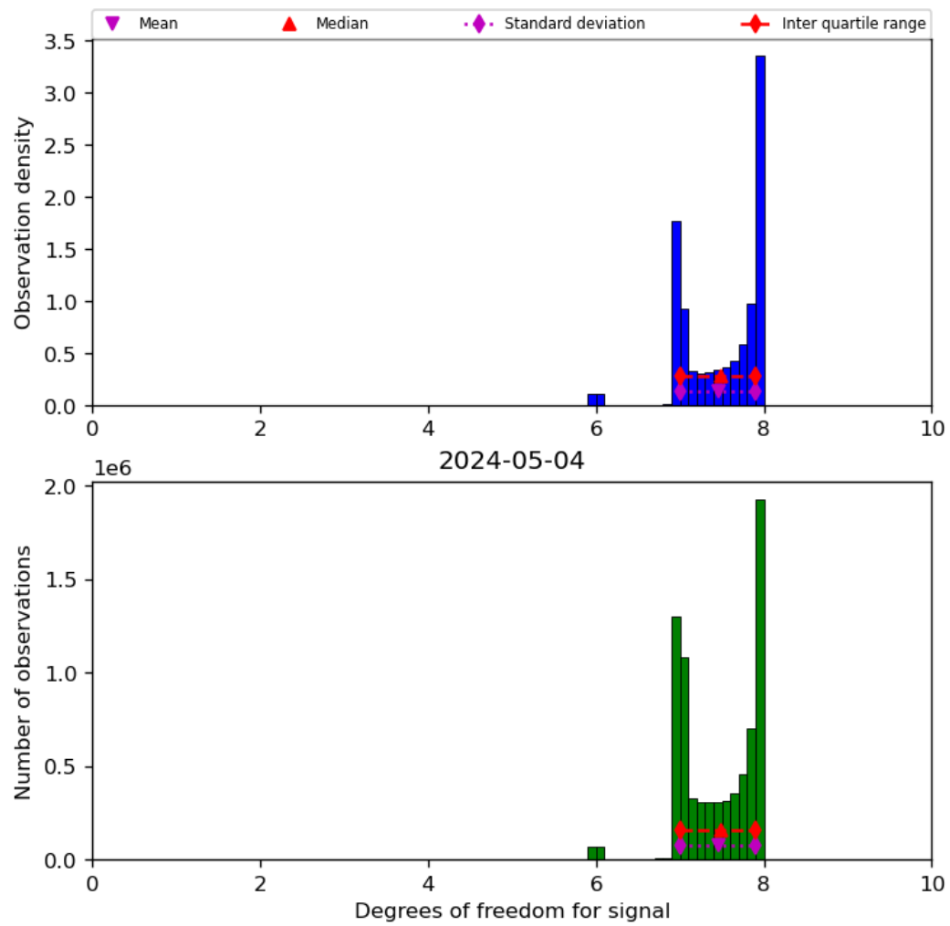
Figure 23: Histogram of “Degrees of freedom for signal” for 2024-05-03 to 2024-05-05
