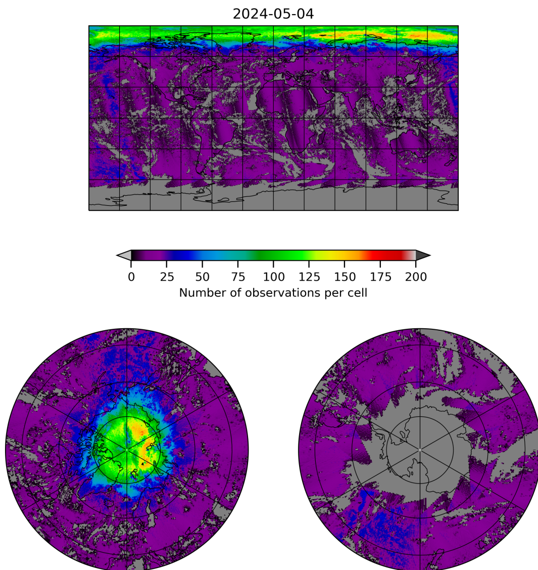
Figure 8: Map of the number of observations for 2024-05-03 to 2024-05-05
