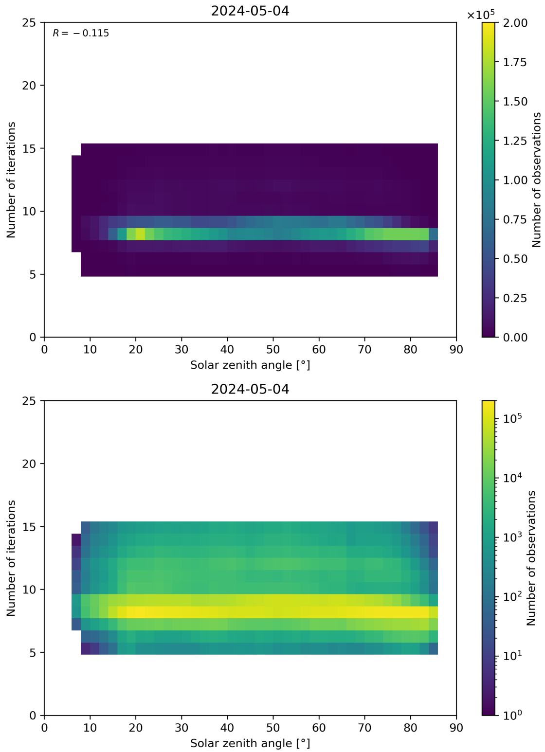
Figure 67: Scatter density plot of “Solar zenith angle” against “Number of iterations” for 2024-05-03 to 2024-05-05.
