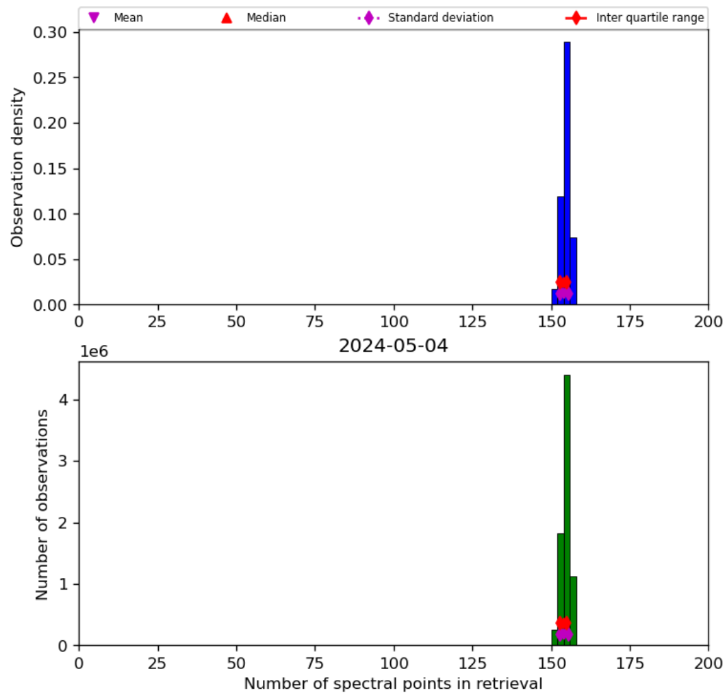
Figure 21: Histogram of “Number of spectral points in retrieval” for 2024-05-03 to 2024-05-05
