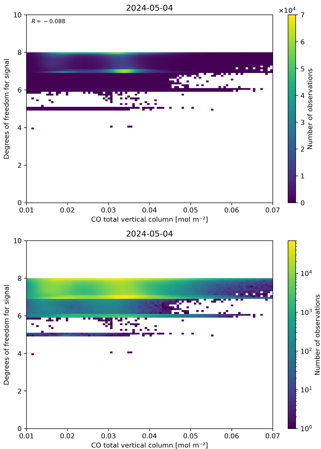
Figure 41: Scatter density plot of “CO total vertical column” against “Degrees of freedom for signal” for 2024-05-03 to 2024-05-05.
