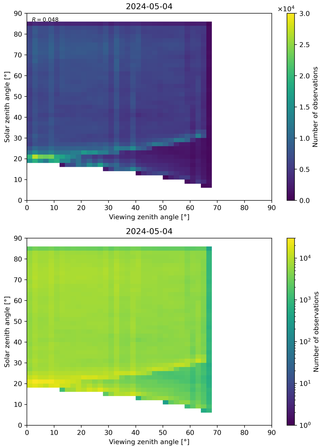
Figure 77: Scatter density plot of “Viewing zenith angle” against “Solar zenith angle” for 2024-05-03 to 2024-05-05.
