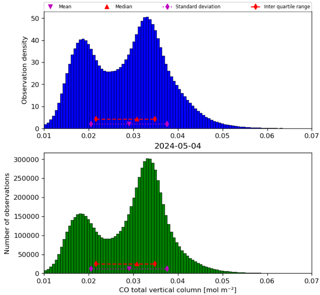
Figure 18: Histogram of “CO total vertical column” for 2024-05-03 to 2024-05-05
