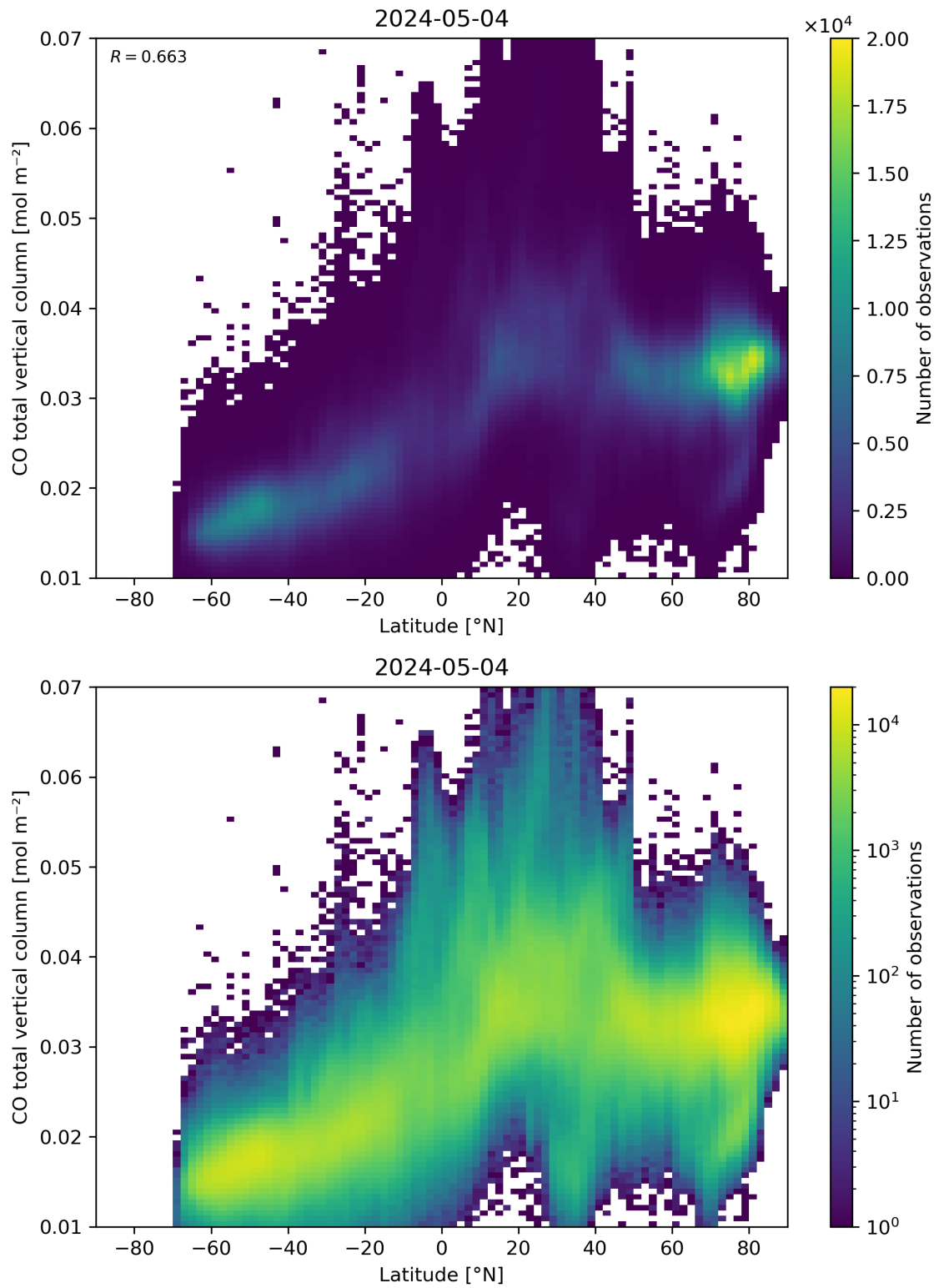
Figure 51: Scatter density plot of “Latitude” against “CO total vertical column” for 2024-05-03 to 2024-05-05.
