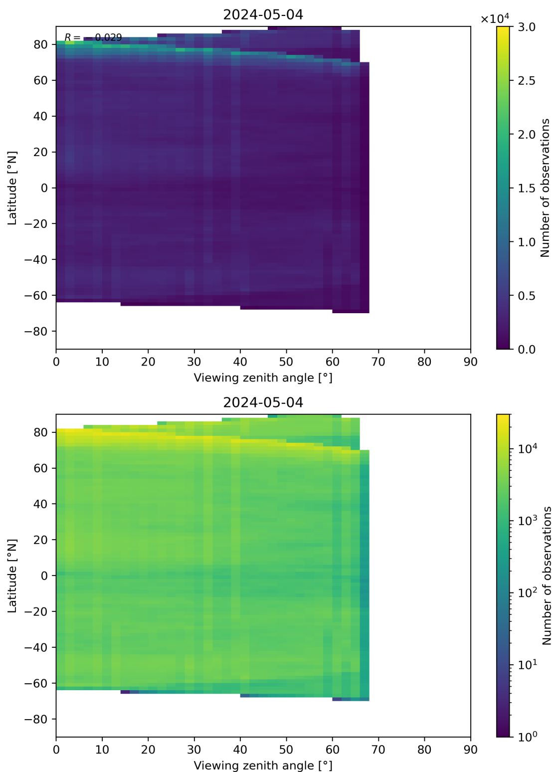
Figure 74: Scatter density plot of “Viewing zenith angle” against “Latitude” for 2024-05-03 to 2024-05-05.
