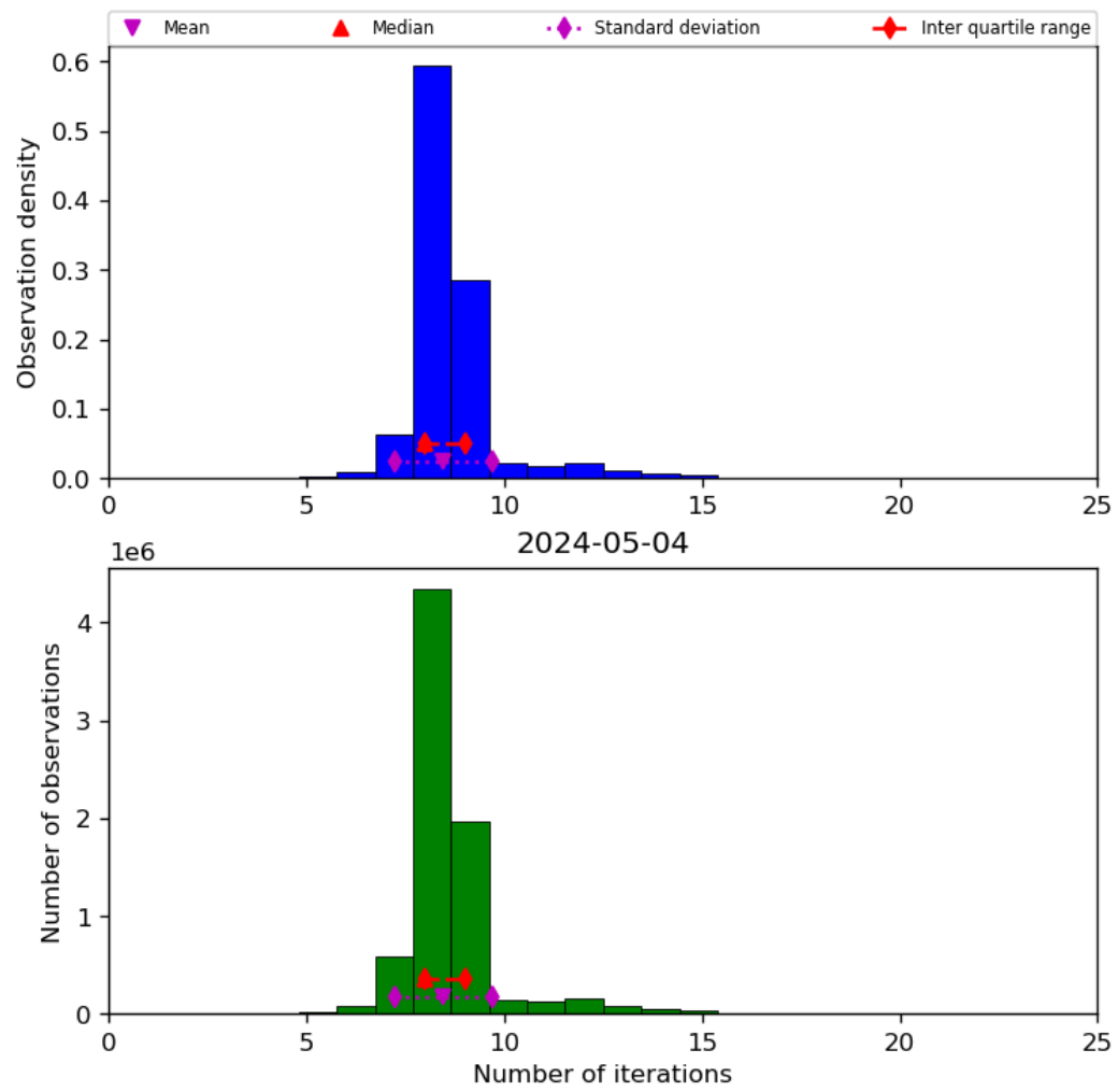
Figure 24: Histogram of "Number of iterations" for 2024-05-03 to 2024-05-05
