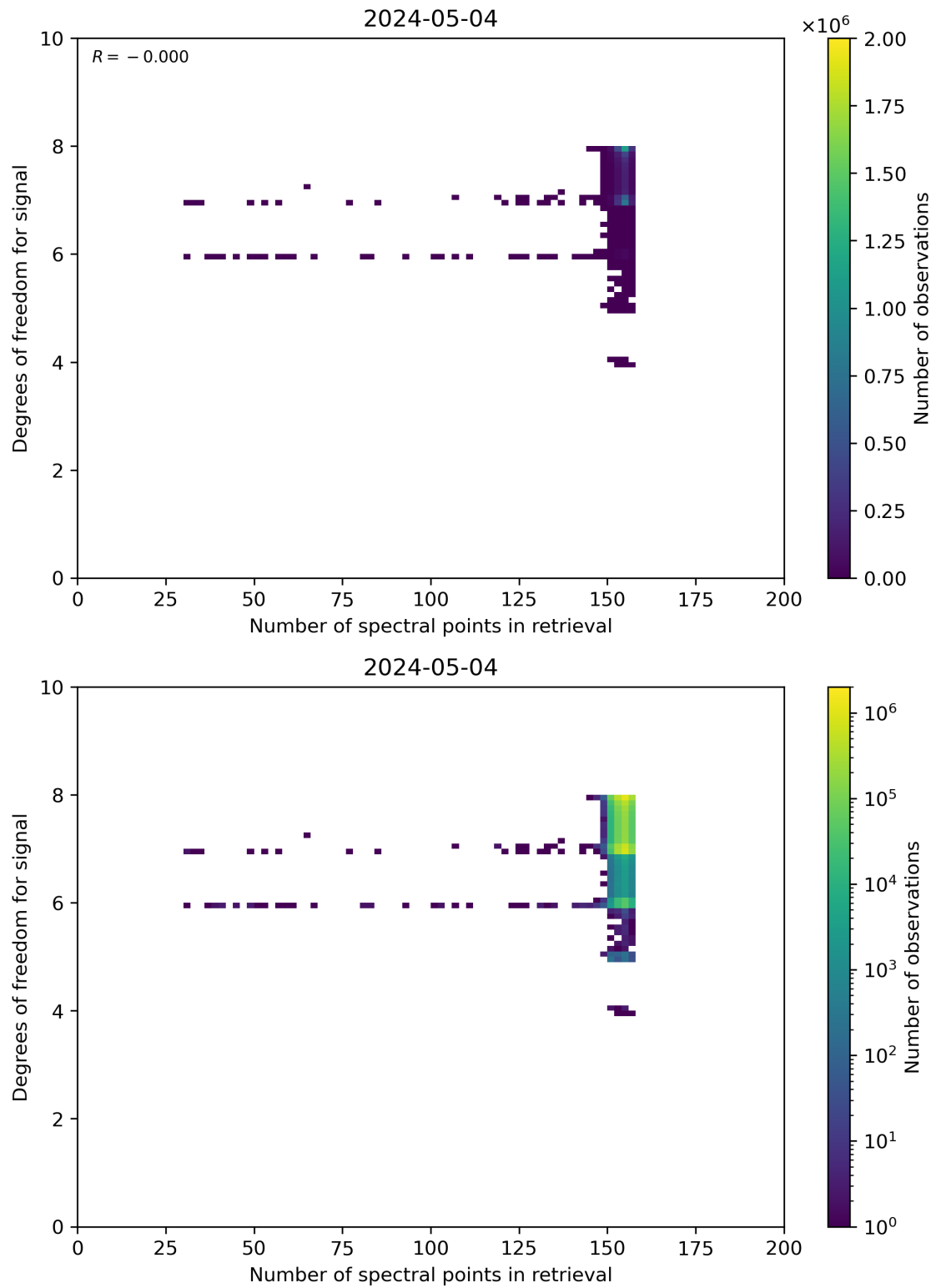
Figure 59: Scatter density plot of “Number of spectral points in retrieval” against “Degrees of freedom for signal” for 2024-05-03 to 2024-05-05.
