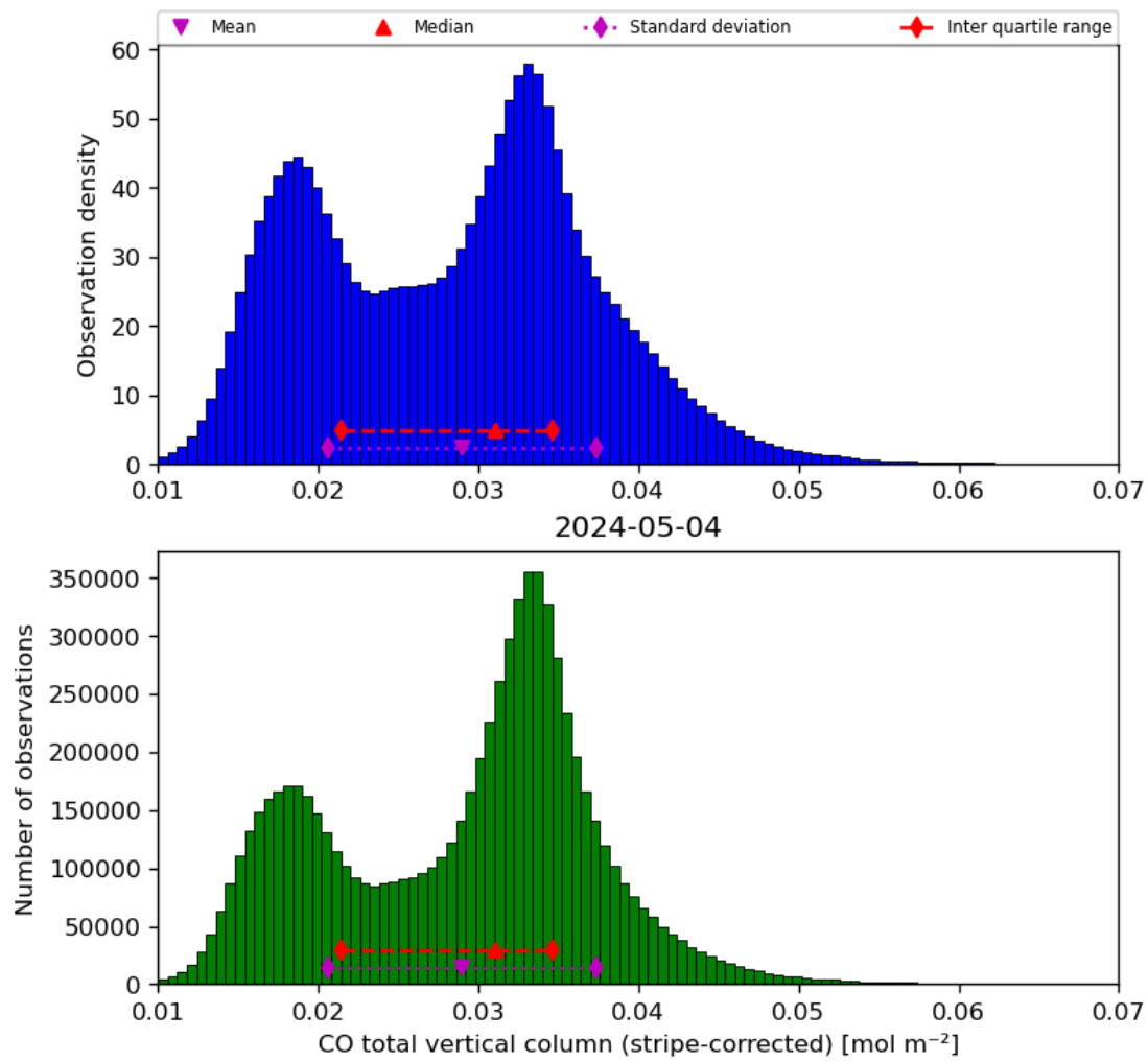
Figure 19: Histogram of “CO total vertical column (stripe-corrected)” for 2024-05-03 to 2024-05-05
