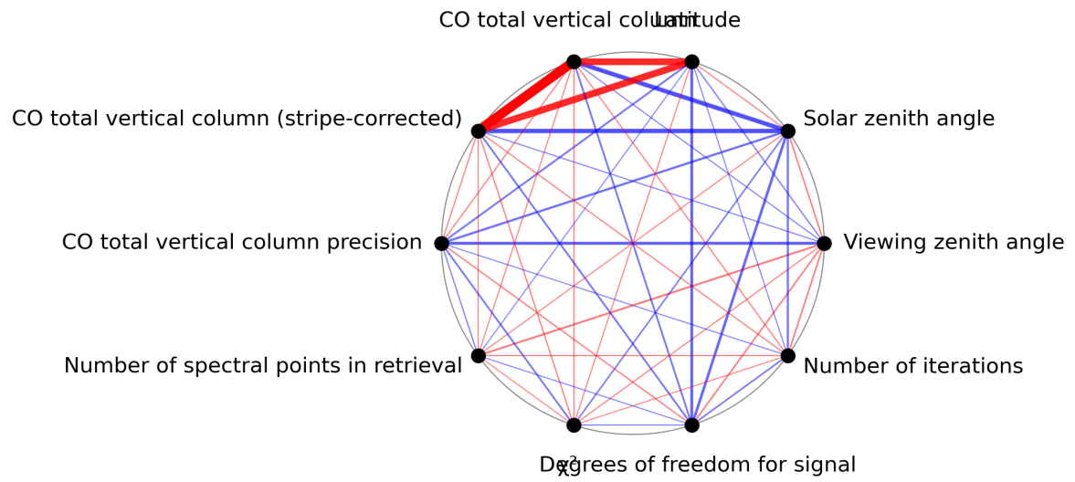
Figure 1: Map of correlation graph for 2024-05-03 to 2024-05-05.
