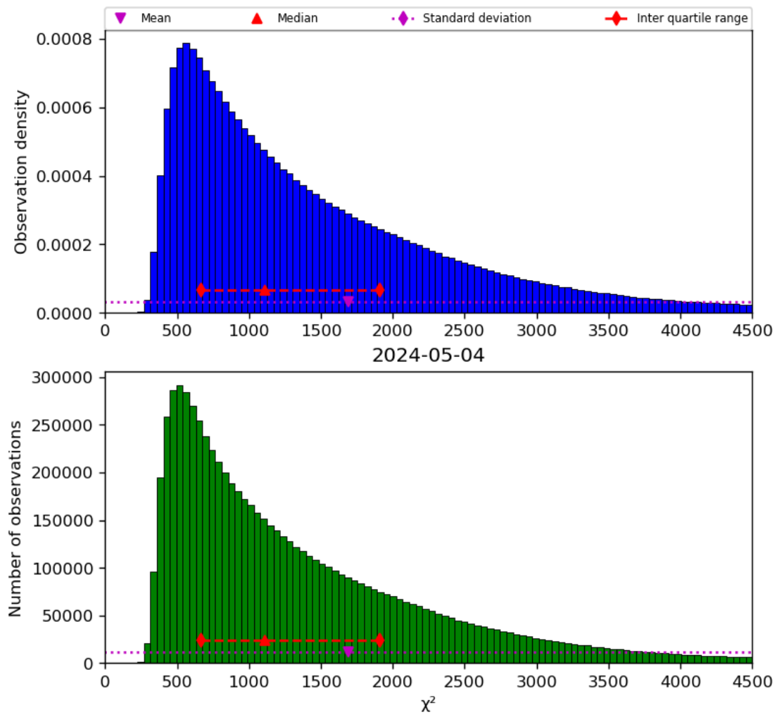
Figure 22: Histogram of “ \chi^2 ” for 2024-05-03 to 2024-05-05
