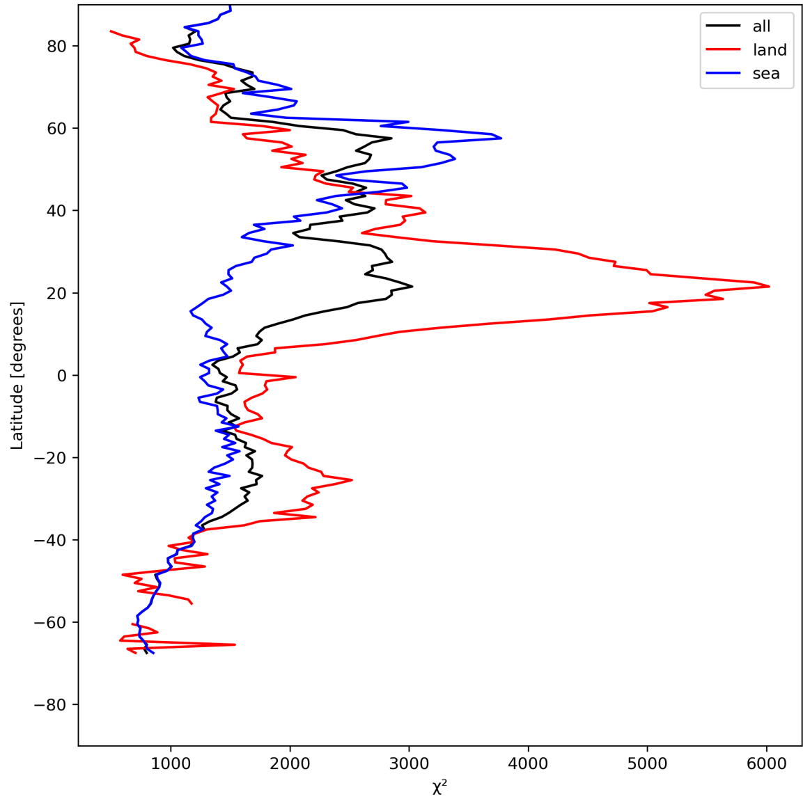
Figure 14: Zonal average of “ \chi^2 ” for 2024-05-05 to 2024-05-07.
