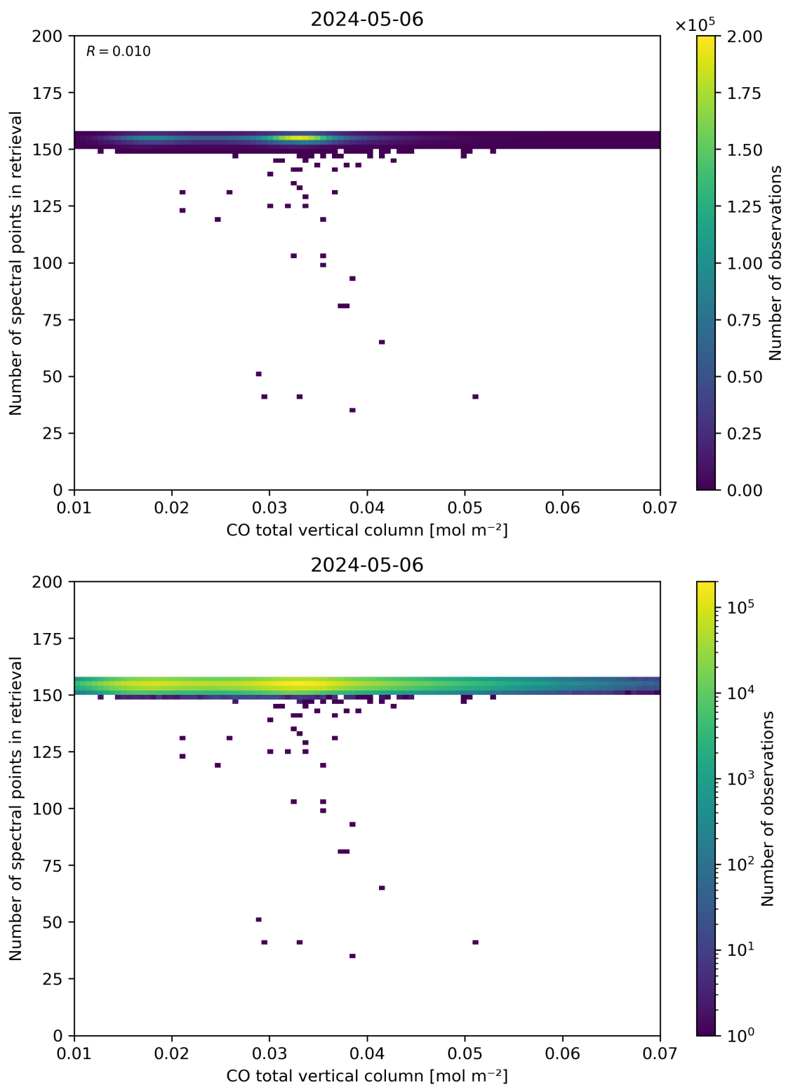
Figure 43: Scatter density plot of “CO total vertical column” against “Number of spectral points in retrieval” for 2024-05-05 to 2024-05-07.
