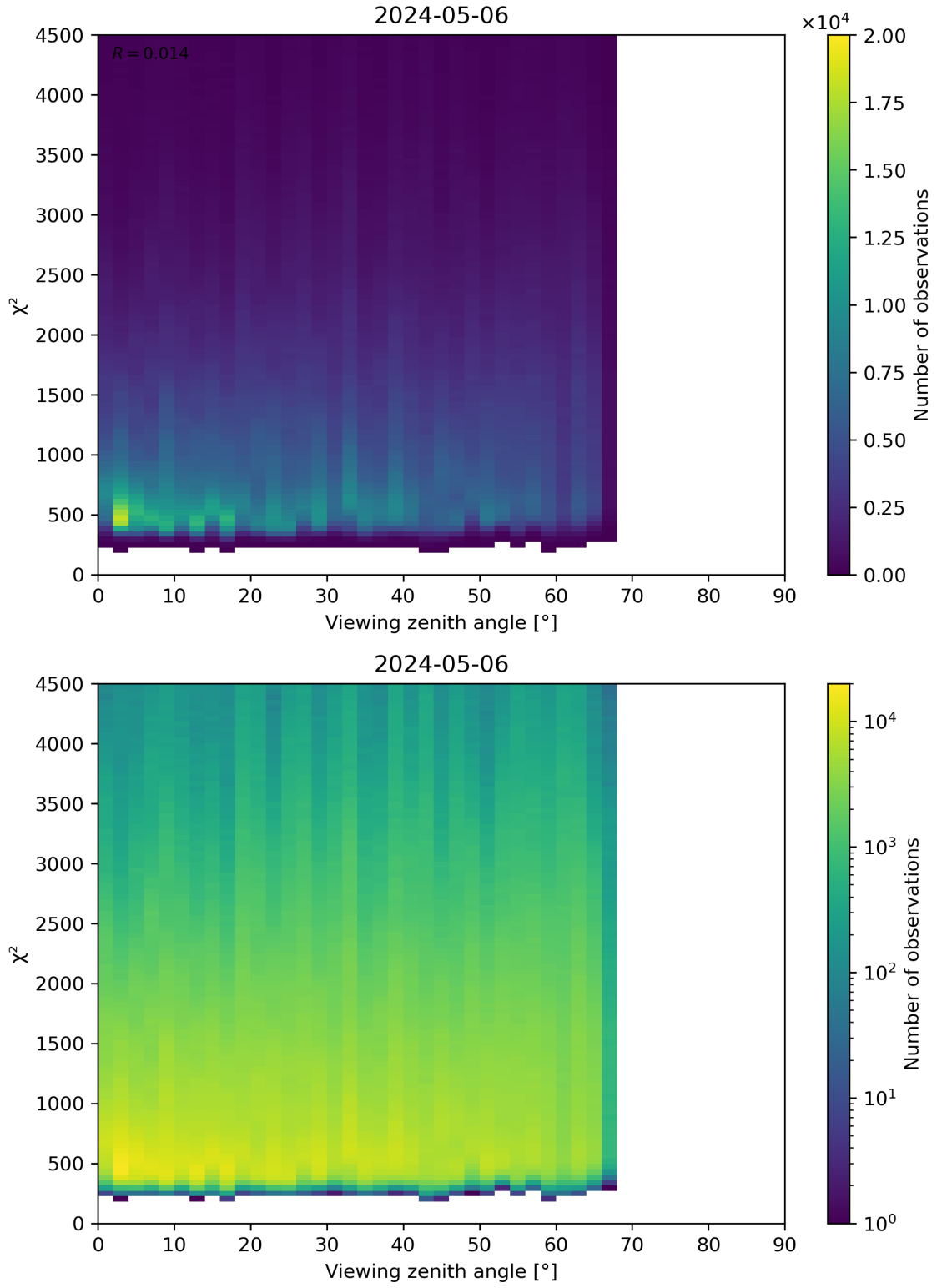
Figure 72: Scatter density plot of “Viewing zenith angle” against “ \chi^2 ” for 2024-05-05 to 2024-05-07.
