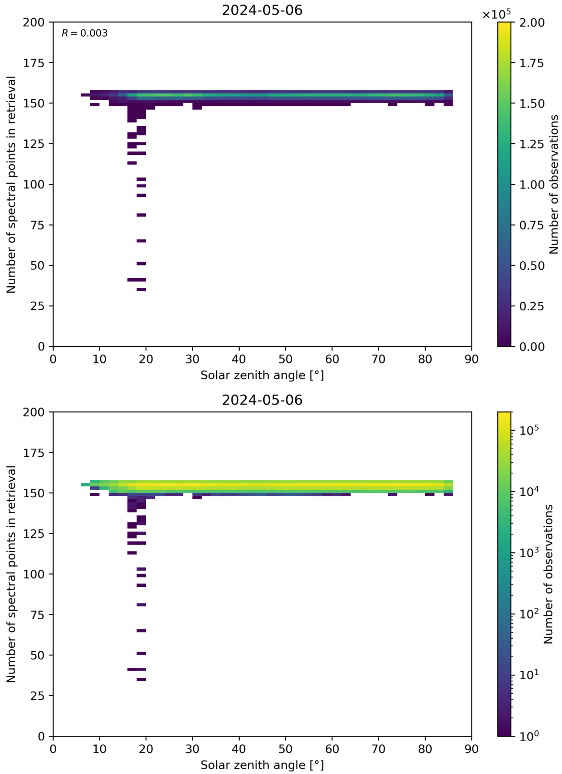
Figure 68: Scatter density plot of “Solar zenith angle” against “Number of spectral points in retrieval” for 2024-05-05 to 2024-05-07.
