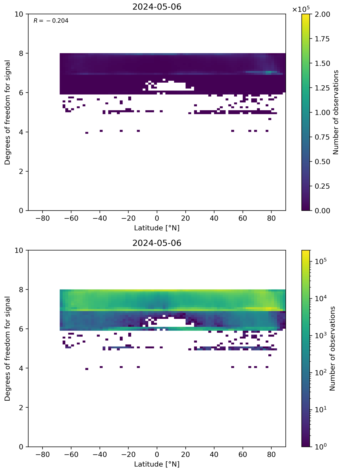
Figure 55: Scatter density plot of “Latitude” against “Degrees of freedom for signal” for 2024-05-05 to 2024-05-07.
