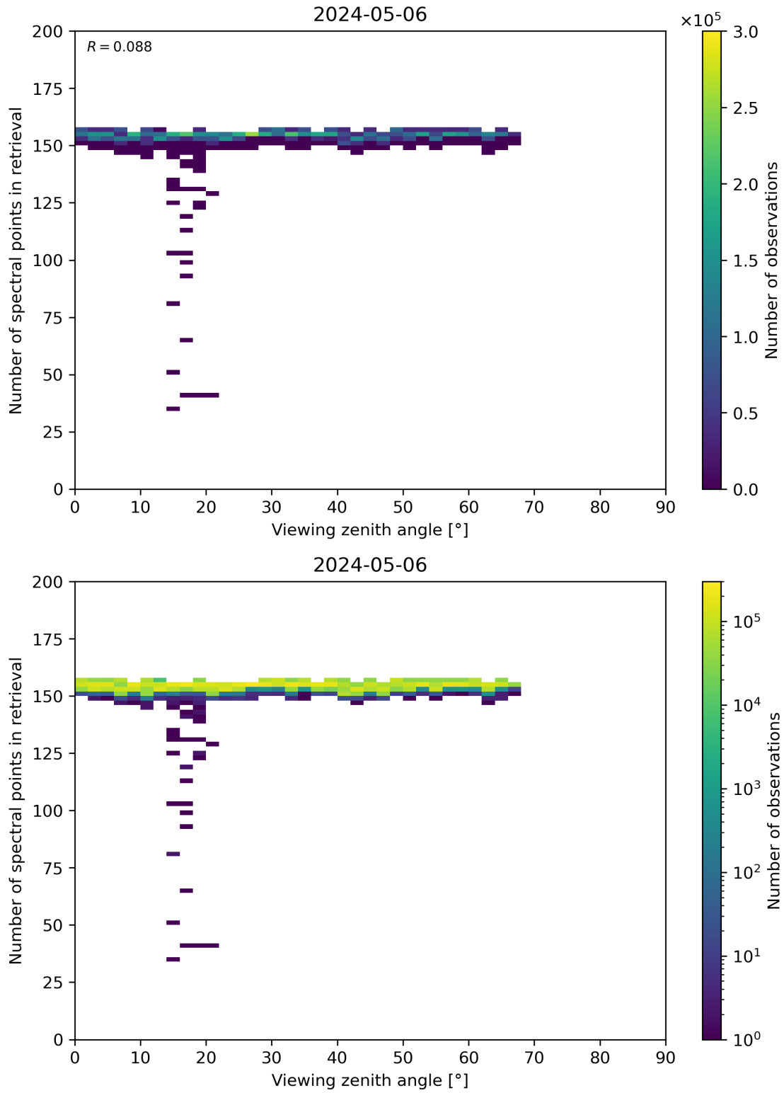
Figure 76: Scatter density plot of “Viewing zenith angle” against “Number of spectral points in retrieval” for 2024-05-05 to 2024-05-07.
