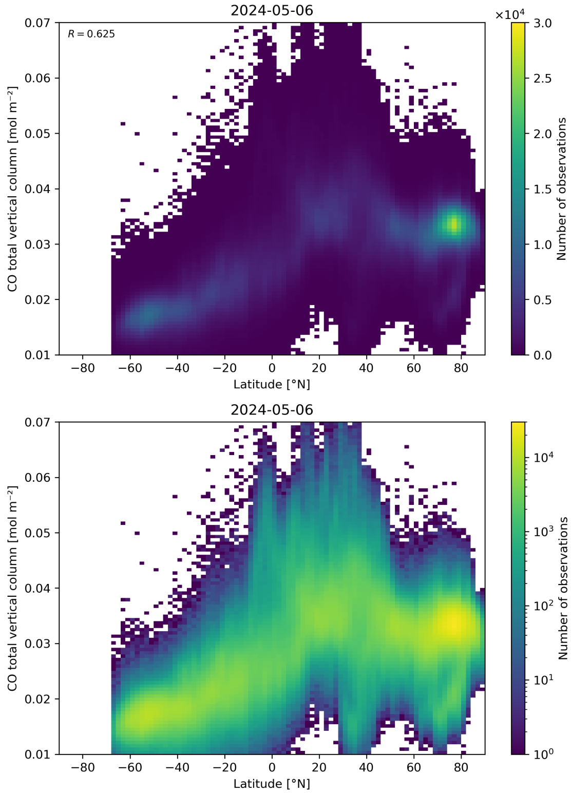
Figure 51: Scatter density plot of “Latitude” against “CO total vertical column” for 2024-05-05 to 2024-05-07.
