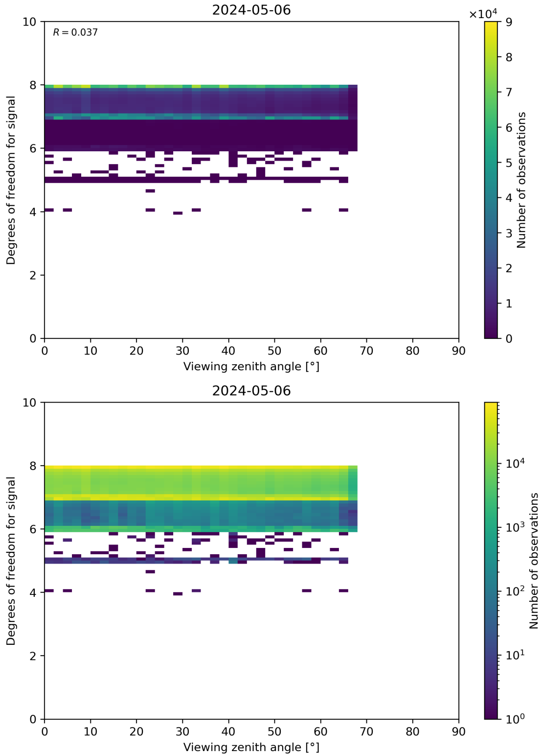
Figure 73: Scatter density plot of “Viewing zenith angle” against “Degrees of freedom for signal” for 2024-05-05 to 2024-05-07.
