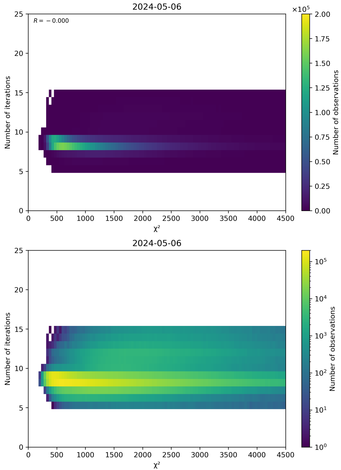
Figure 49: Scatter density plot of “ \chi^2 ” against “Number of iterations” for 2024-05-05 to 2024-05-07.
