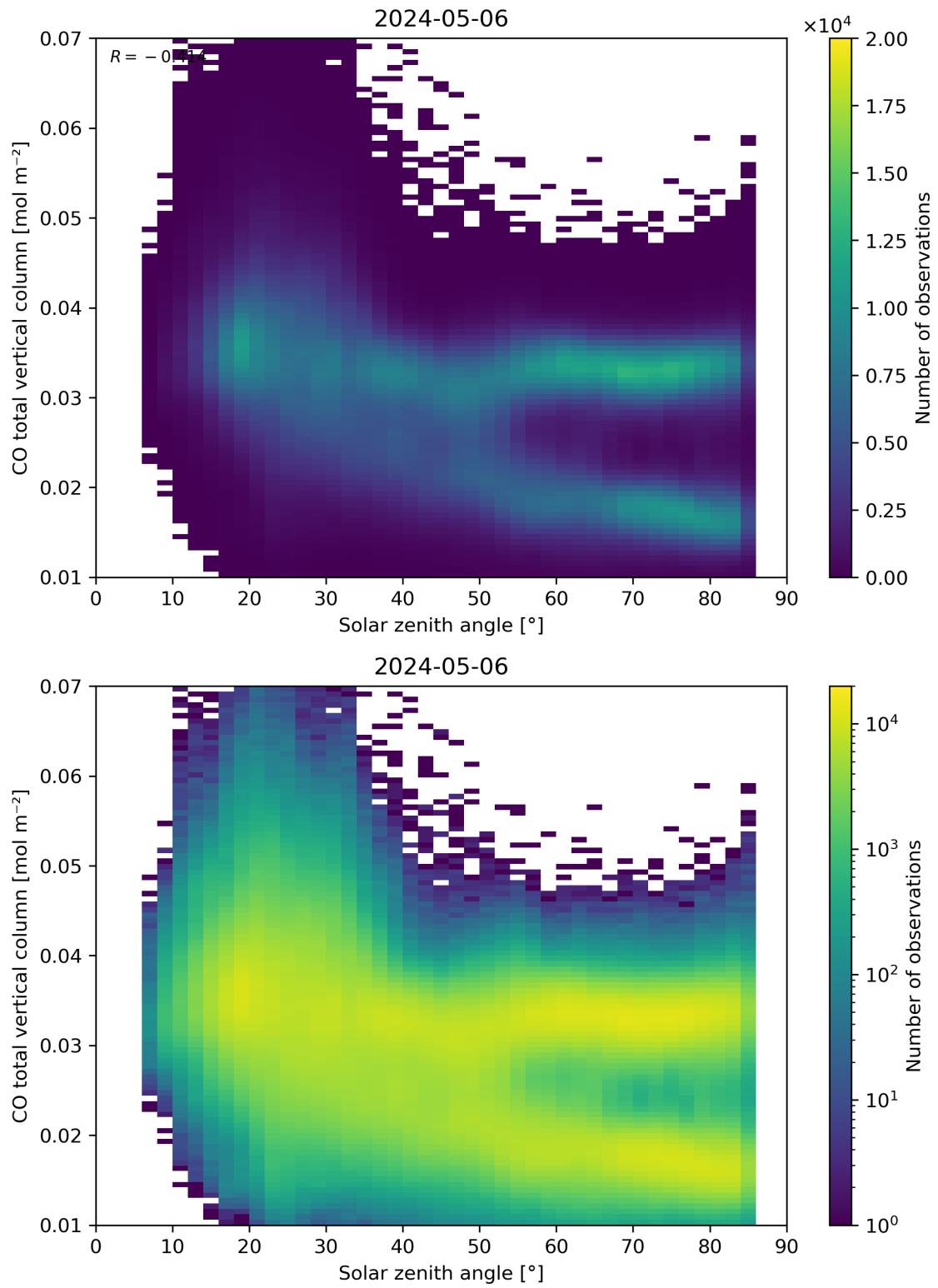
Figure 61: Scatter density plot of “Solar zenith angle” against “CO total vertical column” for 2024-05-05 to 2024-05-07.
