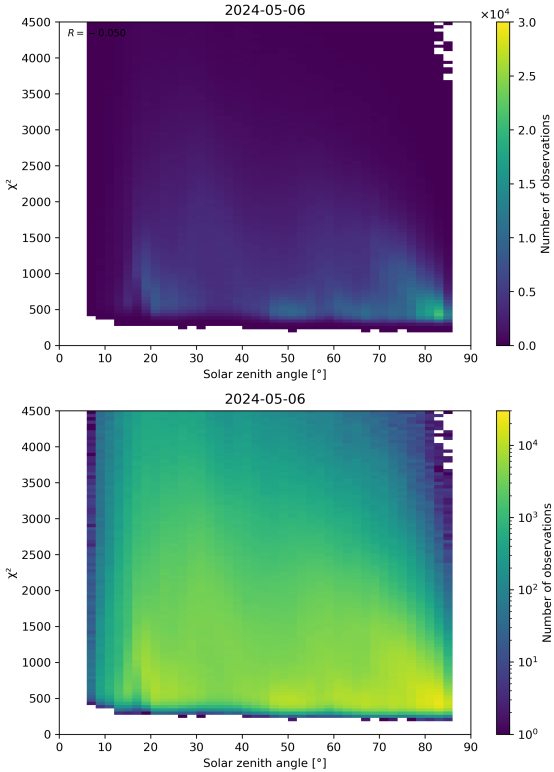
Figure 64: Scatter density plot of “Solar zenith angle” against “ \chi^2 ” for 2024-05-05 to 2024-05-07.
