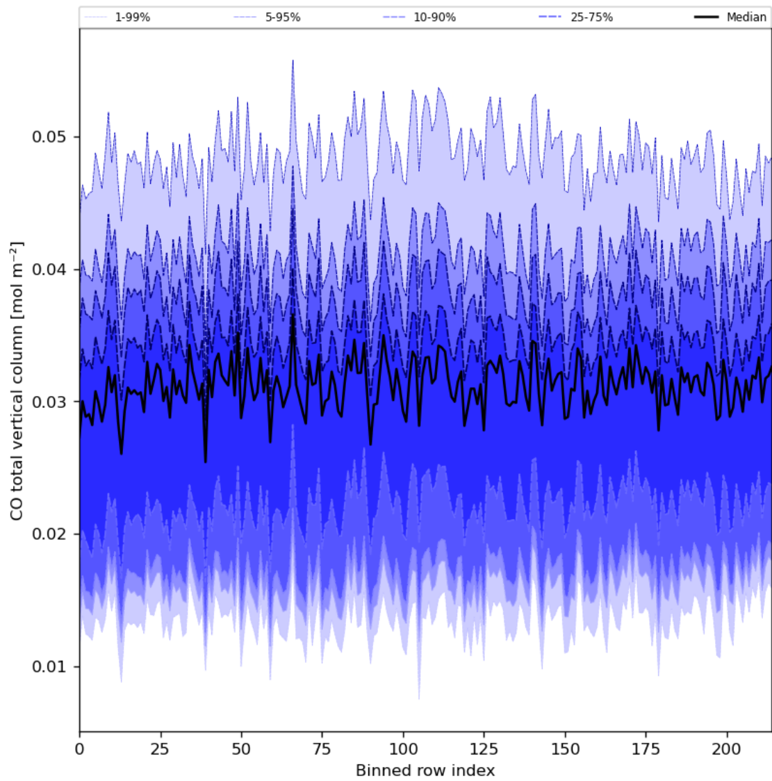
Figure 26: Along track statistics of “CO total vertical column” for 2024-05-05 to 2024-05-07
