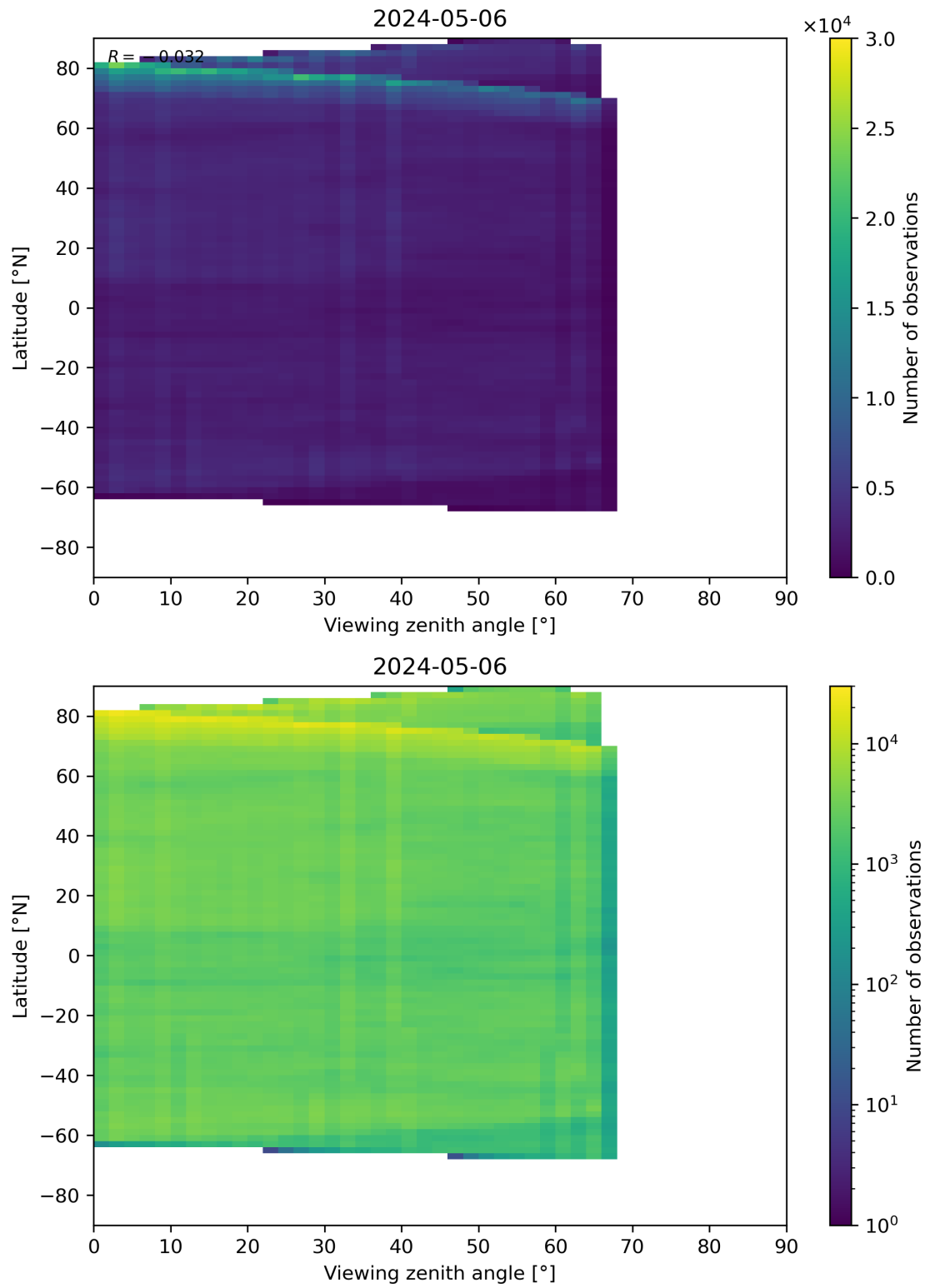
Figure 74: Scatter density plot of “Viewing zenith angle” against “Latitude” for 2024-05-05 to 2024-05-07.
