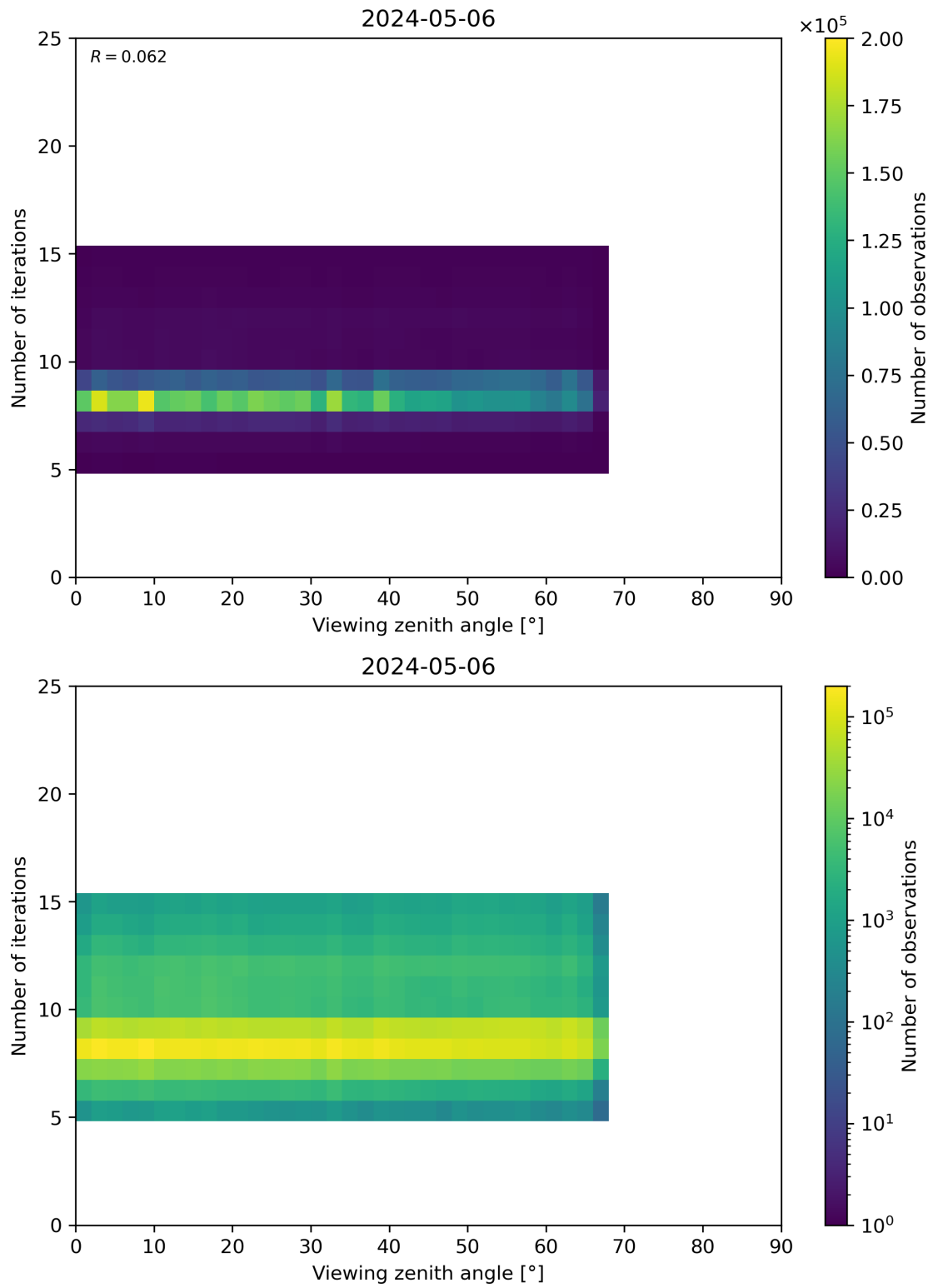
Figure 75: Scatter density plot of “Viewing zenith angle” against “Number of iterations” for 2024-05-05 to 2024-05-07.
