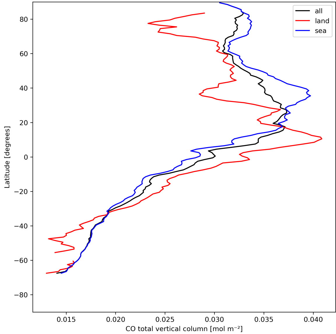
Figure 10: Zonal average of “CO total vertical column” for 2024-05-05 to 2024-05-07.
