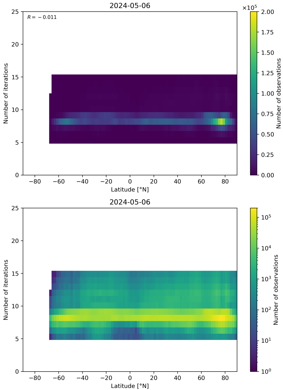
Figure 56: Scatter density plot of “Latitude” against “Number of iterations” for 2024-05-05 to 2024-05-07.
