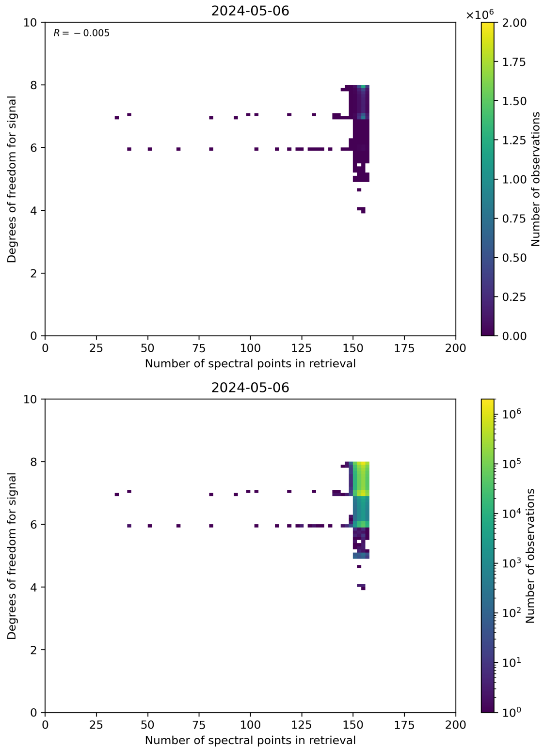
Figure 59: Scatter density plot of “Number of spectral points in retrieval” against “Degrees of freedom for signal” for 2024-05-05 to 2024-05-07.
