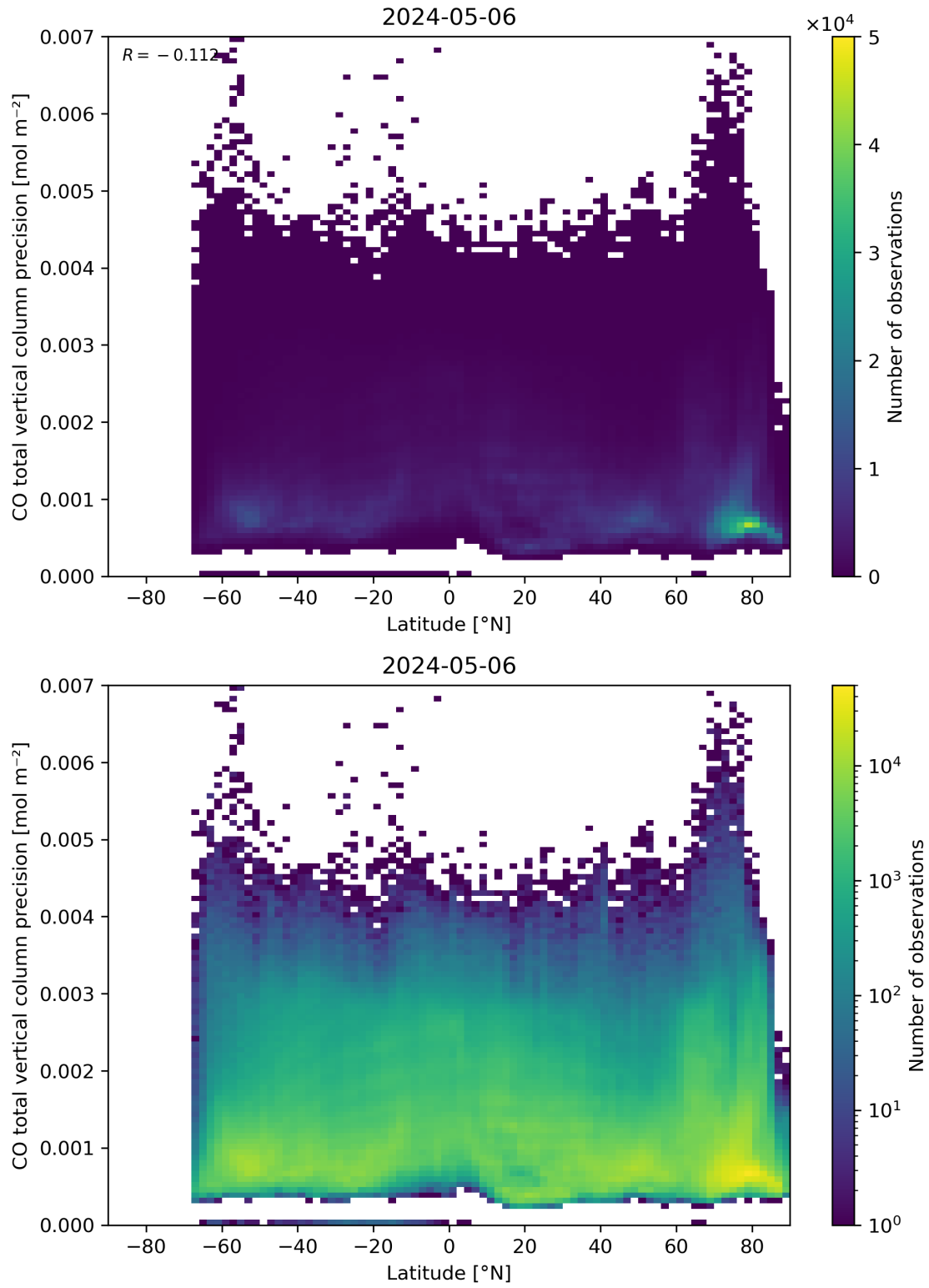
Figure 53: Scatter density plot of “Latitude” against “CO total vertical column precision” for 2024-05-05 to 2024-05-07.
