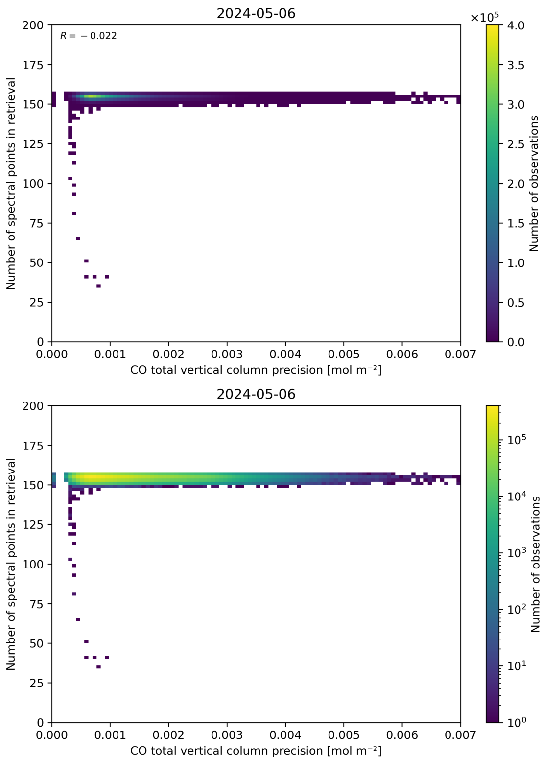
Figure 47: Scatter density plot of “CO total vertical column precision” against “Number of spectral points in retrieval” for 2024-05-05 to 2024-05-07.
