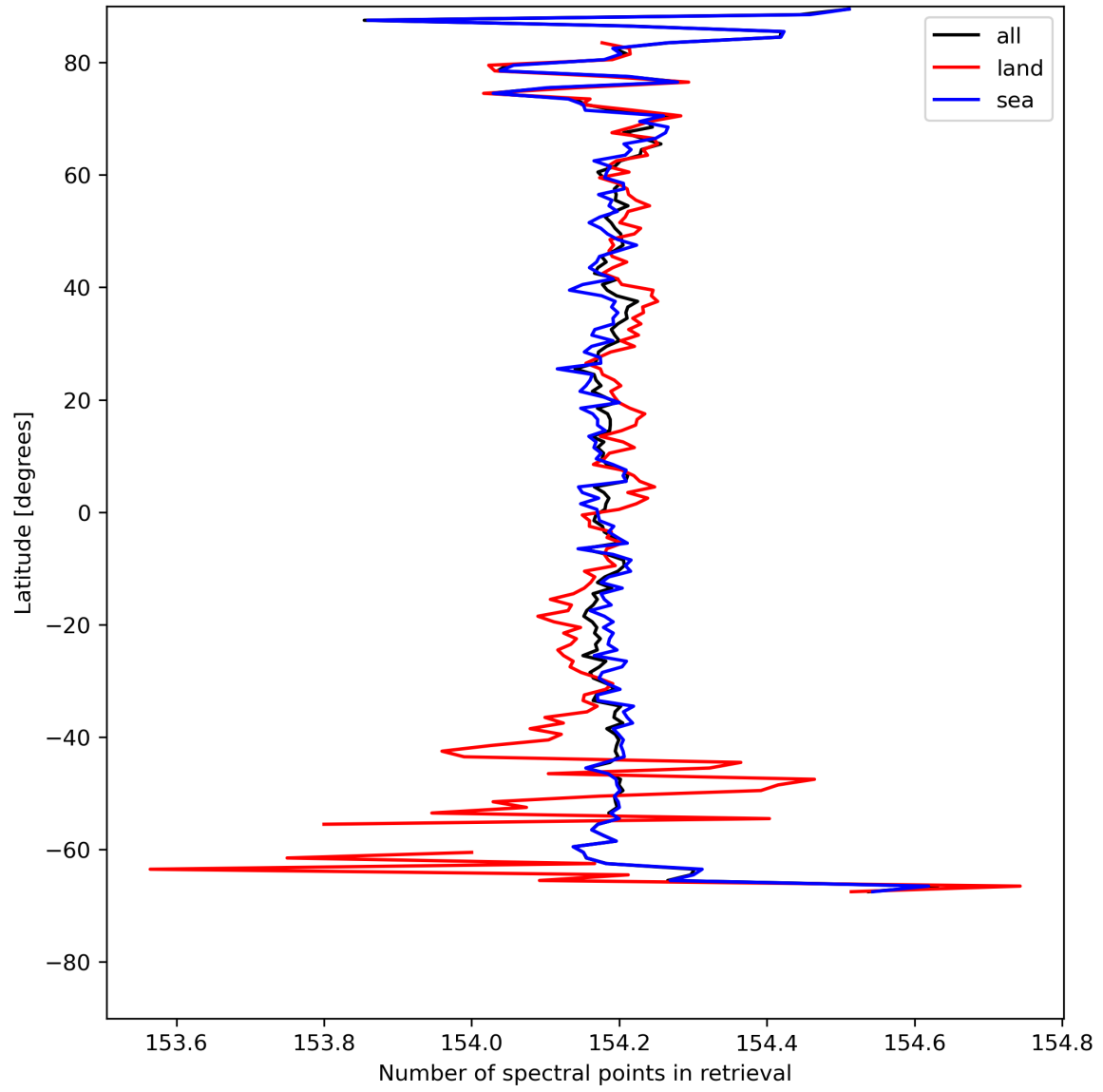
Figure 13: Zonal average of “Number of spectral points in retrieval” for 2024-05-05 to 2024-05-07.
