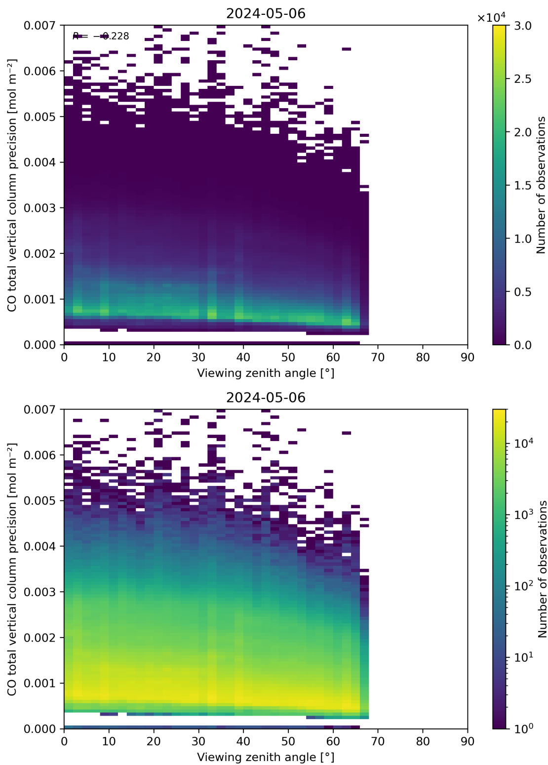
Figure 71: Scatter density plot of “Viewing zenith angle” against “CO total vertical column precision” for 2024-05-05 to 2024-05-07.
