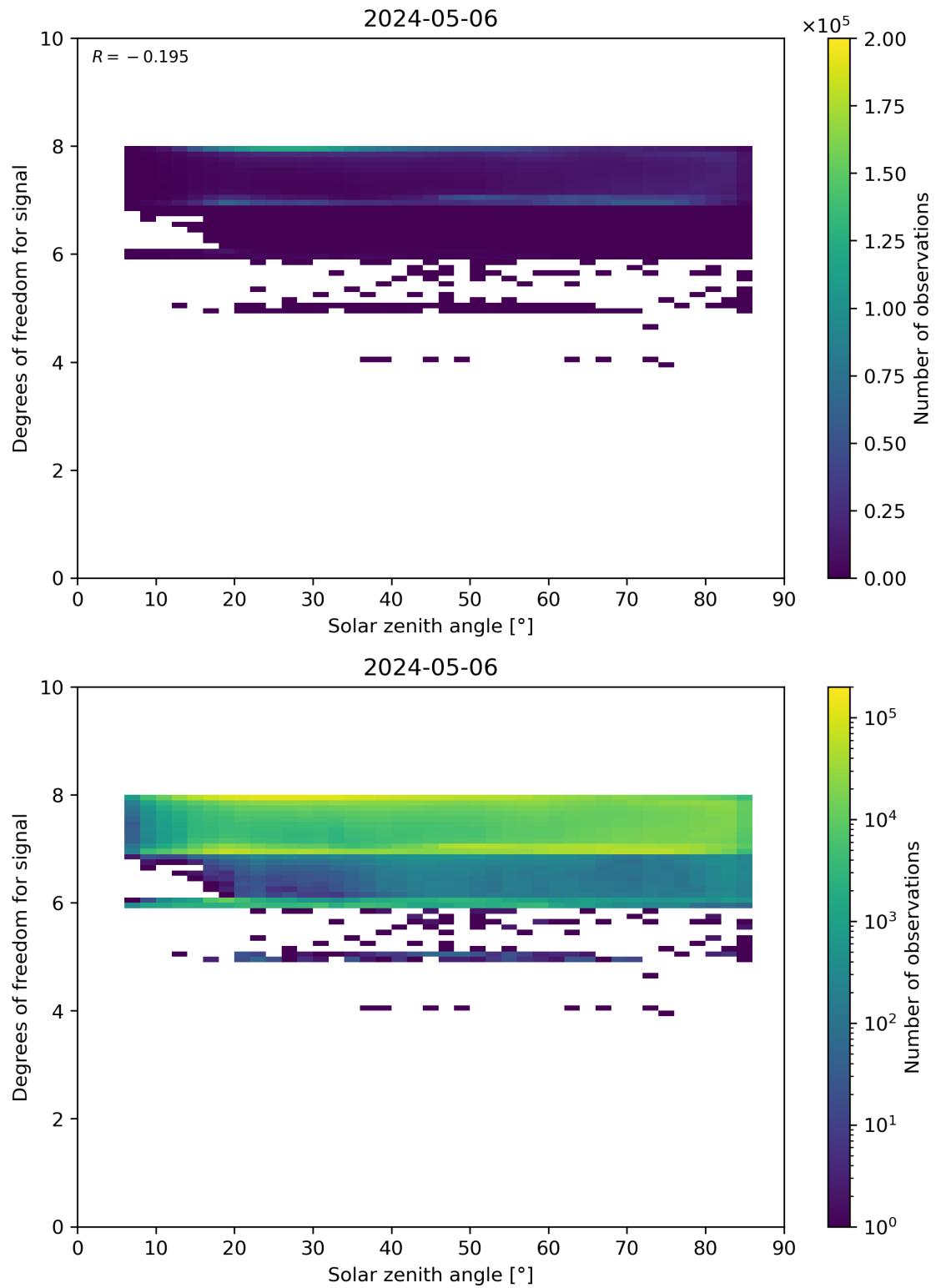
Figure 65: Scatter density plot of “Solar zenith angle” against “Degrees of freedom for signal” for 2024-05-05 to 2024-05-07.
