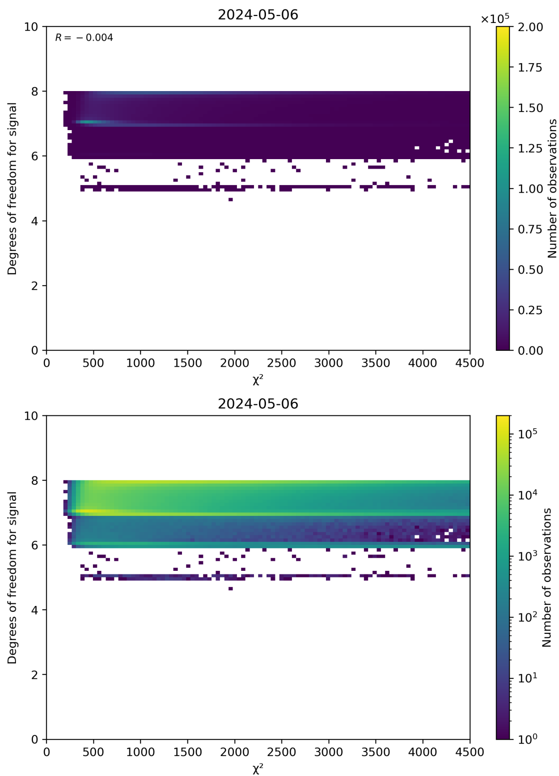
Figure 48: Scatter density plot of “ \chi^2 ” against “Degrees of freedom for signal” for 2024-05-05 to 2024-05-07.
