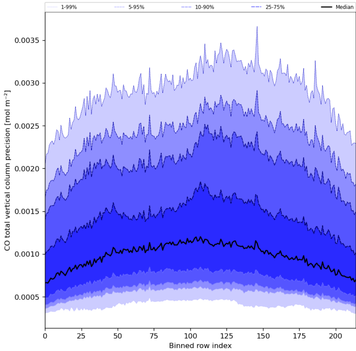
Figure 28: Along track statistics of “CO total vertical column precision” for 2024-05-05 to 2024-05-07
