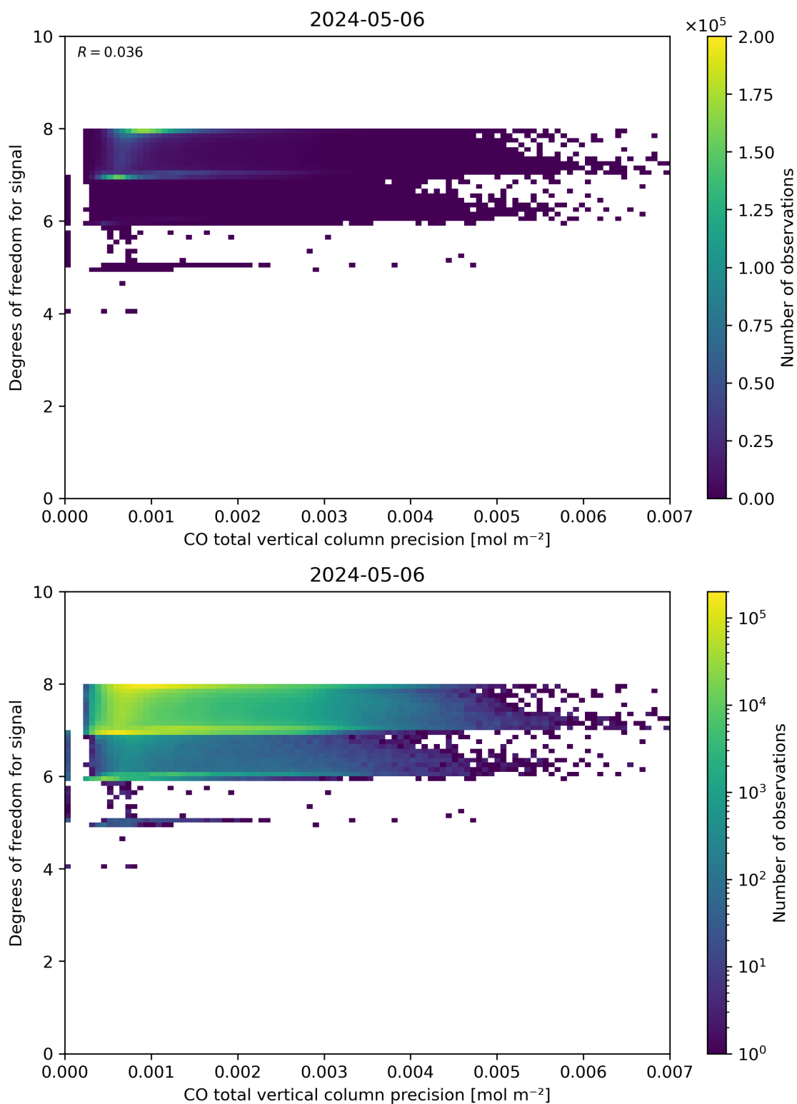
Figure 45: Scatter density plot of “CO total vertical column precision” against “Degrees of freedom for signal” for 2024-05-05 to 2024-05-07.
