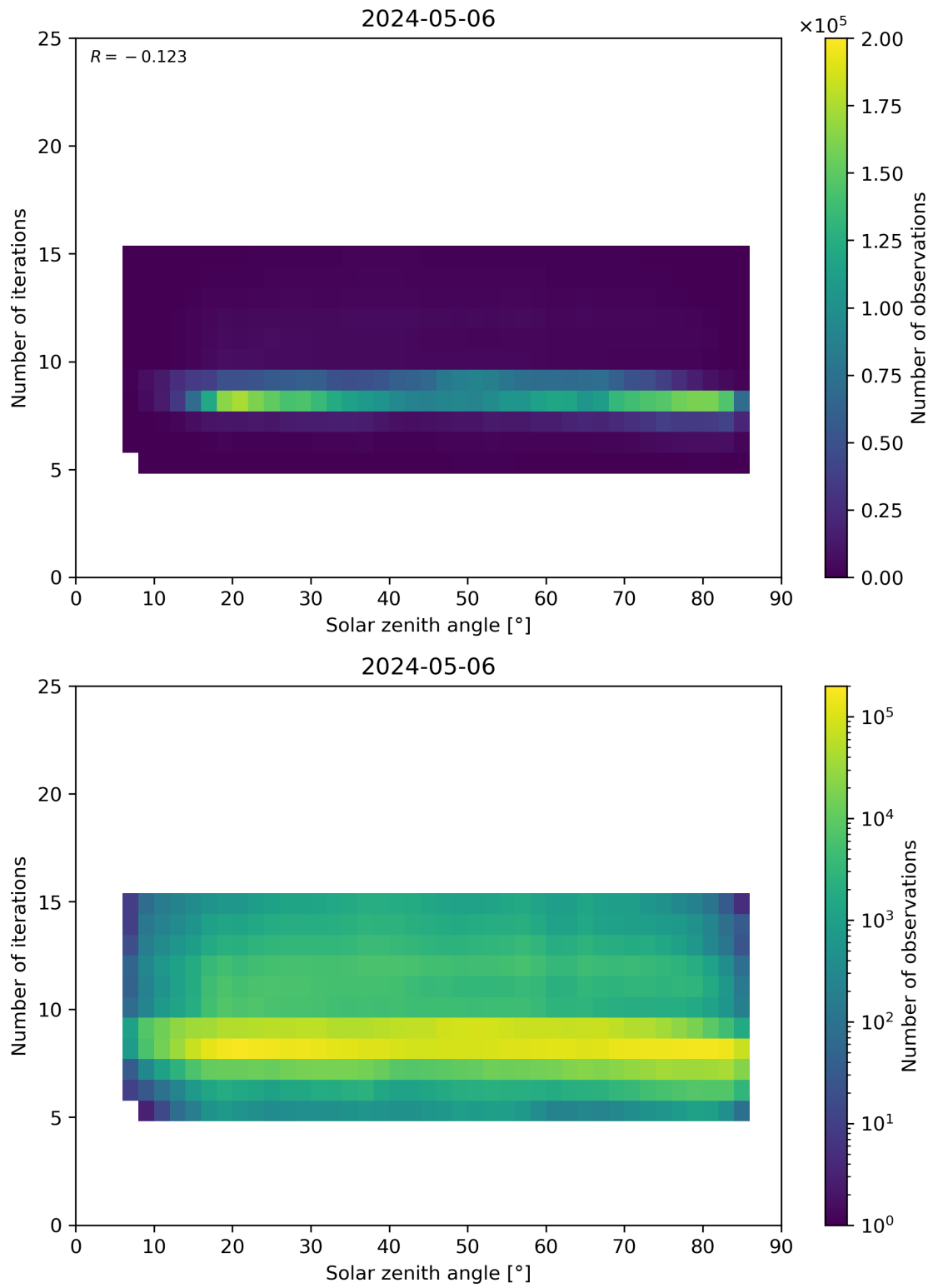
Figure 67: Scatter density plot of “Solar zenith angle” against “Number of iterations” for 2024-05-05 to 2024-05-07.
