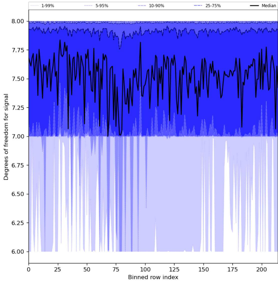
Figure 31: Along track statistics of “Degrees of freedom for signal” for 2024-05-05 to 2024-05-07
