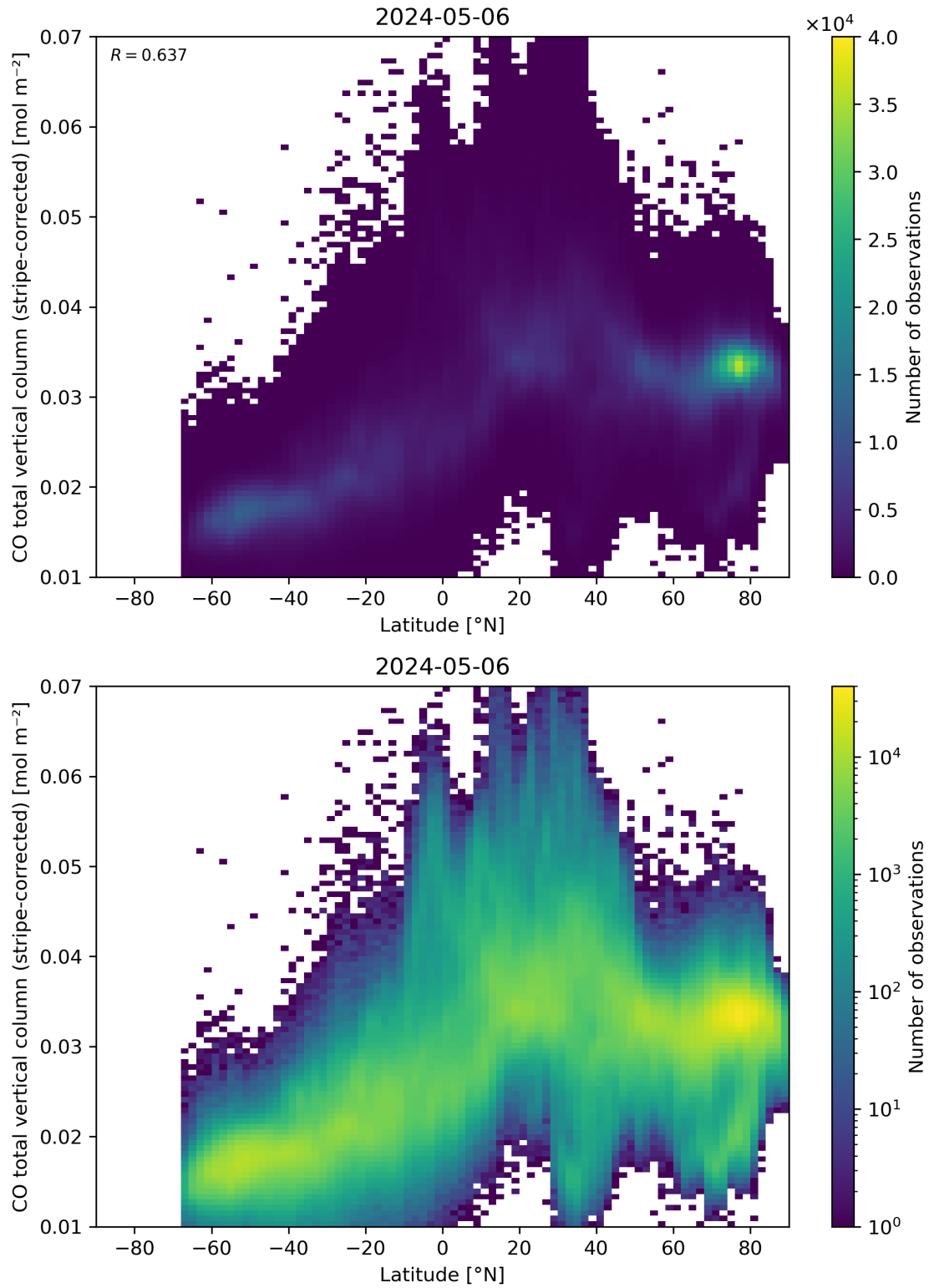
Figure 52: Scatter density plot of “Latitude” against “CO total vertical column (stripe-corrected)” for 2024-05-05 to 2024-05-07.
