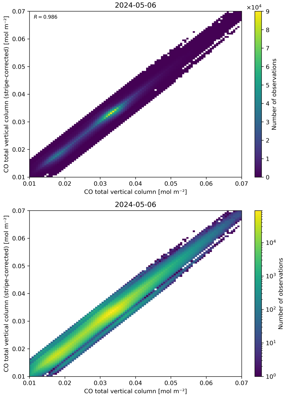
Figure 33: Scatter density plot of “CO total vertical column” against “CO total vertical column (stripe-corrected)” for 2024-05-05 to 2024-05-07.
