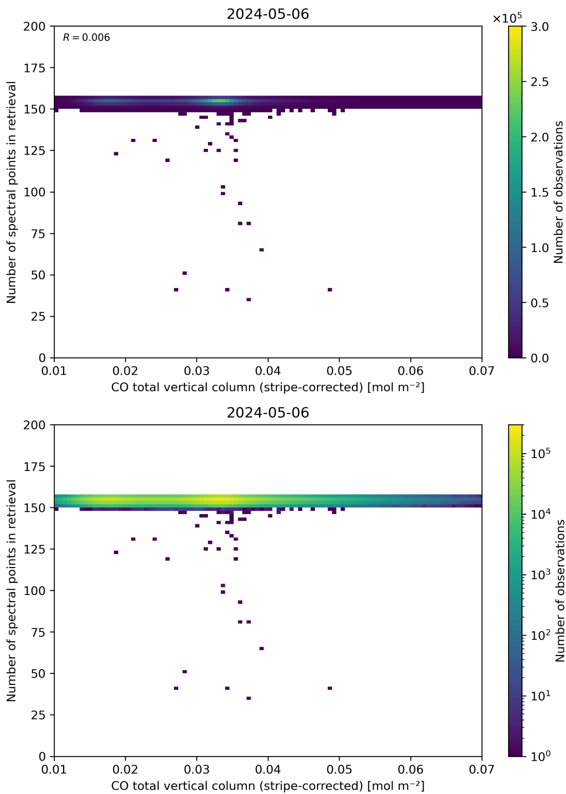
Figure 40: Scatter density plot of “CO total vertical column (stripe-corrected)” against “Number of spectral points in retrieval” for 2024-05-05 to 2024-05-07.
