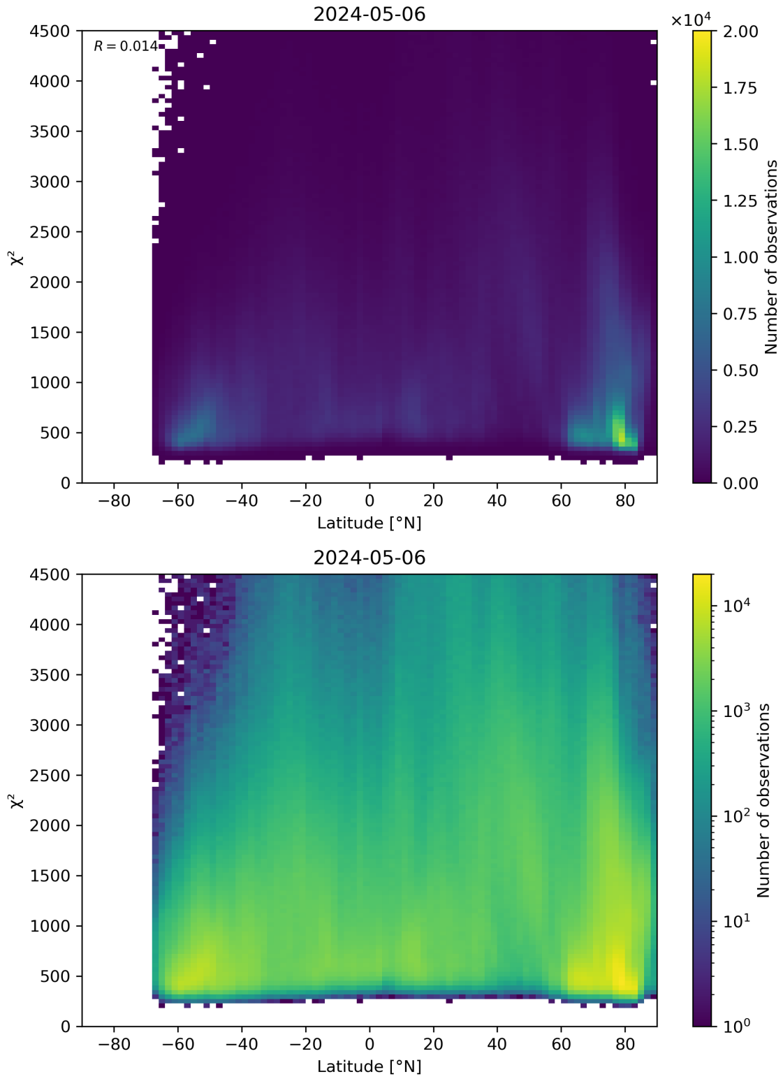
Figure 54: Scatter density plot of “Latitude” against “ \chi^2 ” for 2024-05-05 to 2024-05-07.
