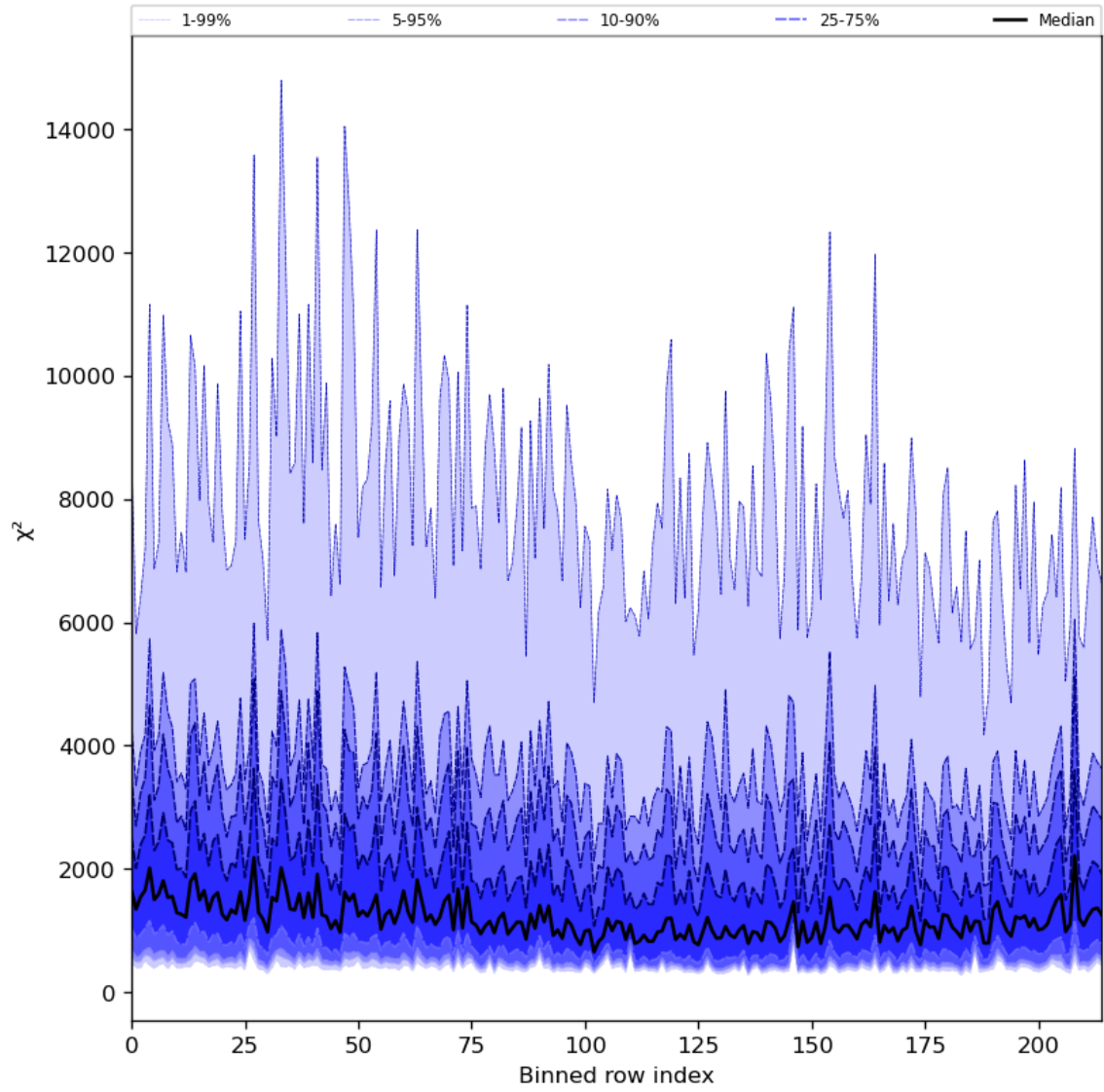
Figure 30: Along track statistics of “ \chi^2 ” for 2024-05-05 to 2024-05-07
