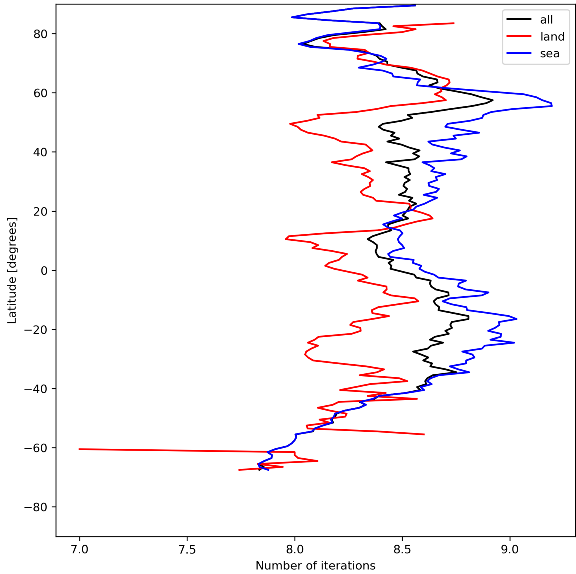
Figure 16: Zonal average of “Number of iterations” for 2024-05-05 to 2024-05-07.
