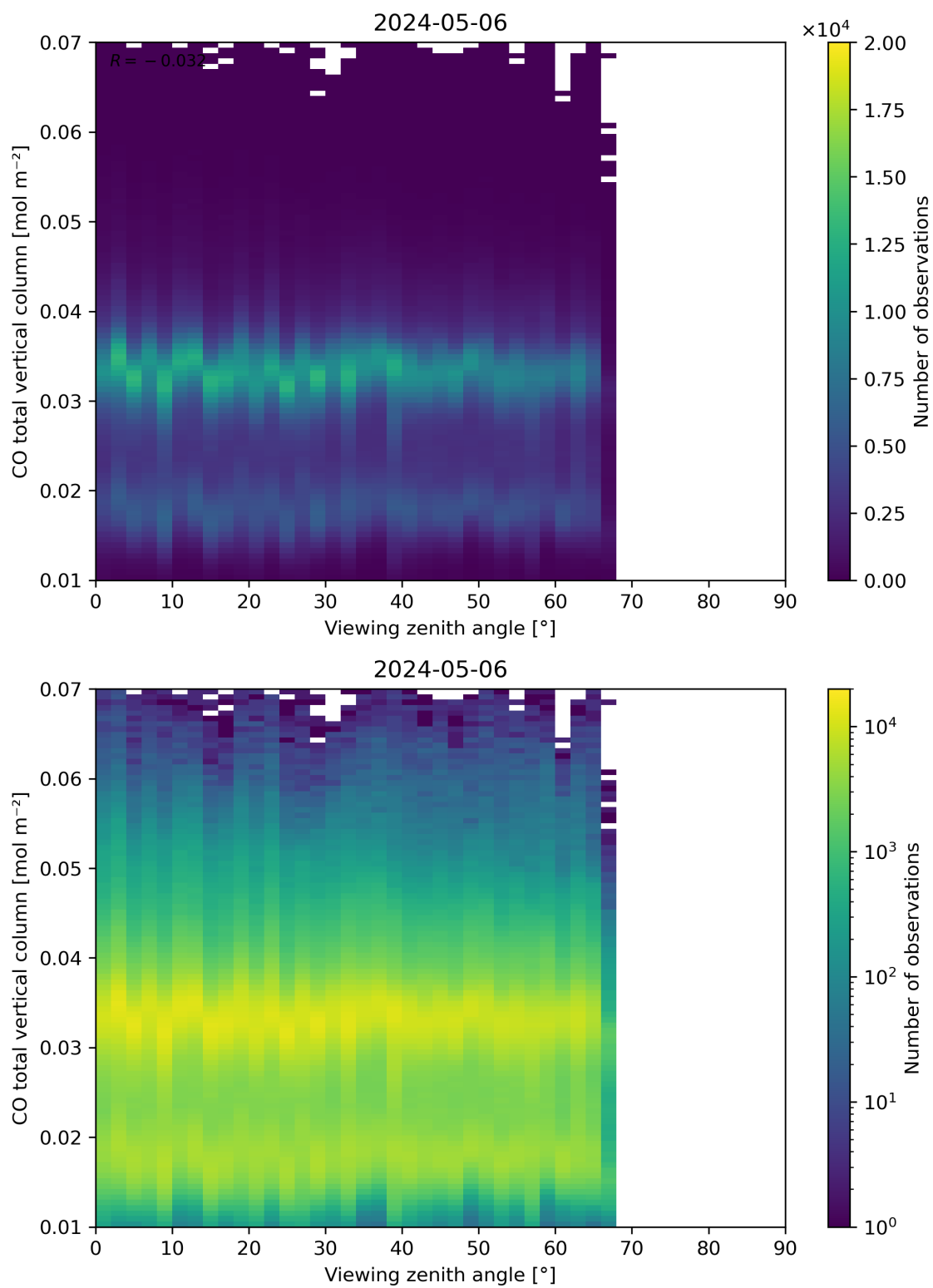
Figure 69: Scatter density plot of “Viewing zenith angle” against “CO total vertical column” for 2024-05-05 to 2024-05-07.
