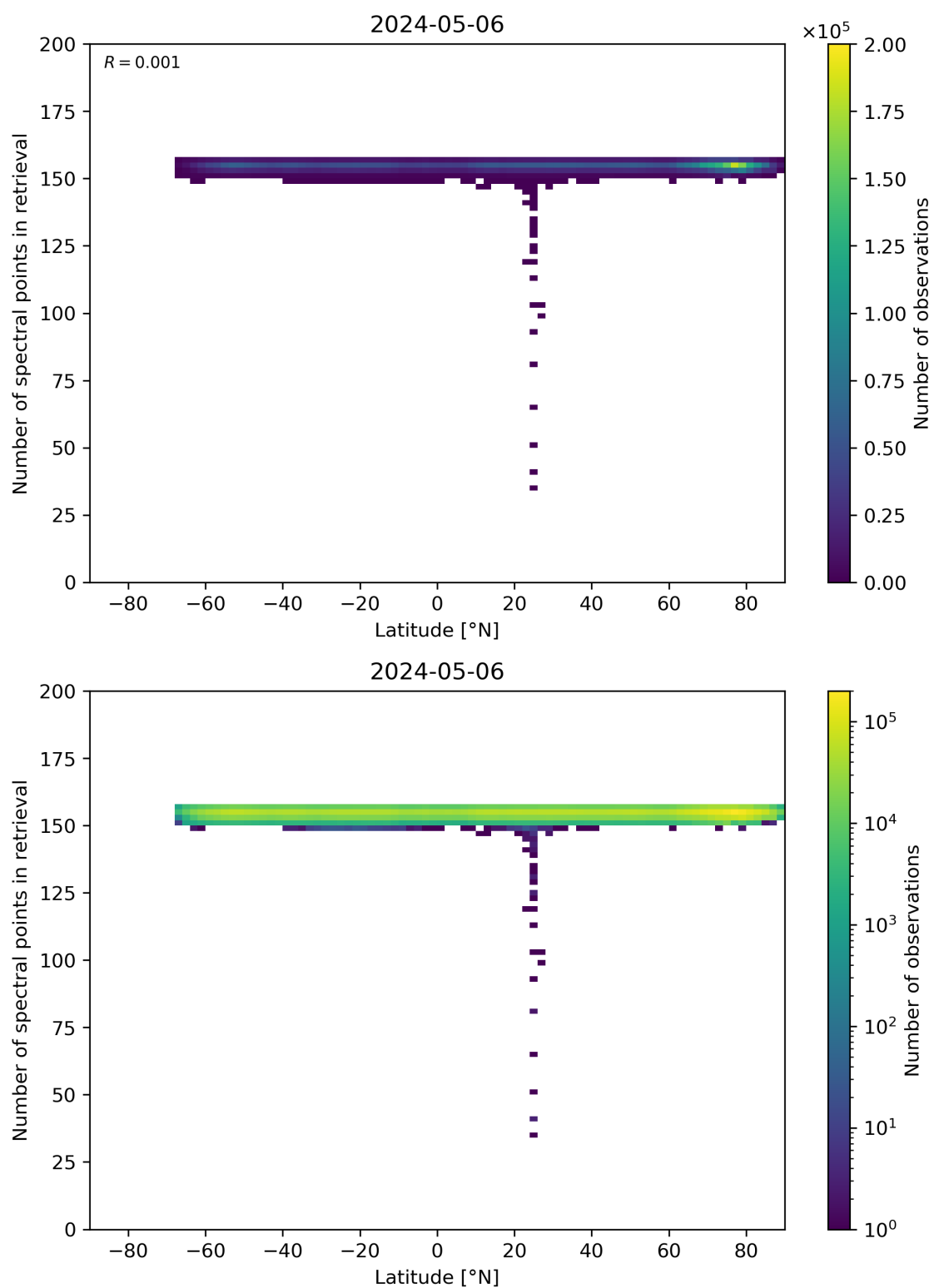
Figure 57: Scatter density plot of “Latitude” against “Number of spectral points in retrieval” for 2024-05-05 to 2024-05-07.
