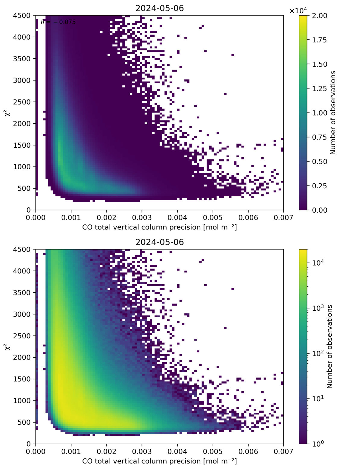
Figure 44: Scatter density plot of “CO total vertical column precision” against “ \chi^2 ” for 2024-05-05 to 2024-05-07.
