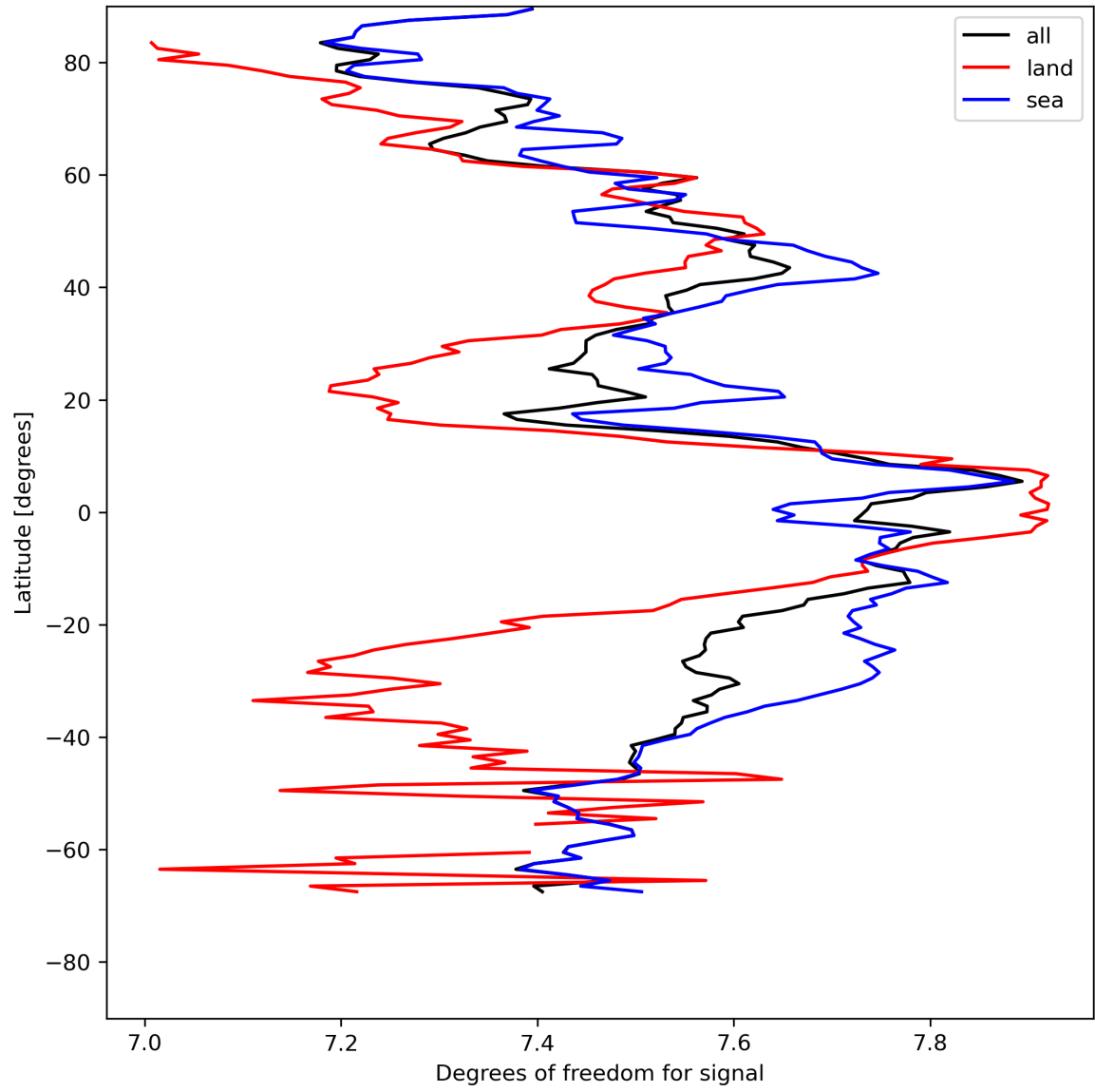
Figure 15: Zonal average of “Degrees of freedom for signal” for 2024-05-05 to 2024-05-07.
