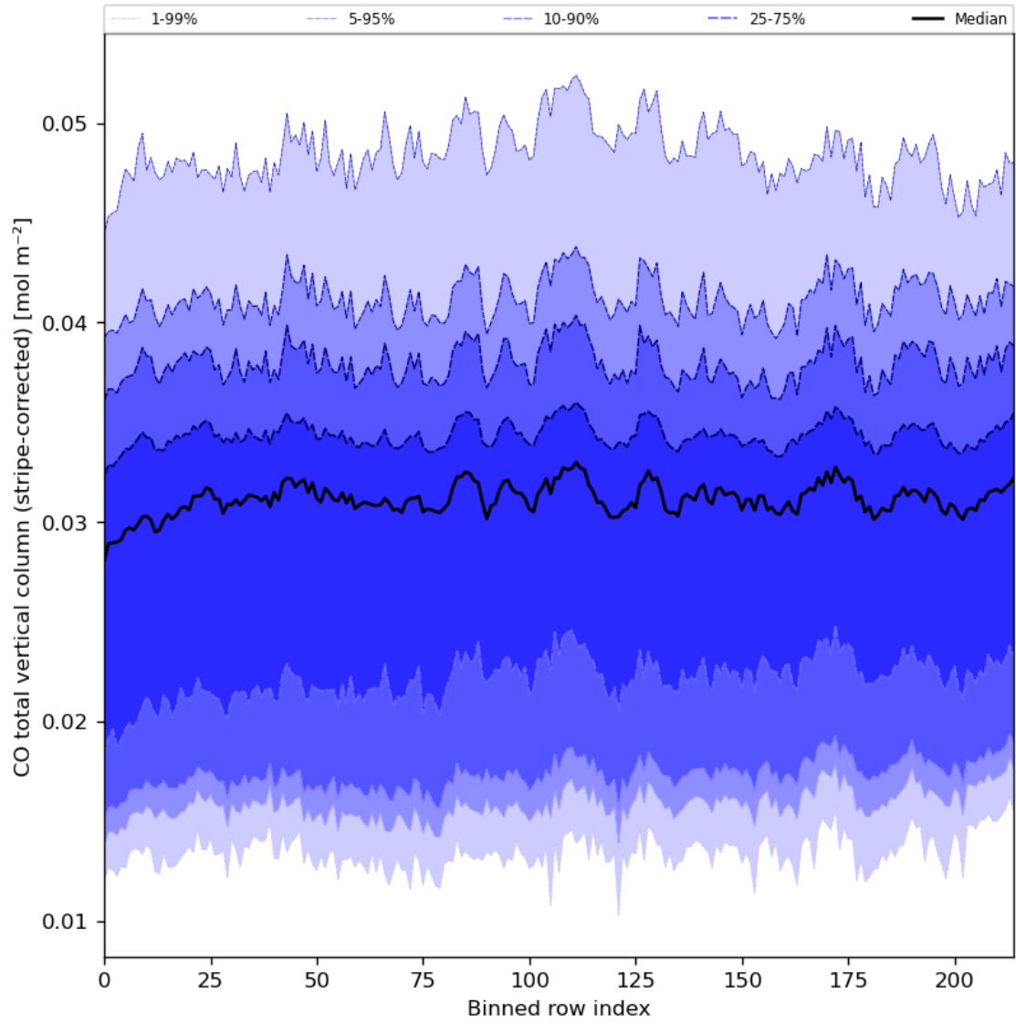
Figure 27: Along track statistics of “CO total vertical column (stripe-corrected)” for 2024-05-05 to 2024-05-07
