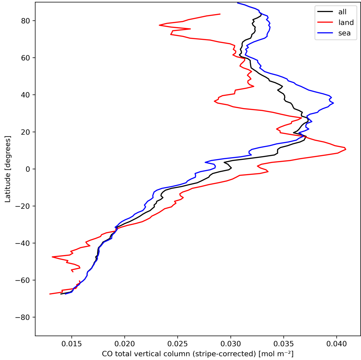
Figure 11: Zonal average of “CO total vertical column (stripe-corrected)” for 2024-05-05 to 2024-05-07.
