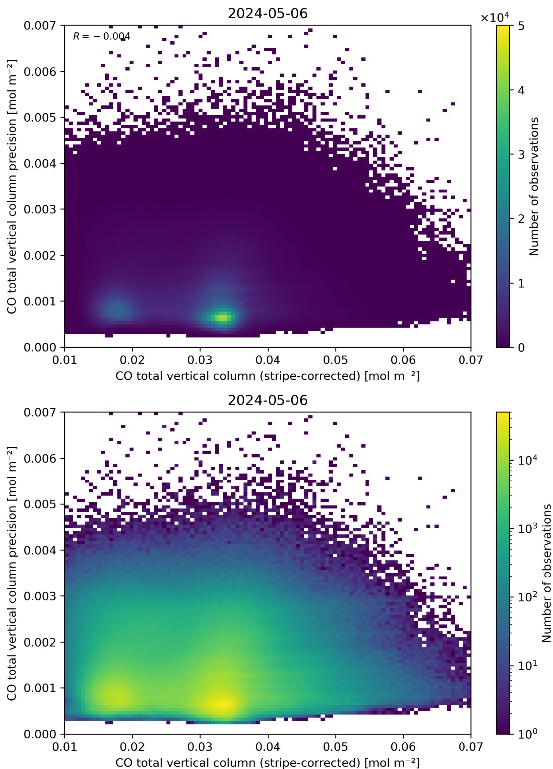
Figure 36: Scatter density plot of “CO total vertical column (stripe-corrected)” against “CO total vertical column precision” for 2024-05-05 to 2024-05-07.
