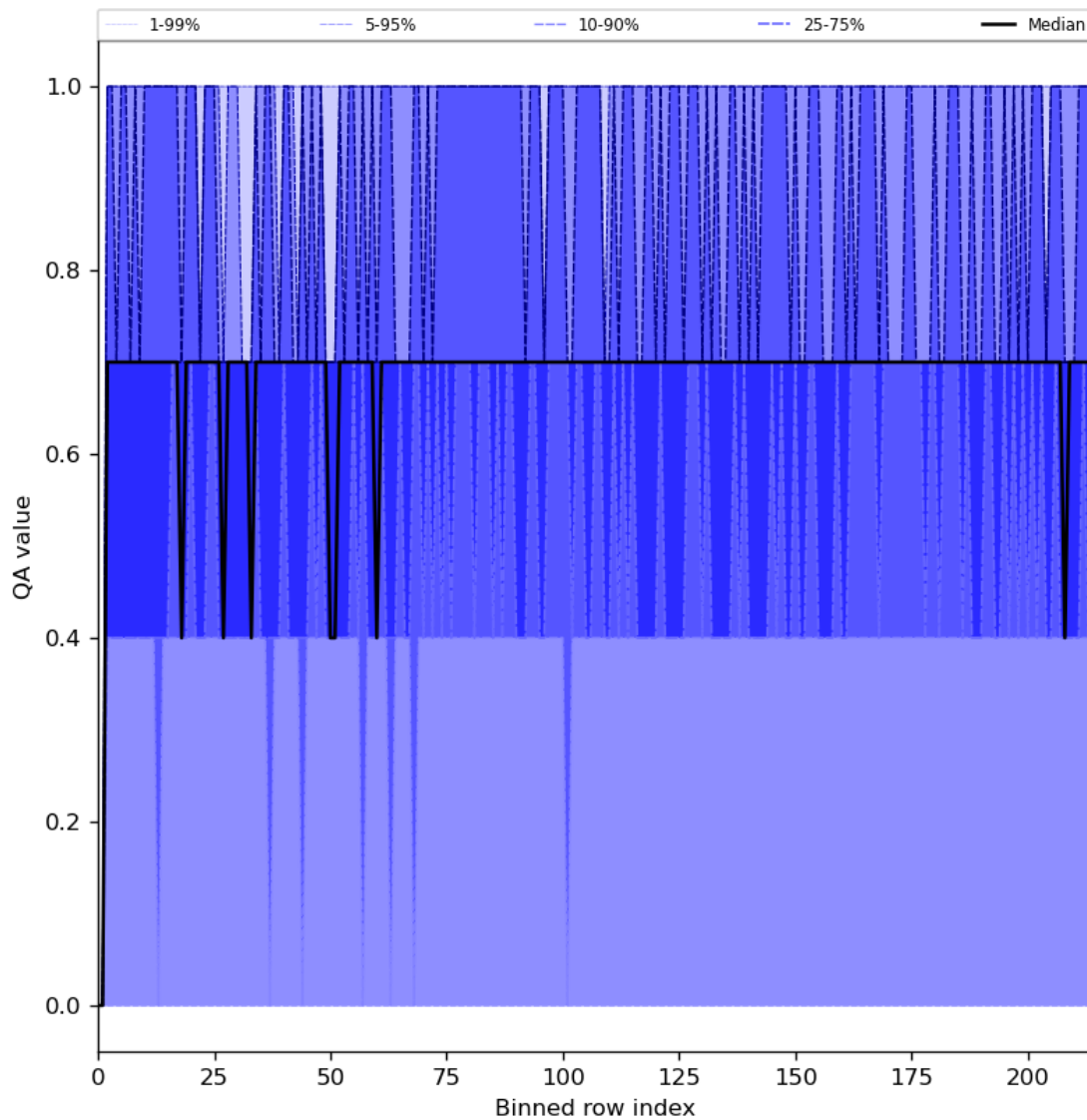
Figure 25: Along track statistics of “QA value” for 2024-05-05 to 2024-05-07
