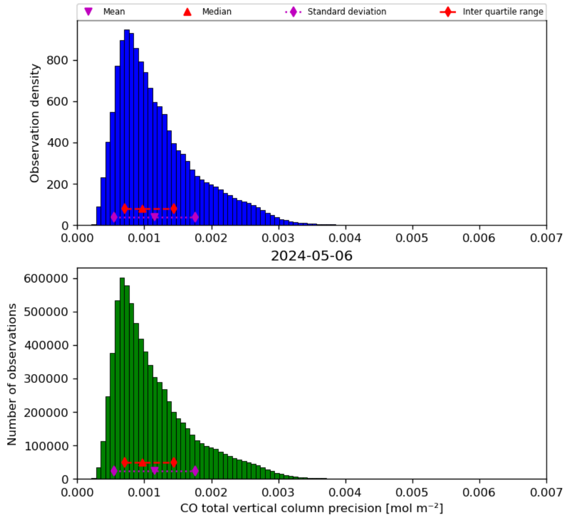
Figure 20: Histogram of “CO total vertical column precision” for 2024-05-05 to 2024-05-07
