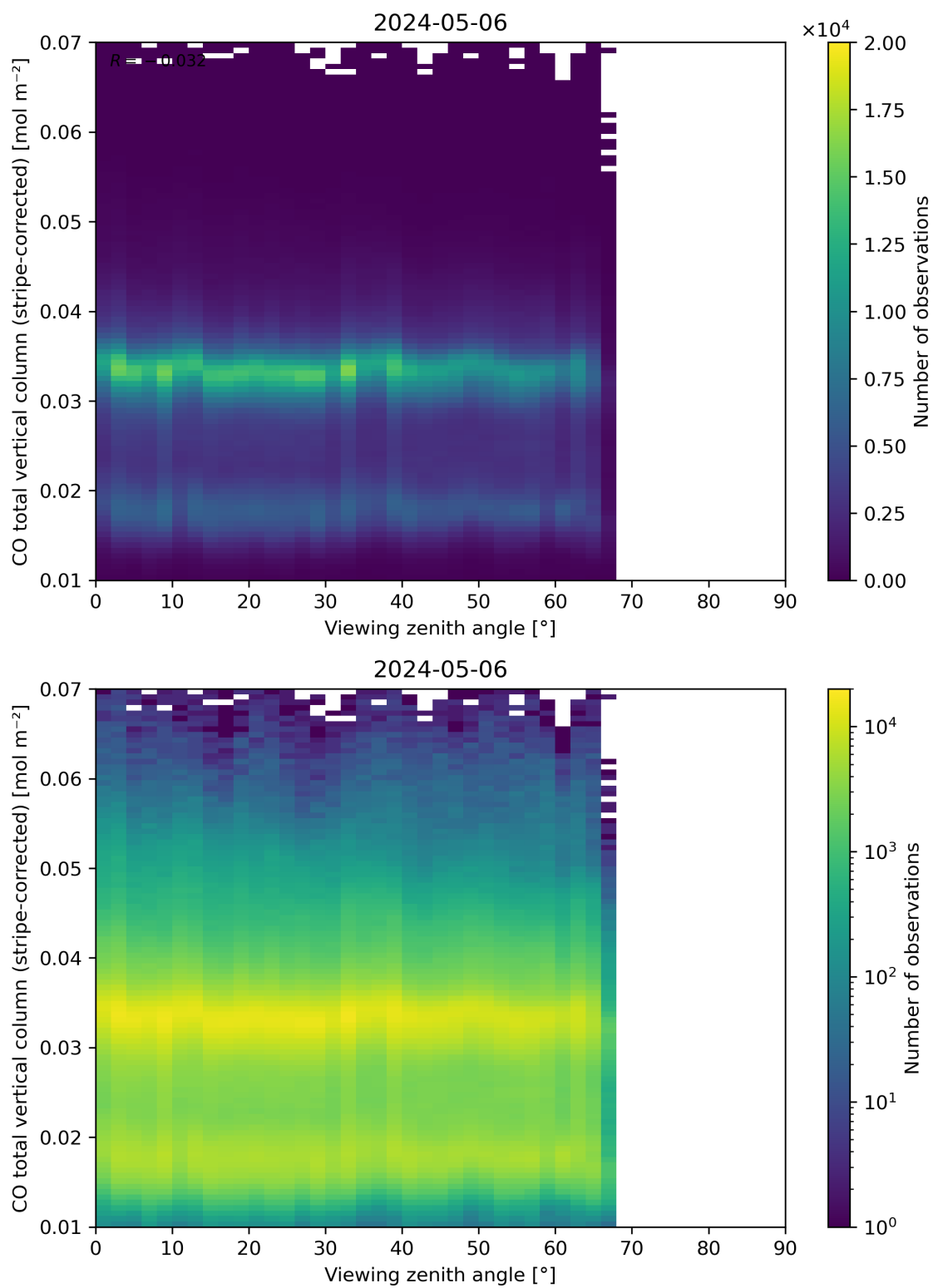
Figure 70: Scatter density plot of “Viewing zenith angle” against “CO total vertical column (stripe-corrected)” for 2024-05-05 to 2024-05-07.
