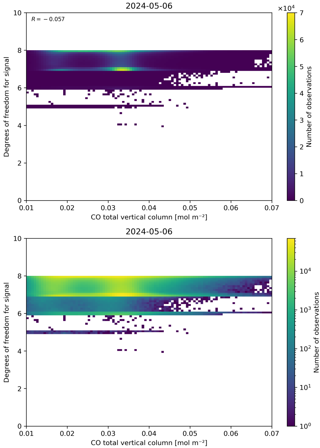
Figure 41: Scatter density plot of “CO total vertical column” against “Degrees of freedom for signal” for 2024-05-05 to 2024-05-07.
