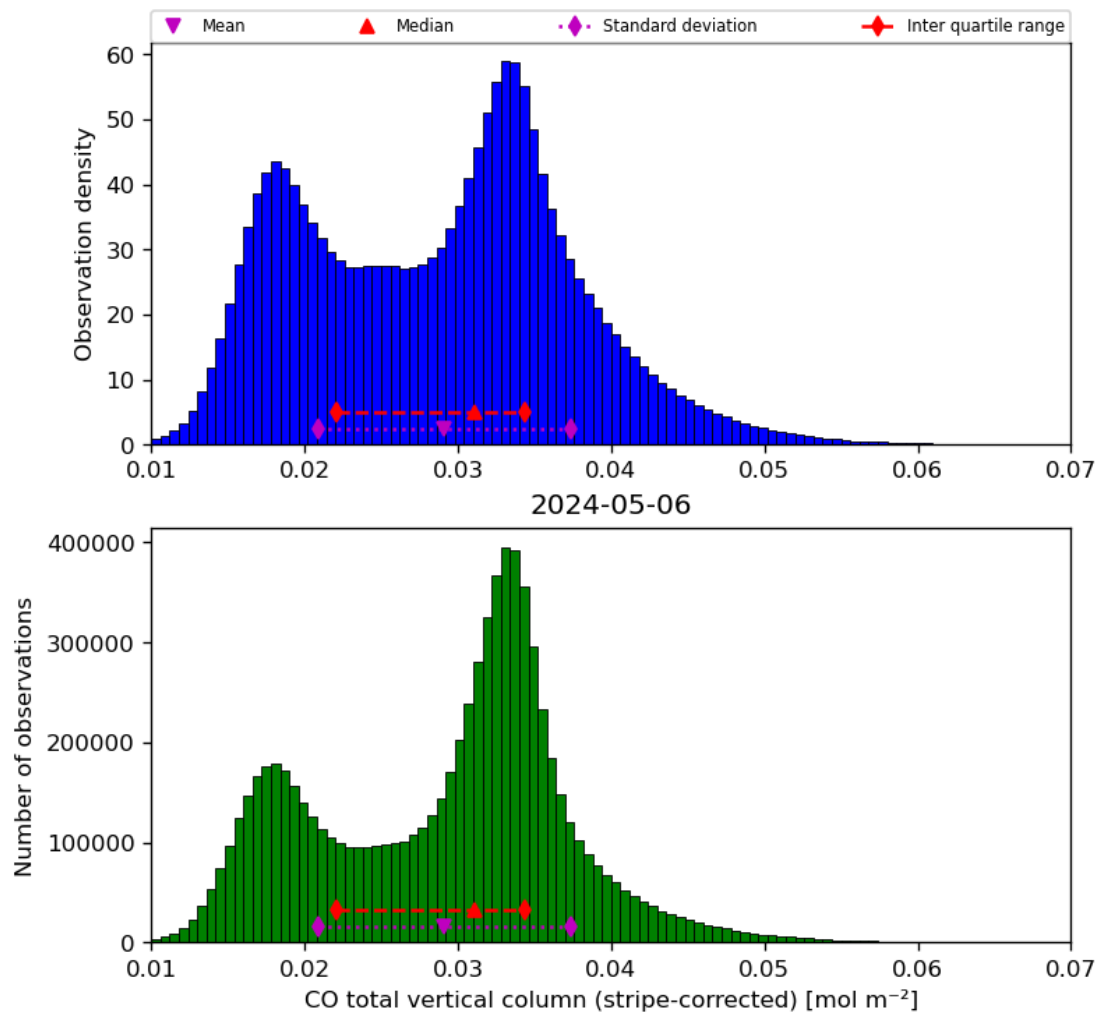
Figure 19: Histogram of “CO total vertical column (stripe-corrected)” for 2024-05-05 to 2024-05-07
