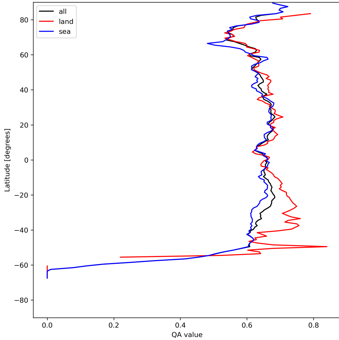
Figure 9: Zonal average of “QA value” for 2024-05-05 to 2024-05-07.
