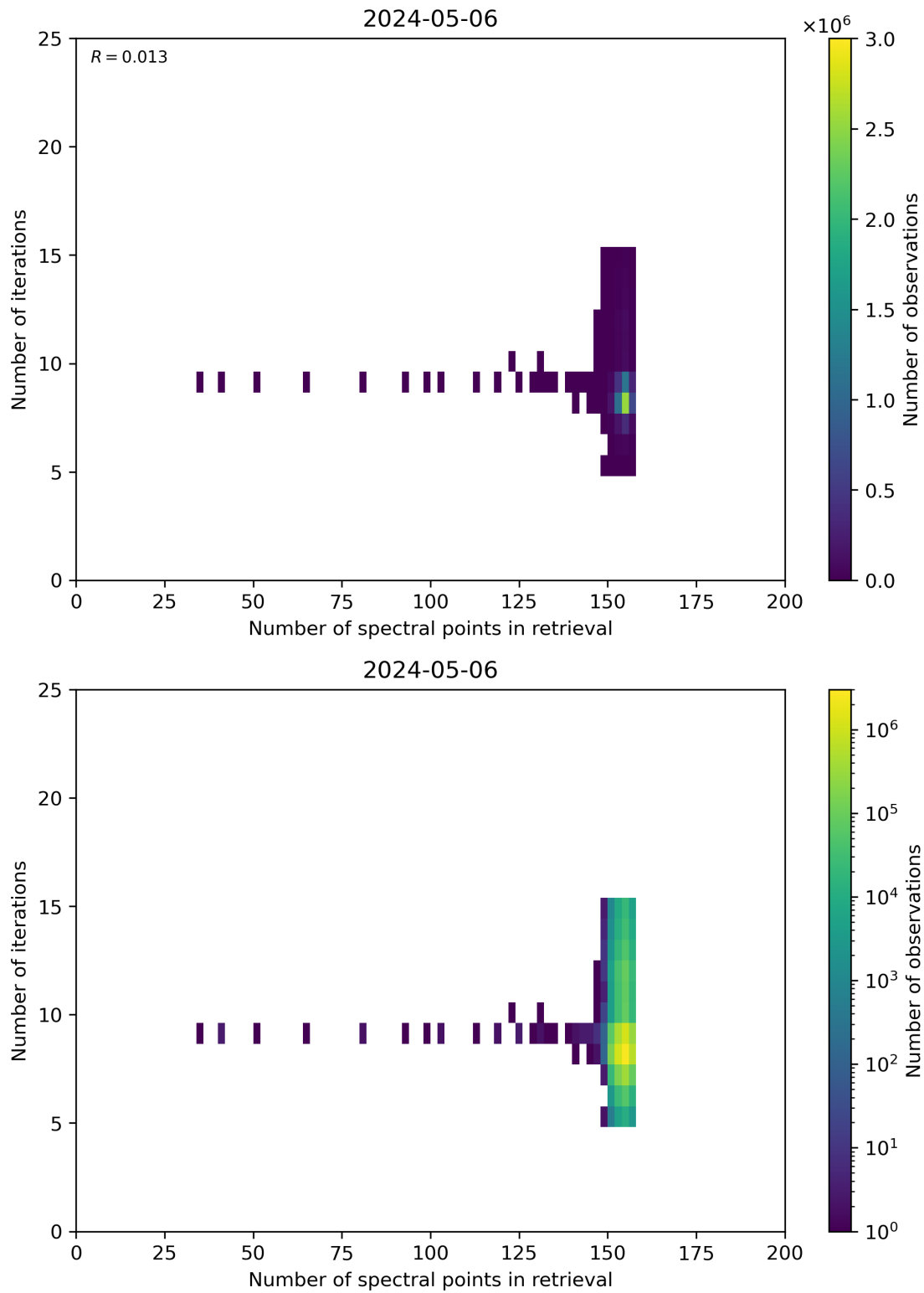
Figure 60: Scatter density plot of “Number of spectral points in retrieval” against “Number of iterations” for 2024-05-05 to 2024-05-07.
