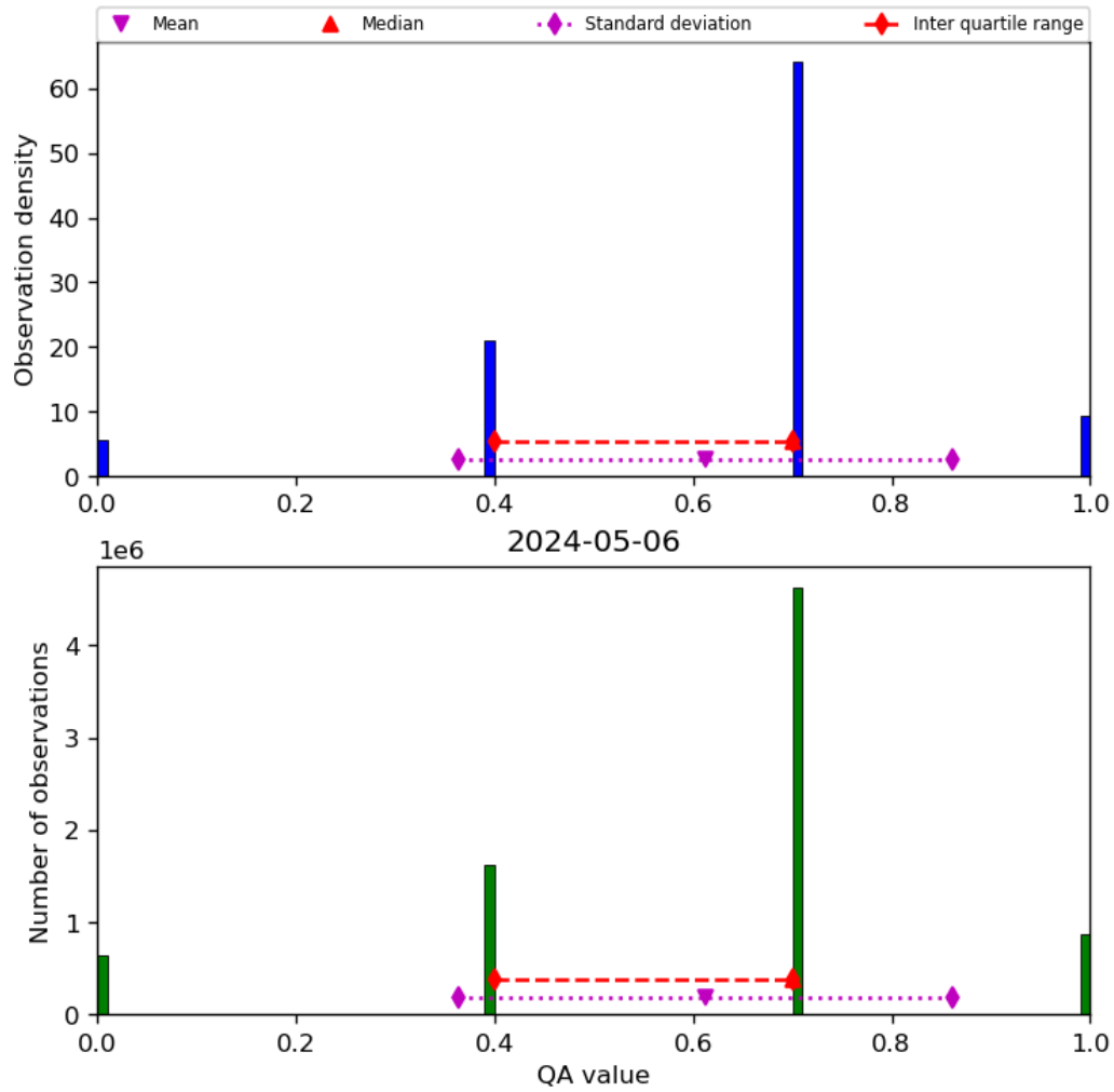
Figure 17: Histogram of “QA value” for 2024-05-05 to 2024-05-07
