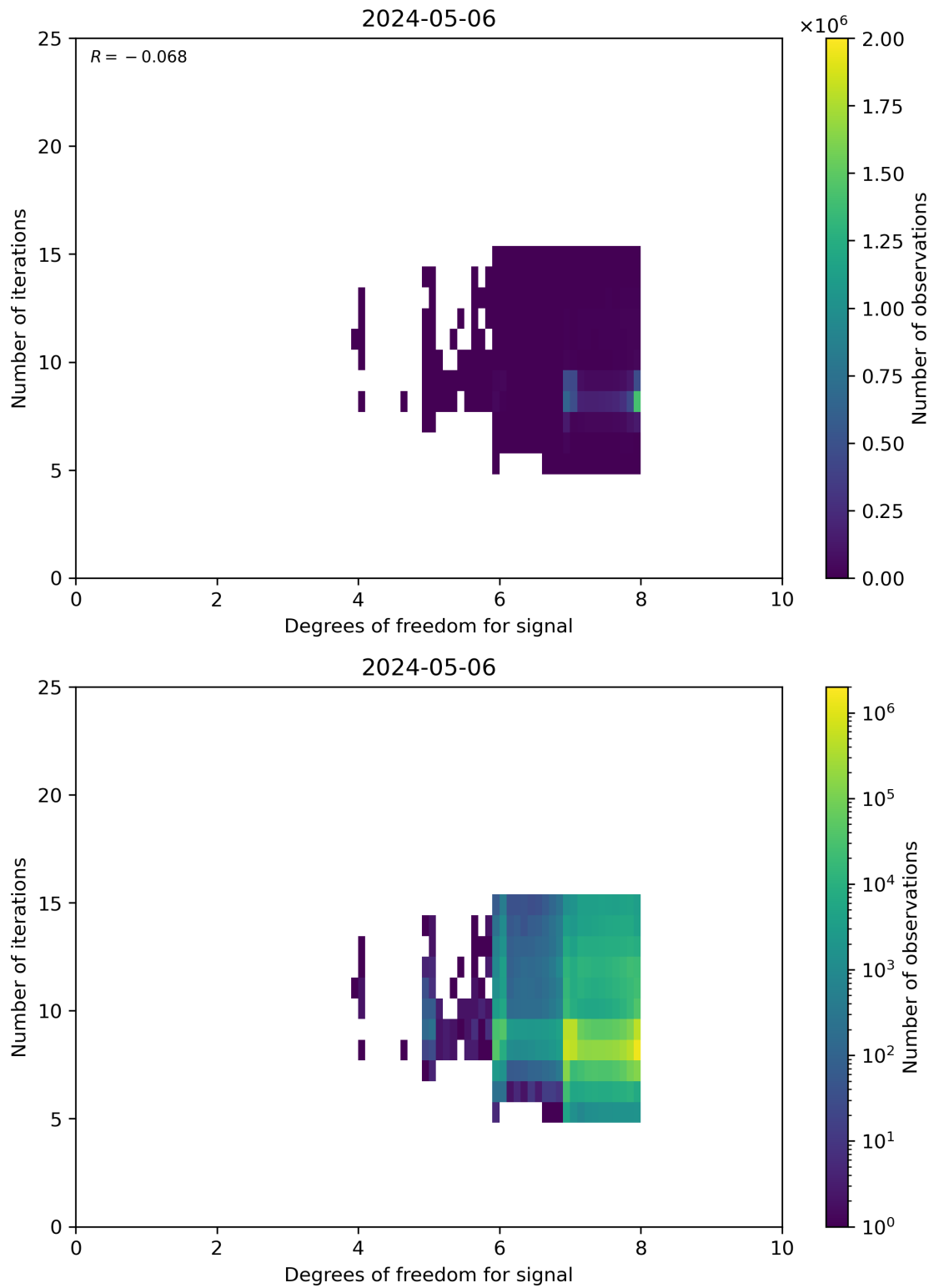
Figure 50: Scatter density plot of “Degrees of freedom for signal” against “Number of iterations” for 2024-05-05 to 2024-05-07.
