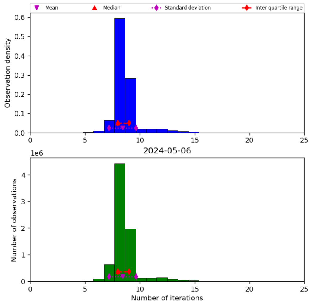
Figure 24: Histogram of “Number of iterations” for 2024-05-05 to 2024-05-07
