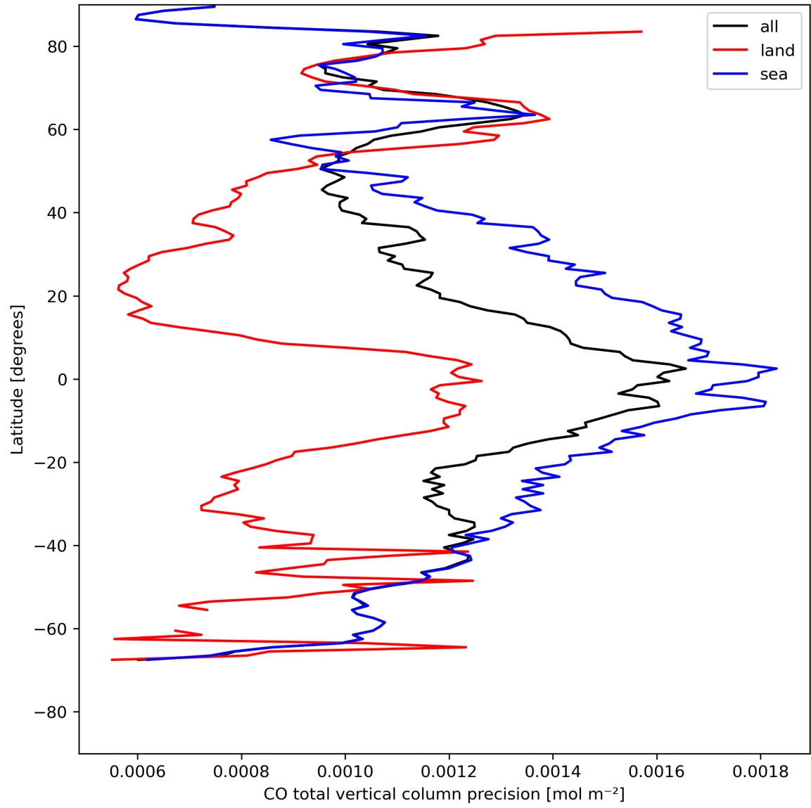
Figure 12: Zonal average of “CO total vertical column precision” for 2024-05-05 to 2024-05-07.
