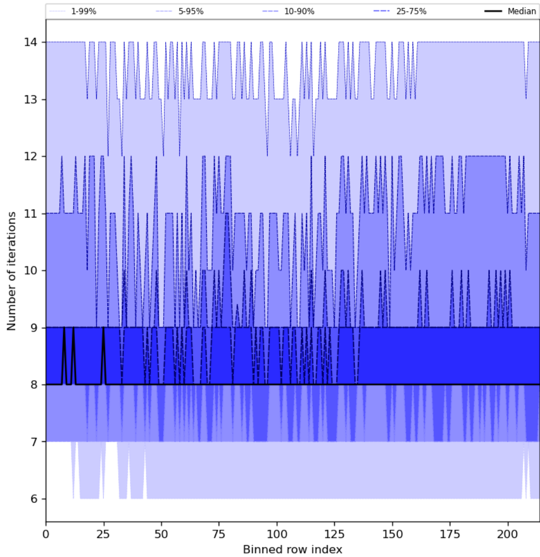
Figure 32: Along track statistics of “Number of iterations” for 2024-05-05 to 2024-05-07
