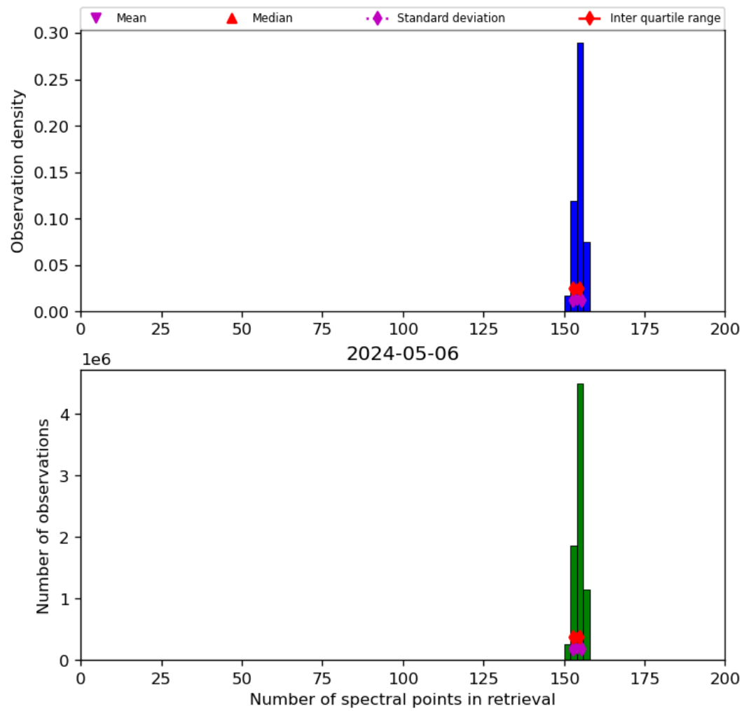
Figure 21: Histogram of “Number of spectral points in retrieval” for 2024-05-05 to 2024-05-07
