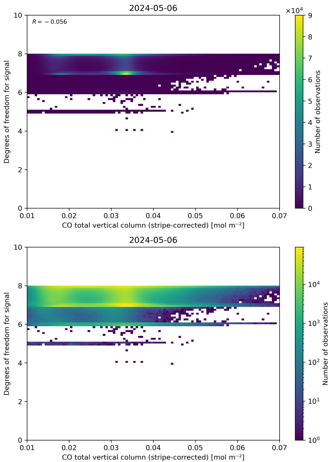
Figure 38: Scatter density plot of “CO total vertical column (stripe-corrected)” against “Degrees of freedom for signal” for 2024-05-05 to 2024-05-07.
