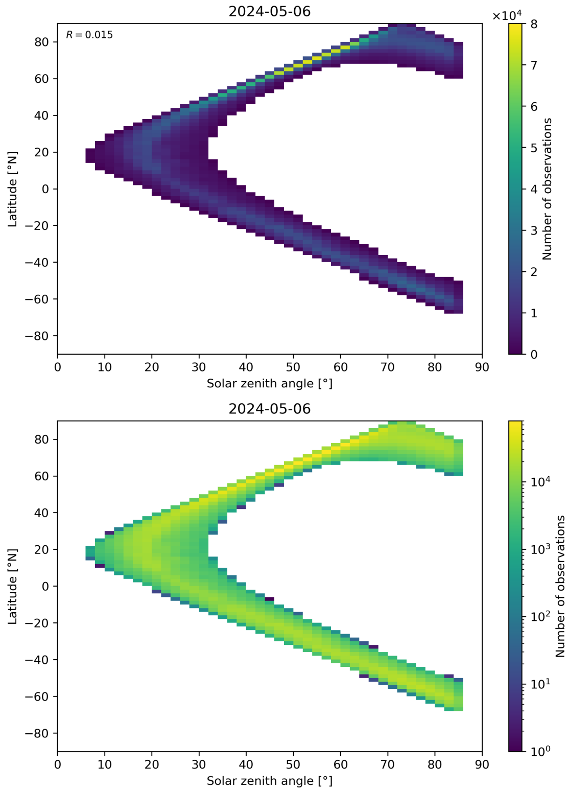
Figure 66: Scatter density plot of “Solar zenith angle” against “Latitude” for 2024-05-05 to 2024-05-07.
