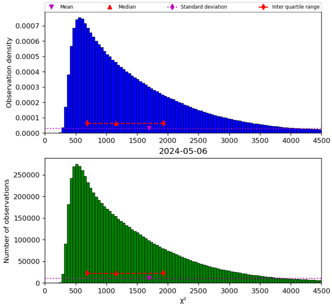
Figure 22: Histogram of “ \chi^2 ” for 2024-05-05 to 2024-05-07
