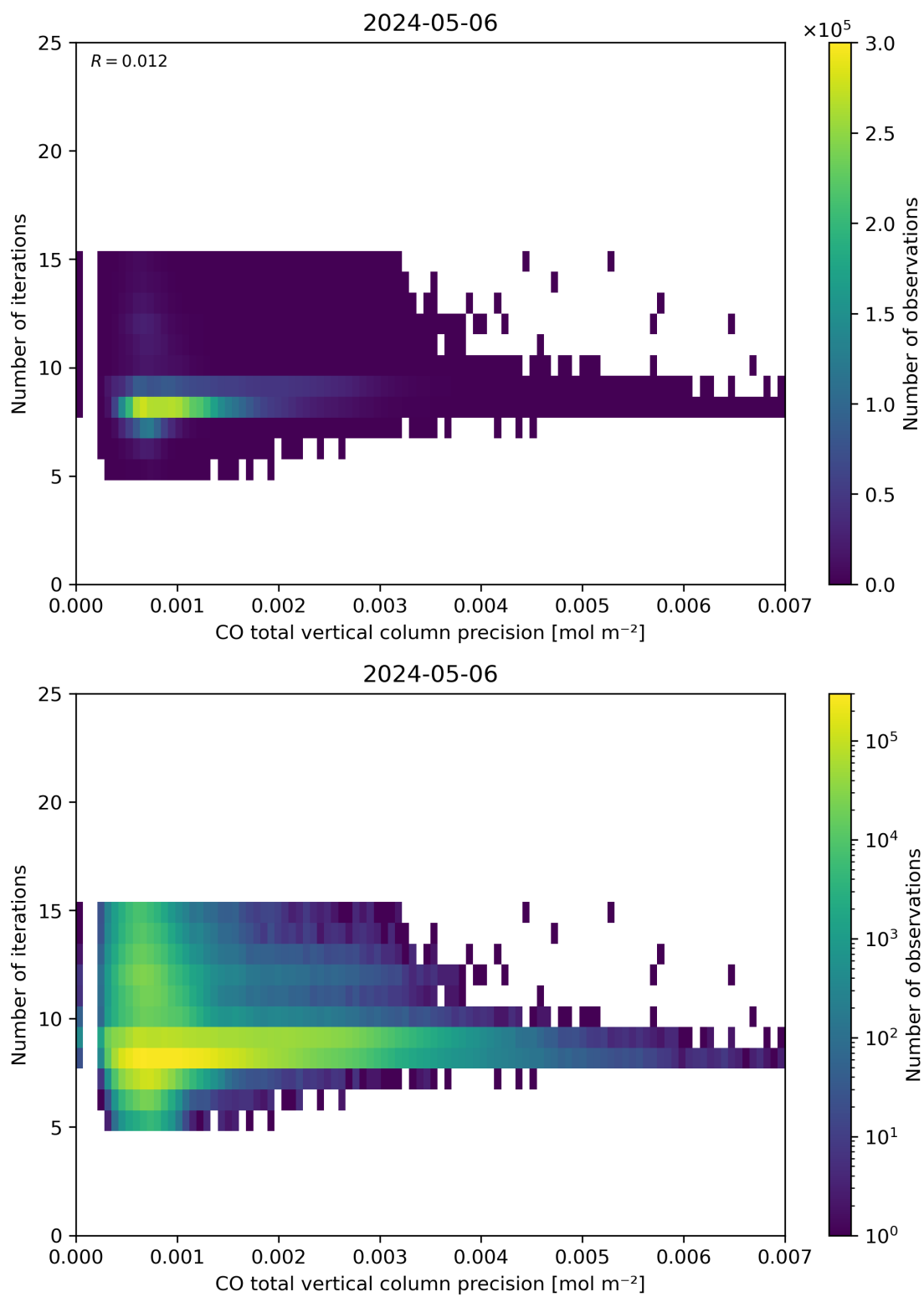
Figure 46: Scatter density plot of “CO total vertical column precision” against “Number of iterations” for 2024-05-05 to 2024-05-07.
