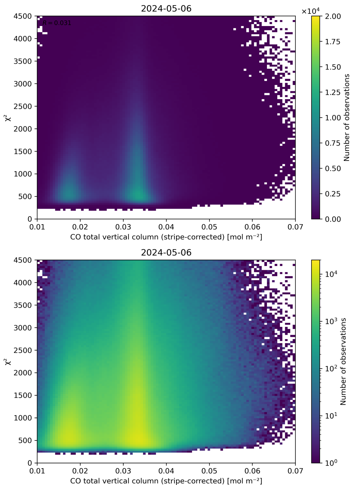
Figure 37: Scatter density plot of “CO total vertical column (stripe-corrected)” against “ \chi^2 ” for 2024-05-05 to 2024-05-07.
