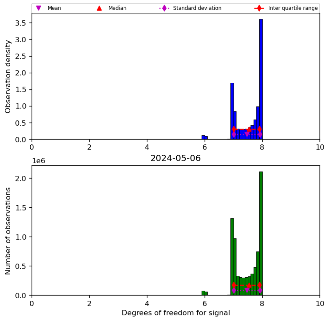
Figure 23: Histogram of “Degrees of freedom for signal” for 2024-05-05 to 2024-05-07
