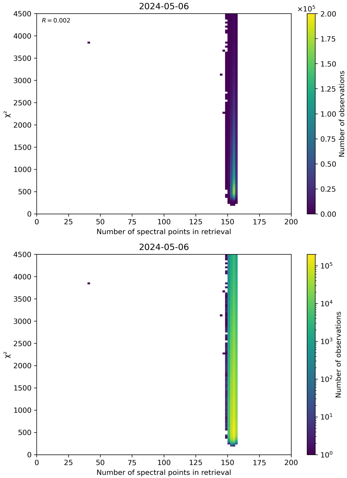
Figure 58: Scatter density plot of “Number of spectral points in retrieval” against “ \chi^2 ” for 2024-05-05 to 2024-05-07.
