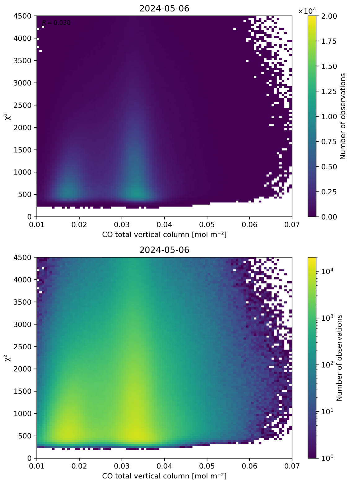
Figure 35: Scatter density plot of “CO total vertical column” against “ \chi^2 ” for 2024-05-05 to 2024-05-07.
