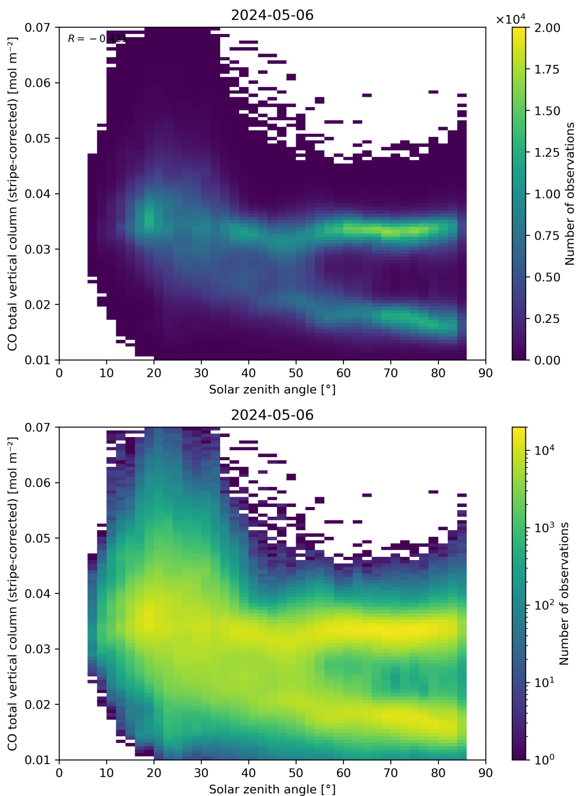
Figure 62: Scatter density plot of “Solar zenith angle” against “CO total vertical column (stripe-corrected)” for 2024-05-05 to 2024-05-07.
