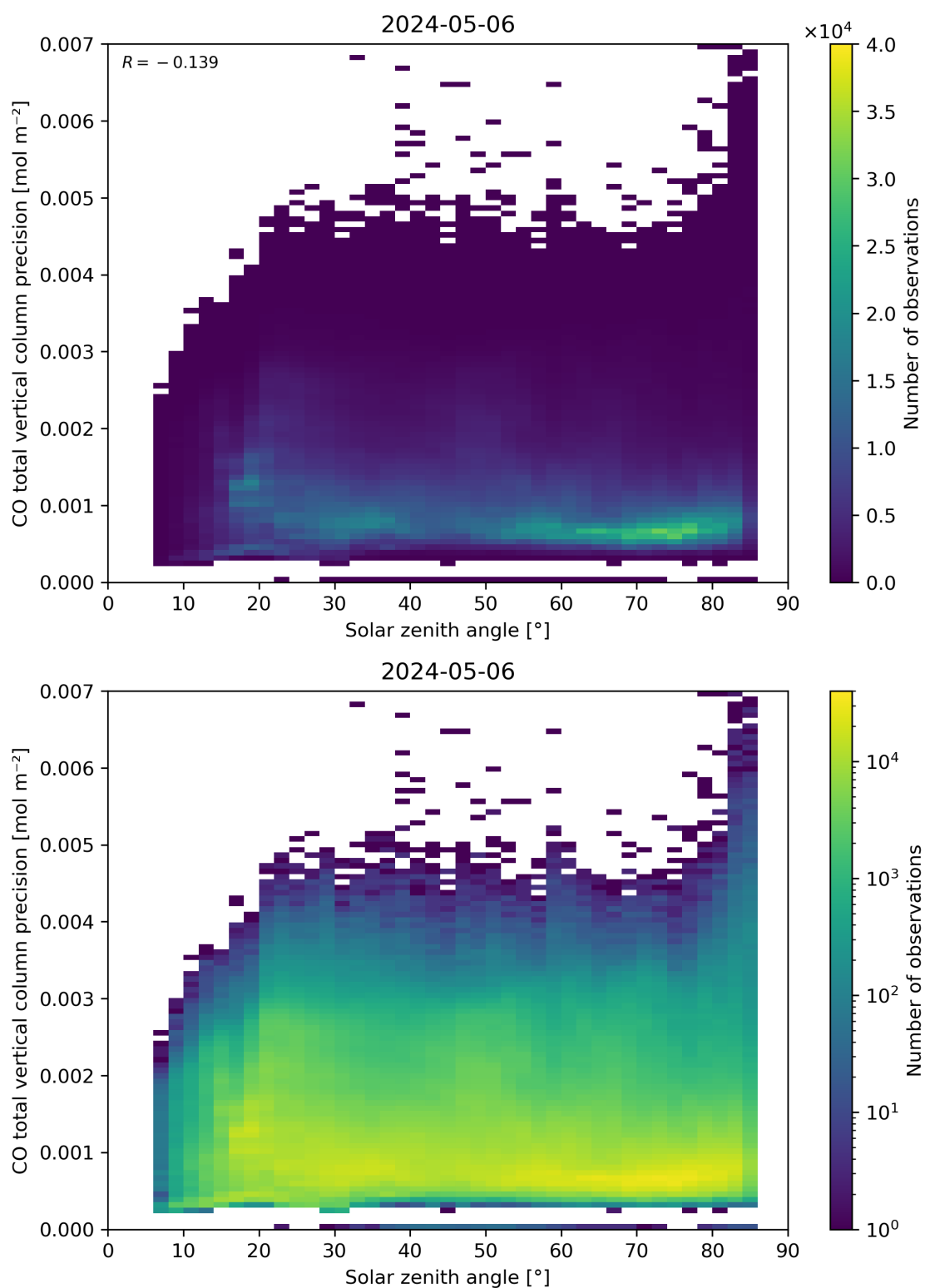
Figure 63: Scatter density plot of “Solar zenith angle” against “CO total vertical column precision” for 2024-05-05 to 2024-05-07.
