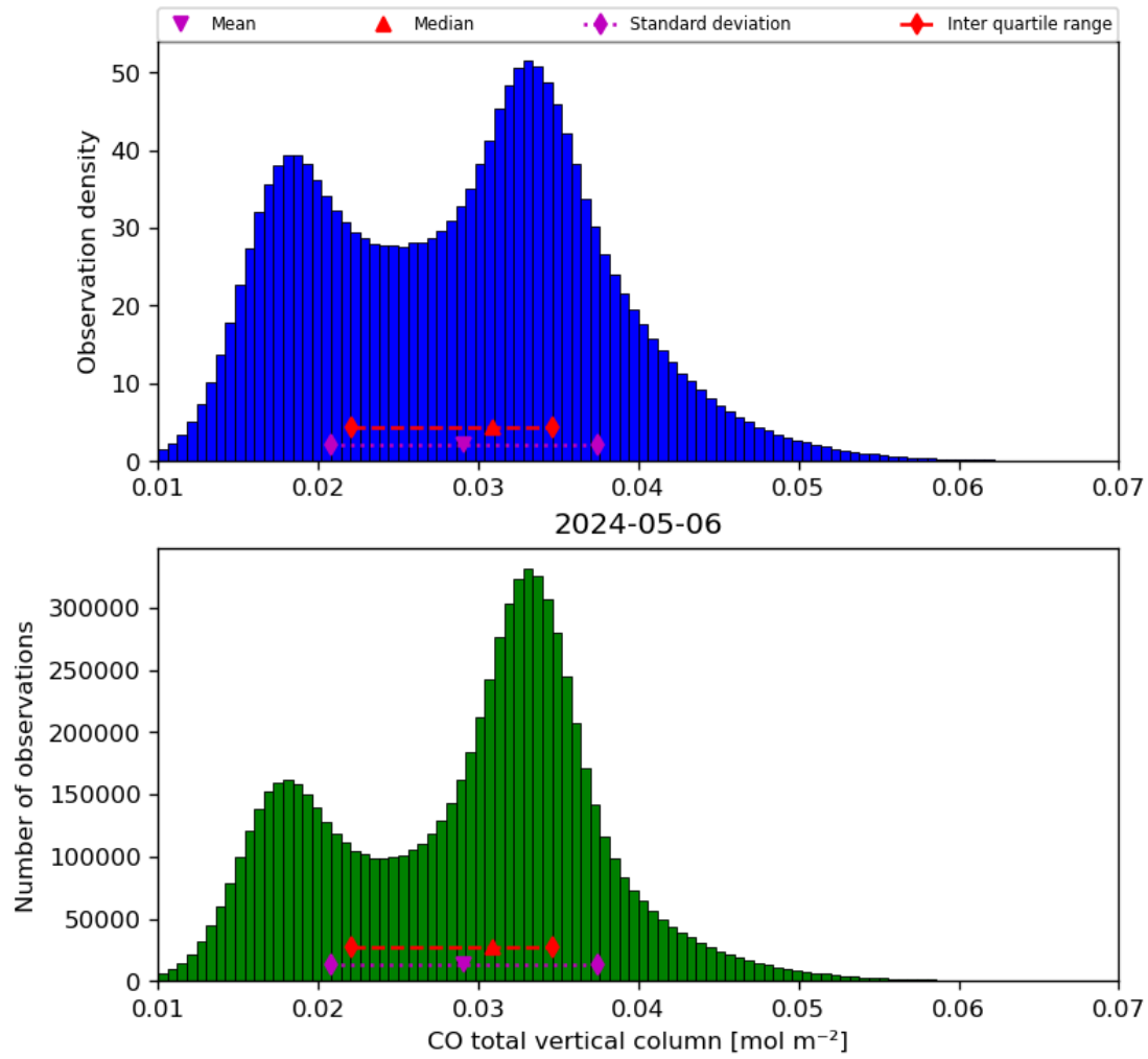
Figure 18: Histogram of “CO total vertical column” for 2024-05-05 to 2024-05-07
