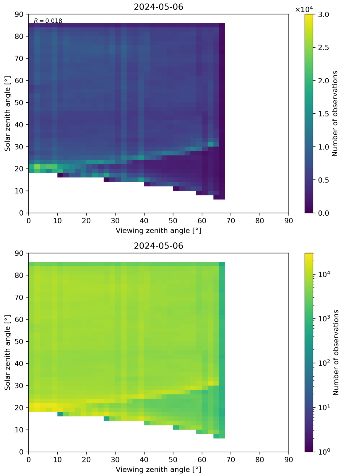
Figure 77: Scatter density plot of “Viewing zenith angle” against “Solar zenith angle” for 2024-05-05 to 2024-05-07.
