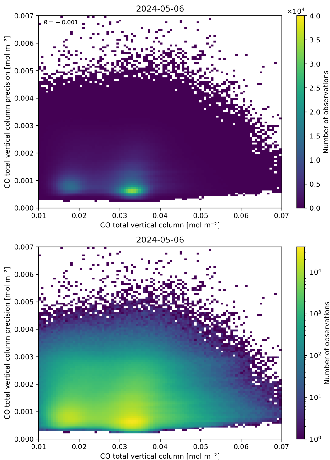
Figure 34: Scatter density plot of “CO total vertical column” against “CO total vertical column precision” for 2024-05-05 to 2024-05-07.
