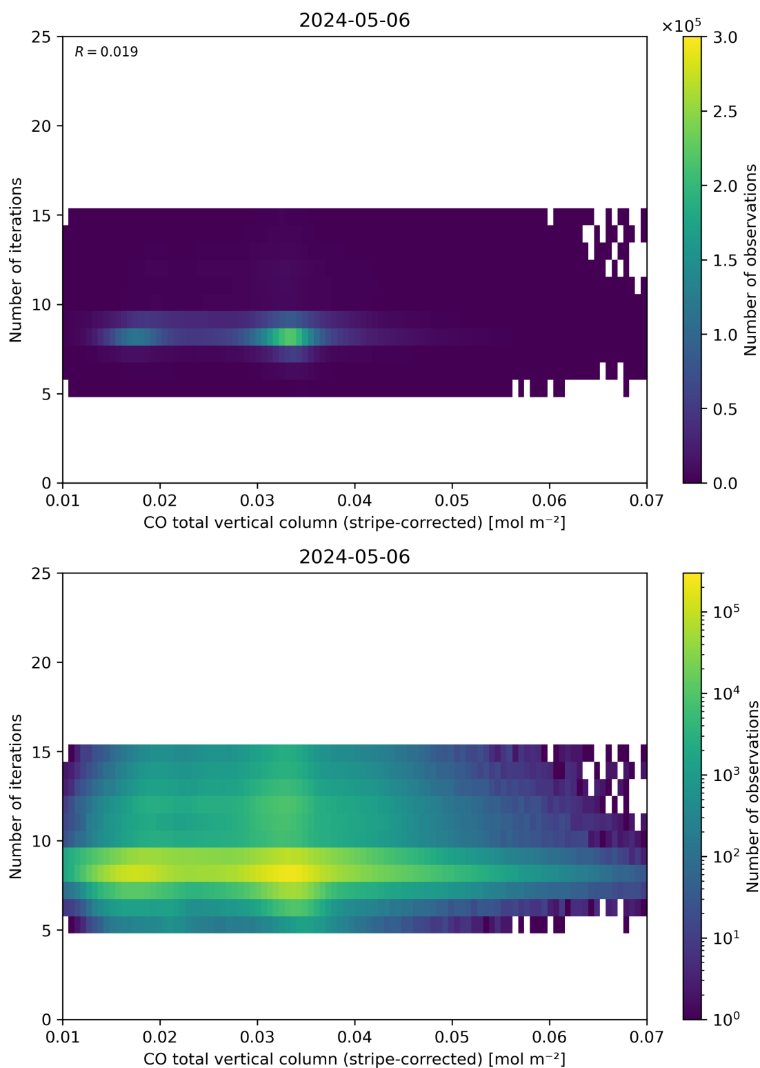
Figure 39: Scatter density plot of “CO total vertical column (stripe-corrected)” against “Number of iterations” for 2024-05-05 to 2024-05-07.
