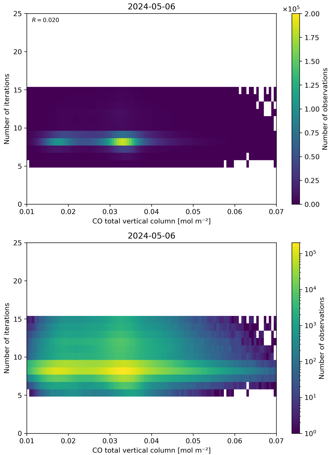
Figure 42: Scatter density plot of “CO total vertical column” against “Number of iterations” for 2024-05-05 to 2024-05-07.
