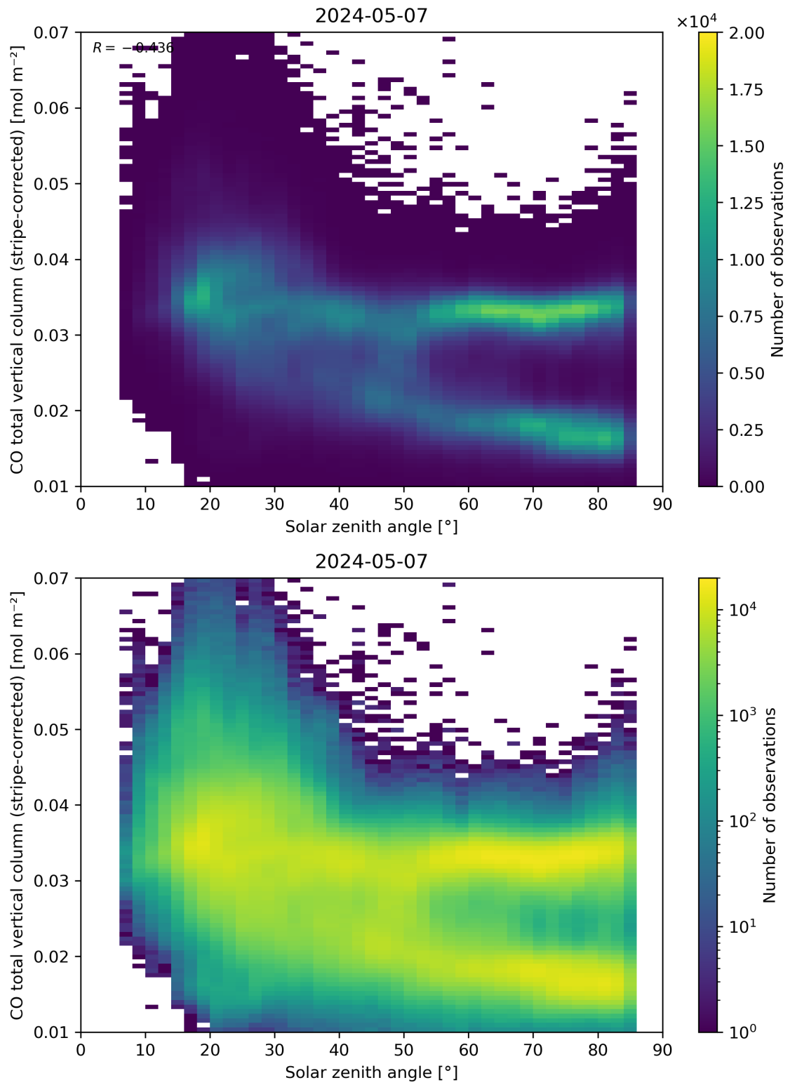
Figure 62: Scatter density plot of “Solar zenith angle” against “CO total vertical column (stripe-corrected)” for 2024-05-07 to 2024-05-08.
