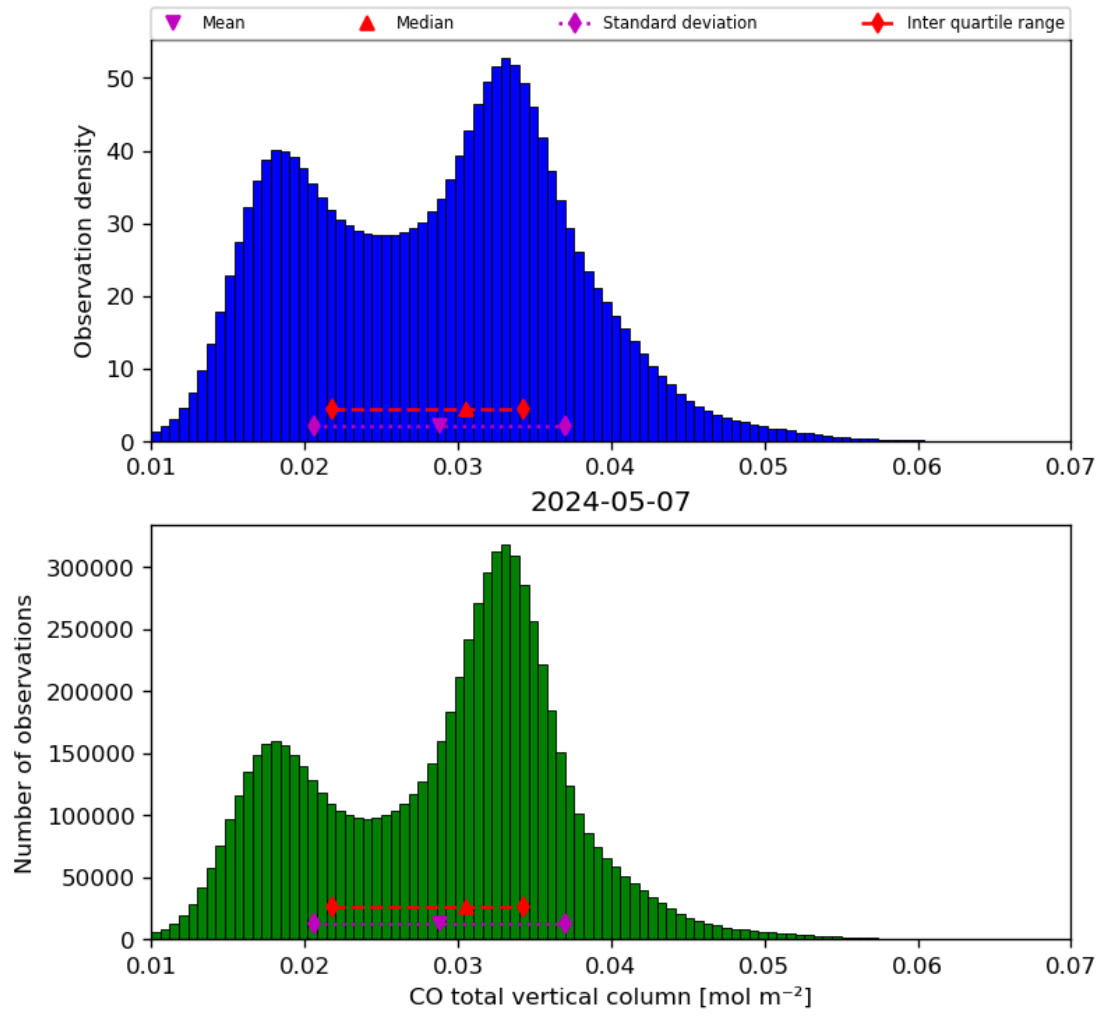
Figure 18: Histogram of “CO total vertical column” for 2024-05-07 to 2024-05-08
