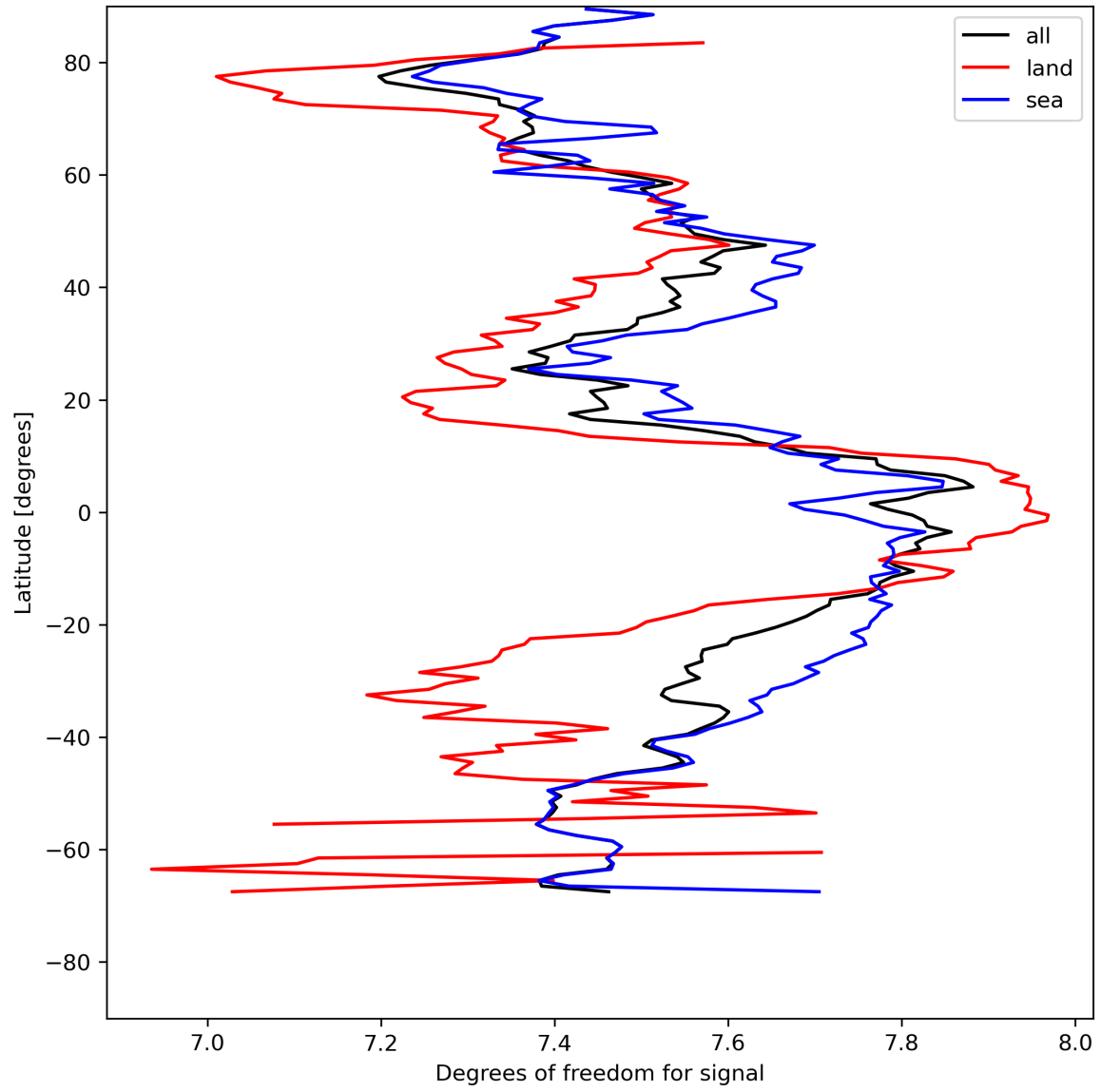
Figure 15: Zonal average of “Degrees of freedom for signal” for 2024-05-07 to 2024-05-08.
