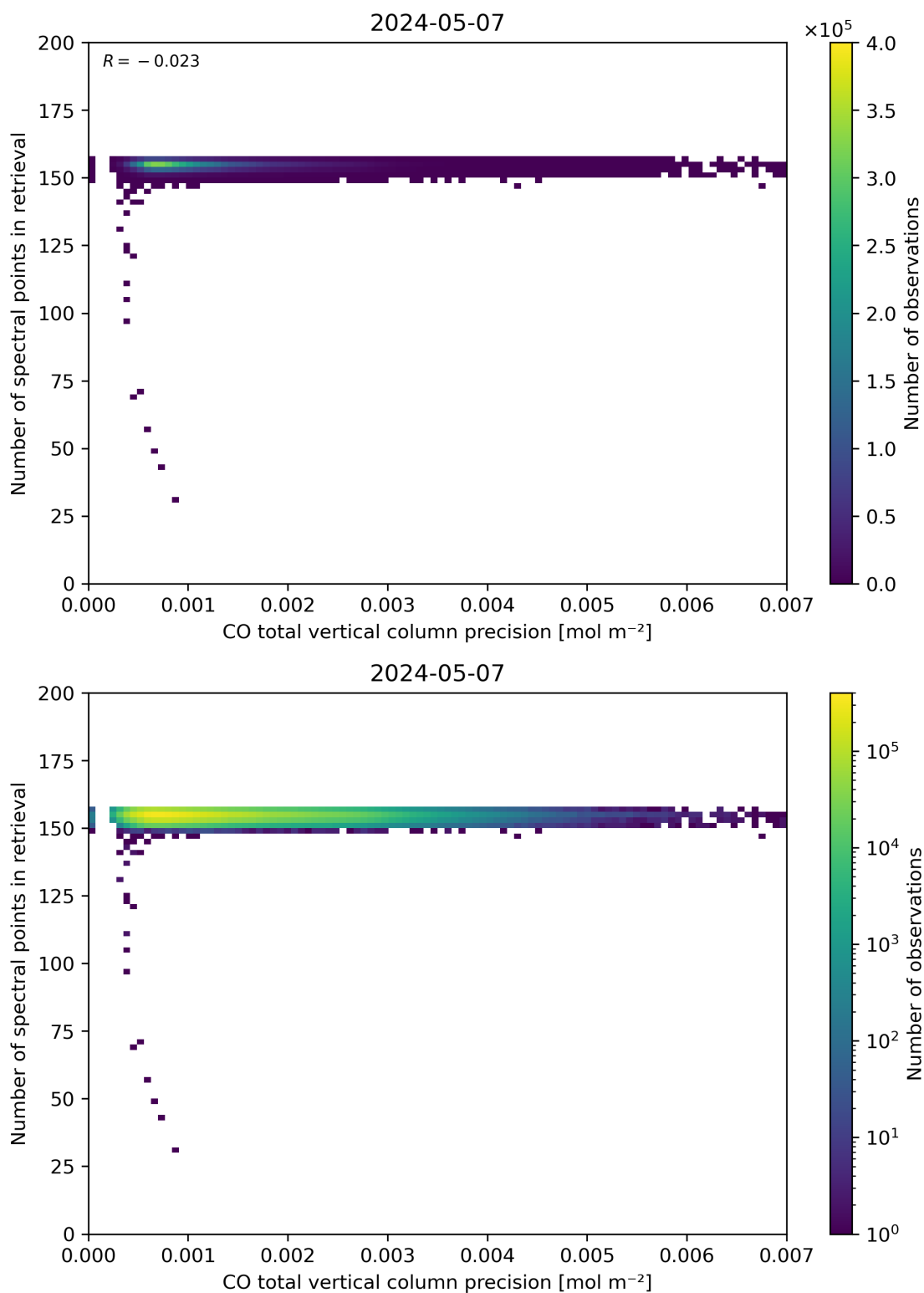
Figure 47: Scatter density plot of “CO total vertical column precision” against “Number of spectral points in retrieval” for 2024-05-07 to 2024-05-08.
