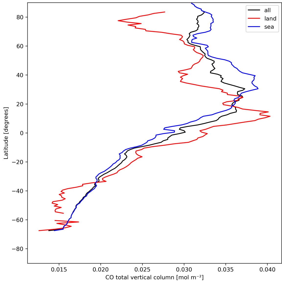
Figure 10: Zonal average of “CO total vertical column” for 2024-05-07 to 2024-05-08.
