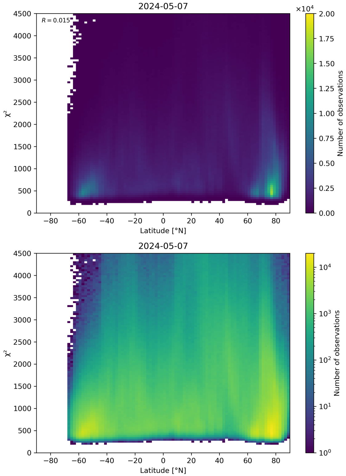
Figure 54: Scatter density plot of “Latitude” against “ \chi^2 ” for 2024-05-07 to 2024-05-08.
