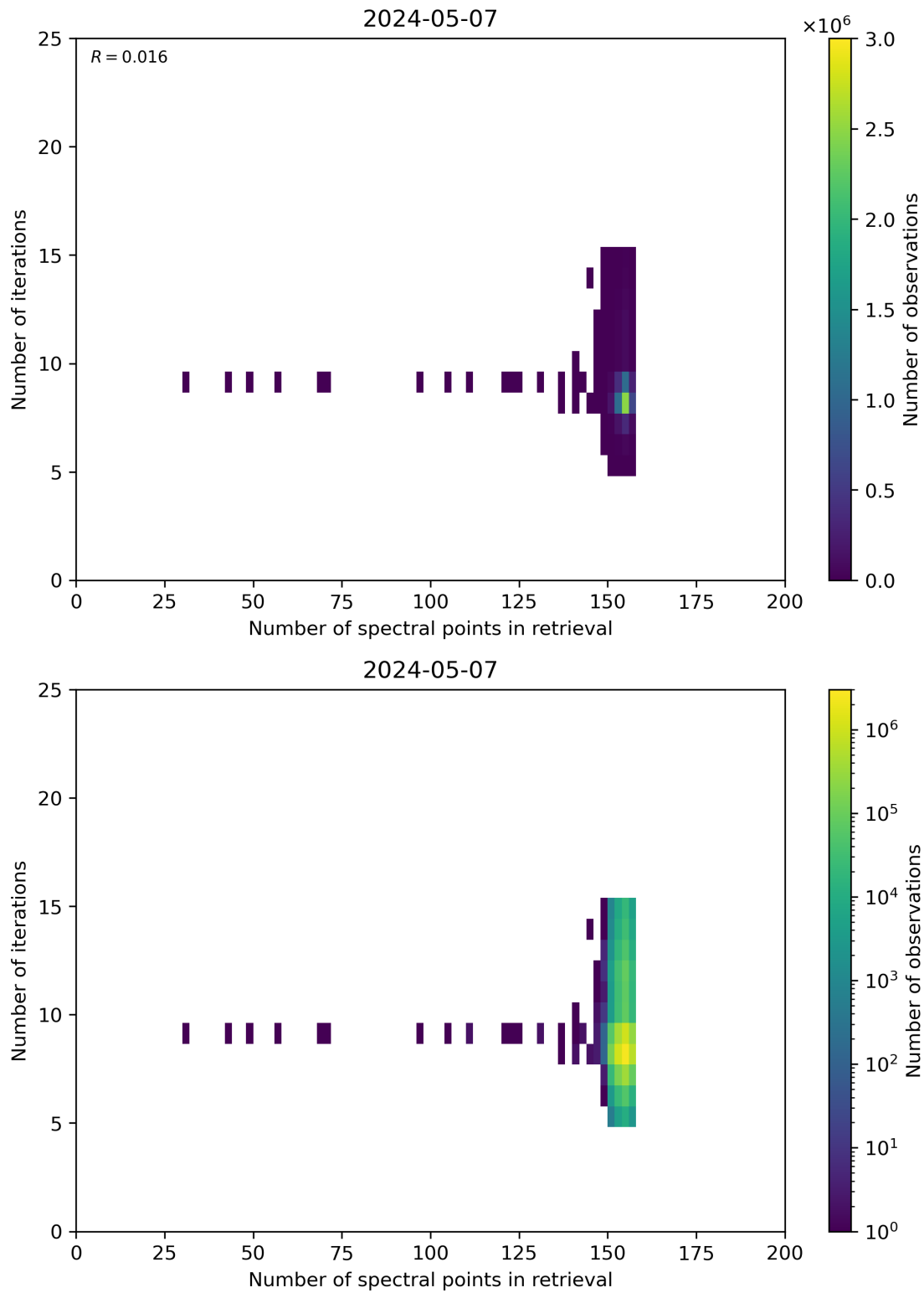
Figure 60: Scatter density plot of “Number of spectral points in retrieval” against “Number of iterations” for 2024-05-07 to 2024-05-08.
