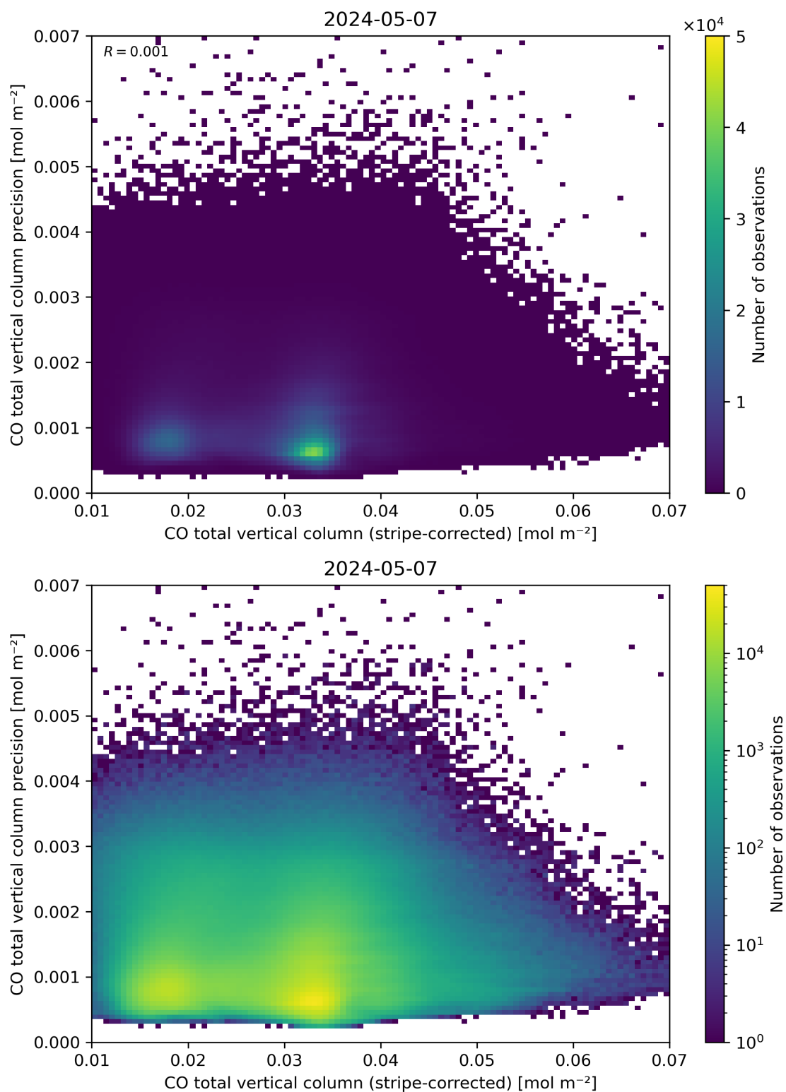
Figure 36: Scatter density plot of “CO total vertical column (stripe-corrected)” against “CO total vertical column precision” for 2024-05-07 to 2024-05-08.
