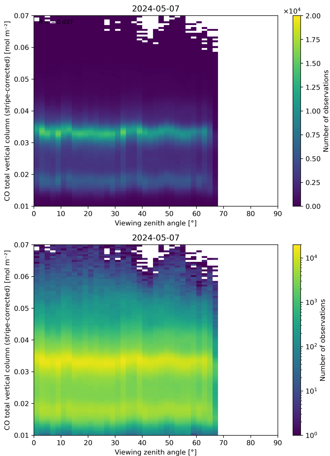
Figure 70: Scatter density plot of “Viewing zenith angle” against “CO total vertical column (stripe-corrected)” for 2024-05-07 to 2024-05-08.
