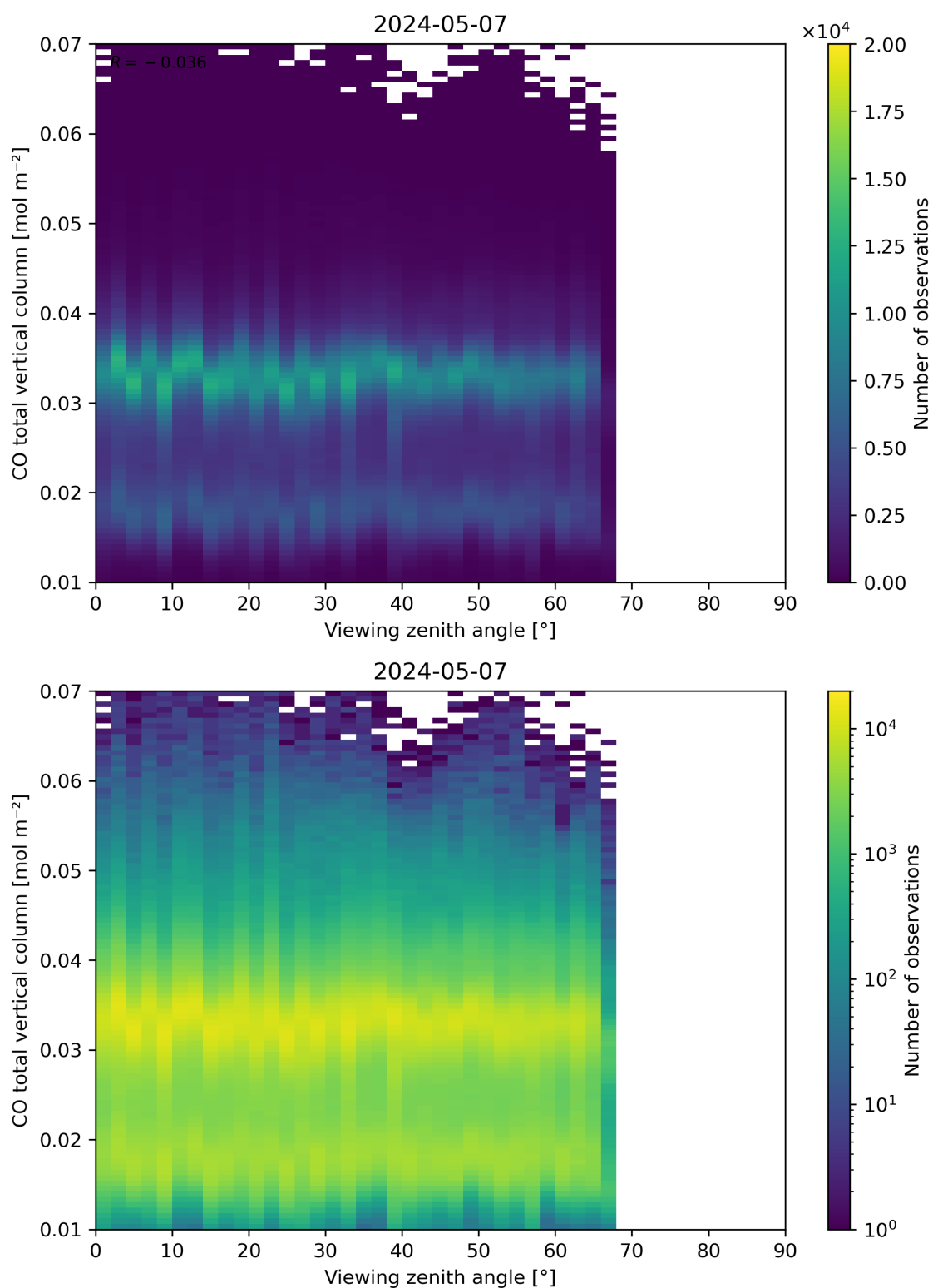
Figure 69: Scatter density plot of “Viewing zenith angle” against “CO total vertical column” for 2024-05-07 to 2024-05-08.
