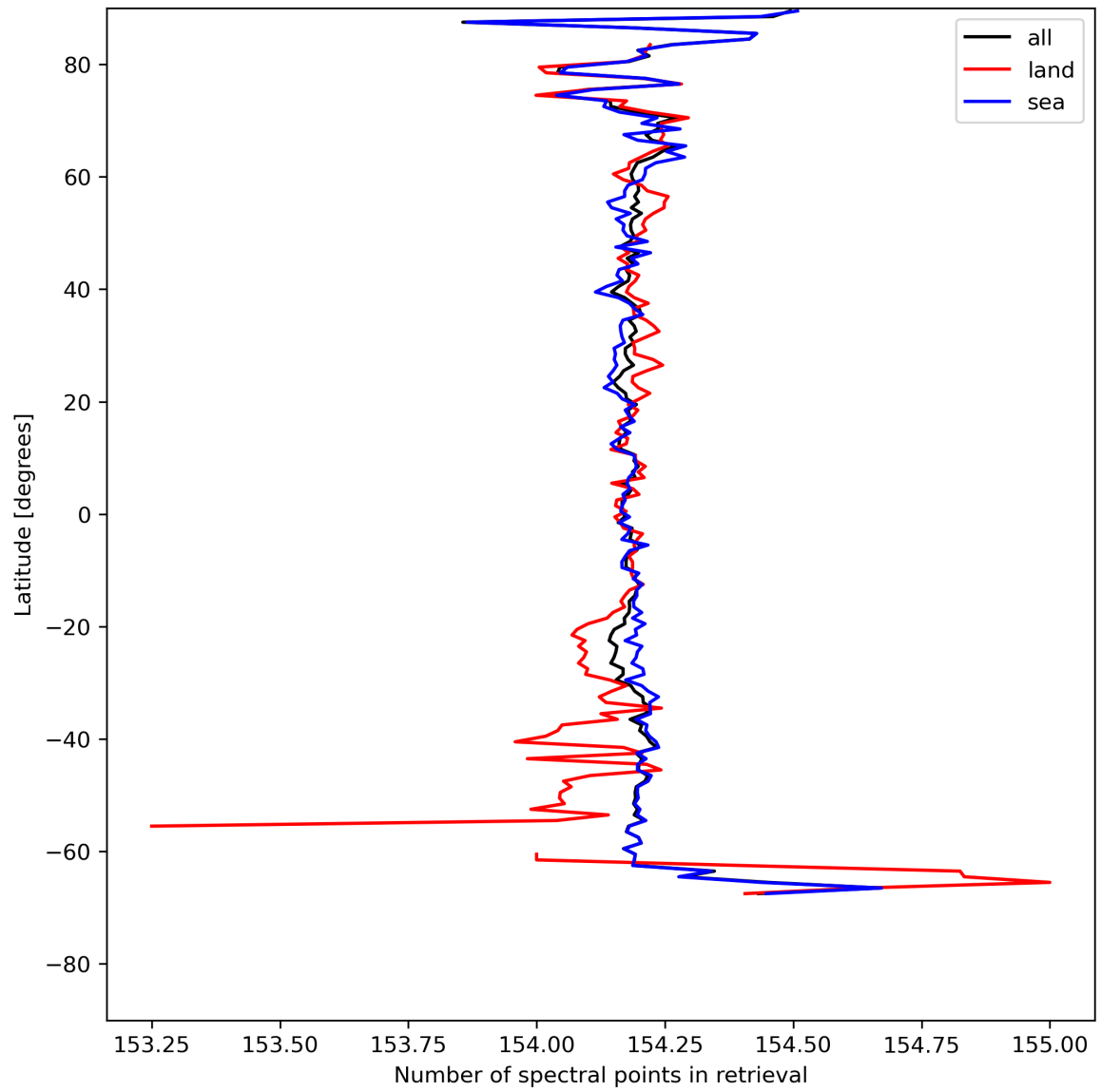
Figure 13: Zonal average of “Number of spectral points in retrieval” for 2024-05-07 to 2024-05-08.
