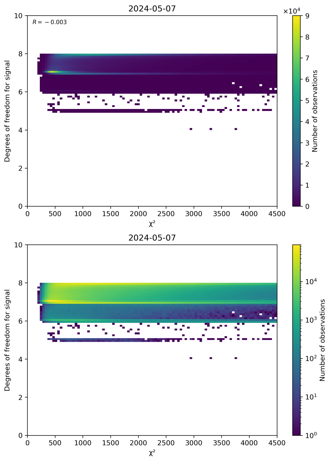
Figure 48: Scatter density plot of “ \chi^2 ” against “Degrees of freedom for signal” for 2024-05-07 to 2024-05-08.
