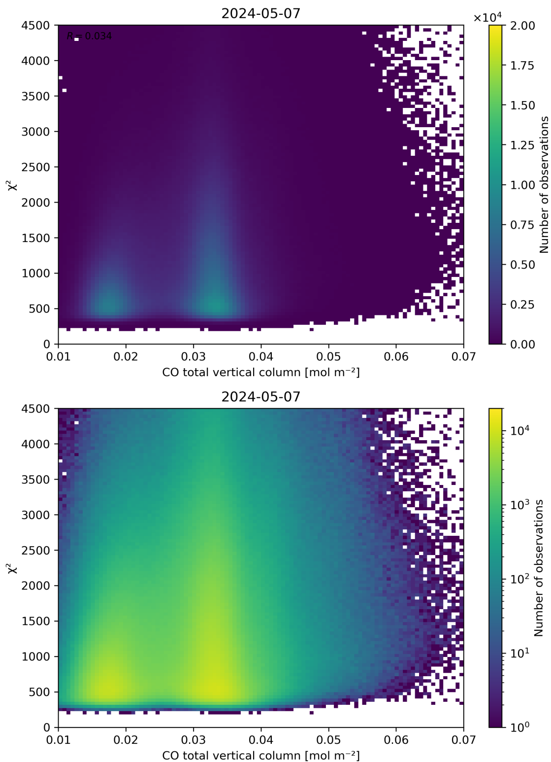
Figure 35: Scatter density plot of “CO total vertical column” against “ \chi^2 ” for 2024-05-07 to 2024-05-08.
