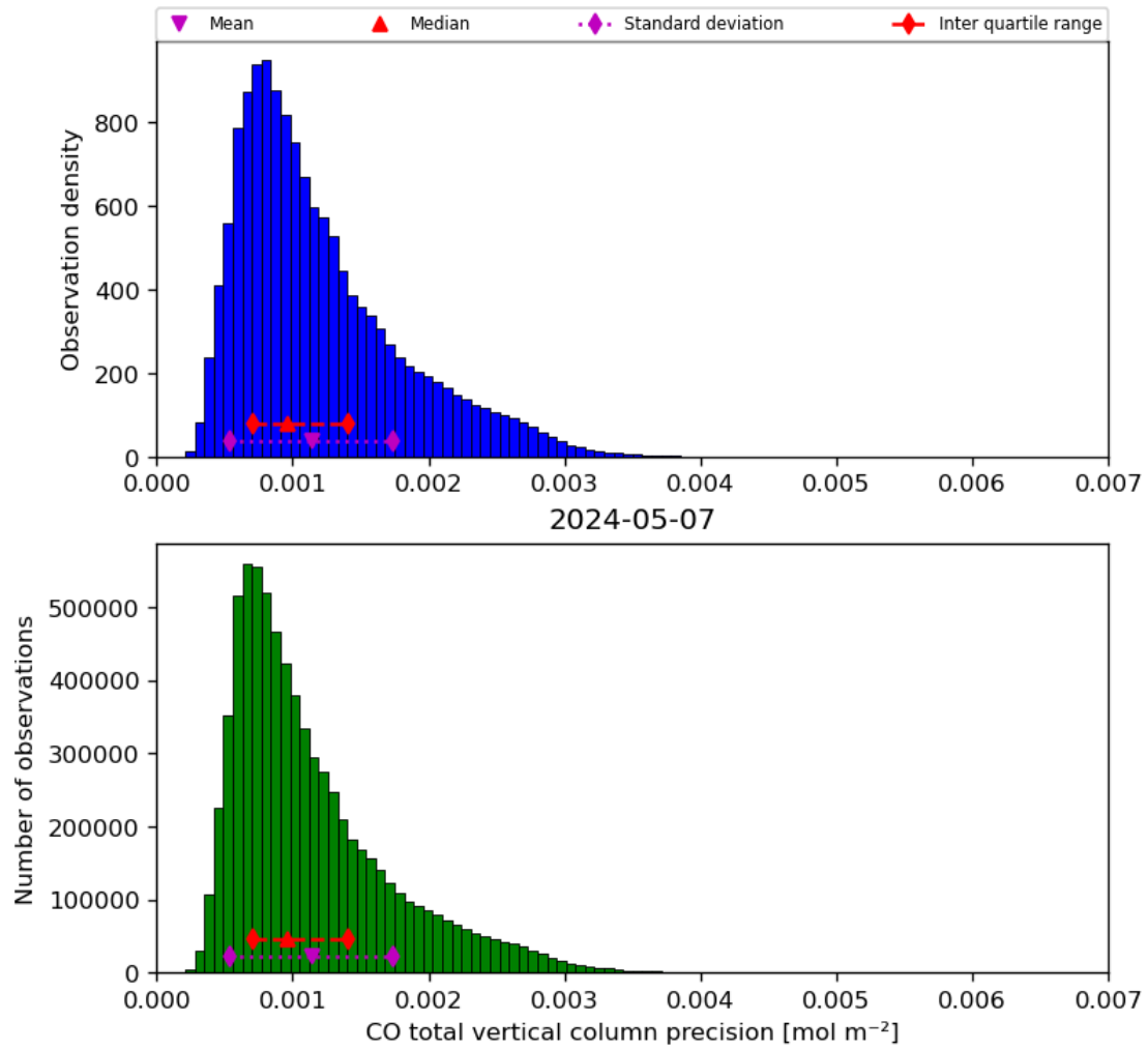
Figure 20: Histogram of “CO total vertical column precision” for 2024-05-07 to 2024-05-08
