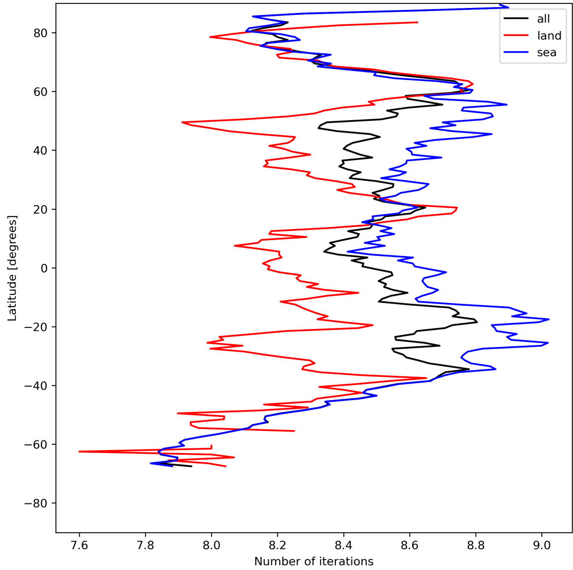
Figure 16: Zonal average of “Number of iterations” for 2024-05-07 to 2024-05-08.
