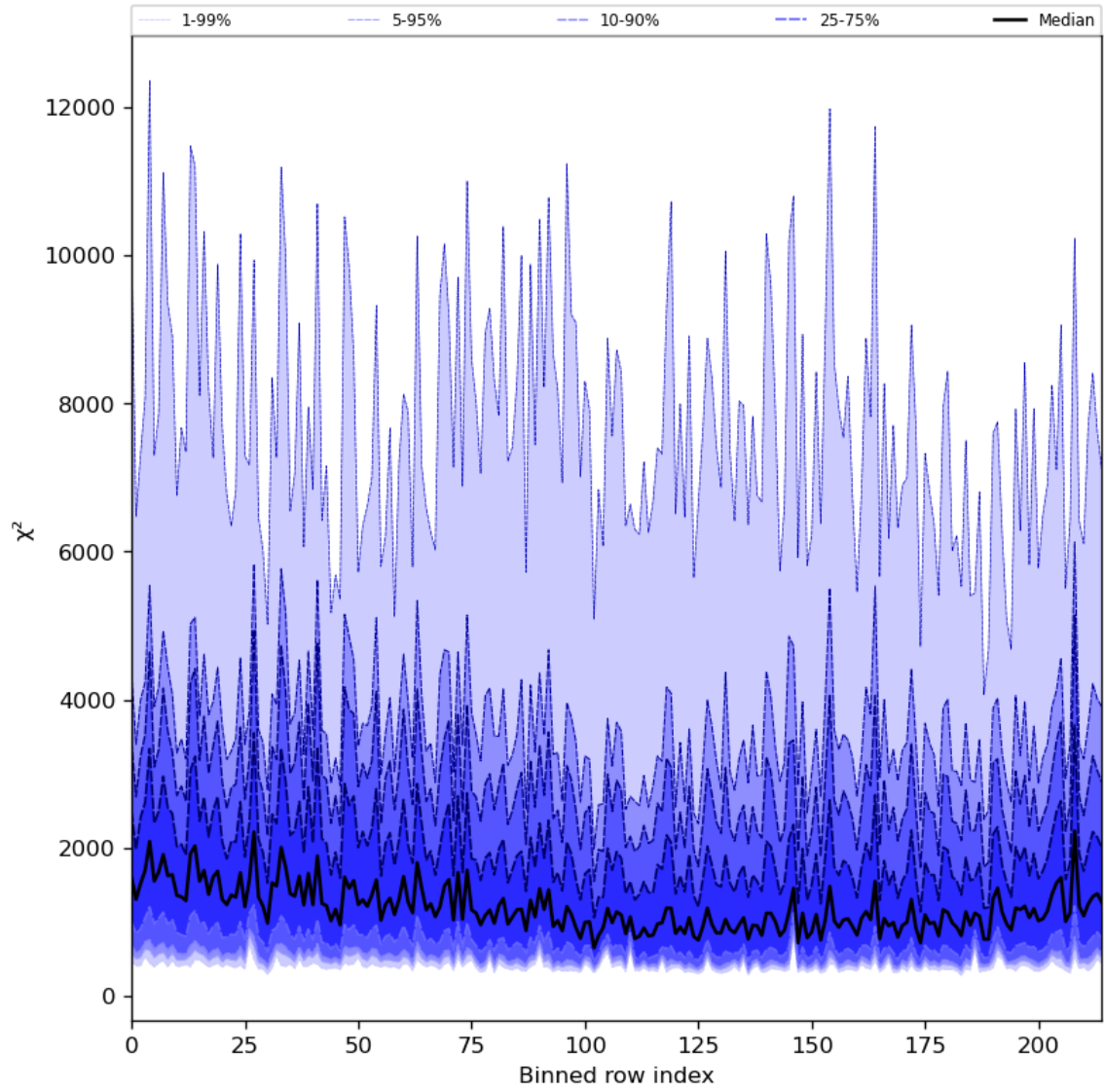
Figure 30: Along track statistics of “ \chi^2 ” for 2024-05-07 to 2024-05-08
