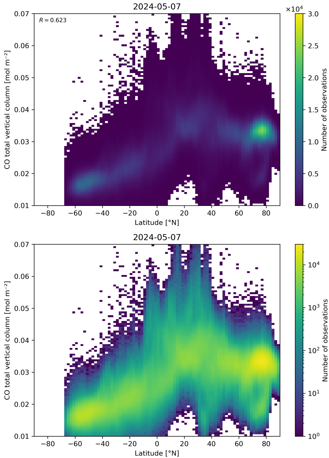
Figure 51: Scatter density plot of “Latitude” against “CO total vertical column” for 2024-05-07 to 2024-05-08.
