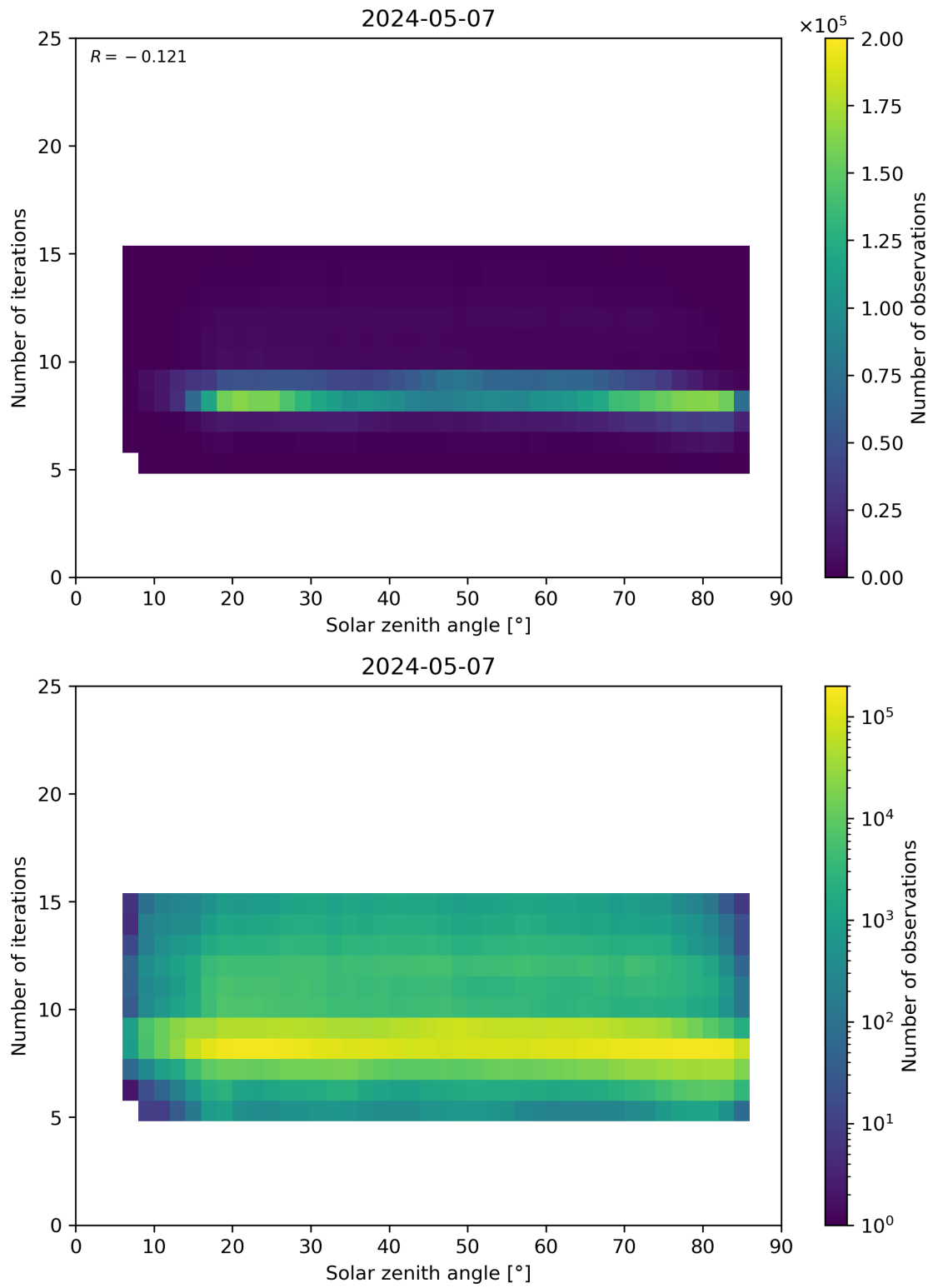
Figure 67: Scatter density plot of “Solar zenith angle” against “Number of iterations” for 2024-05-07 to 2024-05-08.
