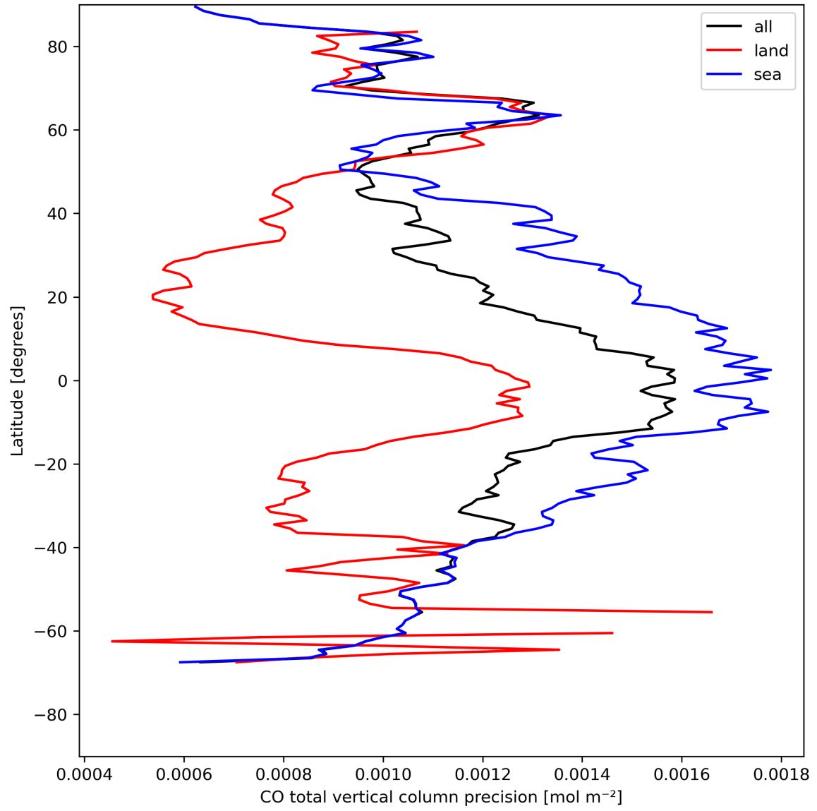
Figure 12: Zonal average of “CO total vertical column precision” for 2024-05-07 to 2024-05-08.
