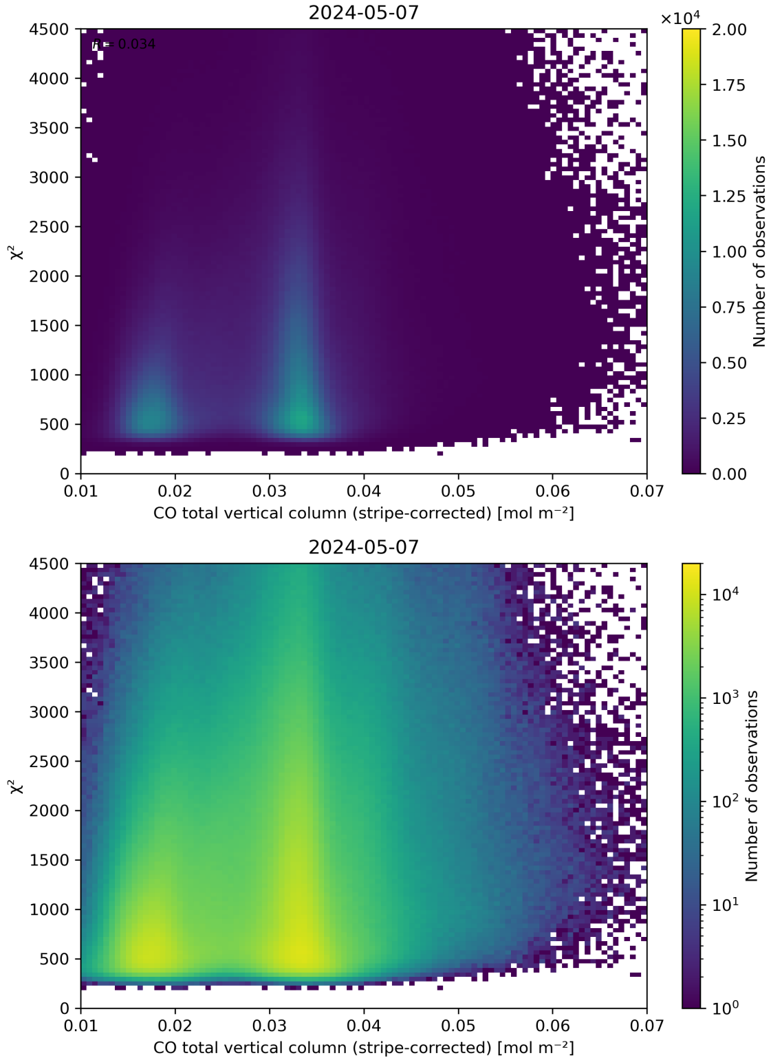
Figure 37: Scatter density plot of “CO total vertical column (stripe-corrected)” against “ \chi^2 ” for 2024-05-07 to 2024-05-08.
