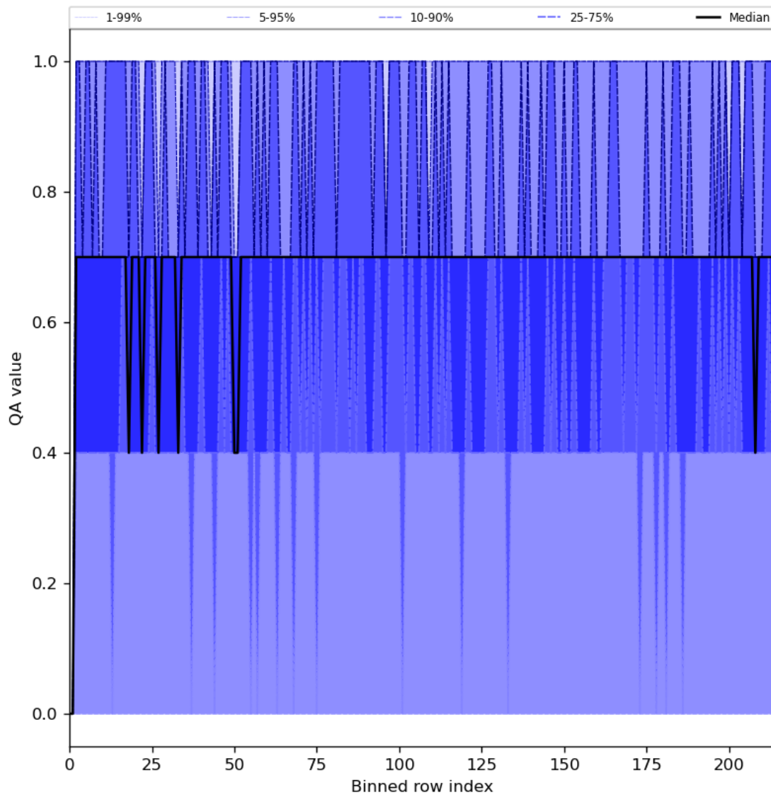
Figure 25: Along track statistics of “QA value” for 2024-05-07 to 2024-05-08
