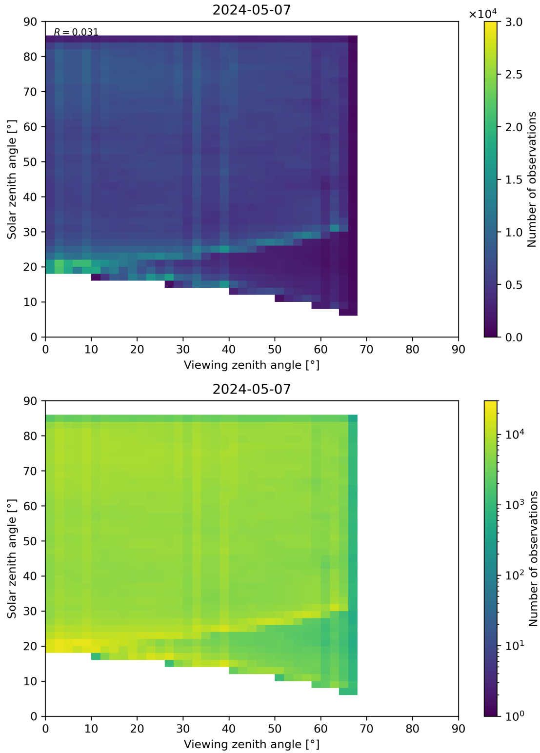
Figure 77: Scatter density plot of “Viewing zenith angle” against “Solar zenith angle” for 2024-05-07 to 2024-05-08.
