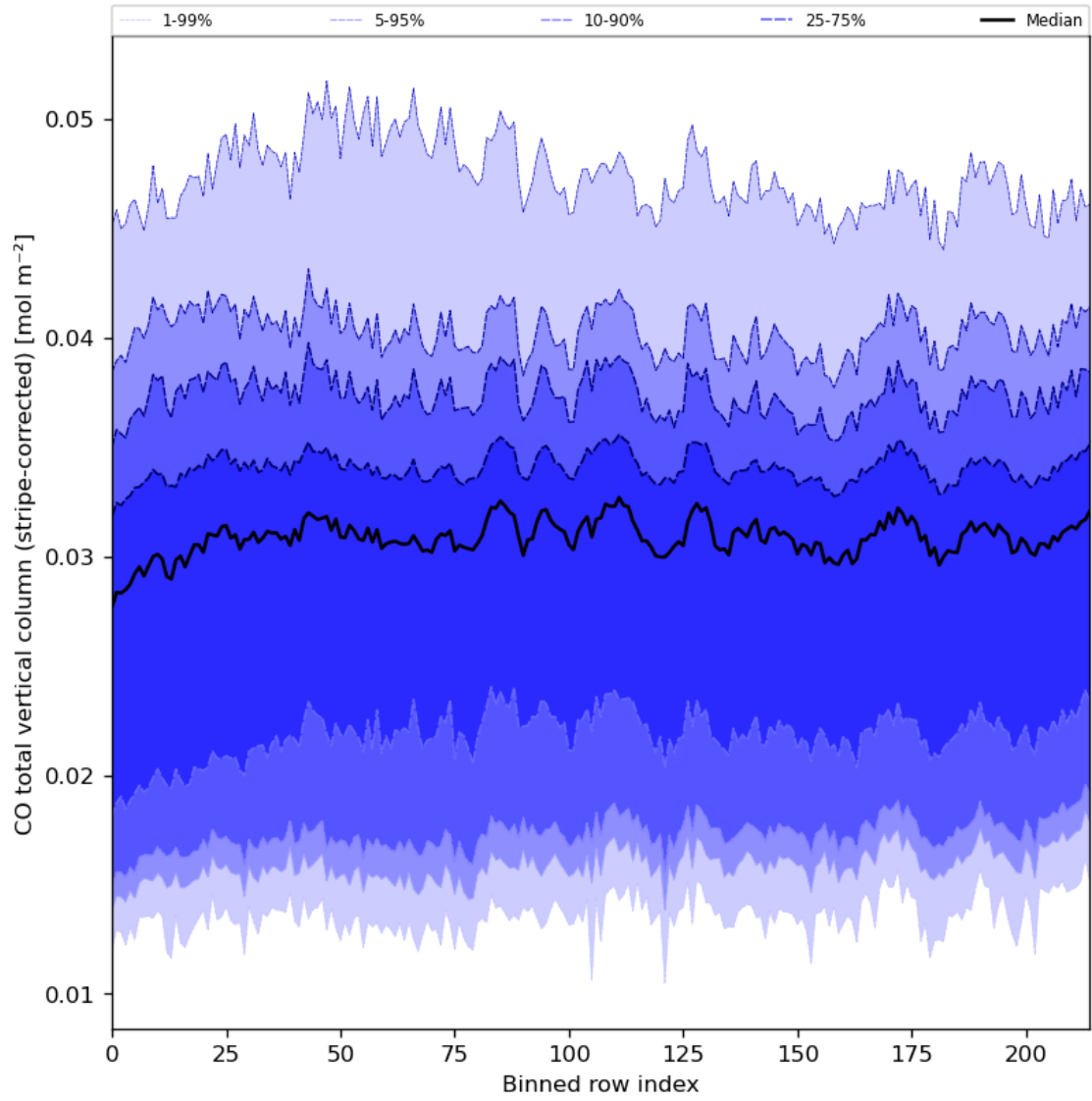
Figure 27: Along track statistics of “CO total vertical column (stripe-corrected)” for 2024-05-07 to 2024-05-08
