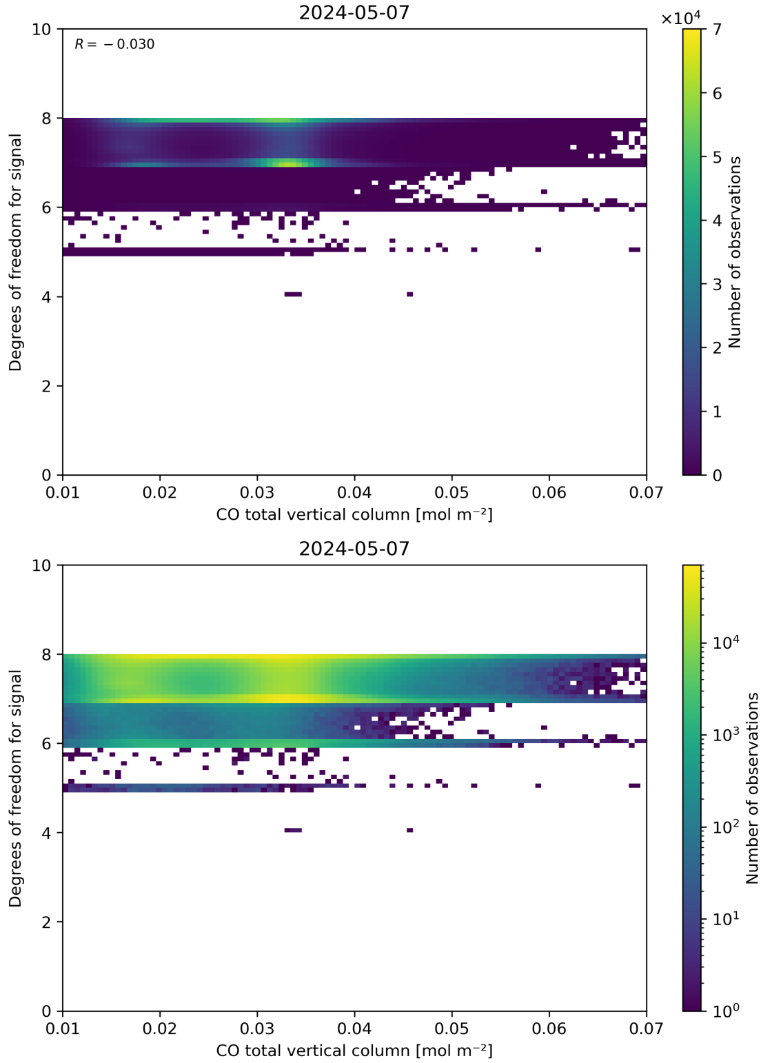
Figure 41: Scatter density plot of “CO total vertical column” against “Degrees of freedom for signal” for 2024-05-07 to 2024-05-08.
