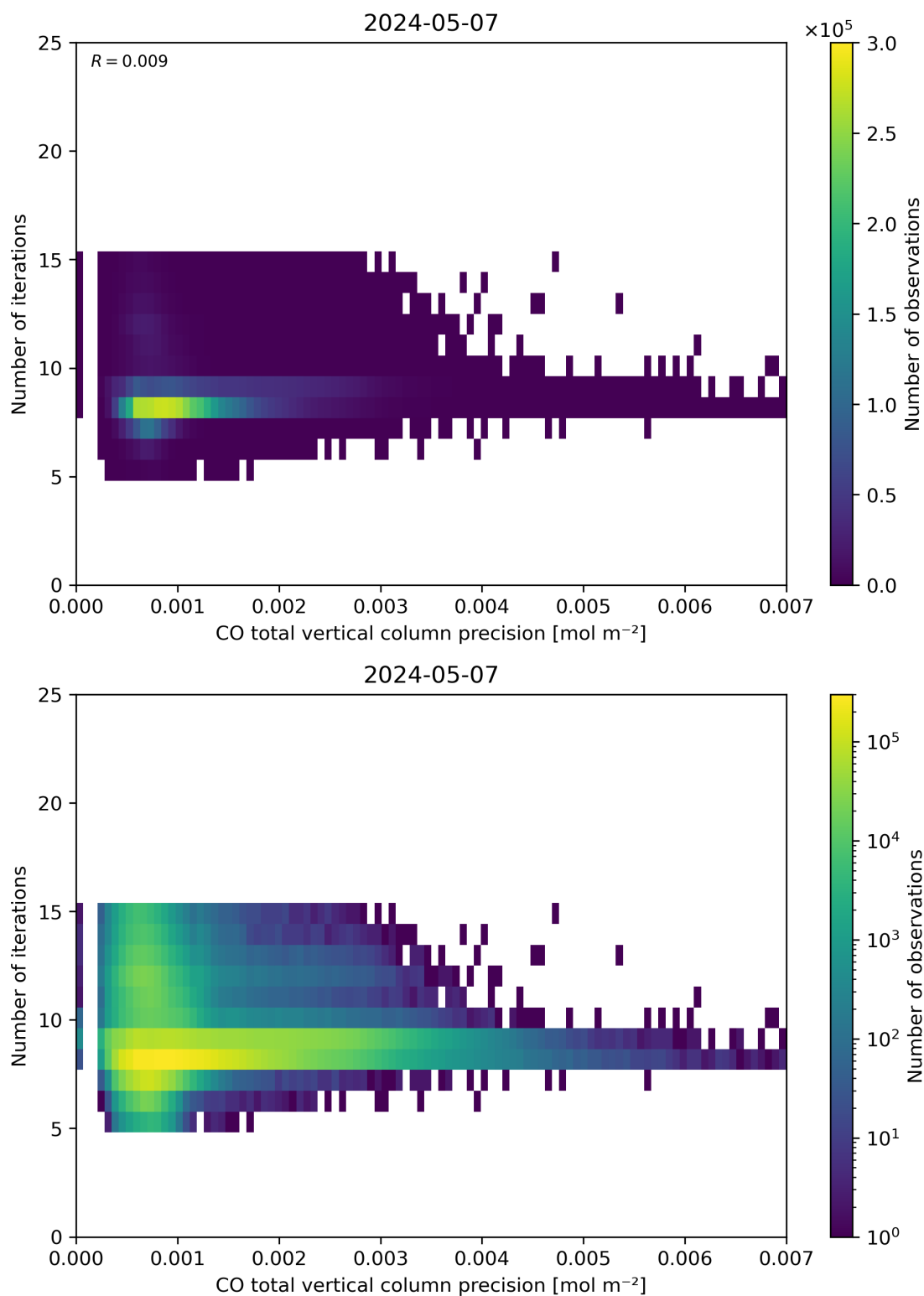
Figure 46: Scatter density plot of “CO total vertical column precision” against “Number of iterations” for 2024-05-07 to 2024-05-08.
