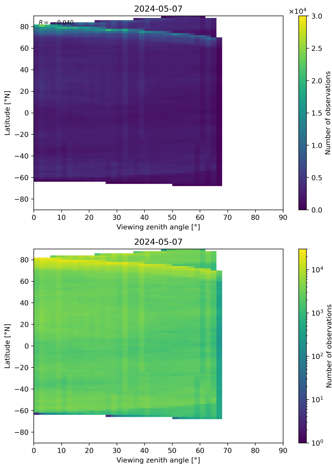
Figure 74: Scatter density plot of “Viewing zenith angle” against “Latitude” for 2024-05-07 to 2024-05-08.
