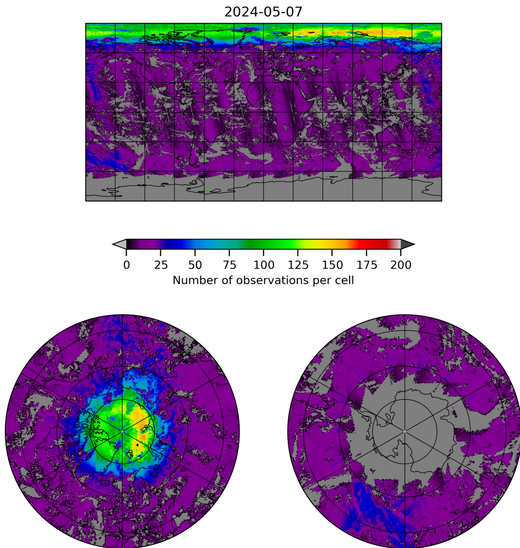
Figure 8: Map of the number of observations for 2024-05-07 to 2024-05-08
