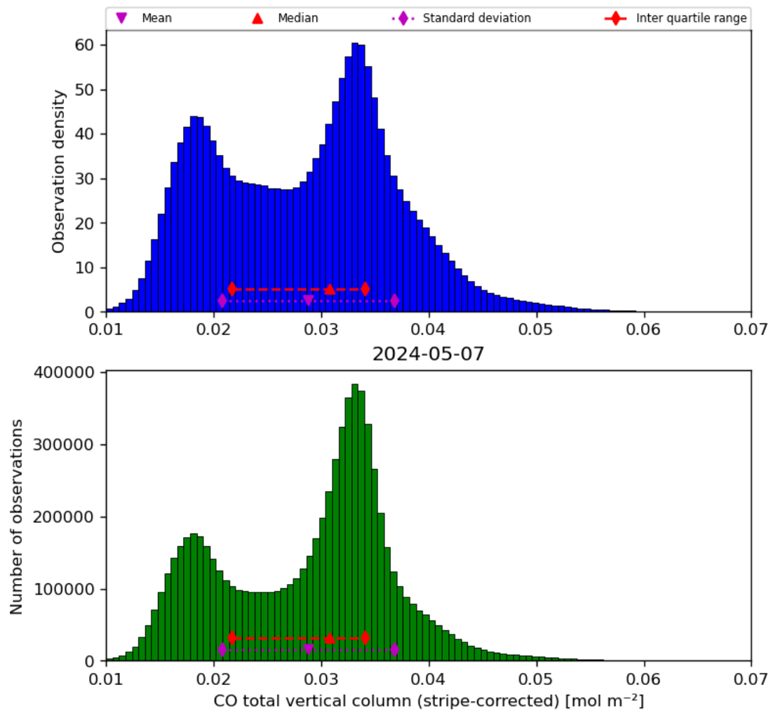
Figure 19: Histogram of “CO total vertical column (stripe-corrected)” for 2024-05-07 to 2024-05-08
