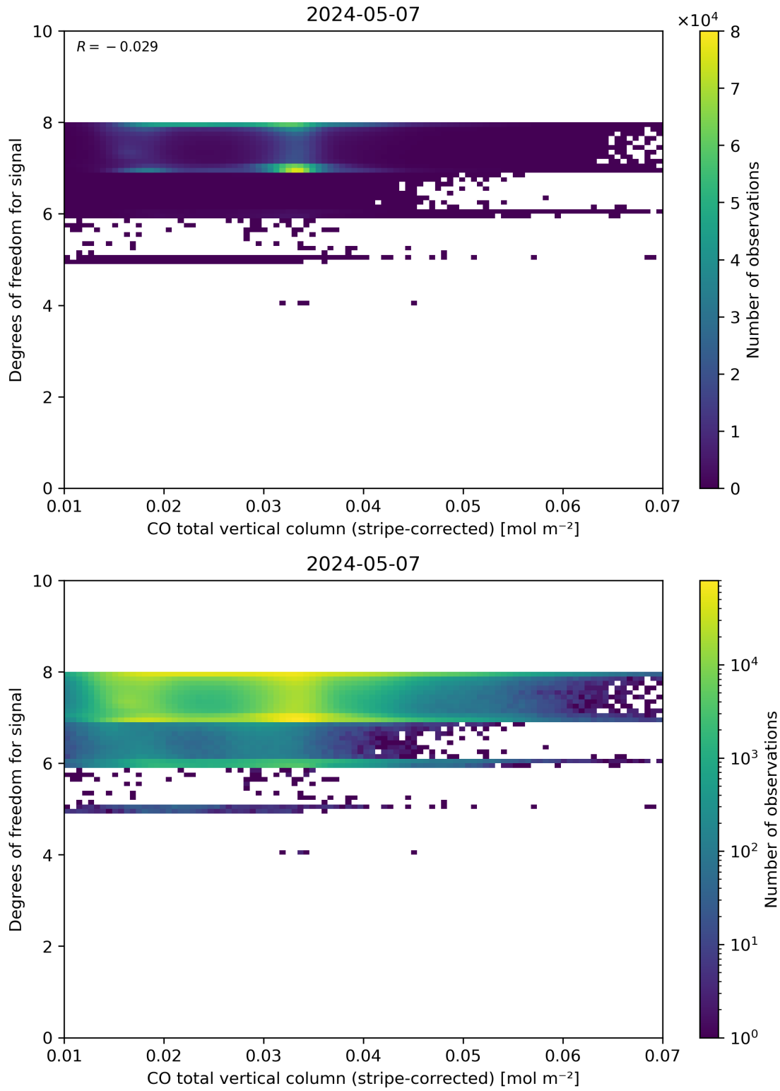
Figure 38: Scatter density plot of “CO total vertical column (stripe-corrected)” against “Degrees of freedom for signal” for 2024-05-07 to 2024-05-08.
