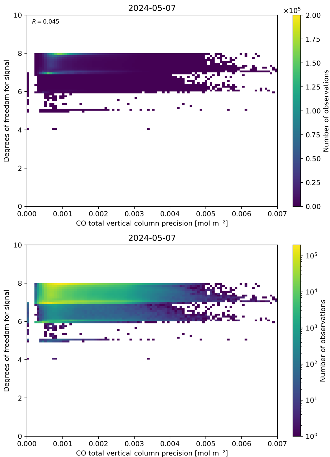
Figure 45: Scatter density plot of “CO total vertical column precision” against “Degrees of freedom for signal” for 2024-05-07 to 2024-05-08.
