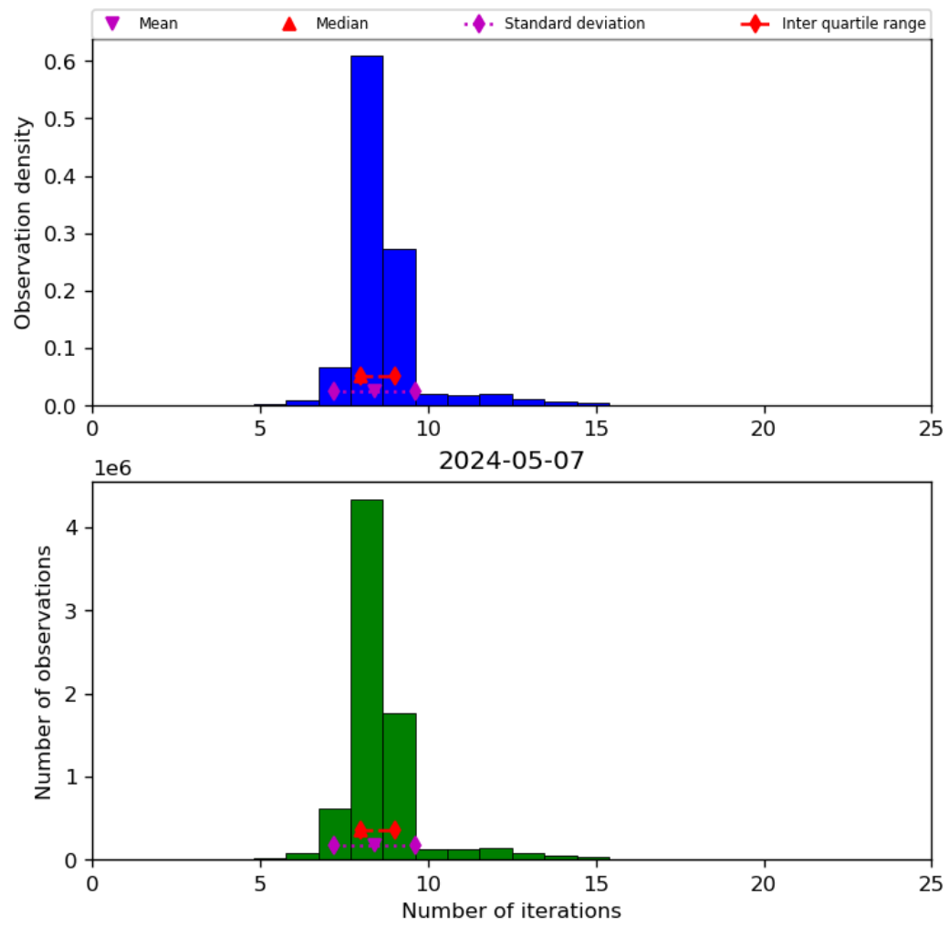
Figure 24: Histogram of “Number of iterations” for 2024-05-07 to 2024-05-08
