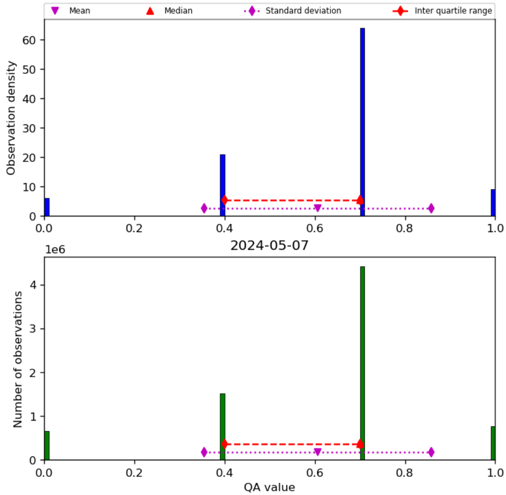
Figure 17: Histogram of “QA value” for 2024-05-07 to 2024-05-08
