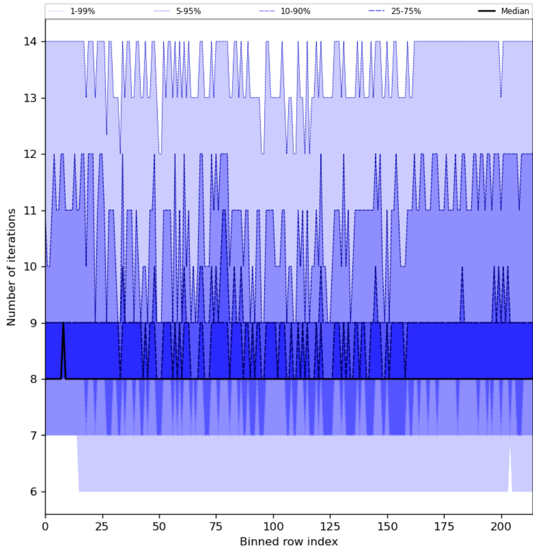
Figure 32: Along track statistics of “Number of iterations” for 2024-05-07 to 2024-05-08
