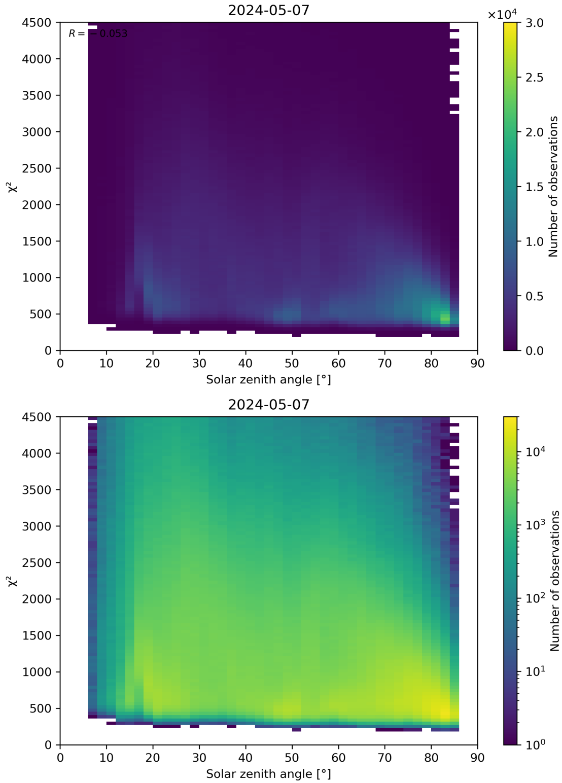
Figure 64: Scatter density plot of “Solar zenith angle” against “ \chi^2 ” for 2024-05-07 to 2024-05-08.
