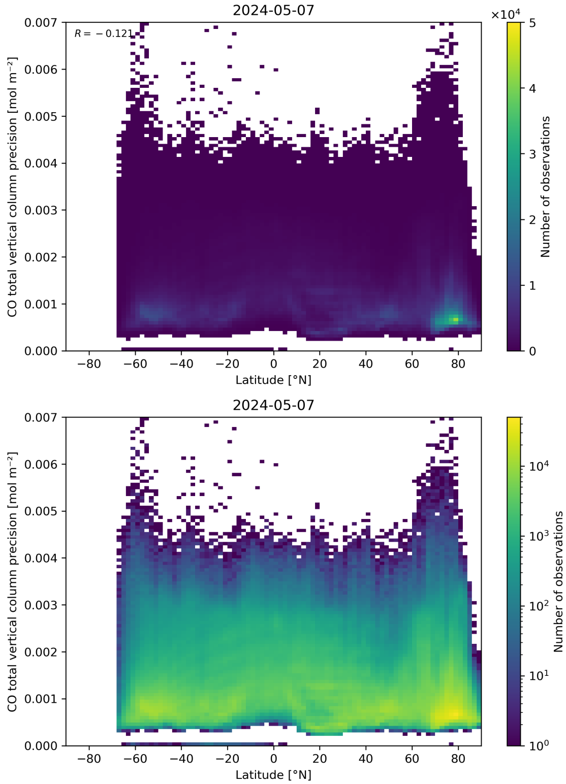
Figure 53: Scatter density plot of “Latitude” against “CO total vertical column precision” for 2024-05-07 to 2024-05-08.
