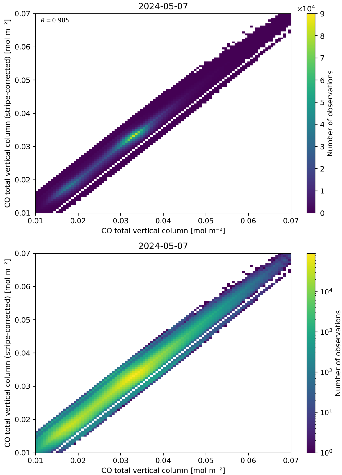
Figure 33: Scatter density plot of “CO total vertical column” against “CO total vertical column (stripe-corrected)” for 2024-05-07 to 2024-05-08.
