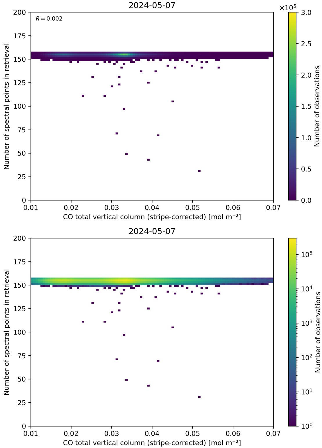
Figure 40: Scatter density plot of “CO total vertical column (stripe-corrected)” against “Number of spectral points in retrieval” for 2024-05-07 to 2024-05-08.
