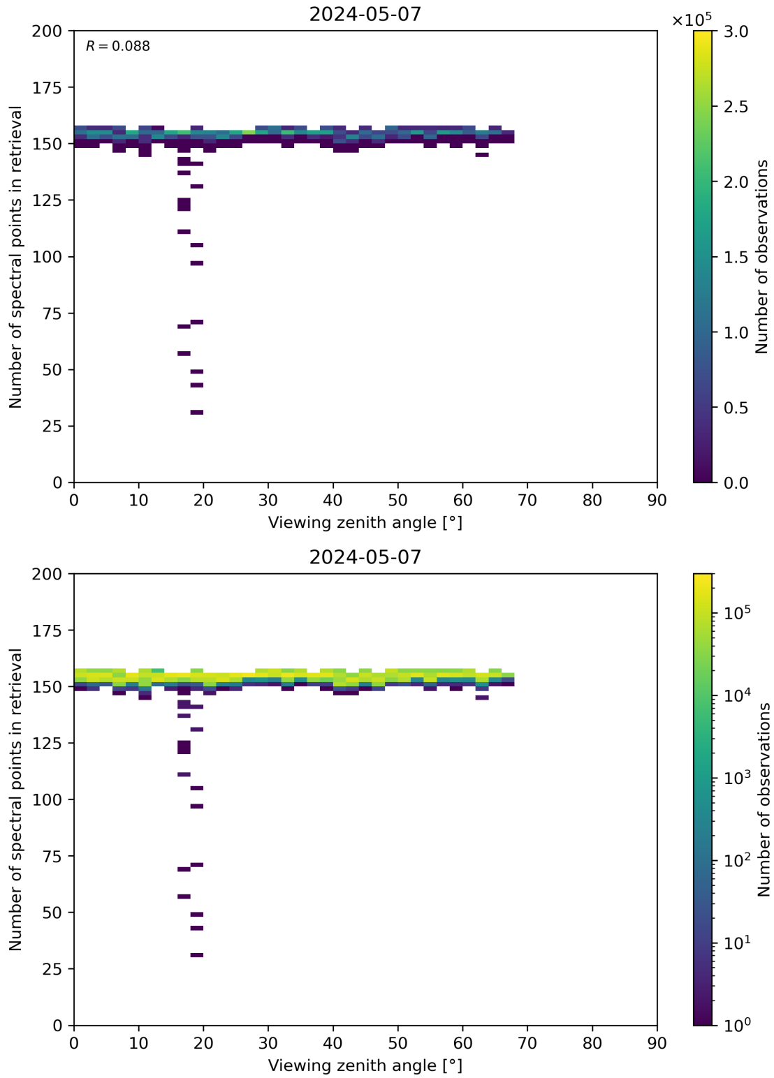
Figure 76: Scatter density plot of “Viewing zenith angle” against “Number of spectral points in retrieval” for 2024-05-07 to 2024-05-08.
