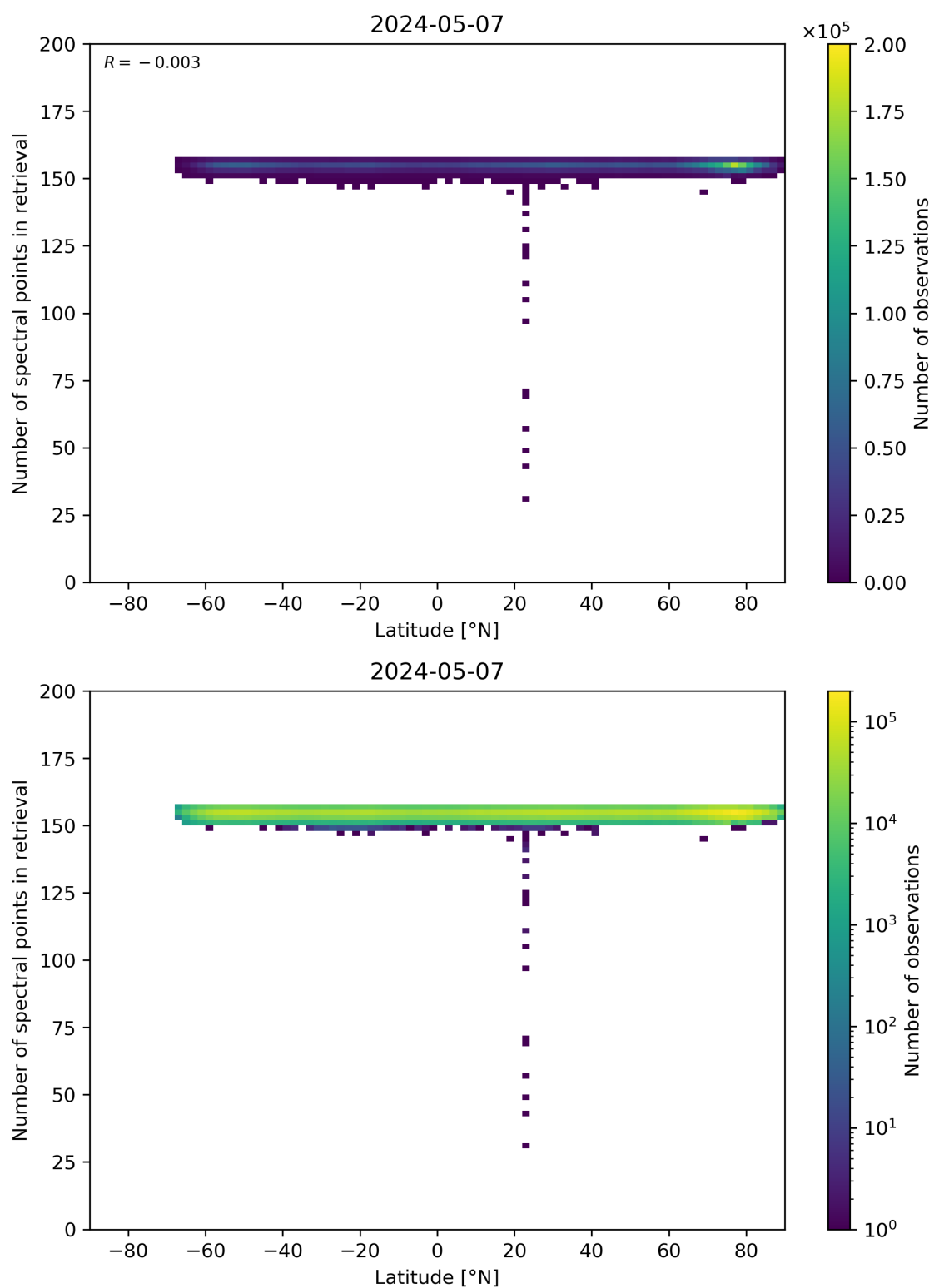
Figure 57: Scatter density plot of “Latitude” against “Number of spectral points in retrieval” for 2024-05-07 to 2024-05-08.
