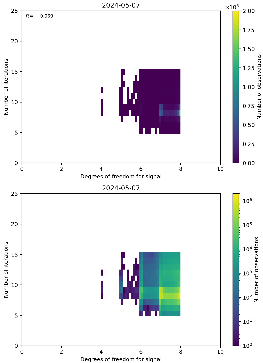
Figure 50: Scatter density plot of “Degrees of freedom for signal” against “Number of iterations” for 2024-05-07 to 2024-05-08.
