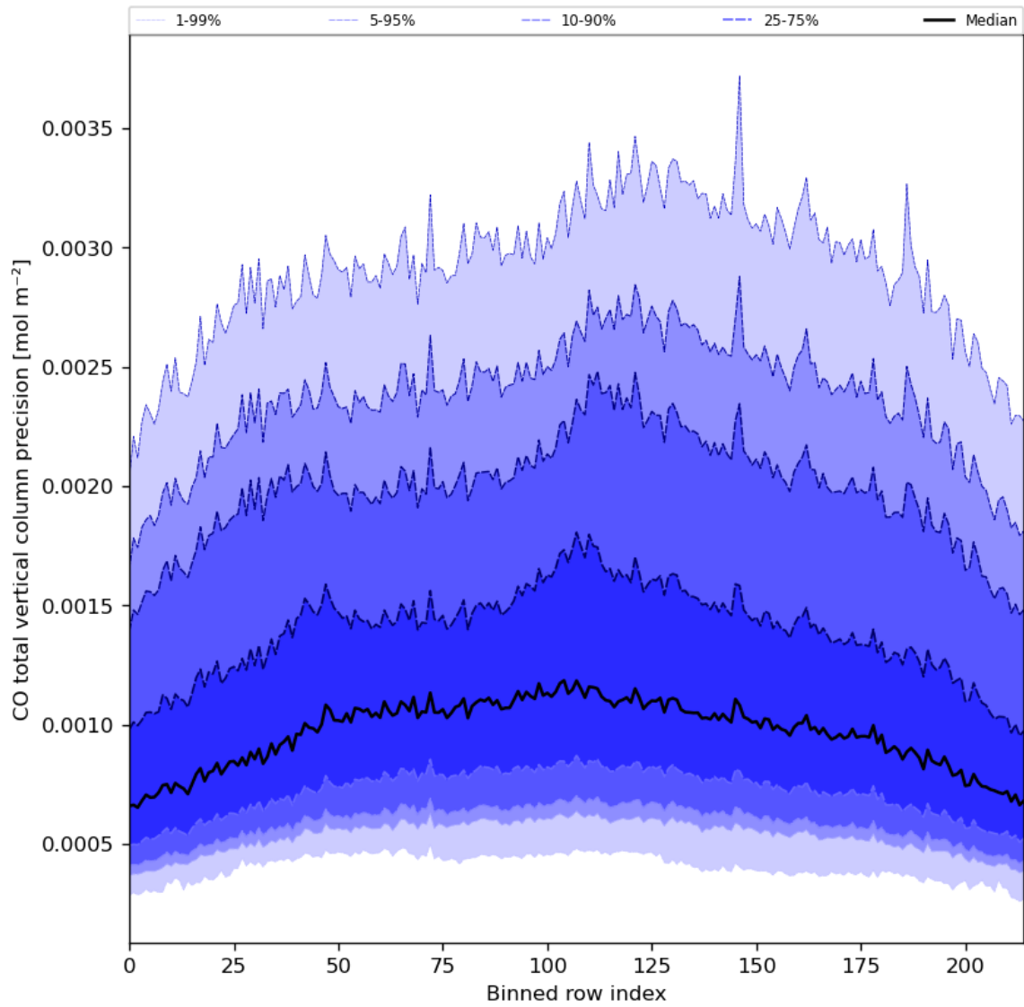
Figure 28: Along track statistics of “CO total vertical column precision” for 2024-05-07 to 2024-05-08
