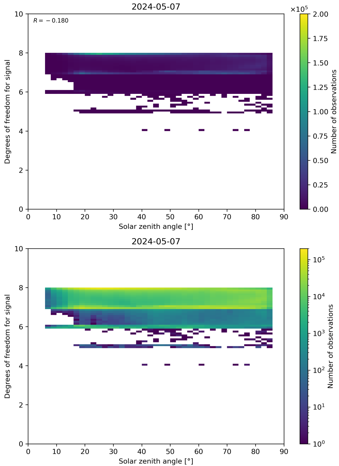
Figure 65: Scatter density plot of “Solar zenith angle” against “Degrees of freedom for signal” for 2024-05-07 to 2024-05-08.
