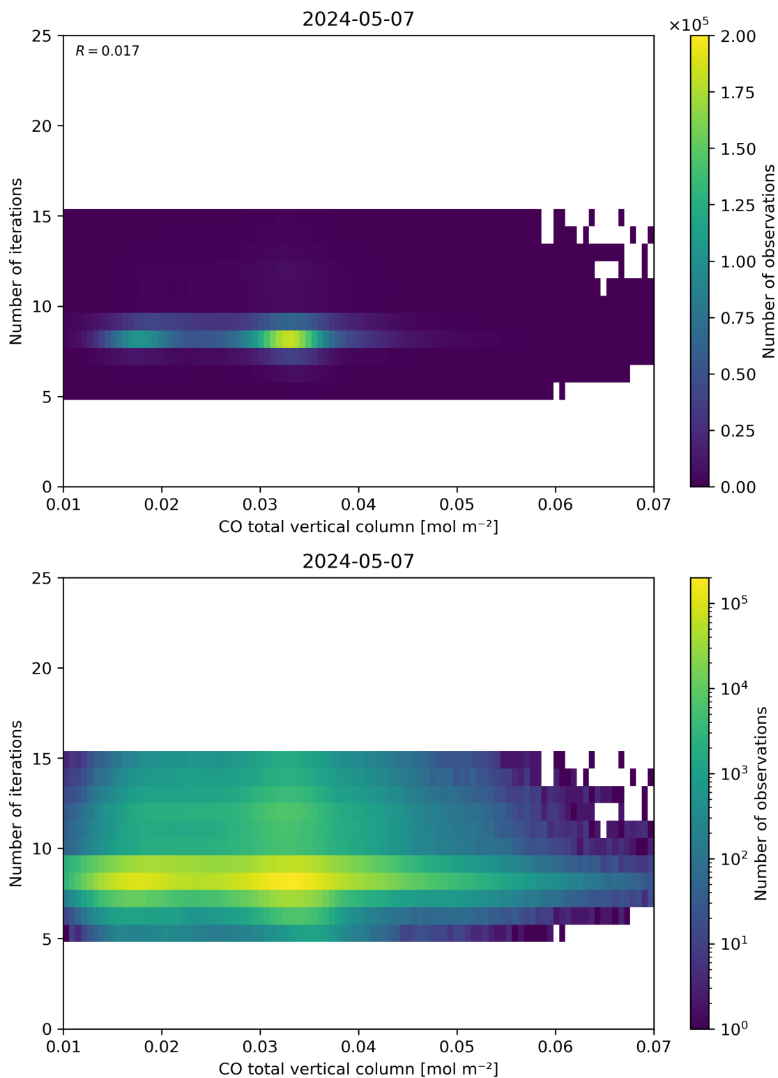
Figure 42: Scatter density plot of “CO total vertical column” against “Number of iterations” for 2024-05-07 to 2024-05-08.
