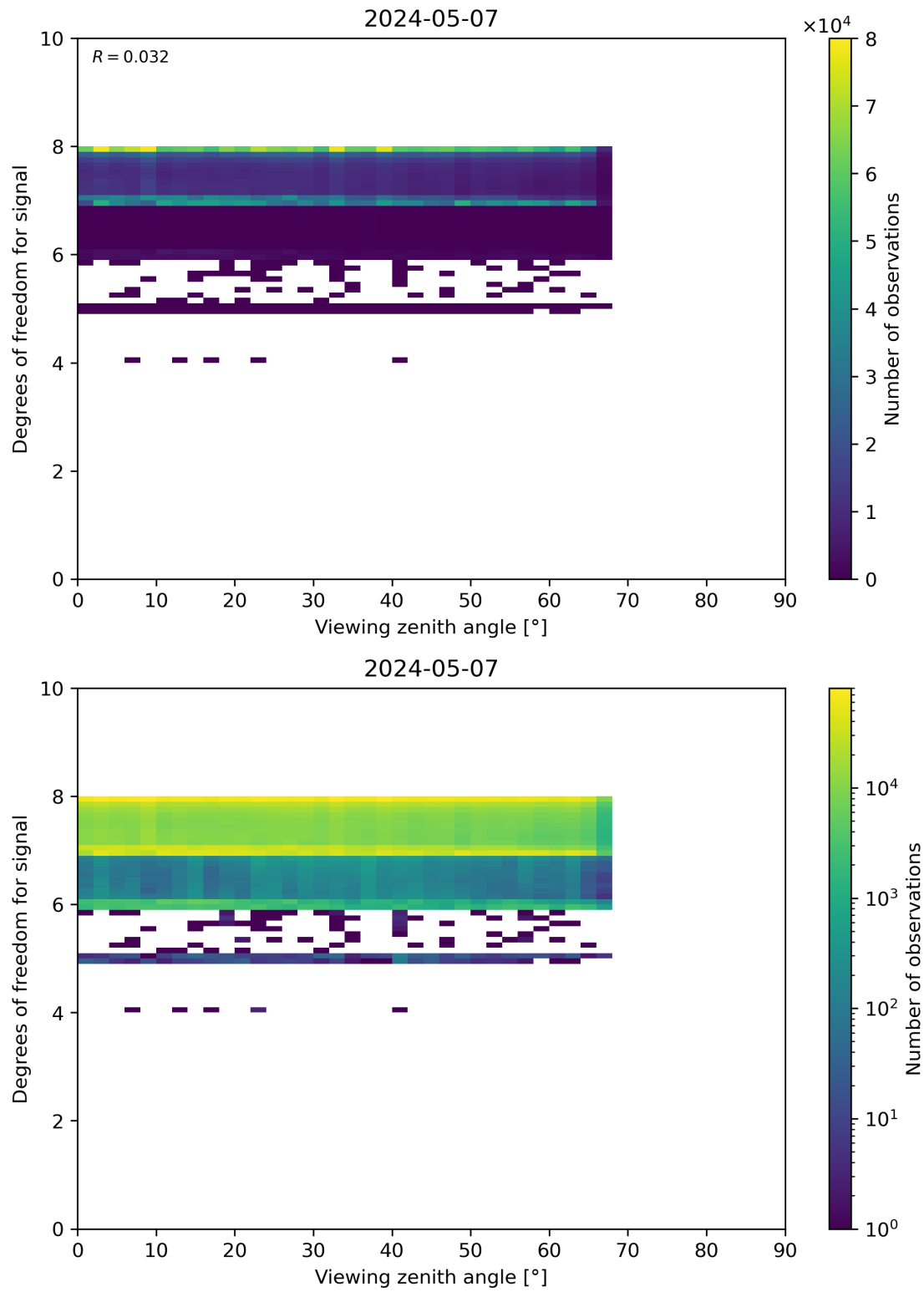
Figure 73: Scatter density plot of “Viewing zenith angle” against “Degrees of freedom for signal” for 2024-05-07 to 2024-05-08.
