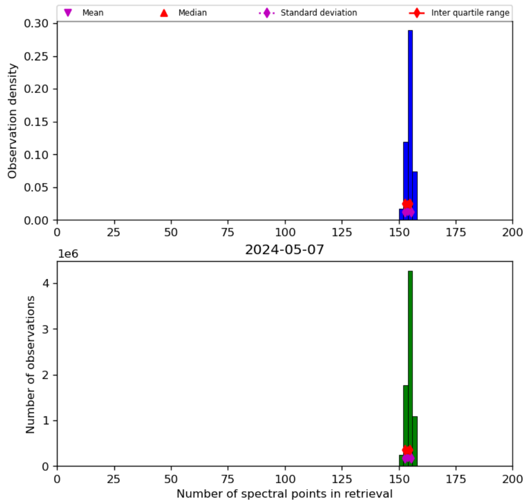
Figure 21: Histogram of “Number of spectral points in retrieval” for 2024-05-07 to 2024-05-08
