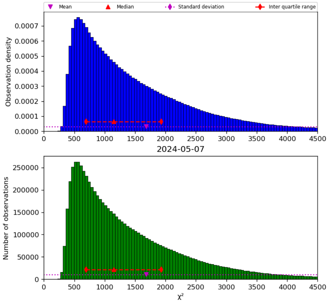
Figure 22: Histogram of “ \chi^2 ” for 2024-05-07 to 2024-05-08
