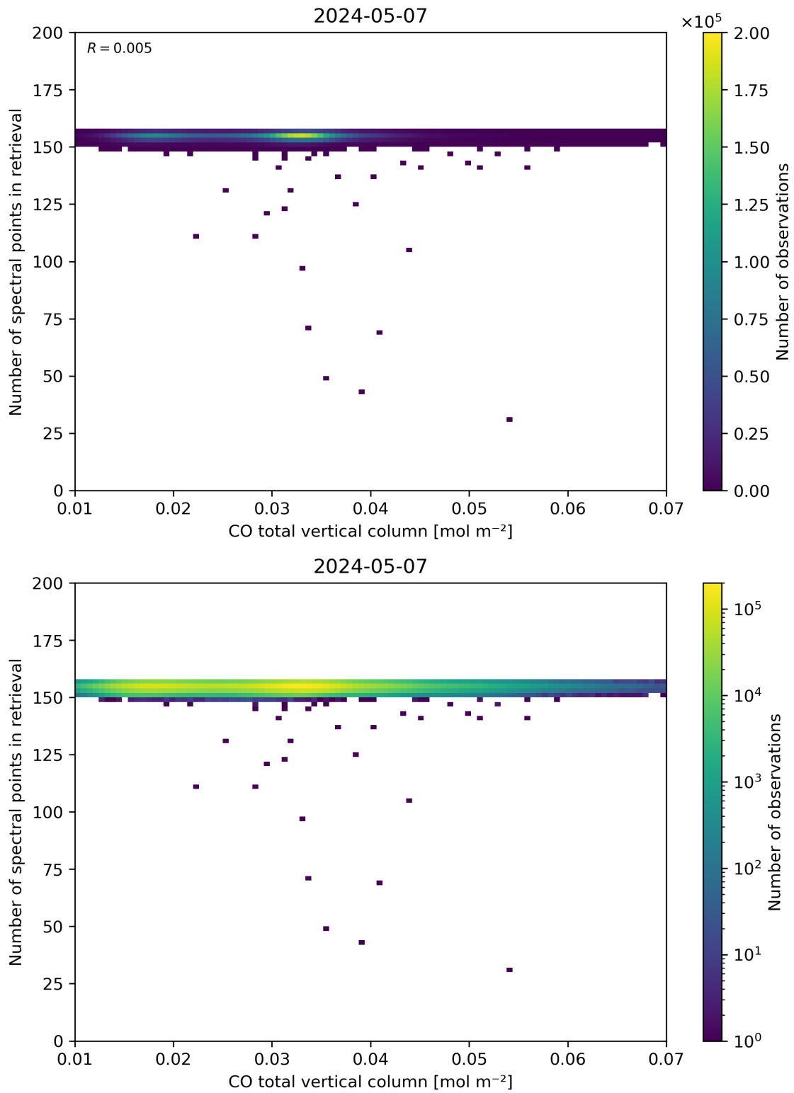
Figure 43: Scatter density plot of “CO total vertical column” against “Number of spectral points in retrieval” for 2024-05-07 to 2024-05-08.
