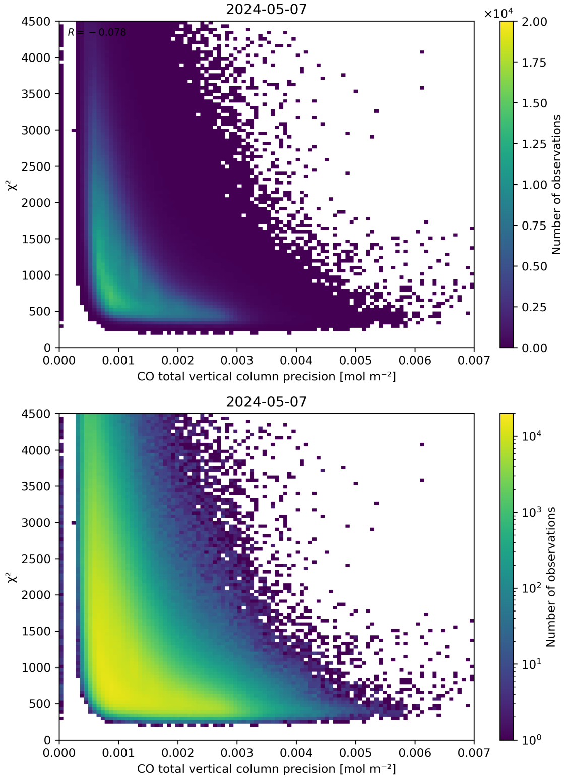
Figure 44: Scatter density plot of “CO total vertical column precision” against “ \chi^2 ” for 2024-05-07 to 2024-05-08.
