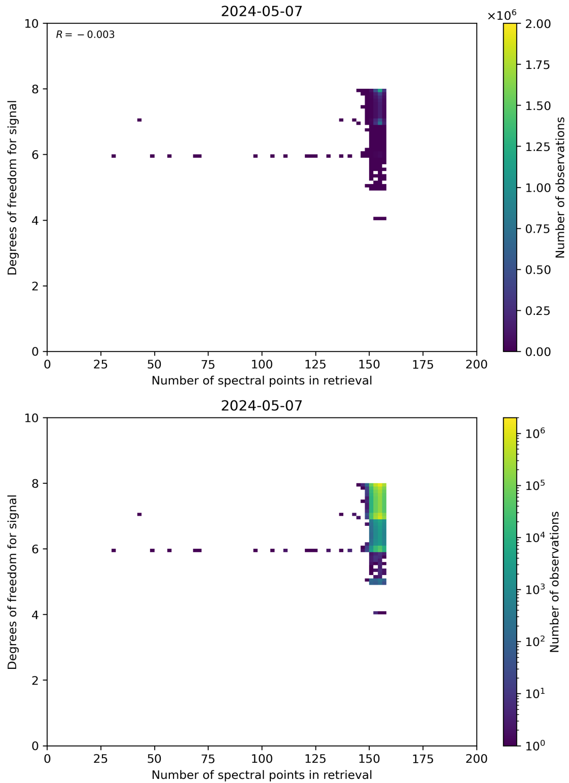
Figure 59: Scatter density plot of “Number of spectral points in retrieval” against “Degrees of freedom for signal” for 2024-05-07 to 2024-05-08.
