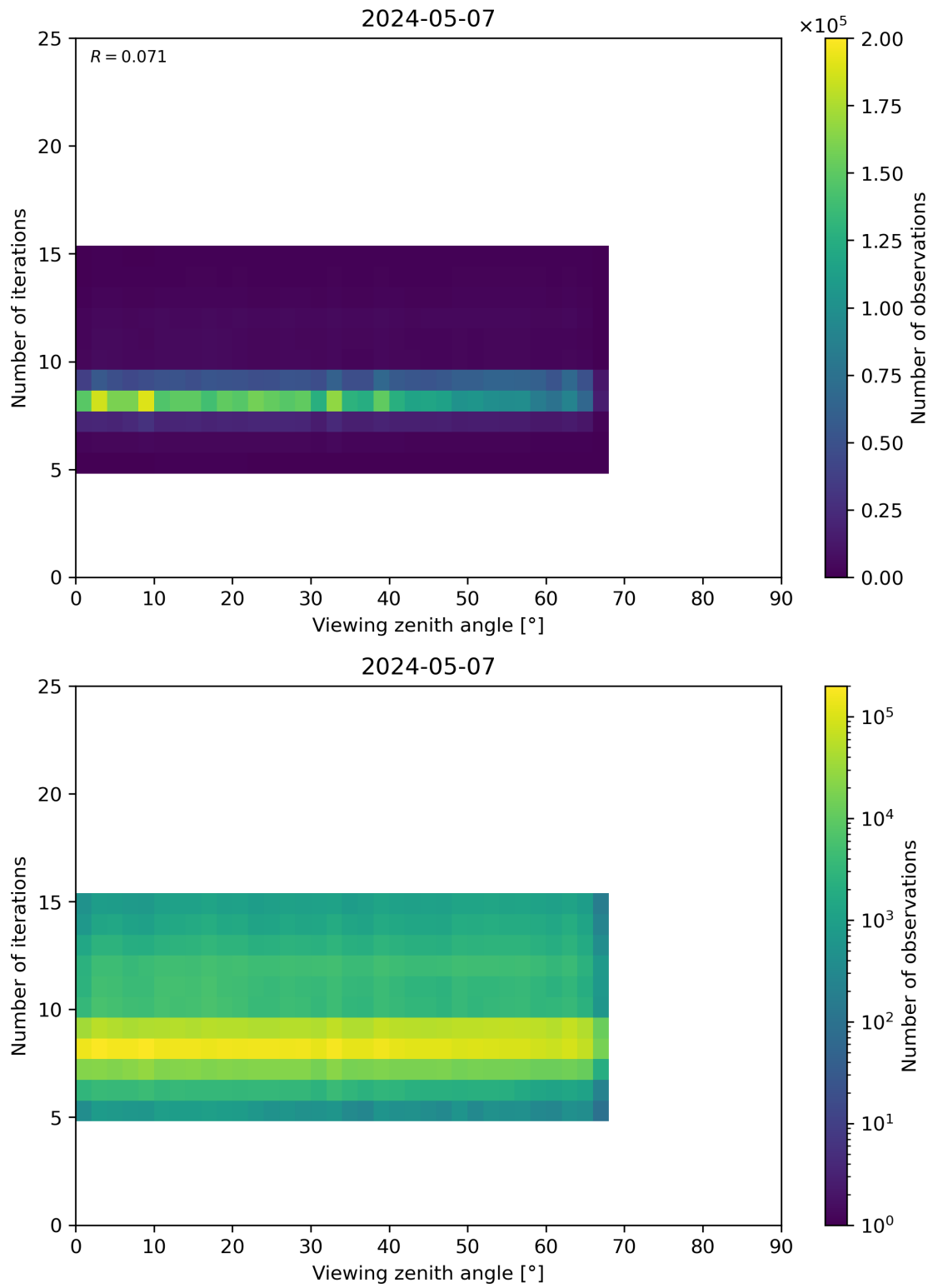
Figure 75: Scatter density plot of “Viewing zenith angle” against “Number of iterations” for 2024-05-07 to 2024-05-08.
