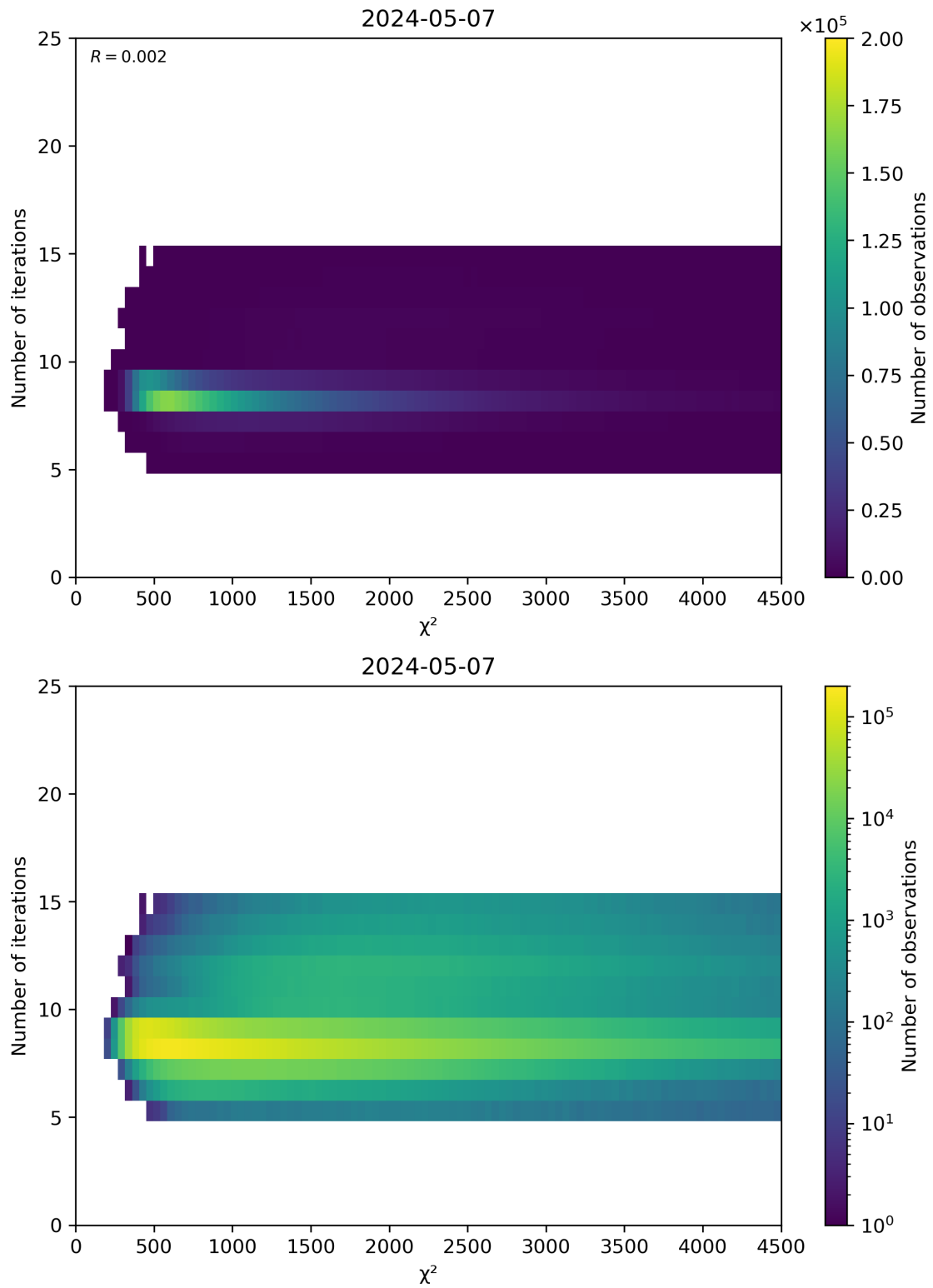
Figure 49: Scatter density plot of “ \chi^2 ” against “Number of iterations” for 2024-05-07 to 2024-05-08.
