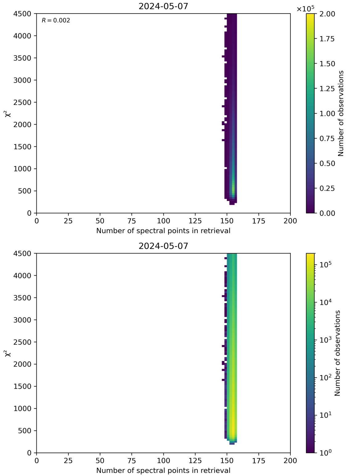
Figure 58: Scatter density plot of “Number of spectral points in retrieval” against “ \chi^2 ” for 2024-05-07 to 2024-05-08.
