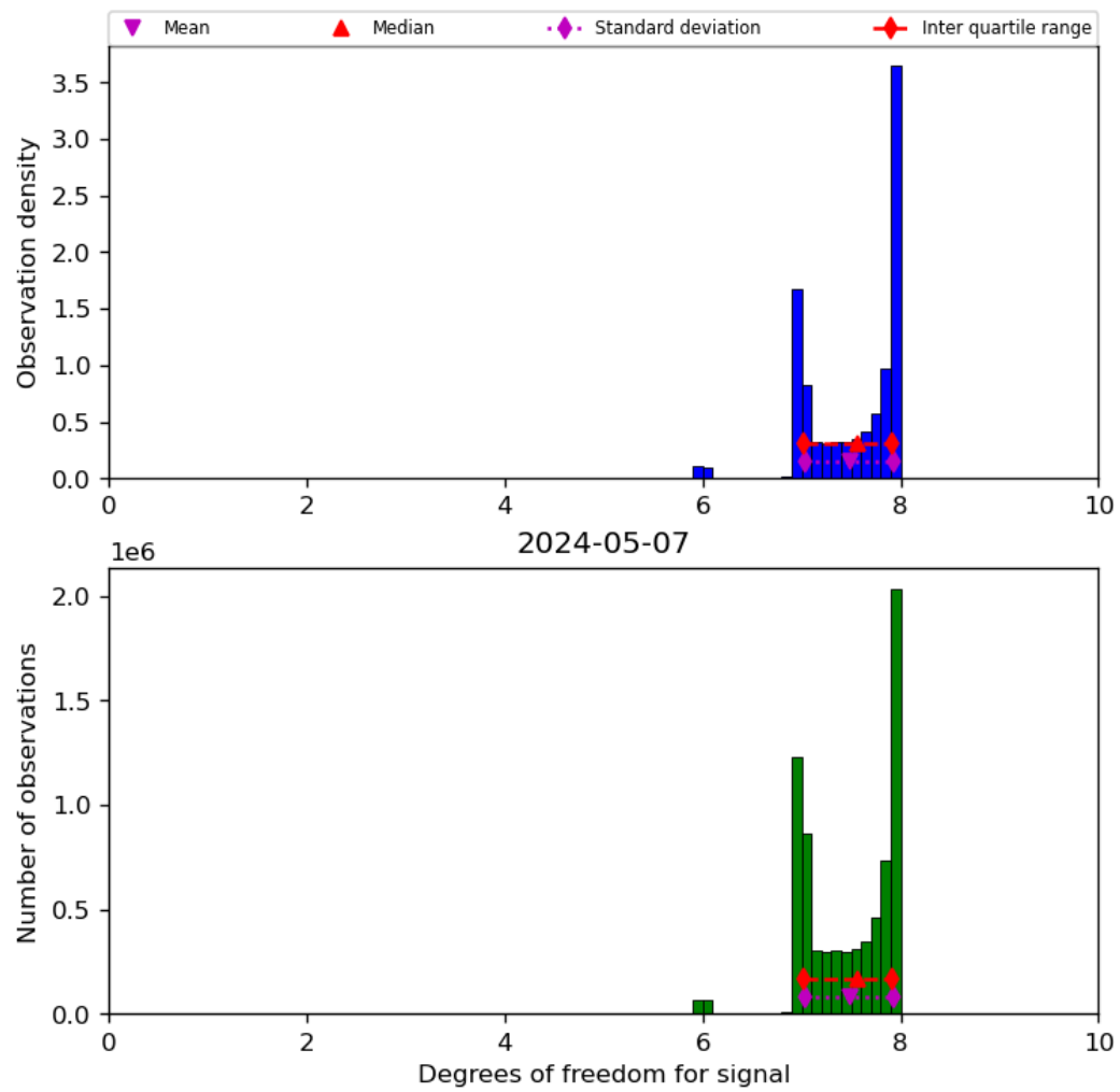
Figure 23: Histogram of “Degrees of freedom for signal” for 2024-05-07 to 2024-05-08
