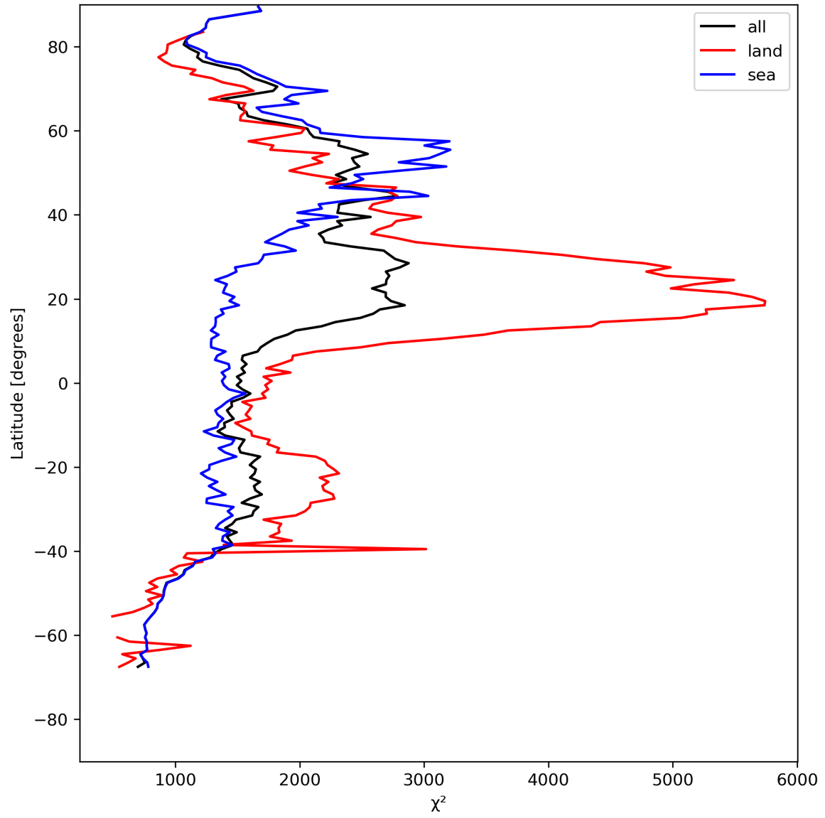
Figure 14: Zonal average of “ \chi^2 ” for 2024-05-07 to 2024-05-08.
