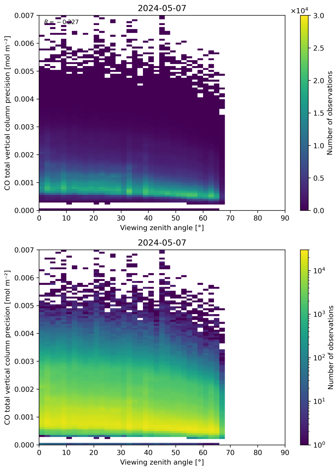
Figure 71: Scatter density plot of “Viewing zenith angle” against “CO total vertical column precision” for 2024-05-07 to 2024-05-08.
