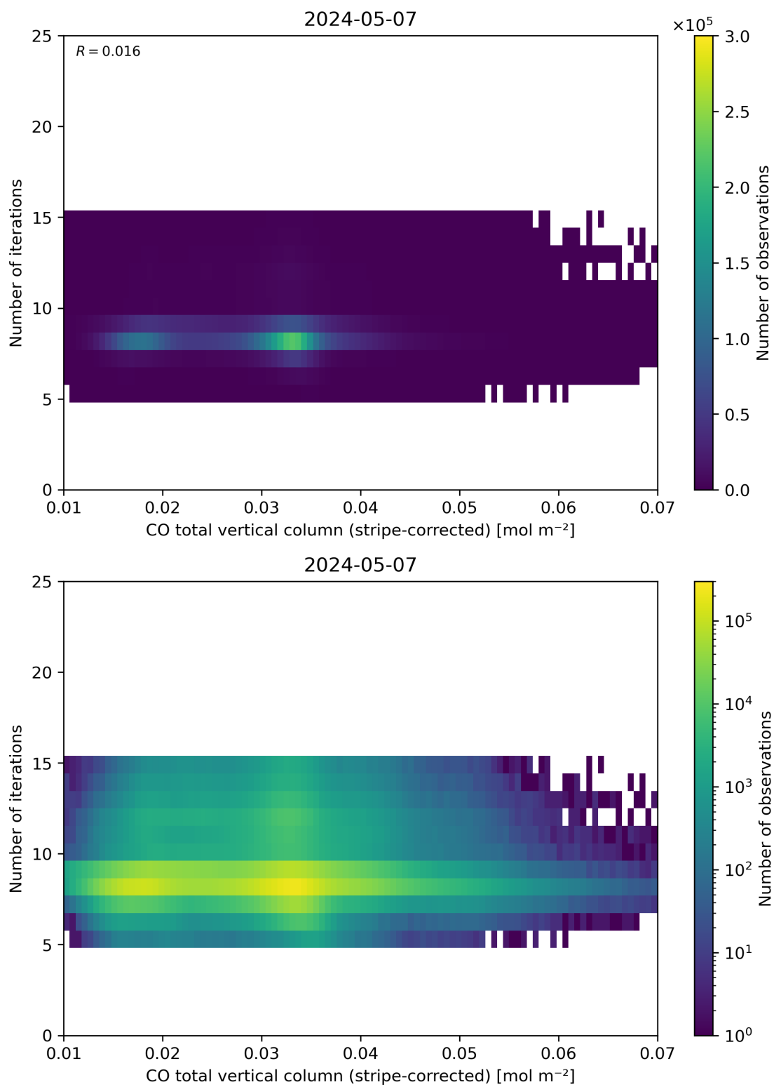
Figure 39: Scatter density plot of “CO total vertical column (stripe-corrected)” against “Number of iterations” for 2024-05-07 to 2024-05-08.
