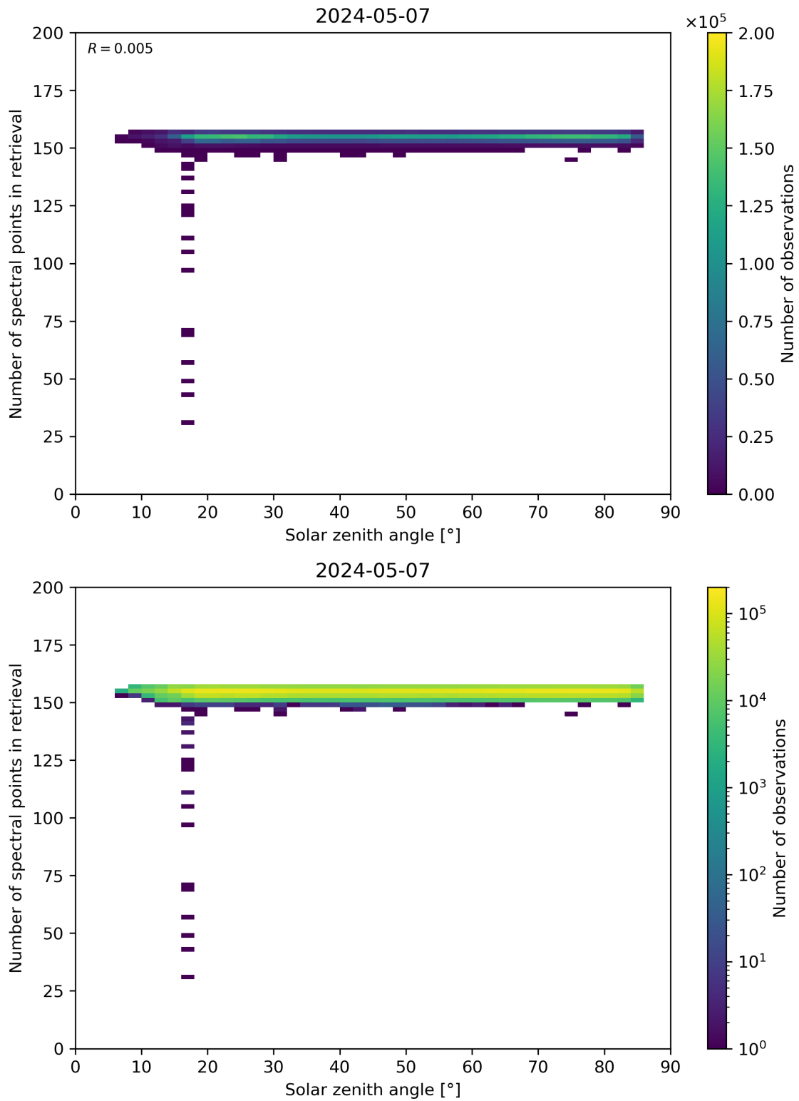
Figure 68: Scatter density plot of “Solar zenith angle” against “Number of spectral points in retrieval” for 2024-05-07 to 2024-05-08.
