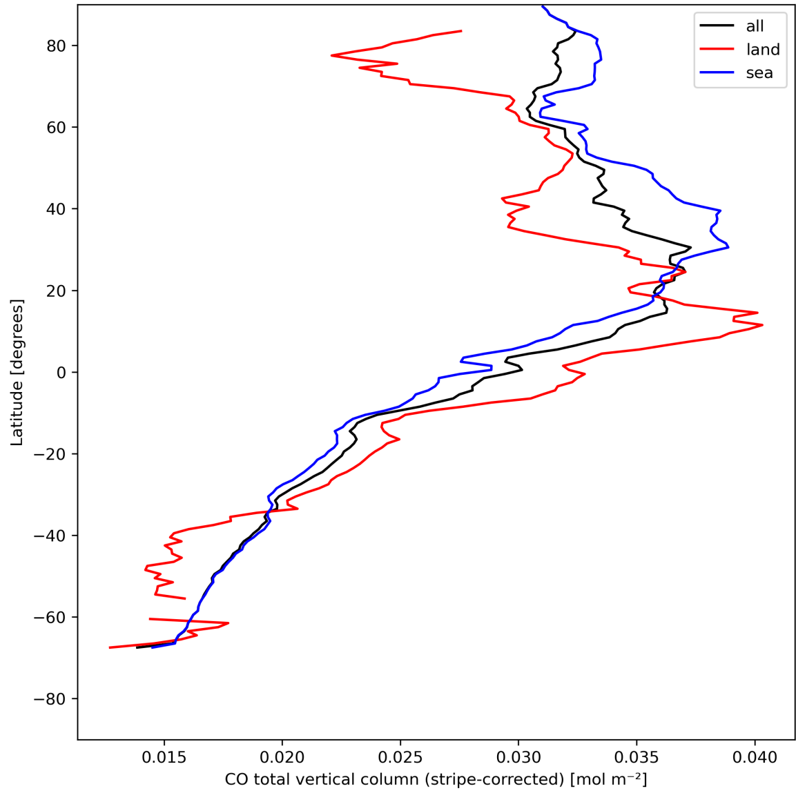
Figure 11: Zonal average of “CO total vertical column (stripe-corrected)” for 2024-05-07 to 2024-05-08.
