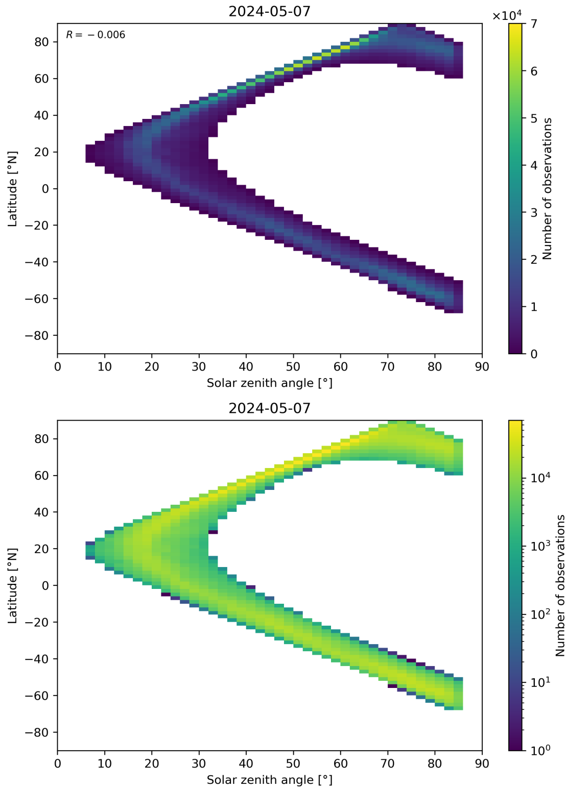
Figure 66: Scatter density plot of “Solar zenith angle” against “Latitude” for 2024-05-07 to 2024-05-08.
