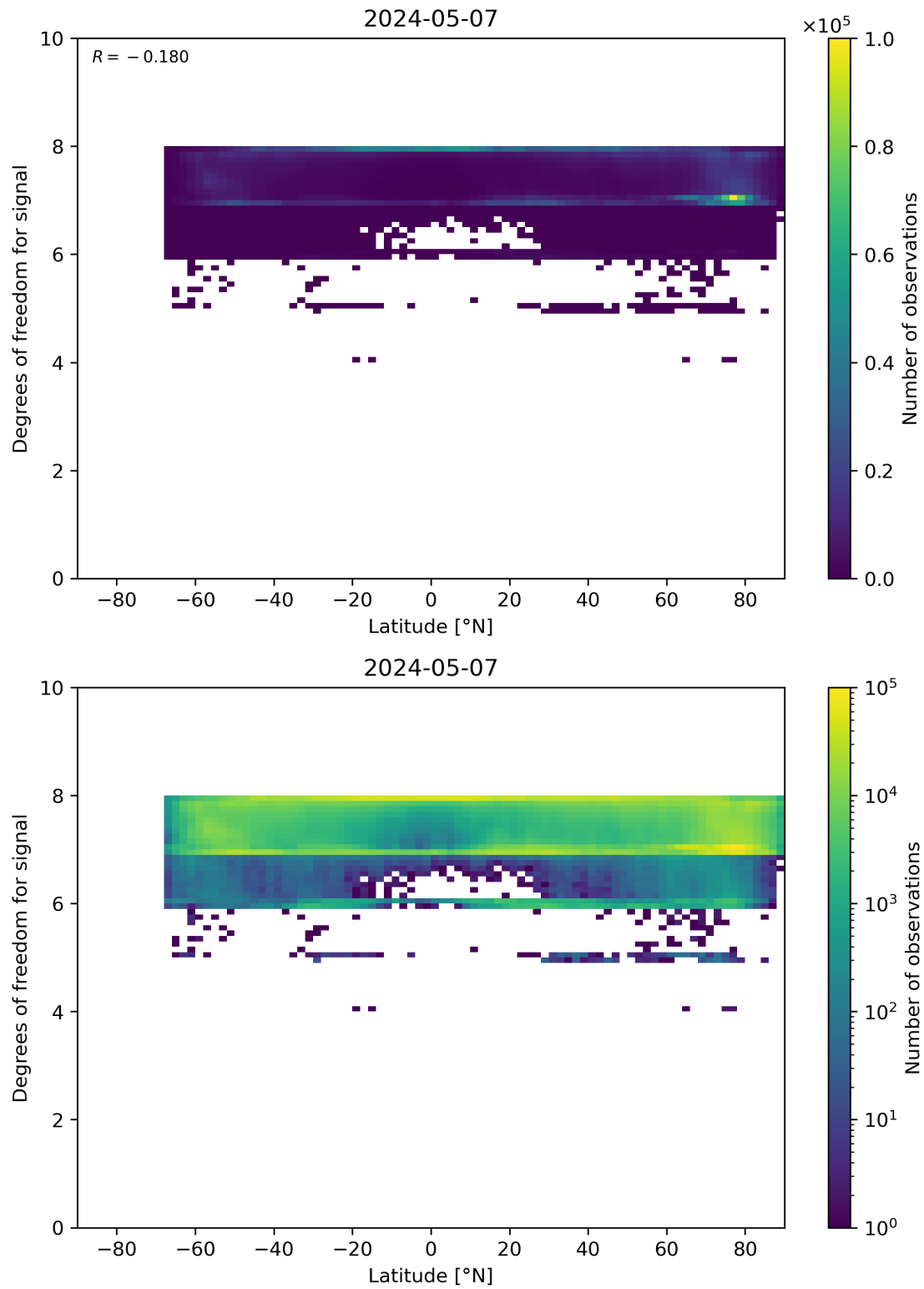
Figure 55: Scatter density plot of “Latitude” against “Degrees of freedom for signal” for 2024-05-07 to 2024-05-08.
