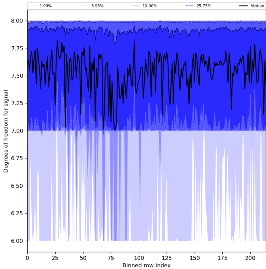
Figure 31: Along track statistics of “Degrees of freedom for signal” for 2024-05-07 to 2024-05-08
