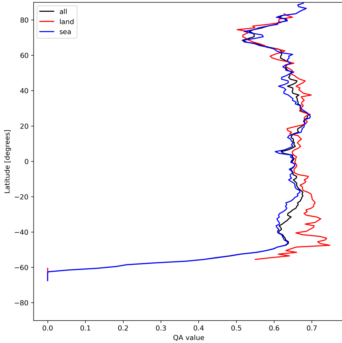
Figure 9: Zonal average of “QA value” for 2024-05-07 to 2024-05-08.
