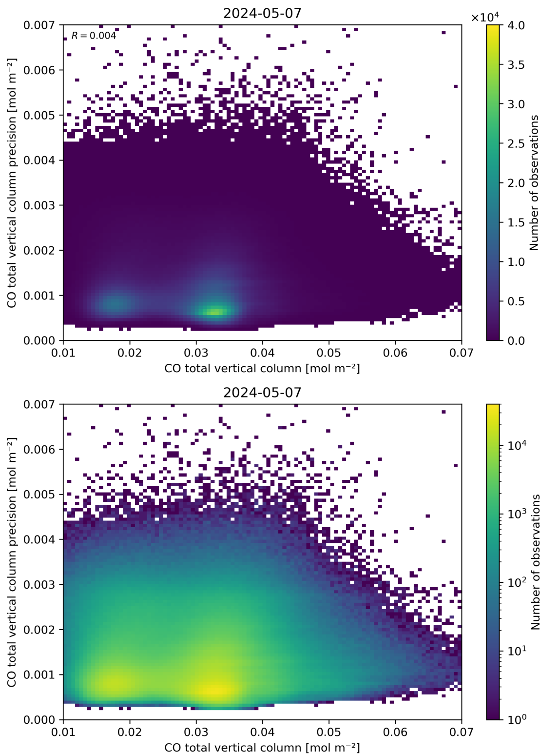
Figure 34: Scatter density plot of “CO total vertical column” against “CO total vertical column precision” for 2024-05-07 to 2024-05-08.
