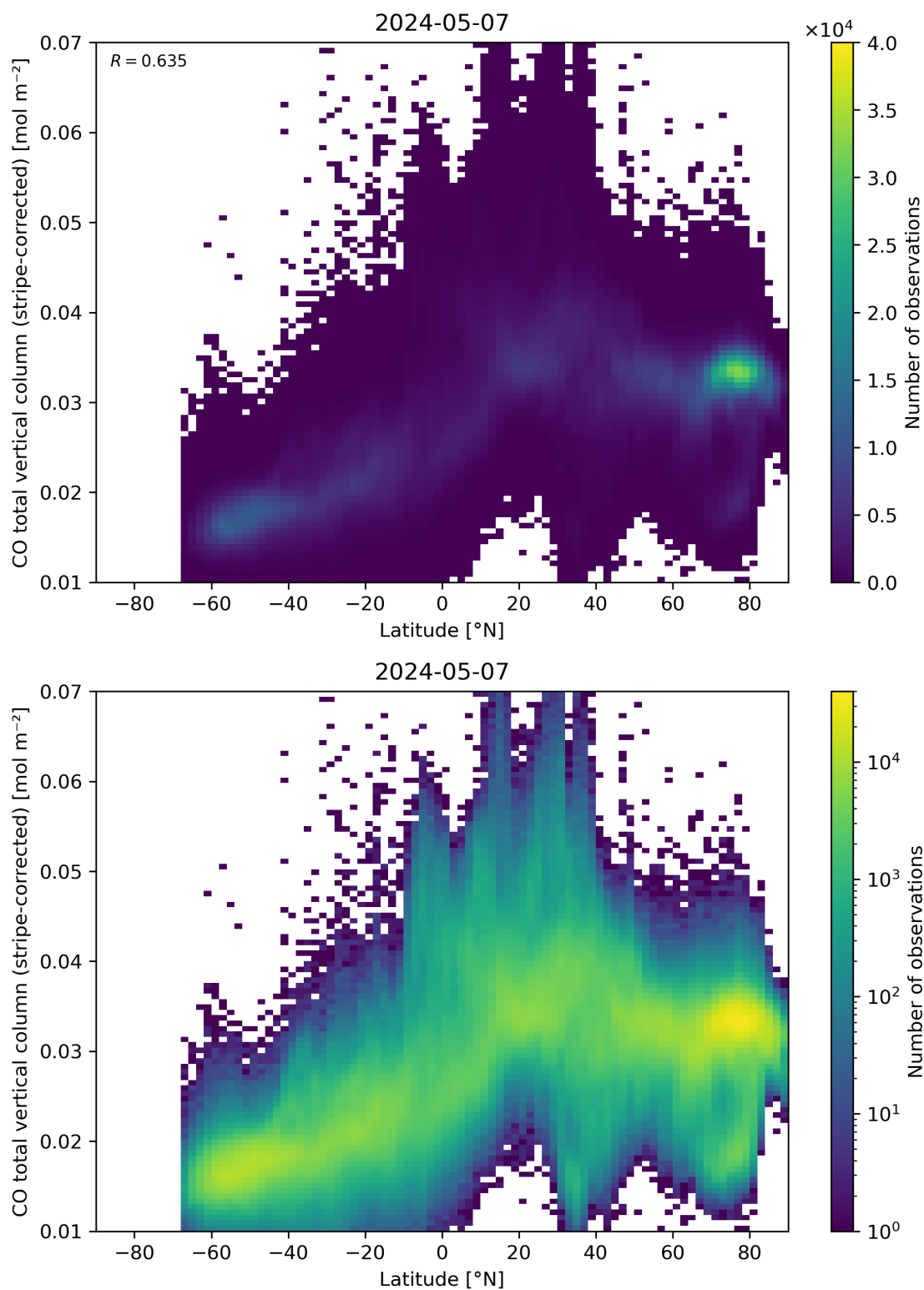
Figure 52: Scatter density plot of “Latitude” against “CO total vertical column (stripe-corrected)” for 2024-05-07 to 2024-05-08.
