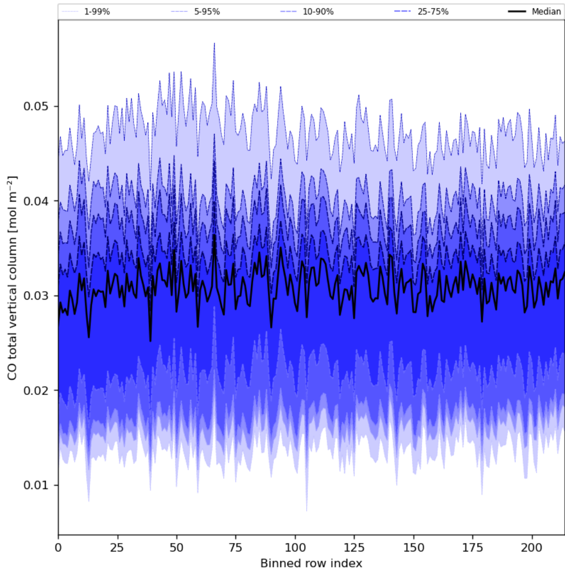
Figure 26: Along track statistics of “CO total vertical column” for 2024-05-07 to 2024-05-08
