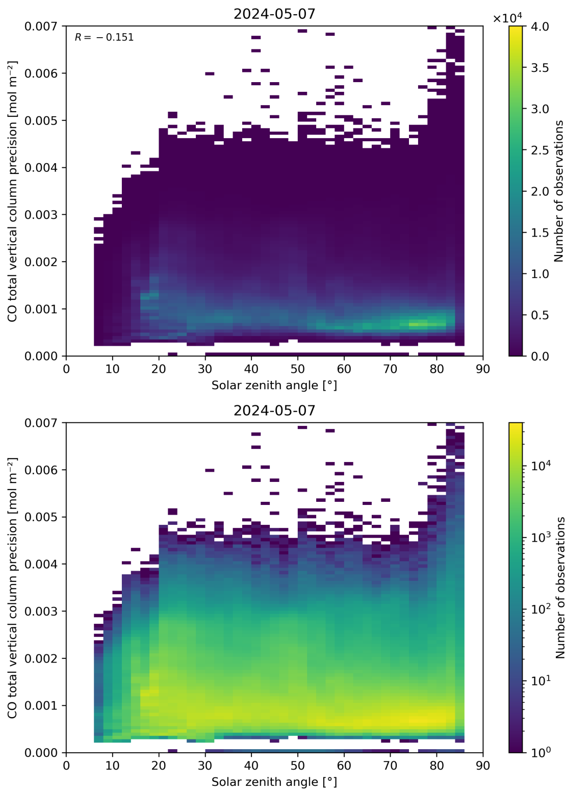
Figure 63: Scatter density plot of “Solar zenith angle” against “CO total vertical column precision” for 2024-05-07 to 2024-05-08.
