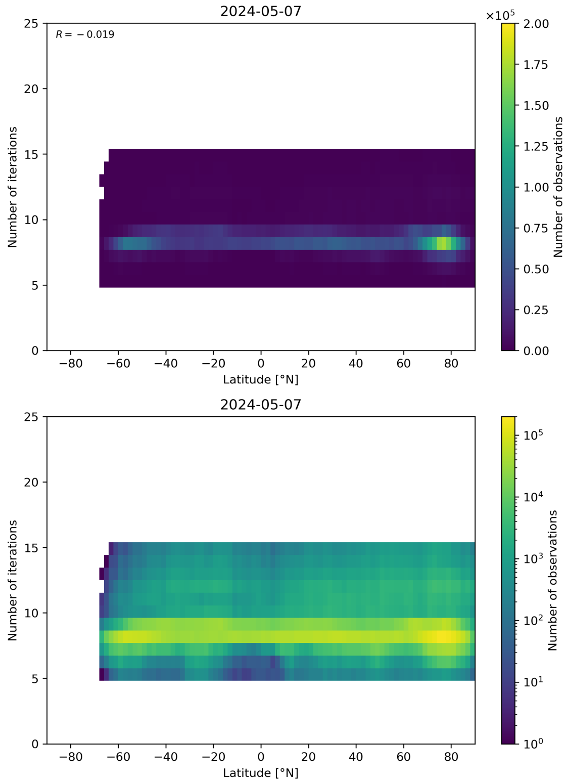
Figure 56: Scatter density plot of “Latitude” against “Number of iterations” for 2024-05-07 to 2024-05-08.
