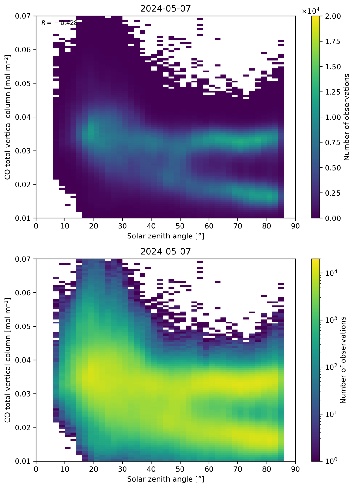
Figure 61: Scatter density plot of “Solar zenith angle” against “CO total vertical column” for 2024-05-07 to 2024-05-08.
