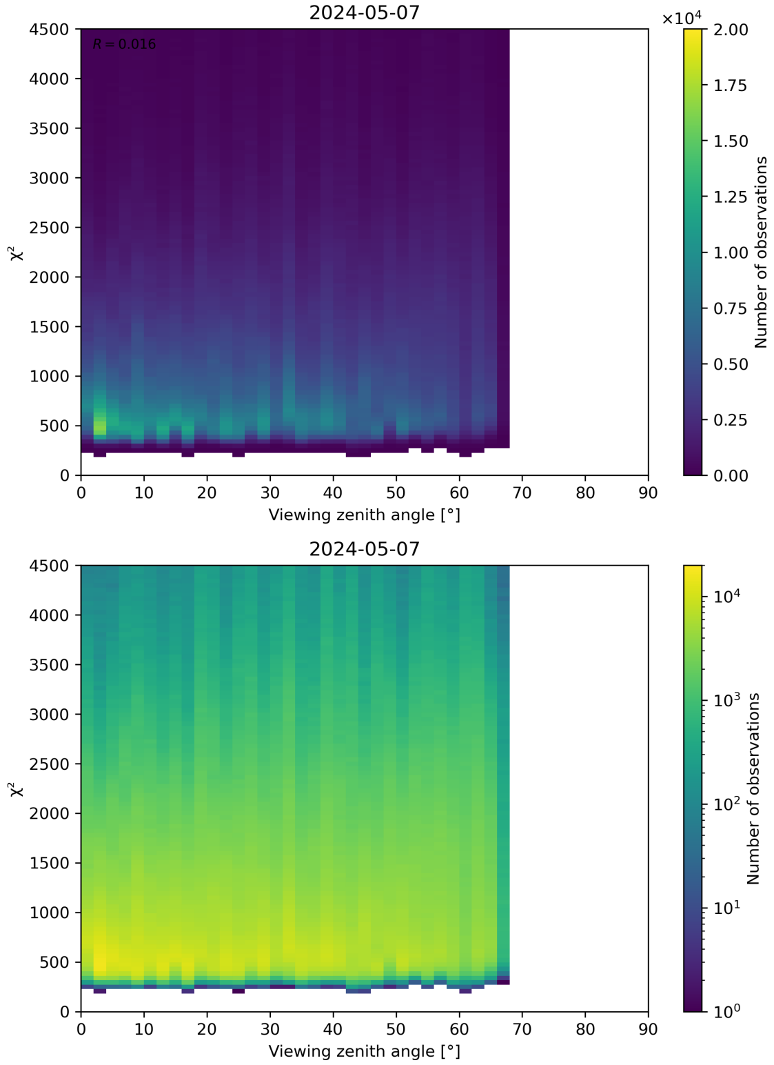
Figure 72: Scatter density plot of “Viewing zenith angle” against “ \chi^2 ” for 2024-05-07 to 2024-05-08.
