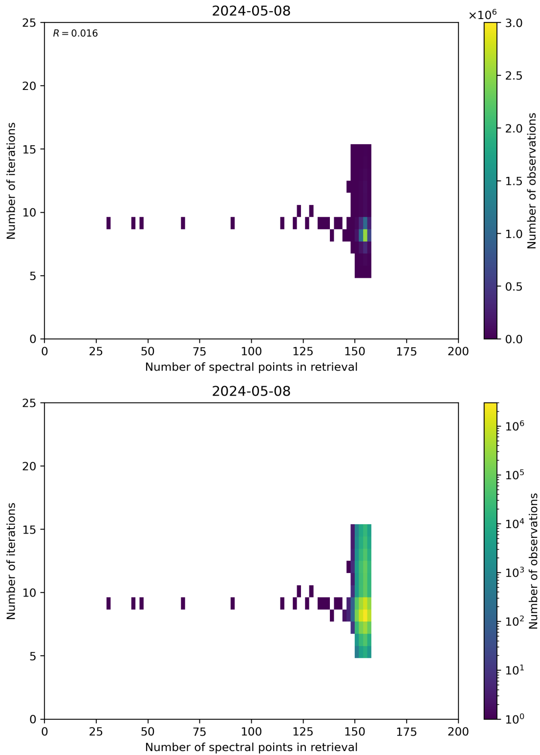
Figure 60: Scatter density plot of “Number of spectral points in retrieval” against “Number of iterations” for 2024-05-07 to 2024-05-09.
