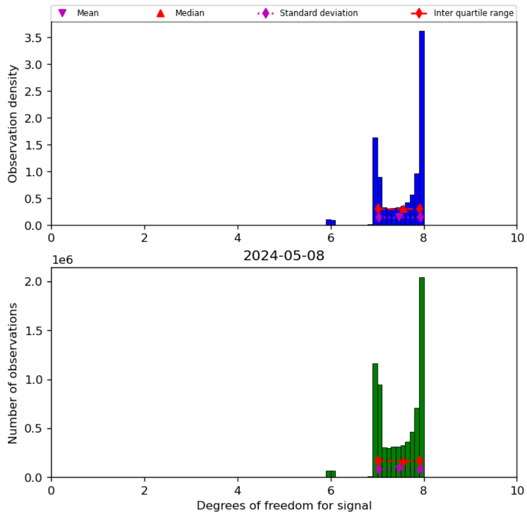
Figure 23: Histogram of “Degrees of freedom for signal” for 2024-05-07 to 2024-05-09
