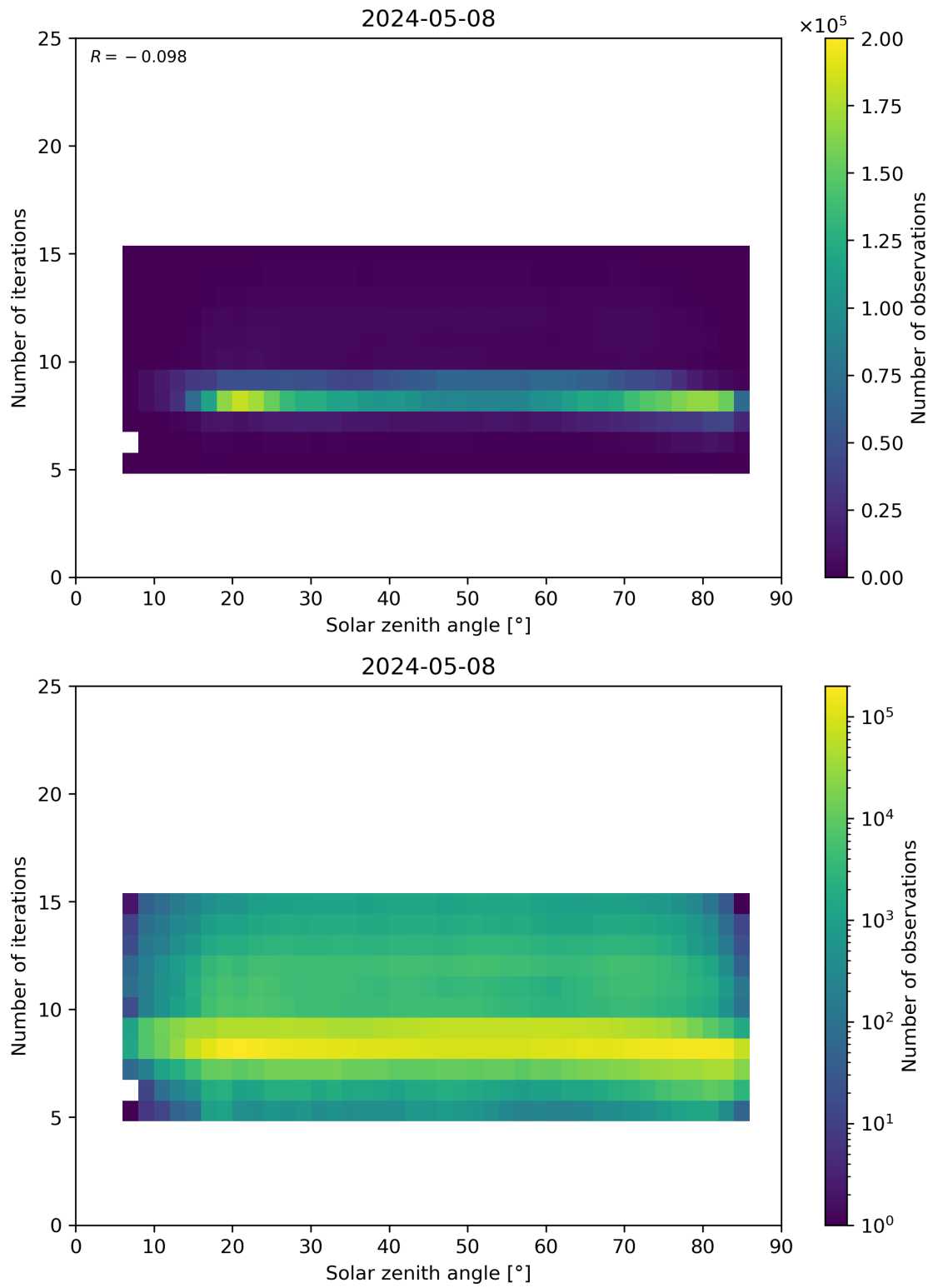
Figure 67: Scatter density plot of “Solar zenith angle” against “Number of iterations” for 2024-05-07 to 2024-05-09.
