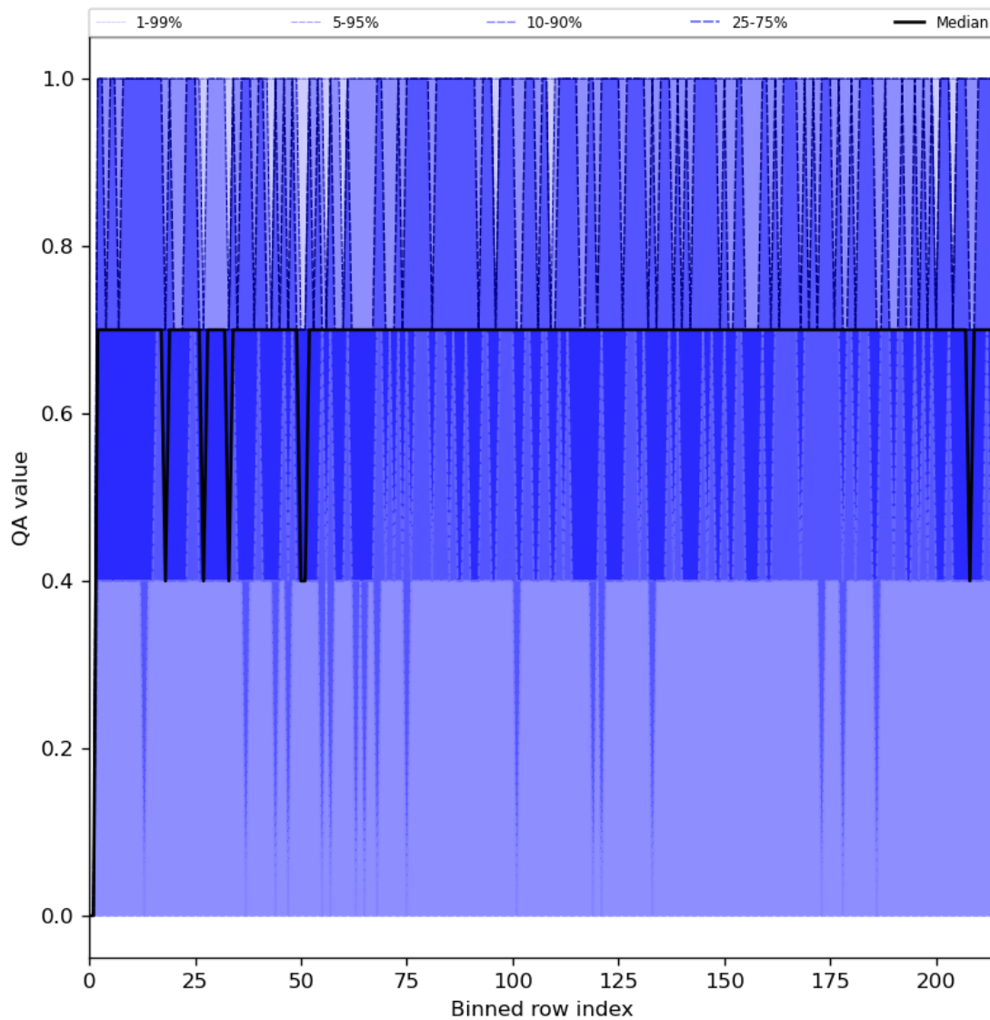
Figure 25: Along track statistics of “QA value” for 2024-05-07 to 2024-05-09
