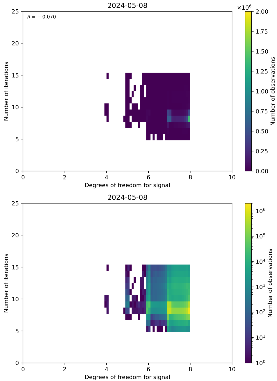
Figure 50: Scatter density plot of “Degrees of freedom for signal” against “Number of iterations” for 2024-05-07 to 2024-05-09.
