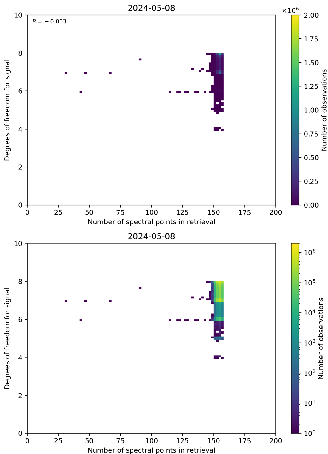
Figure 59: Scatter density plot of “Number of spectral points in retrieval” against “Degrees of freedom for signal” for 2024-05-07 to 2024-05-09.
