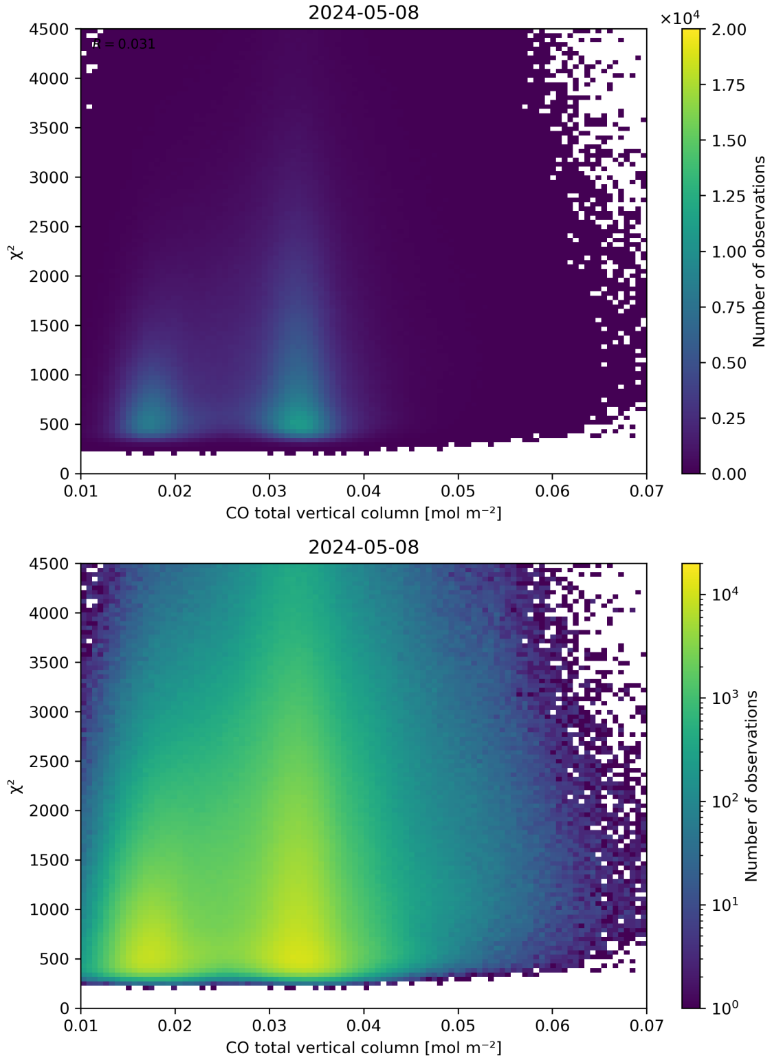
Figure 35: Scatter density plot of “CO total vertical column” against “ \chi^2 ” for 2024-05-07 to 2024-05-09.
