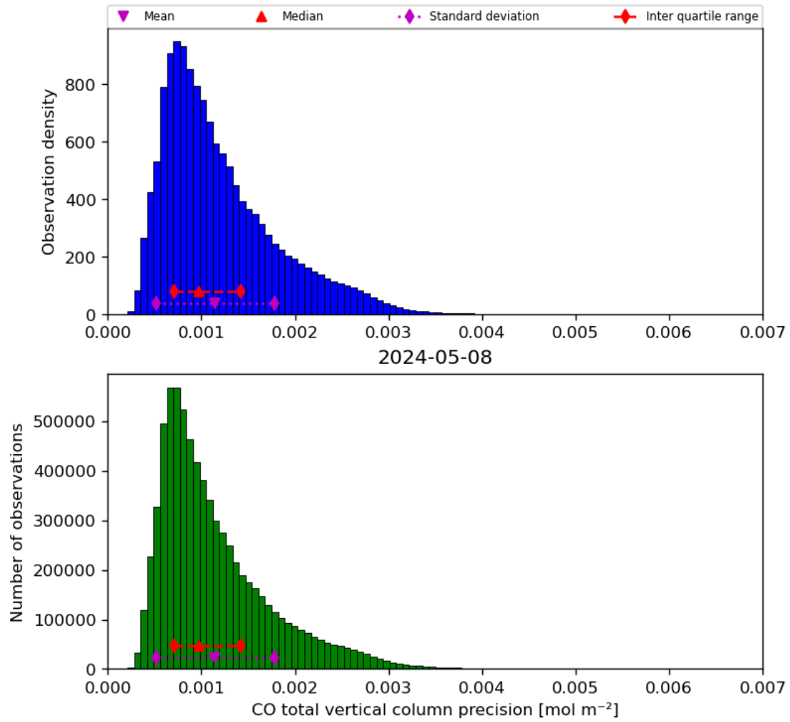
Figure 20: Histogram of “CO total vertical column precision” for 2024-05-07 to 2024-05-09
