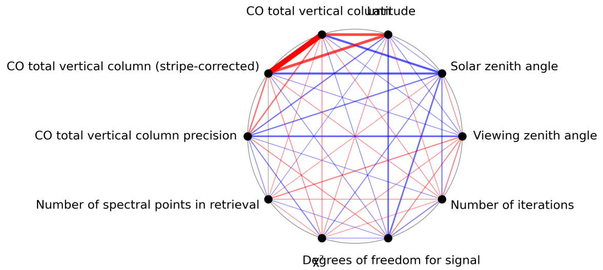
Figure 1: Map of correlation graph for 2024-05-07 to 2024-05-09.
