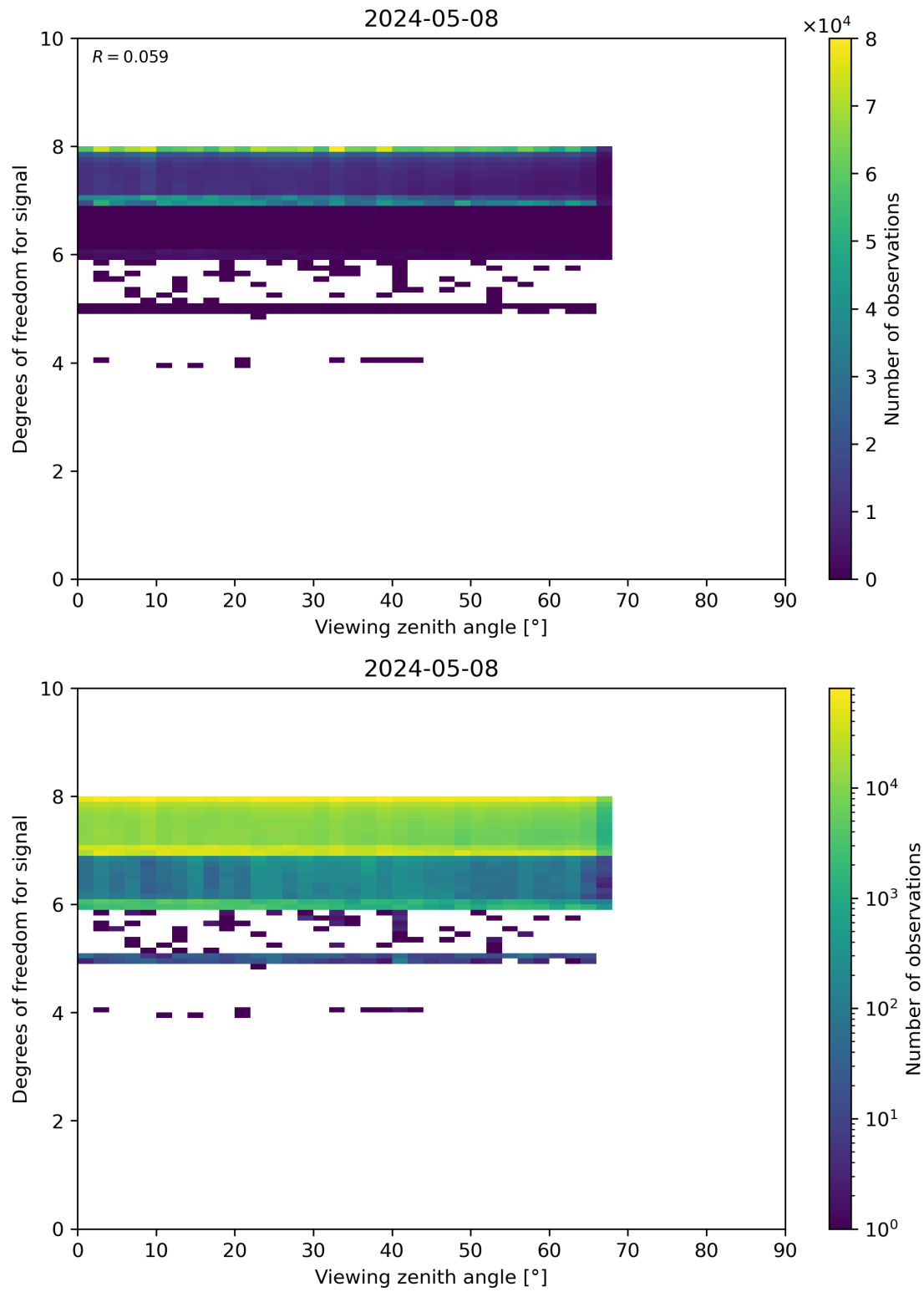
Figure 73: Scatter density plot of “Viewing zenith angle” against “Degrees of freedom for signal” for 2024-05-07 to 2024-05-09.
