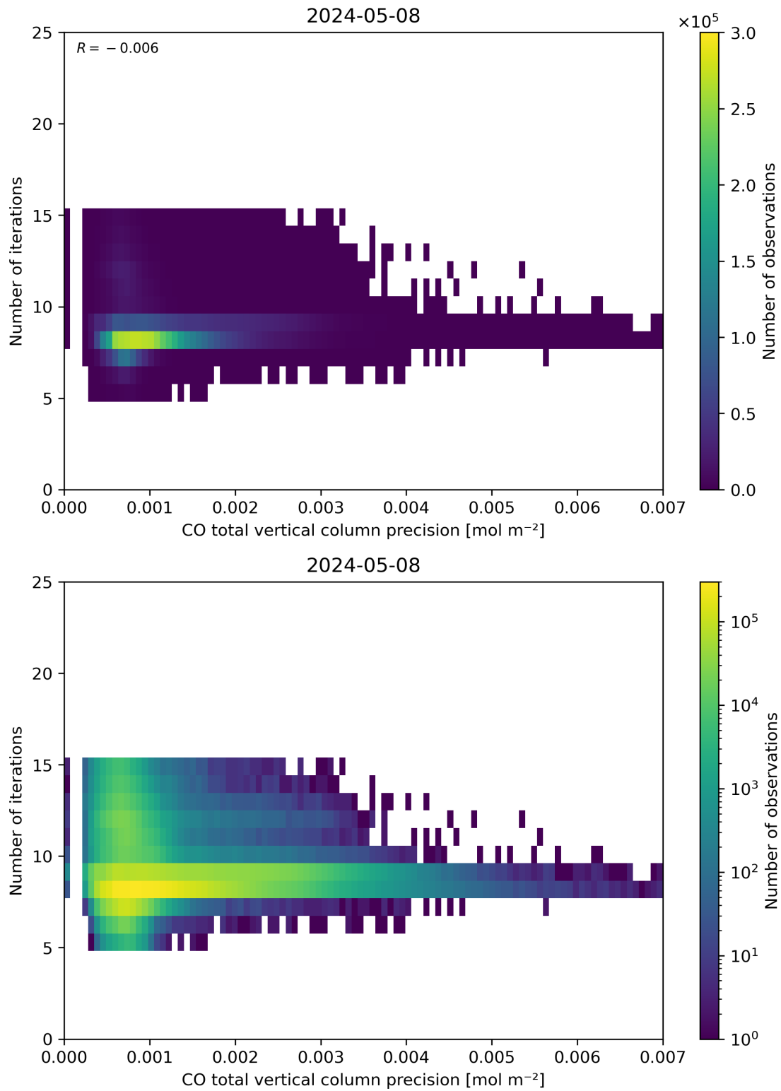
Figure 46: Scatter density plot of “CO total vertical column precision” against “Number of iterations” for 2024-05-07 to 2024-05-09.
