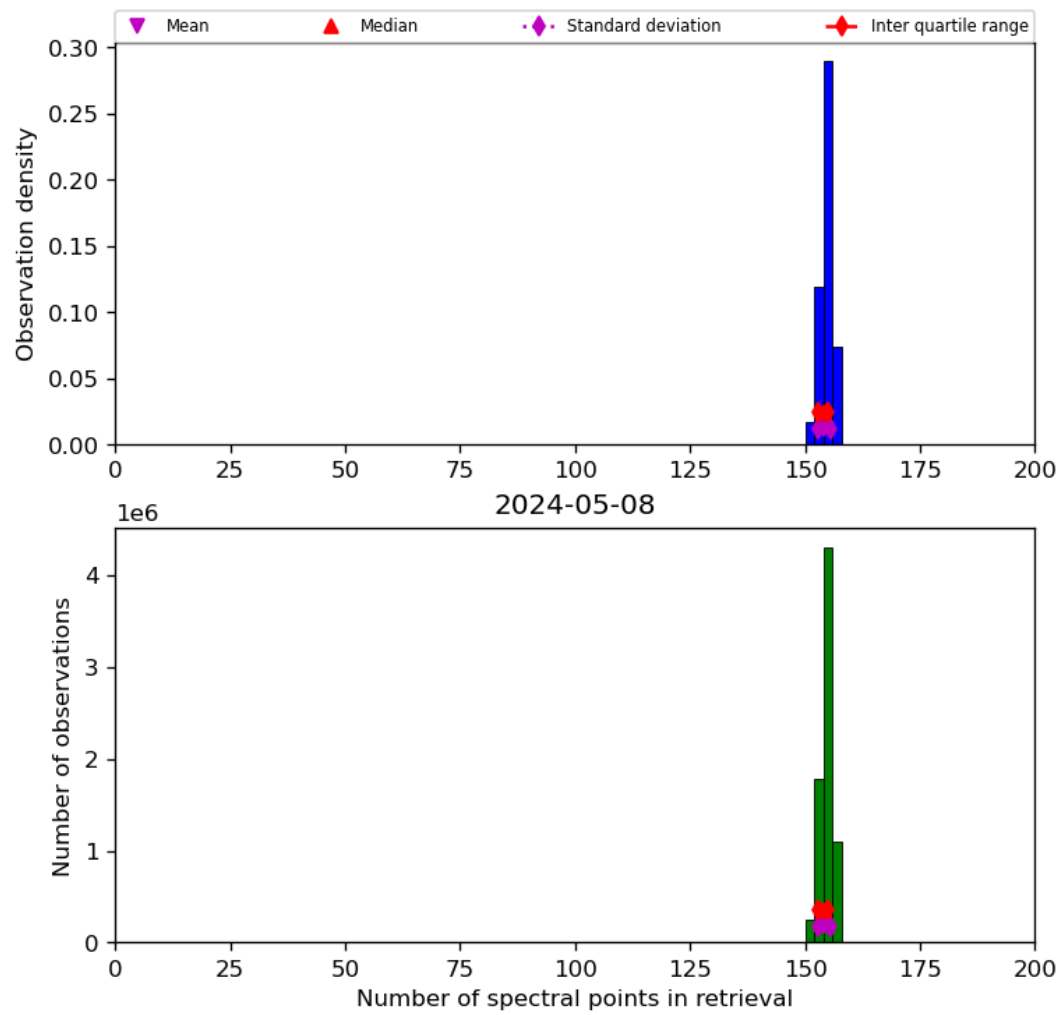
Figure 21: Histogram of “Number of spectral points in retrieval” for 2024-05-07 to 2024-05-09
