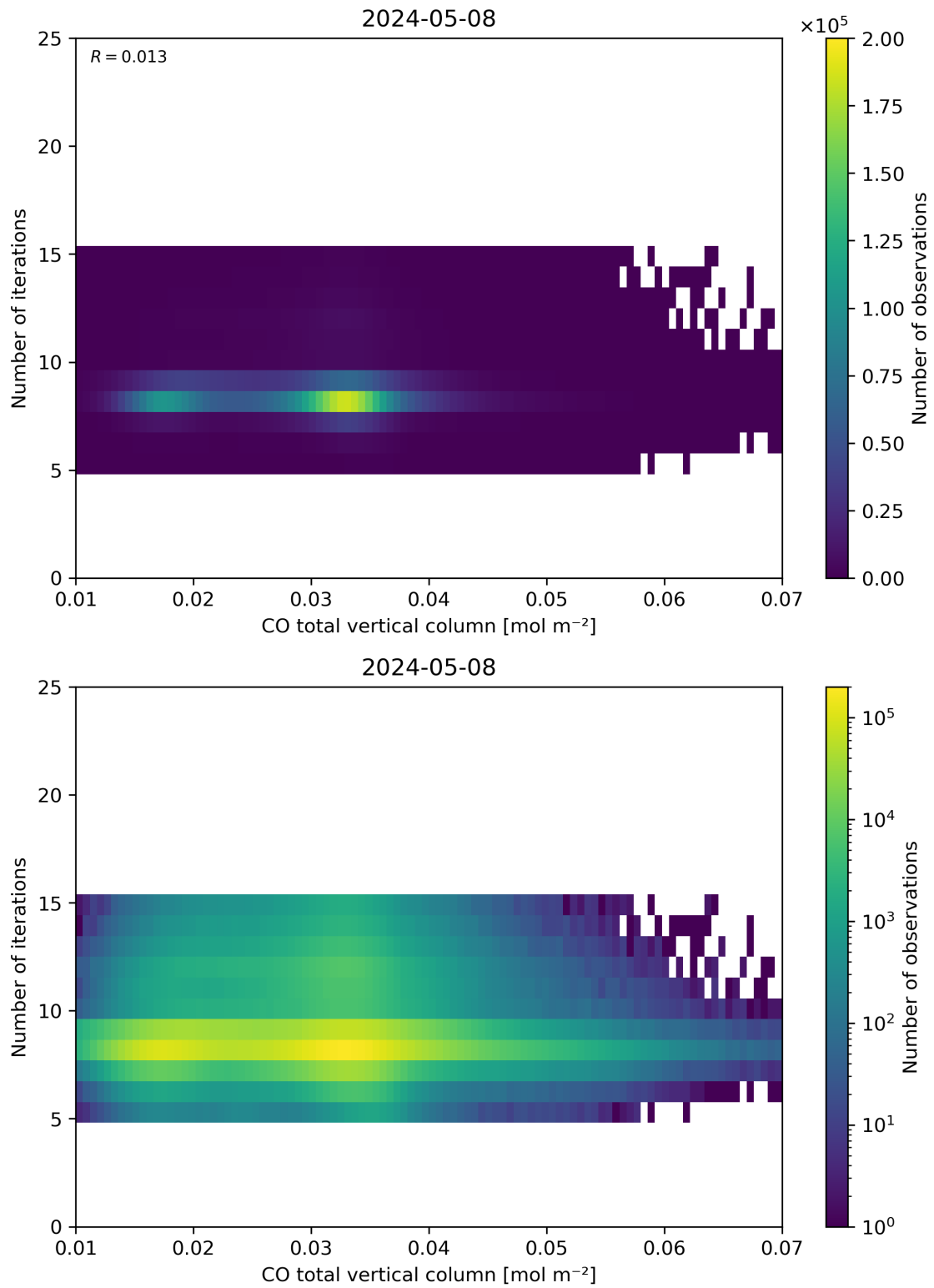
Figure 42: Scatter density plot of “CO total vertical column” against “Number of iterations” for 2024-05-07 to 2024-05-09.
