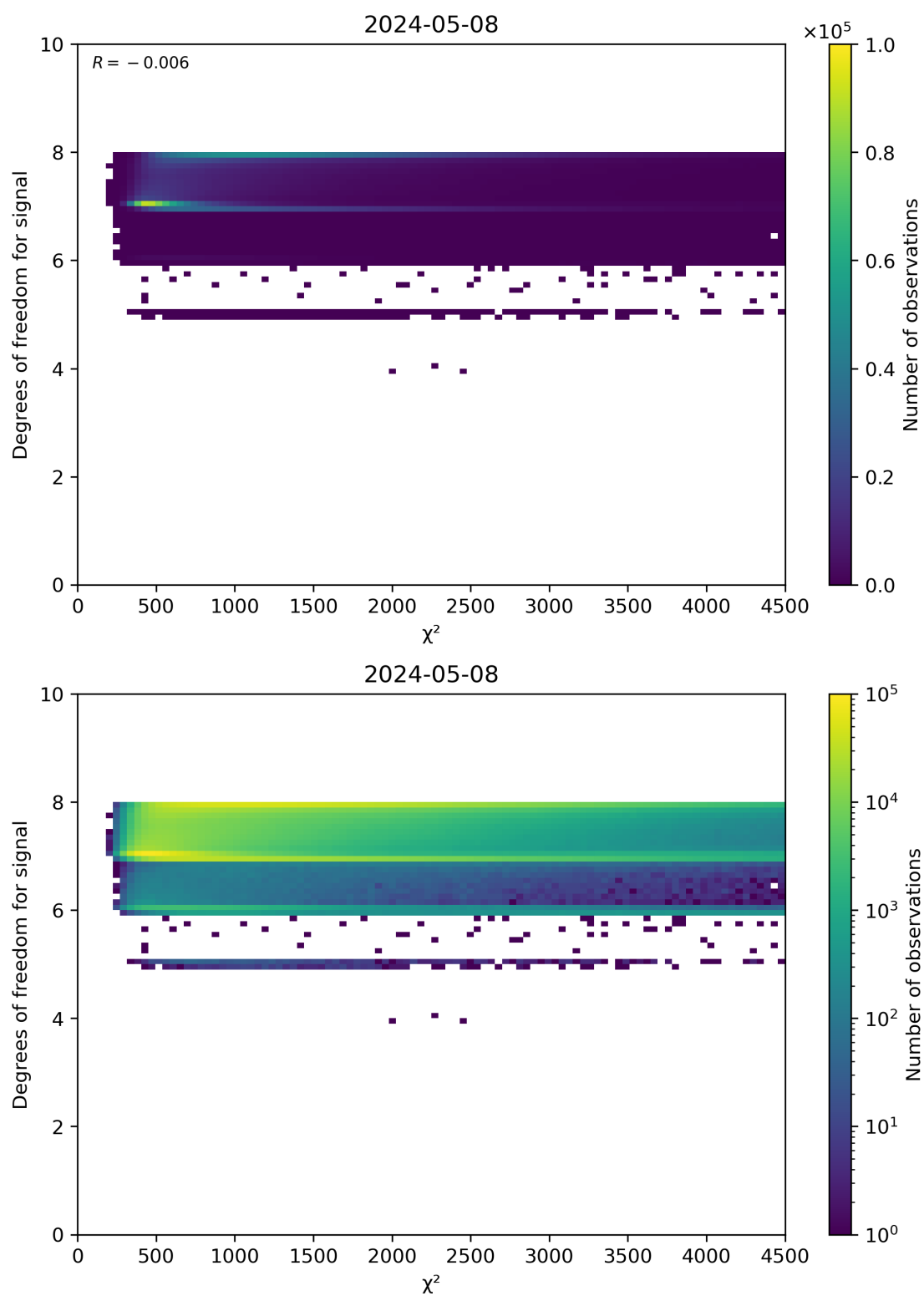
Figure 48: Scatter density plot of “ \chi^2 ” against “Degrees of freedom for signal” for 2024-05-07 to 2024-05-09.
