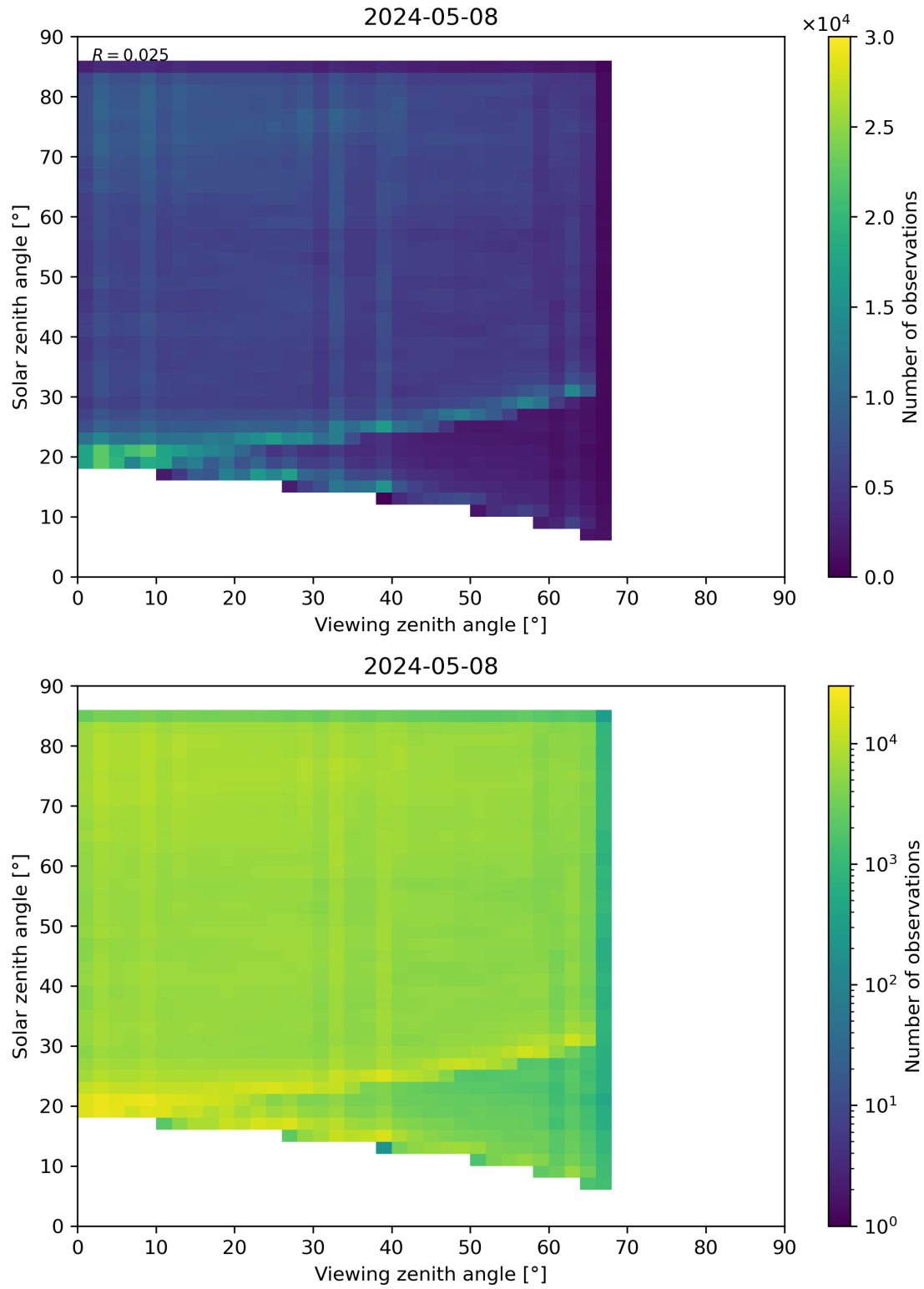
Figure 77: Scatter density plot of “Viewing zenith angle” against “Solar zenith angle” for 2024-05-07 to 2024-05-09.
