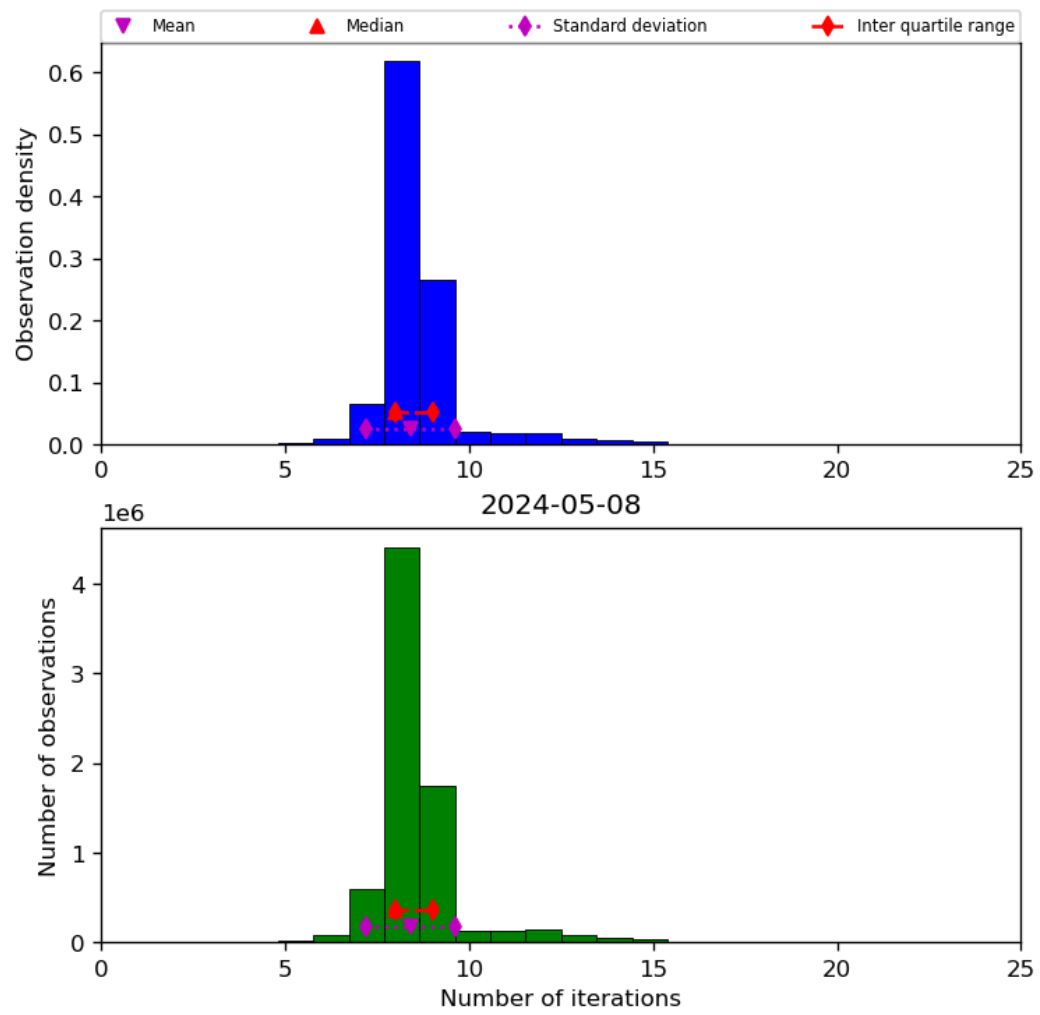
Figure 24: Histogram of “Number of iterations” for 2024-05-07 to 2024-05-09
