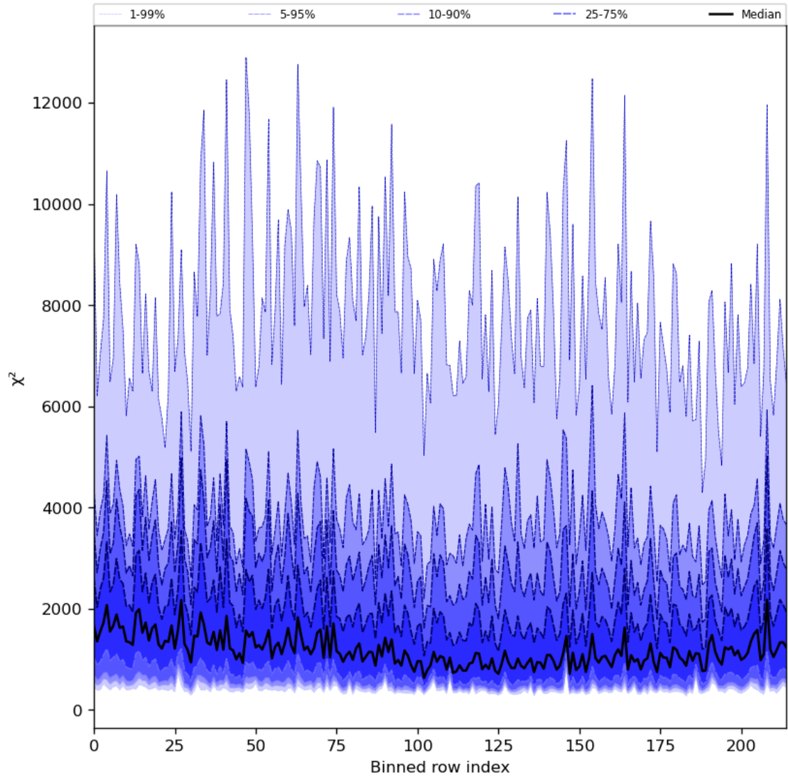
Figure 30: Along track statistics of “ \chi^2 ” for 2024-05-07 to 2024-05-09
