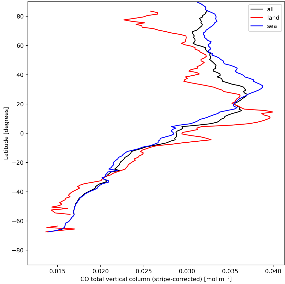
Figure 11: Zonal average of “CO total vertical column (stripe-corrected)” for 2024-05-07 to 2024-05-09.
