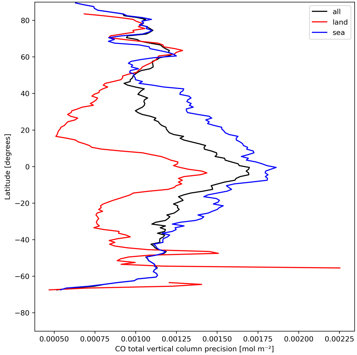
Figure 12: Zonal average of “CO total vertical column precision” for 2024-05-07 to 2024-05-09.
