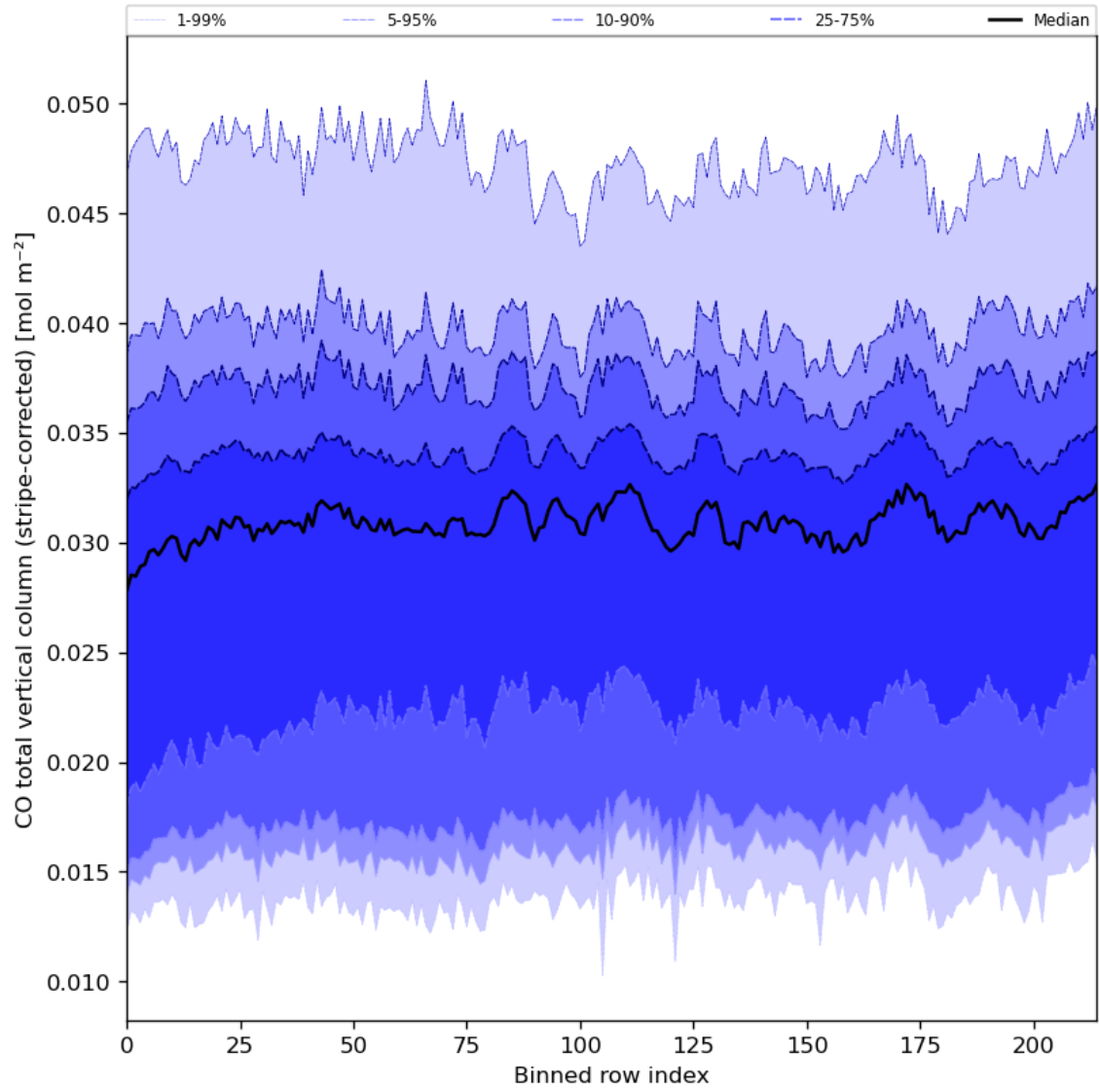
Figure 27: Along track statistics of “CO total vertical column (stripe-corrected)” for 2024-05-07 to 2024-05-09
