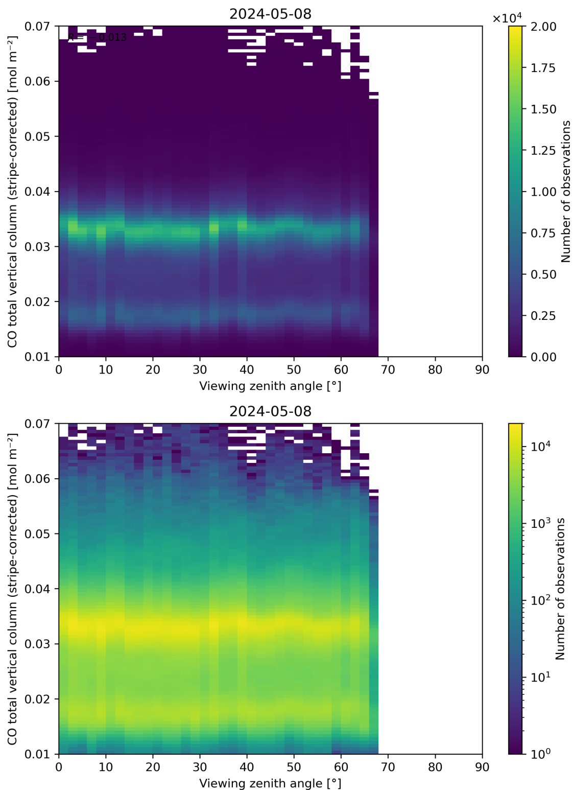
Figure 70: Scatter density plot of “Viewing zenith angle” against “CO total vertical column (stripe-corrected)” for 2024-05-07 to 2024-05-09.
