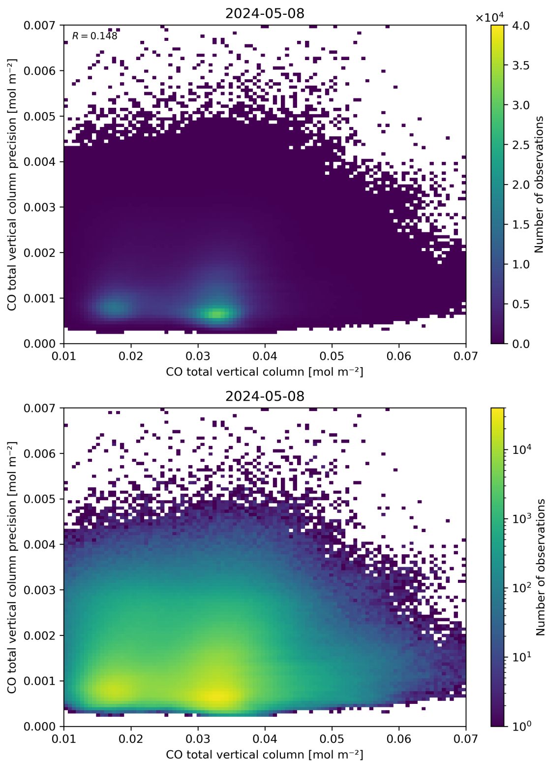
Figure 34: Scatter density plot of “CO total vertical column” against “CO total vertical column precision” for 2024-05-07 to 2024-05-09.
