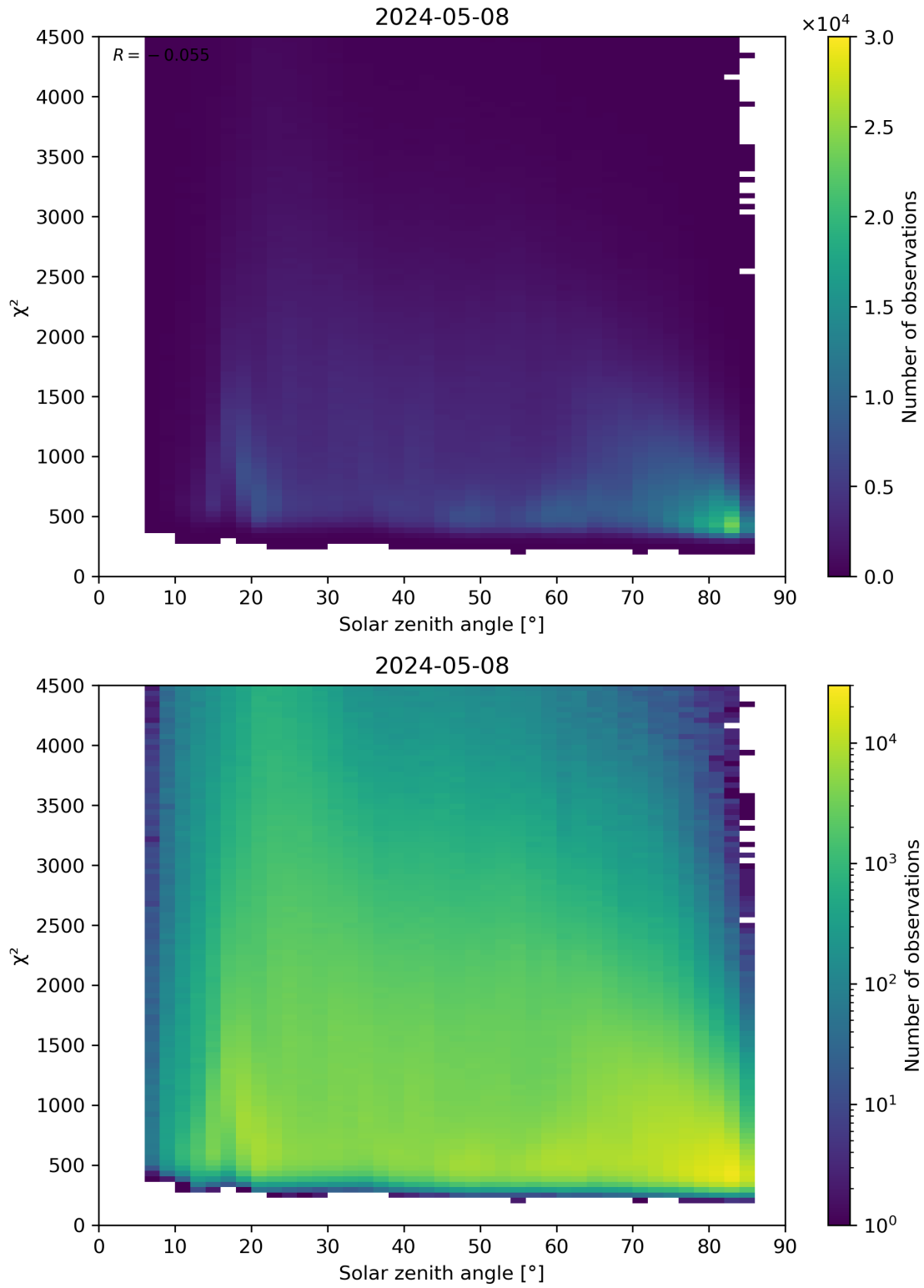
Figure 64: Scatter density plot of “Solar zenith angle” against “ \chi^2 ” for 2024-05-07 to 2024-05-09.
