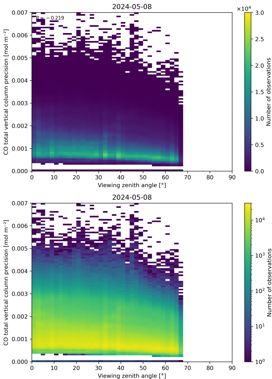
Figure 71: Scatter density plot of “Viewing zenith angle” against “CO total vertical column precision” for 2024-05-07 to 2024-05-09.
