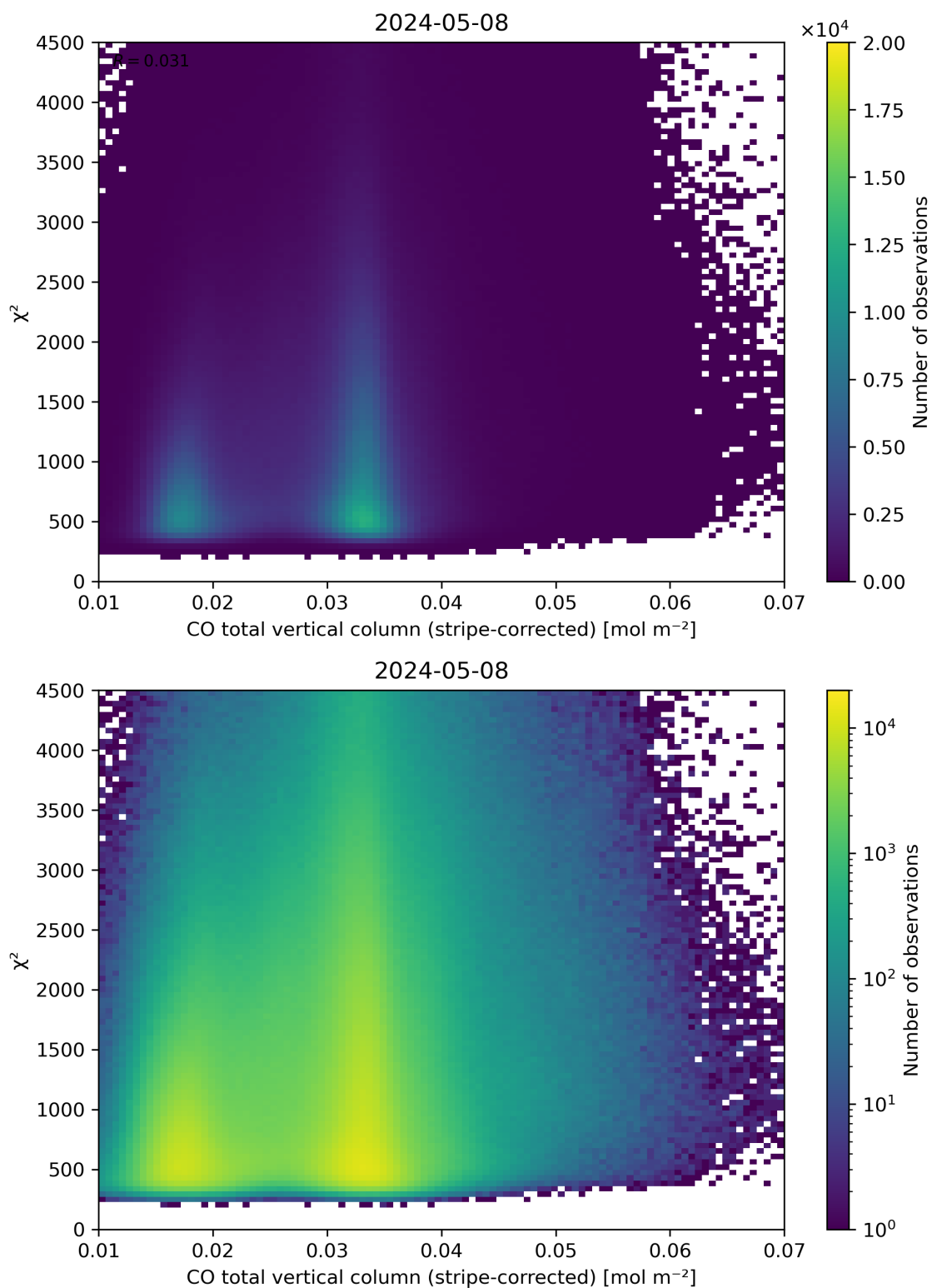
Figure 37: Scatter density plot of “CO total vertical column (stripe-corrected)” against “ \chi^2 ” for 2024-05-07 to 2024-05-09.
