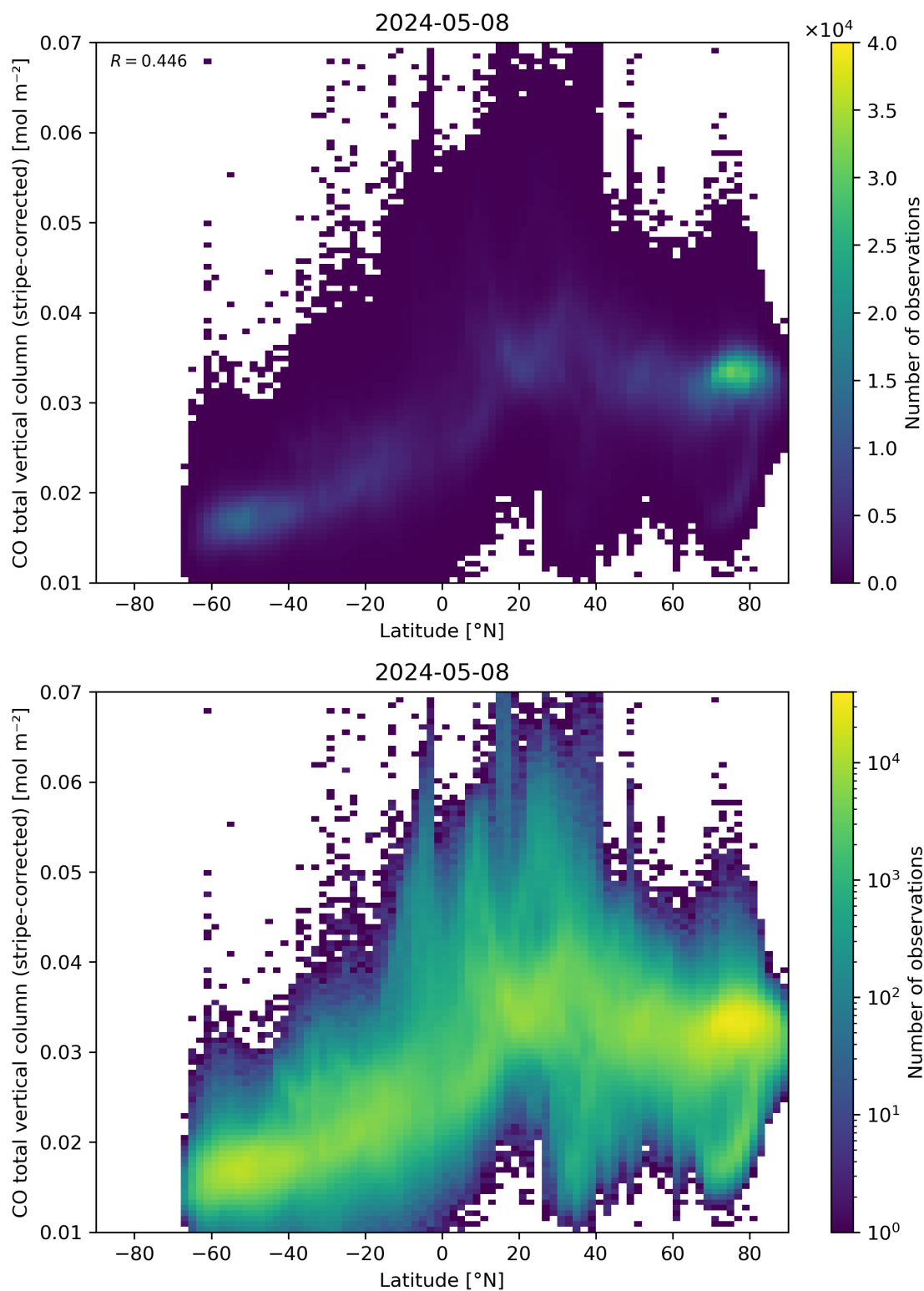
Figure 52: Scatter density plot of “Latitude” against “CO total vertical column (stripe-corrected)” for 2024-05-07 to 2024-05-09.
