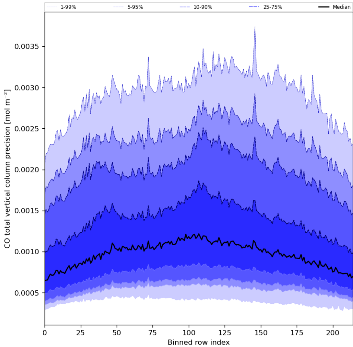
Figure 28: Along track statistics of “CO total vertical column precision” for 2024-05-07 to 2024-05-09
