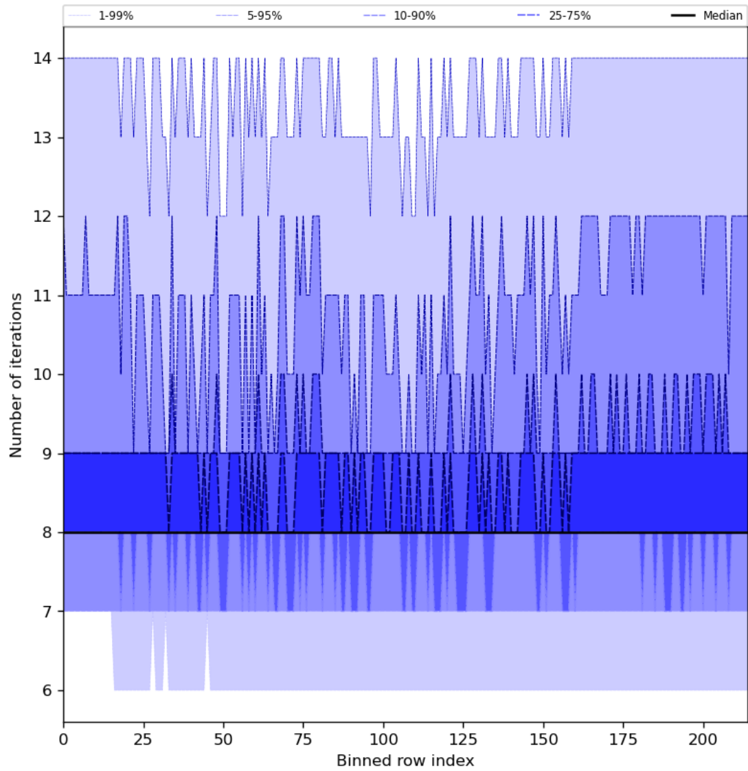
Figure 32: Along track statistics of “Number of iterations” for 2024-05-07 to 2024-05-09
