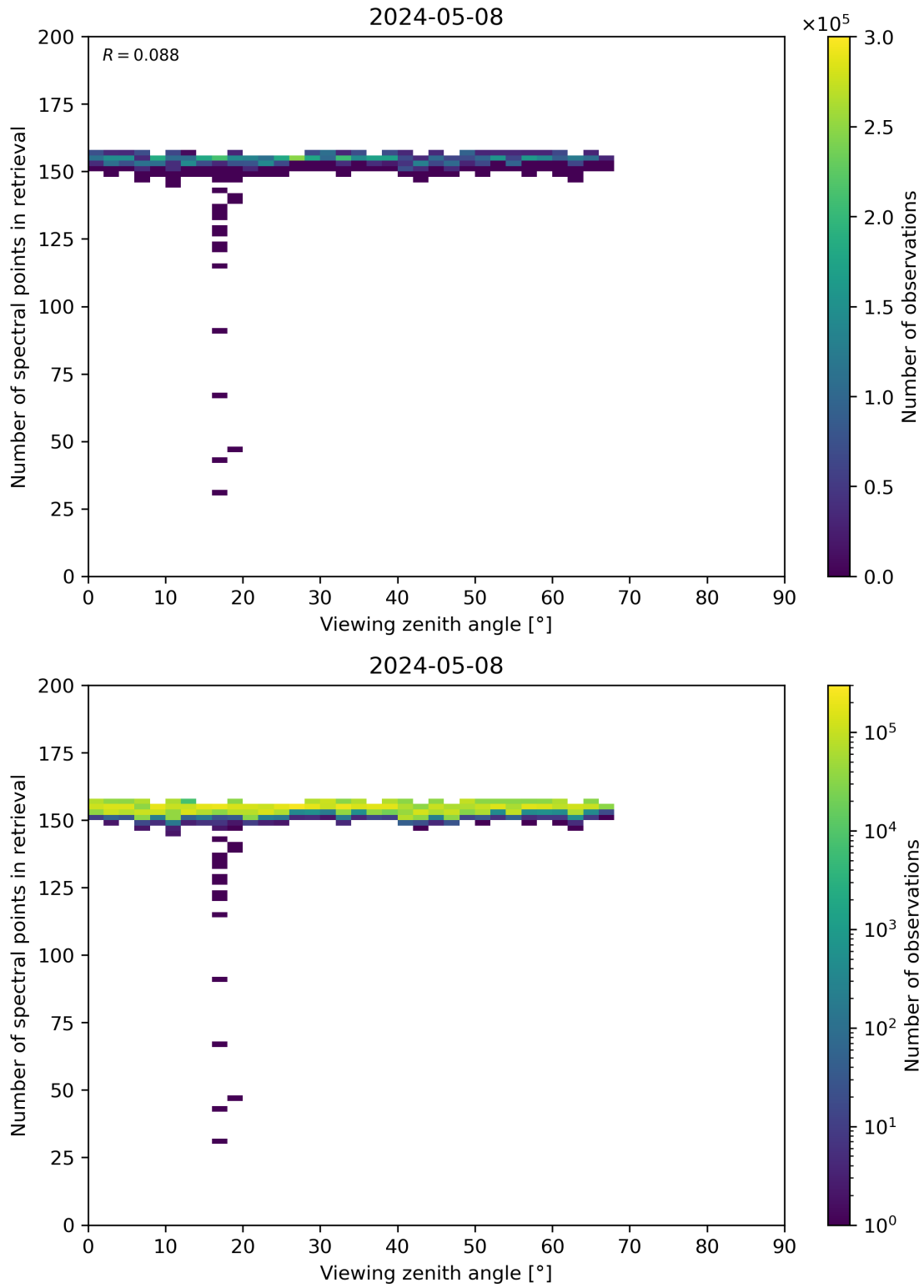
Figure 76: Scatter density plot of “Viewing zenith angle” against “Number of spectral points in retrieval” for 2024-05-07 to 2024-05-09.
