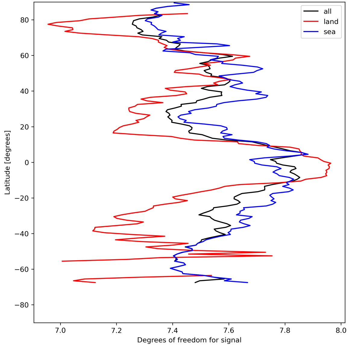
Figure 15: Zonal average of “Degrees of freedom for signal” for 2024-05-07 to 2024-05-09.
