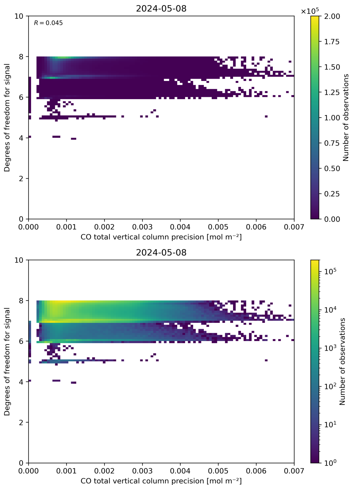
Figure 45: Scatter density plot of “CO total vertical column precision” against “Degrees of freedom for signal” for 2024-05-07 to 2024-05-09.
