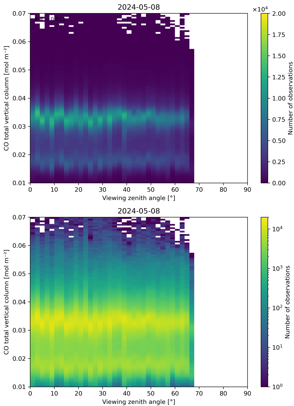
Figure 69: Scatter density plot of “Viewing zenith angle” against “CO total vertical column” for 2024-05-07 to 2024-05-09.
