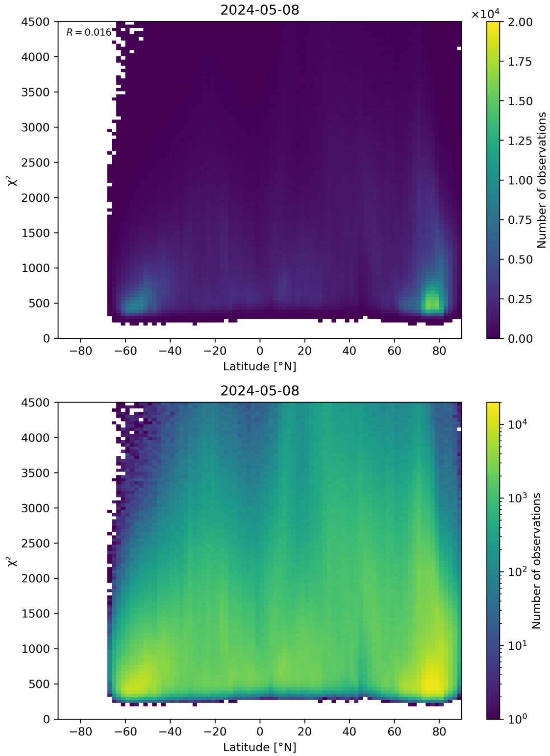
Figure 54: Scatter density plot of “Latitude” against “ \chi^2 ” for 2024-05-07 to 2024-05-09.
