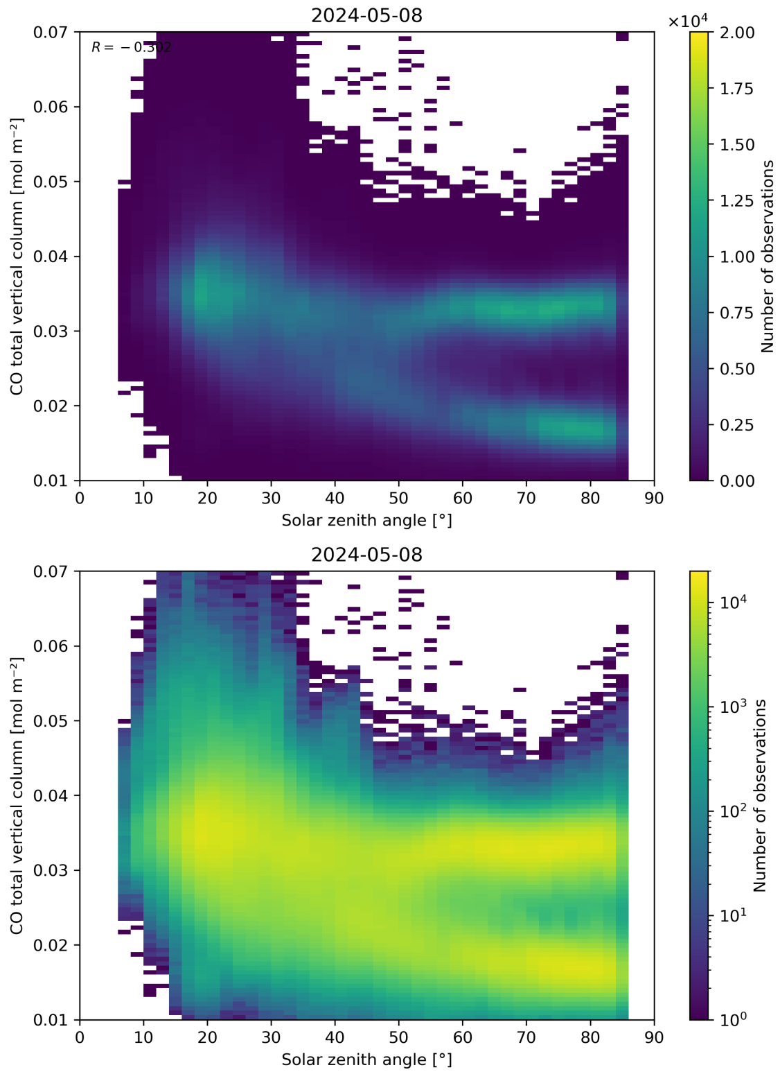
Figure 61: Scatter density plot of “Solar zenith angle” against “CO total vertical column” for 2024-05-07 to 2024-05-09.
