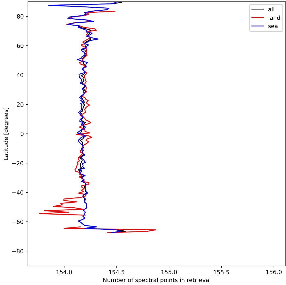
Figure 13: Zonal average of “Number of spectral points in retrieval” for 2024-05-07 to 2024-05-09.
