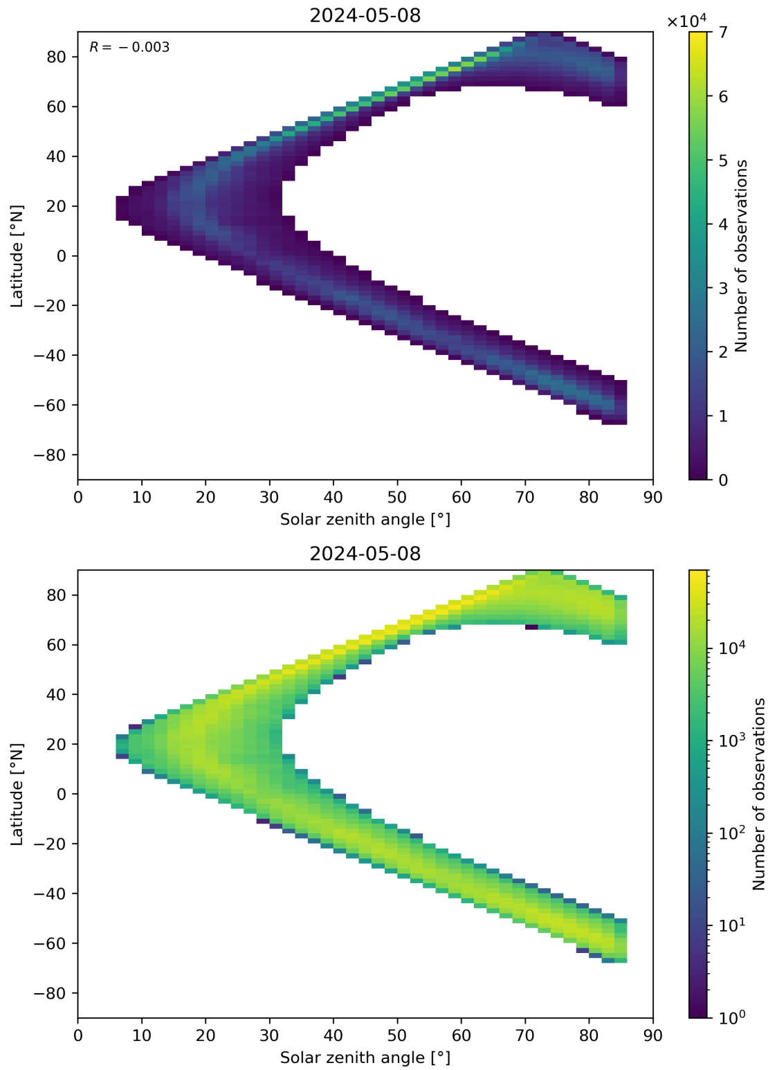
Figure 66: Scatter density plot of “Solar zenith angle” against “Latitude” for 2024-05-07 to 2024-05-09.
