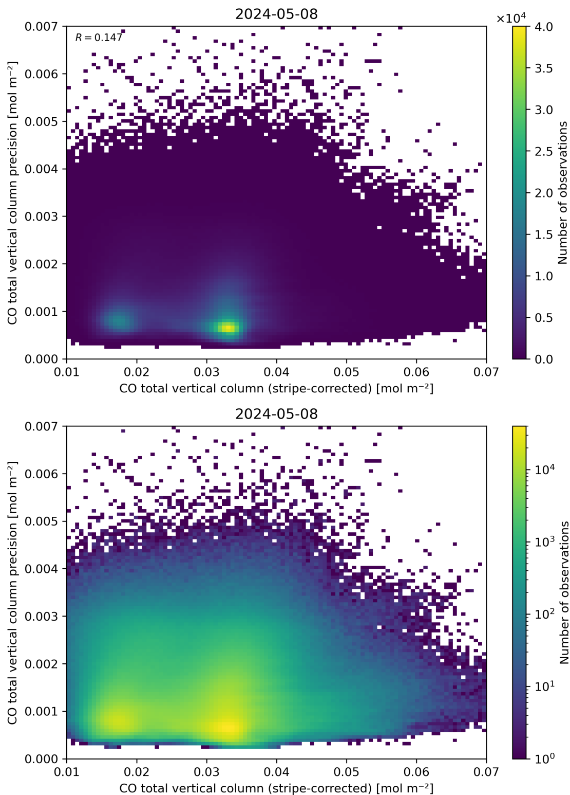
Figure 36: Scatter density plot of “CO total vertical column (stripe-corrected)” against “CO total vertical column precision” for 2024-05-07 to 2024-05-09.
