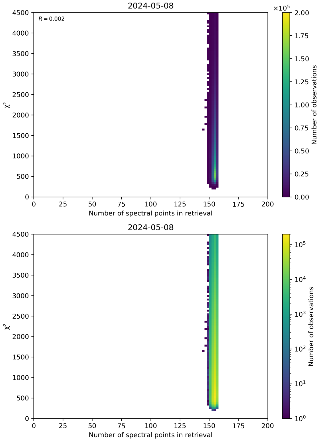
Figure 58: Scatter density plot of “Number of spectral points in retrieval” against “ \chi^2 ” for 2024-05-07 to 2024-05-09.
