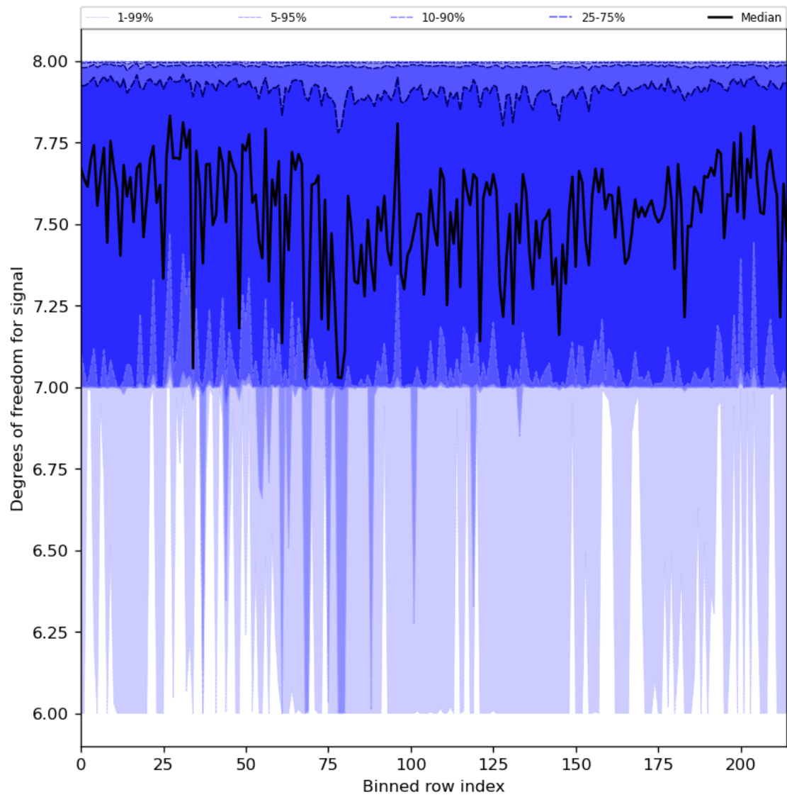
Figure 31: Along track statistics of “Degrees of freedom for signal” for 2024-05-07 to 2024-05-09
