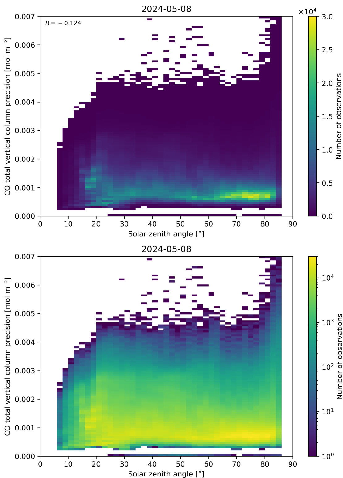
Figure 63: Scatter density plot of “Solar zenith angle” against “CO total vertical column precision” for 2024-05-07 to 2024-05-09.
