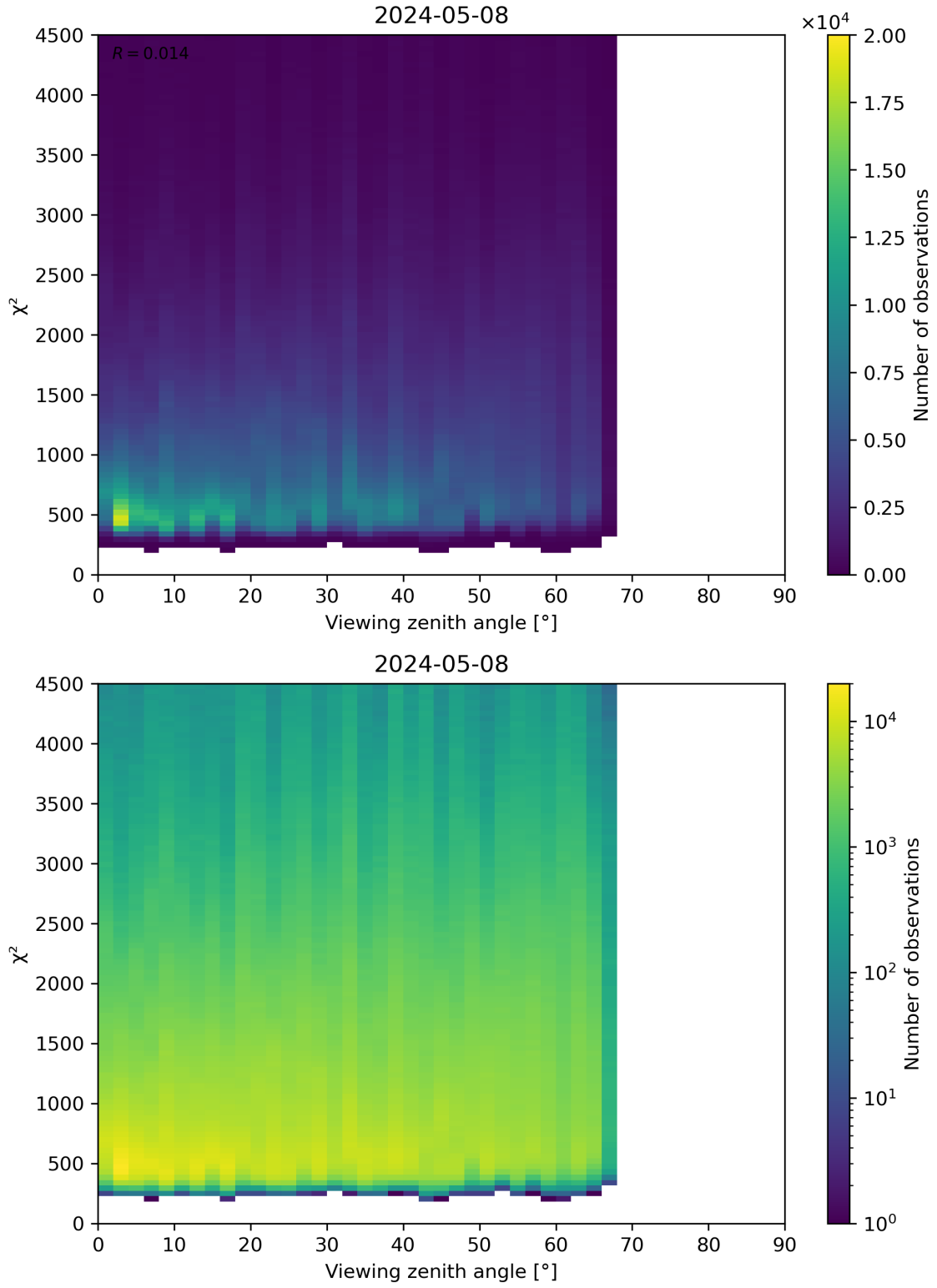
Figure 72: Scatter density plot of “Viewing zenith angle” against “ \chi^2 ” for 2024-05-07 to 2024-05-09.
