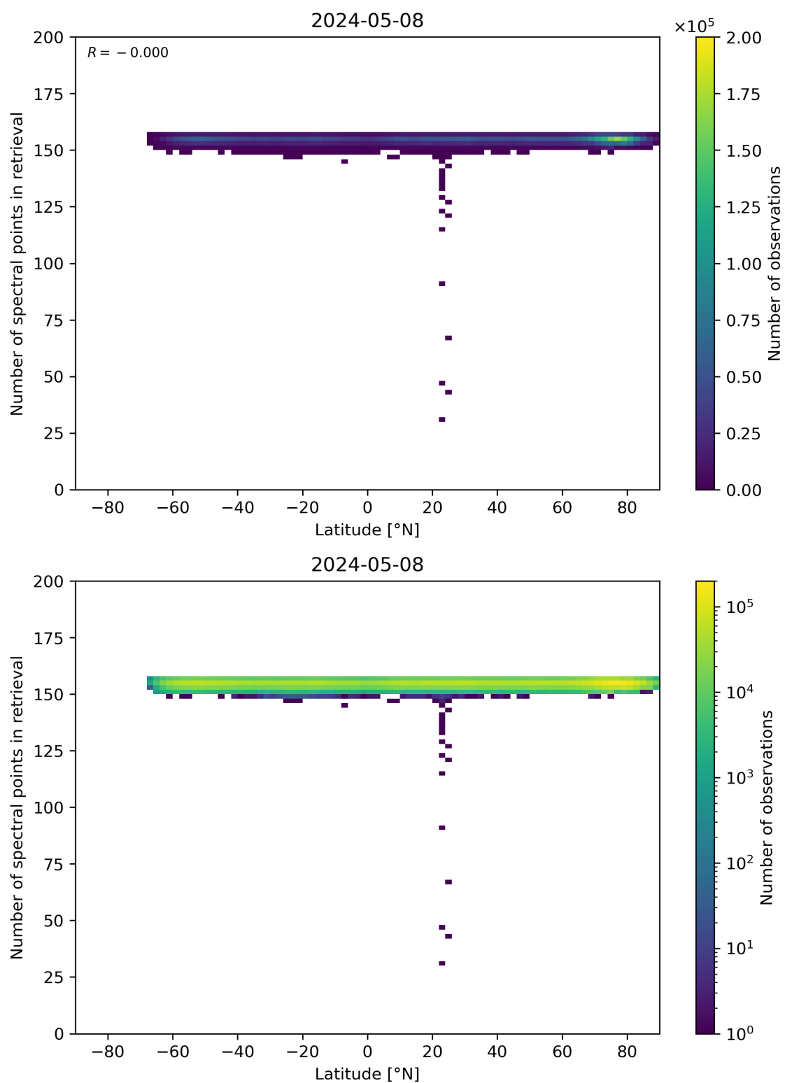
Figure 57: Scatter density plot of “Latitude” against “Number of spectral points in retrieval” for 2024-05-07 to 2024-05-09.
