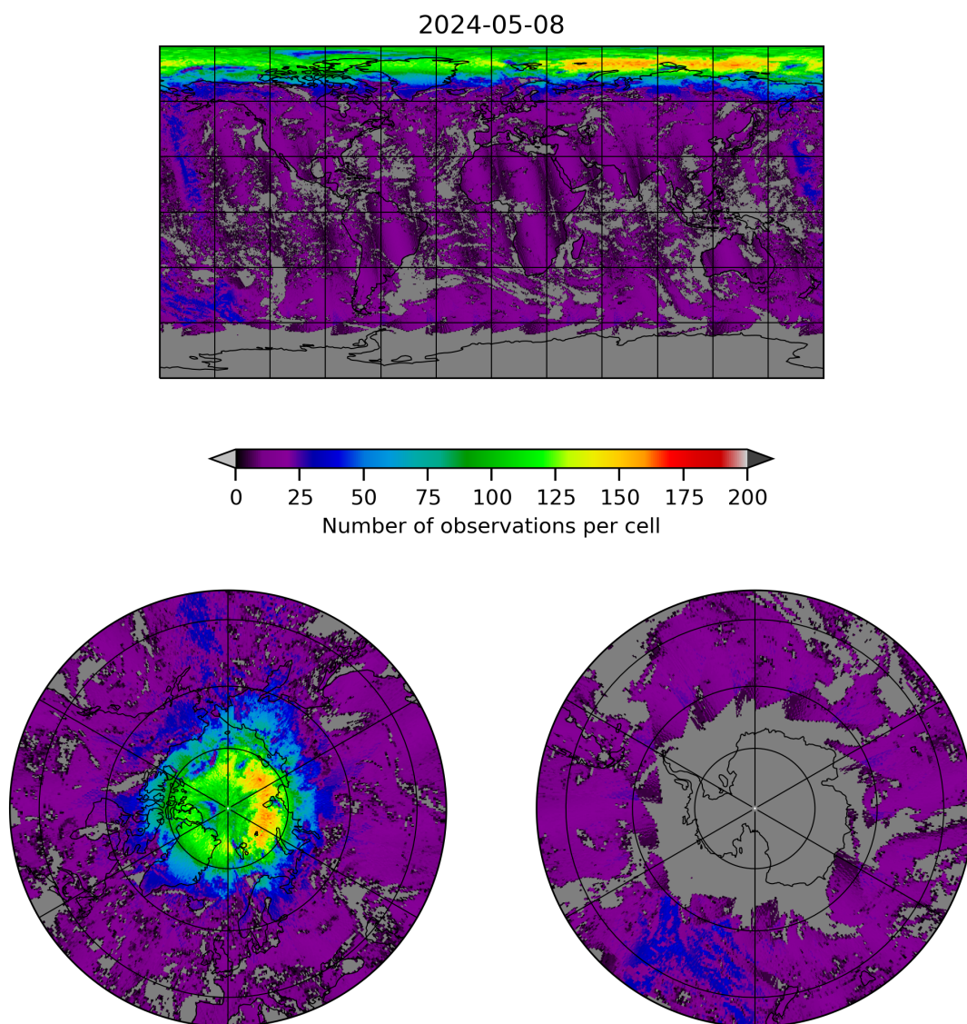
Figure 8: Map of the number of observations for 2024-05-07 to 2024-05-09
