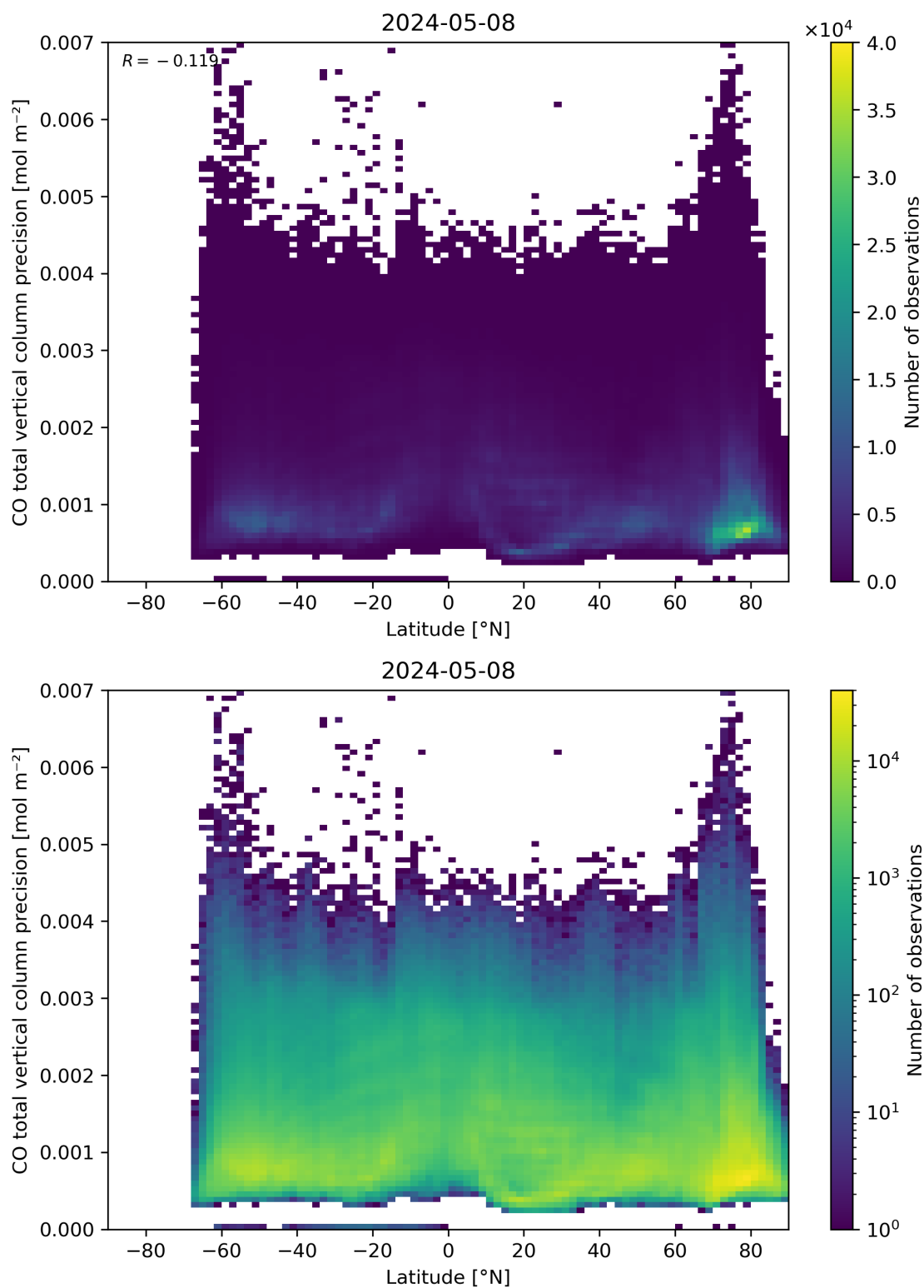
Figure 53: Scatter density plot of “Latitude” against “CO total vertical column precision” for 2024-05-07 to 2024-05-09.
