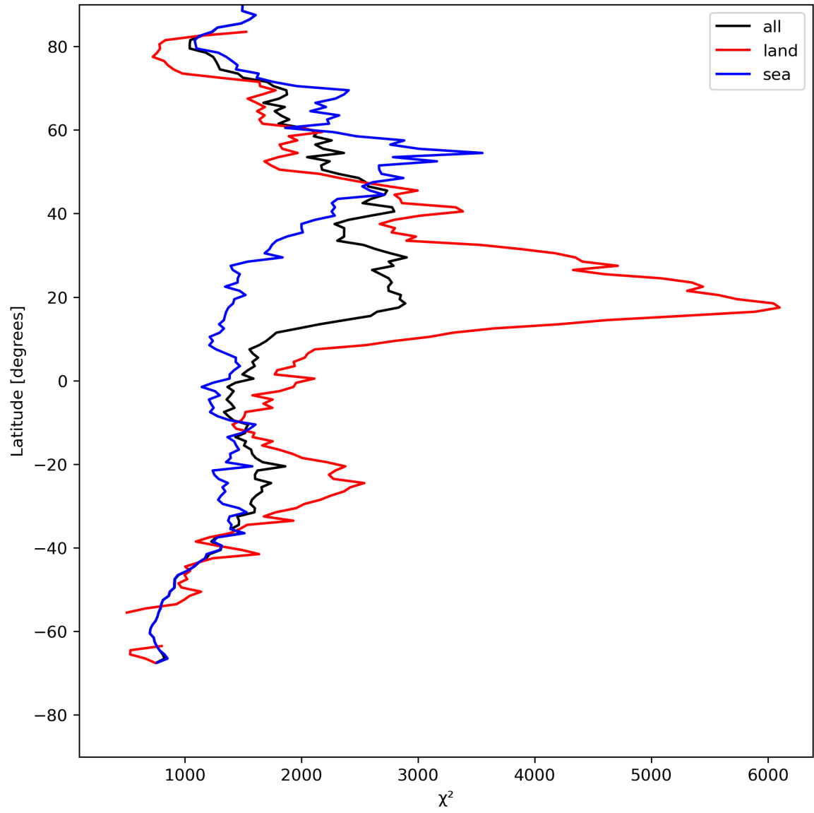
Figure 14: Zonal average of “ \chi^2 ” for 2024-05-07 to 2024-05-09.
