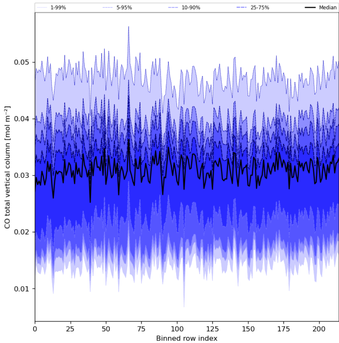
Figure 26: Along track statistics of “CO total vertical column” for 2024-05-07 to 2024-05-09
