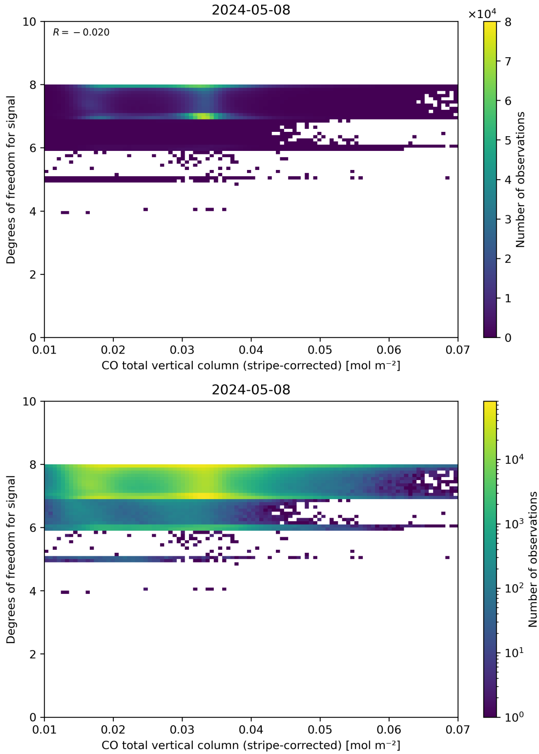
Figure 38: Scatter density plot of “CO total vertical column (stripe-corrected)” against “Degrees of freedom for signal” for 2024-05-07 to 2024-05-09.
