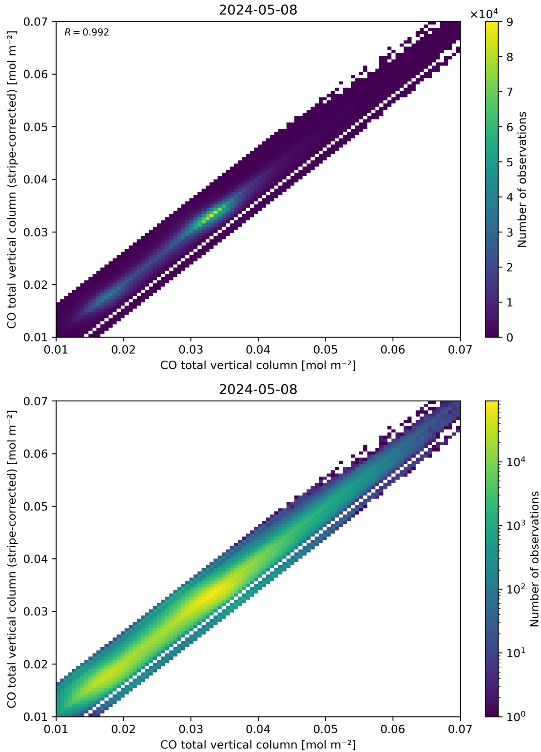
Figure 33: Scatter density plot of “CO total vertical column” against “CO total vertical column (stripe-corrected)” for 2024-05-07 to 2024-05-09.
