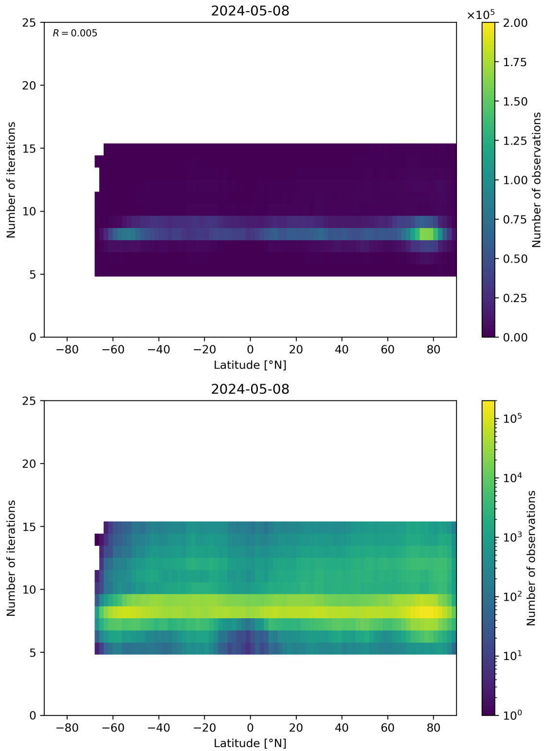
Figure 56: Scatter density plot of “Latitude” against “Number of iterations” for 2024-05-07 to 2024-05-09.
