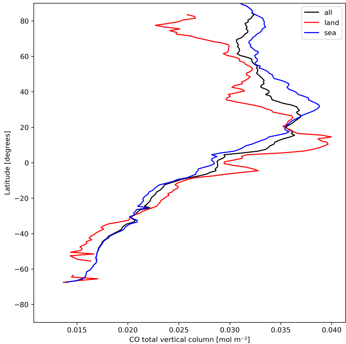
Figure 10: Zonal average of “CO total vertical column” for 2024-05-07 to 2024-05-09.
