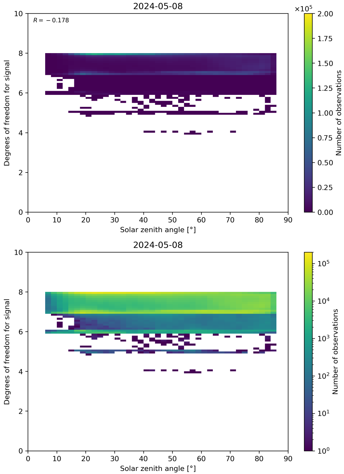
Figure 65: Scatter density plot of “Solar zenith angle” against “Degrees of freedom for signal” for 2024-05-07 to 2024-05-09.
