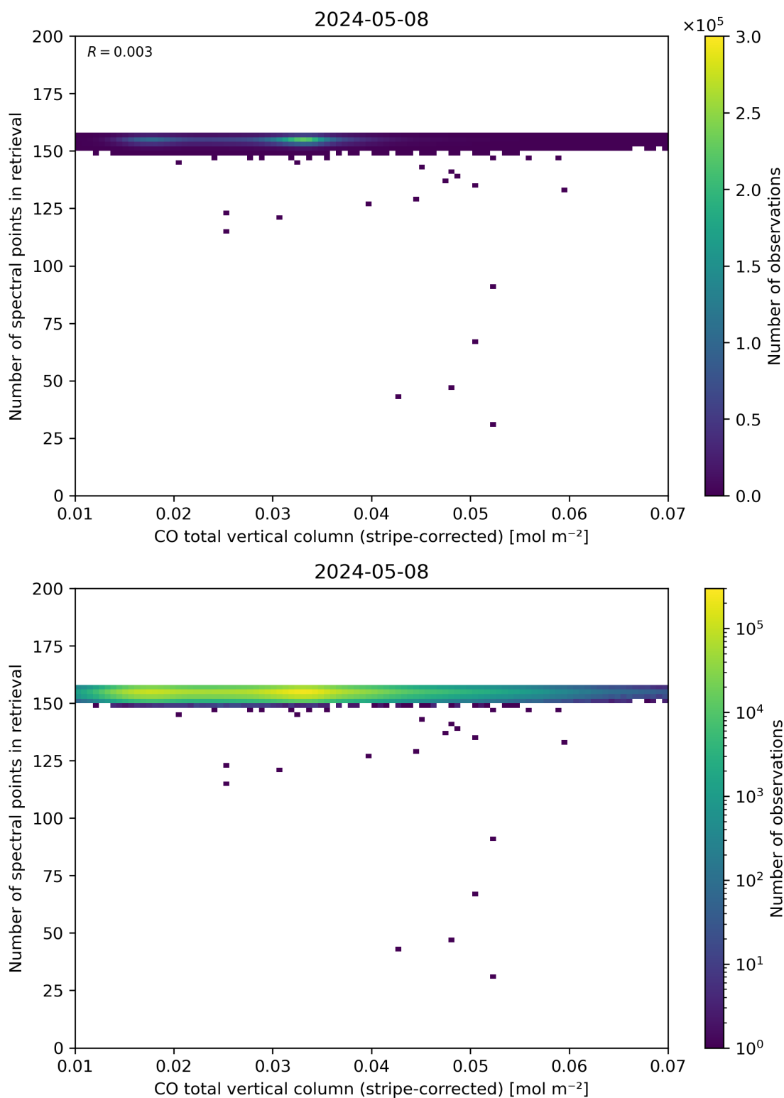
Figure 40: Scatter density plot of “CO total vertical column (stripe-corrected)” against “Number of spectral points in retrieval” for 2024-05-07 to 2024-05-09.
