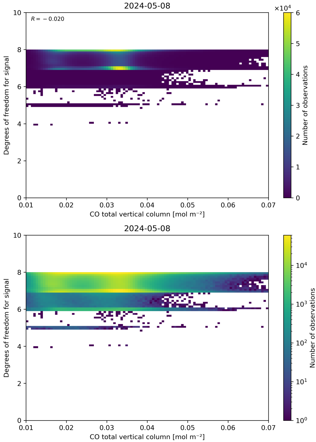
Figure 41: Scatter density plot of “CO total vertical column” against “Degrees of freedom for signal” for 2024-05-07 to 2024-05-09.
