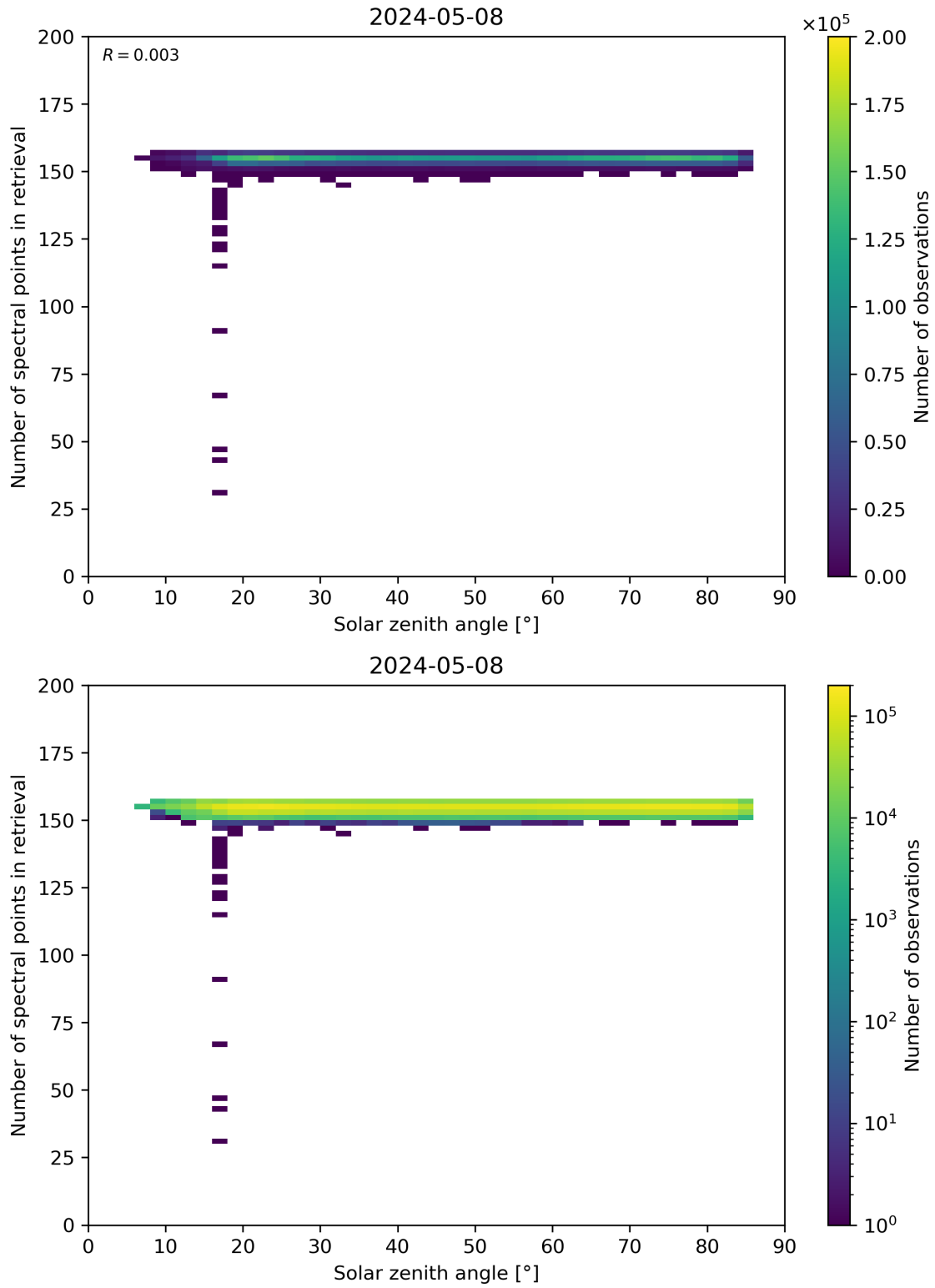
Figure 68: Scatter density plot of “Solar zenith angle” against “Number of spectral points in retrieval” for 2024-05-07 to 2024-05-09.
