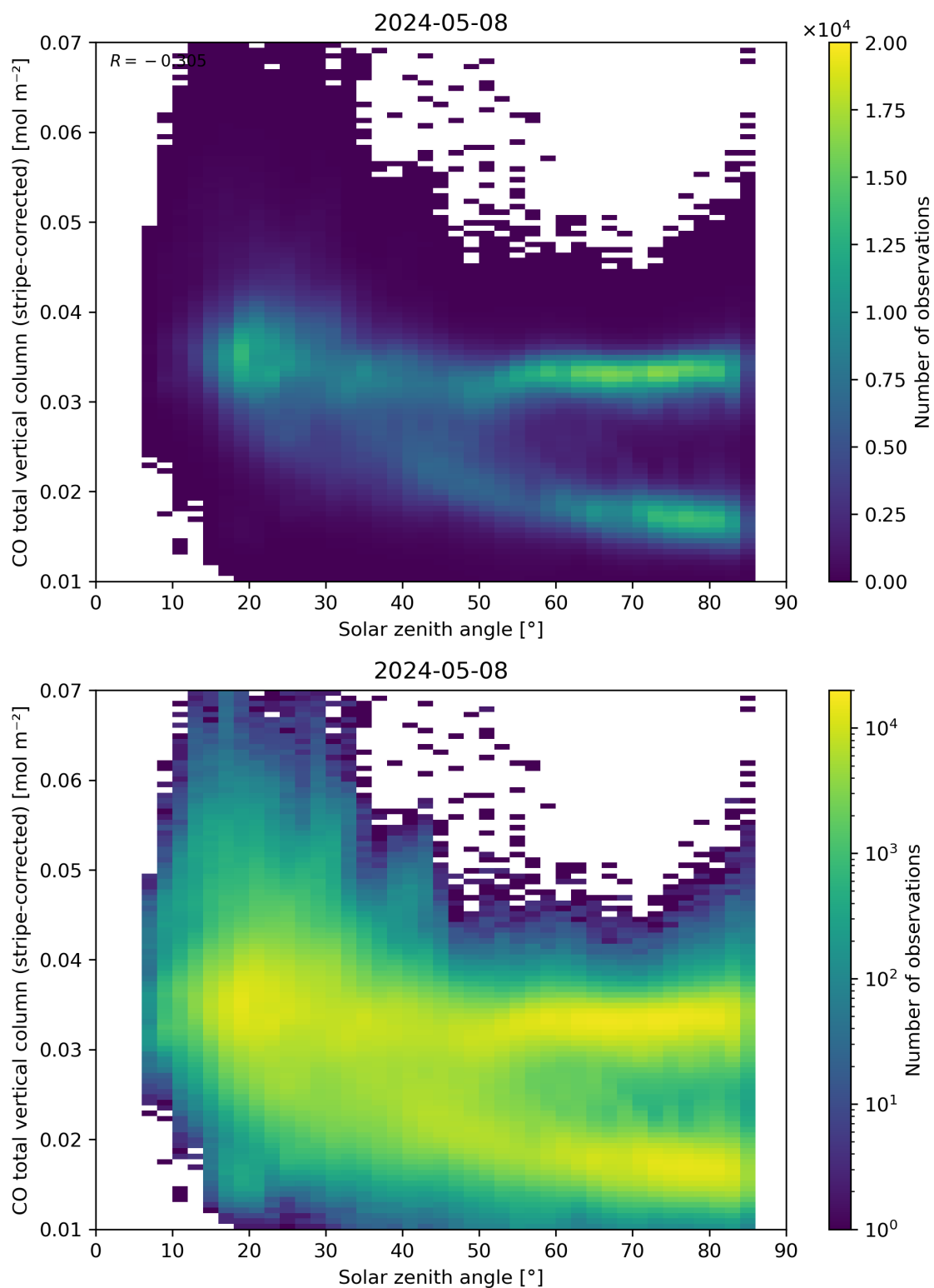
Figure 62: Scatter density plot of “Solar zenith angle” against “CO total vertical column (stripe-corrected)” for 2024-05-07 to 2024-05-09.
