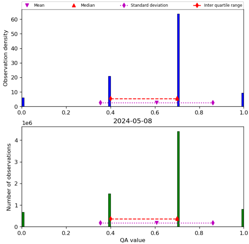
Figure 17: Histogram of “QA value” for 2024-05-07 to 2024-05-09
