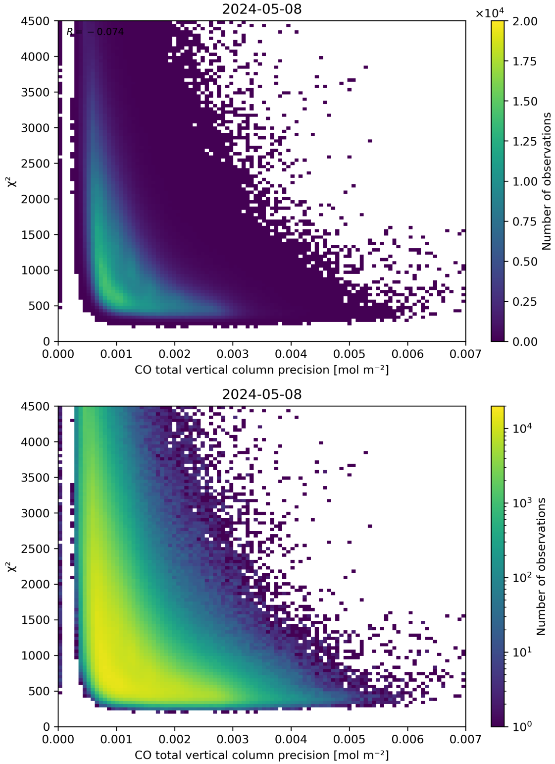
Figure 44: Scatter density plot of “CO total vertical column precision” against “ \chi^2 ” for 2024-05-07 to 2024-05-09.
