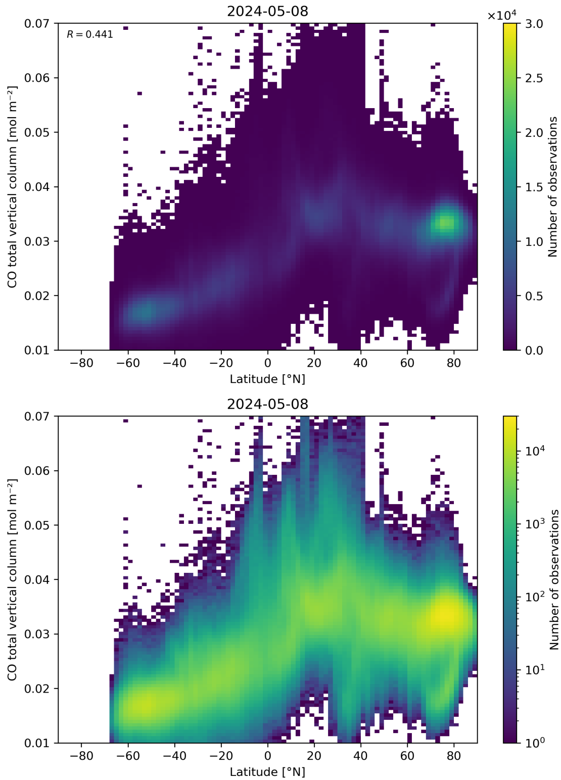
Figure 51: Scatter density plot of “Latitude” against “CO total vertical column” for 2024-05-07 to 2024-05-09.
