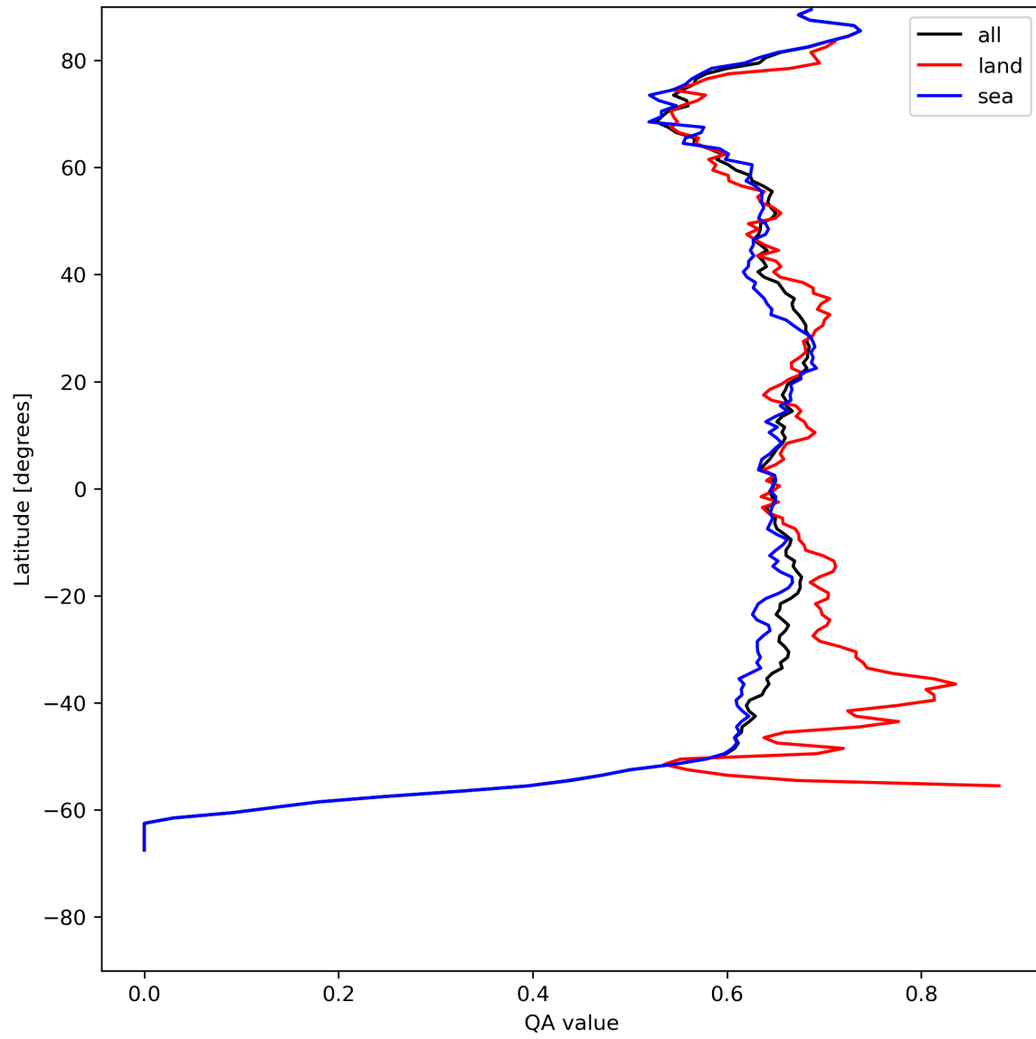
Figure 9: Zonal average of “QA value” for 2024-05-07 to 2024-05-09.
