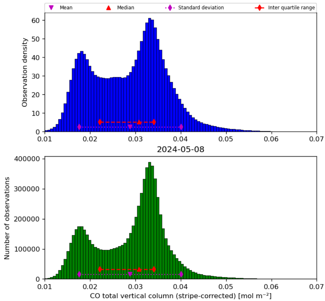
Figure 19: Histogram of “CO total vertical column (stripe-corrected)” for 2024-05-07 to 2024-05-09
