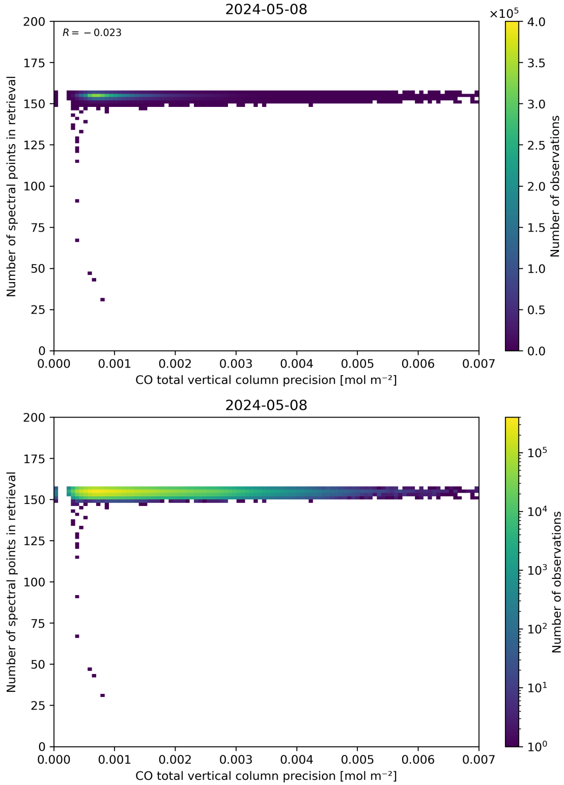
Figure 47: Scatter density plot of “CO total vertical column precision” against “Number of spectral points in retrieval” for 2024-05-07 to 2024-05-09.
