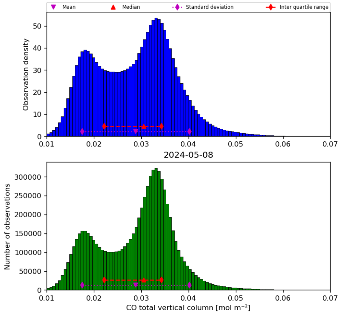
Figure 18: Histogram of “CO total vertical column” for 2024-05-07 to 2024-05-09
