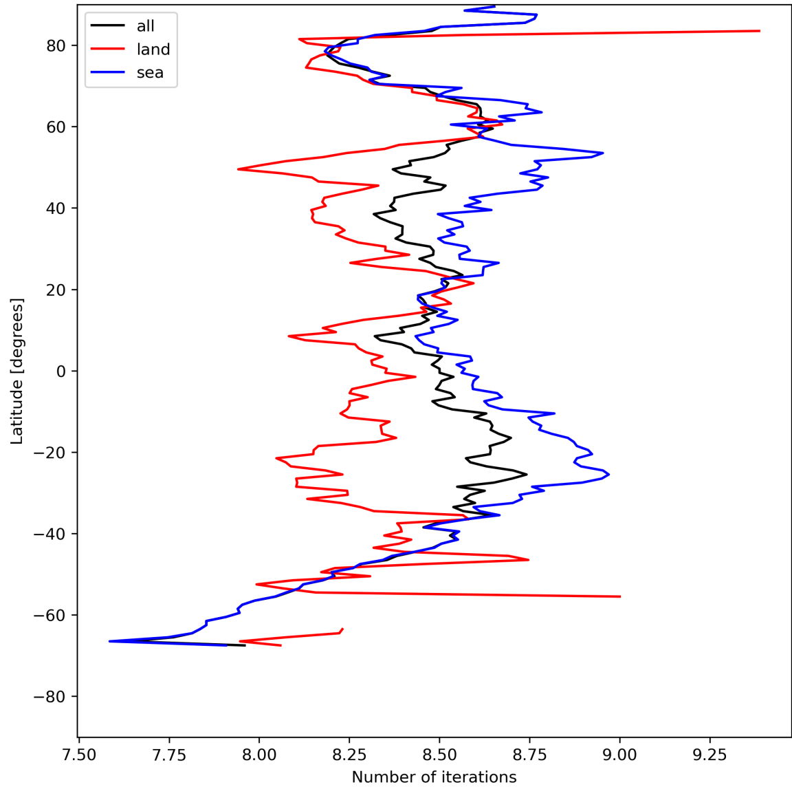
Figure 16: Zonal average of “Number of iterations” for 2024-05-07 to 2024-05-09.
