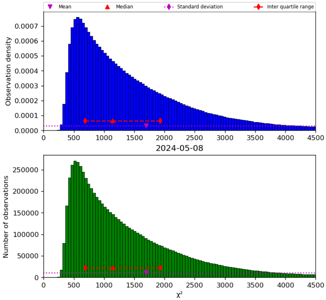
Figure 22: Histogram of “ \chi^2 ” for 2024-05-07 to 2024-05-09
