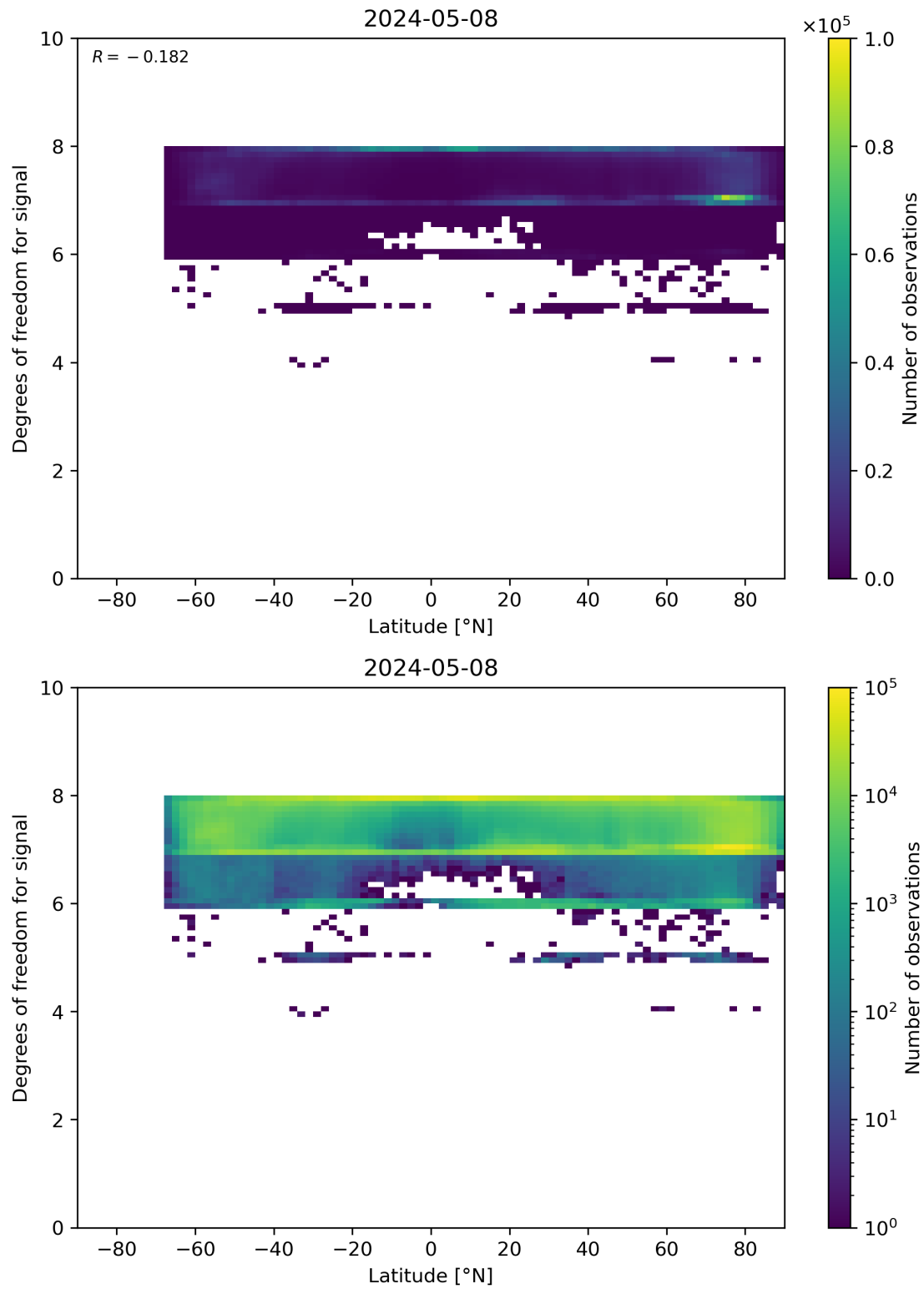
Figure 55: Scatter density plot of “Latitude” against “Degrees of freedom for signal” for 2024-05-07 to 2024-05-09.
