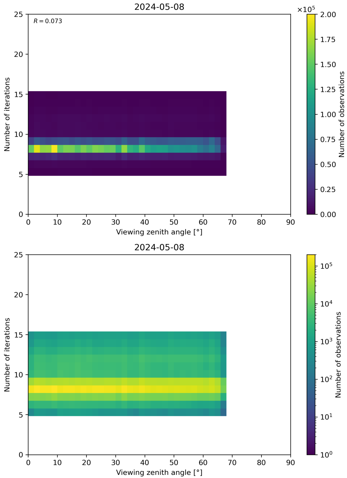
Figure 75: Scatter density plot of “Viewing zenith angle” against “Number of iterations” for 2024-05-07 to 2024-05-09.
