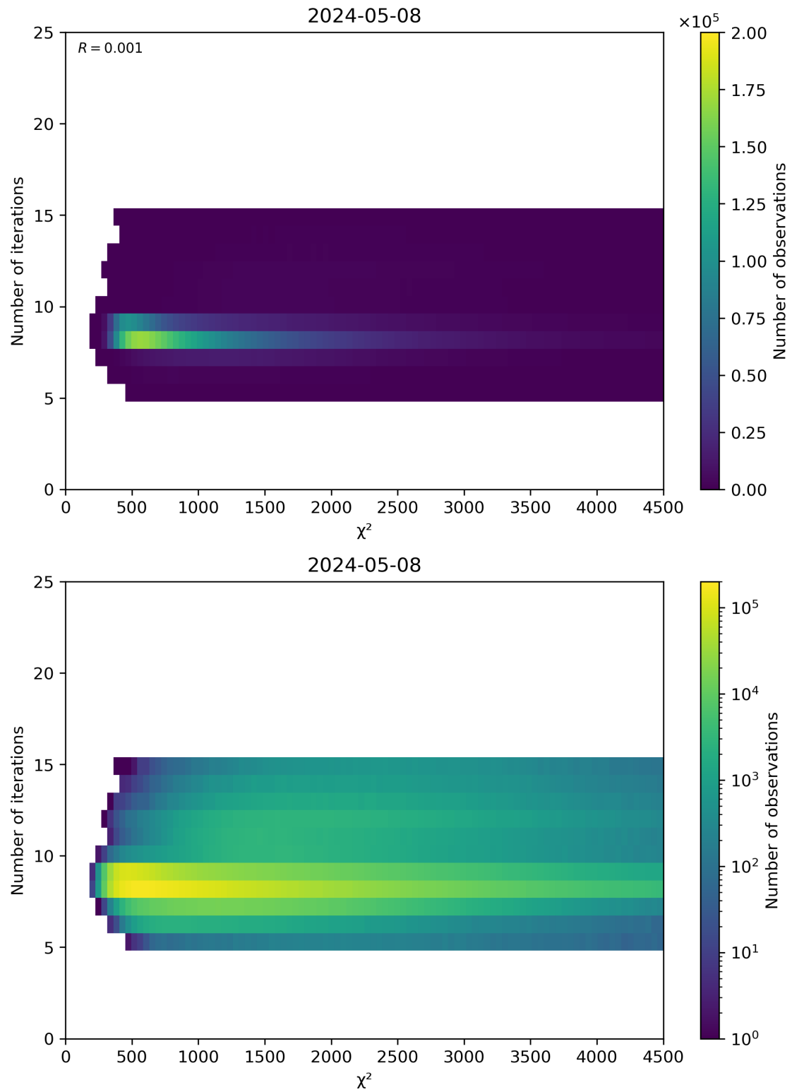
Figure 49: Scatter density plot of “ \chi^2 ” against “Number of iterations” for 2024-05-07 to 2024-05-09.
