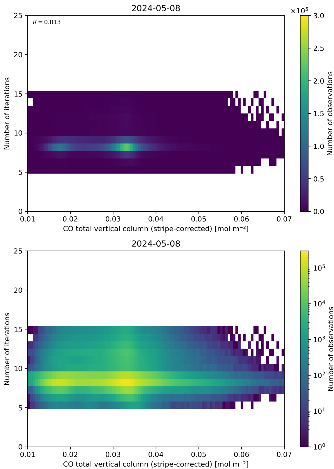
Figure 39: Scatter density plot of “CO total vertical column (stripe-corrected)” against “Number of iterations” for 2024-05-07 to 2024-05-09.
