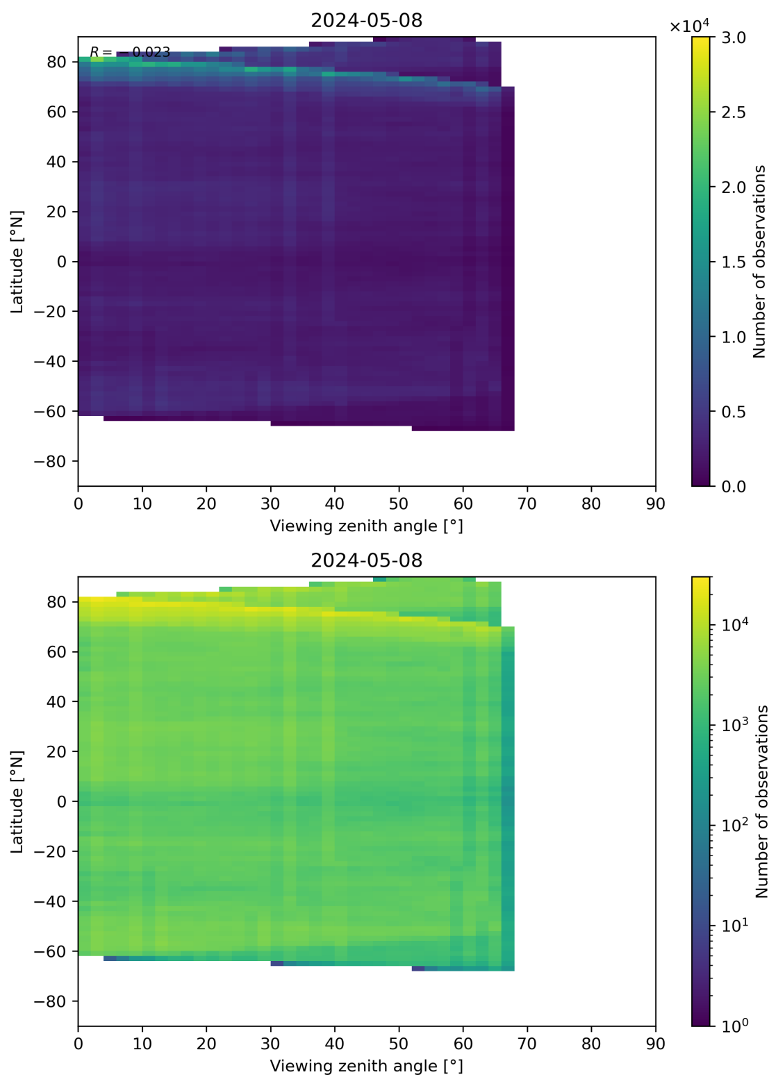
Figure 74: Scatter density plot of “Viewing zenith angle” against “Latitude” for 2024-05-07 to 2024-05-09.
