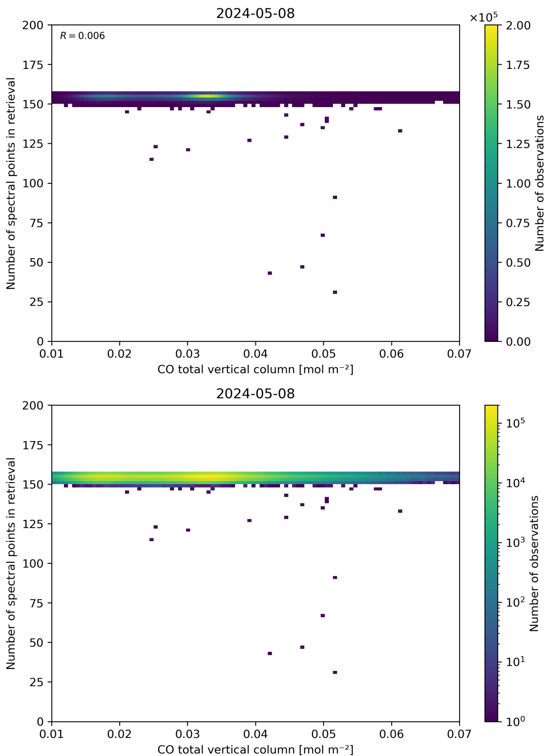
Figure 43: Scatter density plot of “CO total vertical column” against “Number of spectral points in retrieval” for 2024-05-07 to 2024-05-09.
