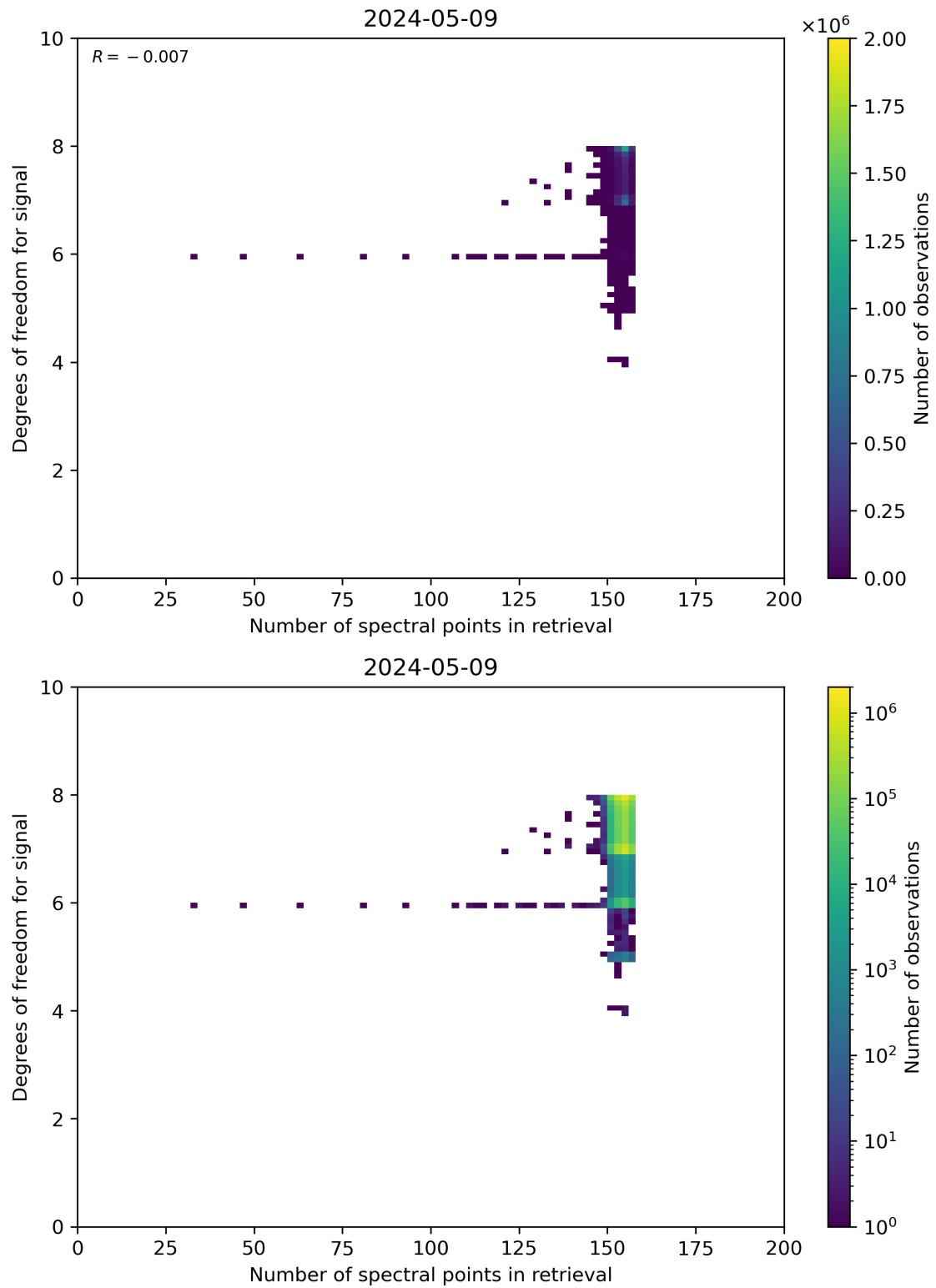
Figure 59: Scatter density plot of “Number of spectral points in retrieval” against “Degrees of freedom for signal” for 2024-05-08 to 2024-05-10.
