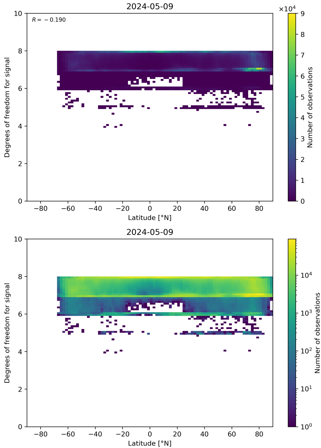
Figure 55: Scatter density plot of “Latitude” against “Degrees of freedom for signal” for 2024-05-08 to 2024-05-10.
