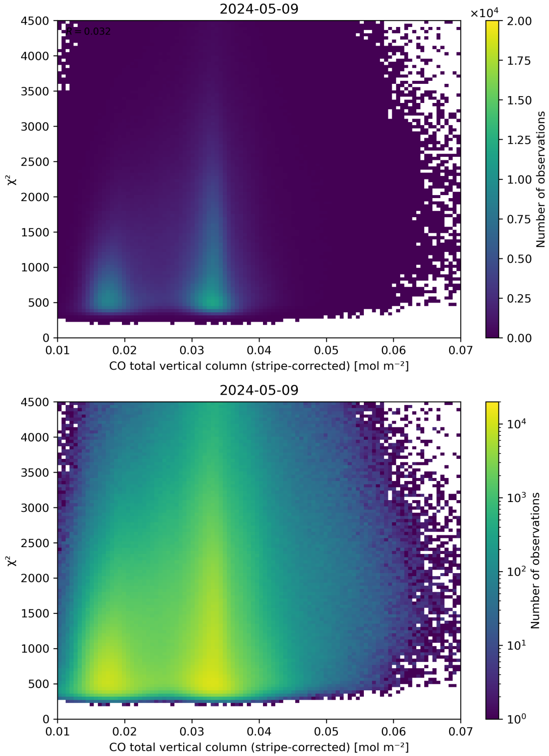
Figure 37: Scatter density plot of “CO total vertical column (stripe-corrected)” against “ \chi^2 ” for 2024-05-08 to 2024-05-10.
