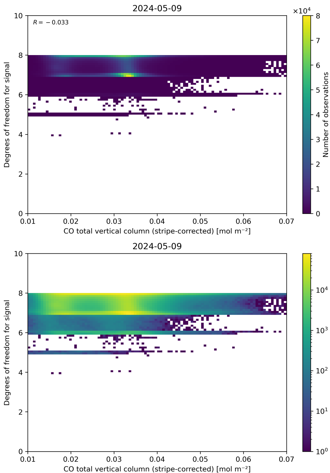
Figure 38: Scatter density plot of “CO total vertical column (stripe-corrected)” against “Degrees of freedom for signal” for 2024-05-08 to 2024-05-10.
