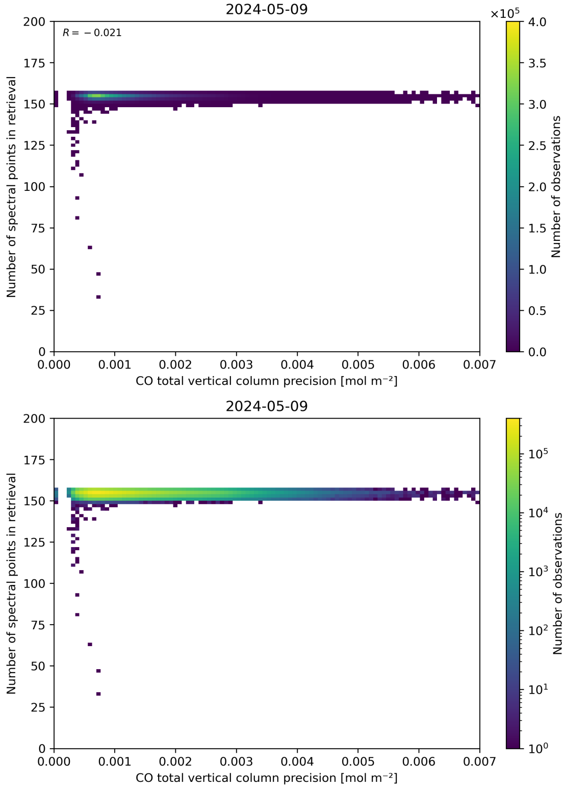
Figure 47: Scatter density plot of “CO total vertical column precision” against “Number of spectral points in retrieval” for 2024-05-08 to 2024-05-10.
