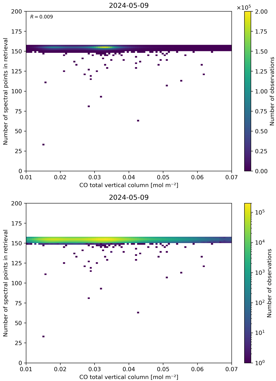
Figure 43: Scatter density plot of “CO total vertical column” against “Number of spectral points in retrieval” for 2024-05-08 to 2024-05-10.
