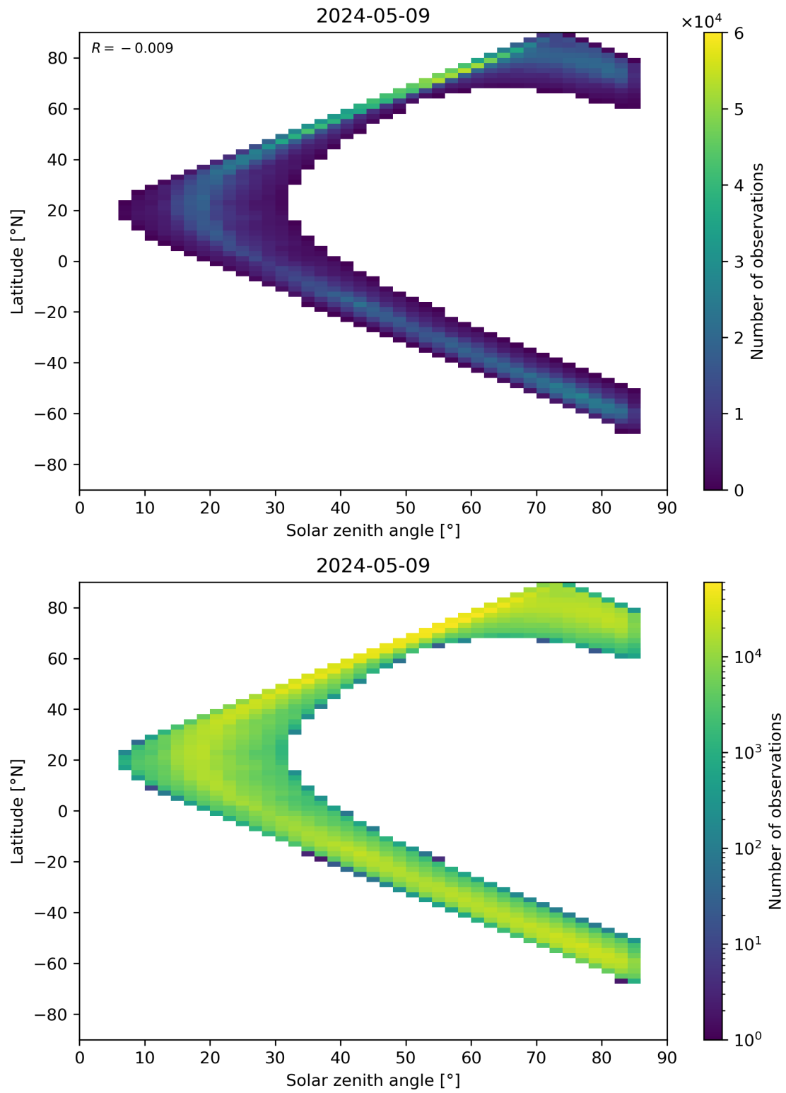
Figure 66: Scatter density plot of “Solar zenith angle” against “Latitude” for 2024-05-08 to 2024-05-10.
