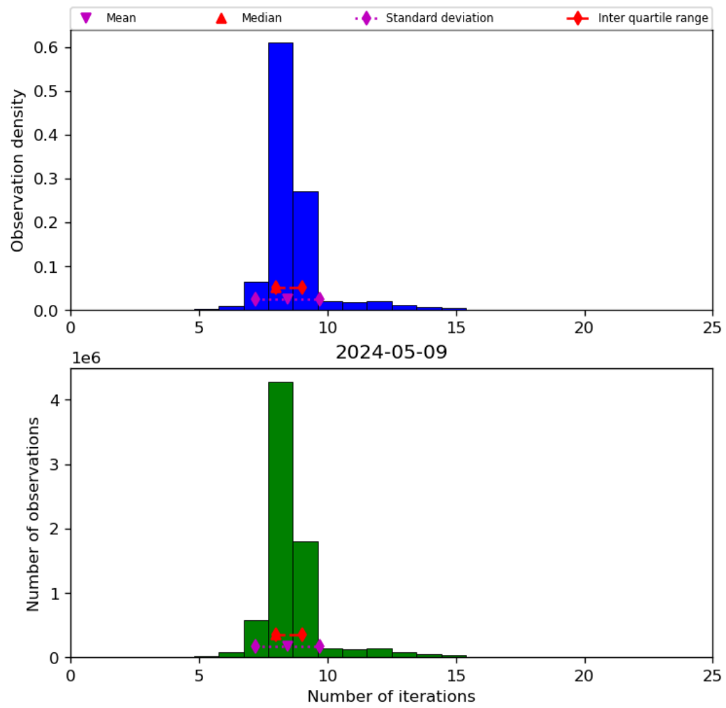
Figure 24: Histogram of “Number of iterations” for 2024-05-08 to 2024-05-10
