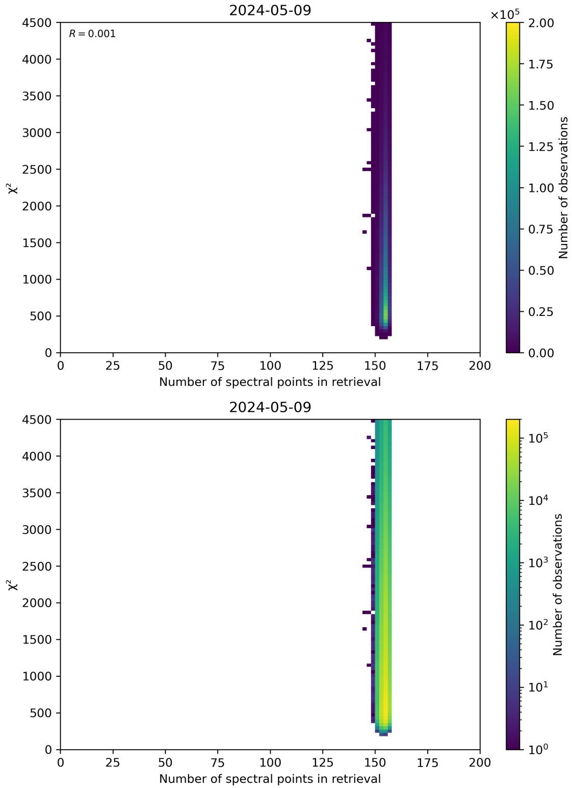
Figure 58: Scatter density plot of “Number of spectral points in retrieval” against “ \chi^2 ” for 2024-05-08 to 2024-05-10.
