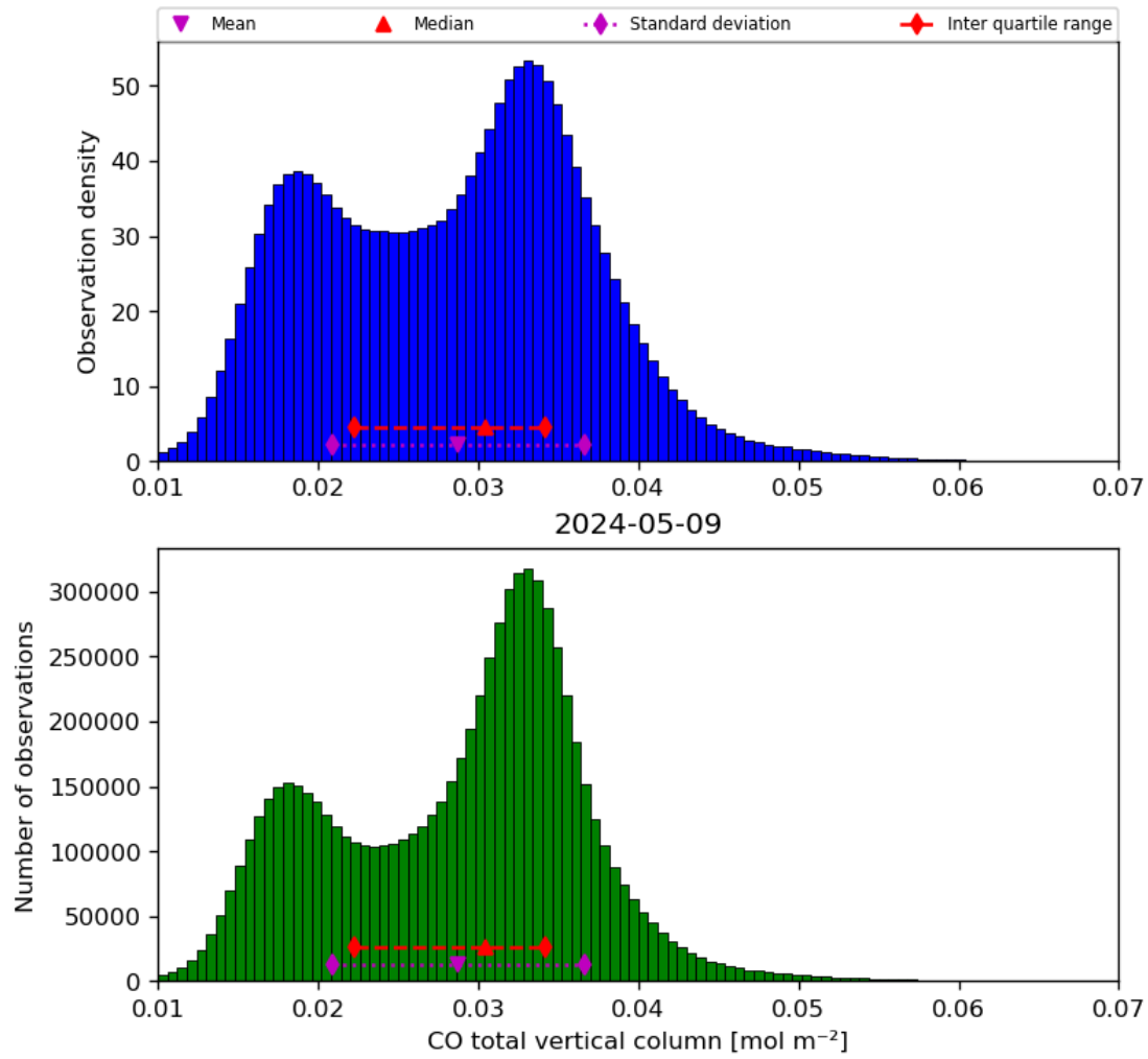
Figure 18: Histogram of “CO total vertical column” for 2024-05-08 to 2024-05-10
