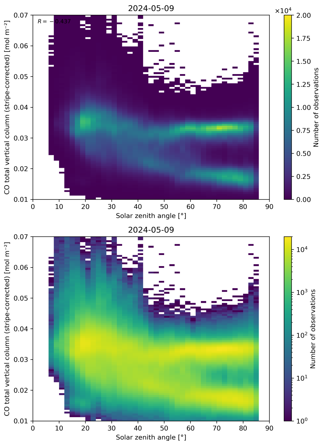
Figure 62: Scatter density plot of “Solar zenith angle” against “CO total vertical column (stripe-corrected)” for 2024-05-08 to 2024-05-10.
