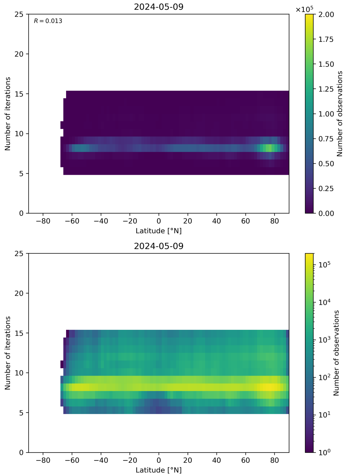
Figure 56: Scatter density plot of “Latitude” against “Number of iterations” for 2024-05-08 to 2024-05-10.
