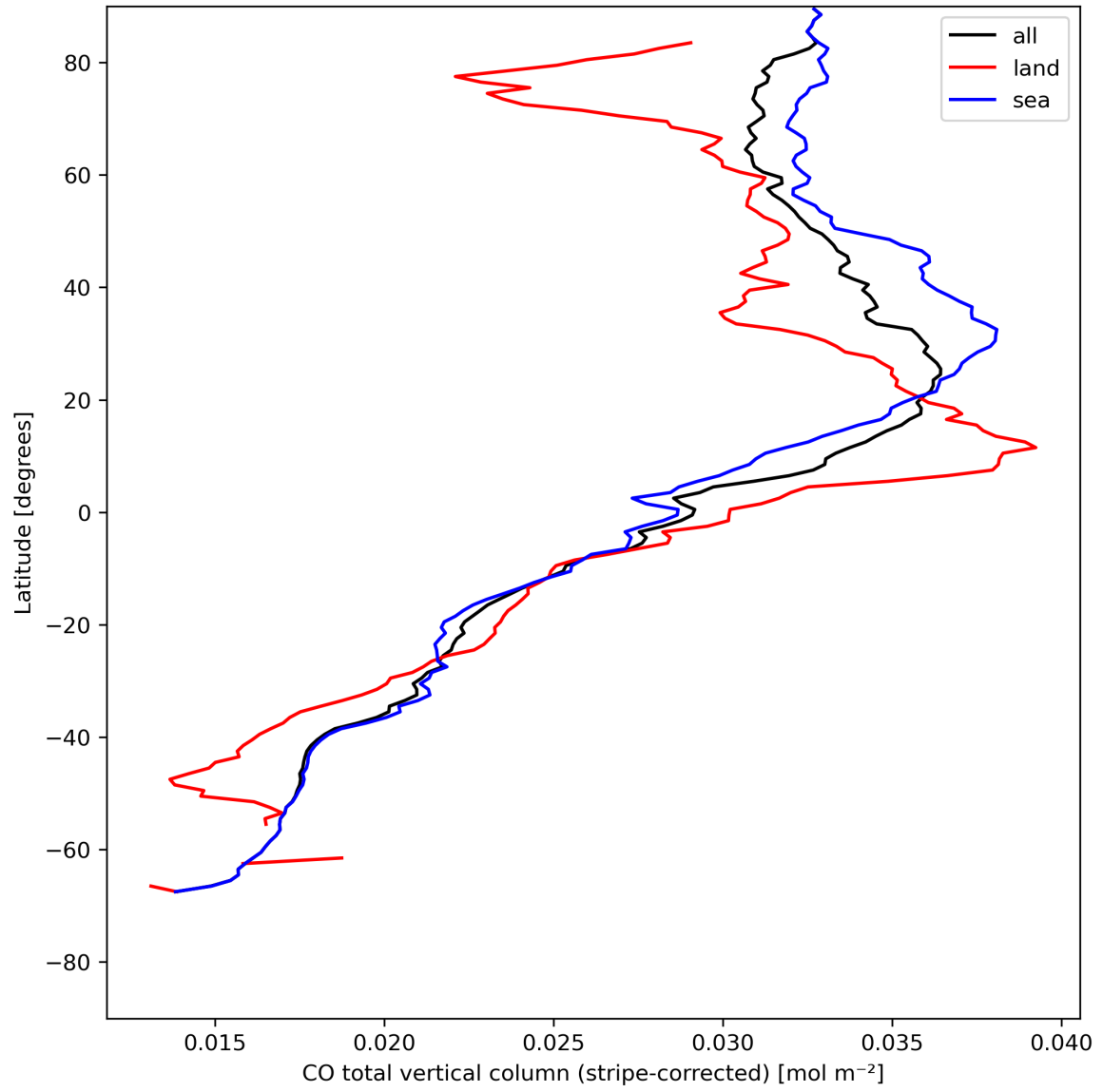
Figure 11: Zonal average of “CO total vertical column (stripe-corrected)” for 2024-05-08 to 2024-05-10.
