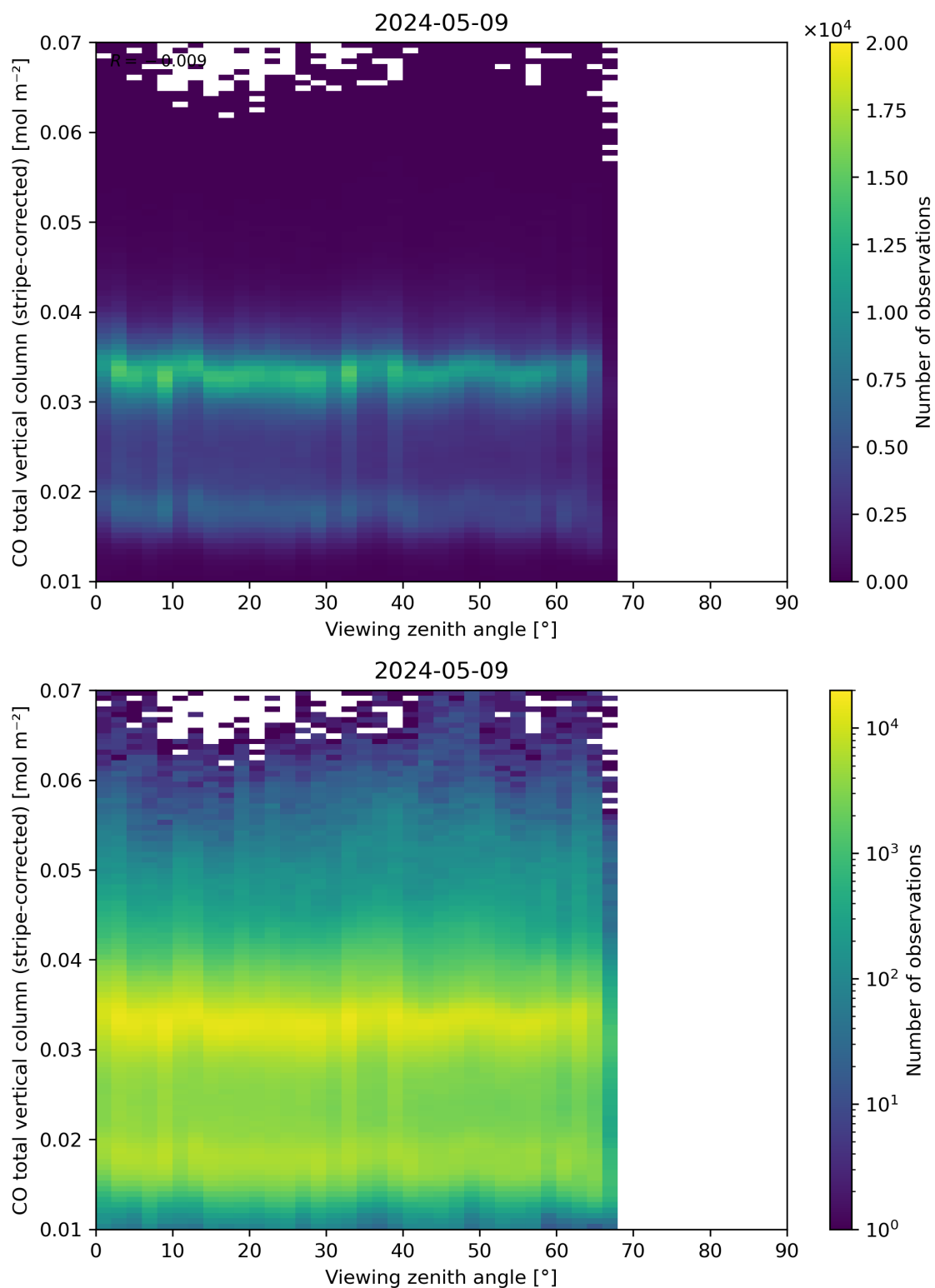
Figure 70: Scatter density plot of “Viewing zenith angle” against “CO total vertical column (stripe-corrected)” for 2024-05-08 to 2024-05-10.
