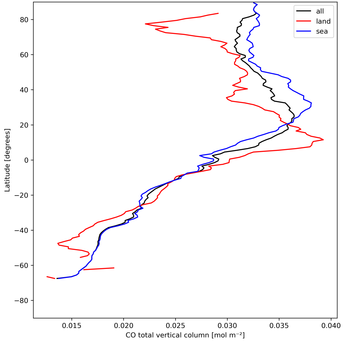
Figure 10: Zonal average of “CO total vertical column” for 2024-05-08 to 2024-05-10.
