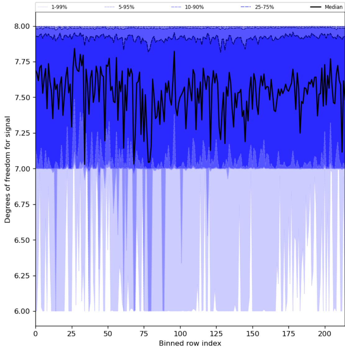
Figure 31: Along track statistics of “Degrees of freedom for signal” for 2024-05-08 to 2024-05-10
