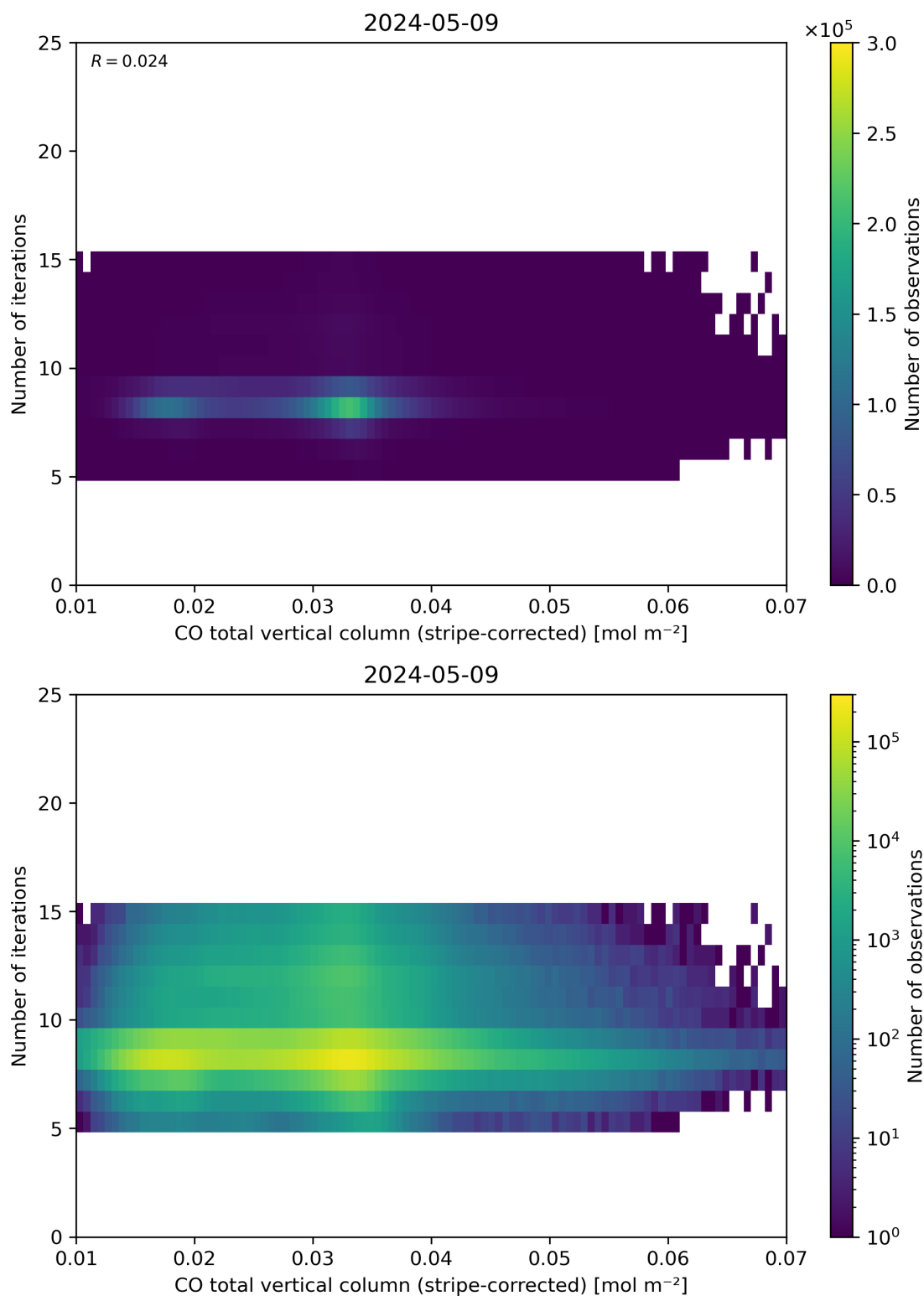
Figure 39: Scatter density plot of “CO total vertical column (stripe-corrected)” against “Number of iterations” for 2024-05-08 to 2024-05-10.
