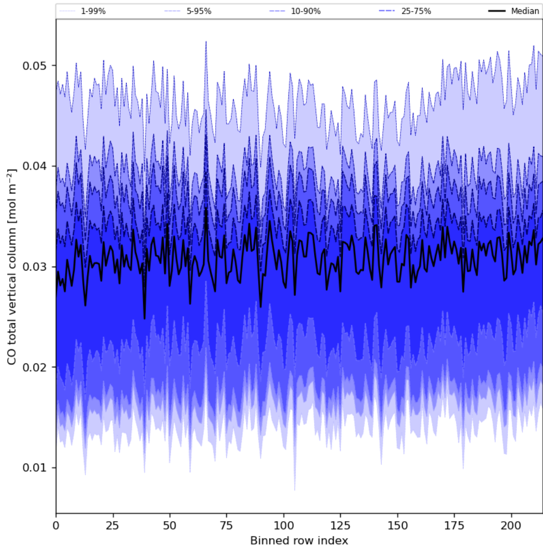
Figure 26: Along track statistics of “CO total vertical column” for 2024-05-08 to 2024-05-10
