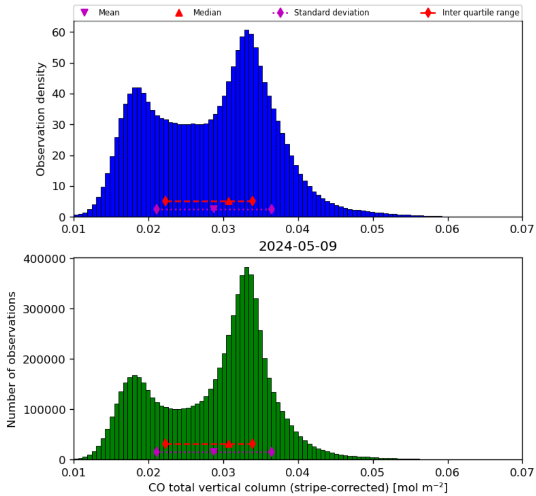
Figure 19: Histogram of “CO total vertical column (stripe-corrected)” for 2024-05-08 to 2024-05-10
