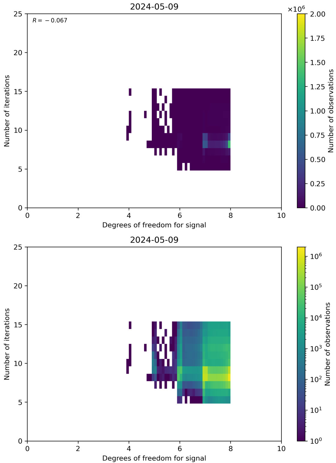
Figure 50: Scatter density plot of “Degrees of freedom for signal” against “Number of iterations” for 2024-05-08 to 2024-05-10.
