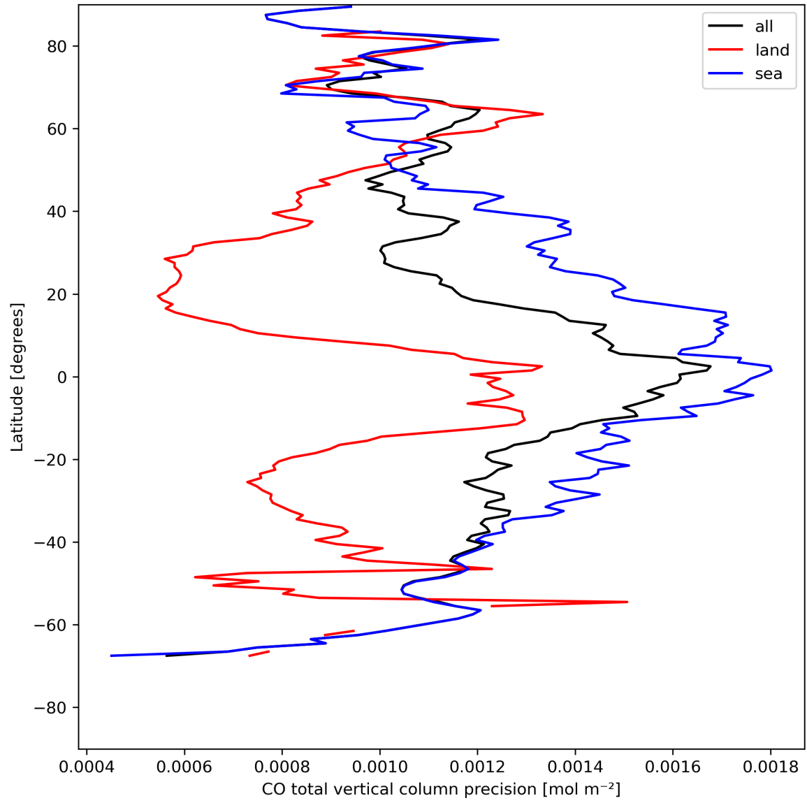
Figure 12: Zonal average of “CO total vertical column precision” for 2024-05-08 to 2024-05-10.
