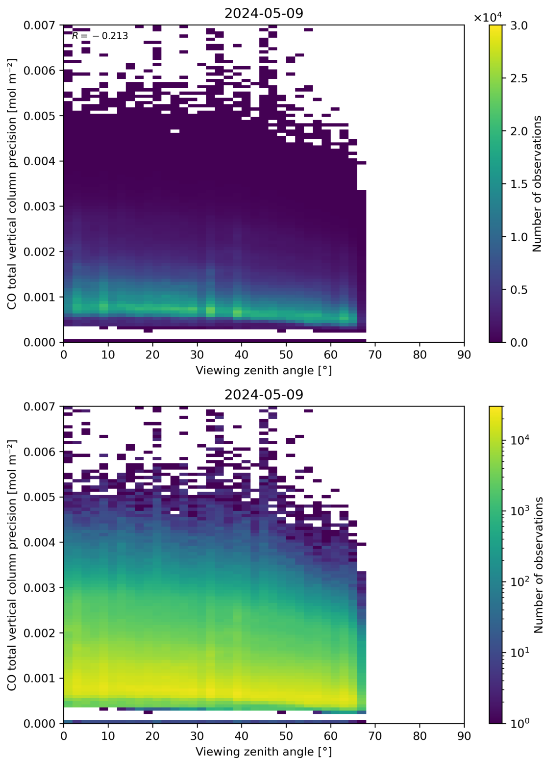
Figure 71: Scatter density plot of “Viewing zenith angle” against “CO total vertical column precision” for 2024-05-08 to 2024-05-10.
