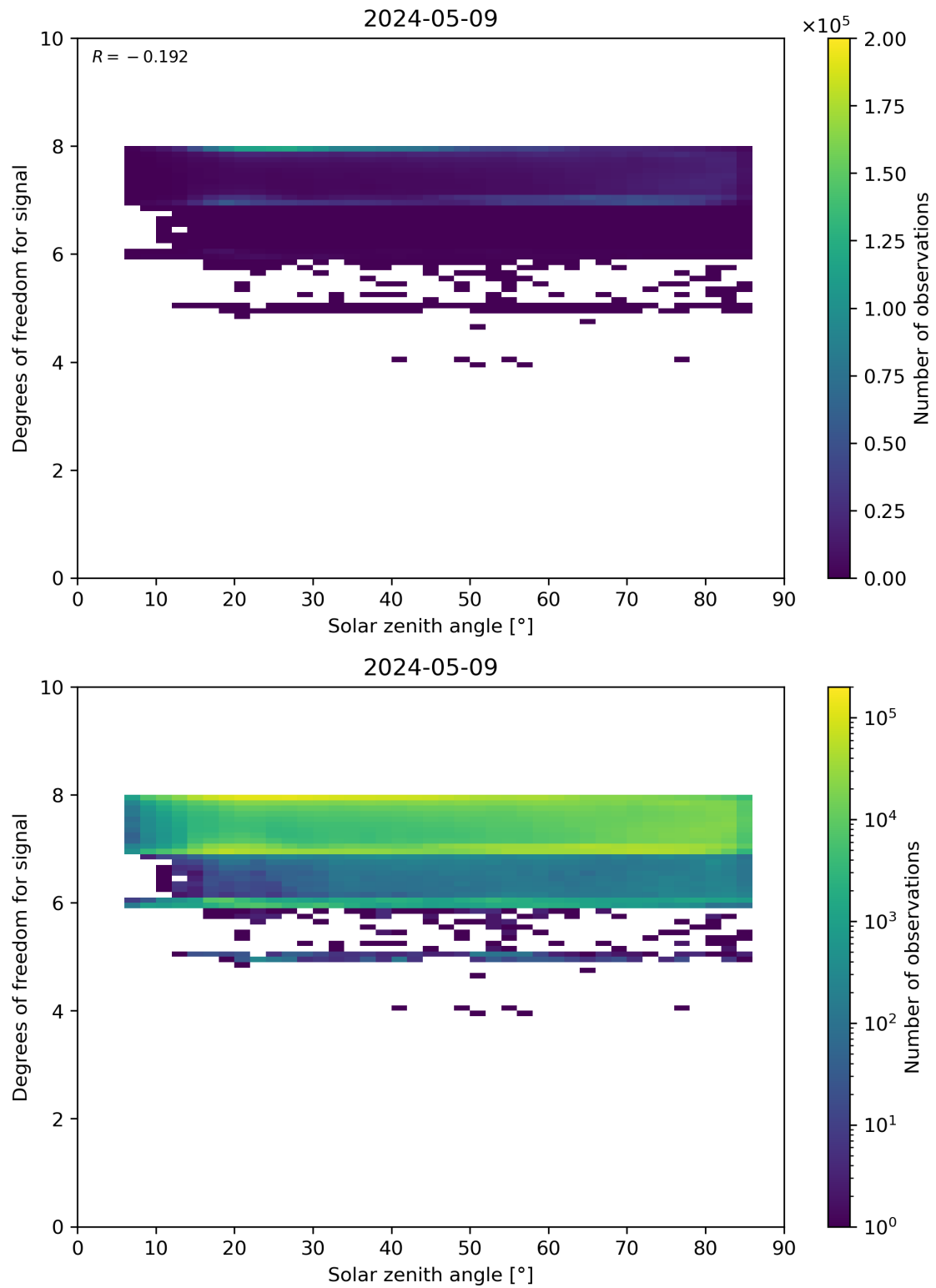
Figure 65: Scatter density plot of “Solar zenith angle” against “Degrees of freedom for signal” for 2024-05-08 to 2024-05-10.
