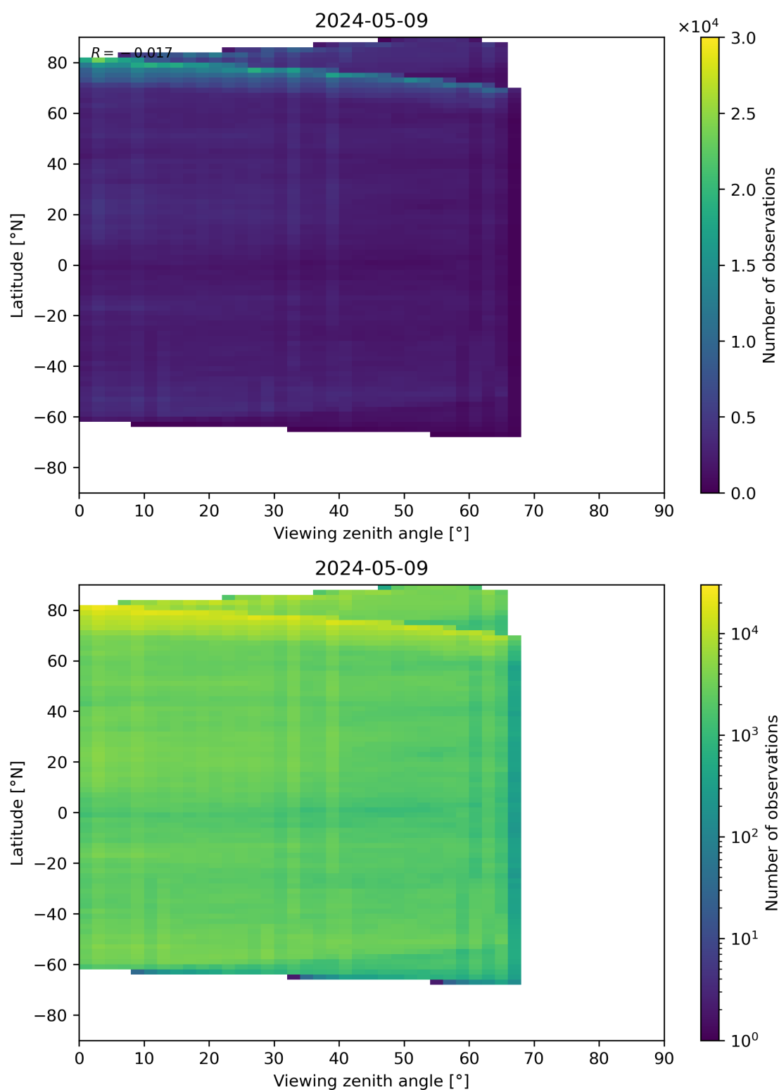
Figure 74: Scatter density plot of “Viewing zenith angle” against “Latitude” for 2024-05-08 to 2024-05-10.
