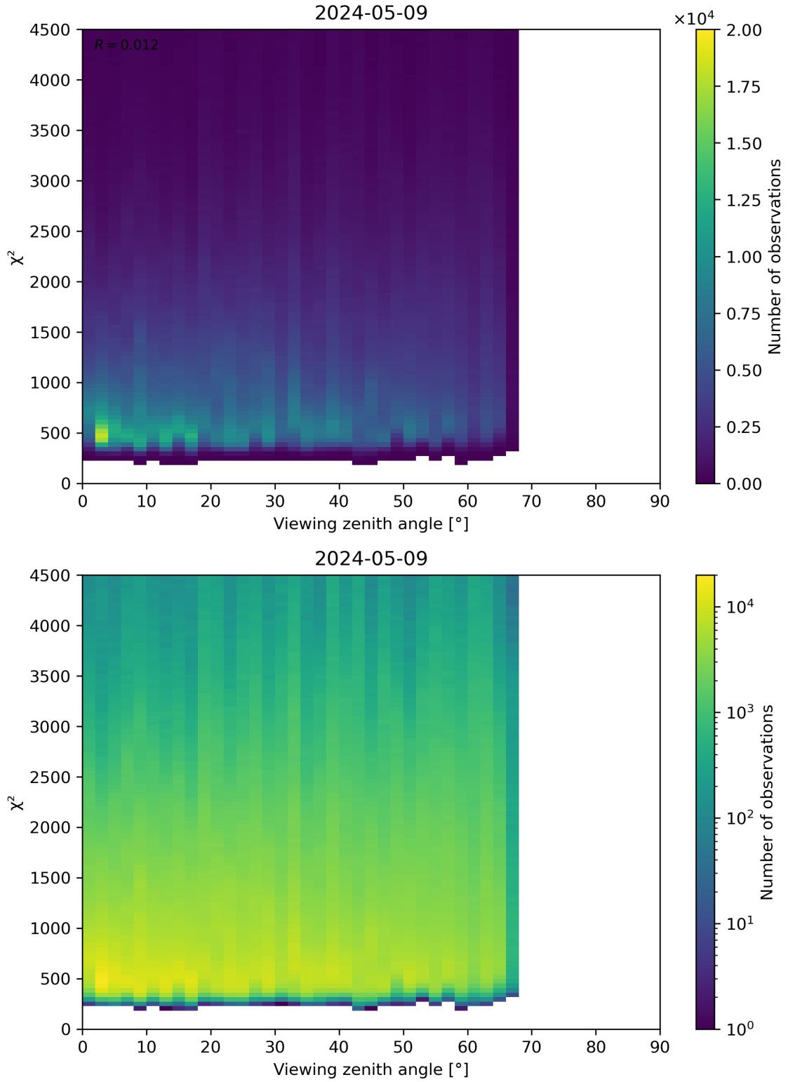
Figure 72: Scatter density plot of “Viewing zenith angle” against “ \chi^2 ” for 2024-05-08 to 2024-05-10.
