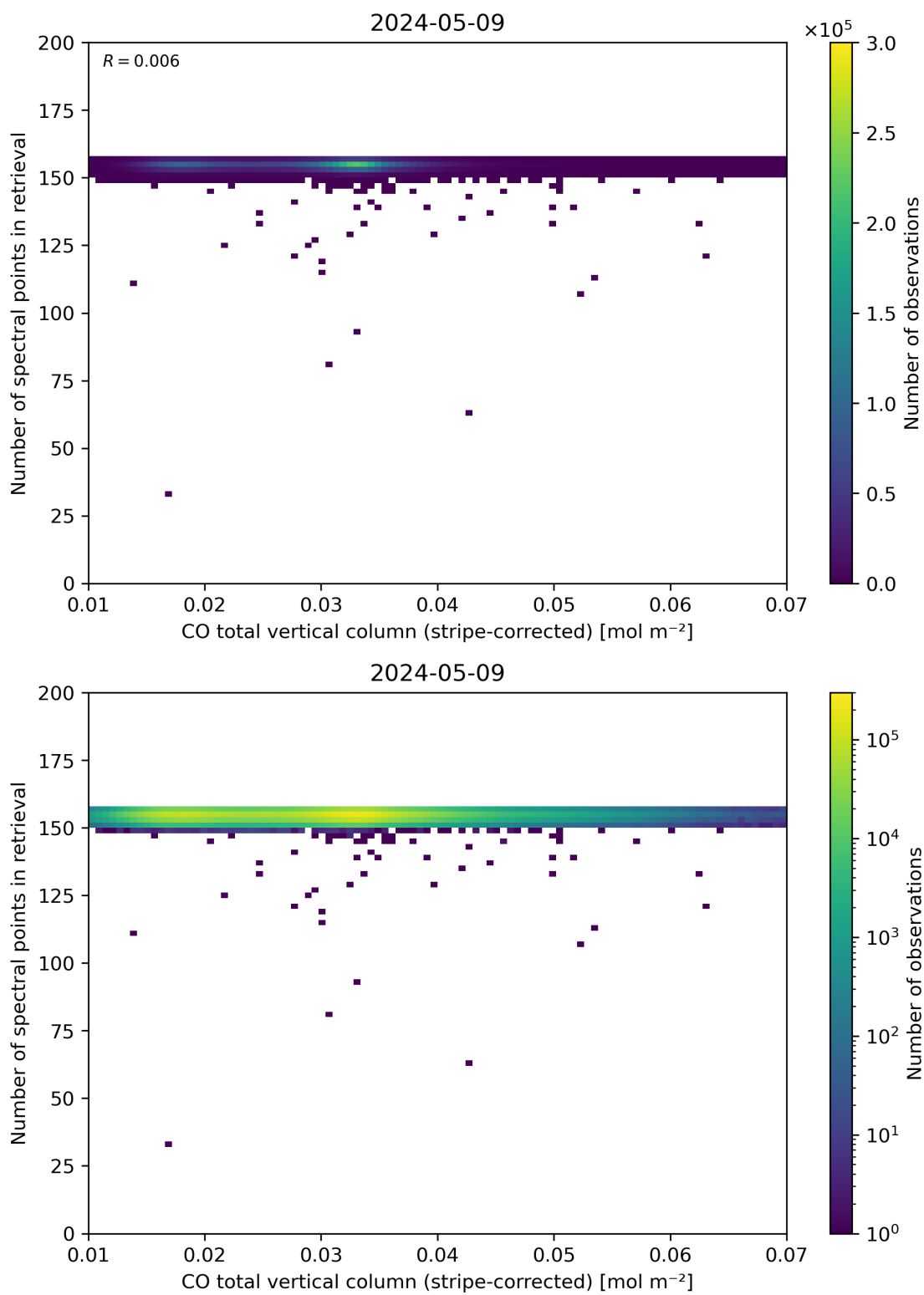
Figure 40: Scatter density plot of “CO total vertical column (stripe-corrected)” against “Number of spectral points in retrieval” for 2024-05-08 to 2024-05-10.
