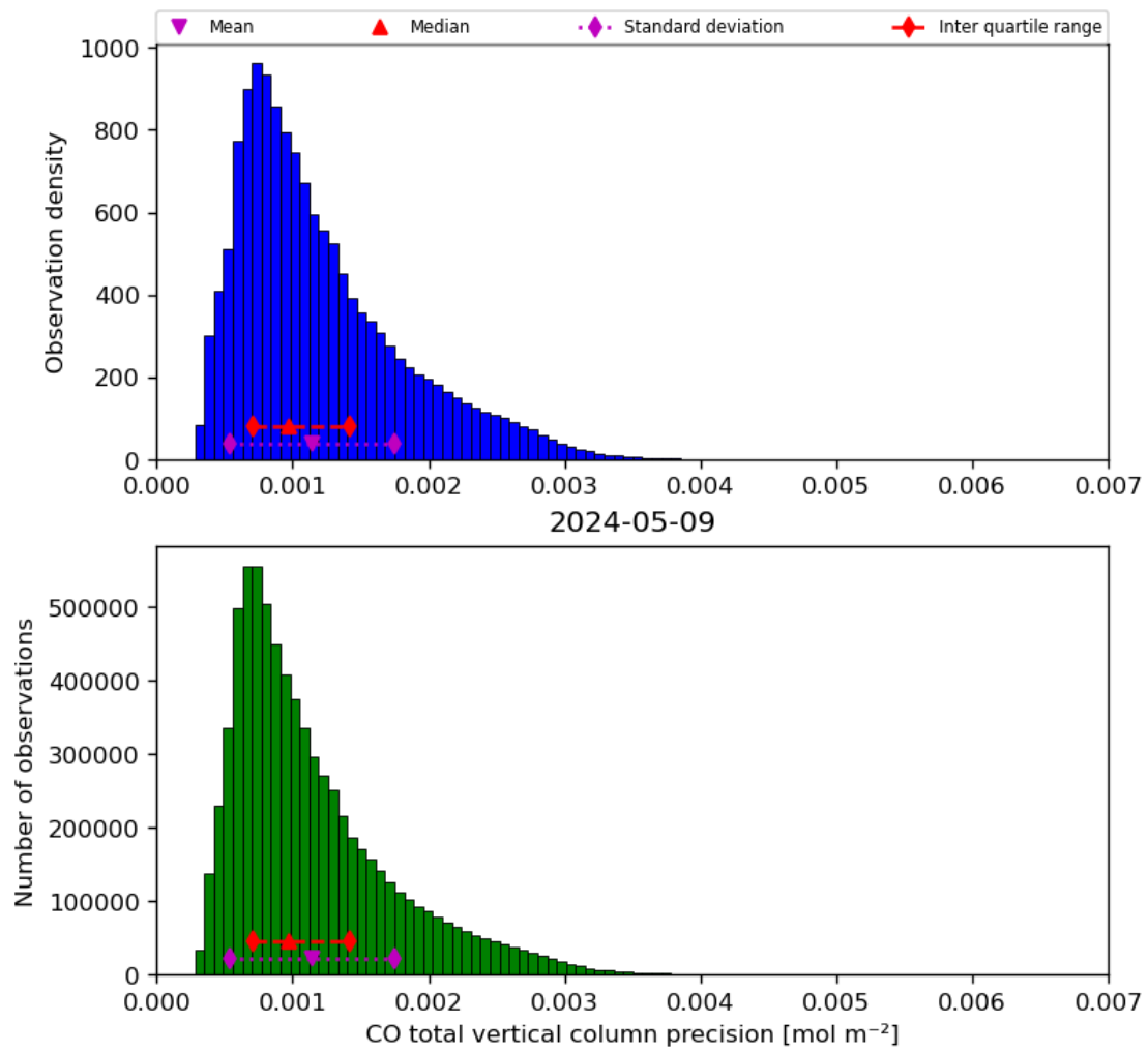
Figure 20: Histogram of “CO total vertical column precision” for 2024-05-08 to 2024-05-10
