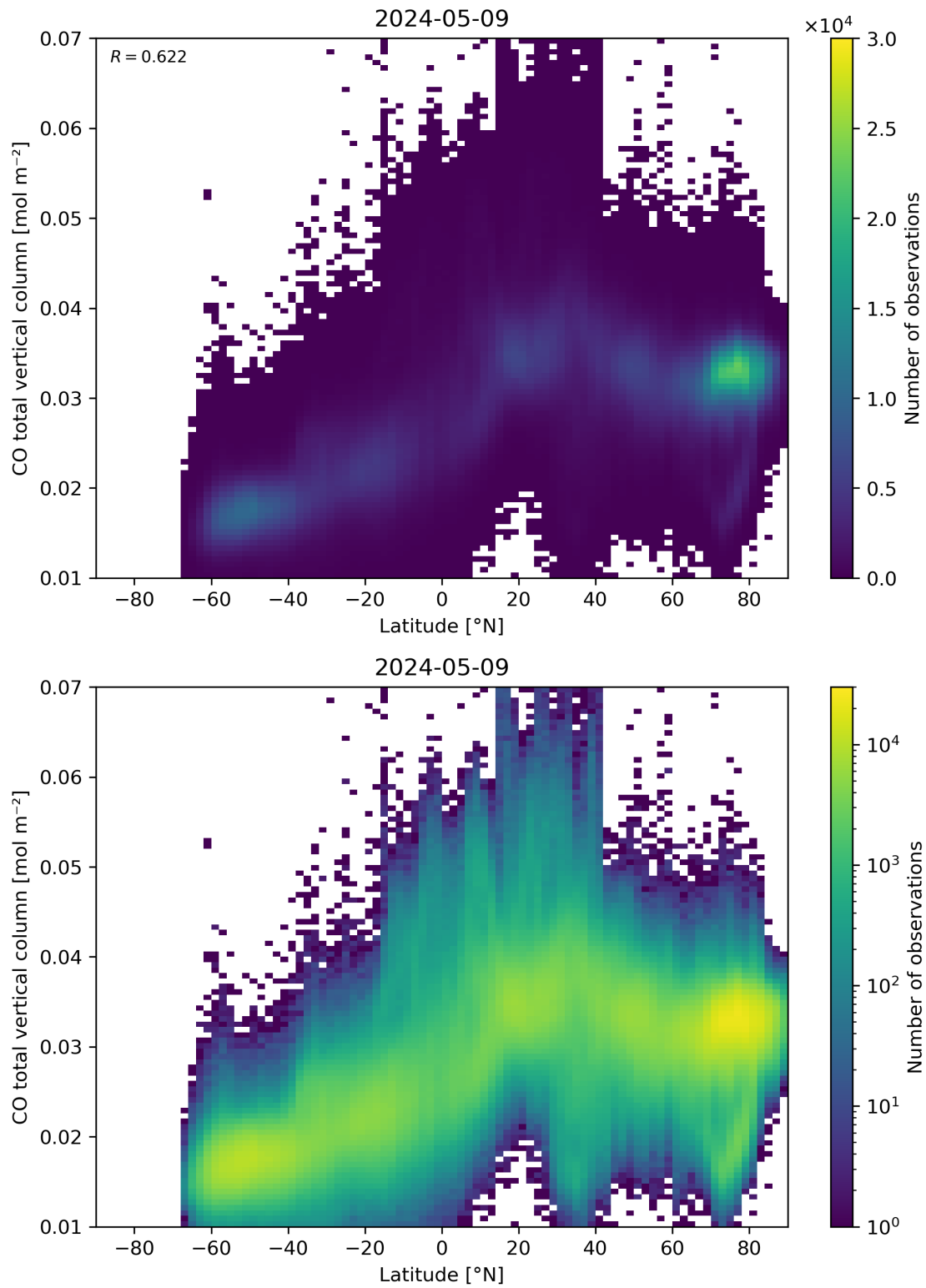
Figure 51: Scatter density plot of “Latitude” against “CO total vertical column” for 2024-05-08 to 2024-05-10.
