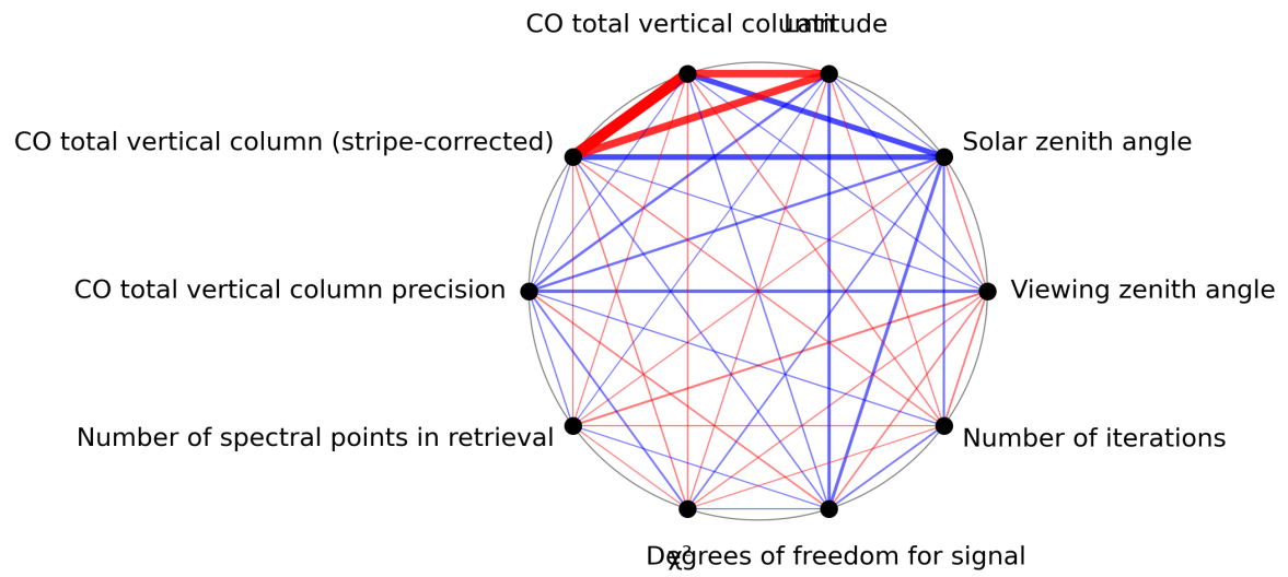
Figure 1: Map of correlation graph for 2024-05-08 to 2024-05-10.
