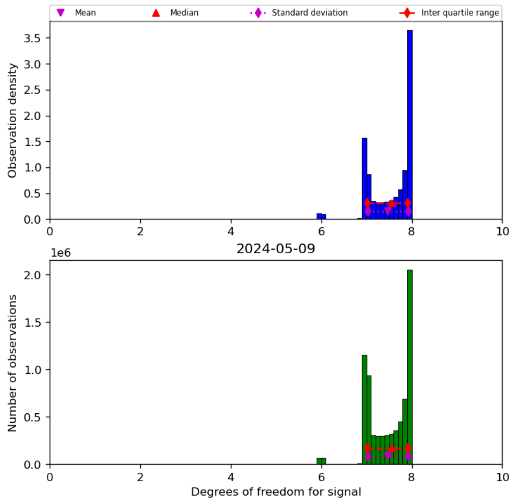
Figure 23: Histogram of “Degrees of freedom for signal” for 2024-05-08 to 2024-05-10
