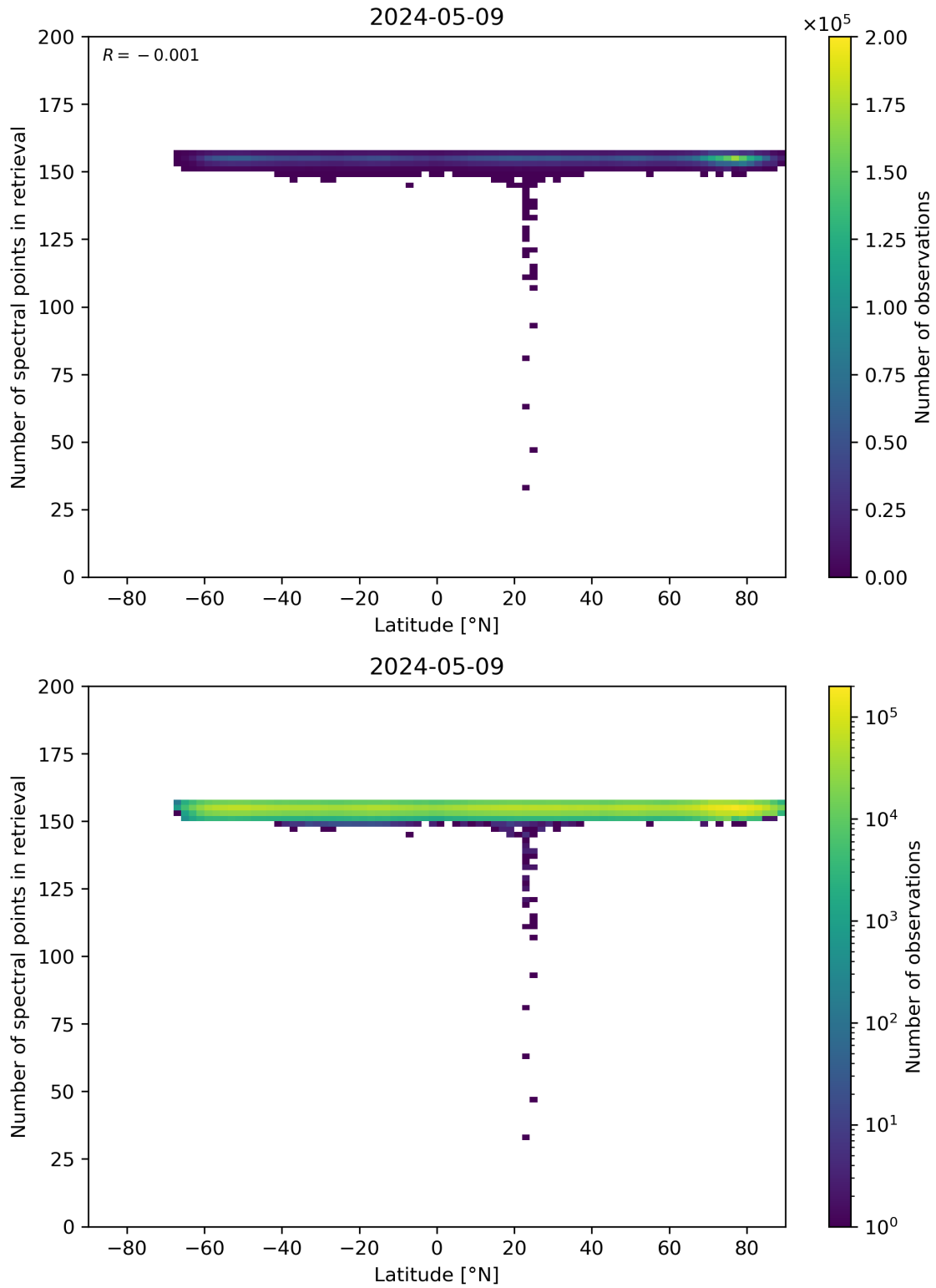
Figure 57: Scatter density plot of “Latitude” against “Number of spectral points in retrieval” for 2024-05-08 to 2024-05-10.
