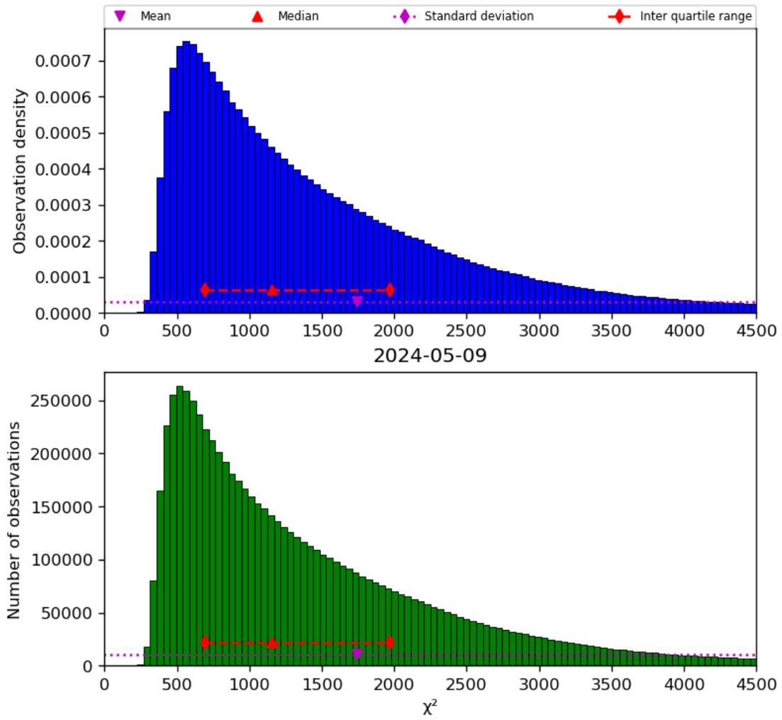
Figure 22: Histogram of “ \chi^2 ” for 2024-05-08 to 2024-05-10
