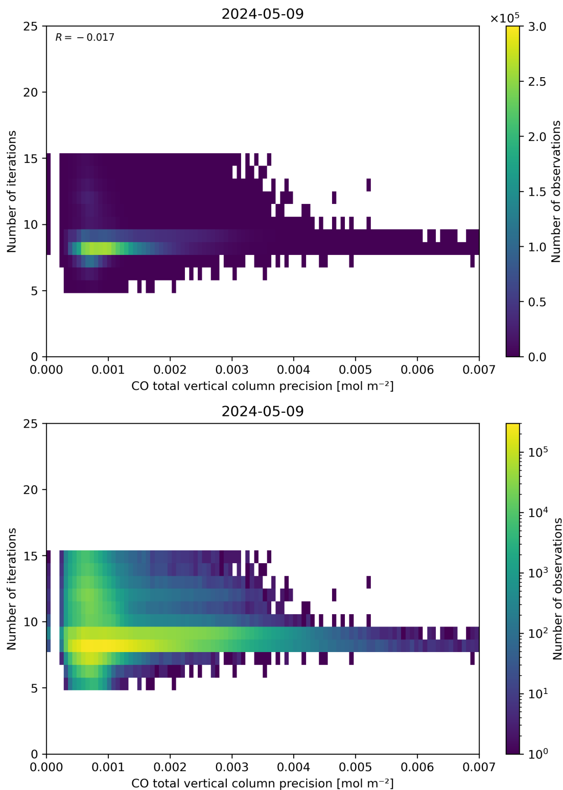
Figure 46: Scatter density plot of “CO total vertical column precision” against “Number of iterations” for 2024-05-08 to 2024-05-10.
