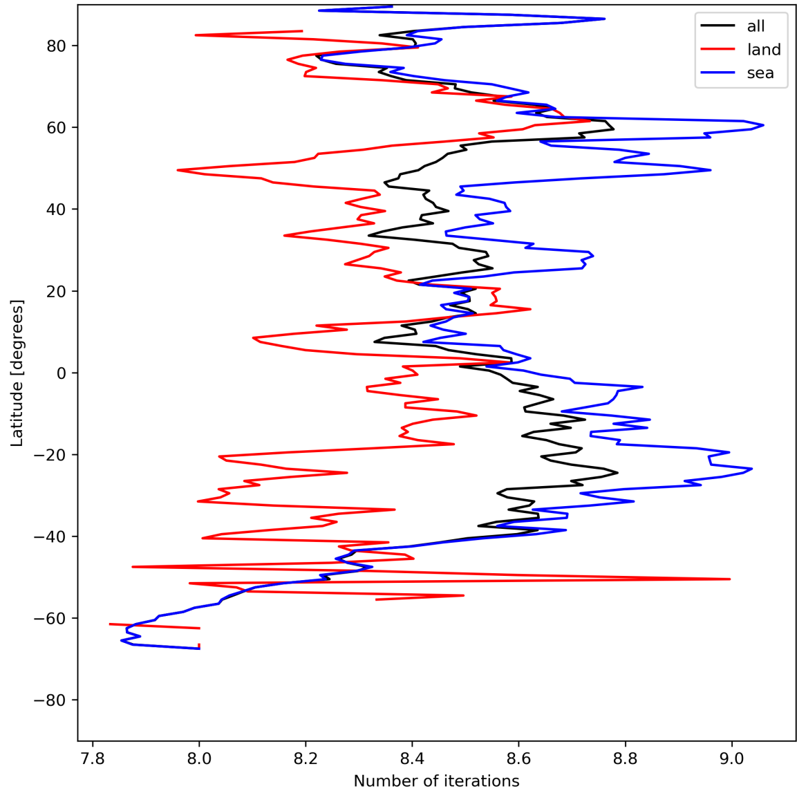
Figure 16: Zonal average of “Number of iterations” for 2024-05-08 to 2024-05-10.
