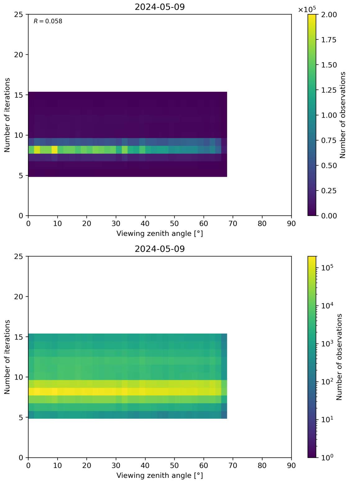
Figure 75: Scatter density plot of “Viewing zenith angle” against “Number of iterations” for 2024-05-08 to 2024-05-10.
