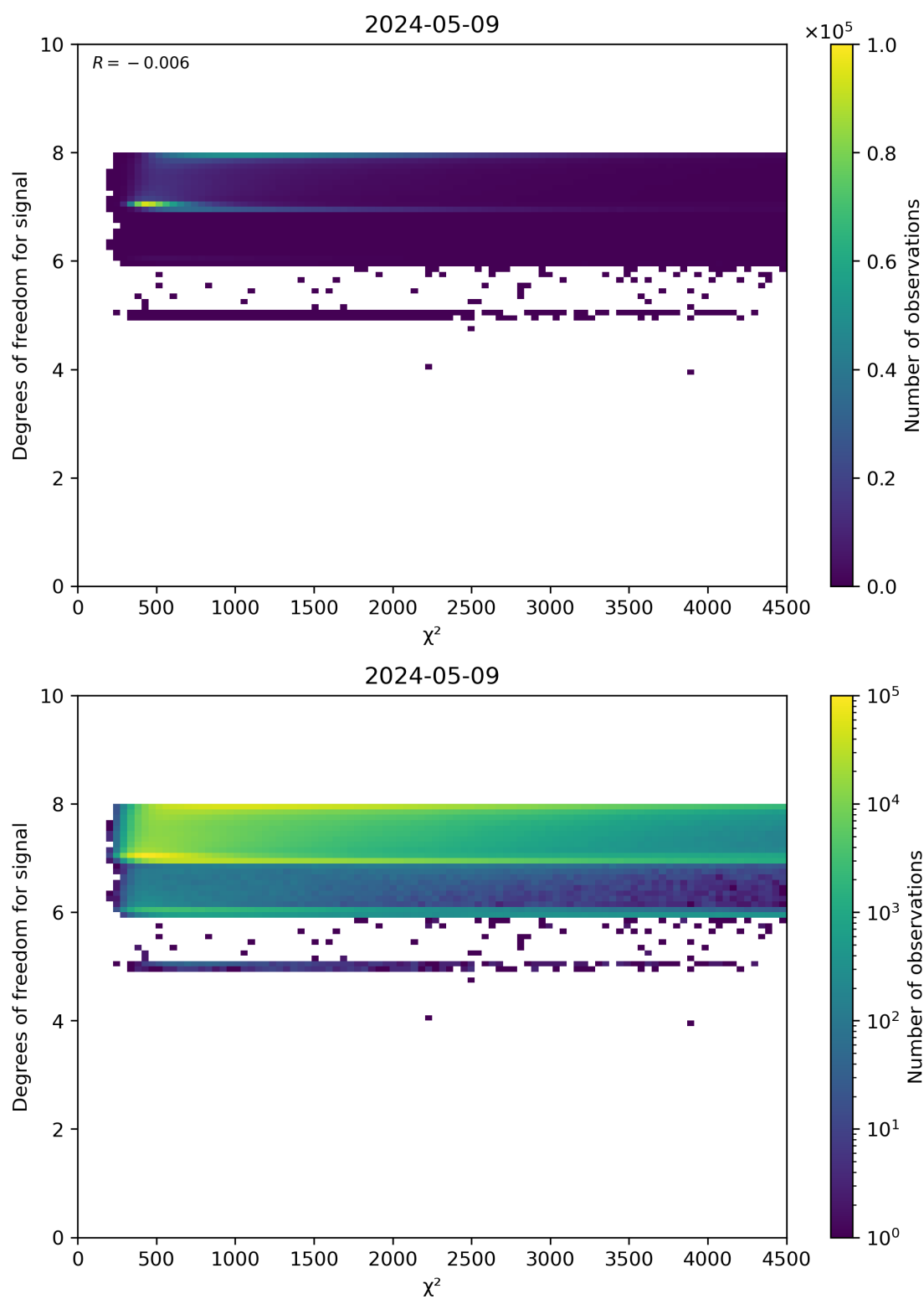
Figure 48: Scatter density plot of “ \chi^2 ” against “Degrees of freedom for signal” for 2024-05-08 to 2024-05-10.
