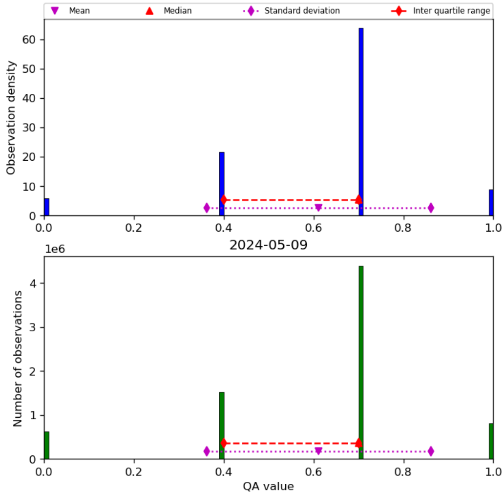
Figure 17: Histogram of “QA value” for 2024-05-08 to 2024-05-10
