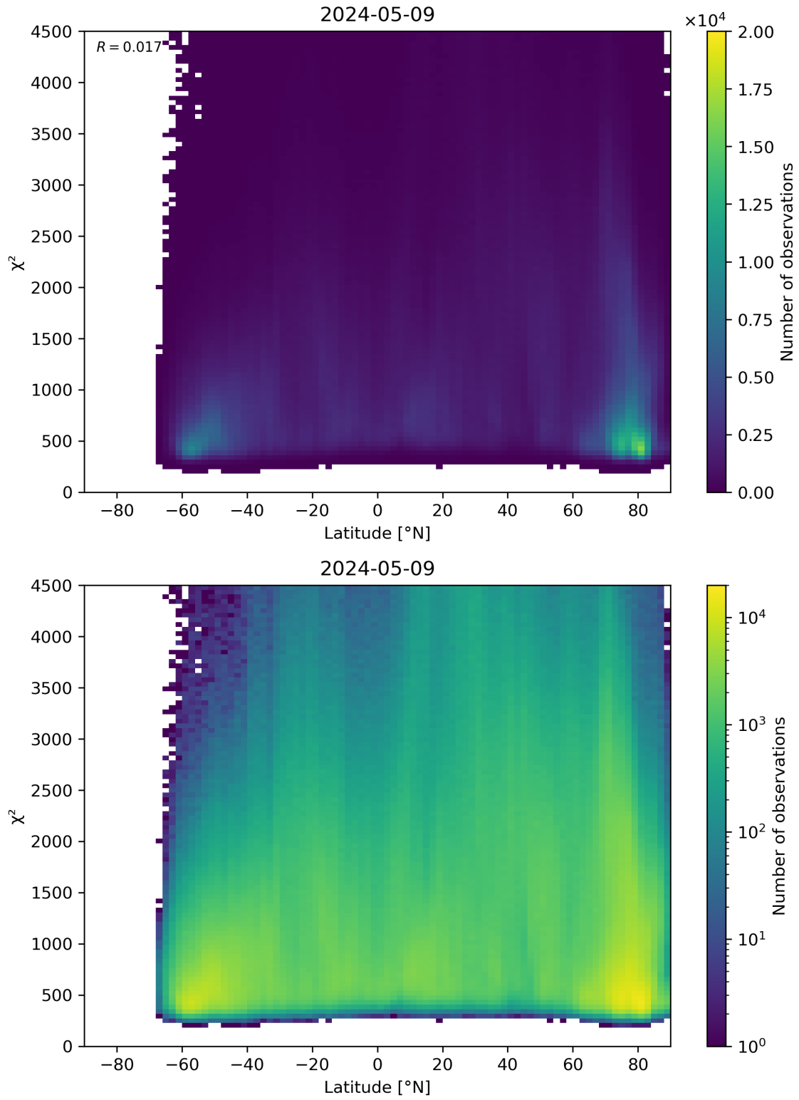
Figure 54: Scatter density plot of “Latitude” against “ \chi^2 ” for 2024-05-08 to 2024-05-10.
