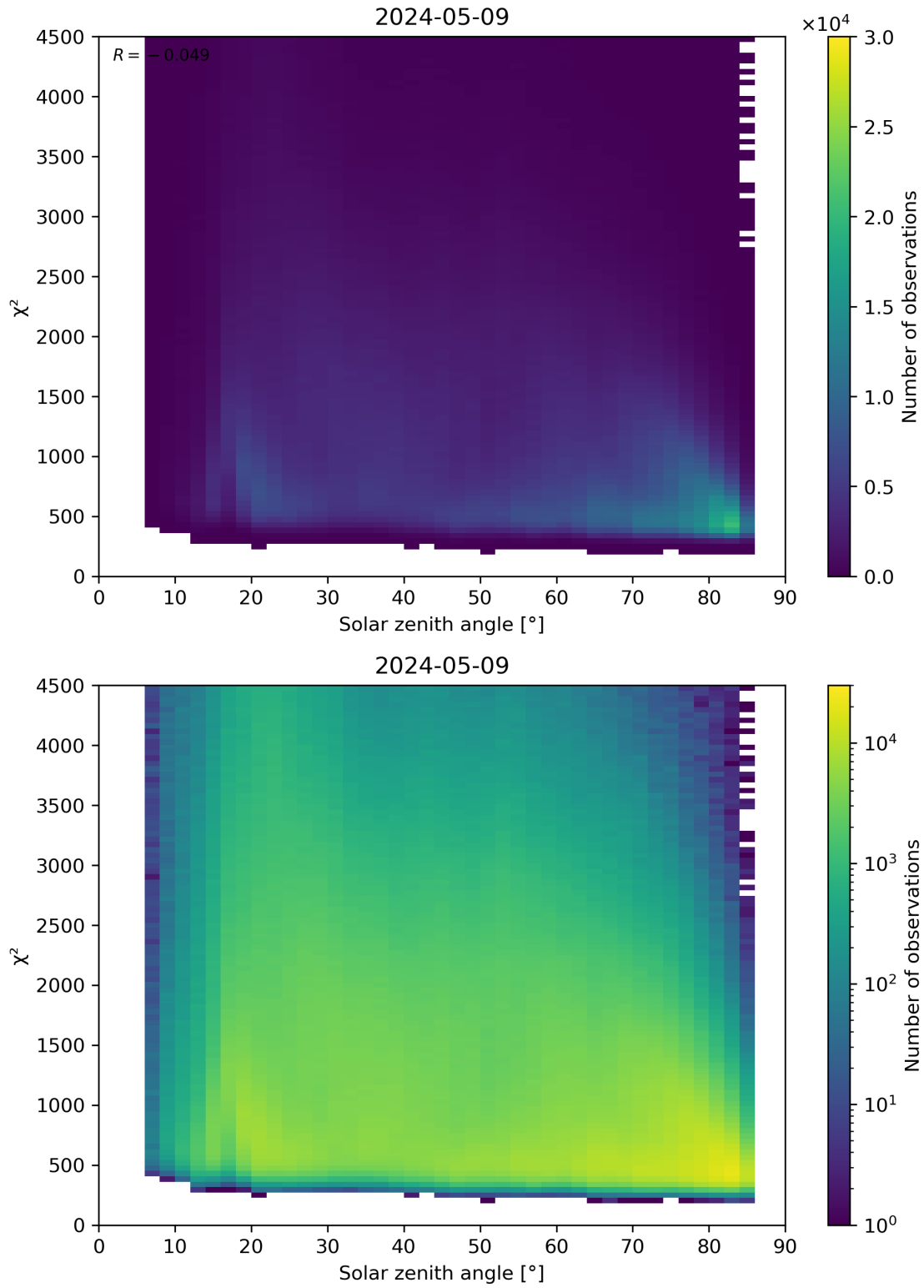
Figure 64: Scatter density plot of “Solar zenith angle” against “ \chi^2 ” for 2024-05-08 to 2024-05-10.
