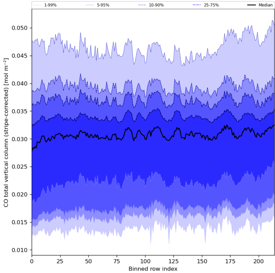
Figure 27: Along track statistics of “CO total vertical column (stripe-corrected)” for 2024-05-08 to 2024-05-10
