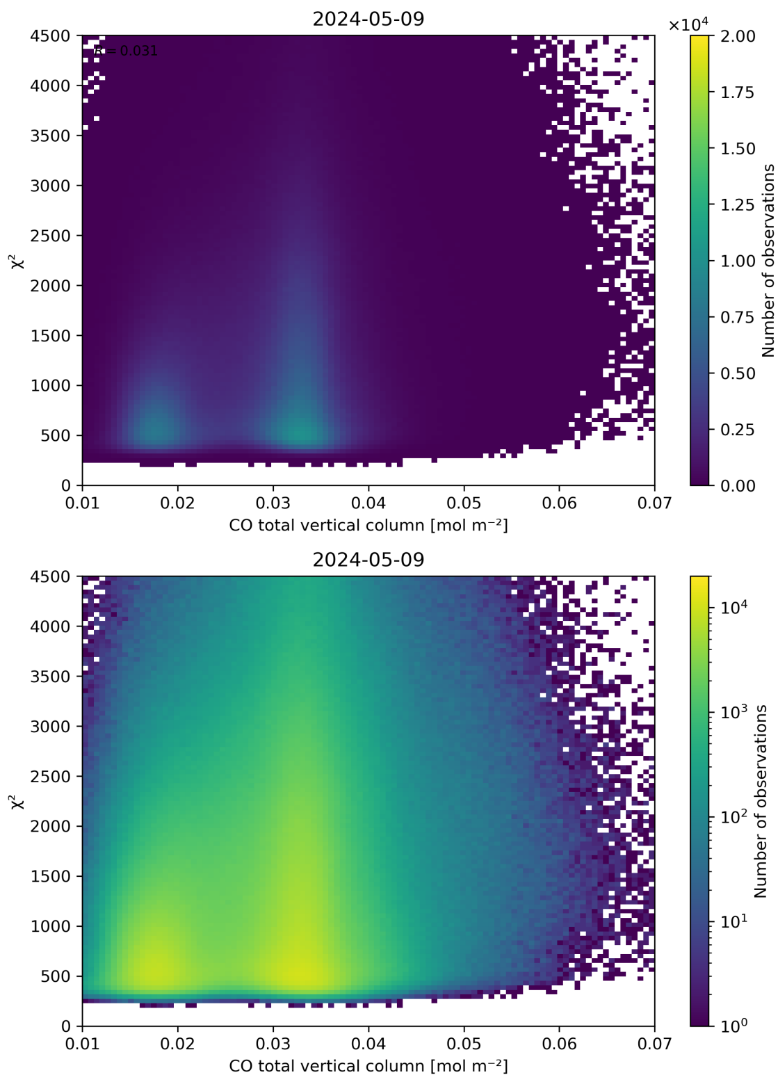
Figure 35: Scatter density plot of “CO total vertical column” against “ \chi^2 ” for 2024-05-08 to 2024-05-10.
