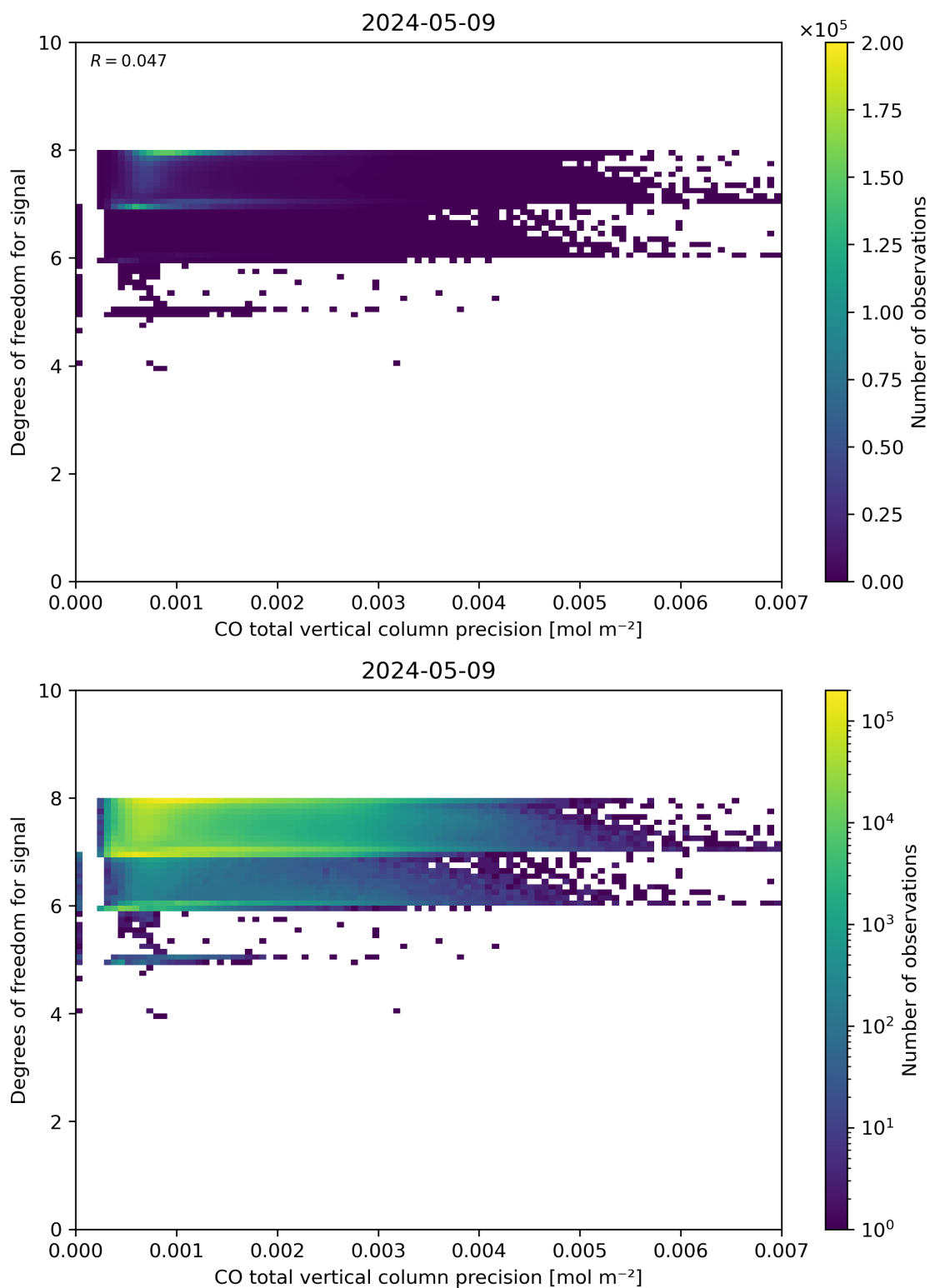
Figure 45: Scatter density plot of “CO total vertical column precision” against “Degrees of freedom for signal” for 2024-05-08 to 2024-05-10.
