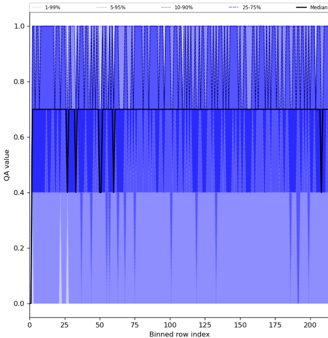
Figure 25: Along track statistics of “QA value” for 2024-05-08 to 2024-05-10
