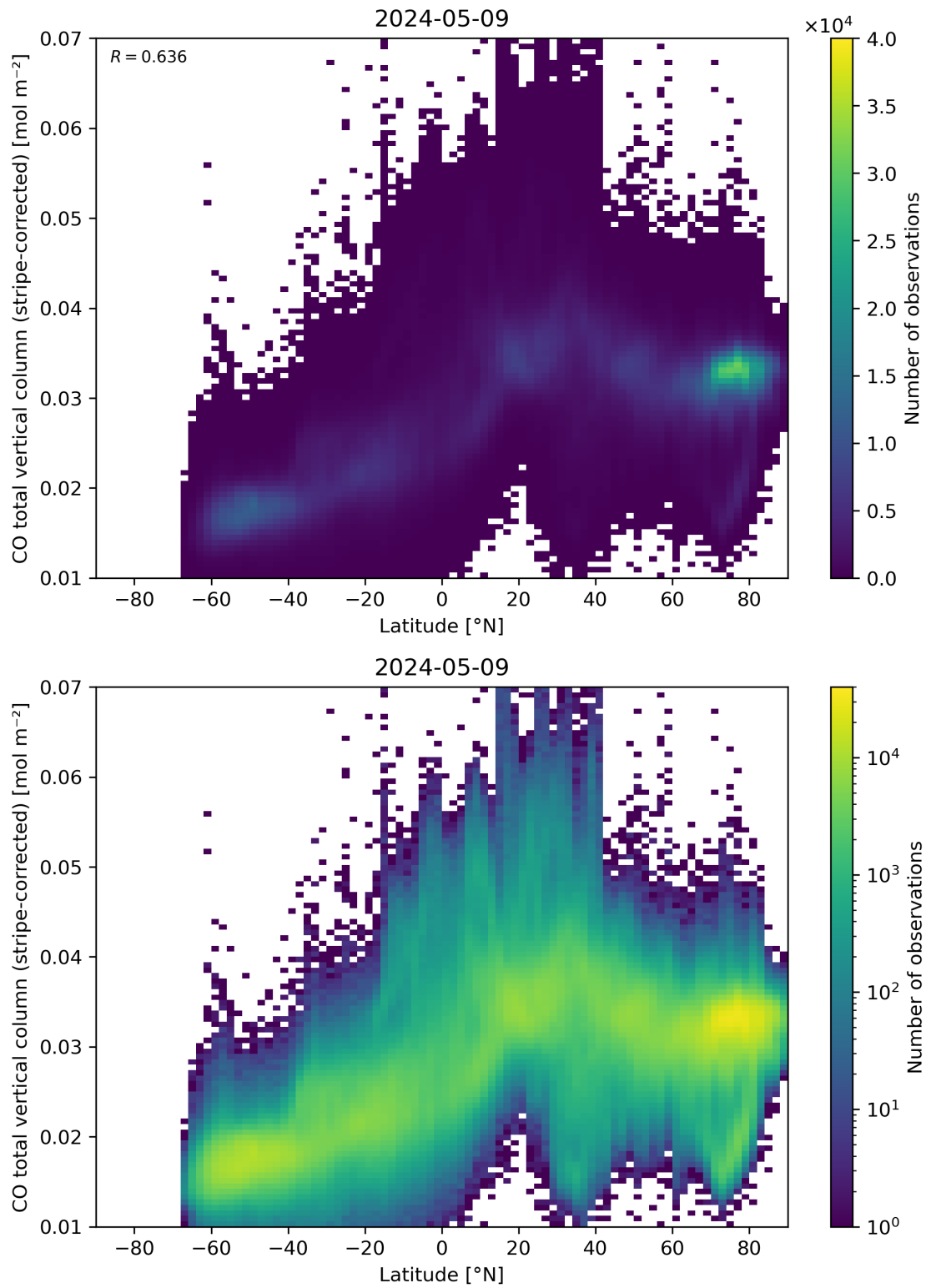
Figure 52: Scatter density plot of “Latitude” against “CO total vertical column (stripe-corrected)” for 2024-05-08 to 2024-05-10.
