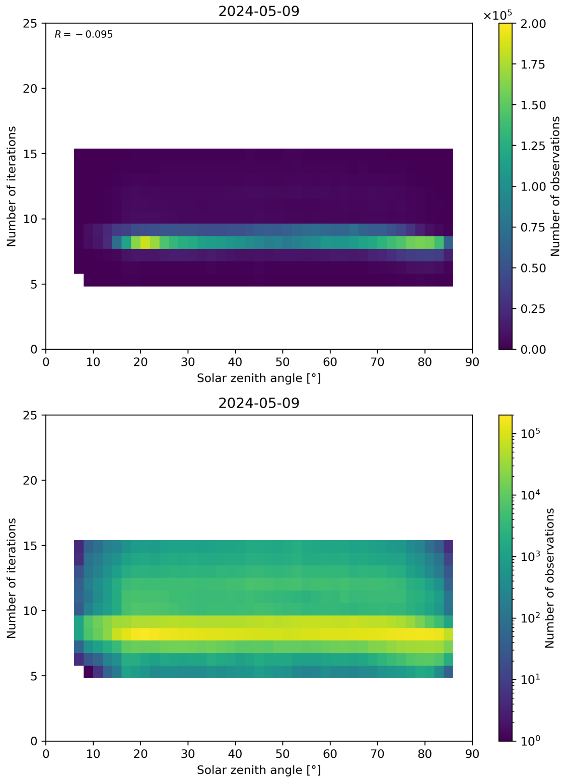
Figure 67: Scatter density plot of “Solar zenith angle” against “Number of iterations” for 2024-05-08 to 2024-05-10.
