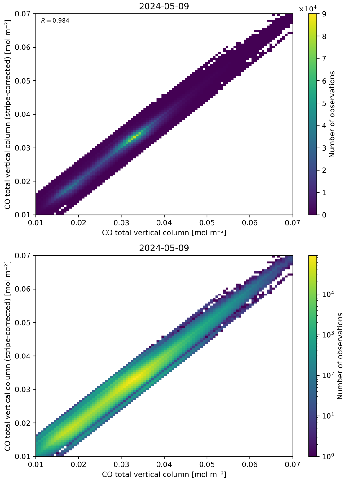
Figure 33: Scatter density plot of “CO total vertical column” against “CO total vertical column (stripe-corrected)” for 2024-05-08 to 2024-05-10.
