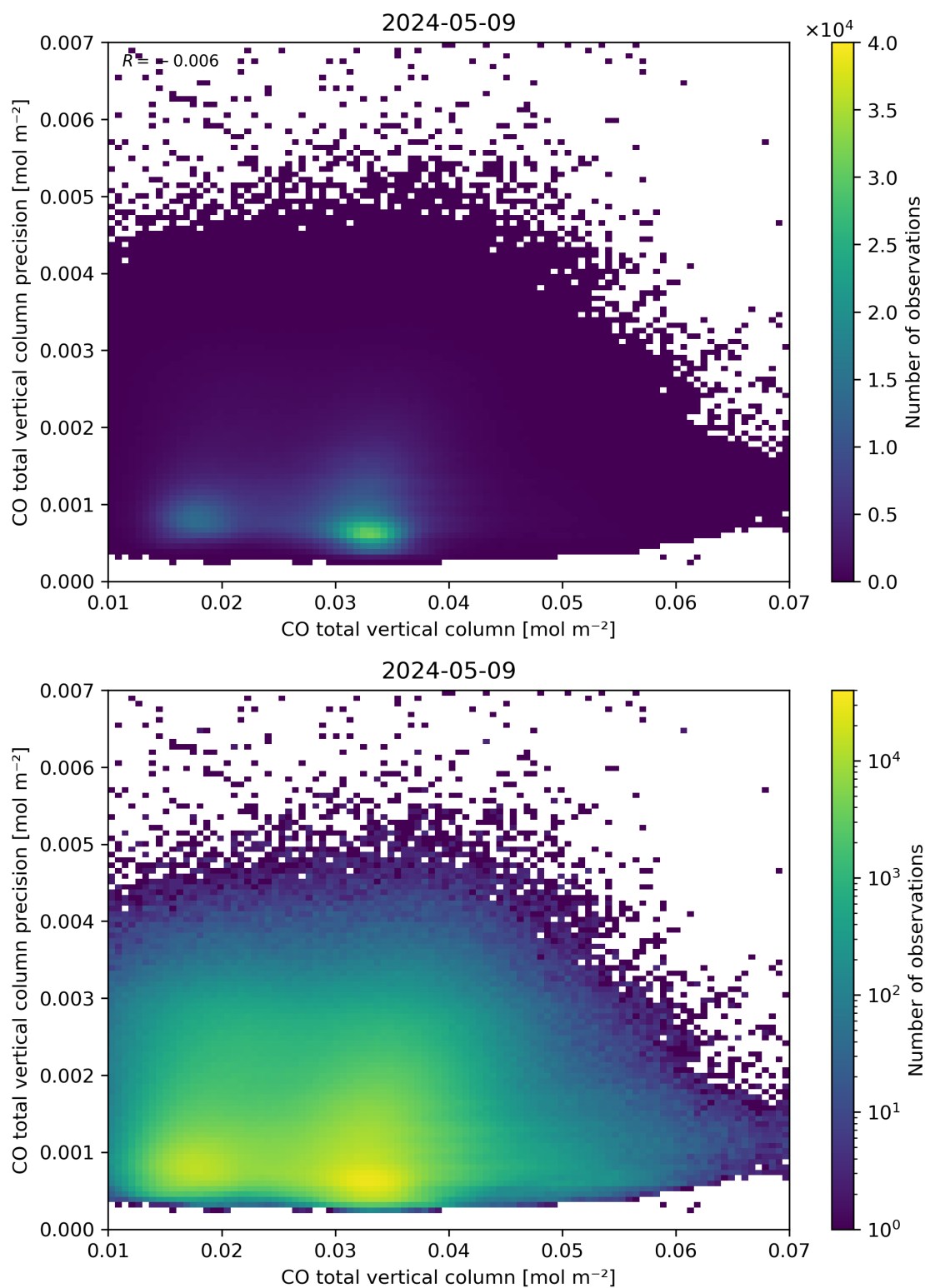
Figure 34: Scatter density plot of “CO total vertical column” against “CO total vertical column precision” for 2024-05-08 to 2024-05-10.
