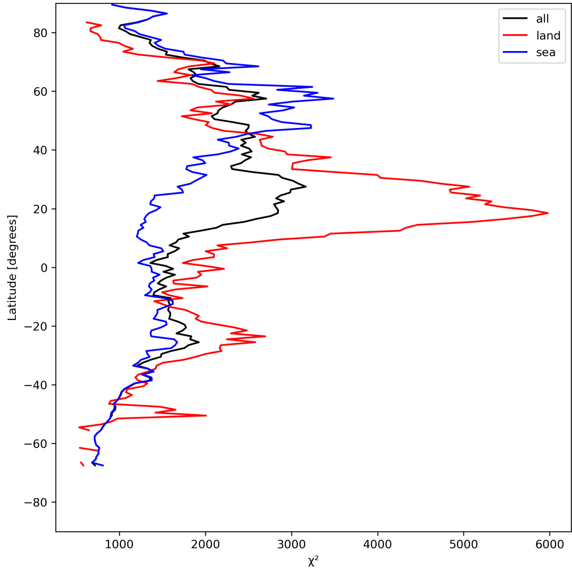
Figure 14: Zonal average of “ \chi^2 ” for 2024-05-08 to 2024-05-10.
