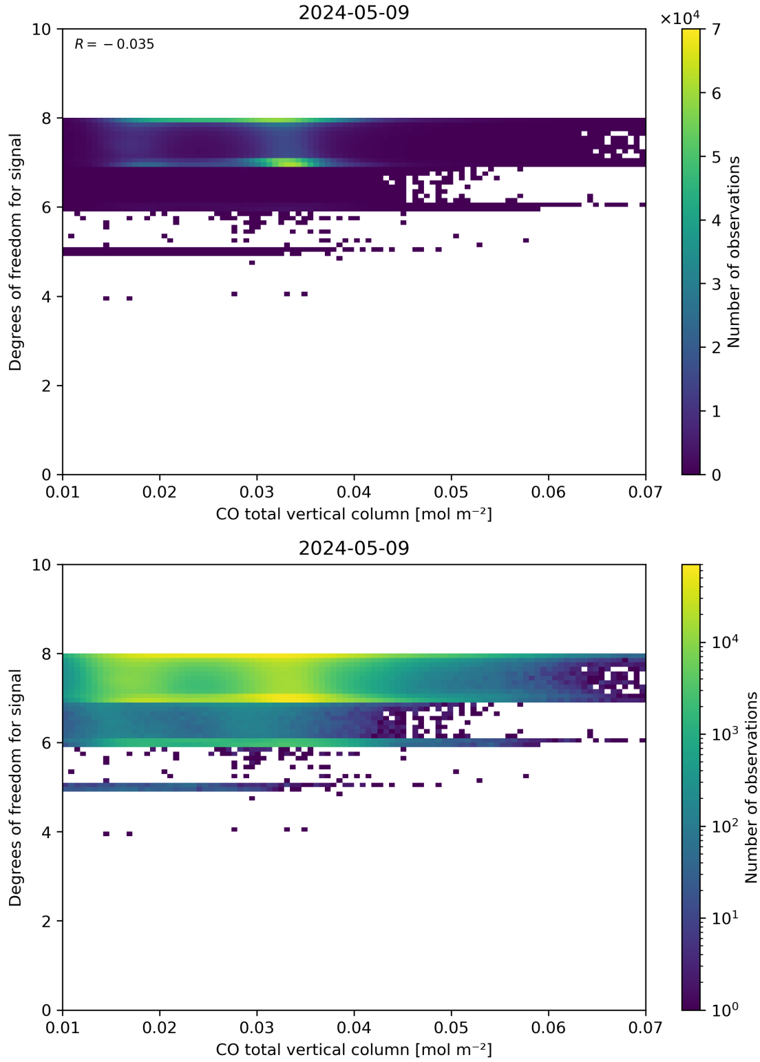
Figure 41: Scatter density plot of “CO total vertical column” against “Degrees of freedom for signal” for 2024-05-08 to 2024-05-10.
