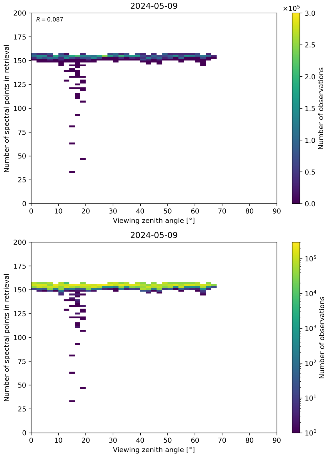
Figure 76: Scatter density plot of “Viewing zenith angle” against “Number of spectral points in retrieval” for 2024-05-08 to 2024-05-10.
