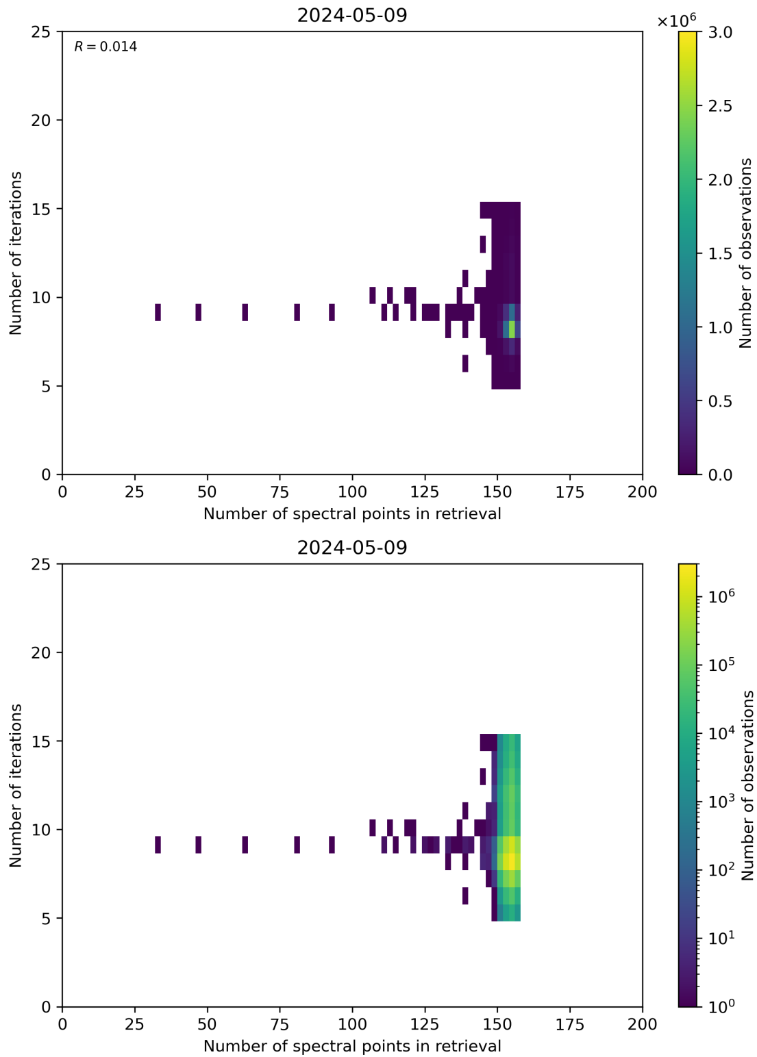
Figure 60: Scatter density plot of “Number of spectral points in retrieval” against “Number of iterations” for 2024-05-08 to 2024-05-10.
