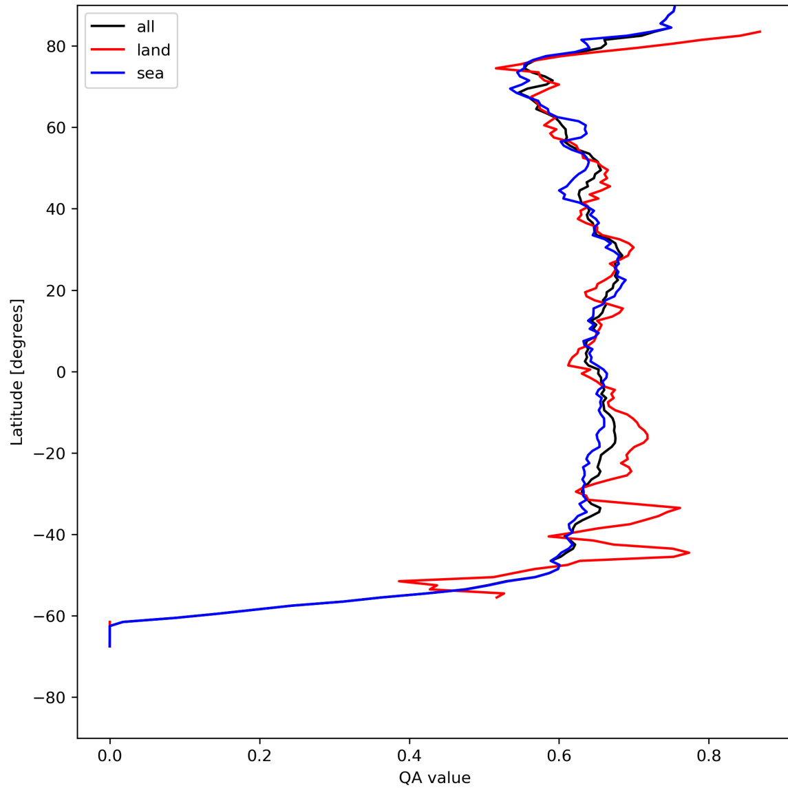
Figure 9: Zonal average of “QA value” for 2024-05-08 to 2024-05-10.
