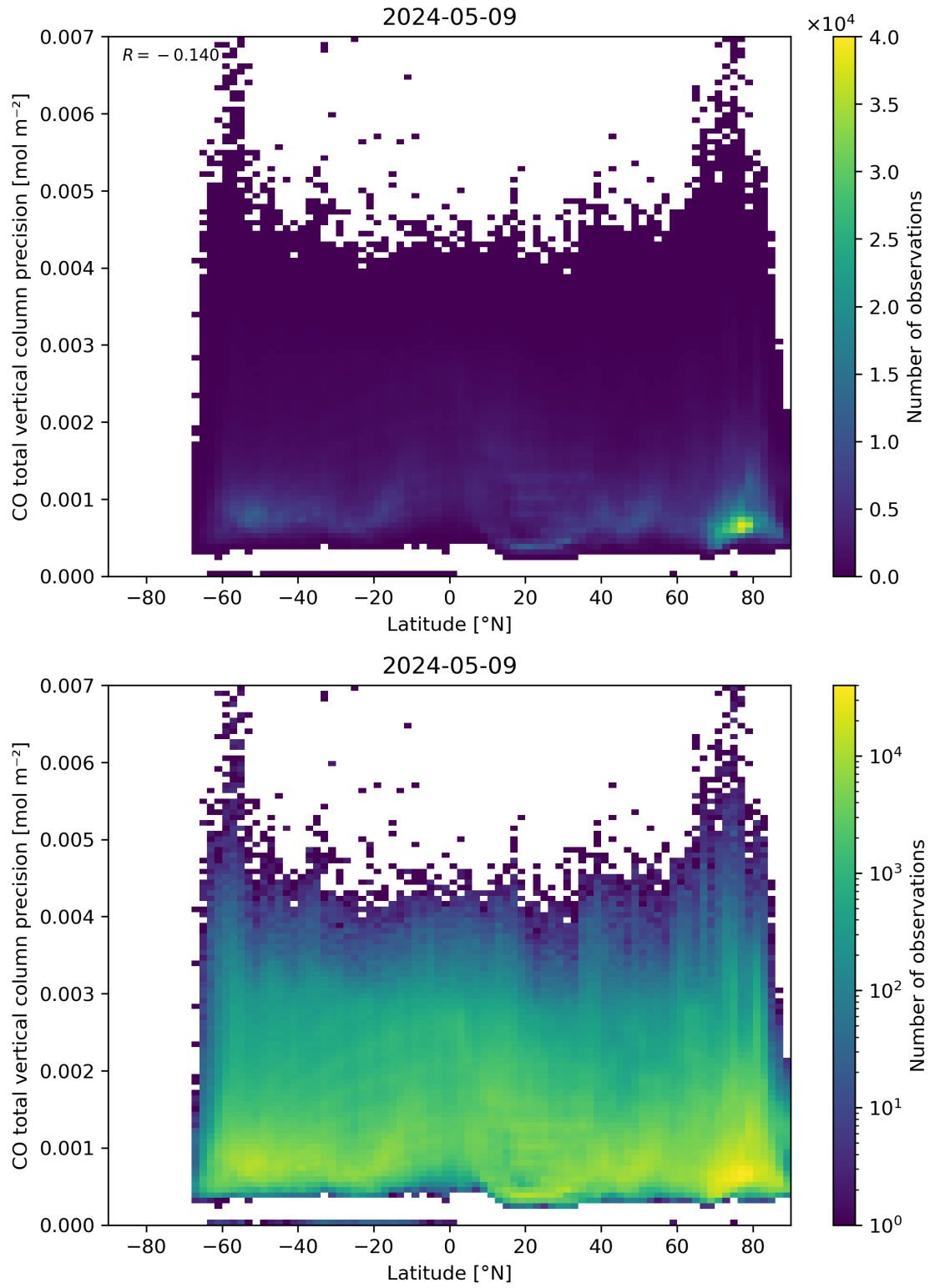
Figure 53: Scatter density plot of “Latitude” against “CO total vertical column precision” for 2024-05-08 to 2024-05-10.
