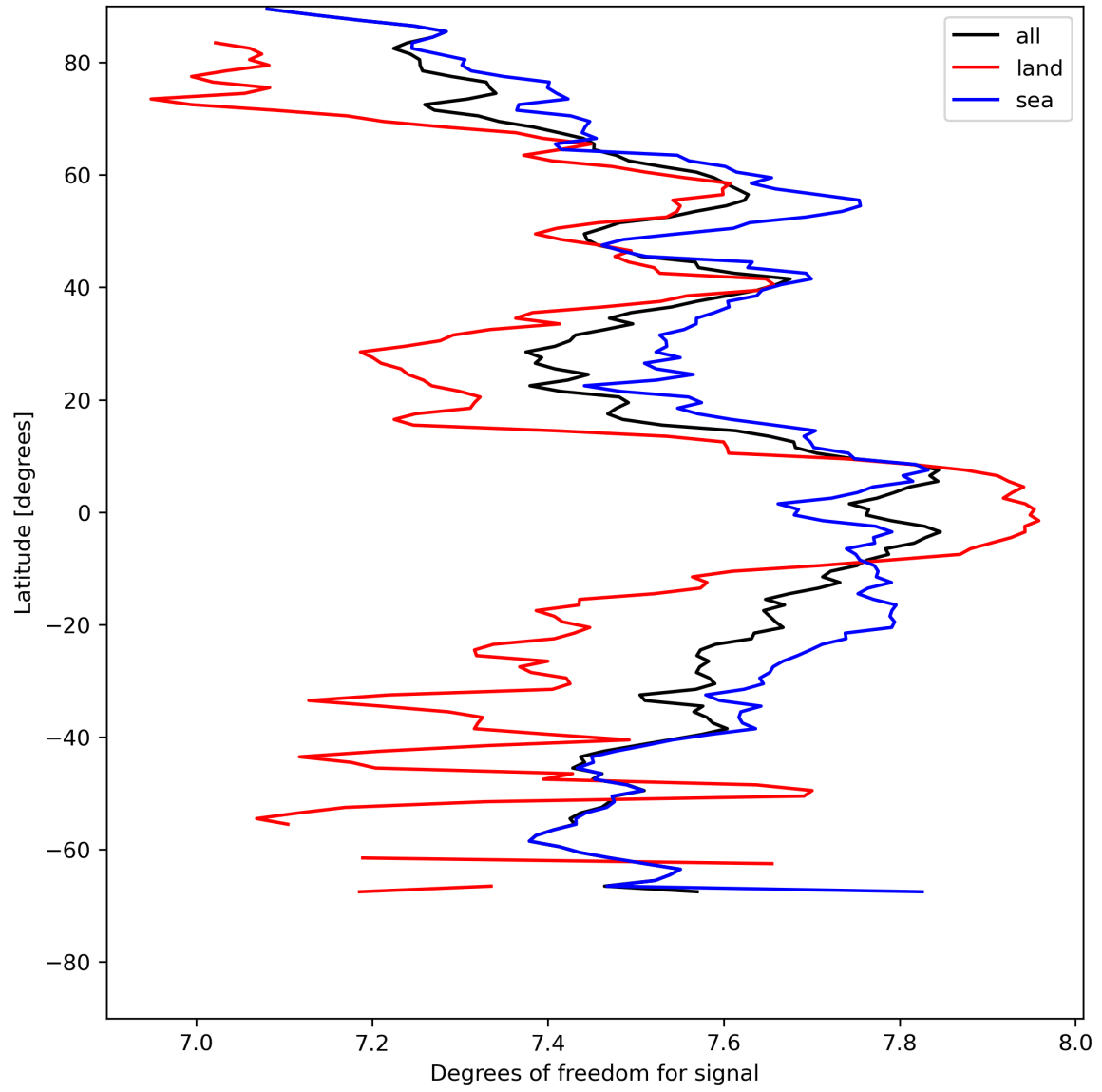
Figure 15: Zonal average of “Degrees of freedom for signal” for 2024-05-08 to 2024-05-10.
