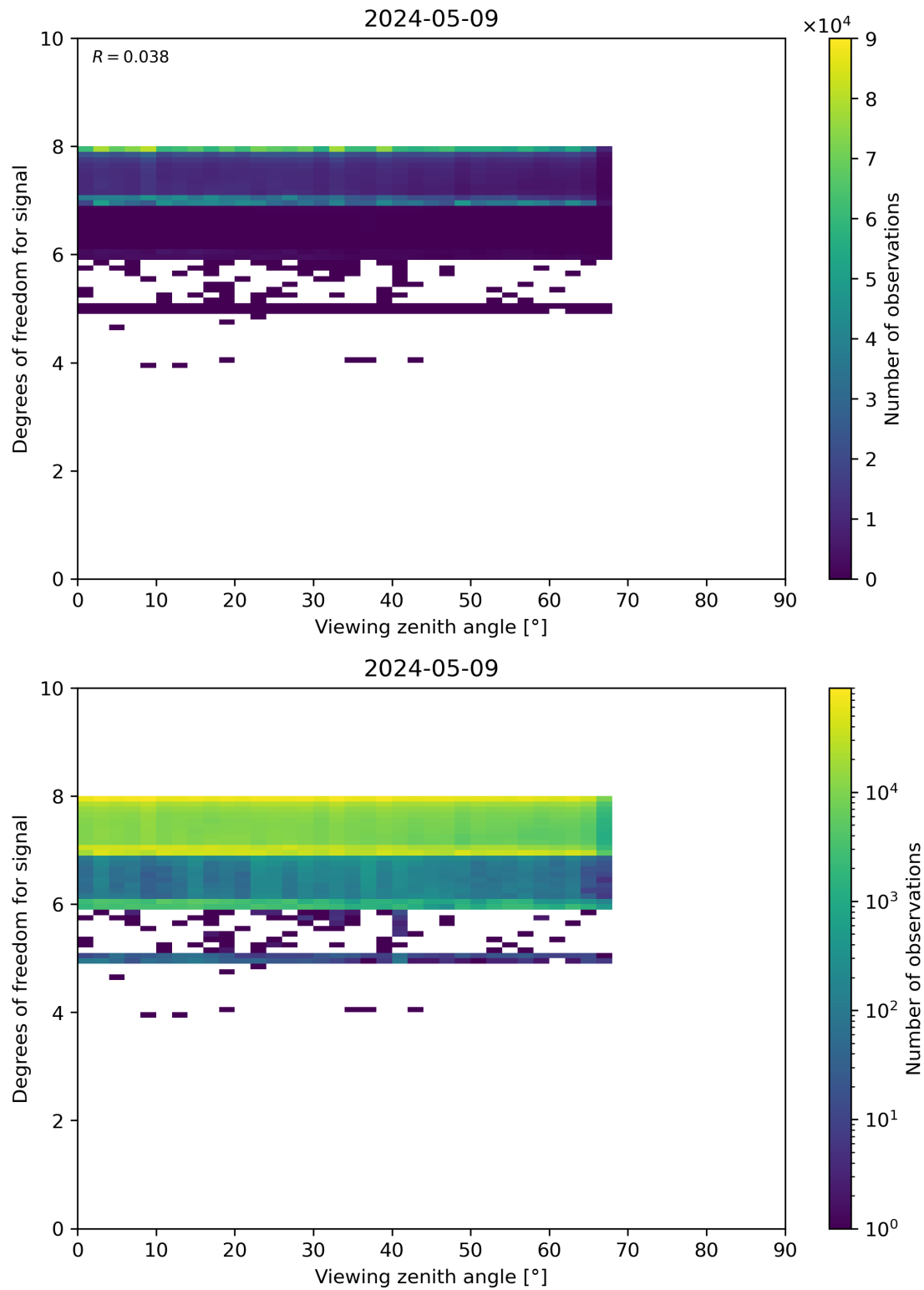
Figure 73: Scatter density plot of “Viewing zenith angle” against “Degrees of freedom for signal” for 2024-05-08 to 2024-05-10.
