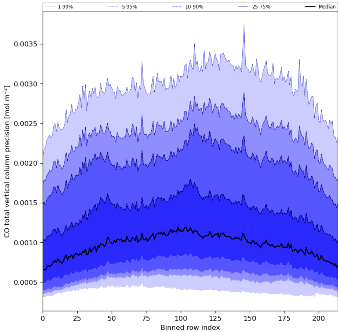
Figure 28: Along track statistics of “CO total vertical column precision” for 2024-05-08 to 2024-05-10
