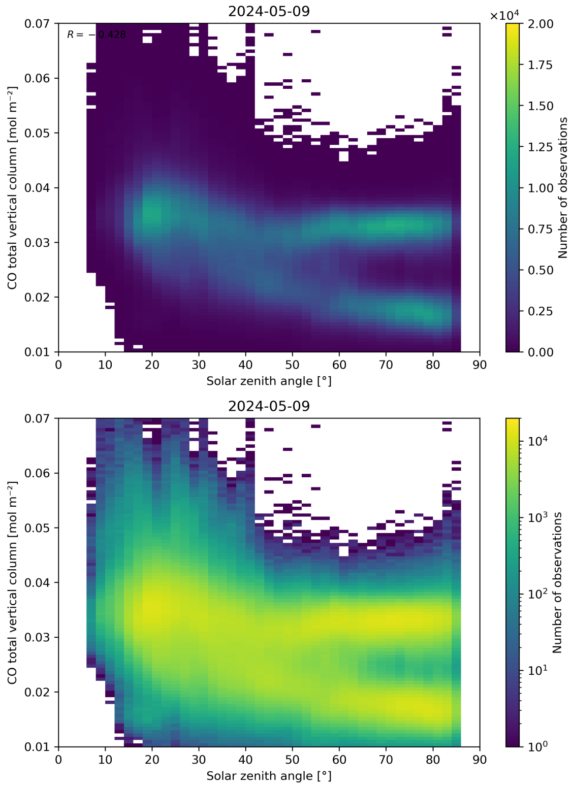
Figure 61: Scatter density plot of “Solar zenith angle” against “CO total vertical column” for 2024-05-08 to 2024-05-10.
