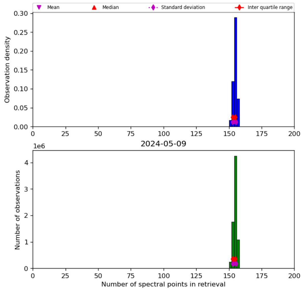
Figure 21: Histogram of “Number of spectral points in retrieval” for 2024-05-08 to 2024-05-10
