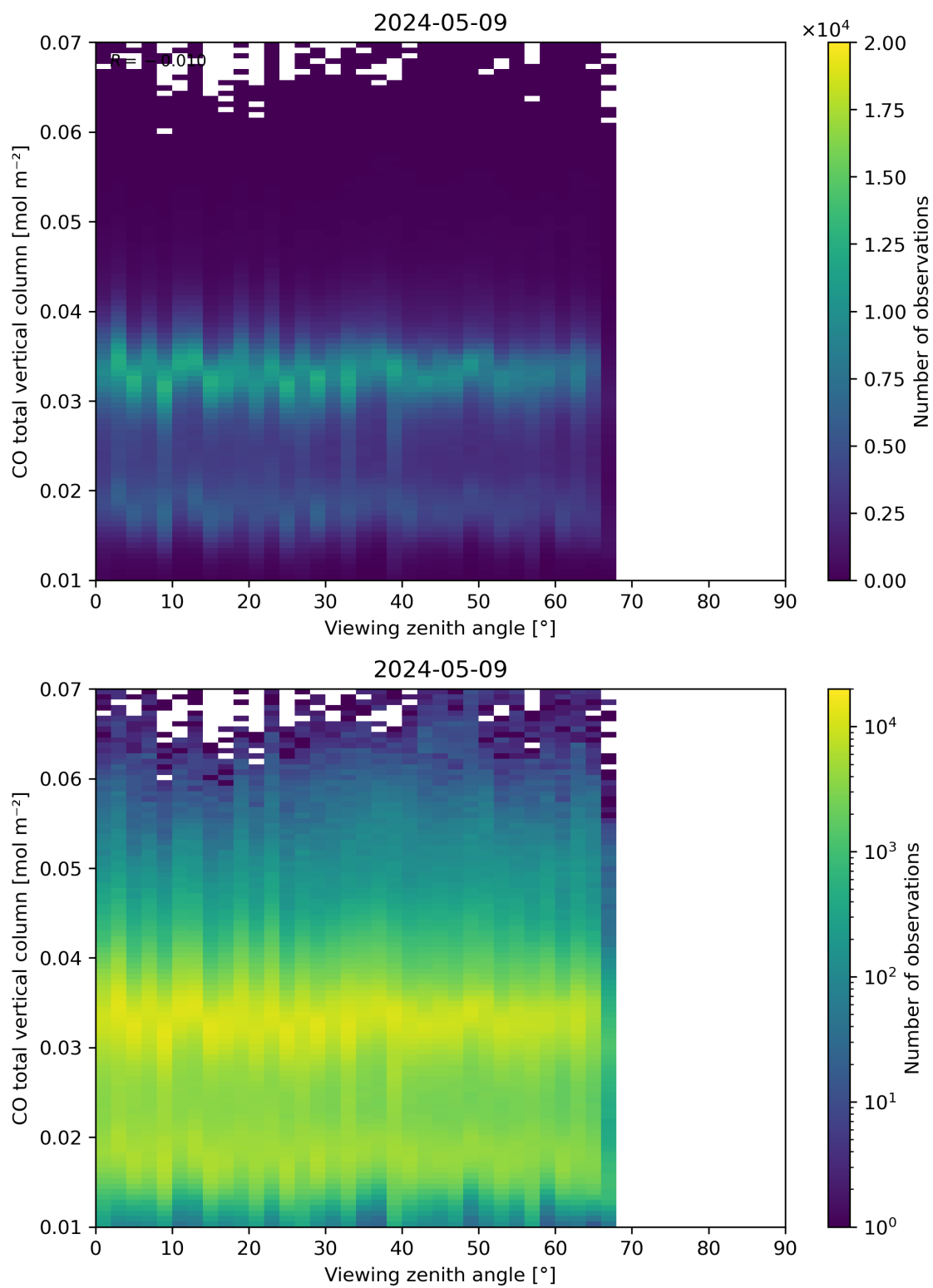
Figure 69: Scatter density plot of “Viewing zenith angle” against “CO total vertical column” for 2024-05-08 to 2024-05-10.
