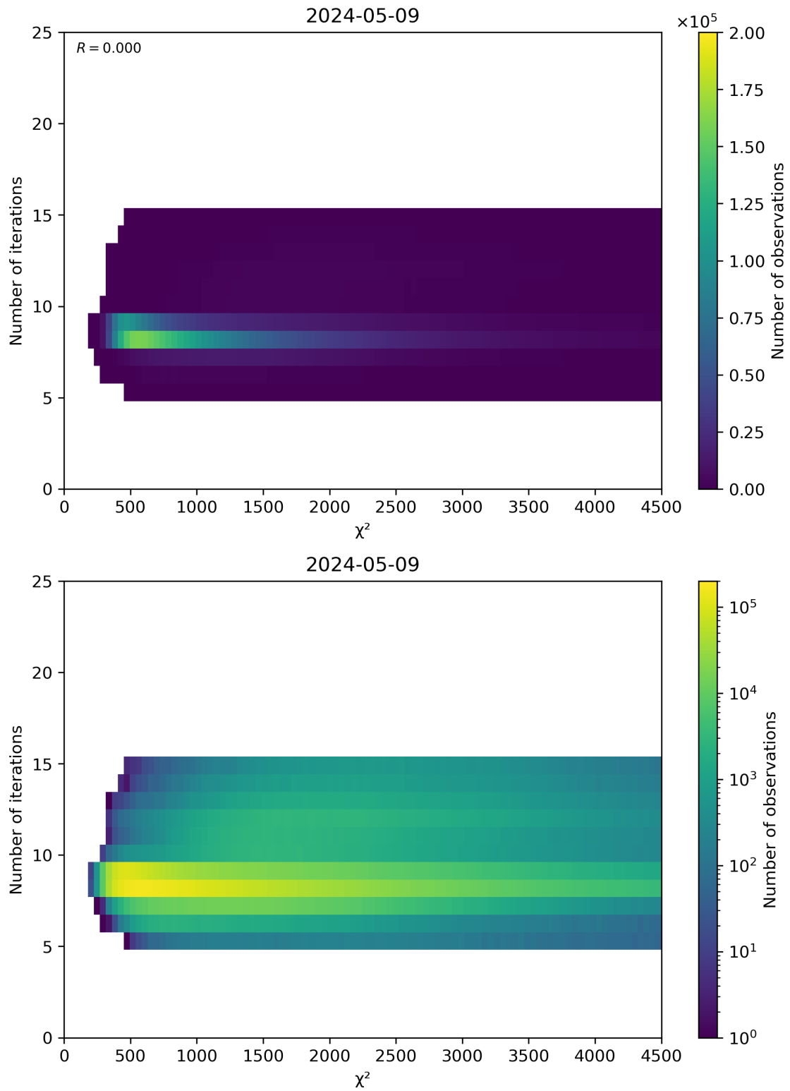
Figure 49: Scatter density plot of “ \chi^2 ” against “Number of iterations” for 2024-05-08 to 2024-05-10.
