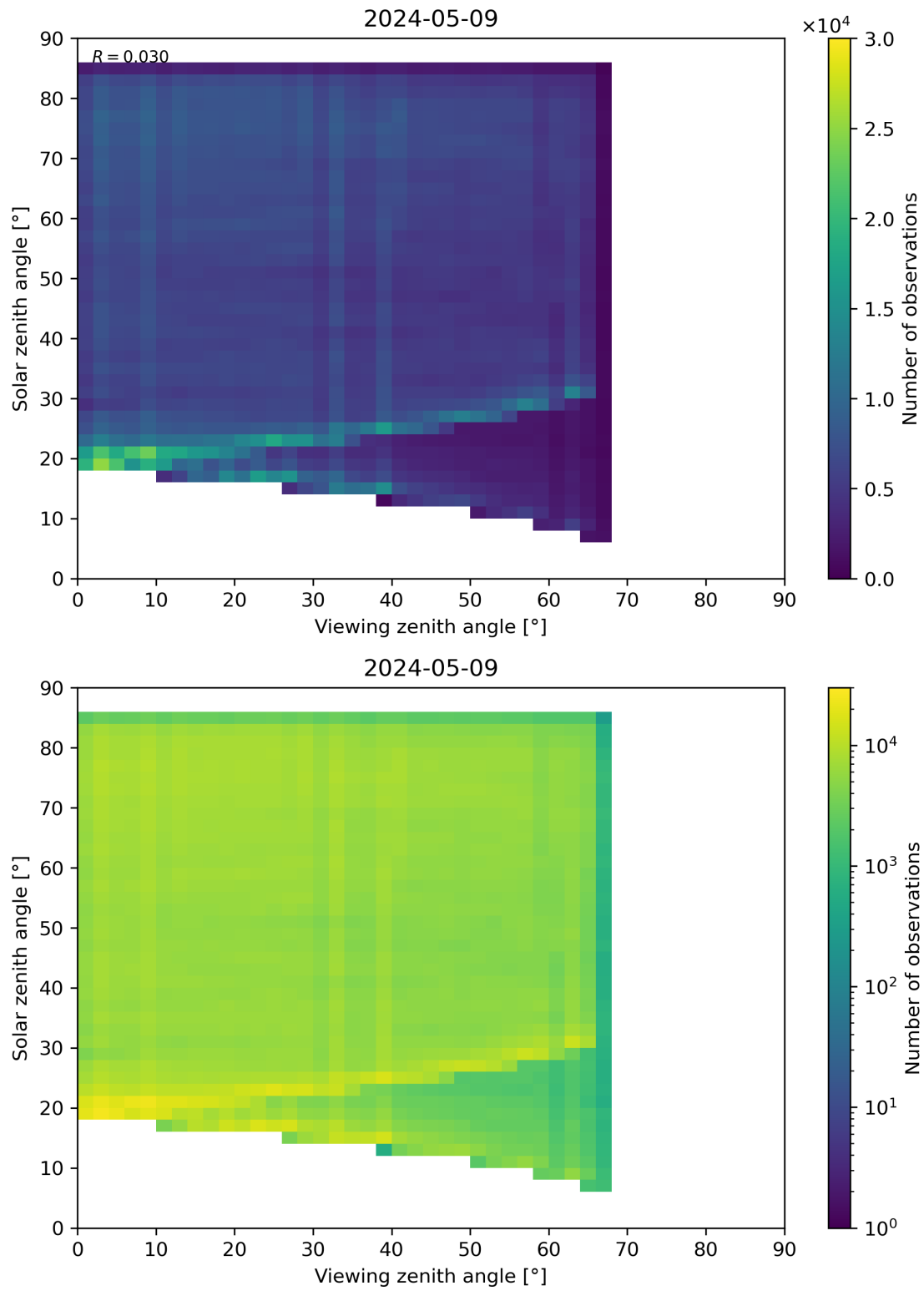
Figure 77: Scatter density plot of “Viewing zenith angle” against “Solar zenith angle” for 2024-05-08 to 2024-05-10.
