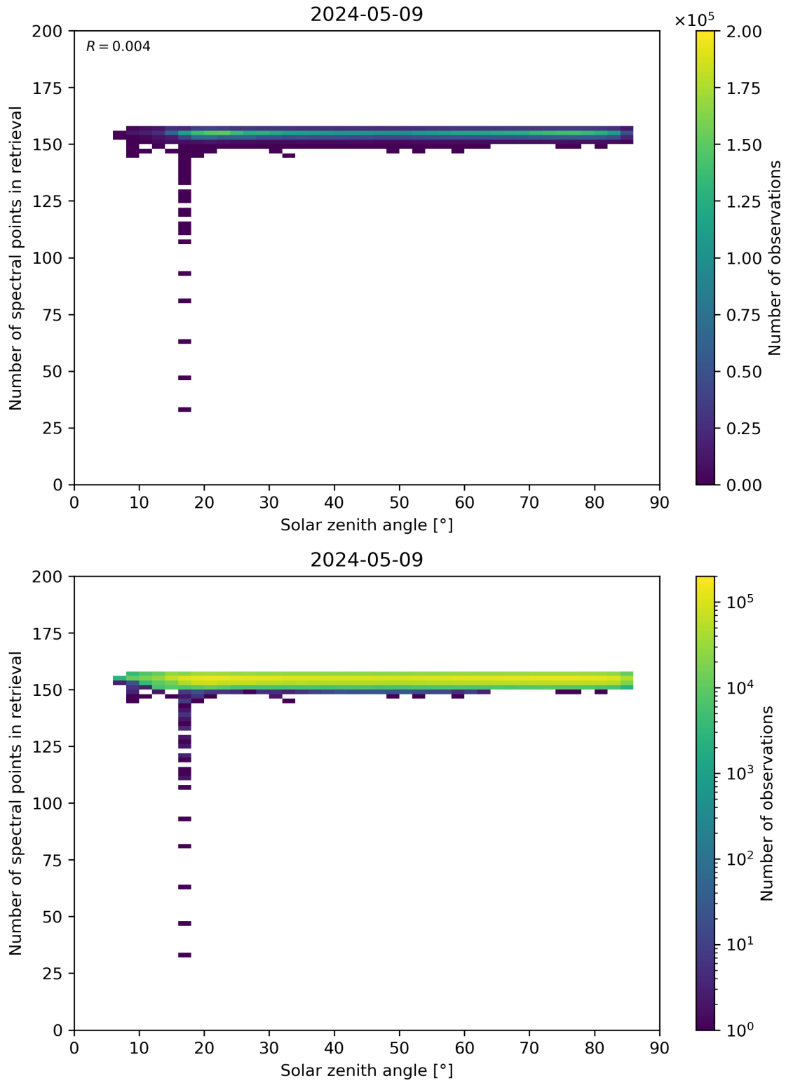
Figure 68: Scatter density plot of “Solar zenith angle” against “Number of spectral points in retrieval” for 2024-05-08 to 2024-05-10.
