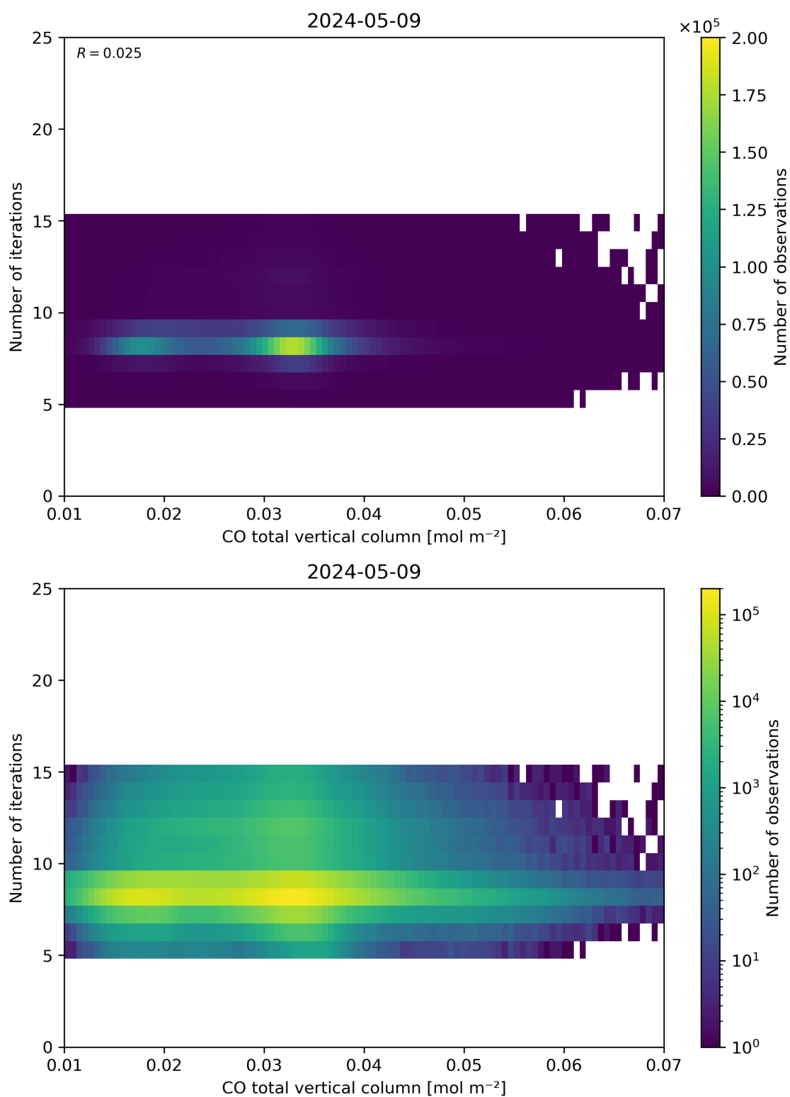
Figure 42: Scatter density plot of “CO total vertical column” against “Number of iterations” for 2024-05-08 to 2024-05-10.
