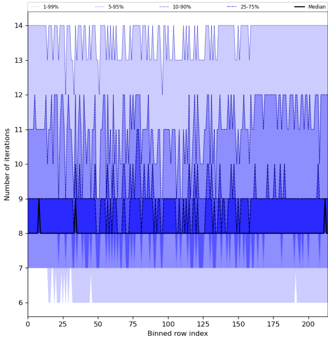
Figure 32: Along track statistics of “Number of iterations” for 2024-05-08 to 2024-05-10
