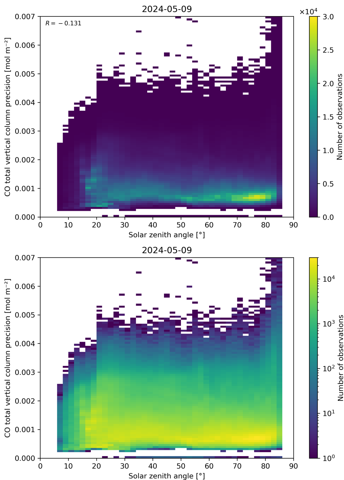
Figure 63: Scatter density plot of “Solar zenith angle” against “CO total vertical column precision” for 2024-05-08 to 2024-05-10.
