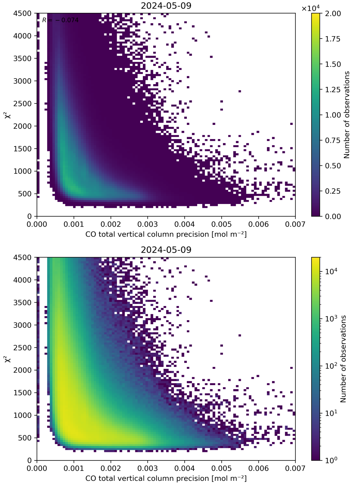
Figure 44: Scatter density plot of “CO total vertical column precision” against “ \chi^2 ” for 2024-05-08 to 2024-05-10.
