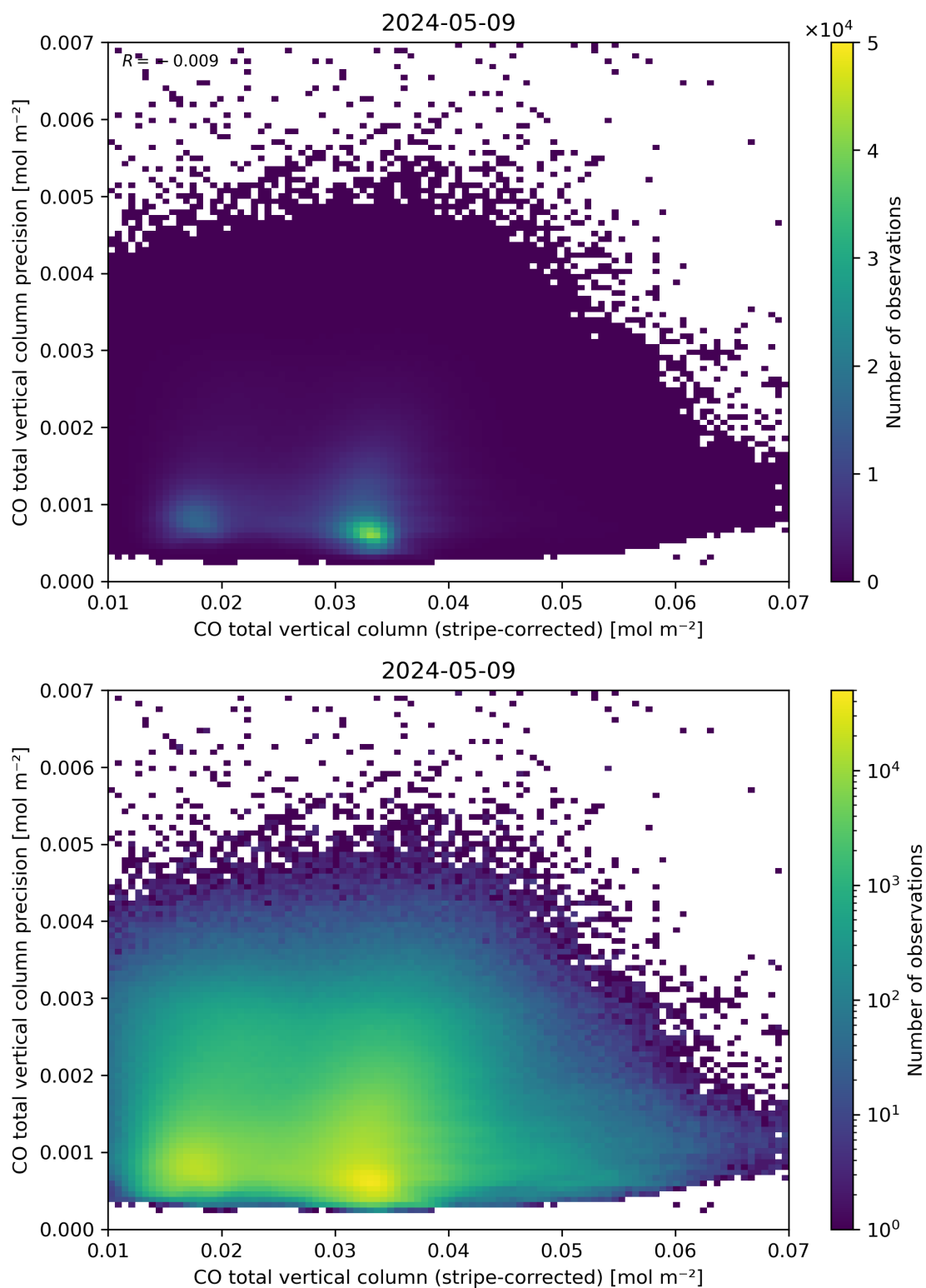
Figure 36: Scatter density plot of “CO total vertical column (stripe-corrected)” against “CO total vertical column precision” for 2024-05-08 to 2024-05-10.
