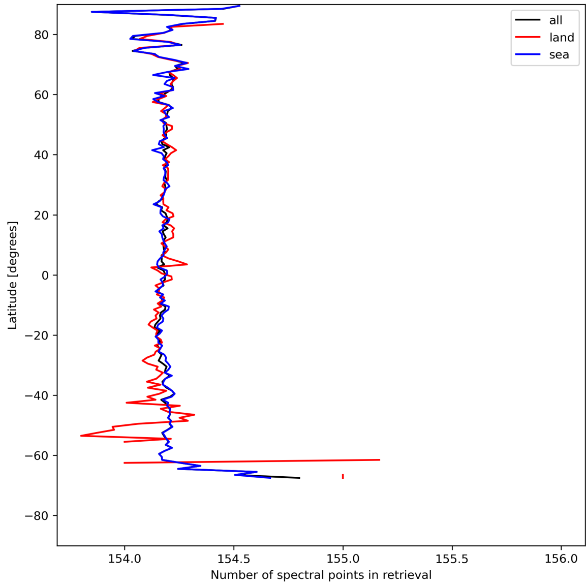
Figure 13: Zonal average of “Number of spectral points in retrieval” for 2024-05-08 to 2024-05-10.
