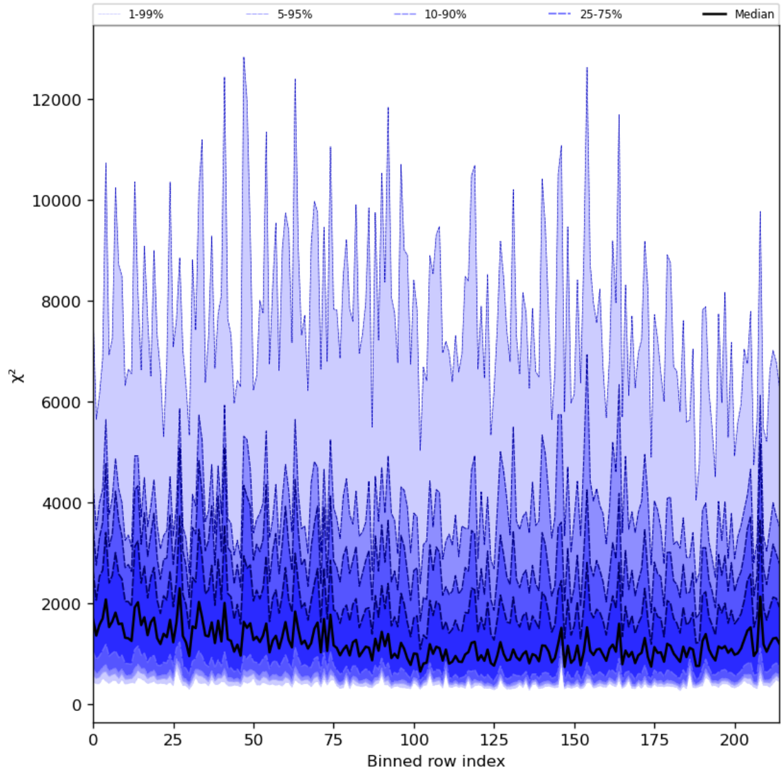
Figure 30: Along track statistics of “ \chi^2 ” for 2024-05-08 to 2024-05-10
