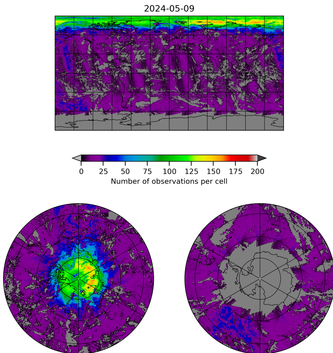
Figure 8: Map of the number of observations for 2024-05-08 to 2024-05-10
