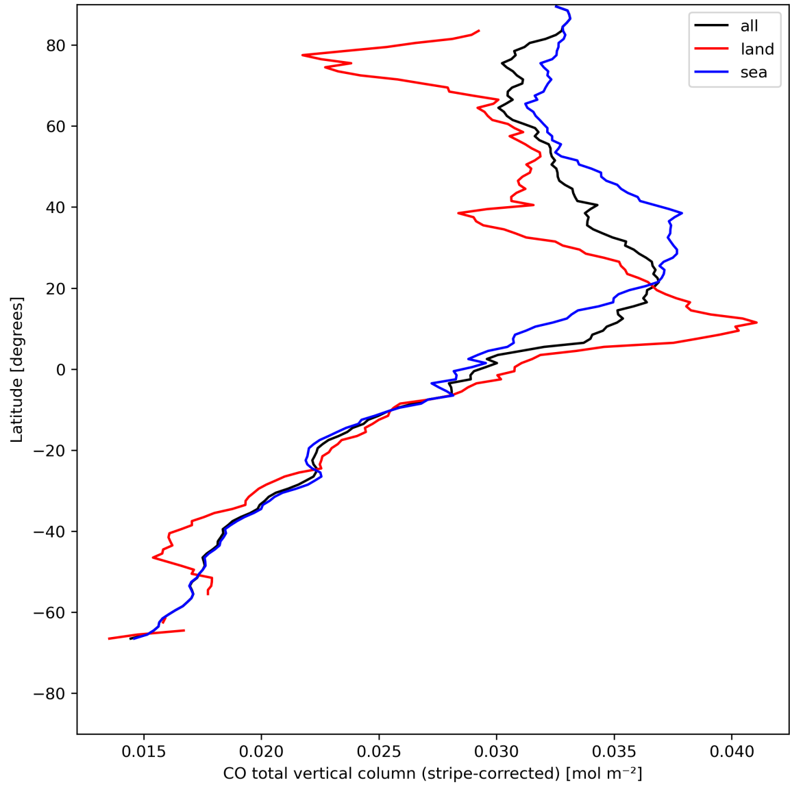
Figure 11: Zonal average of “CO total vertical column (stripe-corrected)” for 2024-05-09 to 2024-05-11.
