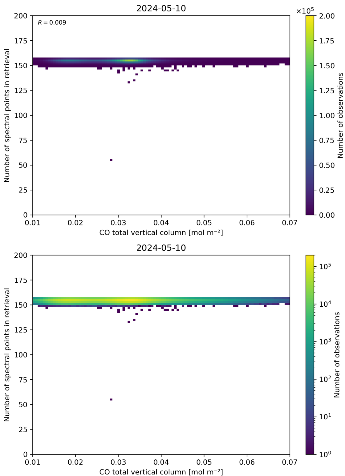
Figure 43: Scatter density plot of “CO total vertical column” against “Number of spectral points in retrieval” for 2024-05-09 to 2024-05-11.
