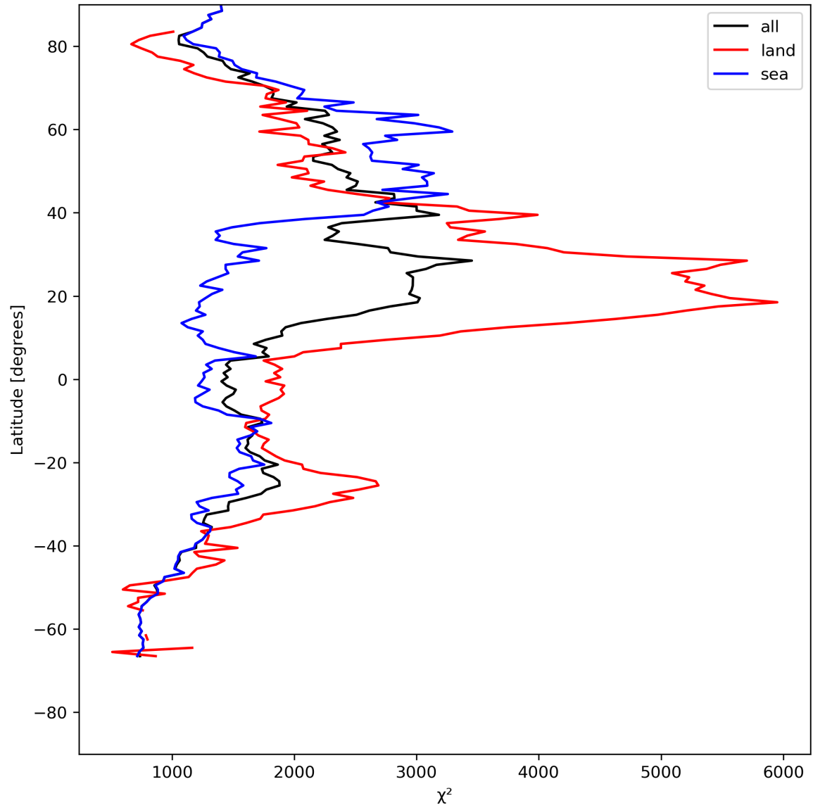
Figure 14: Zonal average of “ \chi^2 ” for 2024-05-09 to 2024-05-11.
