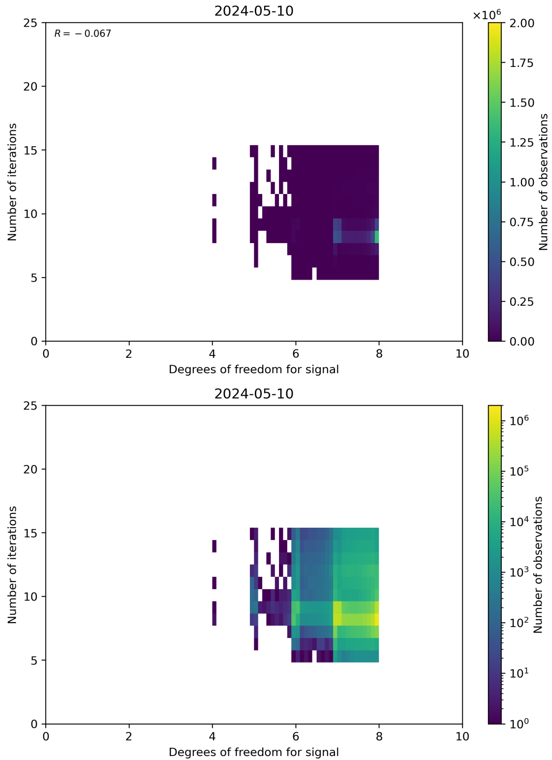
Figure 50: Scatter density plot of “Degrees of freedom for signal” against “Number of iterations” for 2024-05-09 to 2024-05-11.
