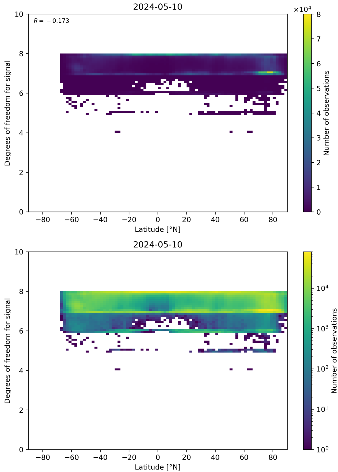
Figure 55: Scatter density plot of “Latitude” against “Degrees of freedom for signal” for 2024-05-09 to 2024-05-11.
