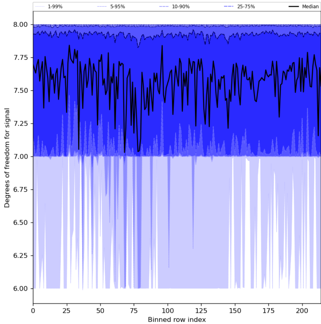
Figure 31: Along track statistics of “Degrees of freedom for signal” for 2024-05-09 to 2024-05-11
