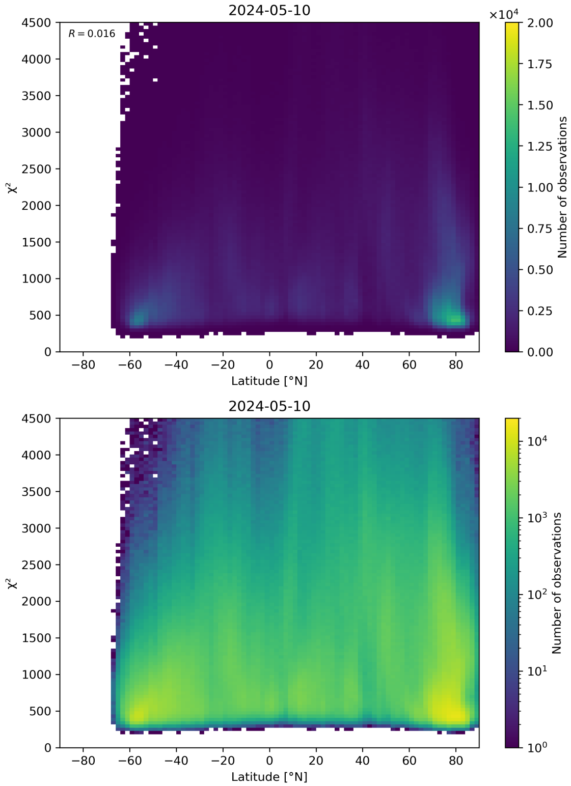
Figure 54: Scatter density plot of “Latitude” against “ \chi^2 ” for 2024-05-09 to 2024-05-11.
