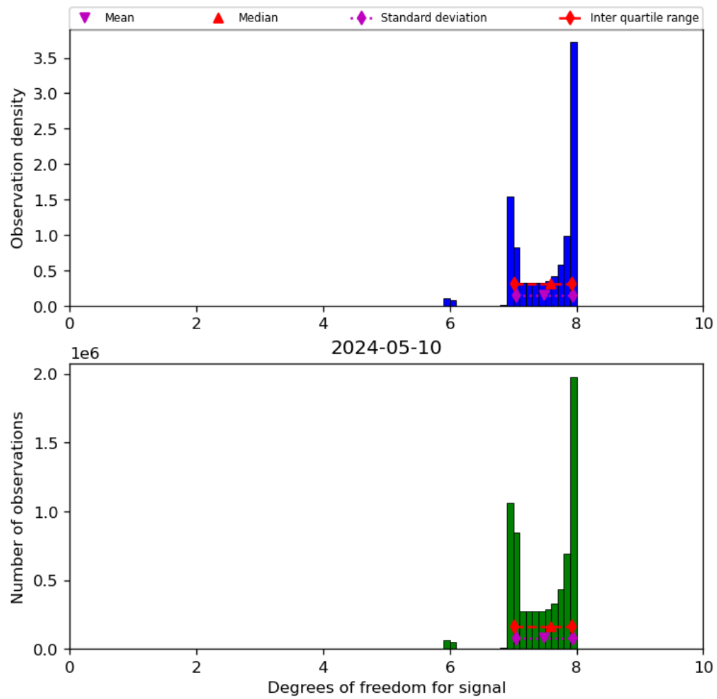
Figure 23: Histogram of “Degrees of freedom for signal” for 2024-05-09 to 2024-05-11
