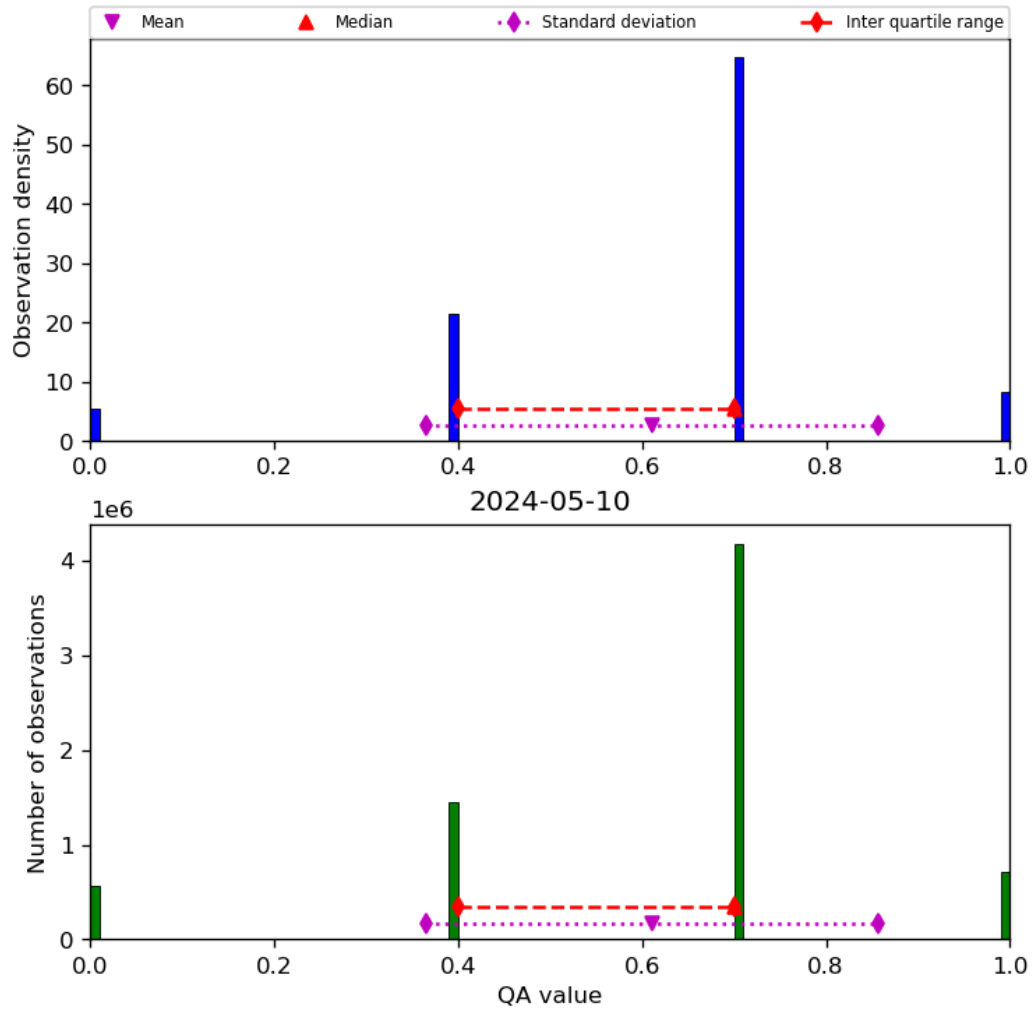
Figure 17: Histogram of “QA value” for 2024-05-09 to 2024-05-11
