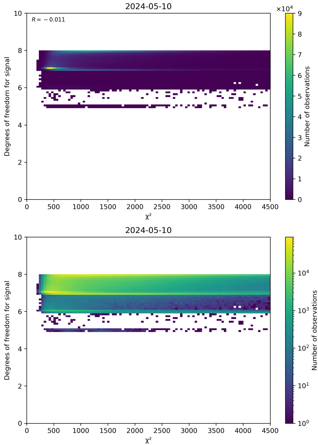
Figure 48: Scatter density plot of “ \chi^2 ” against “Degrees of freedom for signal” for 2024-05-09 to 2024-05-11.
