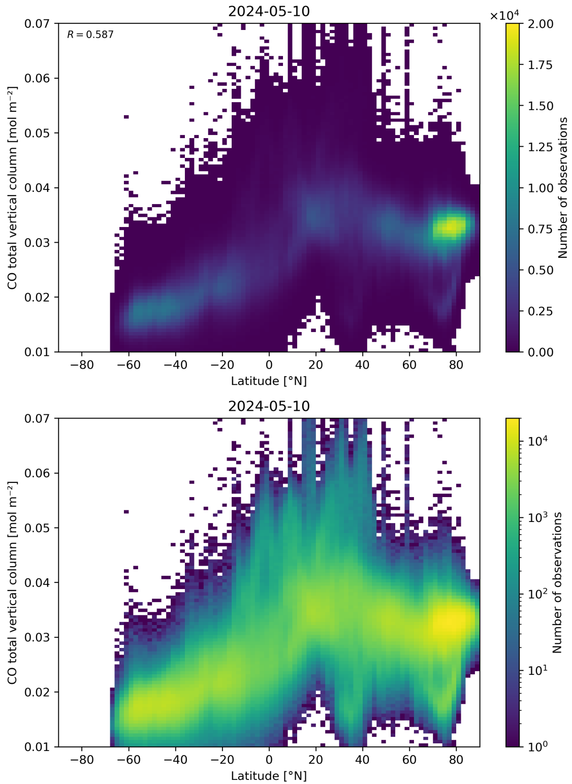
Figure 51: Scatter density plot of “Latitude” against “CO total vertical column” for 2024-05-09 to 2024-05-11.
