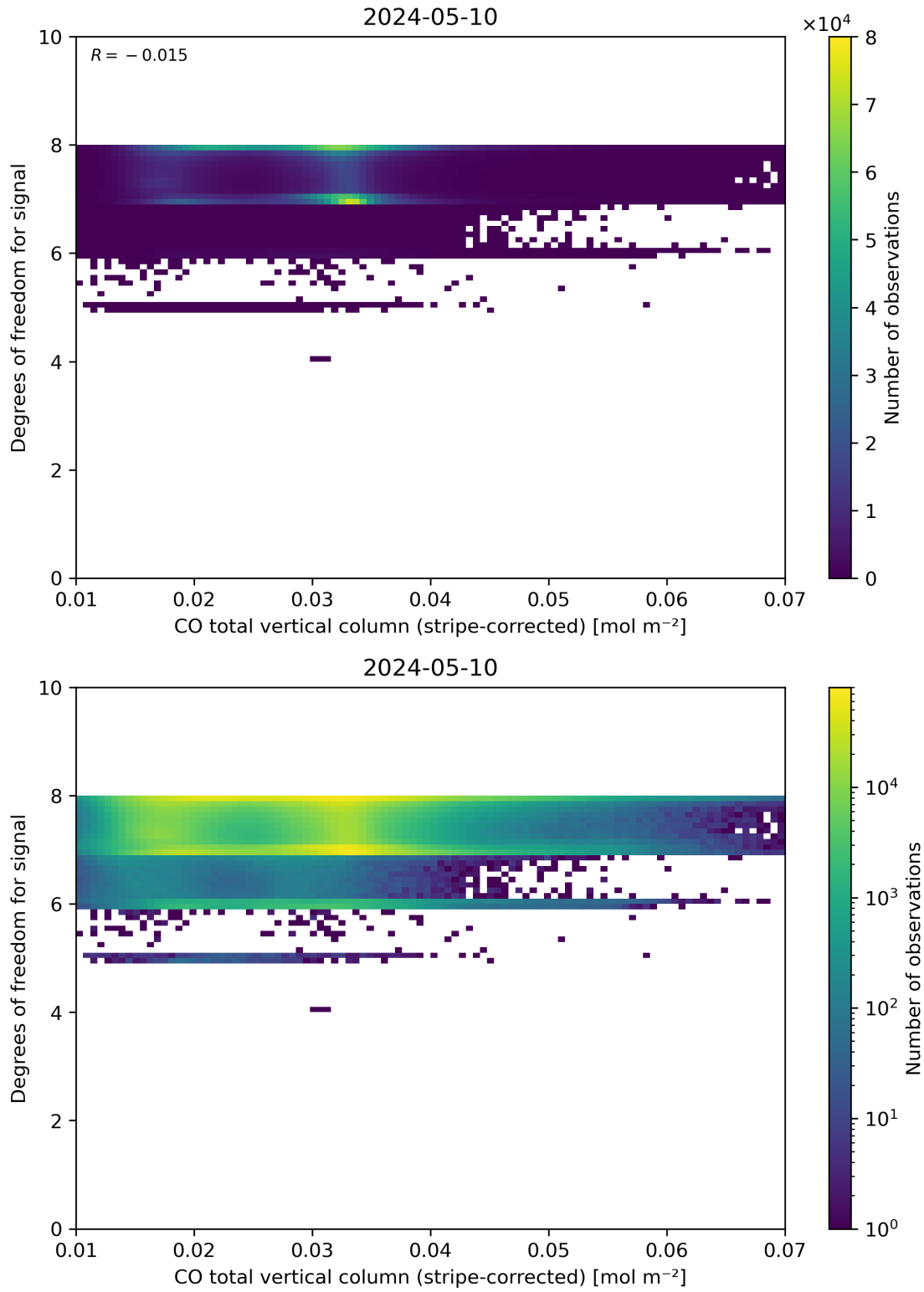
Figure 38: Scatter density plot of “CO total vertical column (stripe-corrected)” against “Degrees of freedom for signal” for 2024-05-09 to 2024-05-11.
