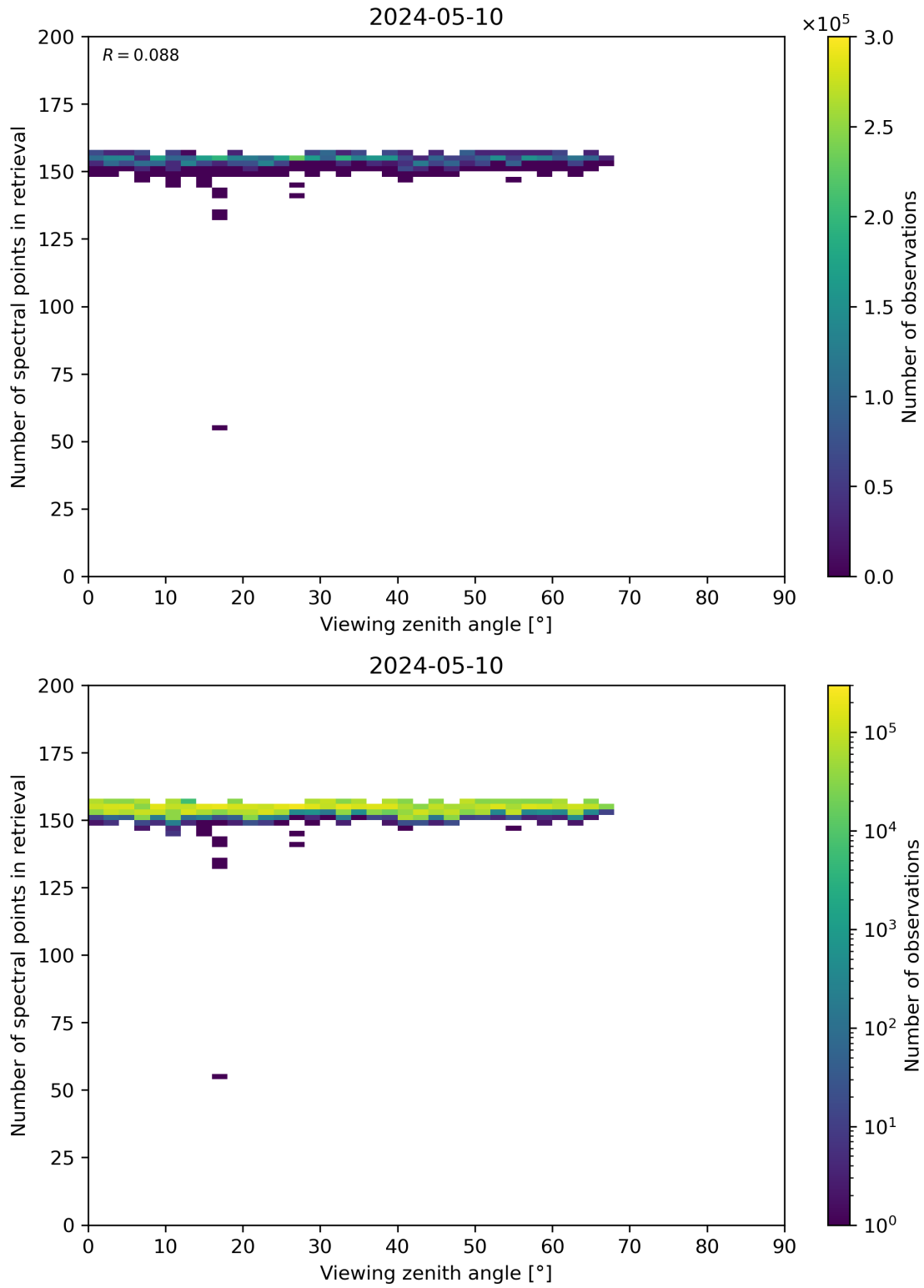
Figure 76: Scatter density plot of “Viewing zenith angle” against “Number of spectral points in retrieval” for 2024-05-09 to 2024-05-11.
