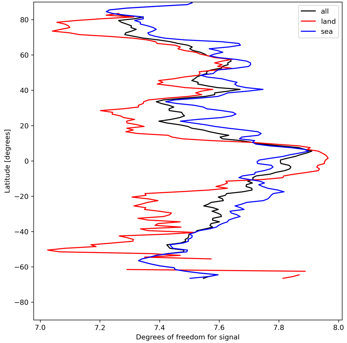
Figure 15: Zonal average of “Degrees of freedom for signal” for 2024-05-09 to 2024-05-11.
