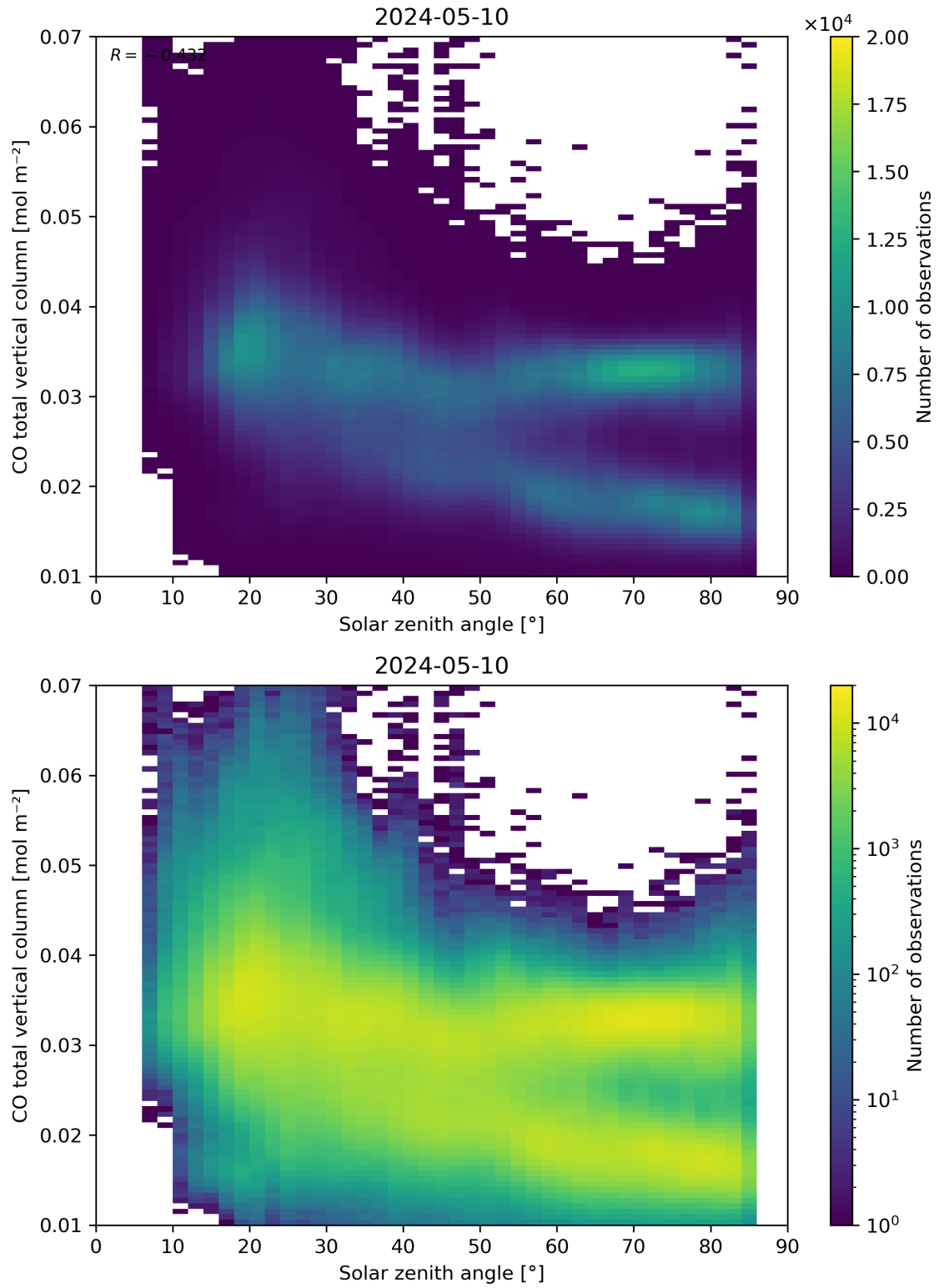
Figure 61: Scatter density plot of “Solar zenith angle” against “CO total vertical column” for 2024-05-09 to 2024-05-11.
