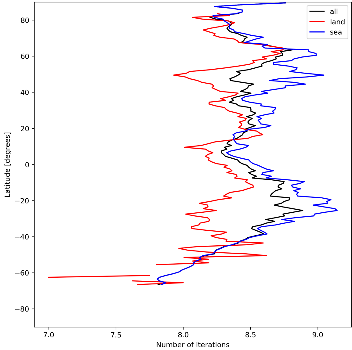
Figure 16: Zonal average of “Number of iterations” for 2024-05-09 to 2024-05-11.
