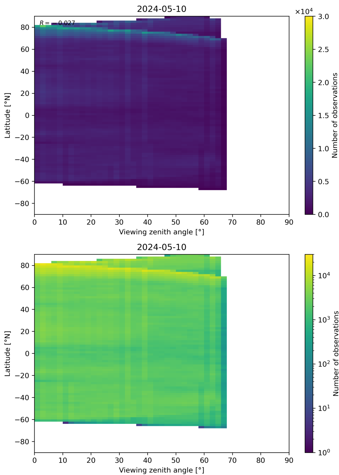
Figure 74: Scatter density plot of “Viewing zenith angle” against “Latitude” for 2024-05-09 to 2024-05-11.
