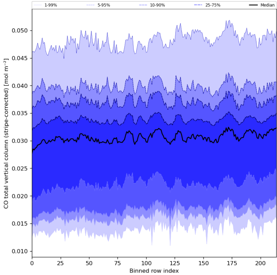
Figure 27: Along track statistics of “CO total vertical column (stripe-corrected)” for 2024-05-09 to 2024-05-11
