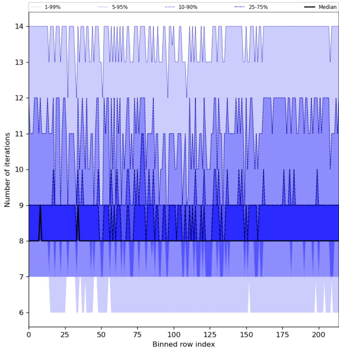
Figure 32: Along track statistics of “Number of iterations” for 2024-05-09 to 2024-05-11
