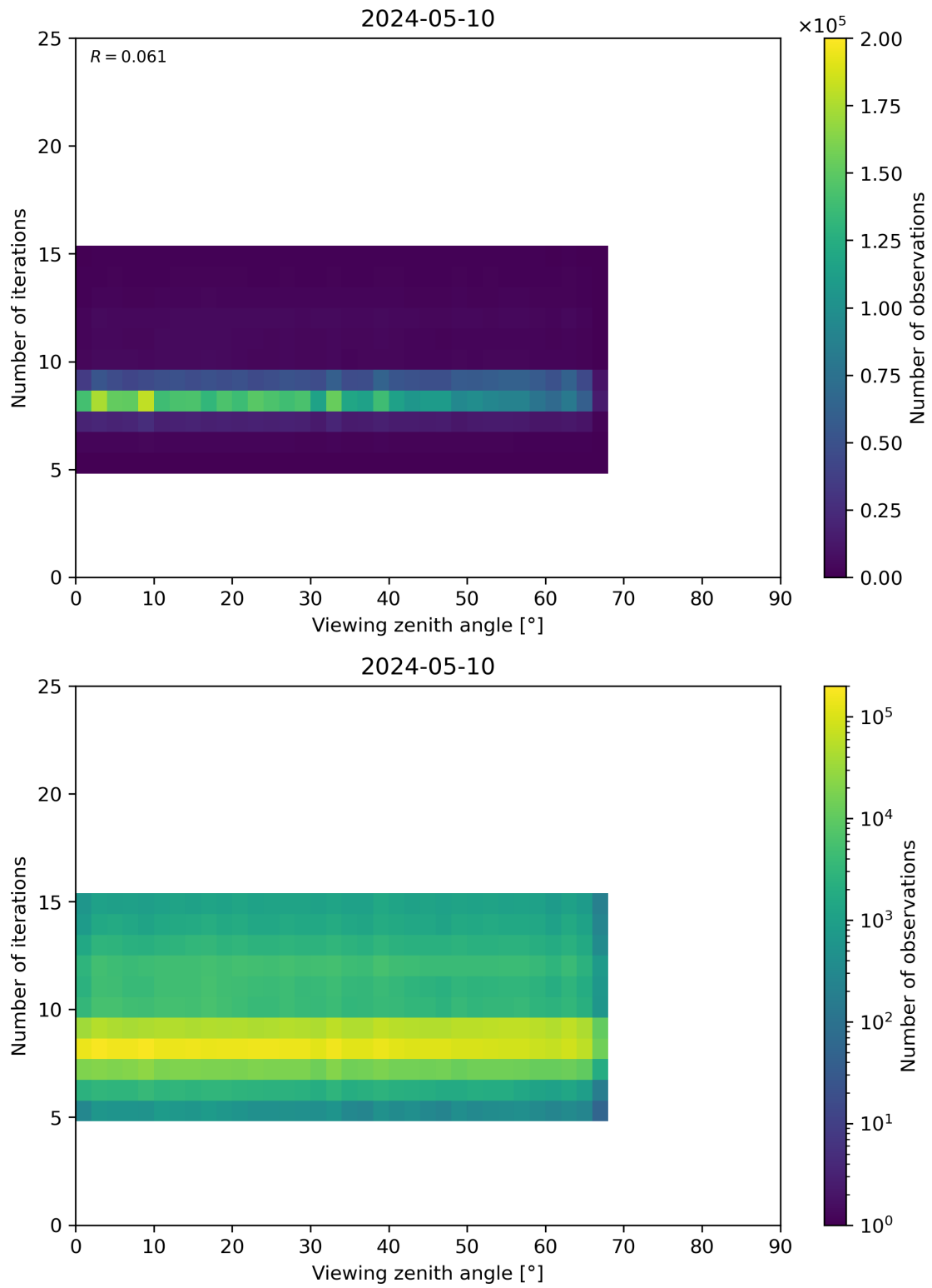
Figure 75: Scatter density plot of “Viewing zenith angle” against “Number of iterations” for 2024-05-09 to 2024-05-11.
