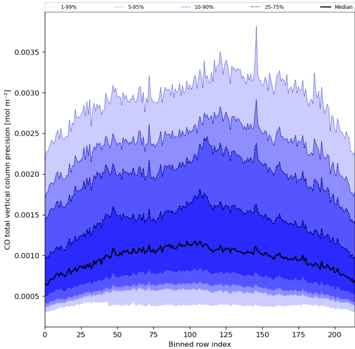
Figure 28: Along track statistics of “CO total vertical column precision” for 2024-05-09 to 2024-05-11
