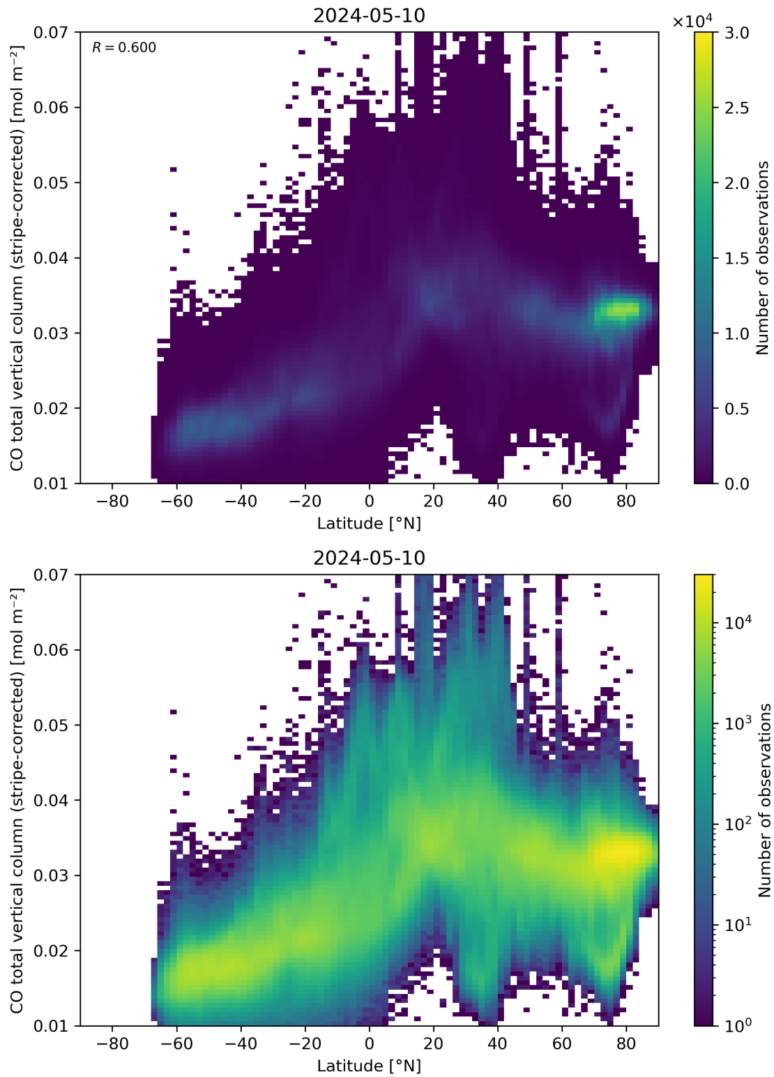
Figure 52: Scatter density plot of “Latitude” against “CO total vertical column (stripe-corrected)” for 2024-05-09 to 2024-05-11.
