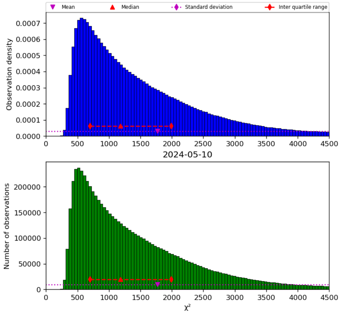
Figure 22: Histogram of “ \chi^2 ” for 2024-05-09 to 2024-05-11
