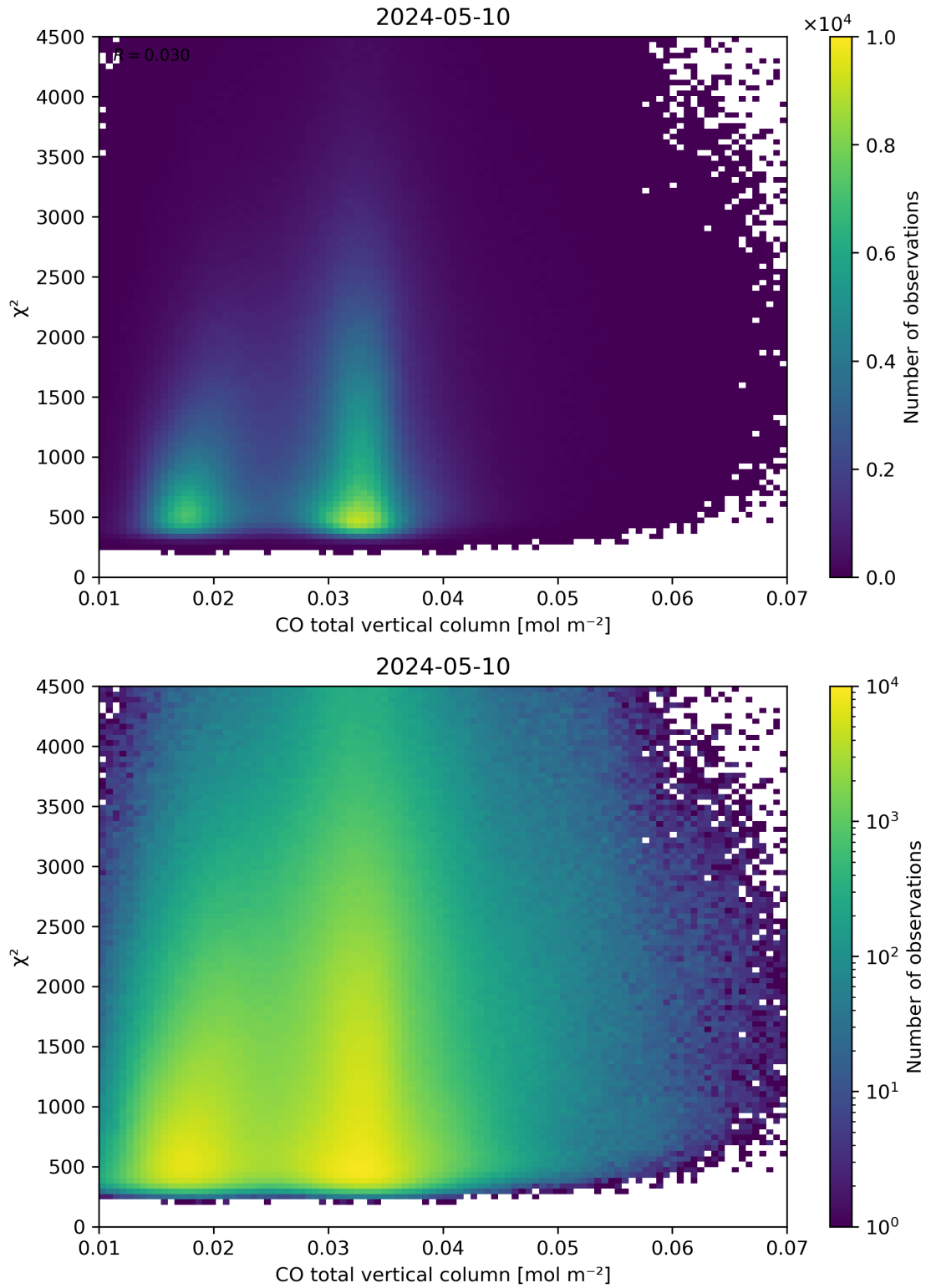
Figure 35: Scatter density plot of “CO total vertical column” against “ \chi^2 ” for 2024-05-09 to 2024-05-11.
