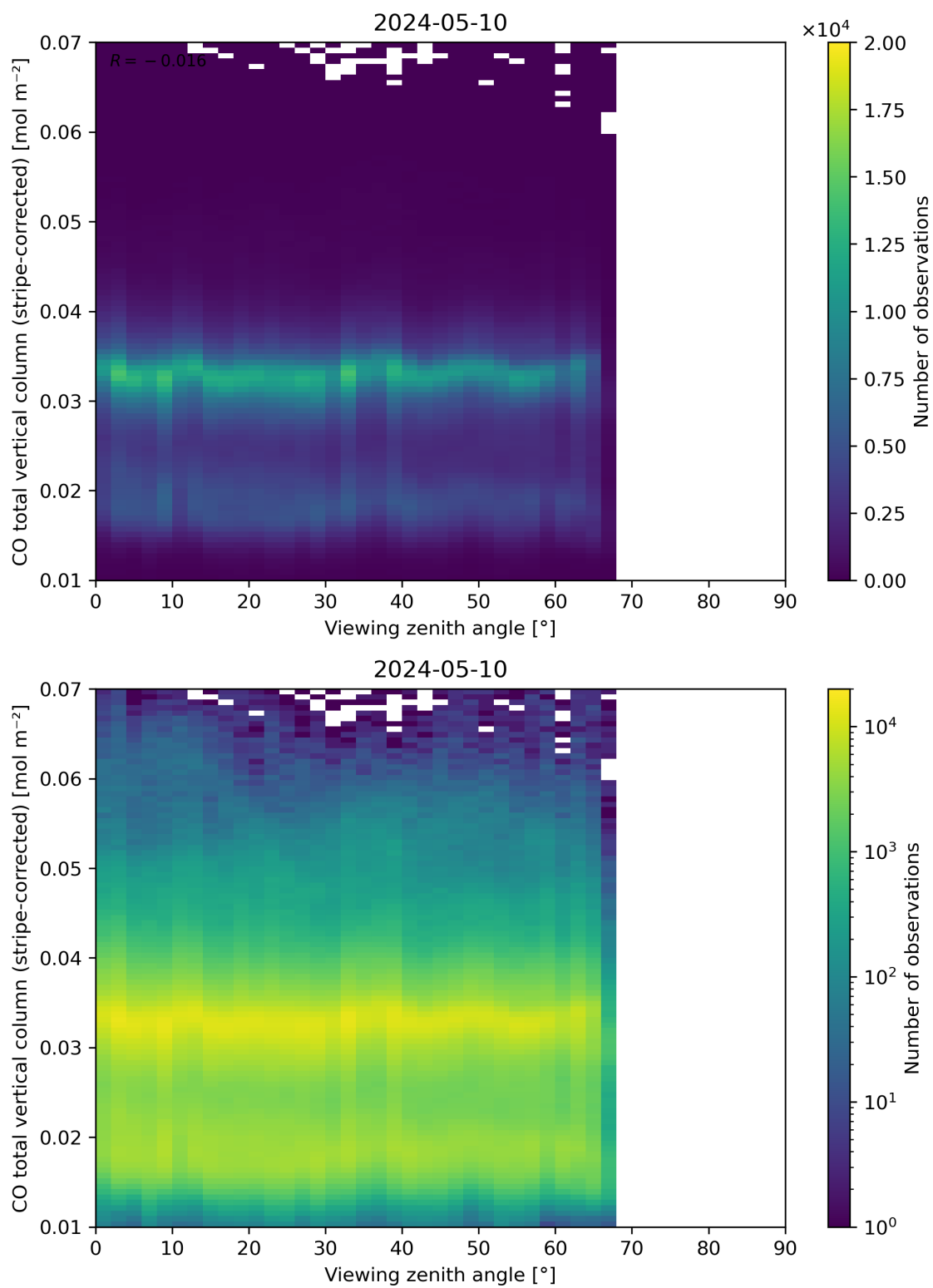
Figure 70: Scatter density plot of “Viewing zenith angle” against “CO total vertical column (stripe-corrected)” for 2024-05-09 to 2024-05-11.
