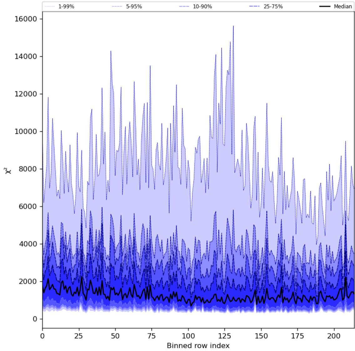
Figure 30: Along track statistics of “ \chi^2 ” for 2024-05-09 to 2024-05-11
