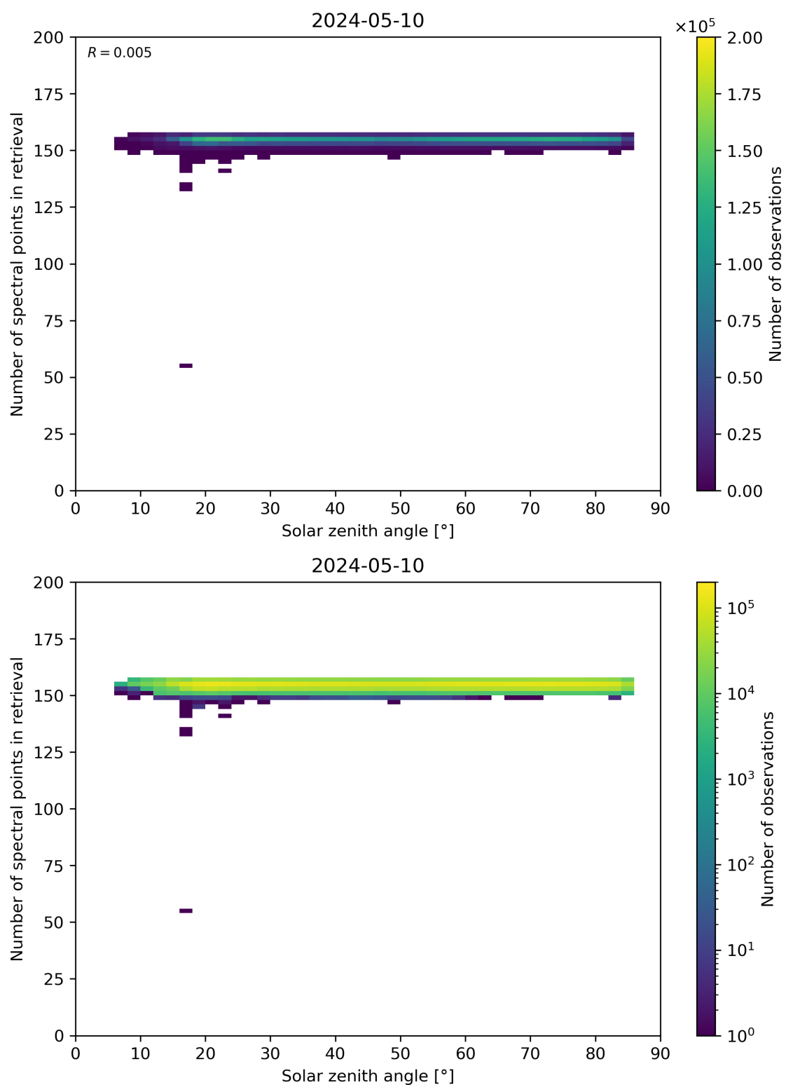
Figure 68: Scatter density plot of “Solar zenith angle” against “Number of spectral points in retrieval” for 2024-05-09 to 2024-05-11.
