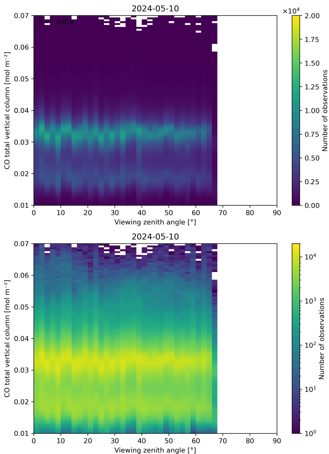
Figure 69: Scatter density plot of “Viewing zenith angle” against “CO total vertical column” for 2024-05-09 to 2024-05-11.
