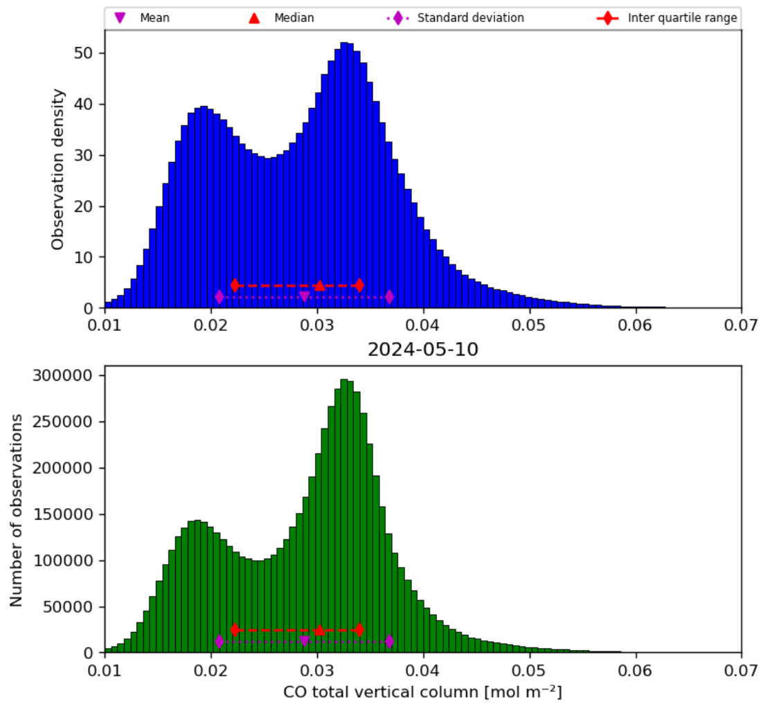
Figure 18: Histogram of “CO total vertical column” for 2024-05-09 to 2024-05-11
