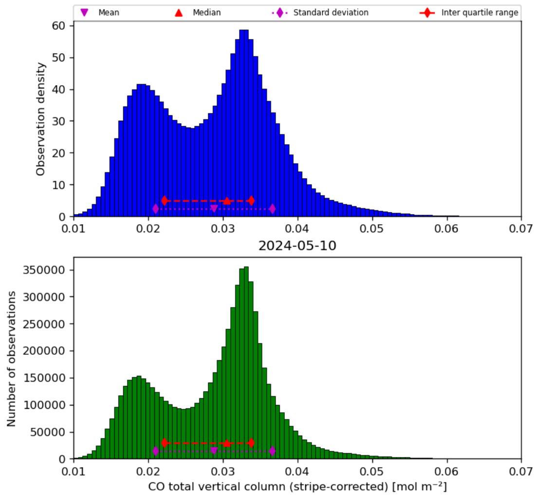
Figure 19: Histogram of “CO total vertical column (stripe-corrected)” for 2024-05-09 to 2024-05-11
