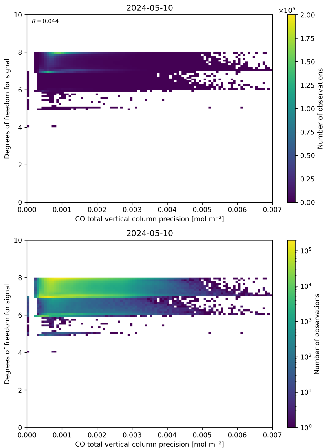
Figure 45: Scatter density plot of “CO total vertical column precision” against “Degrees of freedom for signal” for 2024-05-09 to 2024-05-11.
