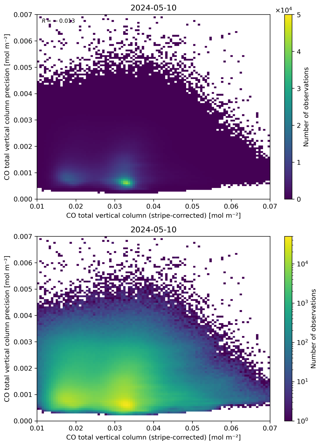
Figure 36: Scatter density plot of “CO total vertical column (stripe-corrected)” against “CO total vertical column precision” for 2024-05-09 to 2024-05-11.
