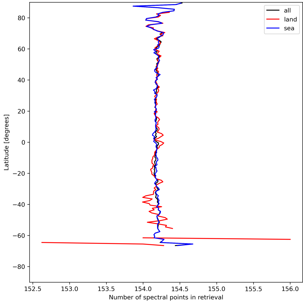
Figure 13: Zonal average of “Number of spectral points in retrieval” for 2024-05-09 to 2024-05-11.
