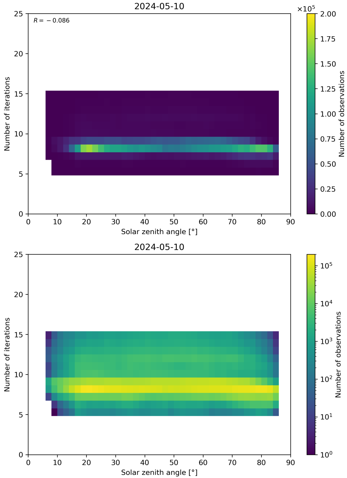
Figure 67: Scatter density plot of “Solar zenith angle” against “Number of iterations” for 2024-05-09 to 2024-05-11.
