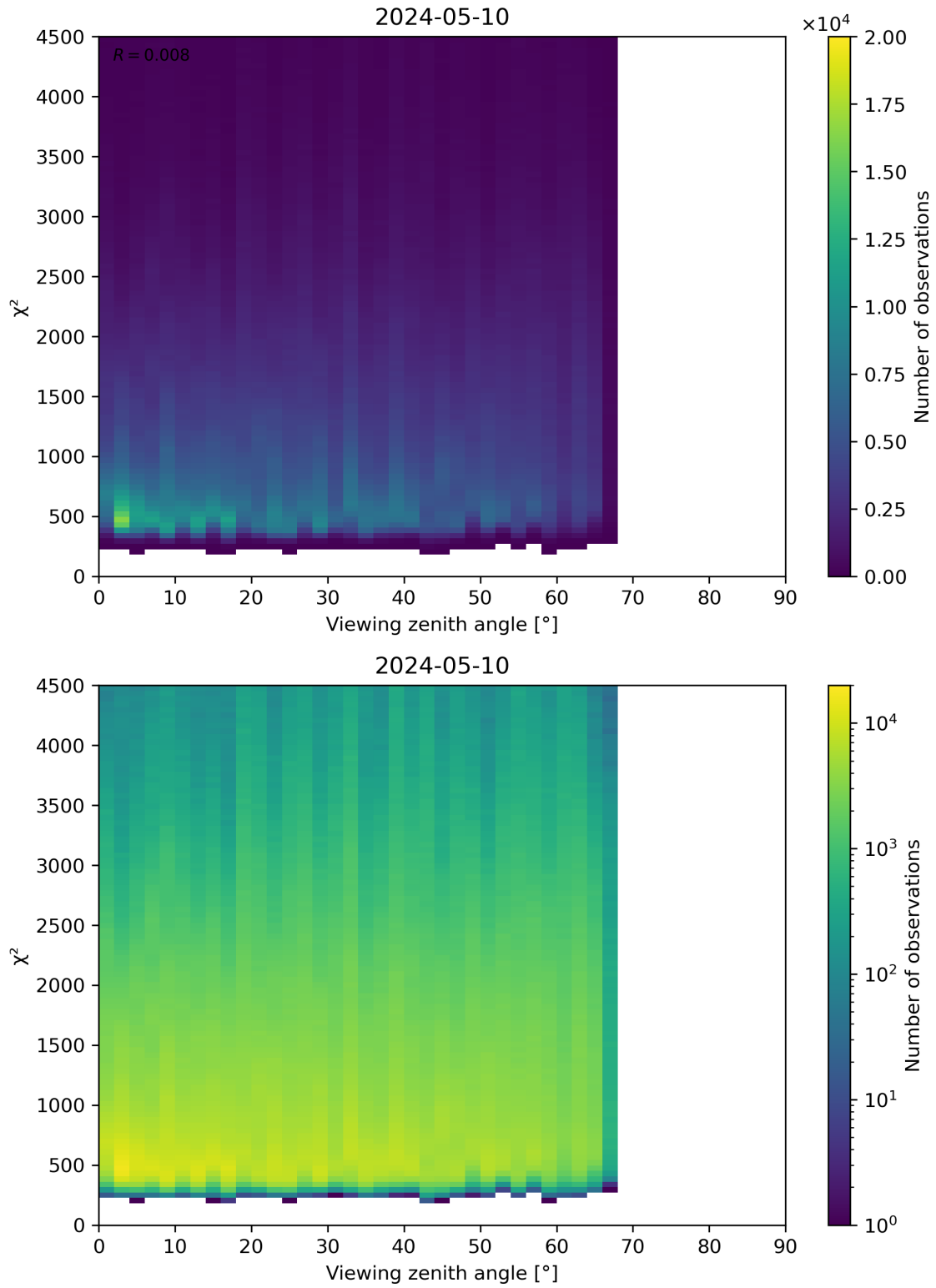
Figure 72: Scatter density plot of “Viewing zenith angle” against “ \chi^2 ” for 2024-05-09 to 2024-05-11.
