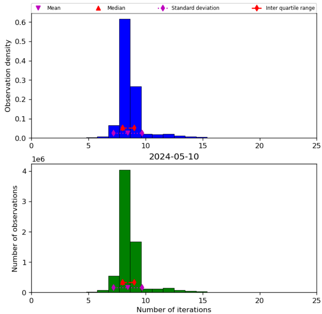
Figure 24: Histogram of “Number of iterations” for 2024-05-09 to 2024-05-11
