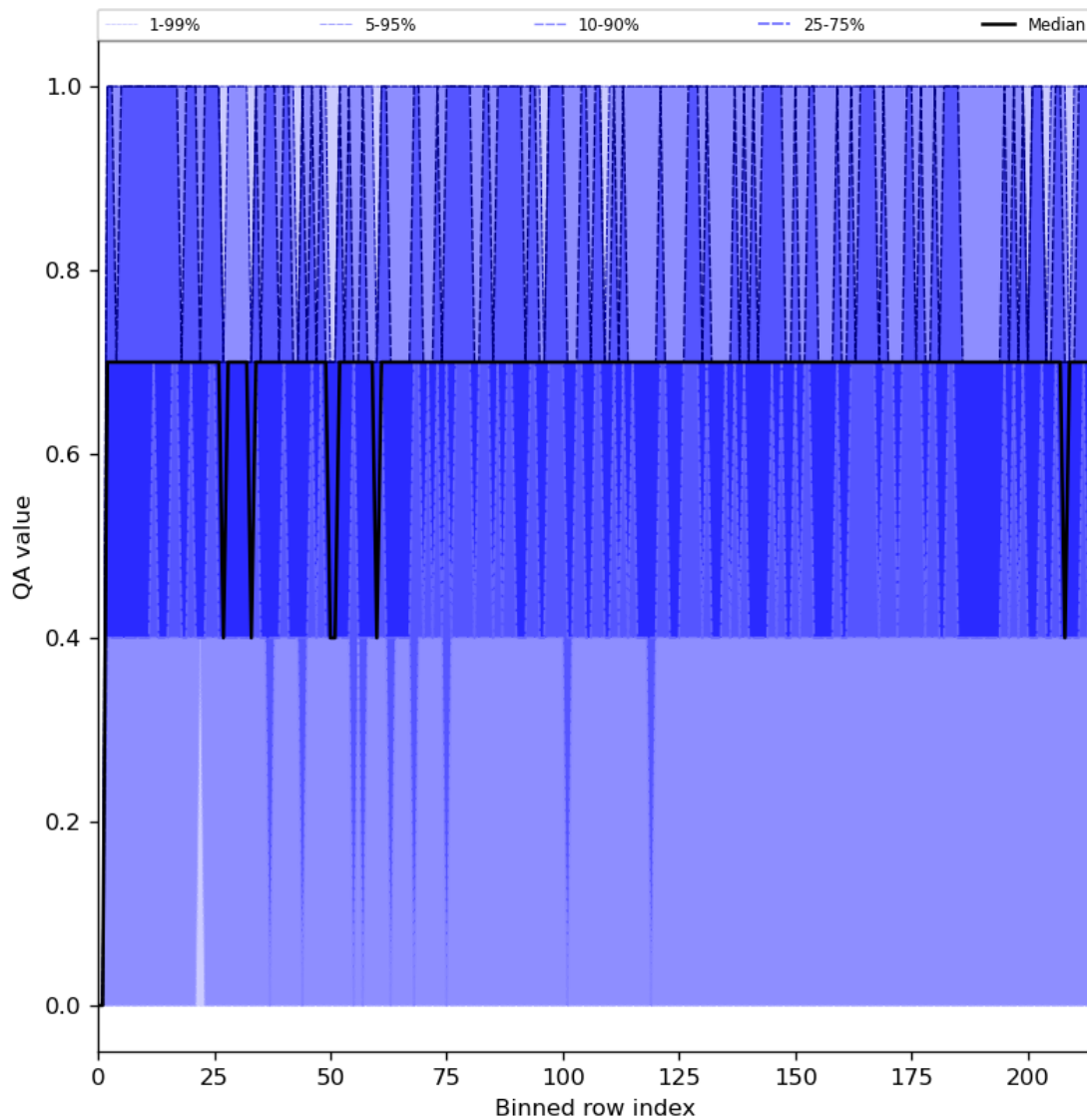
Figure 25: Along track statistics of “QA value” for 2024-05-09 to 2024-05-11
