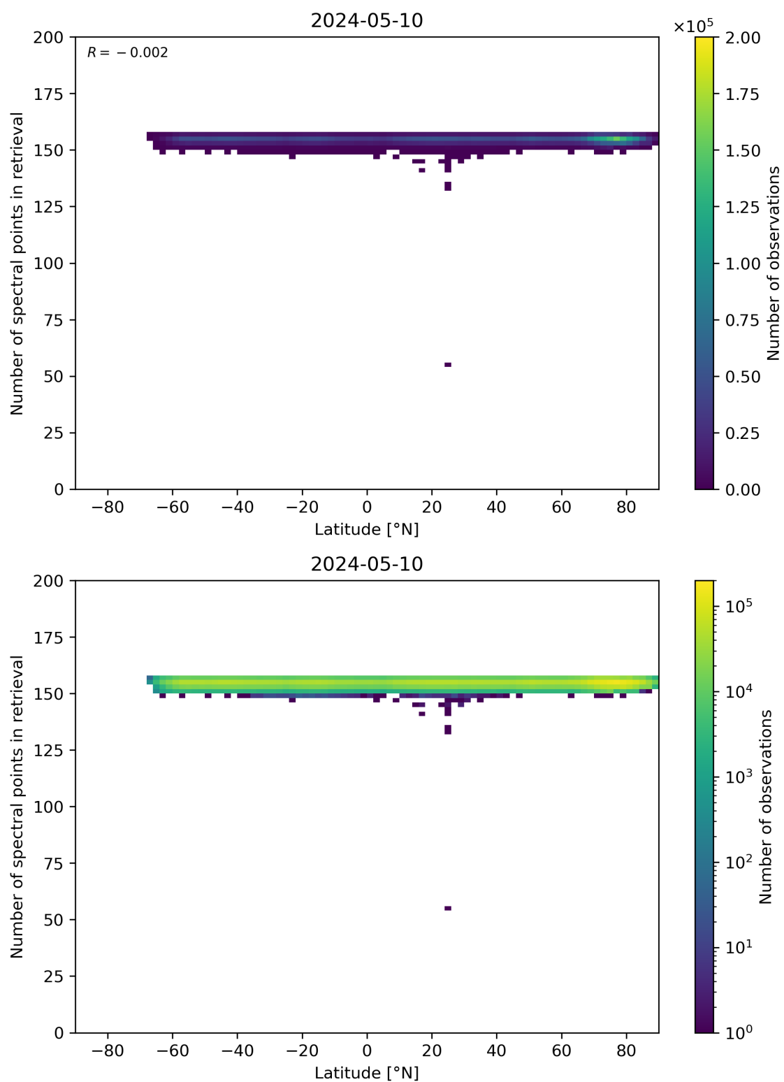
Figure 57: Scatter density plot of “Latitude” against “Number of spectral points in retrieval” for 2024-05-09 to 2024-05-11.
