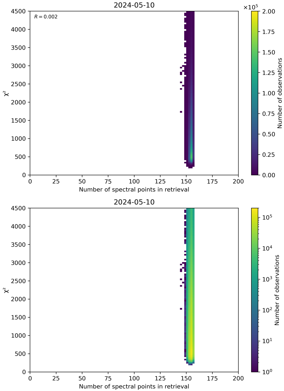
Figure 58: Scatter density plot of “Number of spectral points in retrieval” against “ \chi^2 ” for 2024-05-09 to 2024-05-11.
