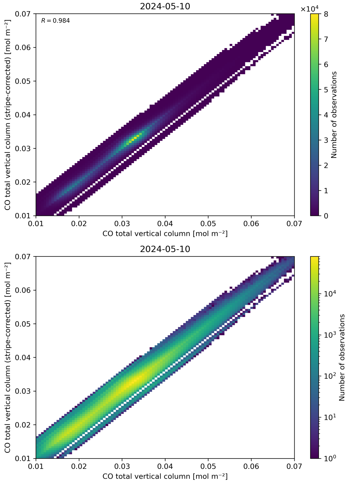
Figure 33: Scatter density plot of “CO total vertical column” against “CO total vertical column (stripe-corrected)” for 2024-05-09 to 2024-05-11.
