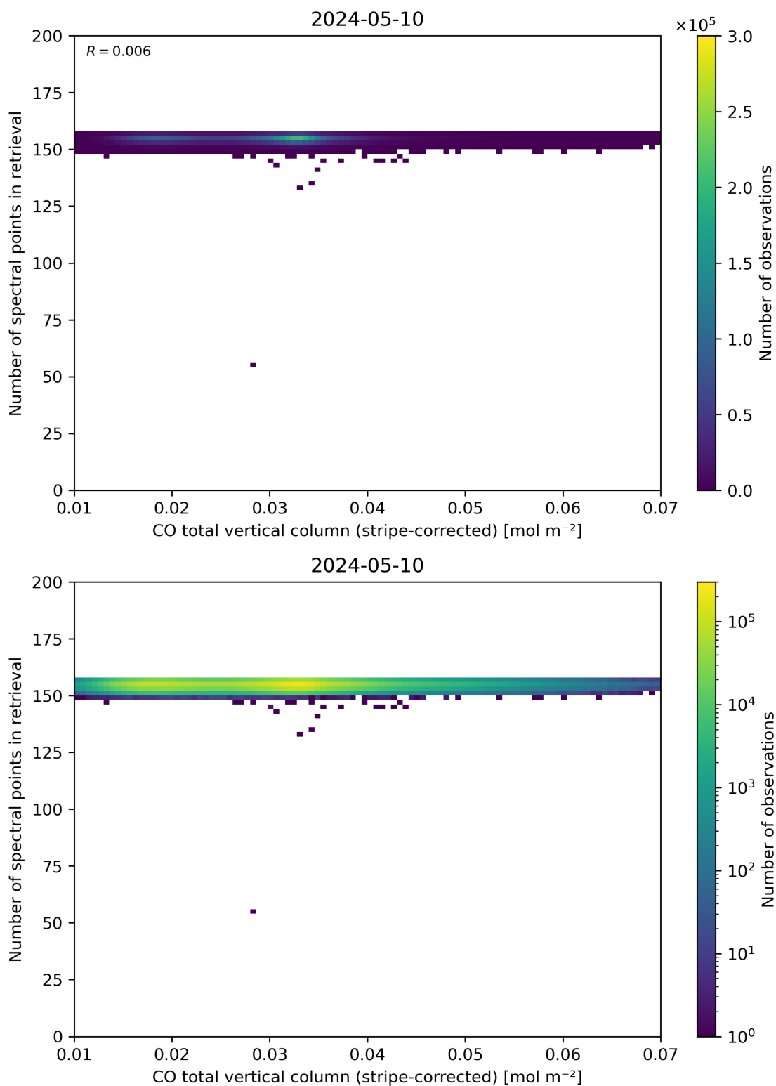
Figure 40: Scatter density plot of “CO total vertical column (stripe-corrected)” against “Number of spectral points in retrieval” for 2024-05-09 to 2024-05-11.
