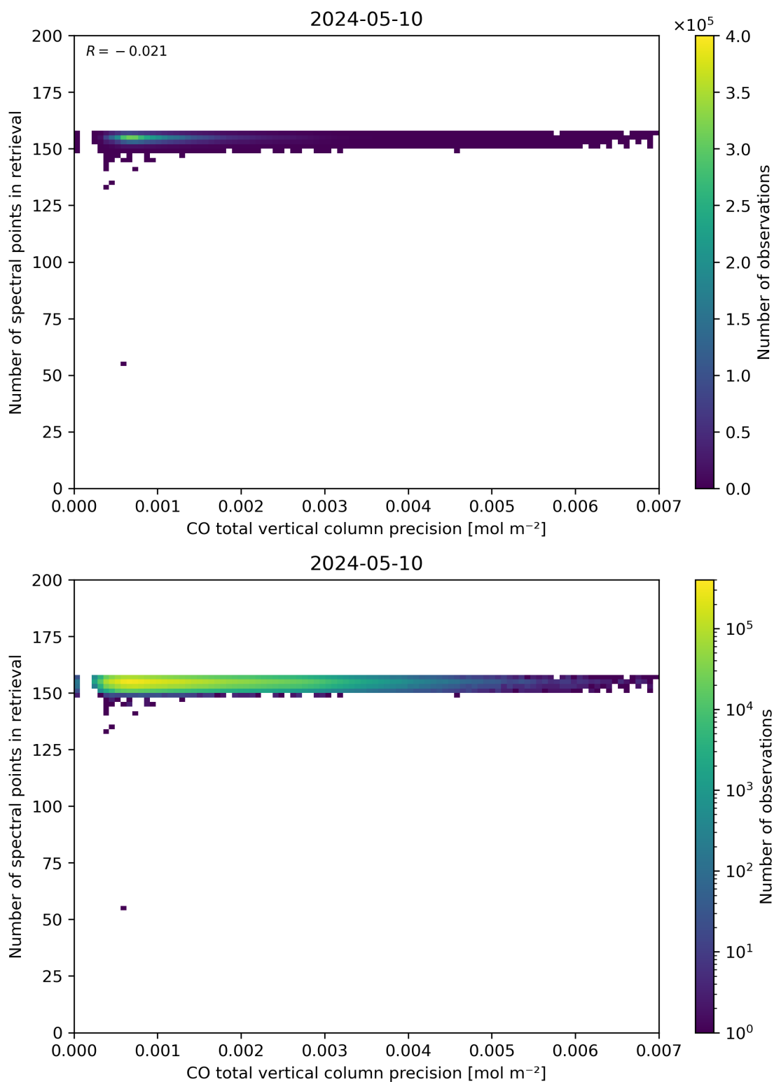
Figure 47: Scatter density plot of “CO total vertical column precision” against “Number of spectral points in retrieval” for 2024-05-09 to 2024-05-11.
