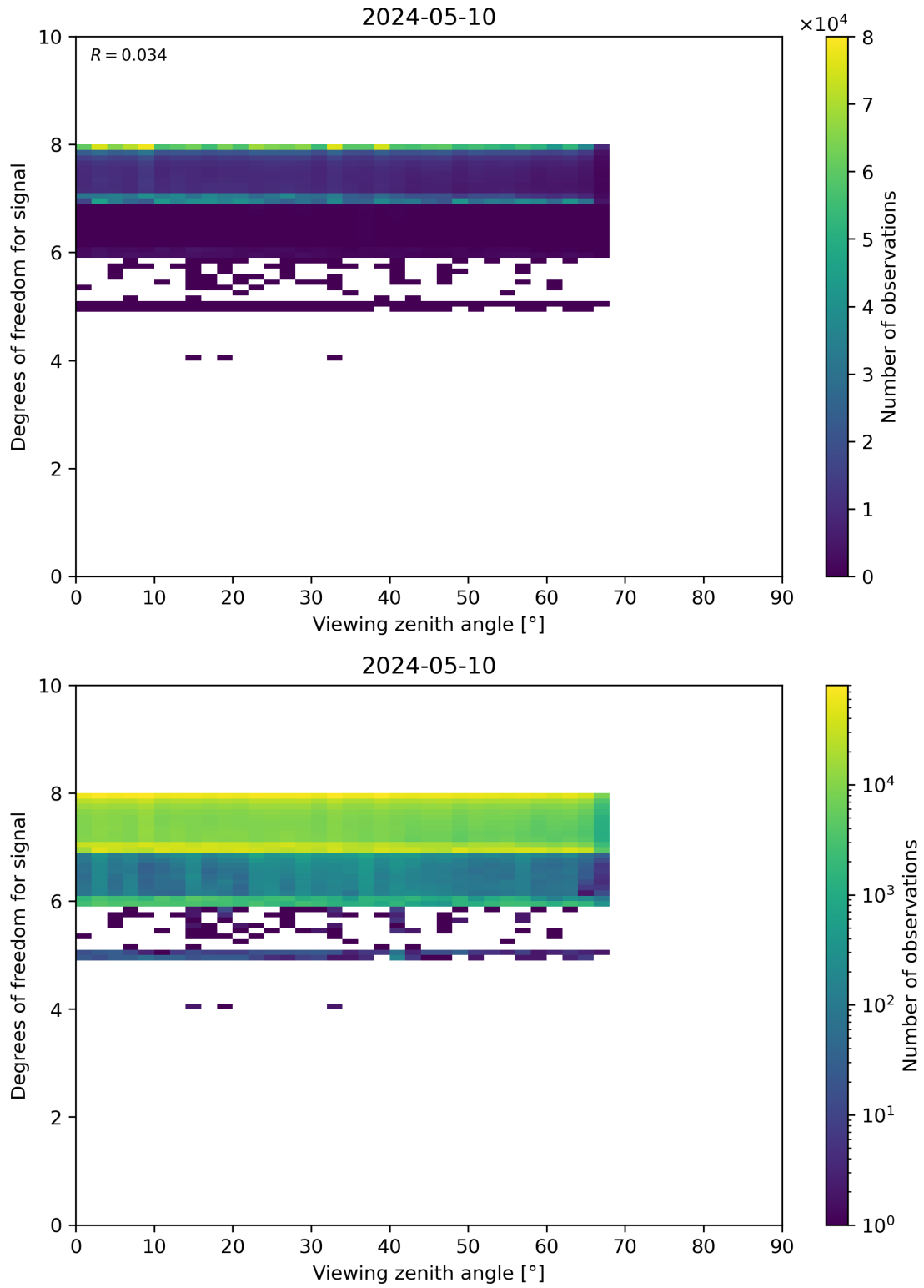
Figure 73: Scatter density plot of “Viewing zenith angle” against “Degrees of freedom for signal” for 2024-05-09 to 2024-05-11.
