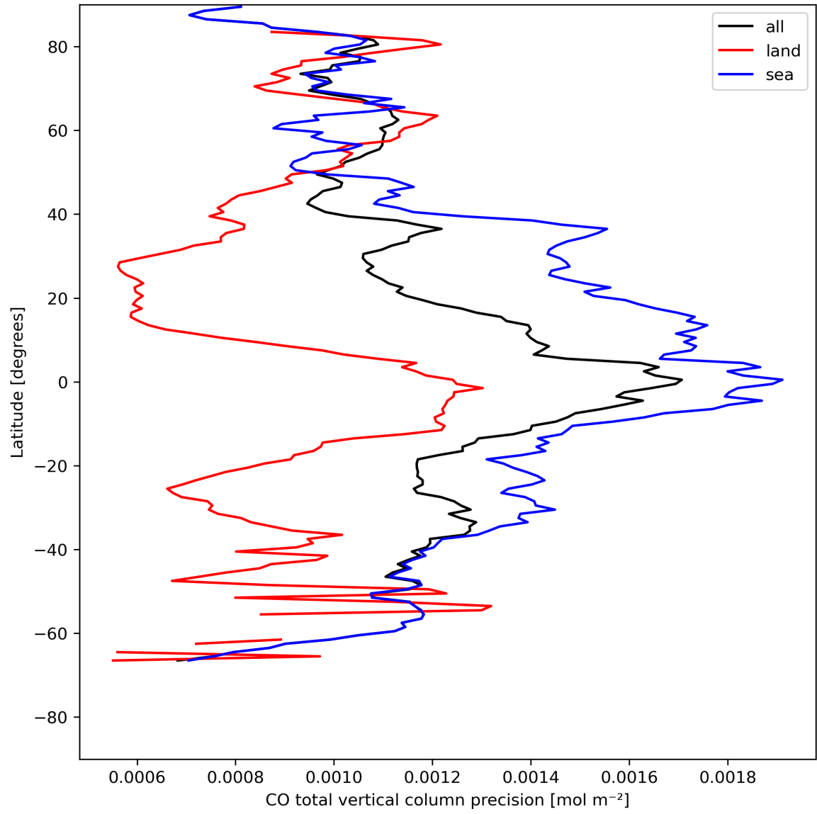
Figure 12: Zonal average of “CO total vertical column precision” for 2024-05-09 to 2024-05-11.
