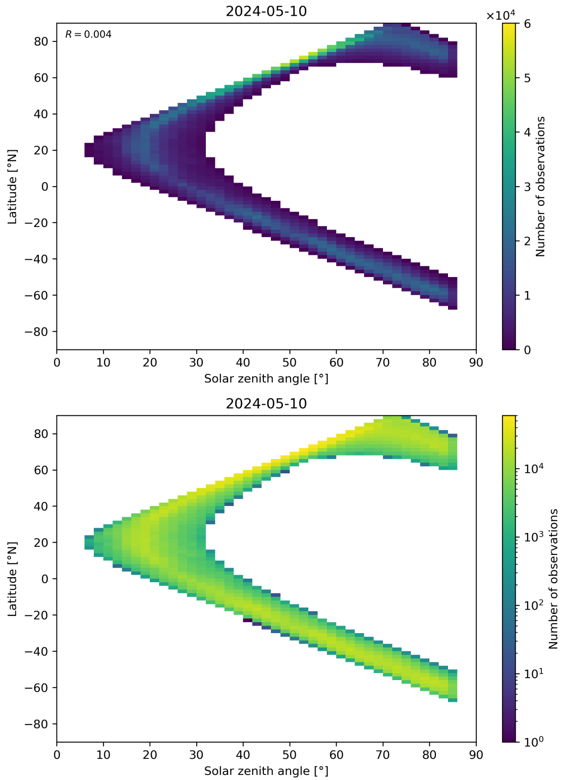
Figure 66: Scatter density plot of “Solar zenith angle” against “Latitude” for 2024-05-09 to 2024-05-11.
