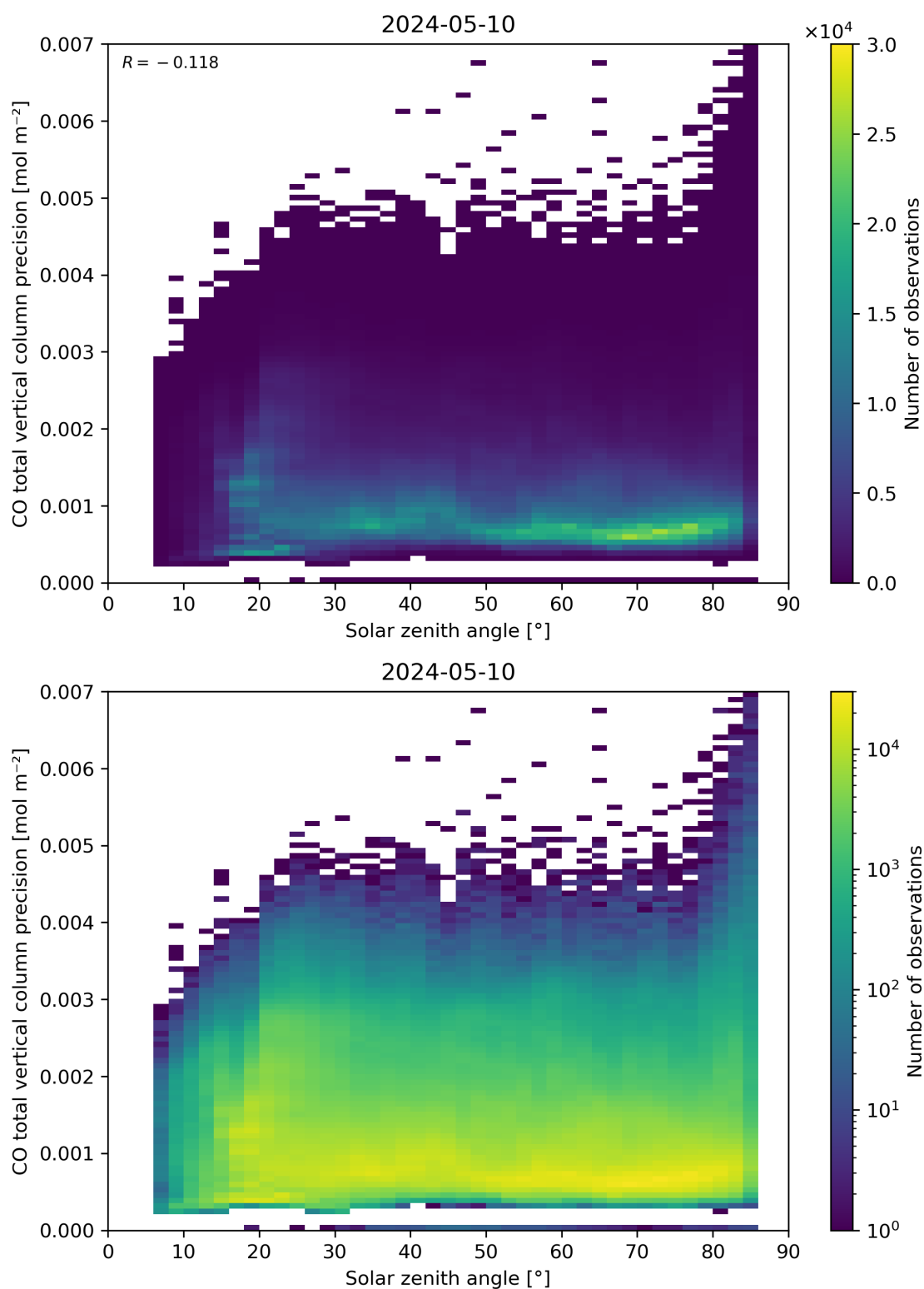
Figure 63: Scatter density plot of “Solar zenith angle” against “CO total vertical column precision” for 2024-05-09 to 2024-05-11.
