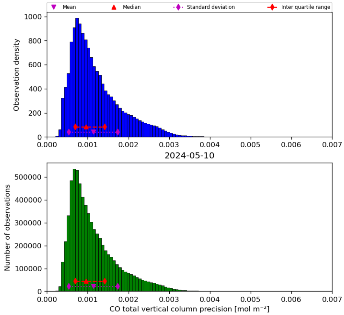
Figure 20: Histogram of “CO total vertical column precision” for 2024-05-09 to 2024-05-11
