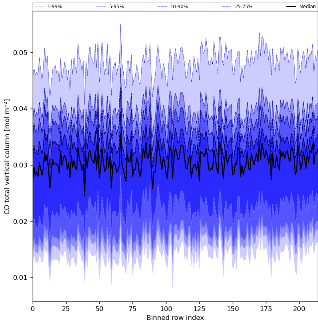
Figure 26: Along track statistics of “CO total vertical column” for 2024-05-09 to 2024-05-11
