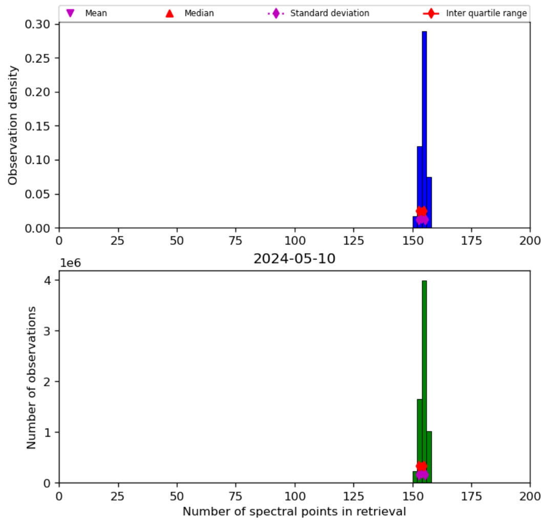
Figure 21: Histogram of “Number of spectral points in retrieval” for 2024-05-09 to 2024-05-11
