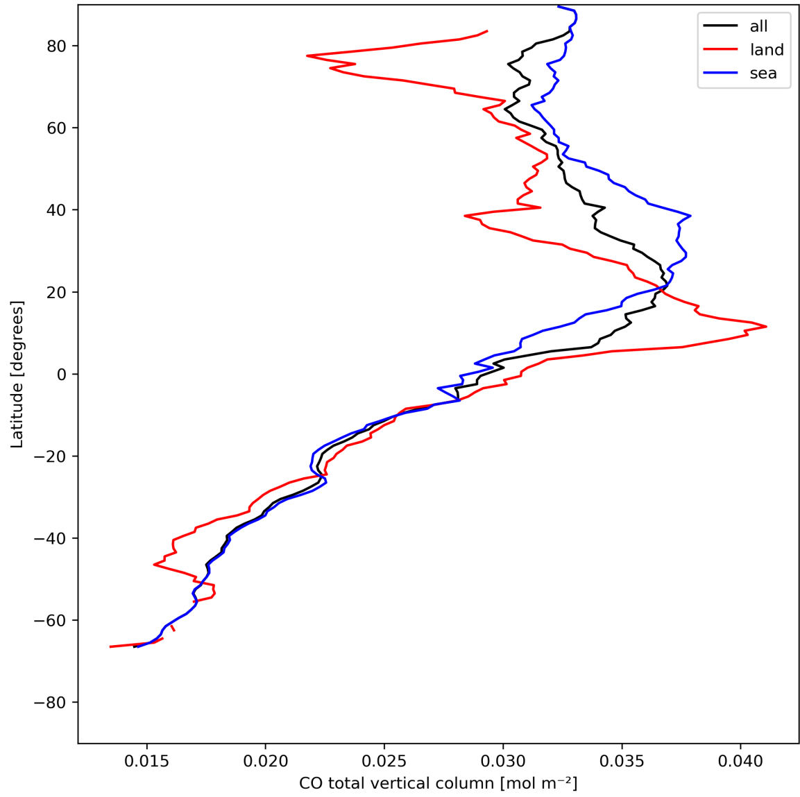
Figure 10: Zonal average of “CO total vertical column” for 2024-05-09 to 2024-05-11.
