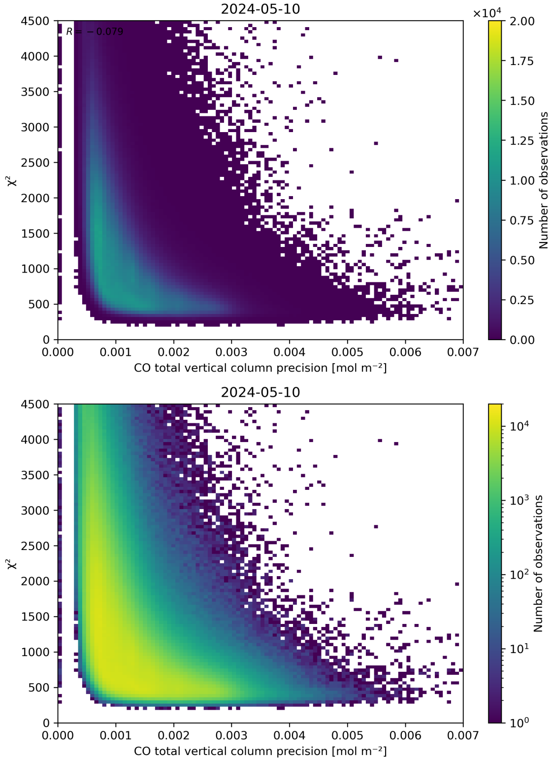
Figure 44: Scatter density plot of “CO total vertical column precision” against “ \chi^2 ” for 2024-05-09 to 2024-05-11.
