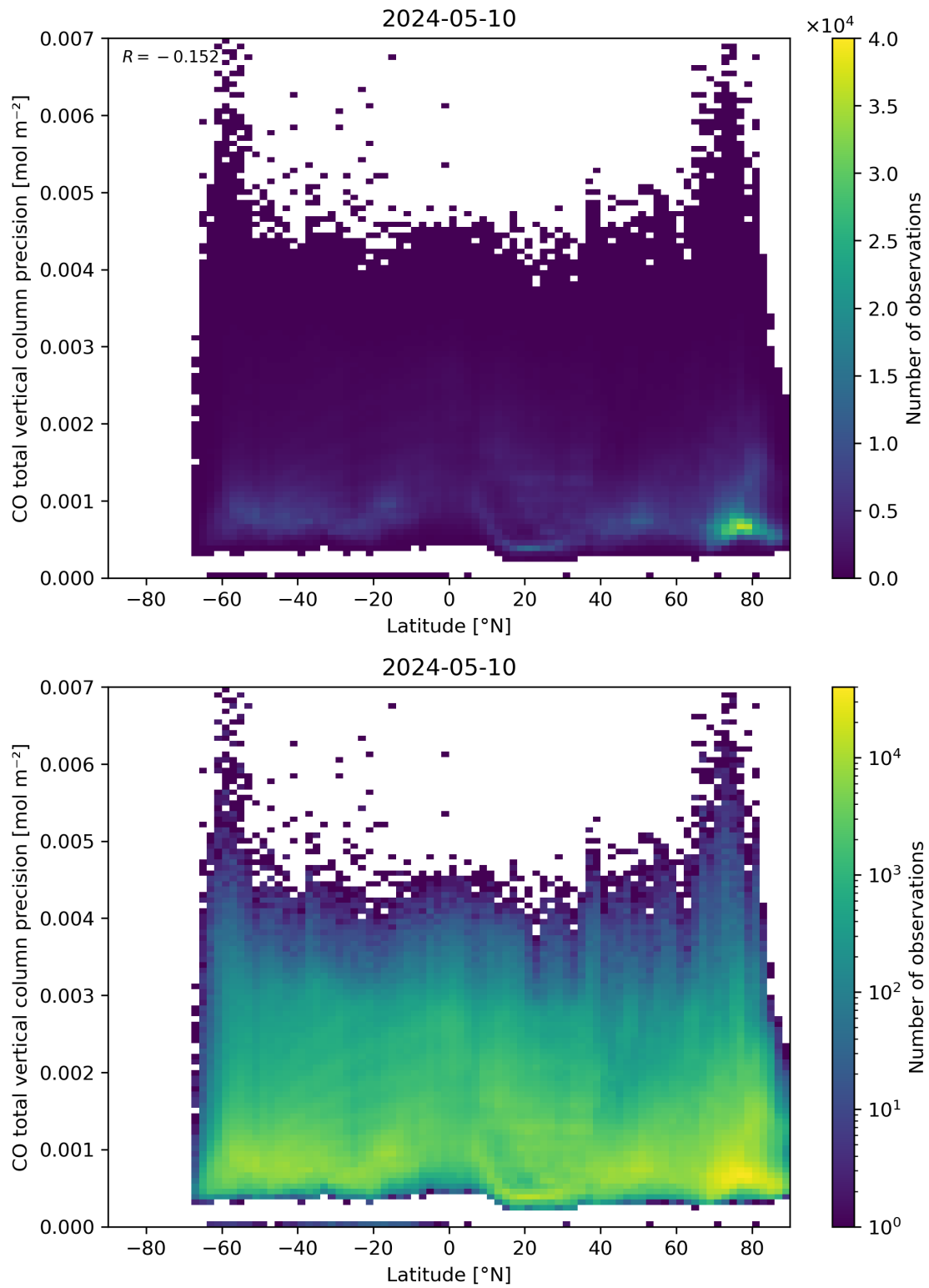
Figure 53: Scatter density plot of “Latitude” against “CO total vertical column precision” for 2024-05-09 to 2024-05-11.
