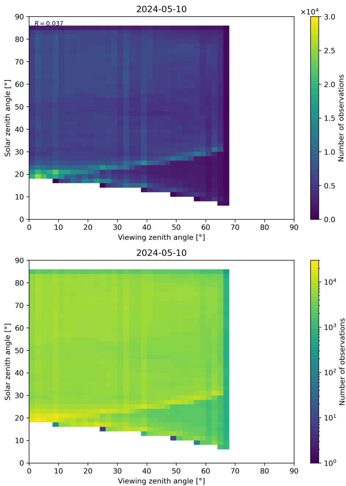
Figure 77: Scatter density plot of “Viewing zenith angle” against “Solar zenith angle” for 2024-05-09 to 2024-05-11.
