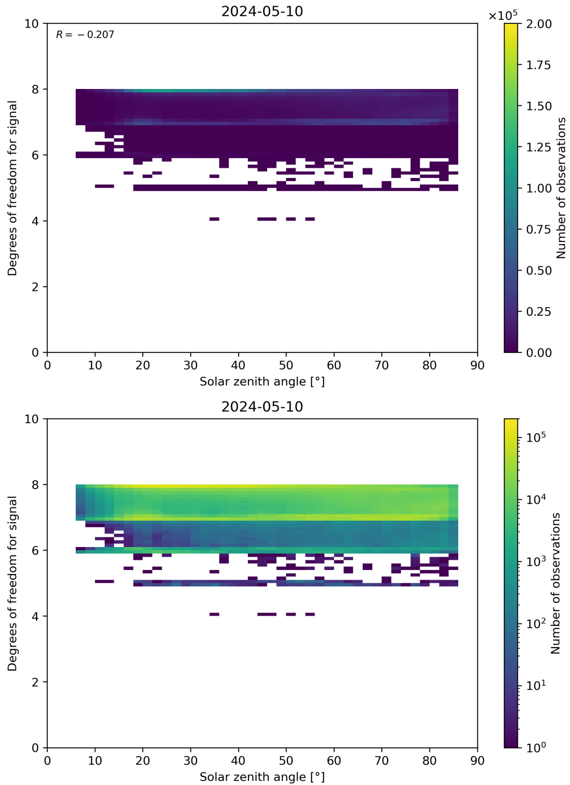
Figure 65: Scatter density plot of “Solar zenith angle” against “Degrees of freedom for signal” for 2024-05-09 to 2024-05-11.
