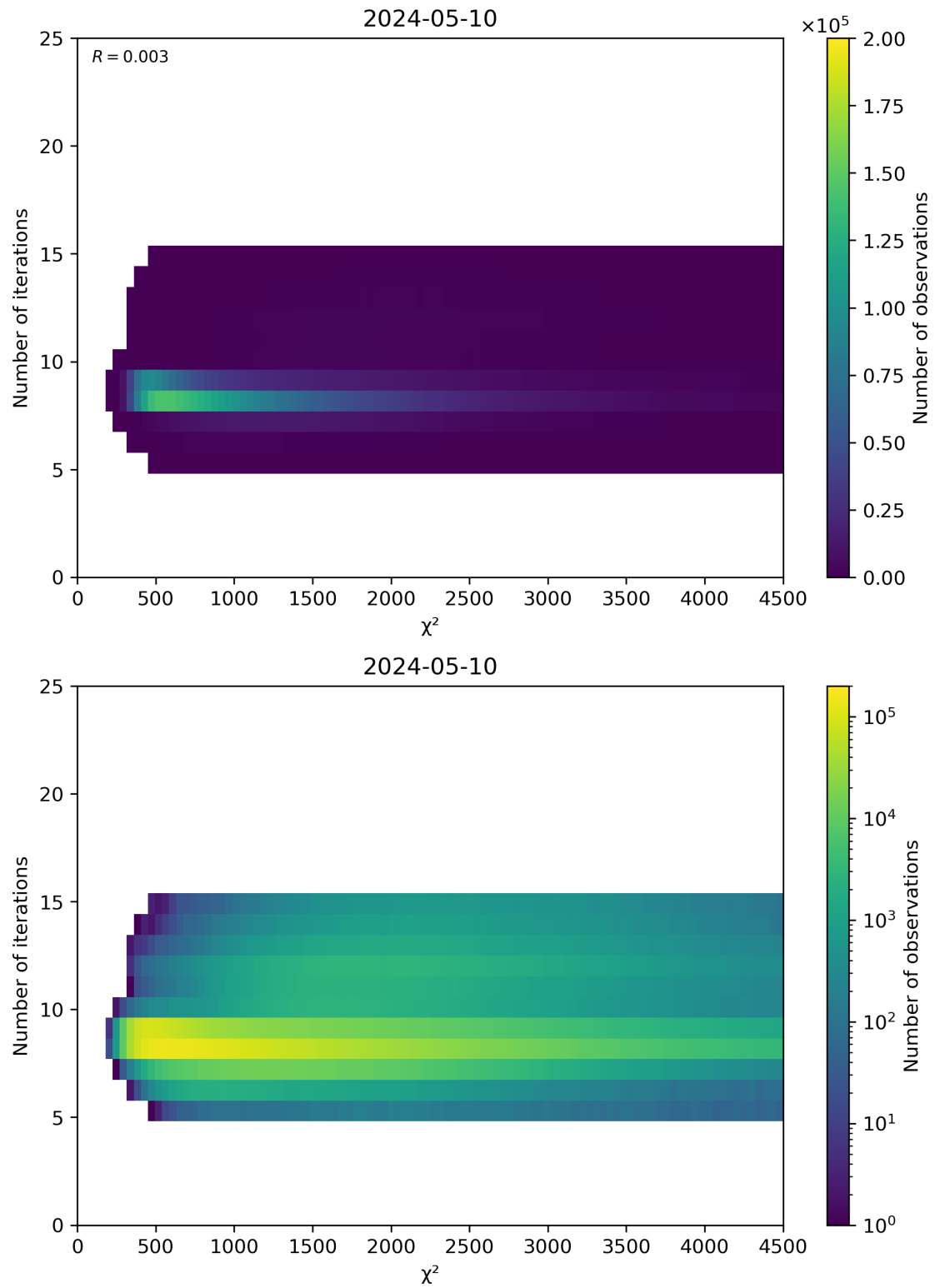
Figure 49: Scatter density plot of “ \chi^2 ” against “Number of iterations” for 2024-05-09 to 2024-05-11.
