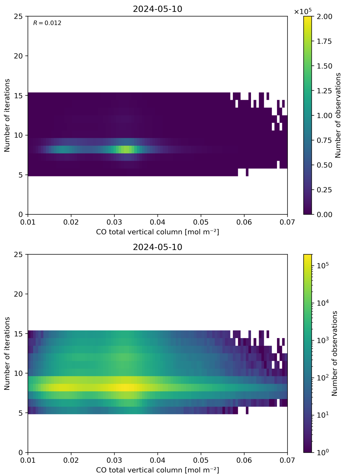
Figure 42: Scatter density plot of “CO total vertical column” against “Number of iterations” for 2024-05-09 to 2024-05-11.
