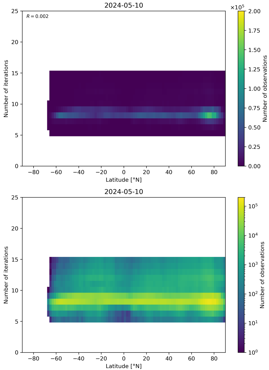
Figure 56: Scatter density plot of “Latitude” against “Number of iterations” for 2024-05-09 to 2024-05-11.
