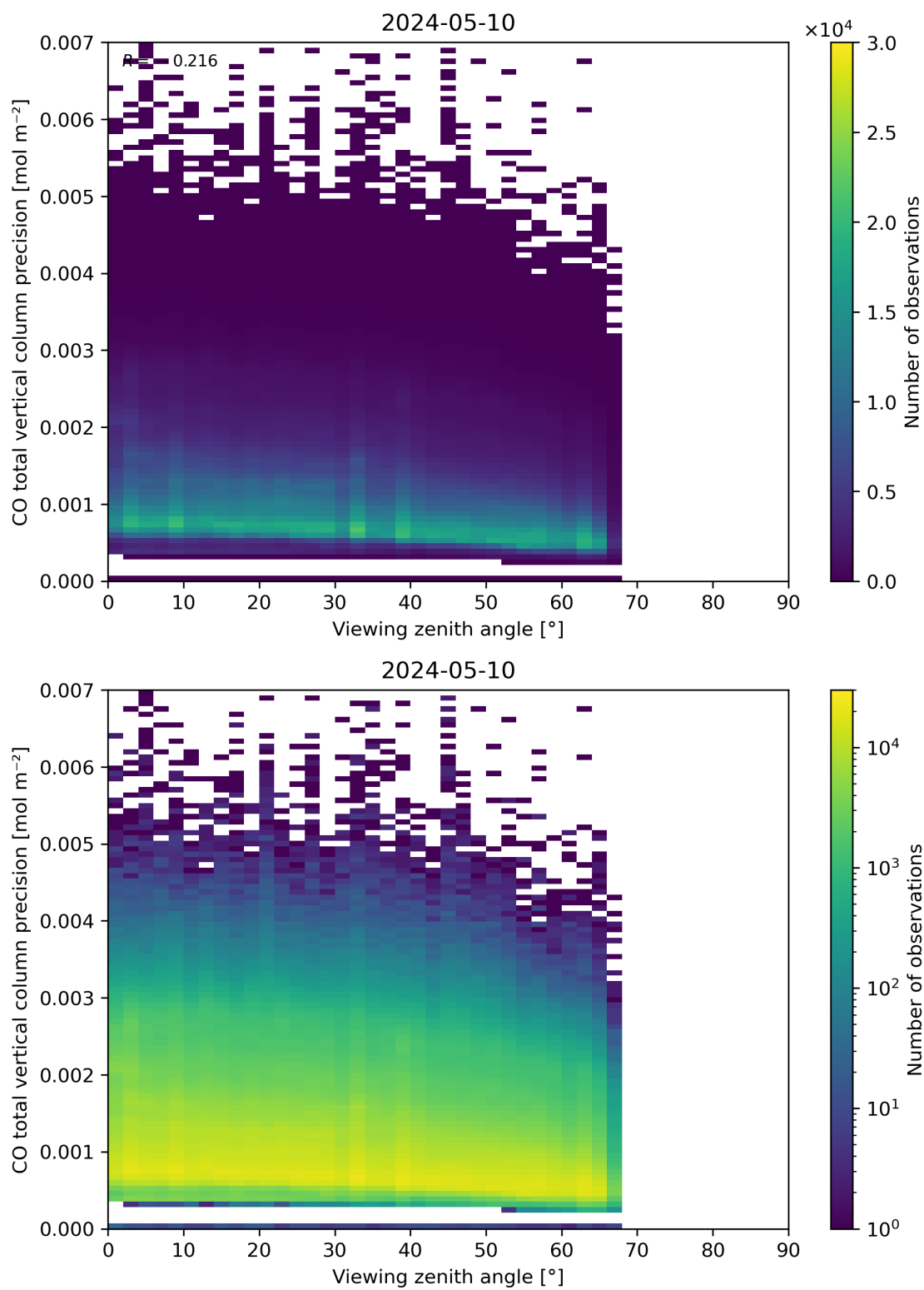
Figure 71: Scatter density plot of “Viewing zenith angle” against “CO total vertical column precision” for 2024-05-09 to 2024-05-11.
