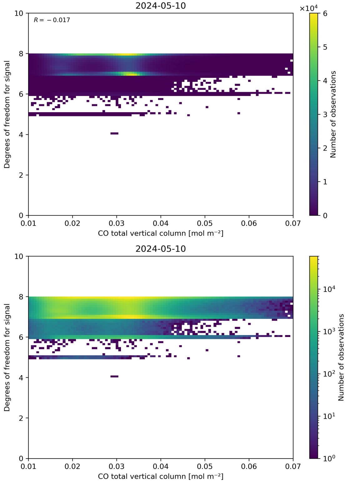
Figure 41: Scatter density plot of “CO total vertical column” against “Degrees of freedom for signal” for 2024-05-09 to 2024-05-11.
