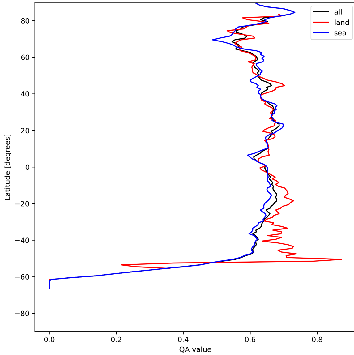
Figure 9: Zonal average of “QA value” for 2024-05-09 to 2024-05-11.
