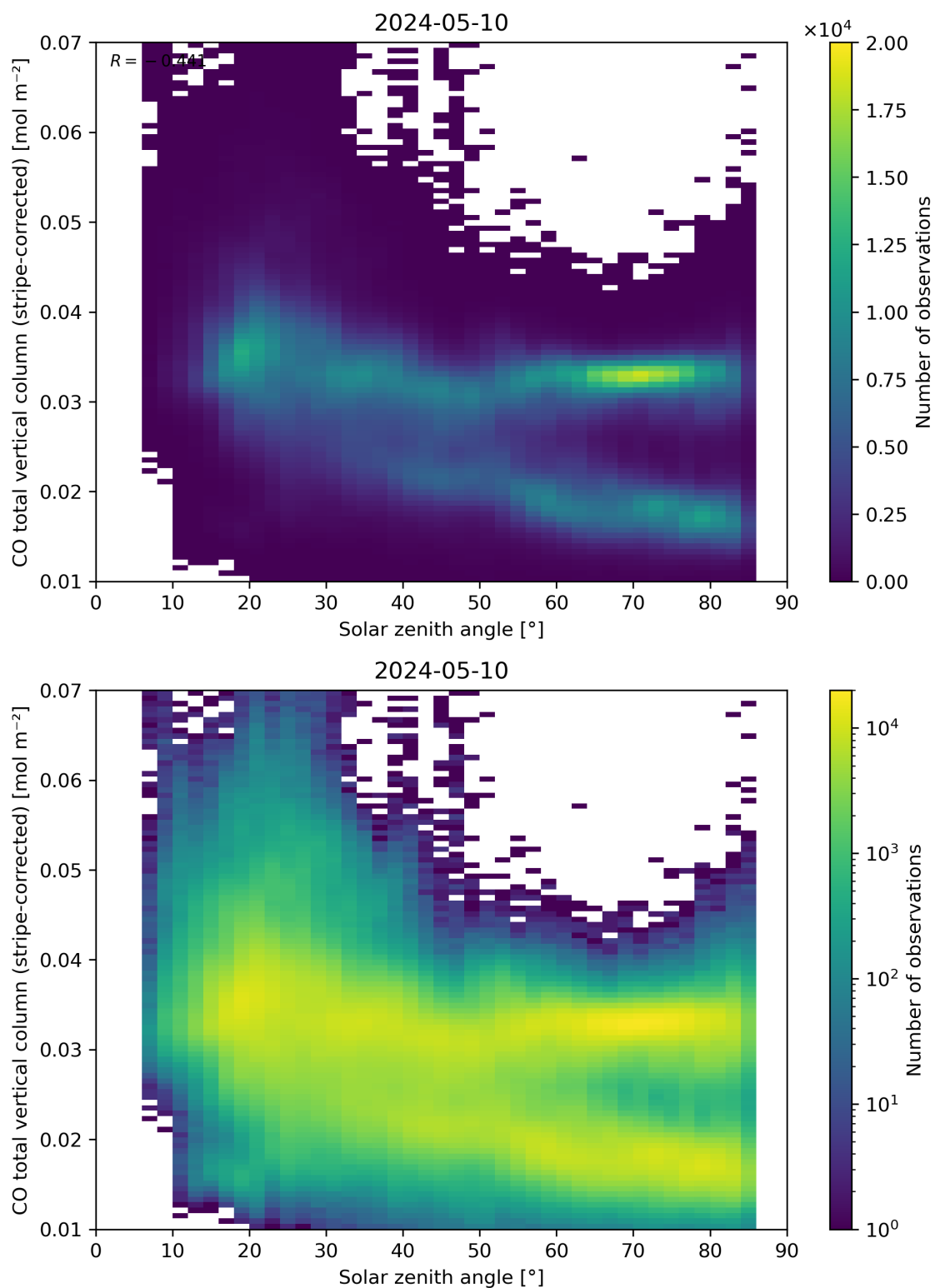
Figure 62: Scatter density plot of “Solar zenith angle” against “CO total vertical column (stripe-corrected)” for 2024-05-09 to 2024-05-11.
