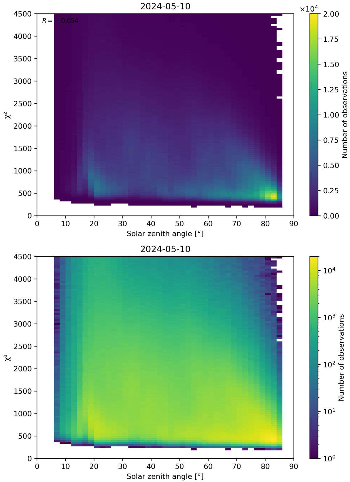
Figure 64: Scatter density plot of “Solar zenith angle” against “ \chi^2 ” for 2024-05-09 to 2024-05-11.
