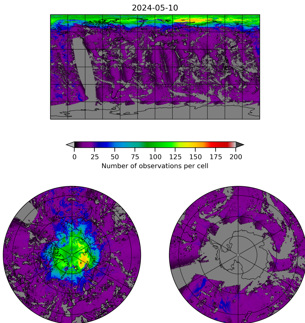
Figure 8: Map of the number of observations for 2024-05-09 to 2024-05-11
