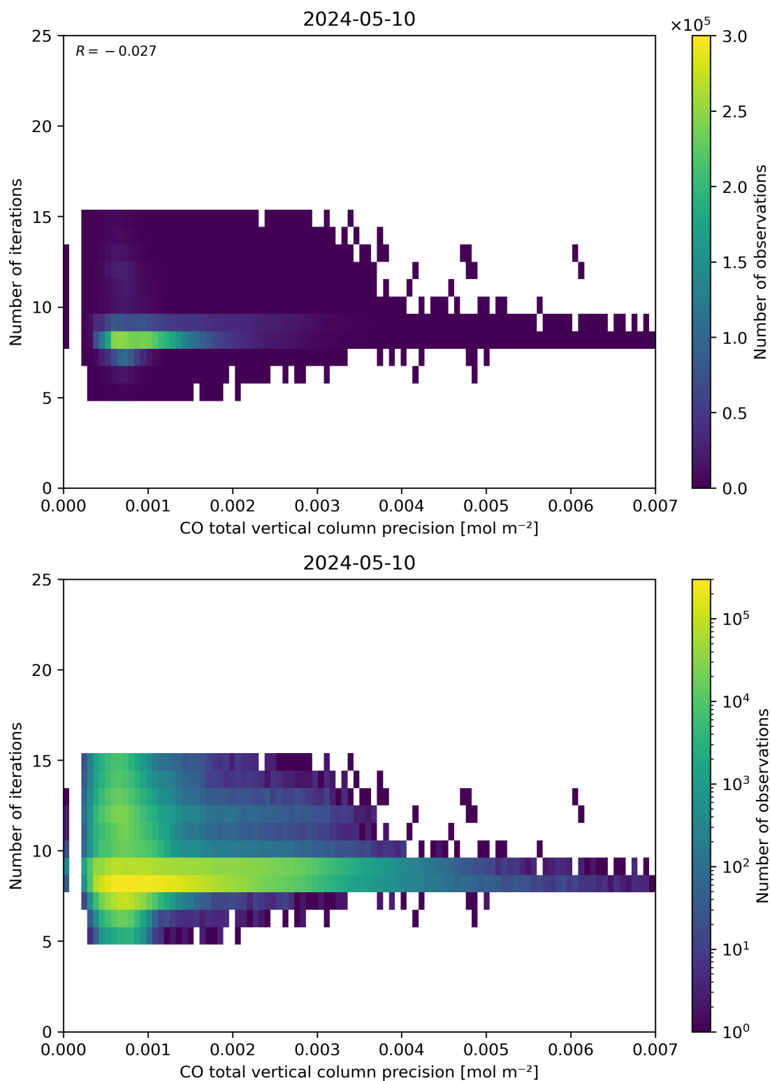
Figure 46: Scatter density plot of “CO total vertical column precision” against “Number of iterations” for 2024-05-09 to 2024-05-11.
