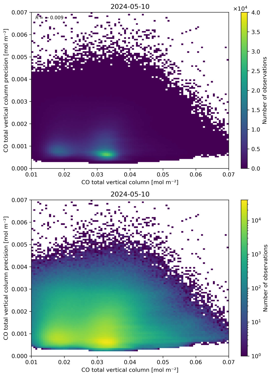
Figure 34: Scatter density plot of “CO total vertical column” against “CO total vertical column precision” for 2024-05-09 to 2024-05-11.
