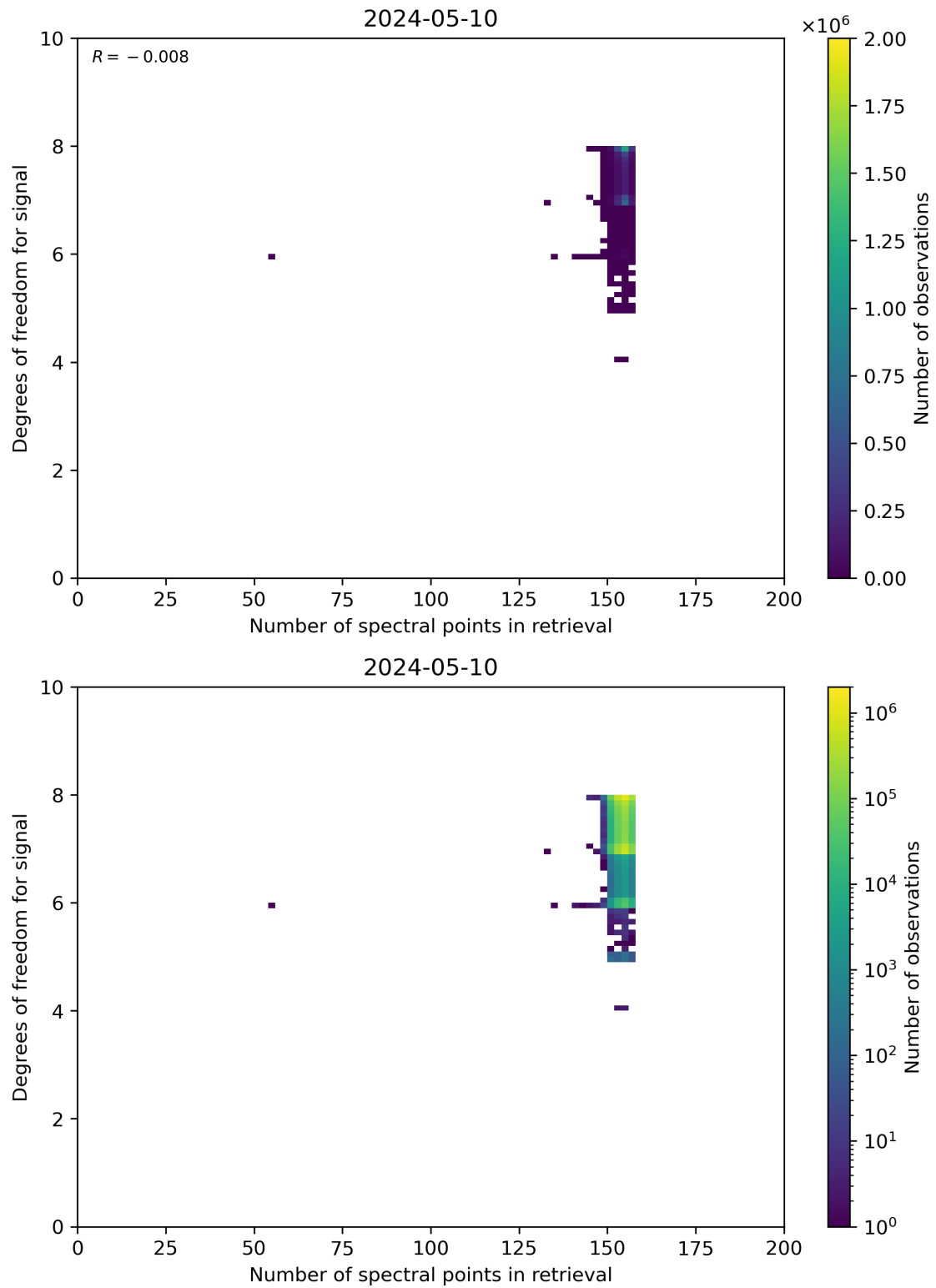
Figure 59: Scatter density plot of “Number of spectral points in retrieval” against “Degrees of freedom for signal” for 2024-05-09 to 2024-05-11.
