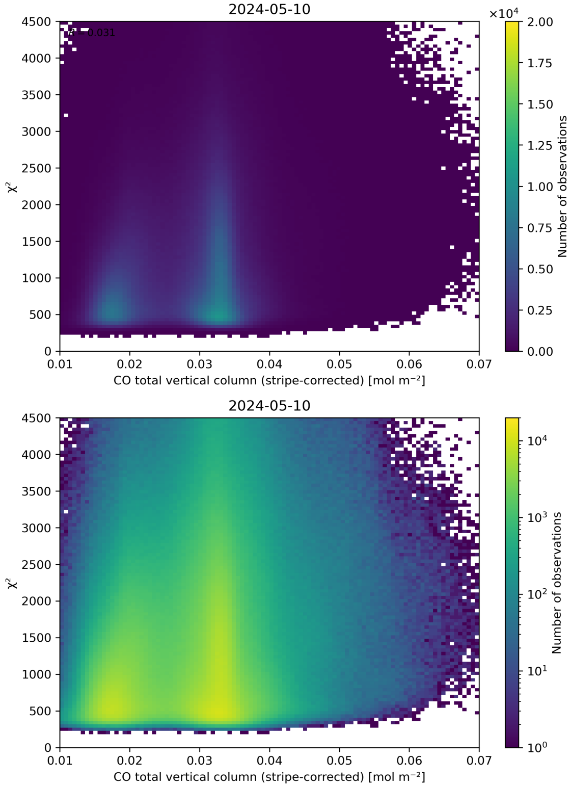
Figure 37: Scatter density plot of “CO total vertical column (stripe-corrected)” against “ \chi^2 ” for 2024-05-09 to 2024-05-11.
