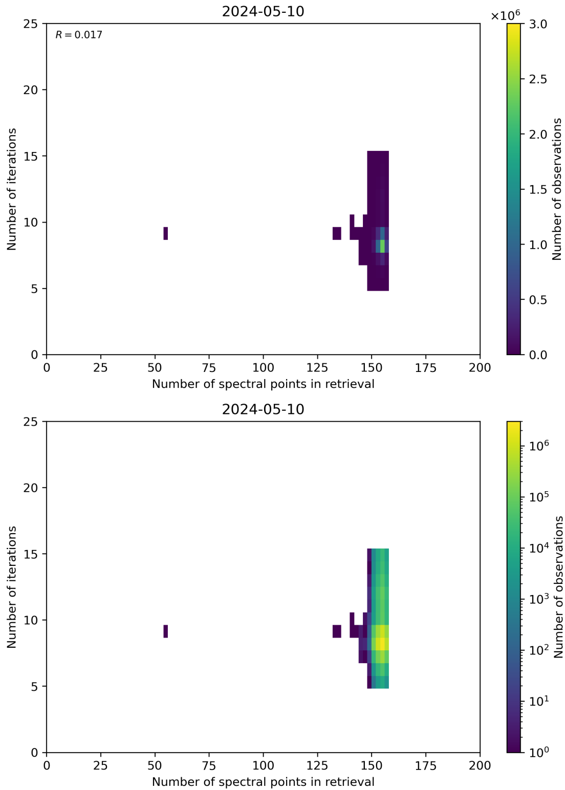
Figure 60: Scatter density plot of “Number of spectral points in retrieval” against “Number of iterations” for 2024-05-09 to 2024-05-11.
