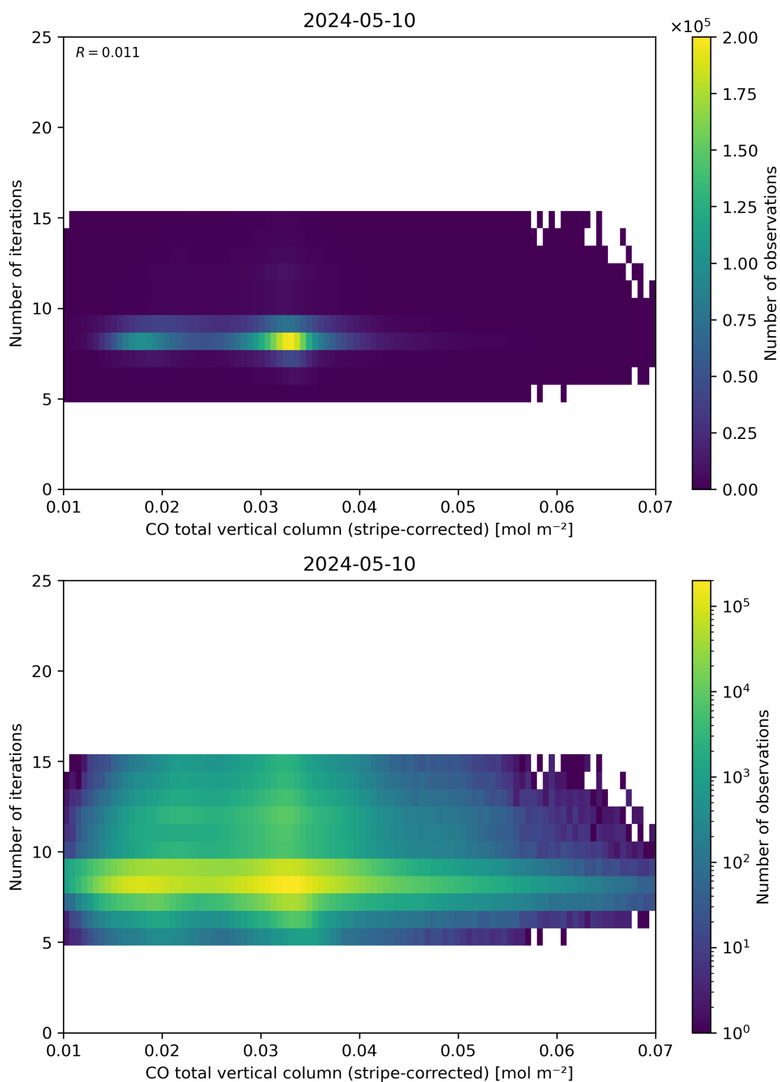
Figure 39: Scatter density plot of “CO total vertical column (stripe-corrected)” against “Number of iterations” for 2024-05-09 to 2024-05-11.
