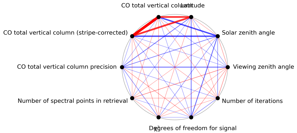
Figure 1: Map of correlation graph for 2024-05-09 to 2024-05-11.
