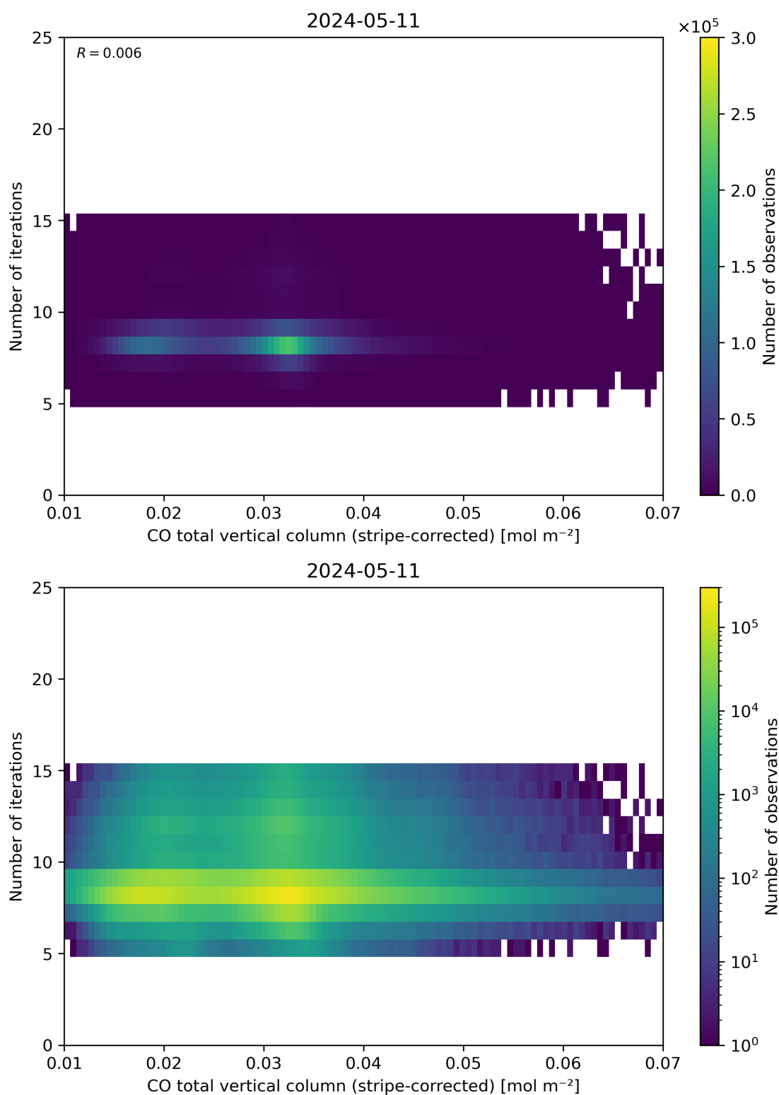
Figure 39: Scatter density plot of “CO total vertical column (stripe-corrected)” against “Number of iterations” for 2024-05-10 to 2024-05-12.
