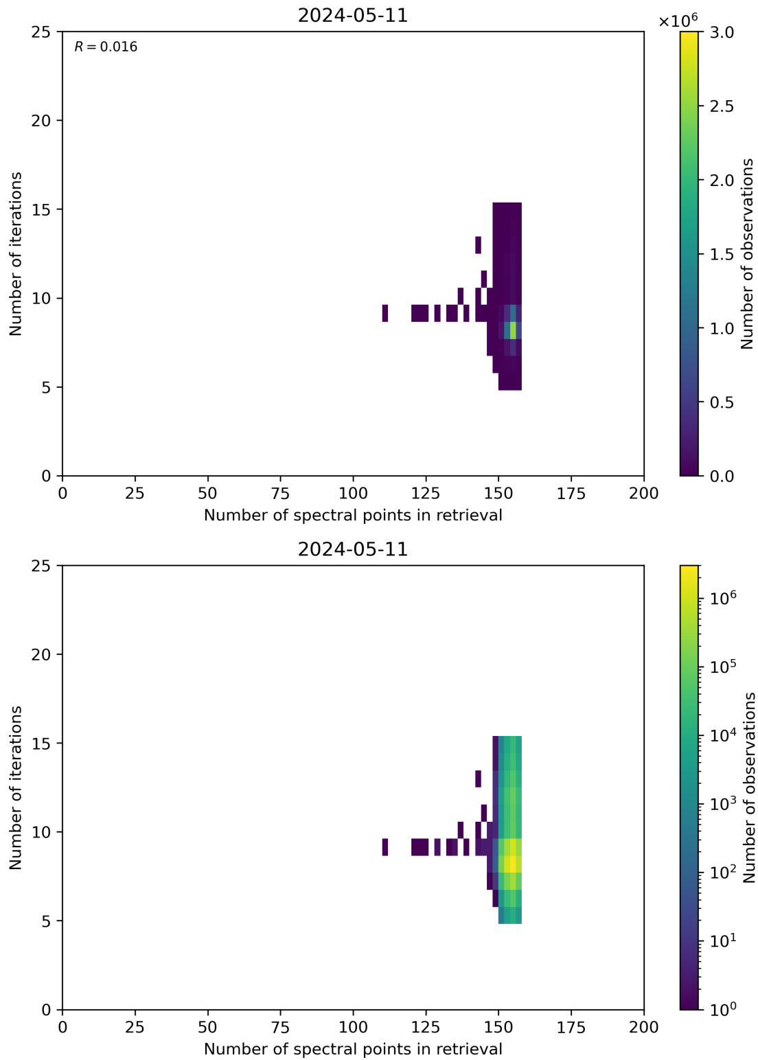
Figure 60: Scatter density plot of “Number of spectral points in retrieval” against “Number of iterations” for 2024-05-10 to 2024-05-12.
