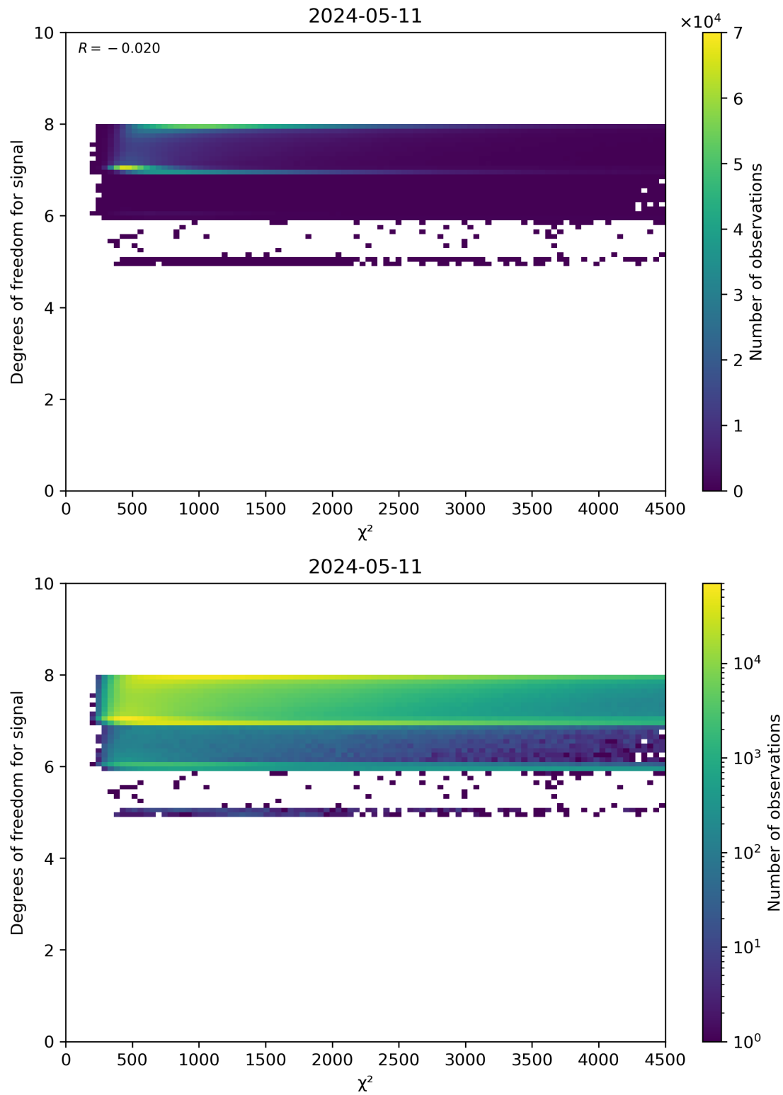
Figure 48: Scatter density plot of “ \chi^2 ” against “Degrees of freedom for signal” for 2024-05-10 to 2024-05-12.
