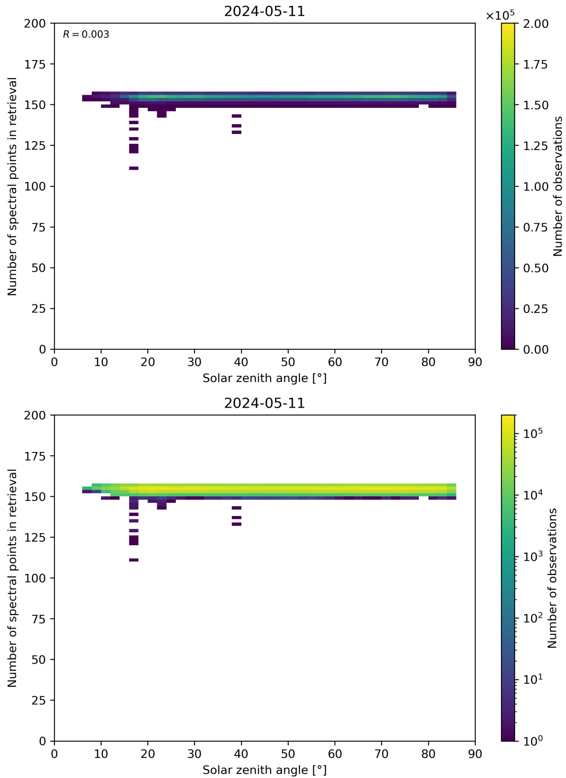
Figure 68: Scatter density plot of “Solar zenith angle” against “Number of spectral points in retrieval” for 2024-05-10 to 2024-05-12.
