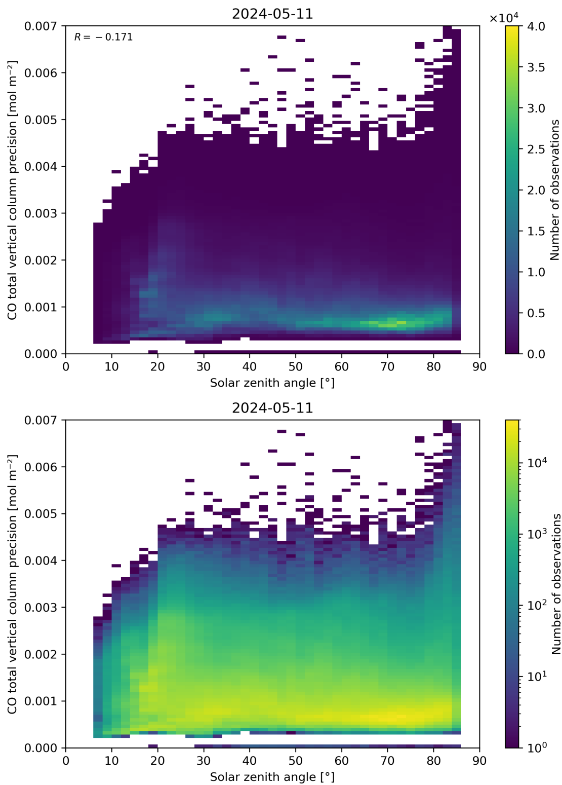
Figure 63: Scatter density plot of “Solar zenith angle” against “CO total vertical column precision” for 2024-05-10 to 2024-05-12.
