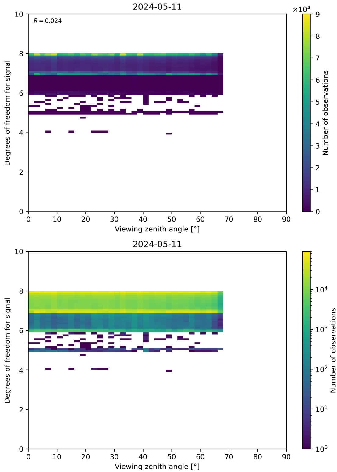
Figure 73: Scatter density plot of “Viewing zenith angle” against “Degrees of freedom for signal” for 2024-05-10 to 2024-05-12.
