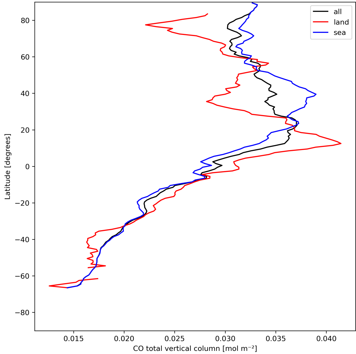
Figure 10: Zonal average of “CO total vertical column” for 2024-05-10 to 2024-05-12.
