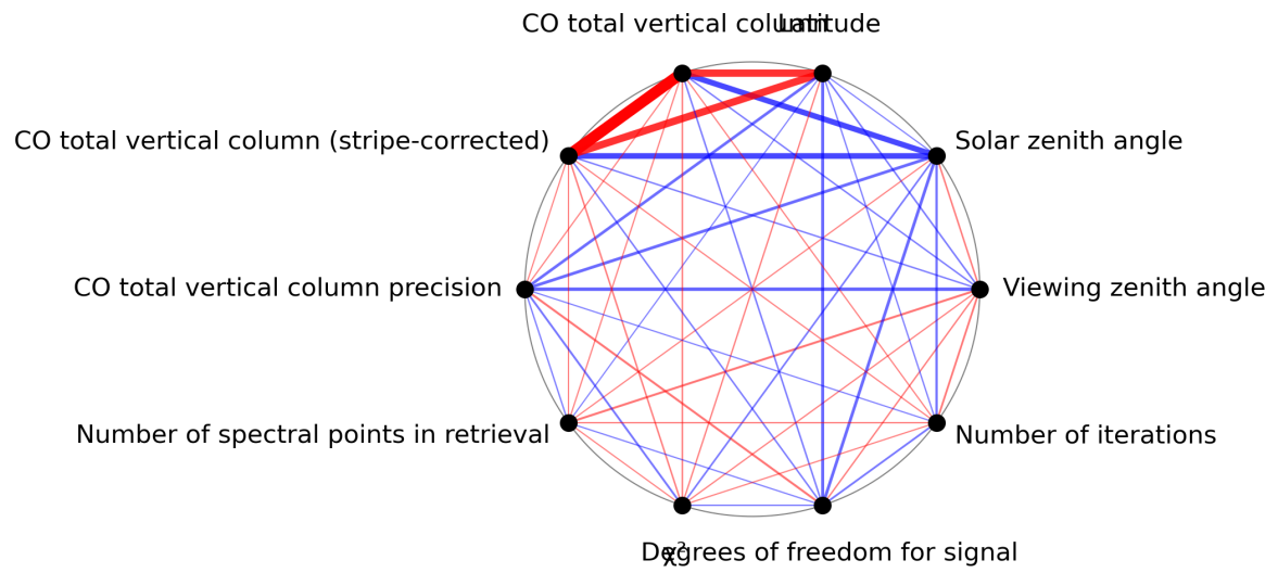
Figure 1: Map of correlation graph for 2024-05-10 to 2024-05-12.
