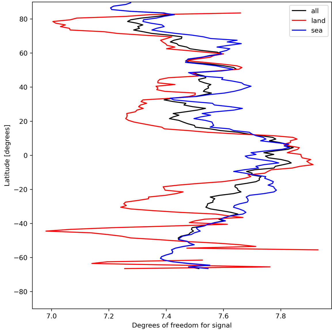
Figure 15: Zonal average of “Degrees of freedom for signal” for 2024-05-10 to 2024-05-12.
