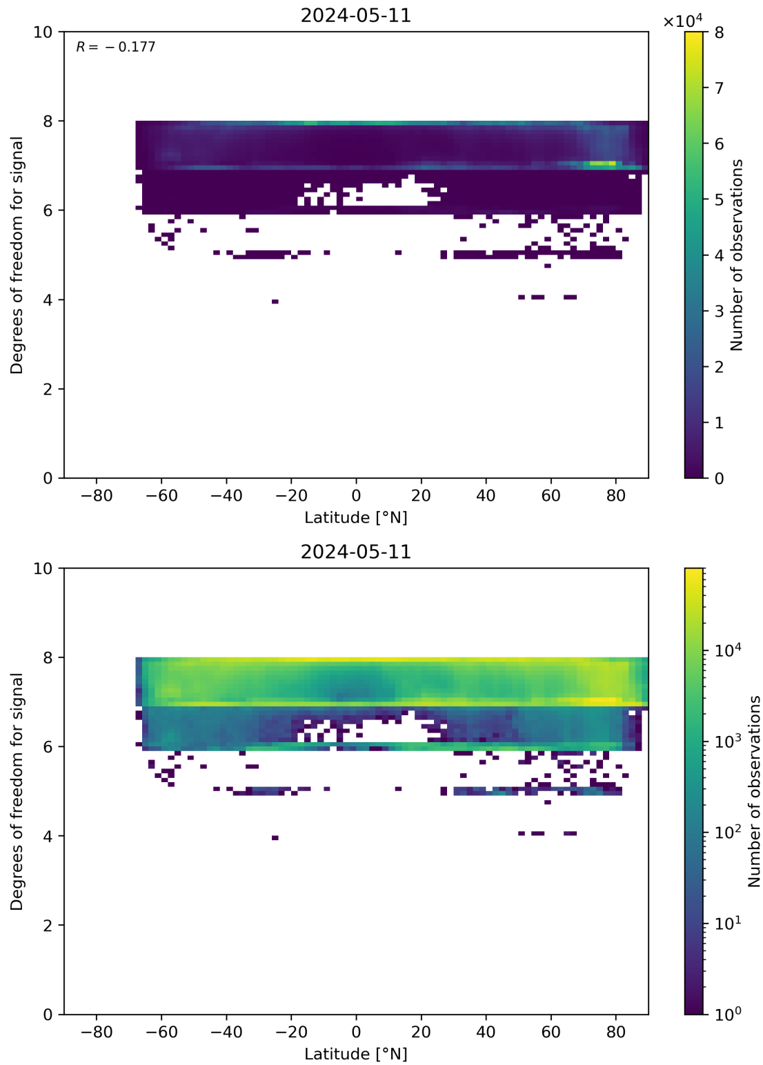
Figure 55: Scatter density plot of “Latitude” against “Degrees of freedom for signal” for 2024-05-10 to 2024-05-12.
