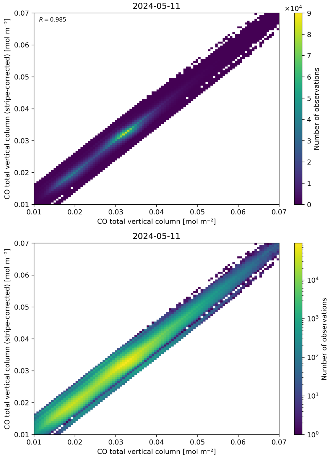
Figure 33: Scatter density plot of “CO total vertical column” against “CO total vertical column (stripe-corrected)” for 2024-05-10 to 2024-05-12.
