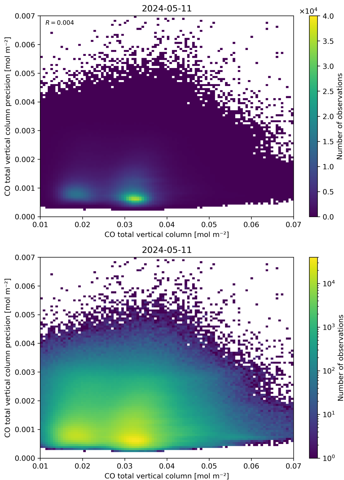
Figure 34: Scatter density plot of “CO total vertical column” against “CO total vertical column precision” for 2024-05-10 to 2024-05-12.
