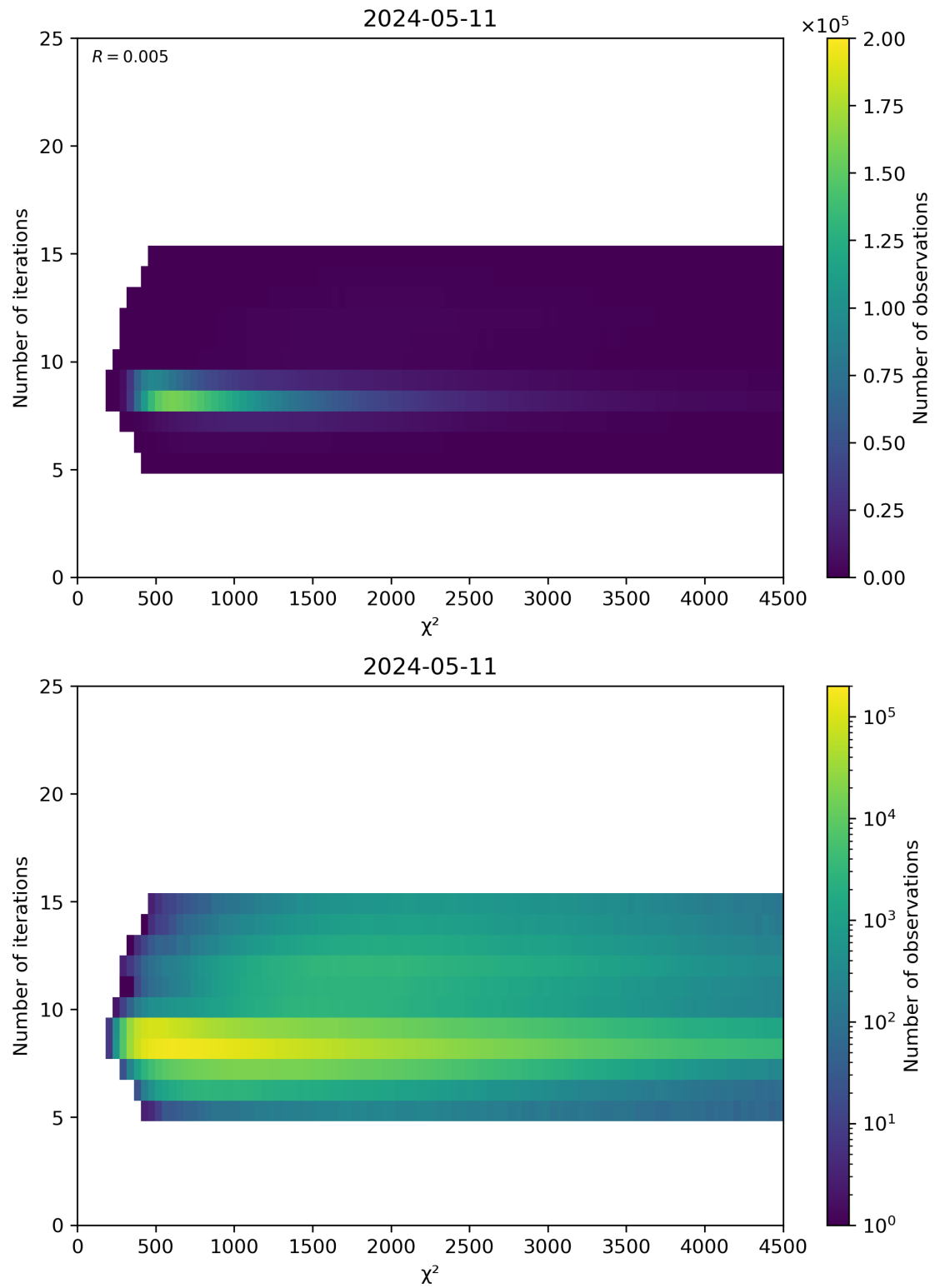
Figure 49: Scatter density plot of “ \chi^2 ” against “Number of iterations” for 2024-05-10 to 2024-05-12.
