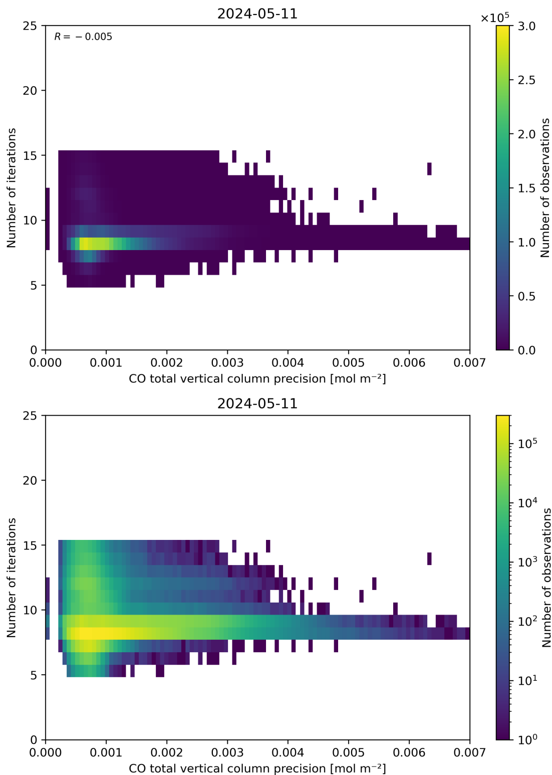
Figure 46: Scatter density plot of “CO total vertical column precision” against “Number of iterations” for 2024-05-10 to 2024-05-12.
