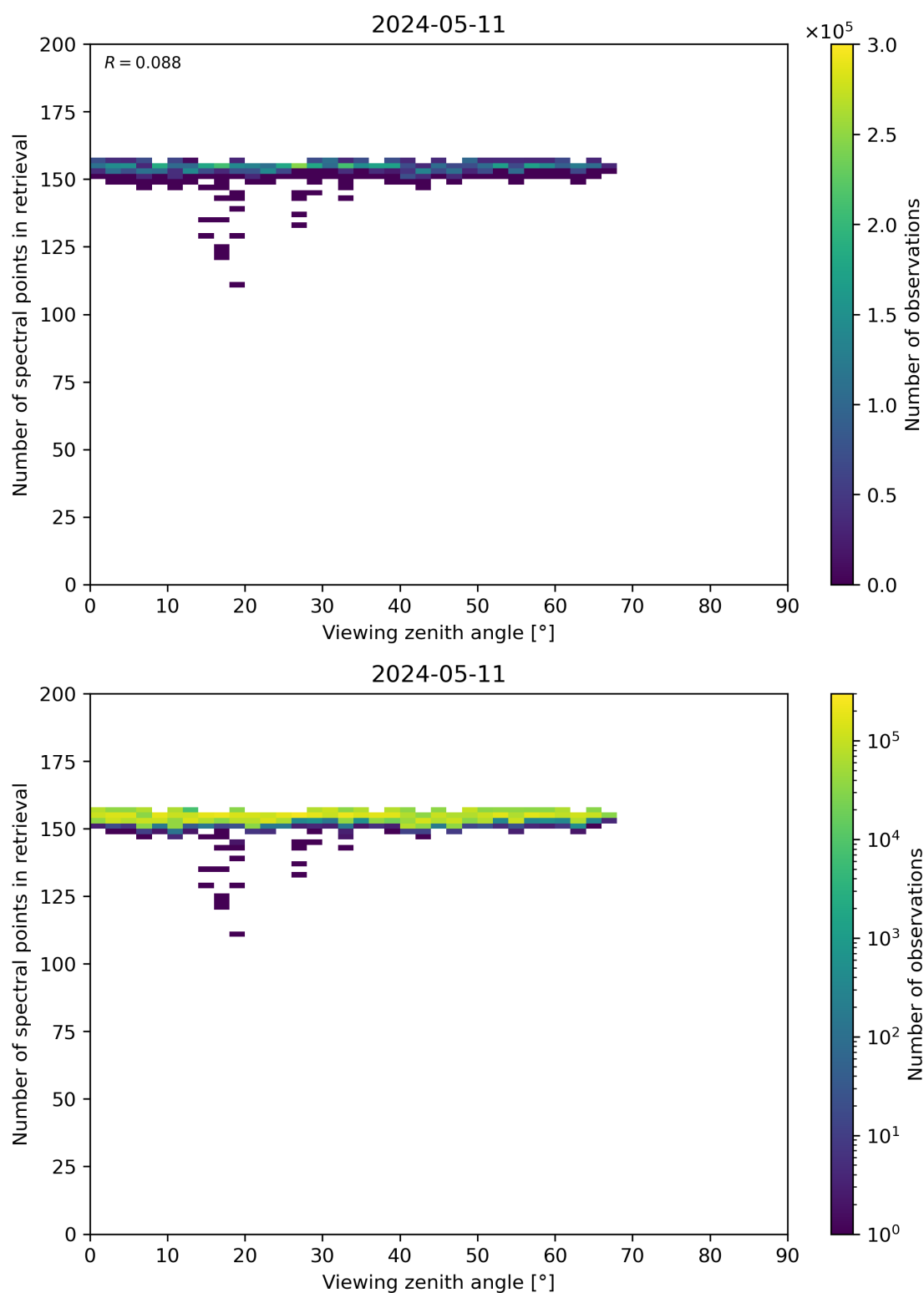
Figure 76: Scatter density plot of “Viewing zenith angle” against “Number of spectral points in retrieval” for 2024-05-10 to 2024-05-12.
