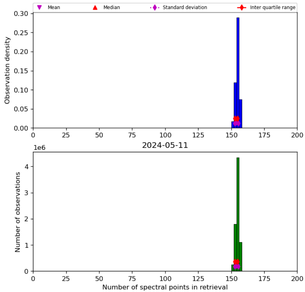
Figure 21: Histogram of “Number of spectral points in retrieval” for 2024-05-10 to 2024-05-12
