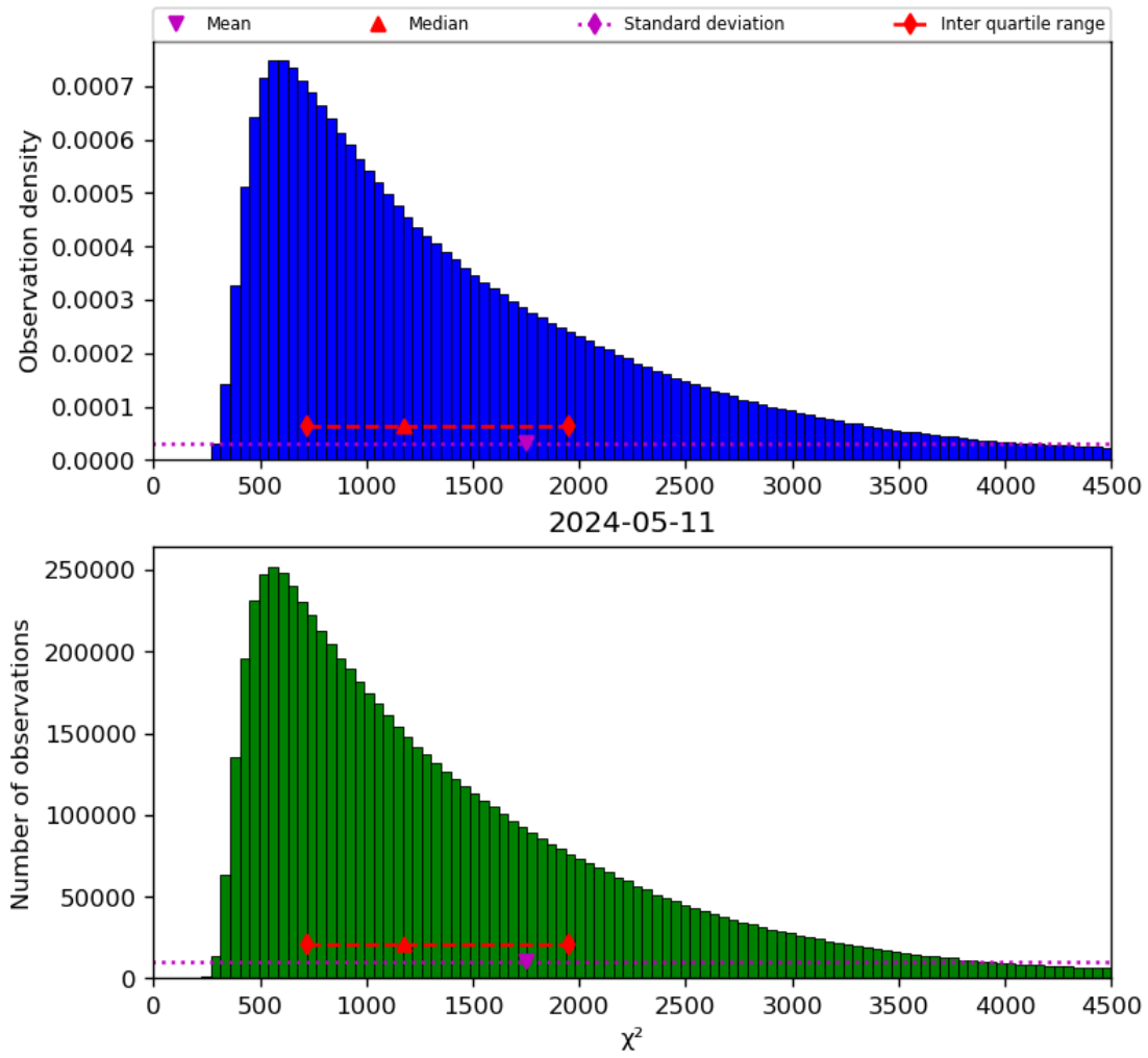
Figure 22: Histogram of “ \chi^2 ” for 2024-05-10 to 2024-05-12
