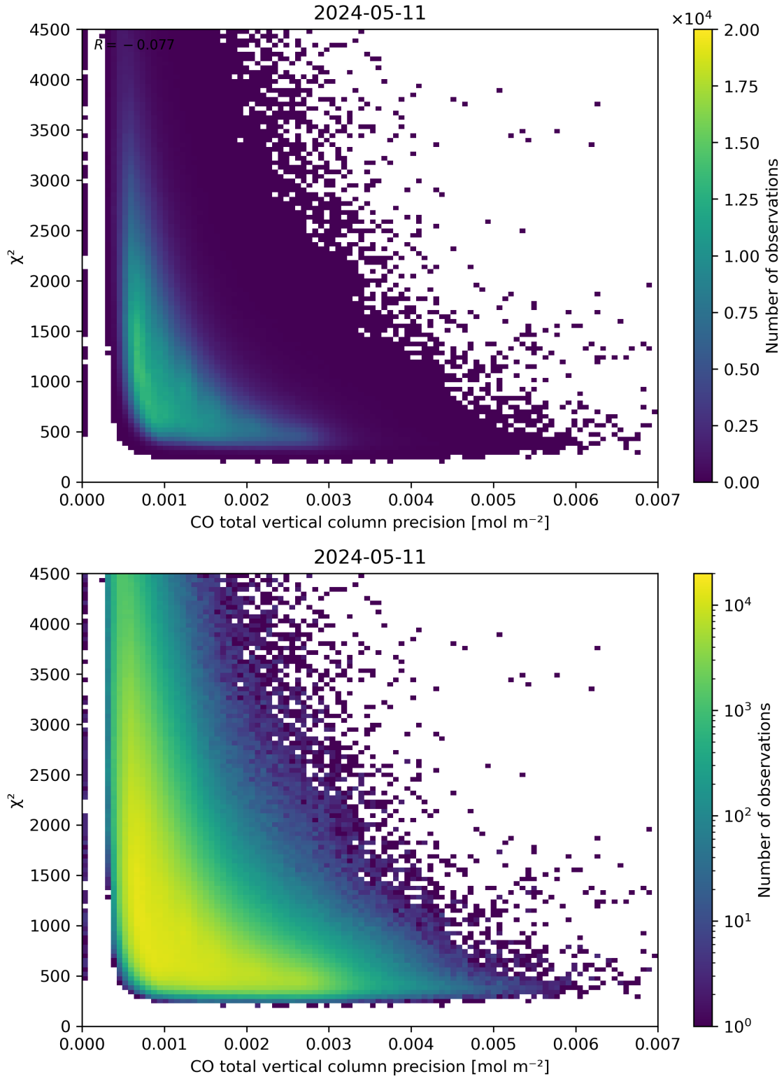
Figure 44: Scatter density plot of “CO total vertical column precision” against “ \chi^2 ” for 2024-05-10 to 2024-05-12.
