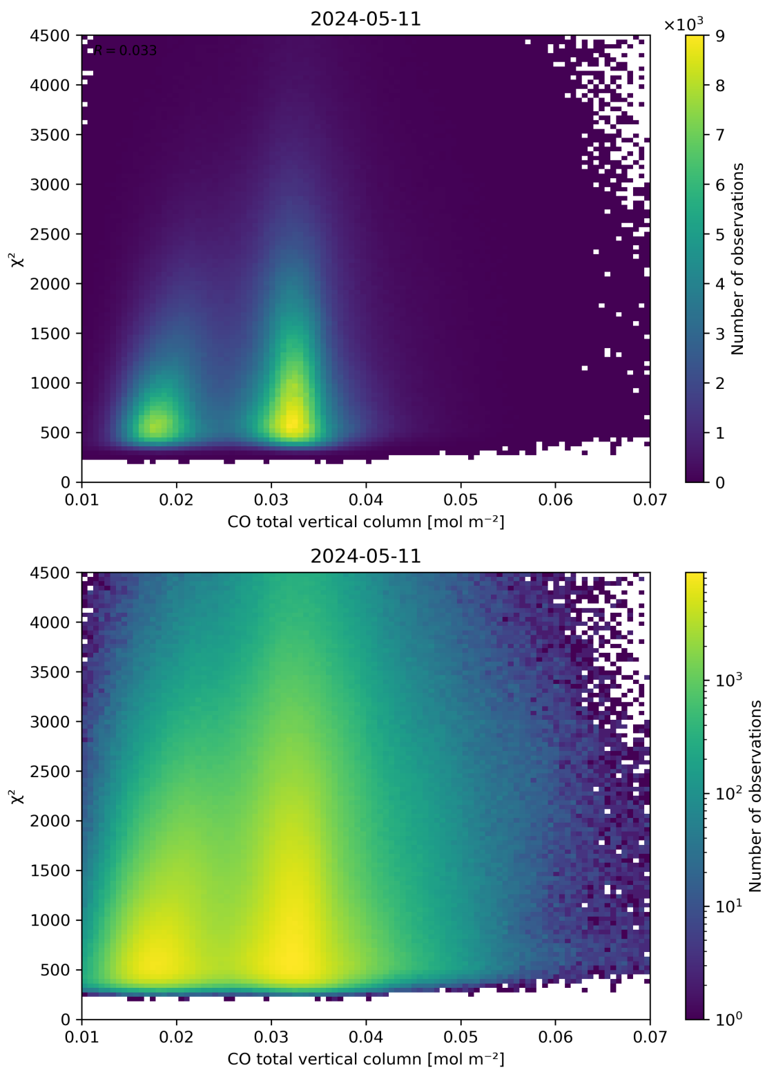
Figure 35: Scatter density plot of “CO total vertical column” against “ \chi^2 ” for 2024-05-10 to 2024-05-12.
