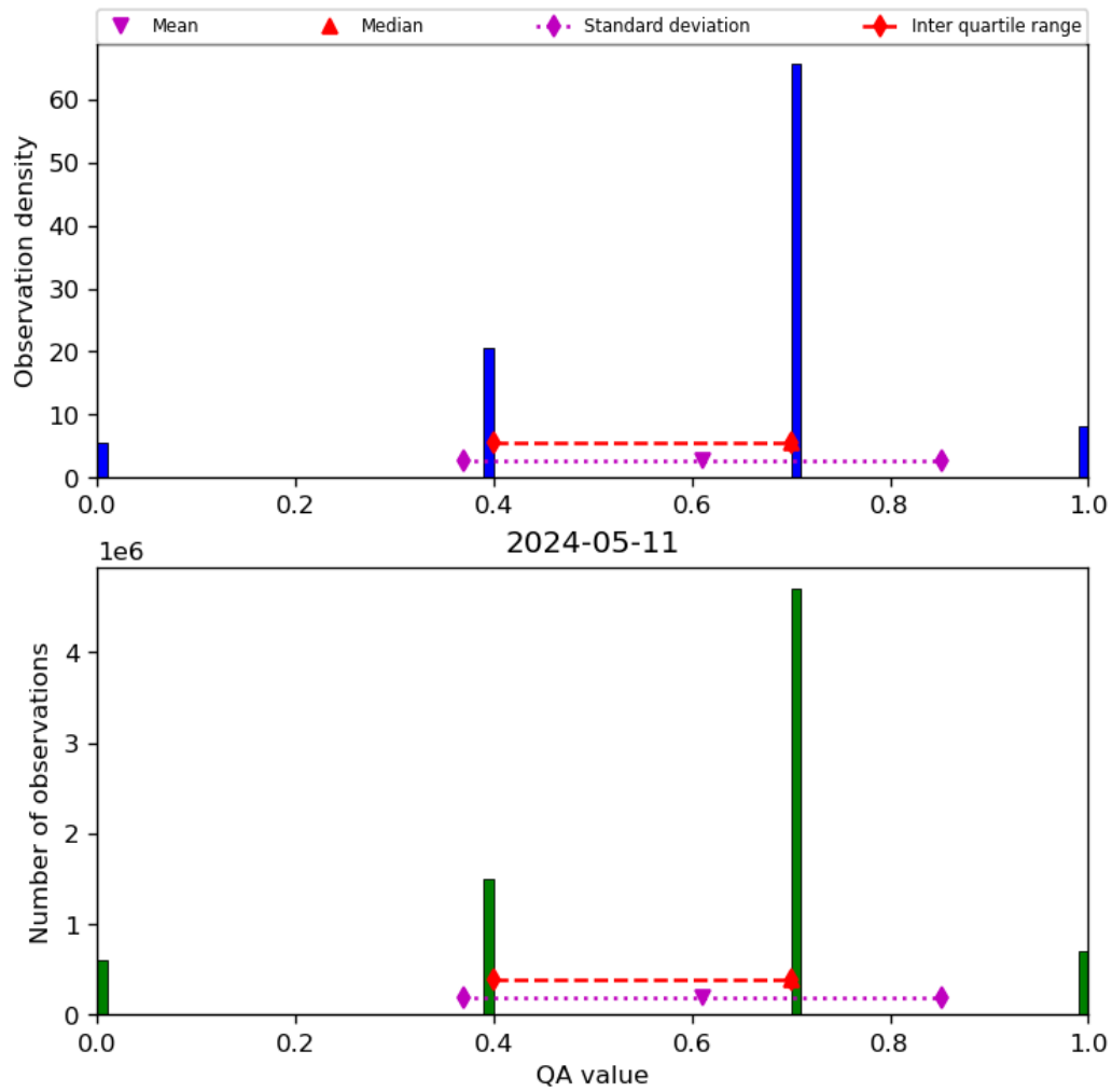
Figure 17: Histogram of “QA value” for 2024-05-10 to 2024-05-12
