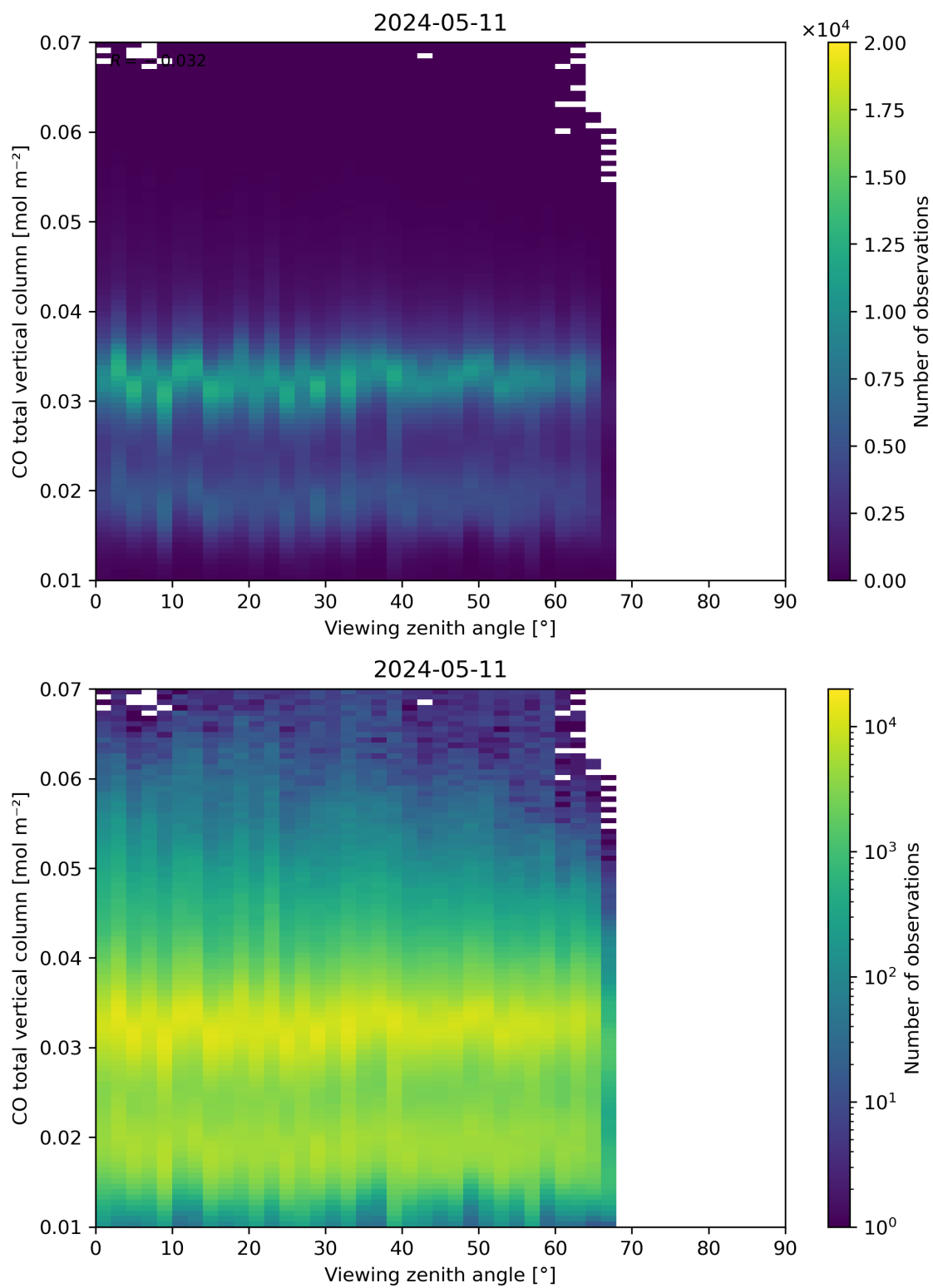
Figure 69: Scatter density plot of “Viewing zenith angle” against “CO total vertical column” for 2024-05-10 to 2024-05-12.
