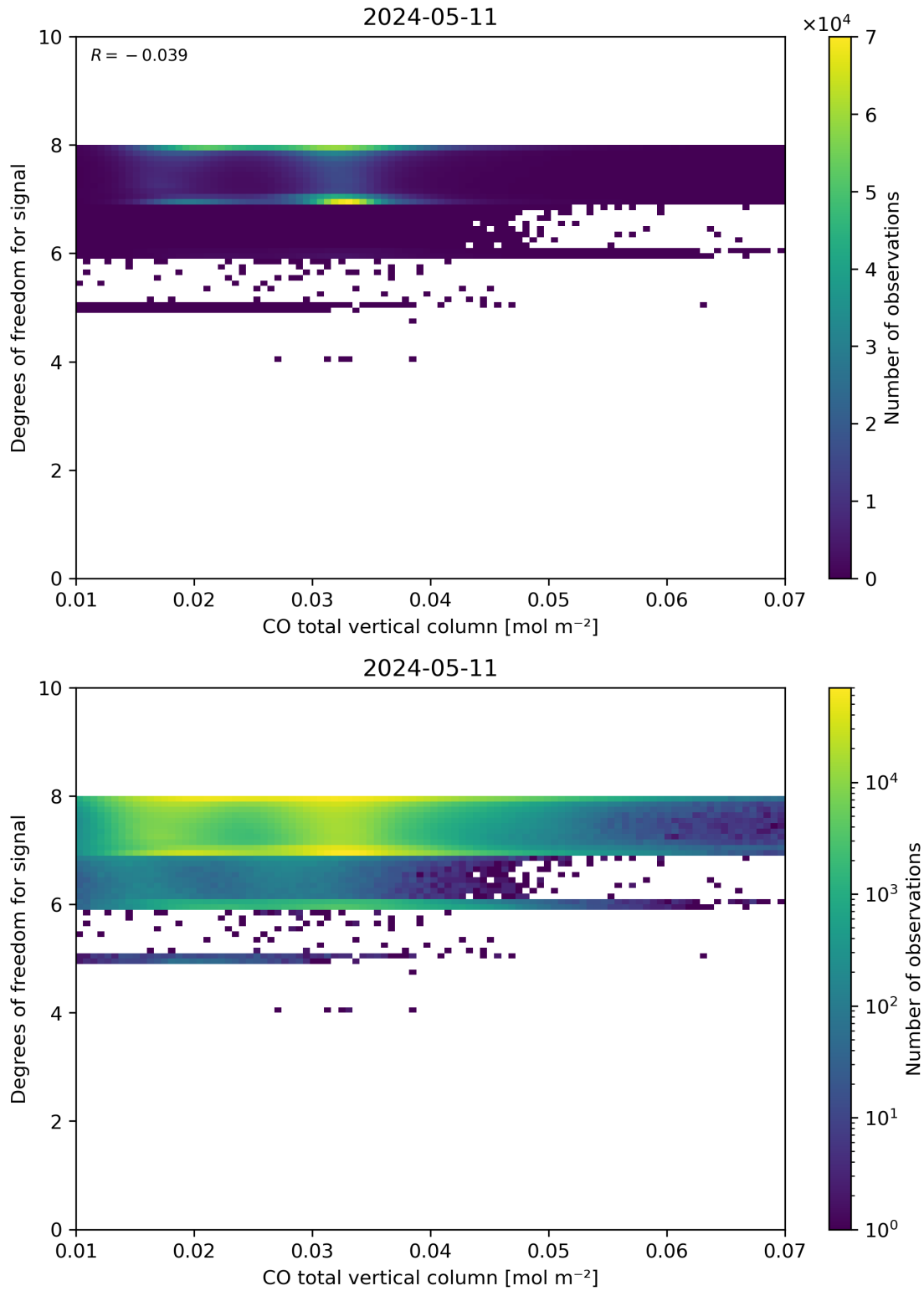
Figure 41: Scatter density plot of “CO total vertical column” against “Degrees of freedom for signal” for 2024-05-10 to 2024-05-12.
