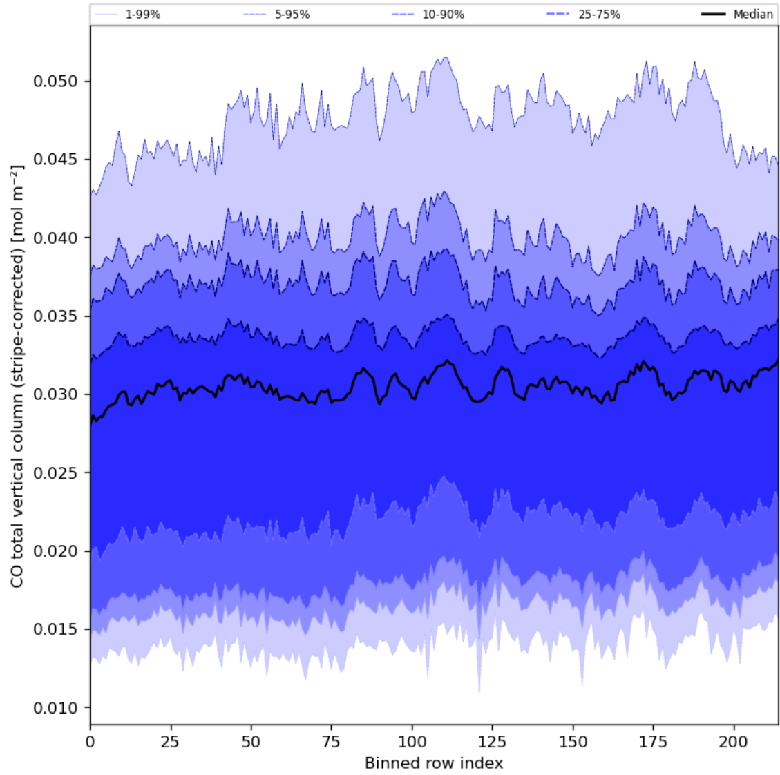
Figure 27: Along track statistics of “CO total vertical column (stripe-corrected)” for 2024-05-10 to 2024-05-12
