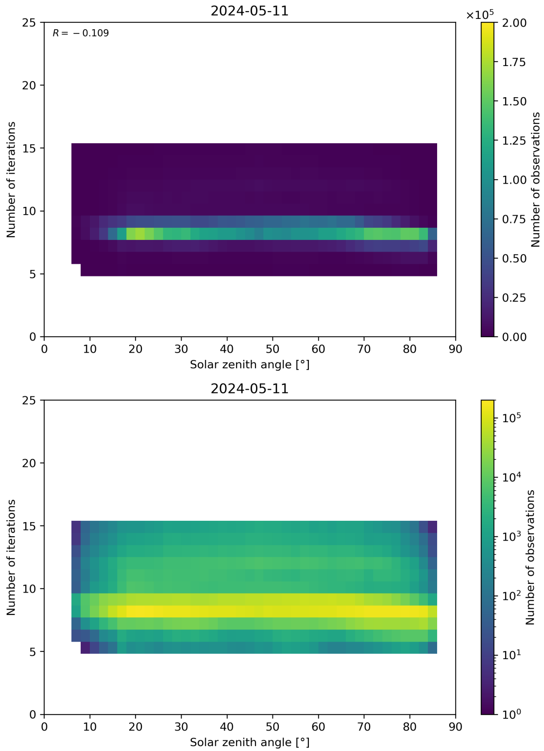
Figure 67: Scatter density plot of “Solar zenith angle” against “Number of iterations” for 2024-05-10 to 2024-05-12.
