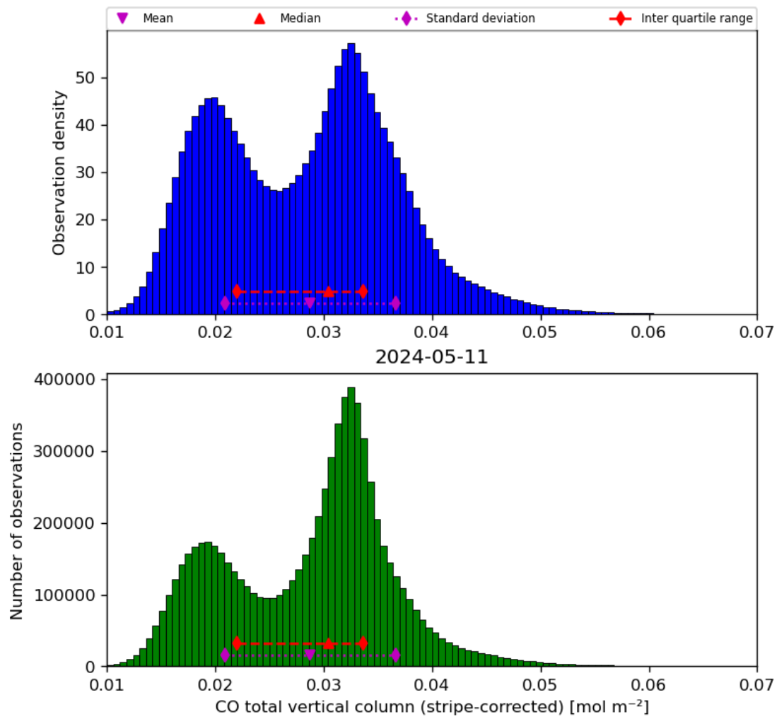
Figure 19: Histogram of “CO total vertical column (stripe-corrected)” for 2024-05-10 to 2024-05-12
