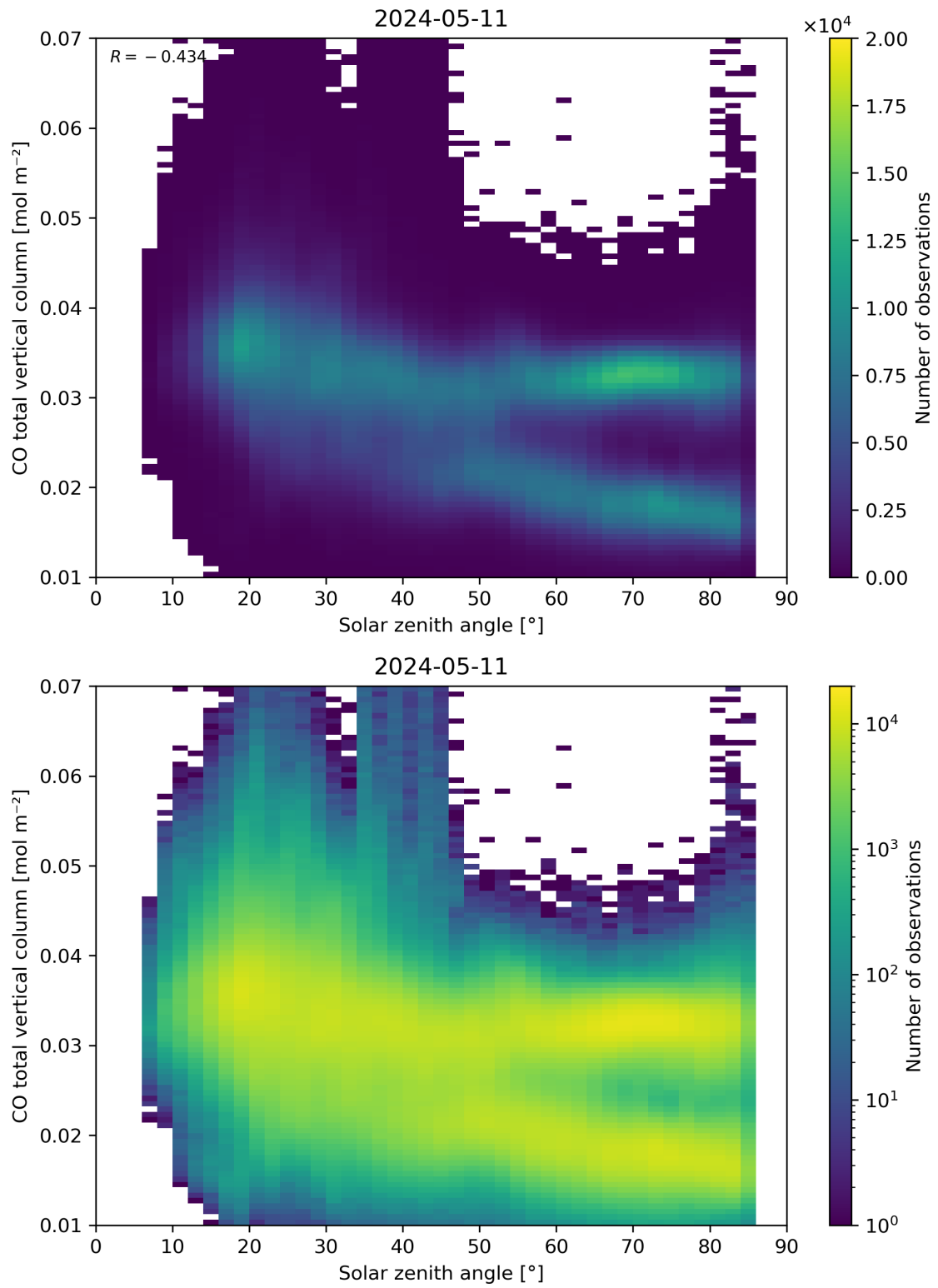
Figure 61: Scatter density plot of “Solar zenith angle” against “CO total vertical column” for 2024-05-10 to 2024-05-12.
