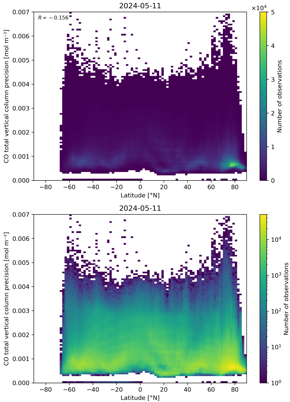
Figure 53: Scatter density plot of “Latitude” against “CO total vertical column precision” for 2024-05-10 to 2024-05-12.
