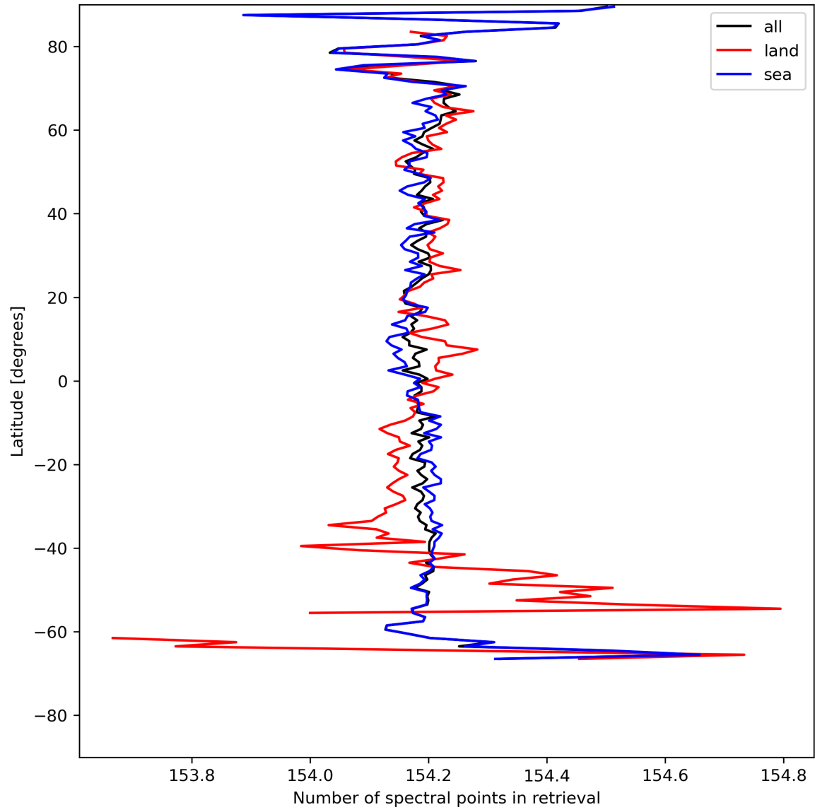
Figure 13: Zonal average of “Number of spectral points in retrieval” for 2024-05-10 to 2024-05-12.
