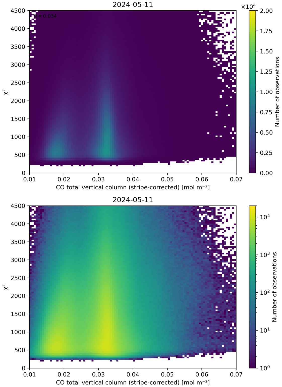
Figure 37: Scatter density plot of “CO total vertical column (stripe-corrected)” against “ \chi^2 ” for 2024-05-10 to 2024-05-12.
