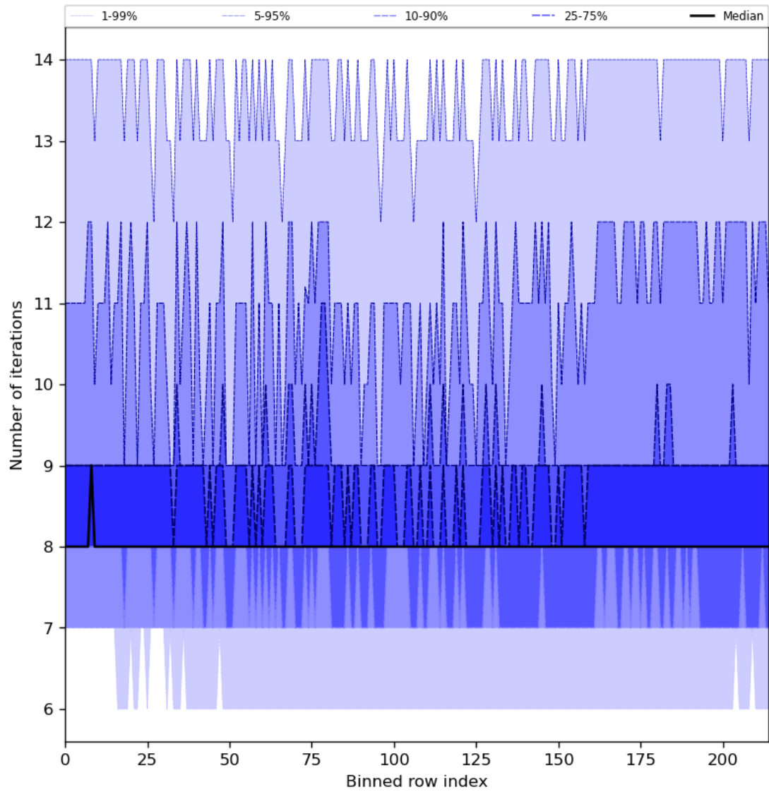
Figure 32: Along track statistics of “Number of iterations” for 2024-05-10 to 2024-05-12
