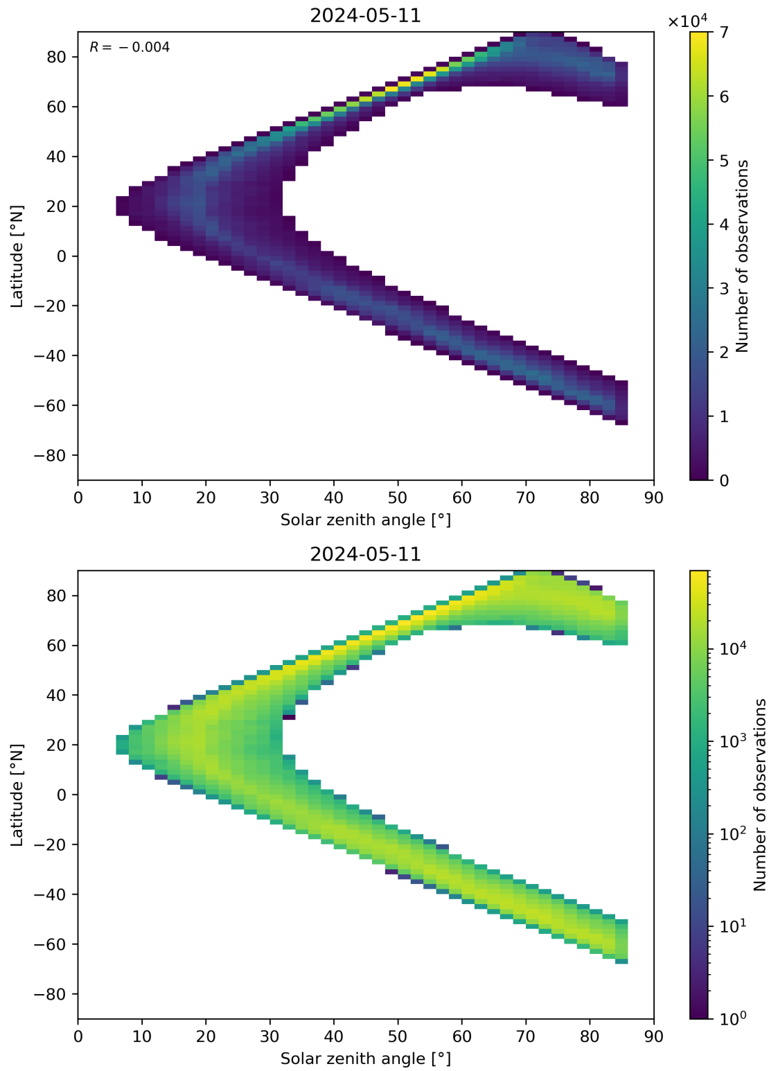
Figure 66: Scatter density plot of “Solar zenith angle” against “Latitude” for 2024-05-10 to 2024-05-12.
