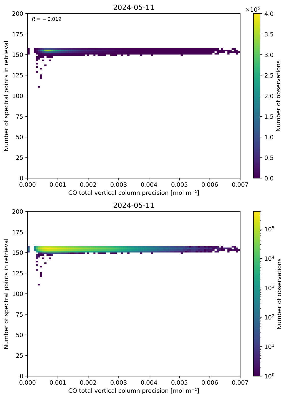
Figure 47: Scatter density plot of “CO total vertical column precision” against “Number of spectral points in retrieval” for 2024-05-10 to 2024-05-12.
