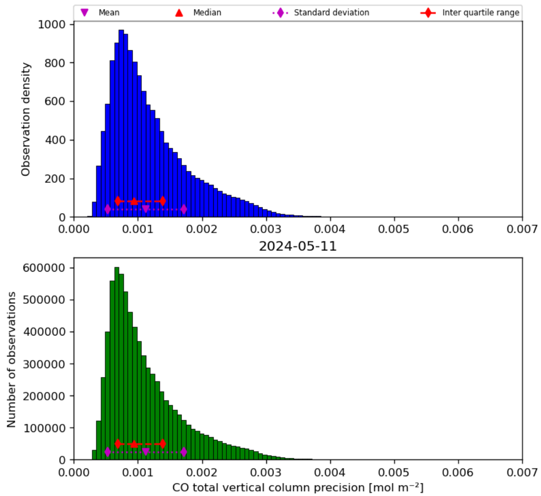
Figure 20: Histogram of “CO total vertical column precision” for 2024-05-10 to 2024-05-12
