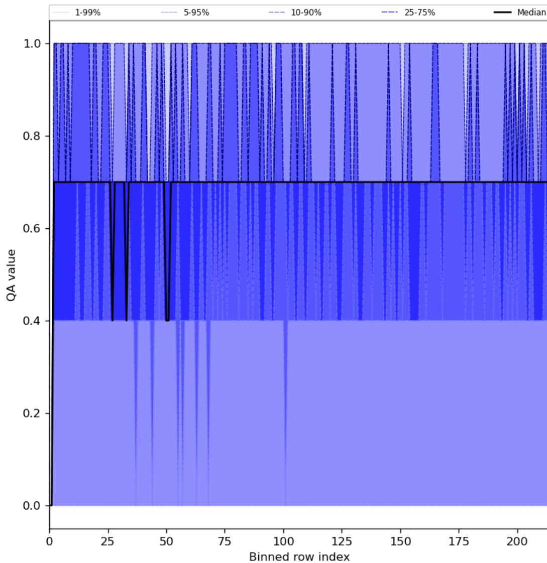
Figure 25: Along track statistics of “QA value” for 2024-05-10 to 2024-05-12
