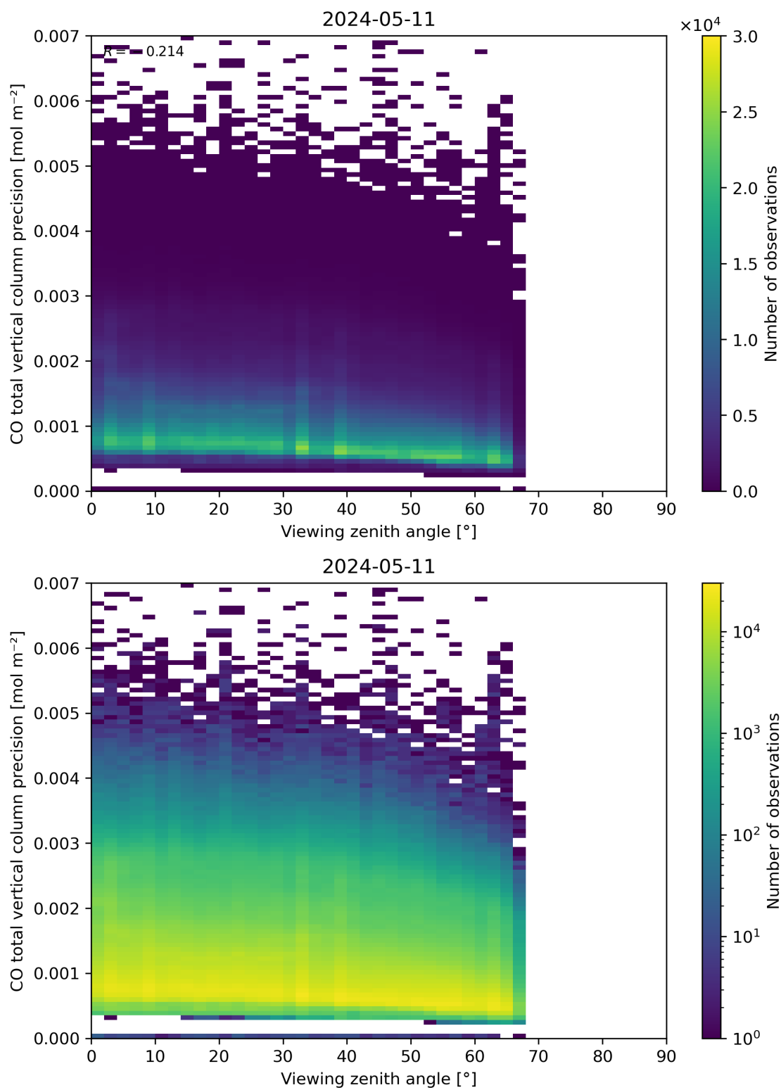
Figure 71: Scatter density plot of “Viewing zenith angle” against “CO total vertical column precision” for 2024-05-10 to 2024-05-12.
