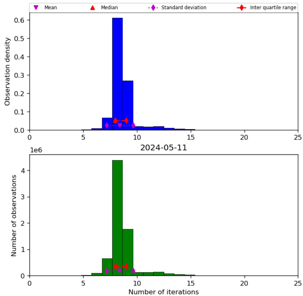
Figure 24: Histogram of “Number of iterations” for 2024-05-10 to 2024-05-12
