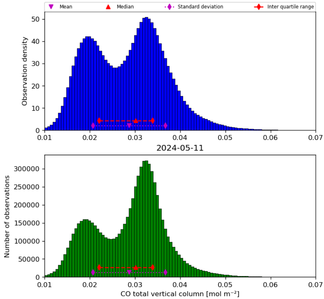
Figure 18: Histogram of “CO total vertical column” for 2024-05-10 to 2024-05-12
