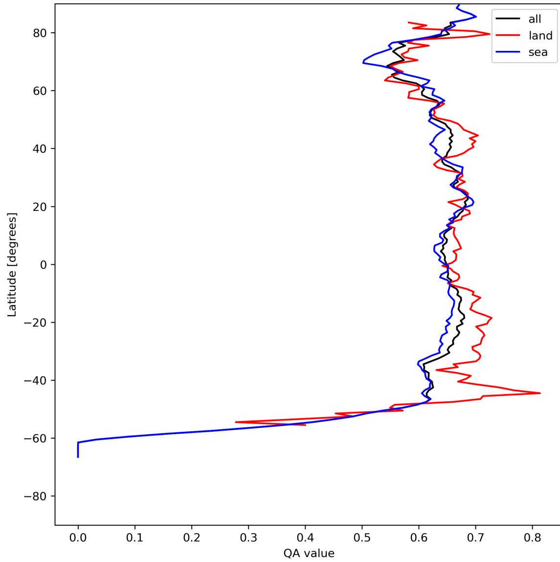
Figure 9: Zonal average of “QA value” for 2024-05-10 to 2024-05-12.
