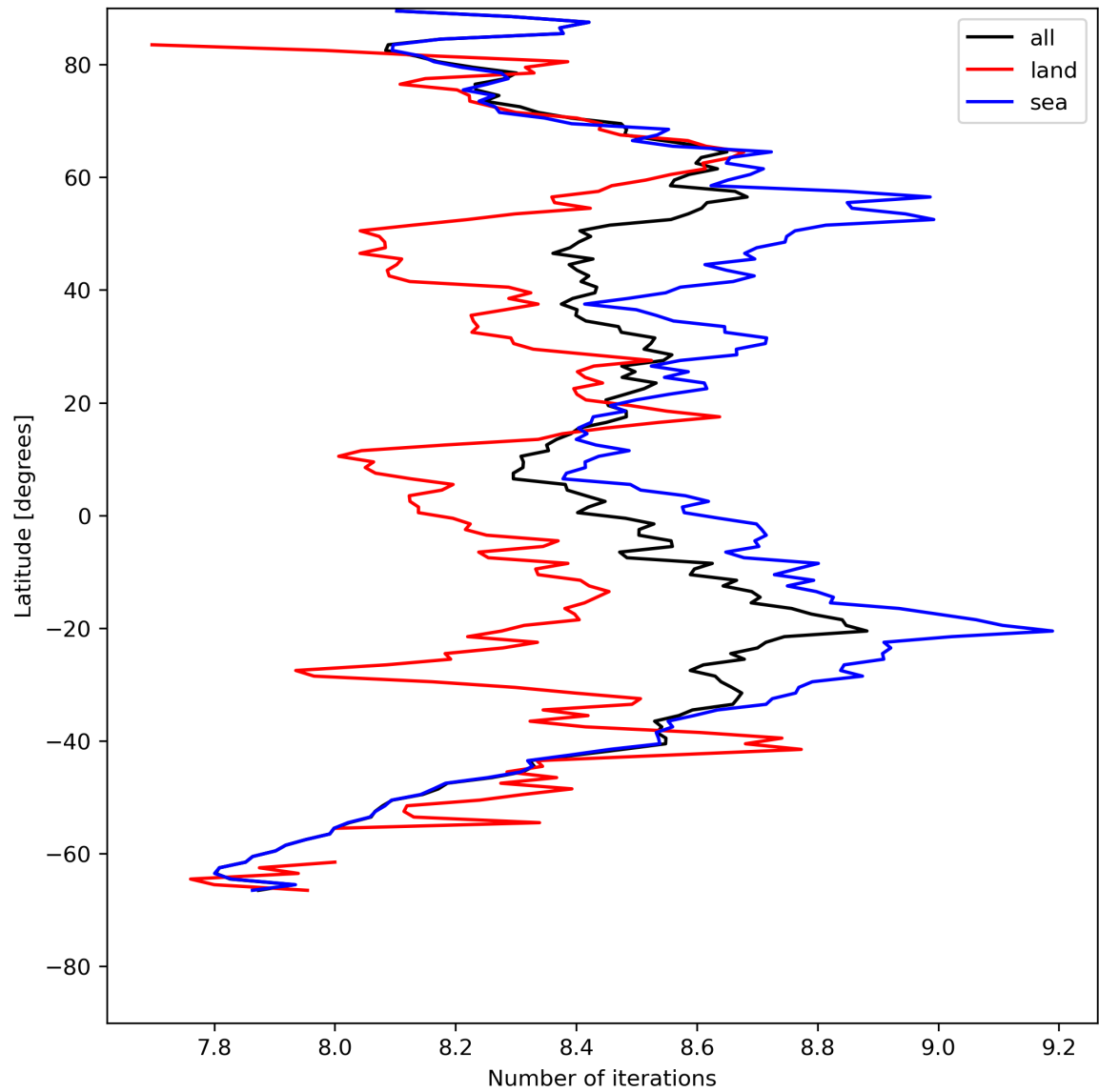
Figure 16: Zonal average of “Number of iterations” for 2024-05-10 to 2024-05-12.
