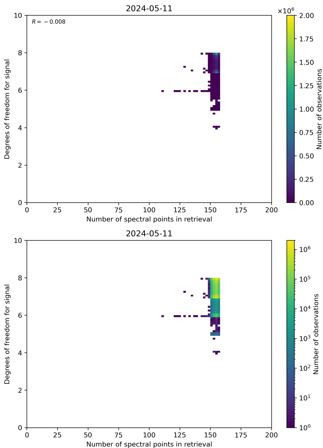
Figure 59: Scatter density plot of “Number of spectral points in retrieval” against “Degrees of freedom for signal” for 2024-05-10 to 2024-05-12.
