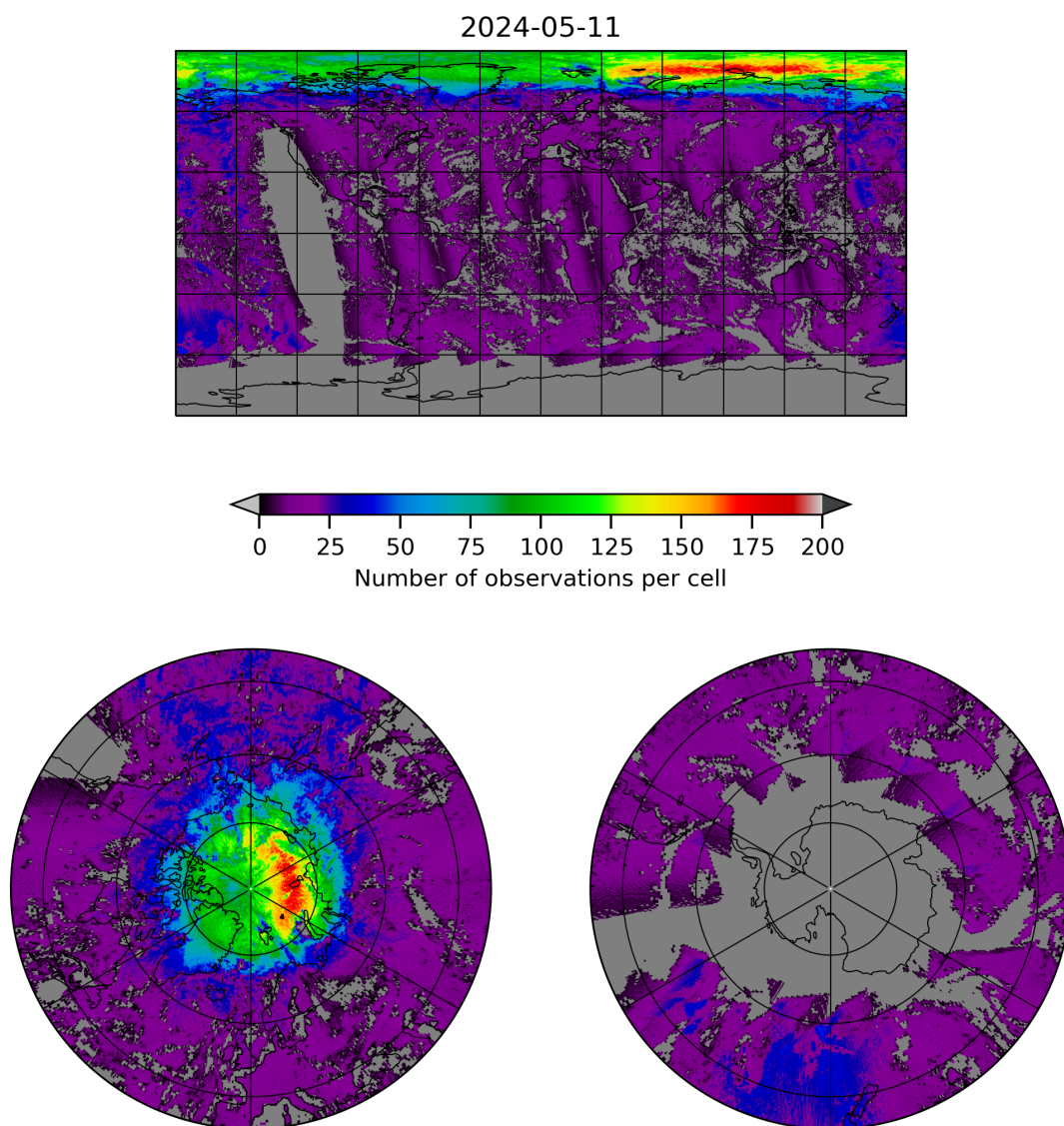
Figure 8: Map of the number of observations for 2024-05-10 to 2024-05-12
