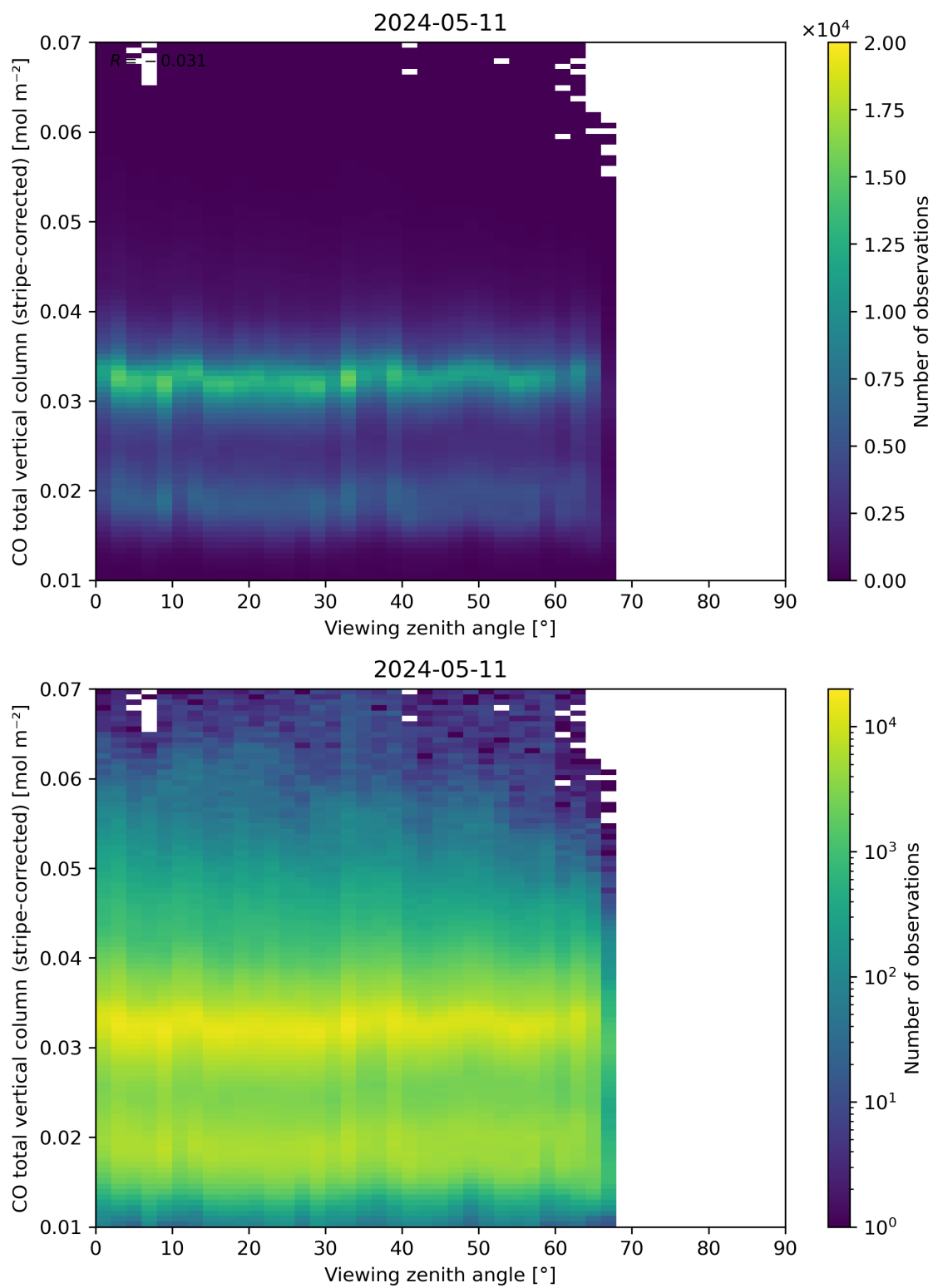
Figure 70: Scatter density plot of “Viewing zenith angle” against “CO total vertical column (stripe-corrected)” for 2024-05-10 to 2024-05-12.
