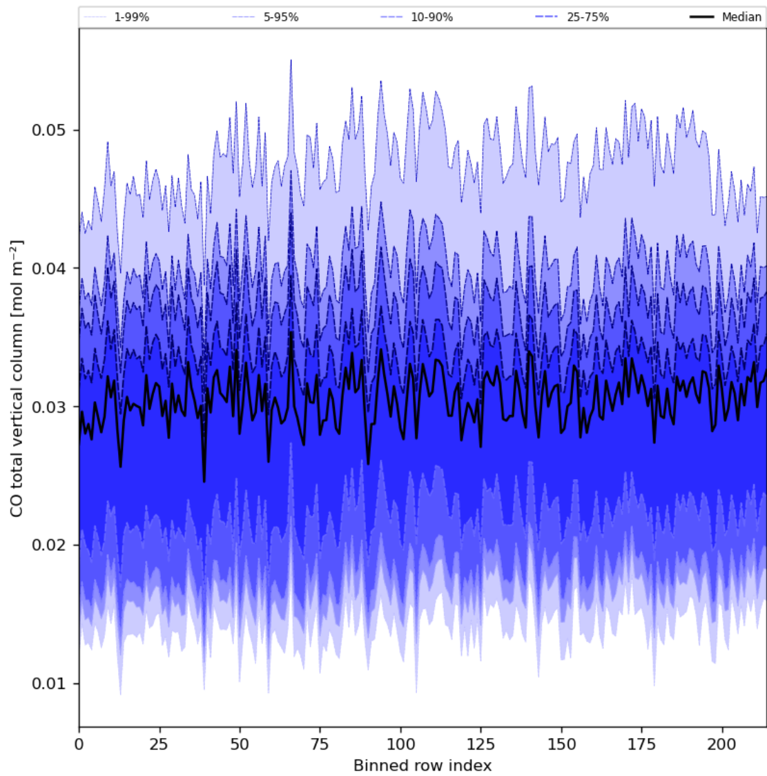
Figure 26: Along track statistics of “CO total vertical column” for 2024-05-10 to 2024-05-12
