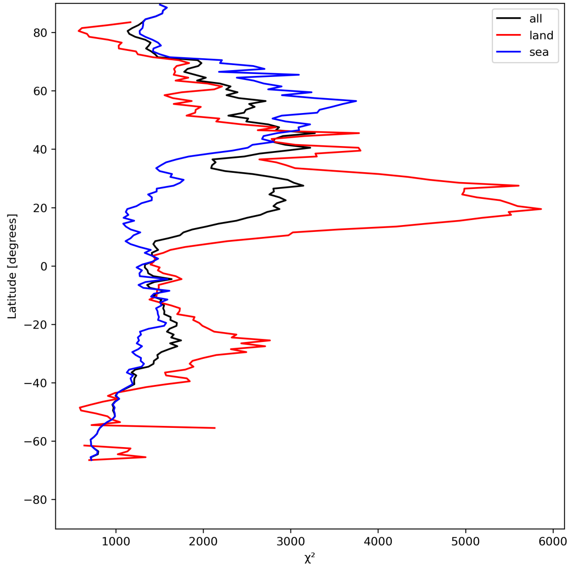
Figure 14: Zonal average of “ \chi^2 ” for 2024-05-10 to 2024-05-12.
