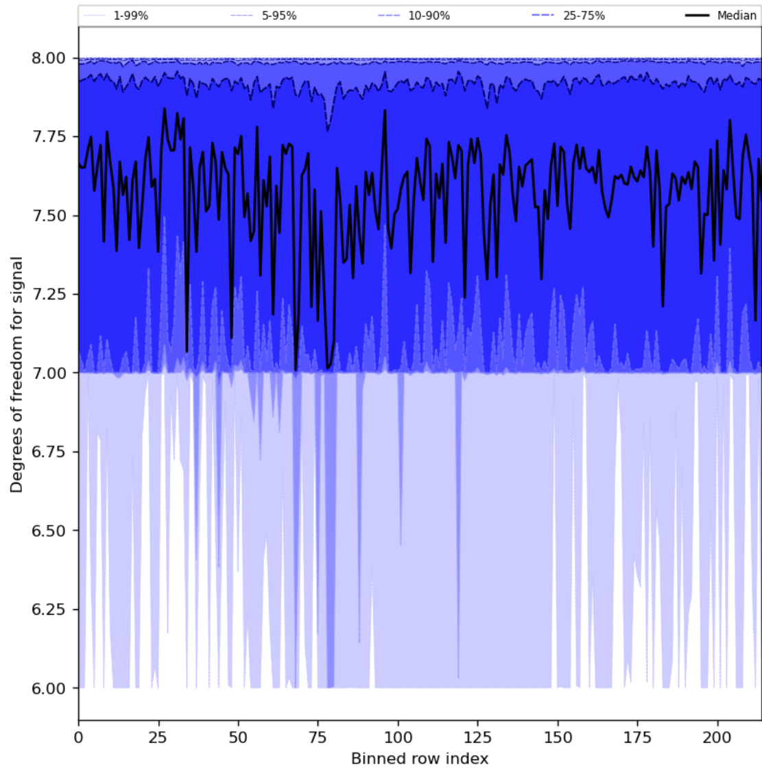
Figure 31: Along track statistics of “Degrees of freedom for signal” for 2024-05-10 to 2024-05-12
