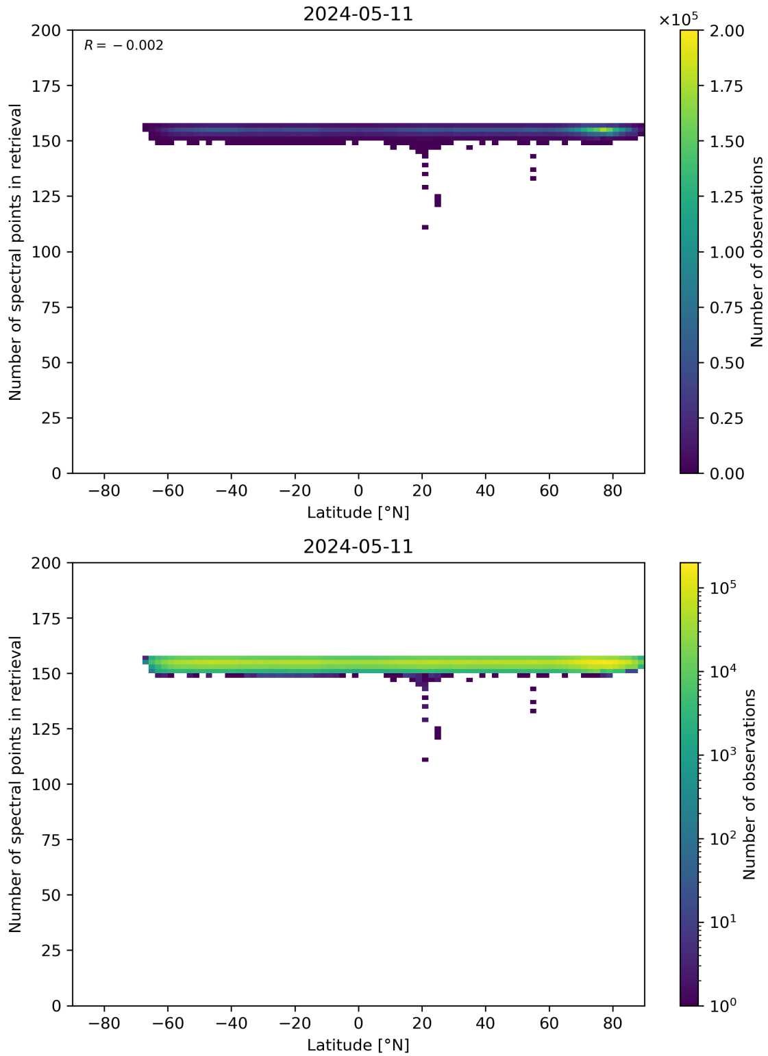
Figure 57: Scatter density plot of “Latitude” against “Number of spectral points in retrieval” for 2024-05-10 to 2024-05-12.
