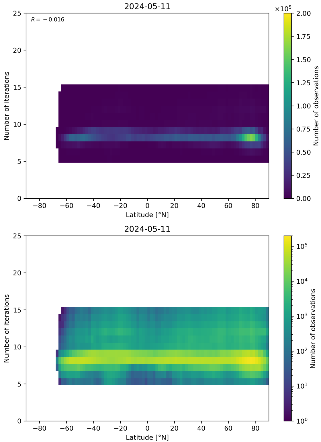
Figure 56: Scatter density plot of “Latitude” against “Number of iterations” for 2024-05-10 to 2024-05-12.
