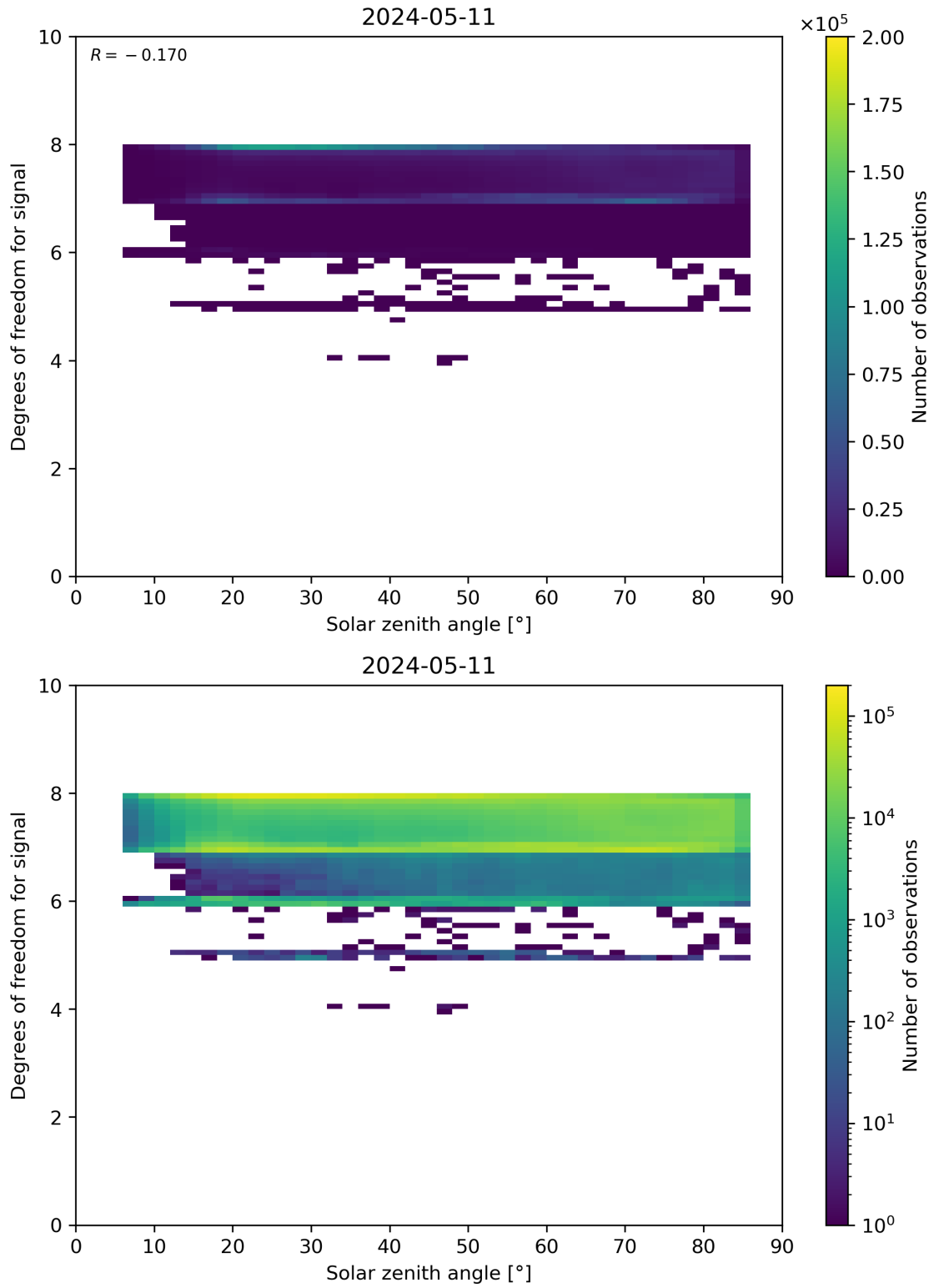
Figure 65: Scatter density plot of “Solar zenith angle” against “Degrees of freedom for signal” for 2024-05-10 to 2024-05-12.
