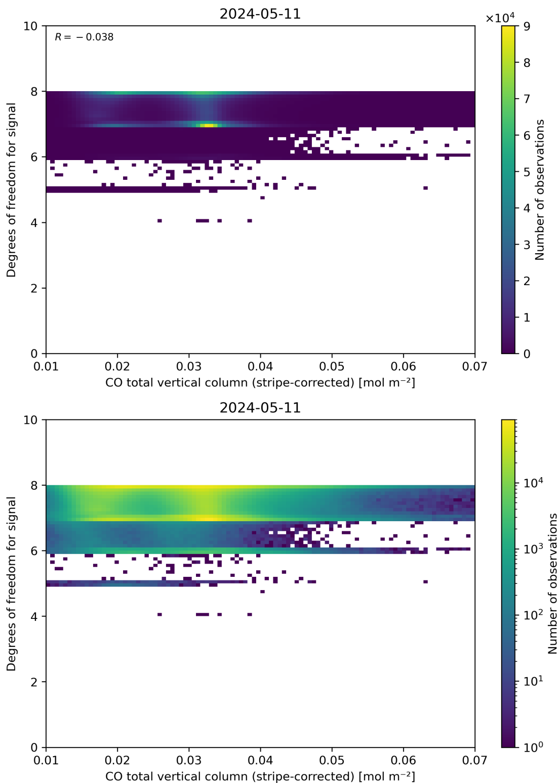
Figure 38: Scatter density plot of “CO total vertical column (stripe-corrected)” against “Degrees of freedom for signal” for 2024-05-10 to 2024-05-12.
