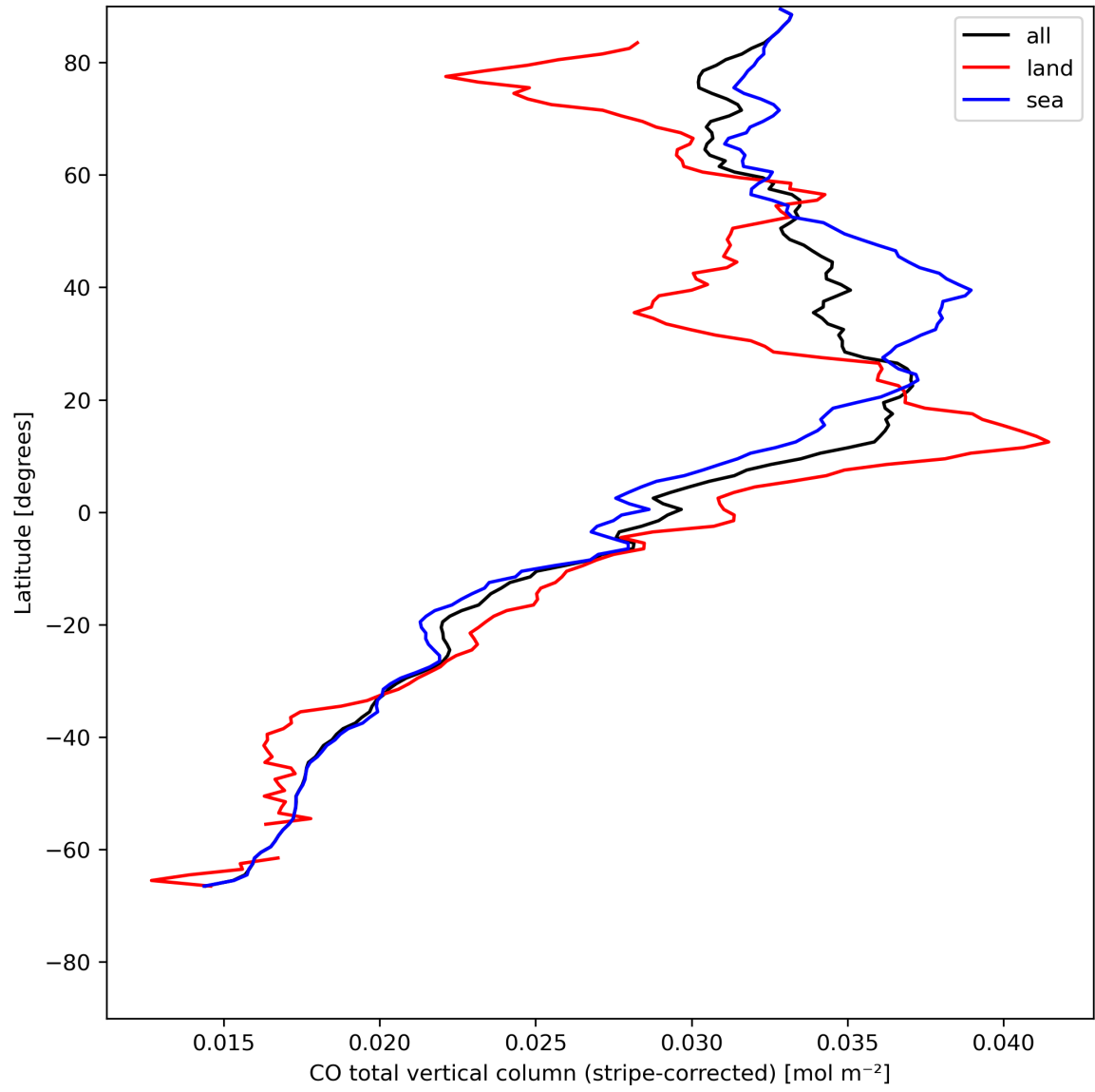
Figure 11: Zonal average of “CO total vertical column (stripe-corrected)” for 2024-05-10 to 2024-05-12.
