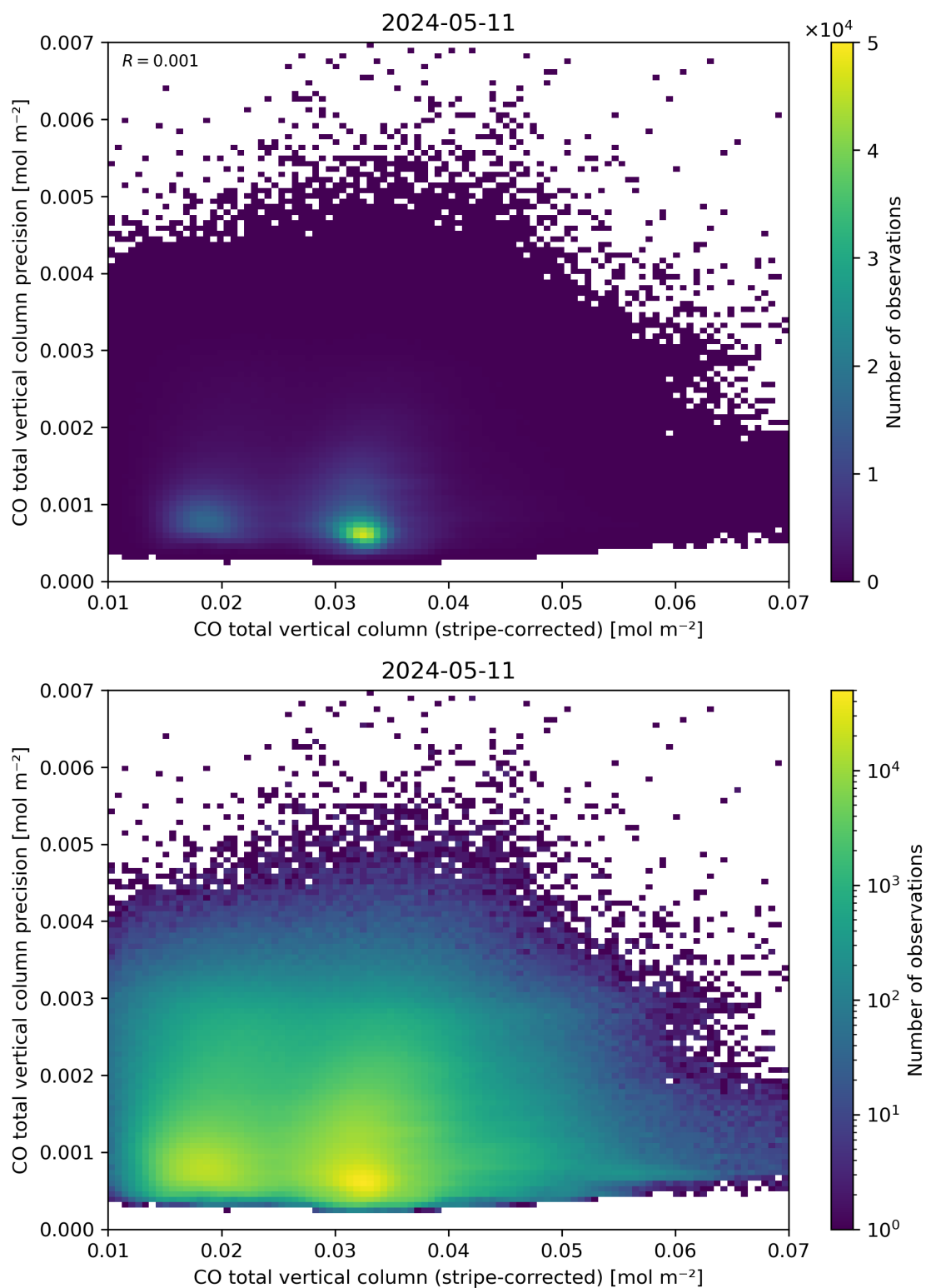
Figure 36: Scatter density plot of “CO total vertical column (stripe-corrected)” against “CO total vertical column precision” for 2024-05-10 to 2024-05-12.
