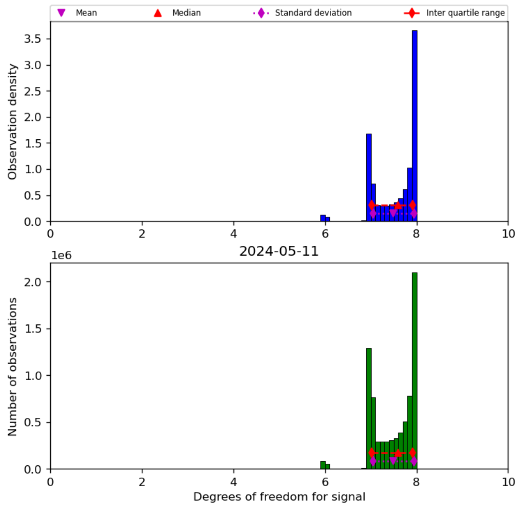
Figure 23: Histogram of “Degrees of freedom for signal” for 2024-05-10 to 2024-05-12
