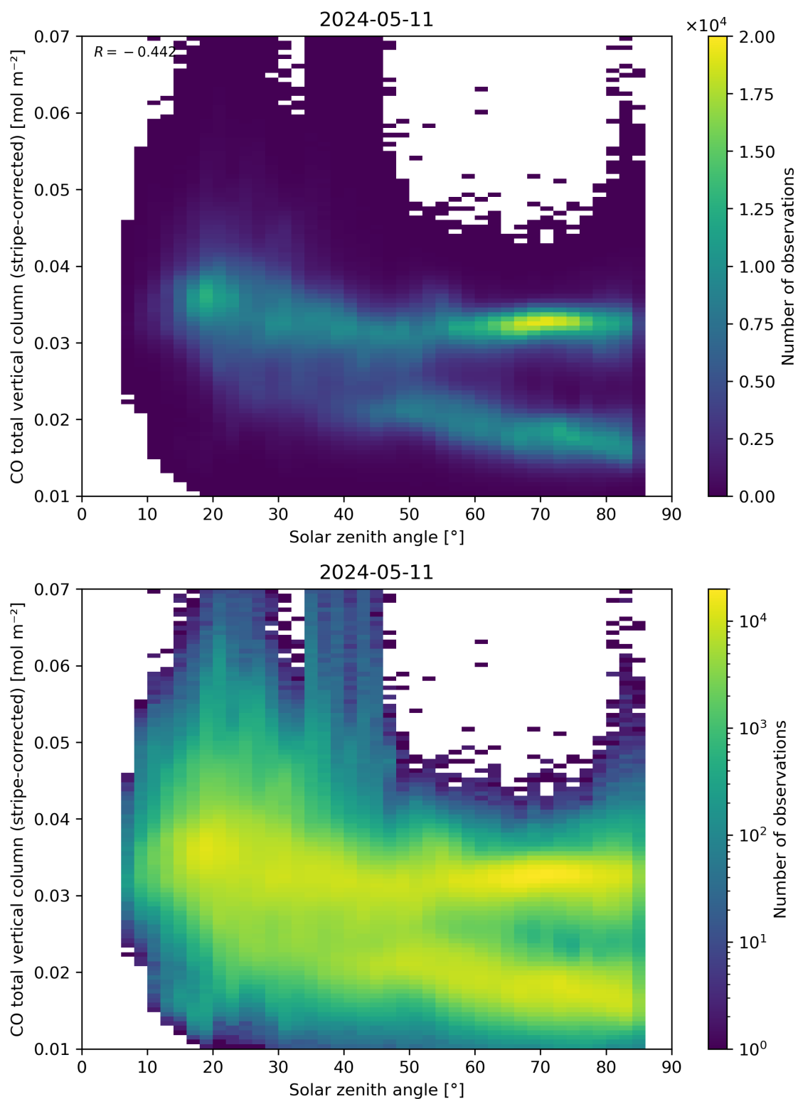
Figure 62: Scatter density plot of “Solar zenith angle” against “CO total vertical column (stripe-corrected)” for 2024-05-10 to 2024-05-12.
