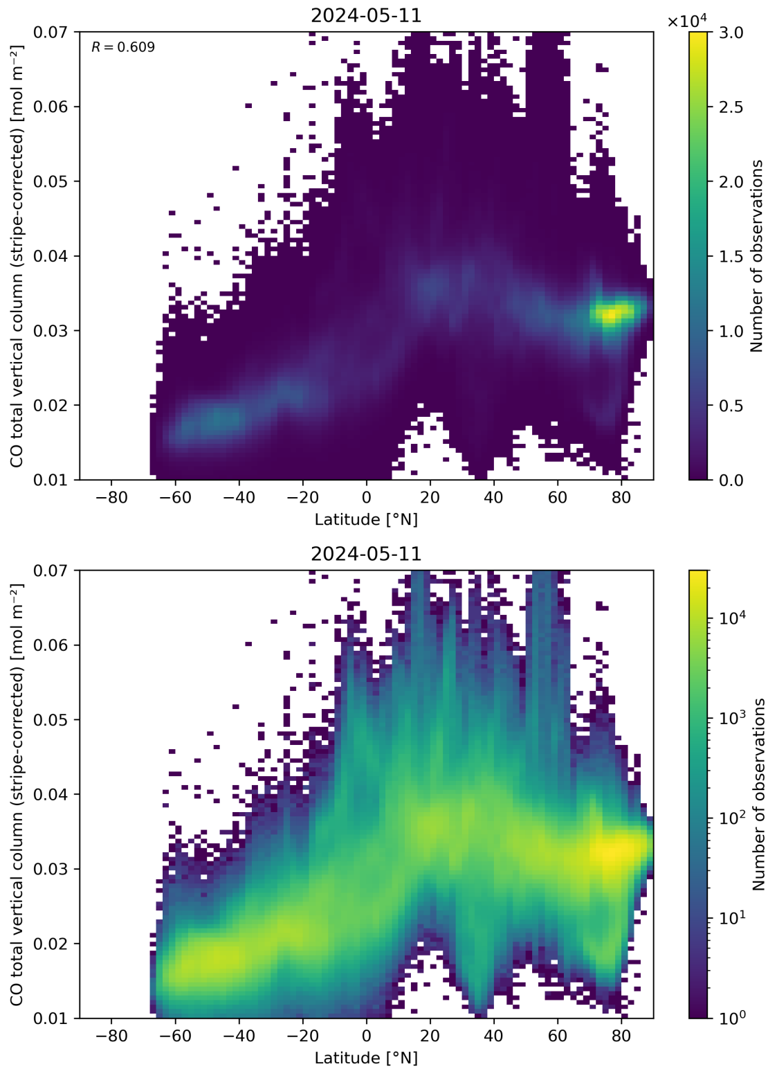
Figure 52: Scatter density plot of “Latitude” against “CO total vertical column (stripe-corrected)” for 2024-05-10 to 2024-05-12.
