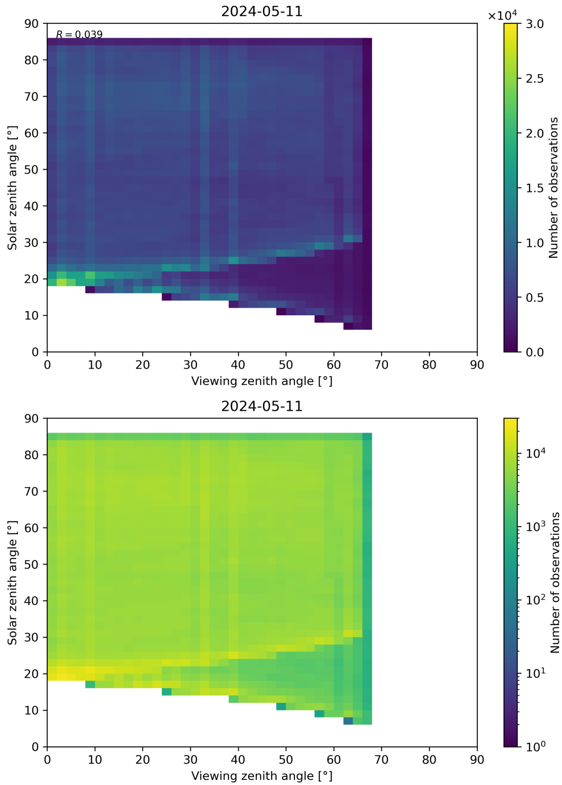
Figure 77: Scatter density plot of “Viewing zenith angle” against “Solar zenith angle” for 2024-05-10 to 2024-05-12.
