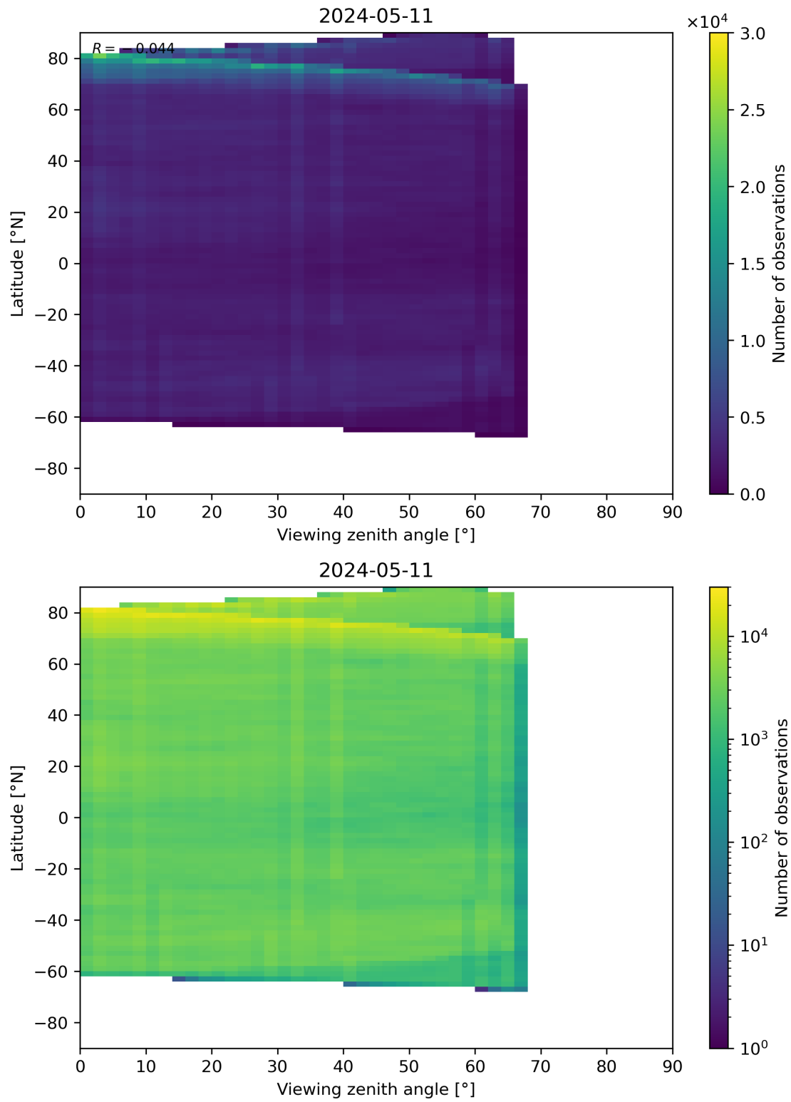
Figure 74: Scatter density plot of “Viewing zenith angle” against “Latitude” for 2024-05-10 to 2024-05-12.
