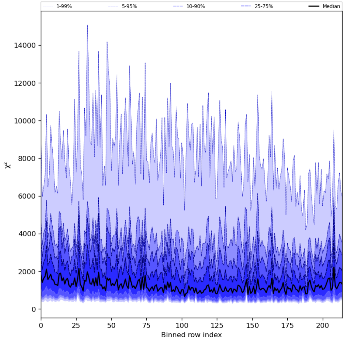
Figure 30: Along track statistics of “ \chi^2 ” for 2024-05-10 to 2024-05-12
