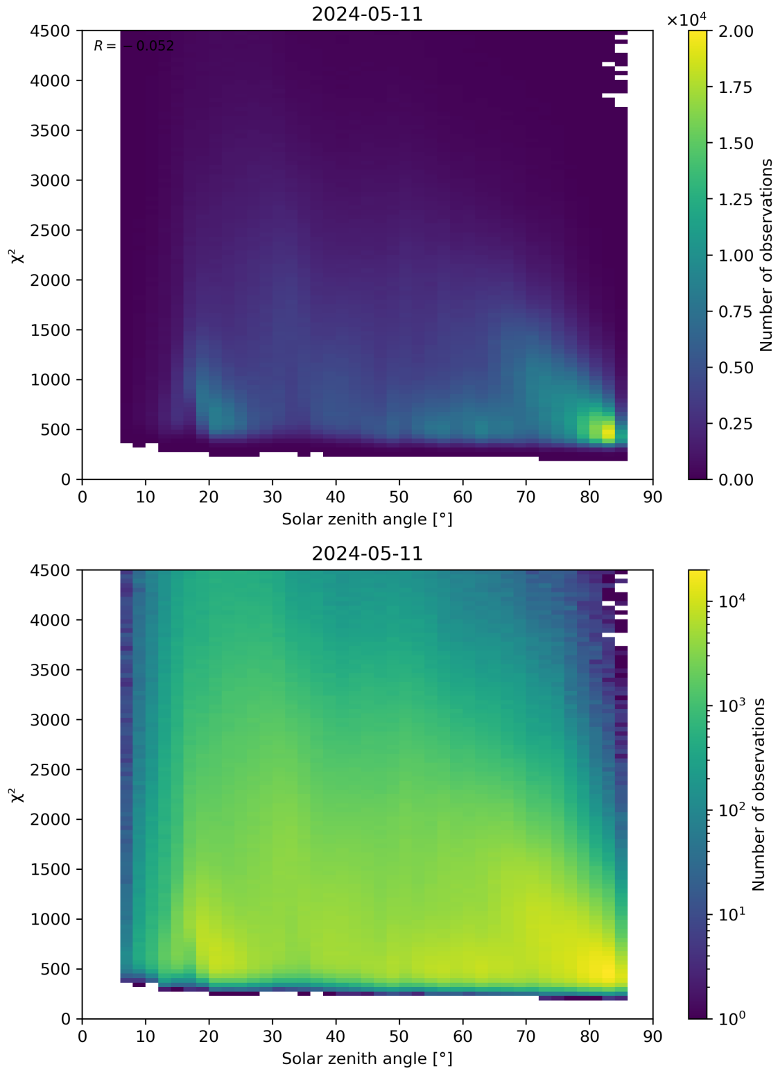
Figure 64: Scatter density plot of “Solar zenith angle” against “ \chi^2 ” for 2024-05-10 to 2024-05-12.
