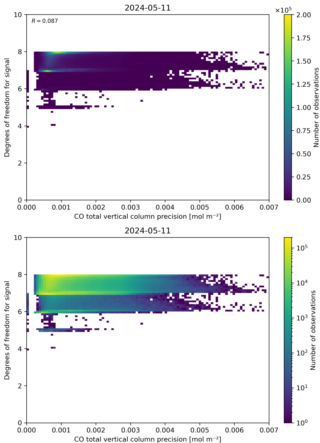
Figure 45: Scatter density plot of “CO total vertical column precision” against “Degrees of freedom for signal” for 2024-05-10 to 2024-05-12.
