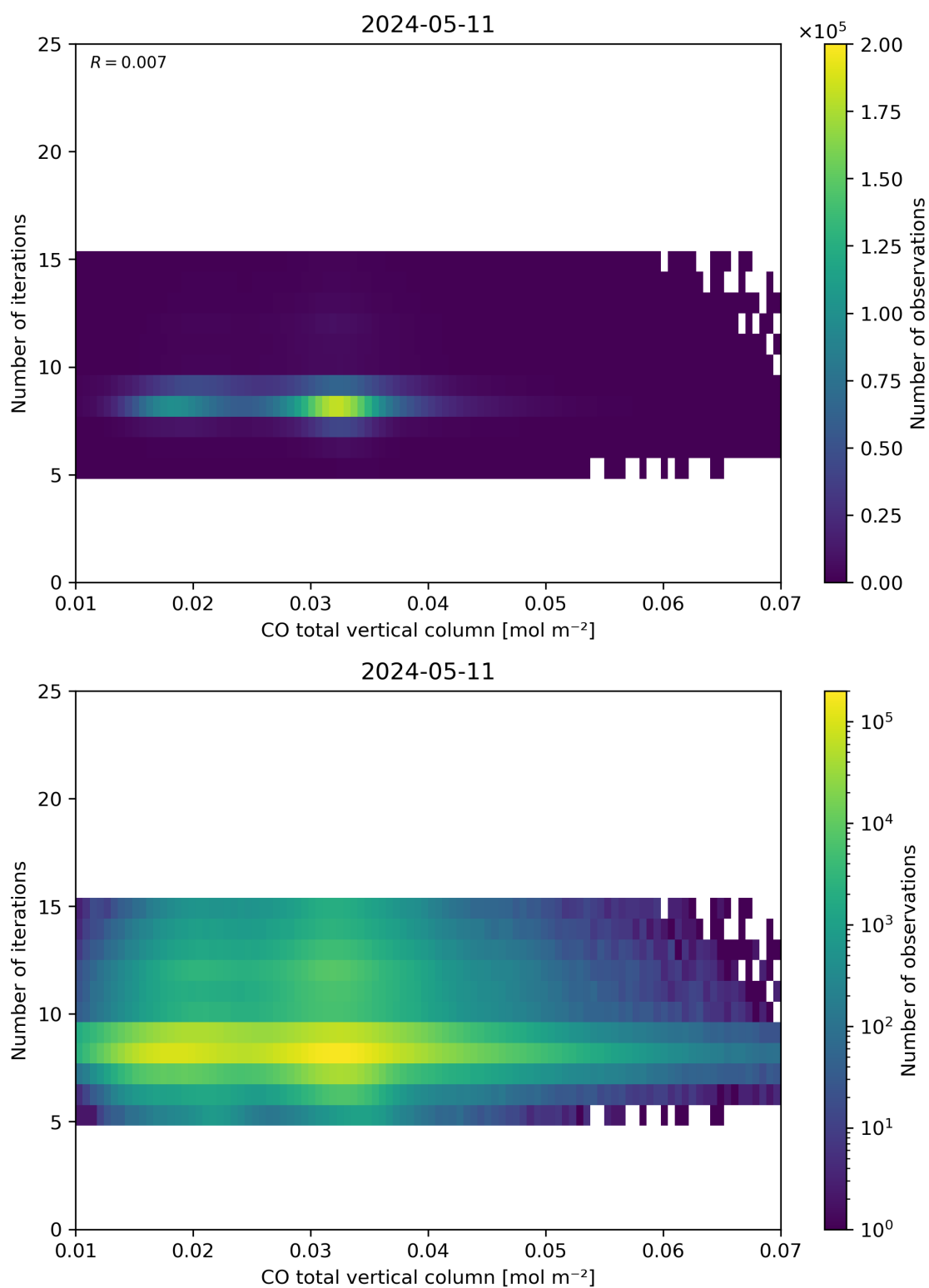
Figure 42: Scatter density plot of “CO total vertical column” against “Number of iterations” for 2024-05-10 to 2024-05-12.
