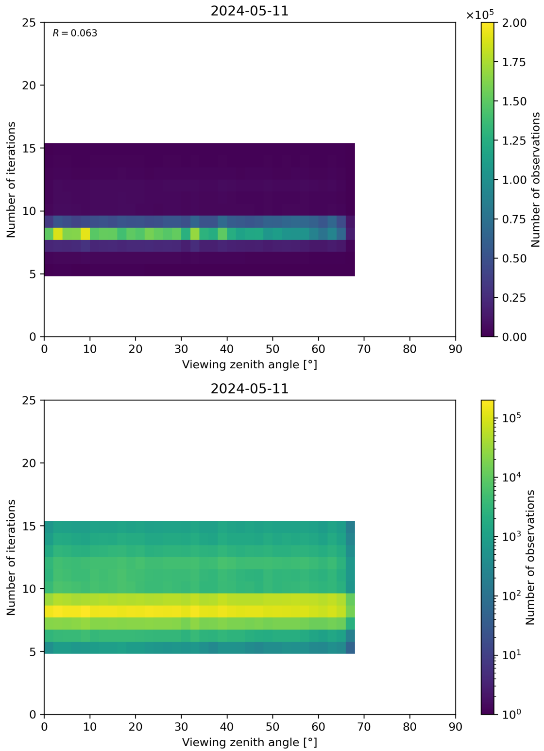
Figure 75: Scatter density plot of “Viewing zenith angle” against “Number of iterations” for 2024-05-10 to 2024-05-12.
