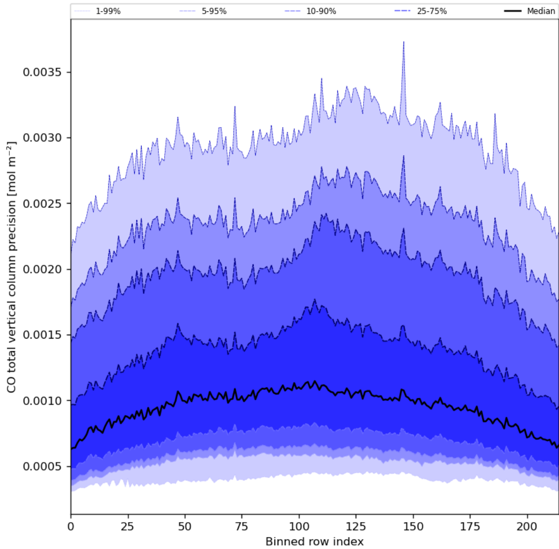
Figure 28: Along track statistics of “CO total vertical column precision” for 2024-05-10 to 2024-05-12
