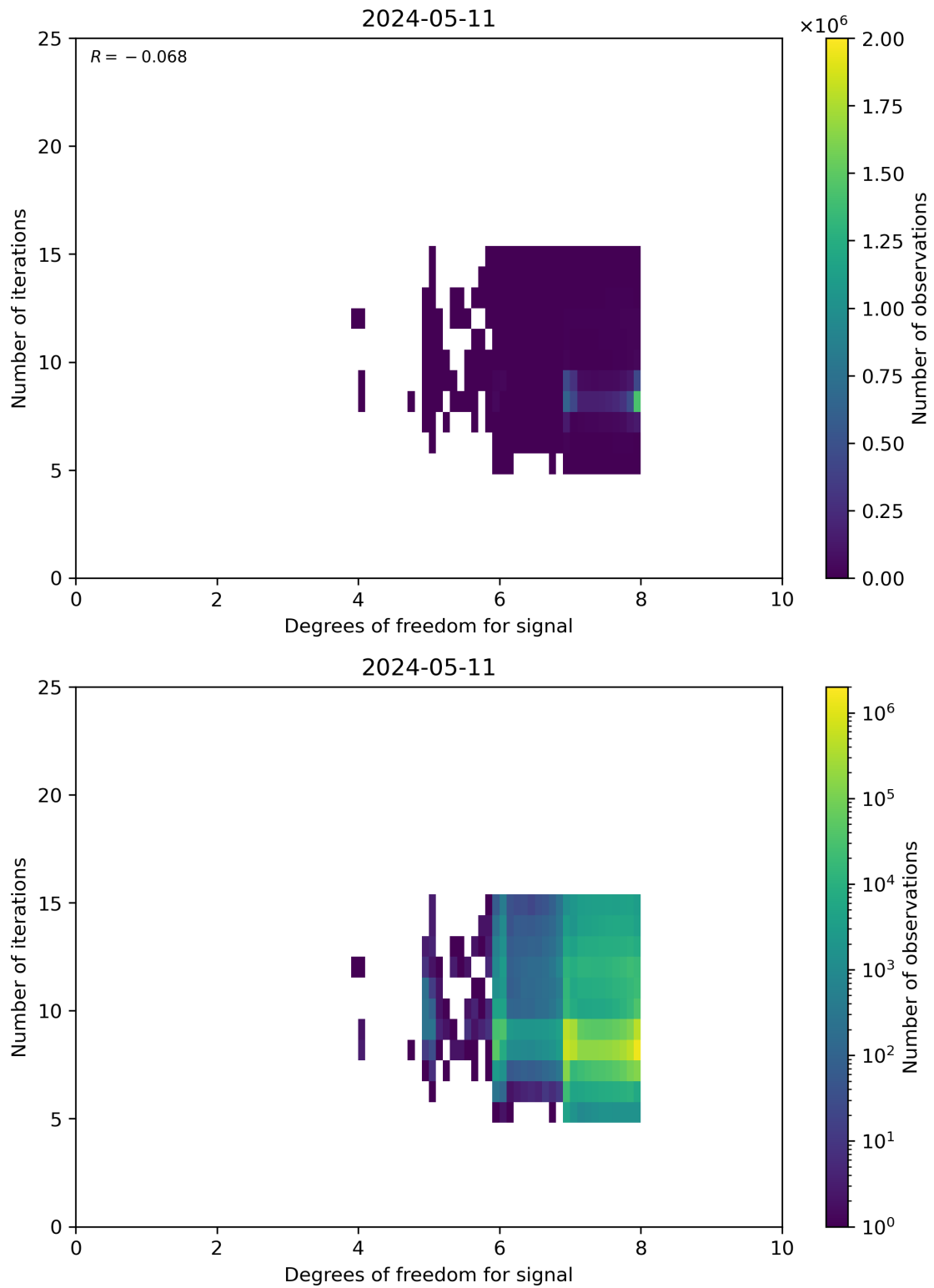
Figure 50: Scatter density plot of “Degrees of freedom for signal” against “Number of iterations” for 2024-05-10 to 2024-05-12.
