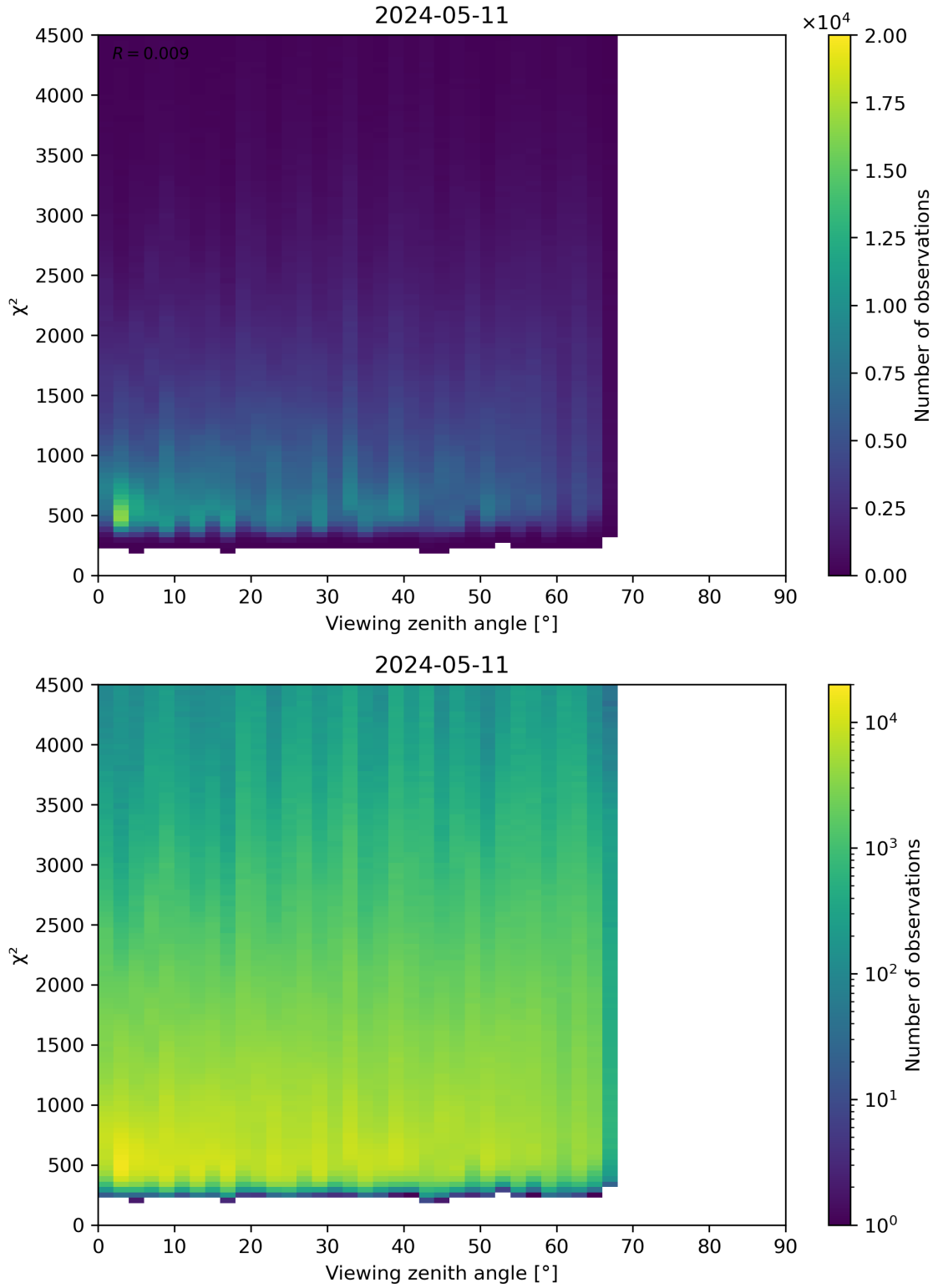
Figure 72: Scatter density plot of “Viewing zenith angle” against “ \chi^2 ” for 2024-05-10 to 2024-05-12.
