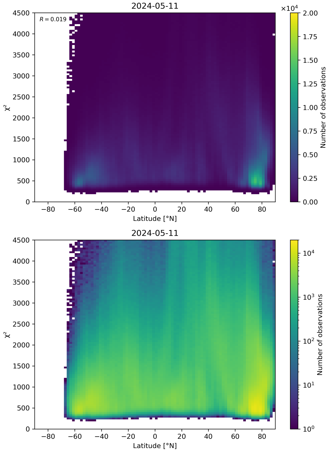
Figure 54: Scatter density plot of “Latitude” against “ \chi^2 ” for 2024-05-10 to 2024-05-12.
