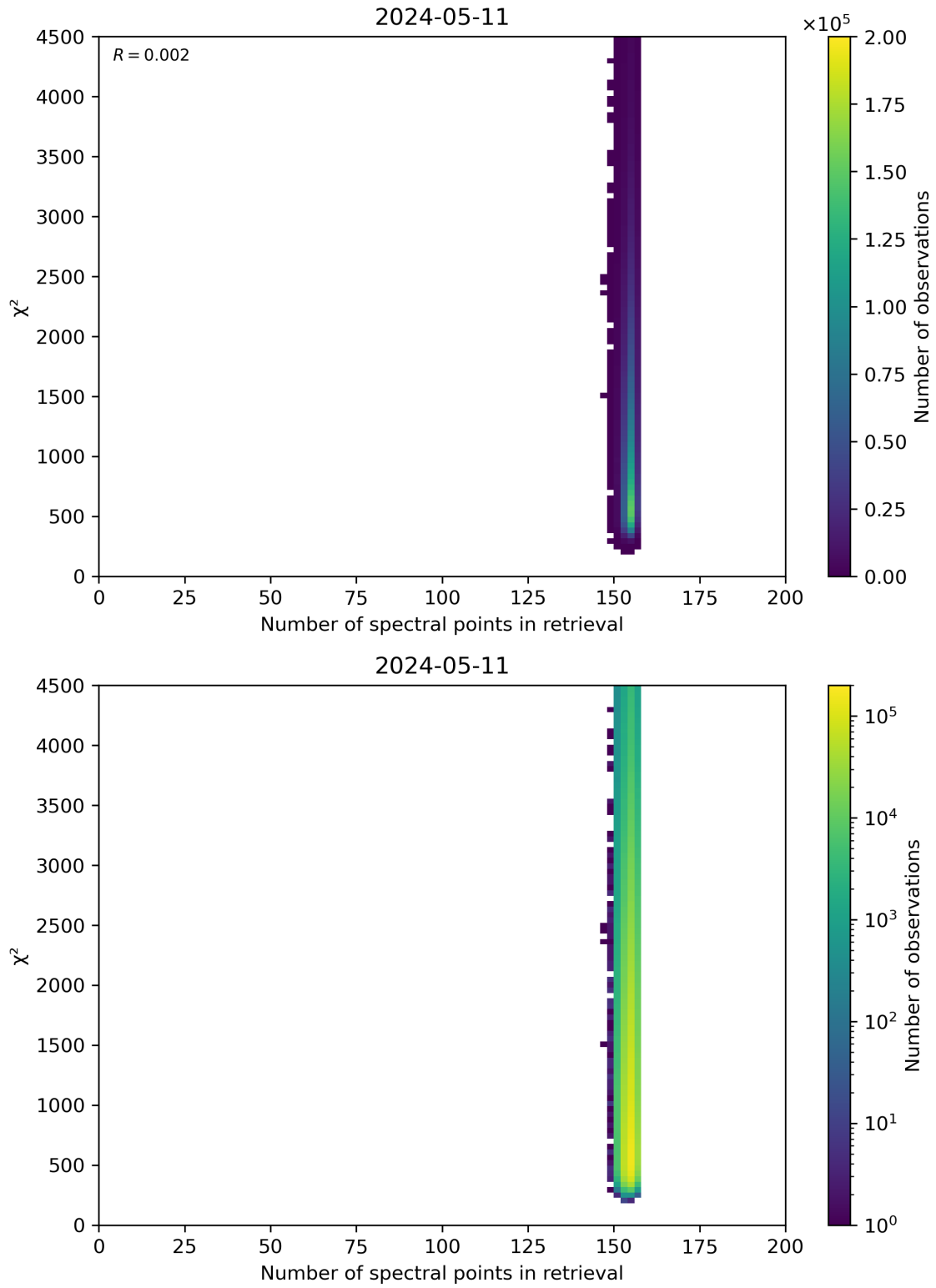
Figure 58: Scatter density plot of “Number of spectral points in retrieval” against “ \chi^2 ” for 2024-05-10 to 2024-05-12.
