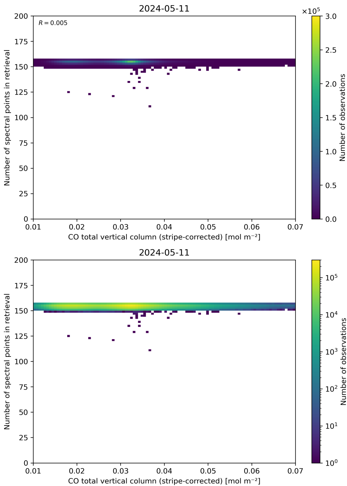
Figure 40: Scatter density plot of “CO total vertical column (stripe-corrected)” against “Number of spectral points in retrieval” for 2024-05-10 to 2024-05-12.
