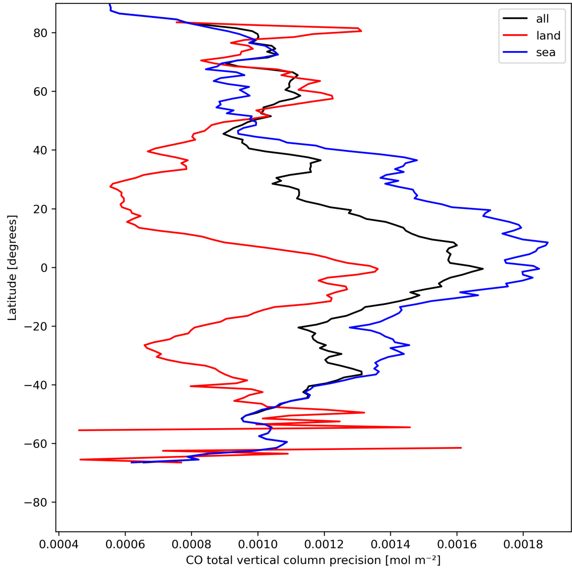
Figure 12: Zonal average of “CO total vertical column precision” for 2024-05-10 to 2024-05-12.
