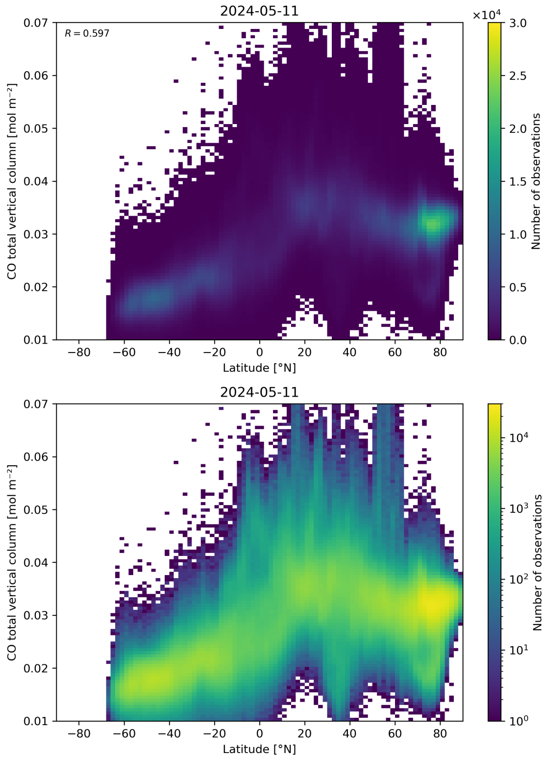
Figure 51: Scatter density plot of “Latitude” against “CO total vertical column” for 2024-05-10 to 2024-05-12.
