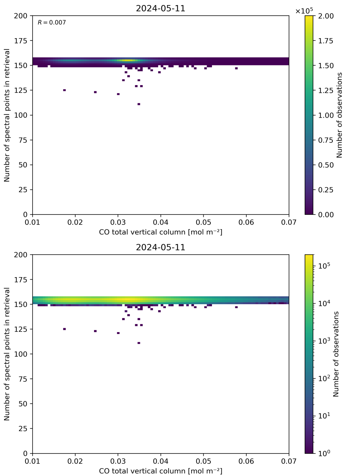
Figure 43: Scatter density plot of “CO total vertical column” against “Number of spectral points in retrieval” for 2024-05-10 to 2024-05-12.
