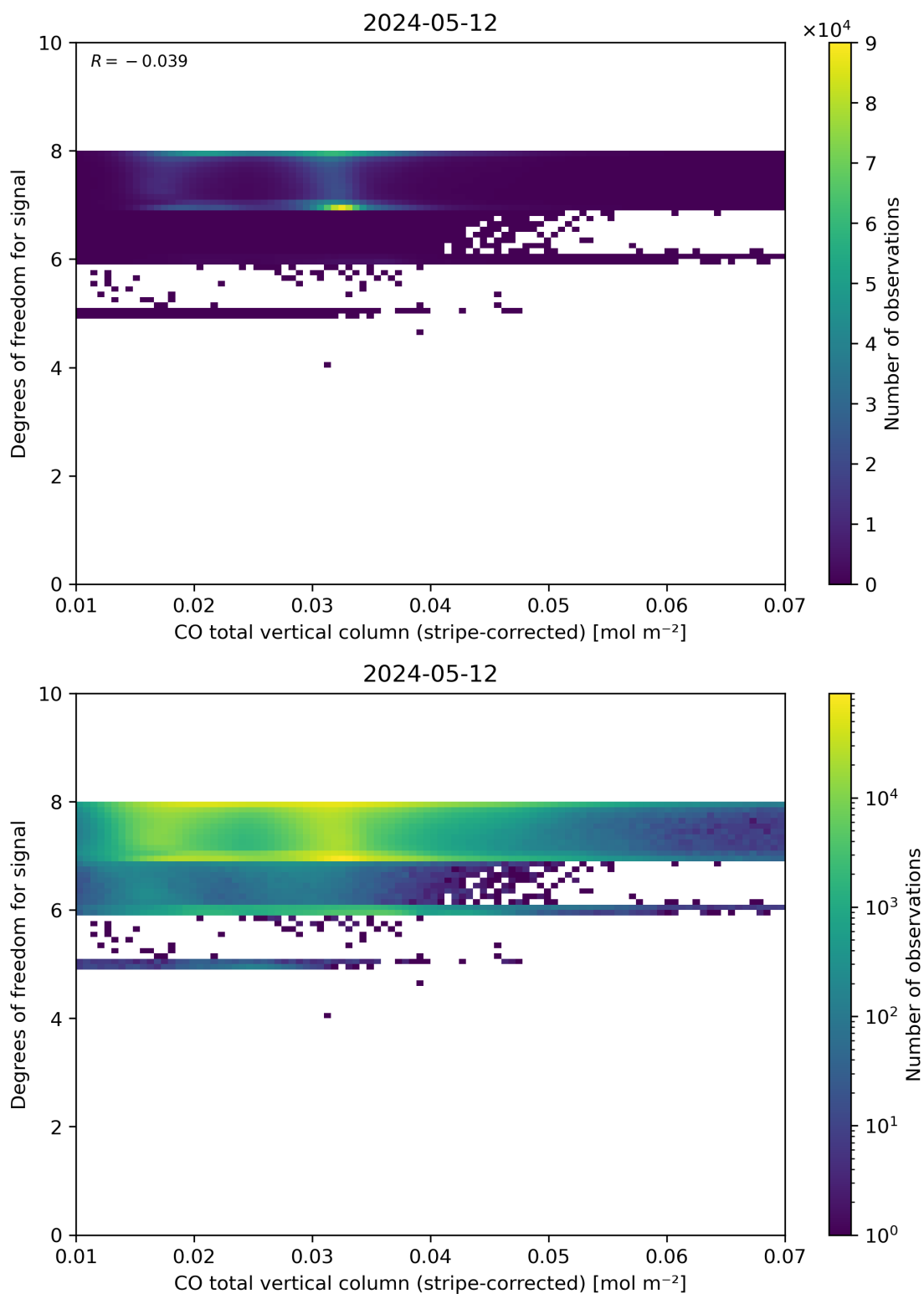
Figure 38: Scatter density plot of “CO total vertical column (stripe-corrected)” against “Degrees of freedom for signal” for 2024-05-12 to 2024-05-13.
