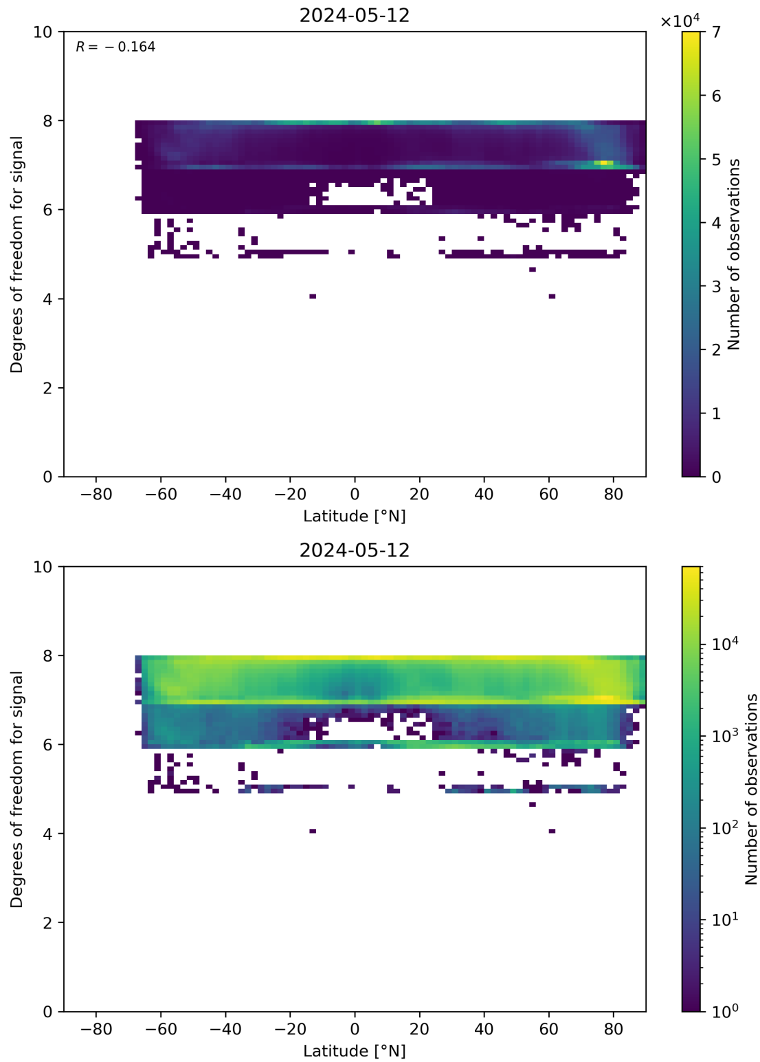
Figure 55: Scatter density plot of “Latitude” against “Degrees of freedom for signal” for 2024-05-12 to 2024-05-13.
