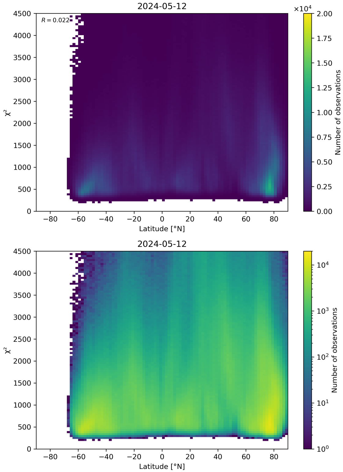
Figure 54: Scatter density plot of “Latitude” against “ \chi^2 ” for 2024-05-12 to 2024-05-13.
