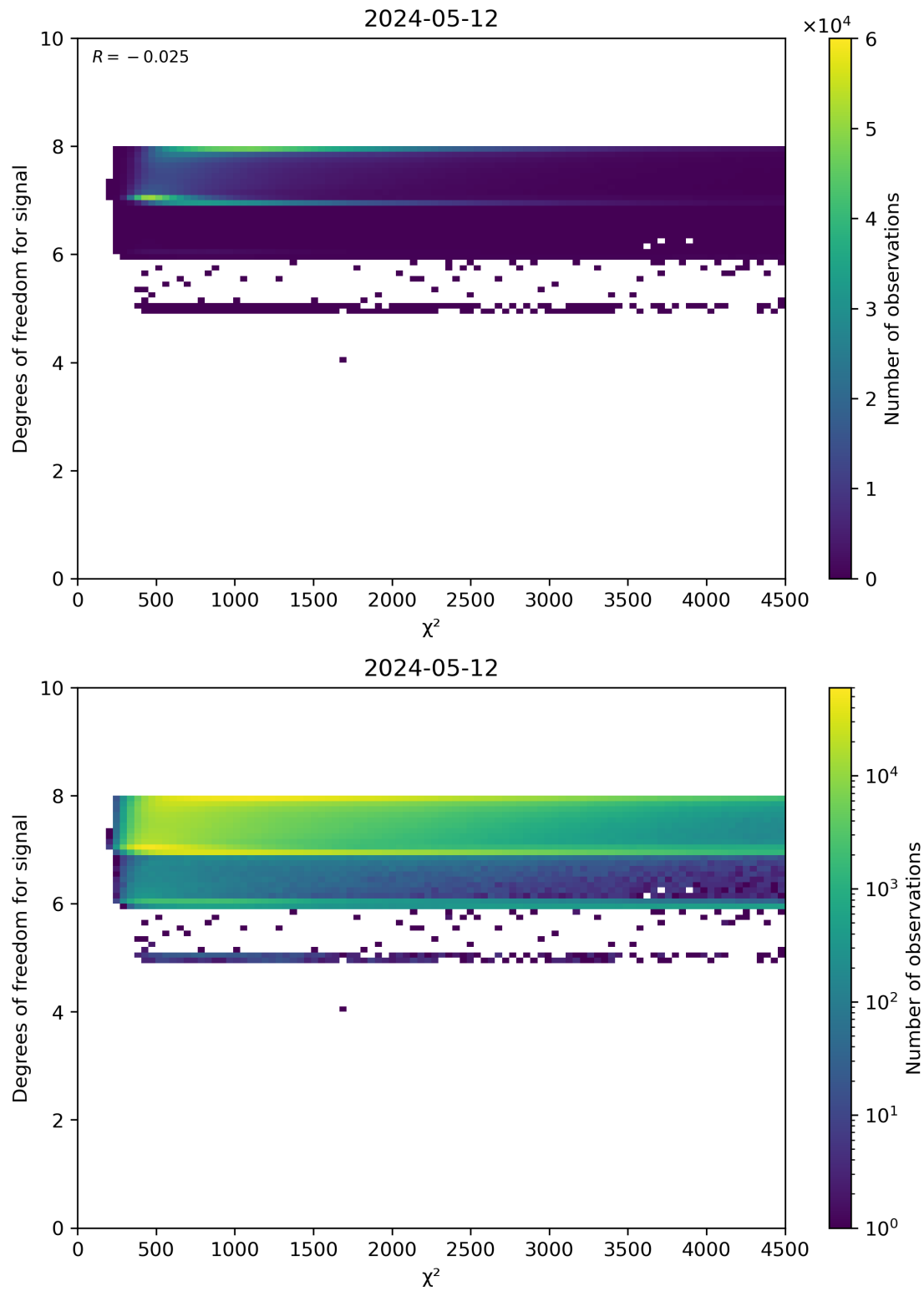
Figure 48: Scatter density plot of “ \chi^2 ” against “Degrees of freedom for signal” for 2024-05-12 to 2024-05-13.
