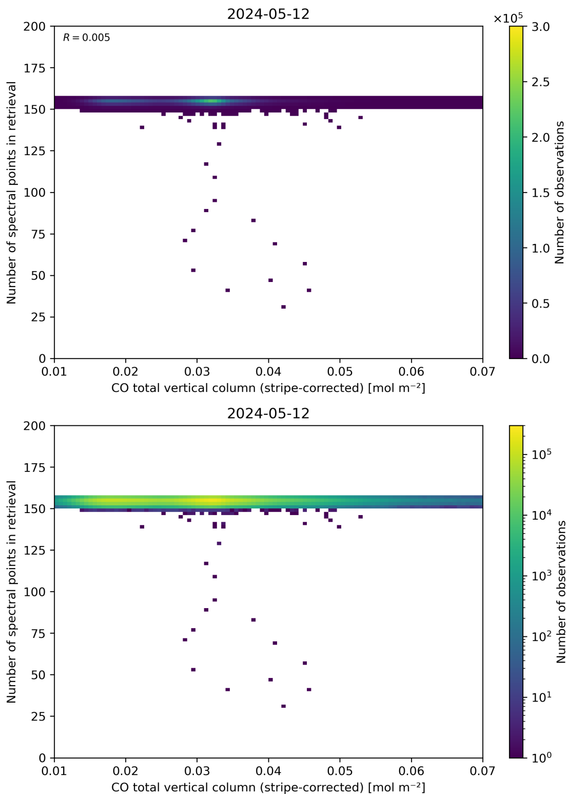
Figure 40: Scatter density plot of “CO total vertical column (stripe-corrected)” against “Number of spectral points in retrieval” for 2024-05-12 to 2024-05-13.
