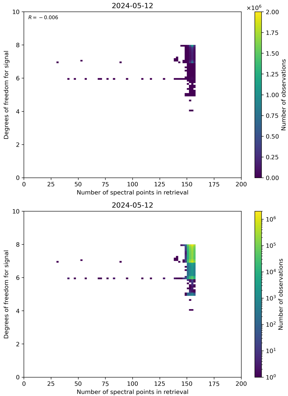
Figure 59: Scatter density plot of “Number of spectral points in retrieval” against “Degrees of freedom for signal” for 2024-05-12 to 2024-05-13.
