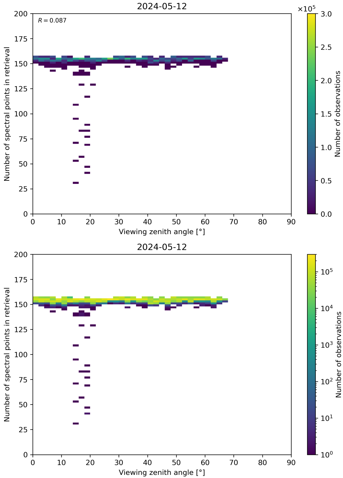
Figure 76: Scatter density plot of “Viewing zenith angle” against “Number of spectral points in retrieval” for 2024-05-12 to 2024-05-13.
