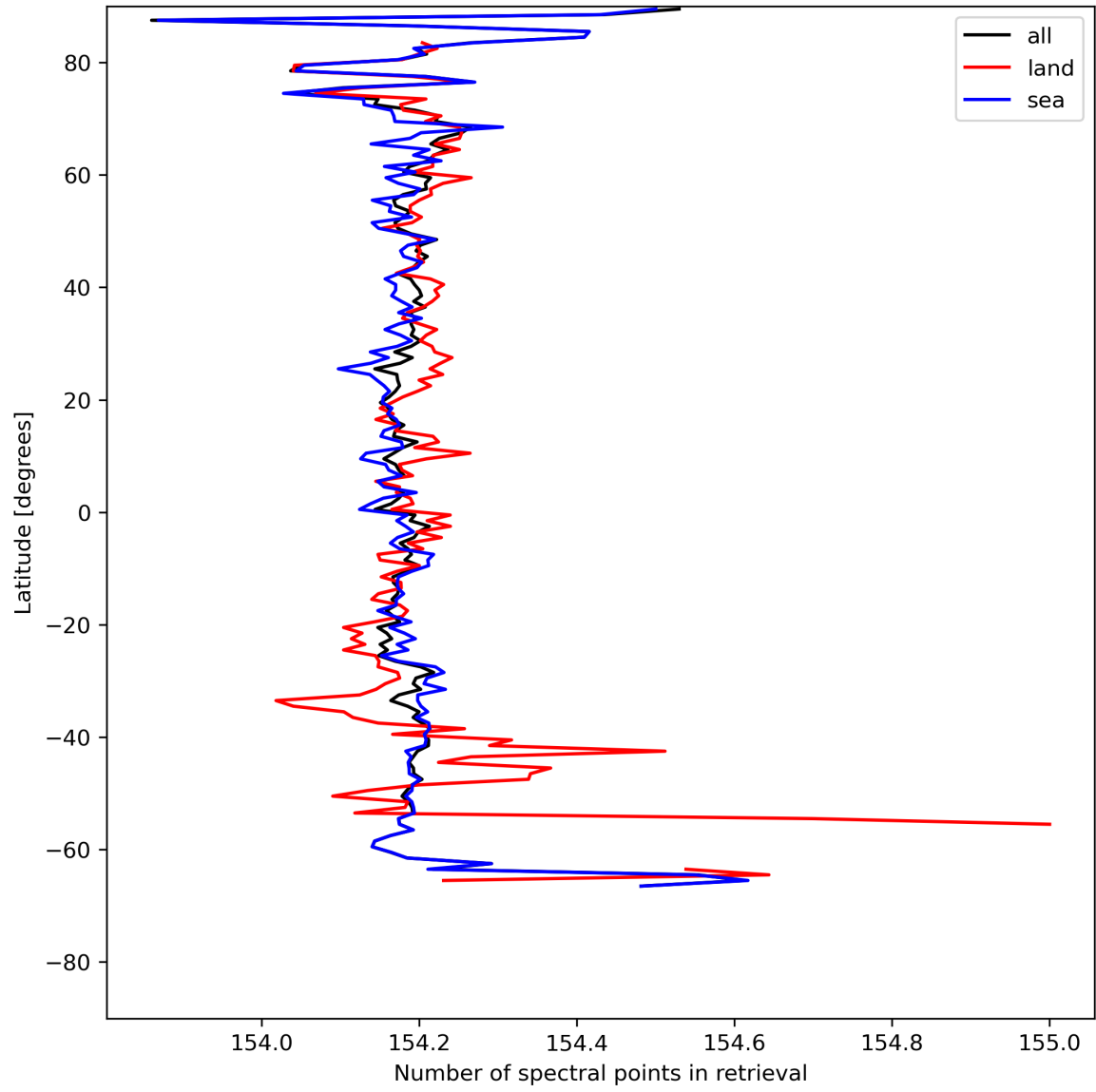
Figure 13: Zonal average of “Number of spectral points in retrieval” for 2024-05-12 to 2024-05-13.
