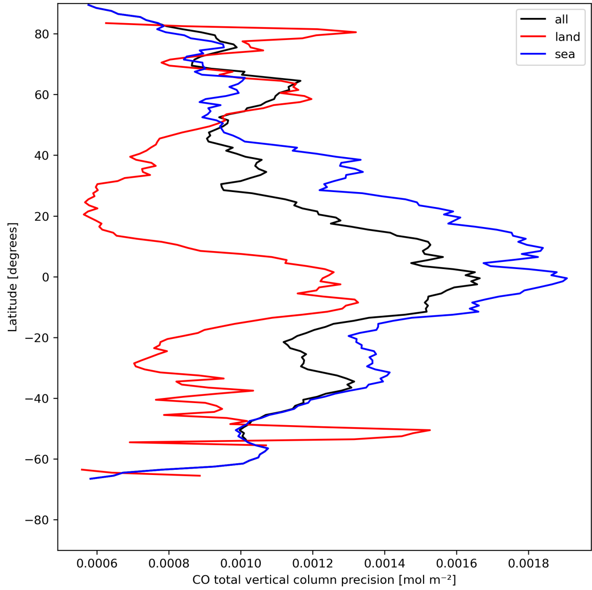
Figure 12: Zonal average of “CO total vertical column precision” for 2024-05-12 to 2024-05-13.
