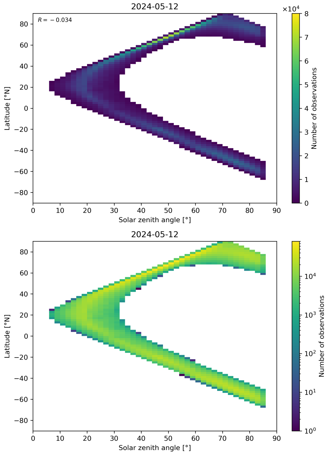
Figure 66: Scatter density plot of “Solar zenith angle” against “Latitude” for 2024-05-12 to 2024-05-13.
