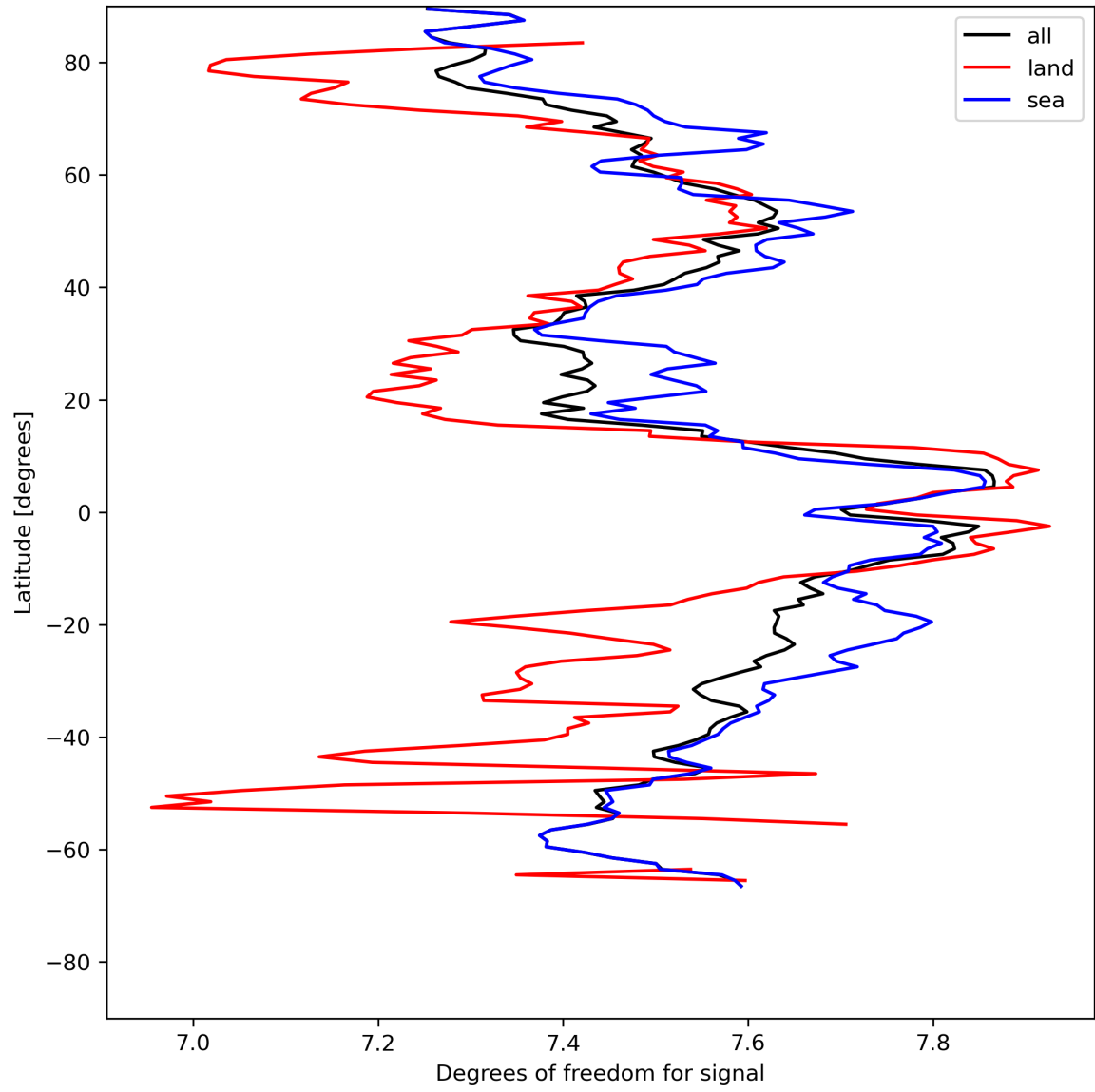
Figure 15: Zonal average of “Degrees of freedom for signal” for 2024-05-12 to 2024-05-13.
