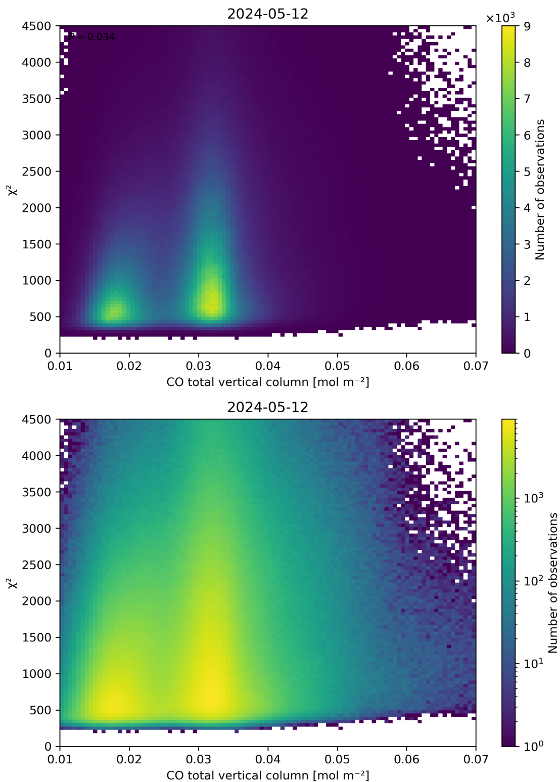
Figure 35: Scatter density plot of “CO total vertical column” against “ \chi^2 ” for 2024-05-12 to 2024-05-13.
