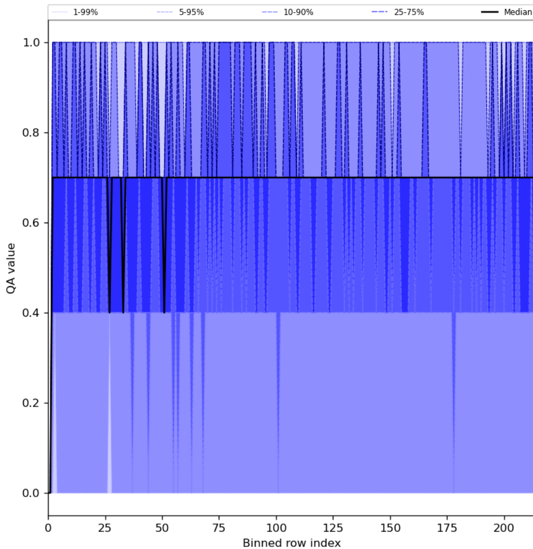
Figure 25: Along track statistics of “QA value” for 2024-05-12 to 2024-05-13
