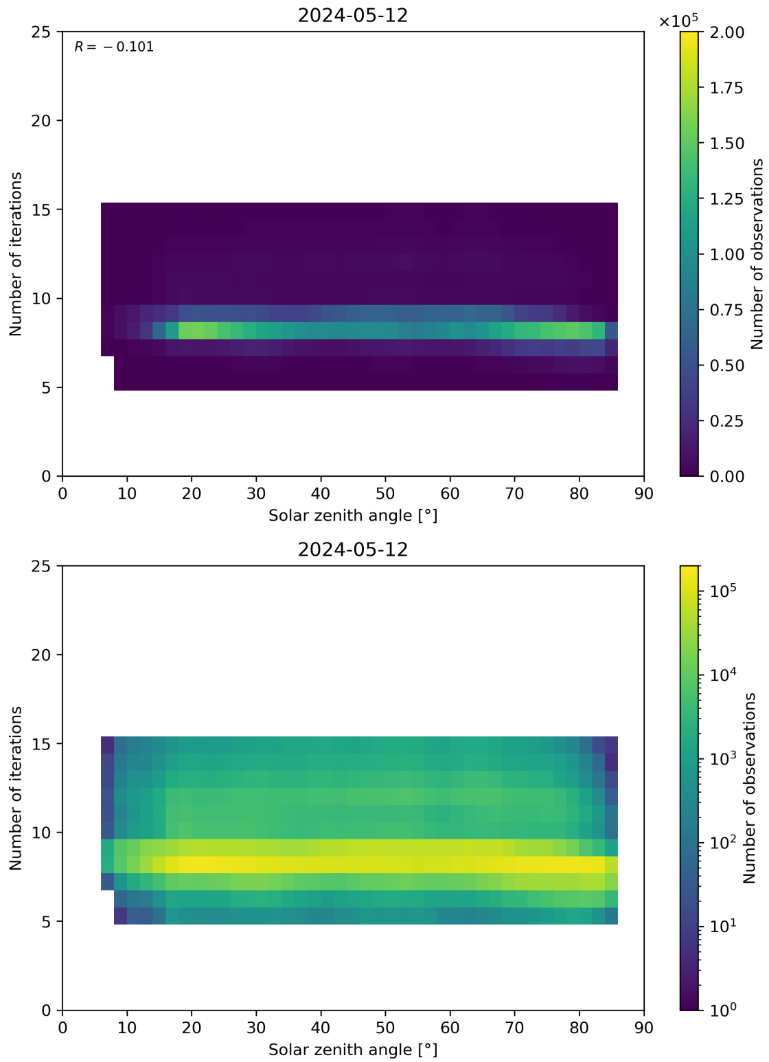
Figure 67: Scatter density plot of “Solar zenith angle” against “Number of iterations” for 2024-05-12 to 2024-05-13.
