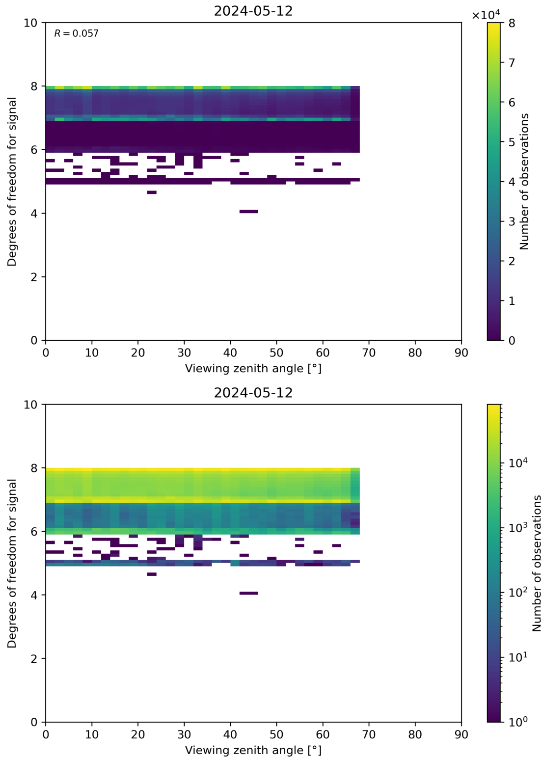
Figure 73: Scatter density plot of “Viewing zenith angle” against “Degrees of freedom for signal” for 2024-05-12 to 2024-05-13.
