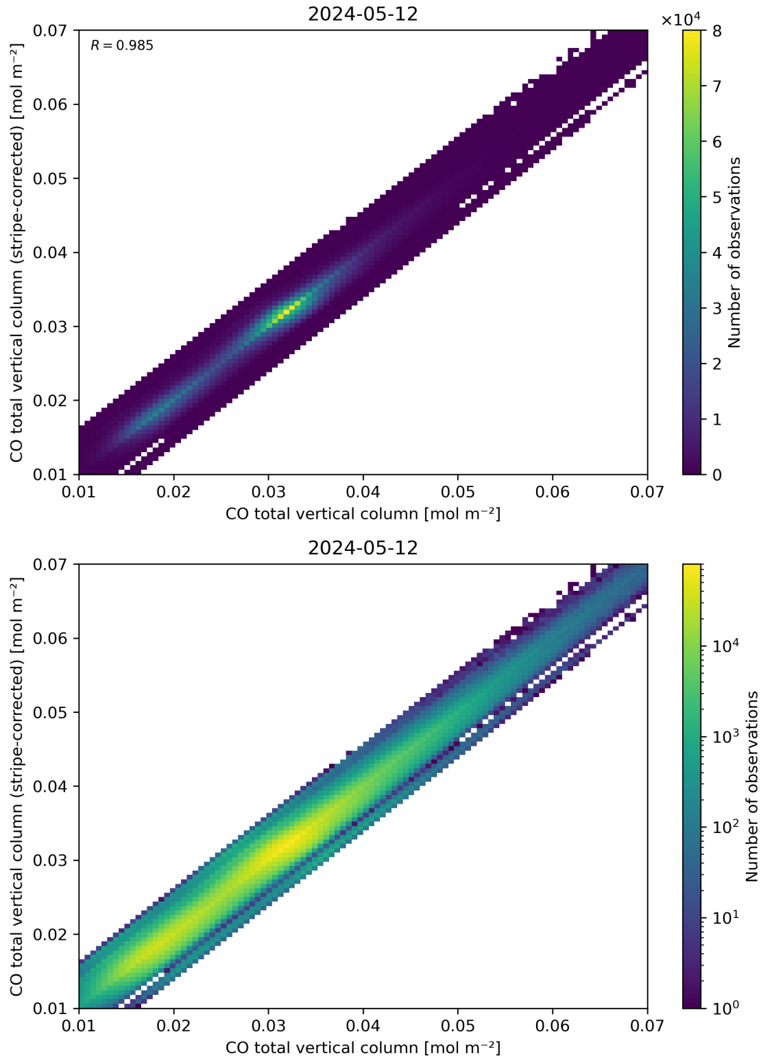
Figure 33: Scatter density plot of “CO total vertical column” against “CO total vertical column (stripe-corrected)” for 2024-05-12 to 2024-05-13.
