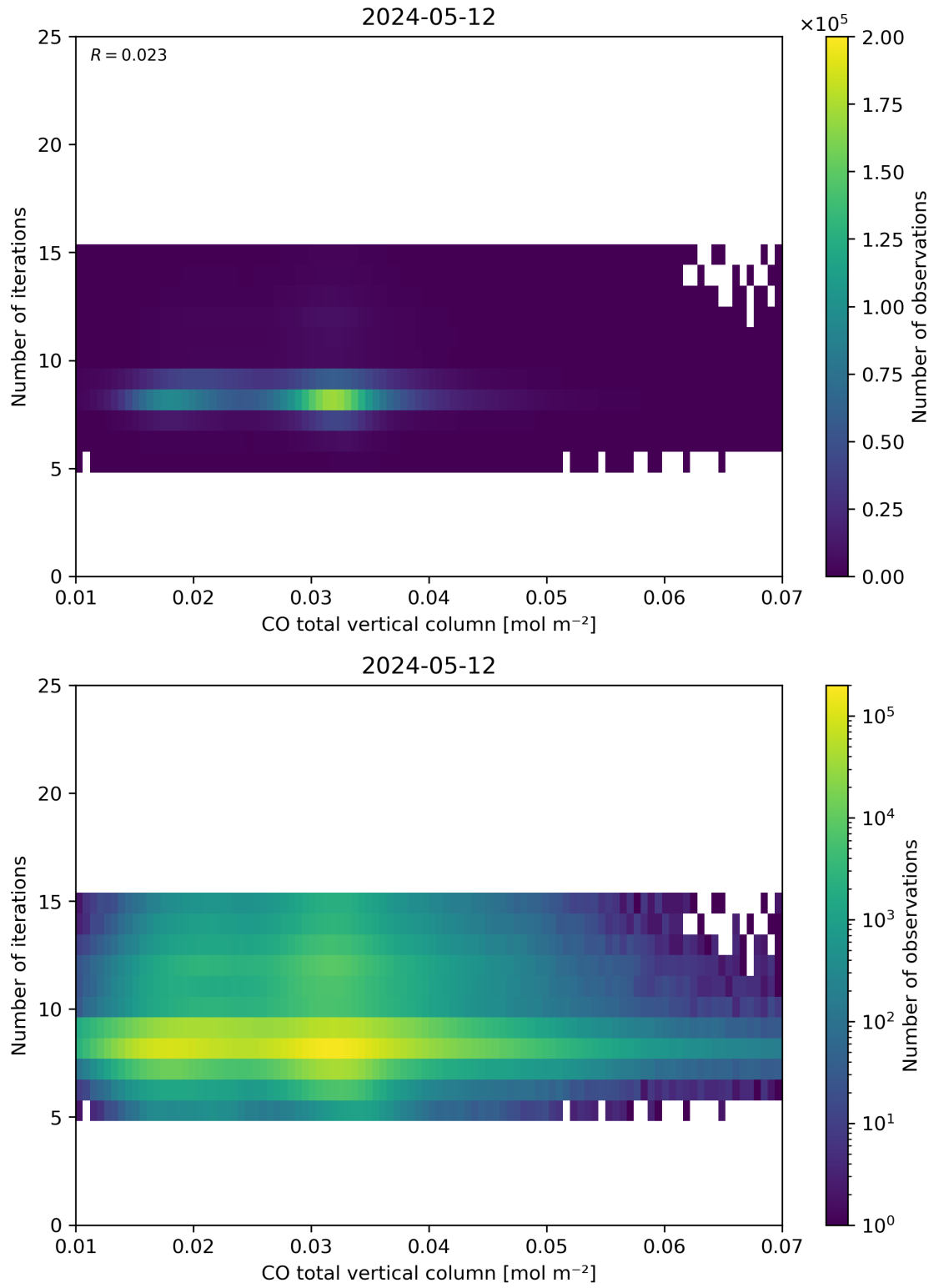
Figure 42: Scatter density plot of “CO total vertical column” against “Number of iterations” for 2024-05-12 to 2024-05-13.
