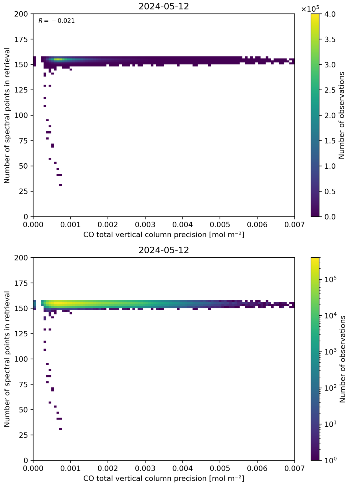
Figure 47: Scatter density plot of “CO total vertical column precision” against “Number of spectral points in retrieval” for 2024-05-12 to 2024-05-13.
