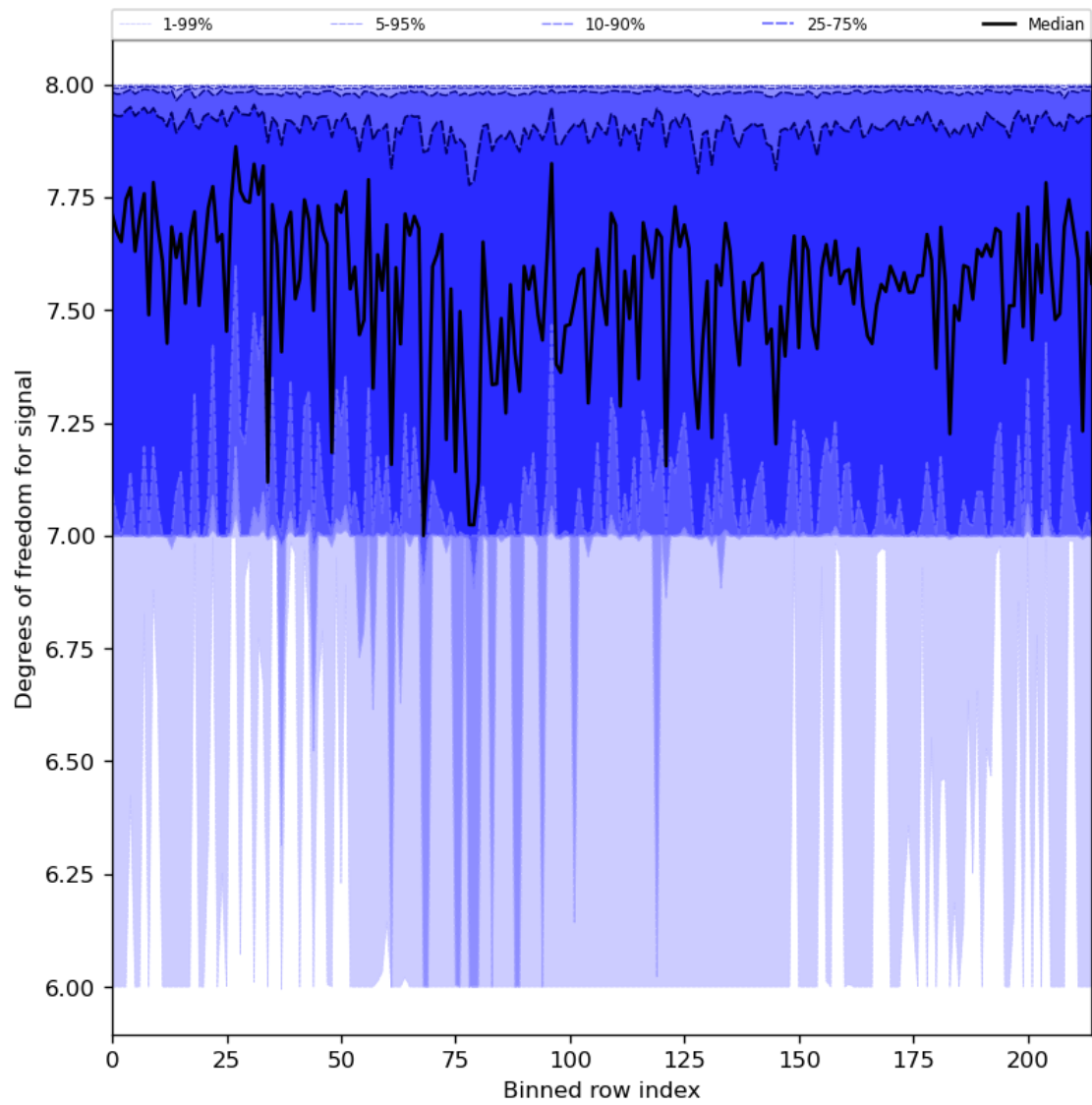
Figure 31: Along track statistics of “Degrees of freedom for signal” for 2024-05-12 to 2024-05-13
