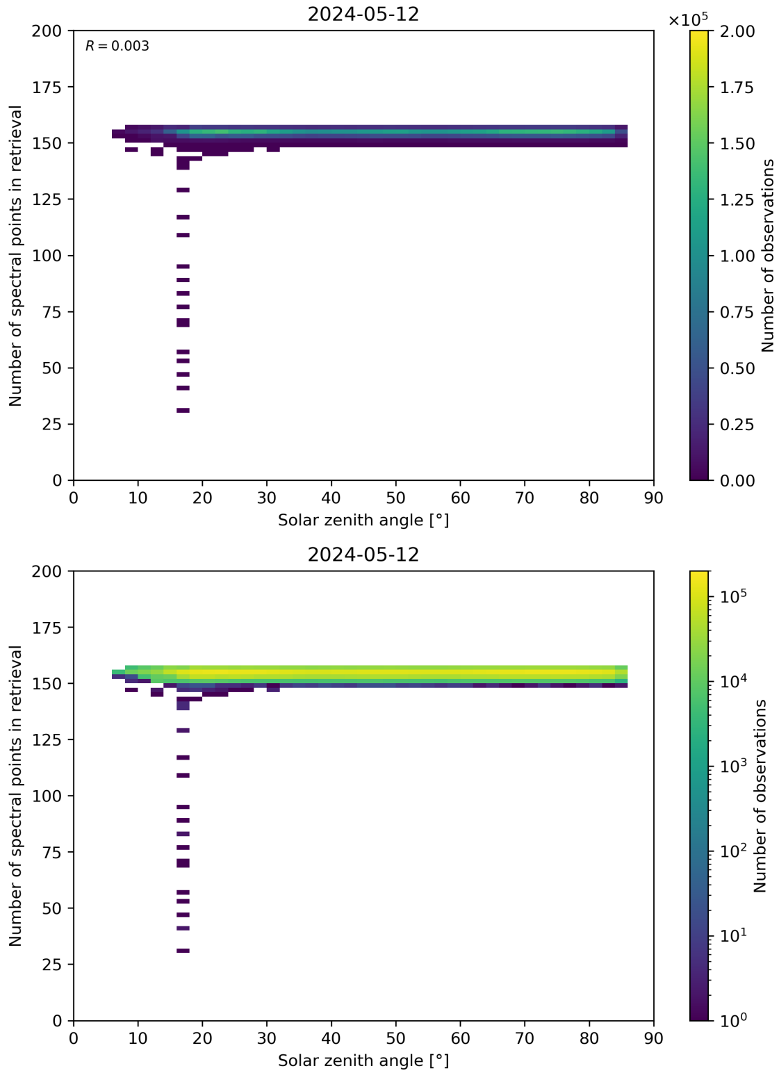
Figure 68: Scatter density plot of “Solar zenith angle” against “Number of spectral points in retrieval” for 2024-05-12 to 2024-05-13.
