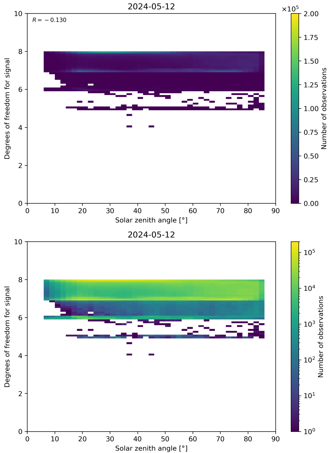
Figure 65: Scatter density plot of “Solar zenith angle” against “Degrees of freedom for signal” for 2024-05-12 to 2024-05-13.
