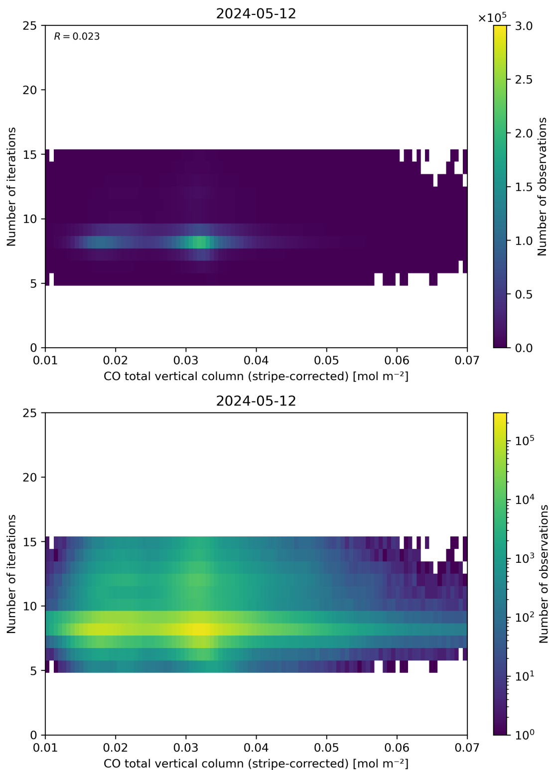
Figure 39: Scatter density plot of “CO total vertical column (stripe-corrected)” against “Number of iterations” for 2024-05-12 to 2024-05-13.
