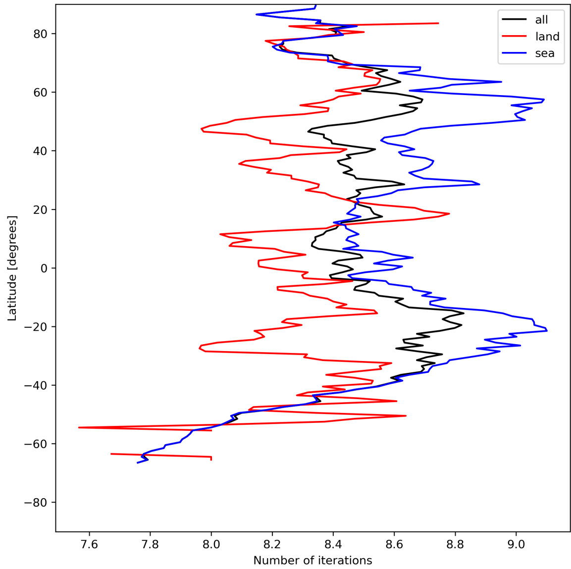
Figure 16: Zonal average of “Number of iterations” for 2024-05-12 to 2024-05-13.
