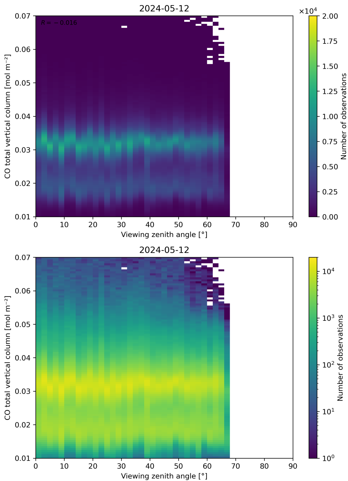
Figure 69: Scatter density plot of “Viewing zenith angle” against “CO total vertical column” for 2024-05-12 to 2024-05-13.
