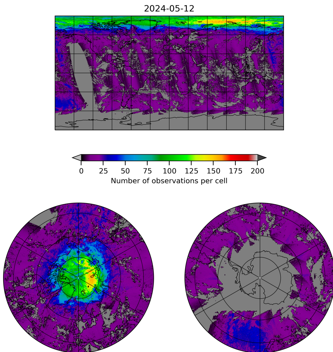
Figure 8: Map of the number of observations for 2024-05-12 to 2024-05-13
