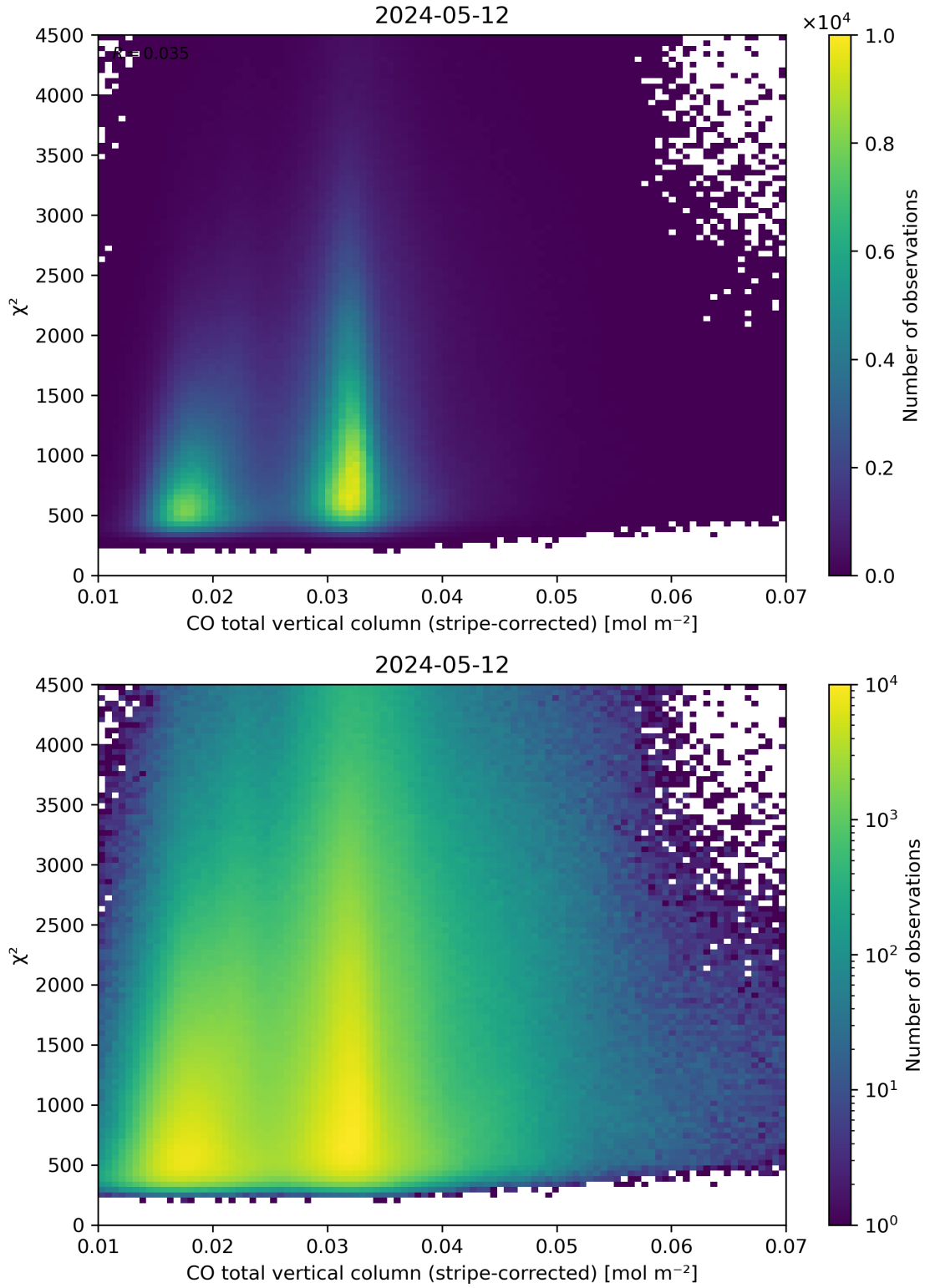
Figure 37: Scatter density plot of “CO total vertical column (stripe-corrected)” against “ \chi^2 ” for 2024-05-12 to 2024-05-13.
