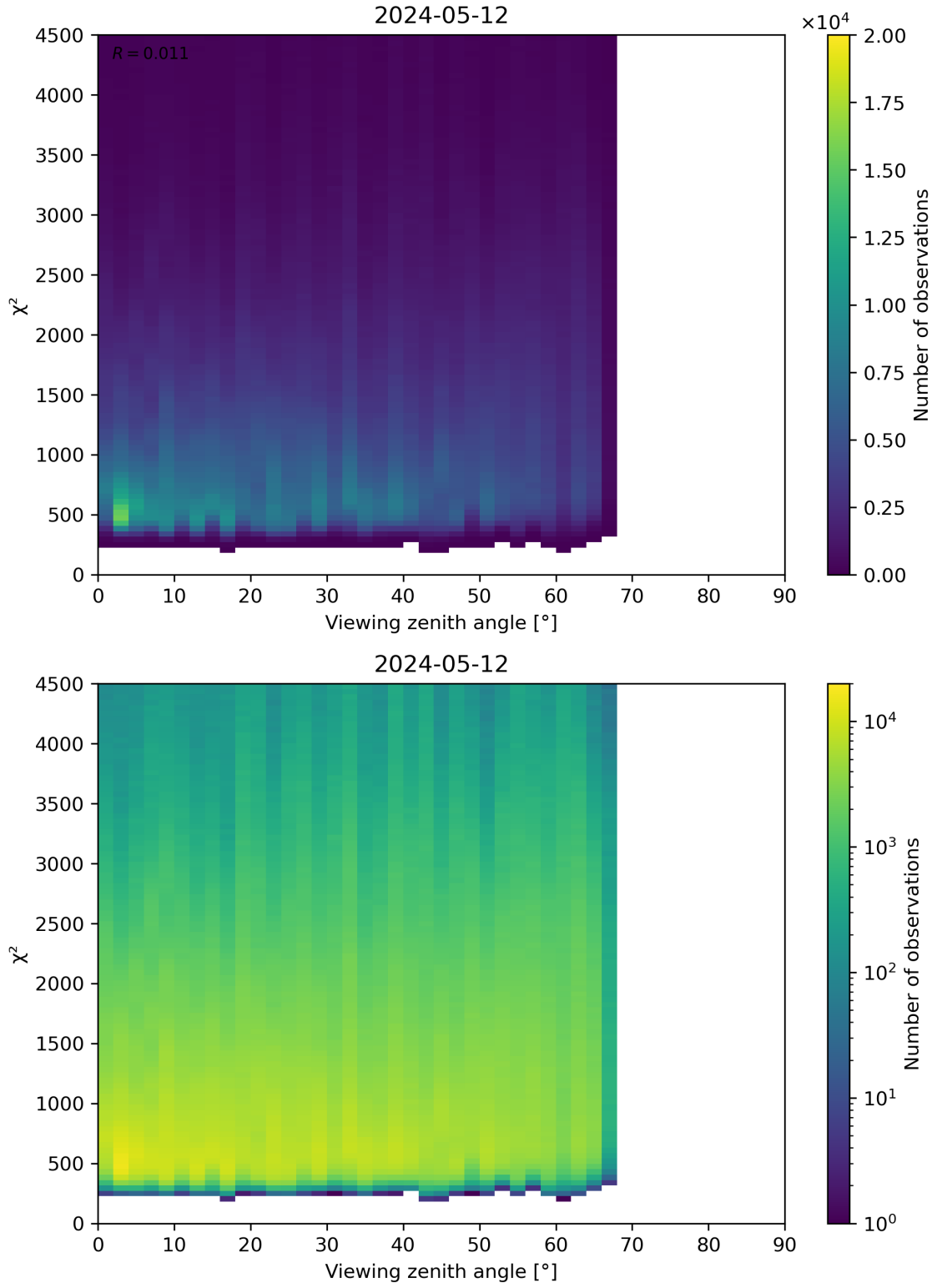
Figure 72: Scatter density plot of “Viewing zenith angle” against “ \chi^2 ” for 2024-05-12 to 2024-05-13.
