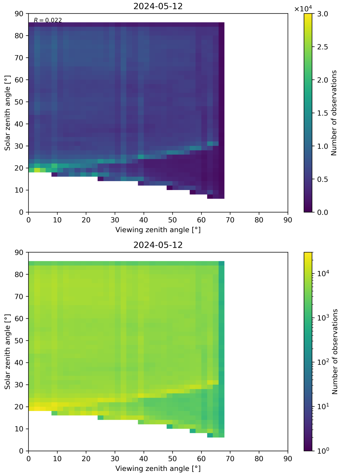
Figure 77: Scatter density plot of “Viewing zenith angle” against “Solar zenith angle” for 2024-05-12 to 2024-05-13.
