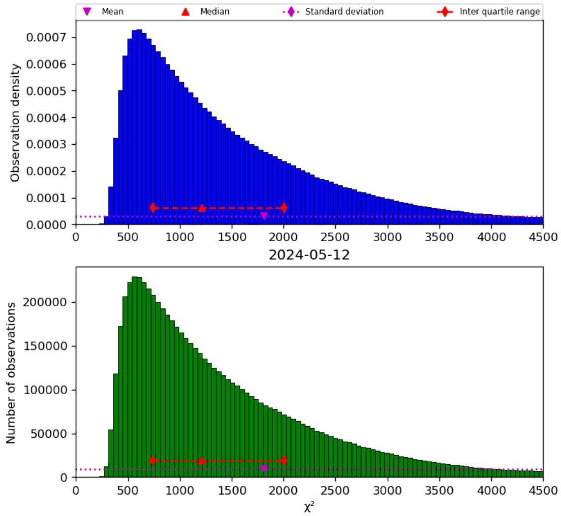
Figure 22: Histogram of “ \chi^2 ” for 2024-05-12 to 2024-05-13
