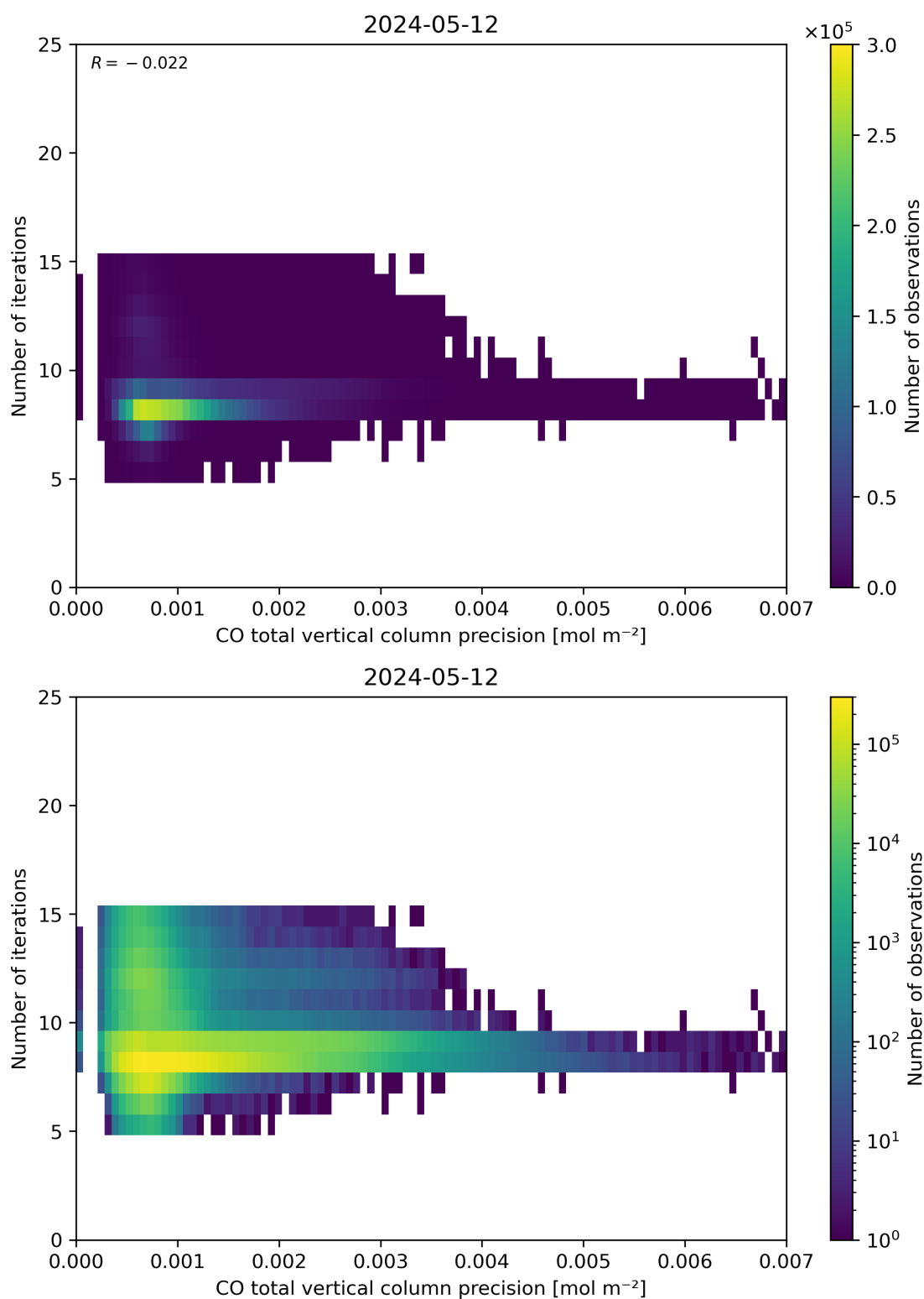
Figure 46: Scatter density plot of “CO total vertical column precision” against “Number of iterations” for 2024-05-12 to 2024-05-13.
