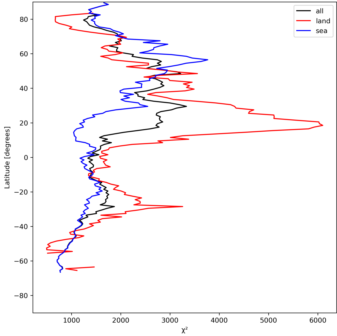
Figure 14: Zonal average of “ \chi^2 ” for 2024-05-12 to 2024-05-13.
