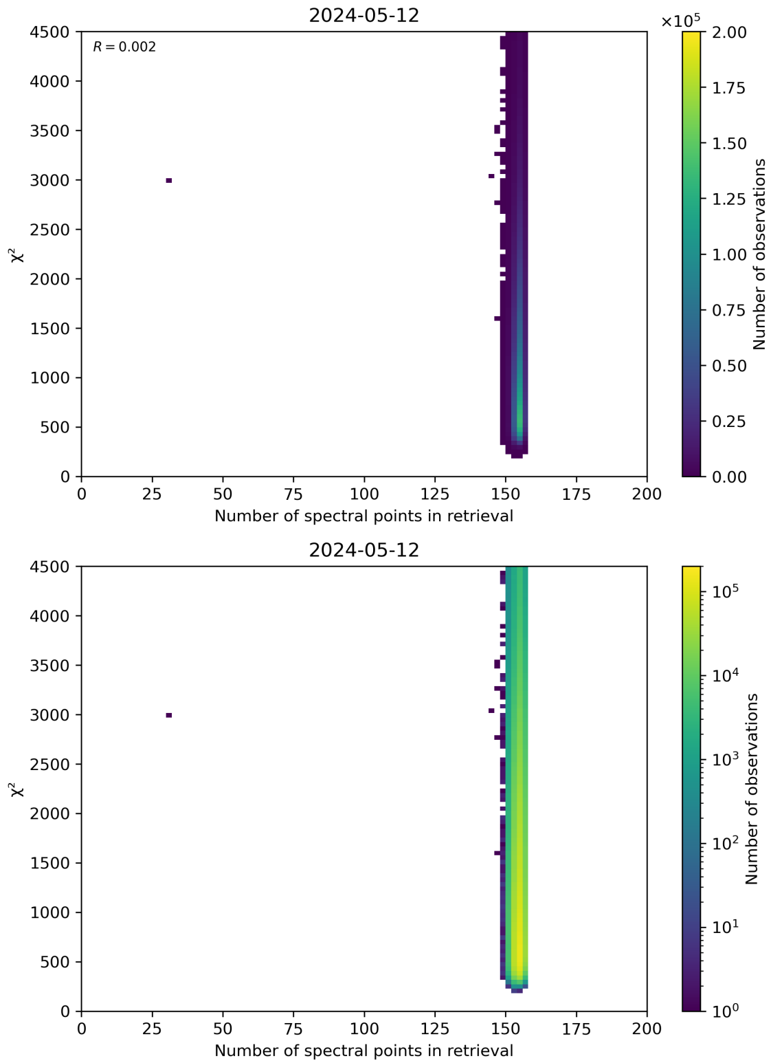
Figure 58: Scatter density plot of “Number of spectral points in retrieval” against “ \chi^2 ” for 2024-05-12 to 2024-05-13.
