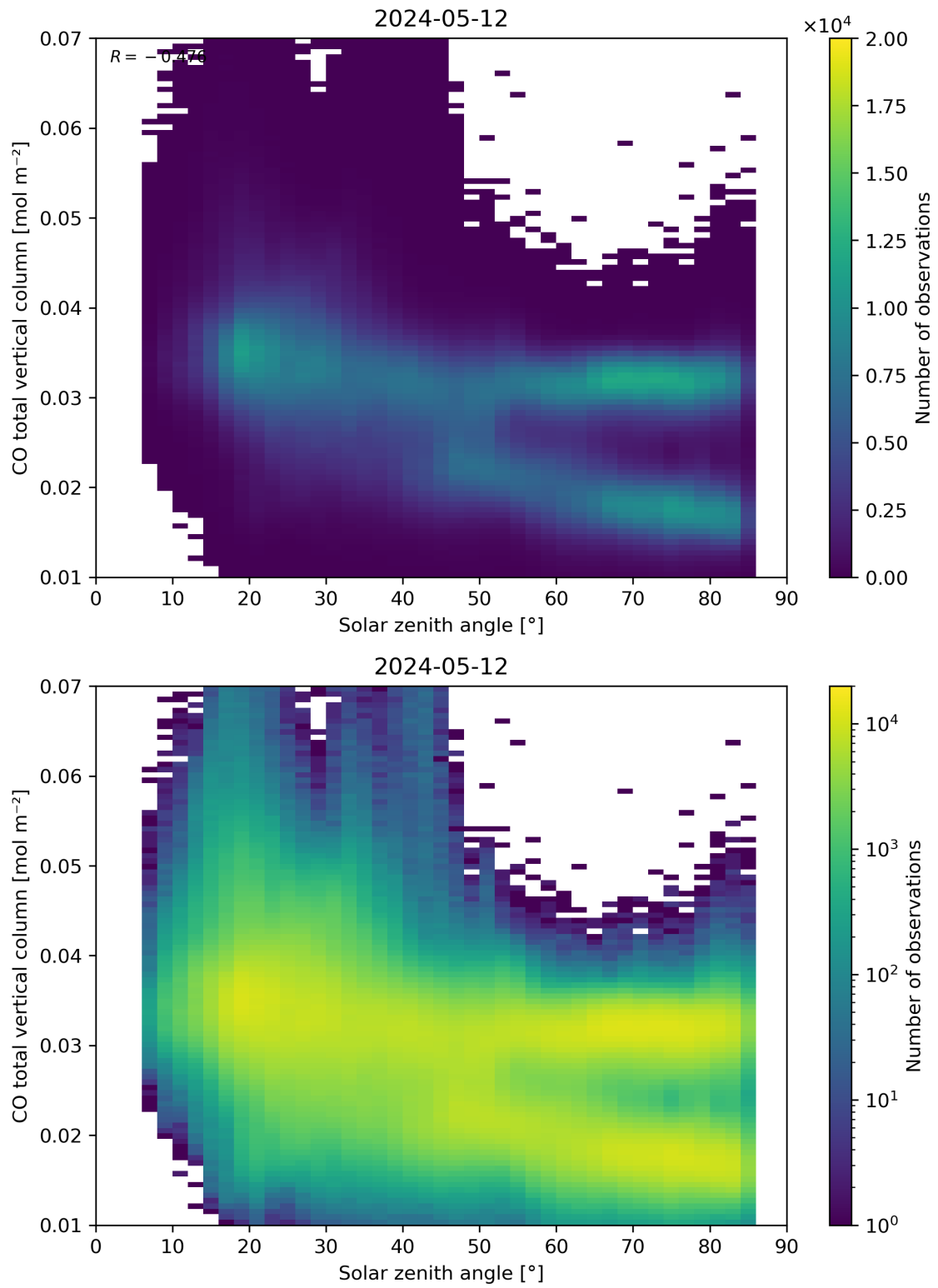
Figure 61: Scatter density plot of “Solar zenith angle” against “CO total vertical column” for 2024-05-12 to 2024-05-13.
