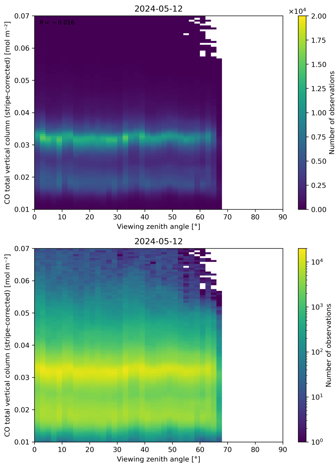
Figure 70: Scatter density plot of “Viewing zenith angle” against “CO total vertical column (stripe-corrected)” for 2024-05-12 to 2024-05-13.
