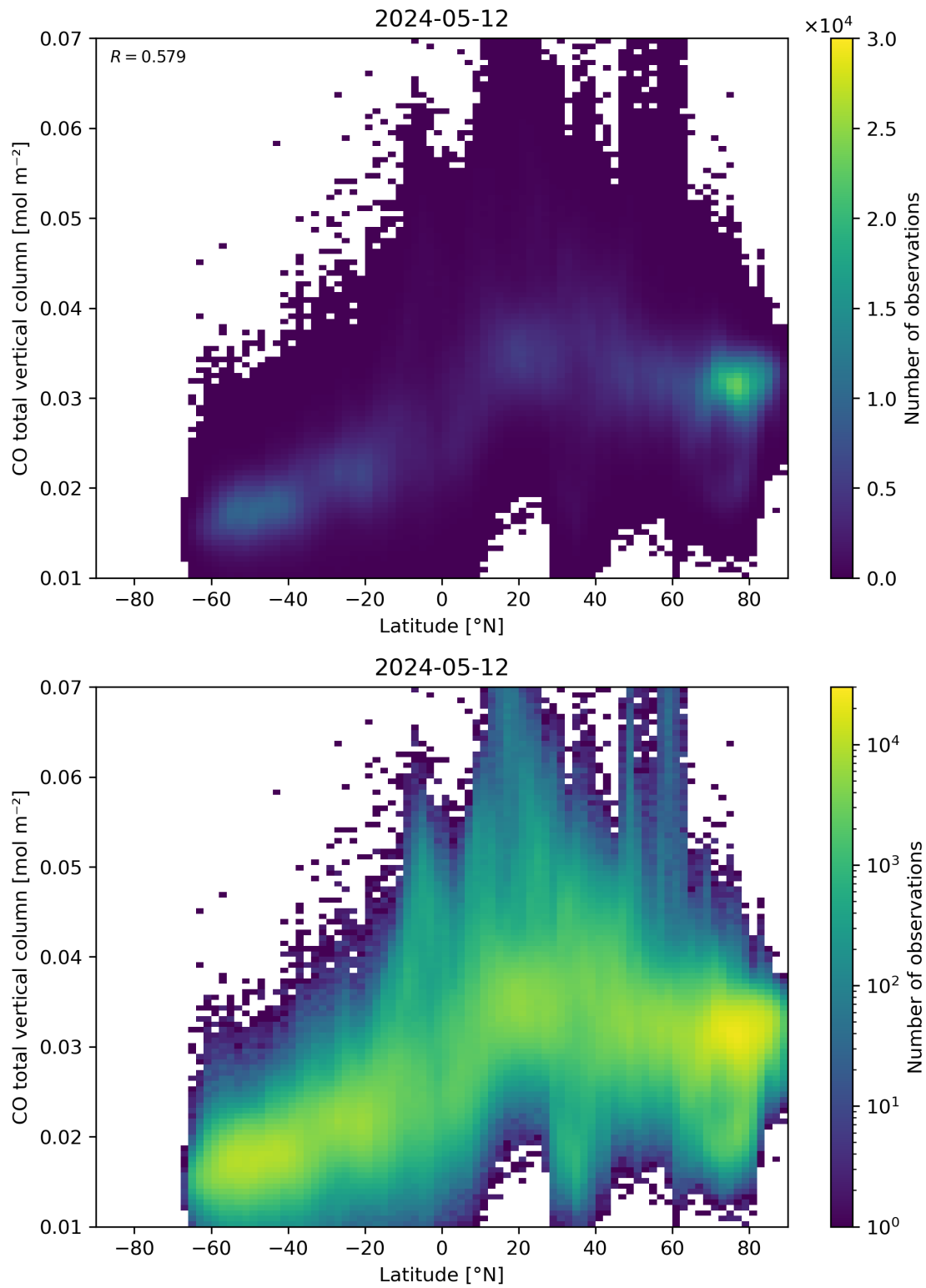
Figure 51: Scatter density plot of “Latitude” against “CO total vertical column” for 2024-05-12 to 2024-05-13.
