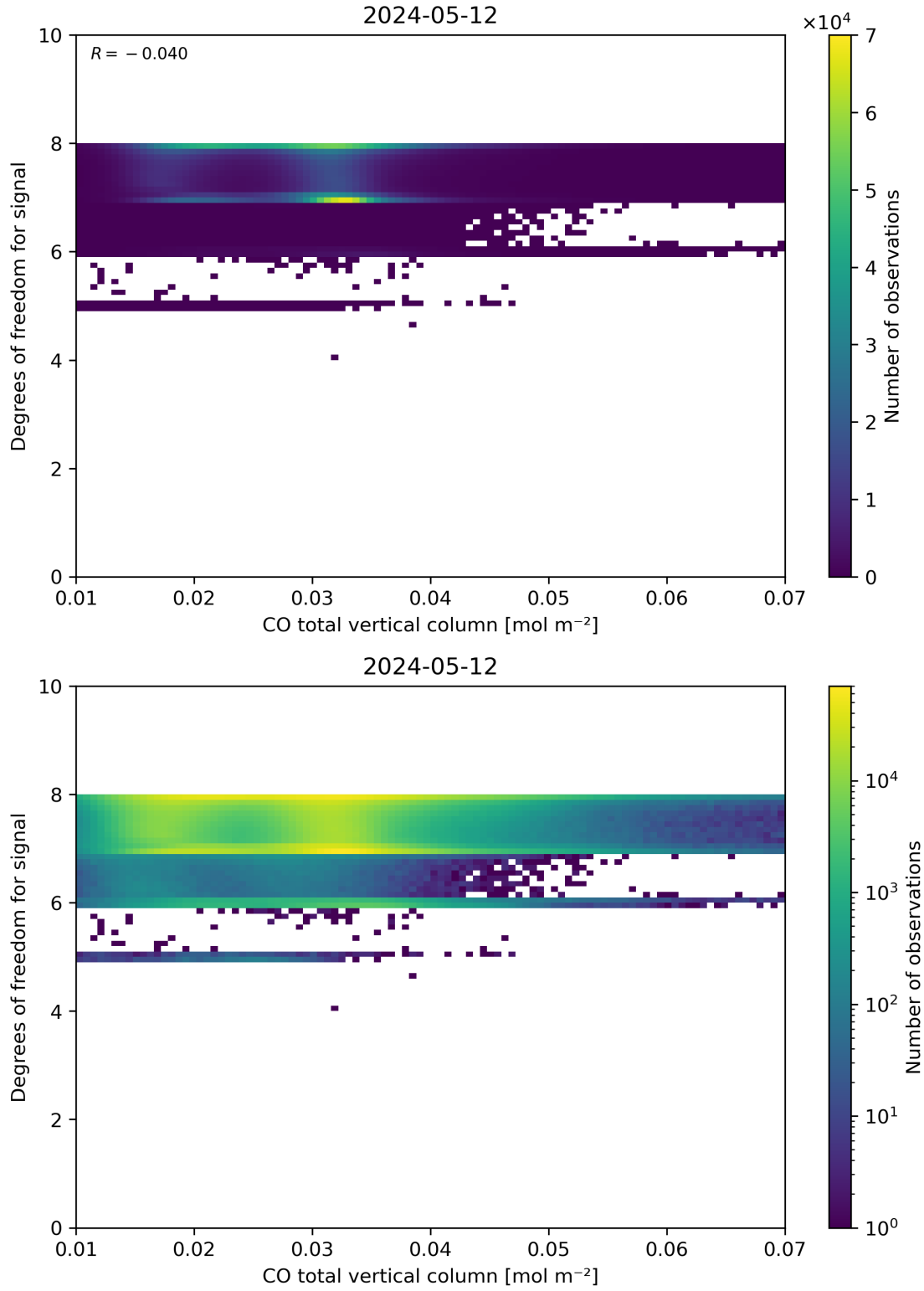
Figure 41: Scatter density plot of “CO total vertical column” against “Degrees of freedom for signal” for 2024-05-12 to 2024-05-13.
