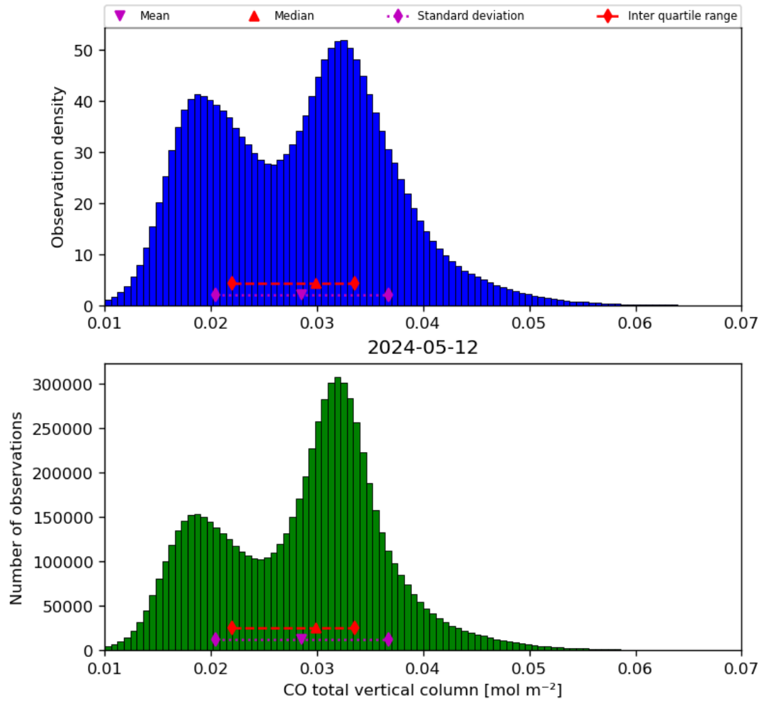
Figure 18: Histogram of “CO total vertical column” for 2024-05-12 to 2024-05-13
