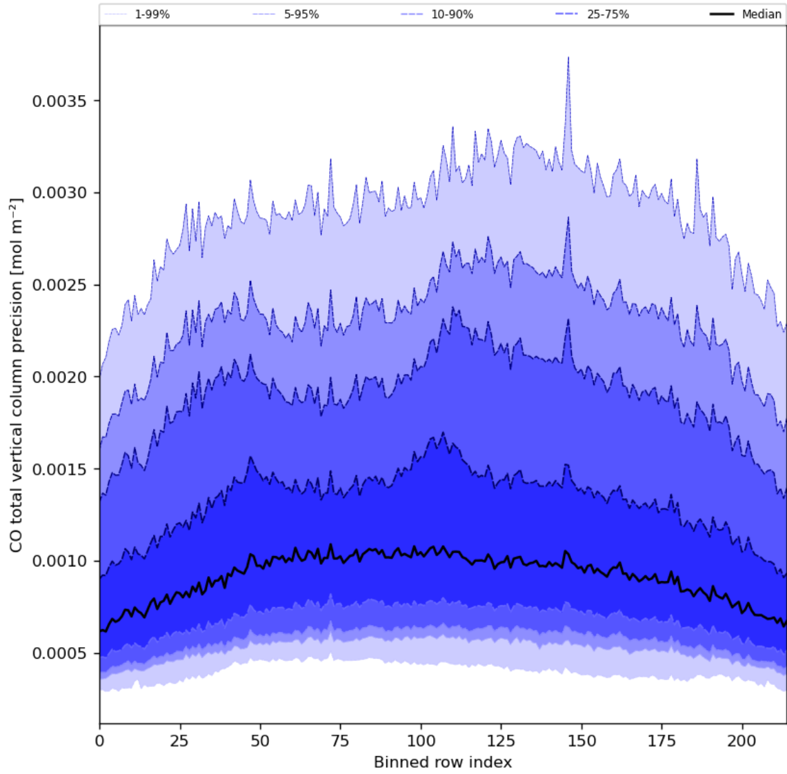
Figure 28: Along track statistics of “CO total vertical column precision” for 2024-05-12 to 2024-05-13
