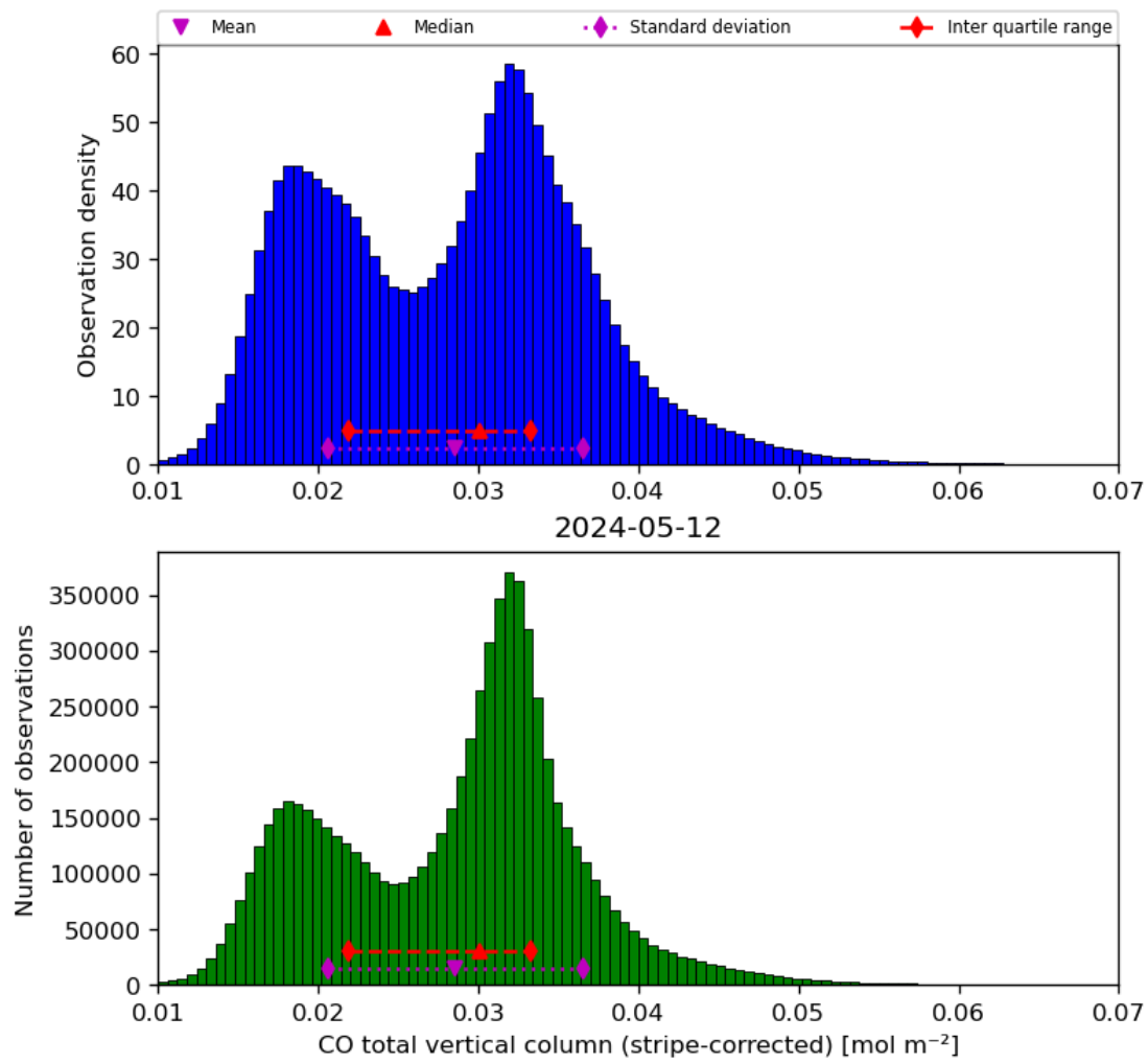
Figure 19: Histogram of “CO total vertical column (stripe-corrected)” for 2024-05-12 to 2024-05-13
