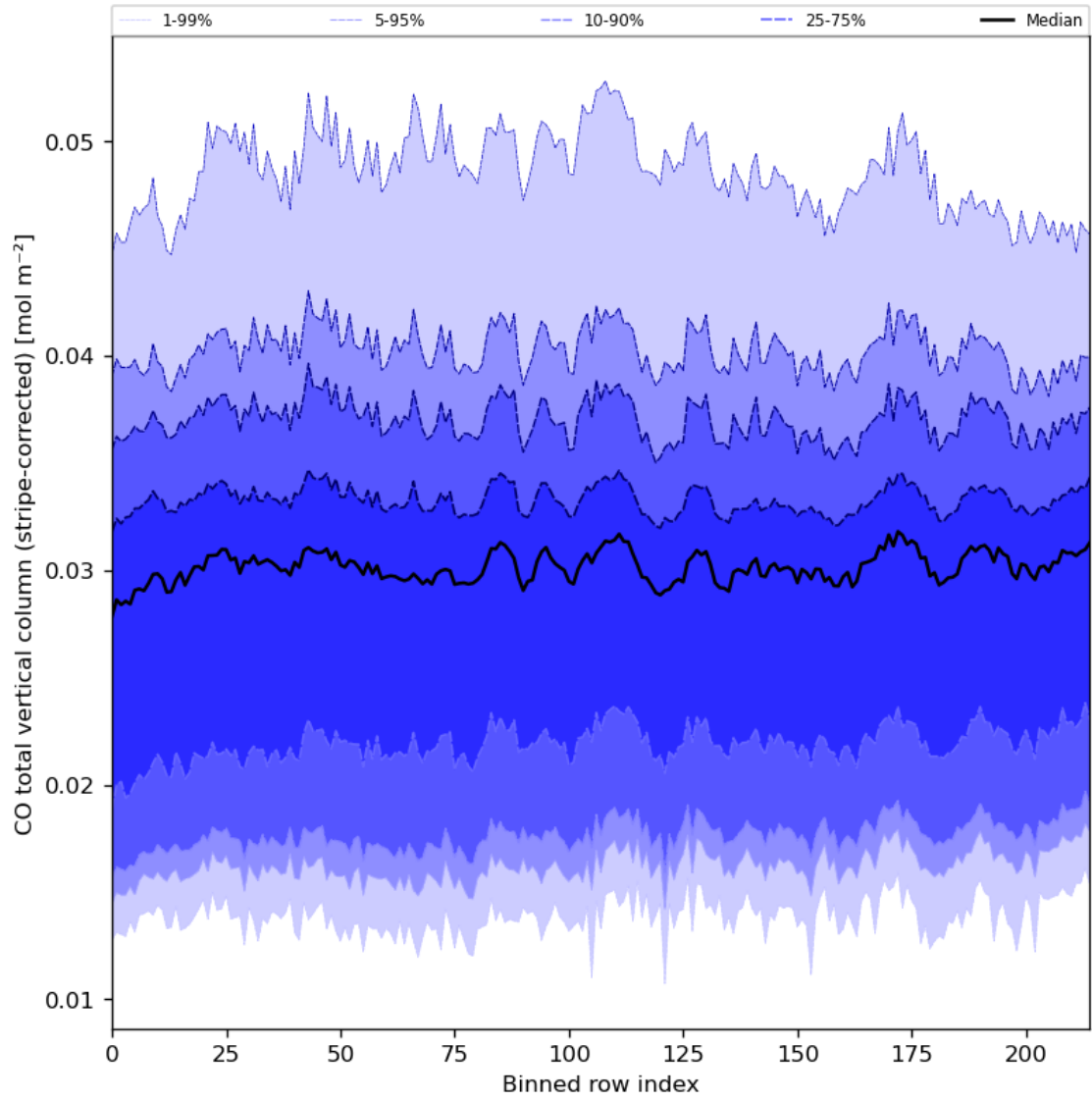
Figure 27: Along track statistics of “CO total vertical column (stripe-corrected)” for 2024-05-12 to 2024-05-13
