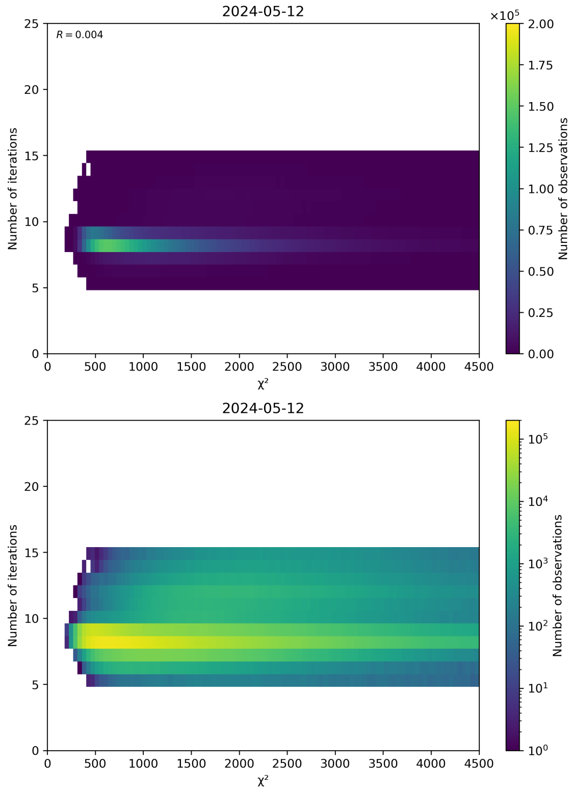
Figure 49: Scatter density plot of “ \chi^2 ” against “Number of iterations” for 2024-05-12 to 2024-05-13.
