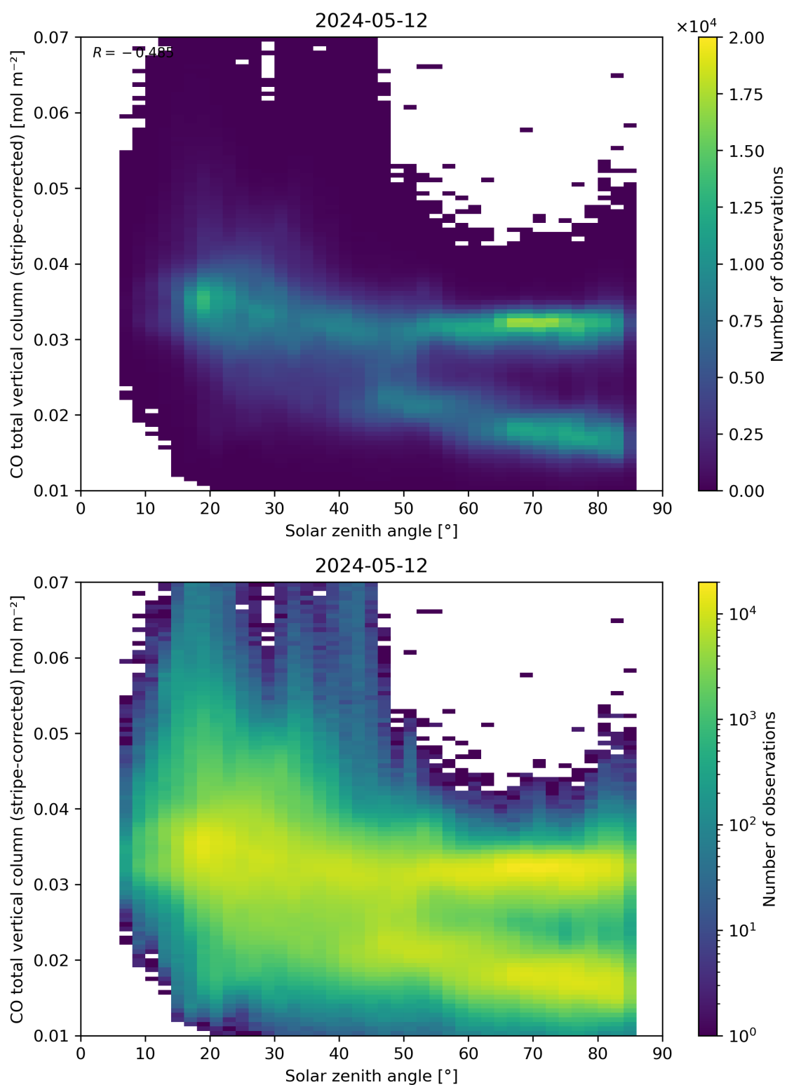
Figure 62: Scatter density plot of “Solar zenith angle” against “CO total vertical column (stripe-corrected)” for 2024-05-12 to 2024-05-13.
