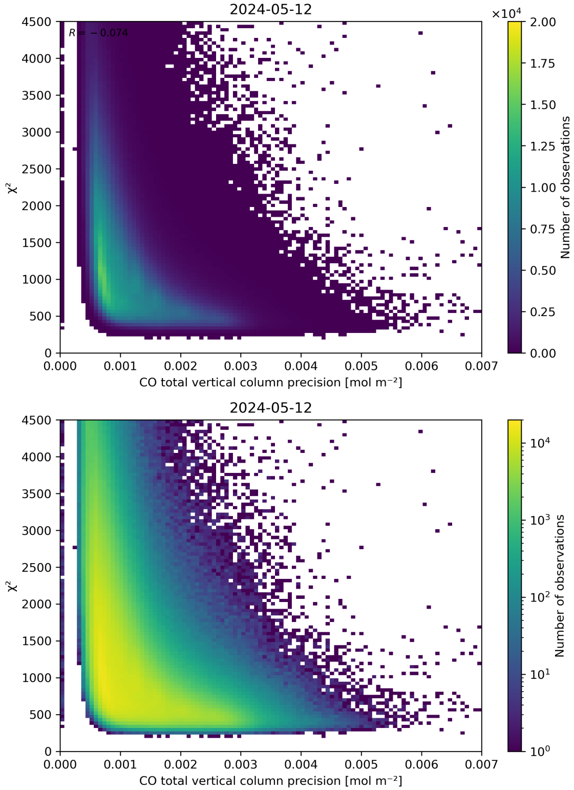
Figure 44: Scatter density plot of “CO total vertical column precision” against “ \chi^2 ” for 2024-05-12 to 2024-05-13.
