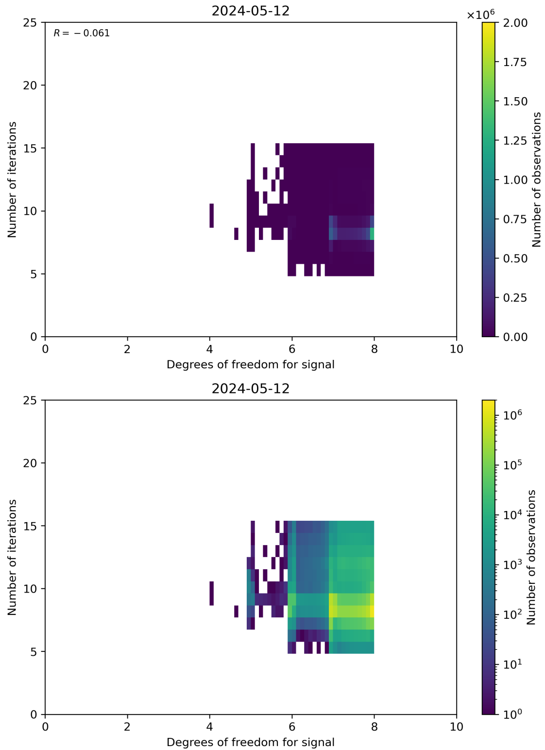
Figure 50: Scatter density plot of “Degrees of freedom for signal” against “Number of iterations” for 2024-05-12 to 2024-05-13.
