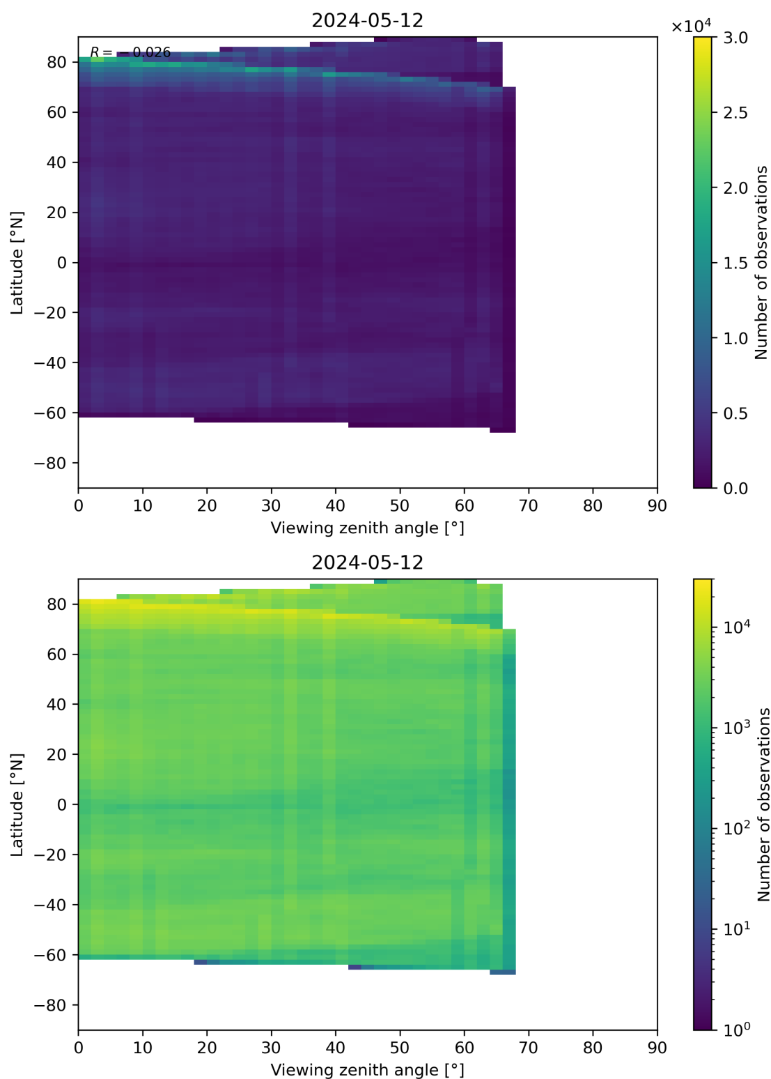
Figure 74: Scatter density plot of “Viewing zenith angle” against “Latitude” for 2024-05-12 to 2024-05-13.
