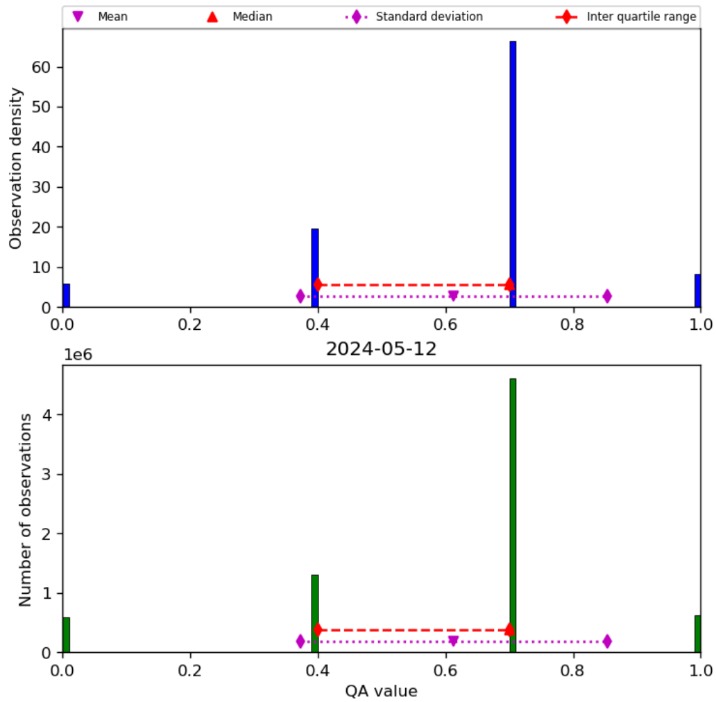
Figure 17: Histogram of “QA value” for 2024-05-12 to 2024-05-13
