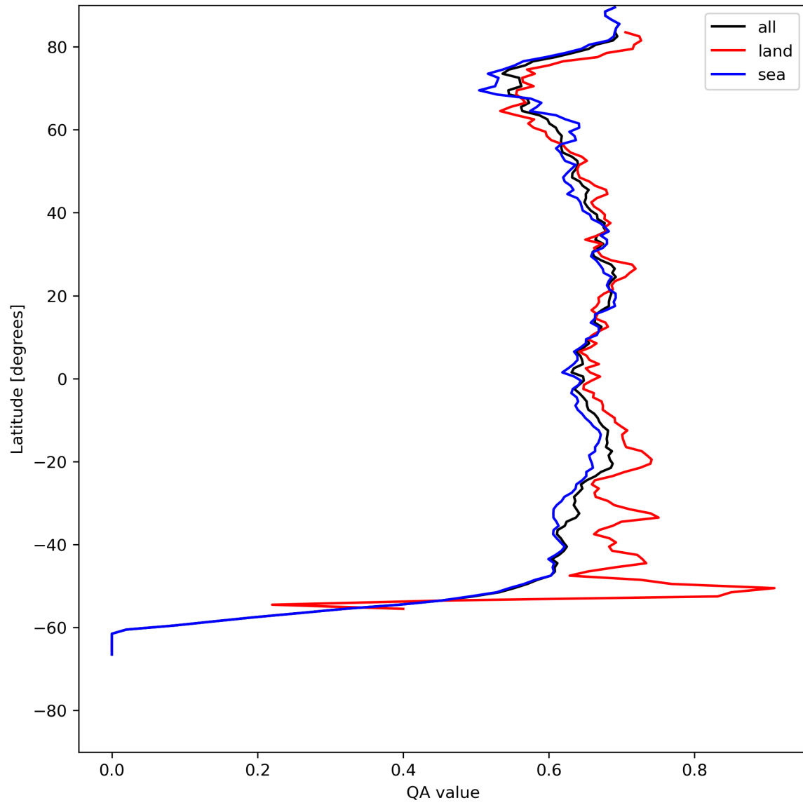
Figure 9: Zonal average of “QA value” for 2024-05-12 to 2024-05-13.
