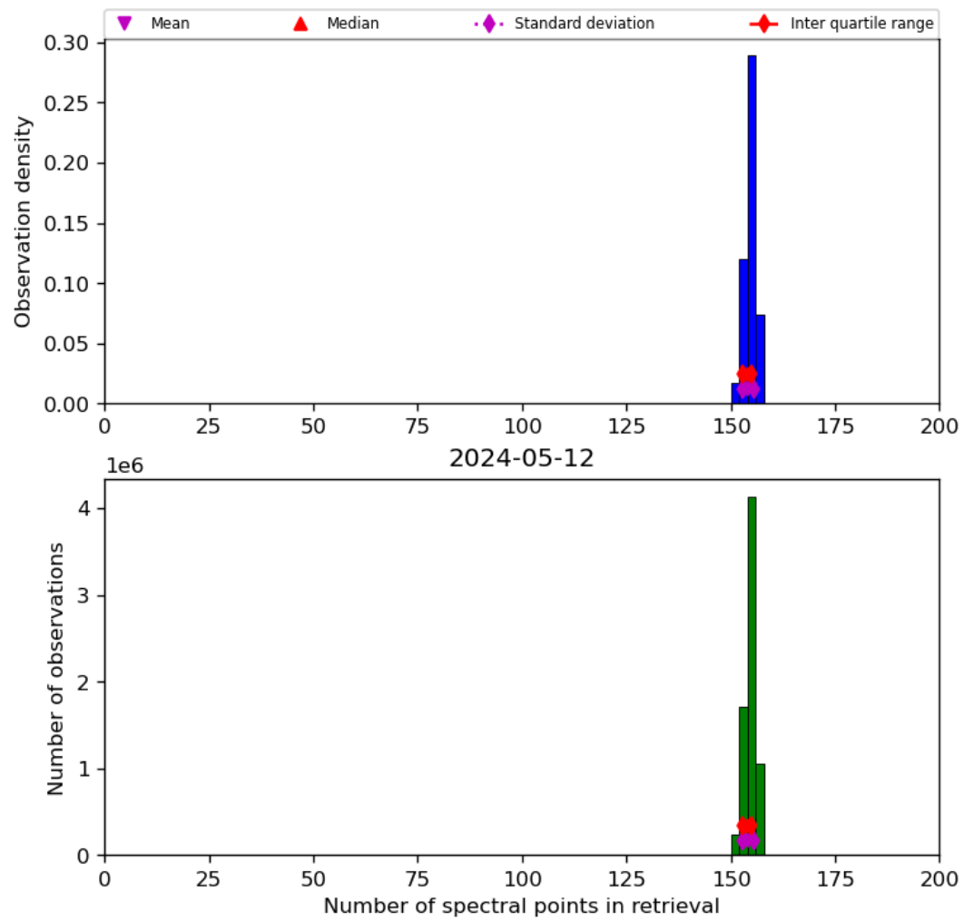
Figure 21: Histogram of “Number of spectral points in retrieval” for 2024-05-12 to 2024-05-13
