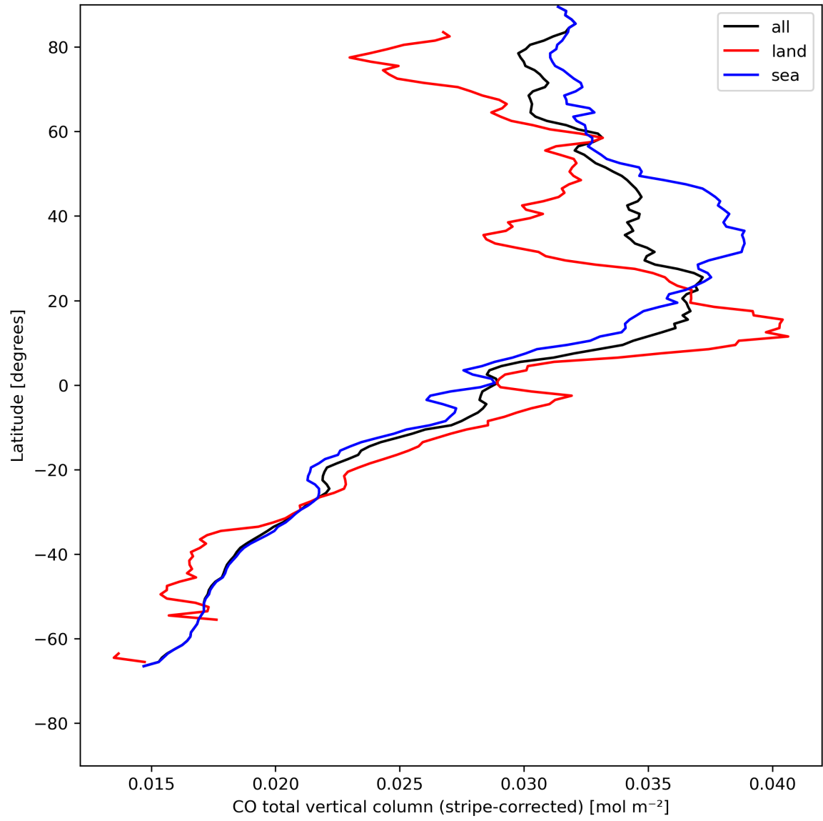
Figure 11: Zonal average of “CO total vertical column (stripe-corrected)” for 2024-05-12 to 2024-05-13.
