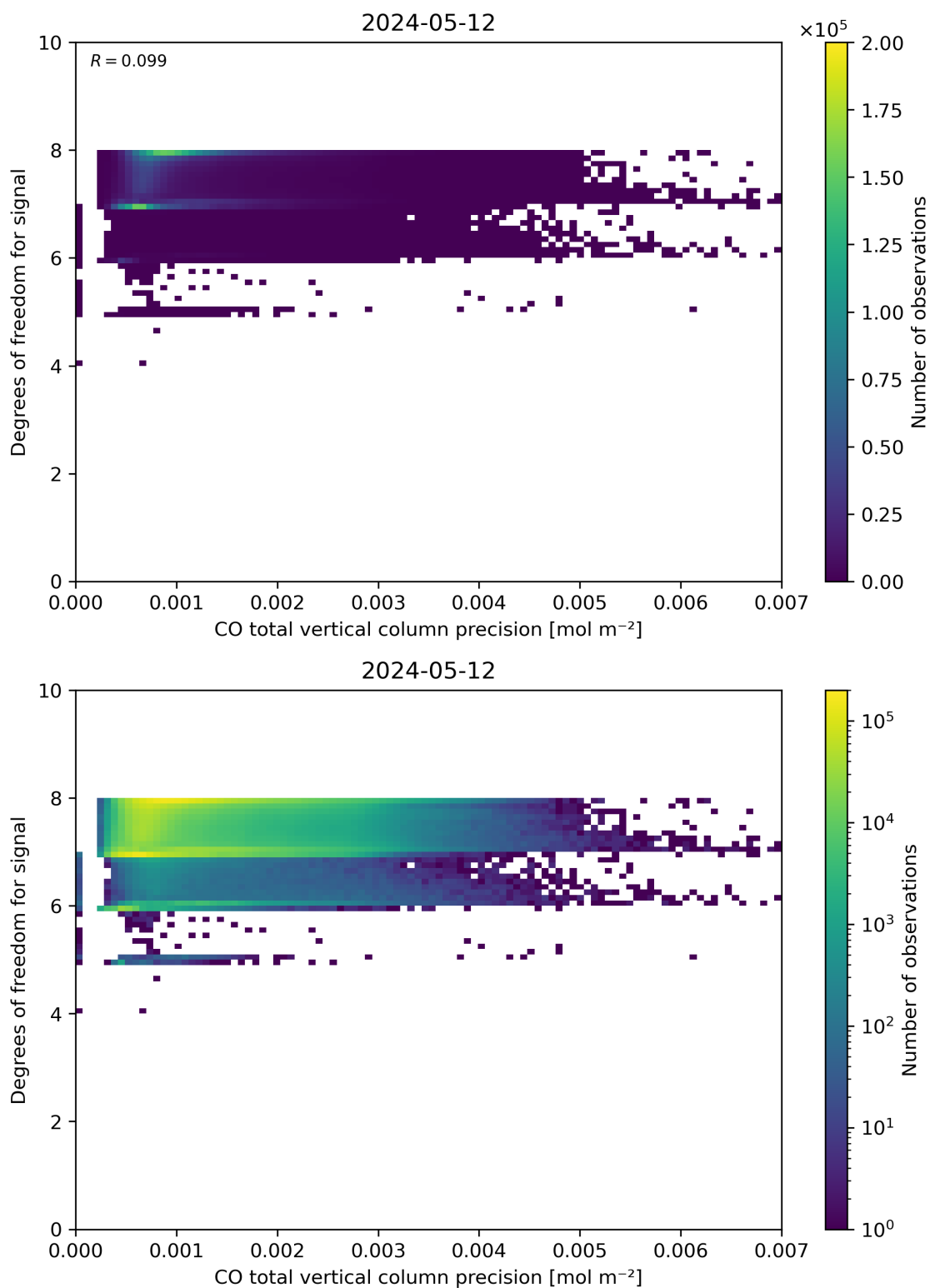
Figure 45: Scatter density plot of “CO total vertical column precision” against “Degrees of freedom for signal” for 2024-05-12 to 2024-05-13.
