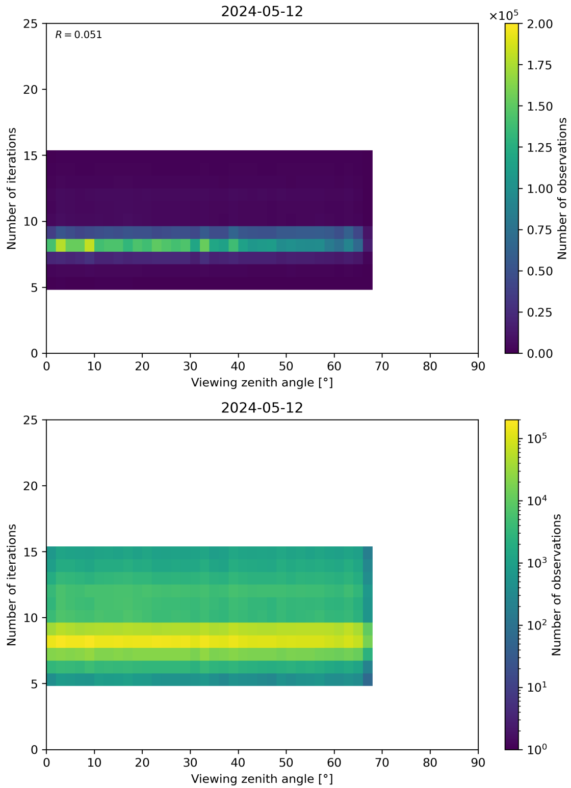
Figure 75: Scatter density plot of “Viewing zenith angle” against “Number of iterations” for 2024-05-12 to 2024-05-13.
