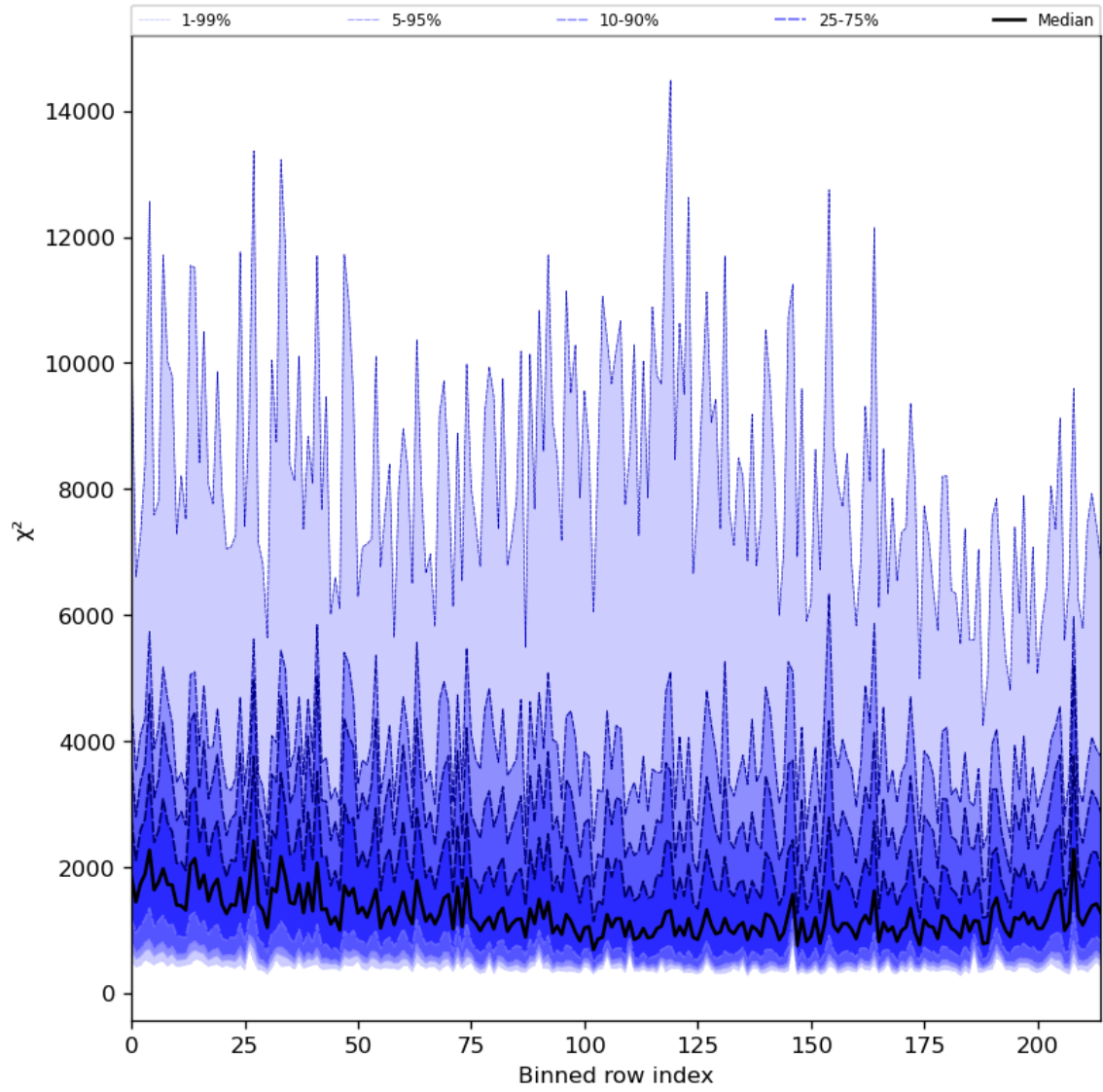
Figure 30: Along track statistics of “ \chi^2 ” for 2024-05-12 to 2024-05-13
