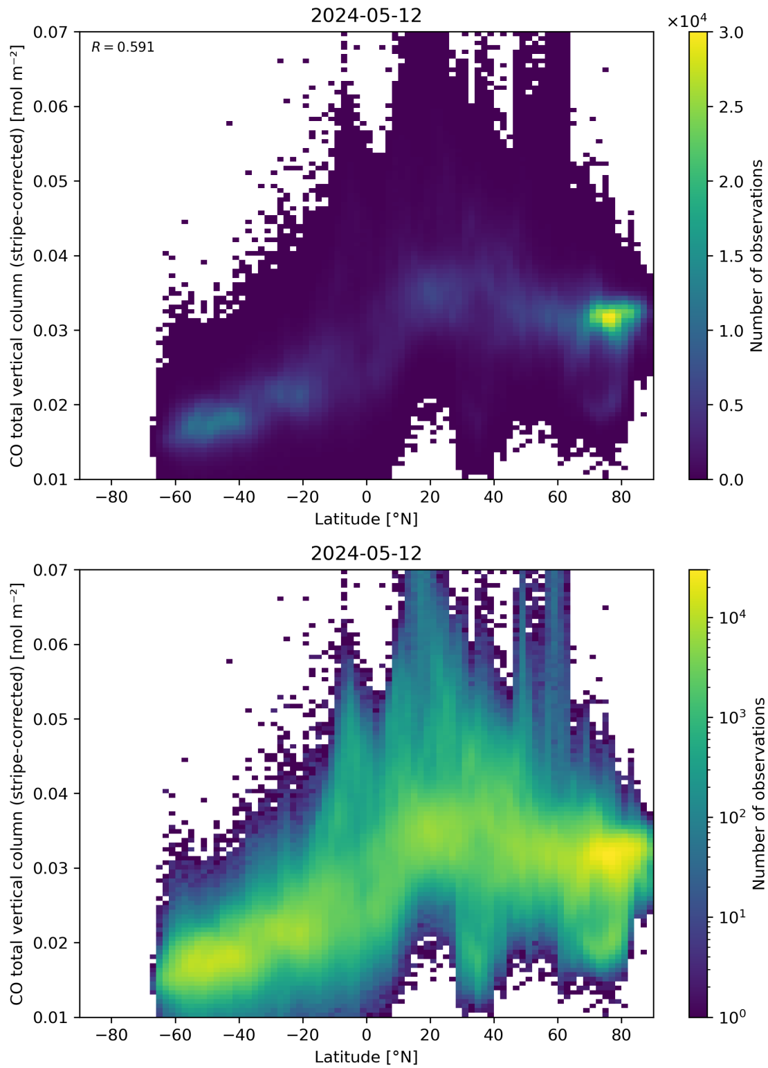
Figure 52: Scatter density plot of “Latitude” against “CO total vertical column (stripe-corrected)” for 2024-05-12 to 2024-05-13.
