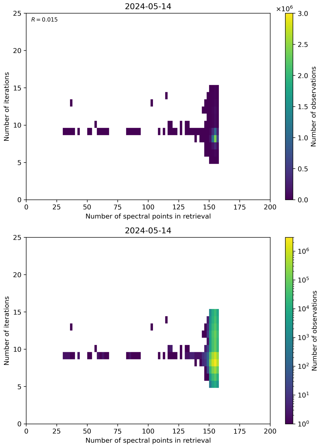
Figure 60: Scatter density plot of “Number of spectral points in retrieval” against “Number of iterations” for 2024-05-13 to 2024-05-15.
