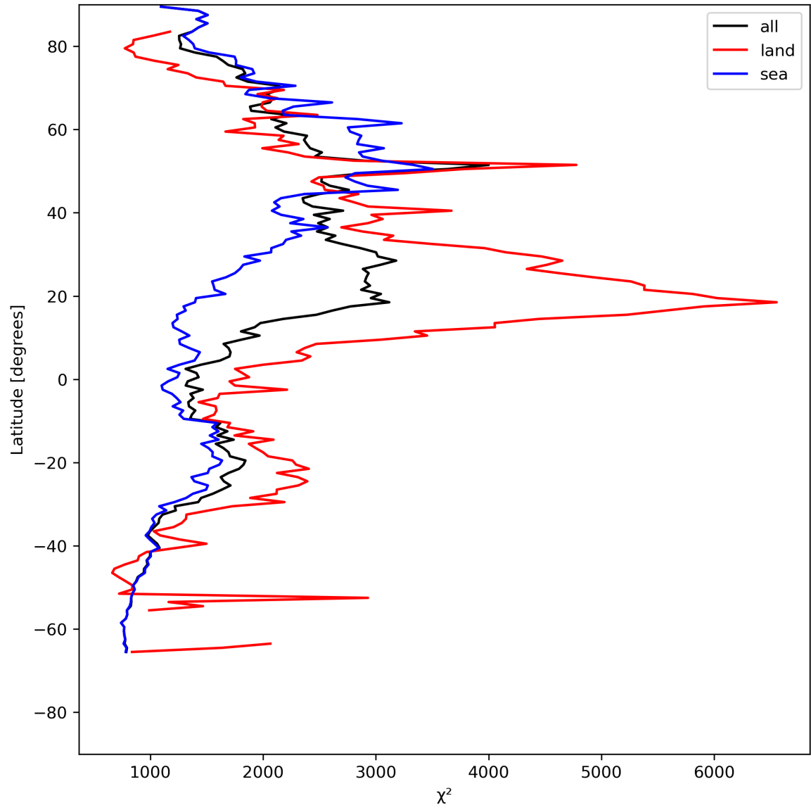
Figure 14: Zonal average of “ \chi^2 ” for 2024-05-13 to 2024-05-15.
