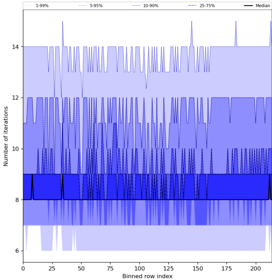
Figure 32: Along track statistics of “Number of iterations” for 2024-05-13 to 2024-05-15
