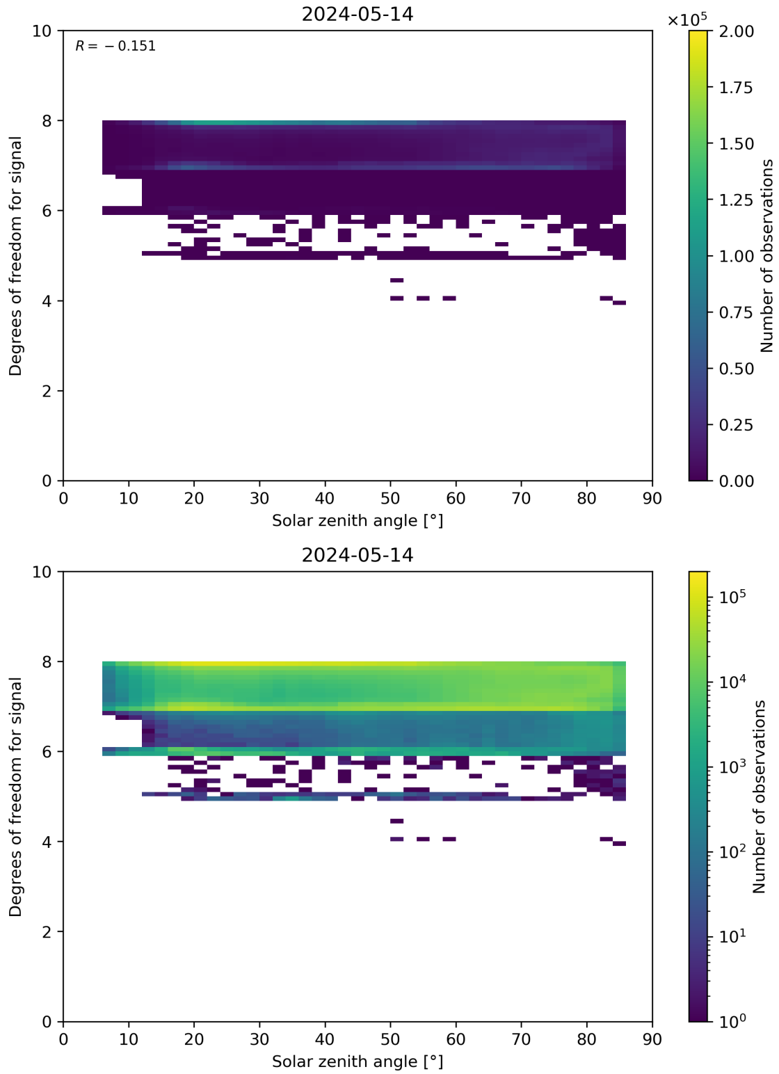
Figure 65: Scatter density plot of “Solar zenith angle” against “Degrees of freedom for signal” for 2024-05-13 to 2024-05-15.
