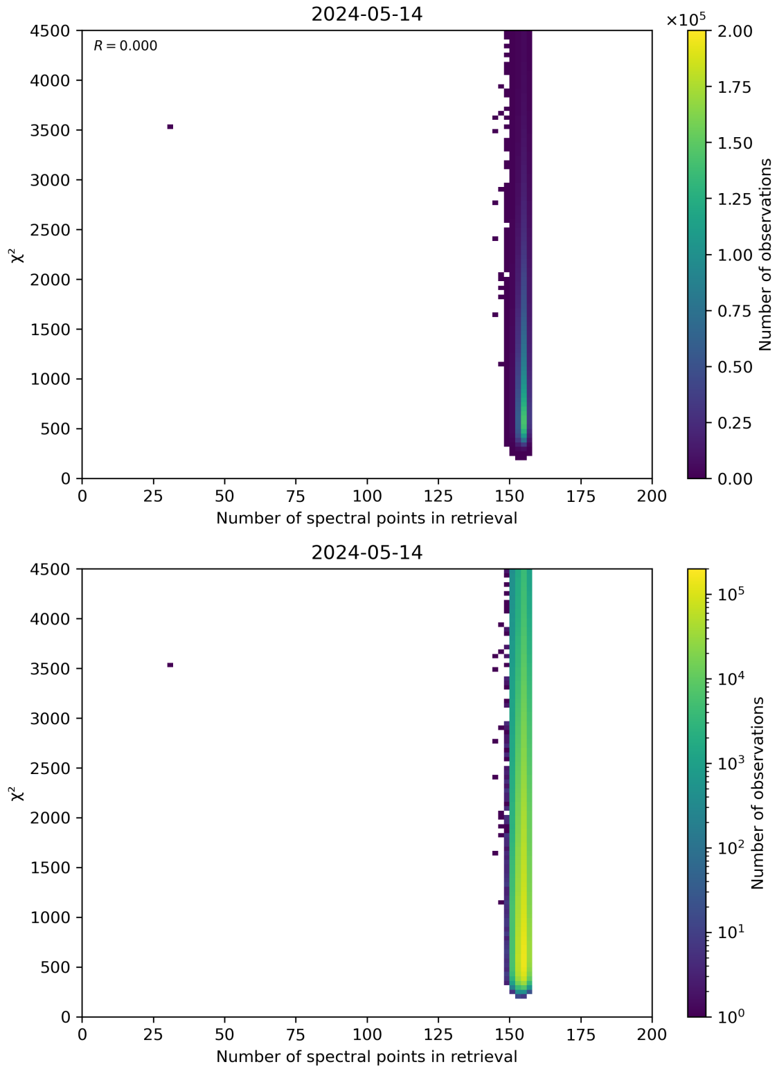
Figure 58: Scatter density plot of “Number of spectral points in retrieval” against “ \chi^2 ” for 2024-05-13 to 2024-05-15.
