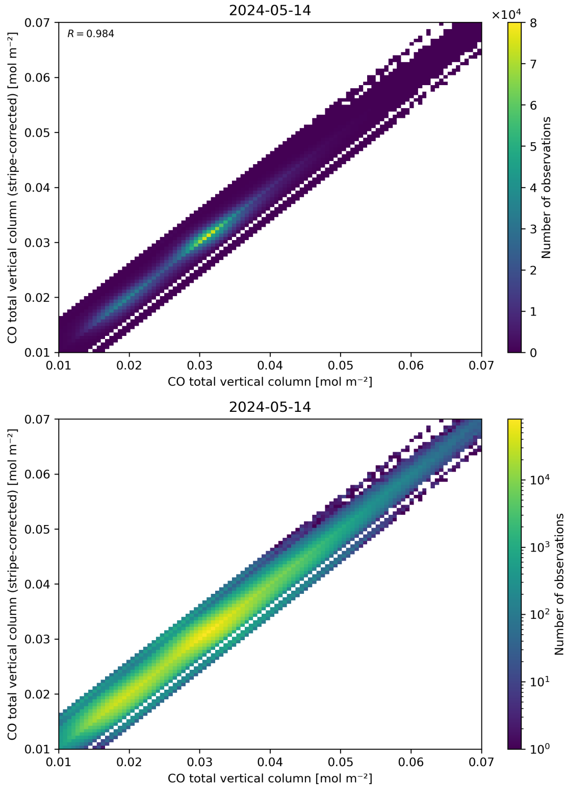
Figure 33: Scatter density plot of “CO total vertical column” against “CO total vertical column (stripe-corrected)” for 2024-05-13 to 2024-05-15.
