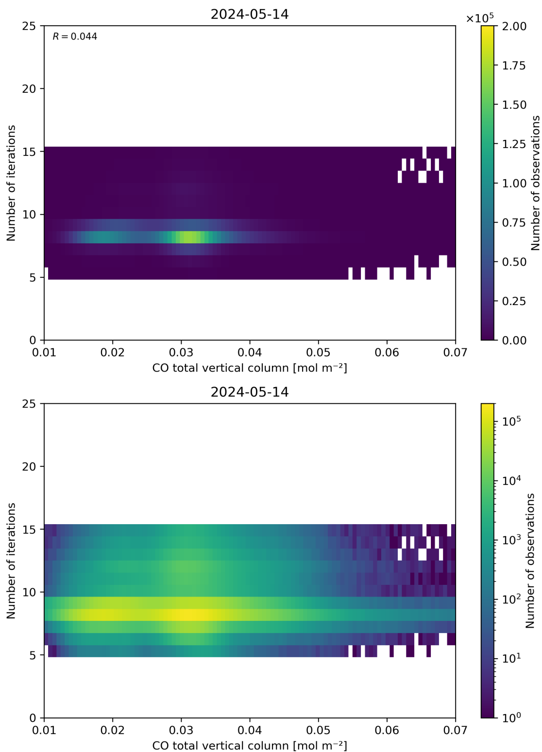
Figure 42: Scatter density plot of “CO total vertical column” against “Number of iterations” for 2024-05-13 to 2024-05-15.
