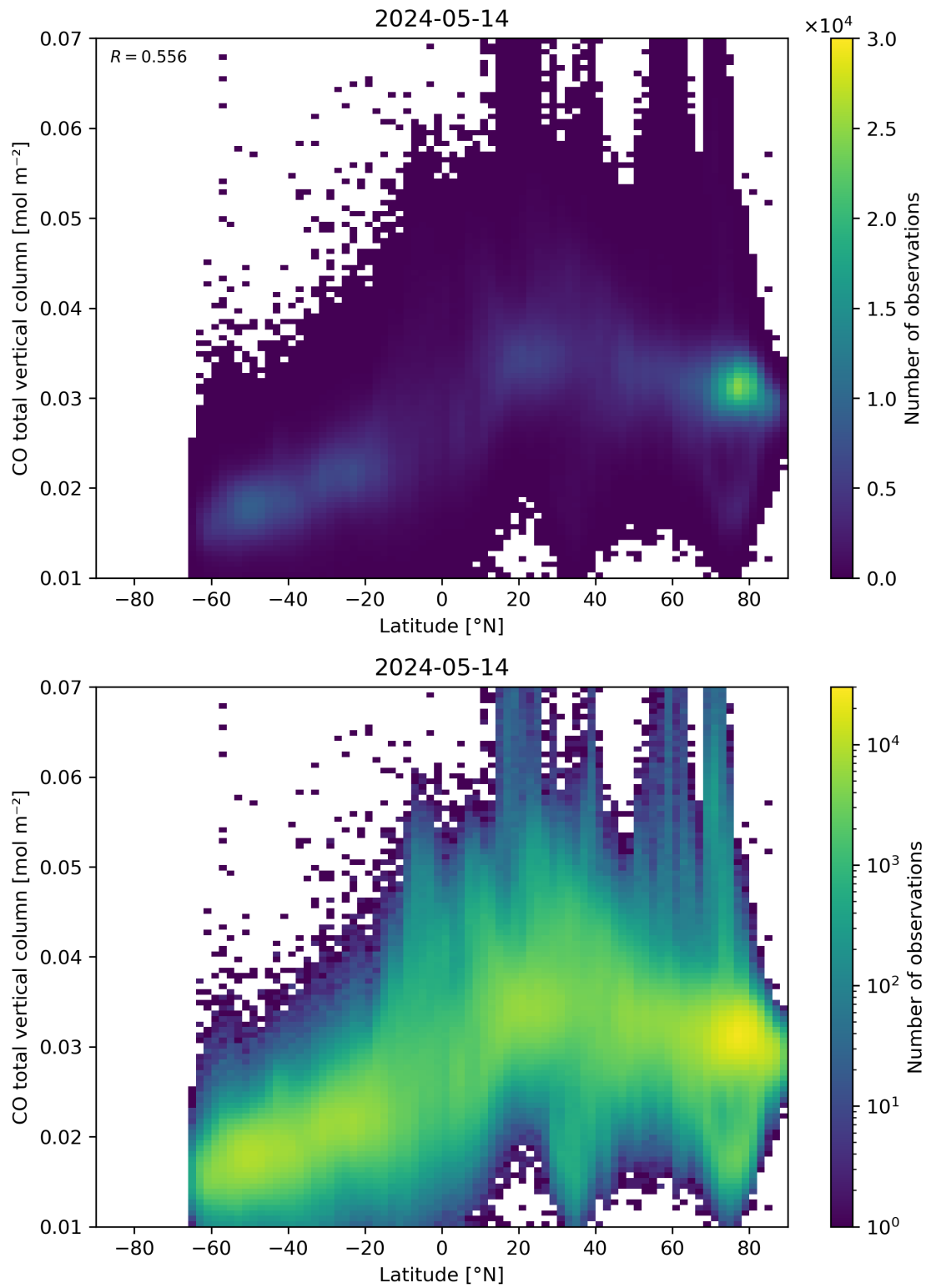
Figure 51: Scatter density plot of “Latitude” against “CO total vertical column” for 2024-05-13 to 2024-05-15.
