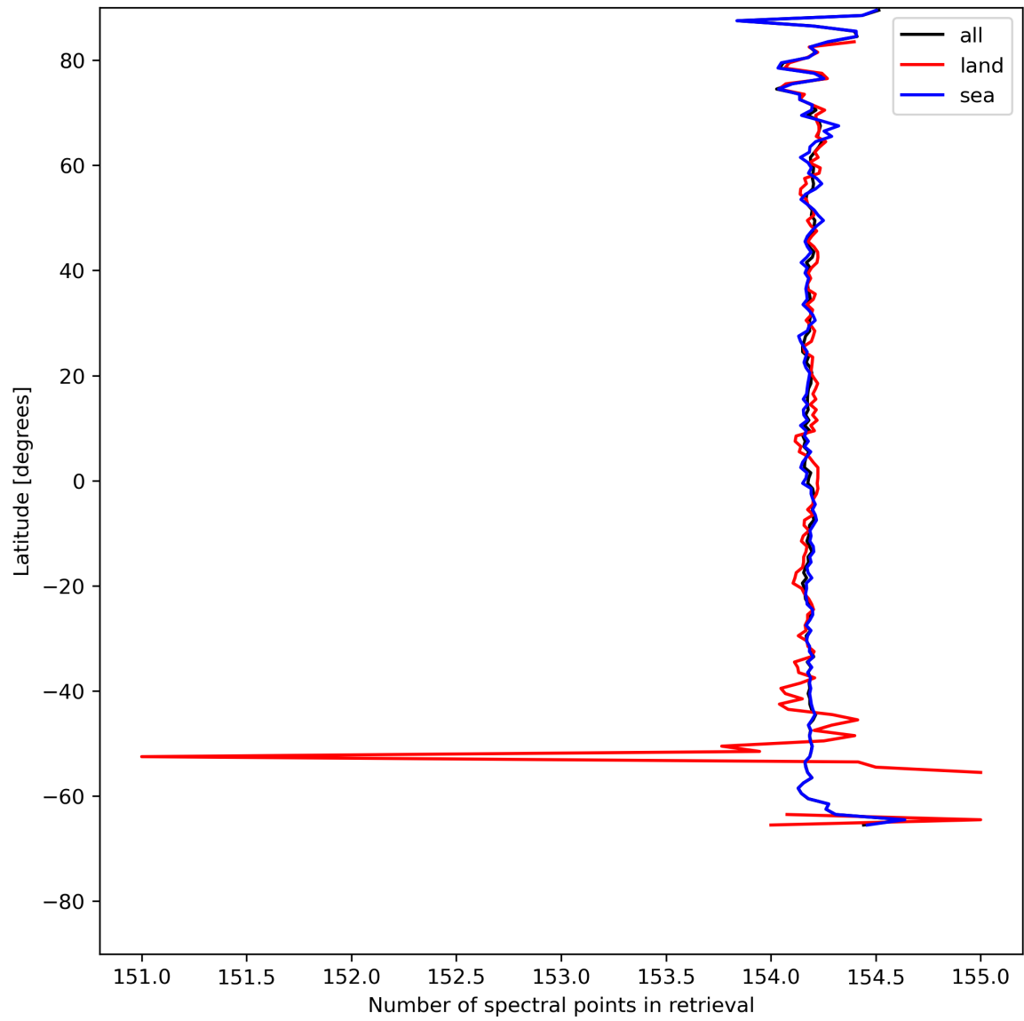
Figure 13: Zonal average of “Number of spectral points in retrieval” for 2024-05-13 to 2024-05-15.
