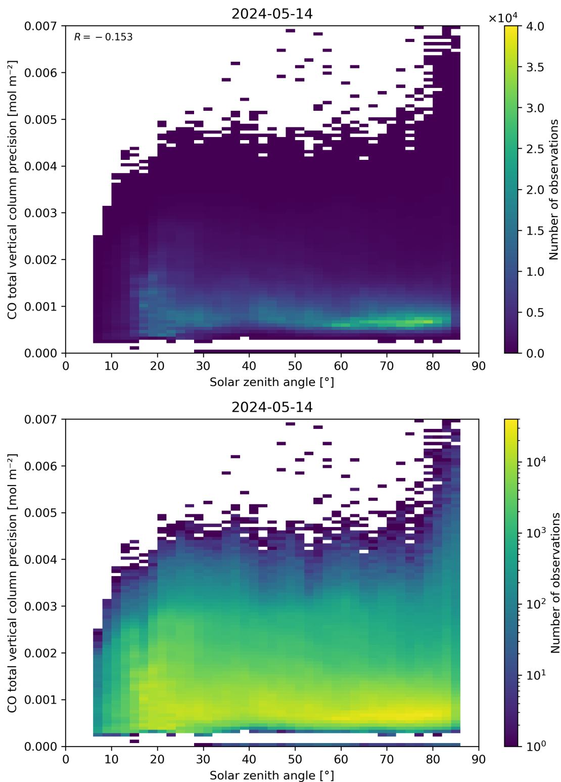
Figure 63: Scatter density plot of “Solar zenith angle” against “CO total vertical column precision” for 2024-05-13 to 2024-05-15.
