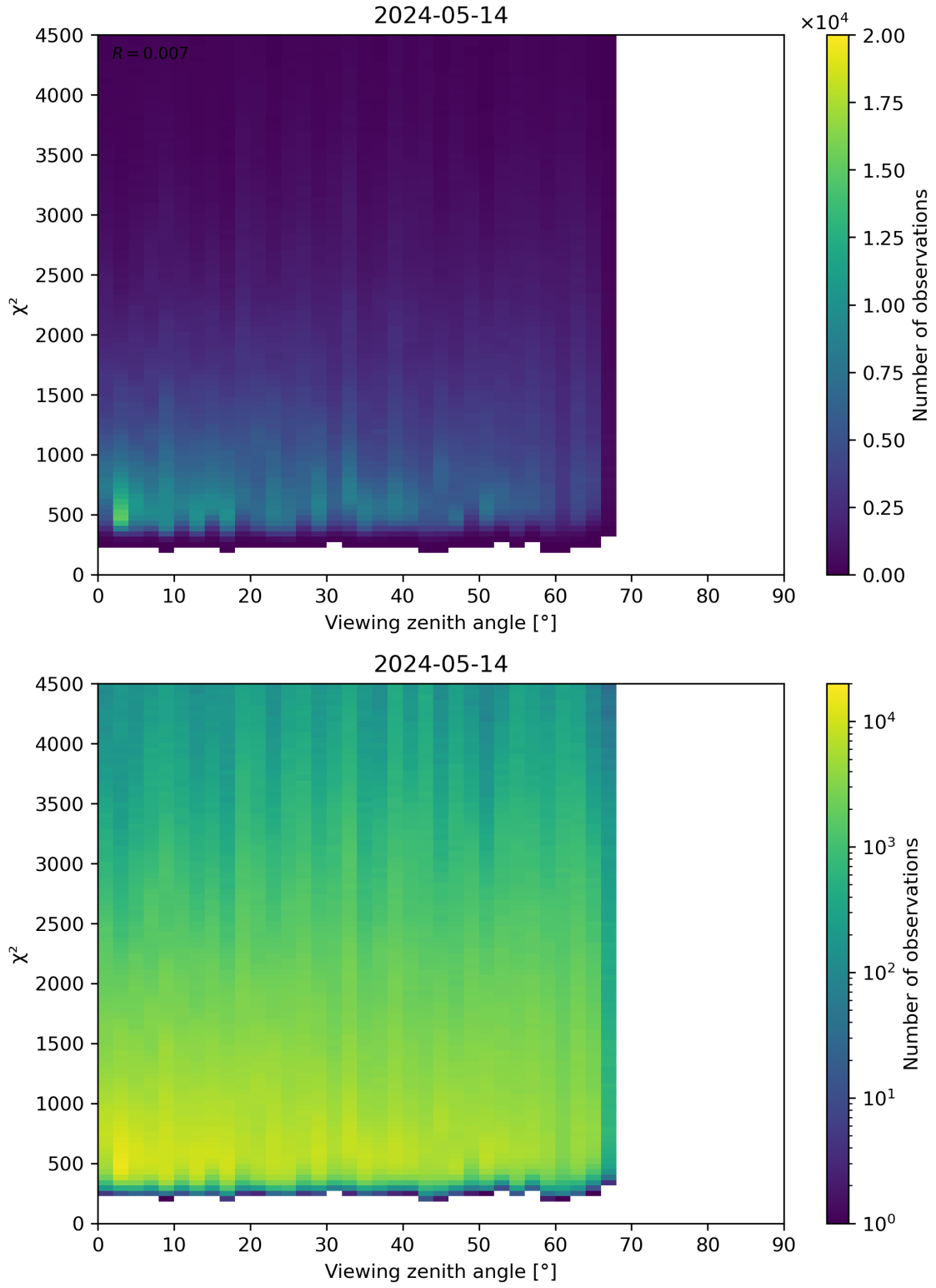
Figure 72: Scatter density plot of “Viewing zenith angle” against “ \chi^2 ” for 2024-05-13 to 2024-05-15.
