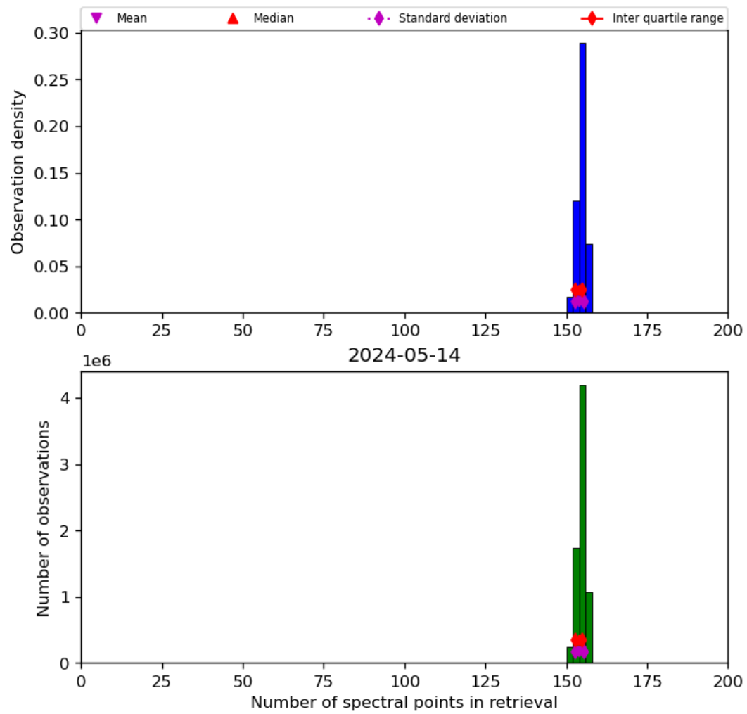
Figure 21: Histogram of “Number of spectral points in retrieval” for 2024-05-13 to 2024-05-15
