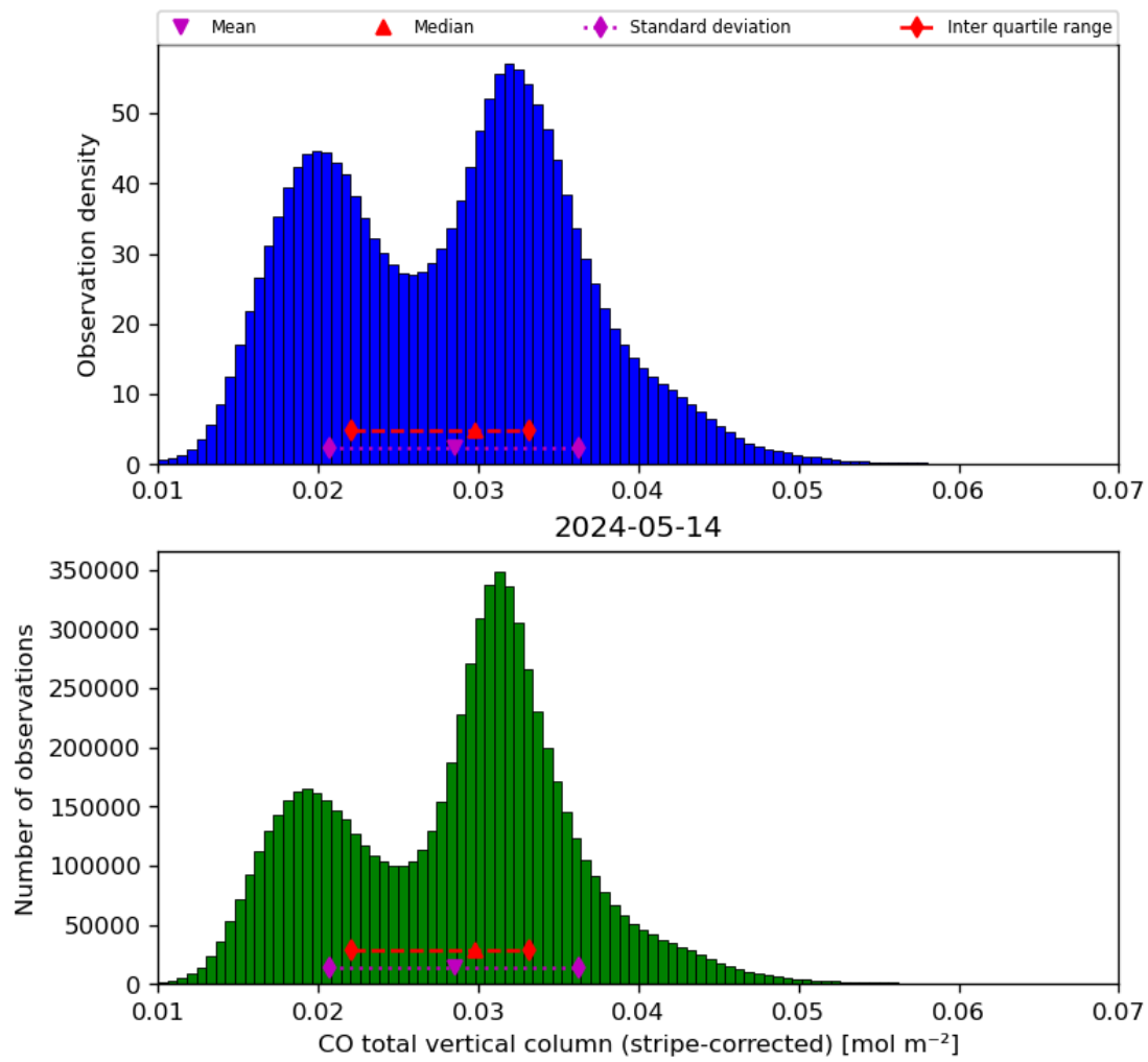
Figure 19: Histogram of “CO total vertical column (stripe-corrected)” for 2024-05-13 to 2024-05-15
