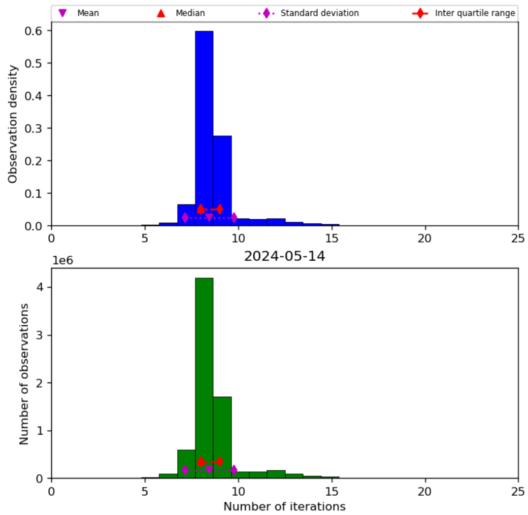
Figure 24: Histogram of “Number of iterations” for 2024-05-13 to 2024-05-15
