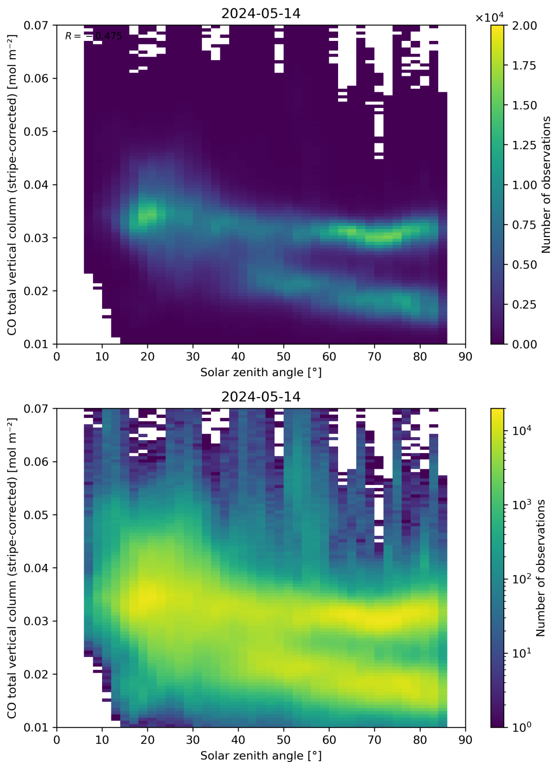
Figure 62: Scatter density plot of “Solar zenith angle” against “CO total vertical column (stripe-corrected)” for 2024-05-13 to 2024-05-15.
