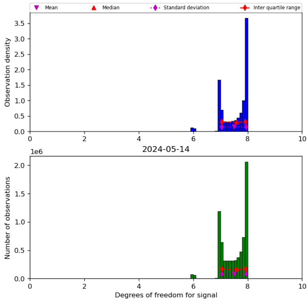
Figure 23: Histogram of “Degrees of freedom for signal” for 2024-05-13 to 2024-05-15
