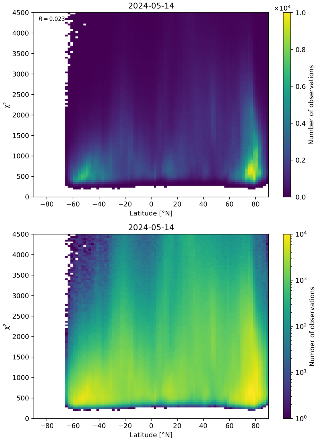
Figure 54: Scatter density plot of “Latitude” against “ \chi^2 ” for 2024-05-13 to 2024-05-15.
