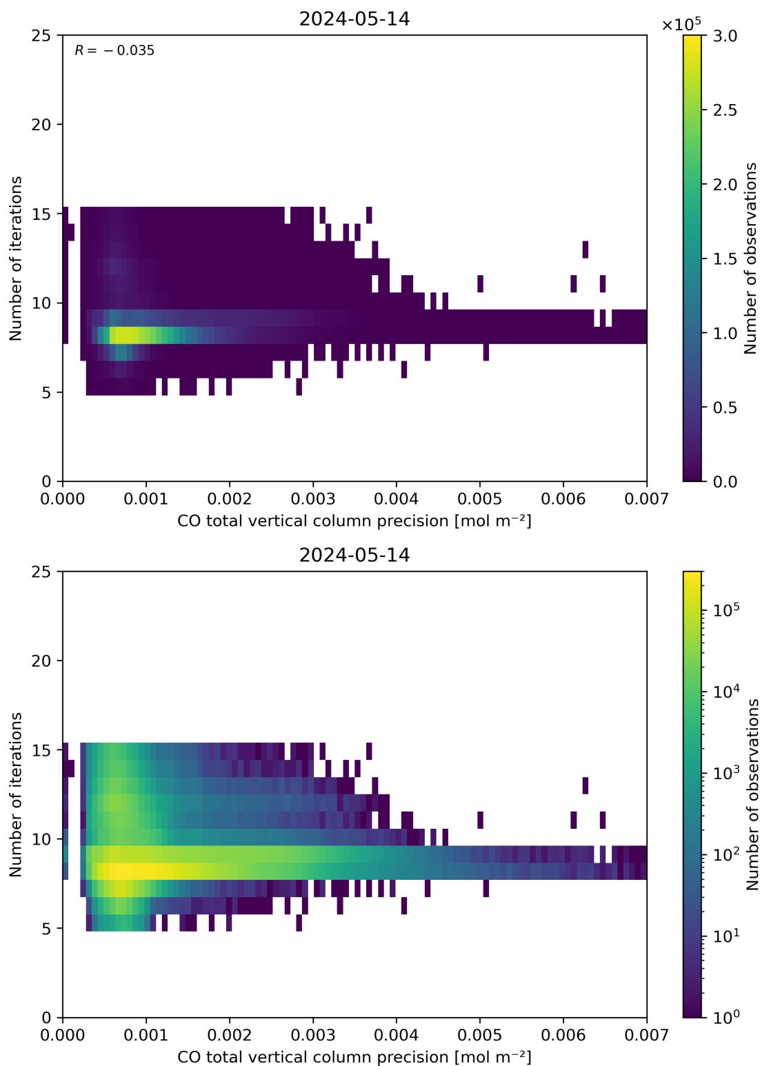
Figure 46: Scatter density plot of “CO total vertical column precision” against “Number of iterations” for 2024-05-13 to 2024-05-15.
