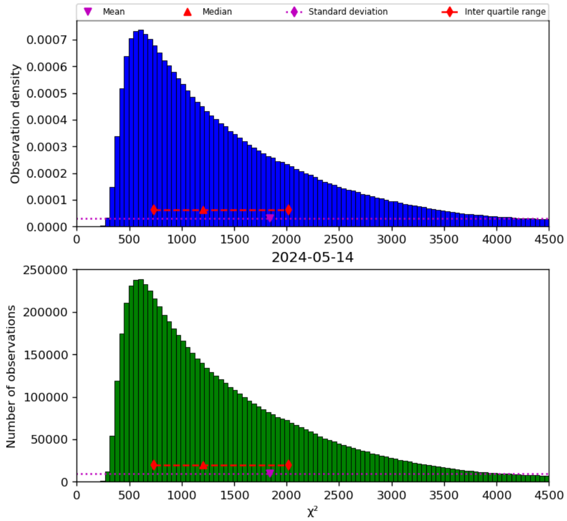
Figure 22: Histogram of “ \chi^2 ” for 2024-05-13 to 2024-05-15
