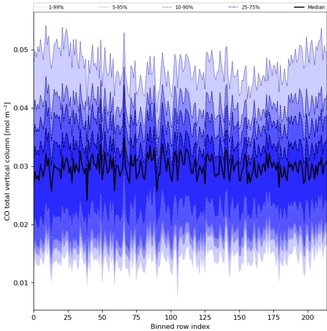
Figure 26: Along track statistics of "CO total vertical column" for 2024-05-13 to 2024-05-15
