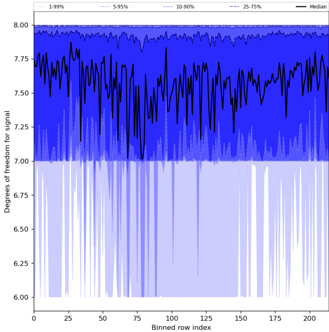
Figure 31: Along track statistics of “Degrees of freedom for signal” for 2024-05-13 to 2024-05-15
