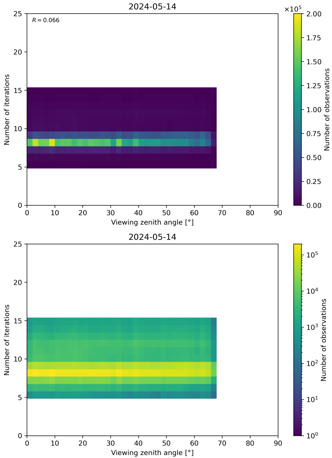
Figure 75: Scatter density plot of “Viewing zenith angle” against “Number of iterations” for 2024-05-13 to 2024-05-15.
