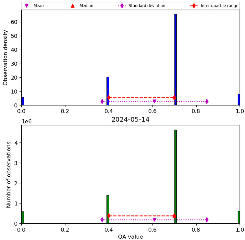
Figure 17: Histogram of “QA value” for 2024-05-13 to 2024-05-15
