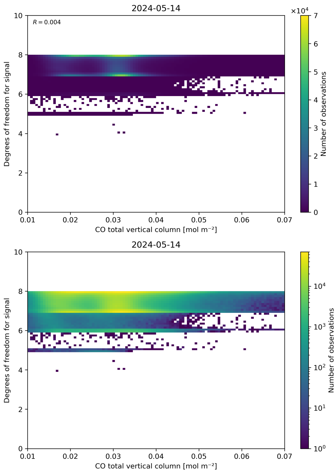
Figure 41: Scatter density plot of “CO total vertical column” against “Degrees of freedom for signal” for 2024-05-13 to 2024-05-15.
