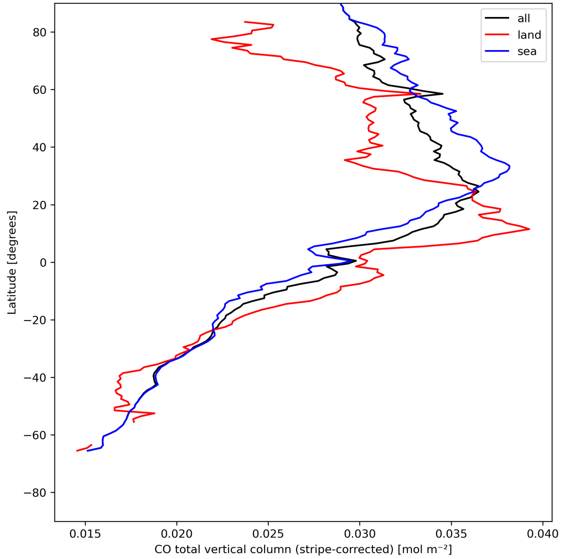
Figure 11: Zonal average of “CO total vertical column (stripe-corrected)” for 2024-05-13 to 2024-05-15.
