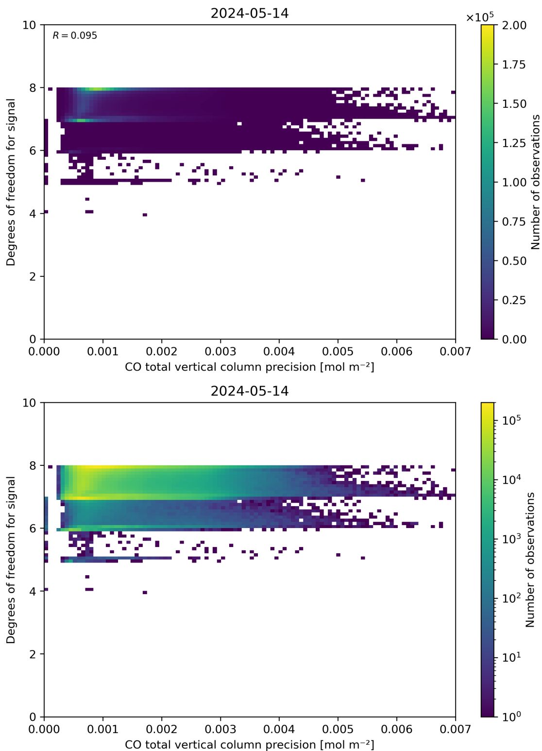
Figure 45: Scatter density plot of “CO total vertical column precision” against “Degrees of freedom for signal” for 2024-05-13 to 2024-05-15.
