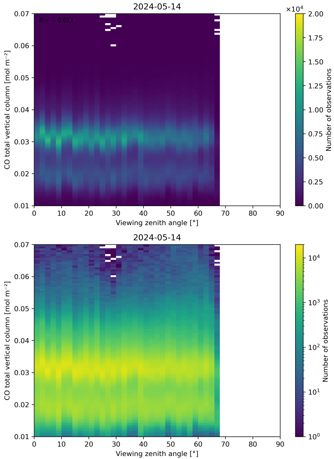
Figure 69: Scatter density plot of “Viewing zenith angle” against “CO total vertical column” for 2024-05-13 to 2024-05-15.
