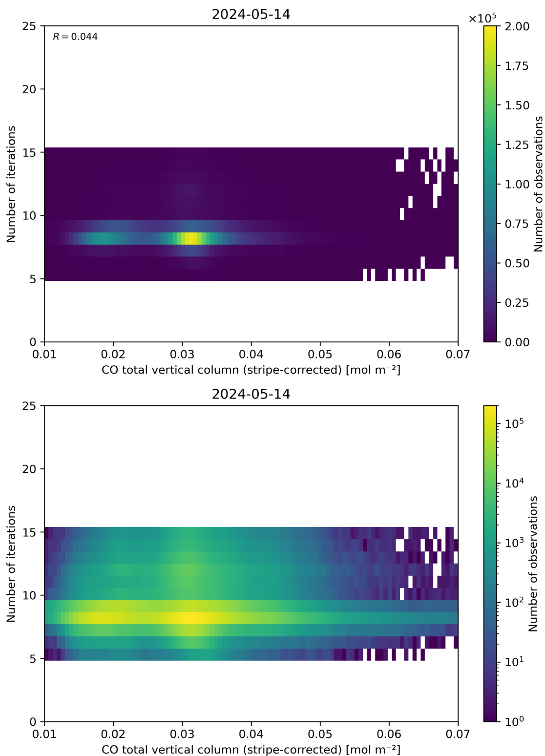
Figure 39: Scatter density plot of “CO total vertical column (stripe-corrected)” against “Number of iterations” for 2024-05-13 to 2024-05-15.
