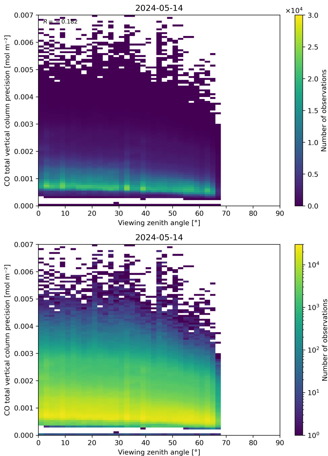
Figure 71: Scatter density plot of “Viewing zenith angle” against “CO total vertical column precision” for 2024-05-13 to 2024-05-15.
