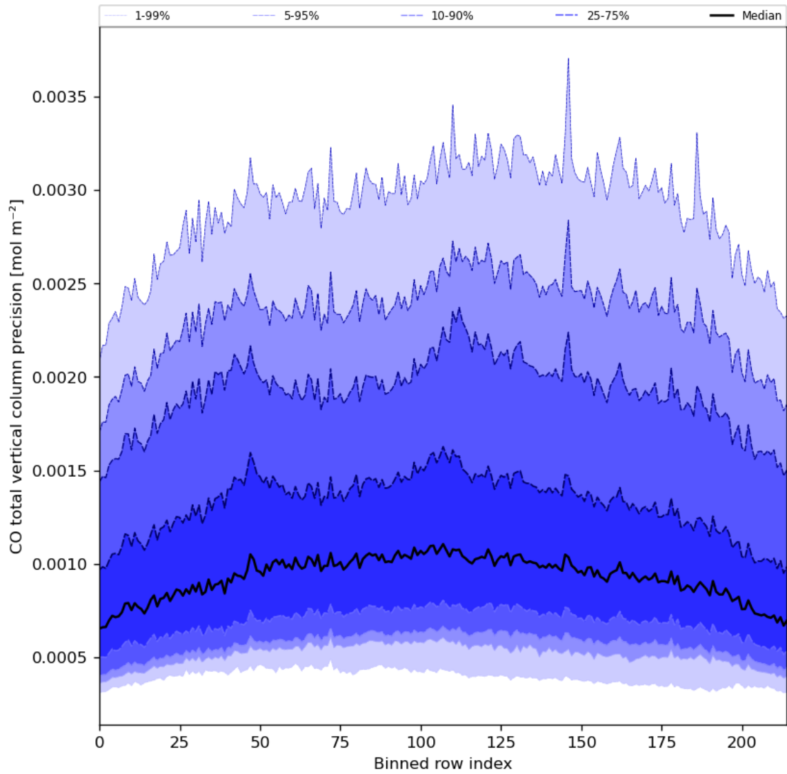
Figure 28: Along track statistics of “CO total vertical column precision” for 2024-05-13 to 2024-05-15
