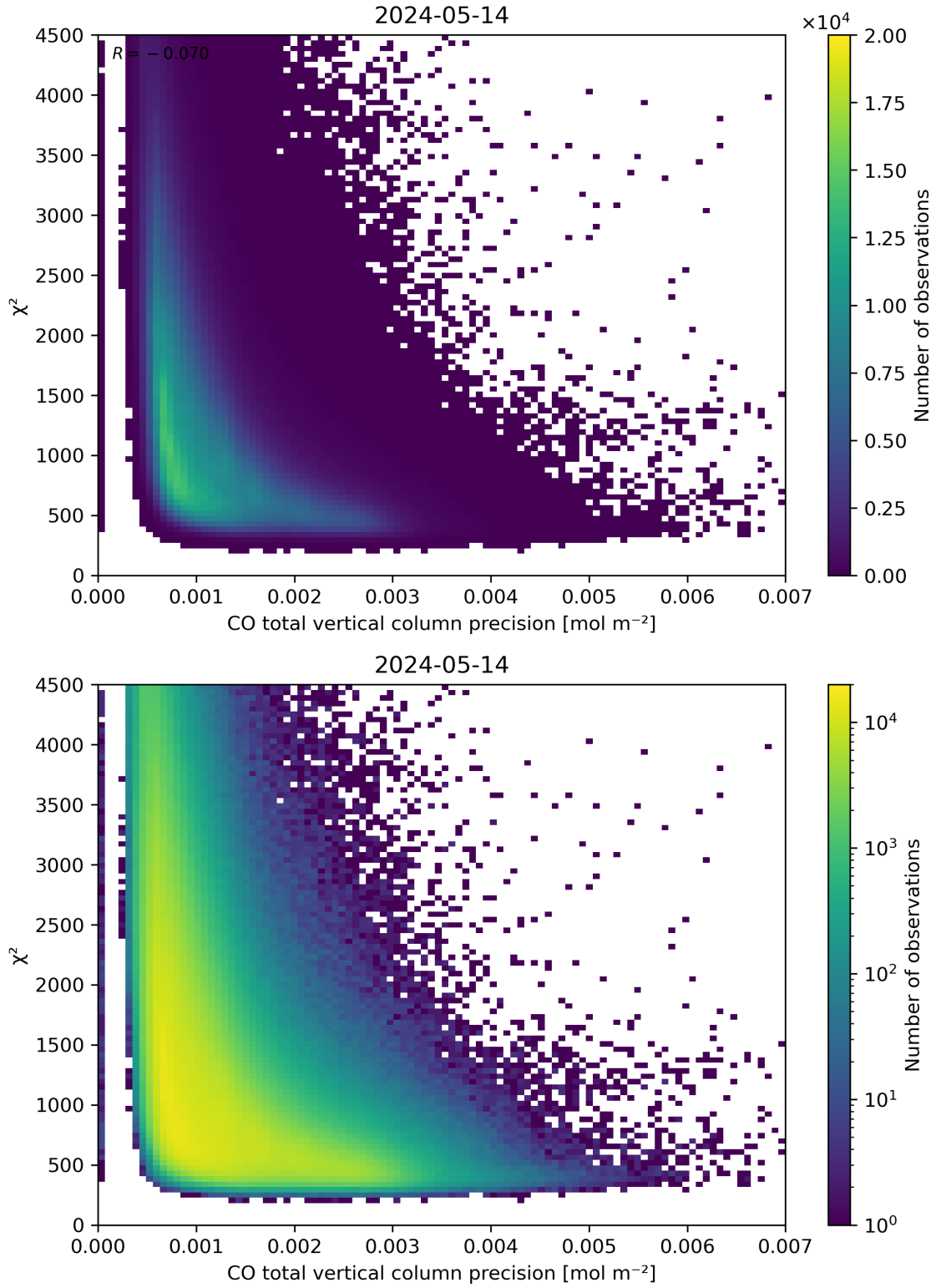
Figure 44: Scatter density plot of “CO total vertical column precision” against “ \chi^2 ” for 2024-05-13 to 2024-05-15.
