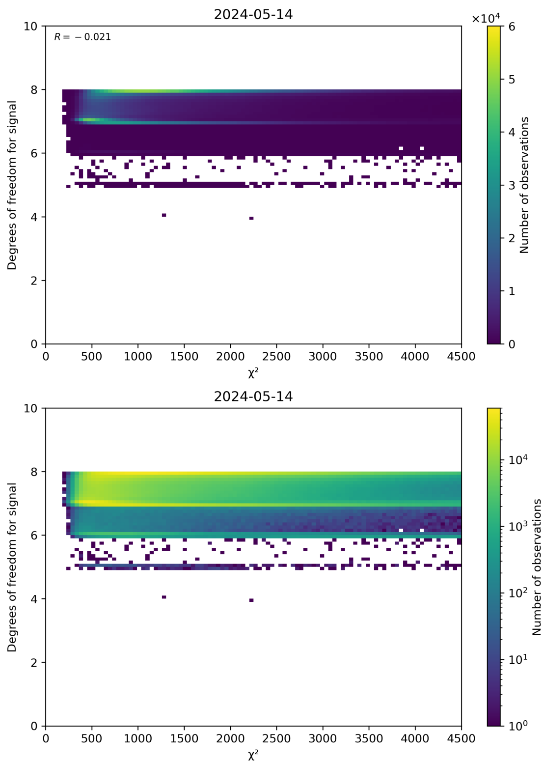
Figure 48: Scatter density plot of “ \chi^2 ” against “Degrees of freedom for signal” for 2024-05-13 to 2024-05-15.
