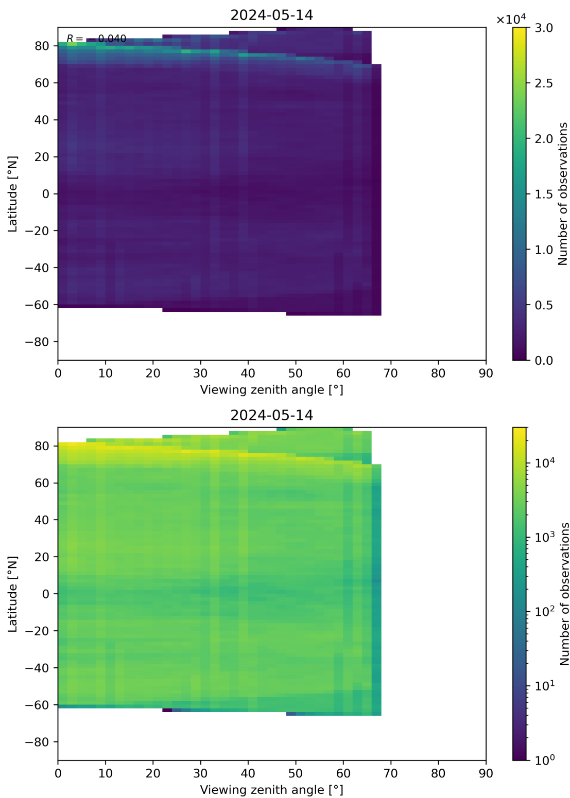
Figure 74: Scatter density plot of “Viewing zenith angle” against “Latitude” for 2024-05-13 to 2024-05-15.
