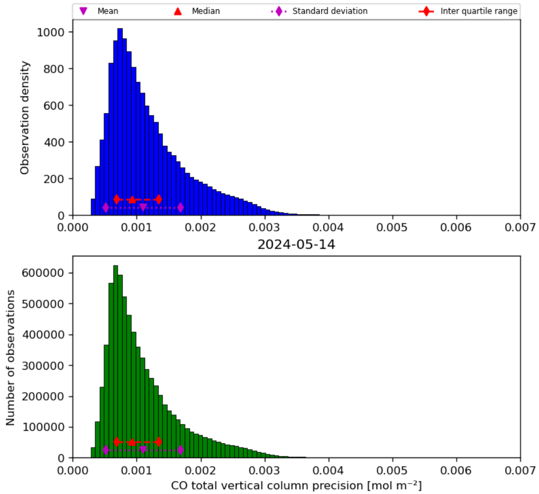
Figure 20: Histogram of “CO total vertical column precision” for 2024-05-13 to 2024-05-15
