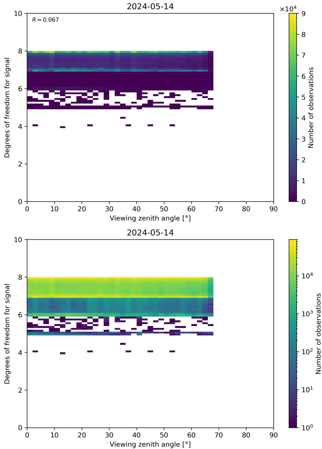
Figure 73: Scatter density plot of “Viewing zenith angle” against “Degrees of freedom for signal” for 2024-05-13 to 2024-05-15.
