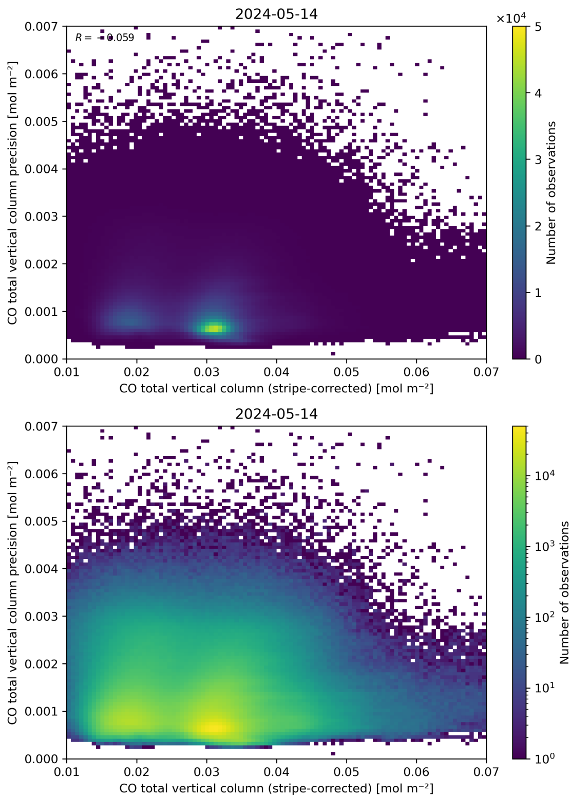
Figure 36: Scatter density plot of “CO total vertical column (stripe-corrected)” against “CO total vertical column precision” for 2024-05-13 to 2024-05-15.
