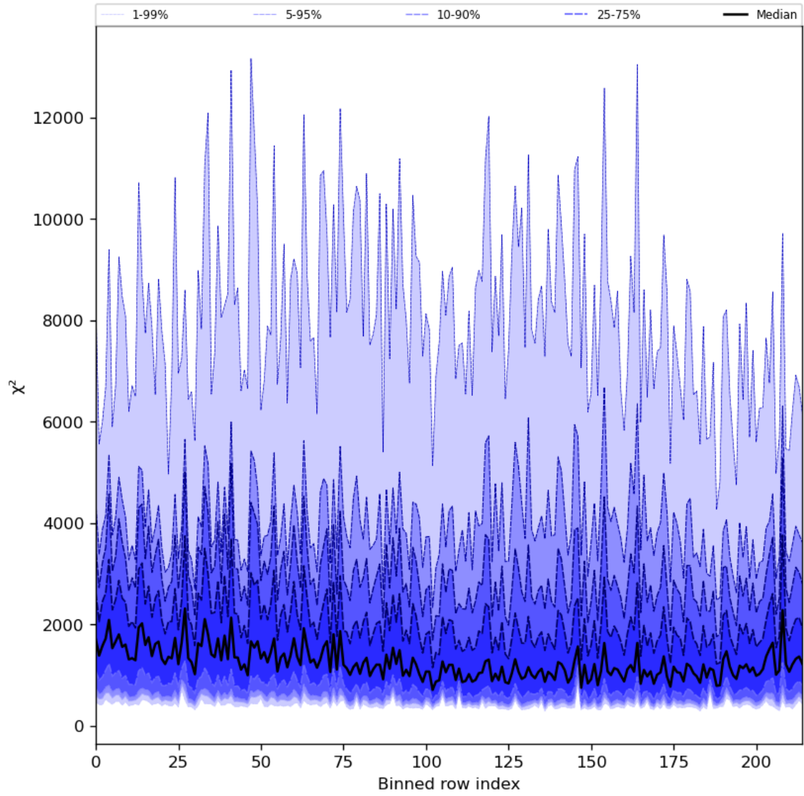
Figure 30: Along track statistics of “ \chi^2 ” for 2024-05-13 to 2024-05-15
