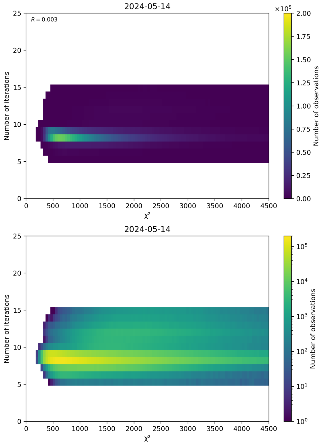
Figure 49: Scatter density plot of “ \chi^2 ” against “Number of iterations” for 2024-05-13 to 2024-05-15.
