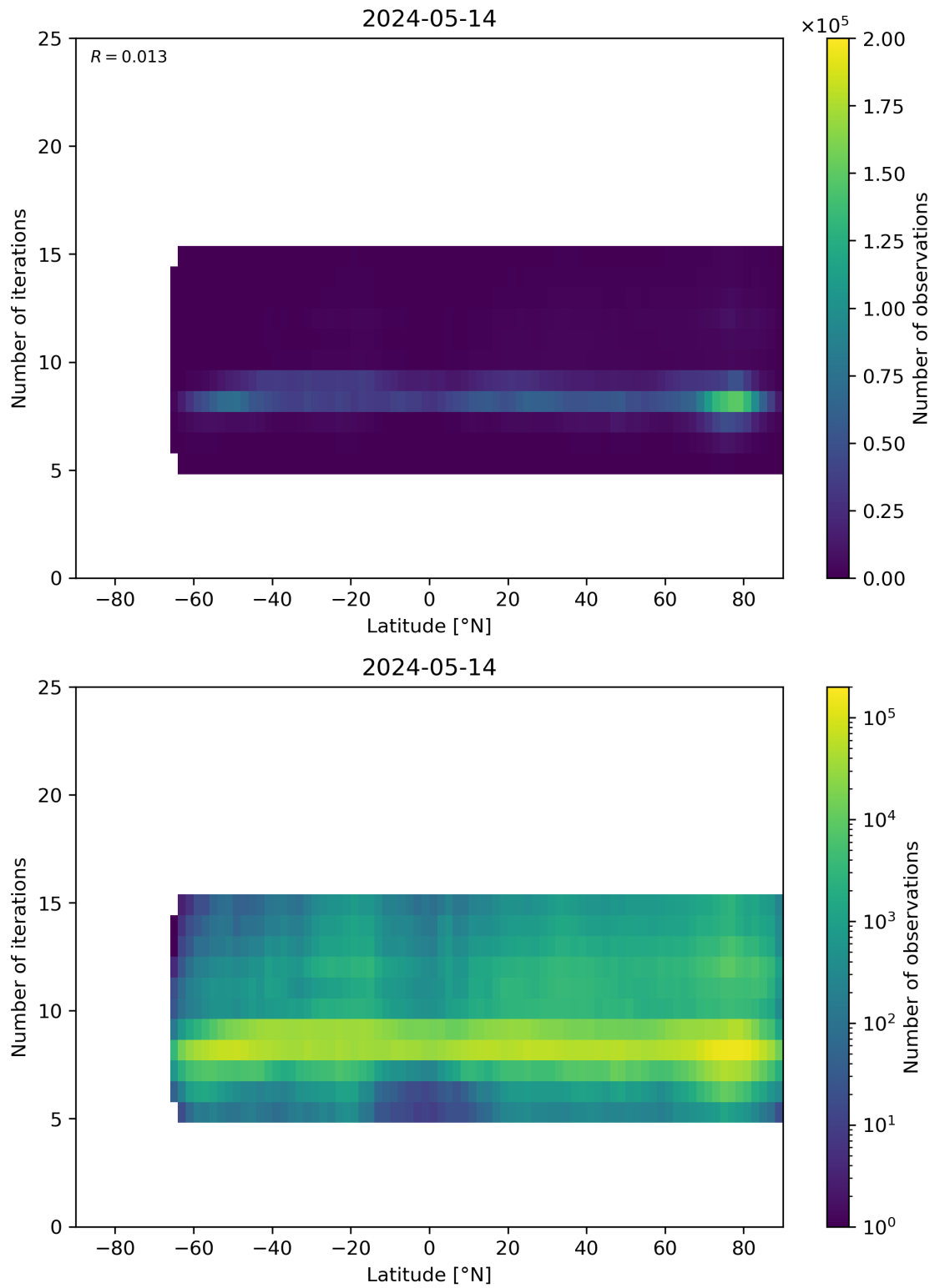
Figure 56: Scatter density plot of “Latitude” against “Number of iterations” for 2024-05-13 to 2024-05-15.
