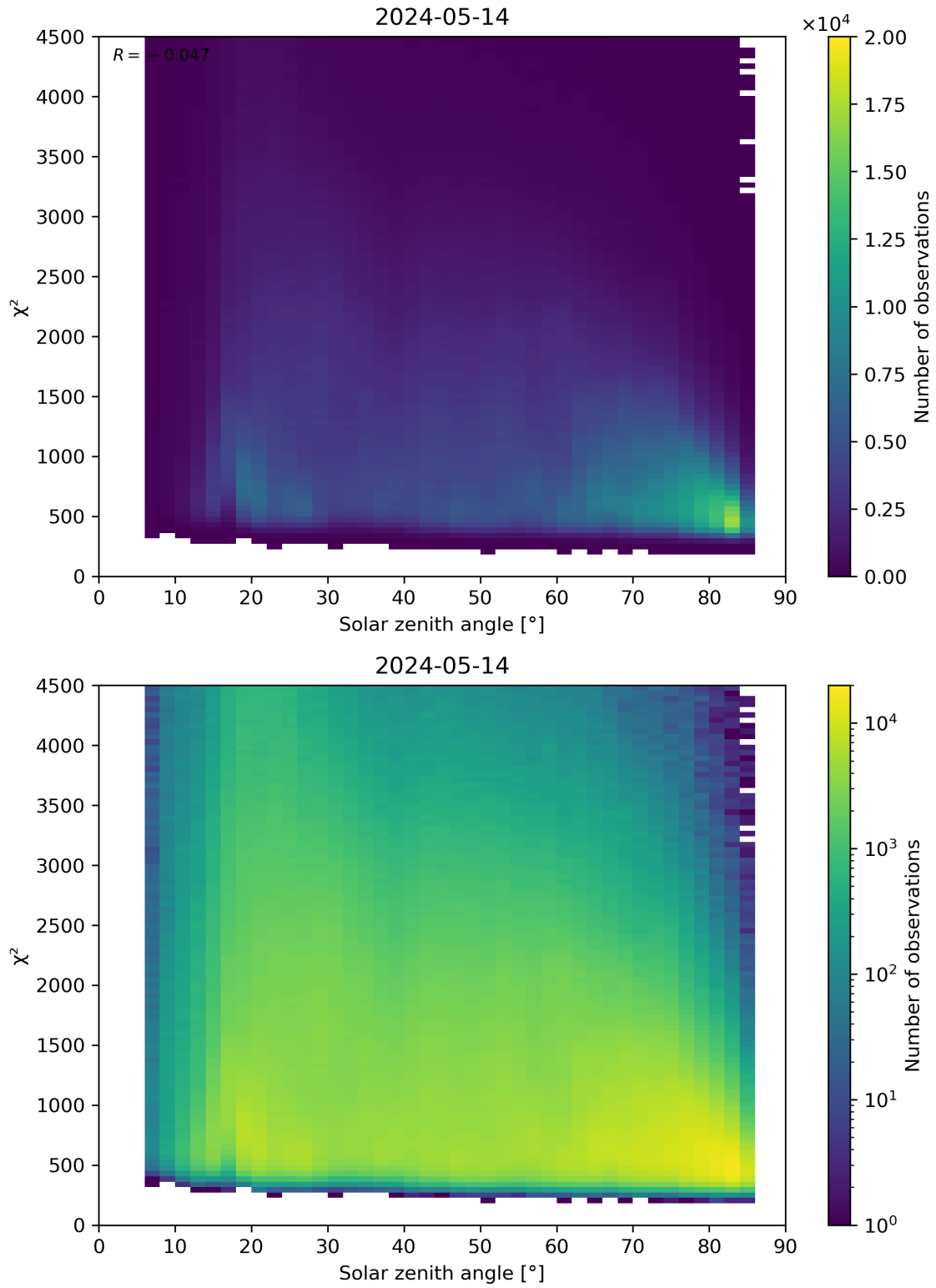
Figure 64: Scatter density plot of “Solar zenith angle” against “ \chi^2 ” for 2024-05-13 to 2024-05-15.
