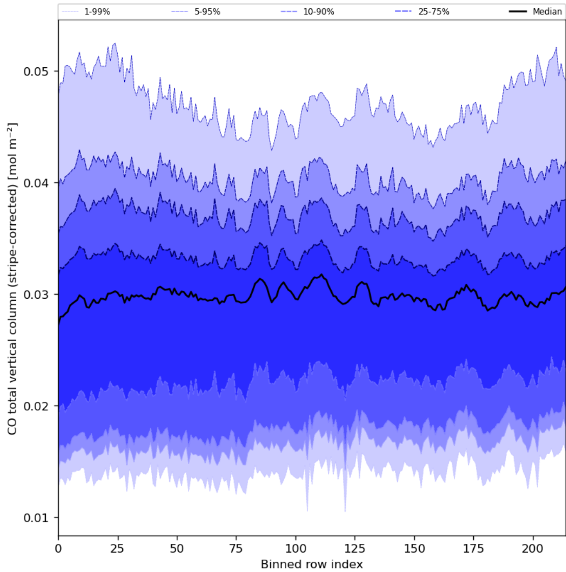
Figure 27: Along track statistics of “CO total vertical column (stripe-corrected)” for 2024-05-13 to 2024-05-15
