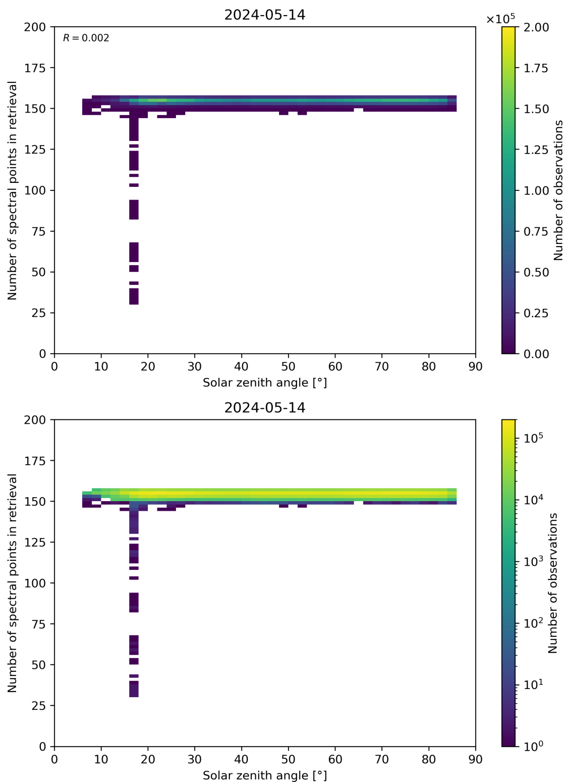
Figure 68: Scatter density plot of “Solar zenith angle” against “Number of spectral points in retrieval” for 2024-05-13 to 2024-05-15.
