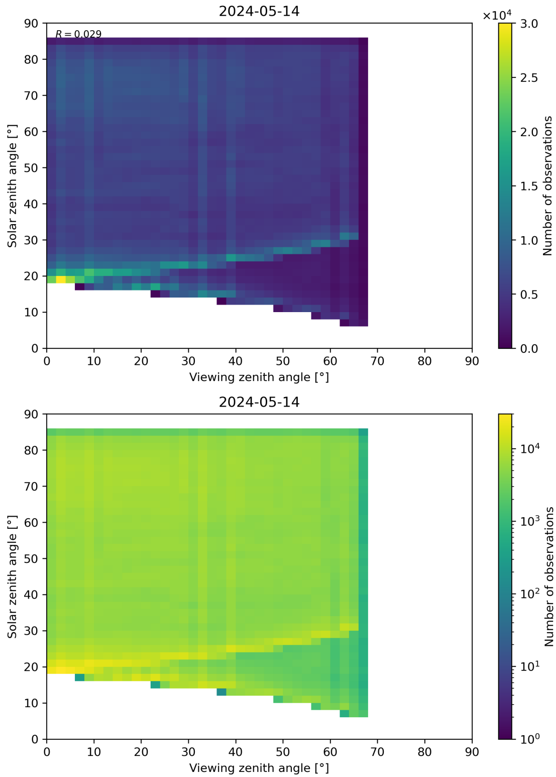
Figure 77: Scatter density plot of “Viewing zenith angle” against “Solar zenith angle” for 2024-05-13 to 2024-05-15.
