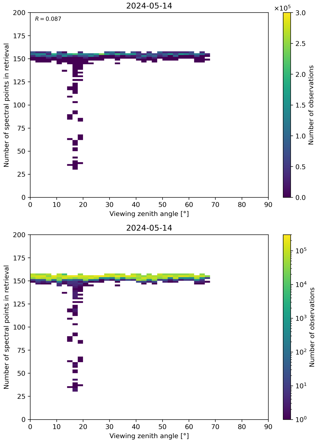
Figure 76: Scatter density plot of “Viewing zenith angle” against “Number of spectral points in retrieval” for 2024-05-13 to 2024-05-15.
