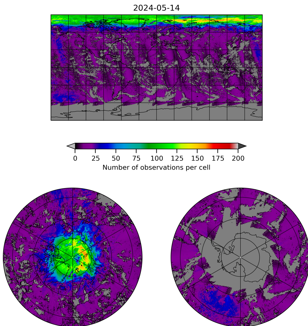
Figure 8: Map of the number of observations for 2024-05-13 to 2024-05-15
