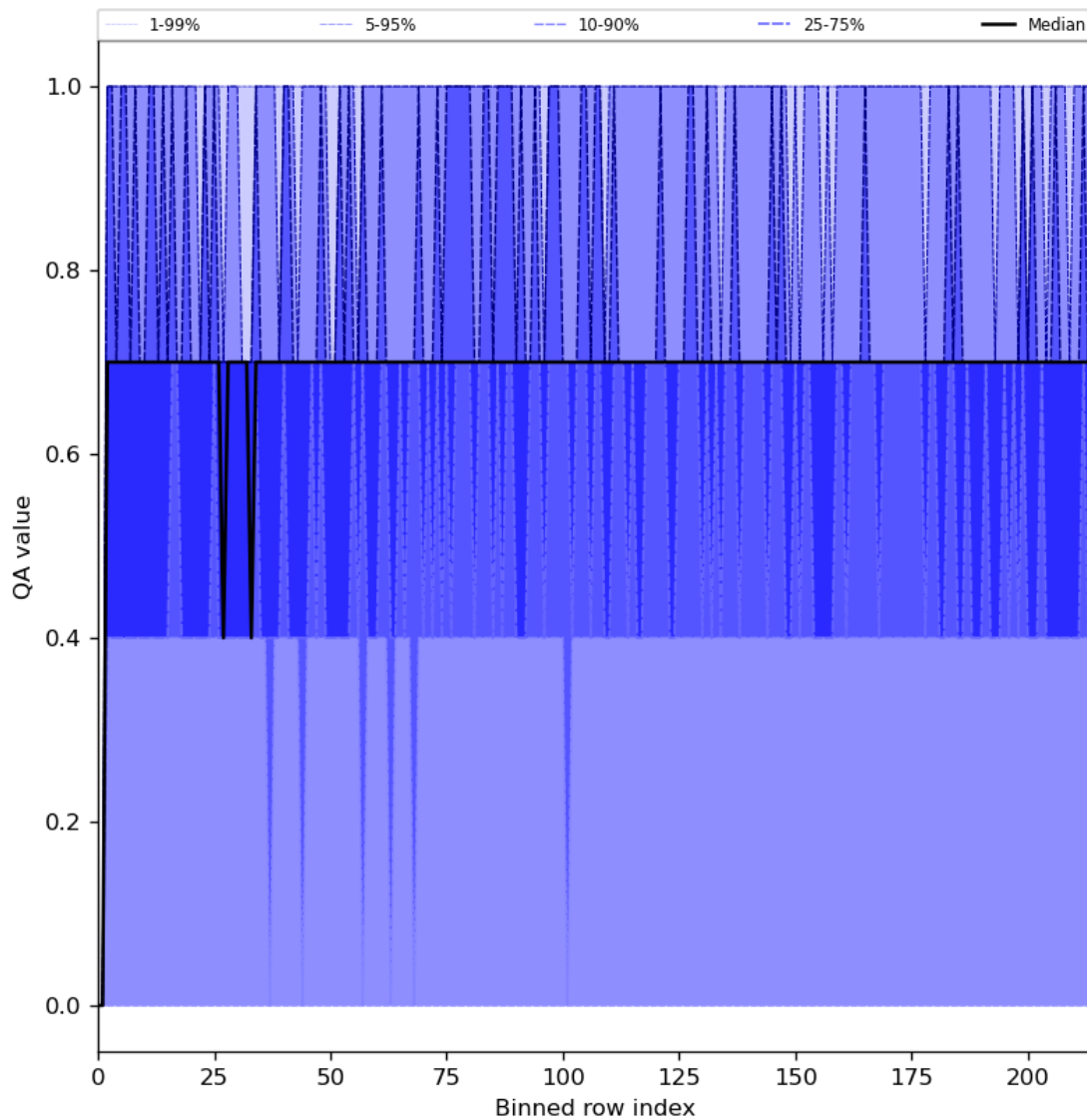
Figure 25: Along track statistics of “QA value” for 2024-05-13 to 2024-05-15
