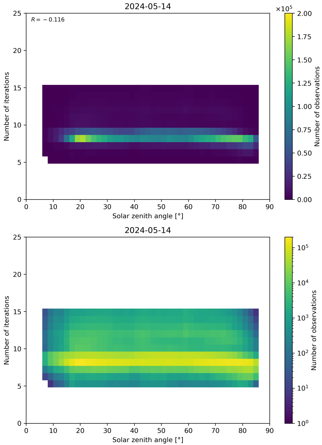
Figure 67: Scatter density plot of “Solar zenith angle” against “Number of iterations” for 2024-05-13 to 2024-05-15.
