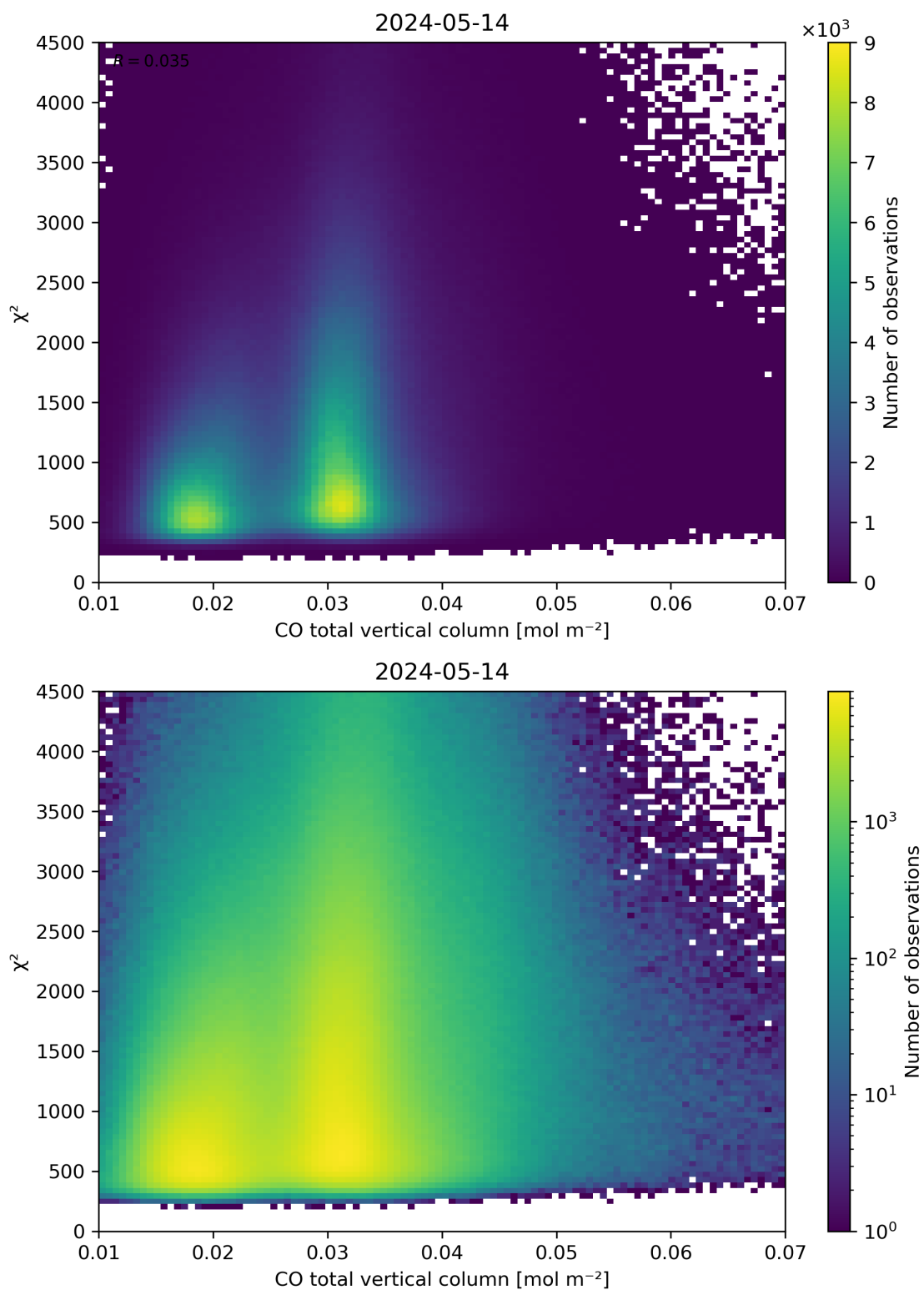
Figure 35: Scatter density plot of “CO total vertical column” against “ \chi^2 ” for 2024-05-13 to 2024-05-15.
