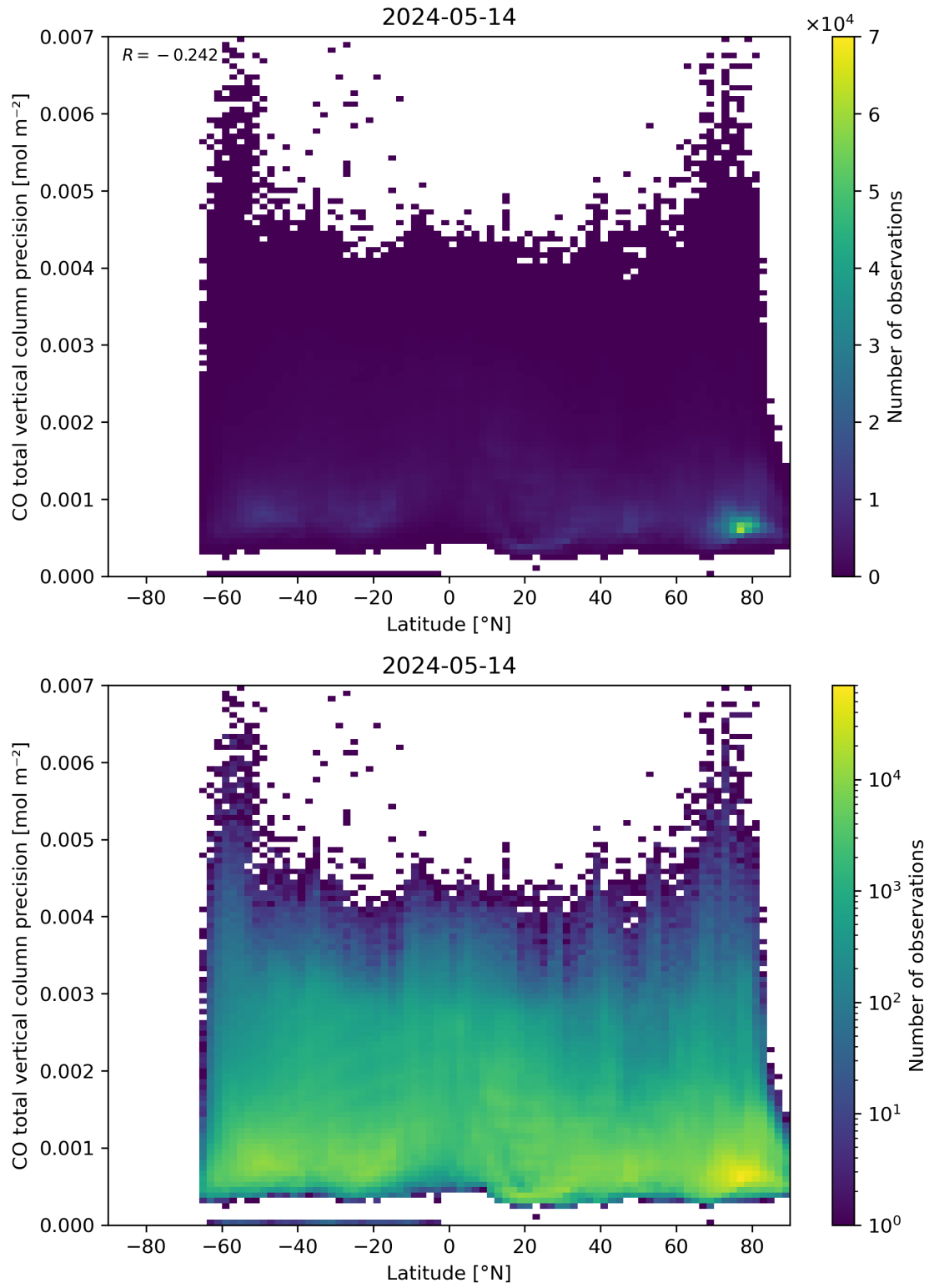
Figure 53: Scatter density plot of “Latitude” against “CO total vertical column precision” for 2024-05-13 to 2024-05-15.
