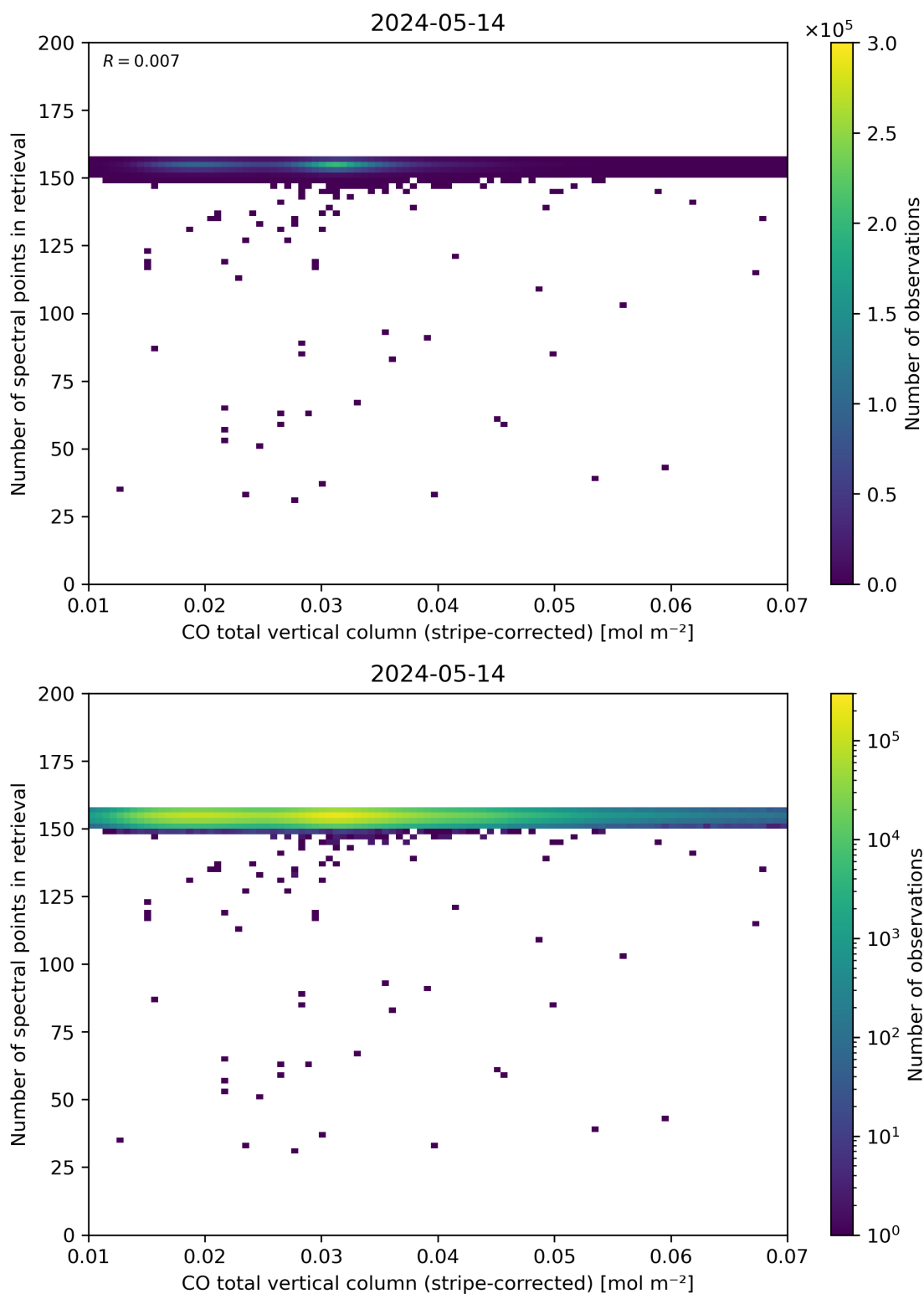
Figure 40: Scatter density plot of “CO total vertical column (stripe-corrected)” against “Number of spectral points in retrieval” for 2024-05-13 to 2024-05-15.
