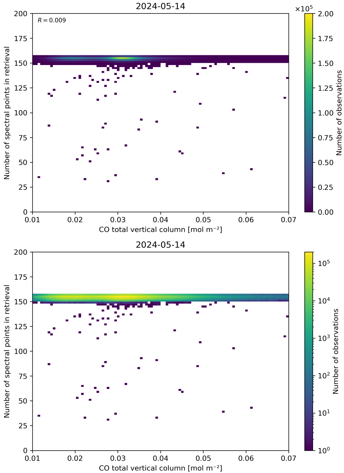
Figure 43: Scatter density plot of “CO total vertical column” against “Number of spectral points in retrieval” for 2024-05-13 to 2024-05-15.
