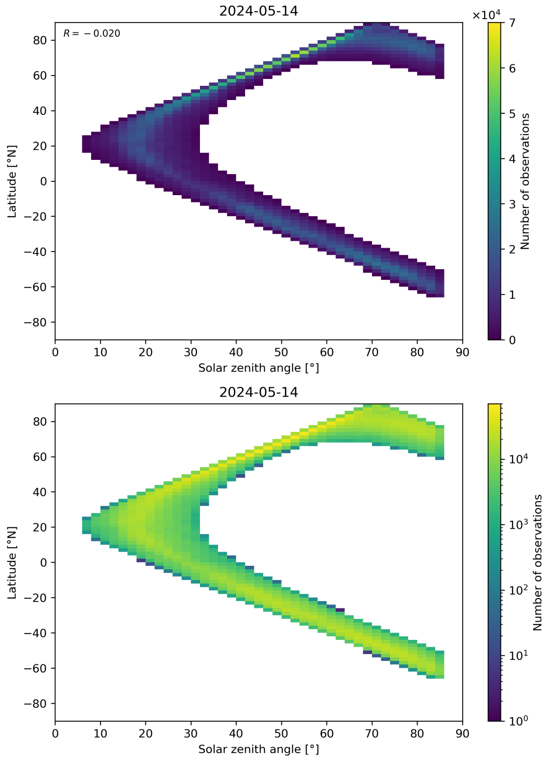
Figure 66: Scatter density plot of “Solar zenith angle” against “Latitude” for 2024-05-13 to 2024-05-15.
