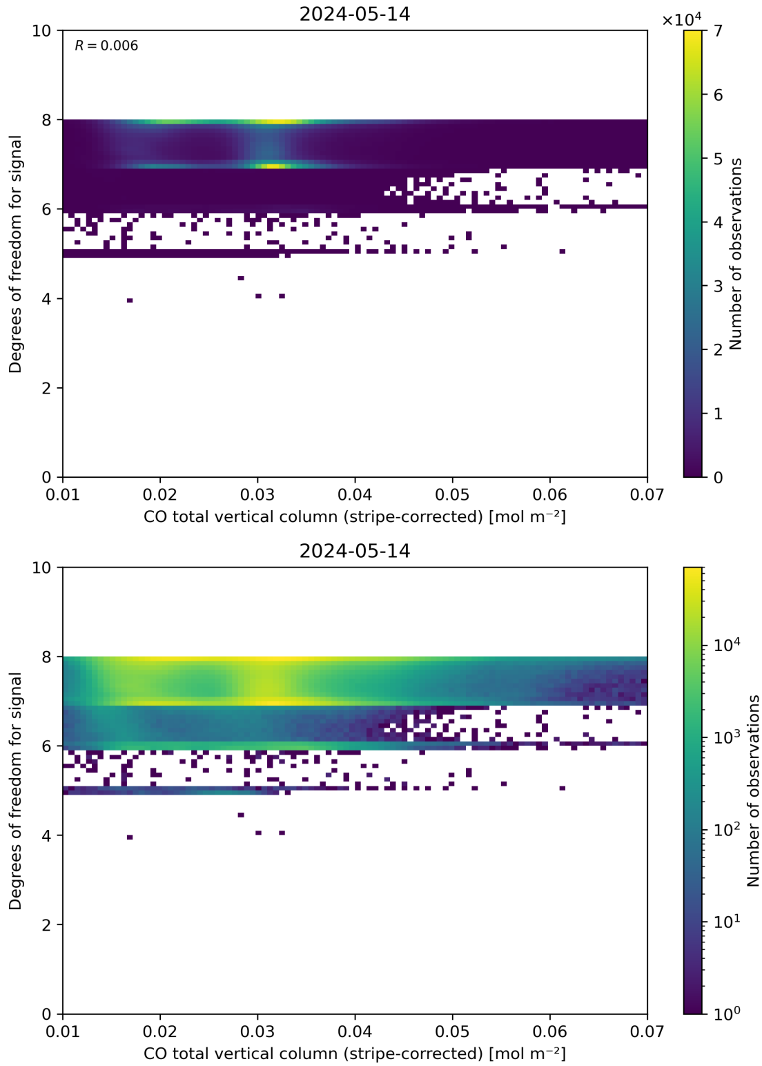
Figure 38: Scatter density plot of “CO total vertical column (stripe-corrected)” against “Degrees of freedom for signal” for 2024-05-13 to 2024-05-15.
