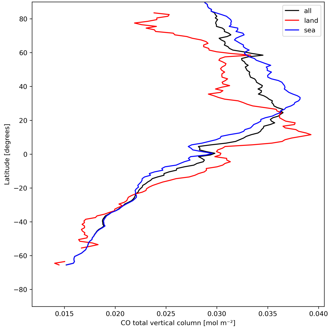
Figure 10: Zonal average of “CO total vertical column” for 2024-05-13 to 2024-05-15.
