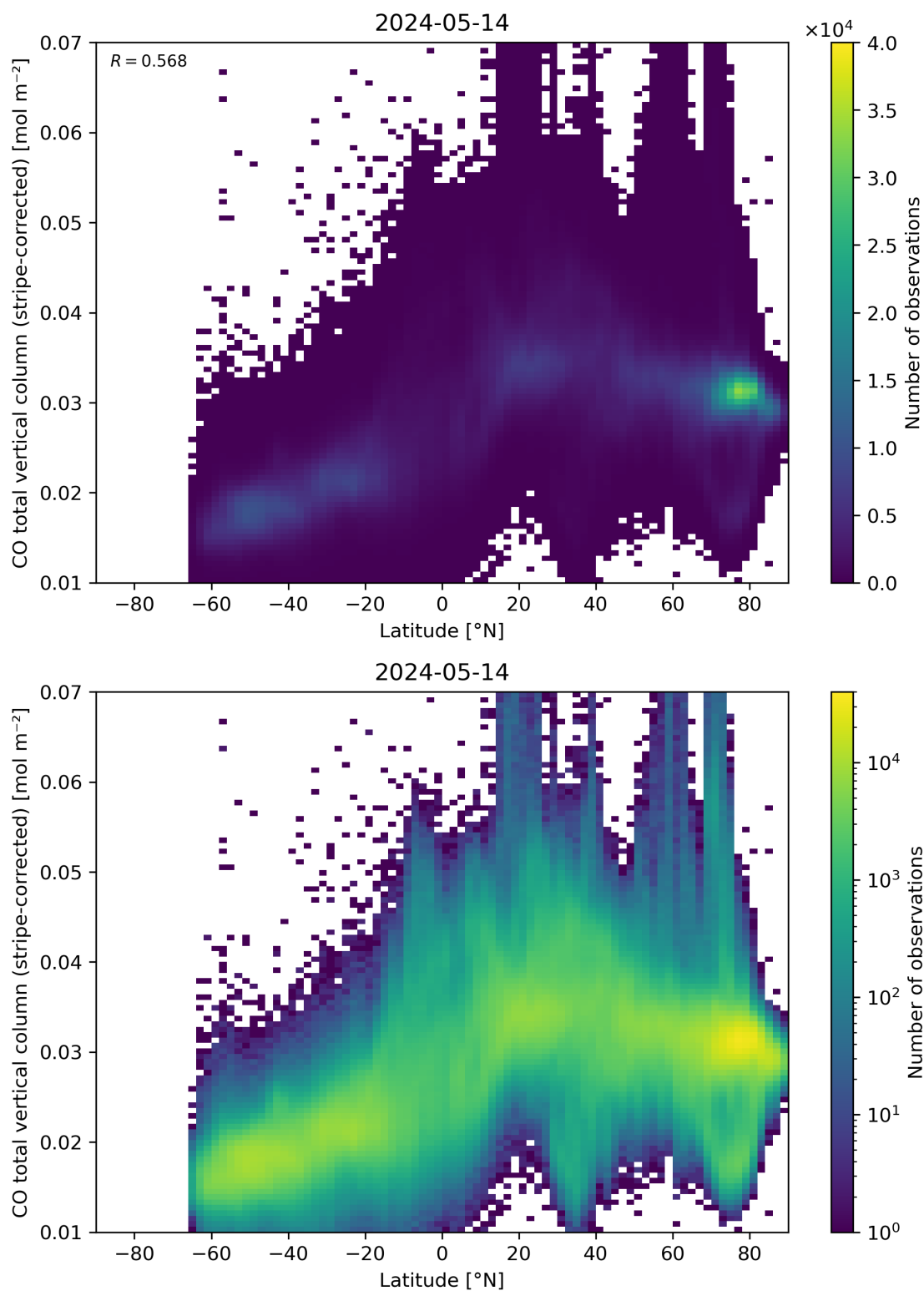
Figure 52: Scatter density plot of “Latitude” against “CO total vertical column (stripe-corrected)” for 2024-05-13 to 2024-05-15.
