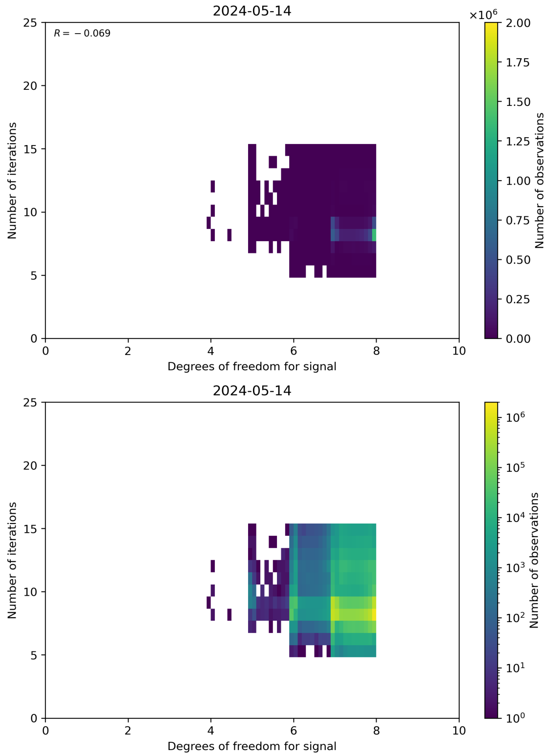
Figure 50: Scatter density plot of “Degrees of freedom for signal” against “Number of iterations” for 2024-05-13 to 2024-05-15.
