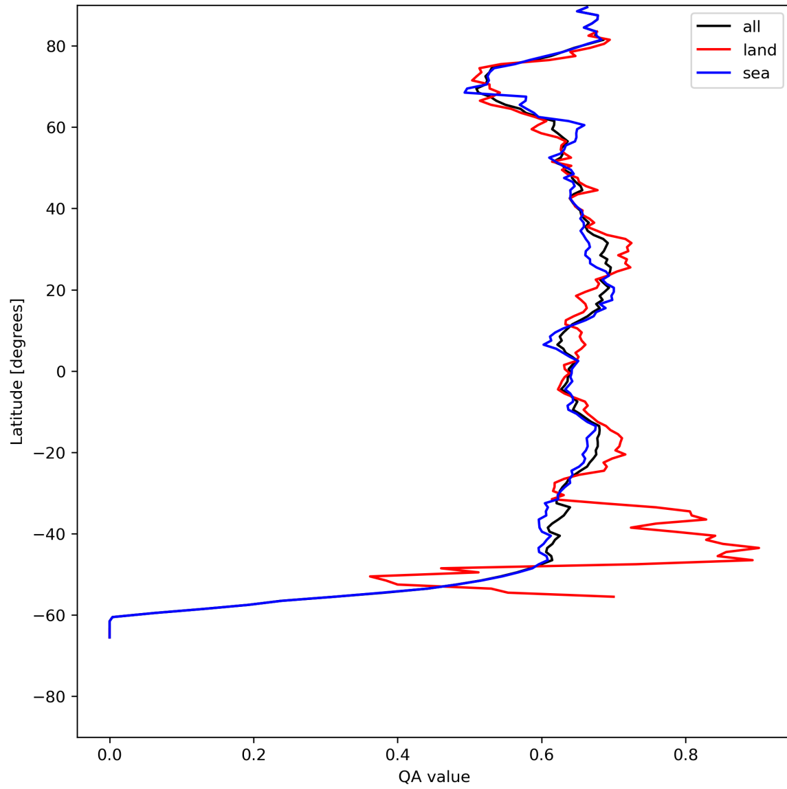
Figure 9: Zonal average of “QA value” for 2024-05-13 to 2024-05-15.
