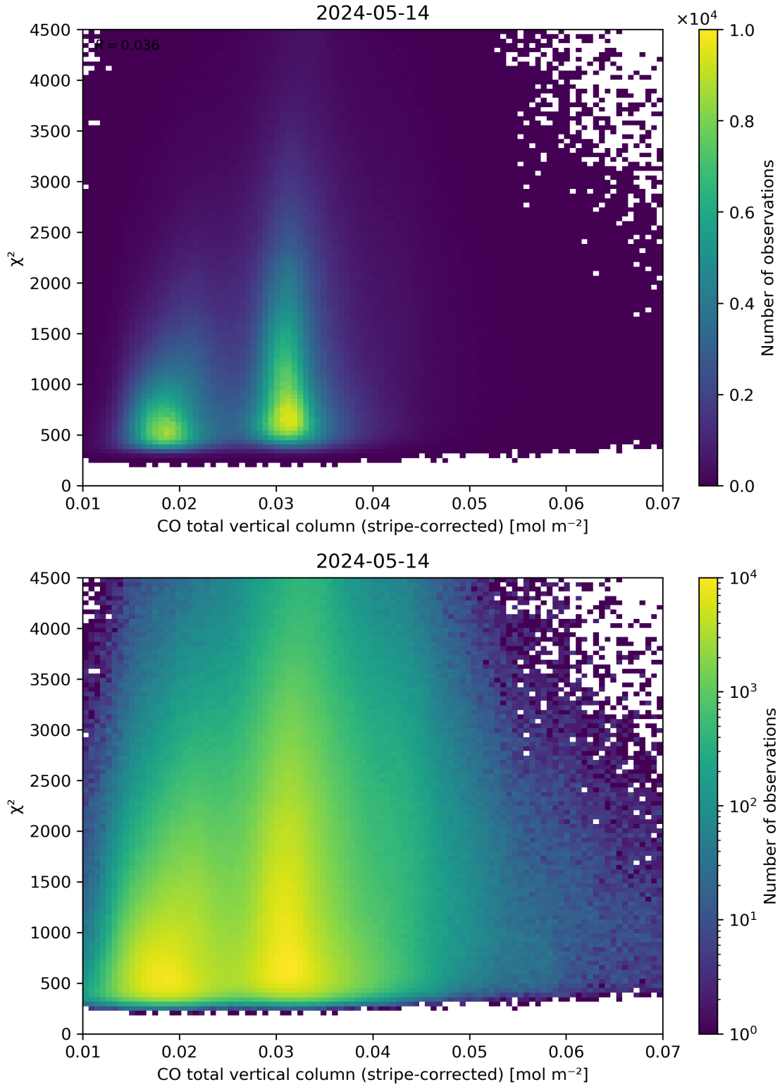
Figure 37: Scatter density plot of “CO total vertical column (stripe-corrected)” against “ \chi^2 ” for 2024-05-13 to 2024-05-15.
