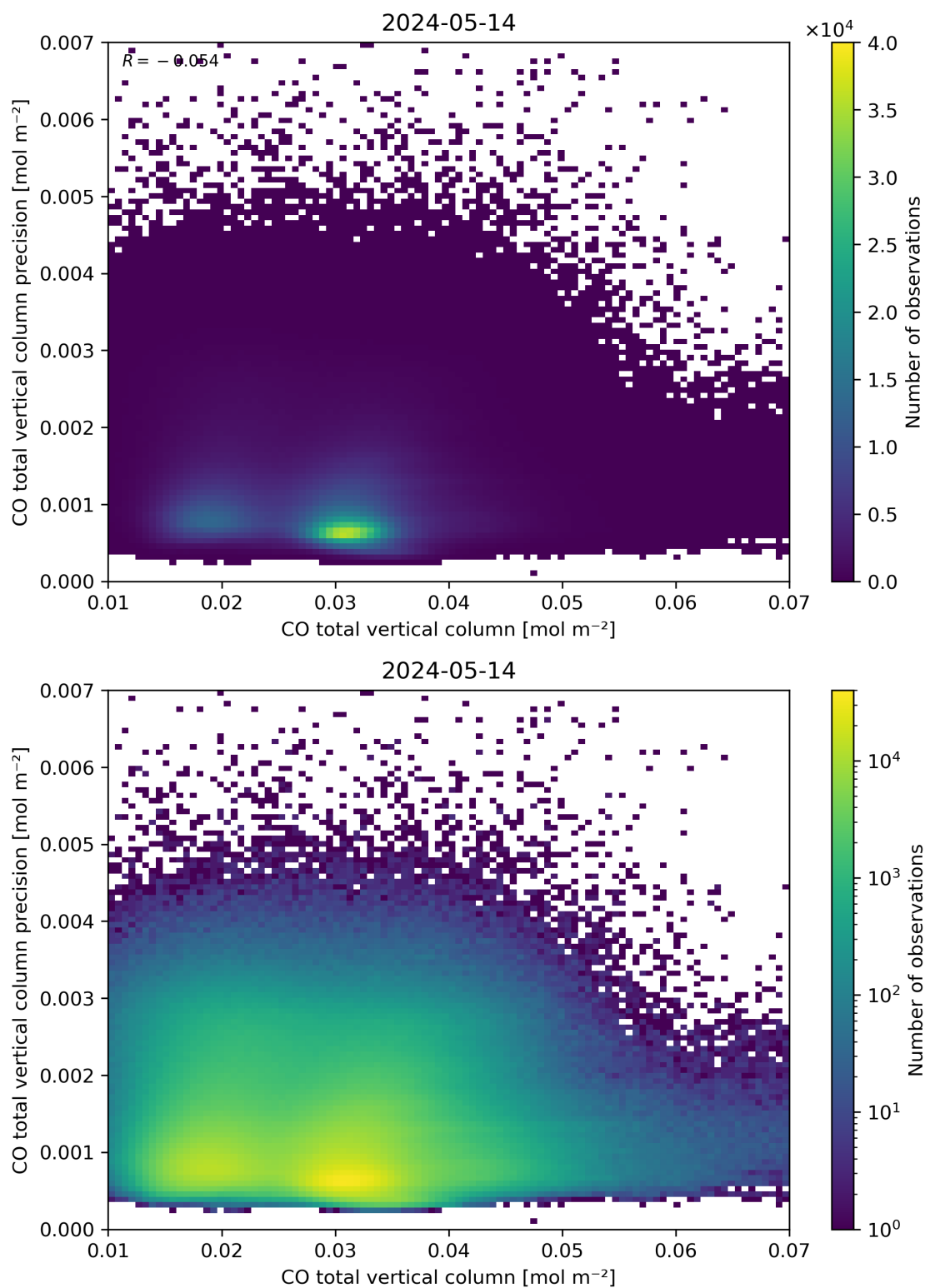
Figure 34: Scatter density plot of “CO total vertical column” against “CO total vertical column precision” for 2024-05-13 to 2024-05-15.
