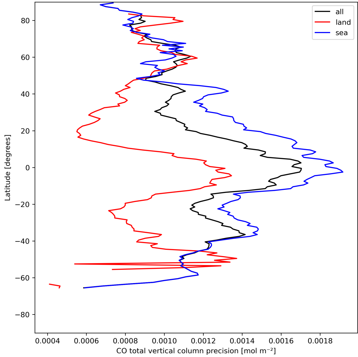
Figure 12: Zonal average of "CO total vertical column precision" for 2024-05-13 to 2024-05-15.
