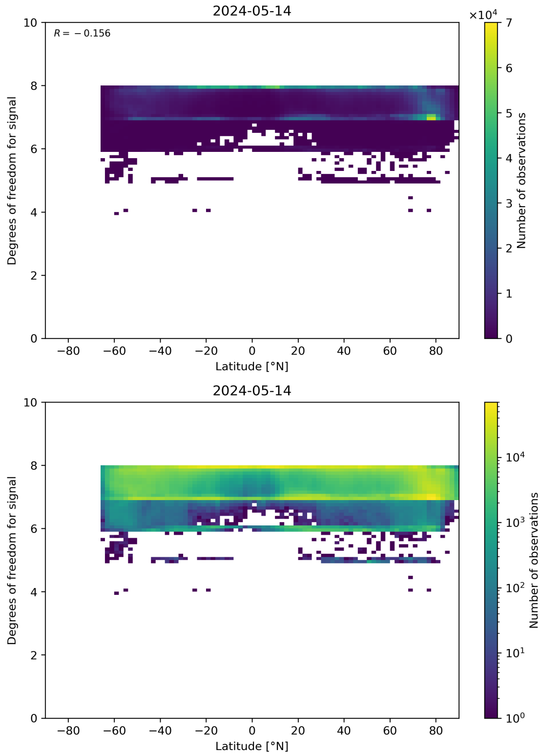
Figure 55: Scatter density plot of “Latitude” against “Degrees of freedom for signal” for 2024-05-13 to 2024-05-15.
