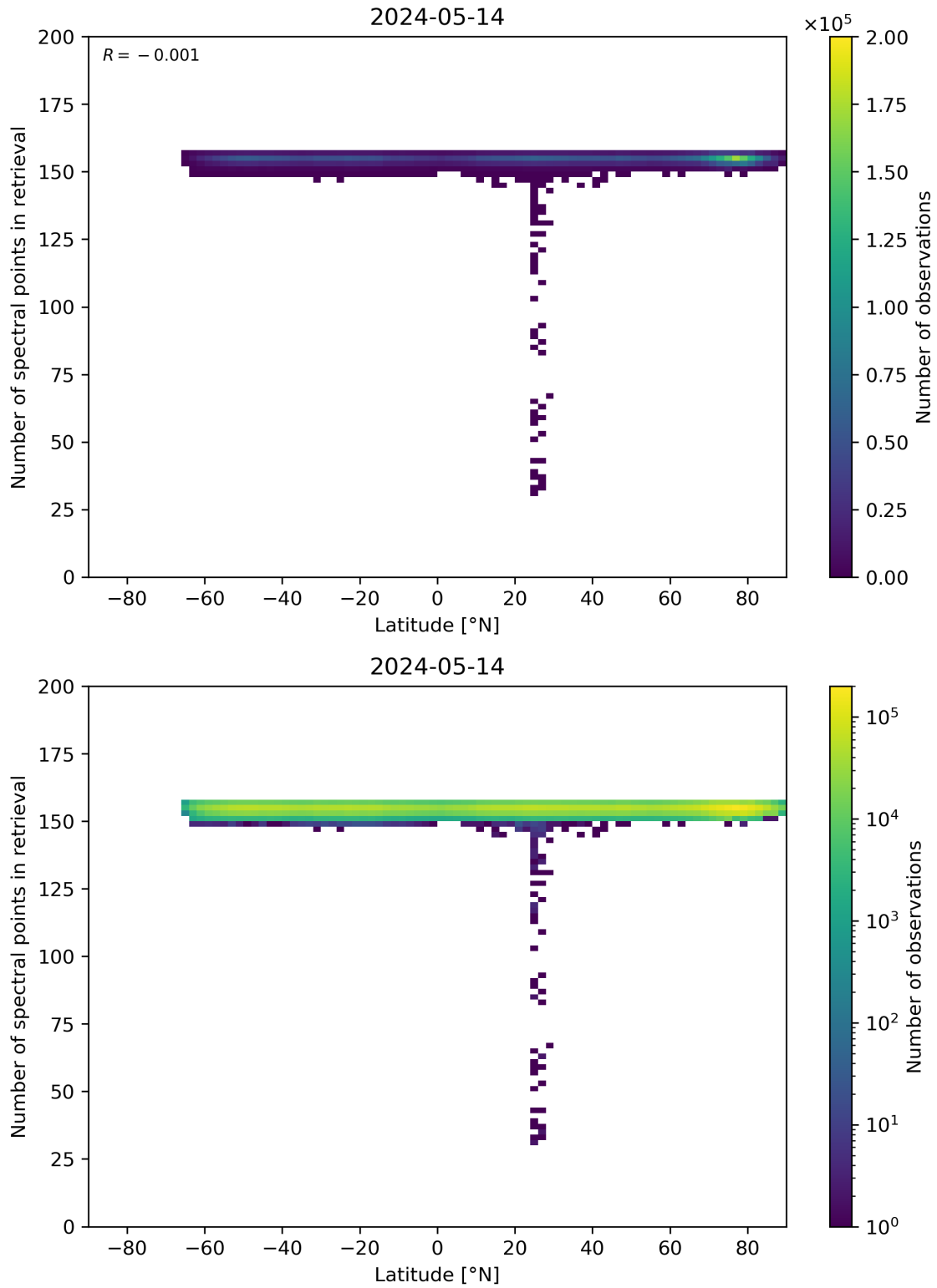
Figure 57: Scatter density plot of “Latitude” against “Number of spectral points in retrieval” for 2024-05-13 to 2024-05-15.
