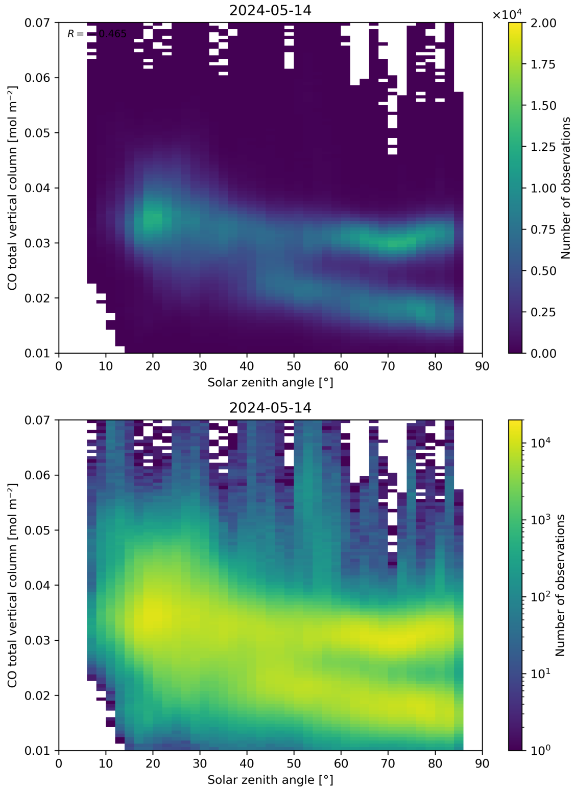
Figure 61: Scatter density plot of “Solar zenith angle” against “CO total vertical column” for 2024-05-13 to 2024-05-15.
