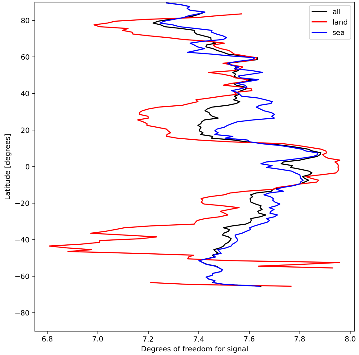
Figure 15: Zonal average of “Degrees of freedom for signal” for 2024-05-13 to 2024-05-15.
