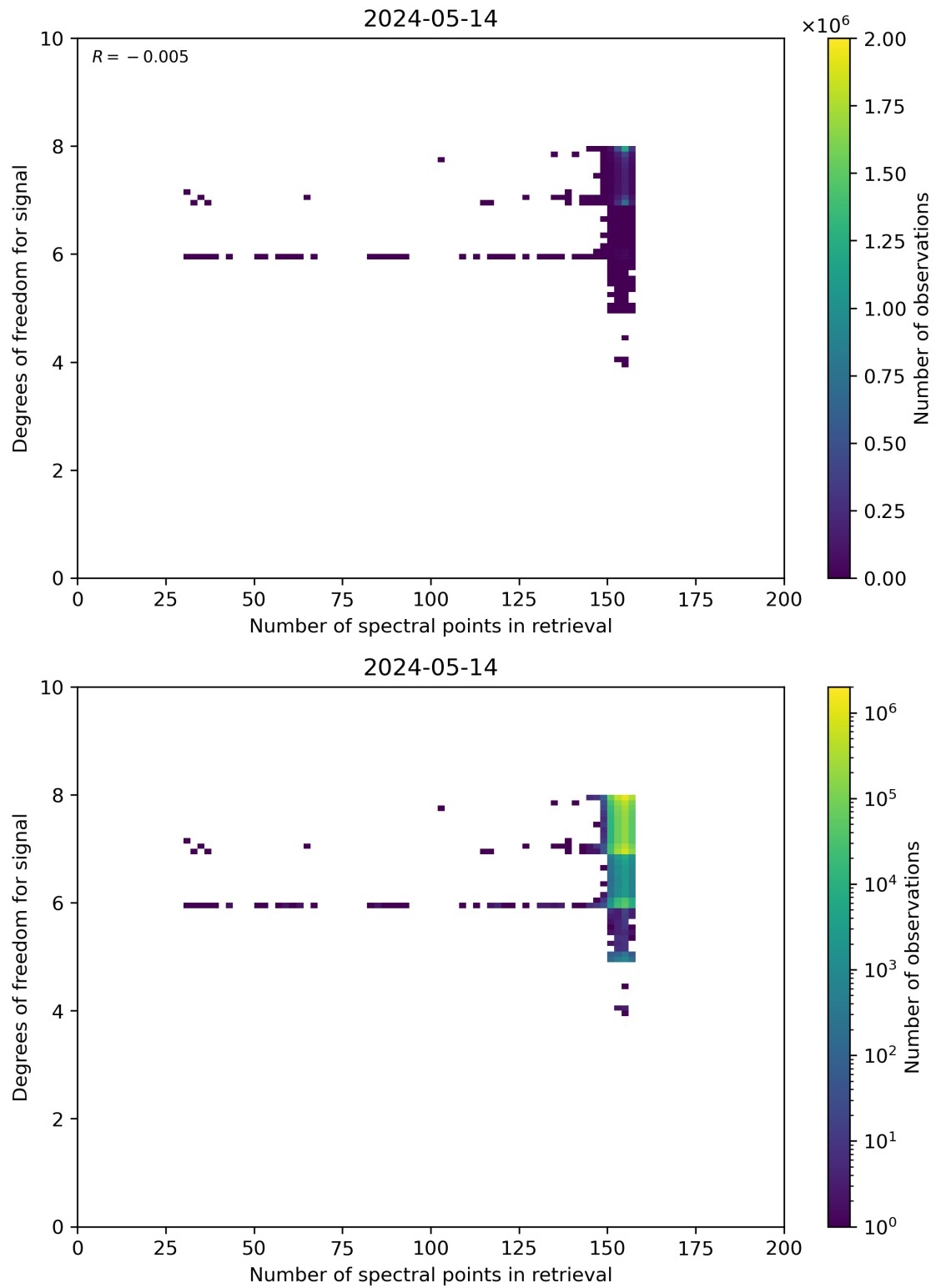
Figure 59: Scatter density plot of “Number of spectral points in retrieval” against “Degrees of freedom for signal” for 2024-05-13 to 2024-05-15.
