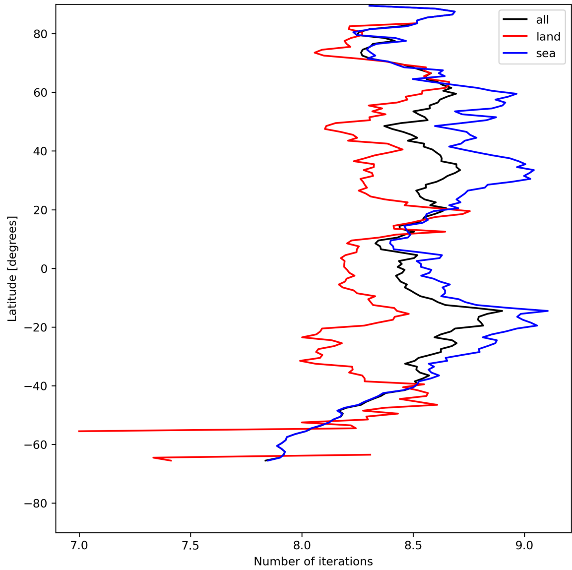
Figure 16: Zonal average of “Number of iterations” for 2024-05-13 to 2024-05-15.
