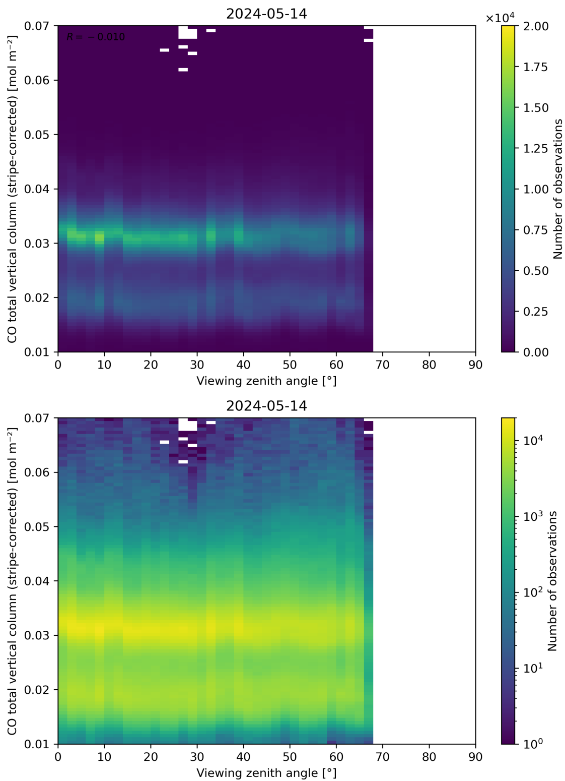
Figure 70: Scatter density plot of “Viewing zenith angle” against “CO total vertical column (stripe-corrected)” for 2024-05-13 to 2024-05-15.
