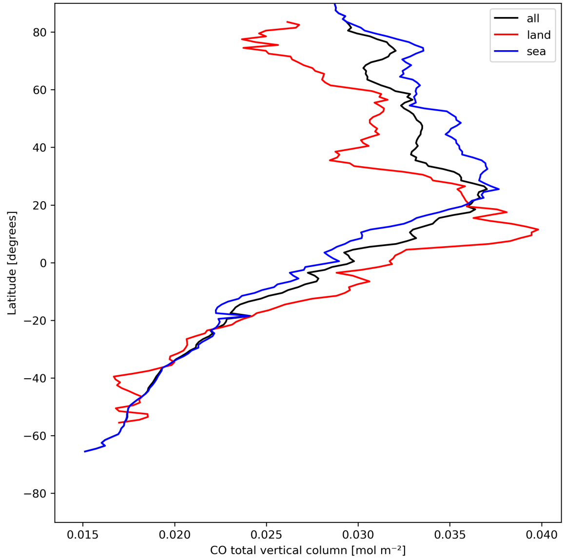
Figure 10: Zonal average of “CO total vertical column” for 2024-05-14 to 2024-05-16.
