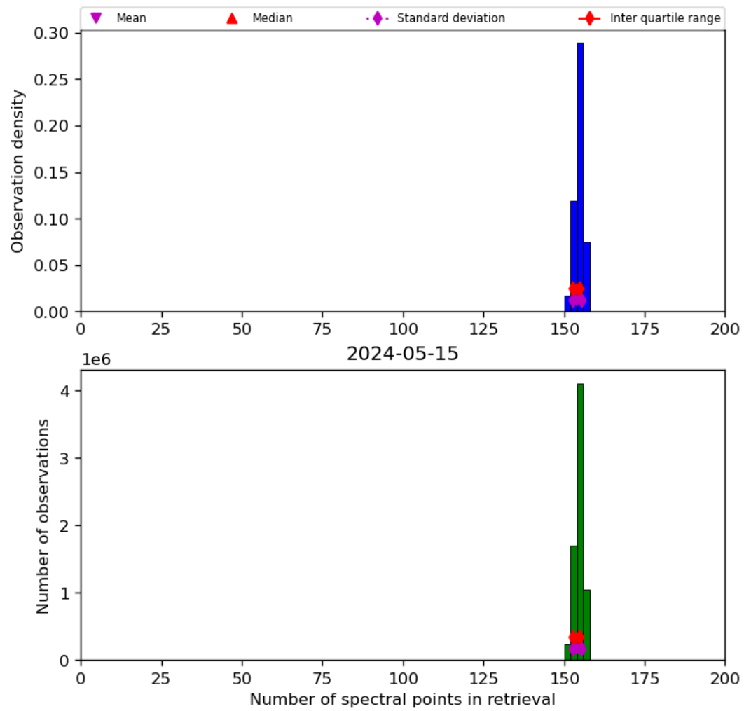
Figure 21: Histogram of “Number of spectral points in retrieval” for 2024-05-14 to 2024-05-16
