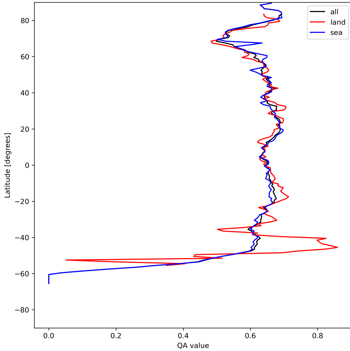
Figure 9: Zonal average of “QA value” for 2024-05-14 to 2024-05-16.
