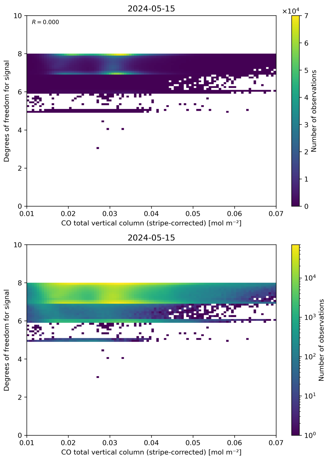
Figure 38: Scatter density plot of “CO total vertical column (stripe-corrected)” against “Degrees of freedom for signal” for 2024-05-14 to 2024-05-16.
