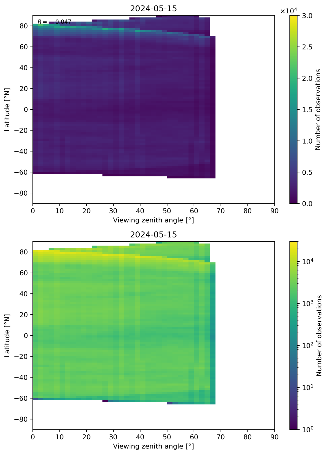
Figure 74: Scatter density plot of “Viewing zenith angle” against “Latitude” for 2024-05-14 to 2024-05-16.
