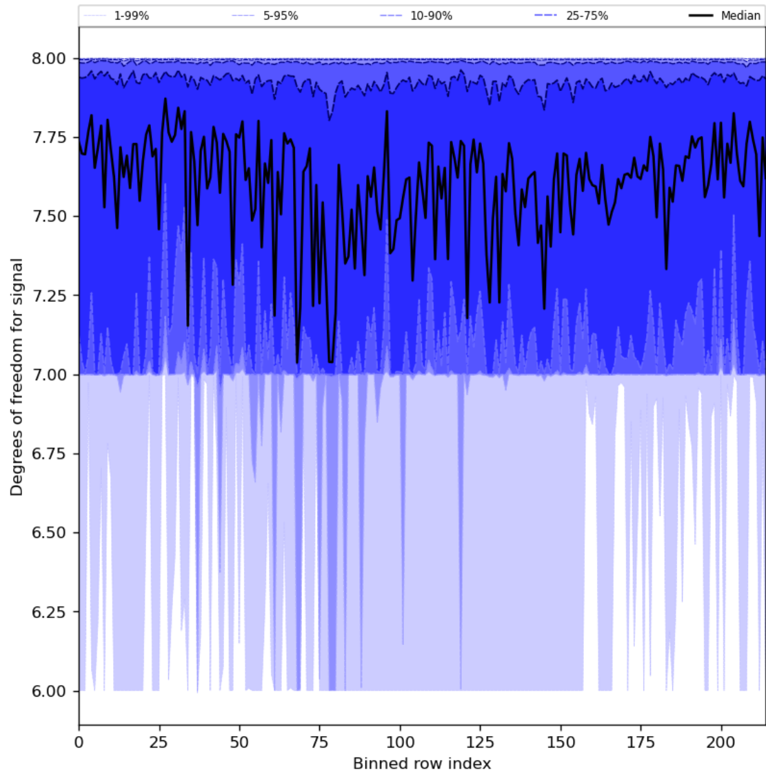
Figure 31: Along track statistics of “Degrees of freedom for signal” for 2024-05-14 to 2024-05-16
