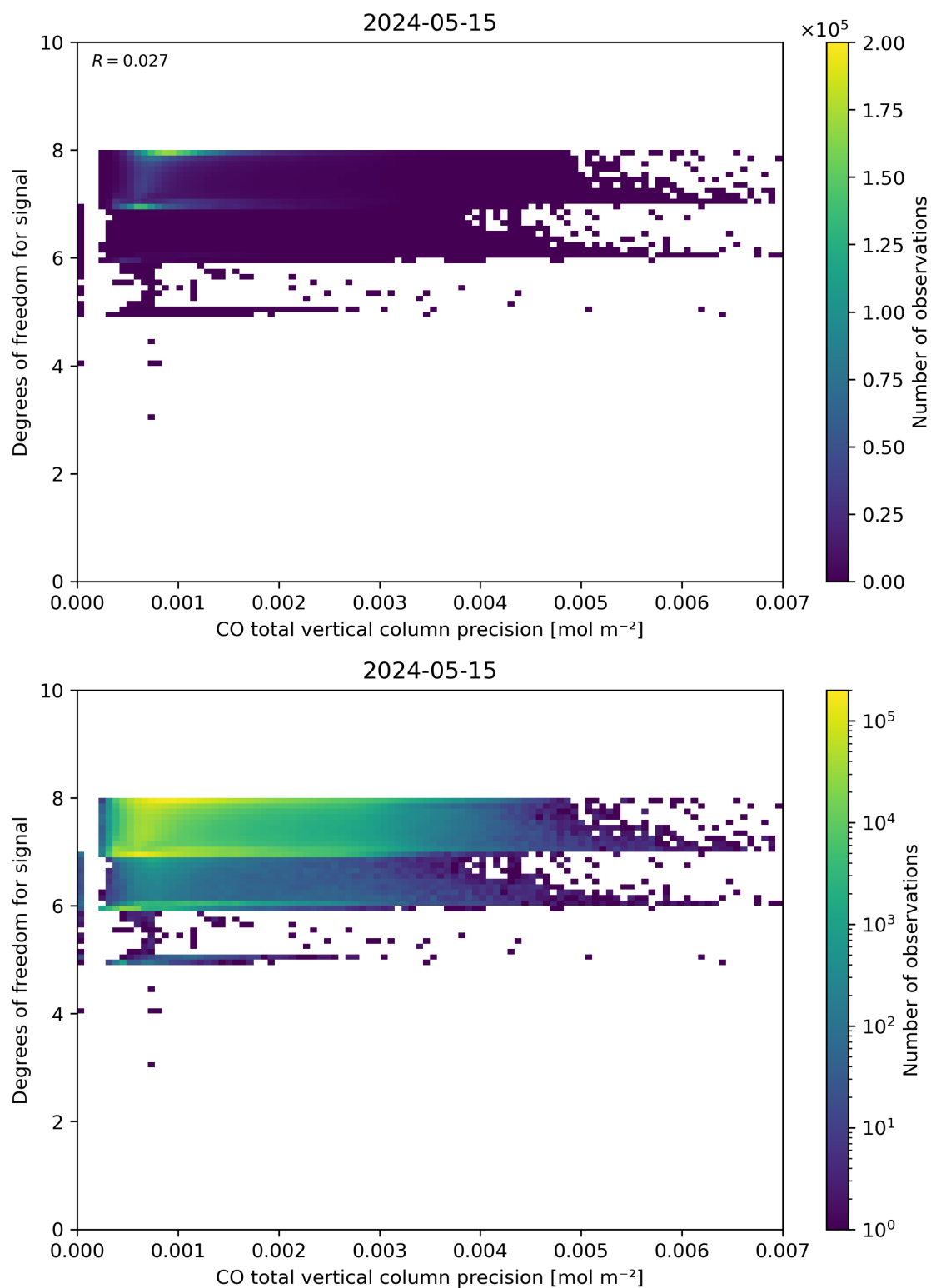
Figure 45: Scatter density plot of “CO total vertical column precision” against “Degrees of freedom for signal” for 2024-05-14 to 2024-05-16.
