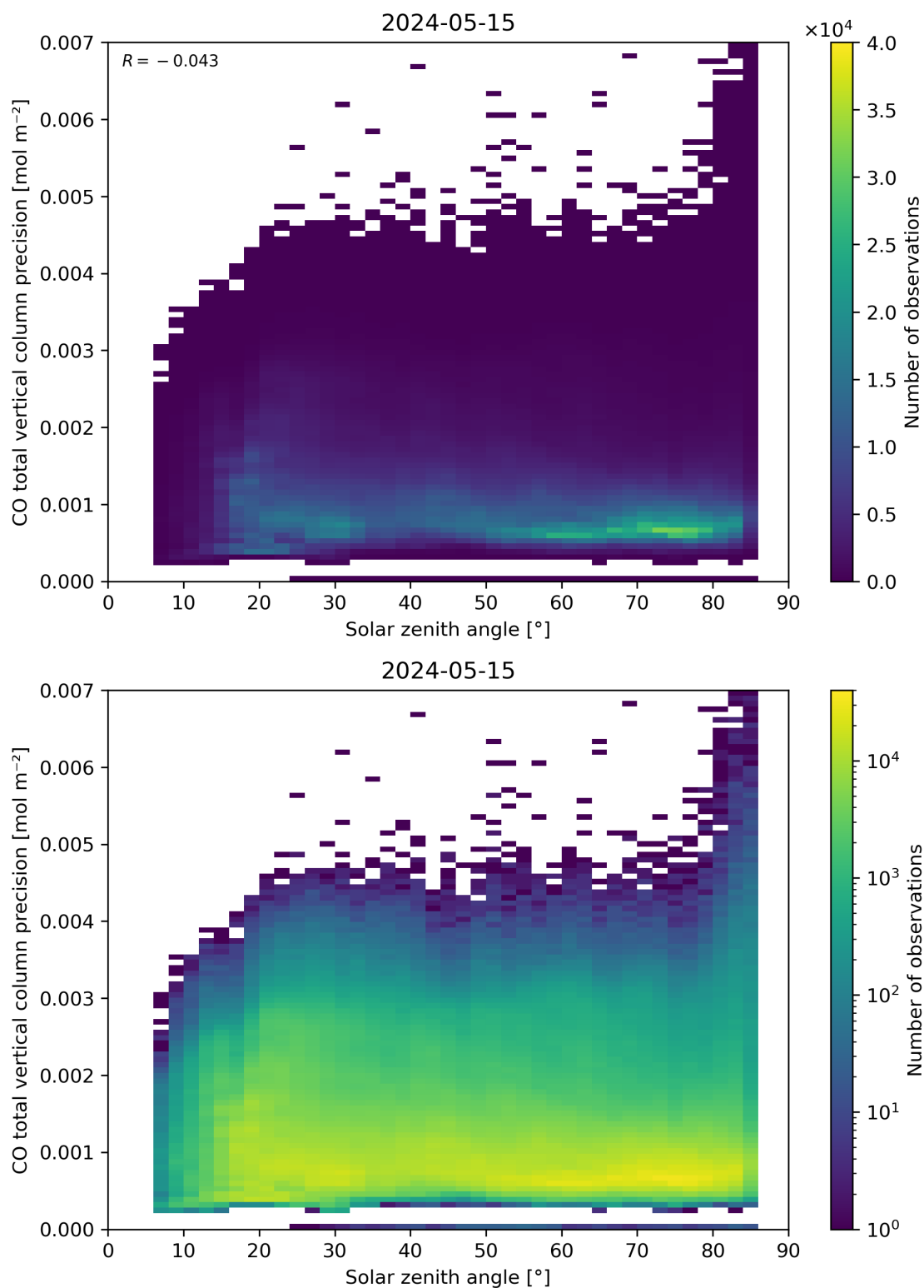
Figure 63: Scatter density plot of “Solar zenith angle” against “CO total vertical column precision” for 2024-05-14 to 2024-05-16.
