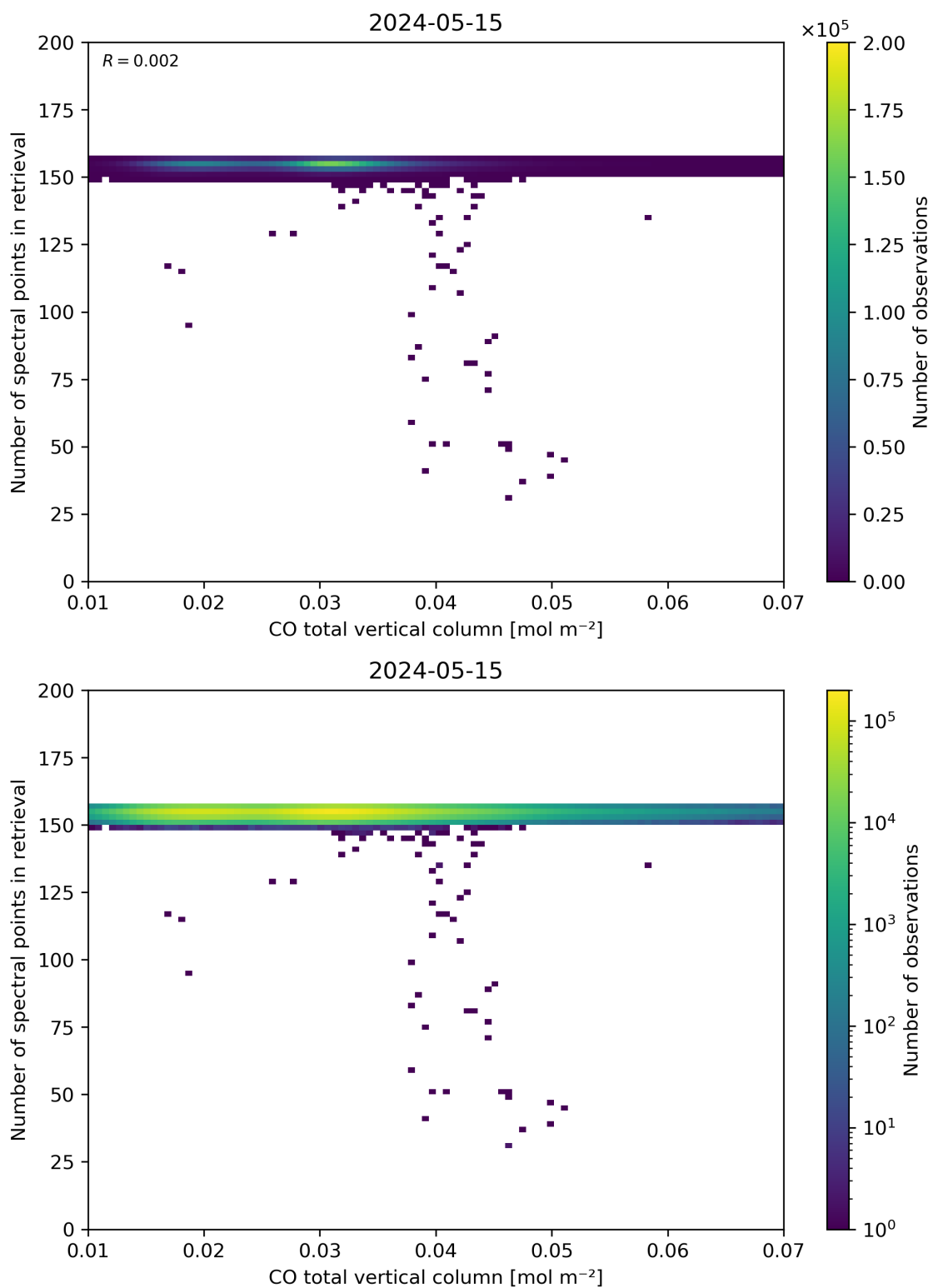
Figure 43: Scatter density plot of “CO total vertical column” against “Number of spectral points in retrieval” for 2024-05-14 to 2024-05-16.
