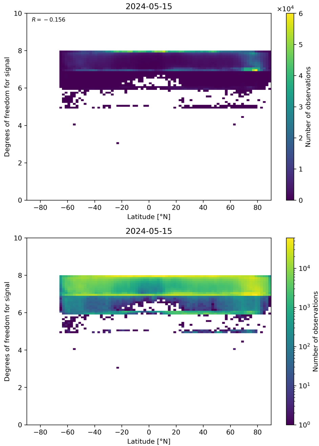
Figure 55: Scatter density plot of “Latitude” against “Degrees of freedom for signal” for 2024-05-14 to 2024-05-16.
