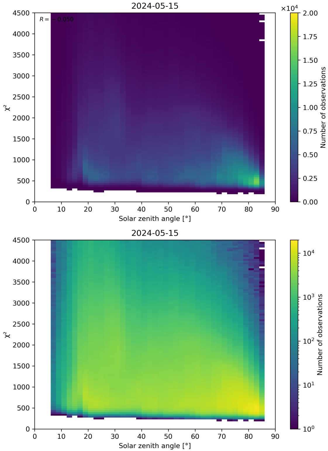
Figure 64: Scatter density plot of “Solar zenith angle” against “ \chi^2 ” for 2024-05-14 to 2024-05-16.
