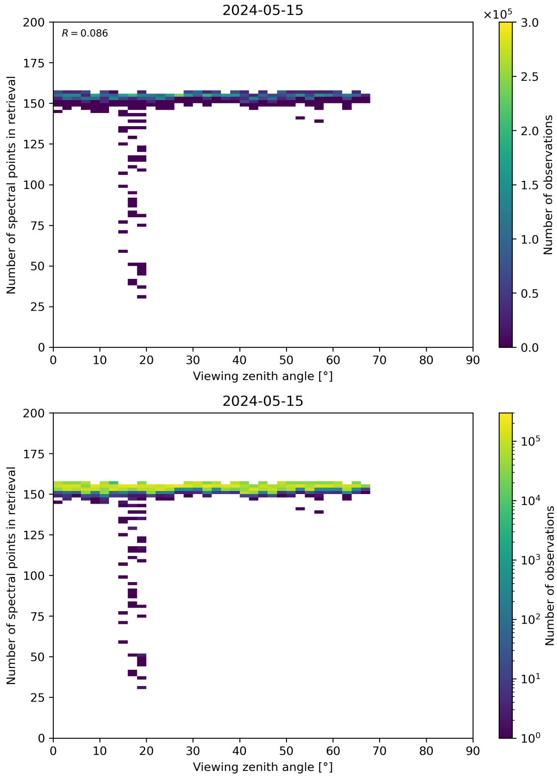
Figure 76: Scatter density plot of “Viewing zenith angle” against “Number of spectral points in retrieval” for 2024-05-14 to 2024-05-16.
