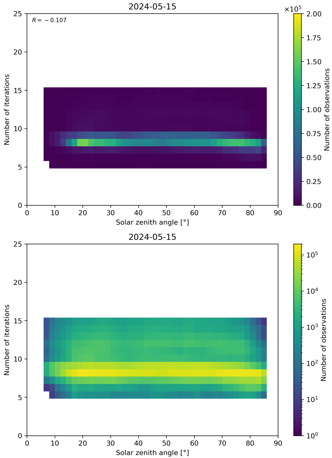
Figure 67: Scatter density plot of “Solar zenith angle” against “Number of iterations” for 2024-05-14 to 2024-05-16.
