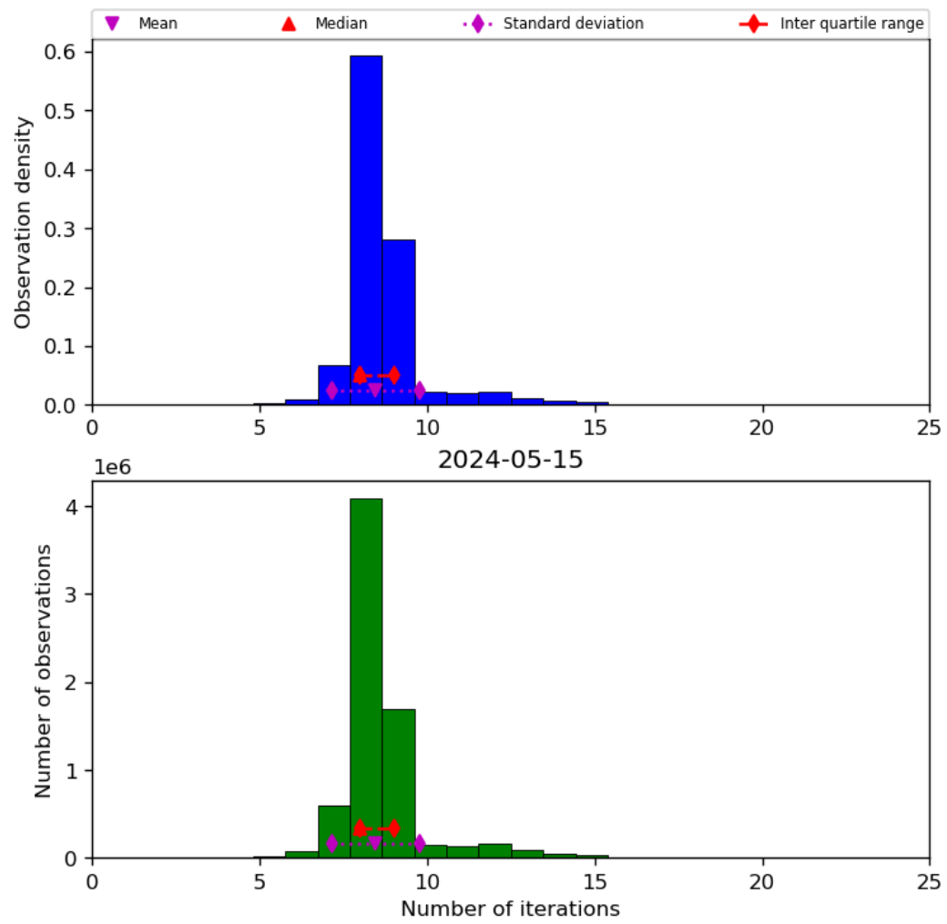
Figure 24: Histogram of “Number of iterations” for 2024-05-14 to 2024-05-16
