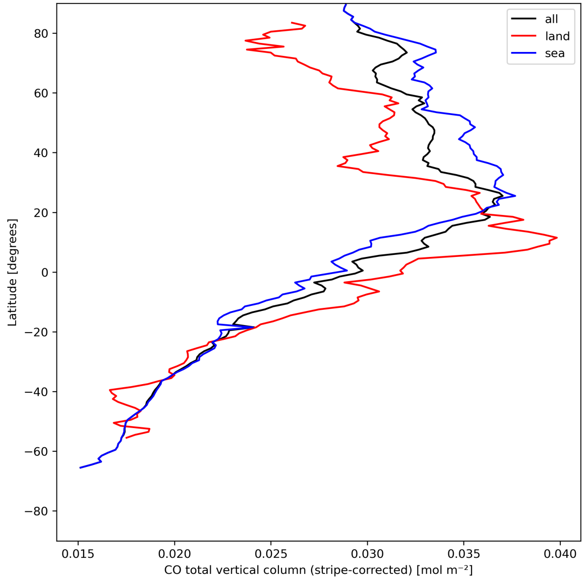
Figure 11: Zonal average of “CO total vertical column (stripe-corrected)” for 2024-05-14 to 2024-05-16.
