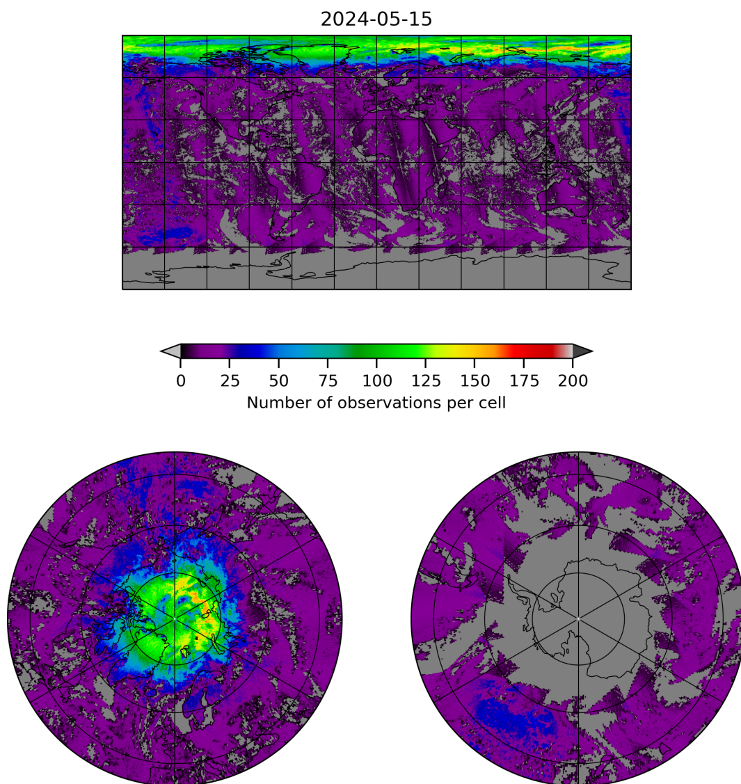
Figure 8: Map of the number of observations for 2024-05-14 to 2024-05-16
