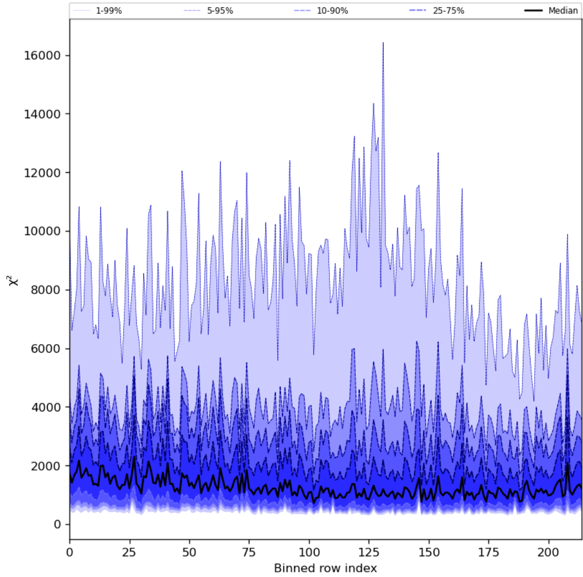
Figure 30: Along track statistics of “ \chi^2 ” for 2024-05-14 to 2024-05-16
