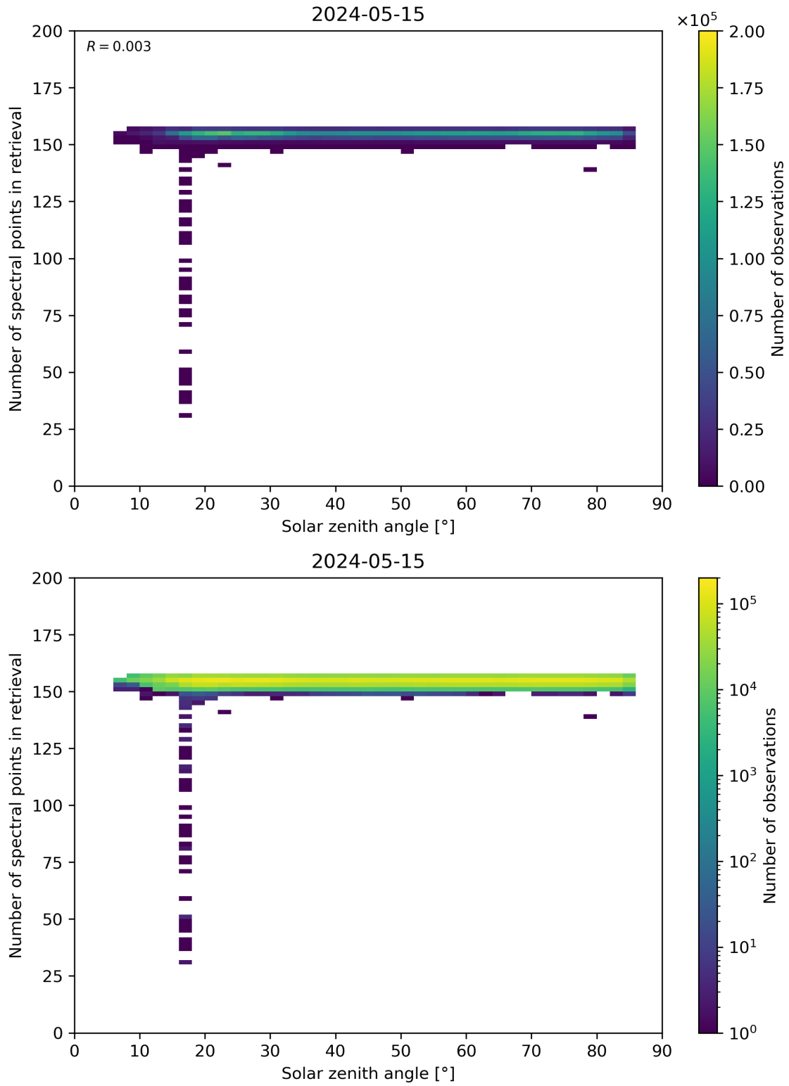
Figure 68: Scatter density plot of “Solar zenith angle” against “Number of spectral points in retrieval” for 2024-05-14 to 2024-05-16.
