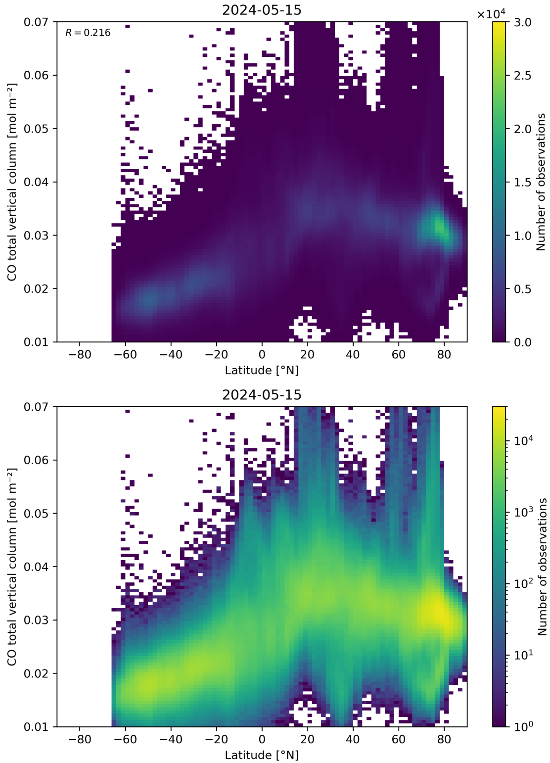
Figure 51: Scatter density plot of “Latitude” against “CO total vertical column” for 2024-05-14 to 2024-05-16.
