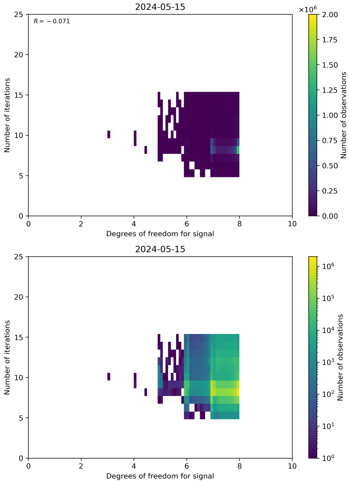
Figure 50: Scatter density plot of “Degrees of freedom for signal” against “Number of iterations” for 2024-05-14 to 2024-05-16.
