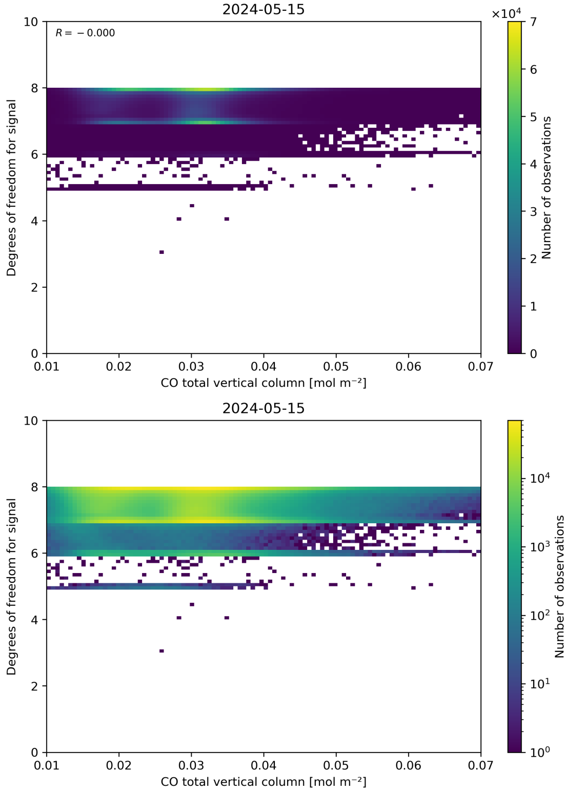
Figure 41: Scatter density plot of “CO total vertical column” against “Degrees of freedom for signal” for 2024-05-14 to 2024-05-16.
