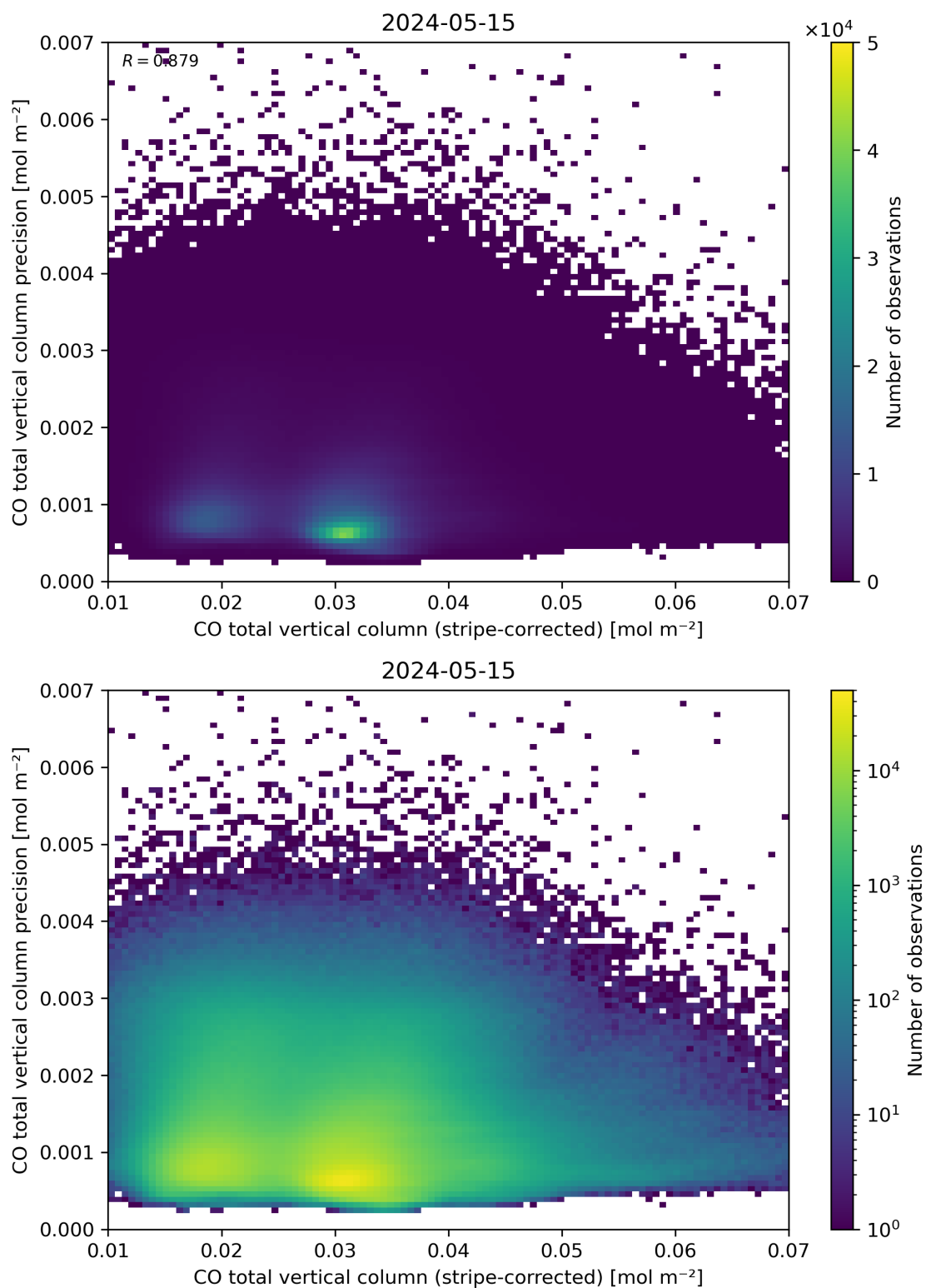
Figure 36: Scatter density plot of “CO total vertical column (stripe-corrected)” against “CO total vertical column precision” for 2024-05-14 to 2024-05-16.
