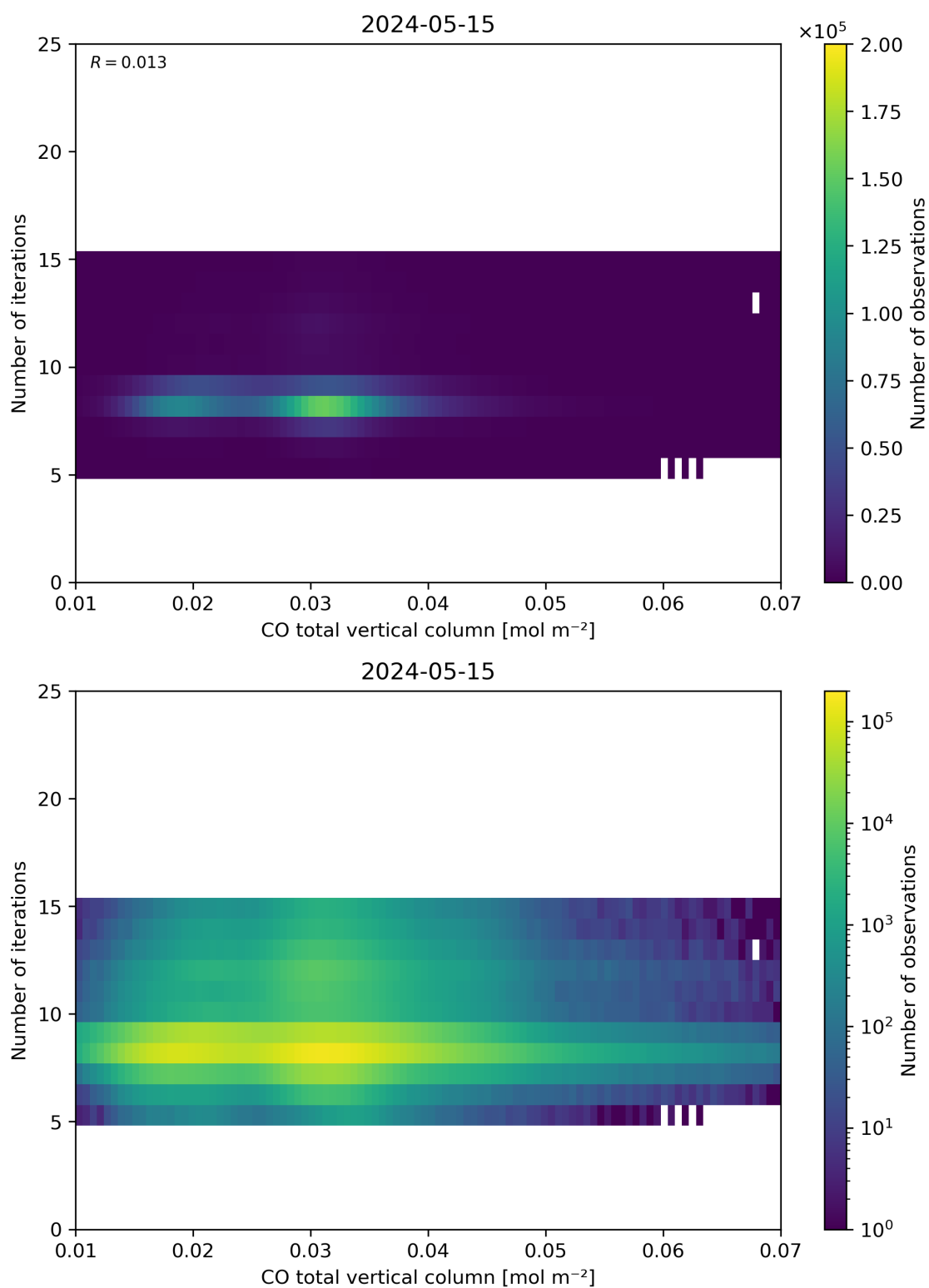
Figure 42: Scatter density plot of “CO total vertical column” against “Number of iterations” for 2024-05-14 to 2024-05-16.
