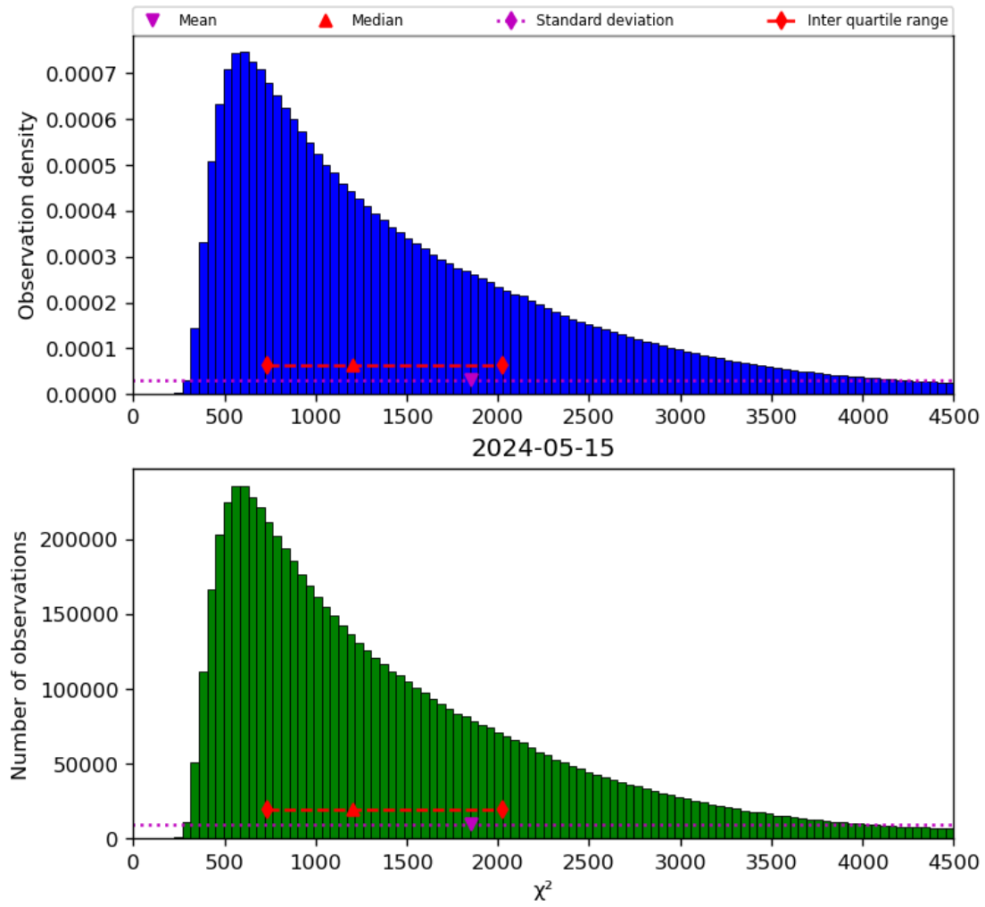
Figure 22: Histogram of “ \chi^2 ” for 2024-05-14 to 2024-05-16
