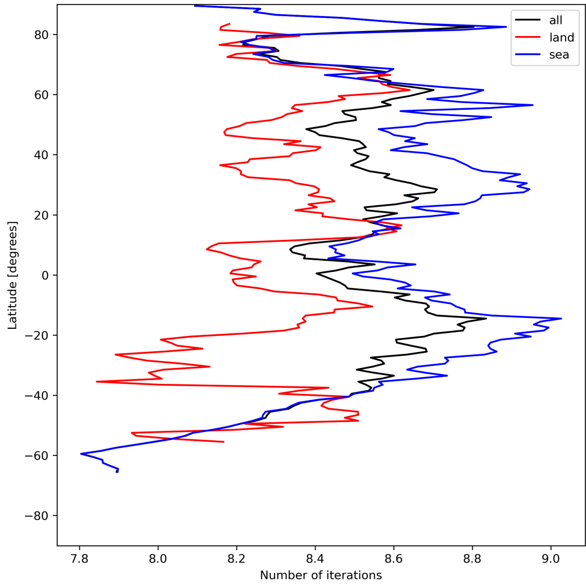
Figure 16: Zonal average of “Number of iterations” for 2024-05-14 to 2024-05-16.
