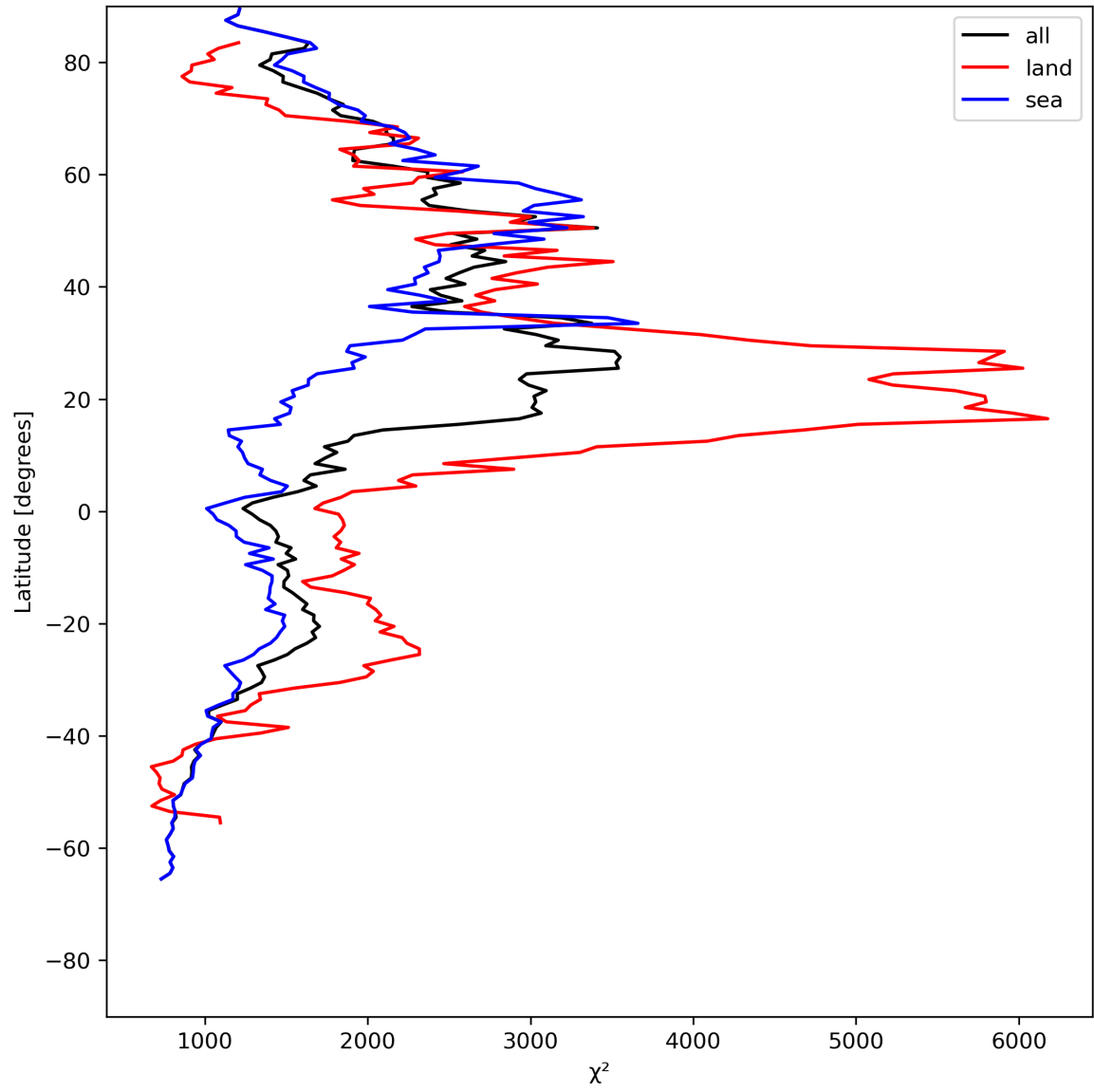
Figure 14: Zonal average of “ \chi^2 ” for 2024-05-14 to 2024-05-16.
