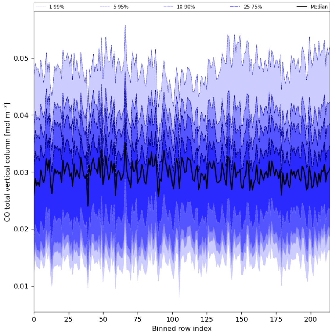
Figure 26: Along track statistics of “CO total vertical column” for 2024-05-14 to 2024-05-16
