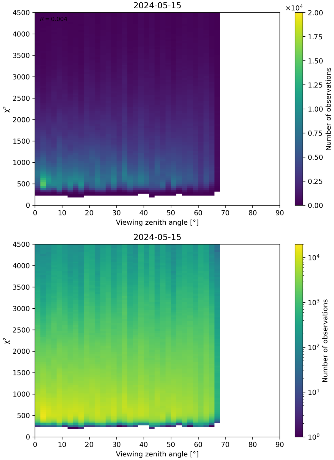
Figure 72: Scatter density plot of “Viewing zenith angle” against “ \chi^2 ” for 2024-05-14 to 2024-05-16.
