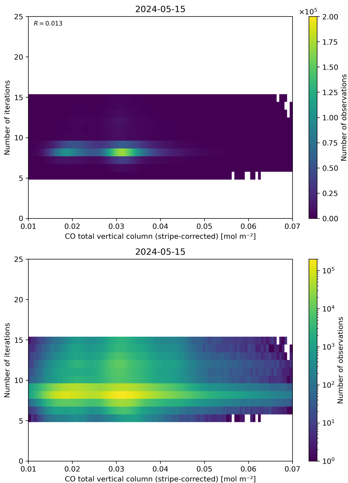
Figure 39: Scatter density plot of “CO total vertical column (stripe-corrected)” against “Number of iterations” for 2024-05-14 to 2024-05-16.
