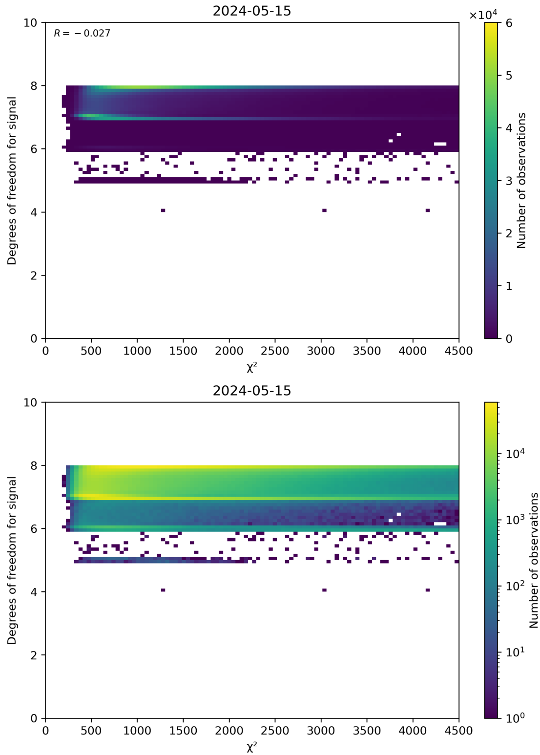
Figure 48: Scatter density plot of “ \chi^2 ” against “Degrees of freedom for signal” for 2024-05-14 to 2024-05-16.
