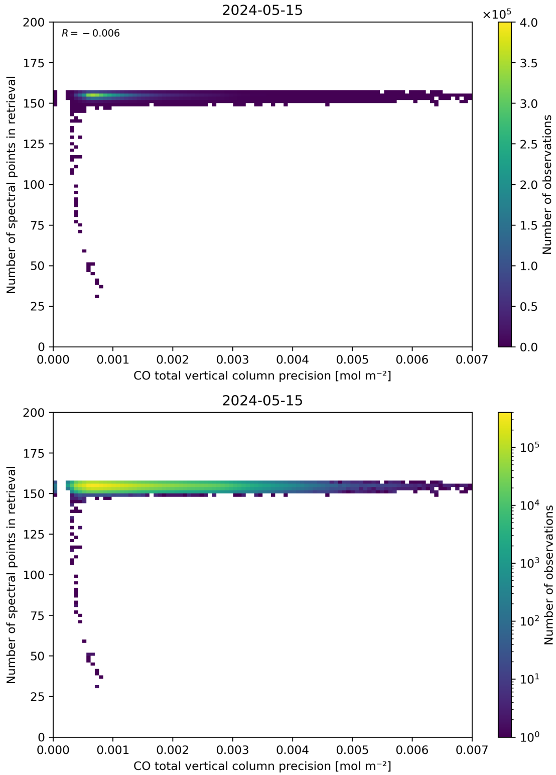
Figure 47: Scatter density plot of “CO total vertical column precision” against “Number of spectral points in retrieval” for 2024-05-14 to 2024-05-16.
