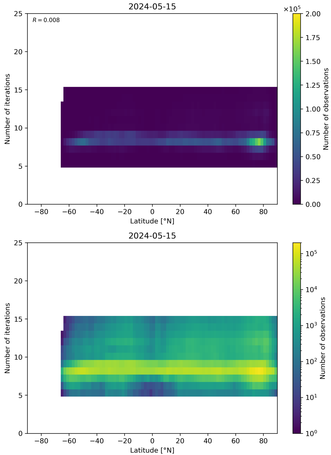
Figure 56: Scatter density plot of “Latitude” against “Number of iterations” for 2024-05-14 to 2024-05-16.
