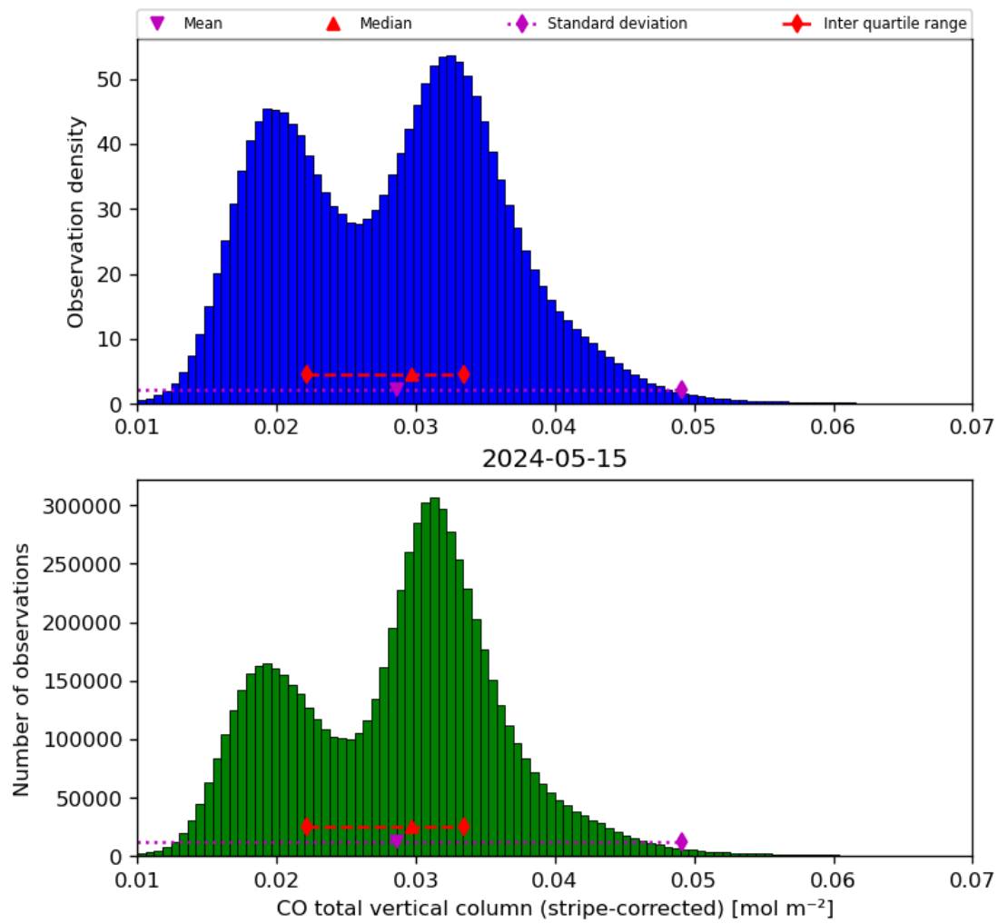
Figure 19: Histogram of “CO total vertical column (stripe-corrected)” for 2024-05-14 to 2024-05-16
