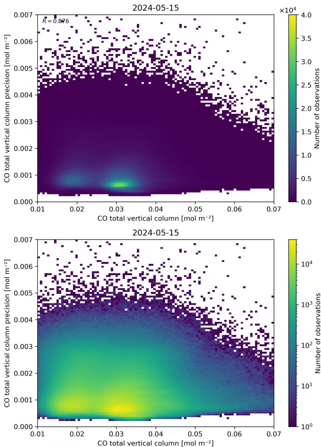
Figure 34: Scatter density plot of “CO total vertical column” against “CO total vertical column precision” for 2024-05-14 to 2024-05-16.
