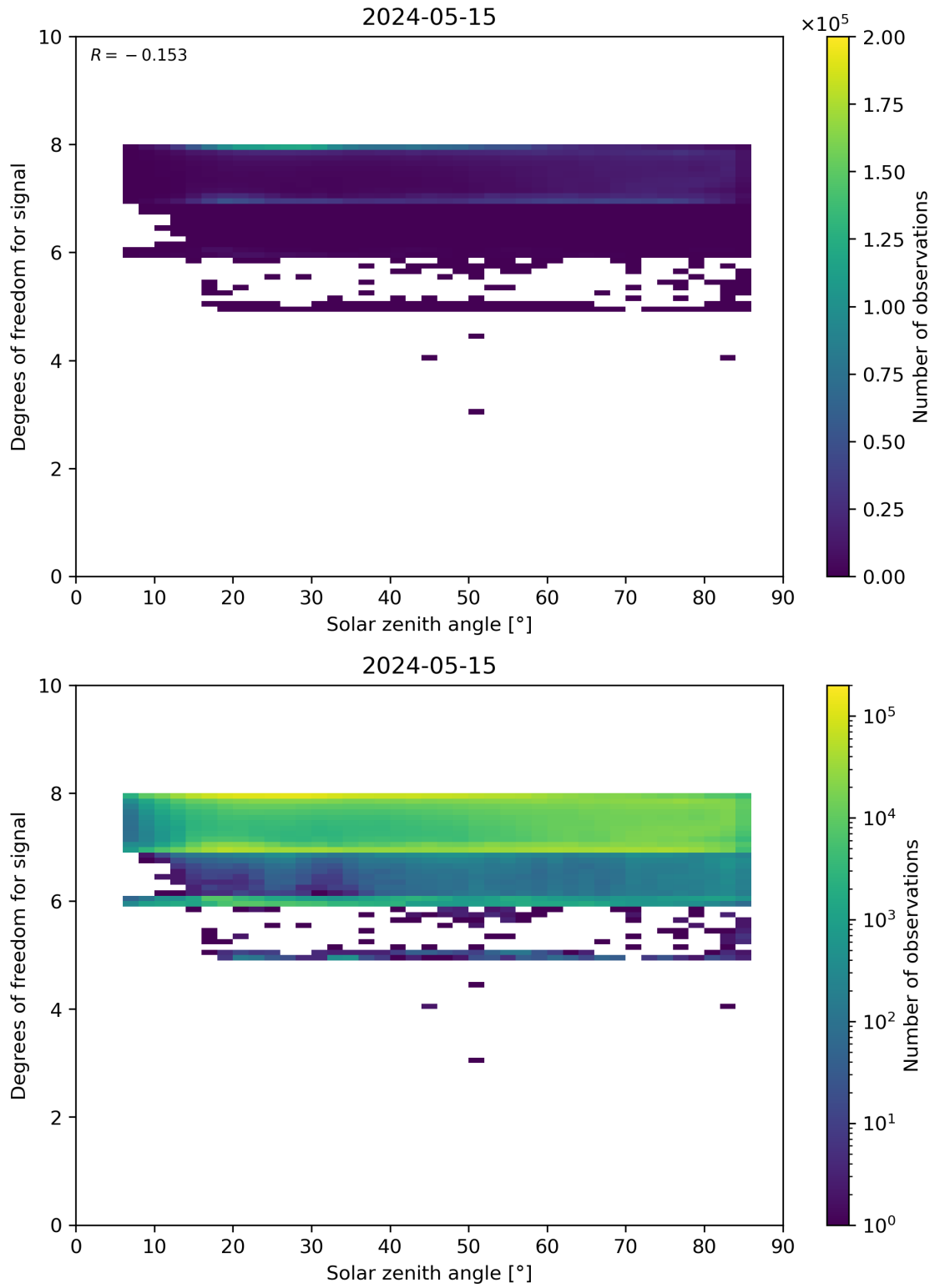
Figure 65: Scatter density plot of “Solar zenith angle” against “Degrees of freedom for signal” for 2024-05-14 to 2024-05-16.
