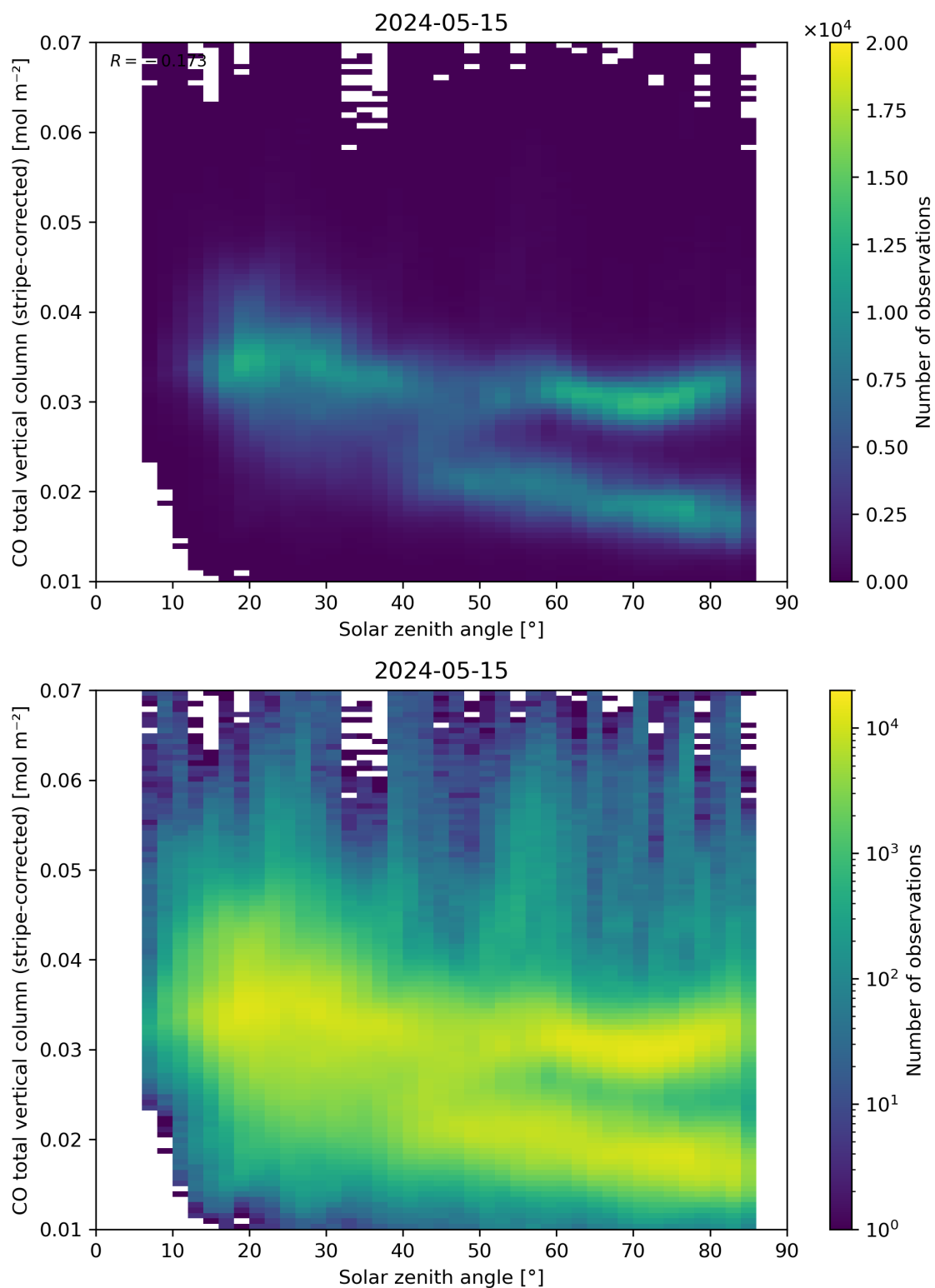
Figure 62: Scatter density plot of “Solar zenith angle” against “CO total vertical column (stripe-corrected)” for 2024-05-14 to 2024-05-16.
