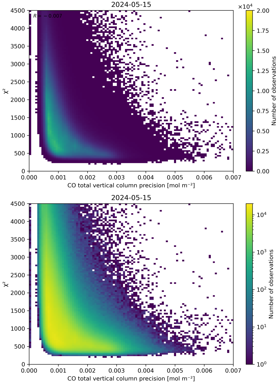
Figure 44: Scatter density plot of “CO total vertical column precision” against “ \chi^2 ” for 2024-05-14 to 2024-05-16.
