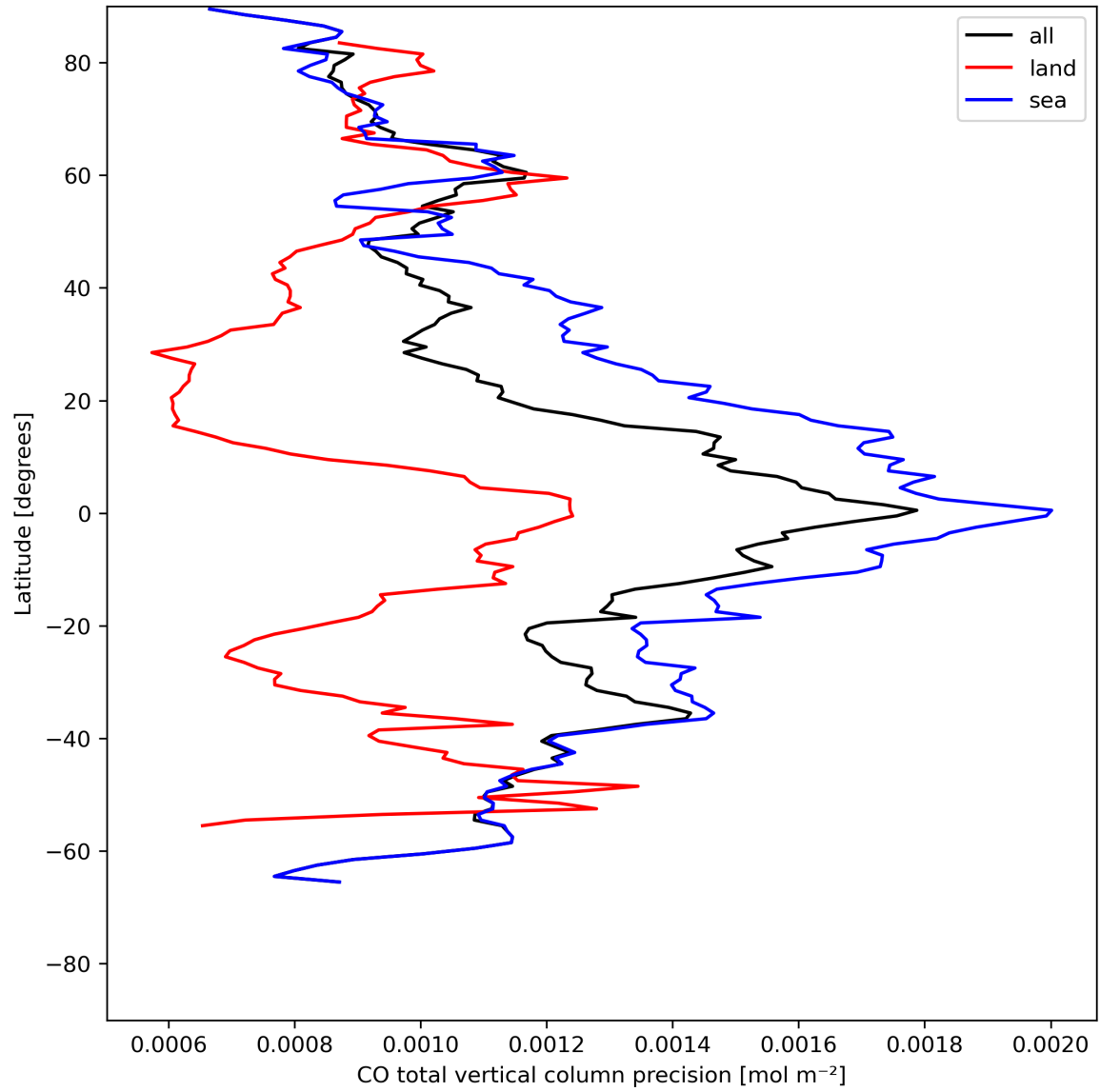
Figure 12: Zonal average of “CO total vertical column precision” for 2024-05-14 to 2024-05-16.
