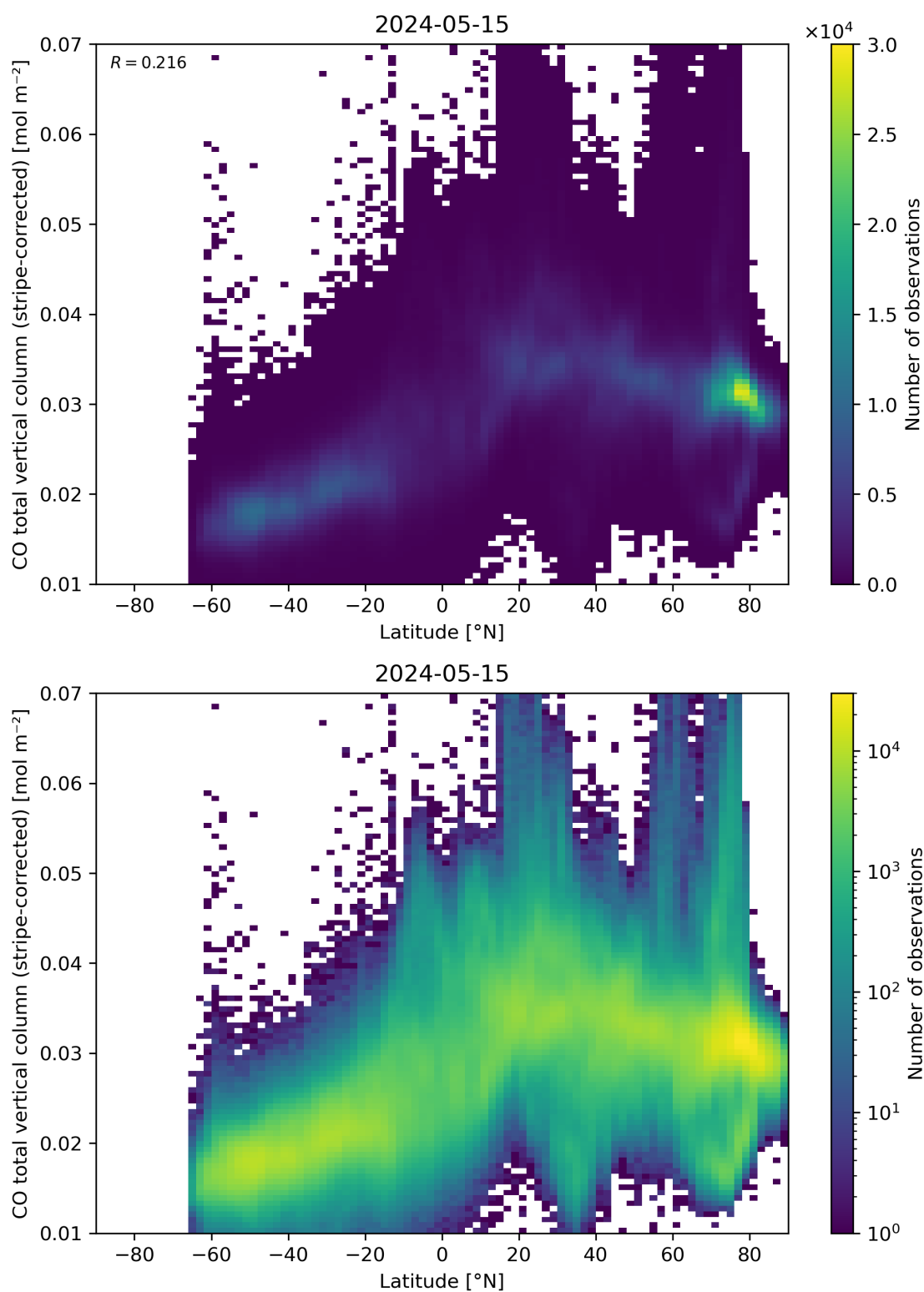
Figure 52: Scatter density plot of “Latitude” against “CO total vertical column (stripe-corrected)” for 2024-05-14 to 2024-05-16.
