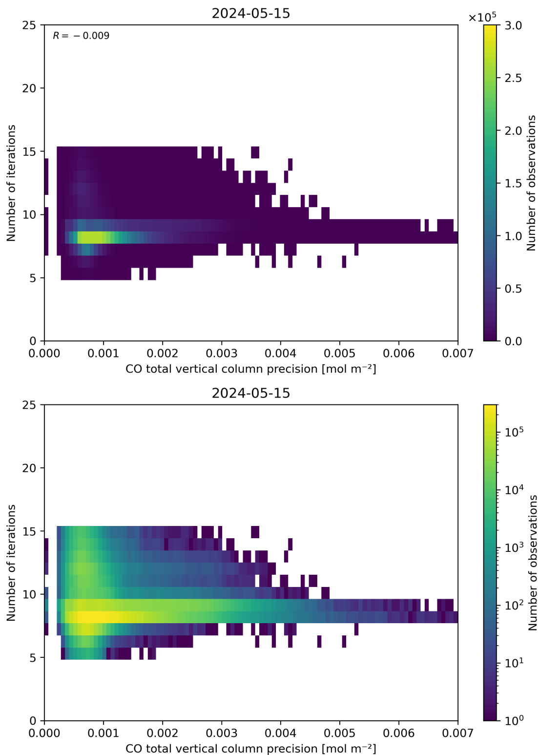
Figure 46: Scatter density plot of “CO total vertical column precision” against “Number of iterations” for 2024-05-14 to 2024-05-16.
