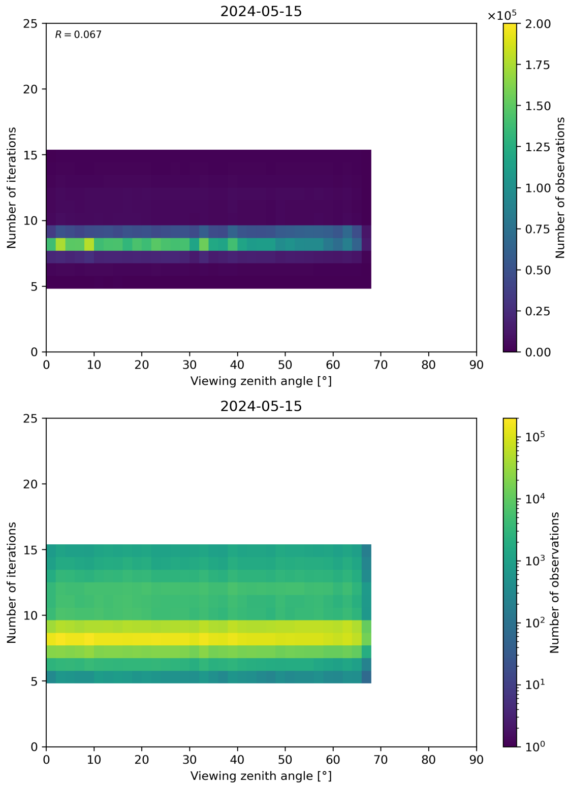
Figure 75: Scatter density plot of “Viewing zenith angle” against “Number of iterations” for 2024-05-14 to 2024-05-16.
