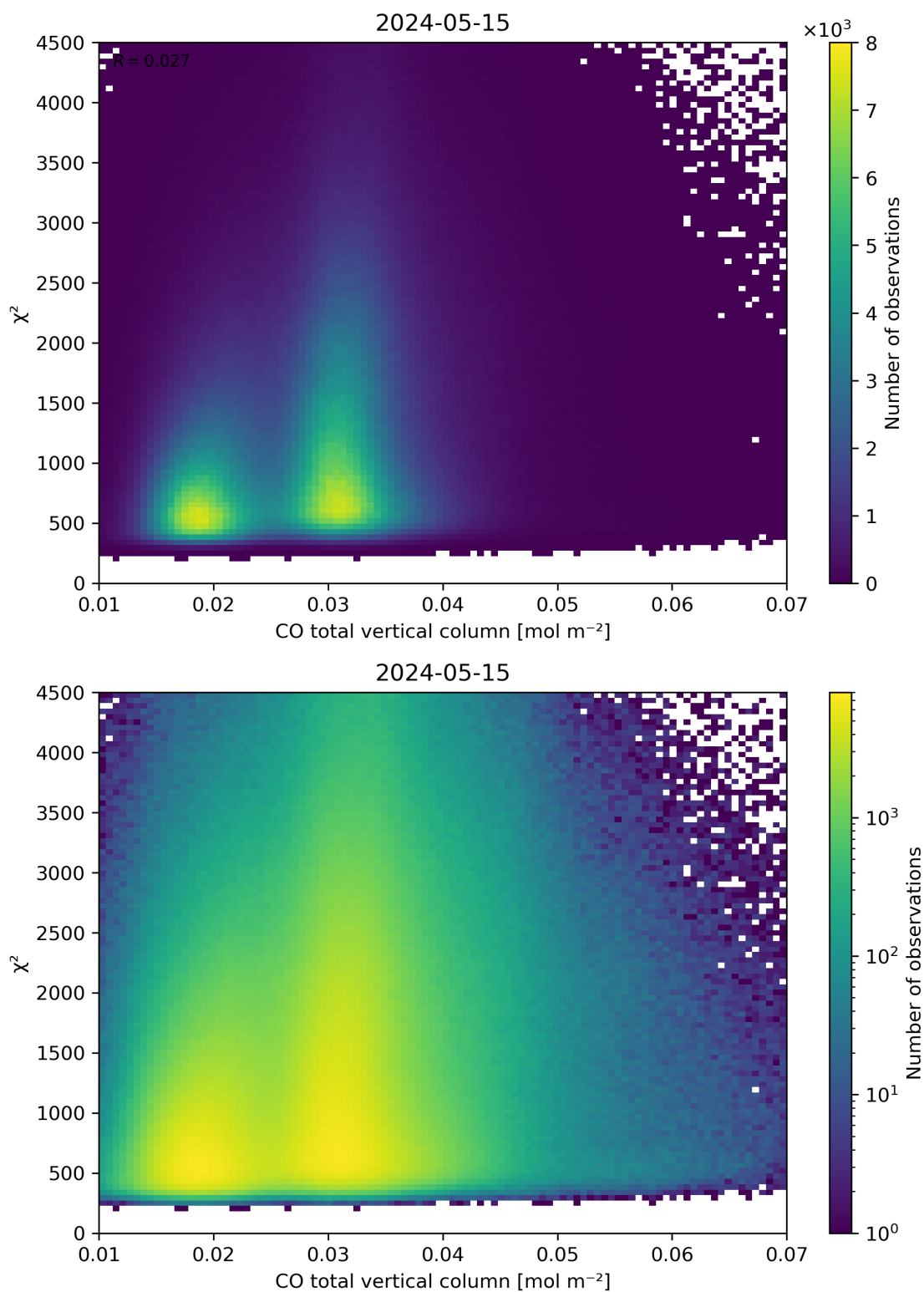
Figure 35: Scatter density plot of “CO total vertical column” against “ \chi^2 ” for 2024-05-14 to 2024-05-16.
