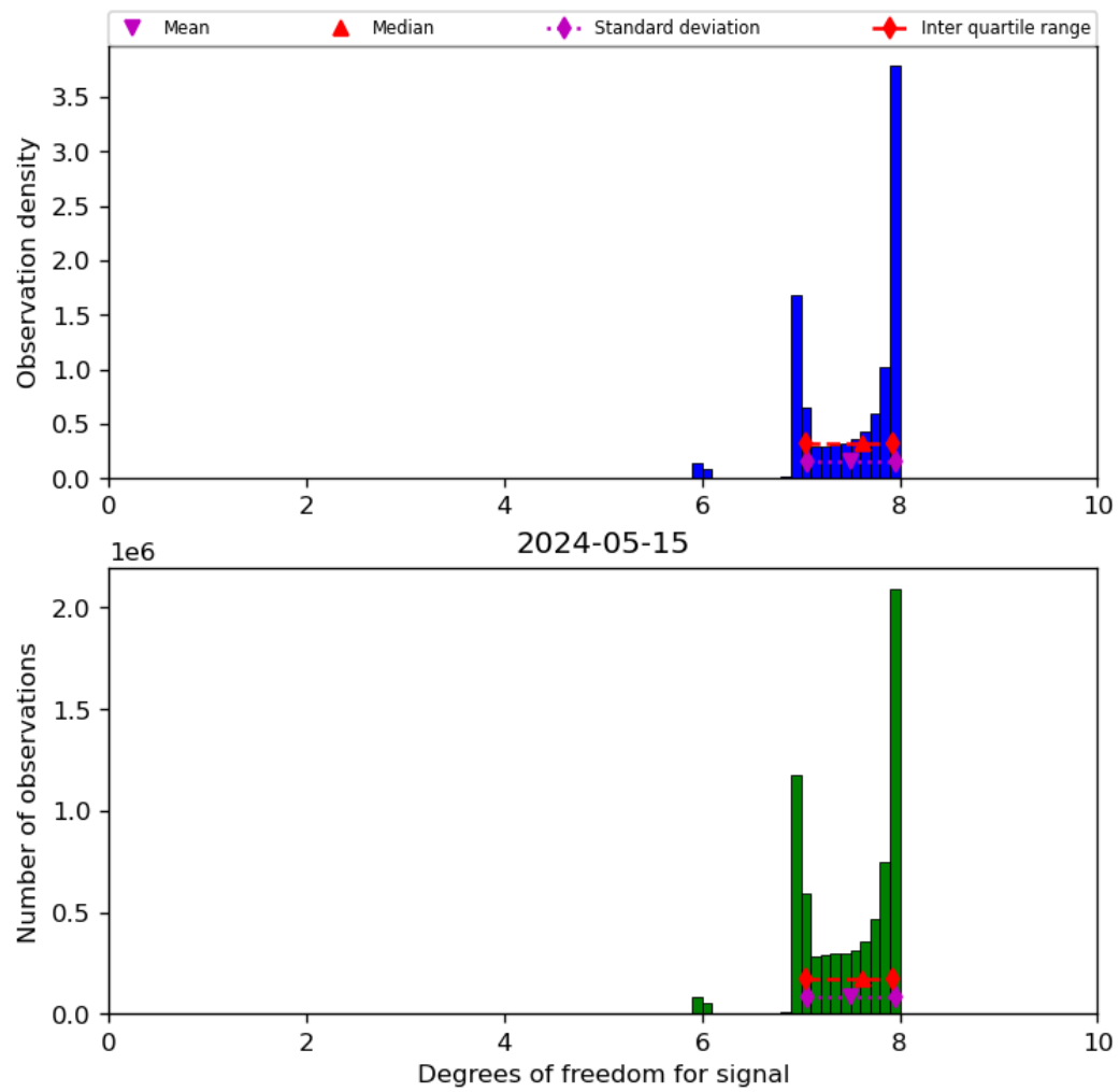
Figure 23: Histogram of “Degrees of freedom for signal” for 2024-05-14 to 2024-05-16
