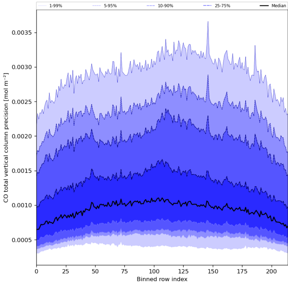
Figure 28: Along track statistics of “CO total vertical column precision” for 2024-05-14 to 2024-05-16
