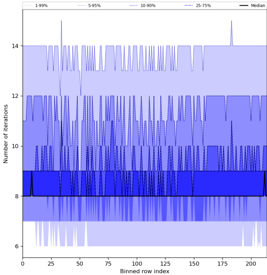
Figure 32: Along track statistics of “Number of iterations” for 2024-05-14 to 2024-05-16
