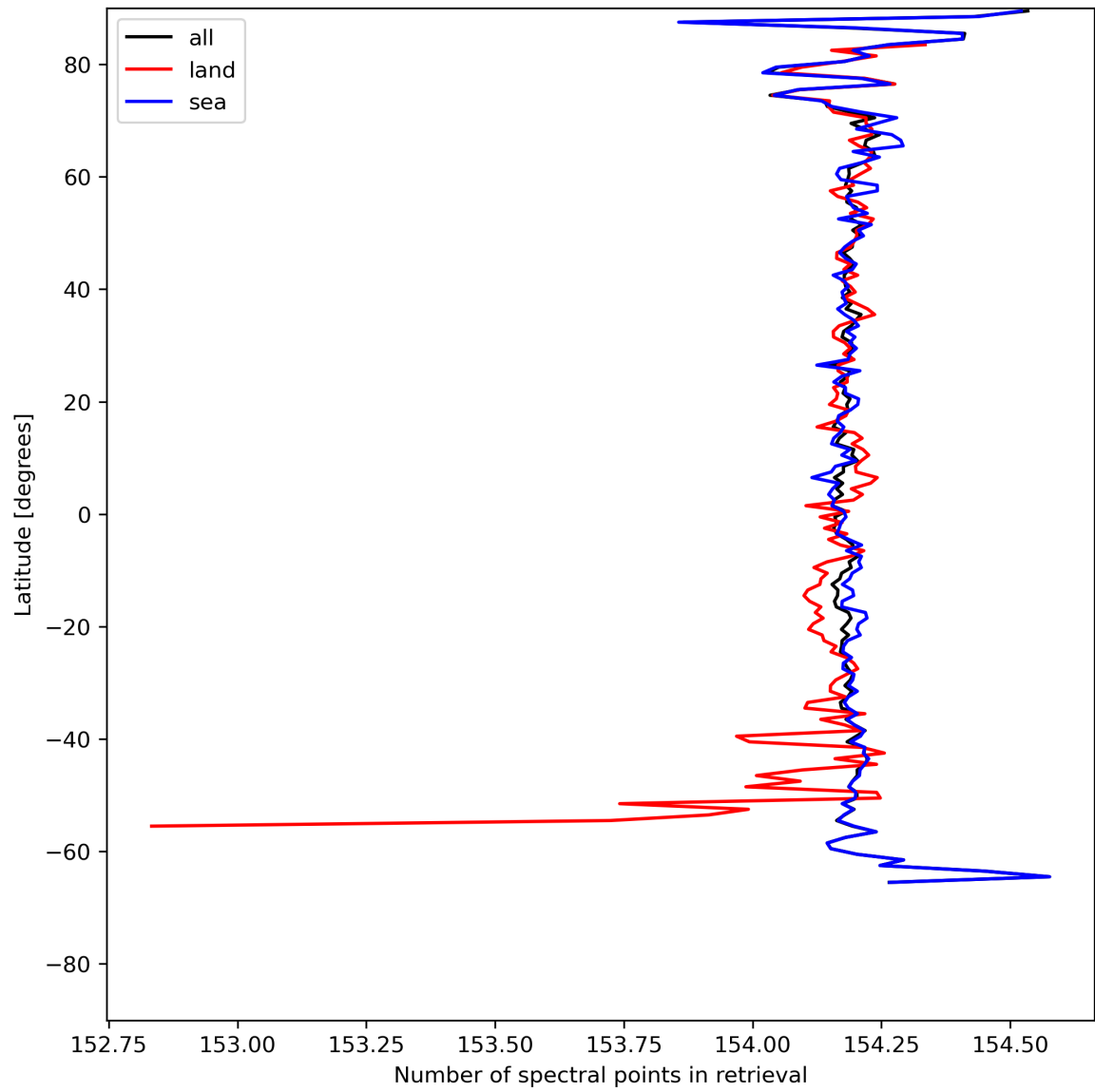
Figure 13: Zonal average of “Number of spectral points in retrieval” for 2024-05-14 to 2024-05-16.
