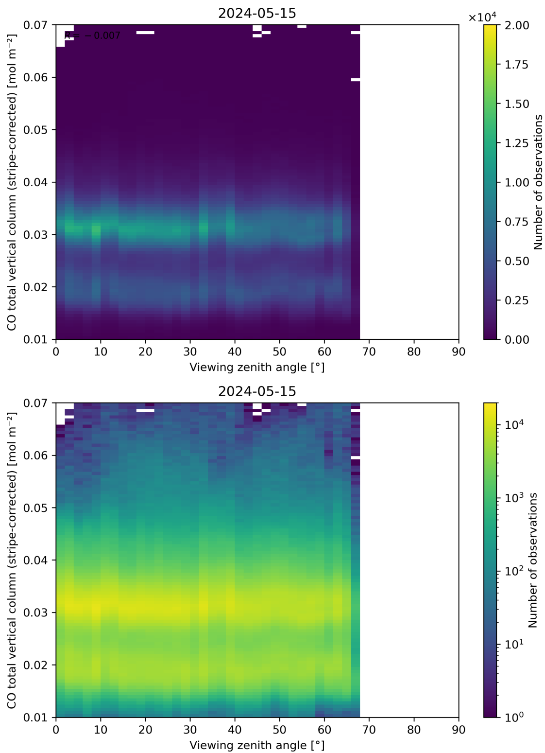
Figure 70: Scatter density plot of “Viewing zenith angle” against “CO total vertical column (stripe-corrected)” for 2024-05-14 to 2024-05-16.
