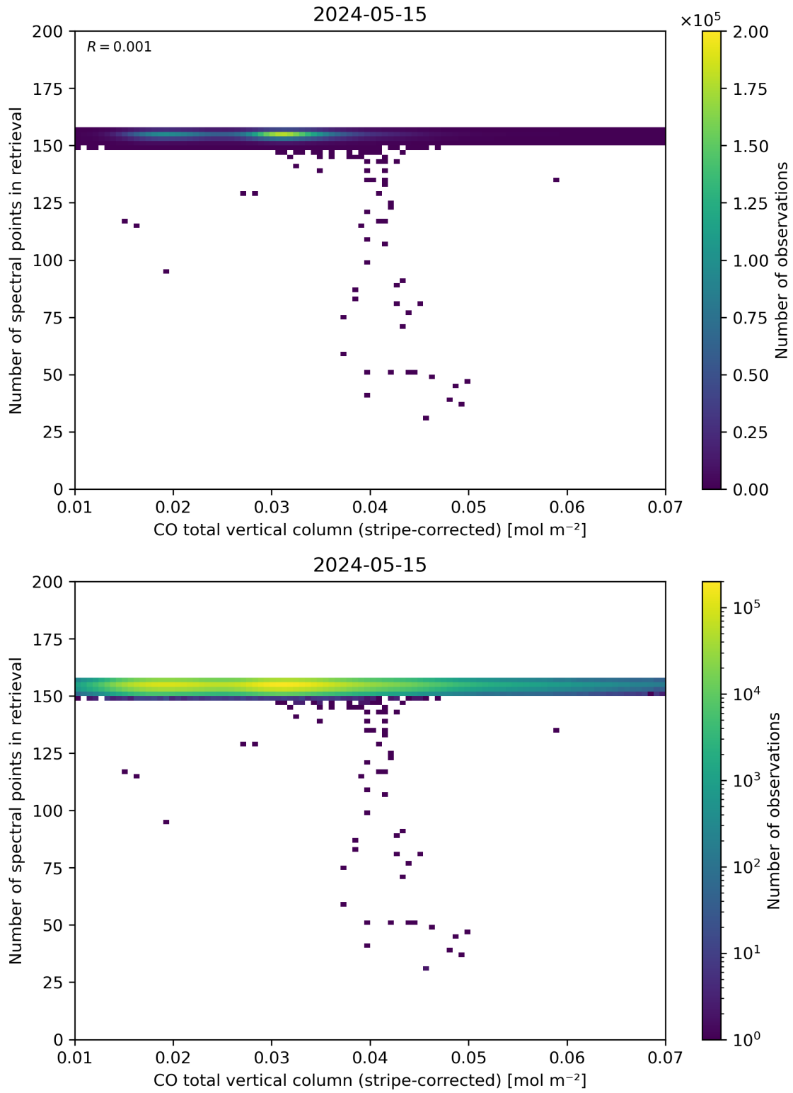
Figure 40: Scatter density plot of “CO total vertical column (stripe-corrected)” against “Number of spectral points in retrieval” for 2024-05-14 to 2024-05-16.
