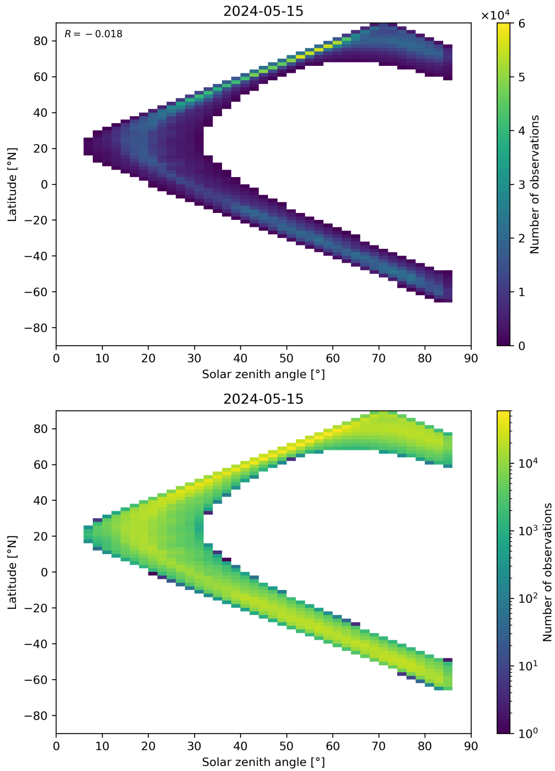
Figure 66: Scatter density plot of “Solar zenith angle” against “Latitude” for 2024-05-14 to 2024-05-16.
