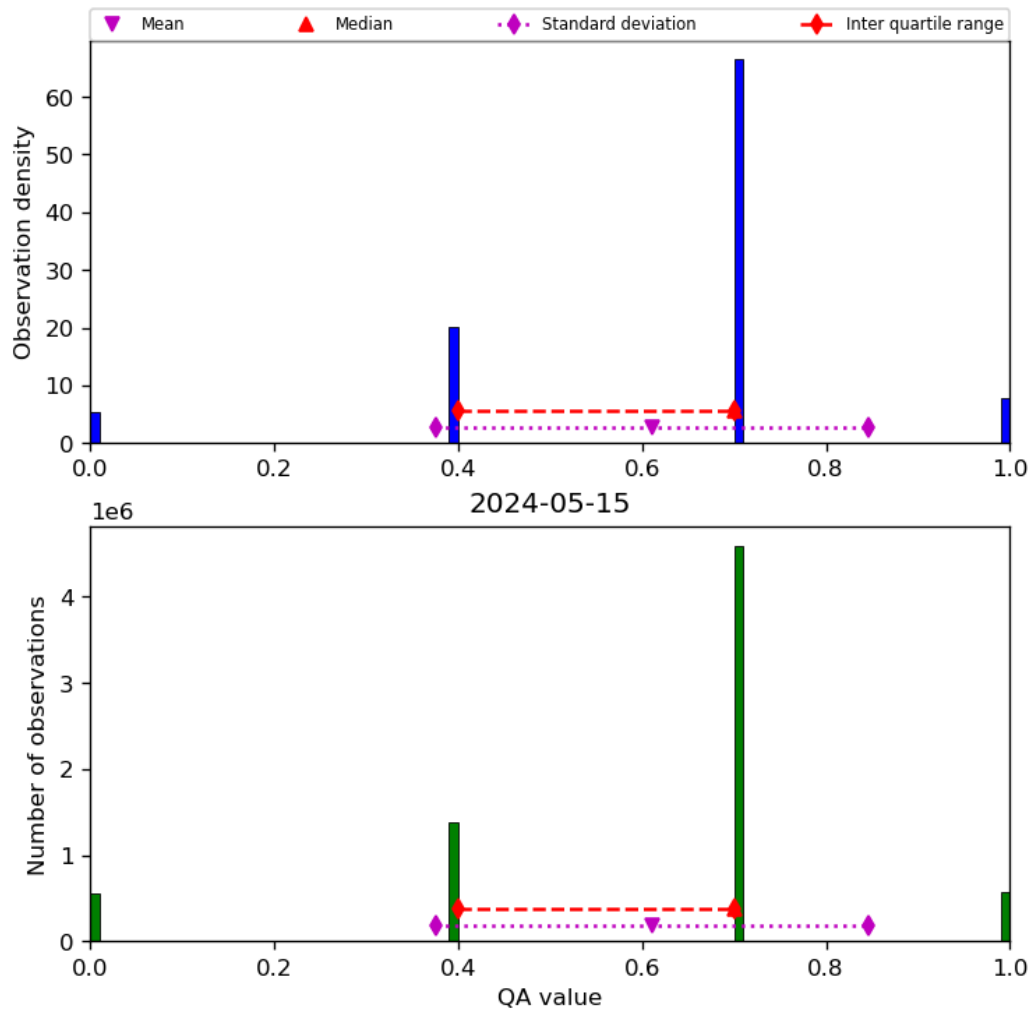
Figure 17: Histogram of “QA value” for 2024-05-14 to 2024-05-16
