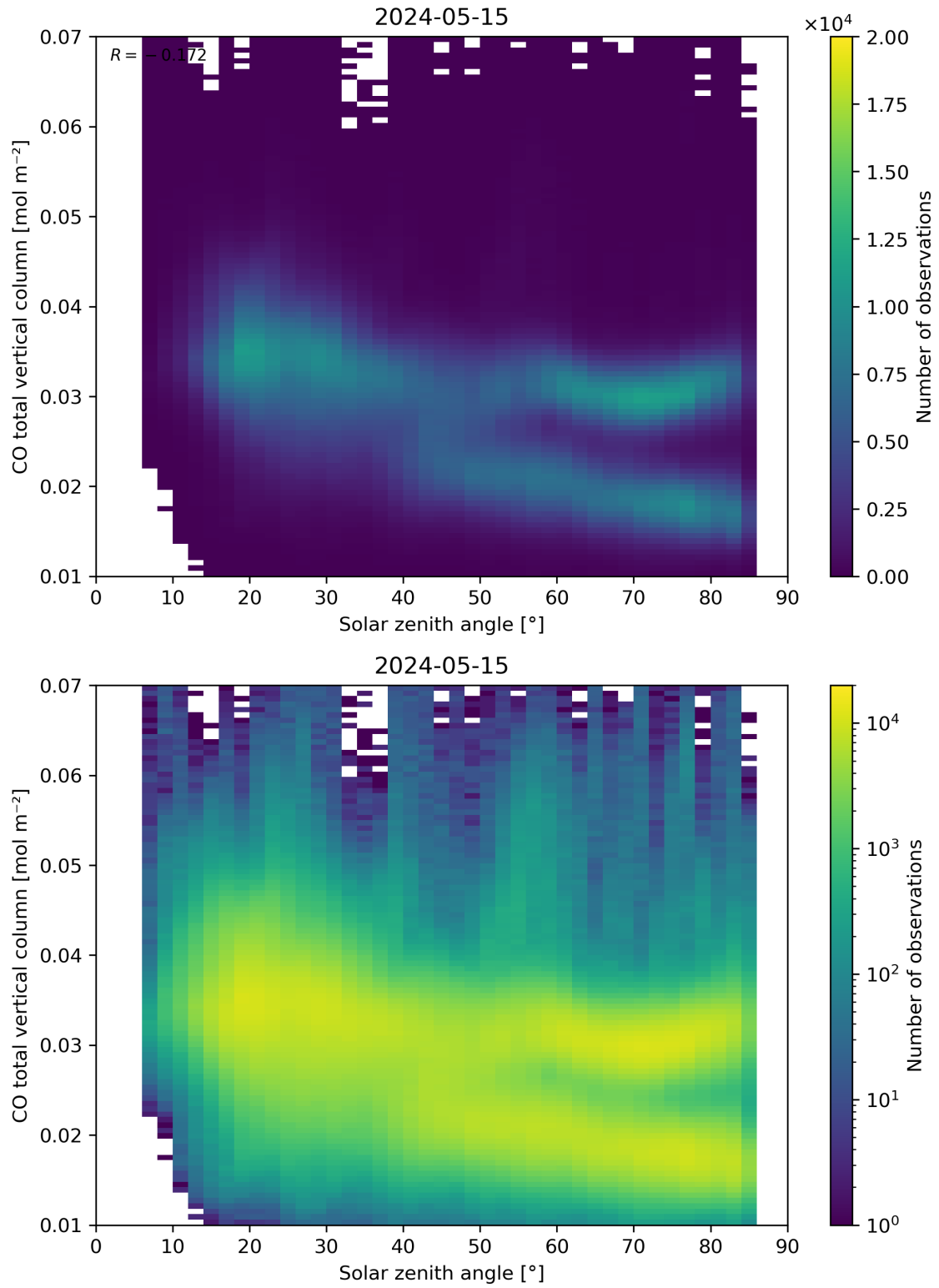
Figure 61: Scatter density plot of “Solar zenith angle” against “CO total vertical column” for 2024-05-14 to 2024-05-16.
