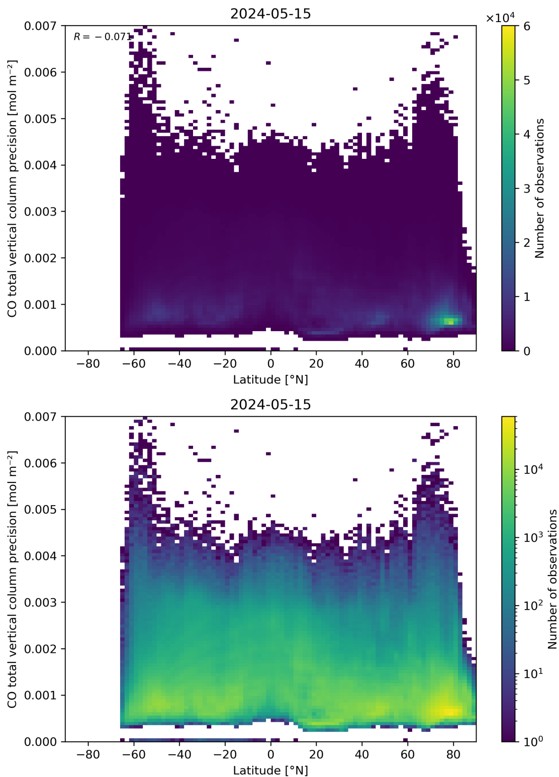
Figure 53: Scatter density plot of “Latitude” against “CO total vertical column precision” for 2024-05-14 to 2024-05-16.
