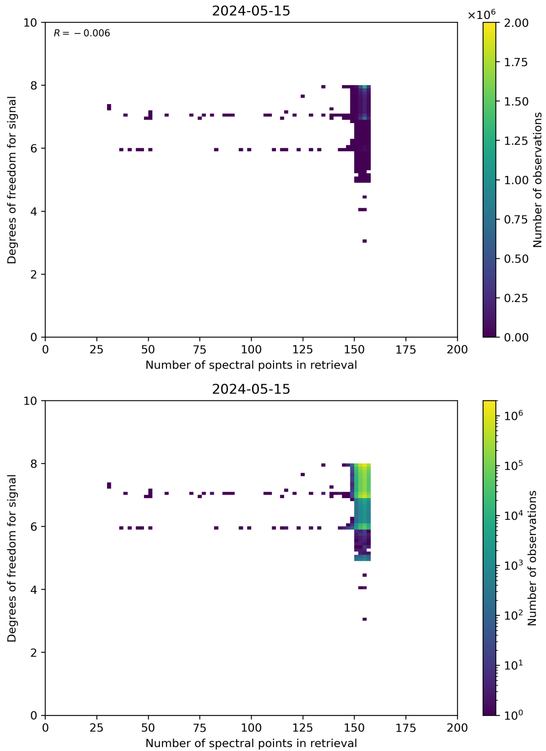
Figure 59: Scatter density plot of “Number of spectral points in retrieval” against “Degrees of freedom for signal” for 2024-05-14 to 2024-05-16.
