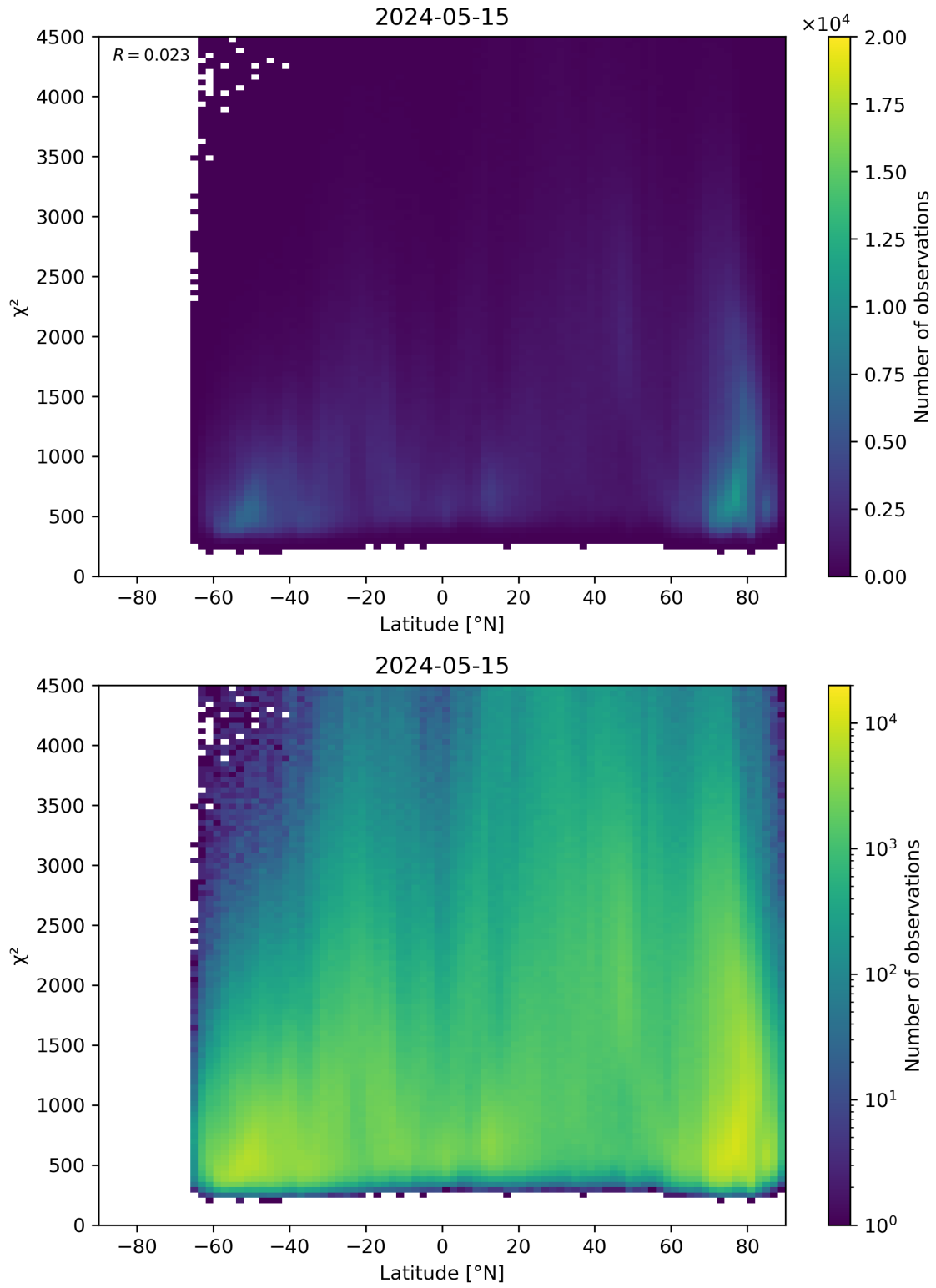
Figure 54: Scatter density plot of “Latitude” against “ \chi^2 ” for 2024-05-14 to 2024-05-16.
