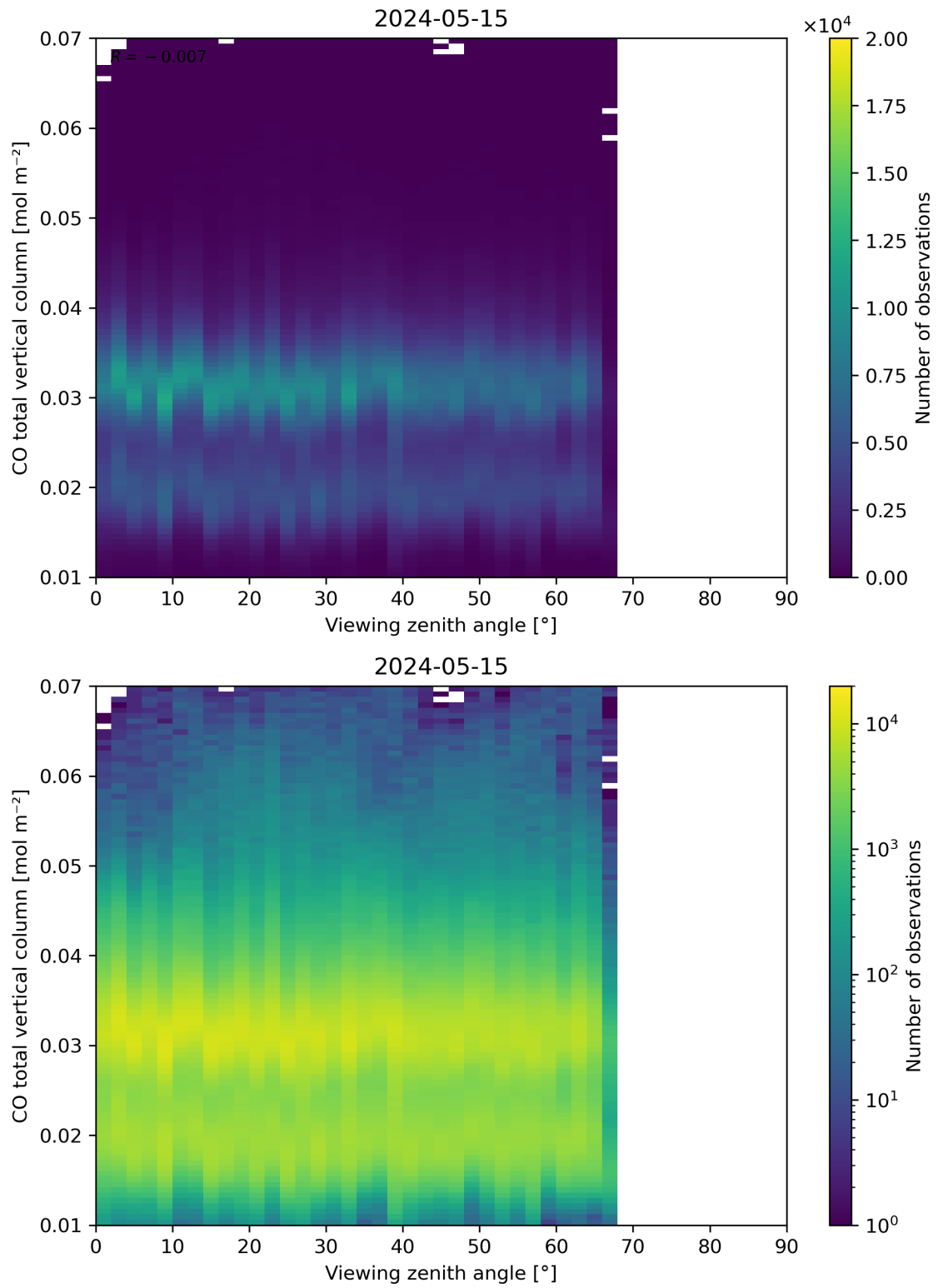
Figure 69: Scatter density plot of “Viewing zenith angle” against “CO total vertical column” for 2024-05-14 to 2024-05-16.
