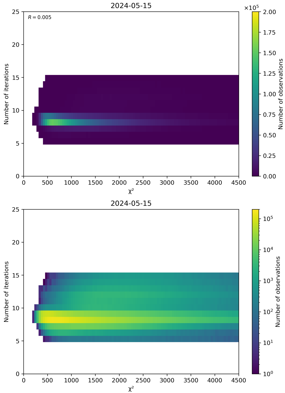
Figure 49: Scatter density plot of " \chi^2 " against "Number of iterations" for 2024-05-14 to 2024-05-16.
