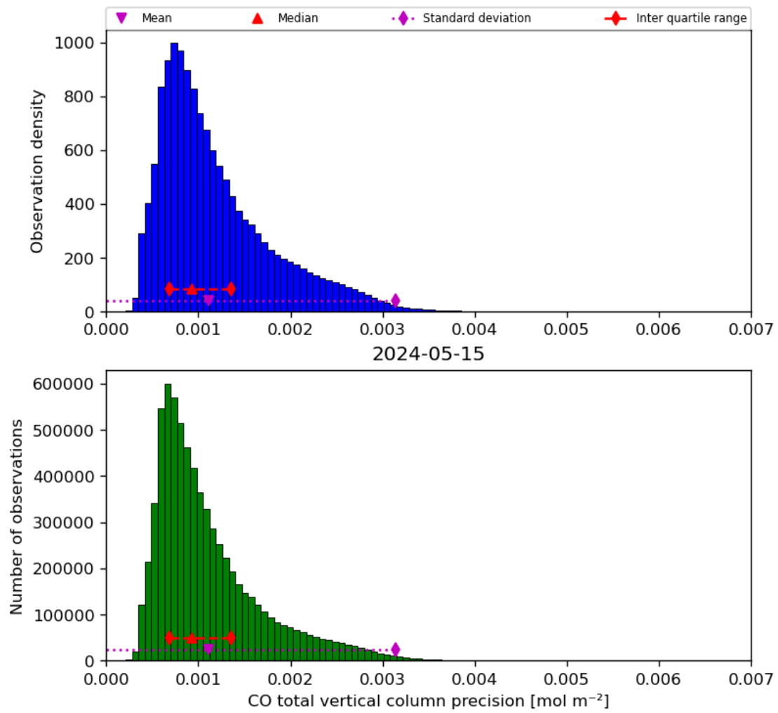
Figure 20: Histogram of “CO total vertical column precision” for 2024-05-14 to 2024-05-16
