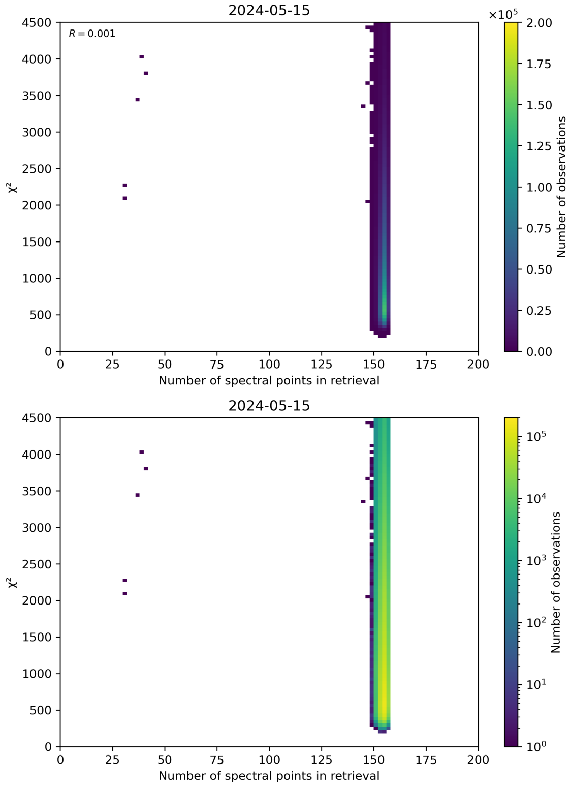
Figure 58: Scatter density plot of “Number of spectral points in retrieval” against “ \chi^2 ” for 2024-05-14 to 2024-05-16.
