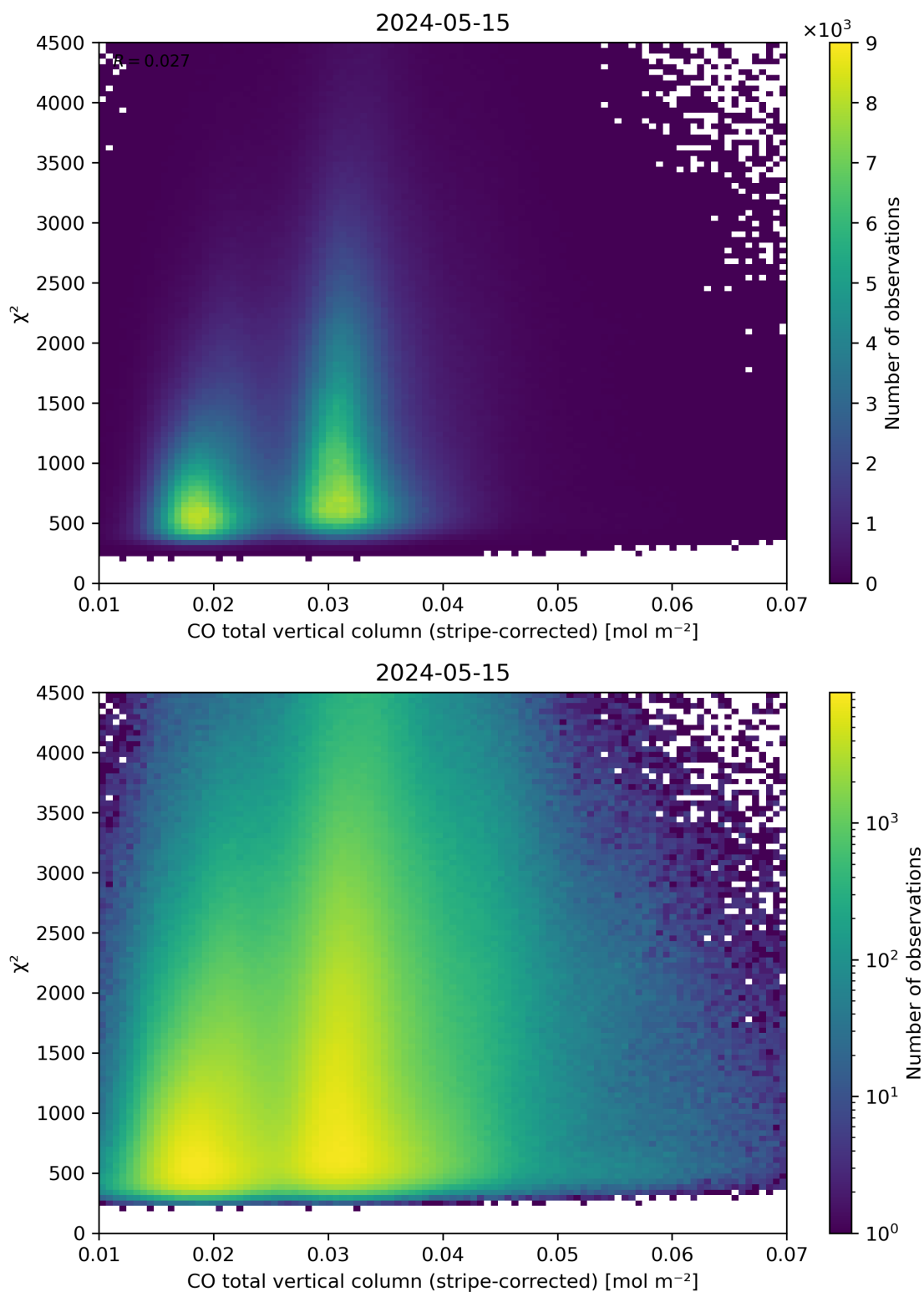
Figure 37: Scatter density plot of “CO total vertical column (stripe-corrected)” against “ \chi^2 ” for 2024-05-14 to 2024-05-16.
