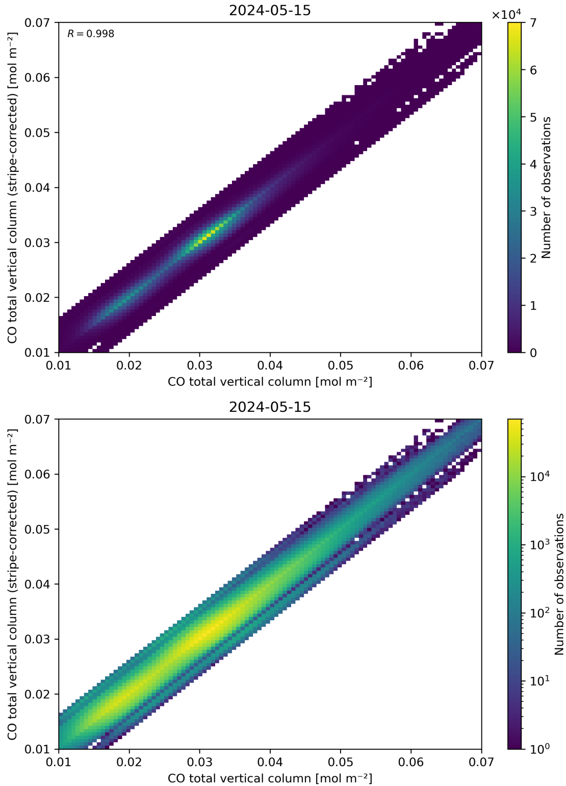
Figure 33: Scatter density plot of “CO total vertical column” against “CO total vertical column (stripe-corrected)” for 2024-05-14 to 2024-05-16.
