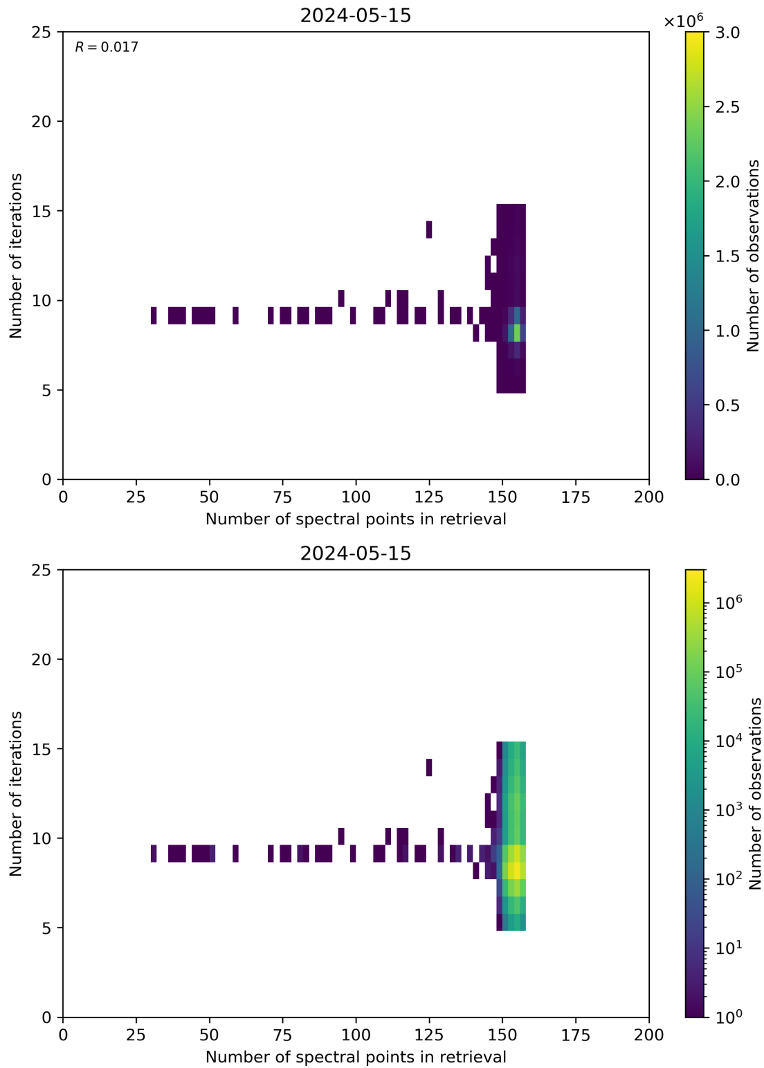
Figure 60: Scatter density plot of “Number of spectral points in retrieval” against “Number of iterations” for 2024-05-14 to 2024-05-16.
