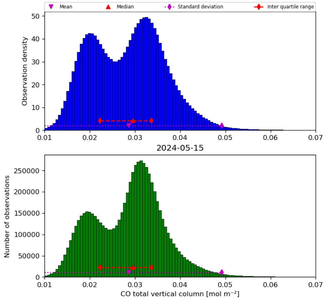
Figure 18: Histogram of “CO total vertical column” for 2024-05-14 to 2024-05-16
