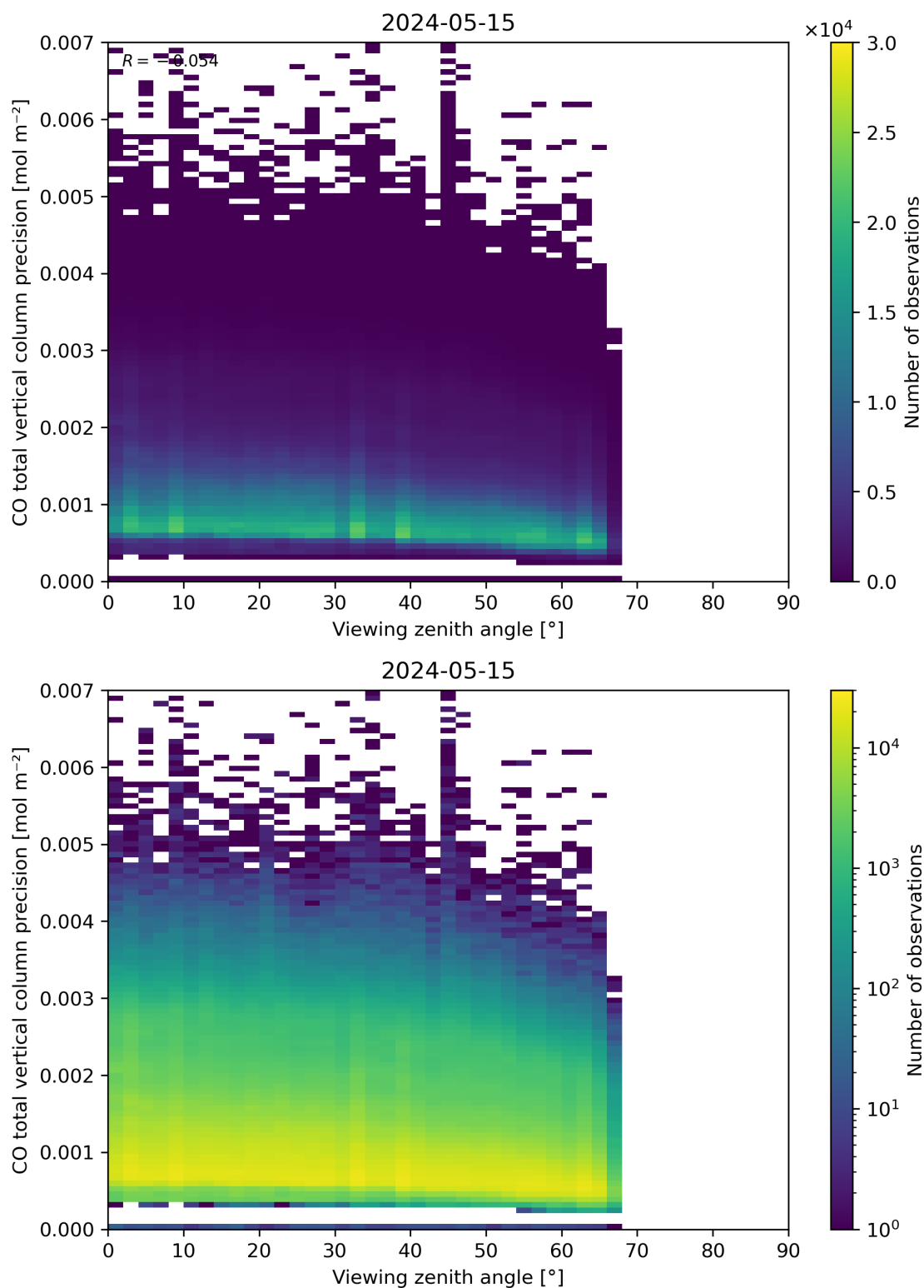
Figure 71: Scatter density plot of “Viewing zenith angle” against “CO total vertical column precision” for 2024-05-14 to 2024-05-16.
