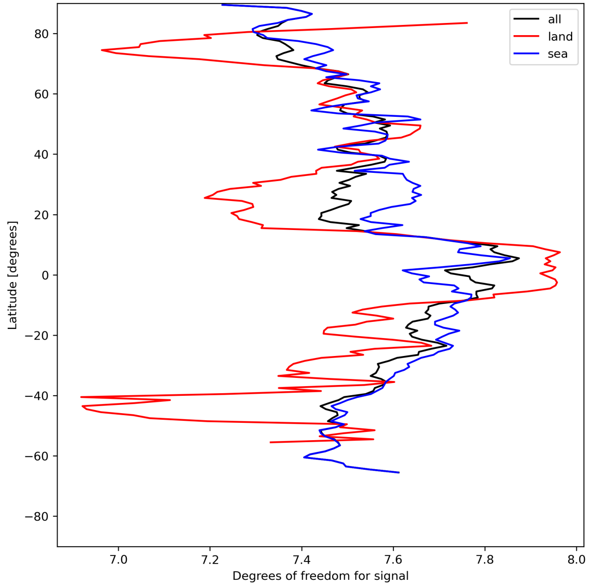
Figure 15: Zonal average of “Degrees of freedom for signal” for 2024-05-14 to 2024-05-16.
