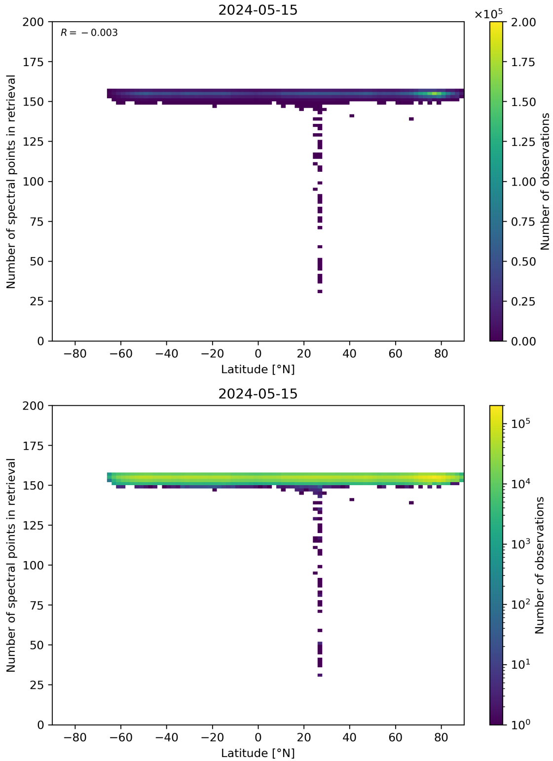
Figure 57: Scatter density plot of “Latitude” against “Number of spectral points in retrieval” for 2024-05-14 to 2024-05-16.
