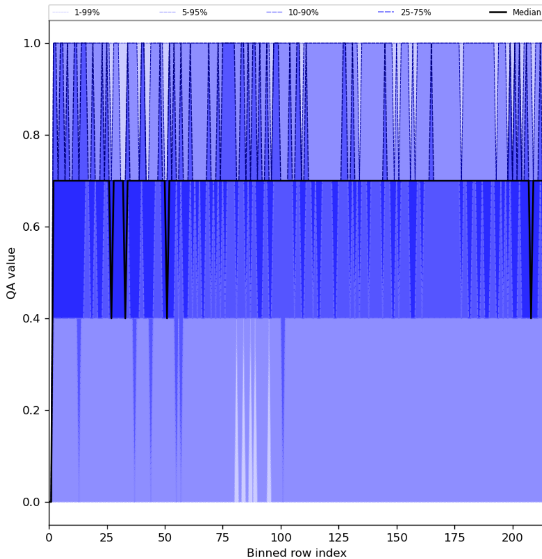
Figure 25: Along track statistics of “QA value” for 2024-05-14 to 2024-05-16
