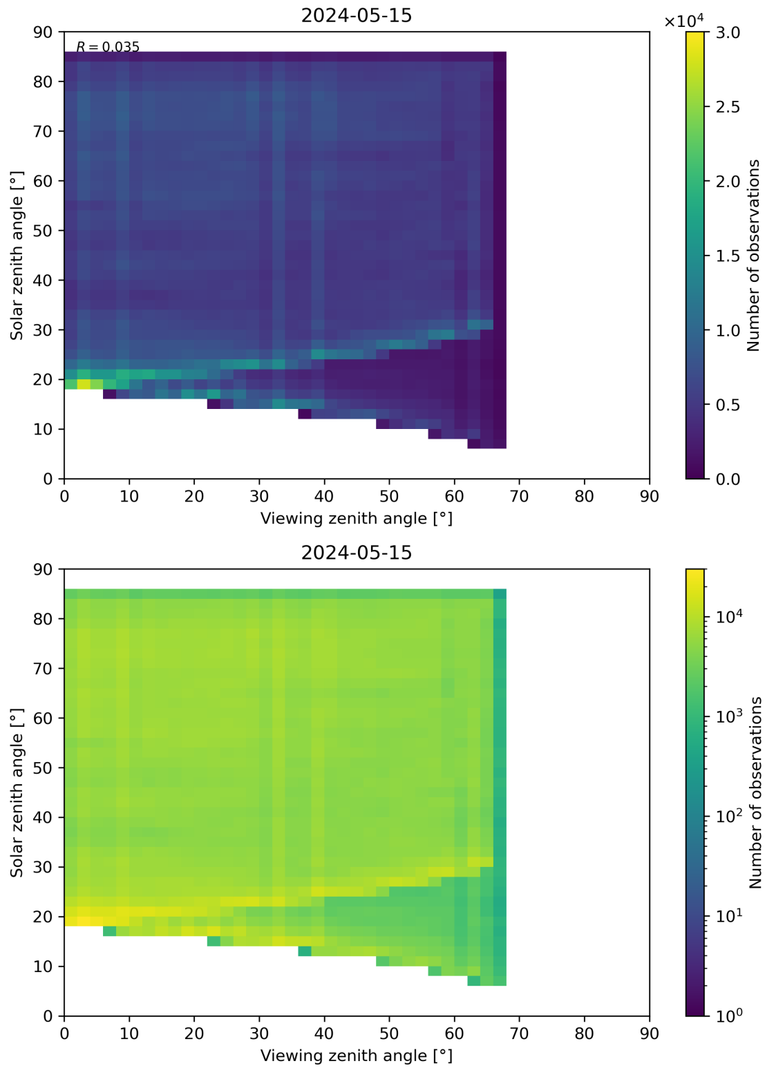
Figure 77: Scatter density plot of “Viewing zenith angle” against “Solar zenith angle” for 2024-05-14 to 2024-05-16.
