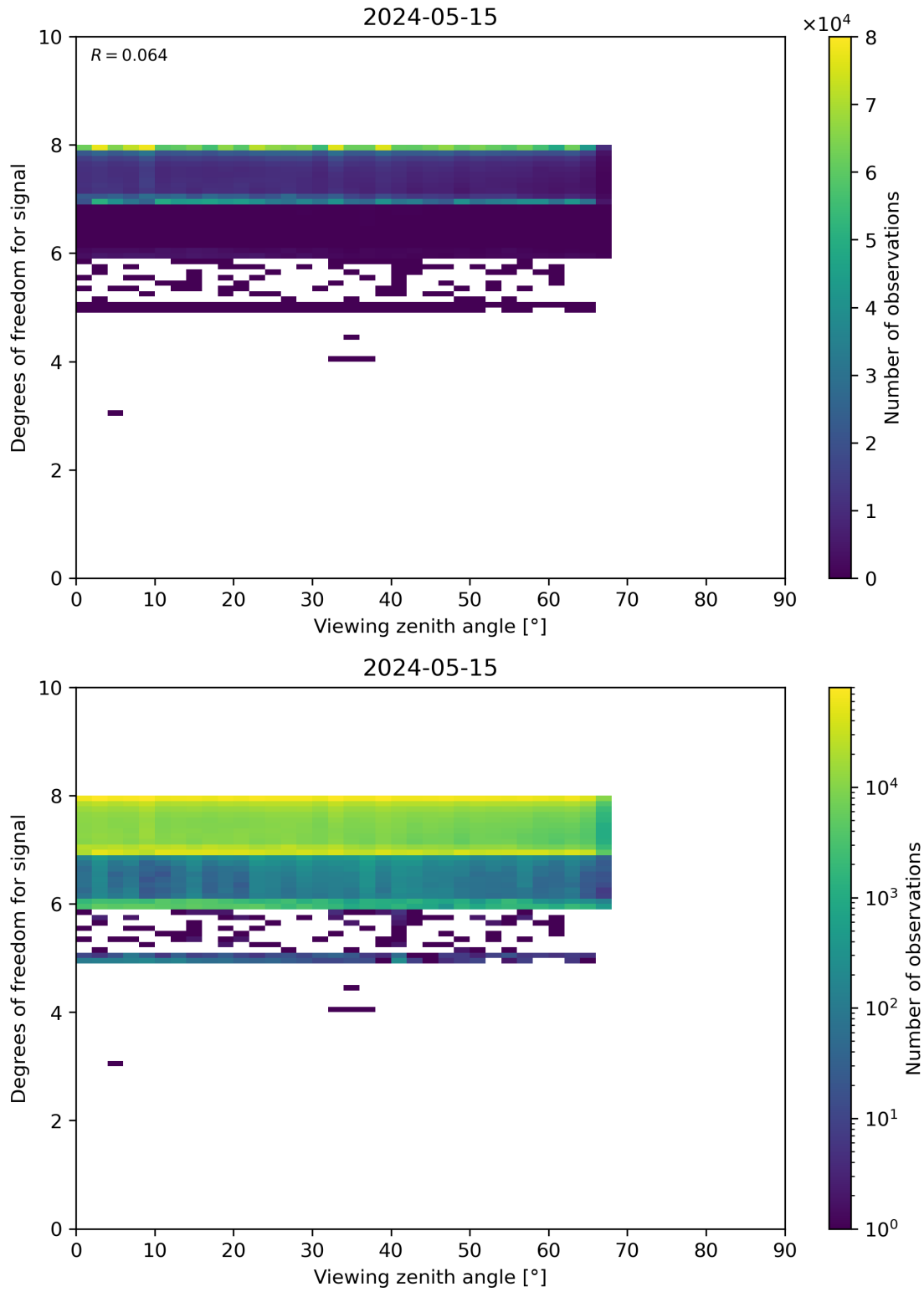
Figure 73: Scatter density plot of “Viewing zenith angle” against “Degrees of freedom for signal” for 2024-05-14 to 2024-05-16.
