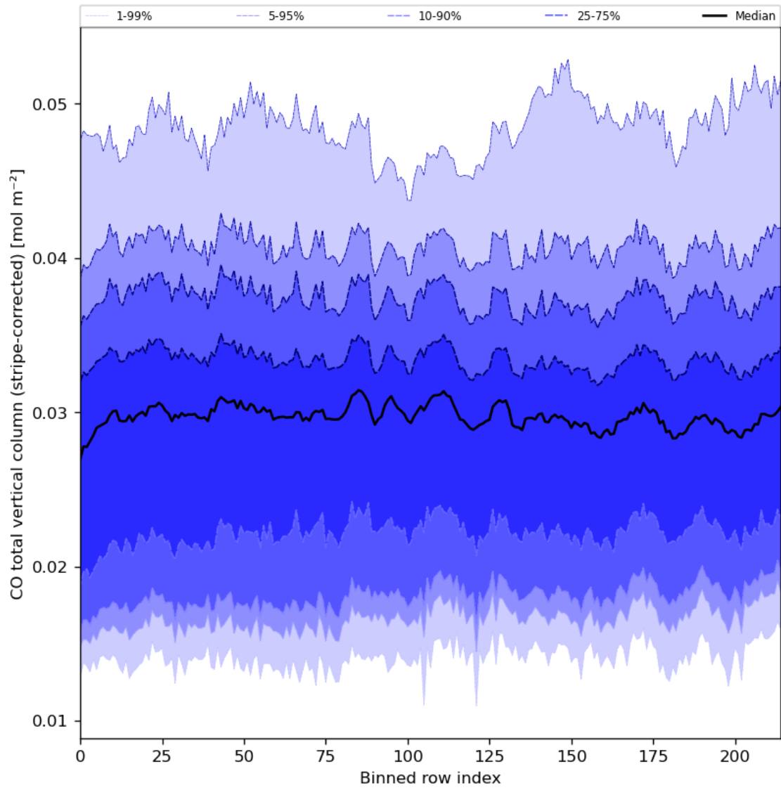
Figure 27: Along track statistics of “CO total vertical column (stripe-corrected)” for 2024-05-14 to 2024-05-16
