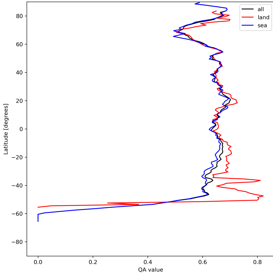
Figure 9: Zonal average of “QA value” for 2024-05-15 to 2024-05-17.
