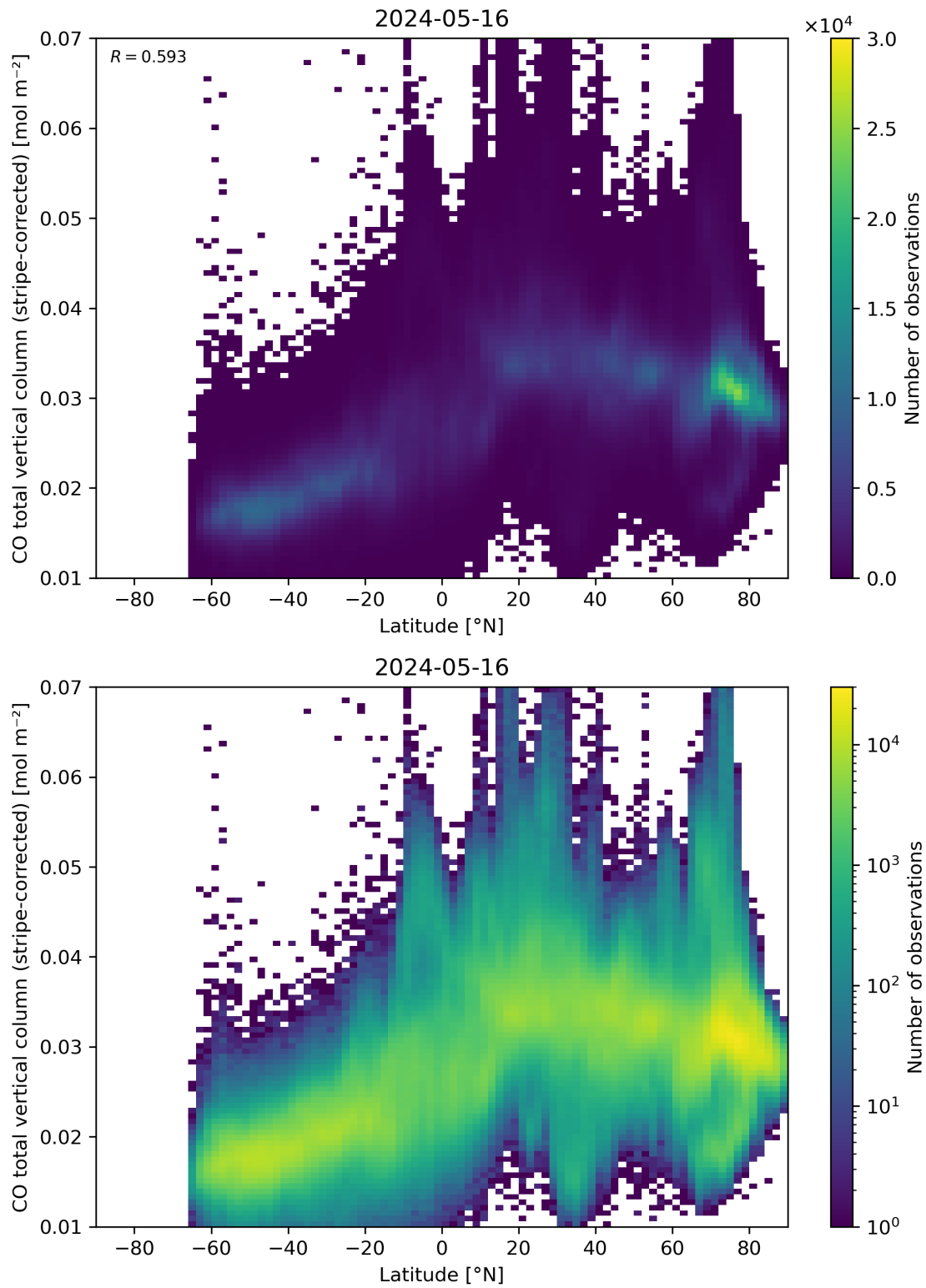
Figure 52: Scatter density plot of “Latitude” against “CO total vertical column (stripe-corrected)” for 2024-05-15 to 2024-05-17.
