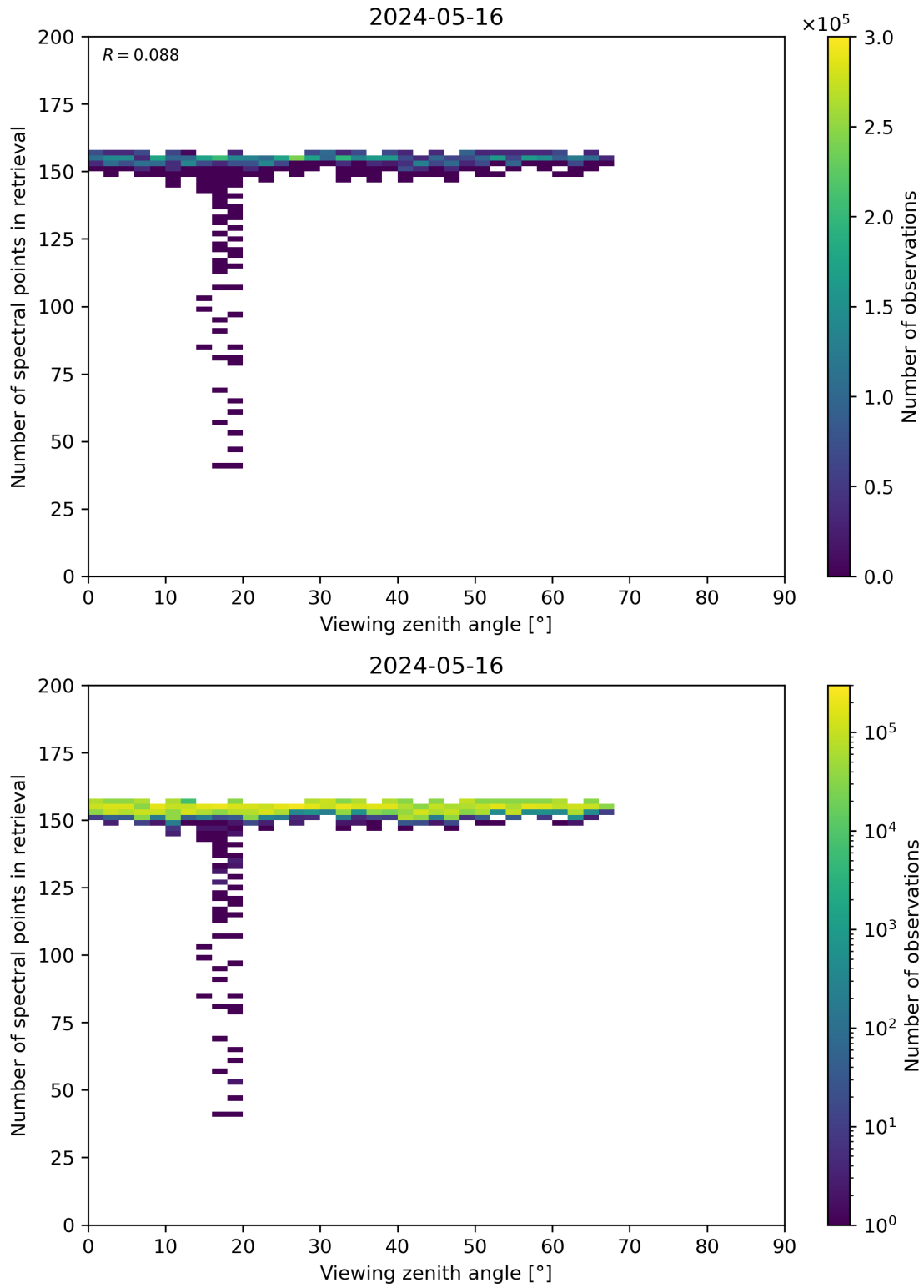
Figure 76: Scatter density plot of “Viewing zenith angle” against “Number of spectral points in retrieval” for 2024-05-15 to 2024-05-17.
