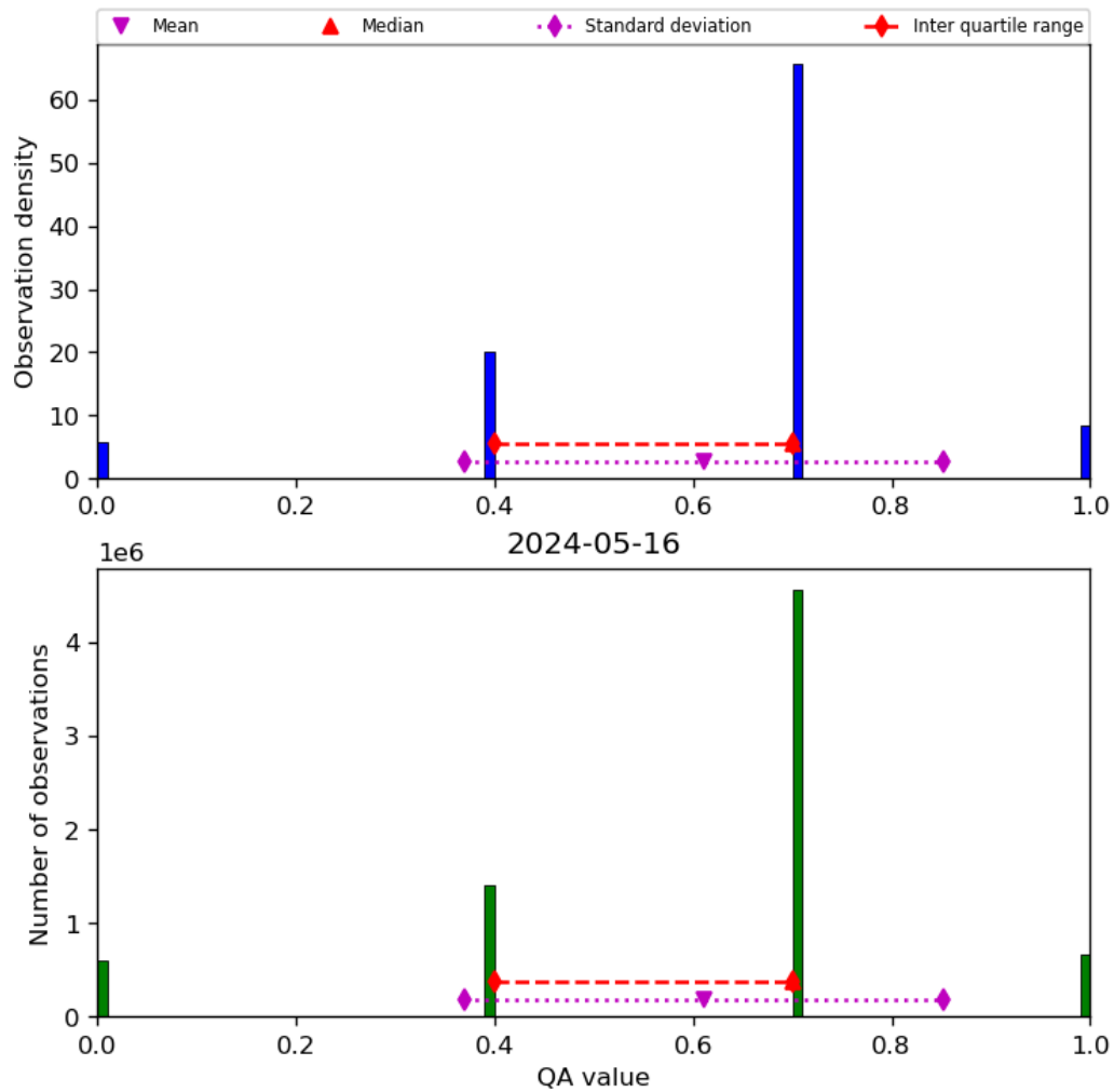
Figure 17: Histogram of “QA value” for 2024-05-15 to 2024-05-17
