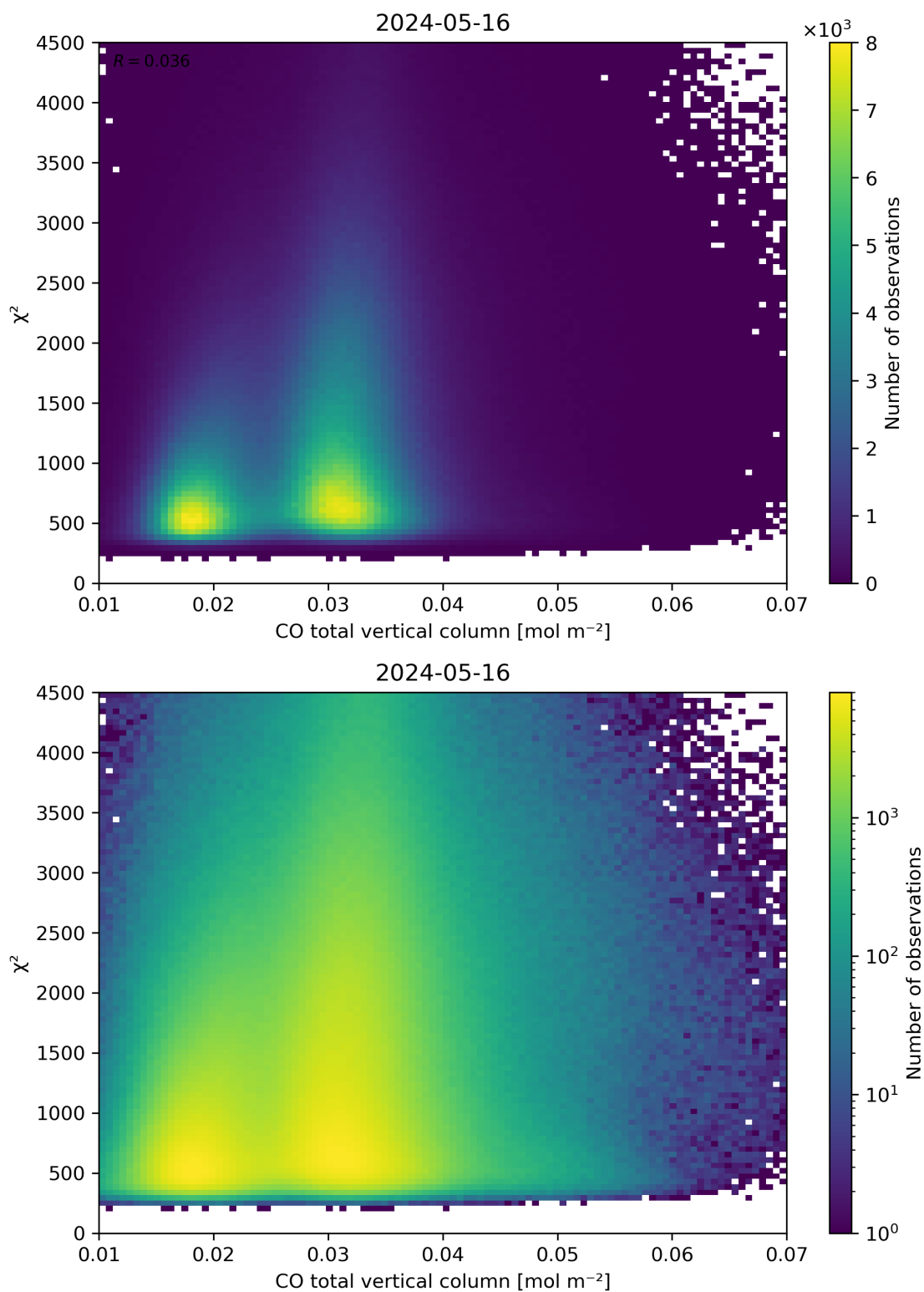
Figure 35: Scatter density plot of “CO total vertical column” against “ \chi^2 ” for 2024-05-15 to 2024-05-17.
