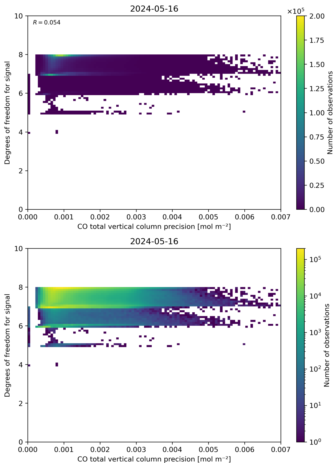
Figure 45: Scatter density plot of “CO total vertical column precision” against “Degrees of freedom for signal” for 2024-05-15 to 2024-05-17.
