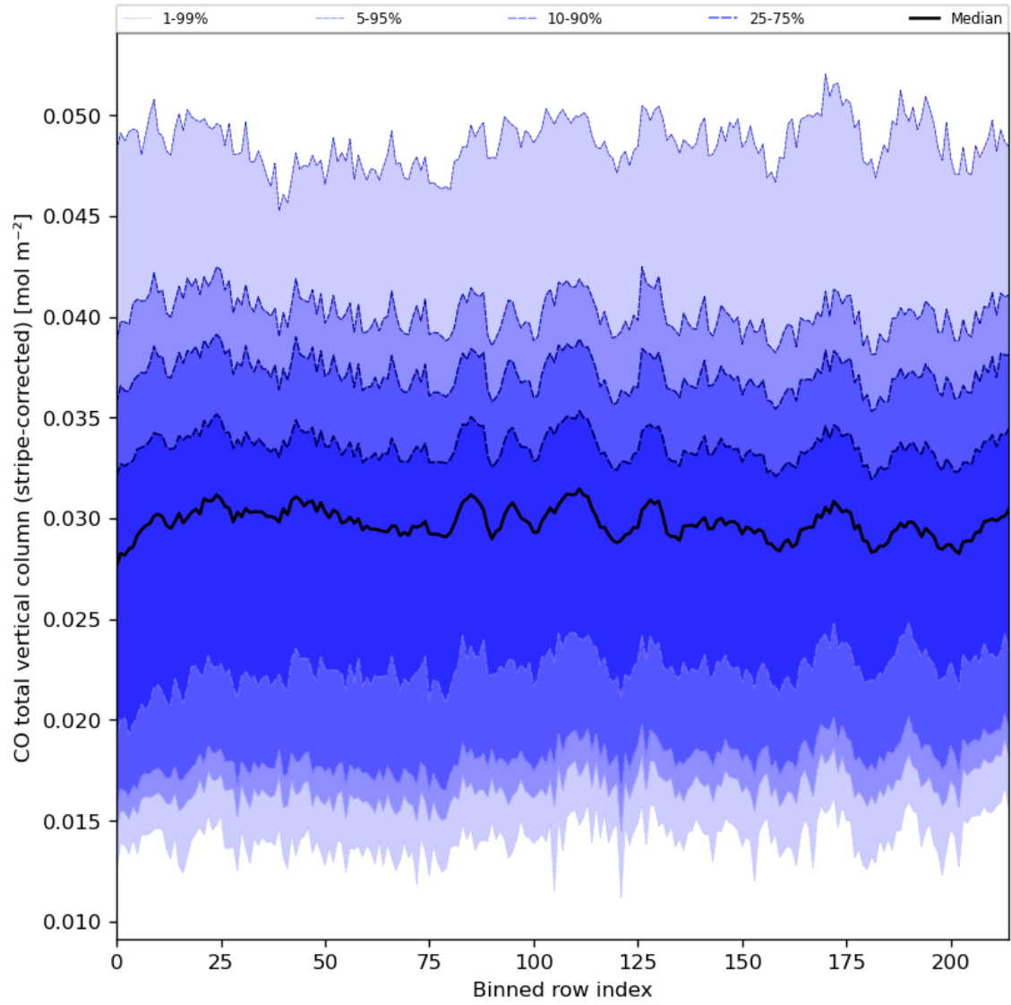
Figure 27: Along track statistics of “CO total vertical column (stripe-corrected)” for 2024-05-15 to 2024-05-17
