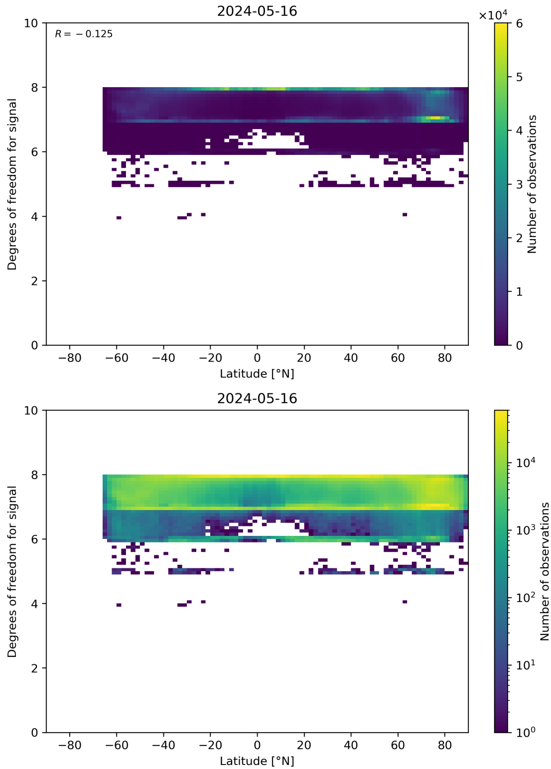
Figure 55: Scatter density plot of “Latitude” against “Degrees of freedom for signal” for 2024-05-15 to 2024-05-17.
