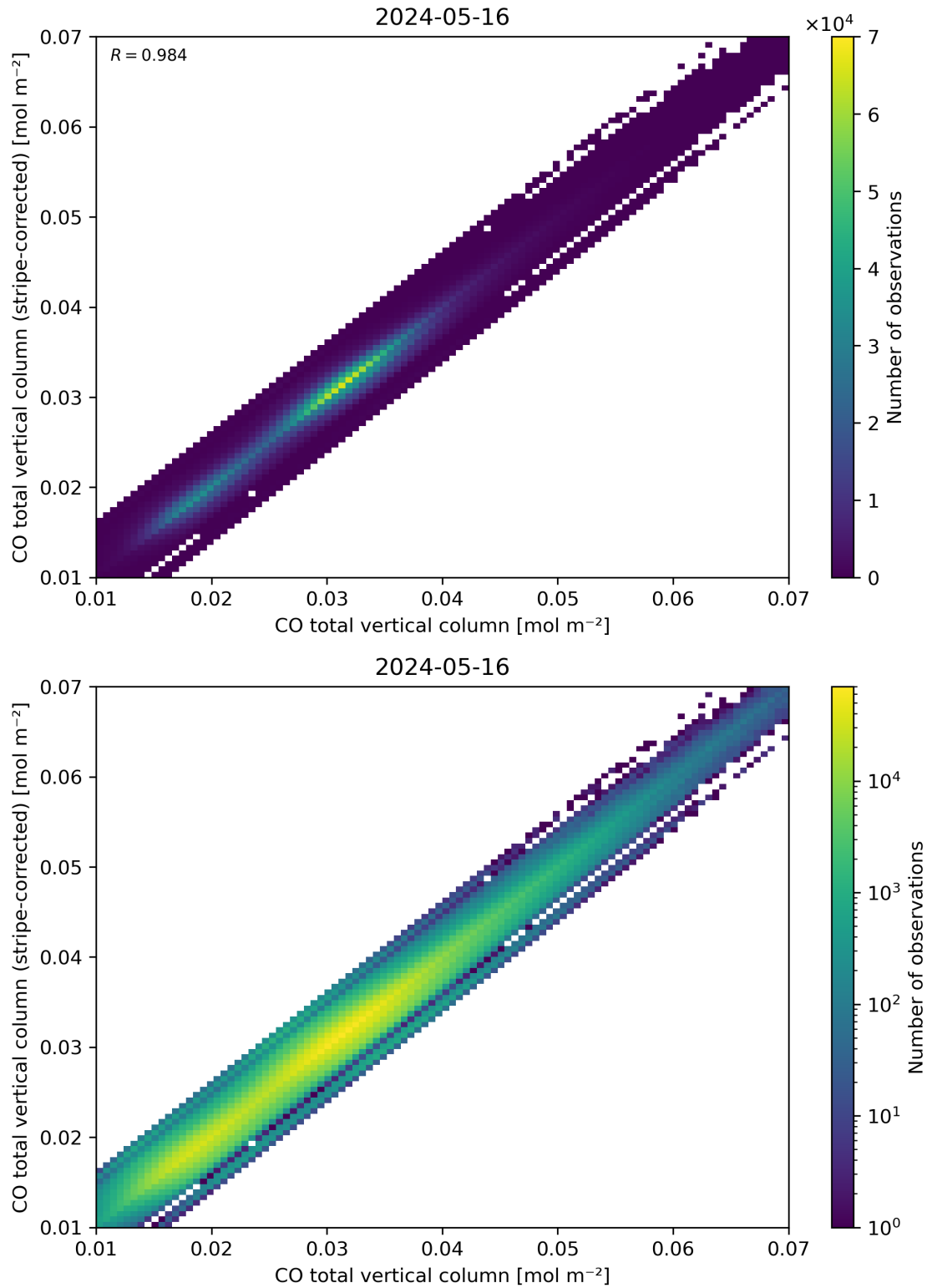
Figure 33: Scatter density plot of “CO total vertical column” against “CO total vertical column (stripe-corrected)” for 2024-05-15 to 2024-05-17.
