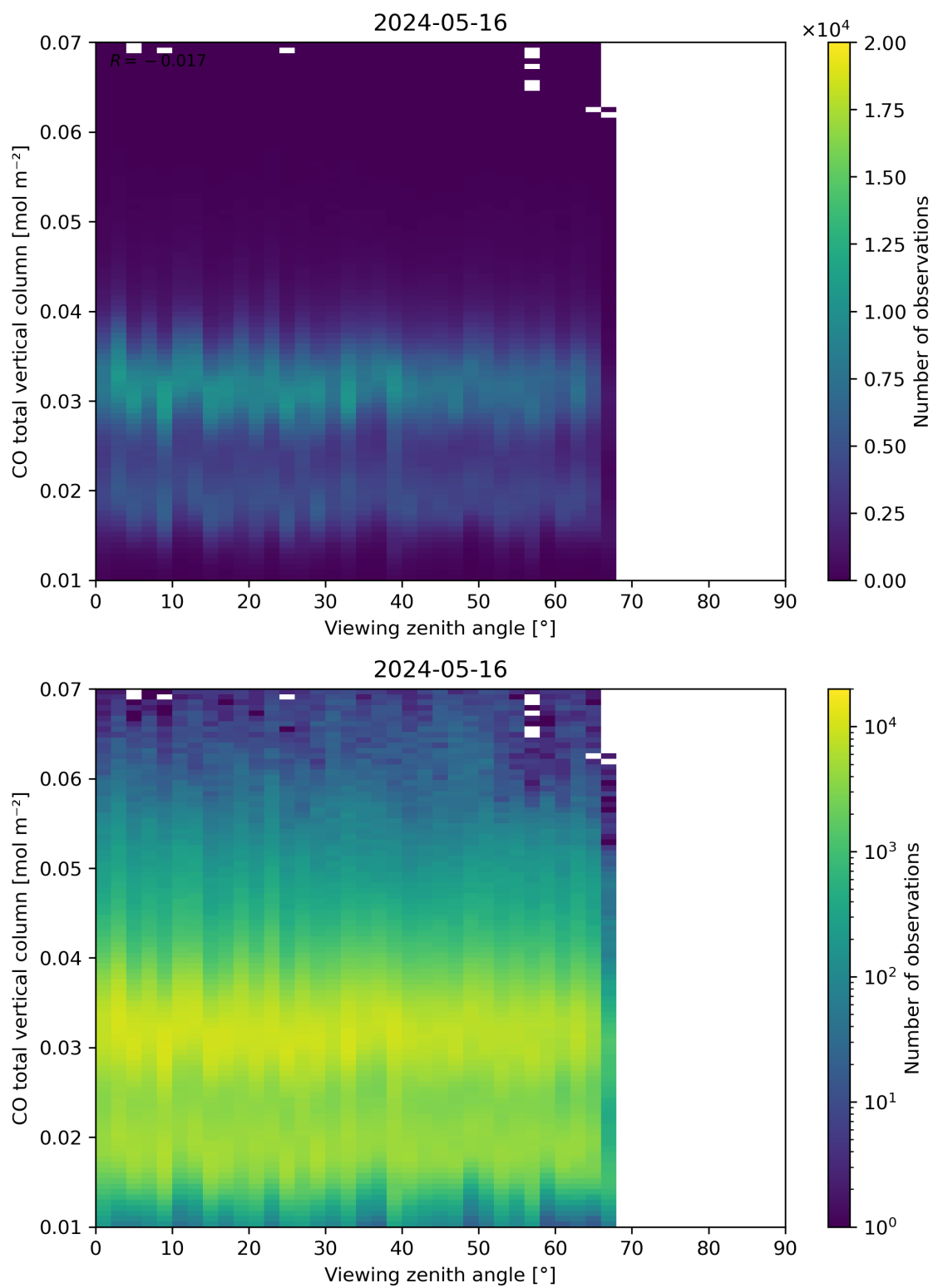
Figure 69: Scatter density plot of “Viewing zenith angle” against “CO total vertical column” for 2024-05-15 to 2024-05-17.
