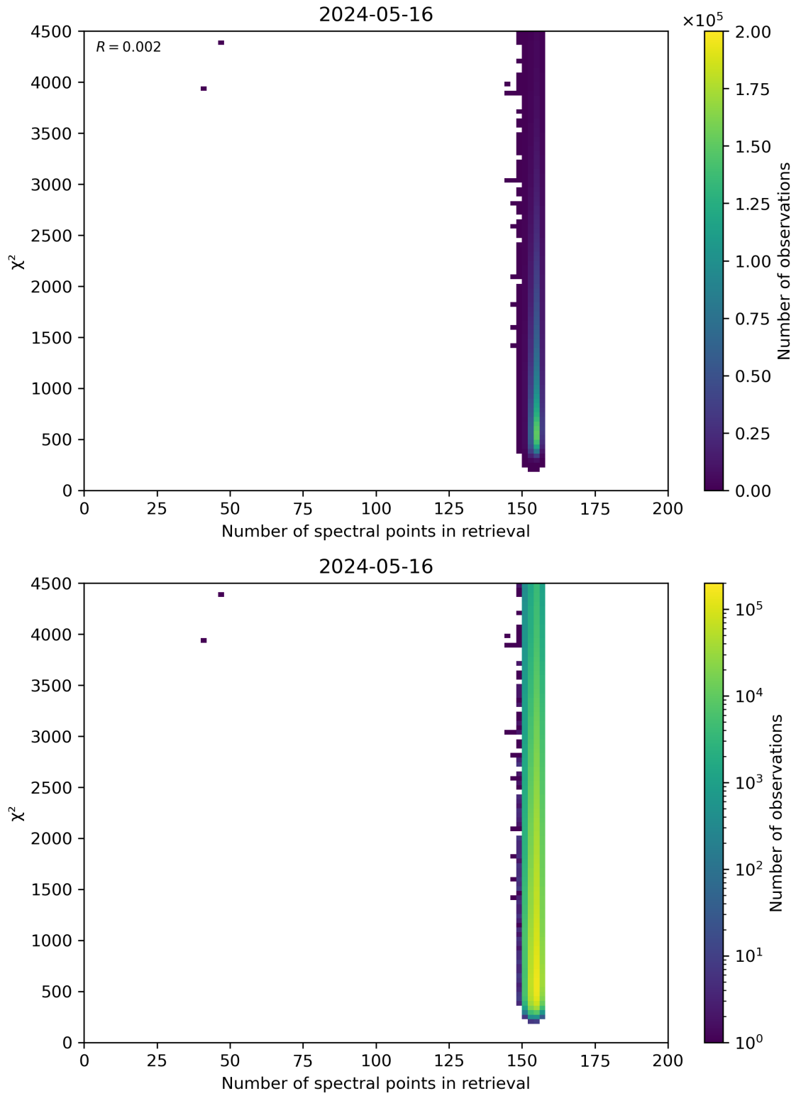
Figure 58: Scatter density plot of “Number of spectral points in retrieval” against “ \chi^2 ” for 2024-05-15 to 2024-05-17.
