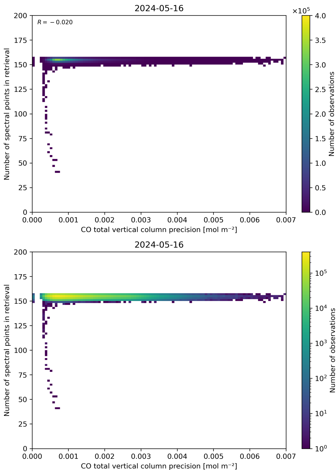
Figure 47: Scatter density plot of “CO total vertical column precision” against “Number of spectral points in retrieval” for 2024-05-15 to 2024-05-17.
