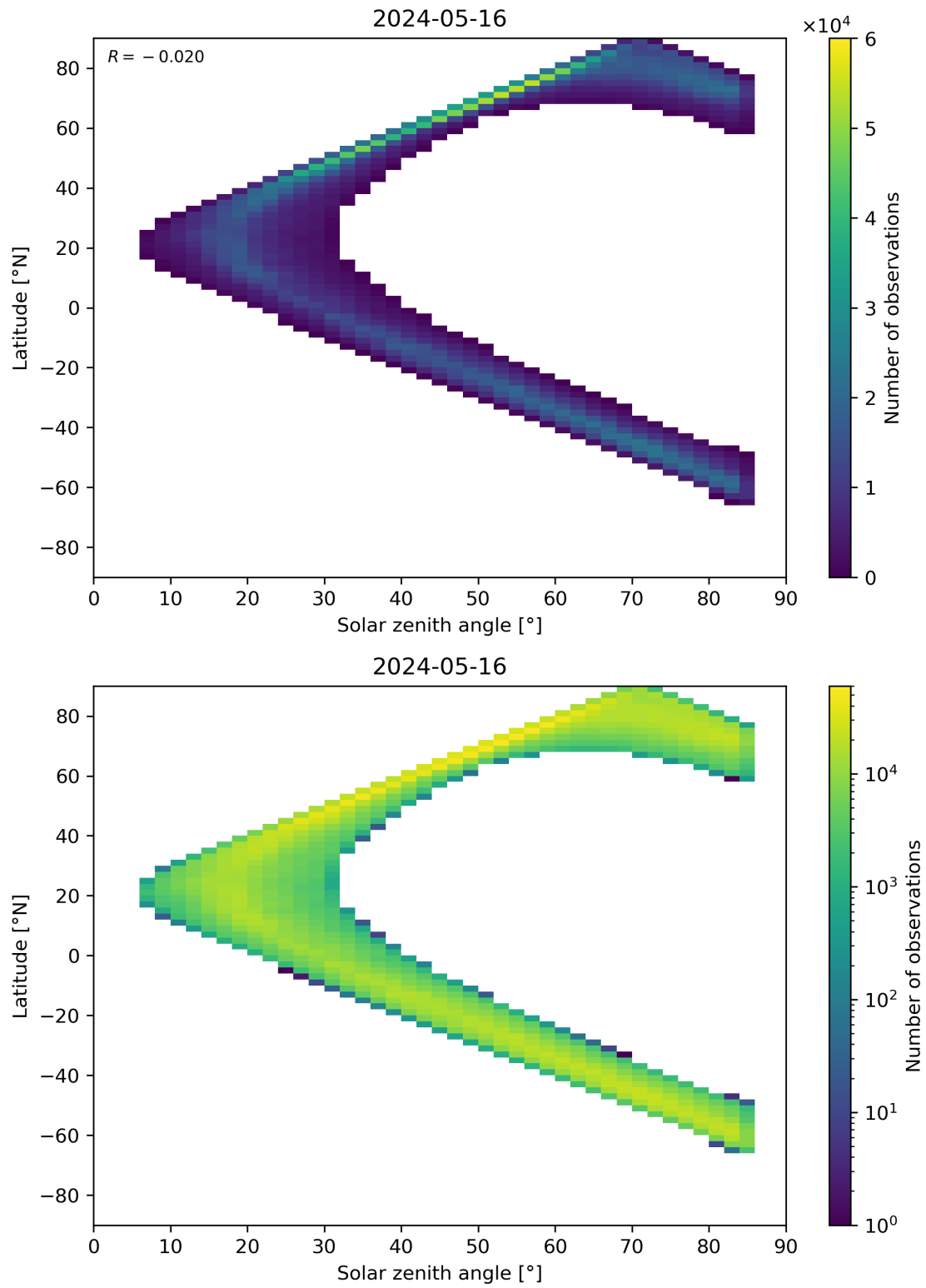
Figure 66: Scatter density plot of “Solar zenith angle” against “Latitude” for 2024-05-15 to 2024-05-17.
