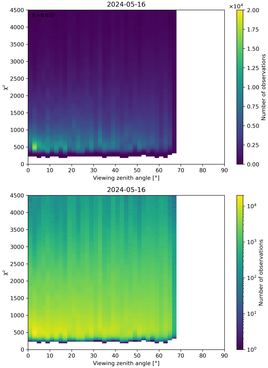
Figure 72: Scatter density plot of “Viewing zenith angle” against “ \chi^2 ” for 2024-05-15 to 2024-05-17.
