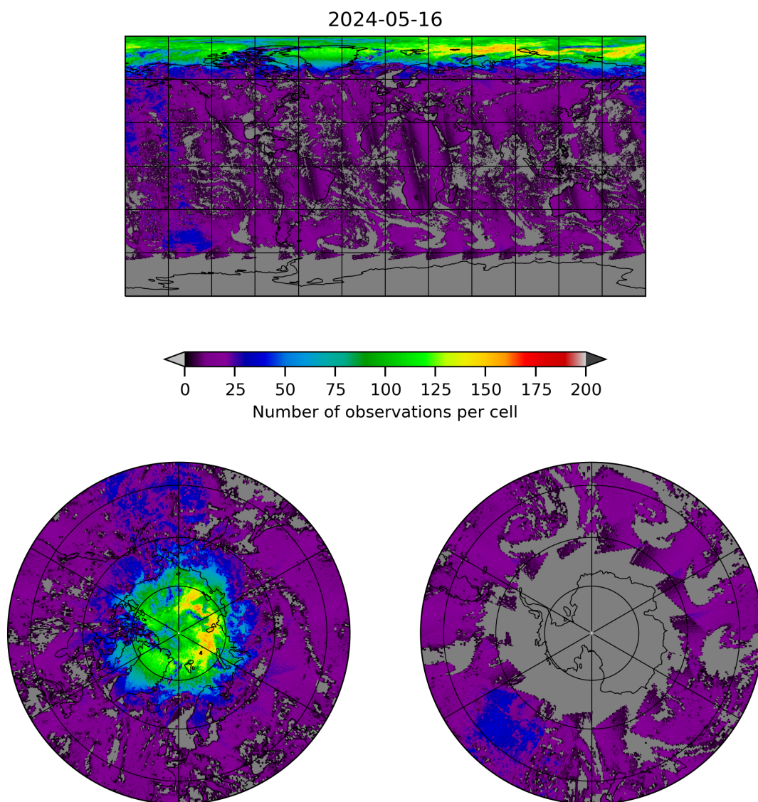
Figure 8: Map of the number of observations for 2024-05-15 to 2024-05-17
