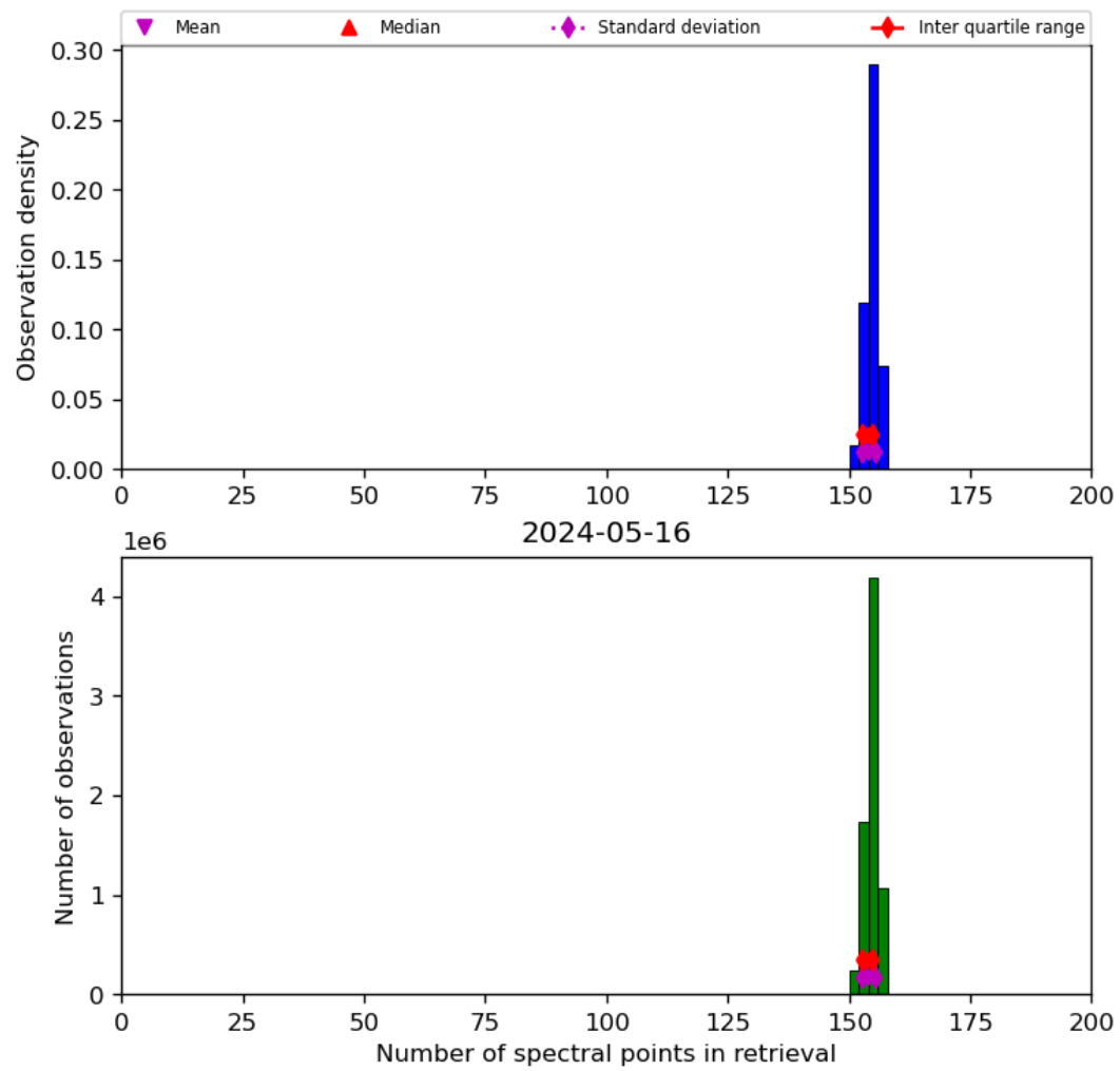
Figure 21: Histogram of “Number of spectral points in retrieval” for 2024-05-15 to 2024-05-17
