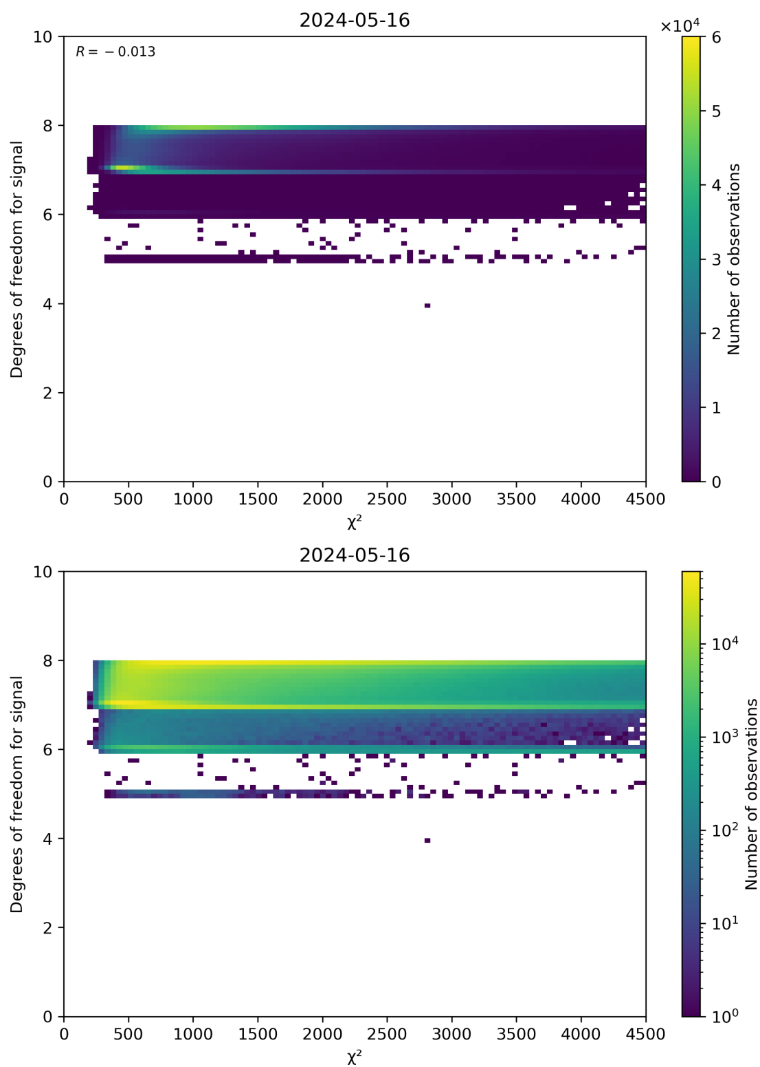
Figure 48: Scatter density plot of “ \chi^2 ” against “Degrees of freedom for signal” for 2024-05-15 to 2024-05-17.
