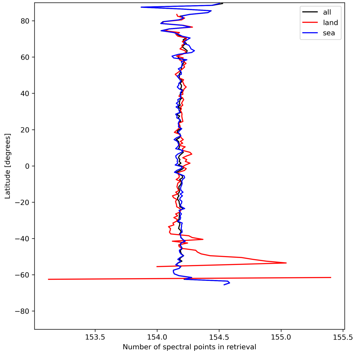
Figure 13: Zonal average of “Number of spectral points in retrieval” for 2024-05-15 to 2024-05-17.
