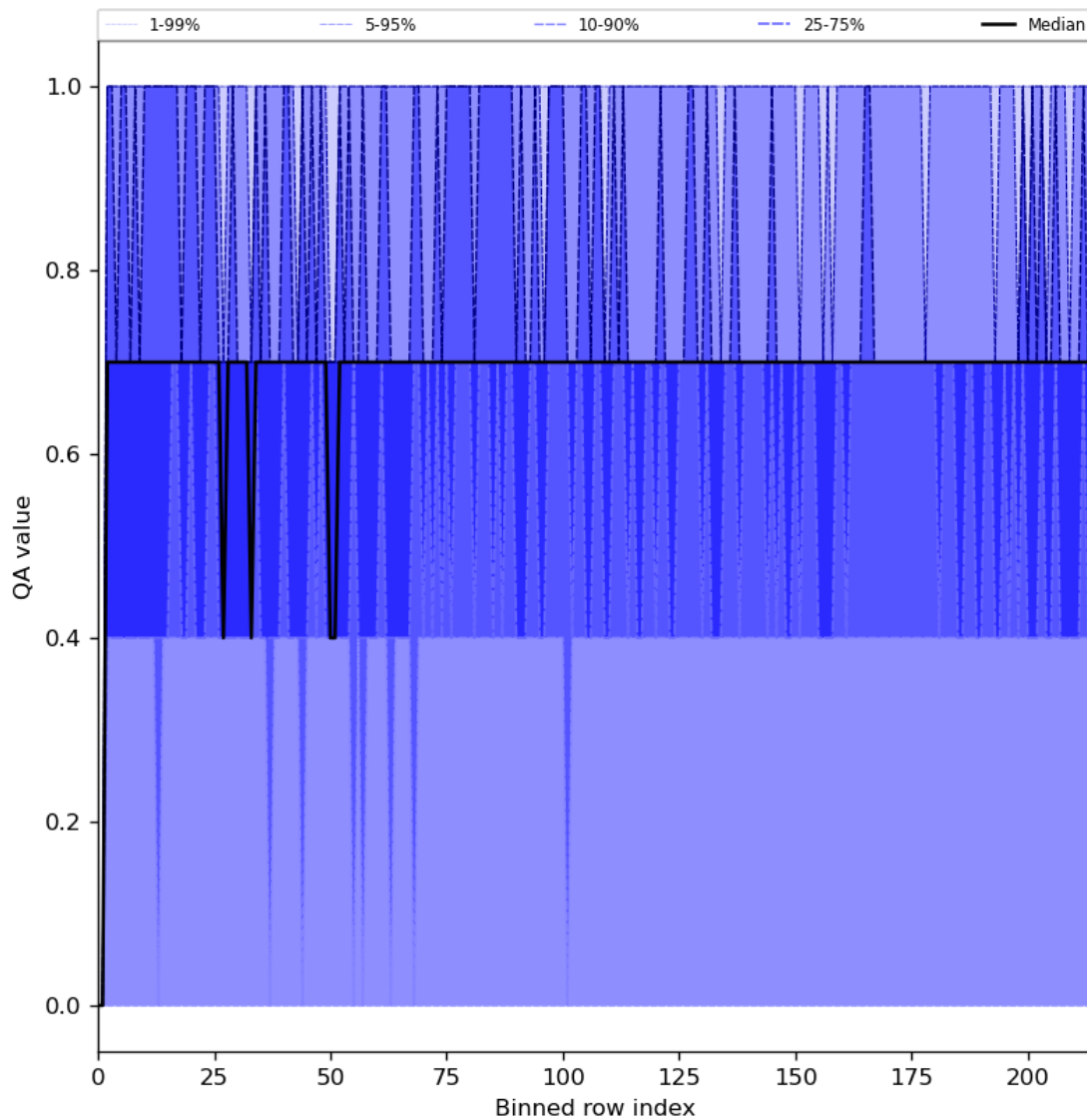
Figure 25: Along track statistics of “QA value” for 2024-05-15 to 2024-05-17
