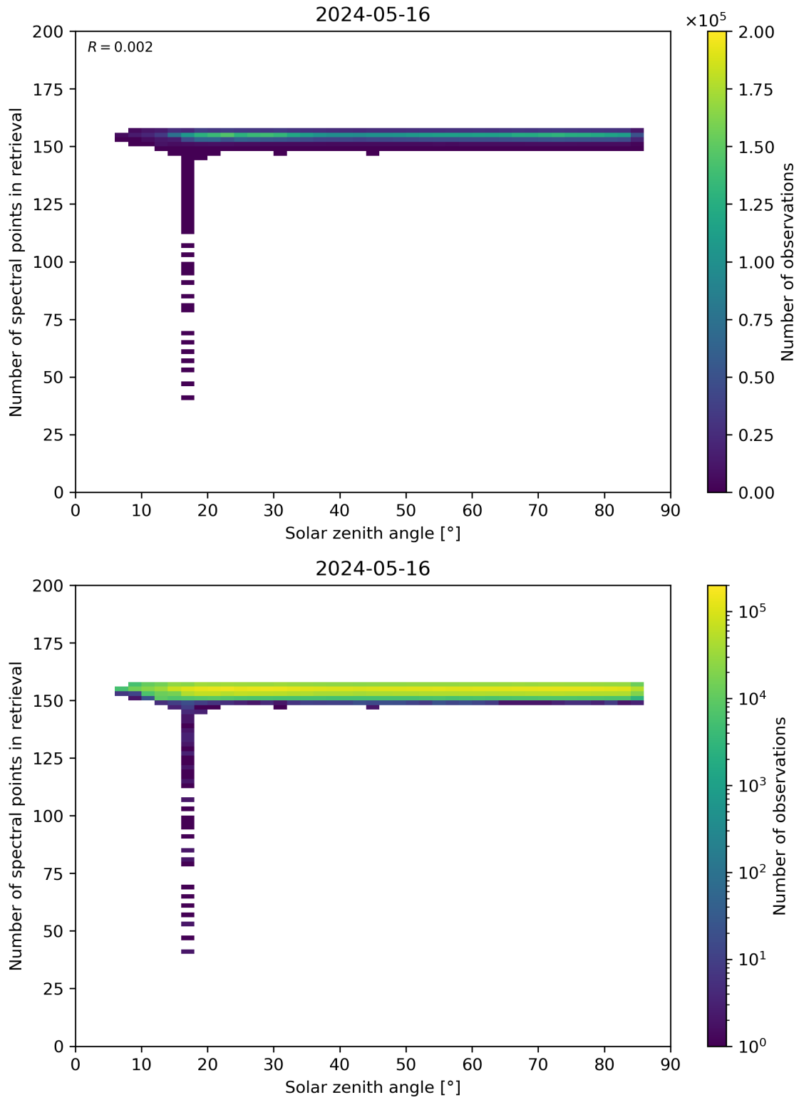
Figure 68: Scatter density plot of “Solar zenith angle” against “Number of spectral points in retrieval” for 2024-05-15 to 2024-05-17.
