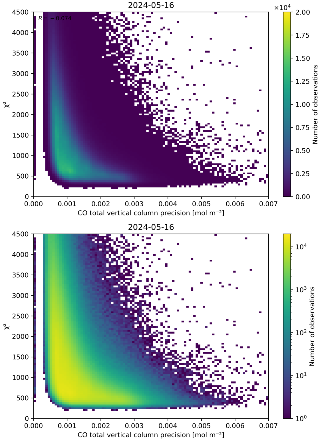
Figure 44: Scatter density plot of “CO total vertical column precision” against “ \chi^2 ” for 2024-05-15 to 2024-05-17.
