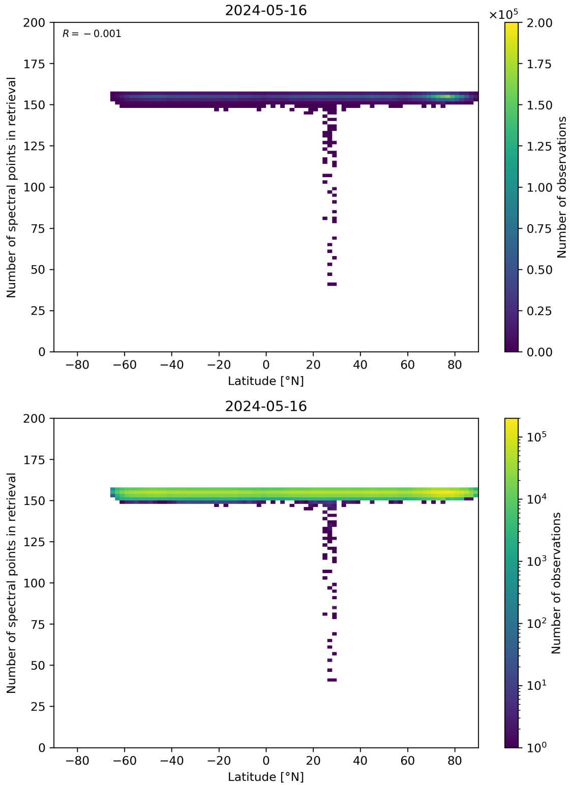
Figure 57: Scatter density plot of “Latitude” against “Number of spectral points in retrieval” for 2024-05-15 to 2024-05-17.
