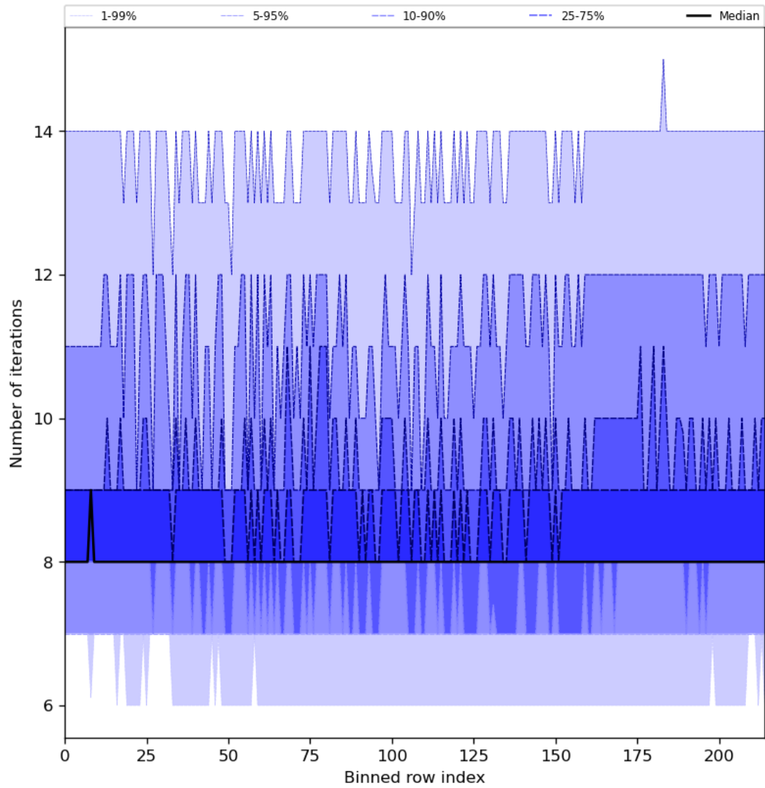
Figure 32: Along track statistics of “Number of iterations” for 2024-05-15 to 2024-05-17
