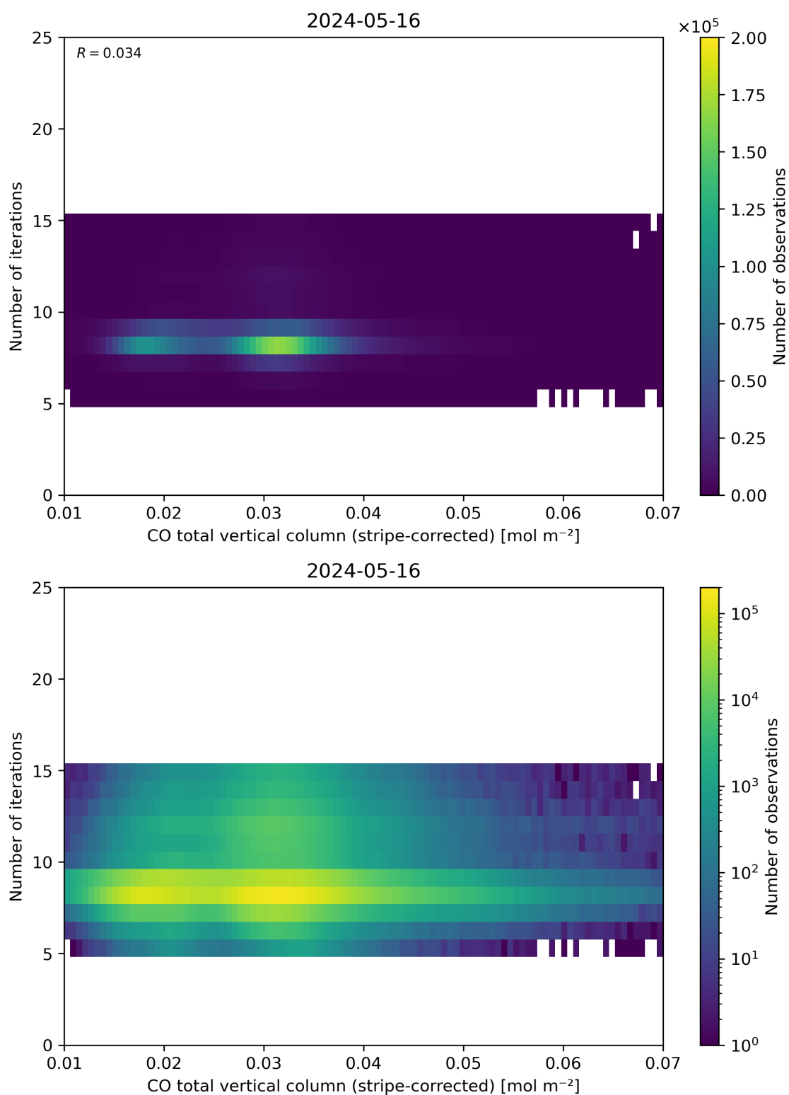
Figure 39: Scatter density plot of “CO total vertical column (stripe-corrected)” against “Number of iterations” for 2024-05-15 to 2024-05-17.
