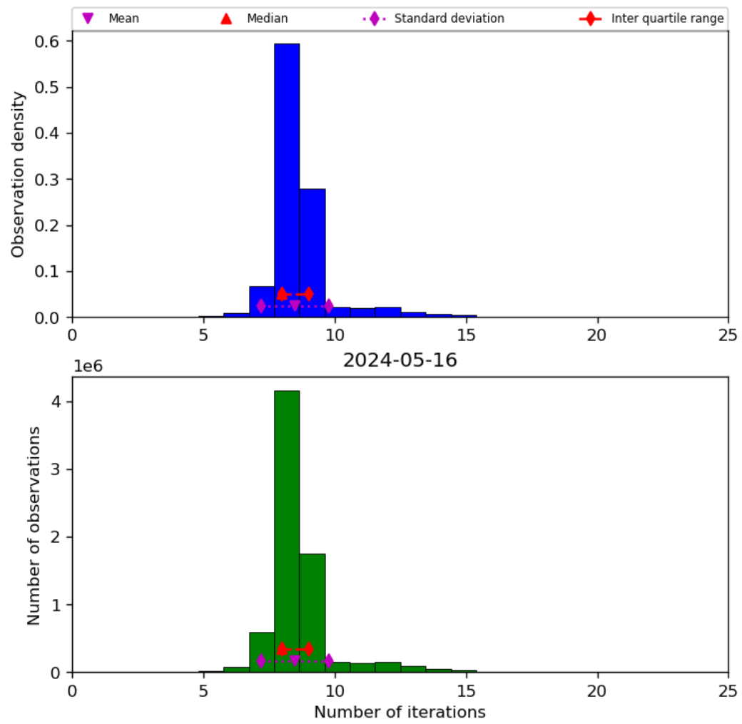
Figure 24: Histogram of “Number of iterations” for 2024-05-15 to 2024-05-17
