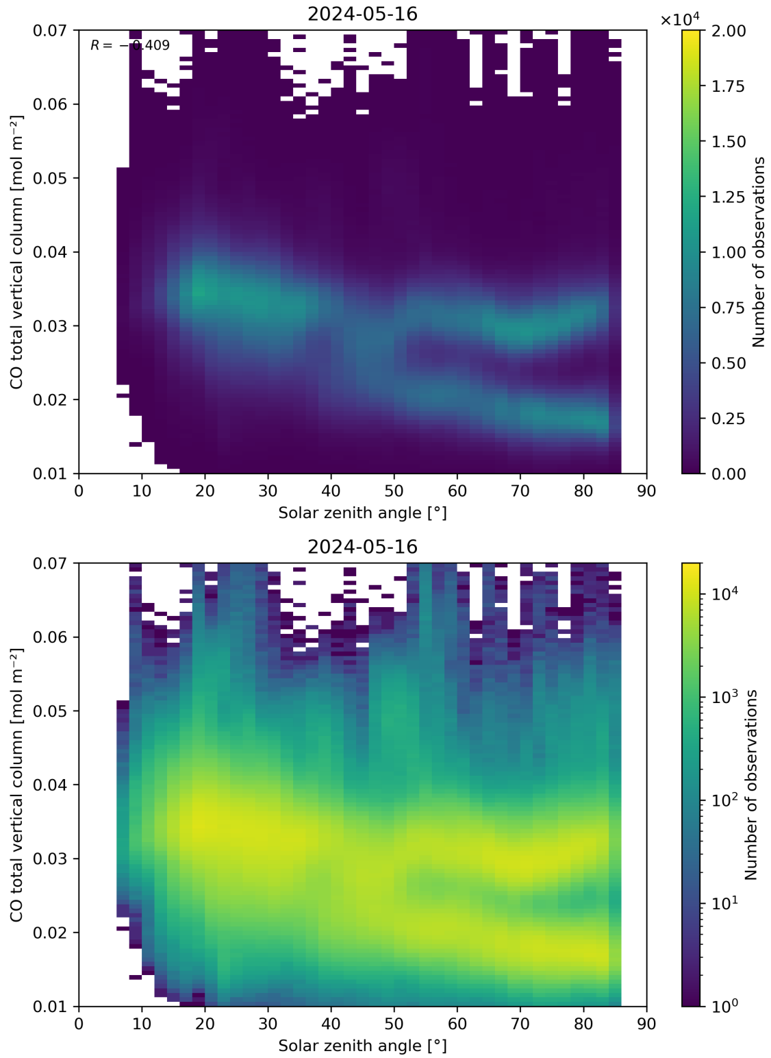
Figure 61: Scatter density plot of “Solar zenith angle” against “CO total vertical column” for 2024-05-15 to 2024-05-17.
