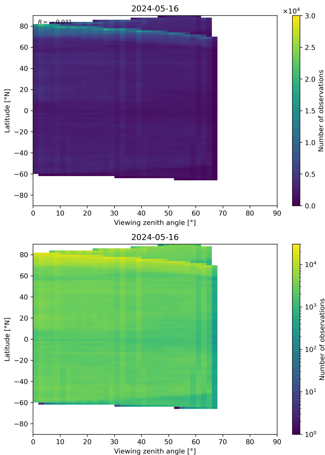
Figure 74: Scatter density plot of “Viewing zenith angle” against “Latitude” for 2024-05-15 to 2024-05-17.
