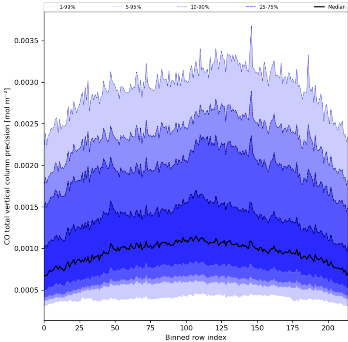
Figure 28: Along track statistics of “CO total vertical column precision” for 2024-05-15 to 2024-05-17
