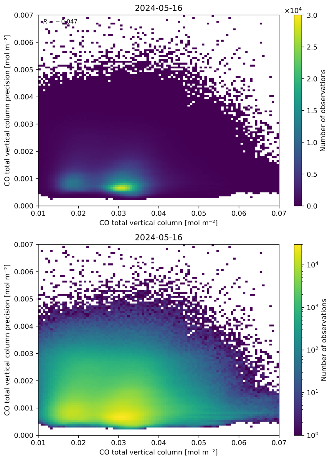
Figure 34: Scatter density plot of “CO total vertical column” against “CO total vertical column precision” for 2024-05-15 to 2024-05-17.
