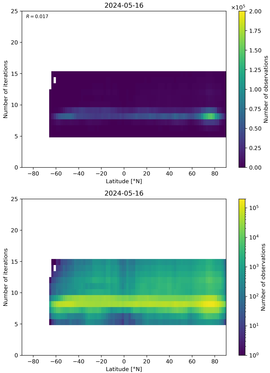
Figure 56: Scatter density plot of “Latitude” against “Number of iterations” for 2024-05-15 to 2024-05-17.
