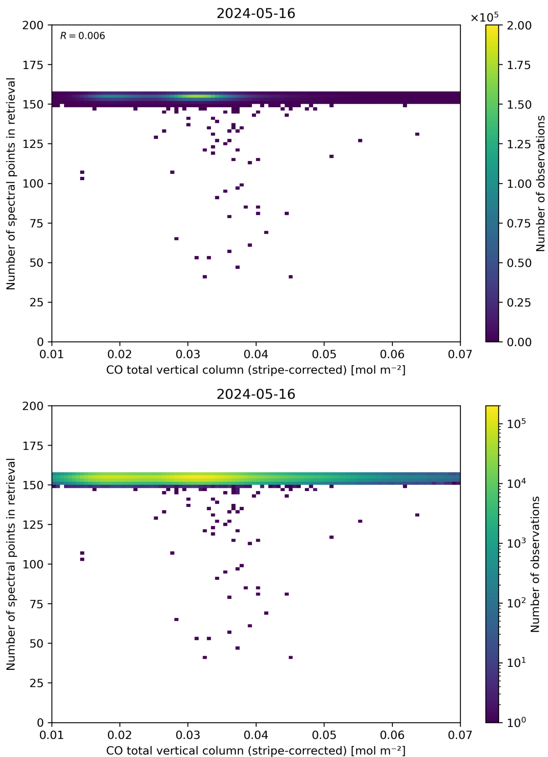
Figure 40: Scatter density plot of “CO total vertical column (stripe-corrected)” against “Number of spectral points in retrieval” for 2024-05-15 to 2024-05-17.
