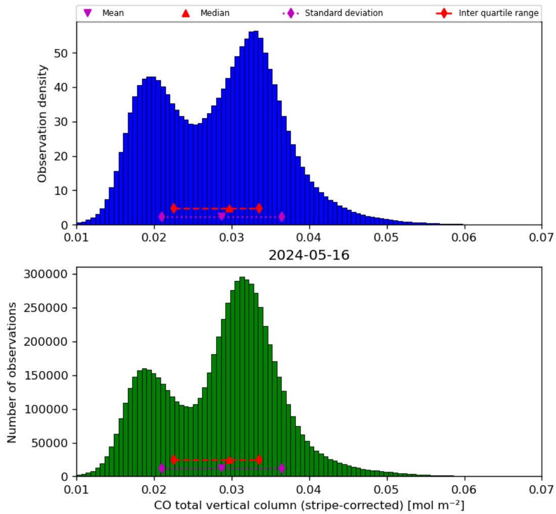
Figure 19: Histogram of “CO total vertical column (stripe-corrected)” for 2024-05-15 to 2024-05-17
