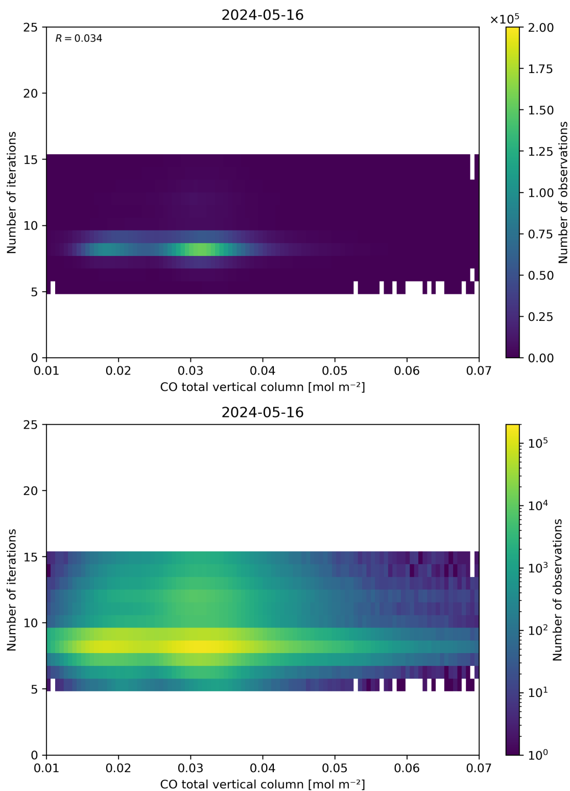
Figure 42: Scatter density plot of “CO total vertical column” against “Number of iterations” for 2024-05-15 to 2024-05-17.
