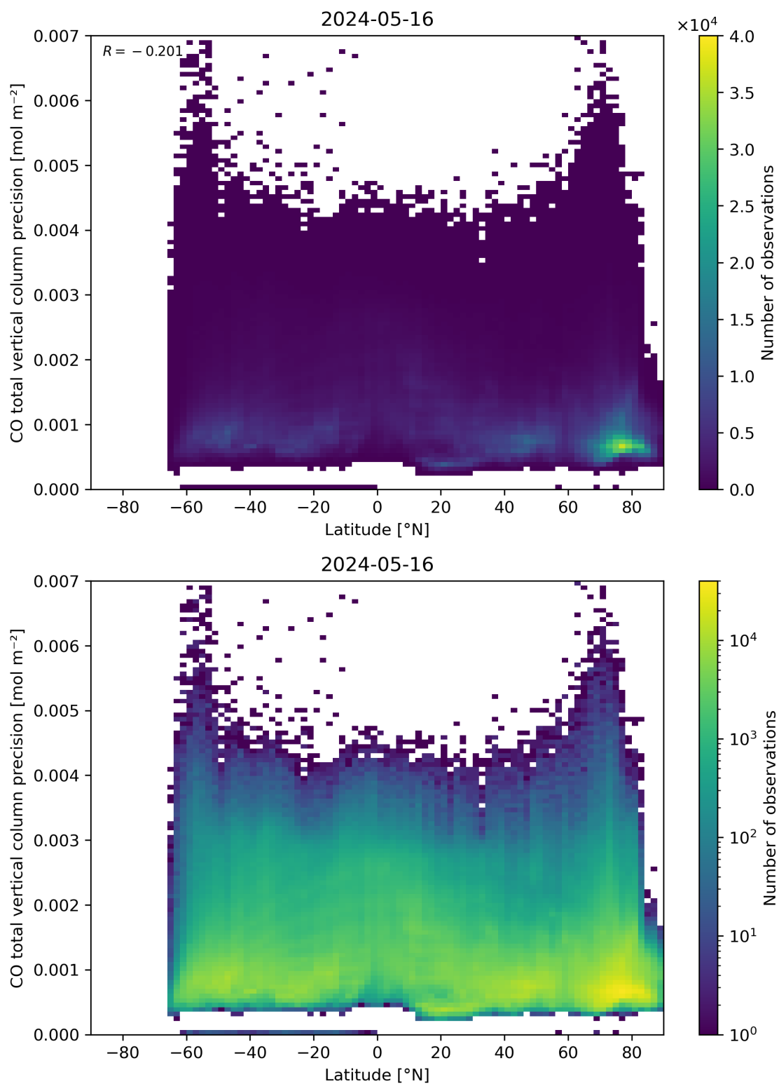
Figure 53: Scatter density plot of “Latitude” against “CO total vertical column precision” for 2024-05-15 to 2024-05-17.
