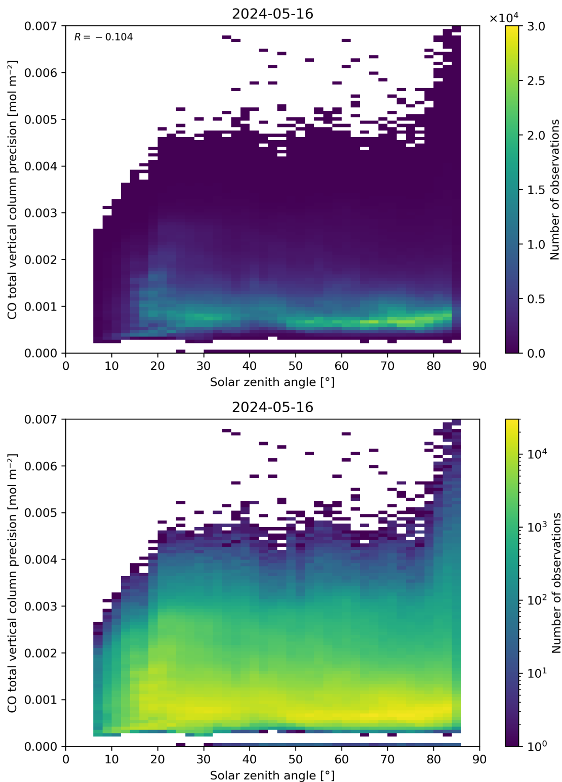
Figure 63: Scatter density plot of “Solar zenith angle” against “CO total vertical column precision” for 2024-05-15 to 2024-05-17.
