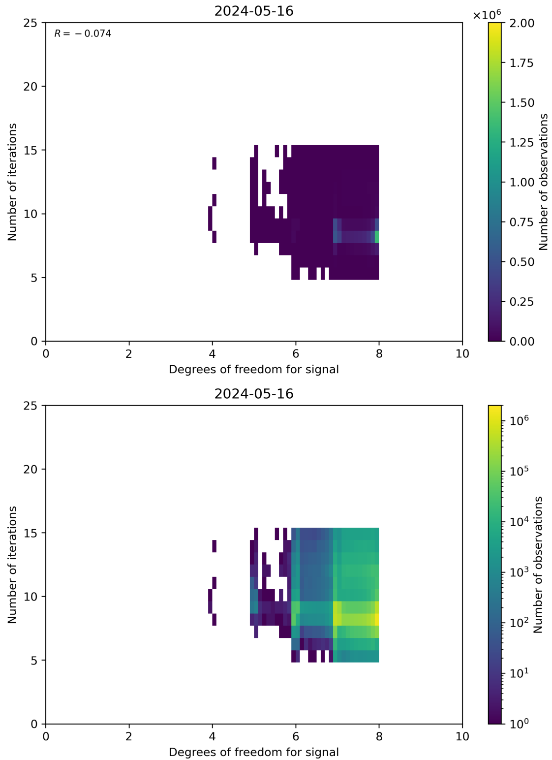
Figure 50: Scatter density plot of “Degrees of freedom for signal” against “Number of iterations” for 2024-05-15 to 2024-05-17.
