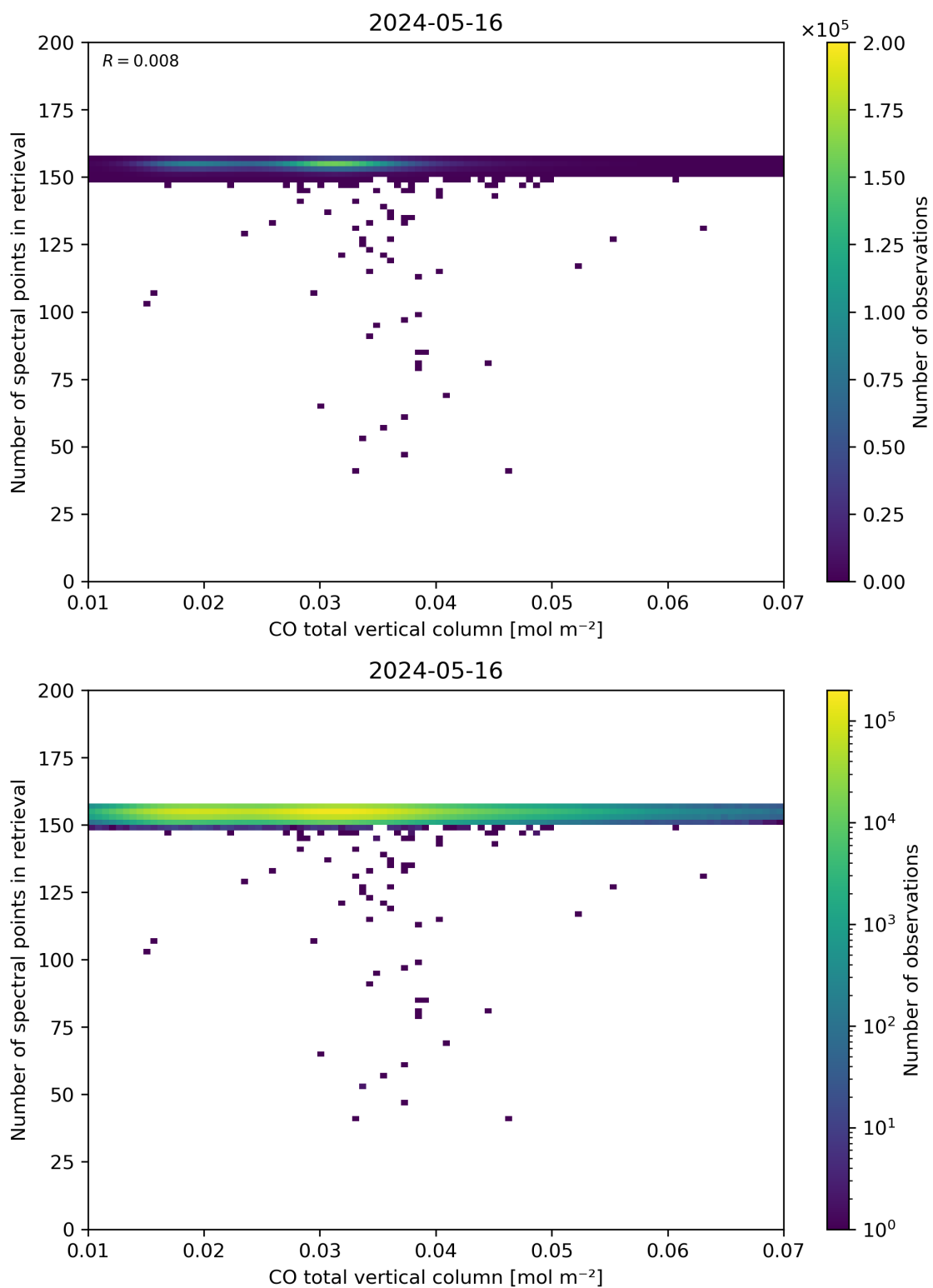
Figure 43: Scatter density plot of “CO total vertical column” against “Number of spectral points in retrieval” for 2024-05-15 to 2024-05-17.
