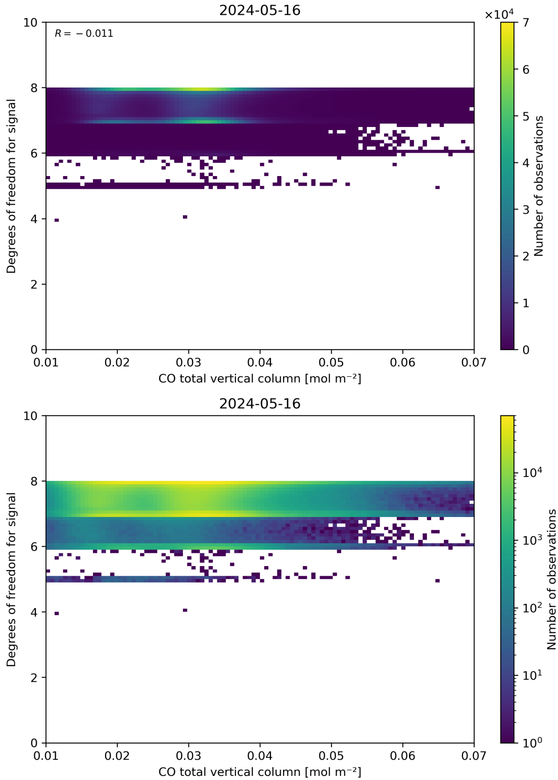
Figure 41: Scatter density plot of “CO total vertical column” against “Degrees of freedom for signal” for 2024-05-15 to 2024-05-17.
