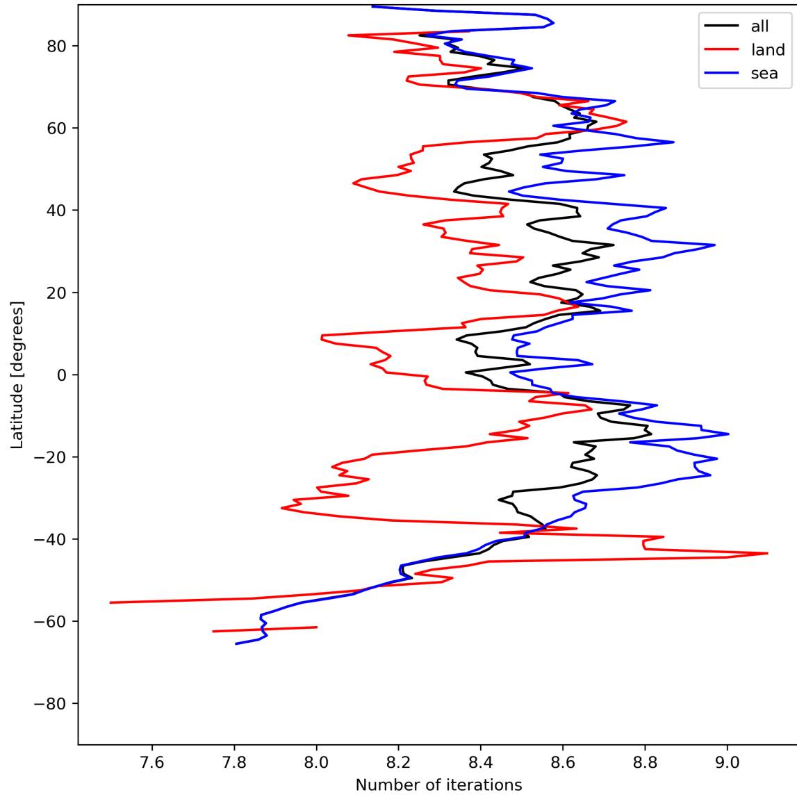
Figure 16: Zonal average of “Number of iterations” for 2024-05-15 to 2024-05-17.
