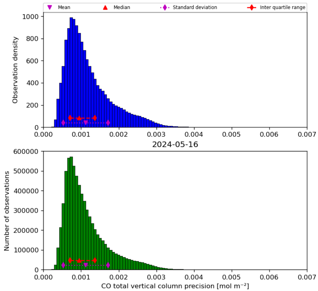
Figure 20: Histogram of “CO total vertical column precision” for 2024-05-15 to 2024-05-17
