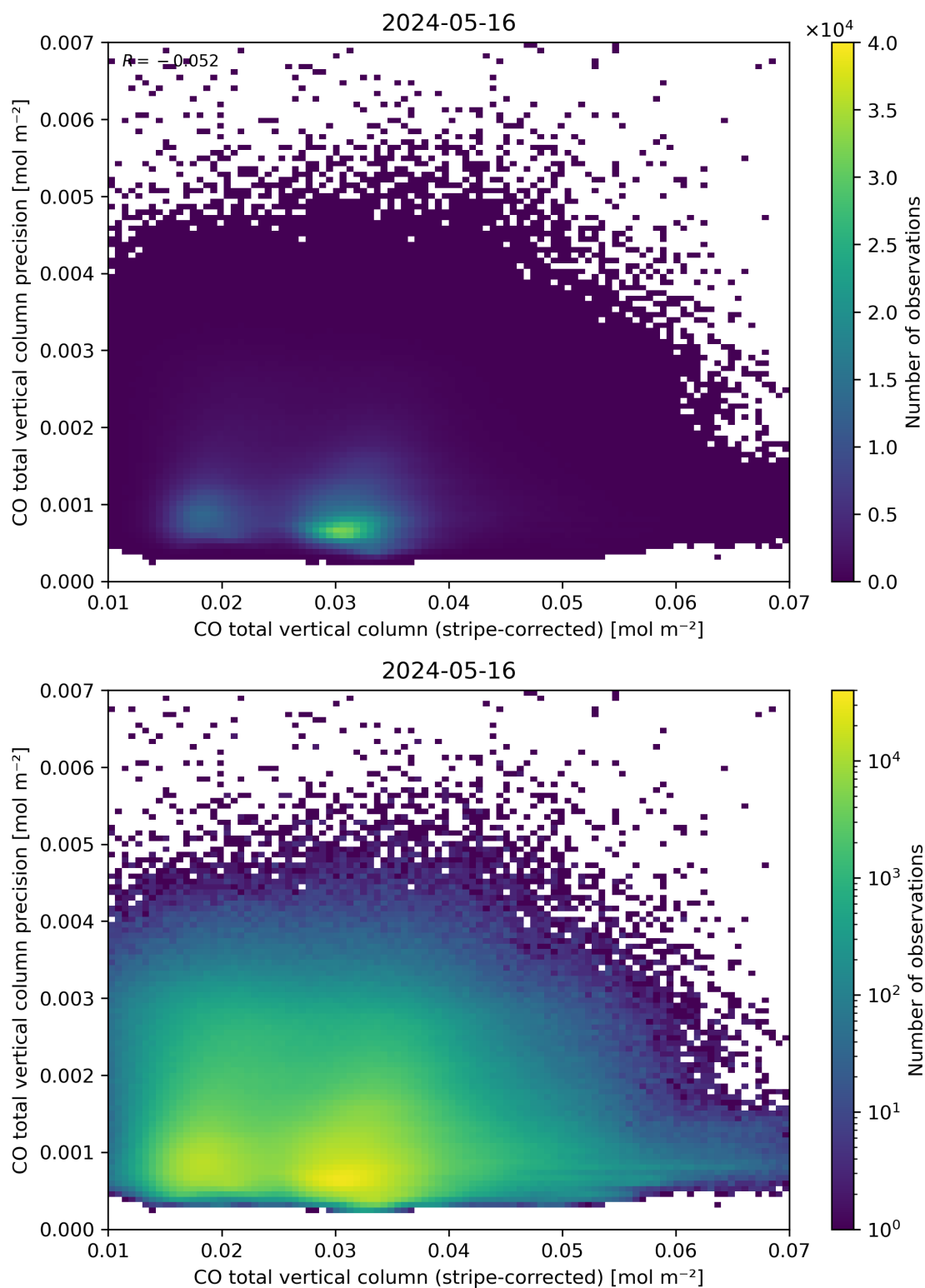
Figure 36: Scatter density plot of “CO total vertical column (stripe-corrected)” against “CO total vertical column precision” for 2024-05-15 to 2024-05-17.
