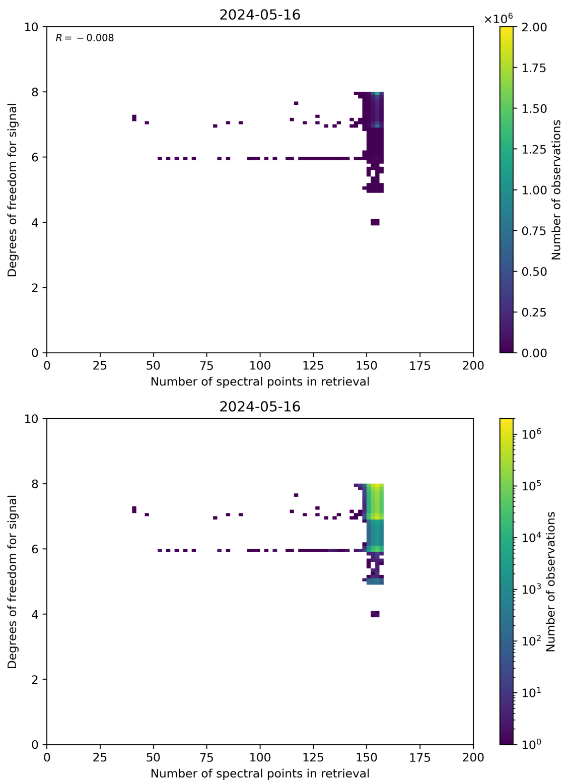
Figure 59: Scatter density plot of “Number of spectral points in retrieval” against “Degrees of freedom for signal” for 2024-05-15 to 2024-05-17.
