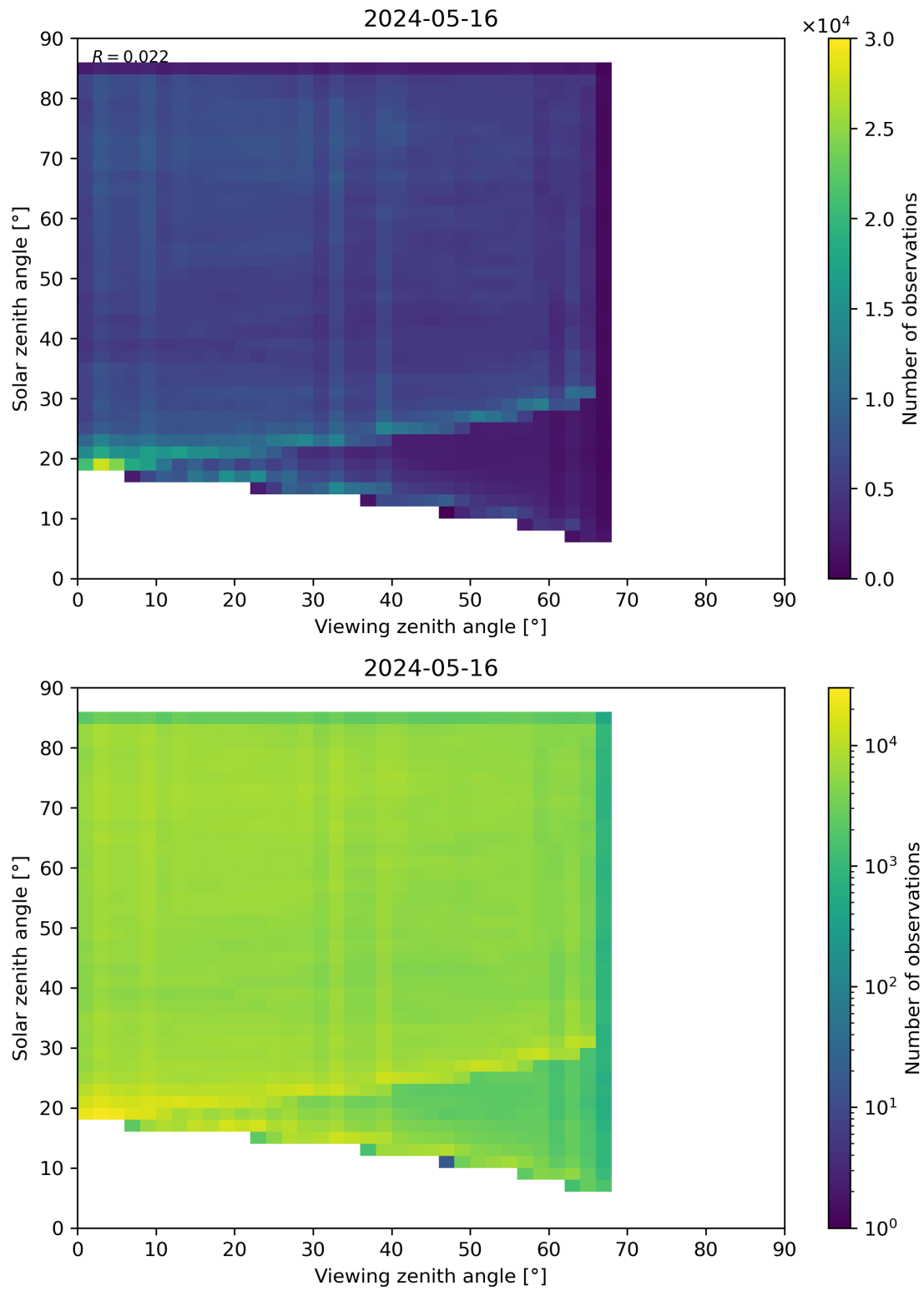
Figure 77: Scatter density plot of “Viewing zenith angle” against “Solar zenith angle” for 2024-05-15 to 2024-05-17.
