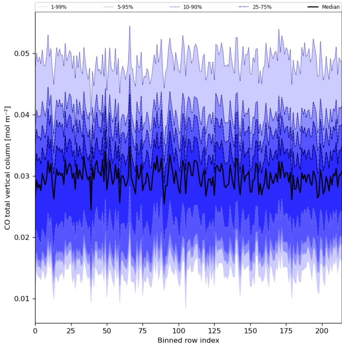
Figure 26: Along track statistics of “CO total vertical column” for 2024-05-15 to 2024-05-17
