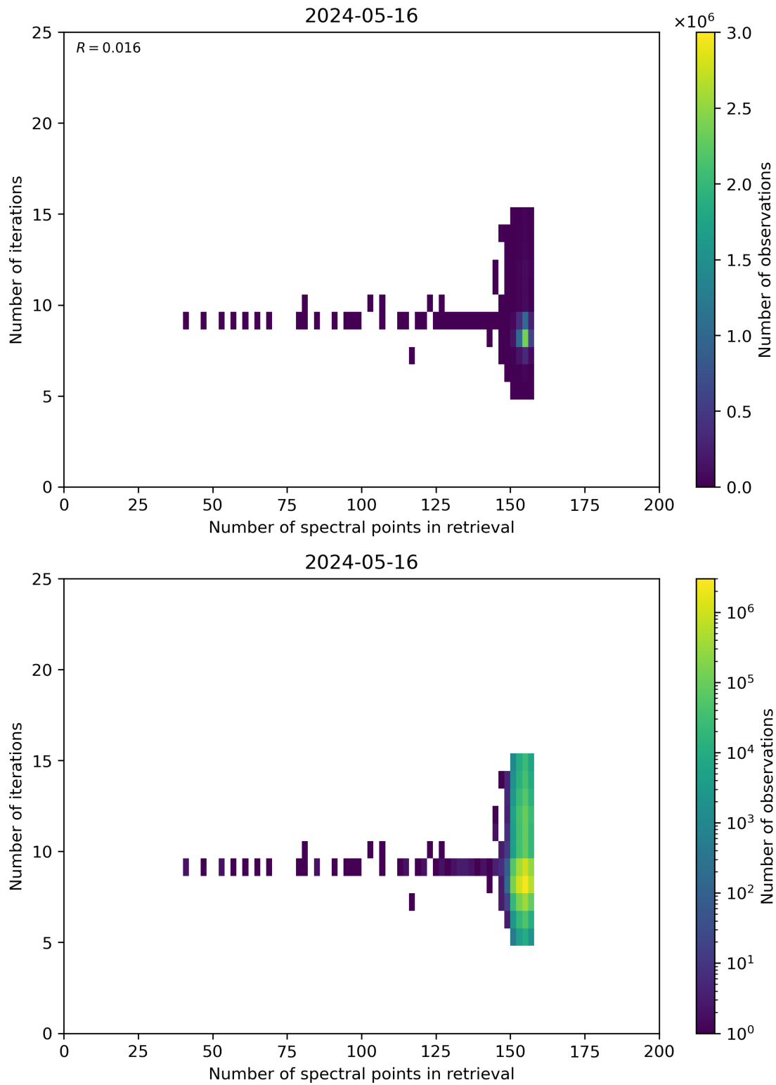
Figure 60: Scatter density plot of “Number of spectral points in retrieval” against “Number of iterations” for 2024-05-15 to 2024-05-17.
