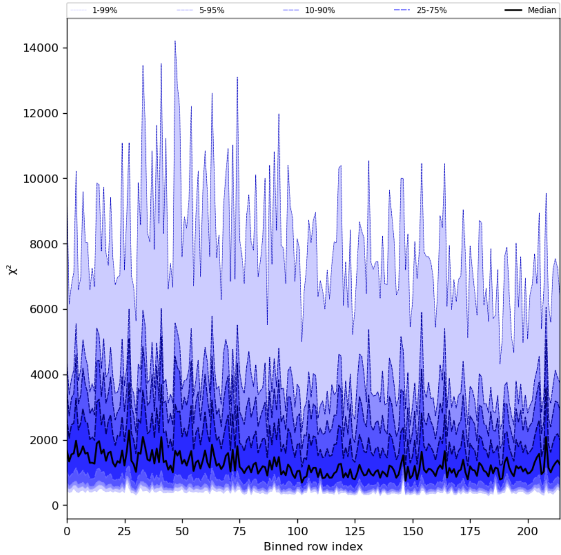
Figure 30: Along track statistics of “ \chi^2 ” for 2024-05-15 to 2024-05-17
