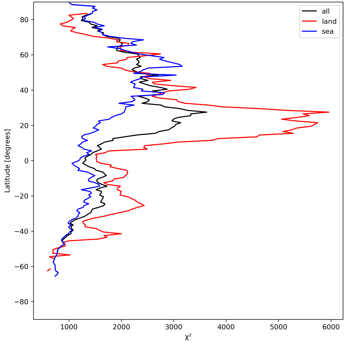
Figure 14: Zonal average of “ \chi^2 ” for 2024-05-15 to 2024-05-17.
