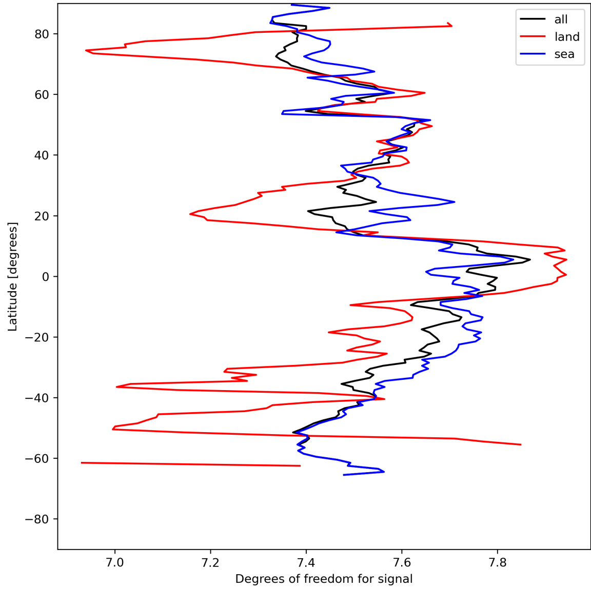
Figure 15: Zonal average of “Degrees of freedom for signal” for 2024-05-15 to 2024-05-17.
