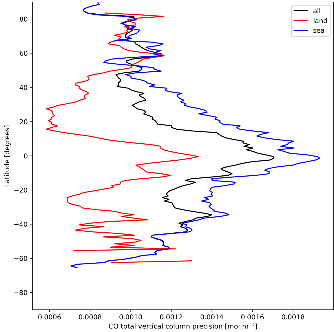
Figure 12: Zonal average of “CO total vertical column precision” for 2024-05-15 to 2024-05-17.
