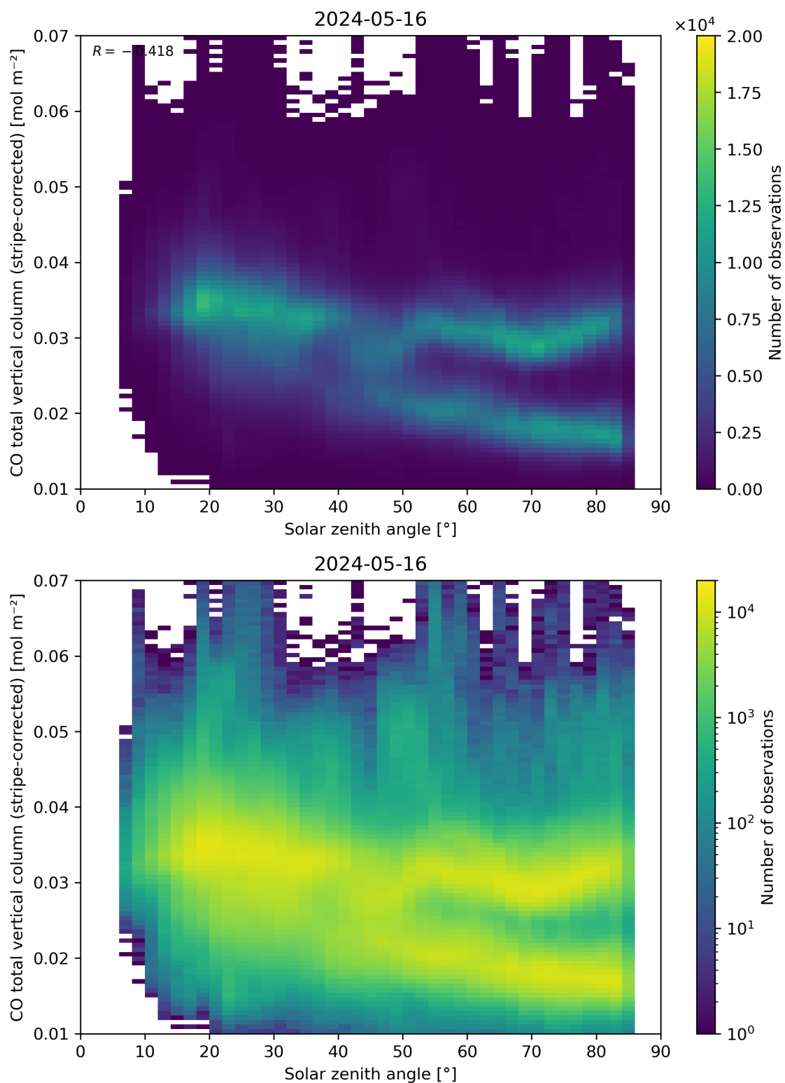
Figure 62: Scatter density plot of “Solar zenith angle” against “CO total vertical column (stripe-corrected)” for 2024-05-15 to 2024-05-17.
