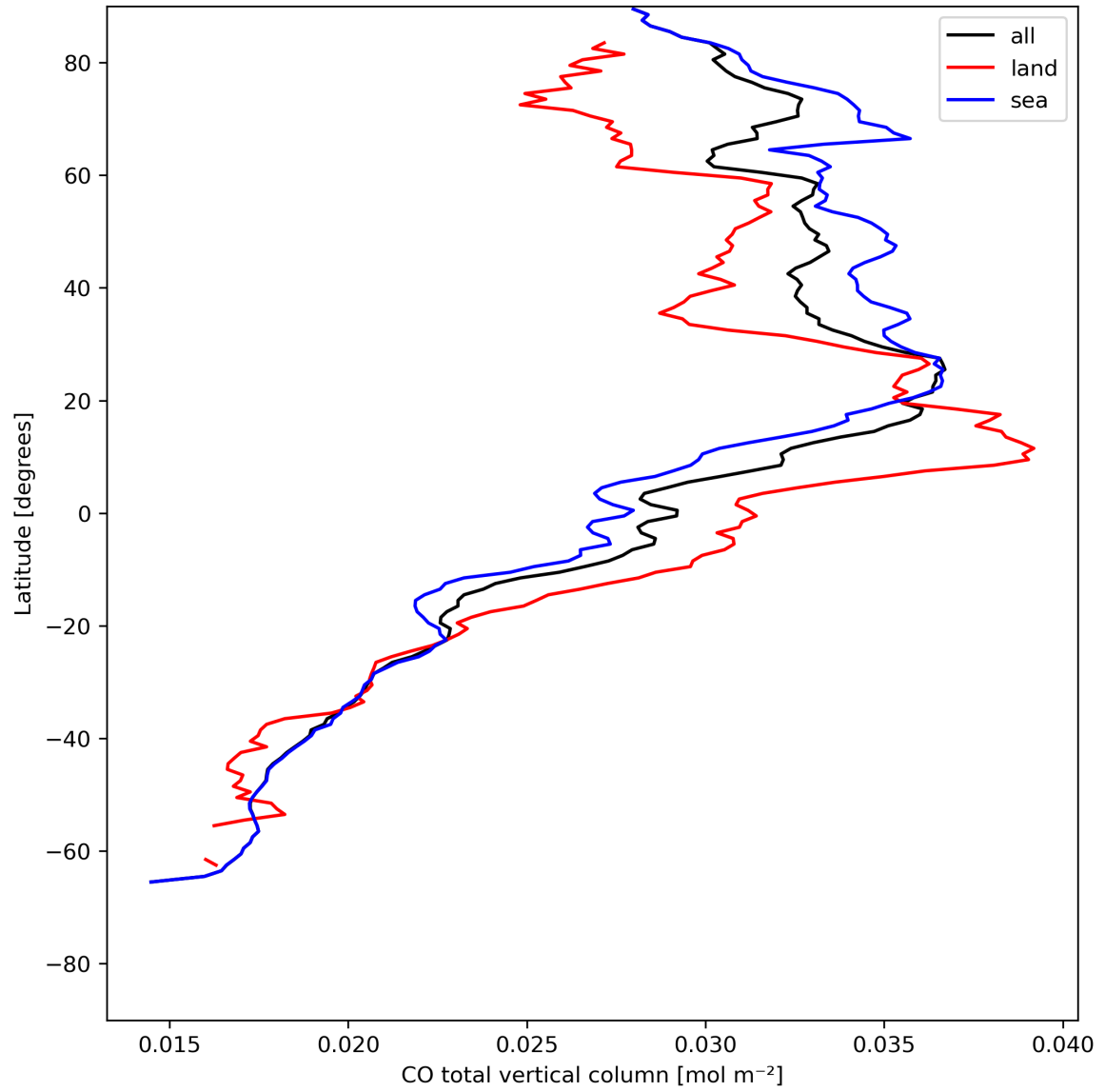
Figure 10: Zonal average of “CO total vertical column” for 2024-05-15 to 2024-05-17.
