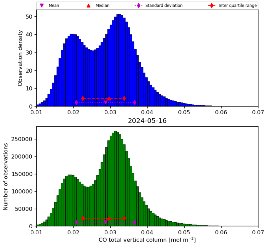
Figure 18: Histogram of “CO total vertical column” for 2024-05-15 to 2024-05-17
