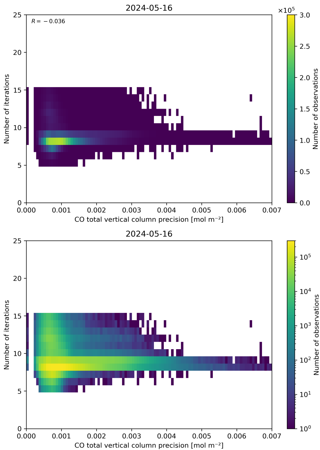
Figure 46: Scatter density plot of “CO total vertical column precision” against “Number of iterations” for 2024-05-15 to 2024-05-17.
