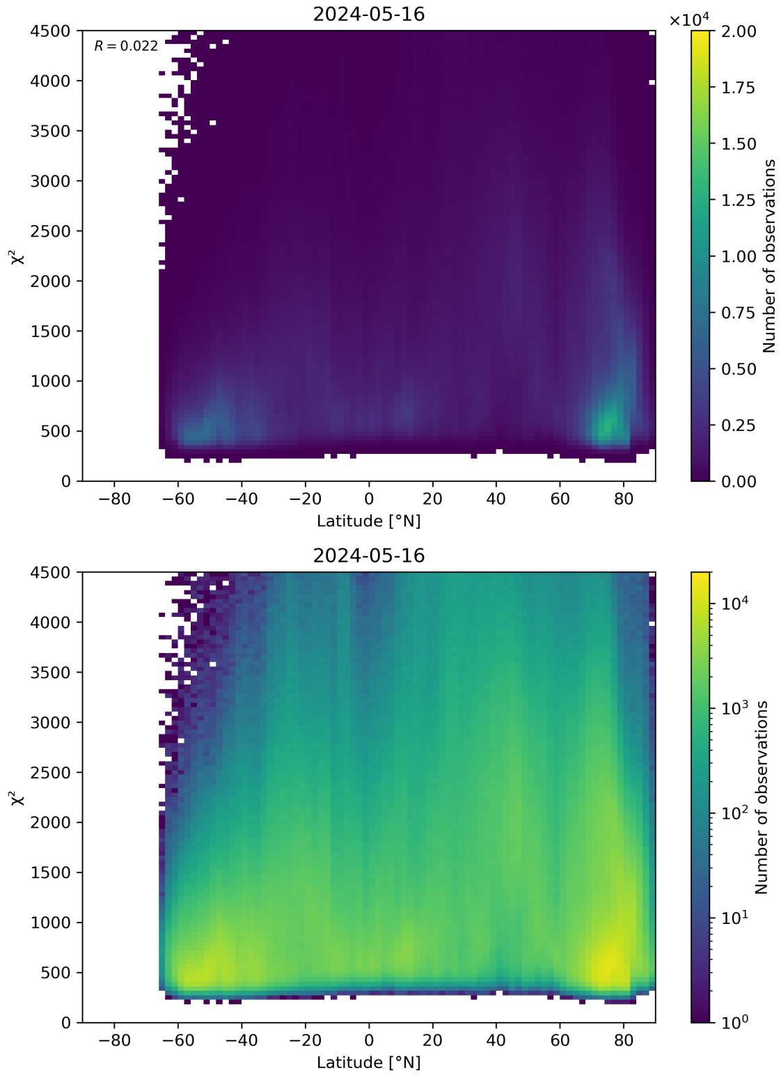
Figure 54: Scatter density plot of “Latitude” against “ \chi^2 ” for 2024-05-15 to 2024-05-17.
