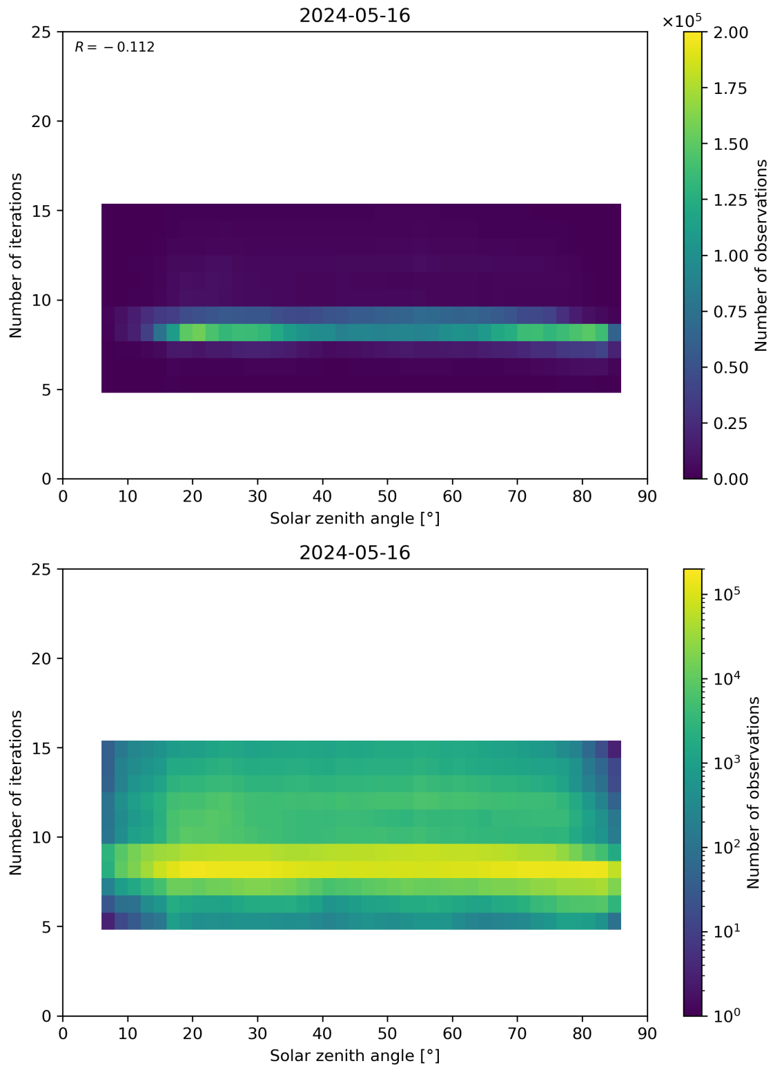
Figure 67: Scatter density plot of “Solar zenith angle” against “Number of iterations” for 2024-05-15 to 2024-05-17.
