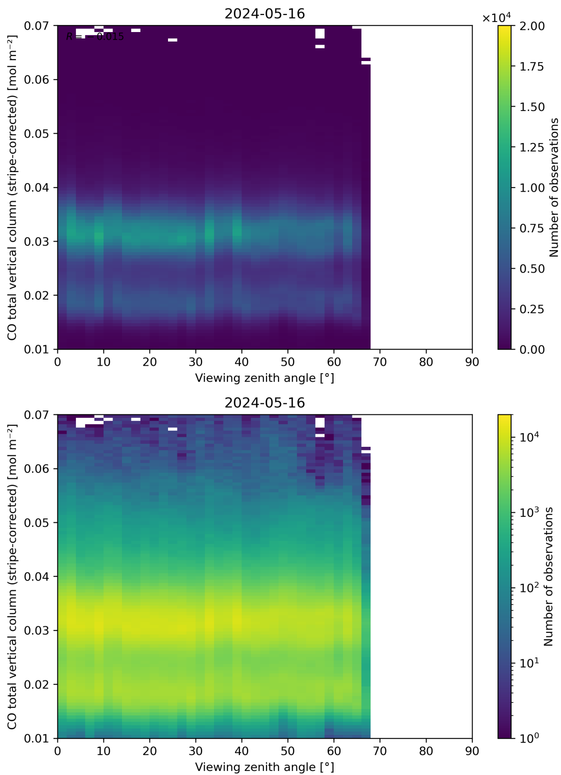
Figure 70: Scatter density plot of “Viewing zenith angle” against “CO total vertical column (stripe-corrected)” for 2024-05-15 to 2024-05-17.
