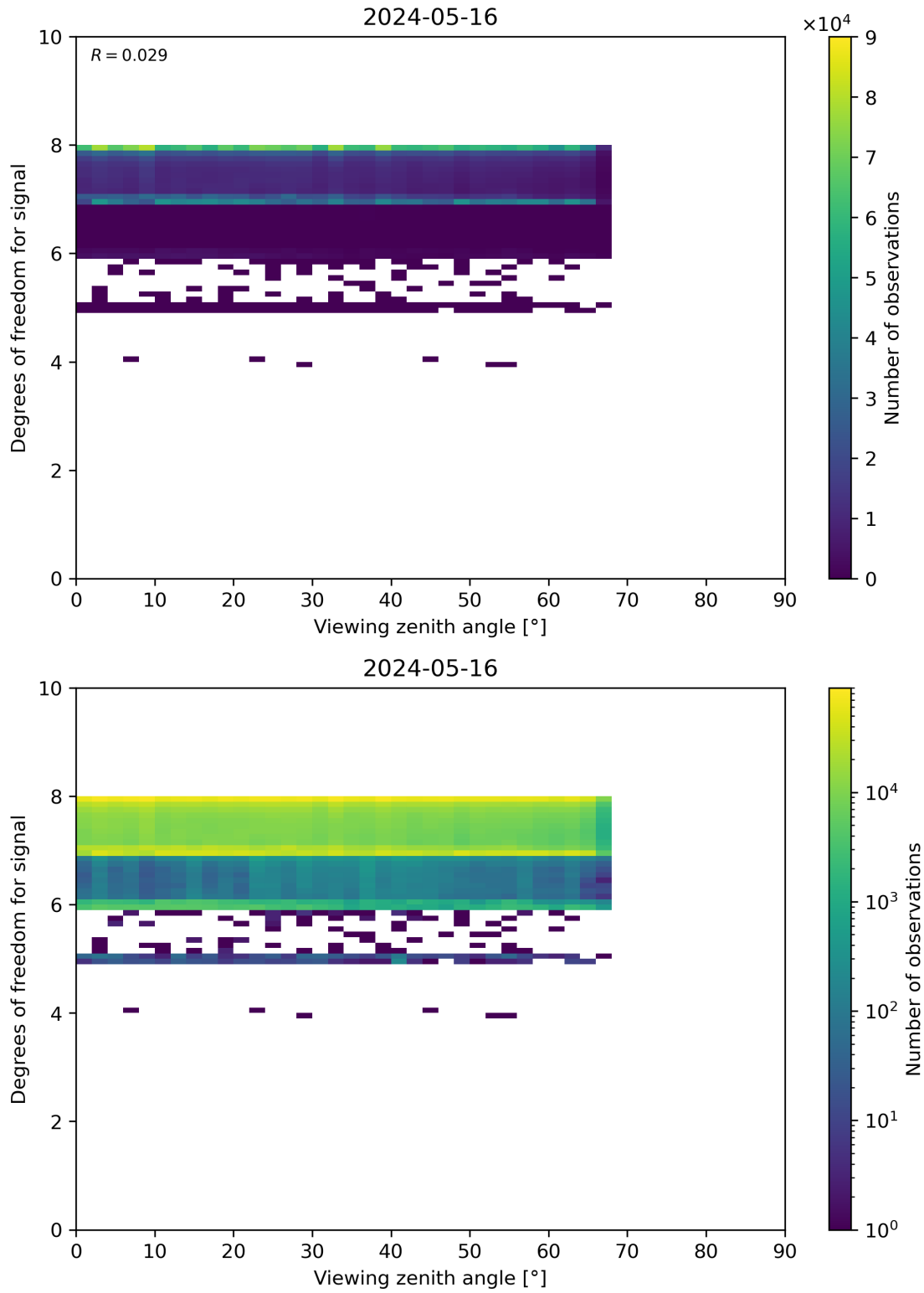
Figure 73: Scatter density plot of “Viewing zenith angle” against “Degrees of freedom for signal” for 2024-05-15 to 2024-05-17.
