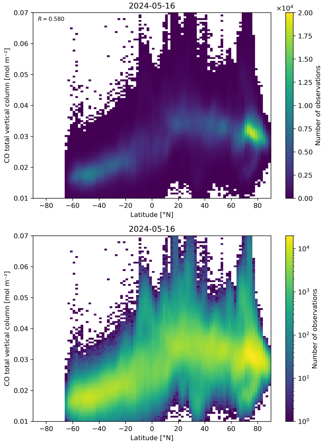
Figure 51: Scatter density plot of “Latitude” against “CO total vertical column” for 2024-05-15 to 2024-05-17.
