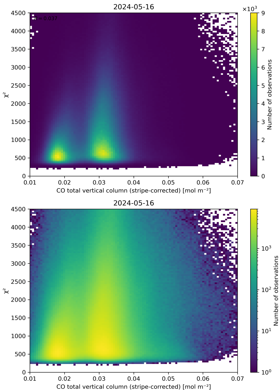
Figure 37: Scatter density plot of “CO total vertical column (stripe-corrected)” against “ \chi^2 ” for 2024-05-15 to 2024-05-17.
