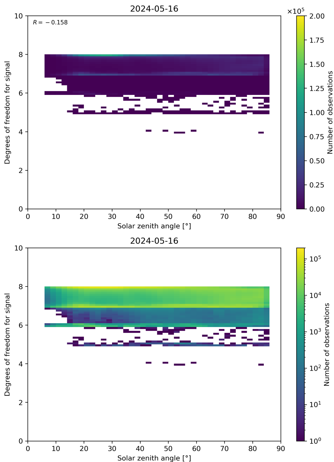
Figure 65: Scatter density plot of “Solar zenith angle” against “Degrees of freedom for signal” for 2024-05-15 to 2024-05-17.
