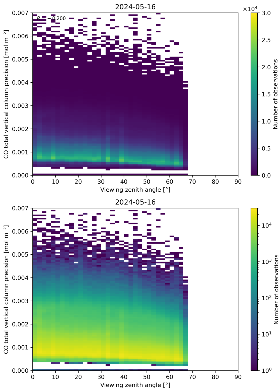
Figure 71: Scatter density plot of “Viewing zenith angle” against “CO total vertical column precision” for 2024-05-15 to 2024-05-17.
