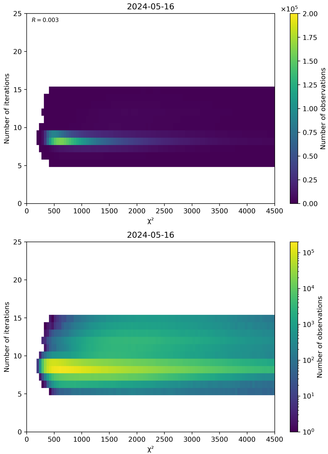
Figure 49: Scatter density plot of “ \chi^2 ” against “Number of iterations” for 2024-05-15 to 2024-05-17.
