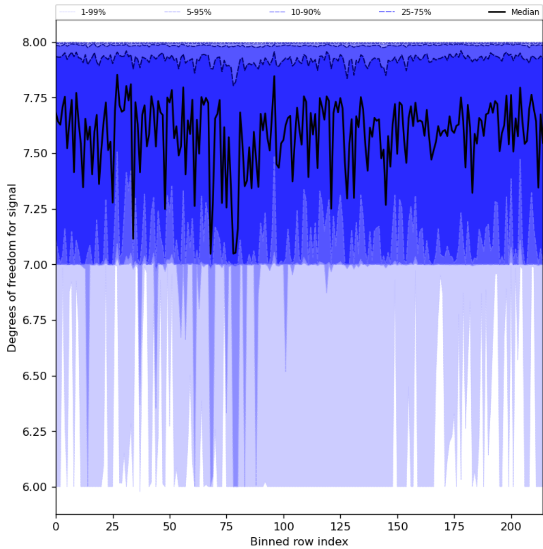
Figure 31: Along track statistics of “Degrees of freedom for signal” for 2024-05-15 to 2024-05-17
