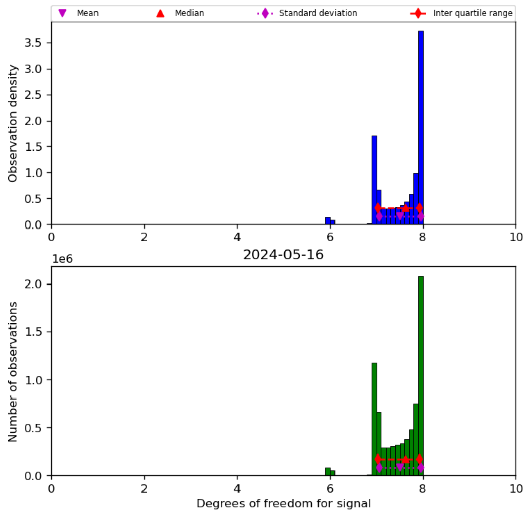
Figure 23: Histogram of “Degrees of freedom for signal” for 2024-05-15 to 2024-05-17
