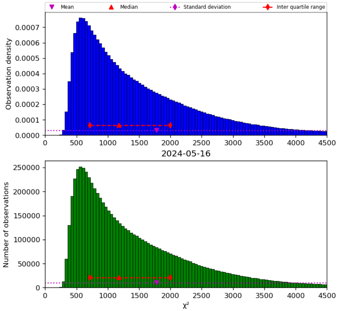
Figure 22: Histogram of “ \chi^2 ” for 2024-05-15 to 2024-05-17
