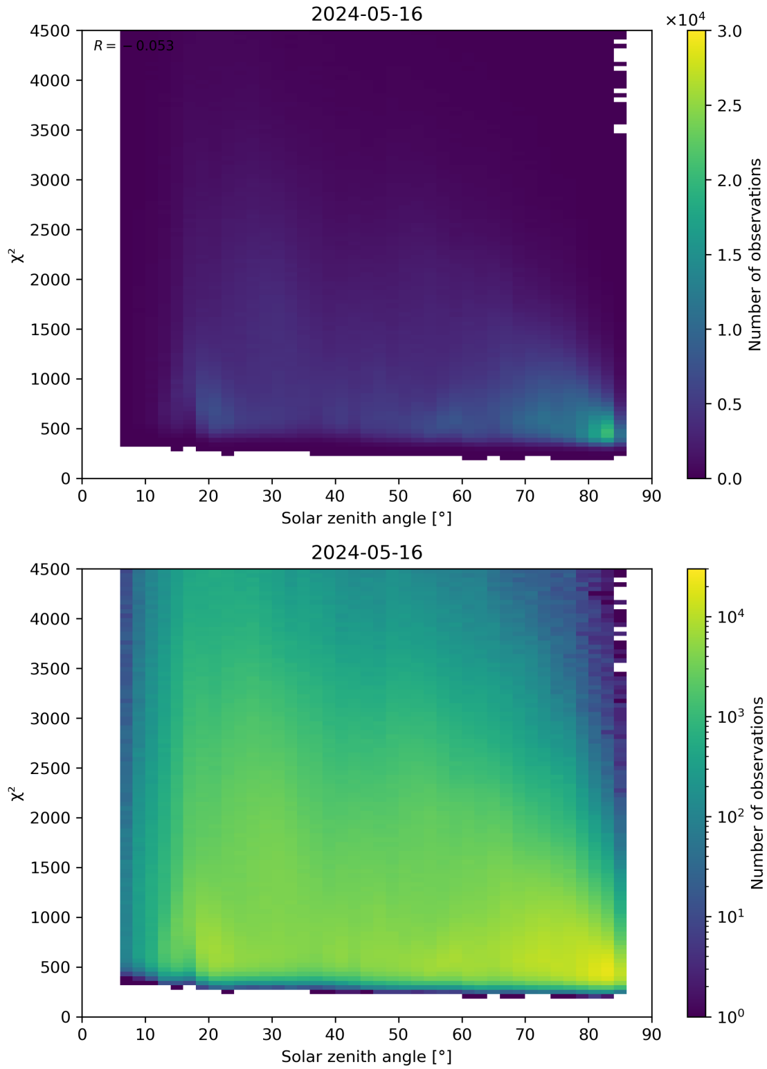
Figure 64: Scatter density plot of “Solar zenith angle” against “ \chi^2 ” for 2024-05-15 to 2024-05-17.
