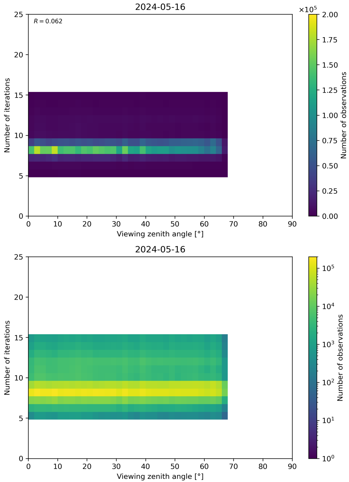
Figure 75: Scatter density plot of “Viewing zenith angle” against “Number of iterations” for 2024-05-15 to 2024-05-17.
