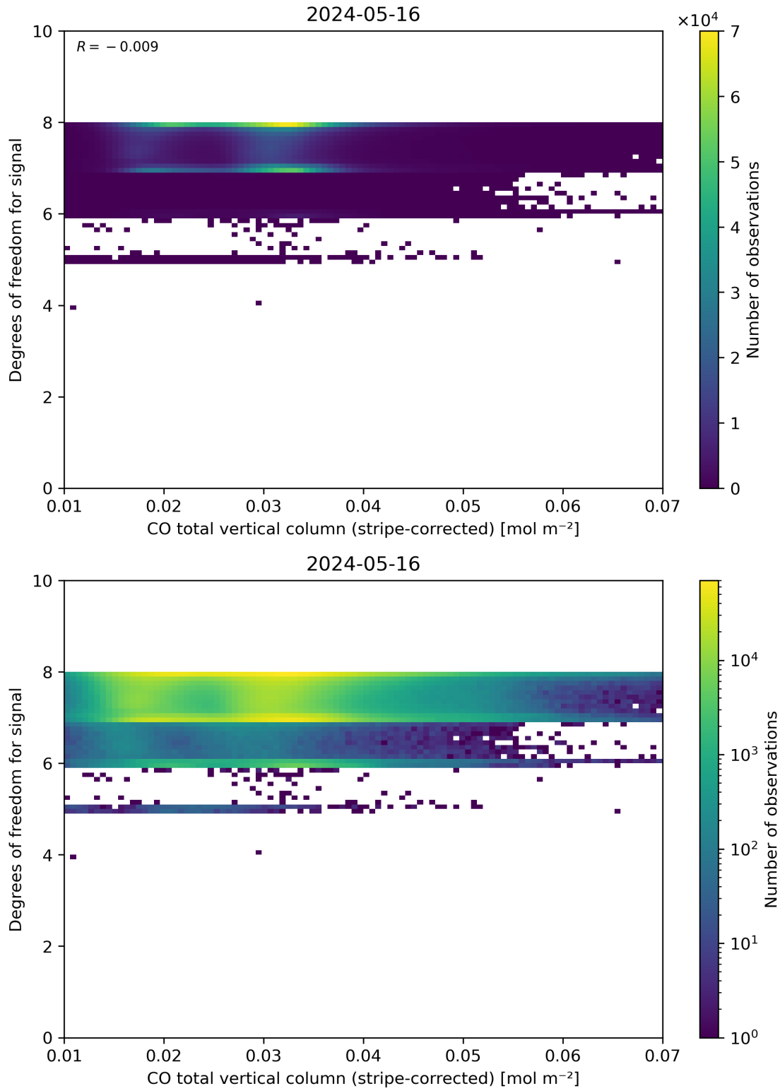
Figure 38: Scatter density plot of “CO total vertical column (stripe-corrected)” against “Degrees of freedom for signal” for 2024-05-15 to 2024-05-17.
