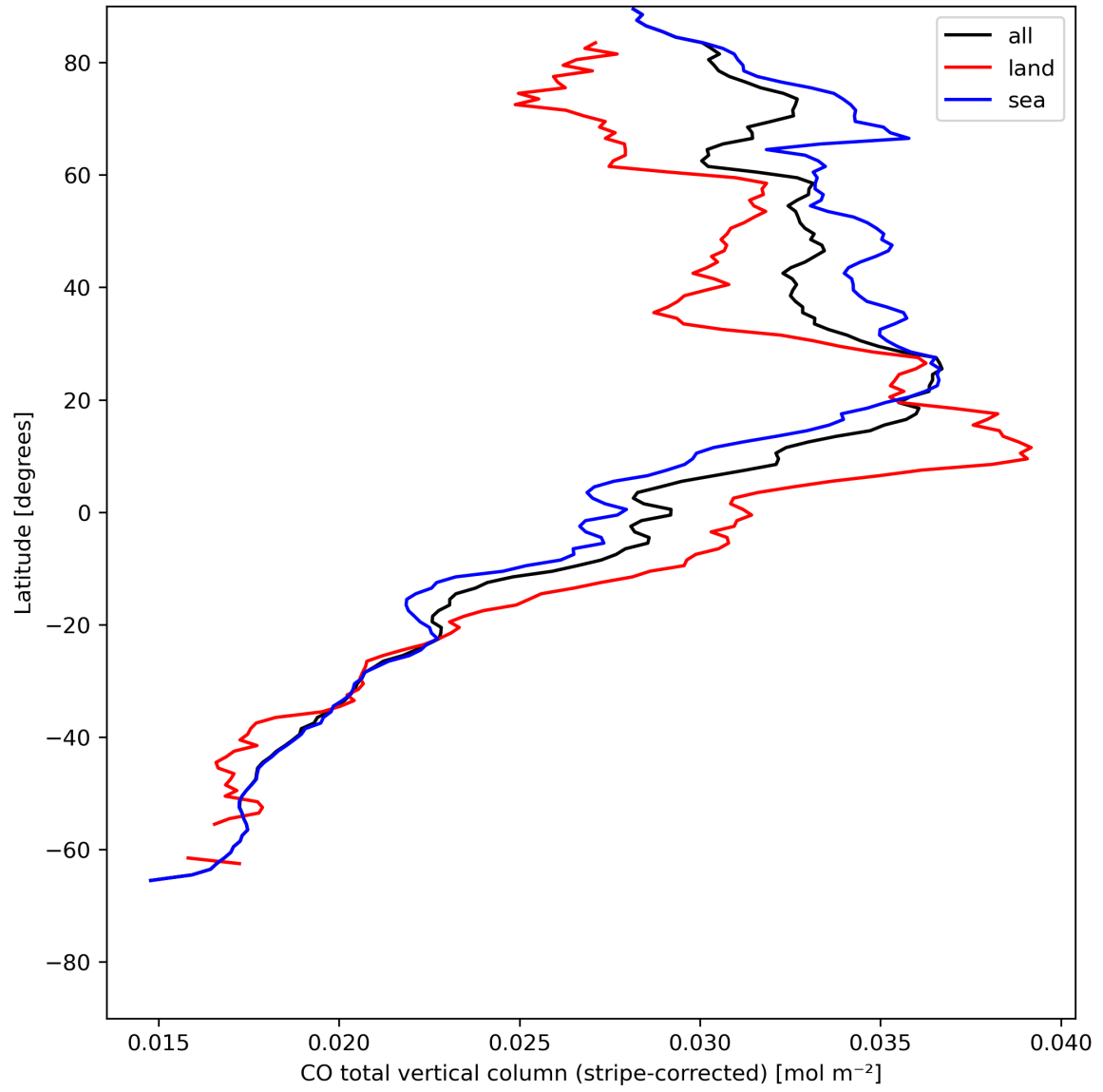
Figure 11: Zonal average of “CO total vertical column (stripe-corrected)” for 2024-05-15 to 2024-05-17.
