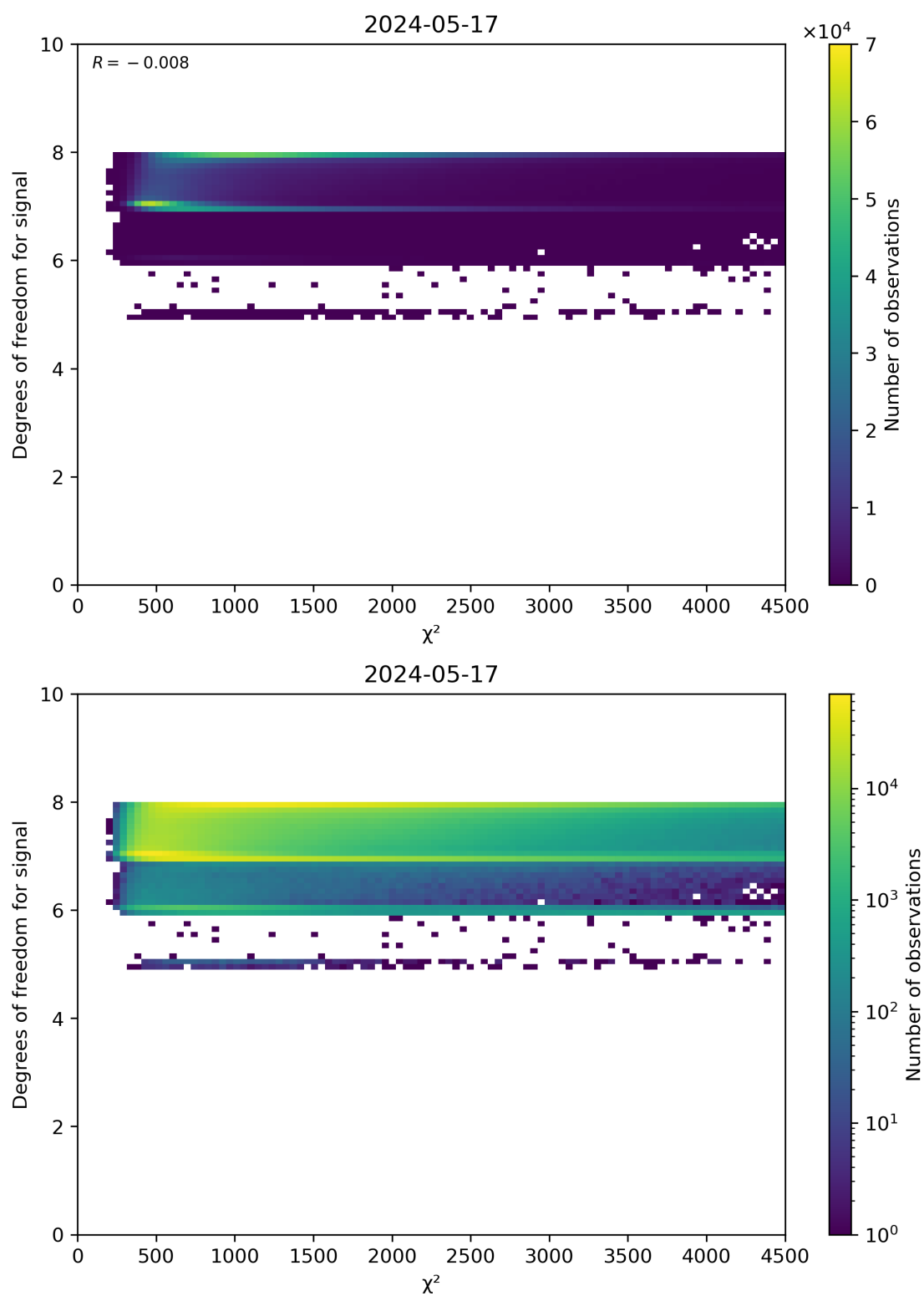
Figure 48: Scatter density plot of “ \chi^2 ” against “Degrees of freedom for signal” for 2024-05-16 to 2024-05-18.
