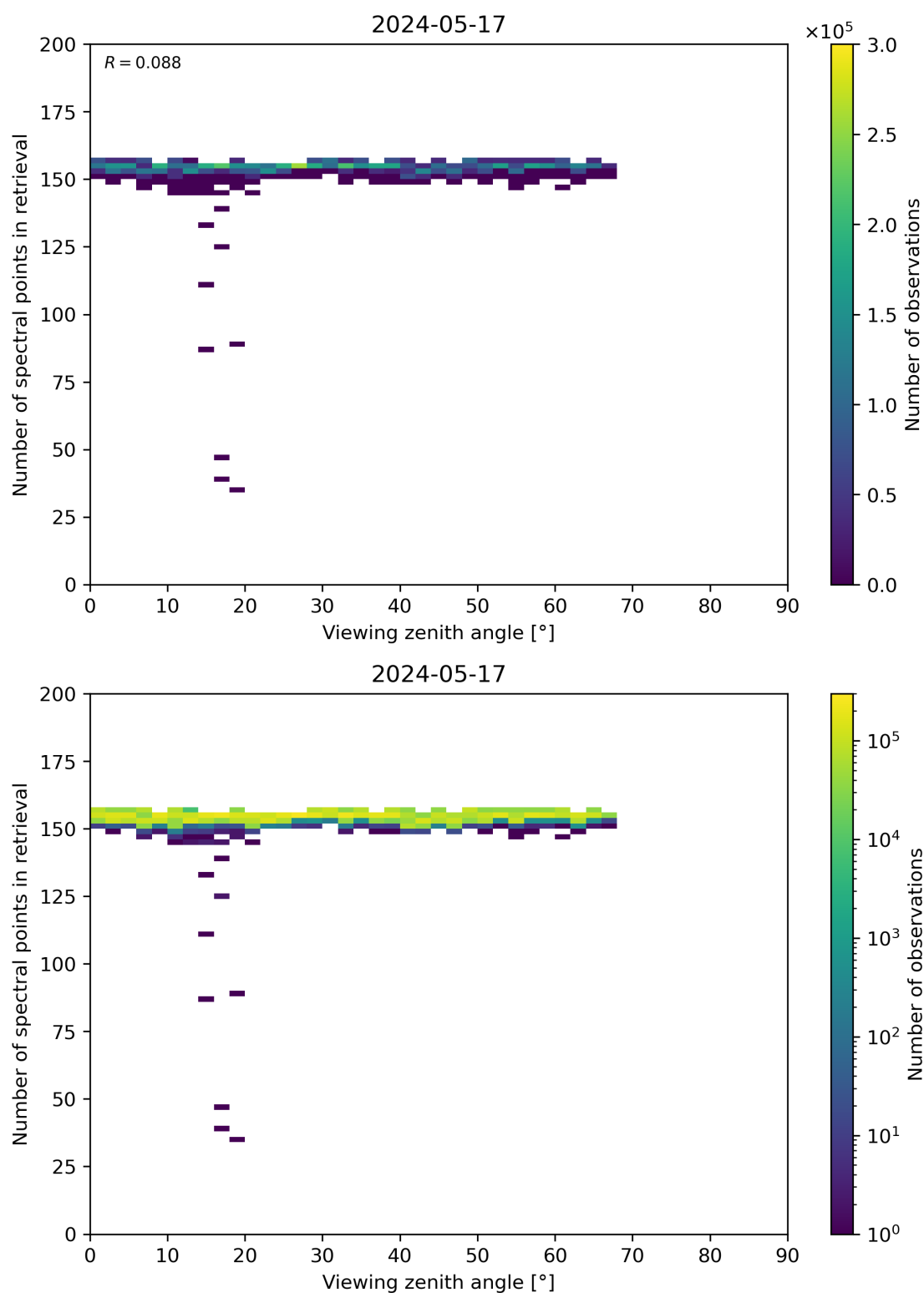
Figure 76: Scatter density plot of “Viewing zenith angle” against “Number of spectral points in retrieval” for 2024-05-16 to 2024-05-18.
