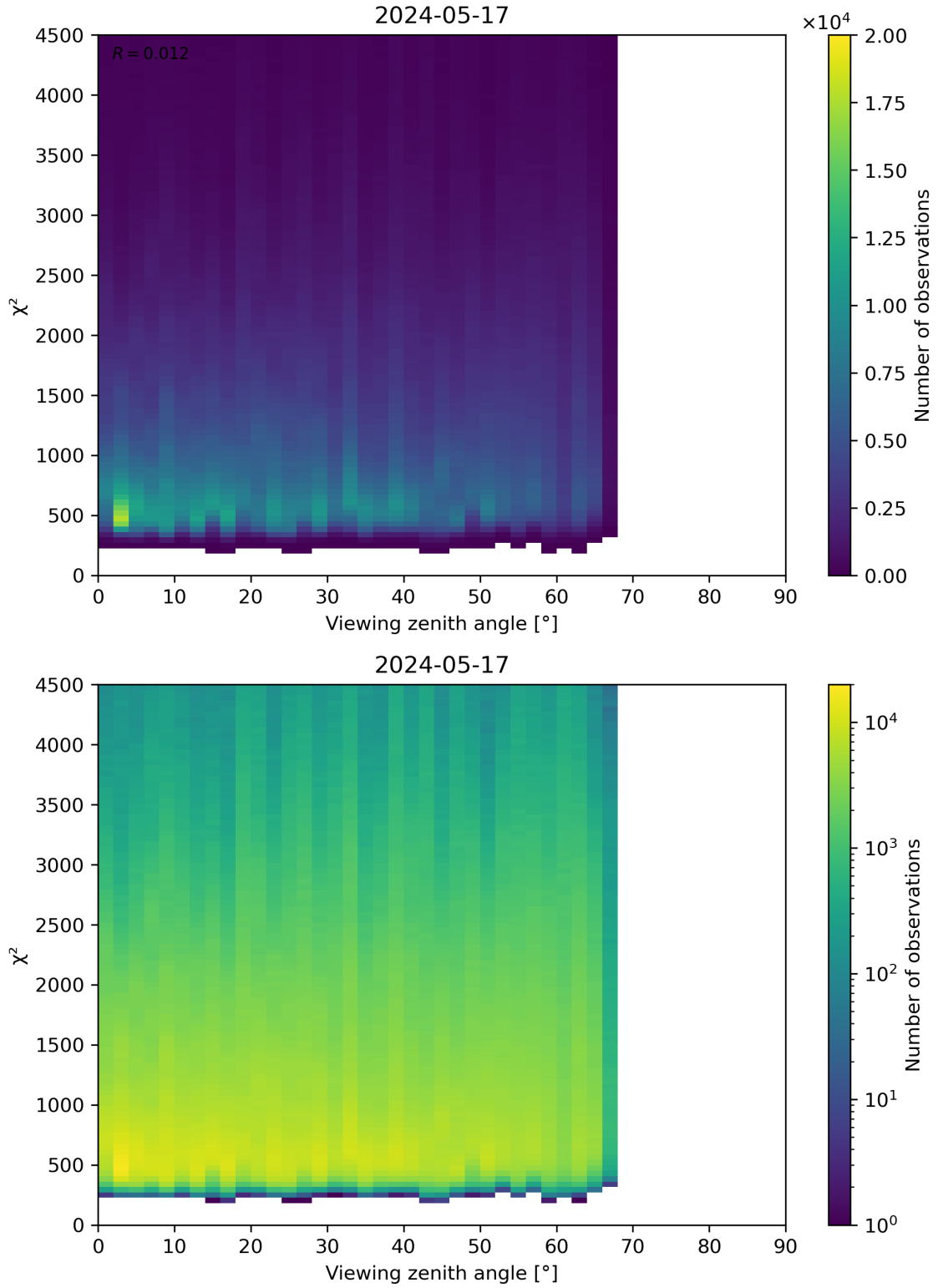
Figure 72: Scatter density plot of “Viewing zenith angle” against “ \chi^2 ” for 2024-05-16 to 2024-05-18.
