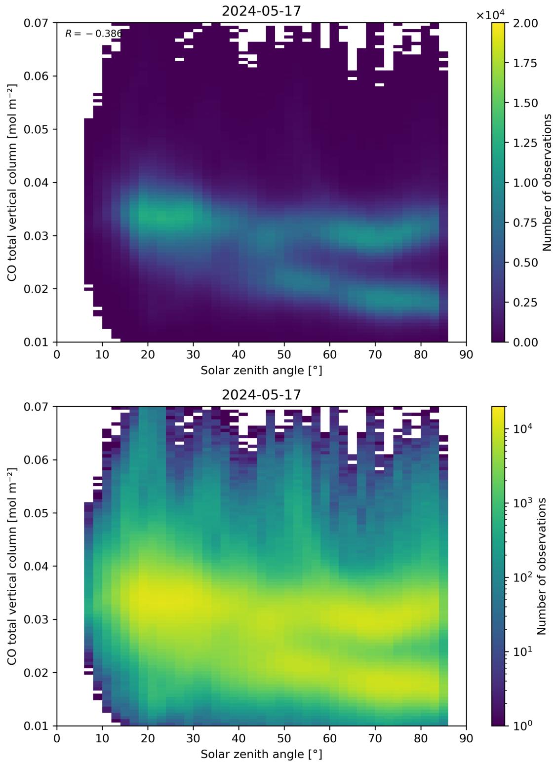
Figure 61: Scatter density plot of “Solar zenith angle” against “CO total vertical column” for 2024-05-16 to 2024-05-18.
