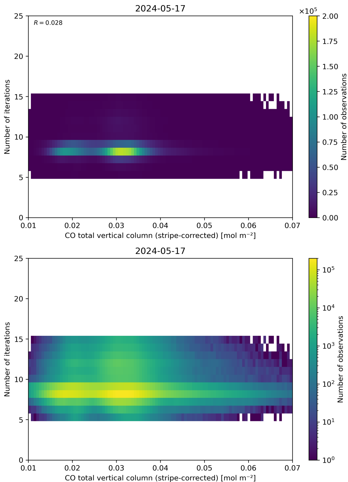
Figure 39: Scatter density plot of “CO total vertical column (stripe-corrected)” against “Number of iterations” for 2024-05-16 to 2024-05-18.
