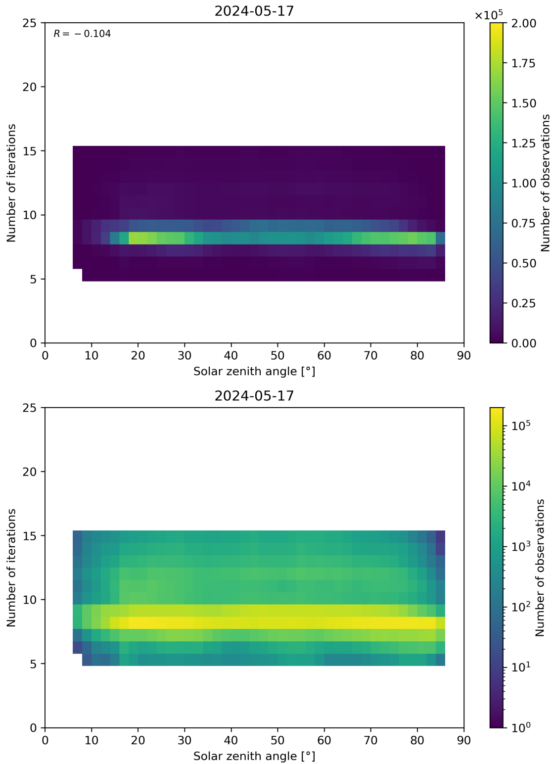
Figure 67: Scatter density plot of “Solar zenith angle” against “Number of iterations” for 2024-05-16 to 2024-05-18.
