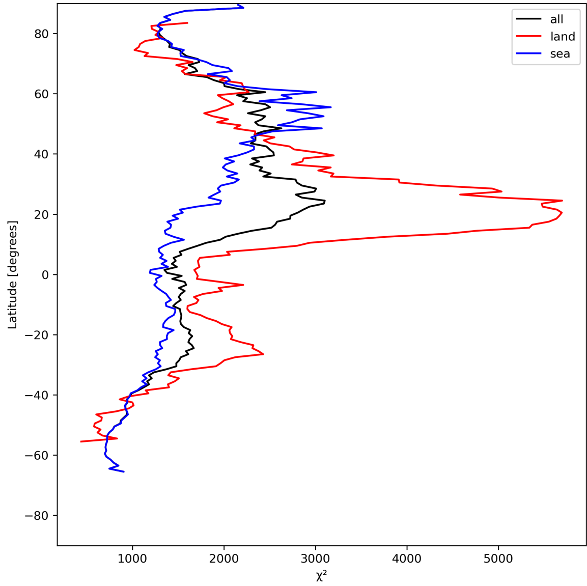
Figure 14: Zonal average of “ \chi^2 ” for 2024-05-16 to 2024-05-18.
