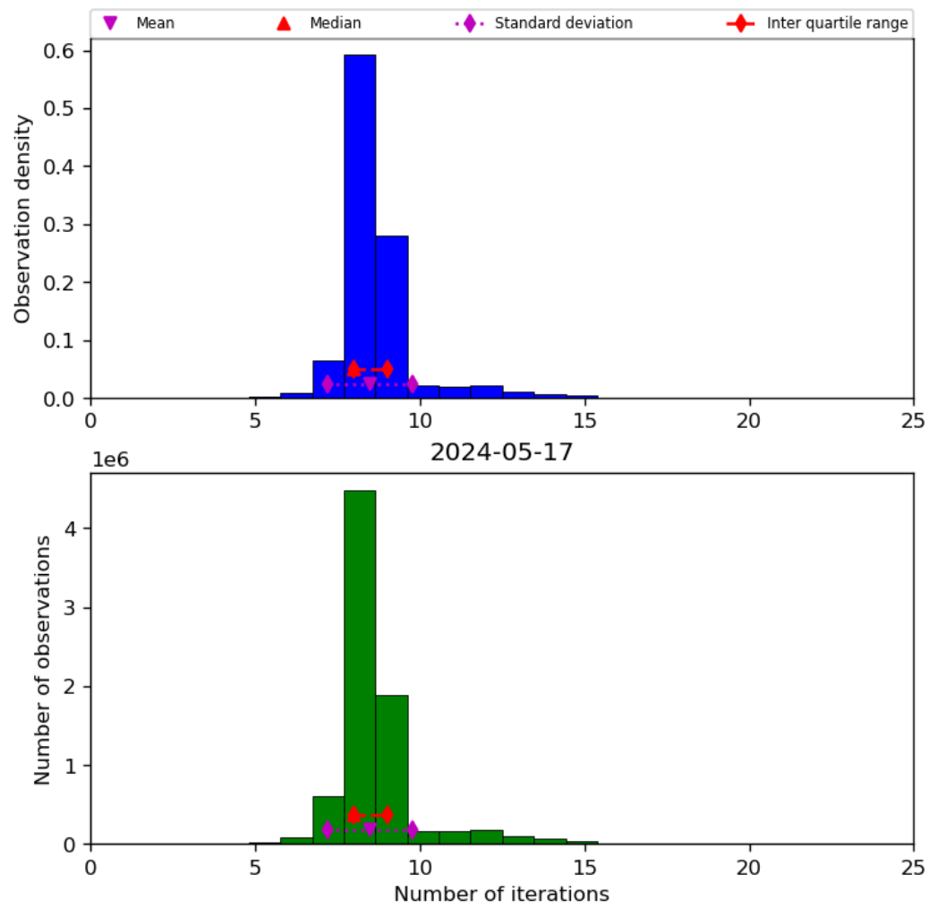
Figure 24: Histogram of “Number of iterations” for 2024-05-16 to 2024-05-18
