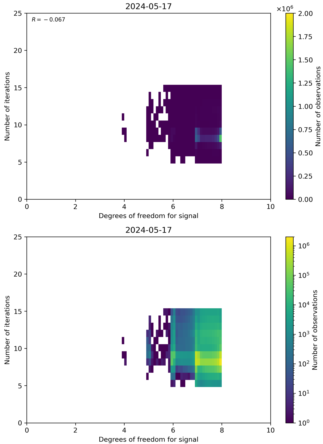
Figure 50: Scatter density plot of “Degrees of freedom for signal” against “Number of iterations” for 2024-05-16 to 2024-05-18.
