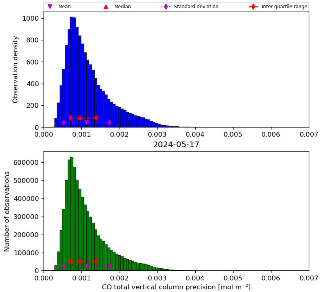
Figure 20: Histogram of “CO total vertical column precision” for 2024-05-16 to 2024-05-18
