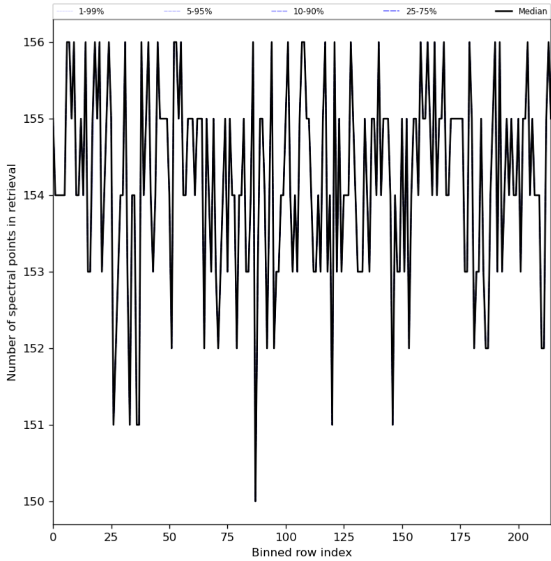
Figure 29: Along track statistics of “Number of spectral points in retrieval” for 2024-05-16 to 2024-05-18
