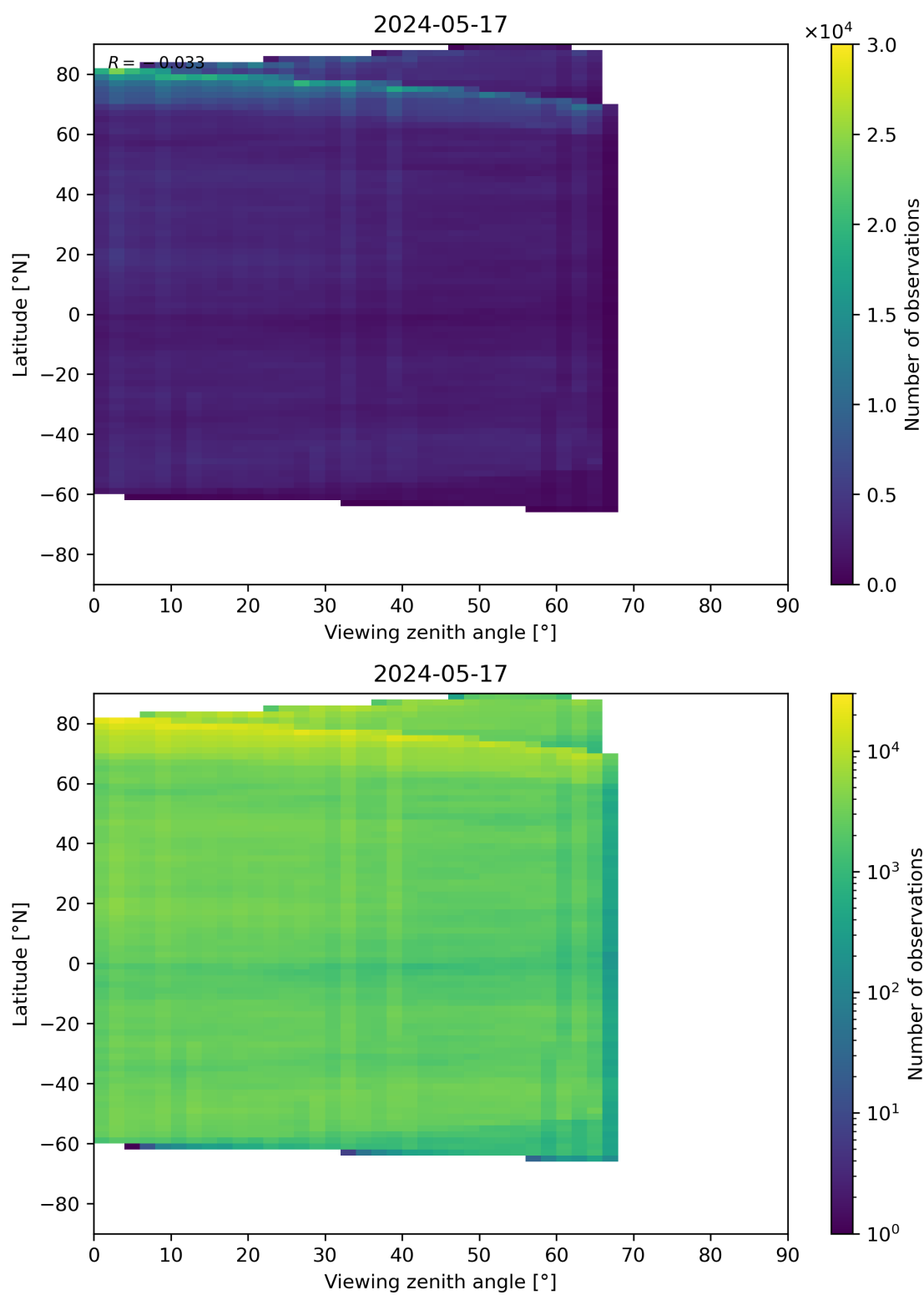
Figure 74: Scatter density plot of “Viewing zenith angle” against “Latitude” for 2024-05-16 to 2024-05-18.
