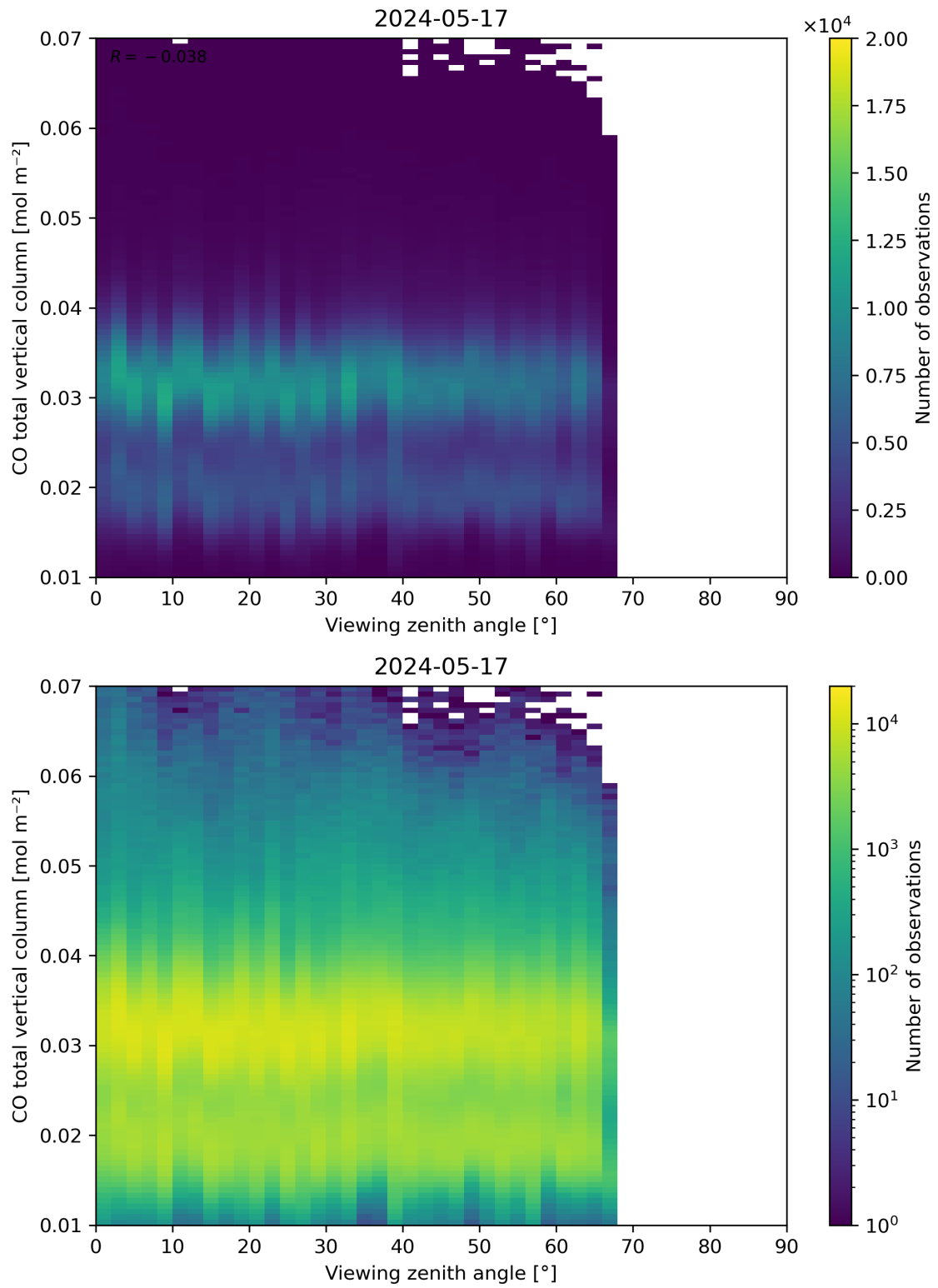
Figure 69: Scatter density plot of “Viewing zenith angle” against “CO total vertical column” for 2024-05-16 to 2024-05-18.
