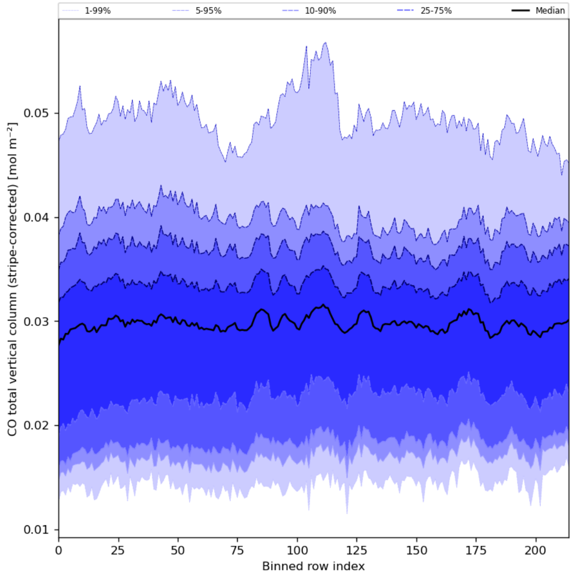
Figure 27: Along track statistics of “CO total vertical column (stripe-corrected)” for 2024-05-16 to 2024-05-18
