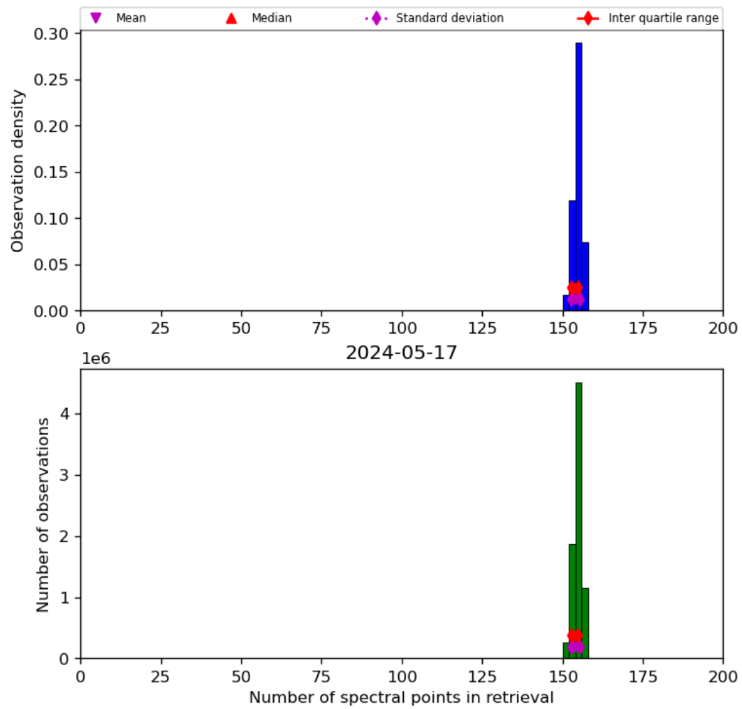
Figure 21: Histogram of “Number of spectral points in retrieval” for 2024-05-16 to 2024-05-18
