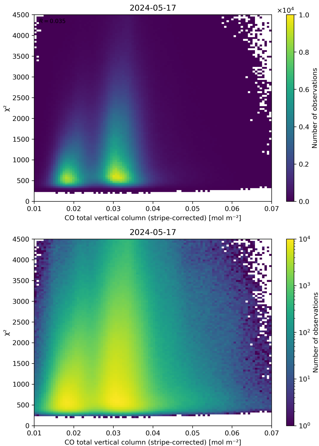
Figure 37: Scatter density plot of “CO total vertical column (stripe-corrected)” against “ \chi^2 ” for 2024-05-16 to 2024-05-18.
