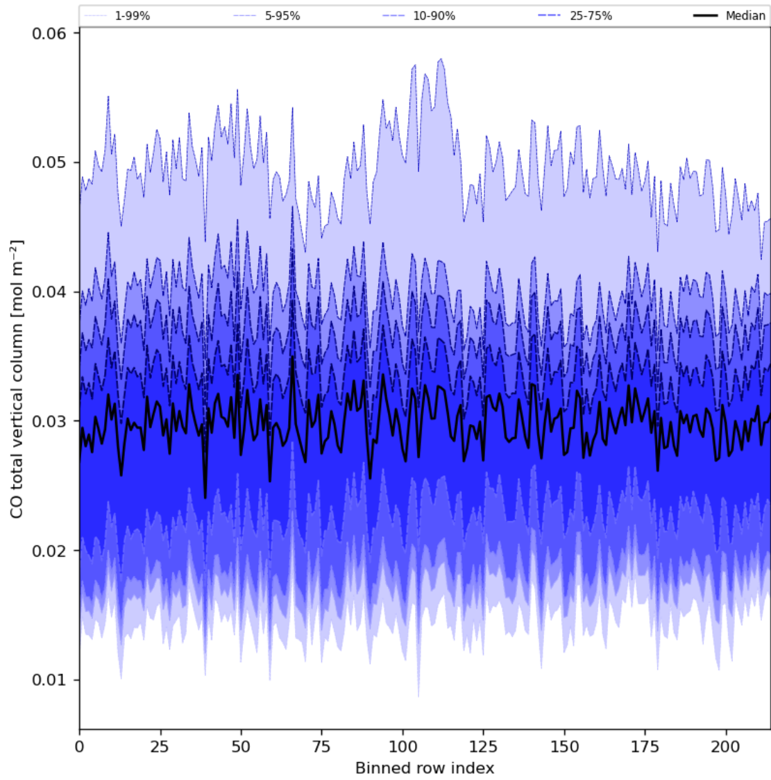
Figure 26: Along track statistics of “CO total vertical column” for 2024-05-16 to 2024-05-18
