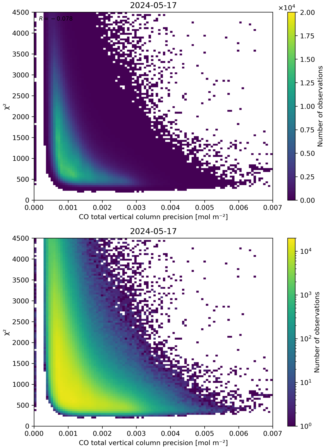
Figure 44: Scatter density plot of “CO total vertical column precision” against “ \chi^2 ” for 2024-05-16 to 2024-05-18.
