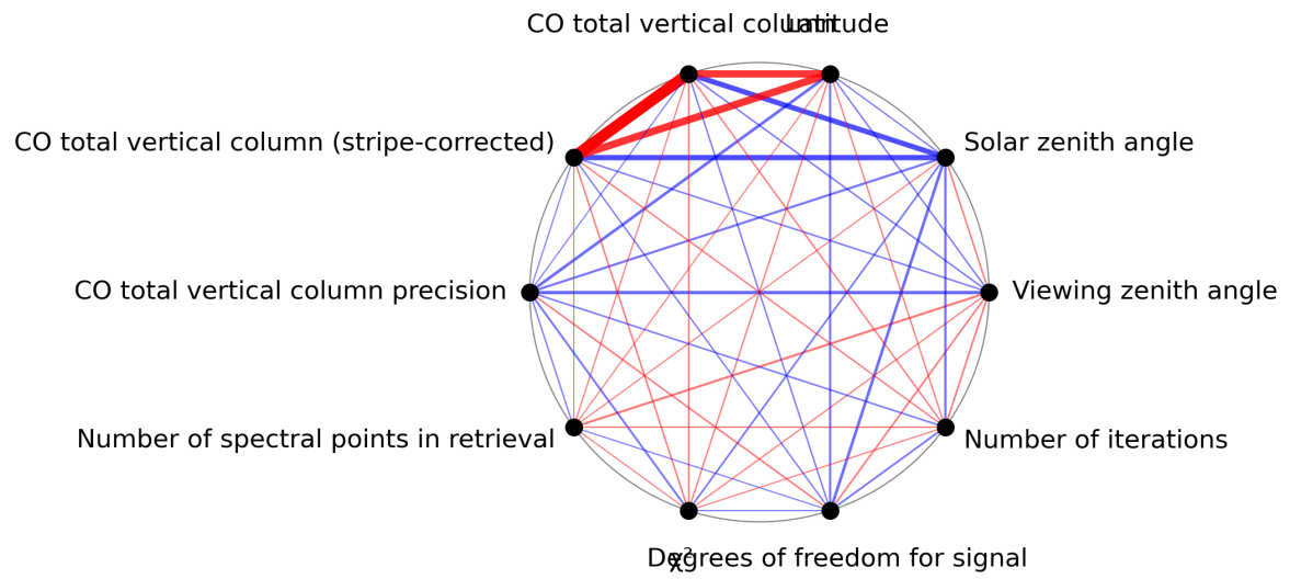
Figure 1: Map of correlation graph for 2024-05-16 to 2024-05-18.
