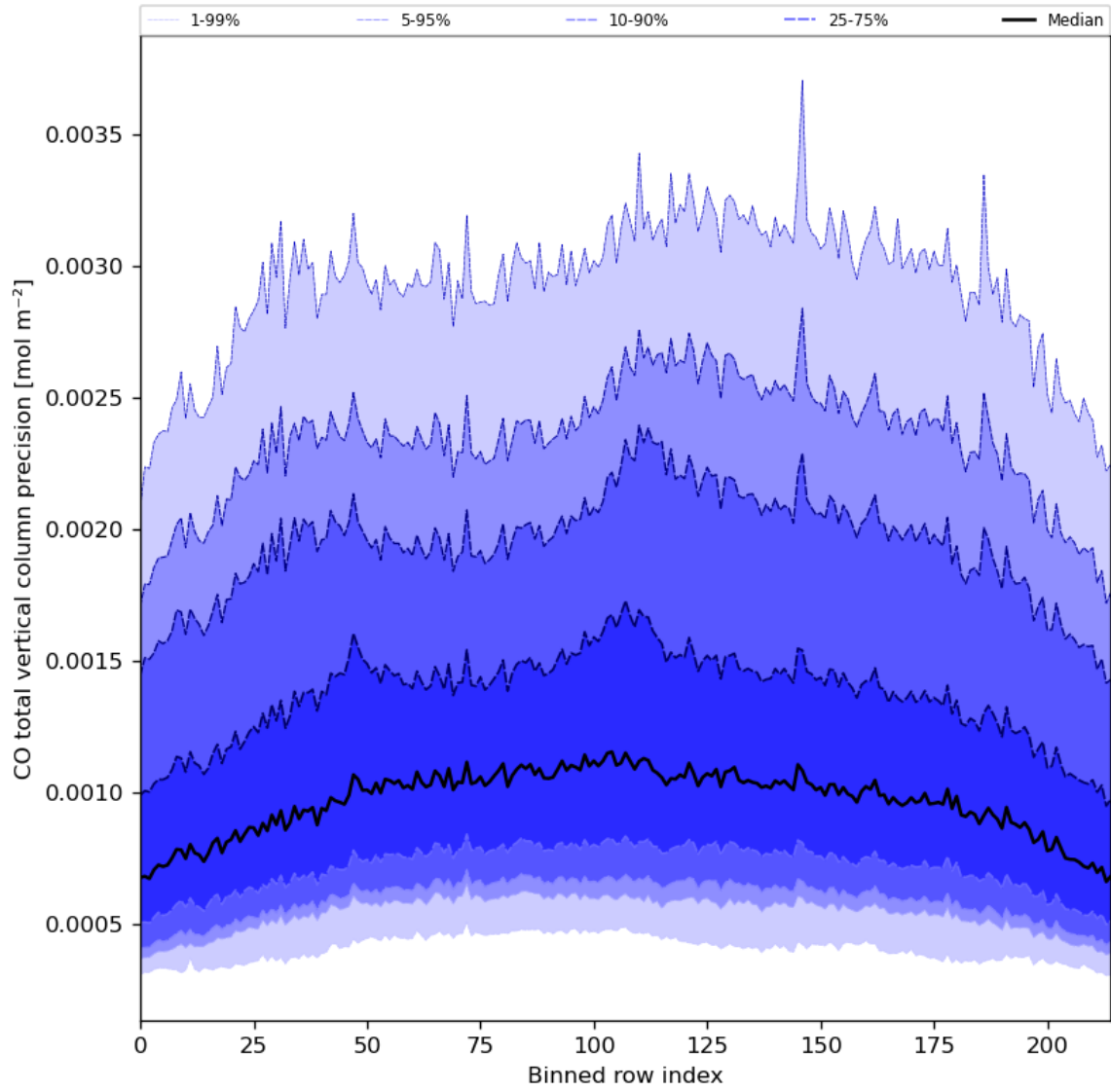
Figure 28: Along track statistics of “CO total vertical column precision” for 2024-05-16 to 2024-05-18
