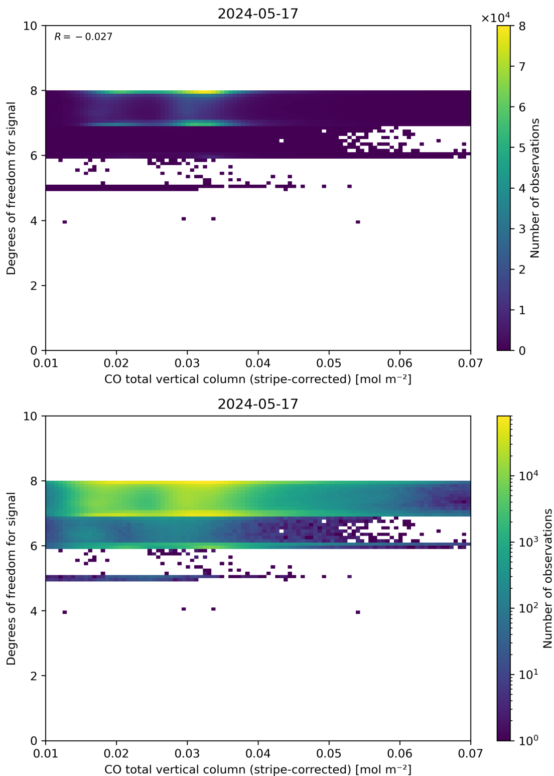
Figure 38: Scatter density plot of “CO total vertical column (stripe-corrected)” against “Degrees of freedom for signal” for 2024-05-16 to 2024-05-18.
