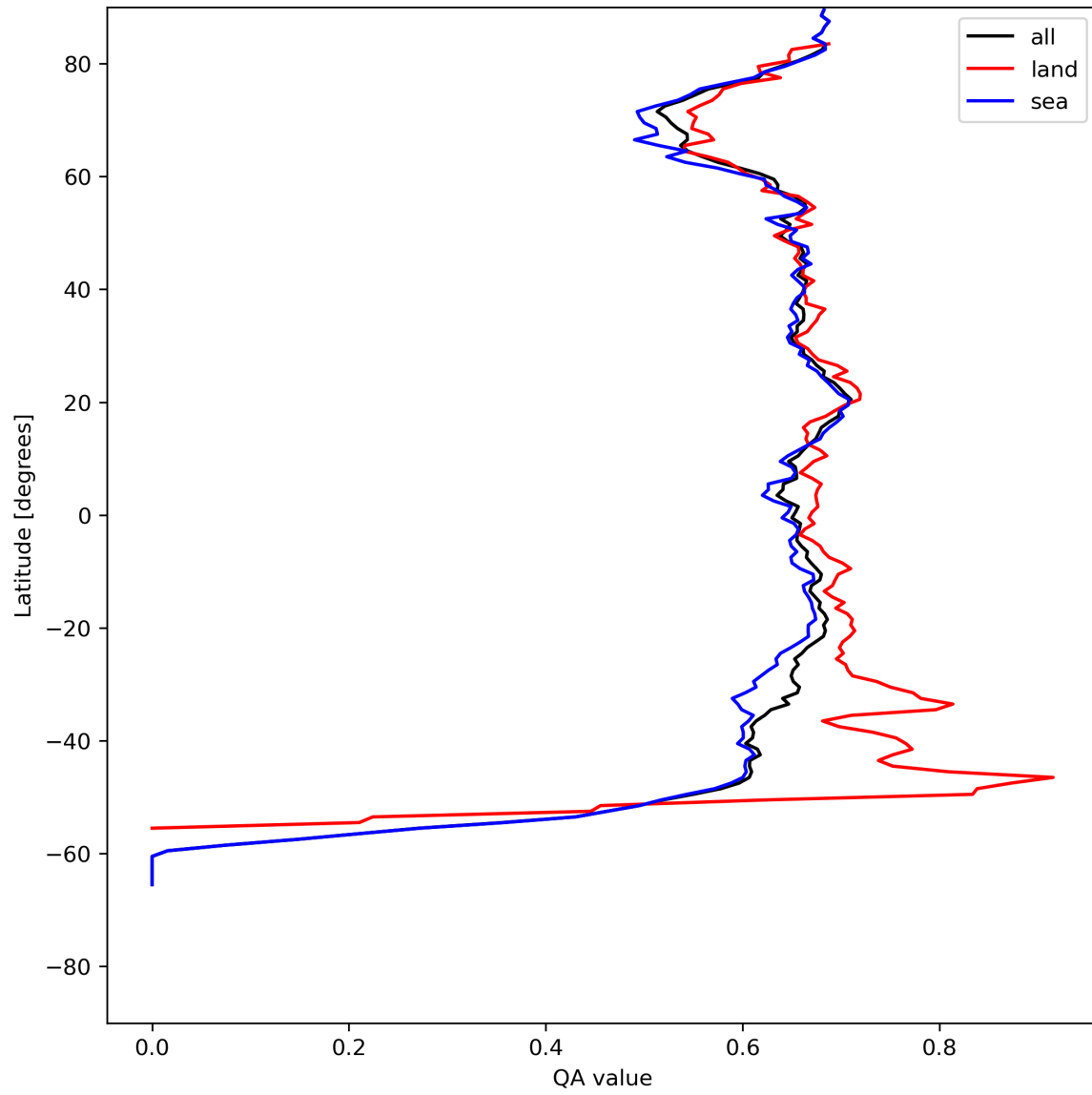
Figure 9: Zonal average of “QA value” for 2024-05-16 to 2024-05-18.
