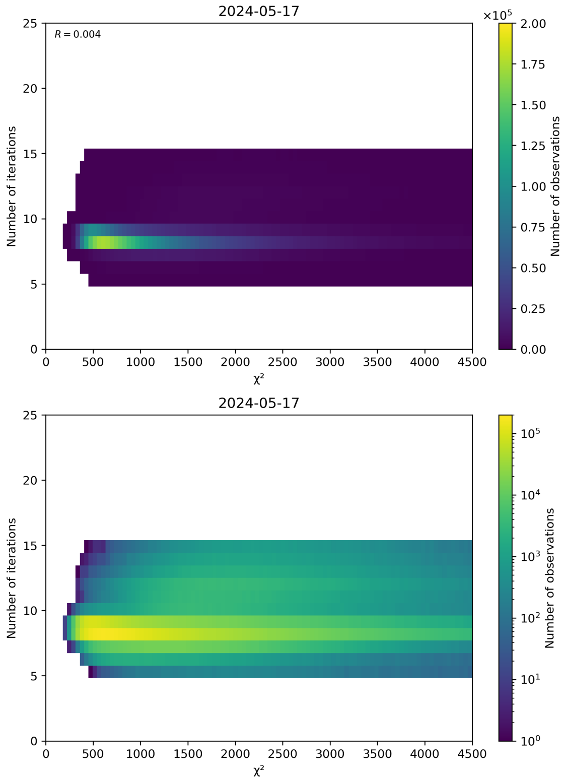
Figure 49: Scatter density plot of “ \chi^2 ” against “Number of iterations” for 2024-05-16 to 2024-05-18.
