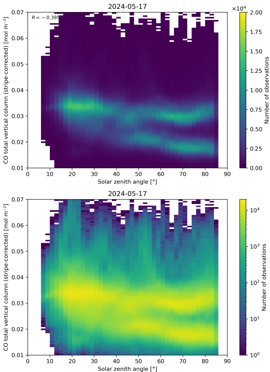
Figure 62: Scatter density plot of “Solar zenith angle” against “CO total vertical column (stripe-corrected)” for 2024-05-16 to 2024-05-18.
