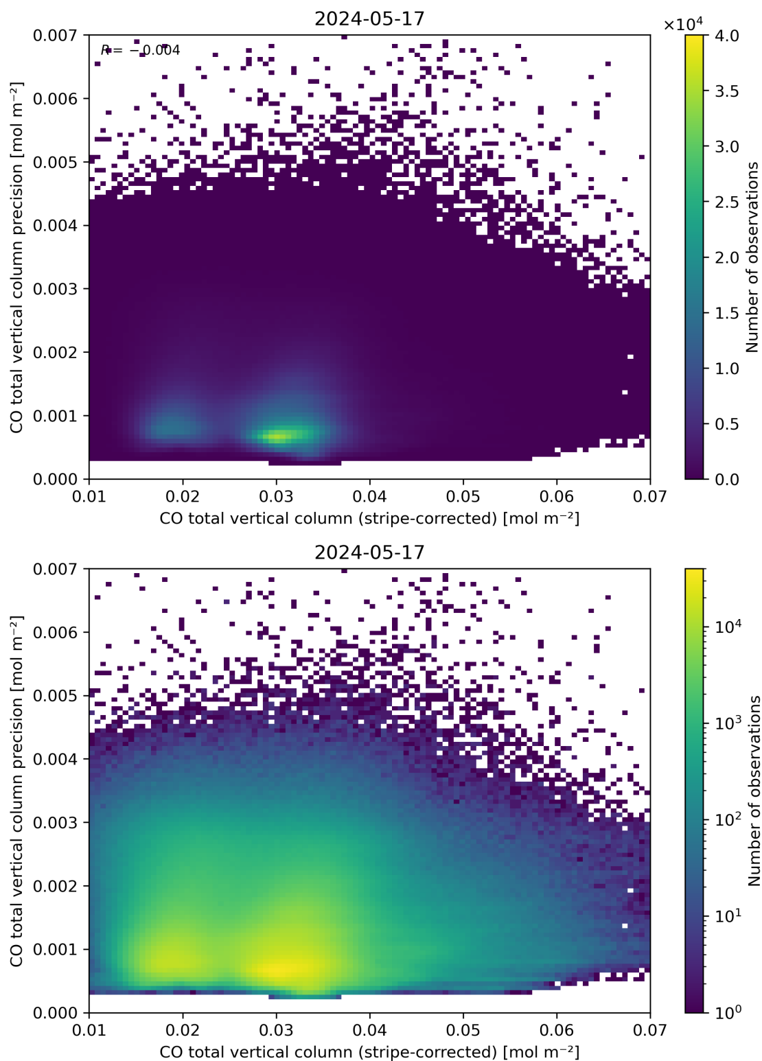
Figure 36: Scatter density plot of “CO total vertical column (stripe-corrected)” against “CO total vertical column precision” for 2024-05-16 to 2024-05-18.
