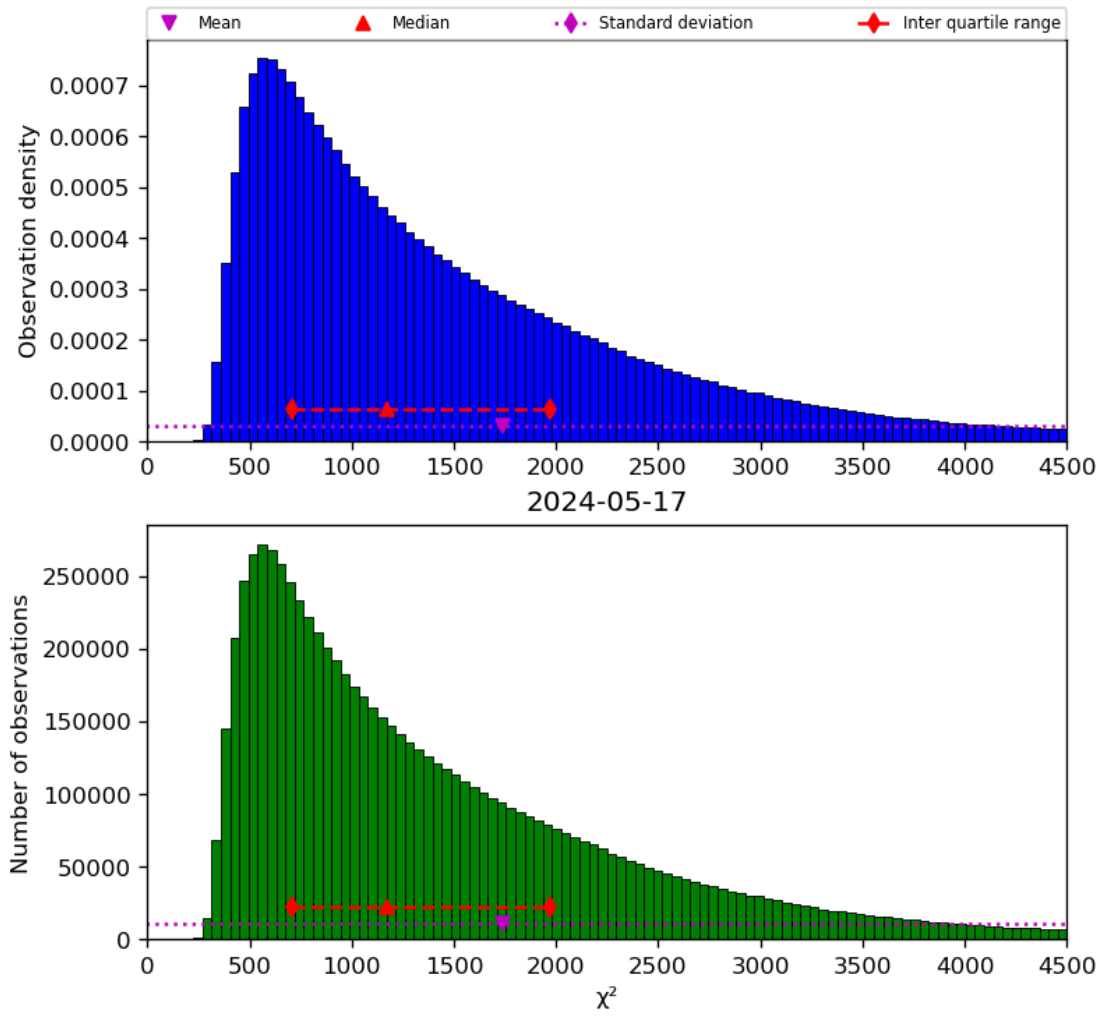
Figure 22: Histogram of “ \chi^2 ” for 2024-05-16 to 2024-05-18
