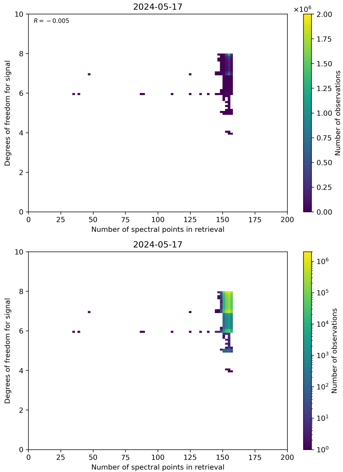
Figure 59: Scatter density plot of “Number of spectral points in retrieval” against “Degrees of freedom for signal” for 2024-05-16 to 2024-05-18.
