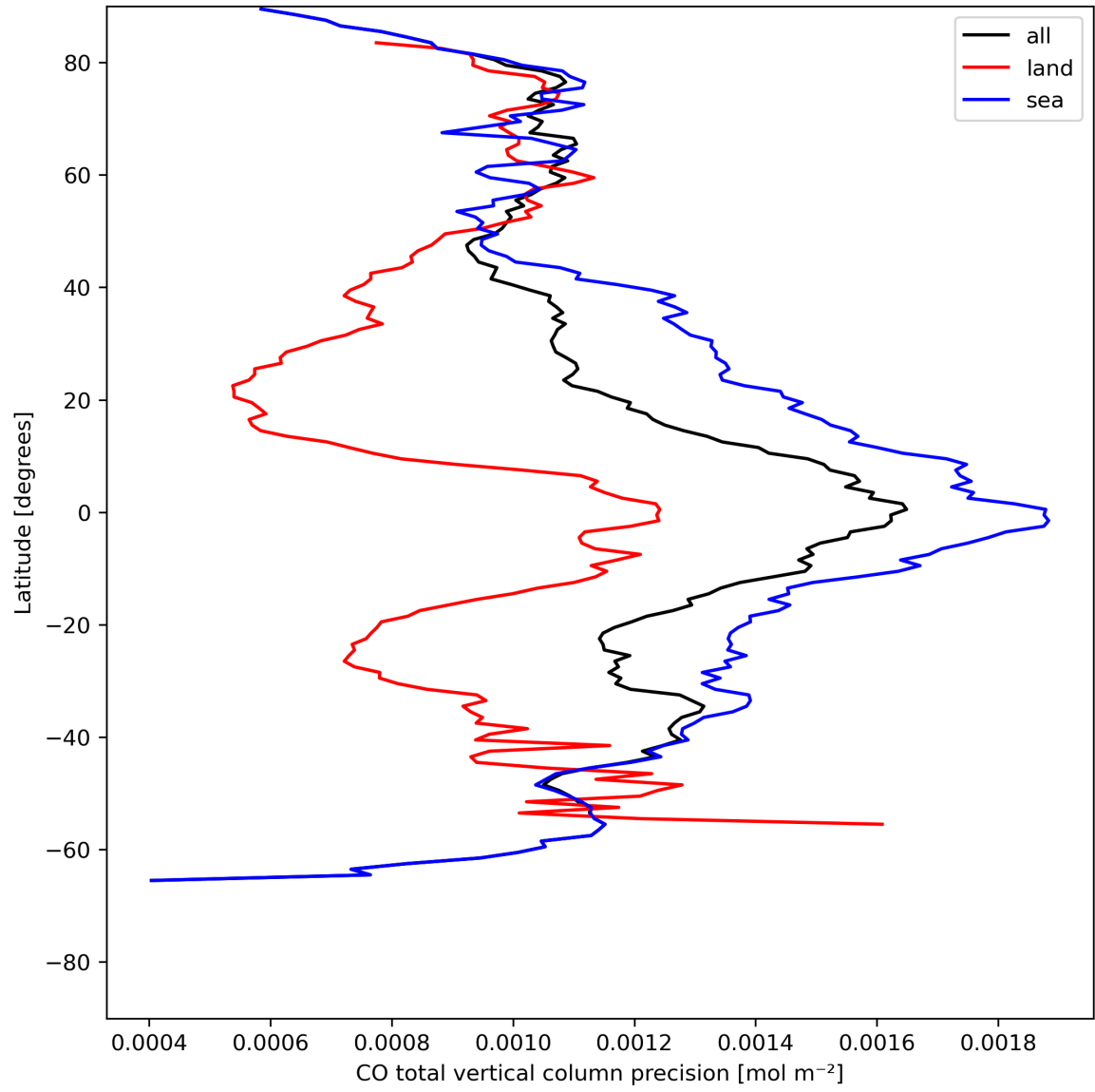
Figure 12: Zonal average of “CO total vertical column precision” for 2024-05-16 to 2024-05-18.
