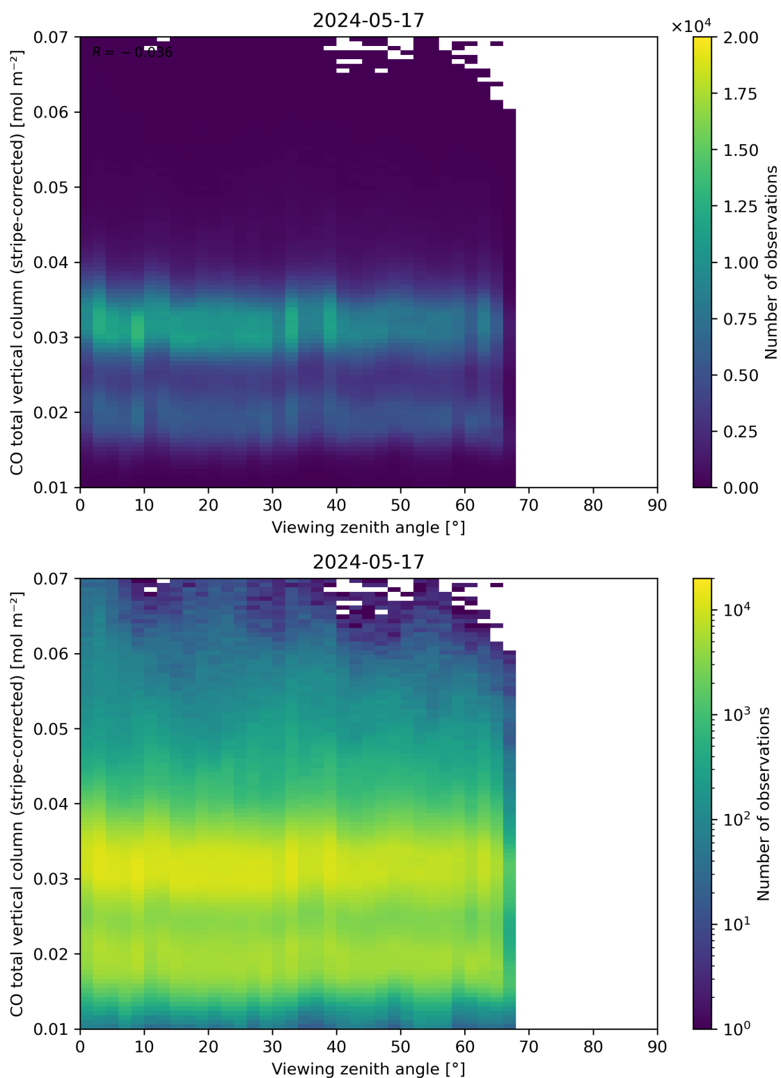
Figure 70: Scatter density plot of “Viewing zenith angle” against “CO total vertical column (stripe-corrected)” for 2024-05-16 to 2024-05-18.
