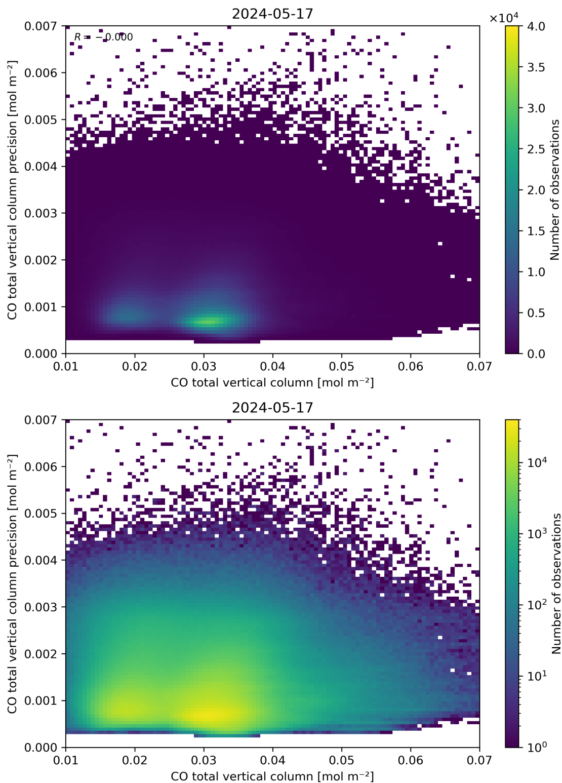
Figure 34: Scatter density plot of “CO total vertical column” against “CO total vertical column precision” for 2024-05-16 to 2024-05-18.
