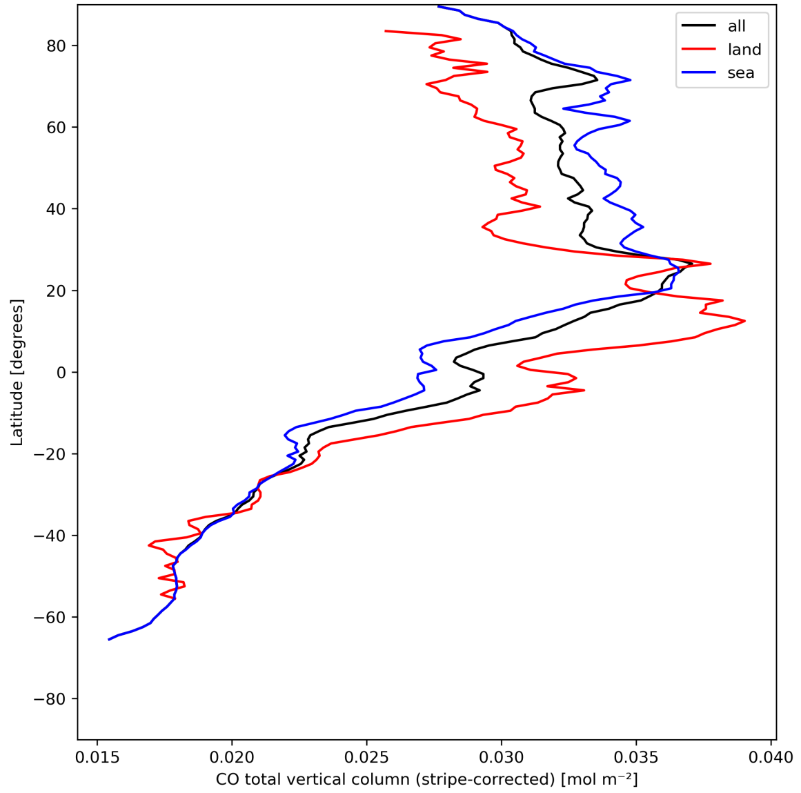
Figure 11: Zonal average of “CO total vertical column (stripe-corrected)” for 2024-05-16 to 2024-05-18.
