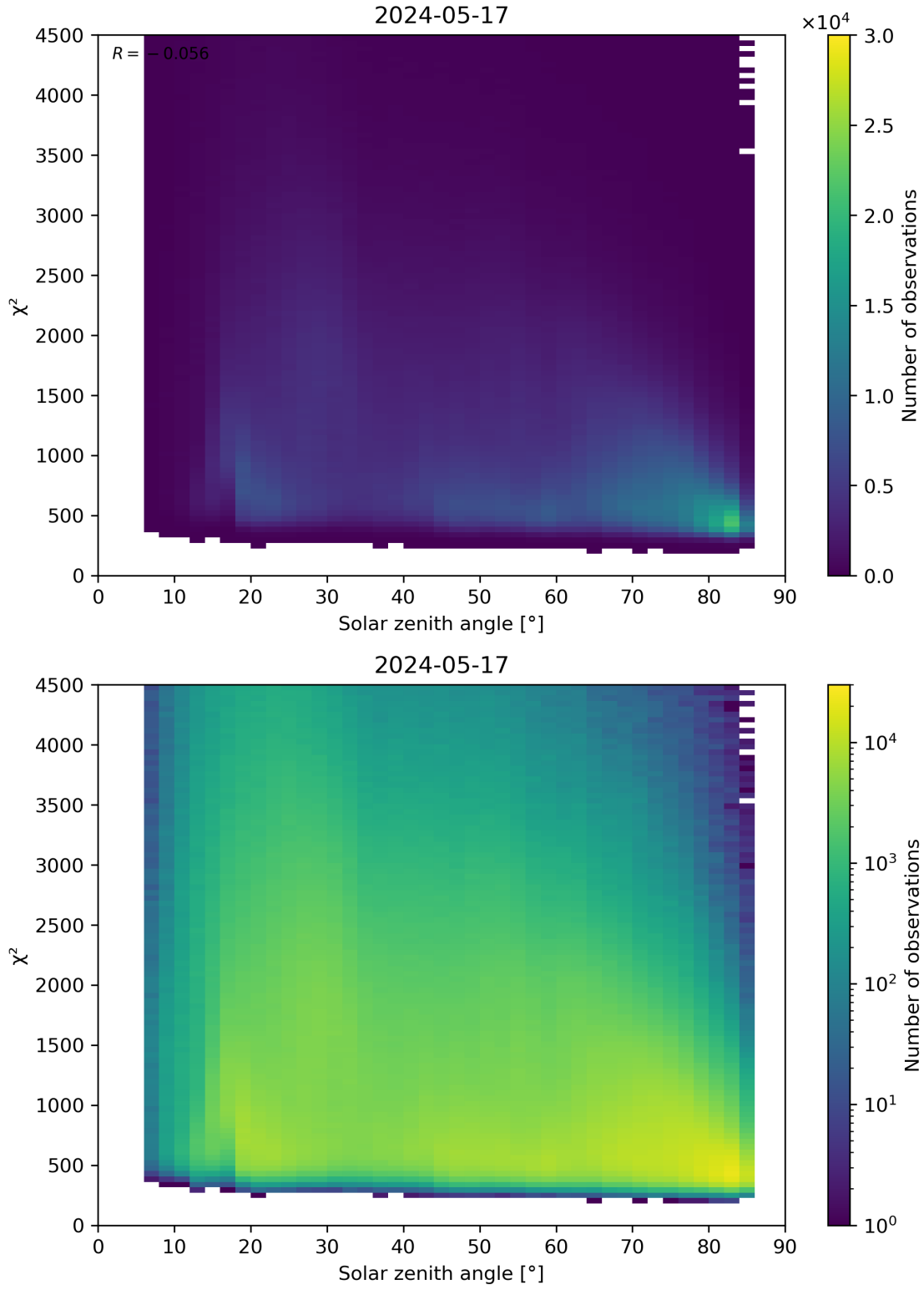
Figure 64: Scatter density plot of “Solar zenith angle” against “ \chi^2 ” for 2024-05-16 to 2024-05-18.
