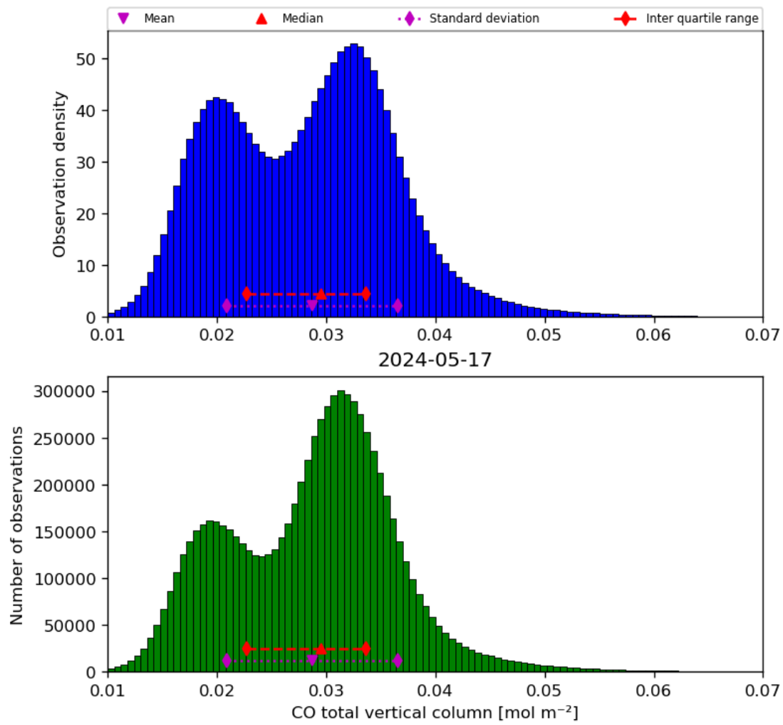
Figure 18: Histogram of “CO total vertical column” for 2024-05-16 to 2024-05-18
