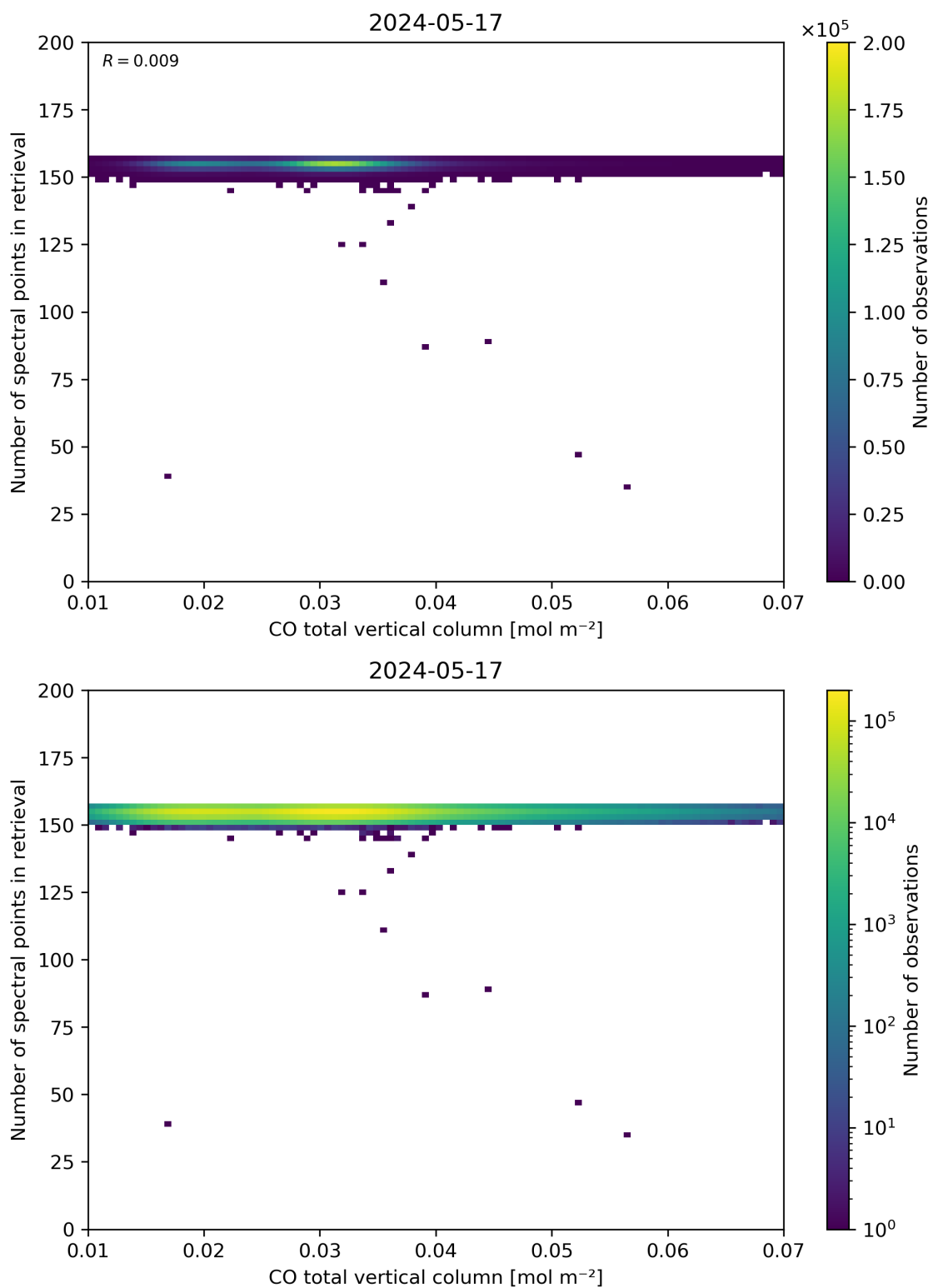
Figure 43: Scatter density plot of “CO total vertical column” against “Number of spectral points in retrieval” for 2024-05-16 to 2024-05-18.
