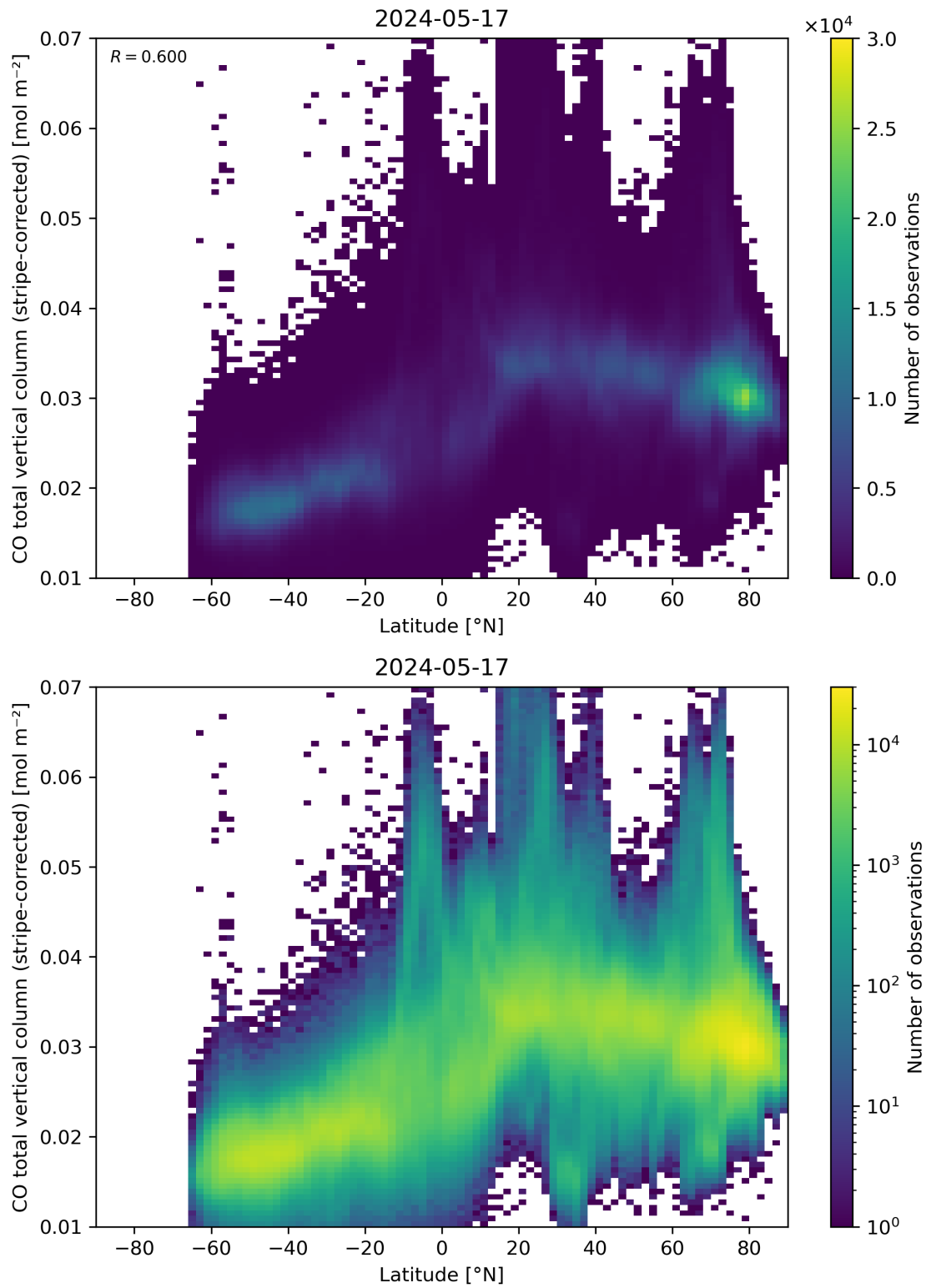
Figure 52: Scatter density plot of “Latitude” against “CO total vertical column (stripe-corrected)” for 2024-05-16 to 2024-05-18.
