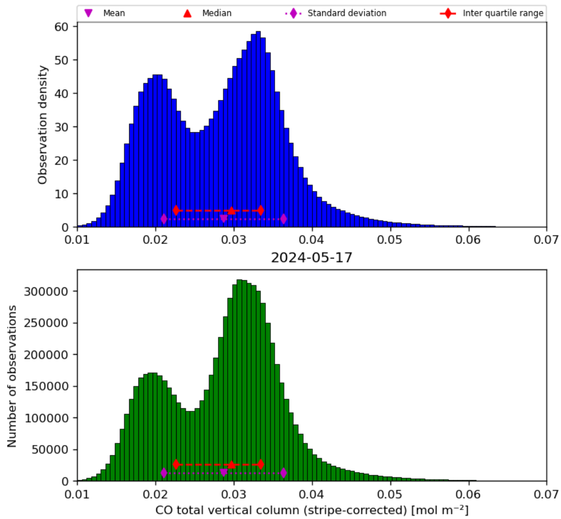
Figure 19: Histogram of “CO total vertical column (stripe-corrected)” for 2024-05-16 to 2024-05-18
