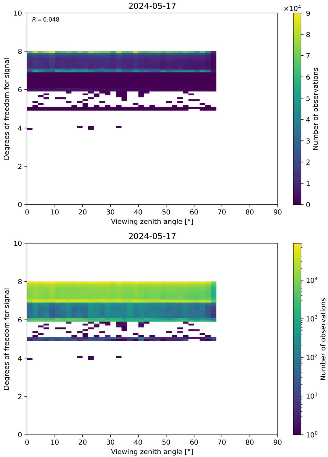
Figure 73: Scatter density plot of “Viewing zenith angle” against “Degrees of freedom for signal” for 2024-05-16 to 2024-05-18.
