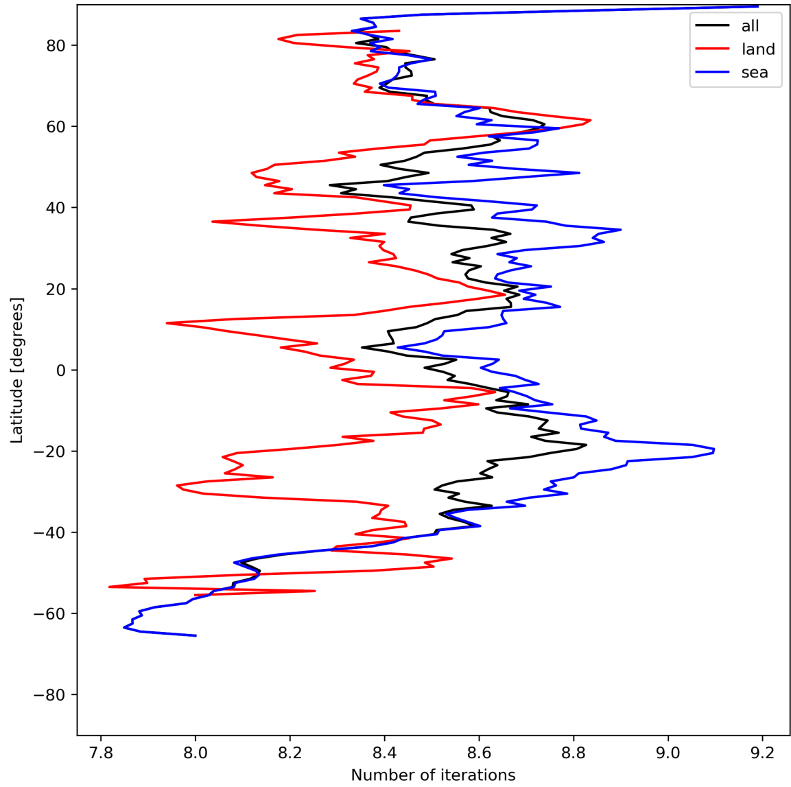
Figure 16: Zonal average of “Number of iterations” for 2024-05-16 to 2024-05-18.
