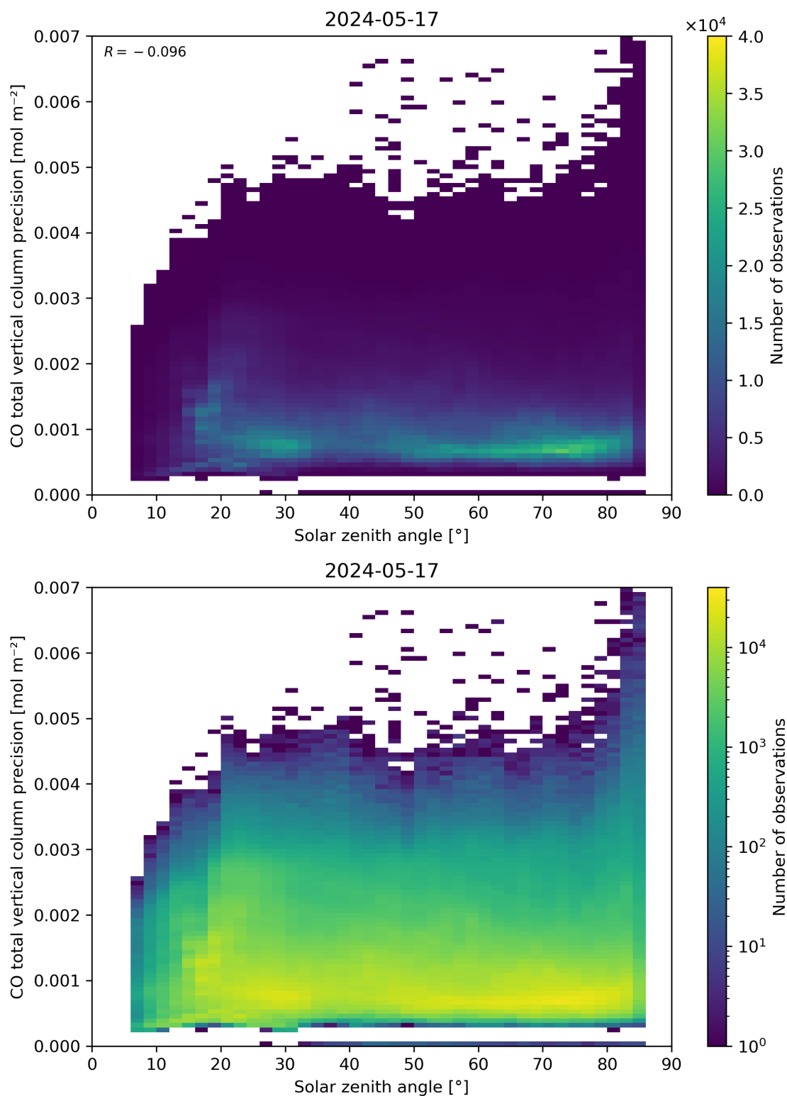
Figure 63: Scatter density plot of “Solar zenith angle” against “CO total vertical column precision” for 2024-05-16 to 2024-05-18.
