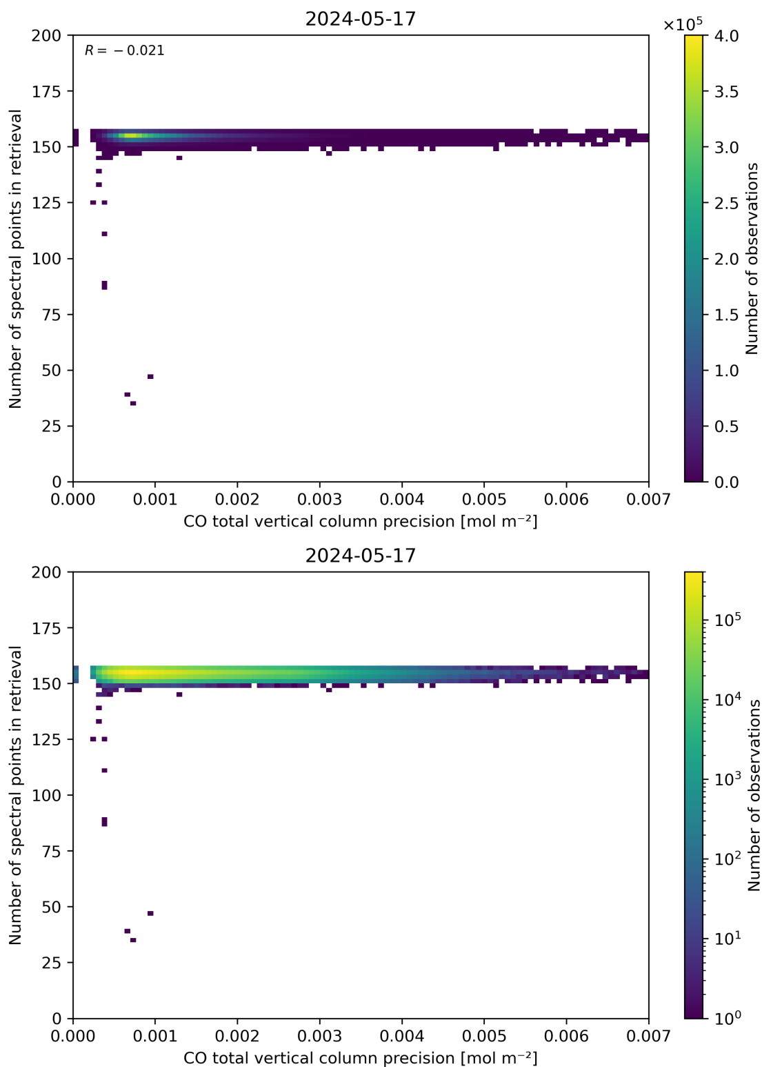
Figure 47: Scatter density plot of “CO total vertical column precision” against “Number of spectral points in retrieval” for 2024-05-16 to 2024-05-18.
