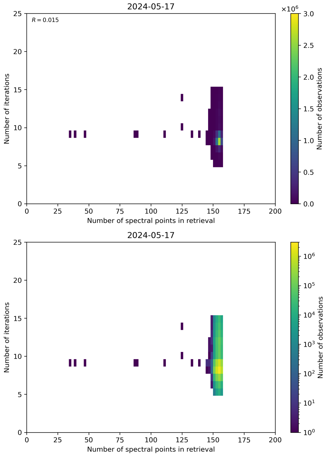
Figure 60: Scatter density plot of “Number of spectral points in retrieval” against “Number of iterations” for 2024-05-16 to 2024-05-18.
