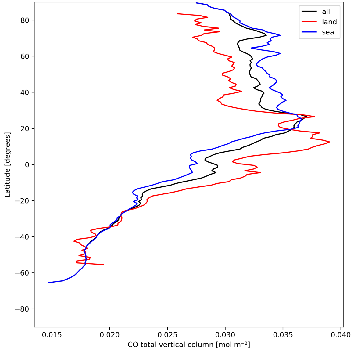
Figure 10: Zonal average of “CO total vertical column” for 2024-05-16 to 2024-05-18.
