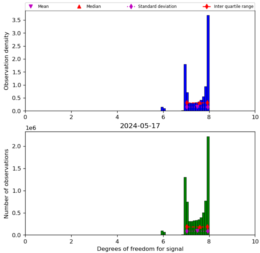
Figure 23: Histogram of “Degrees of freedom for signal” for 2024-05-16 to 2024-05-18
