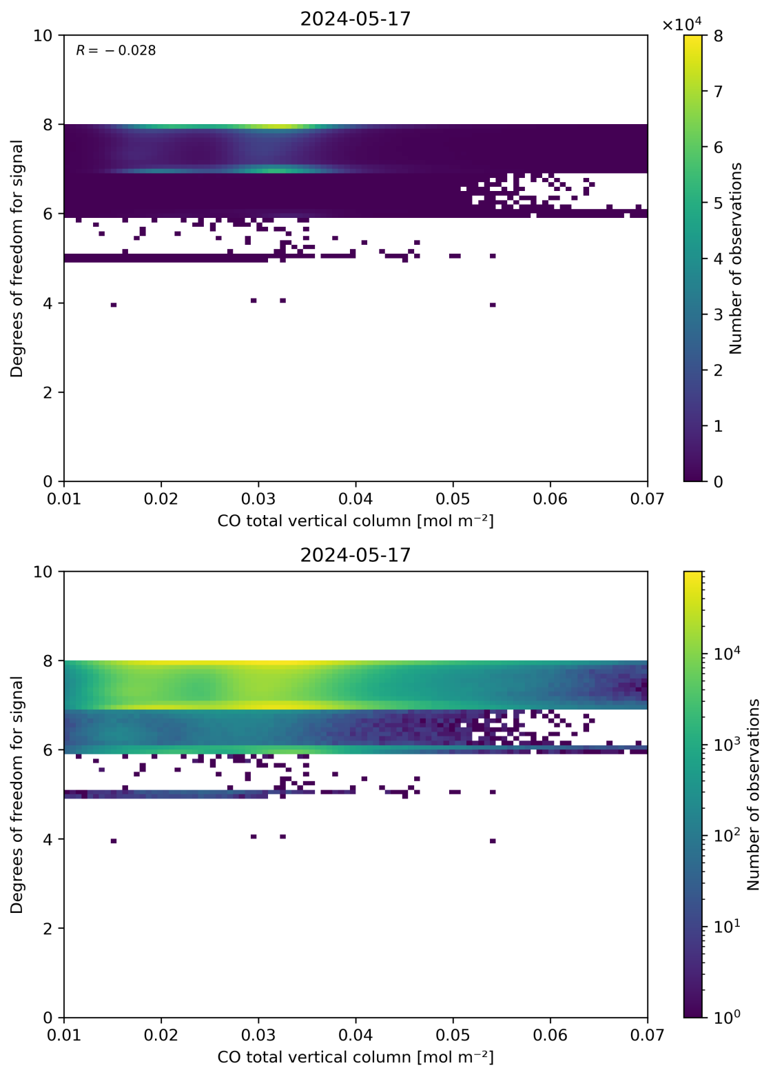
Figure 41: Scatter density plot of “CO total vertical column” against “Degrees of freedom for signal” for 2024-05-16 to 2024-05-18.
