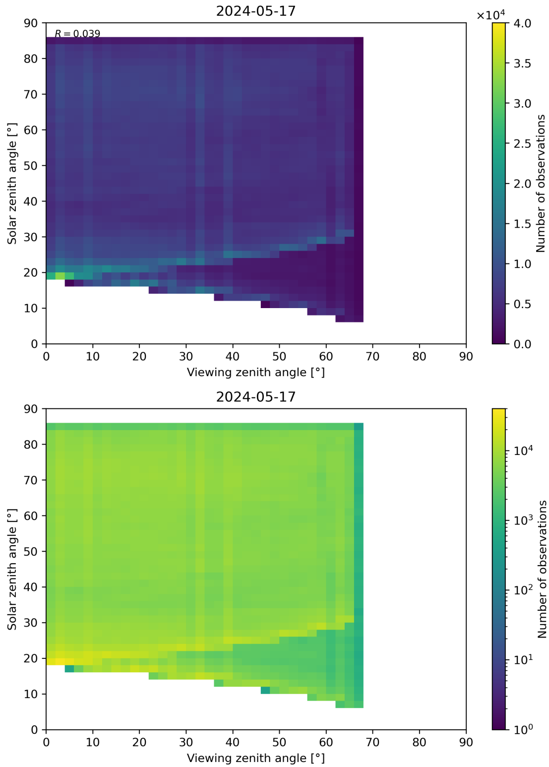
Figure 77: Scatter density plot of “Viewing zenith angle” against “Solar zenith angle” for 2024-05-16 to 2024-05-18.
