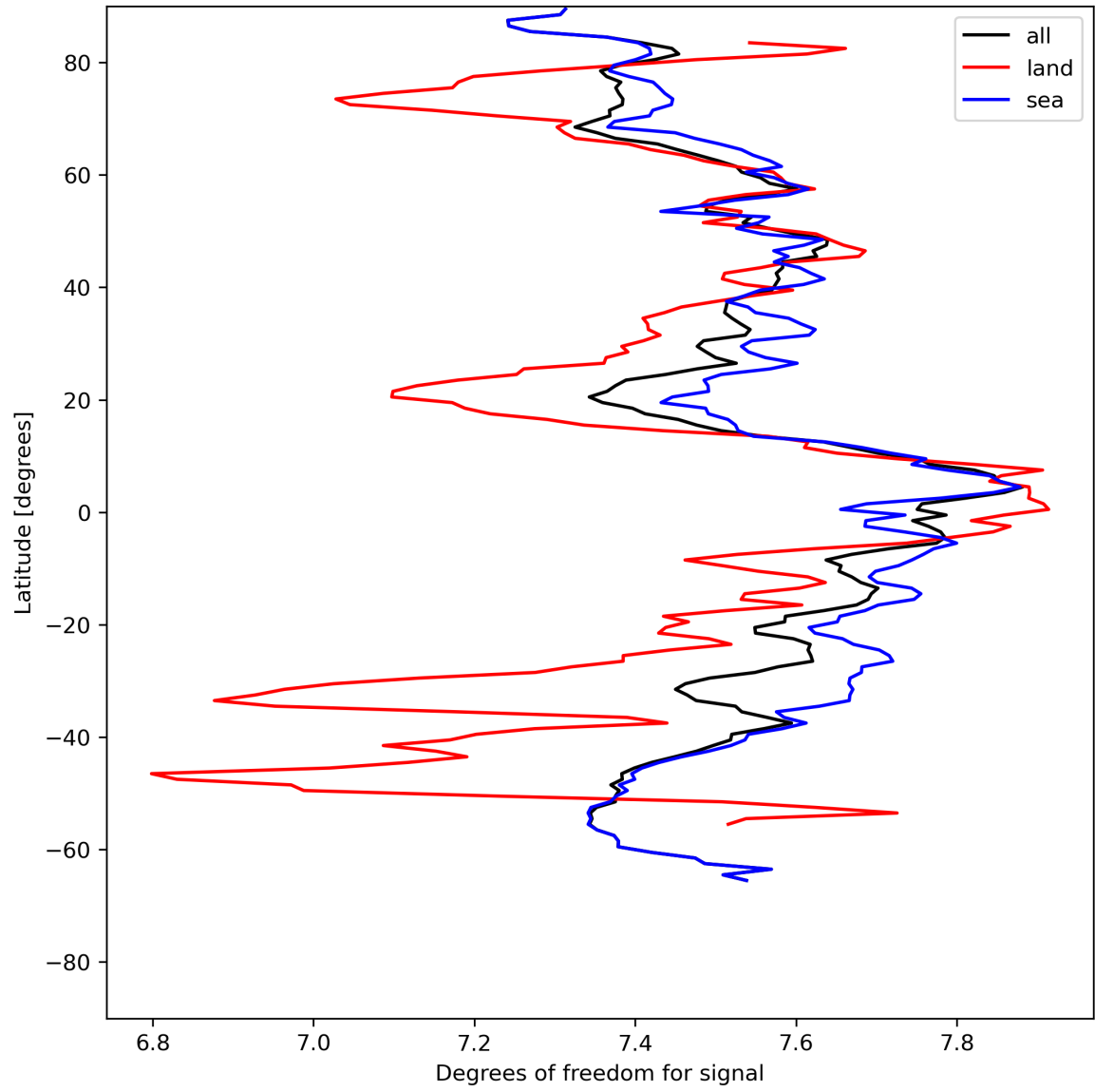
Figure 15: Zonal average of “Degrees of freedom for signal” for 2024-05-16 to 2024-05-18.
