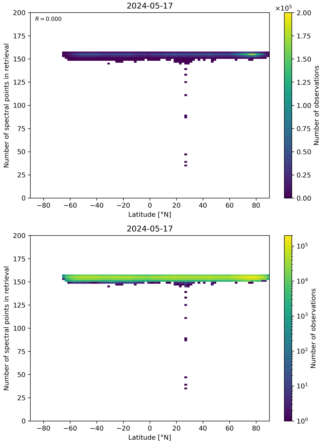
Figure 57: Scatter density plot of “Latitude” against “Number of spectral points in retrieval” for 2024-05-16 to 2024-05-18.
