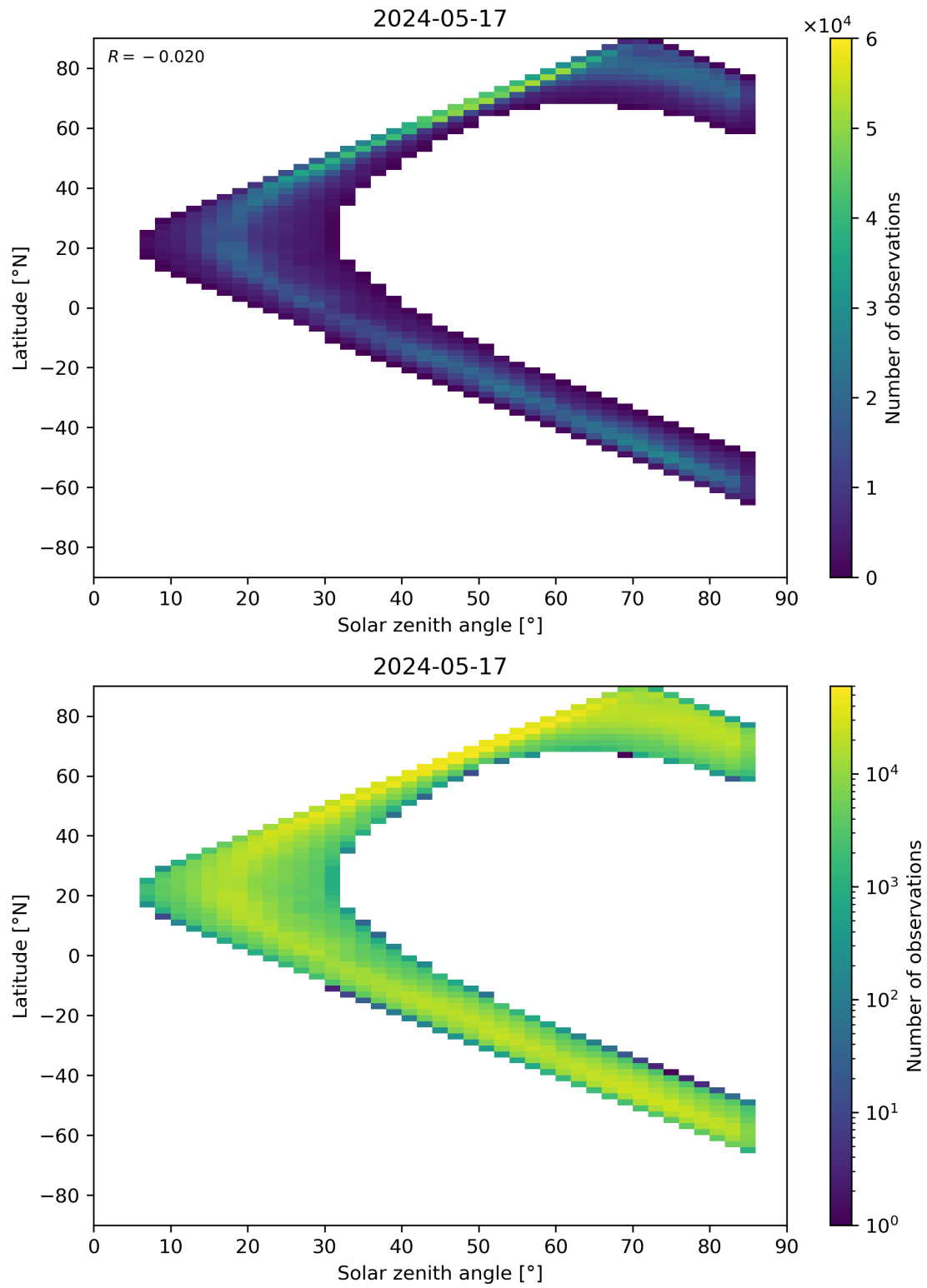
Figure 66: Scatter density plot of “Solar zenith angle” against “Latitude” for 2024-05-16 to 2024-05-18.
