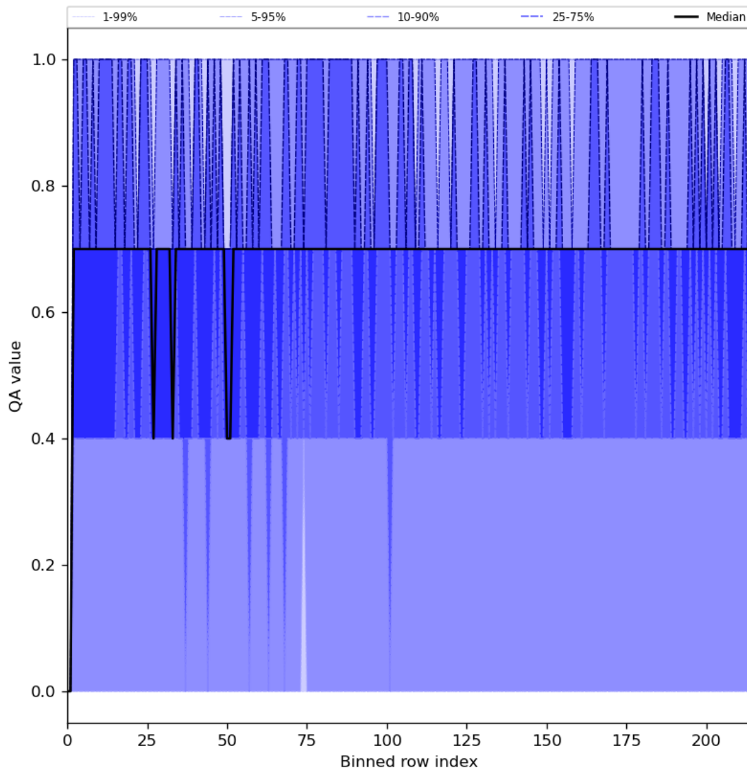
Figure 25: Along track statistics of “QA value” for 2024-05-16 to 2024-05-18
