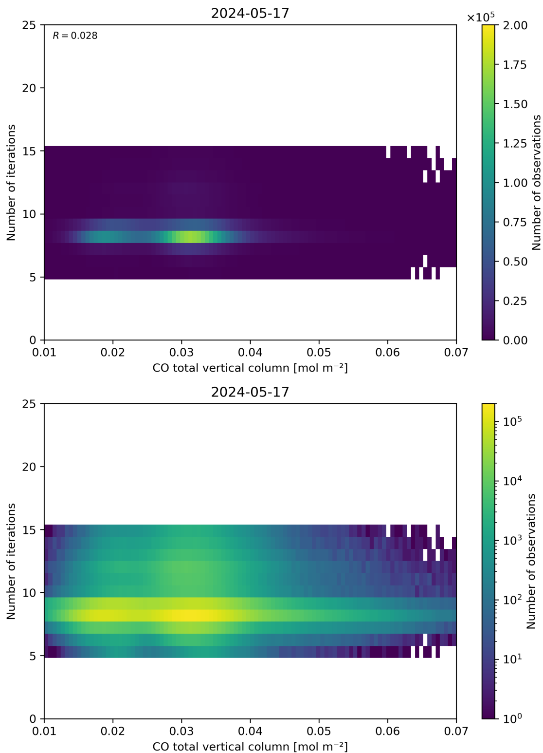
Figure 42: Scatter density plot of “CO total vertical column” against “Number of iterations” for 2024-05-16 to 2024-05-18.
