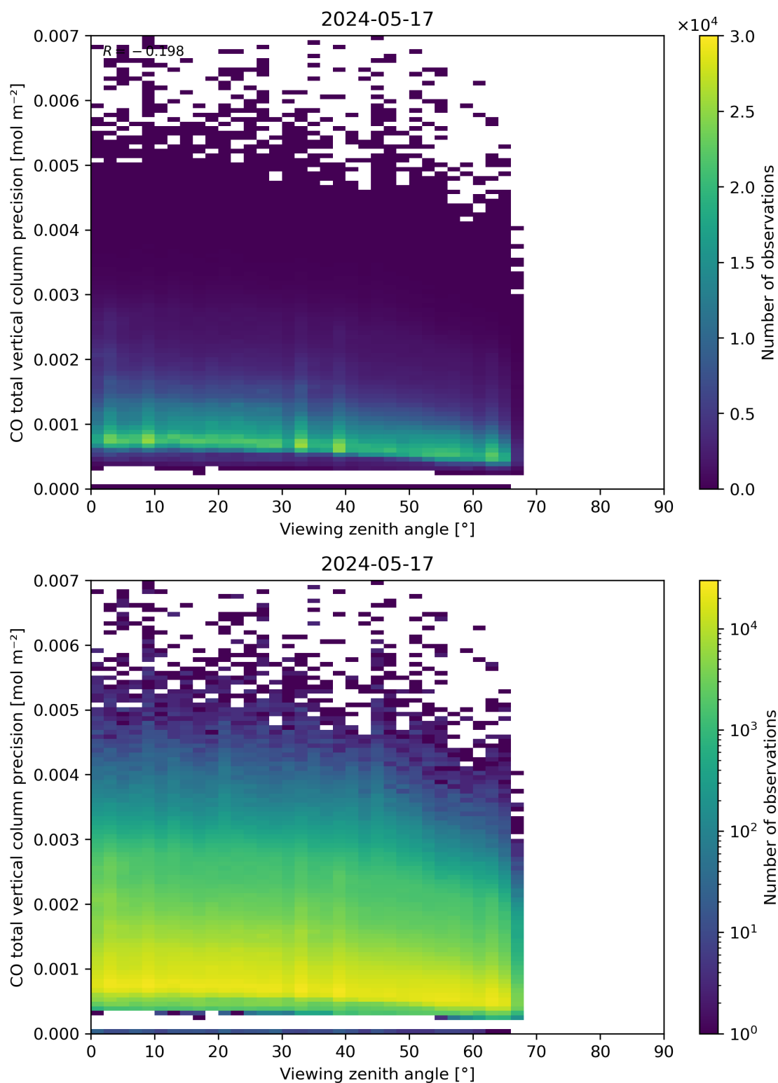
Figure 71: Scatter density plot of “Viewing zenith angle” against “CO total vertical column precision” for 2024-05-16 to 2024-05-18.
