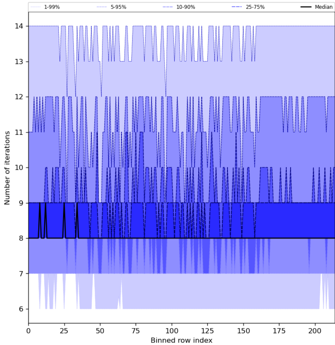
Figure 32: Along track statistics of “Number of iterations” for 2024-05-16 to 2024-05-18
