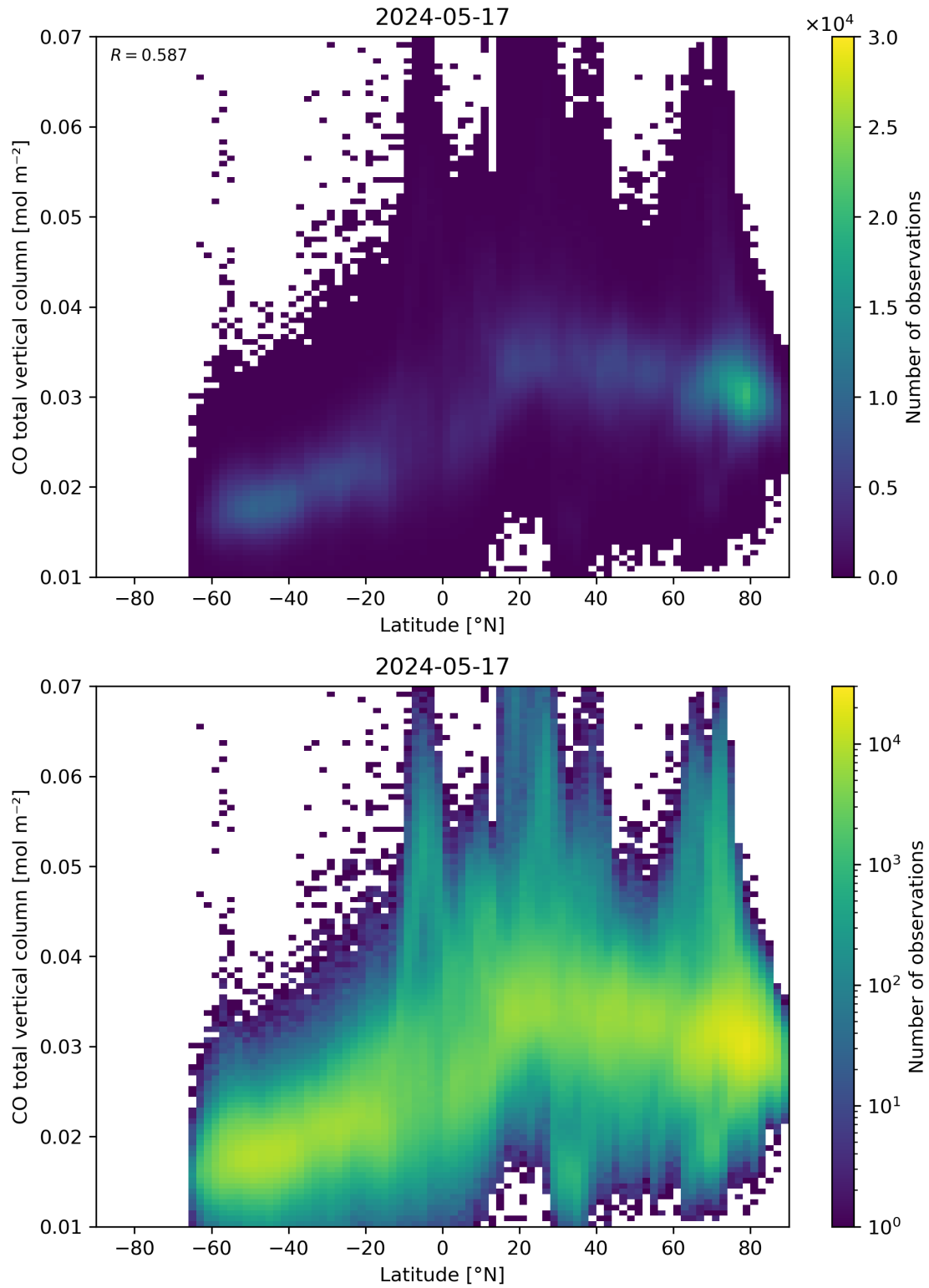
Figure 51: Scatter density plot of “Latitude” against “CO total vertical column” for 2024-05-16 to 2024-05-18.
