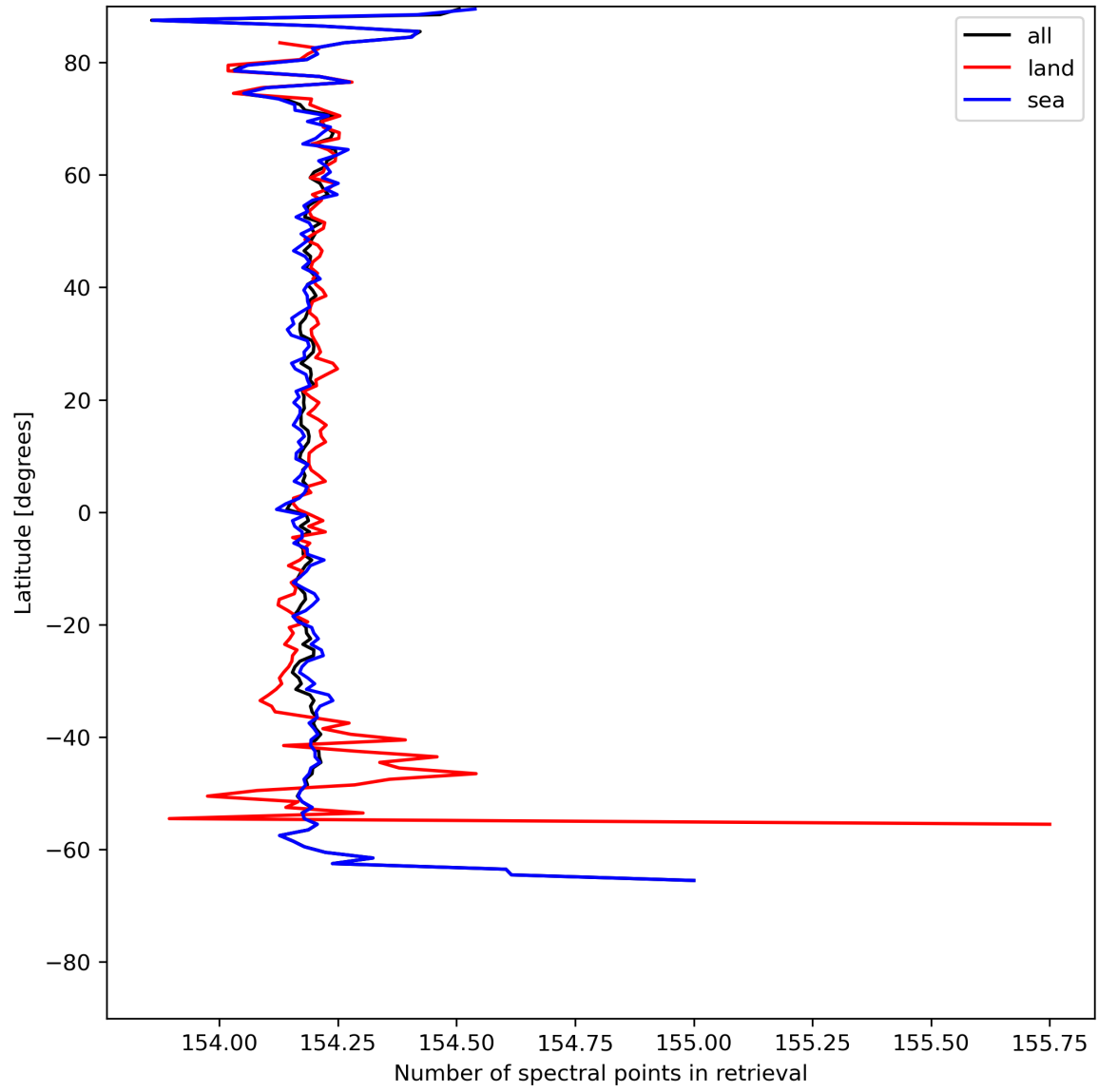
Figure 13: Zonal average of “Number of spectral points in retrieval” for 2024-05-16 to 2024-05-18.
