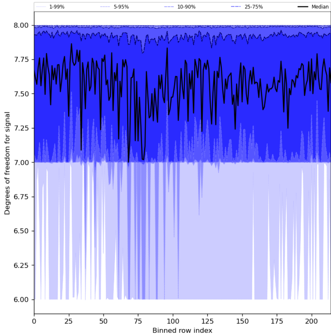
Figure 31: Along track statistics of “Degrees of freedom for signal” for 2024-05-16 to 2024-05-18
