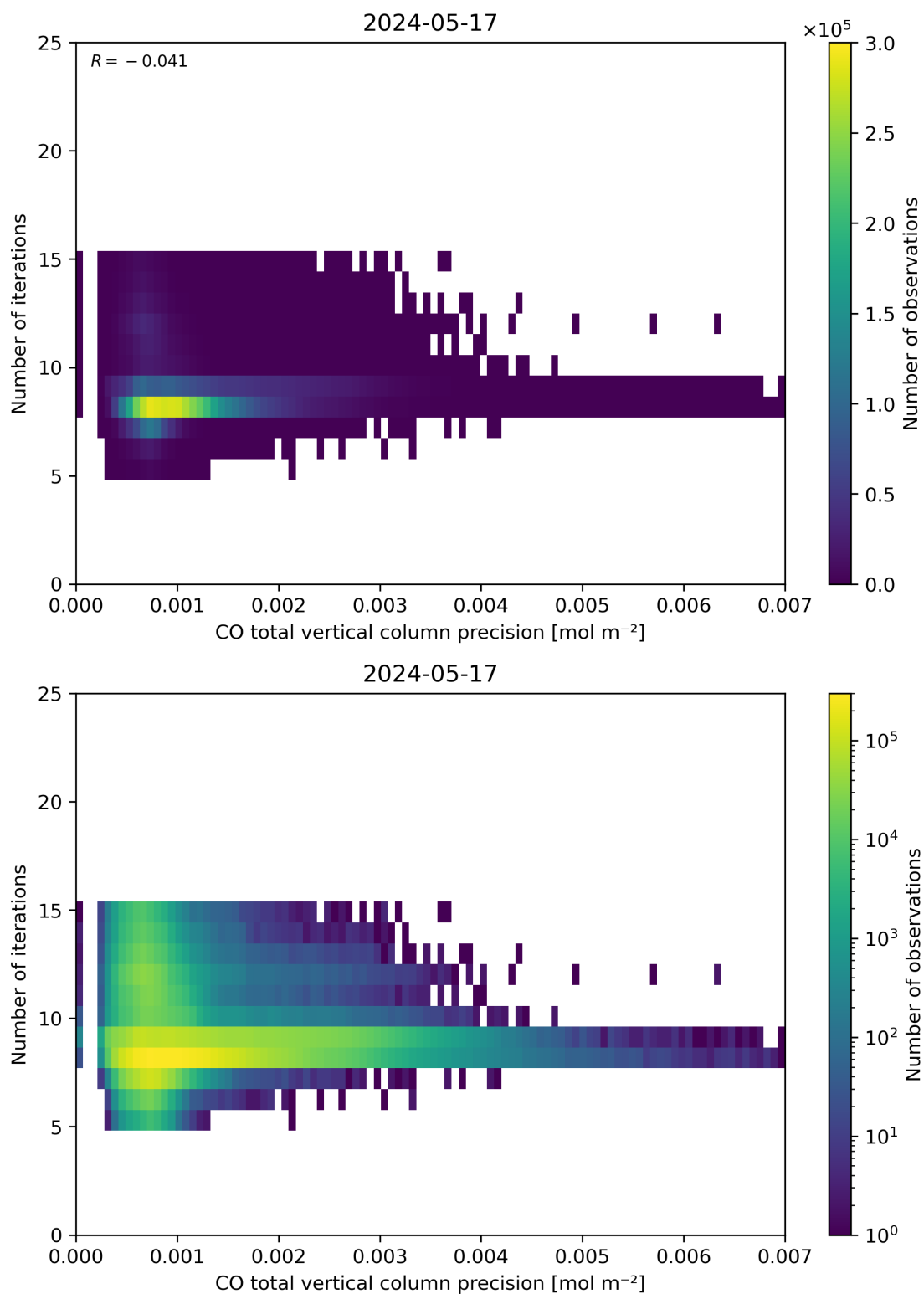
Figure 46: Scatter density plot of “CO total vertical column precision” against “Number of iterations” for 2024-05-16 to 2024-05-18.
