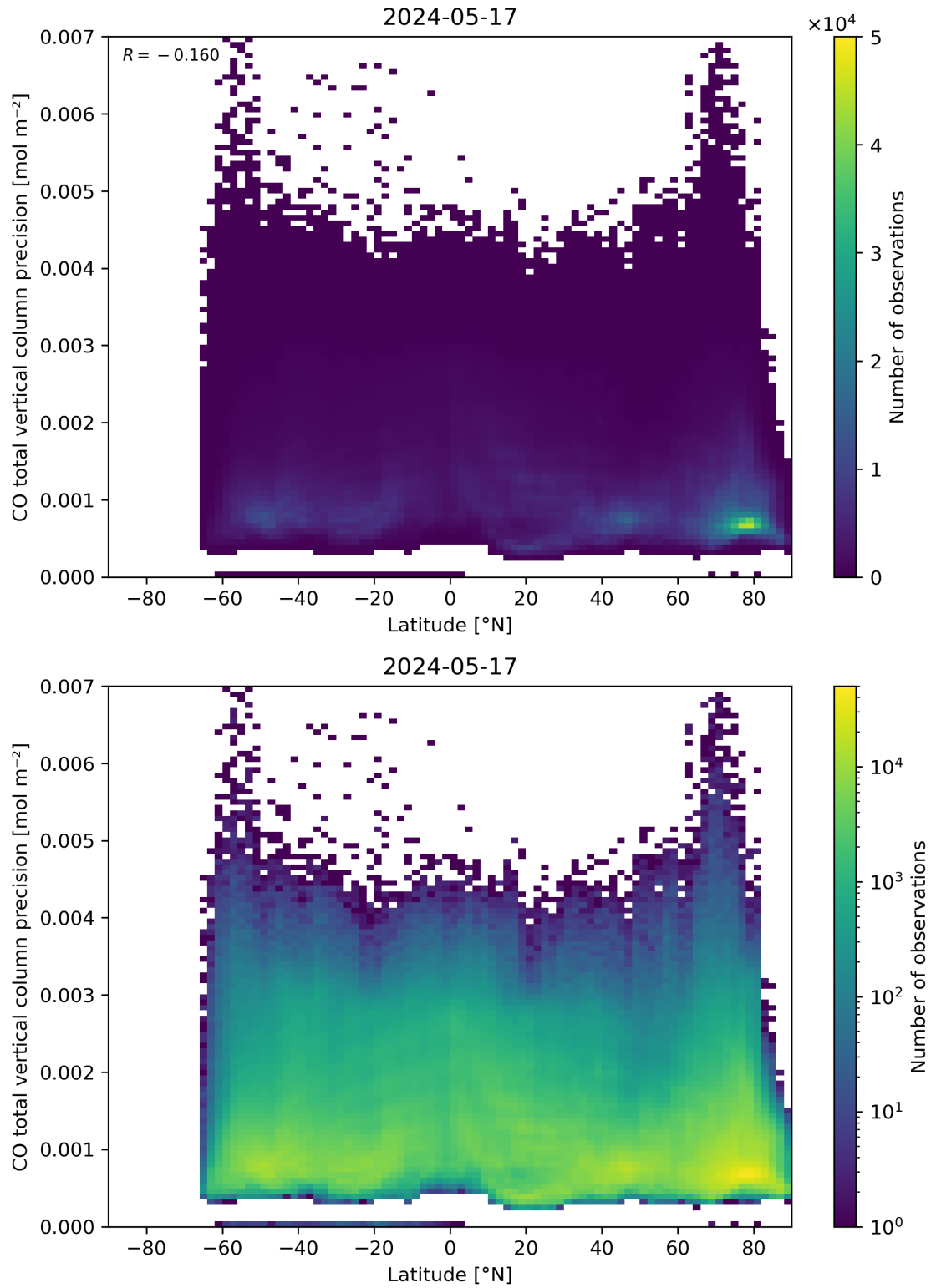
Figure 53: Scatter density plot of “Latitude” against “CO total vertical column precision” for 2024-05-16 to 2024-05-18.
