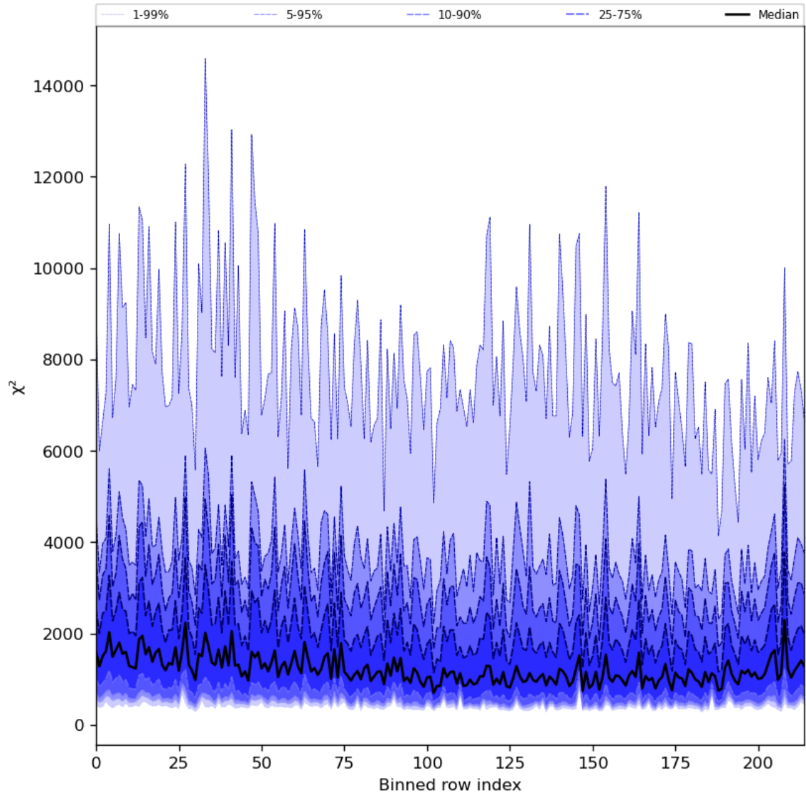
Figure 30: Along track statistics of “ \chi^2 ” for 2024-05-16 to 2024-05-18
