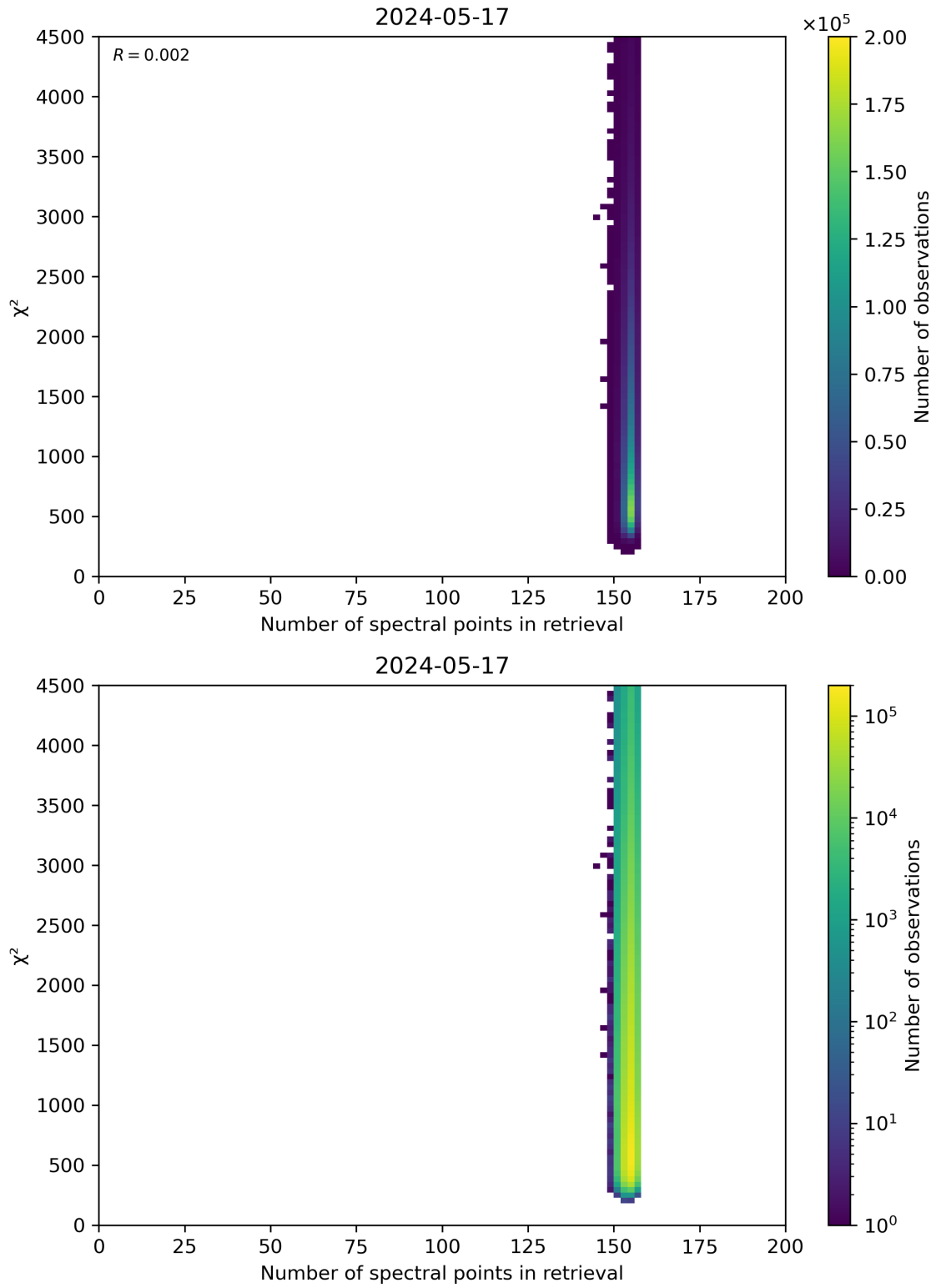
Figure 58: Scatter density plot of “Number of spectral points in retrieval” against “ \chi^2 ” for 2024-05-16 to 2024-05-18.
