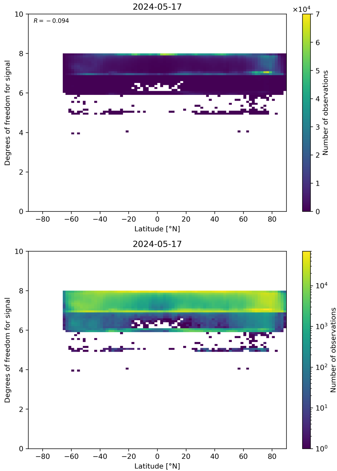
Figure 55: Scatter density plot of “Latitude” against “Degrees of freedom for signal” for 2024-05-16 to 2024-05-18.
