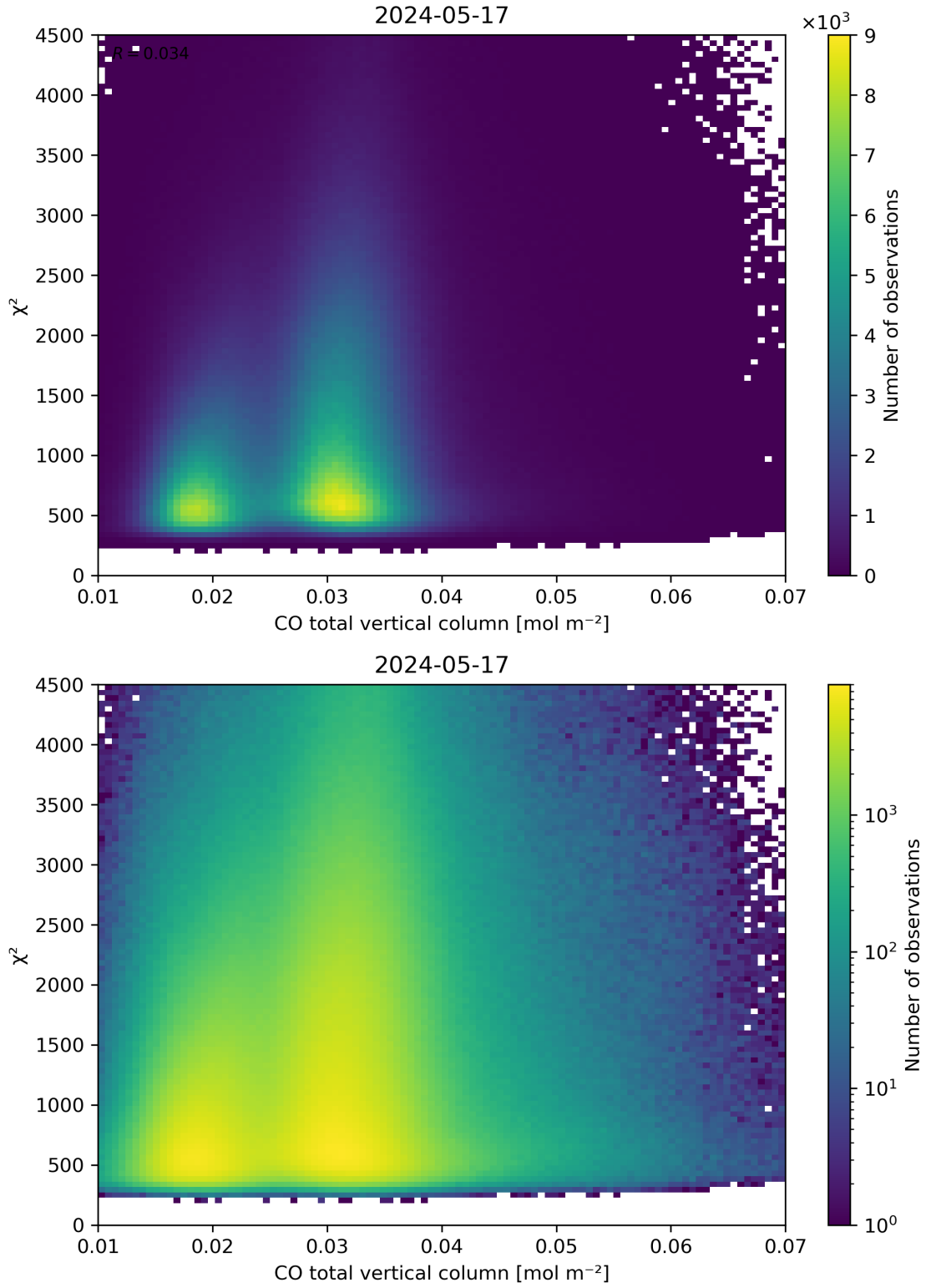
Figure 35: Scatter density plot of “CO total vertical column” against “ \chi^2 ” for 2024-05-16 to 2024-05-18.
