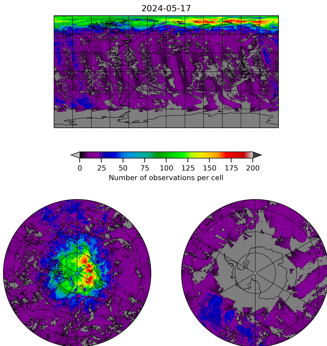
Figure 8: Map of the number of observations for 2024-05-16 to 2024-05-18
