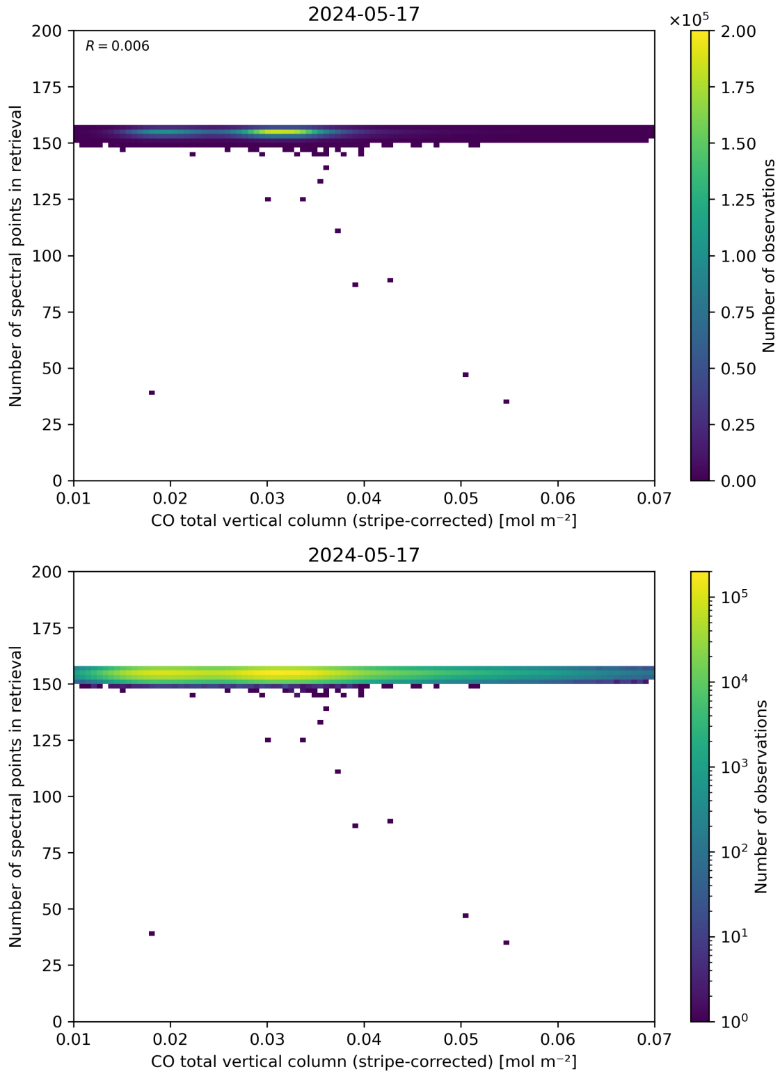
Figure 40: Scatter density plot of “CO total vertical column (stripe-corrected)” against “Number of spectral points in retrieval” for 2024-05-16 to 2024-05-18.
