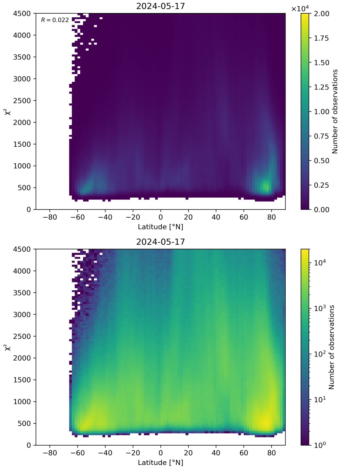
Figure 54: Scatter density plot of “Latitude” against “ \chi^2 ” for 2024-05-16 to 2024-05-18.
