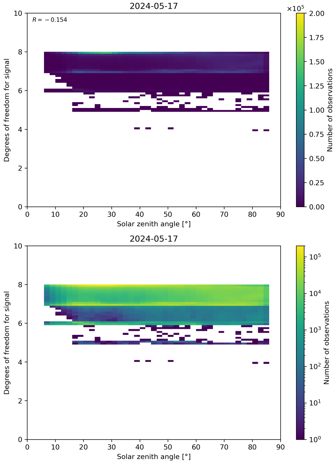
Figure 65: Scatter density plot of “Solar zenith angle” against “Degrees of freedom for signal” for 2024-05-16 to 2024-05-18.
