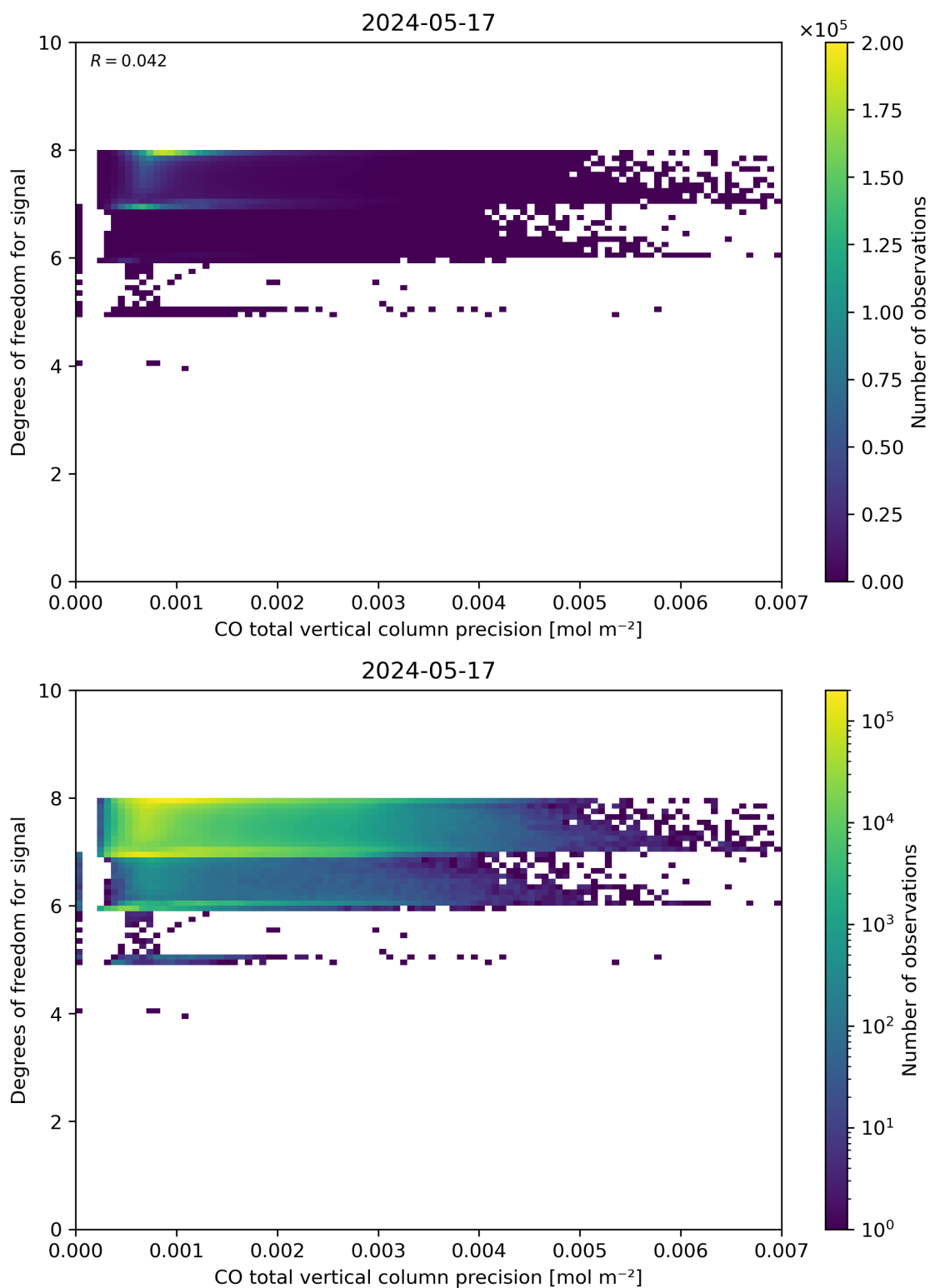
Figure 45: Scatter density plot of “CO total vertical column precision” against “Degrees of freedom for signal” for 2024-05-16 to 2024-05-18.
