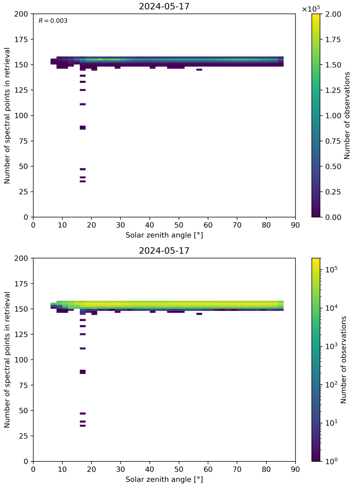
Figure 68: Scatter density plot of “Solar zenith angle” against “Number of spectral points in retrieval” for 2024-05-16 to 2024-05-18.
