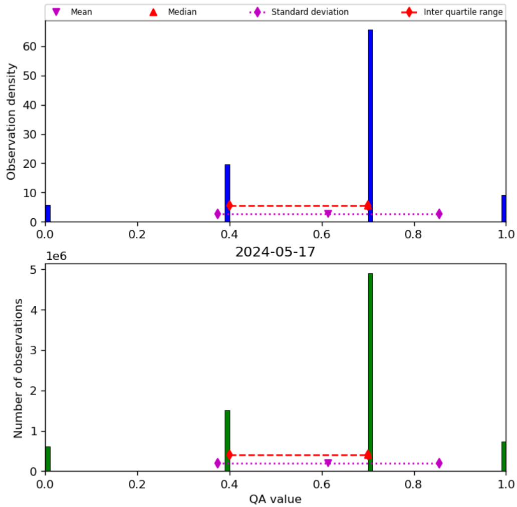
Figure 17: Histogram of “QA value” for 2024-05-16 to 2024-05-18
