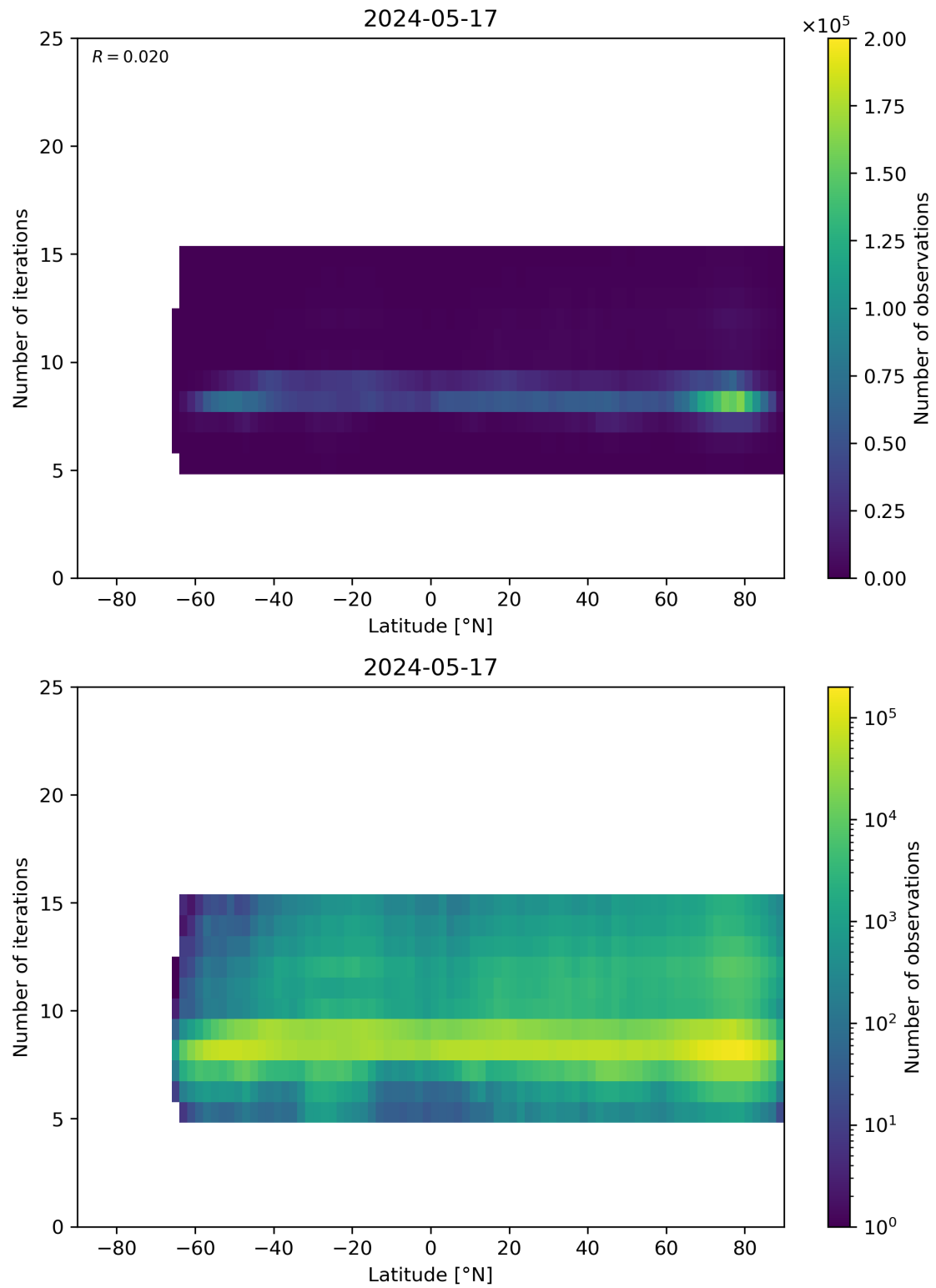
Figure 56: Scatter density plot of “Latitude” against “Number of iterations” for 2024-05-16 to 2024-05-18.
