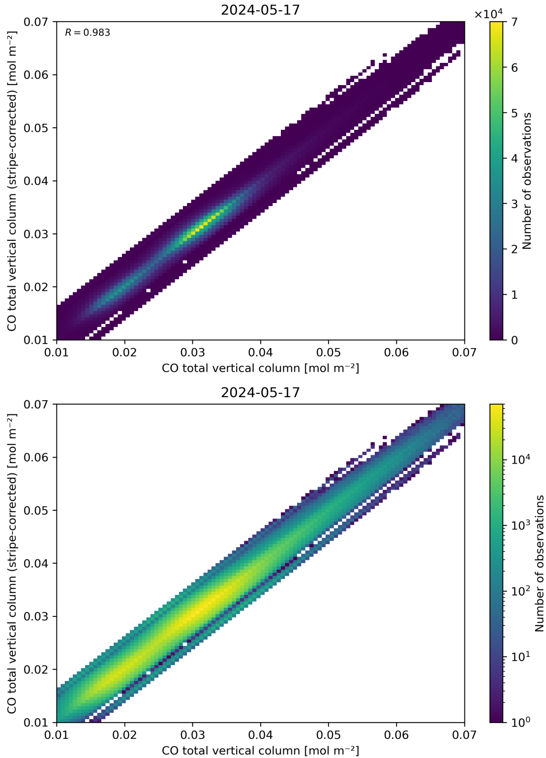
Figure 33: Scatter density plot of “CO total vertical column” against “CO total vertical column (stripe-corrected)” for 2024-05-16 to 2024-05-18.
