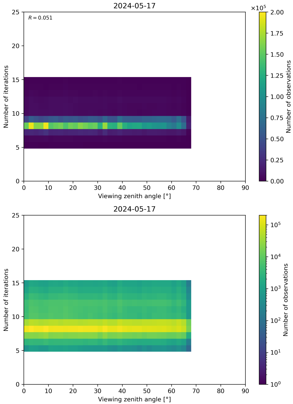
Figure 75: Scatter density plot of “Viewing zenith angle” against “Number of iterations” for 2024-05-16 to 2024-05-18.
