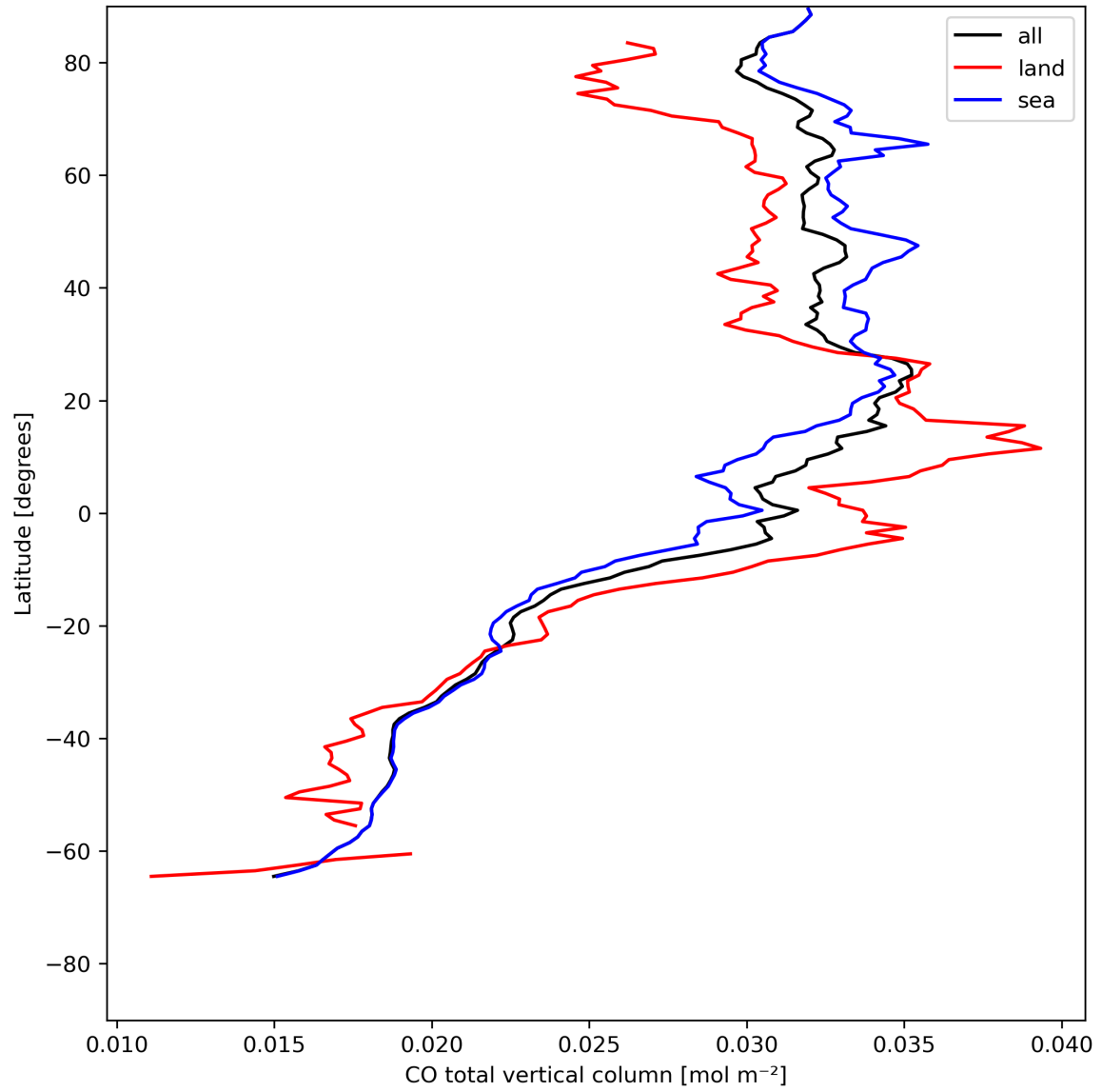
Figure 10: Zonal average of “CO total vertical column” for 2024-05-18 to 2024-05-20.
