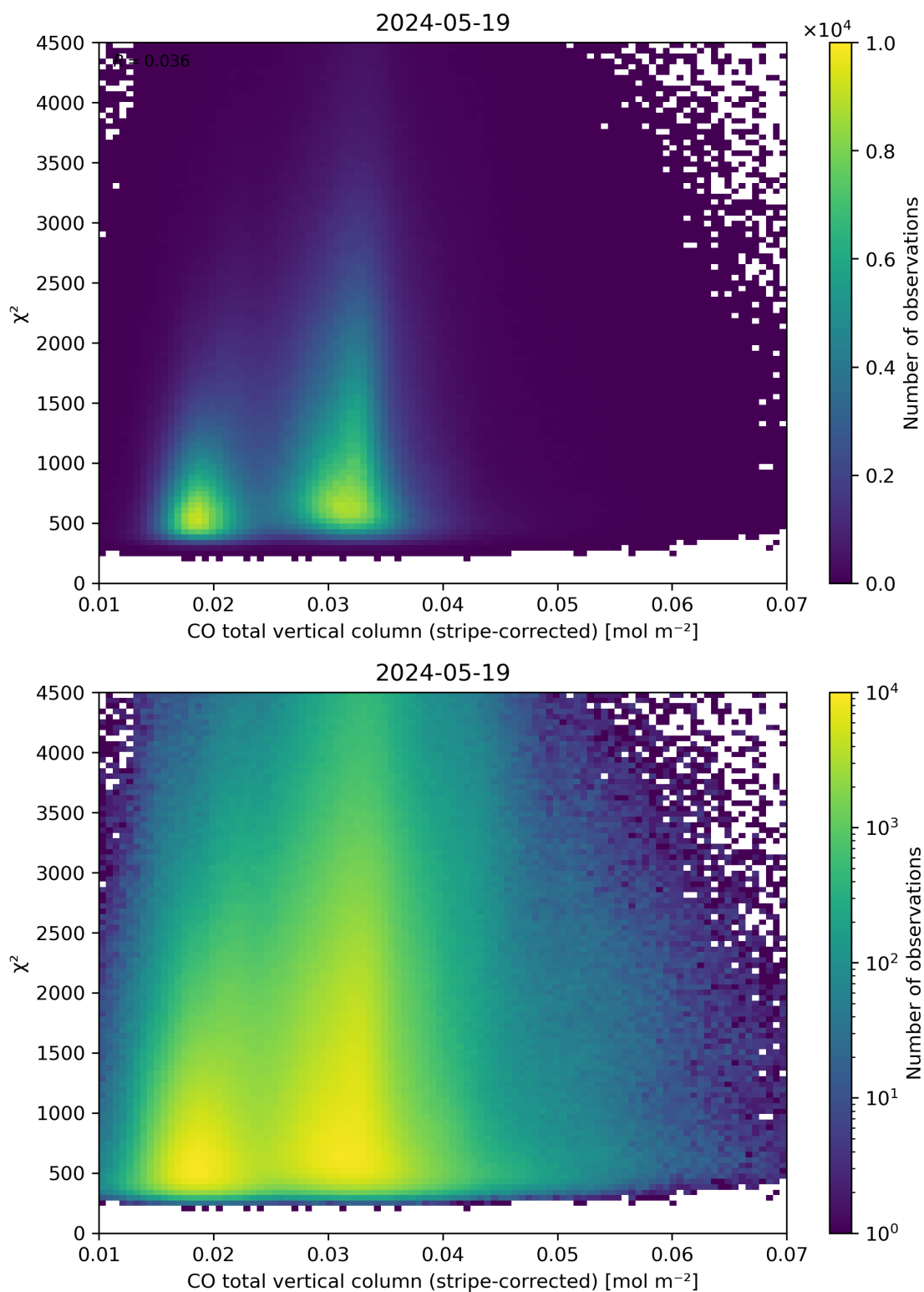
Figure 37: Scatter density plot of “CO total vertical column (stripe-corrected)” against “ \chi^2 ” for 2024-05-18 to 2024-05-20.
