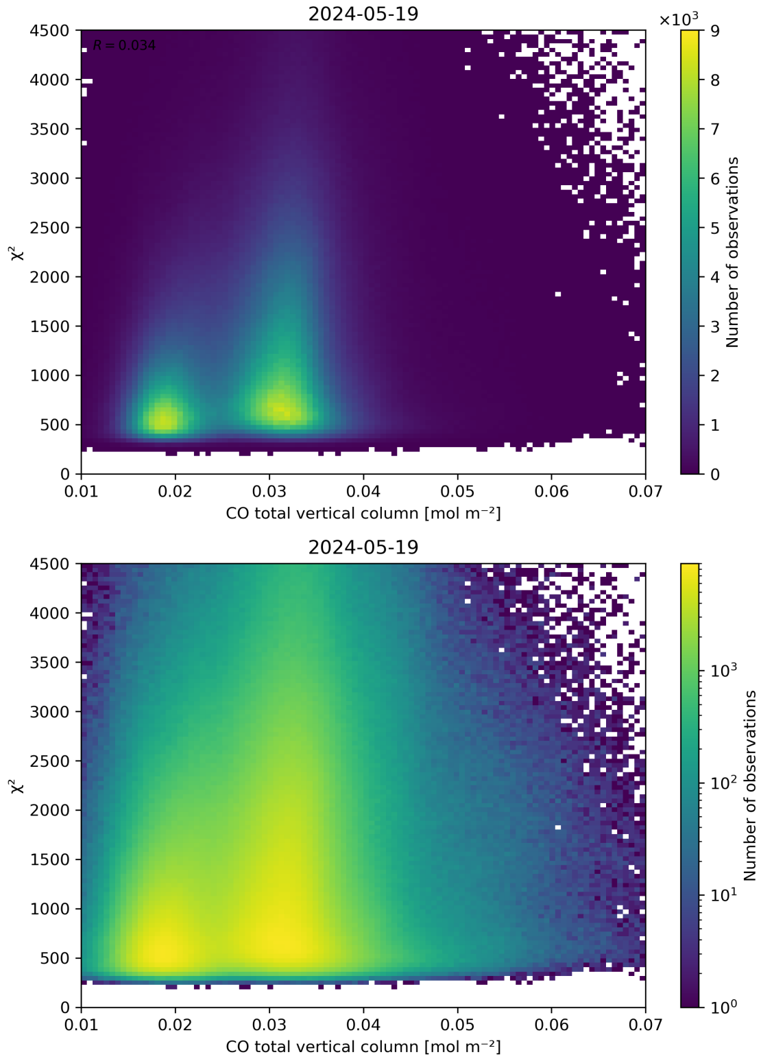
Figure 35: Scatter density plot of “CO total vertical column” against “ \chi^2 ” for 2024-05-18 to 2024-05-20.
