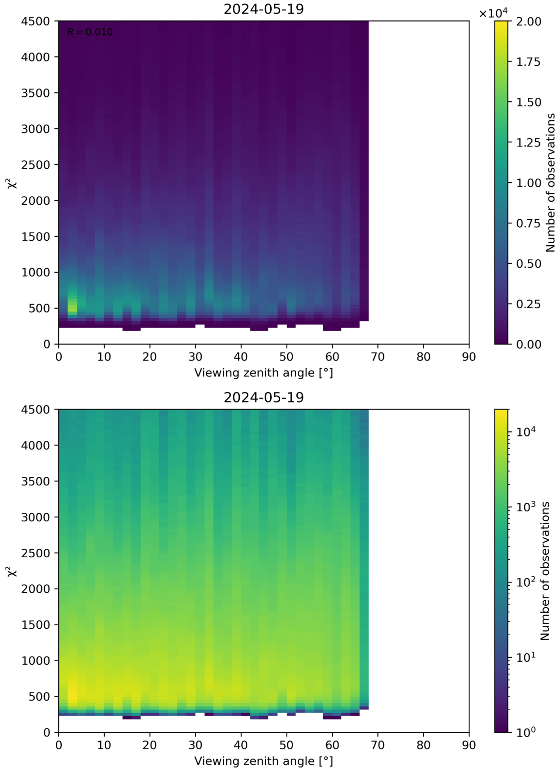
Figure 72: Scatter density plot of “Viewing zenith angle” against “ \chi^2 ” for 2024-05-18 to 2024-05-20.
