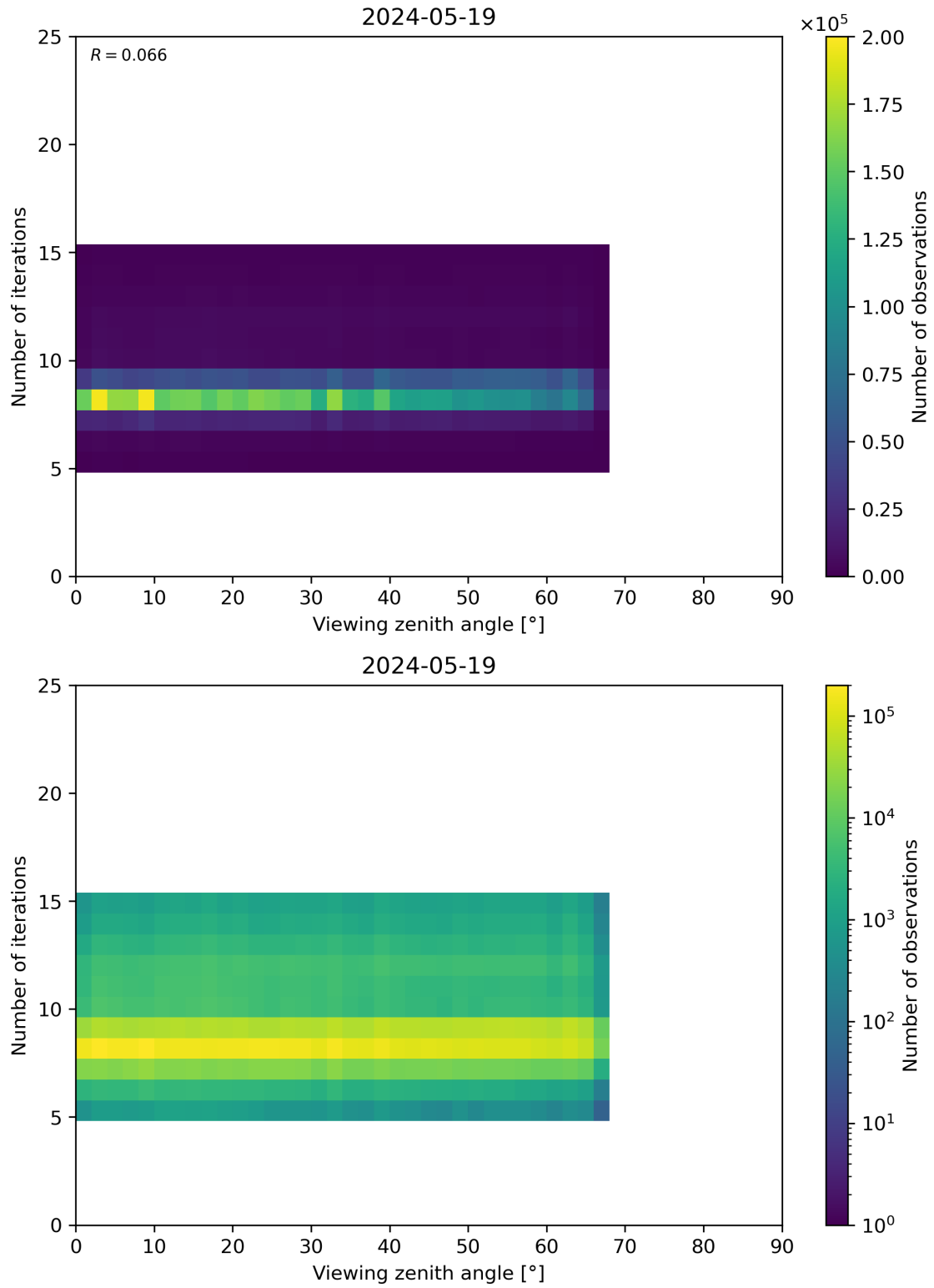
Figure 75: Scatter density plot of “Viewing zenith angle” against “Number of iterations” for 2024-05-18 to 2024-05-20.
