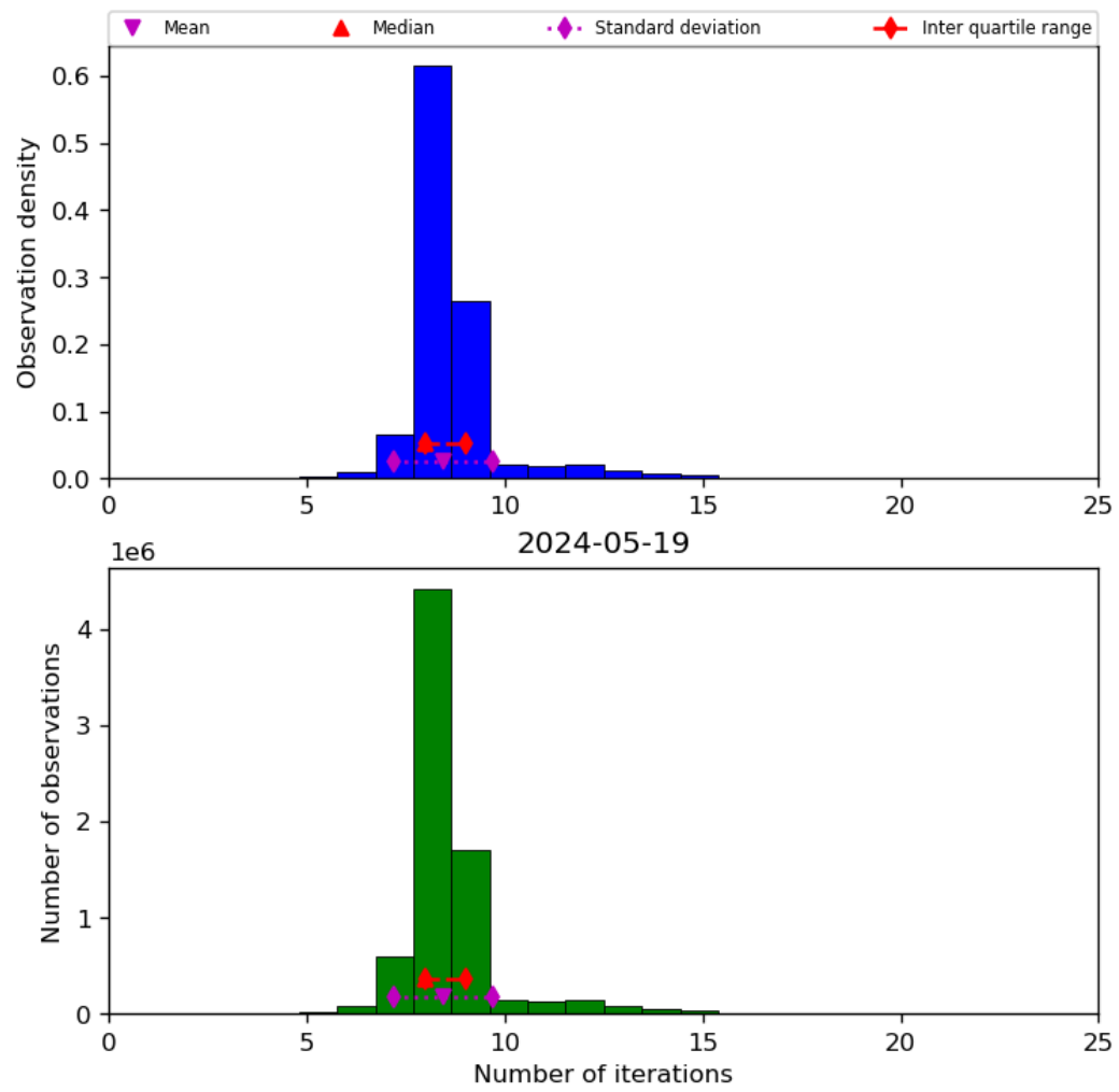
Figure 24: Histogram of “Number of iterations” for 2024-05-18 to 2024-05-20
