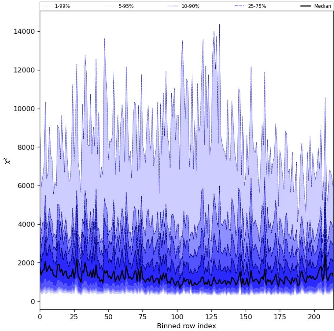
Figure 30: Along track statistics of “ \chi^2 ” for 2024-05-18 to 2024-05-20
