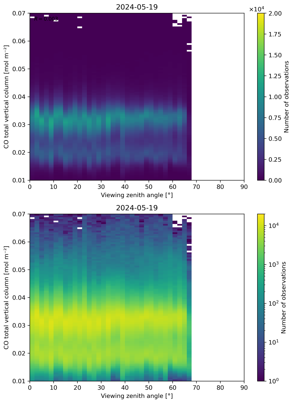
Figure 69: Scatter density plot of “Viewing zenith angle” against “CO total vertical column” for 2024-05-18 to 2024-05-20.
