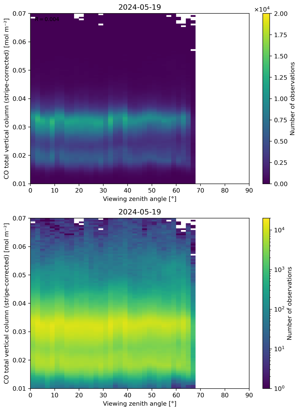
Figure 70: Scatter density plot of “Viewing zenith angle” against “CO total vertical column (stripe-corrected)” for 2024-05-18 to 2024-05-20.
