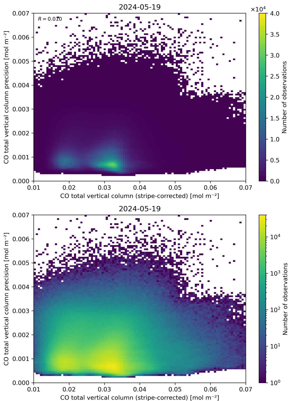
Figure 36: Scatter density plot of “CO total vertical column (stripe-corrected)” against “CO total vertical column precision” for 2024-05-18 to 2024-05-20.
