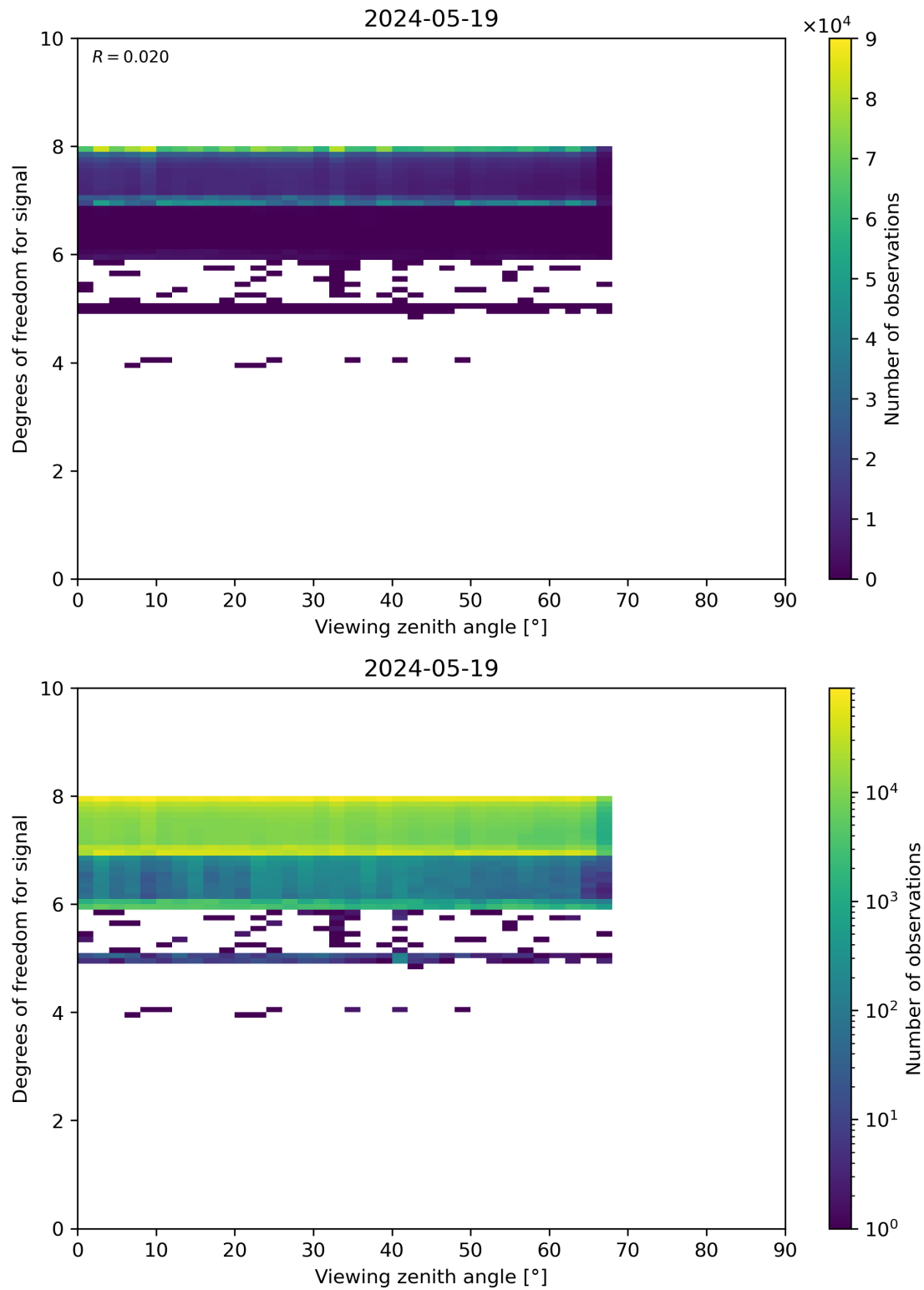
Figure 73: Scatter density plot of “Viewing zenith angle” against “Degrees of freedom for signal” for 2024-05-18 to 2024-05-20.
