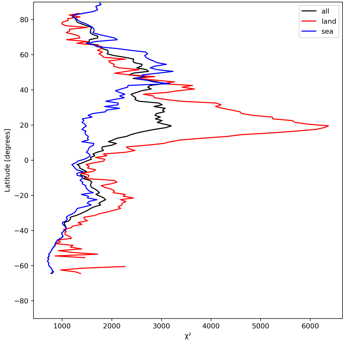
Figure 14: Zonal average of “ \chi^2 ” for 2024-05-18 to 2024-05-20.
