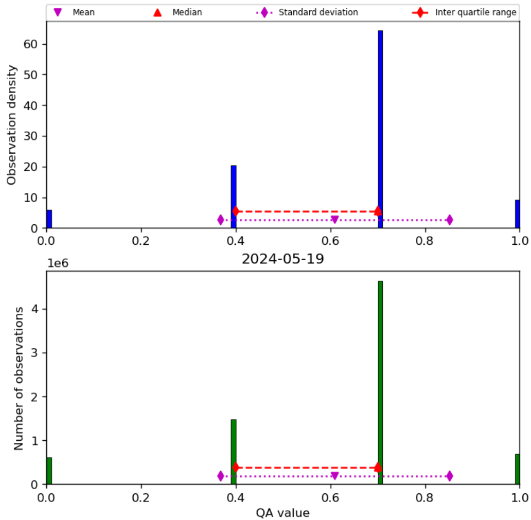
Figure 17: Histogram of “QA value” for 2024-05-18 to 2024-05-20
