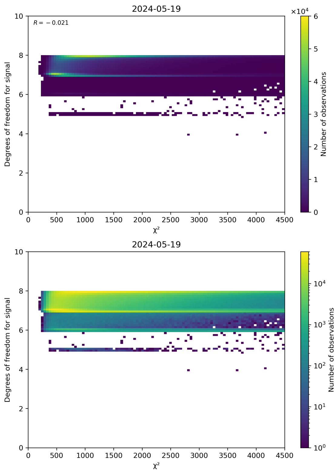
Figure 48: Scatter density plot of “ \chi^2 ” against “Degrees of freedom for signal” for 2024-05-18 to 2024-05-20.
