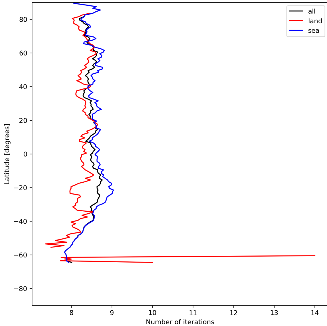
Figure 16: Zonal average of “Number of iterations” for 2024-05-18 to 2024-05-20.
