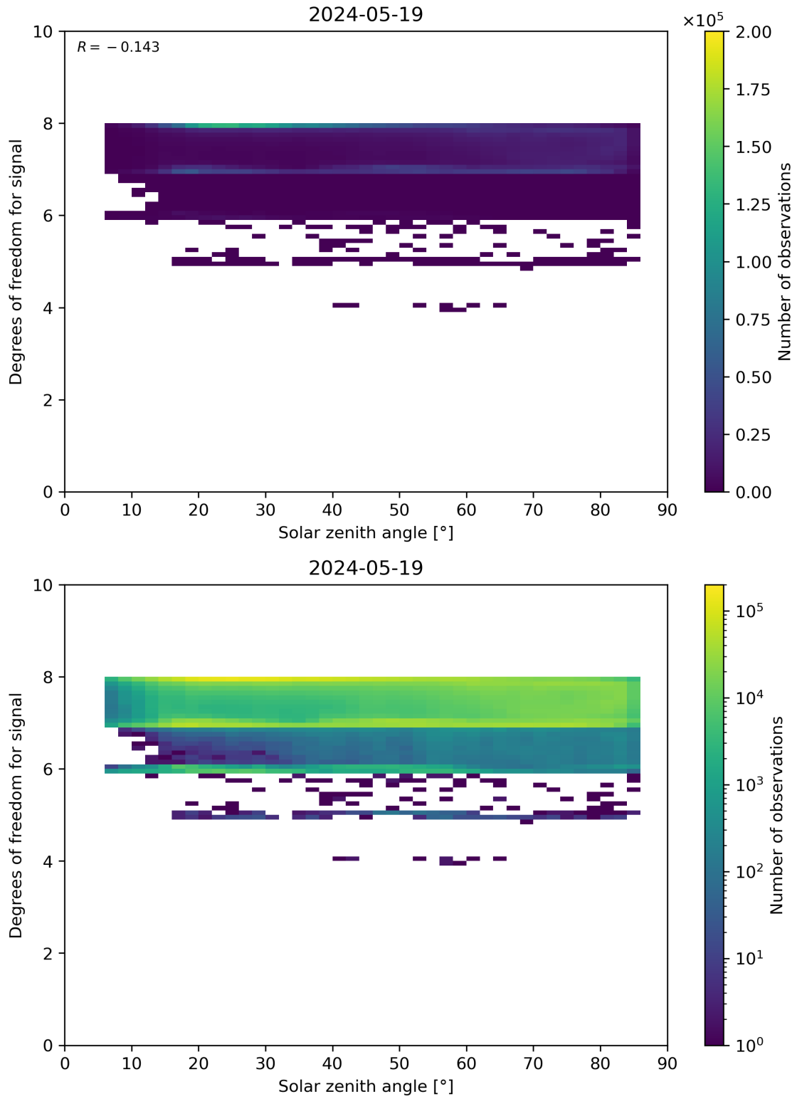
Figure 65: Scatter density plot of “Solar zenith angle” against “Degrees of freedom for signal” for 2024-05-18 to 2024-05-20.
