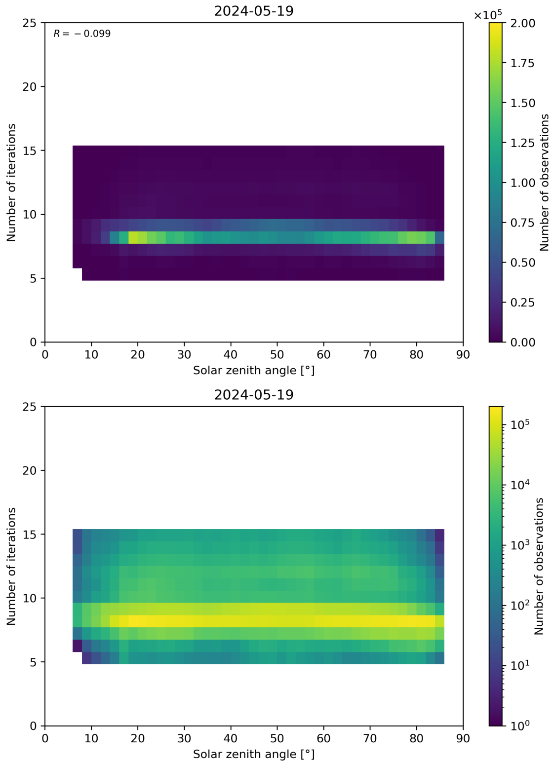
Figure 67: Scatter density plot of “Solar zenith angle” against “Number of iterations” for 2024-05-18 to 2024-05-20.
