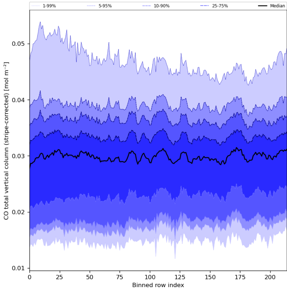
Figure 27: Along track statistics of “CO total vertical column (stripe-corrected)” for 2024-05-18 to 2024-05-20
