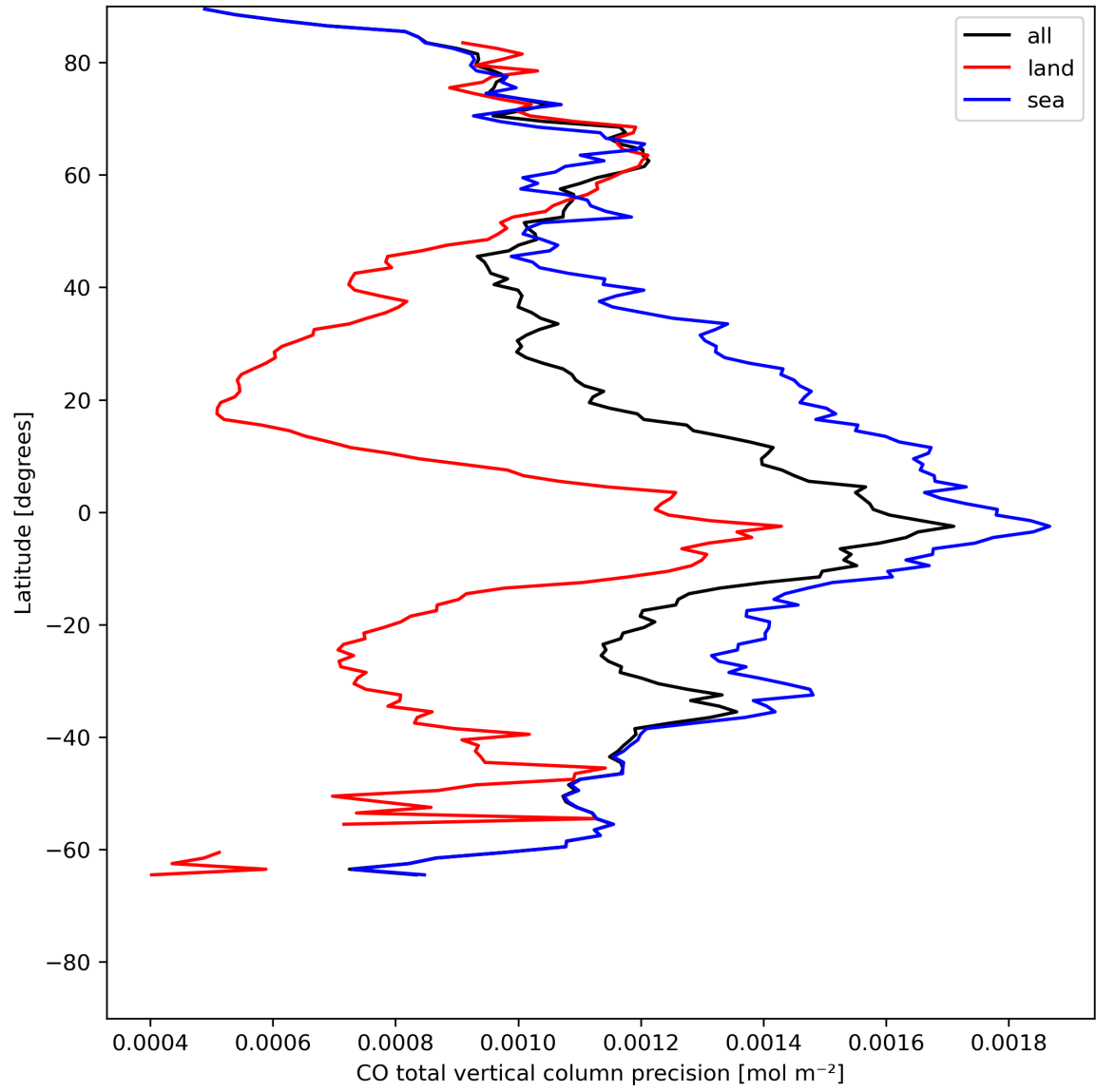
Figure 12: Zonal average of “CO total vertical column precision” for 2024-05-18 to 2024-05-20.
