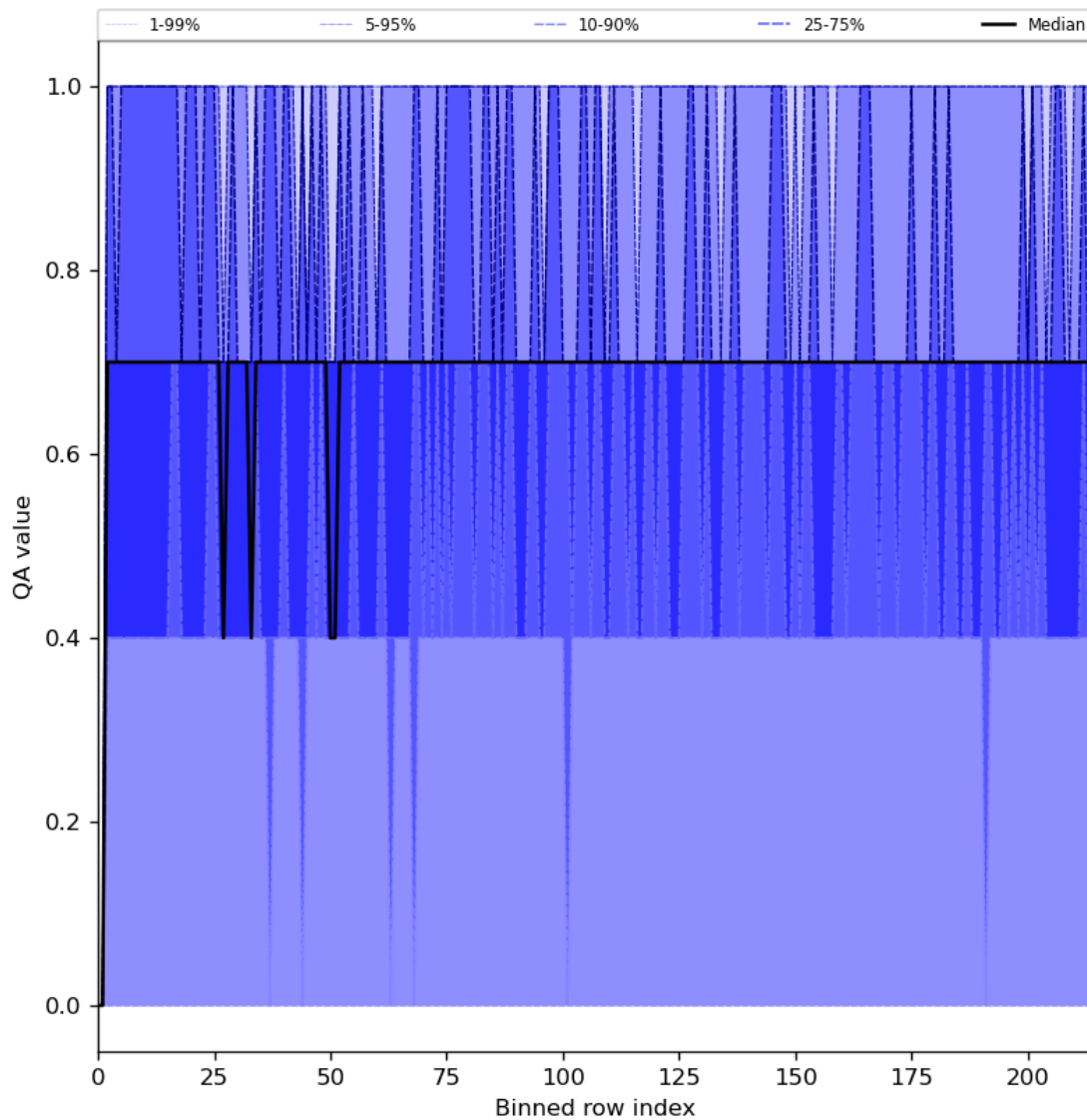
Figure 25: Along track statistics of “QA value” for 2024-05-18 to 2024-05-20
