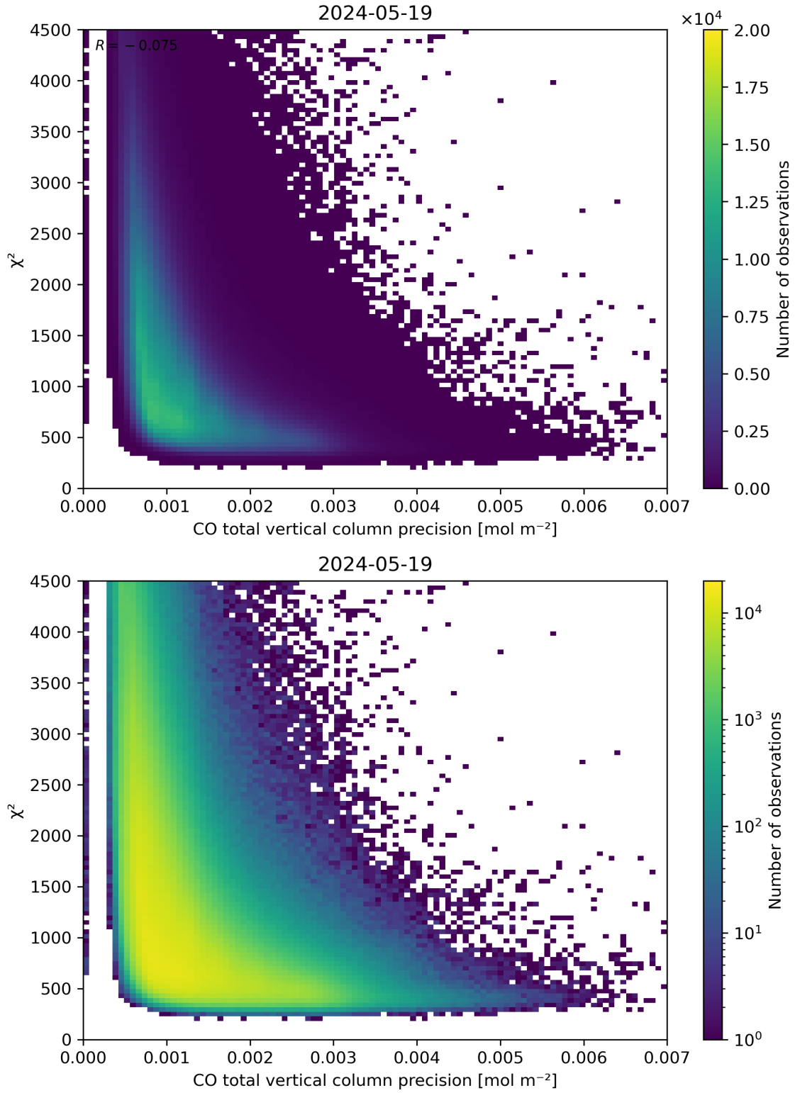
Figure 44: Scatter density plot of “CO total vertical column precision” against “ \chi^2 ” for 2024-05-18 to 2024-05-20.
