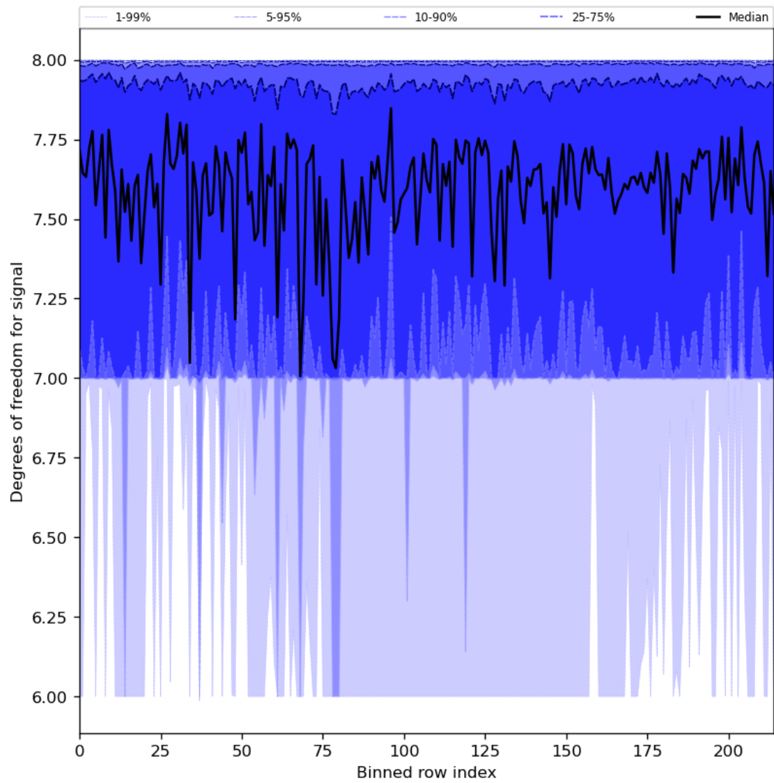
Figure 31: Along track statistics of “Degrees of freedom for signal” for 2024-05-18 to 2024-05-20
