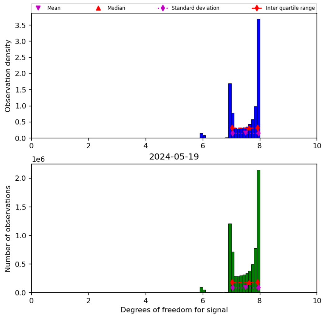
Figure 23: Histogram of “Degrees of freedom for signal” for 2024-05-18 to 2024-05-20
