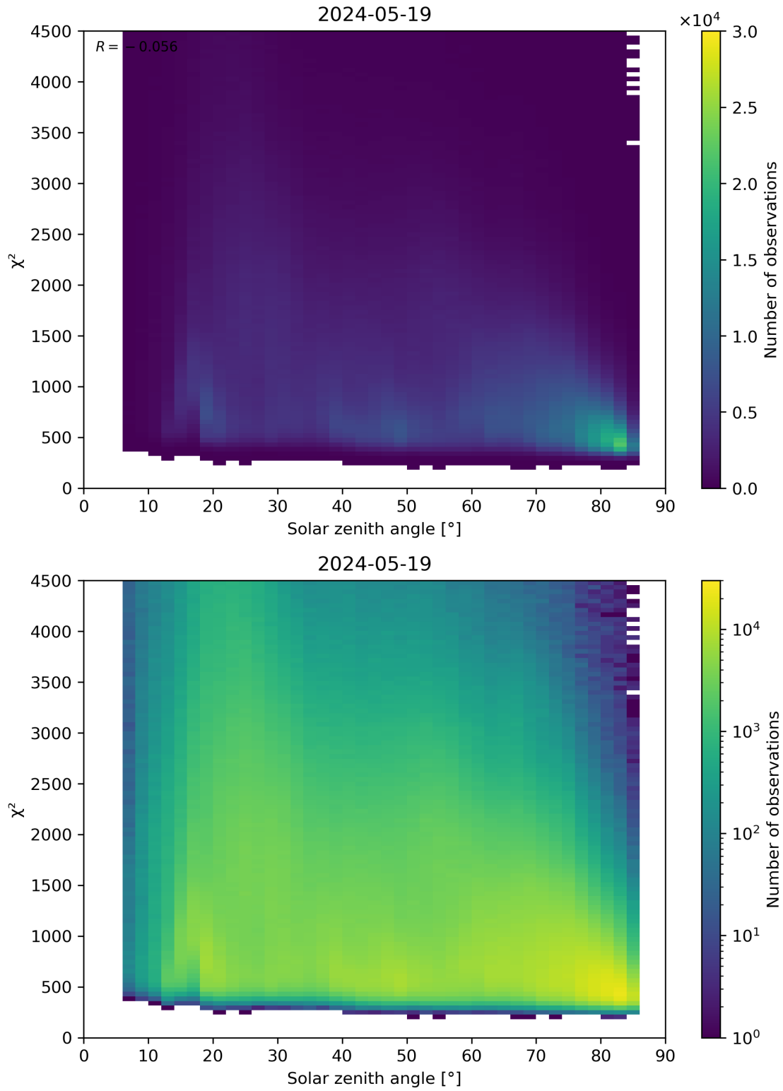
Figure 64: Scatter density plot of “Solar zenith angle” against “ \chi^2 ” for 2024-05-18 to 2024-05-20.
