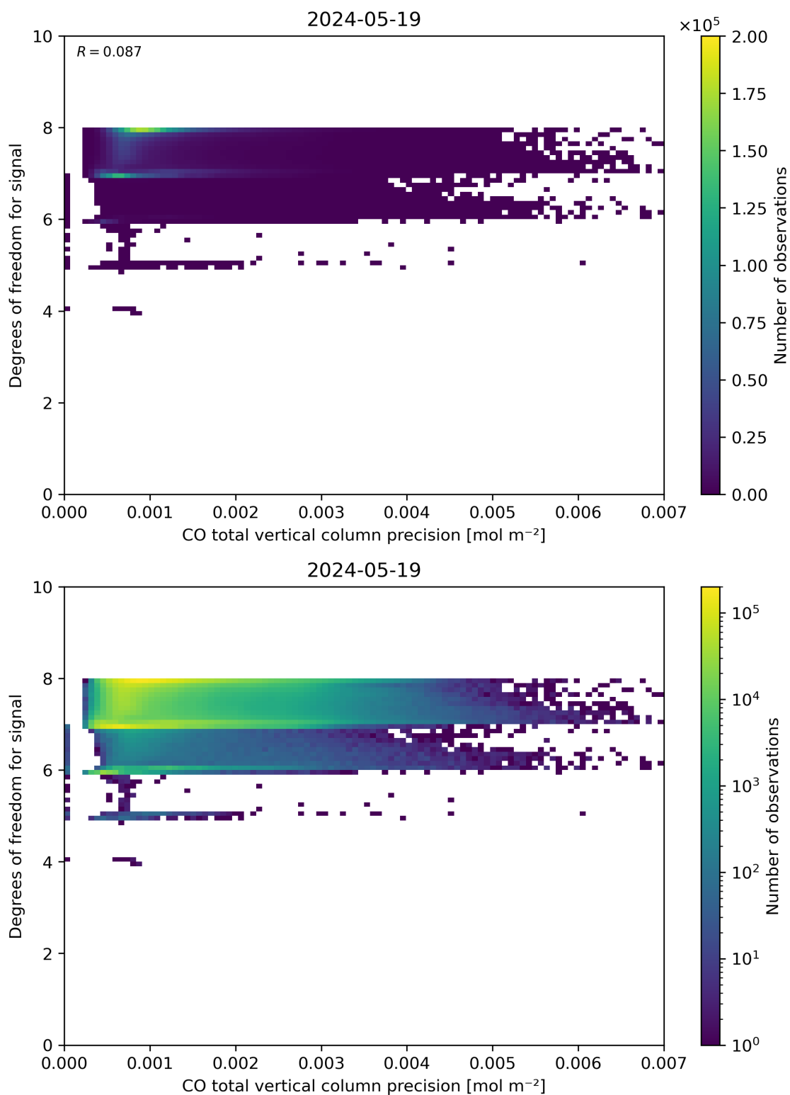
Figure 45: Scatter density plot of “CO total vertical column precision” against “Degrees of freedom for signal” for 2024-05-18 to 2024-05-20.
