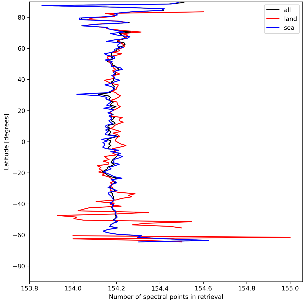
Figure 13: Zonal average of “Number of spectral points in retrieval” for 2024-05-18 to 2024-05-20.
