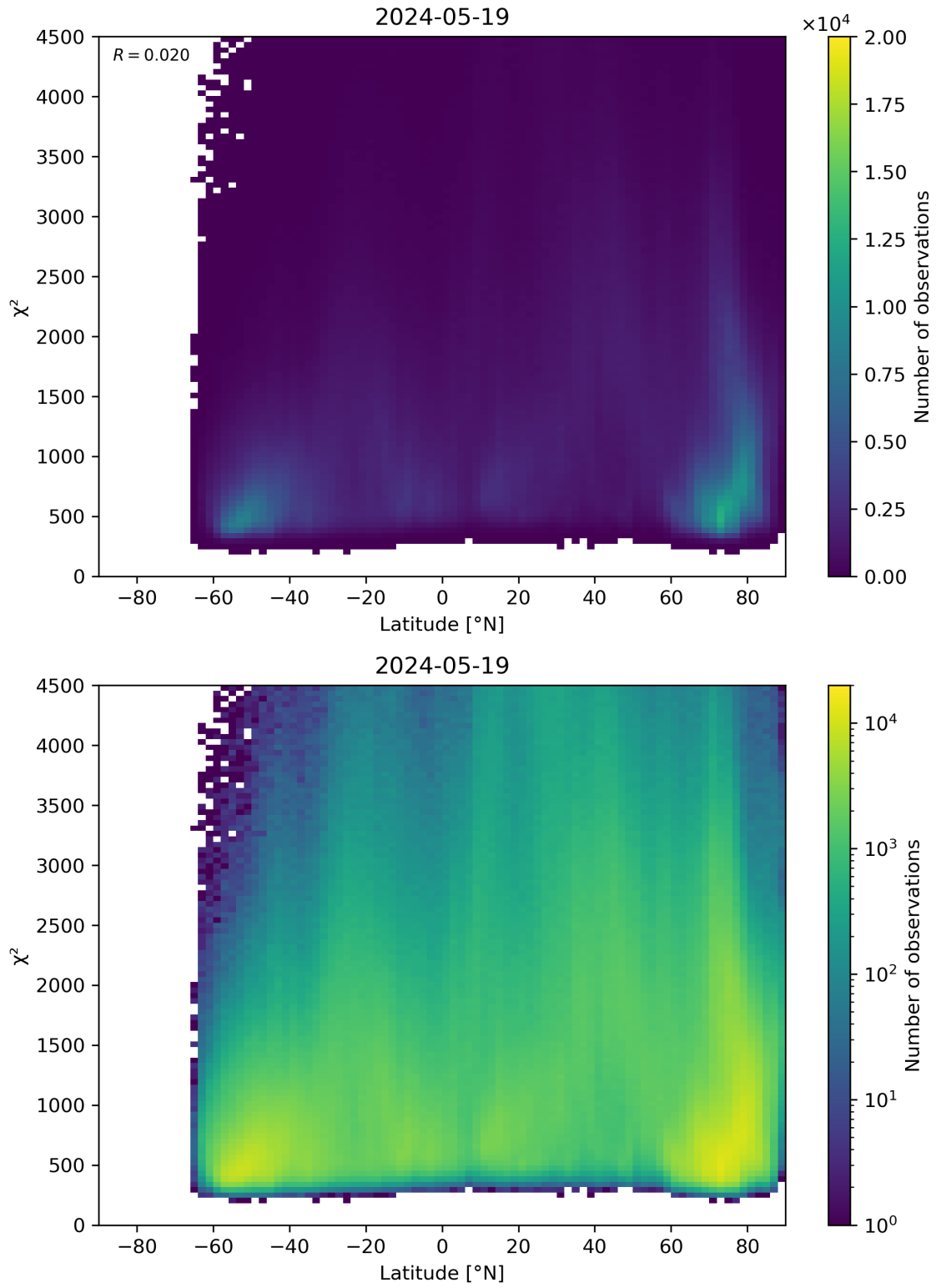
Figure 54: Scatter density plot of “Latitude” against “ \chi^2 ” for 2024-05-18 to 2024-05-20.
