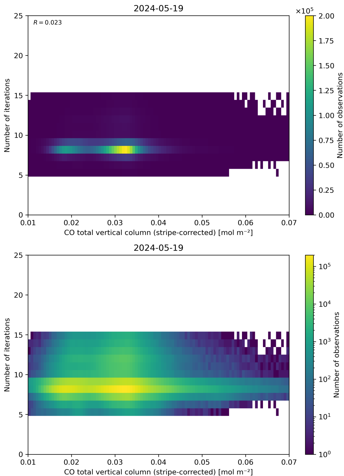
Figure 39: Scatter density plot of “CO total vertical column (stripe-corrected)” against “Number of iterations” for 2024-05-18 to 2024-05-20.
