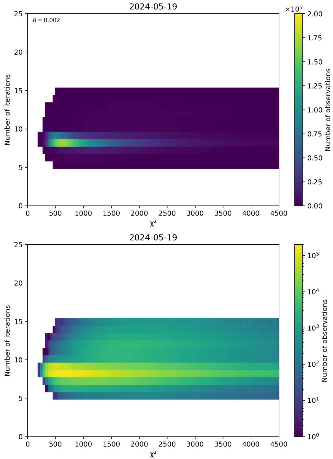
Figure 49: Scatter density plot of “ \chi^2 ” against “Number of iterations” for 2024-05-18 to 2024-05-20.
