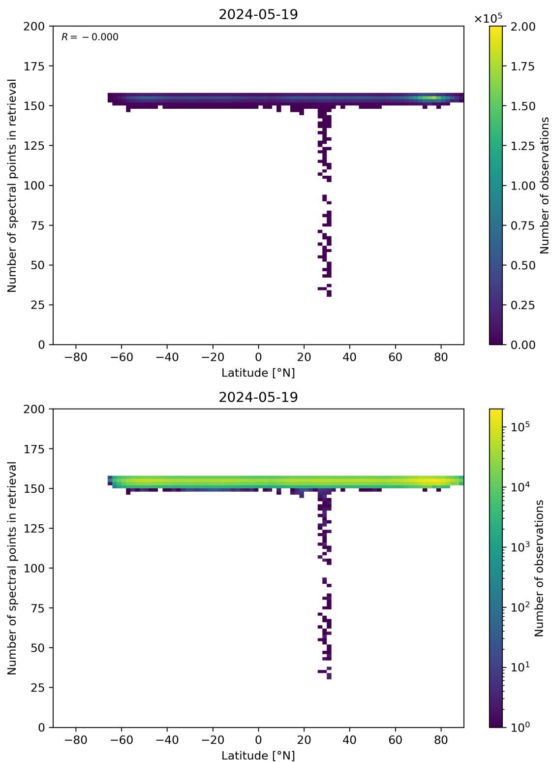
Figure 57: Scatter density plot of “Latitude” against “Number of spectral points in retrieval” for 2024-05-18 to 2024-05-20.
