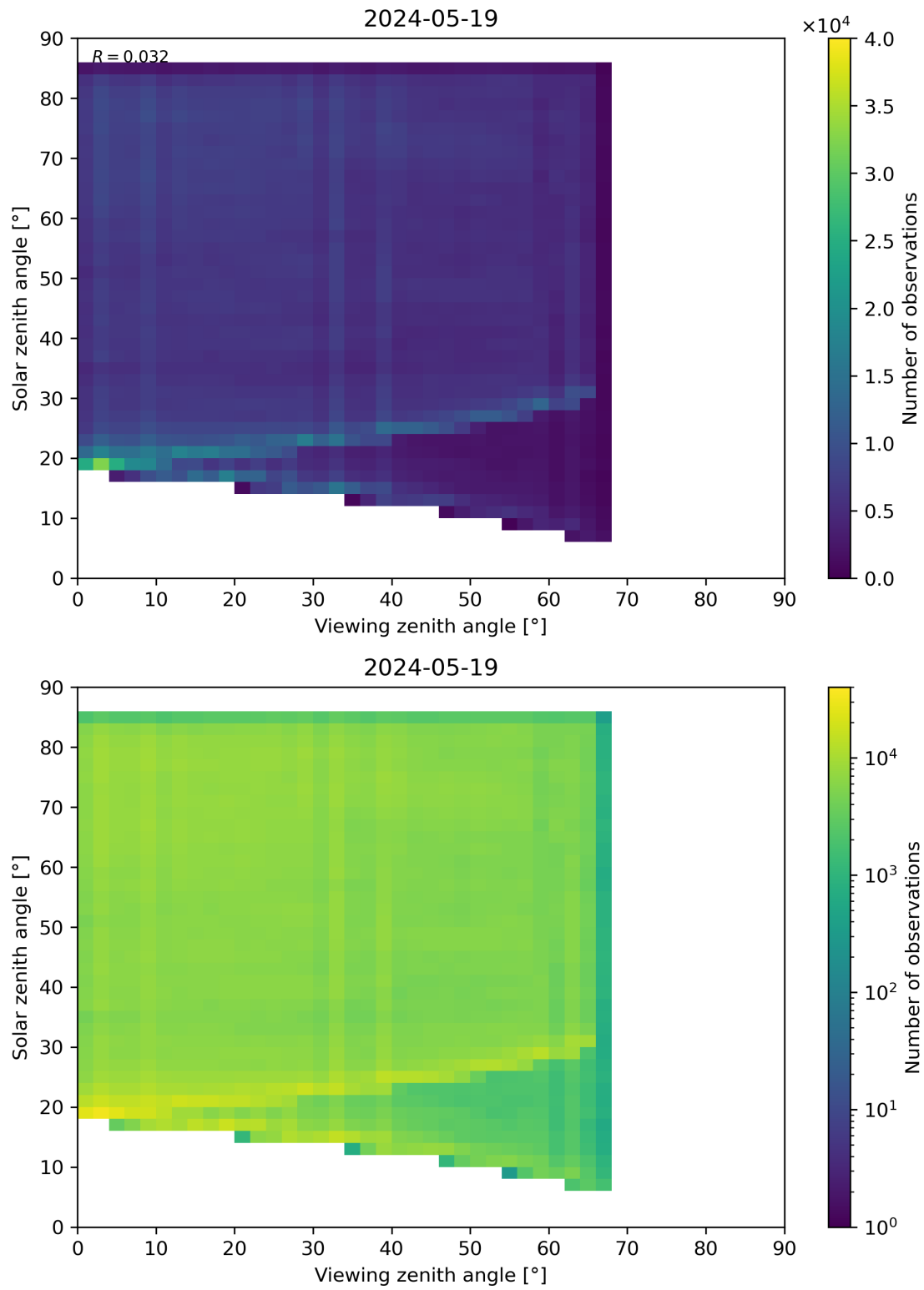
Figure 77: Scatter density plot of “Viewing zenith angle” against “Solar zenith angle” for 2024-05-18 to 2024-05-20.
