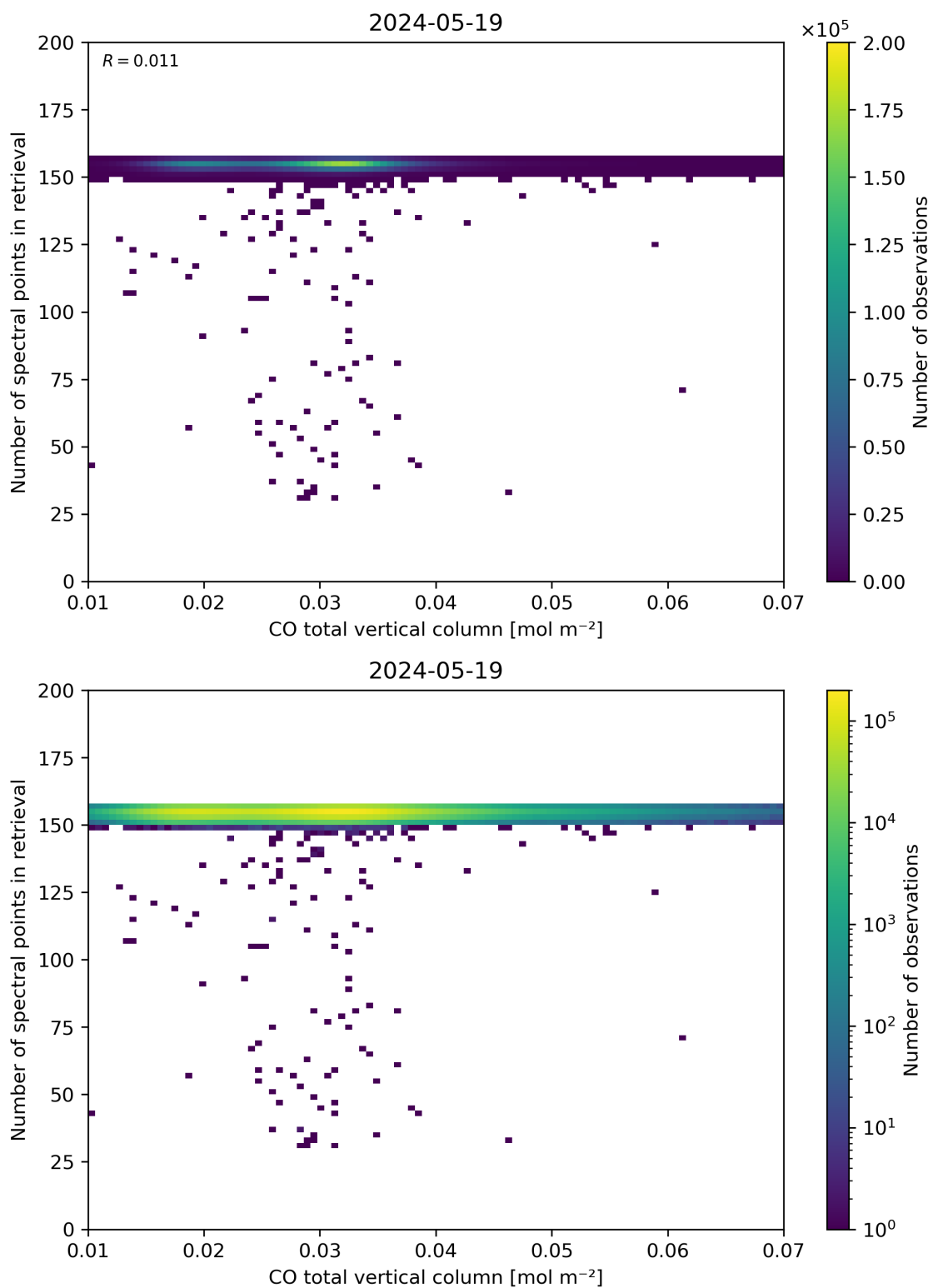
Figure 43: Scatter density plot of “CO total vertical column” against “Number of spectral points in retrieval” for 2024-05-18 to 2024-05-20.
