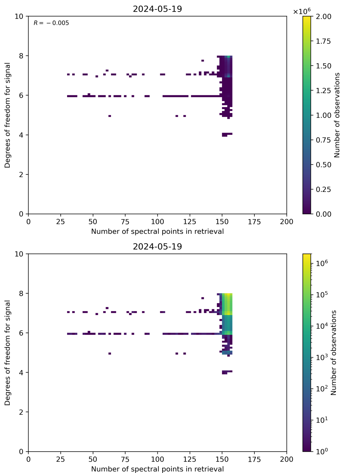
Figure 59: Scatter density plot of “Number of spectral points in retrieval” against “Degrees of freedom for signal” for 2024-05-18 to 2024-05-20.
