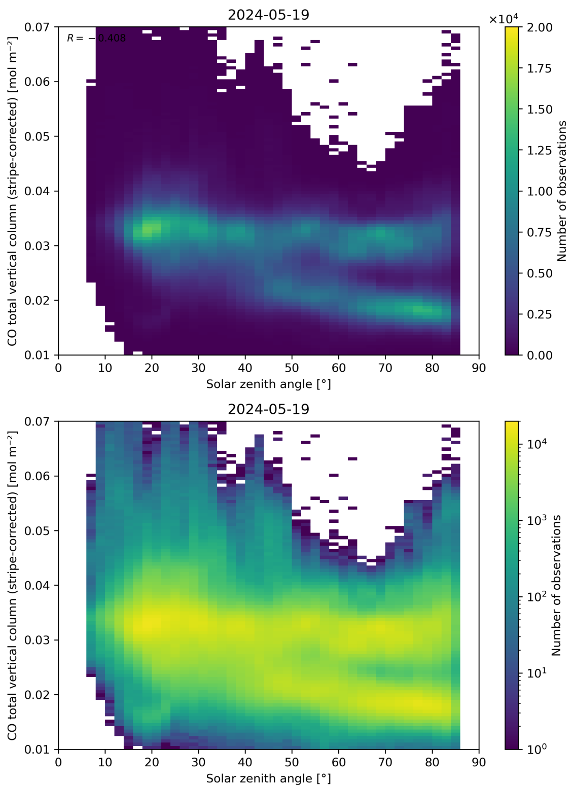
Figure 62: Scatter density plot of “Solar zenith angle” against “CO total vertical column (stripe-corrected)” for 2024-05-18 to 2024-05-20.
