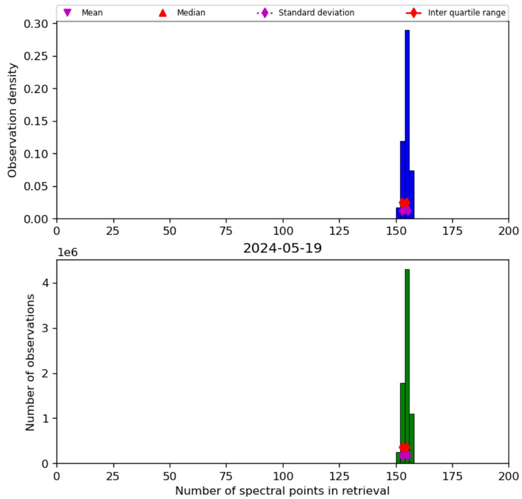
Figure 21: Histogram of “Number of spectral points in retrieval” for 2024-05-18 to 2024-05-20
