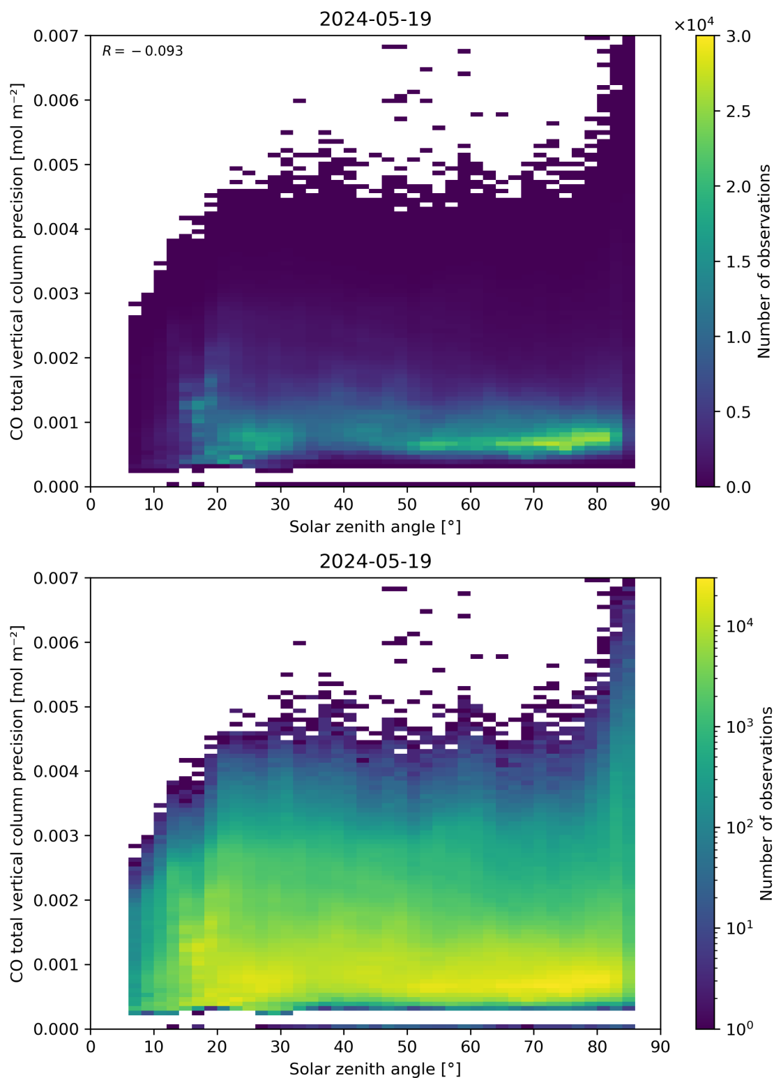
Figure 63: Scatter density plot of “Solar zenith angle” against “CO total vertical column precision” for 2024-05-18 to 2024-05-20.
