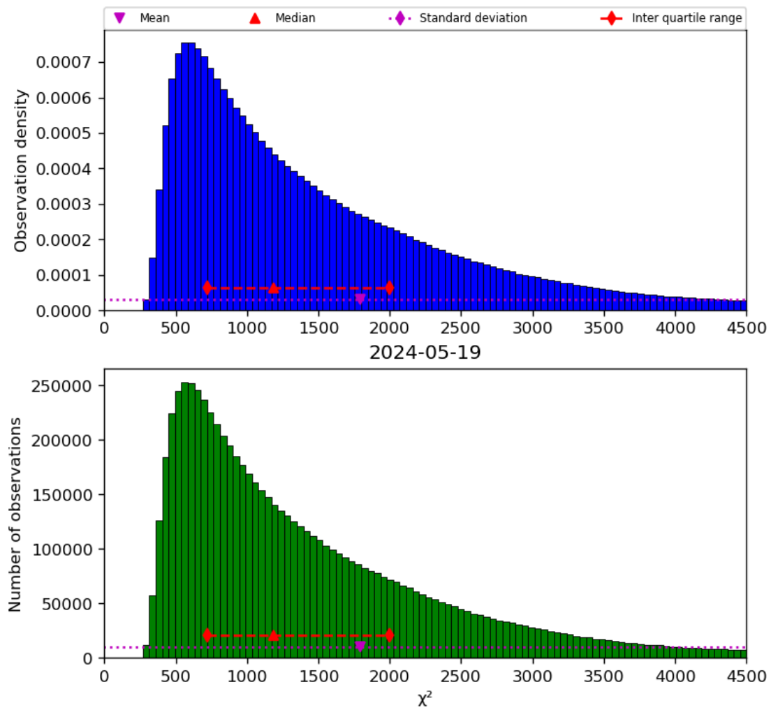
Figure 22: Histogram of “ \chi^2 ” for 2024-05-18 to 2024-05-20
