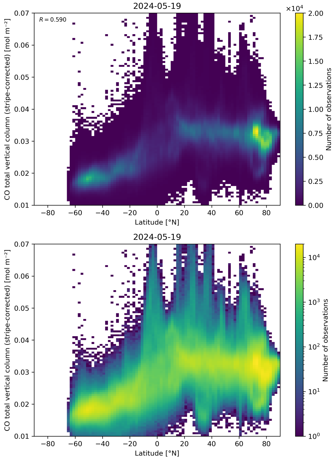
Figure 52: Scatter density plot of “Latitude” against “CO total vertical column (stripe-corrected)” for 2024-05-18 to 2024-05-20.
