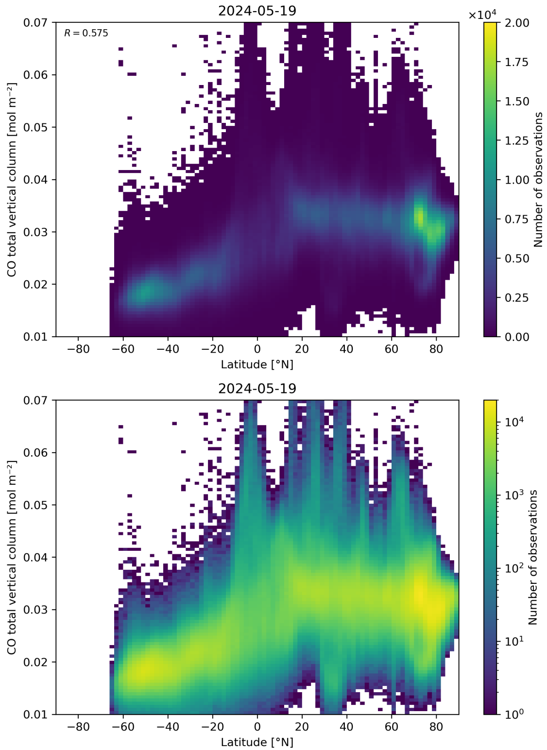
Figure 51: Scatter density plot of “Latitude” against “CO total vertical column” for 2024-05-18 to 2024-05-20.
