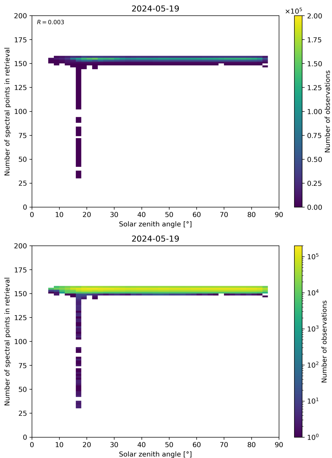
Figure 68: Scatter density plot of “Solar zenith angle” against “Number of spectral points in retrieval” for 2024-05-18 to 2024-05-20.
