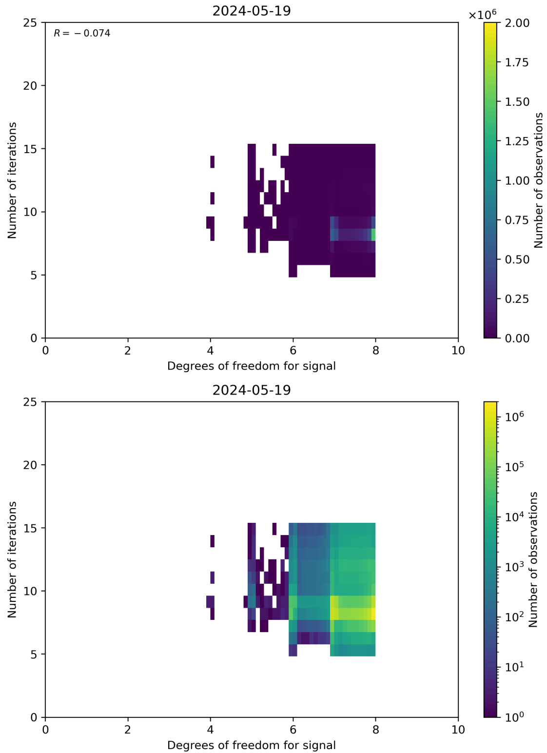
Figure 50: Scatter density plot of “Degrees of freedom for signal” against “Number of iterations” for 2024-05-18 to 2024-05-20.
