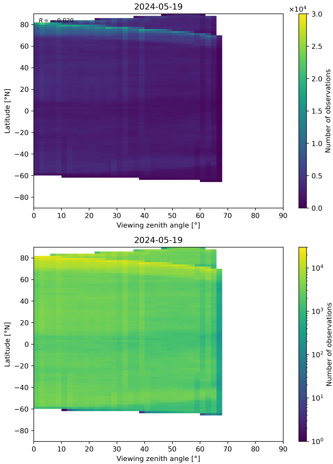
Figure 74: Scatter density plot of “Viewing zenith angle” against “Latitude” for 2024-05-18 to 2024-05-20.
