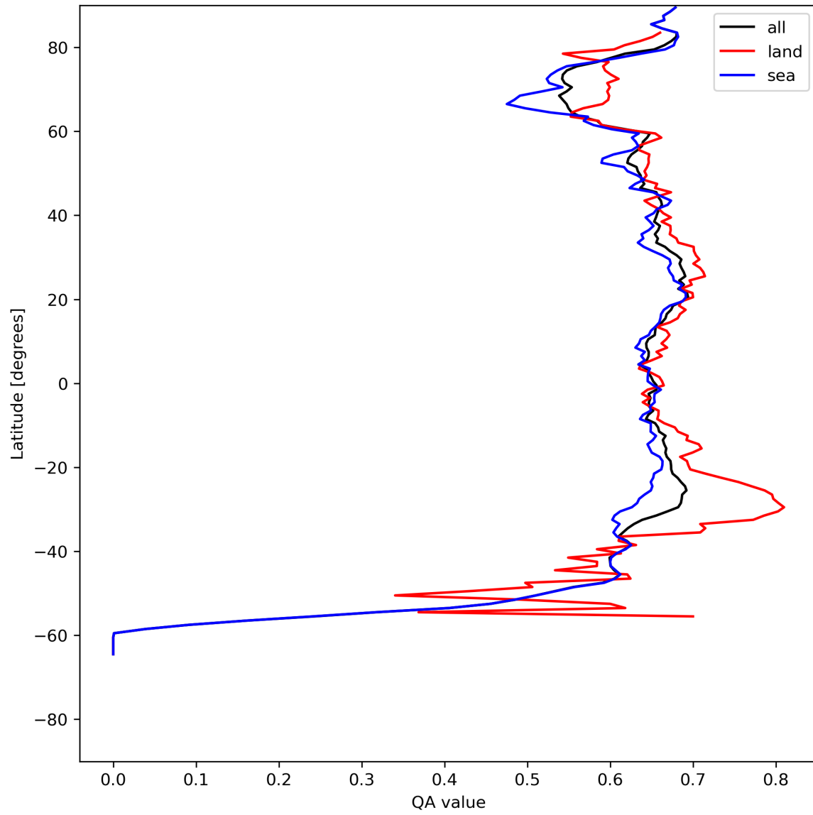
Figure 9: Zonal average of “QA value” for 2024-05-18 to 2024-05-20.
