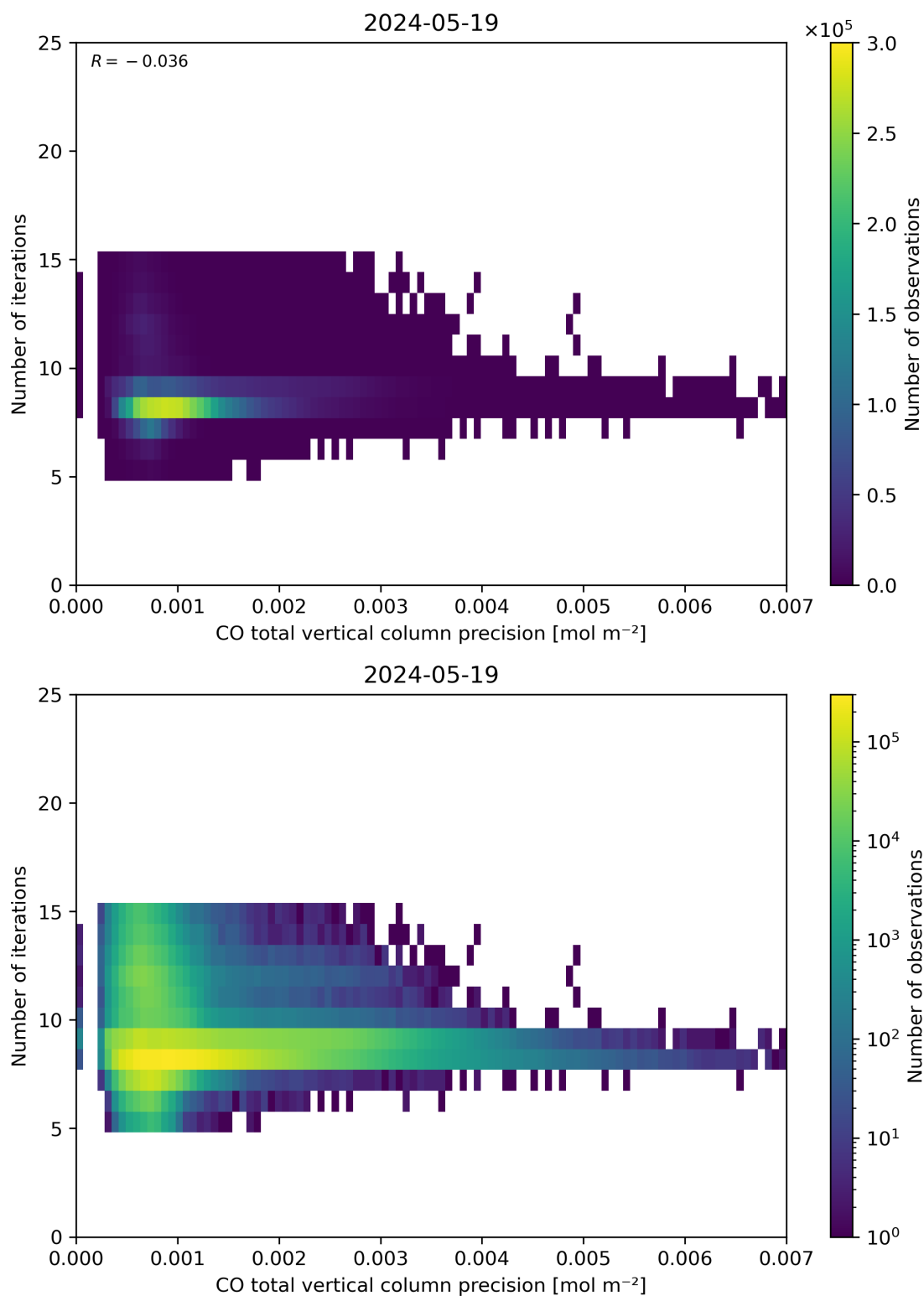
Figure 46: Scatter density plot of “CO total vertical column precision” against “Number of iterations” for 2024-05-18 to 2024-05-20.
