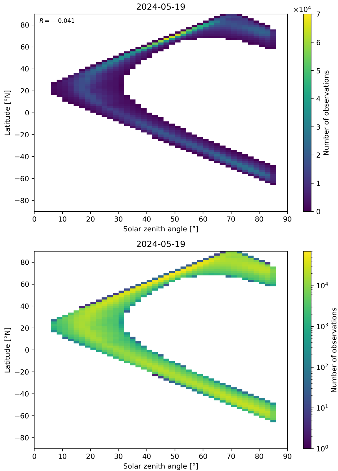
Figure 66: Scatter density plot of “Solar zenith angle” against “Latitude” for 2024-05-18 to 2024-05-20.
