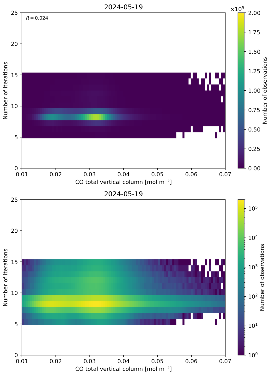
Figure 42: Scatter density plot of “CO total vertical column” against “Number of iterations” for 2024-05-18 to 2024-05-20.
