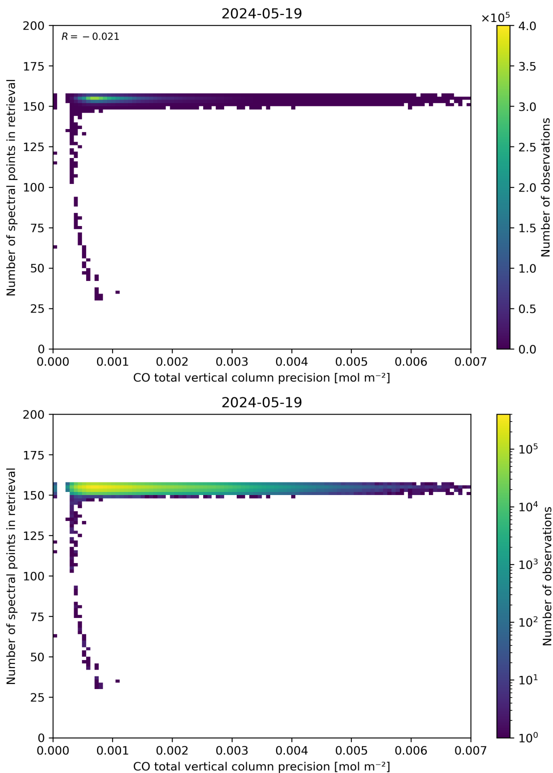
Figure 47: Scatter density plot of “CO total vertical column precision” against “Number of spectral points in retrieval” for 2024-05-18 to 2024-05-20.
