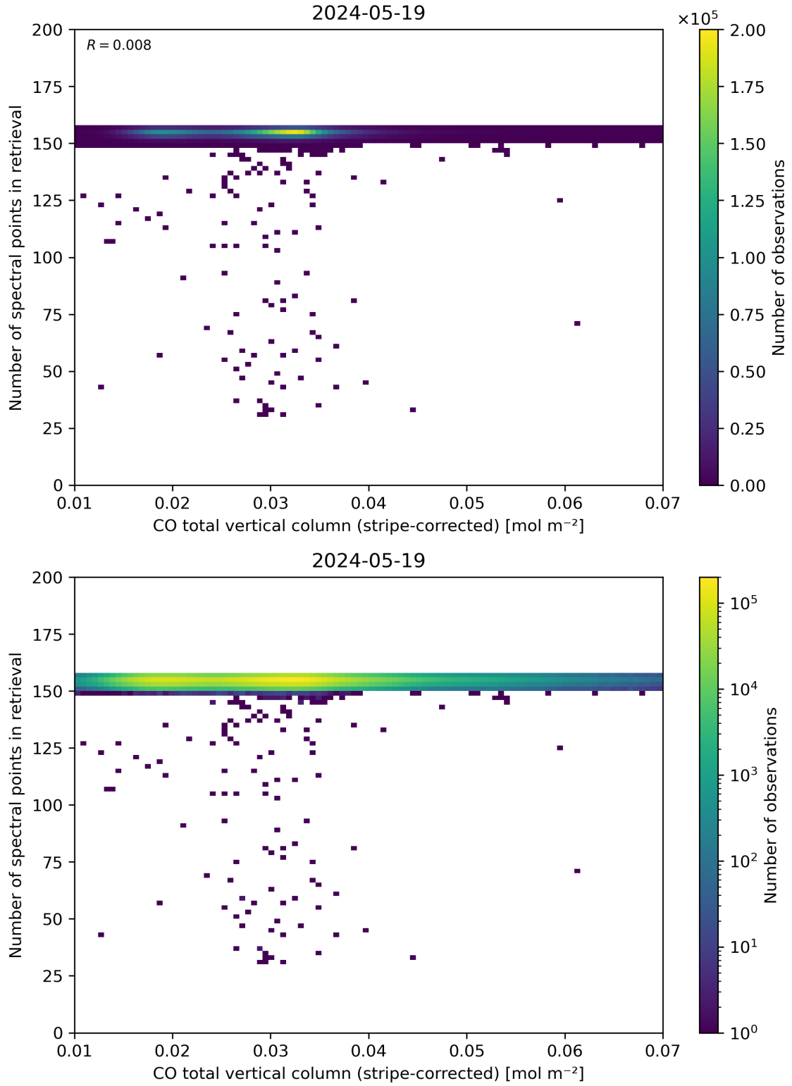
Figure 40: Scatter density plot of “CO total vertical column (stripe-corrected)” against “Number of spectral points in retrieval” for 2024-05-18 to 2024-05-20.
