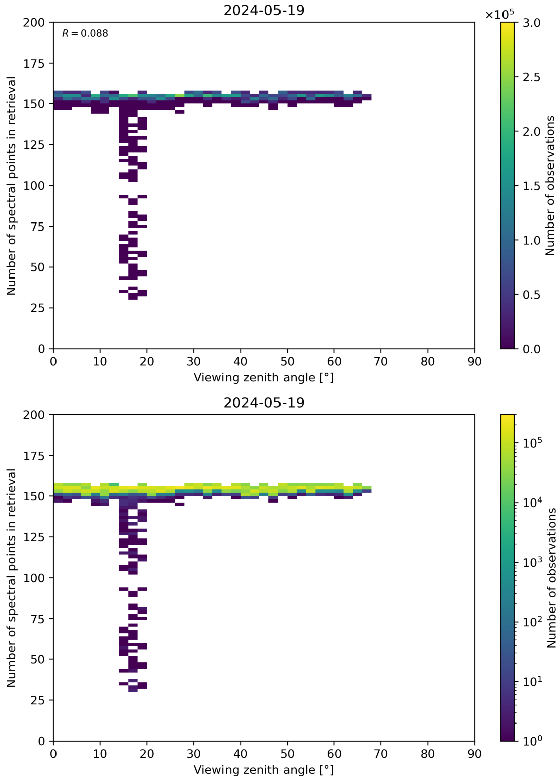
Figure 76: Scatter density plot of “Viewing zenith angle” against “Number of spectral points in retrieval” for 2024-05-18 to 2024-05-20.
