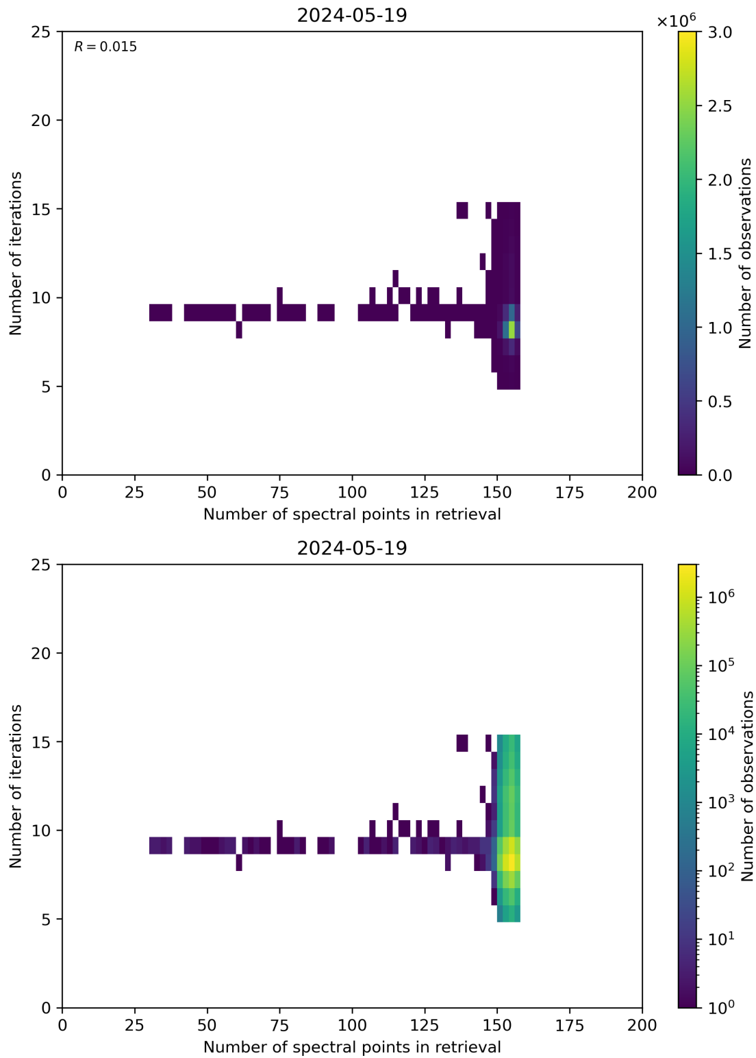
Figure 60: Scatter density plot of “Number of spectral points in retrieval” against “Number of iterations” for 2024-05-18 to 2024-05-20.
