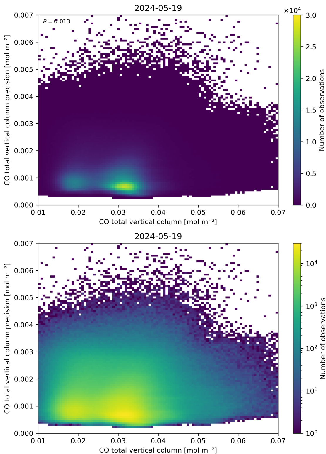
Figure 34: Scatter density plot of “CO total vertical column” against “CO total vertical column precision” for 2024-05-18 to 2024-05-20.
