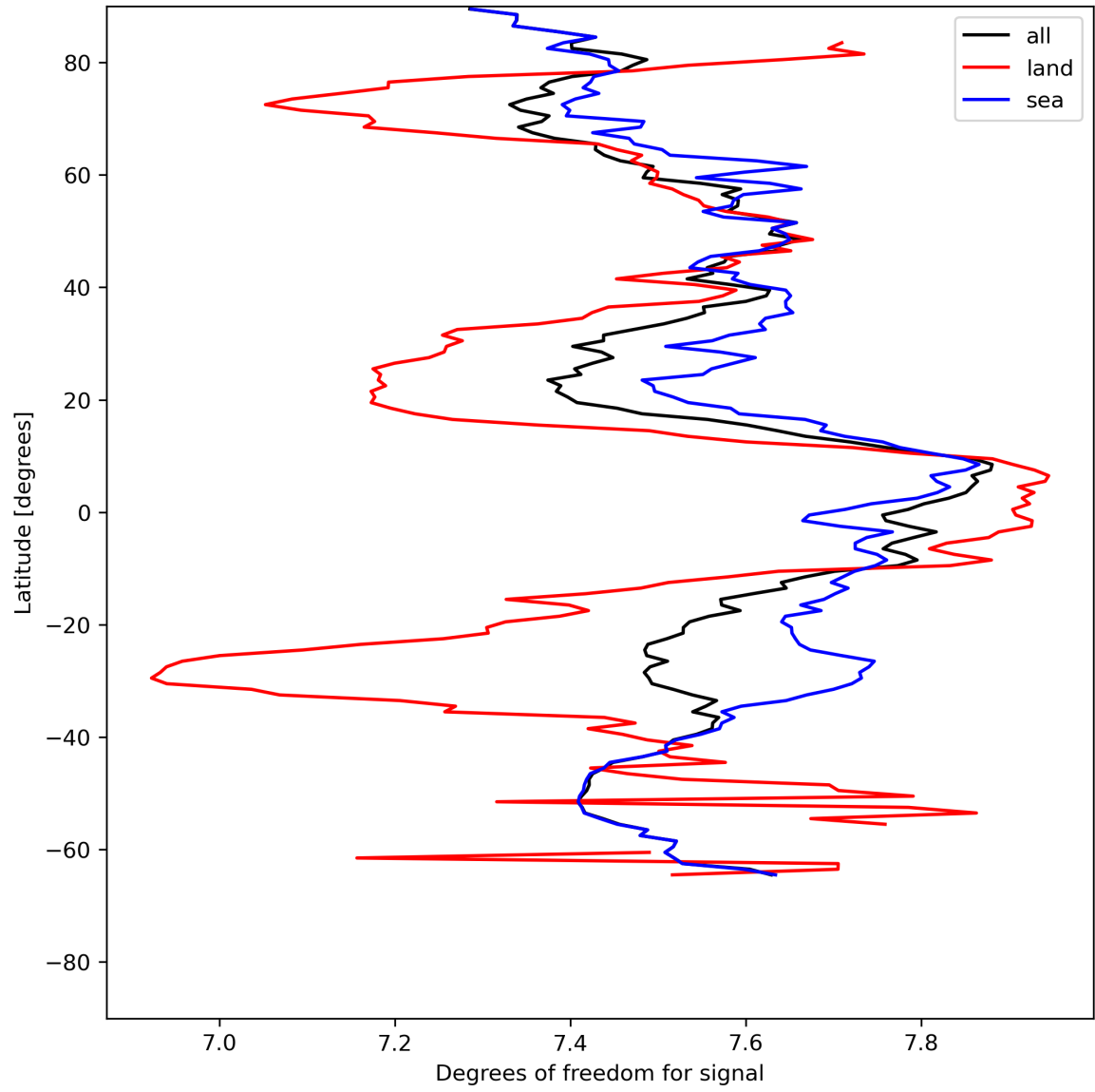
Figure 15: Zonal average of “Degrees of freedom for signal” for 2024-05-18 to 2024-05-20.
