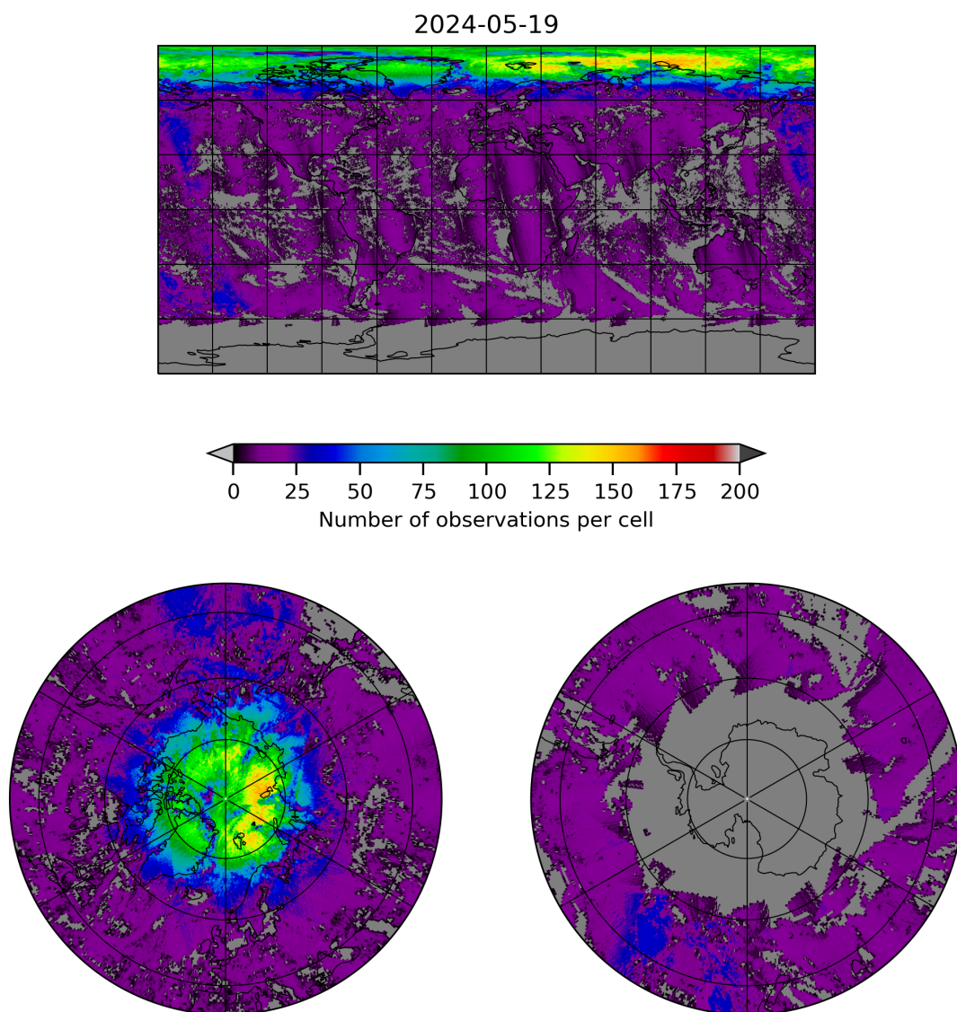
Figure 8: Map of the number of observations for 2024-05-18 to 2024-05-20
