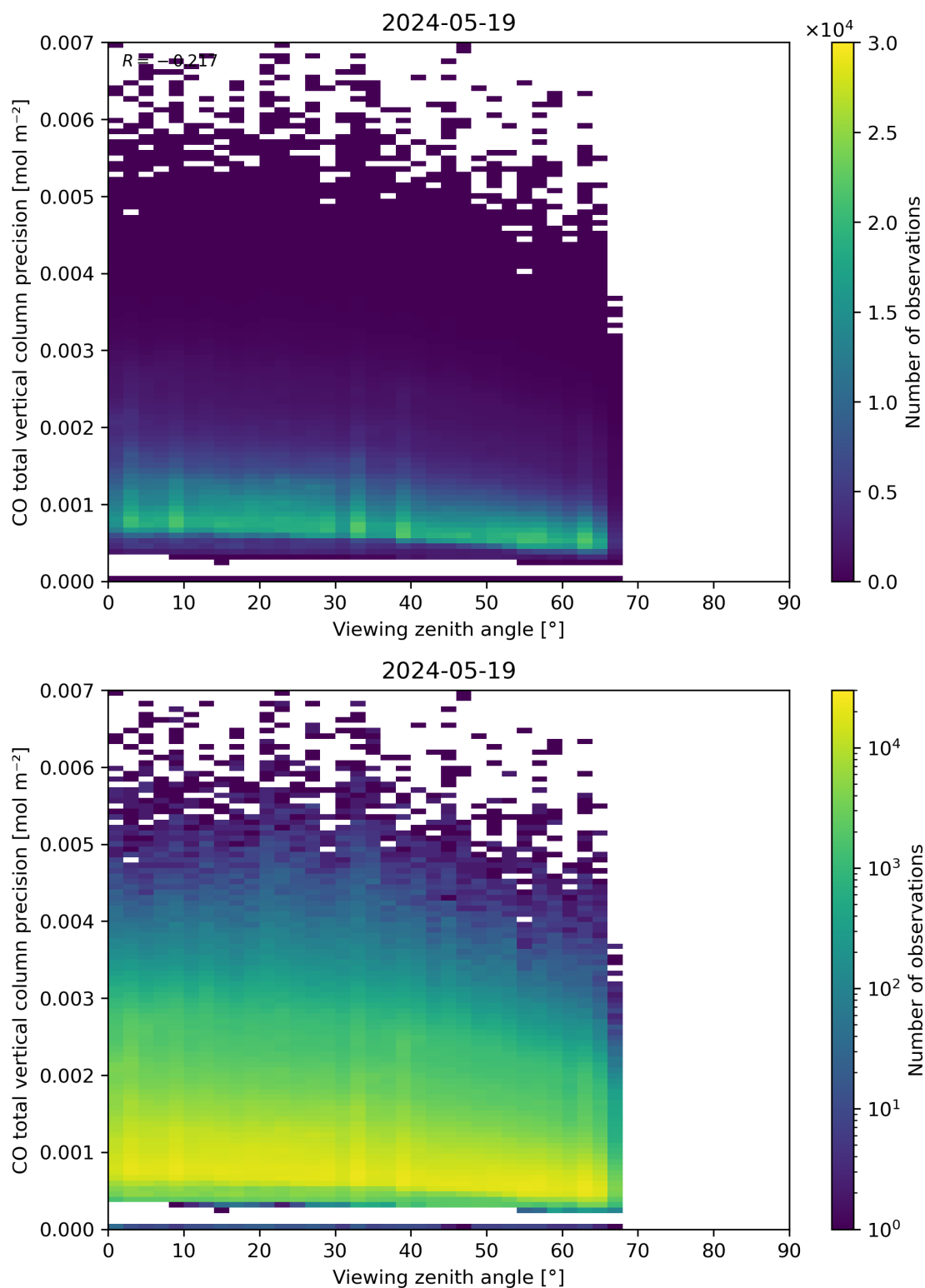
Figure 71: Scatter density plot of “Viewing zenith angle” against “CO total vertical column precision” for 2024-05-18 to 2024-05-20.
