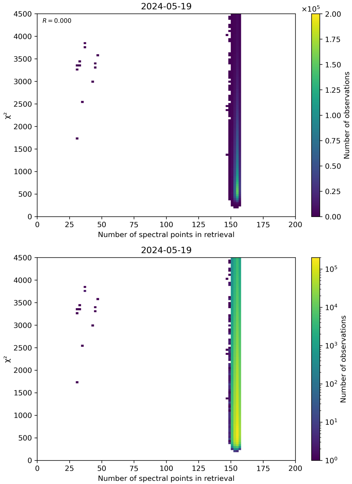
Figure 58: Scatter density plot of “Number of spectral points in retrieval” against “ \chi^2 ” for 2024-05-18 to 2024-05-20.
