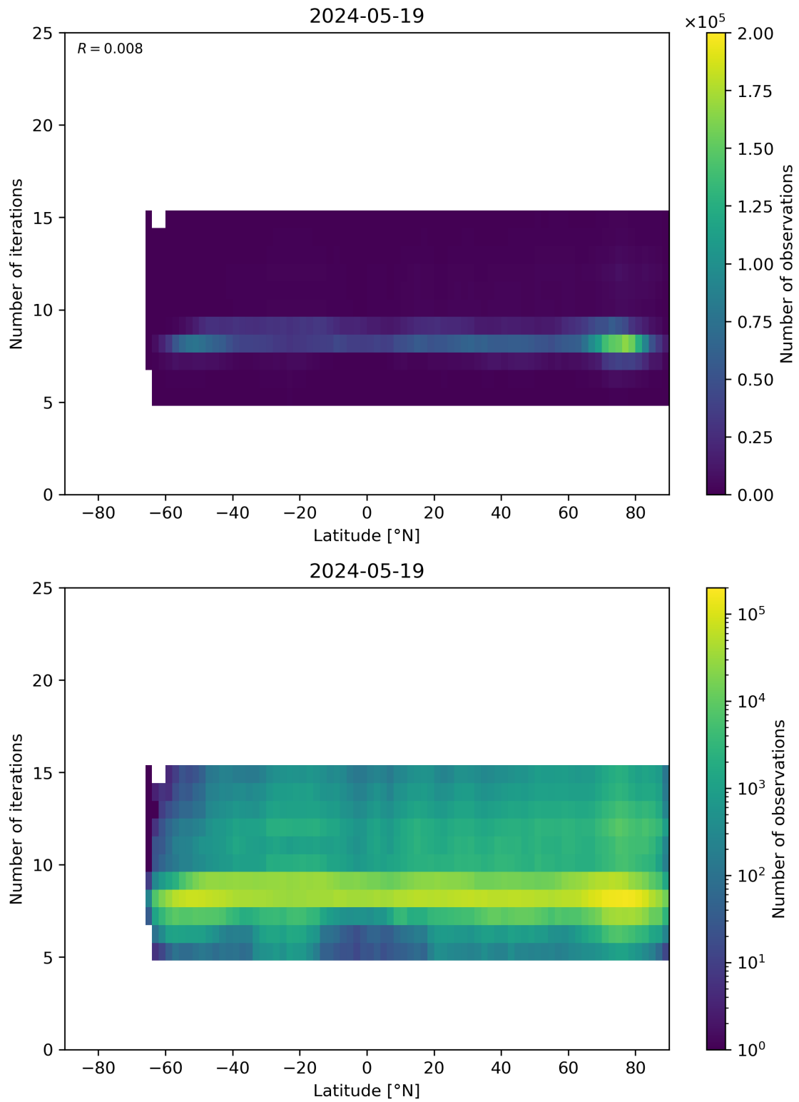
Figure 56: Scatter density plot of “Latitude” against “Number of iterations” for 2024-05-18 to 2024-05-20.
