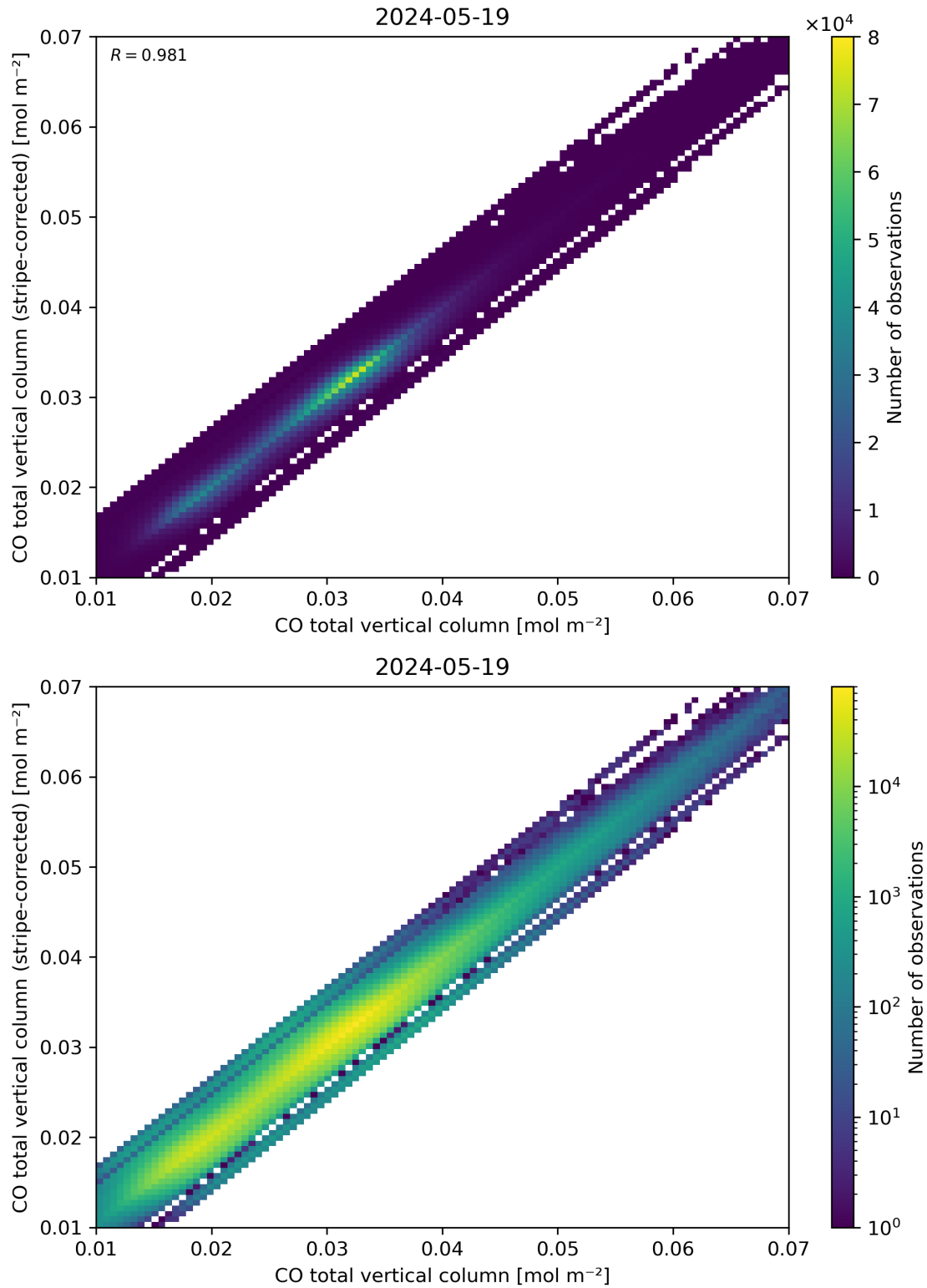
Figure 33: Scatter density plot of “CO total vertical column” against “CO total vertical column (stripe-corrected)” for 2024-05-18 to 2024-05-20.
