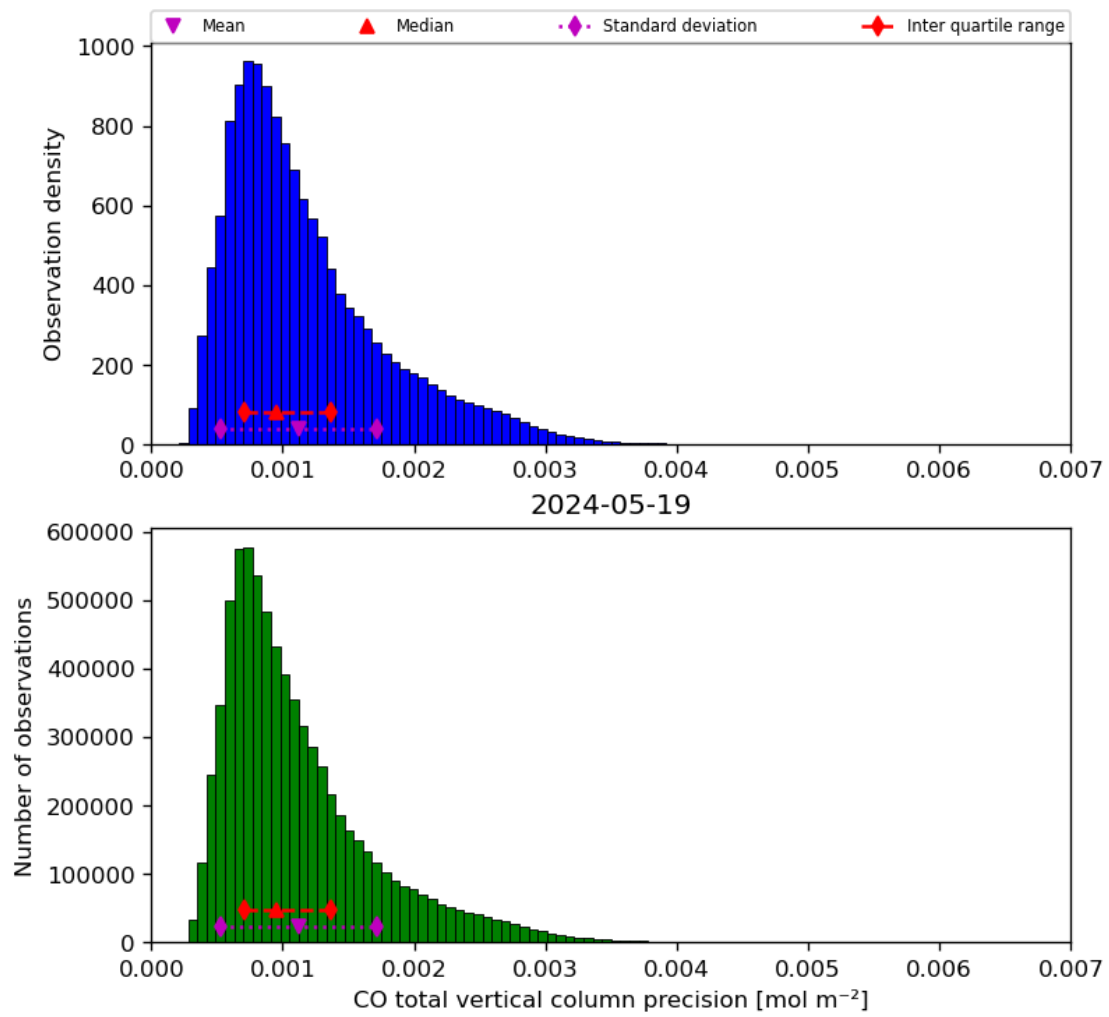
Figure 20: Histogram of “CO total vertical column precision” for 2024-05-18 to 2024-05-20
