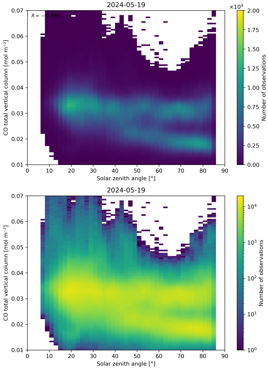
Figure 61: Scatter density plot of “Solar zenith angle” against “CO total vertical column” for 2024-05-18 to 2024-05-20.
