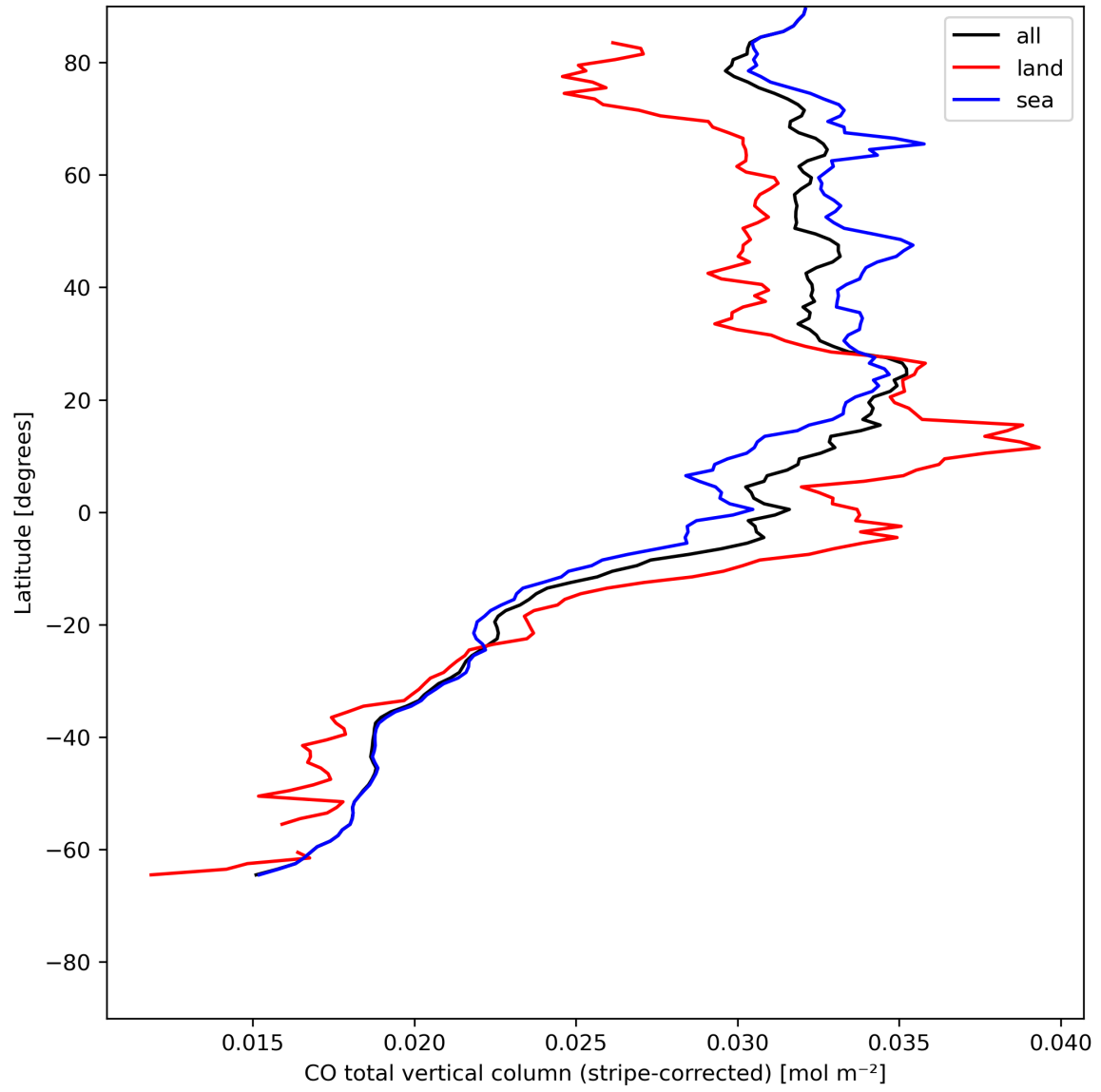
Figure 11: Zonal average of “CO total vertical column (stripe-corrected)” for 2024-05-18 to 2024-05-20.
