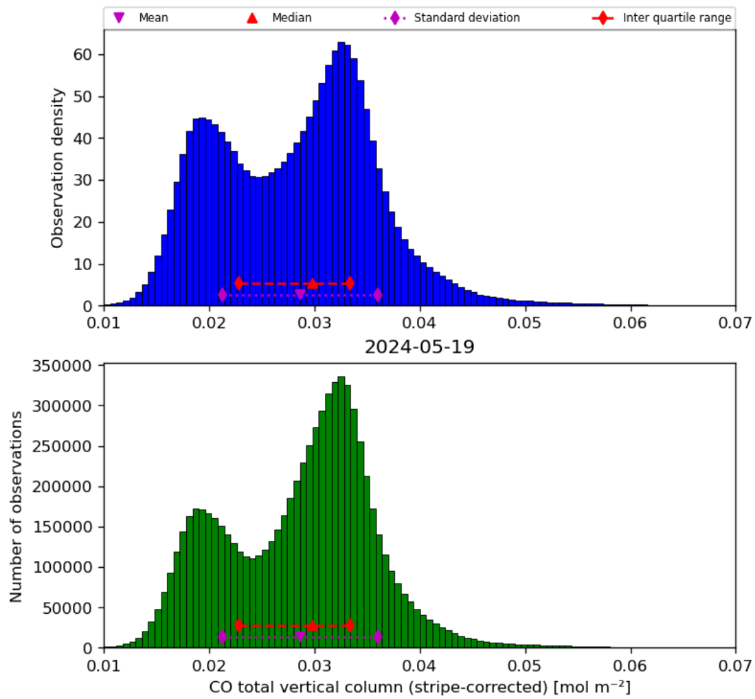
Figure 19: Histogram of “CO total vertical column (stripe-corrected)” for 2024-05-18 to 2024-05-20
