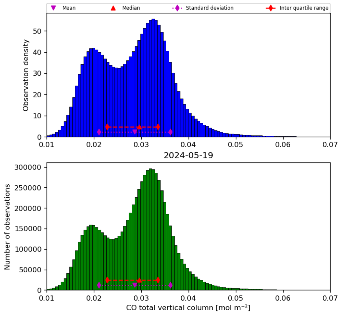
Figure 18: Histogram of “CO total vertical column” for 2024-05-18 to 2024-05-20
