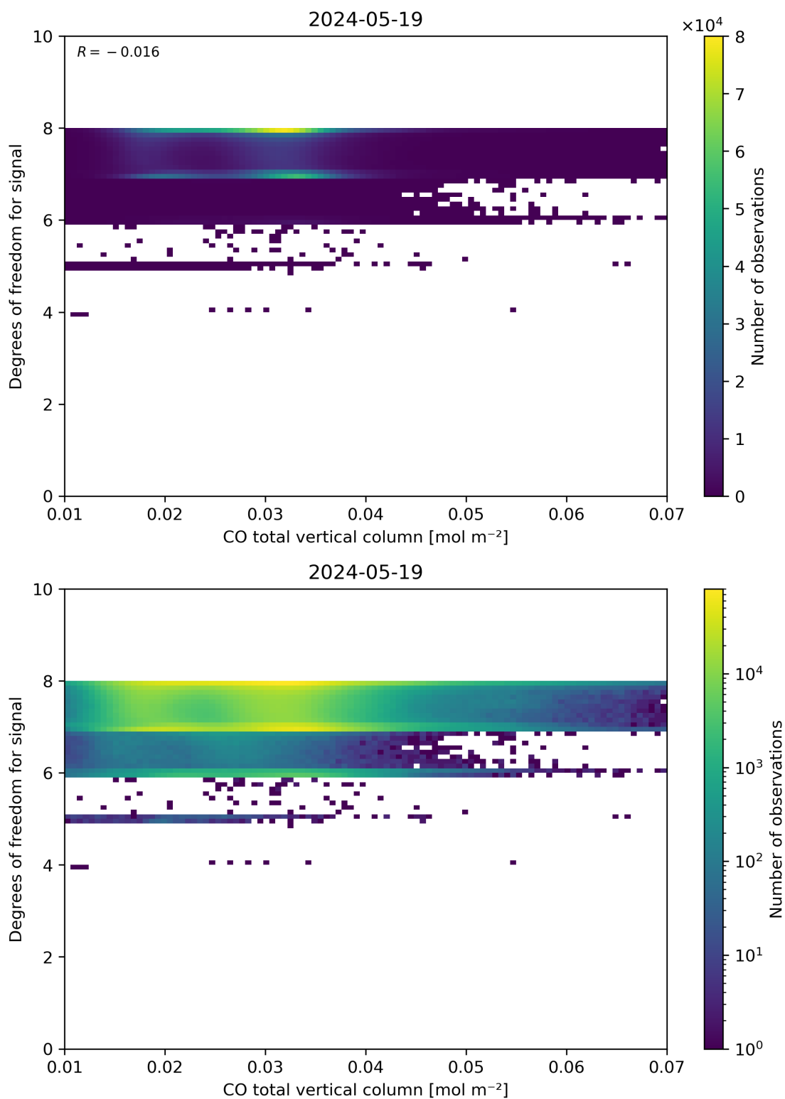
Figure 41: Scatter density plot of “CO total vertical column” against “Degrees of freedom for signal” for 2024-05-18 to 2024-05-20.
