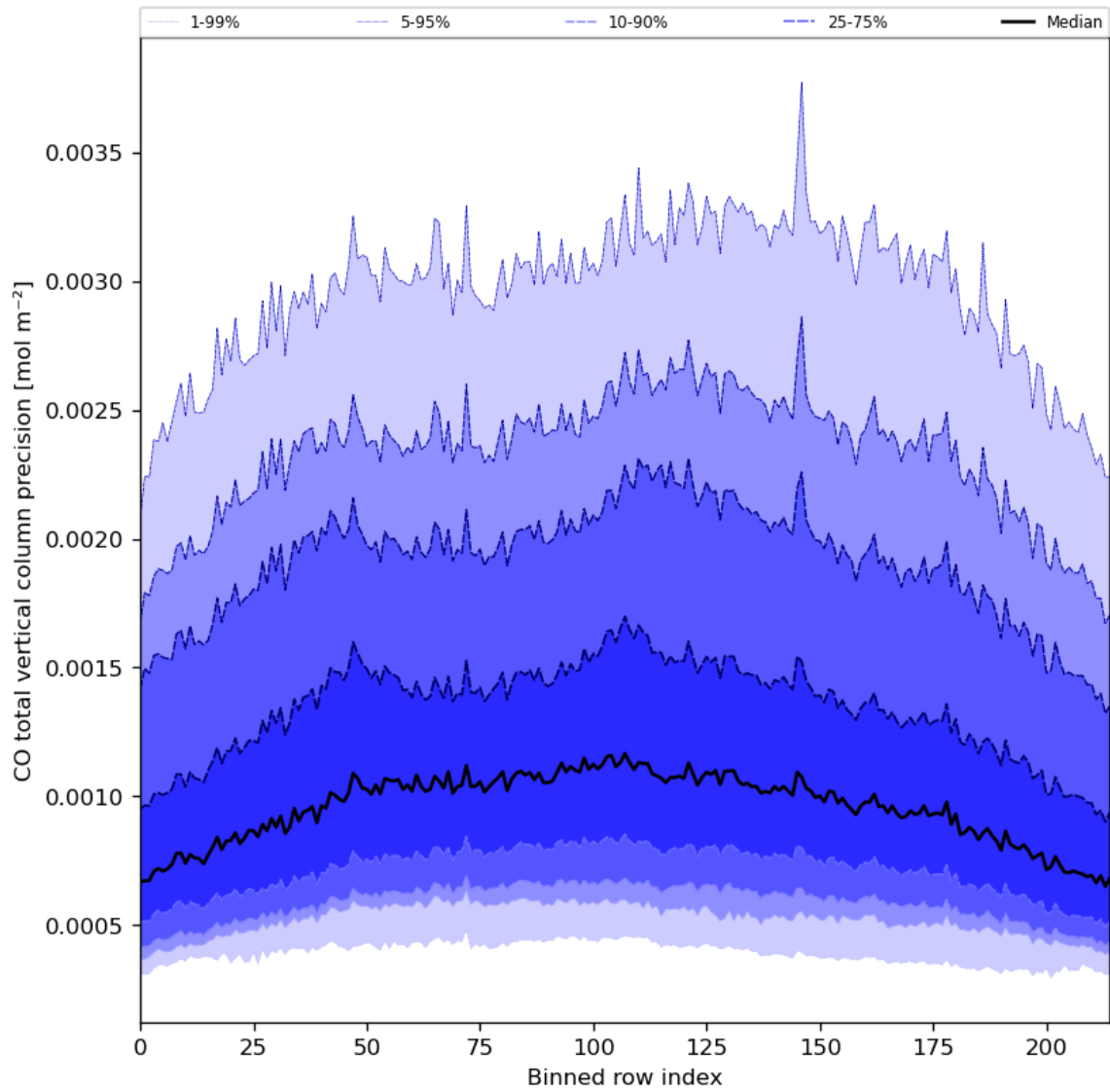
Figure 28: Along track statistics of “CO total vertical column precision” for 2024-05-18 to 2024-05-20
