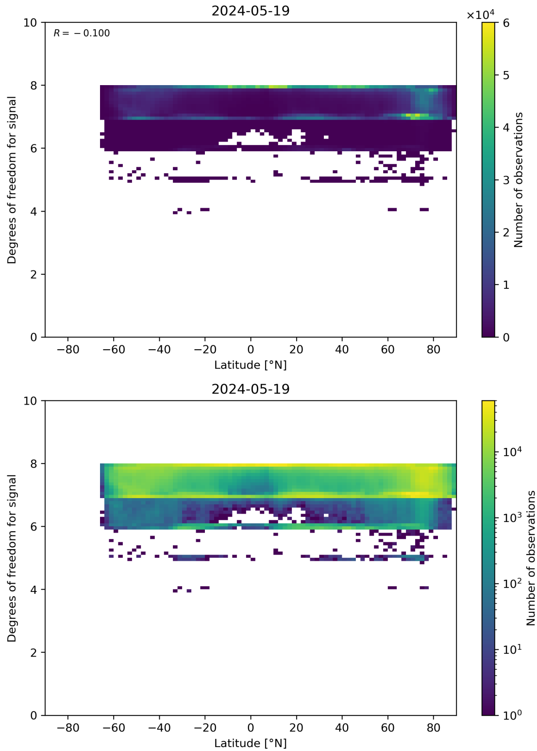
Figure 55: Scatter density plot of “Latitude” against “Degrees of freedom for signal” for 2024-05-18 to 2024-05-20.
