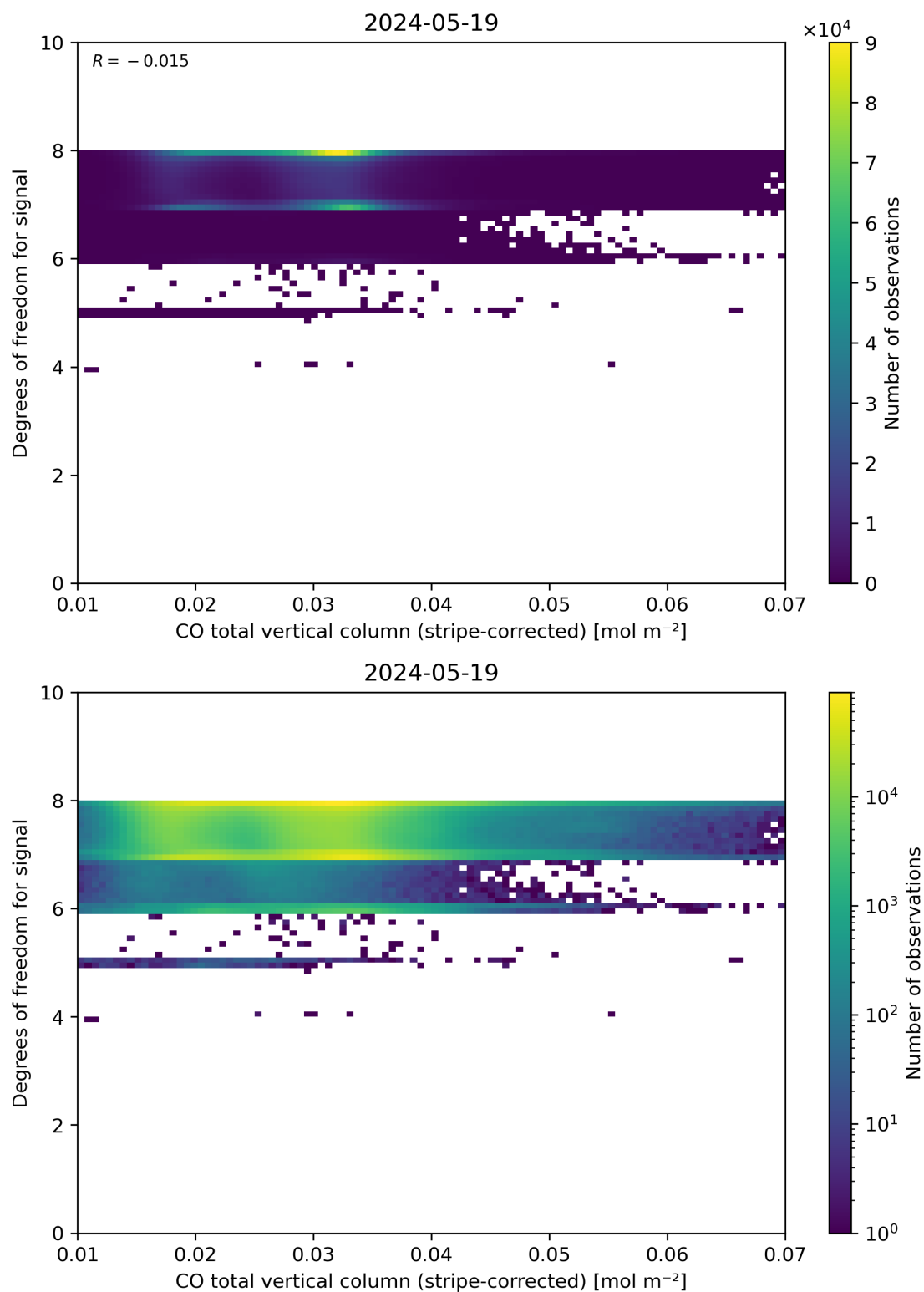
Figure 38: Scatter density plot of “CO total vertical column (stripe-corrected)” against “Degrees of freedom for signal” for 2024-05-18 to 2024-05-20.
