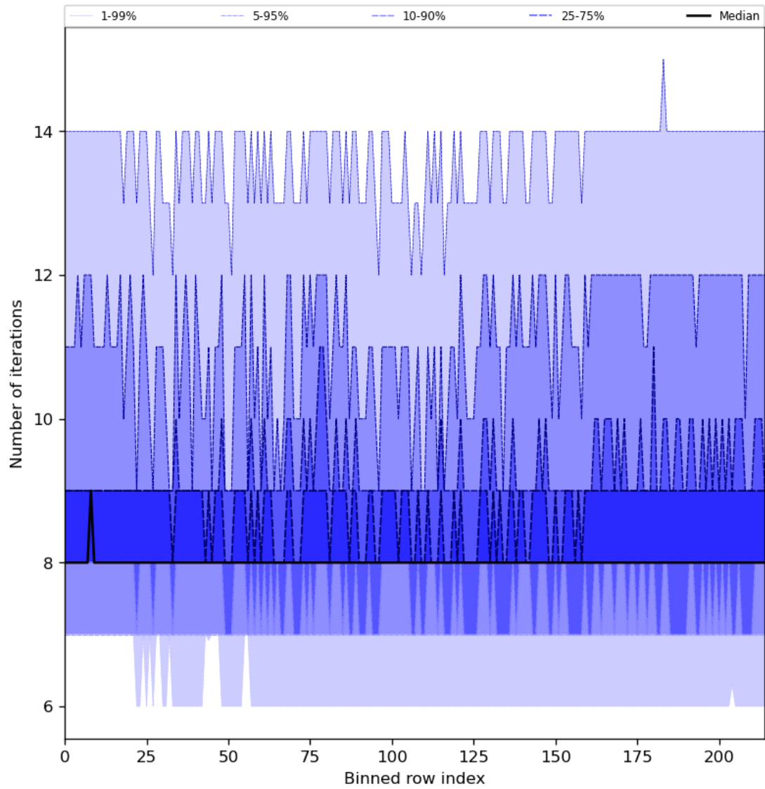
Figure 32: Along track statistics of “Number of iterations” for 2024-05-18 to 2024-05-20
