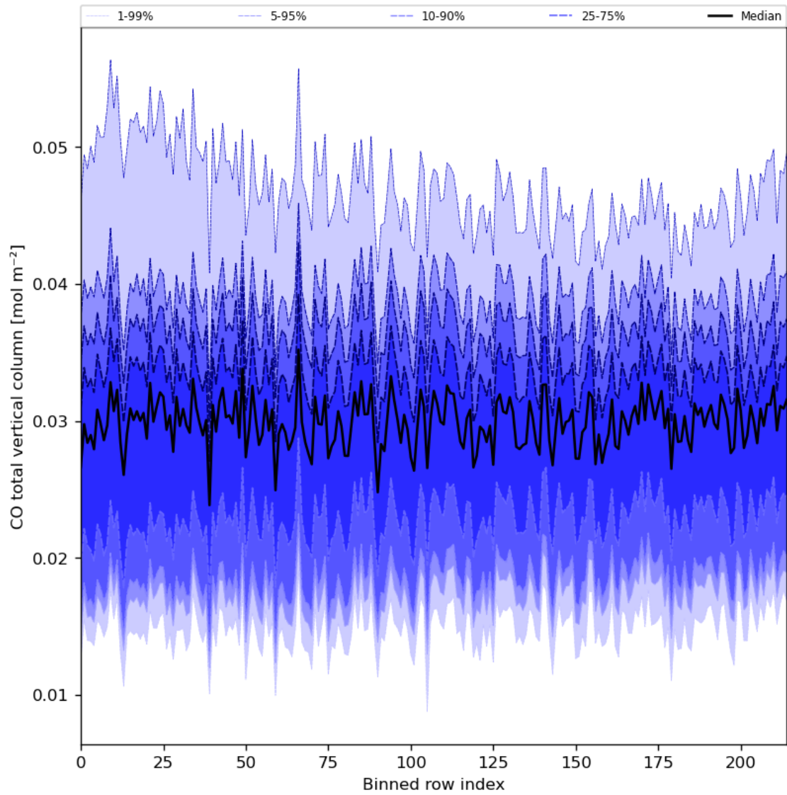
Figure 26: Along track statistics of “CO total vertical column” for 2024-05-18 to 2024-05-20
