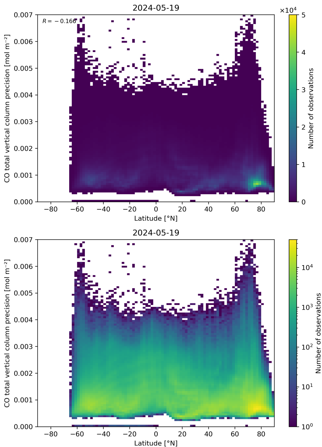
Figure 53: Scatter density plot of “Latitude” against “CO total vertical column precision” for 2024-05-18 to 2024-05-20.
