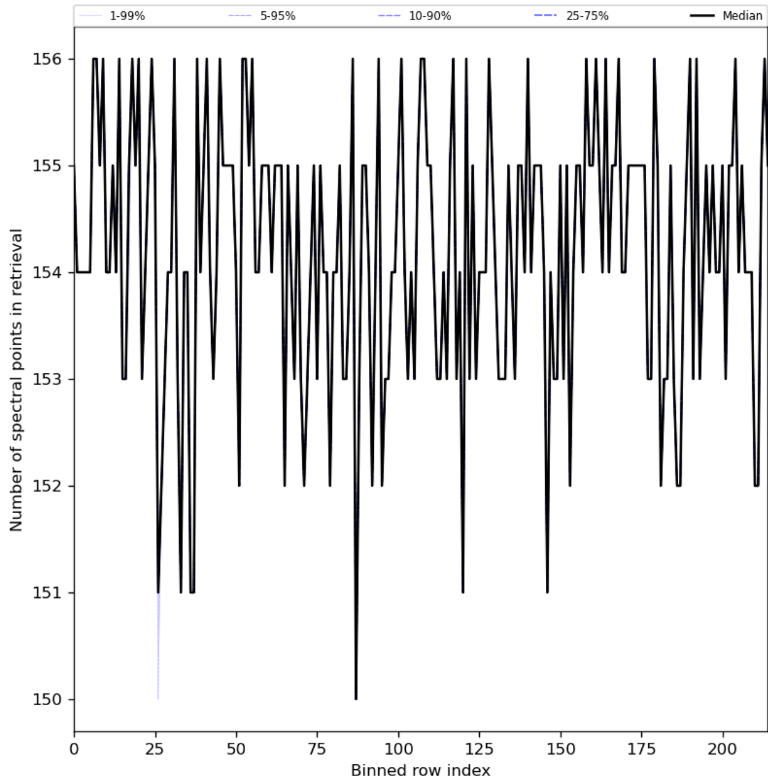
Figure 29: Along track statistics of “Number of spectral points in retrieval” for 2024-05-19 to 2024-05-21
