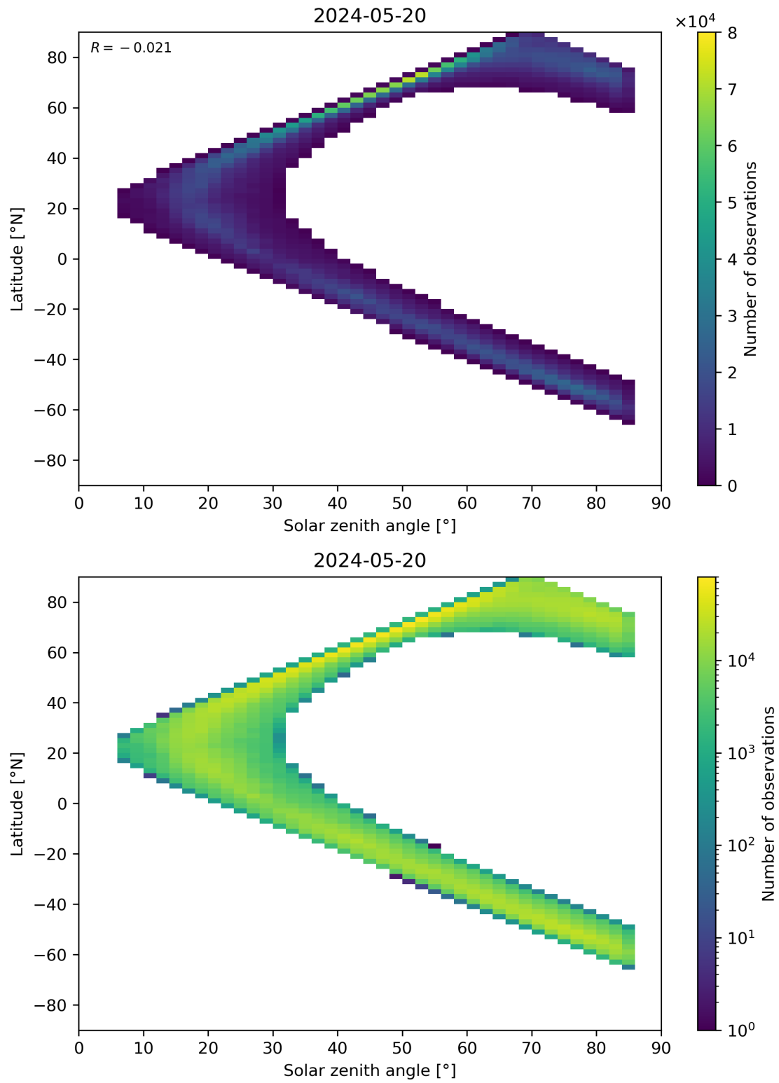
Figure 66: Scatter density plot of “Solar zenith angle” against “Latitude” for 2024-05-19 to 2024-05-21.
