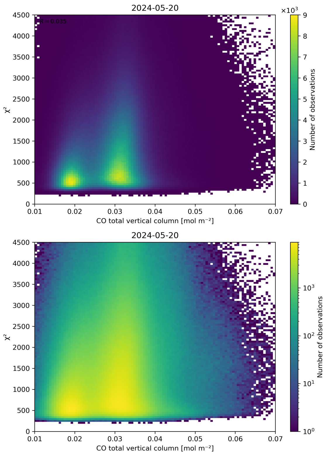
Figure 35: Scatter density plot of “CO total vertical column” against “ \chi^2 ” for 2024-05-19 to 2024-05-21.
