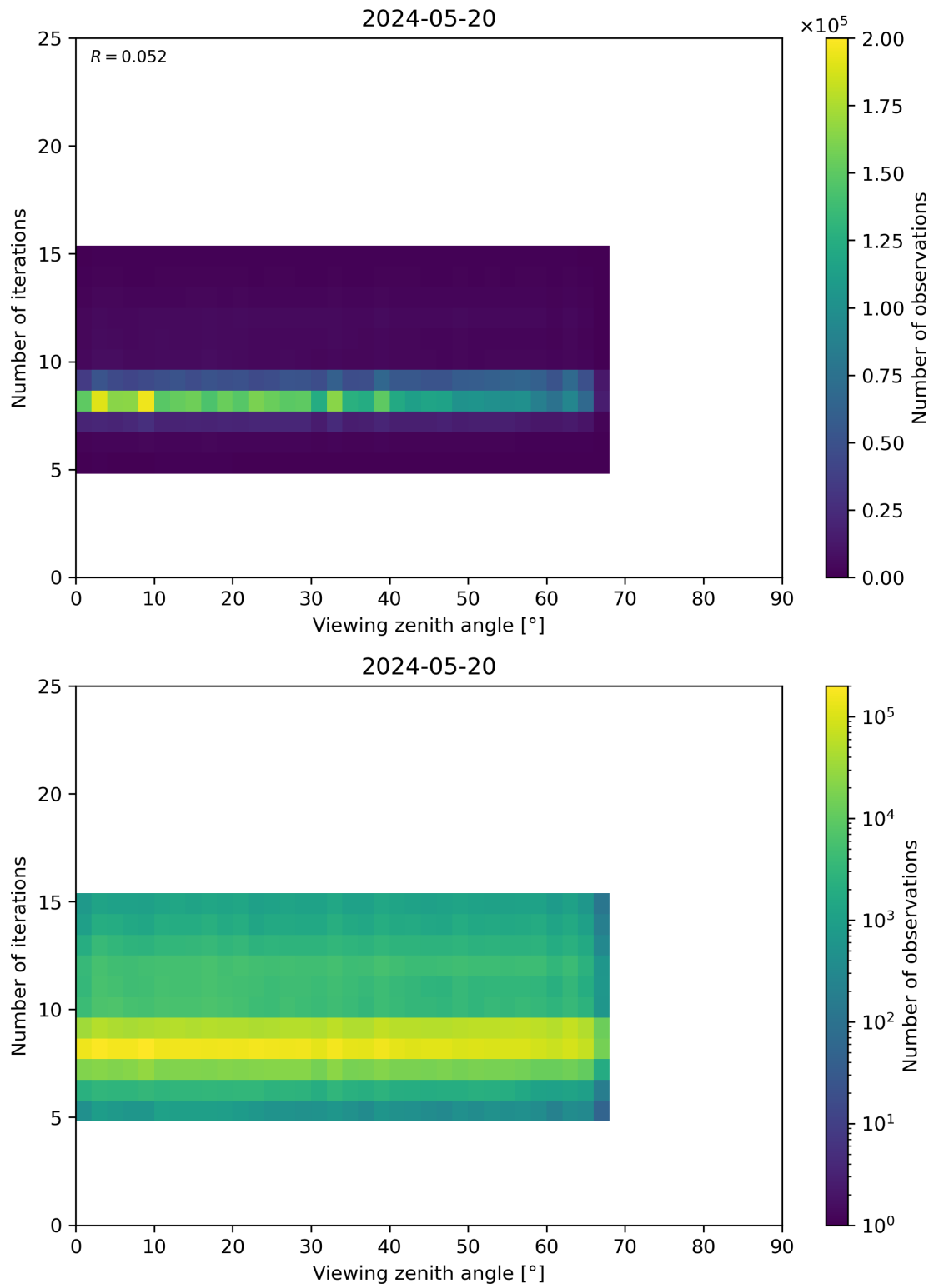
Figure 75: Scatter density plot of “Viewing zenith angle” against “Number of iterations” for 2024-05-19 to 2024-05-21.
