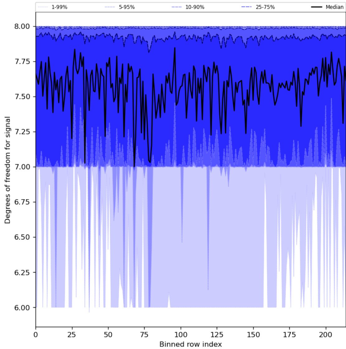
Figure 31: Along track statistics of “Degrees of freedom for signal” for 2024-05-19 to 2024-05-21
