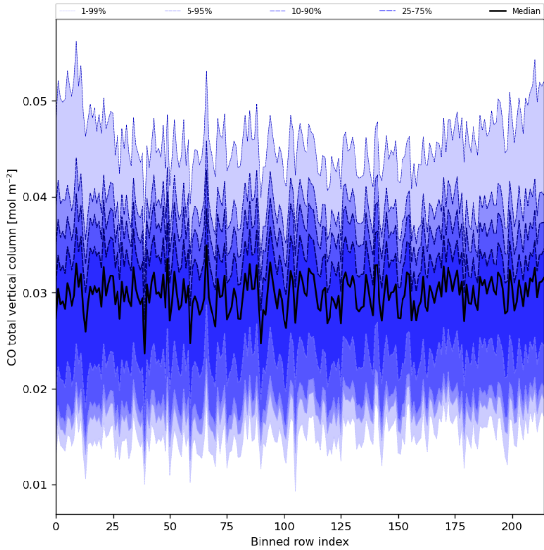
Figure 26: Along track statistics of “CO total vertical column” for 2024-05-19 to 2024-05-21
