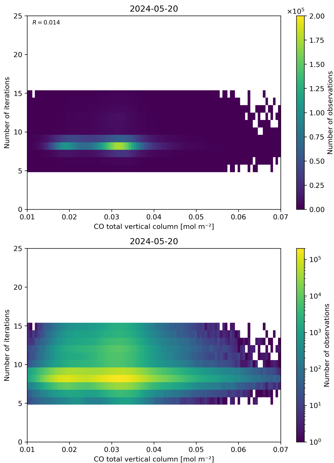
Figure 42: Scatter density plot of “CO total vertical column” against “Number of iterations” for 2024-05-19 to 2024-05-21.
