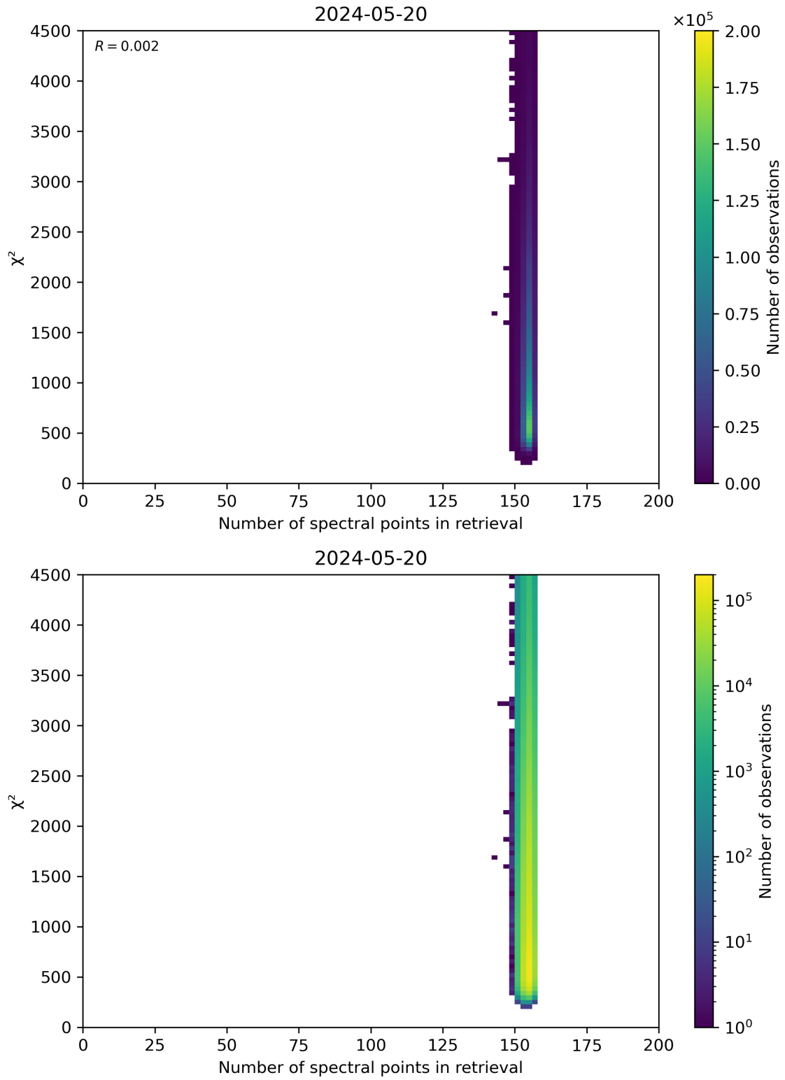
Figure 58: Scatter density plot of “Number of spectral points in retrieval” against “ \chi^2 ” for 2024-05-19 to 2024-05-21.
