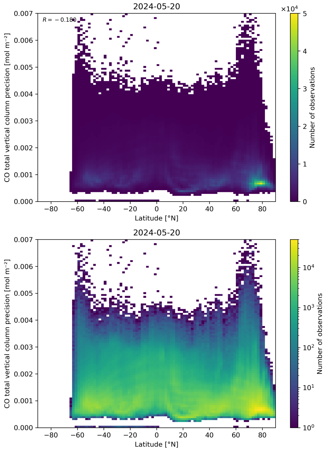
Figure 53: Scatter density plot of “Latitude” against “CO total vertical column precision” for 2024-05-19 to 2024-05-21.
