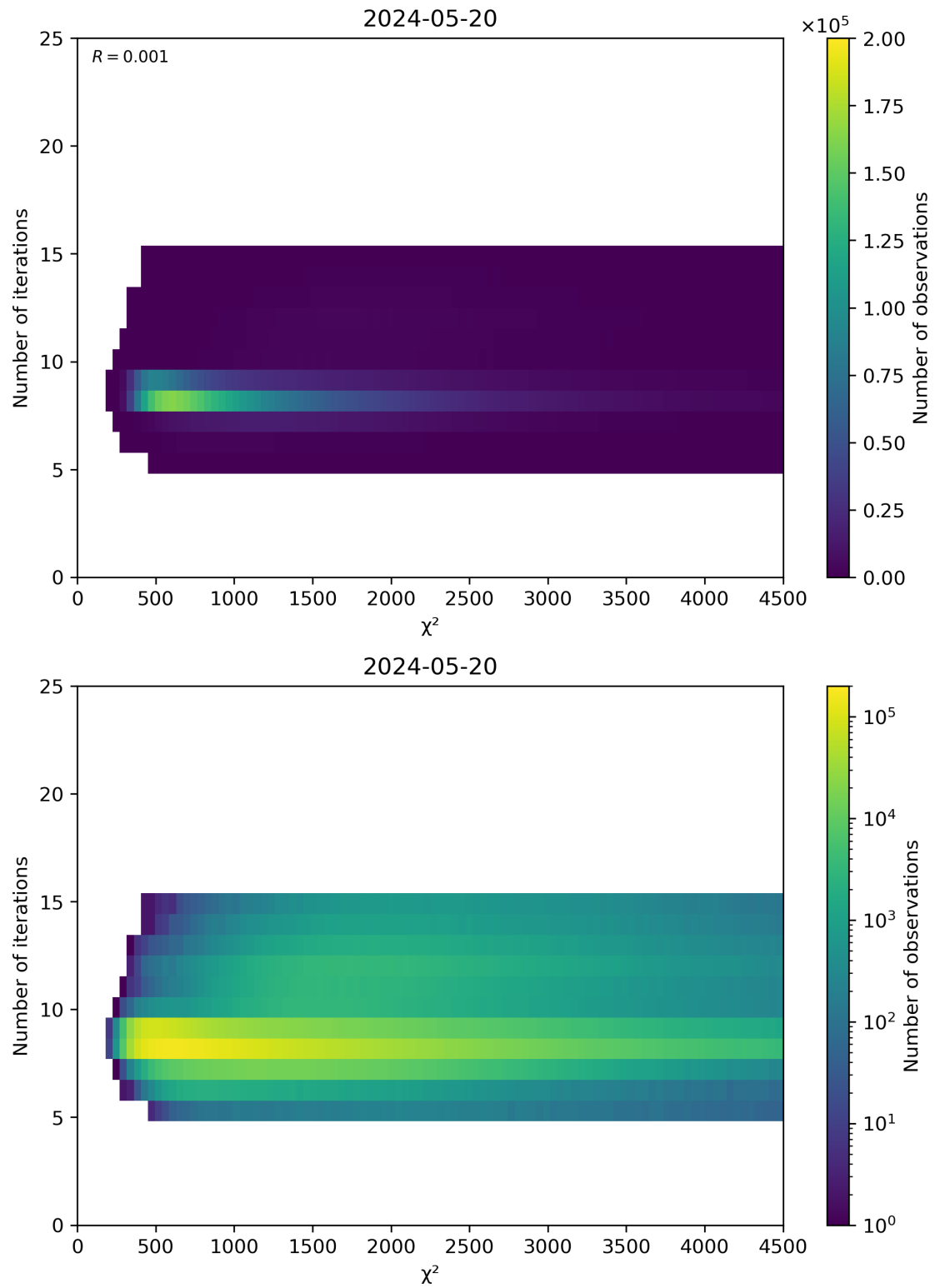
Figure 49: Scatter density plot of “ \chi^2 ” against “Number of iterations” for 2024-05-19 to 2024-05-21.
