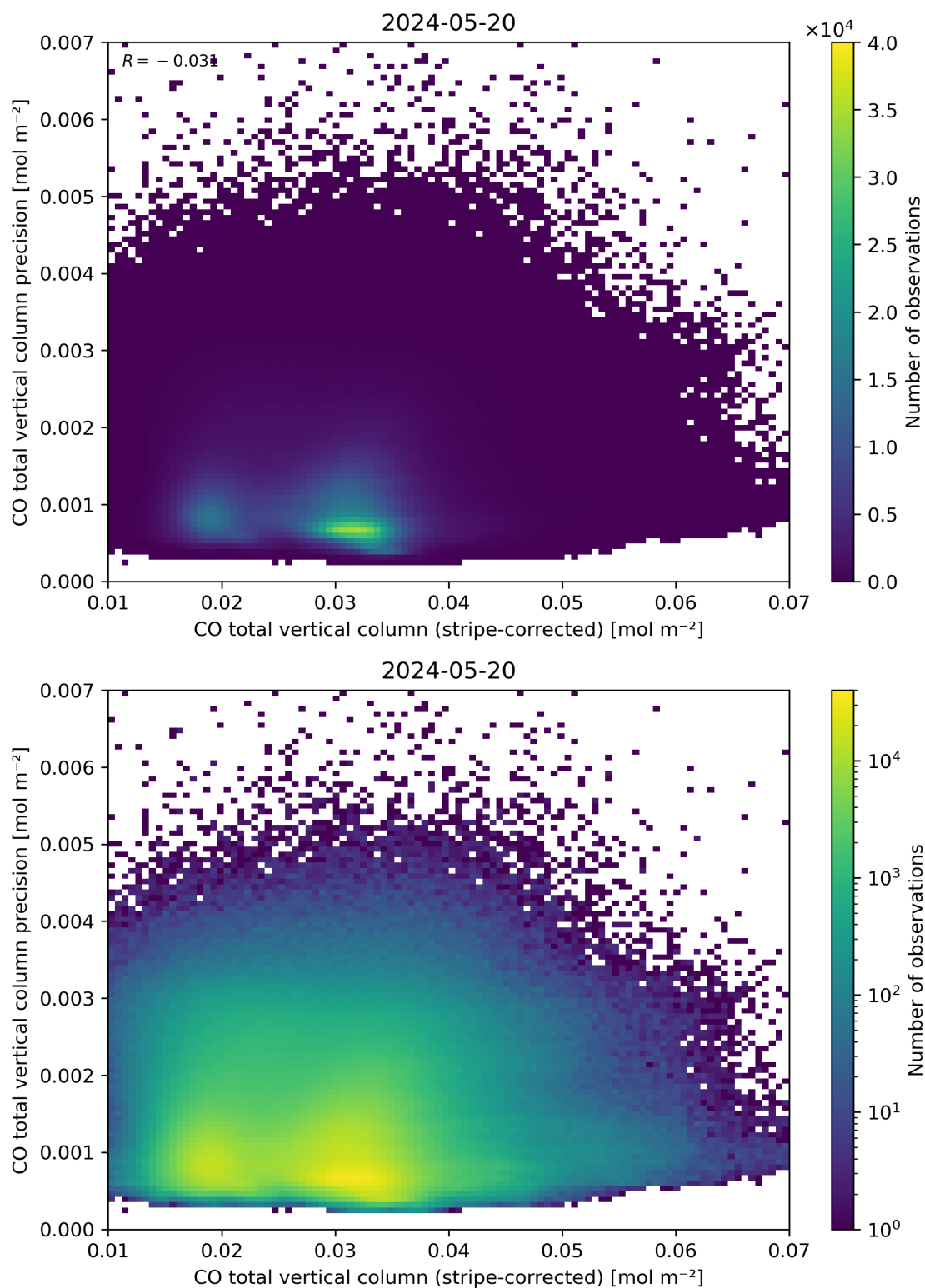
Figure 36: Scatter density plot of “CO total vertical column (stripe-corrected)” against “CO total vertical column precision” for 2024-05-19 to 2024-05-21.
