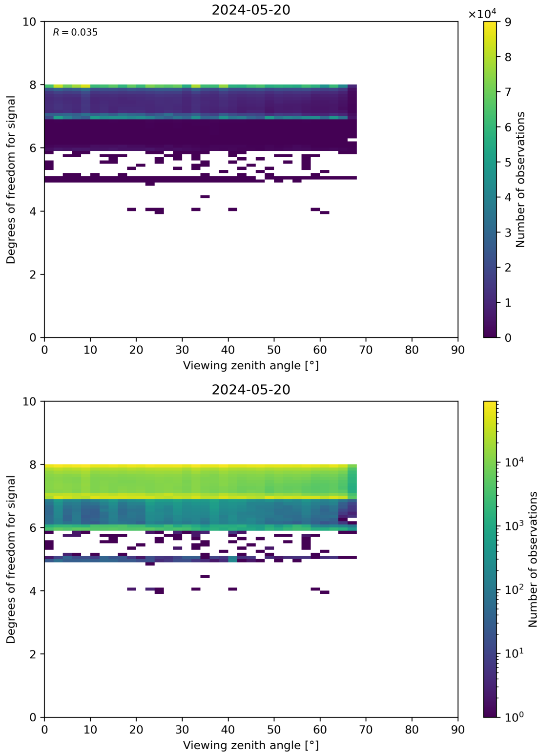
Figure 73: Scatter density plot of “Viewing zenith angle” against “Degrees of freedom for signal” for 2024-05-19 to 2024-05-21.
