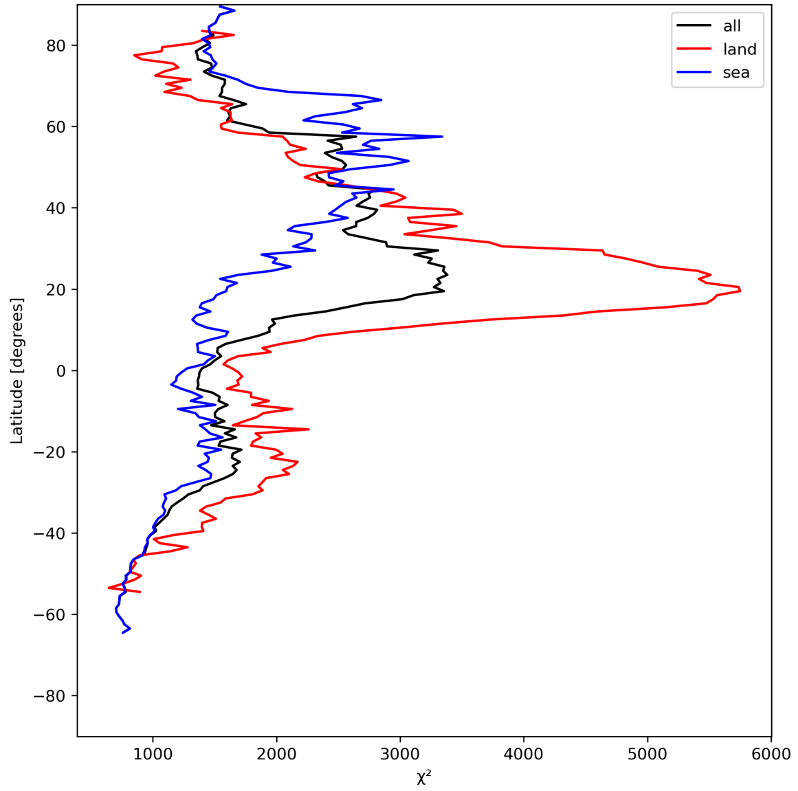
Figure 14: Zonal average of “ \chi^2 ” for 2024-05-19 to 2024-05-21.
