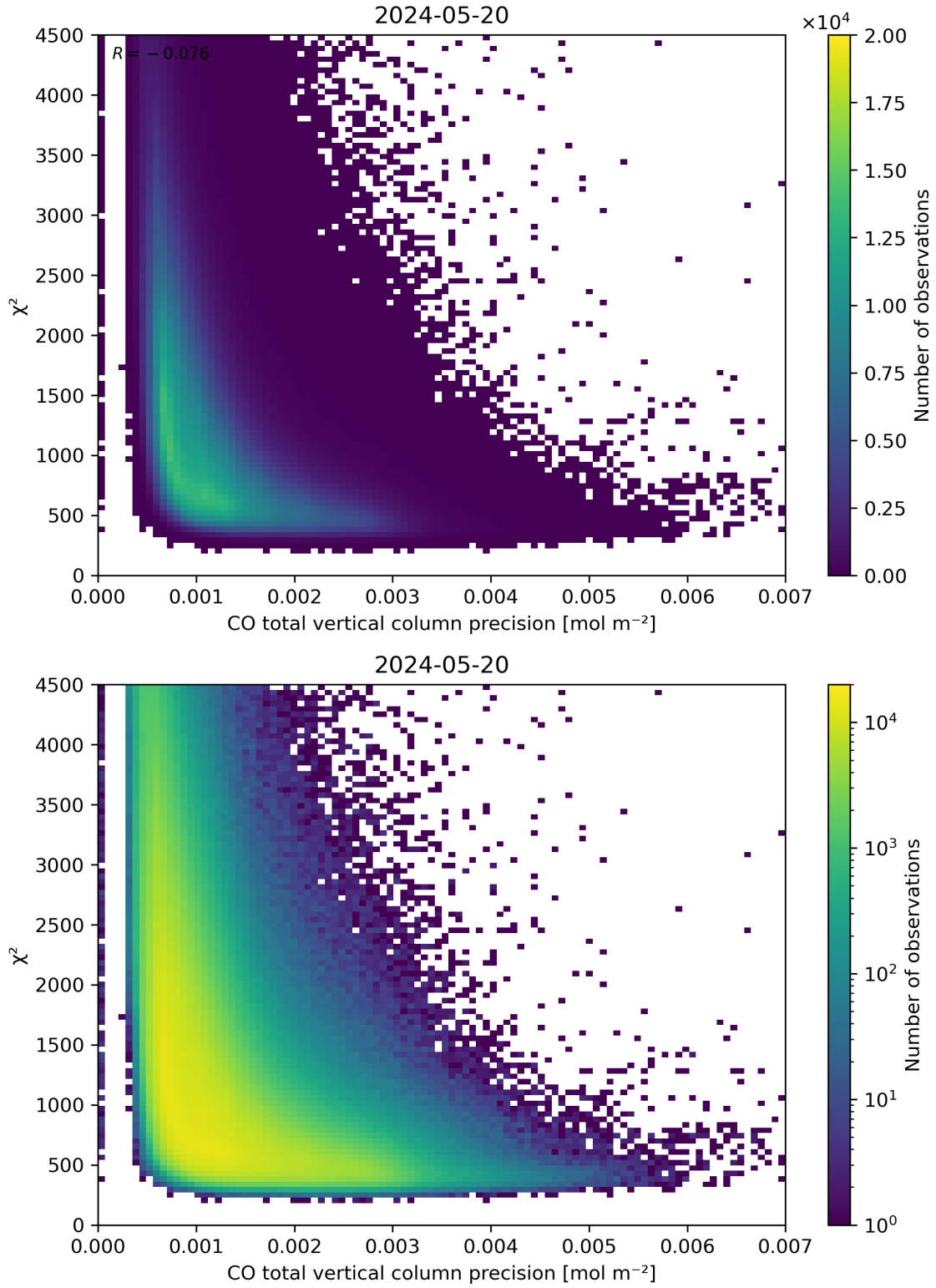
Figure 44: Scatter density plot of “CO total vertical column precision” against “ \chi^2 ” for 2024-05-19 to 2024-05-21.
