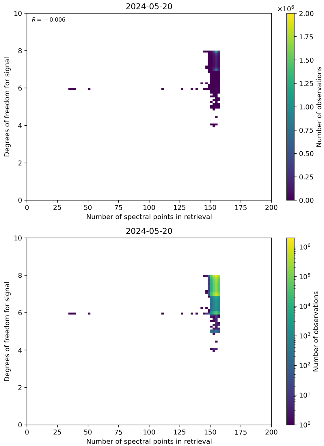
Figure 59: Scatter density plot of “Number of spectral points in retrieval” against “Degrees of freedom for signal” for 2024-05-19 to 2024-05-21.
