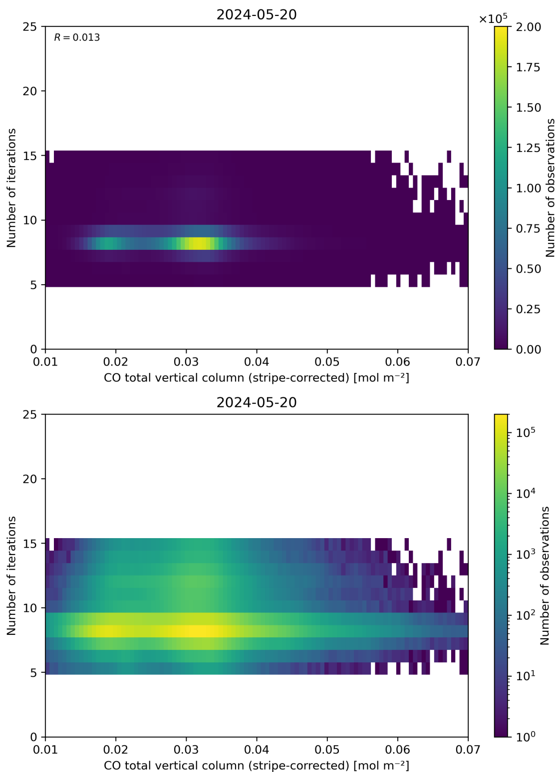
Figure 39: Scatter density plot of “CO total vertical column (stripe-corrected)” against “Number of iterations” for 2024-05-19 to 2024-05-21.
