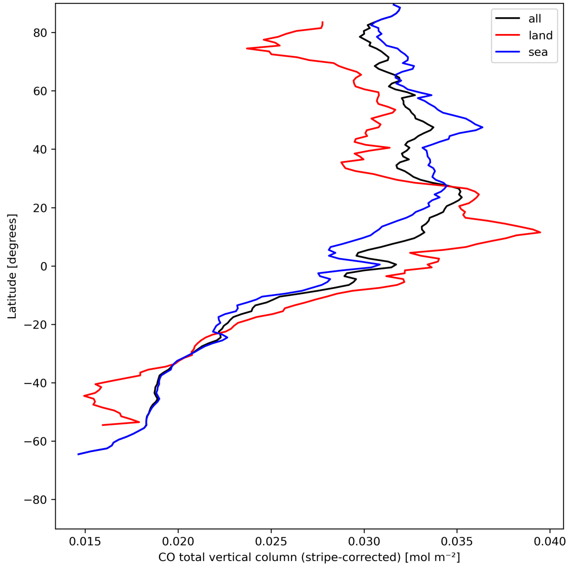
Figure 11: Zonal average of “CO total vertical column (stripe-corrected)” for 2024-05-19 to 2024-05-21.
