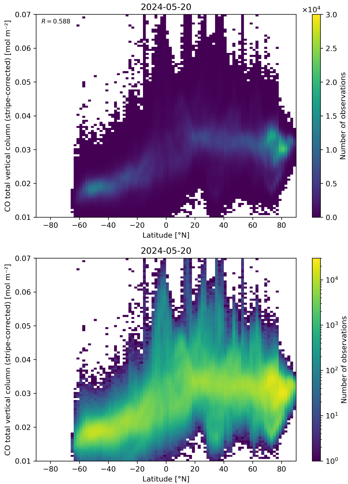
Figure 52: Scatter density plot of “Latitude” against “CO total vertical column (stripe-corrected)” for 2024-05-19 to 2024-05-21.
