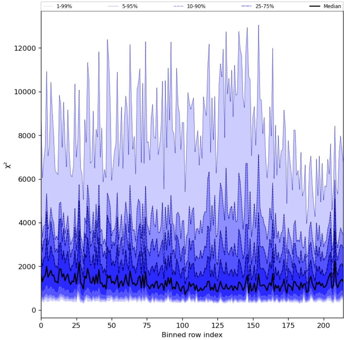
Figure 30: Along track statistics of “ \chi^2 ” for 2024-05-19 to 2024-05-21
