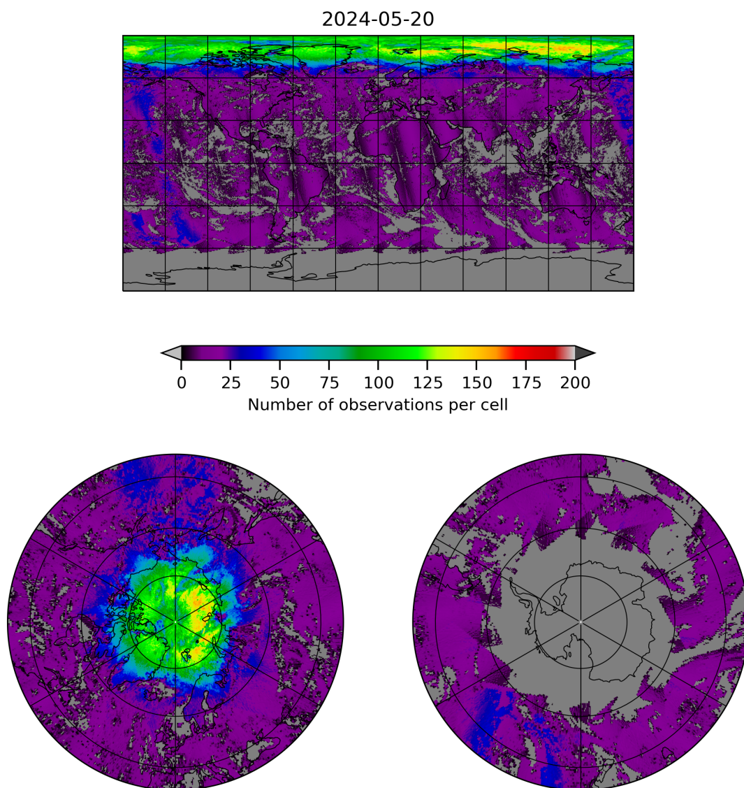
Figure 8: Map of the number of observations for 2024-05-19 to 2024-05-21
