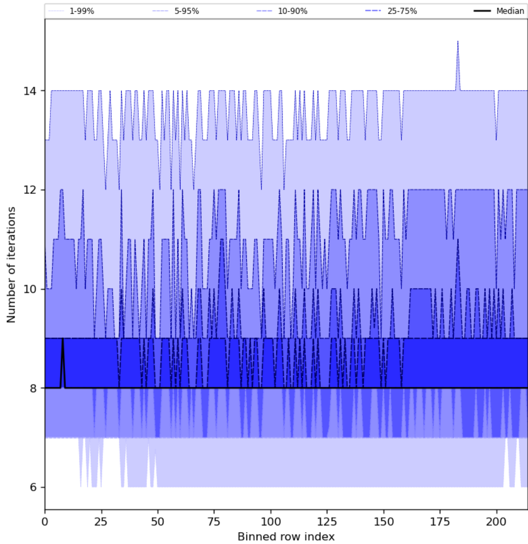
Figure 32: Along track statistics of “Number of iterations” for 2024-05-19 to 2024-05-21
