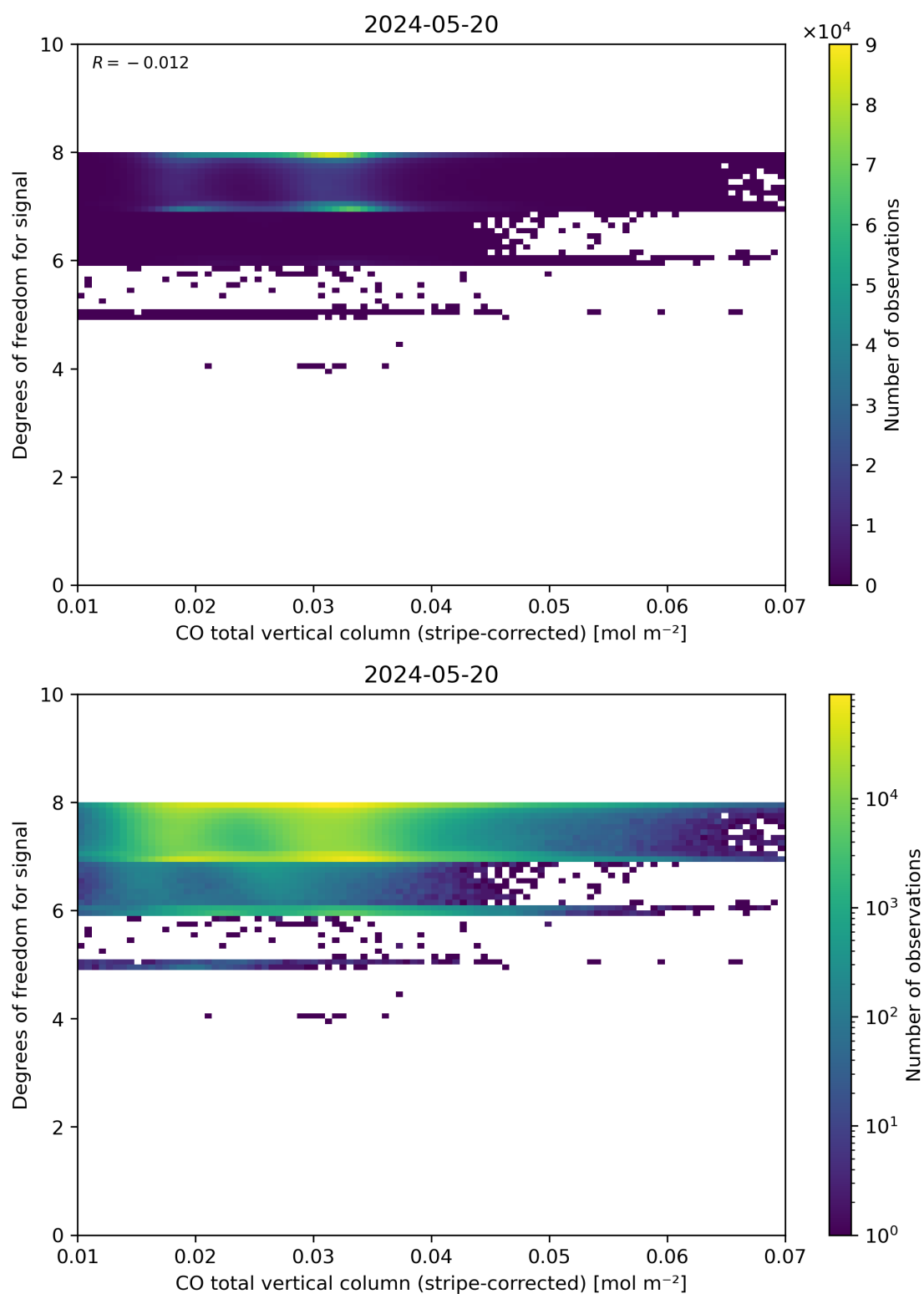
Figure 38: Scatter density plot of “CO total vertical column (stripe-corrected)” against “Degrees of freedom for signal” for 2024-05-19 to 2024-05-21.
