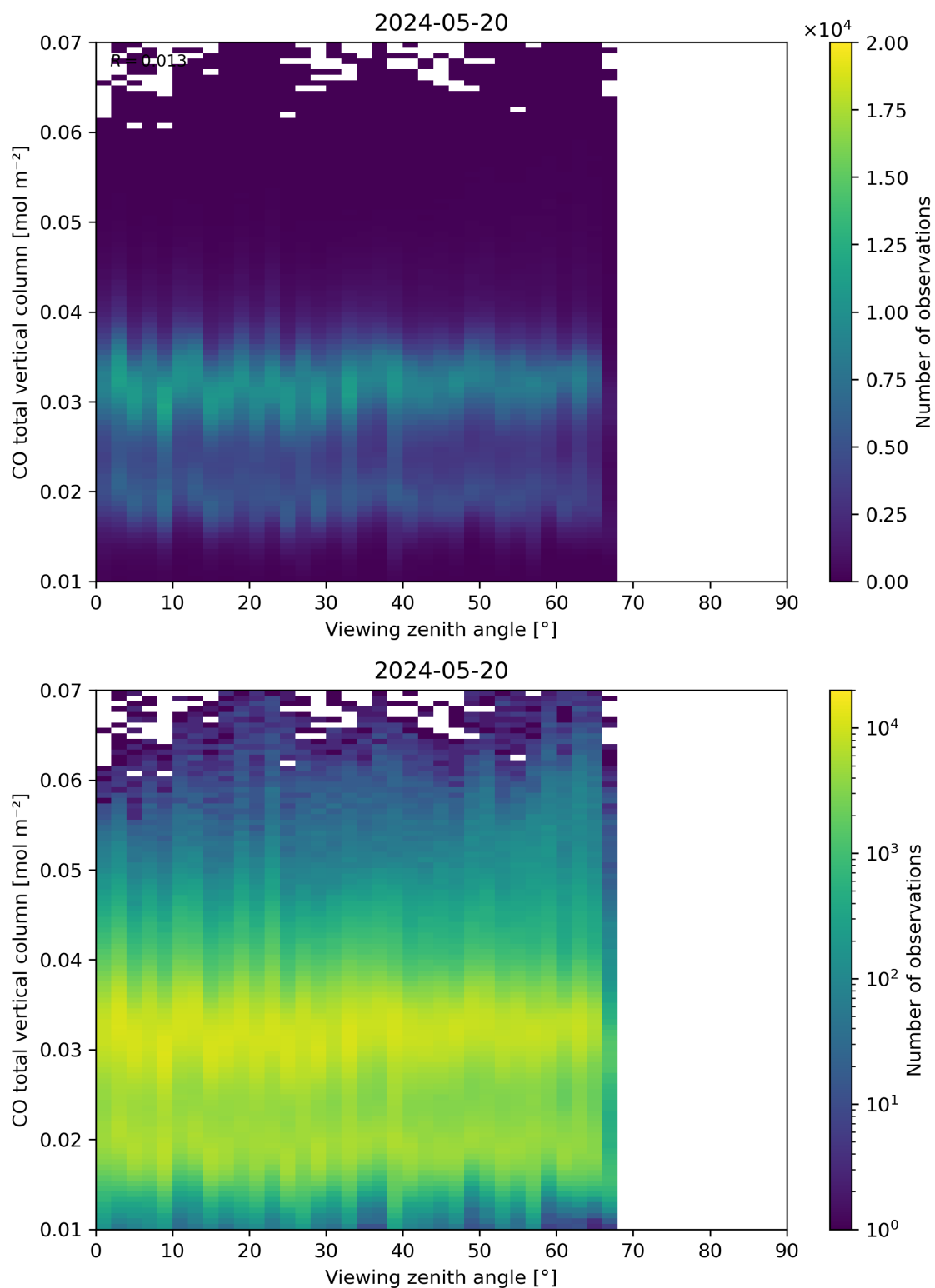
Figure 69: Scatter density plot of “Viewing zenith angle” against “CO total vertical column” for 2024-05-19 to 2024-05-21.
