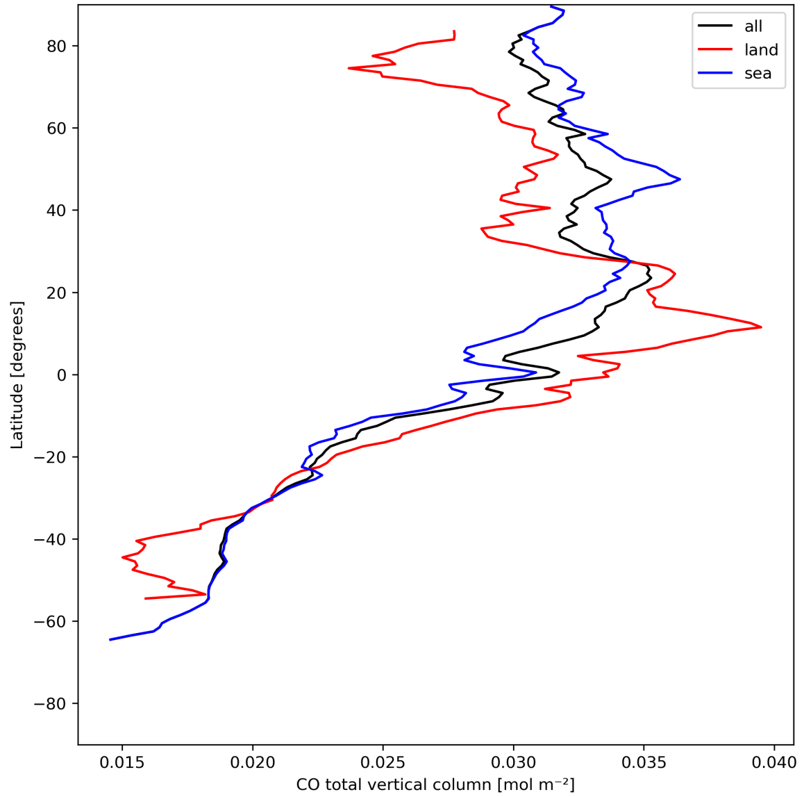
Figure 10: Zonal average of “CO total vertical column” for 2024-05-19 to 2024-05-21.
