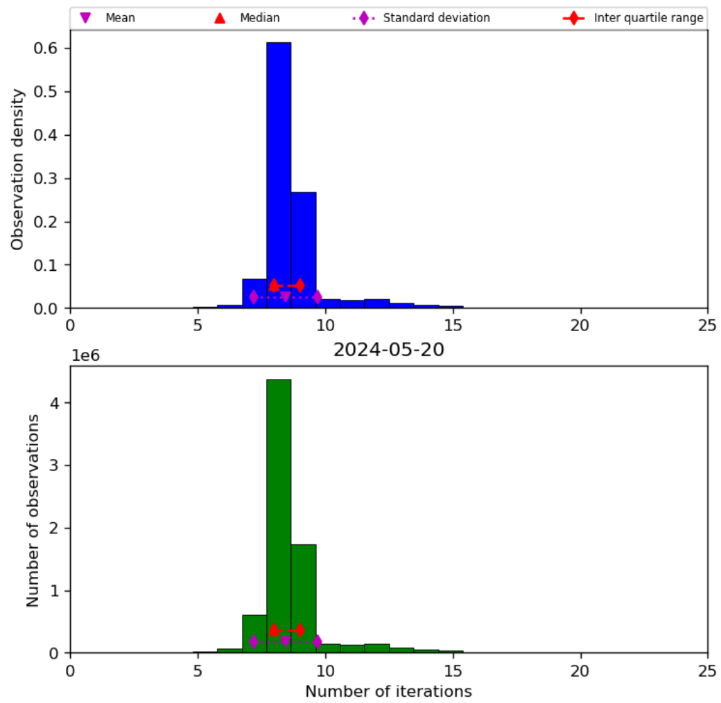
Figure 24: Histogram of “Number of iterations” for 2024-05-19 to 2024-05-21
