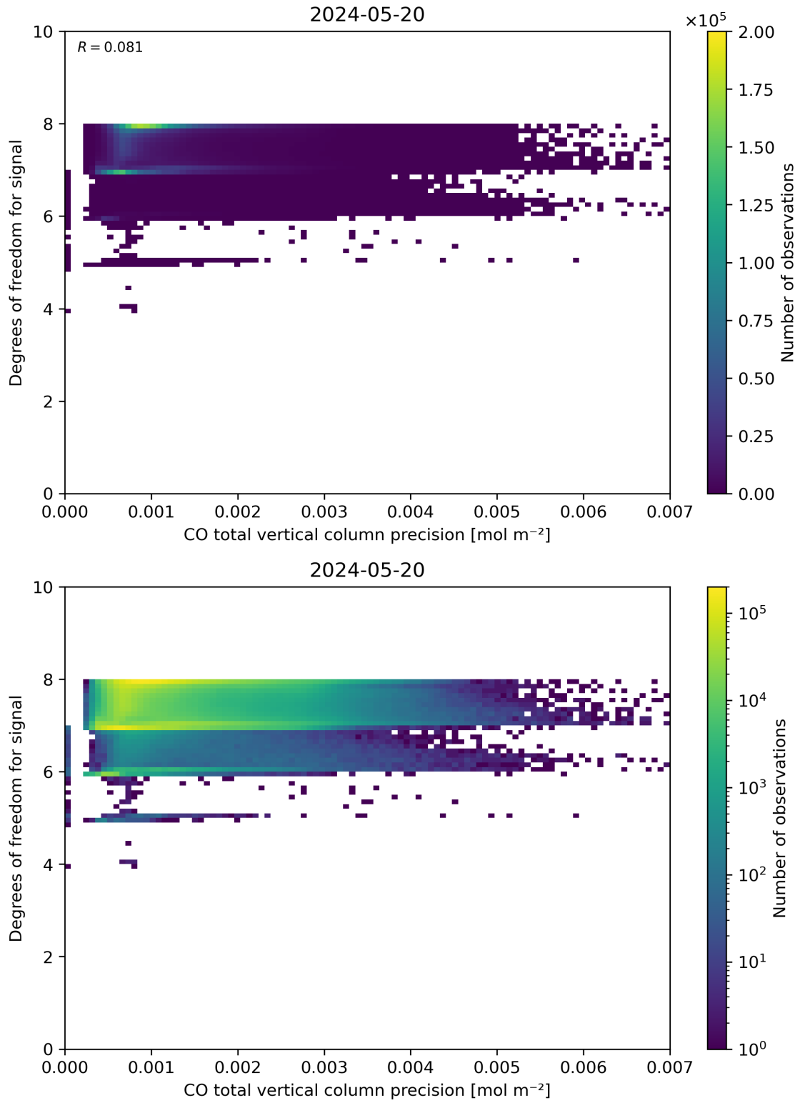
Figure 45: Scatter density plot of “CO total vertical column precision” against “Degrees of freedom for signal” for 2024-05-19 to 2024-05-21.
