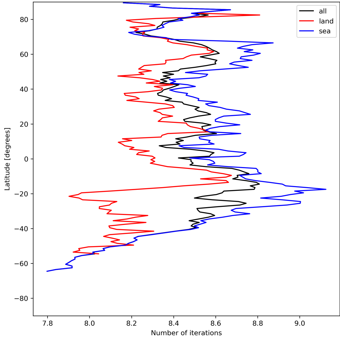
Figure 16: Zonal average of “Number of iterations” for 2024-05-19 to 2024-05-21.
