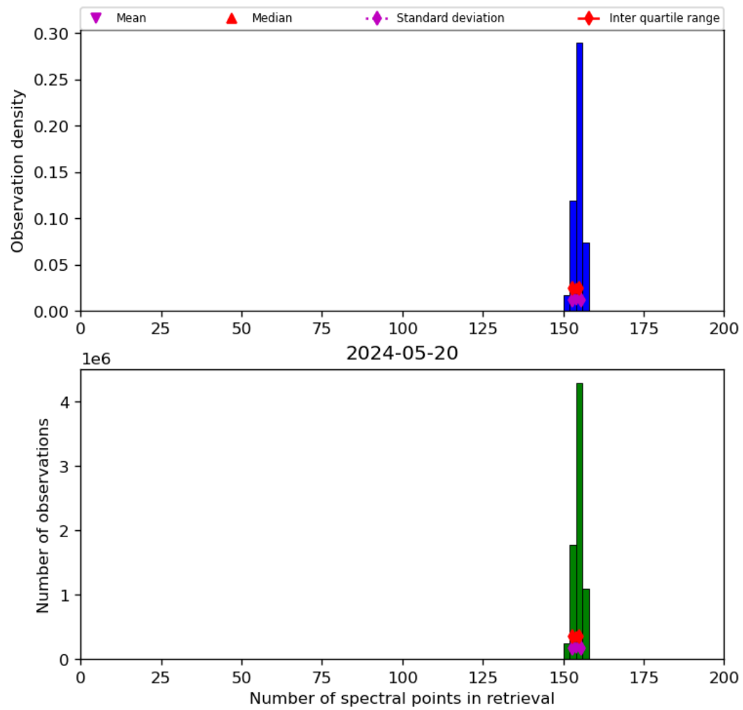
Figure 21: Histogram of “Number of spectral points in retrieval” for 2024-05-19 to 2024-05-21
