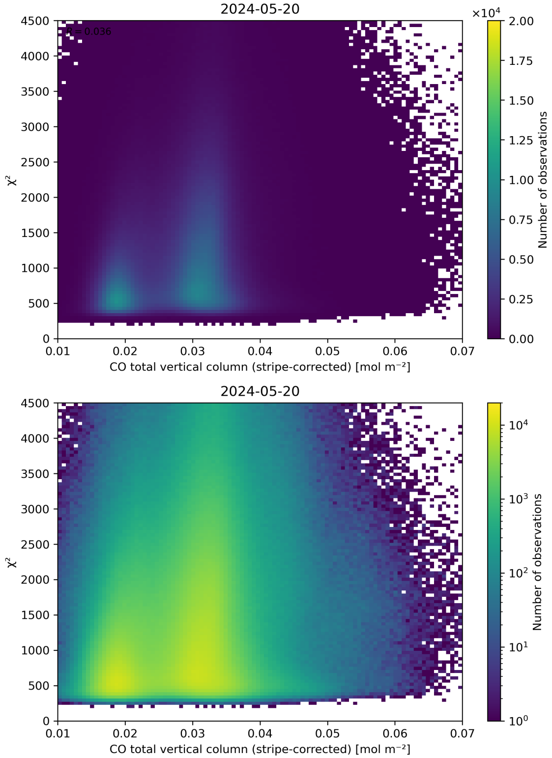
Figure 37: Scatter density plot of “CO total vertical column (stripe-corrected)” against “ \chi^2 ” for 2024-05-19 to 2024-05-21.
