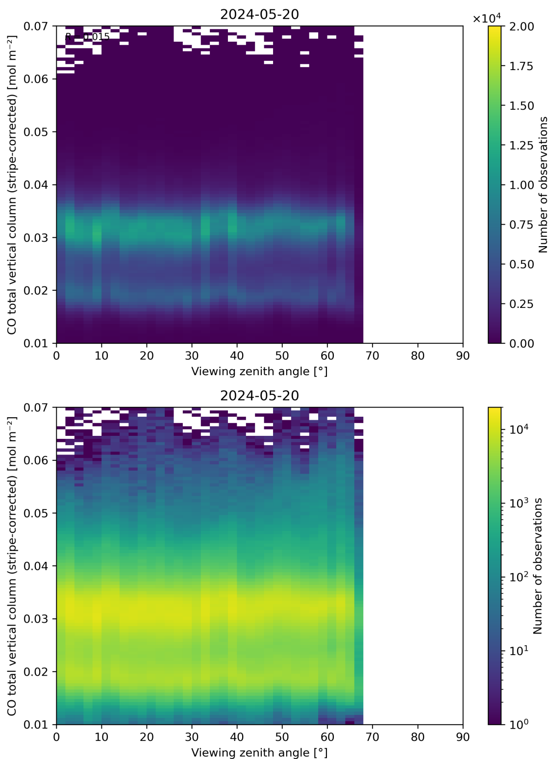
Figure 70: Scatter density plot of “Viewing zenith angle” against “CO total vertical column (stripe-corrected)” for 2024-05-19 to 2024-05-21.
