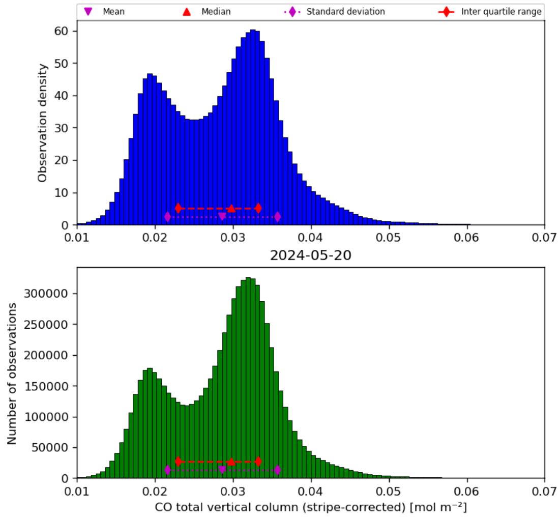
Figure 19: Histogram of “CO total vertical column (stripe-corrected)” for 2024-05-19 to 2024-05-21
