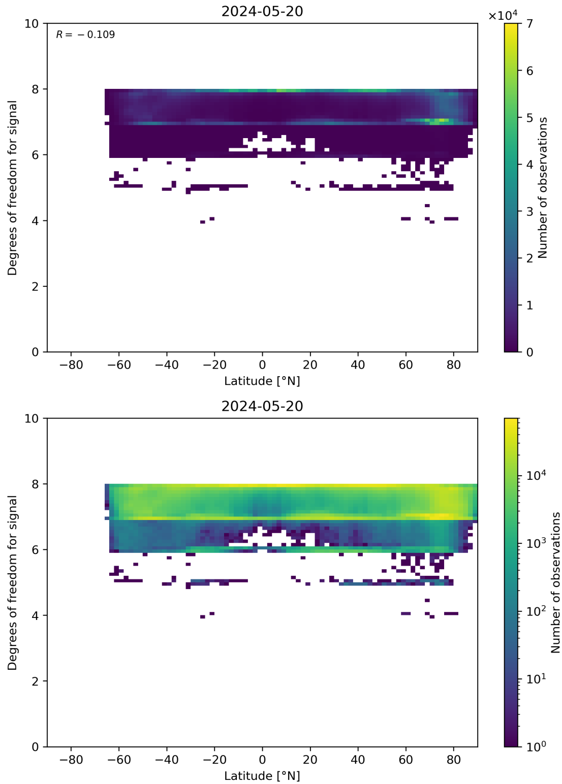
Figure 55: Scatter density plot of “Latitude” against “Degrees of freedom for signal” for 2024-05-19 to 2024-05-21.
