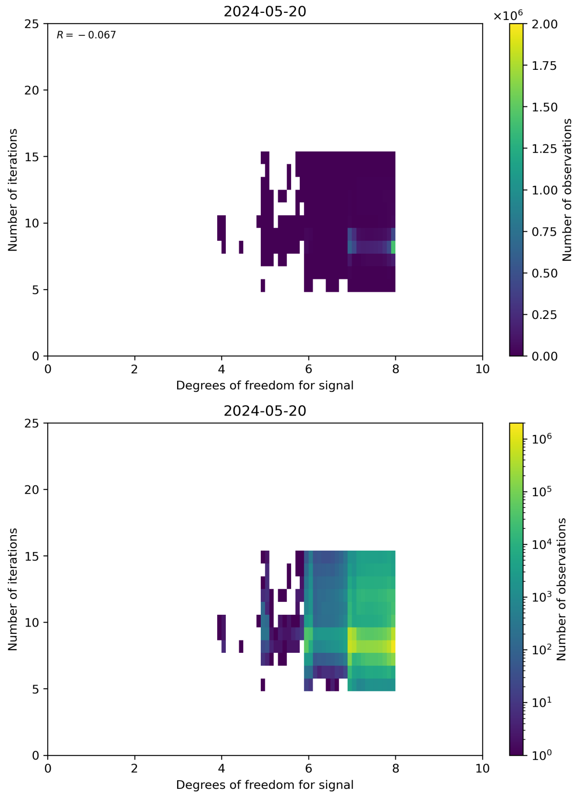
Figure 50: Scatter density plot of “Degrees of freedom for signal” against “Number of iterations” for 2024-05-19 to 2024-05-21.
