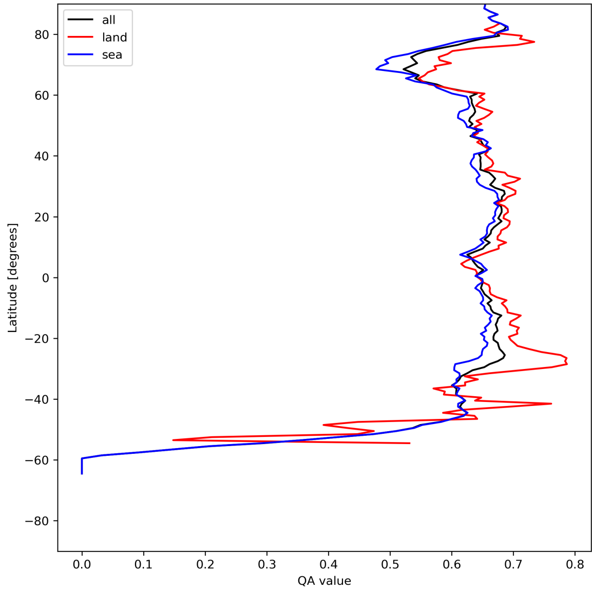
Figure 9: Zonal average of “QA value” for 2024-05-19 to 2024-05-21.
