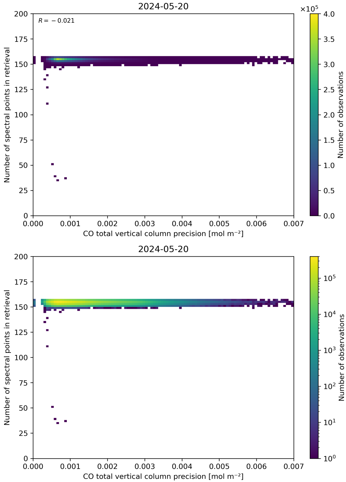
Figure 47: Scatter density plot of “CO total vertical column precision” against “Number of spectral points in retrieval” for 2024-05-19 to 2024-05-21.
