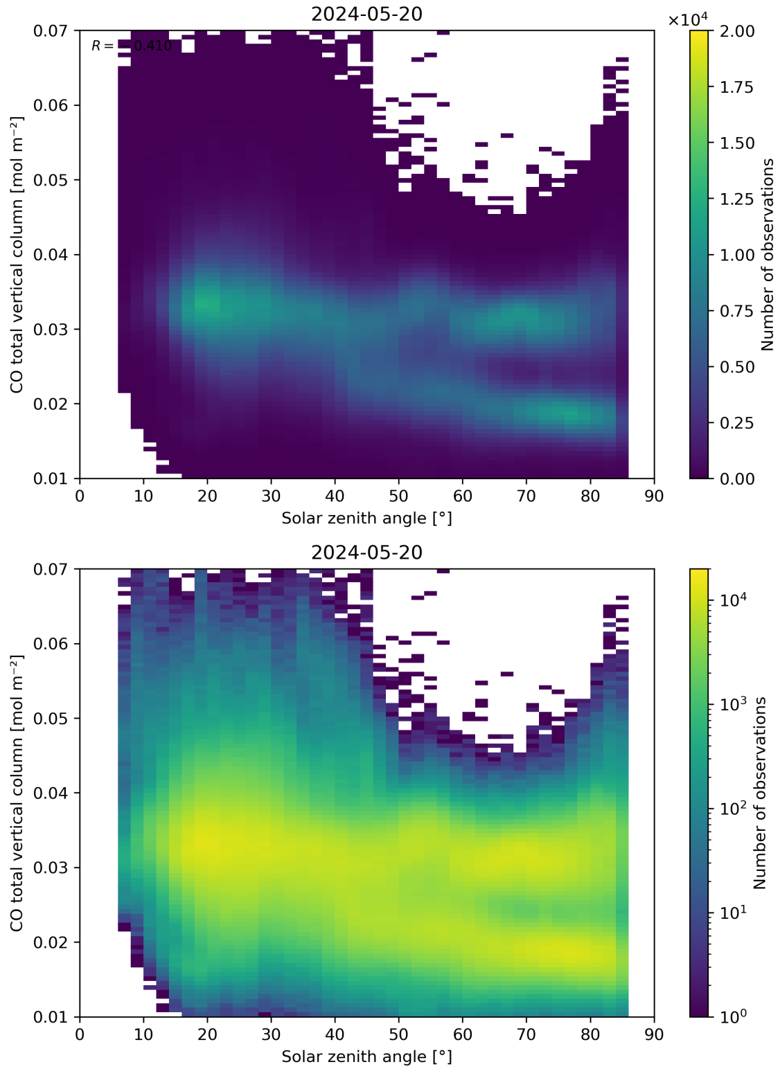
Figure 61: Scatter density plot of “Solar zenith angle” against “CO total vertical column” for 2024-05-19 to 2024-05-21.
