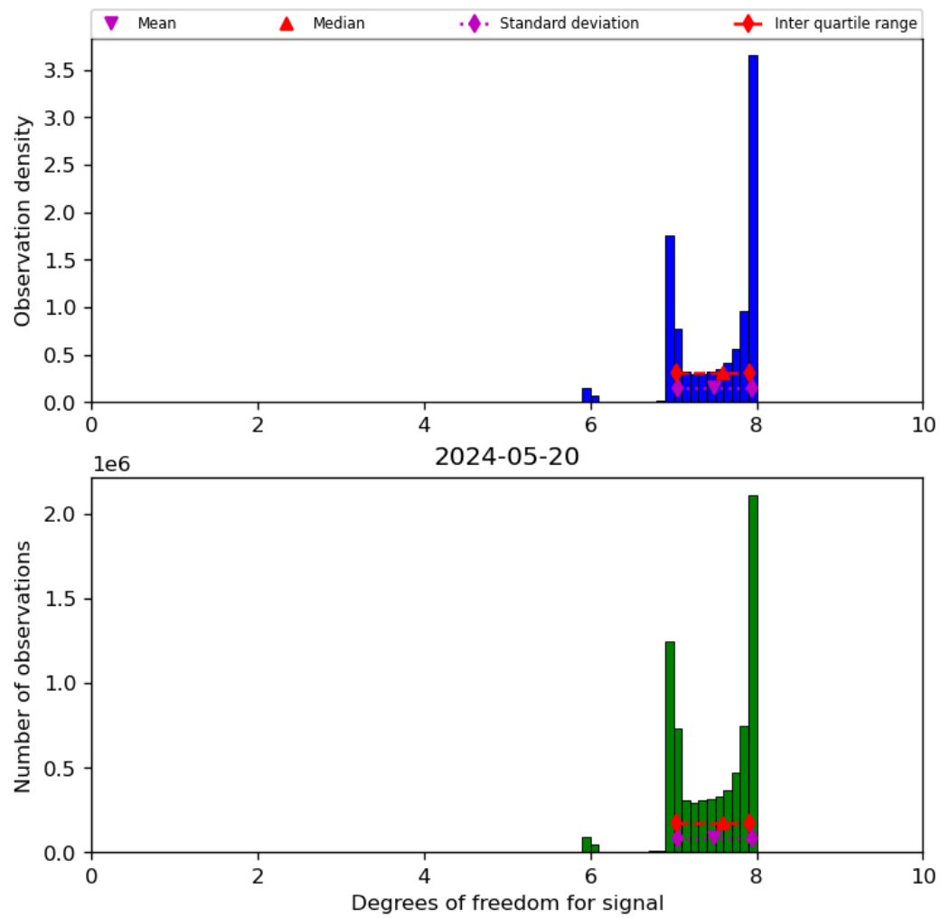
Figure 23: Histogram of “Degrees of freedom for signal” for 2024-05-19 to 2024-05-21
