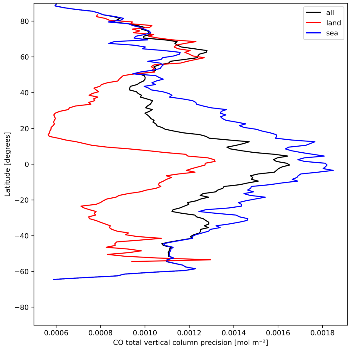
Figure 12: Zonal average of “CO total vertical column precision” for 2024-05-19 to 2024-05-21.
