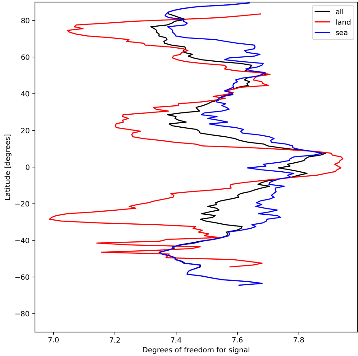
Figure 15: Zonal average of “Degrees of freedom for signal” for 2024-05-19 to 2024-05-21.
