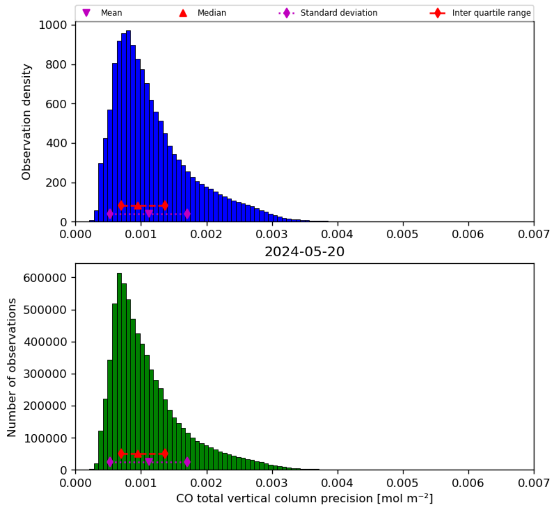
Figure 20: Histogram of “CO total vertical column precision” for 2024-05-19 to 2024-05-21
