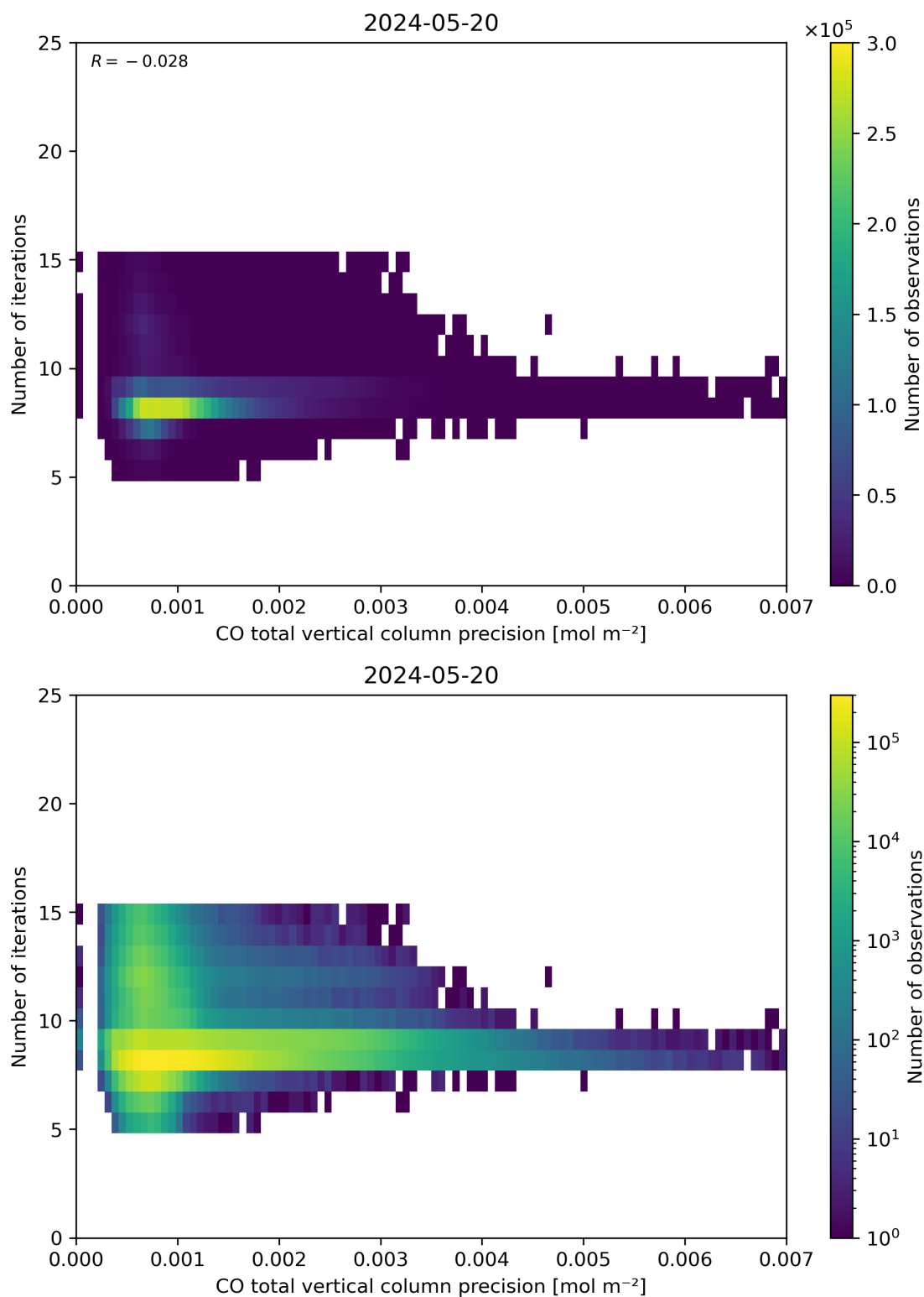
Figure 46: Scatter density plot of “CO total vertical column precision” against “Number of iterations” for 2024-05-19 to 2024-05-21.
