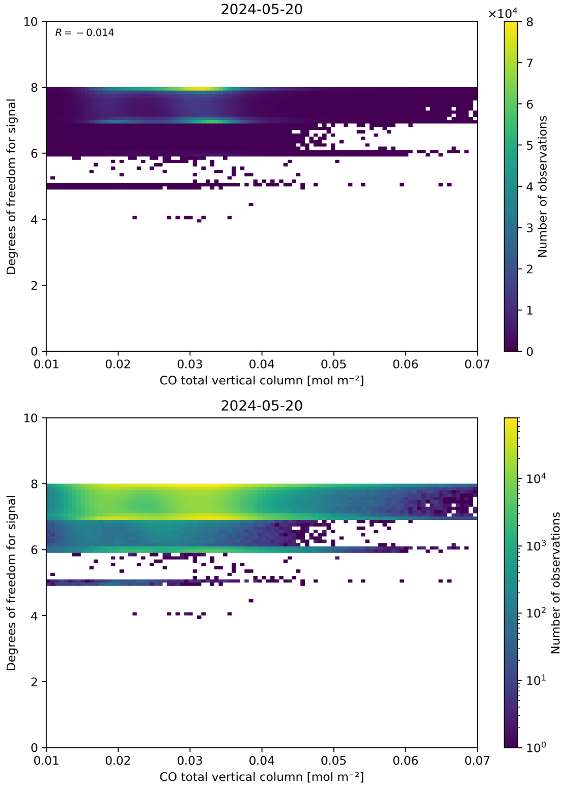
Figure 41: Scatter density plot of “CO total vertical column” against “Degrees of freedom for signal” for 2024-05-19 to 2024-05-21.
