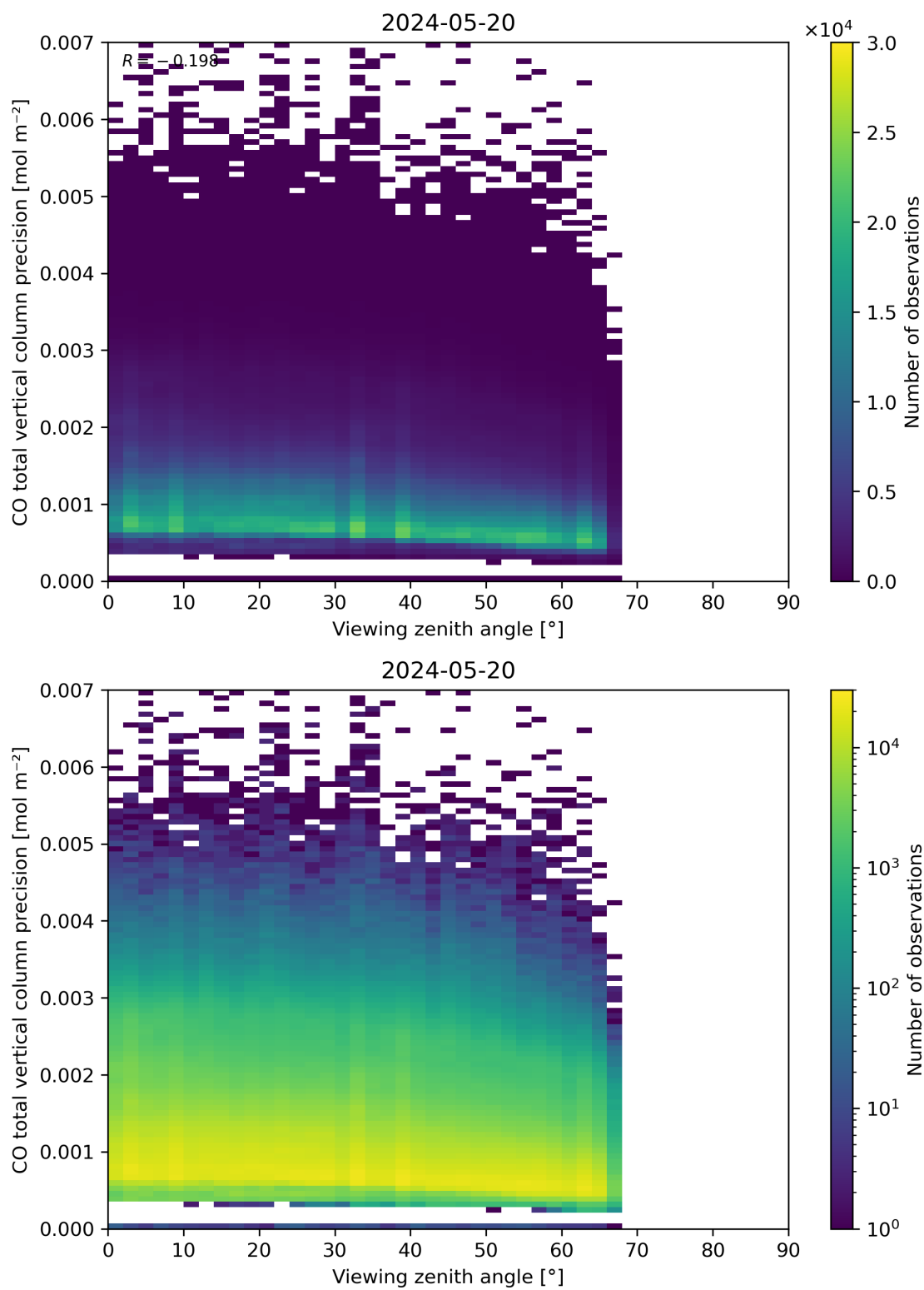
Figure 71: Scatter density plot of “Viewing zenith angle” against “CO total vertical column precision” for 2024-05-19 to 2024-05-21.
