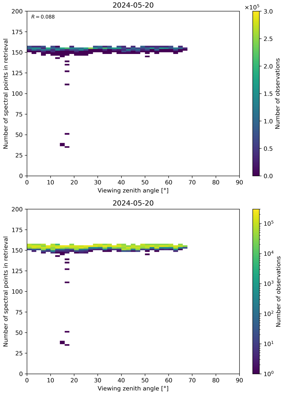
Figure 76: Scatter density plot of “Viewing zenith angle” against “Number of spectral points in retrieval” for 2024-05-19 to 2024-05-21.
