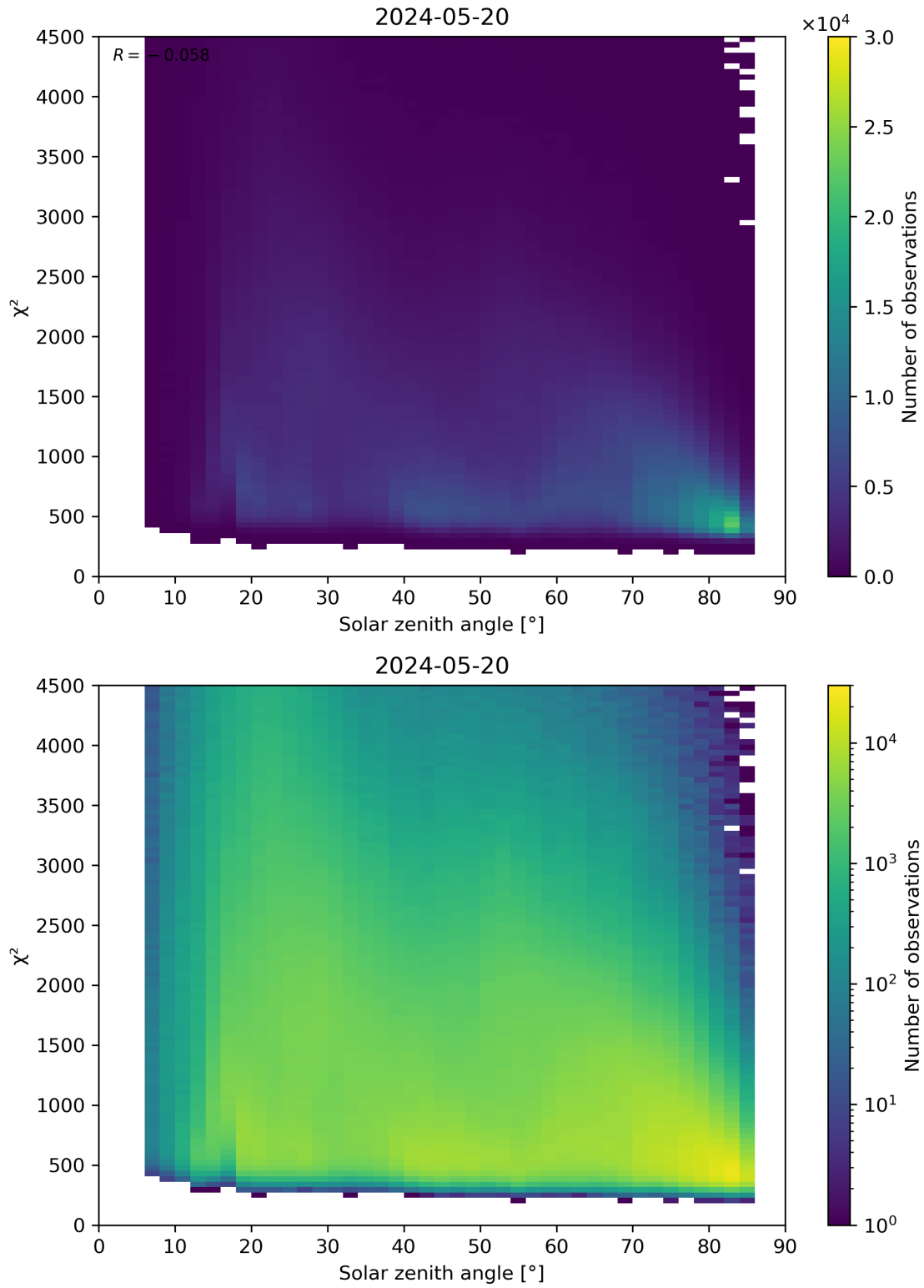
Figure 64: Scatter density plot of “Solar zenith angle” against “ \chi^2 ” for 2024-05-19 to 2024-05-21.
