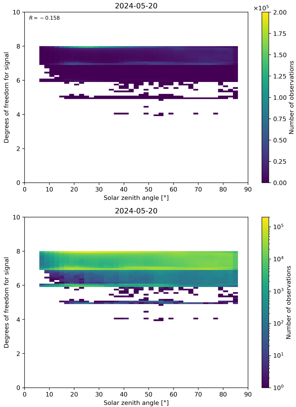
Figure 65: Scatter density plot of “Solar zenith angle” against “Degrees of freedom for signal” for 2024-05-19 to 2024-05-21.
