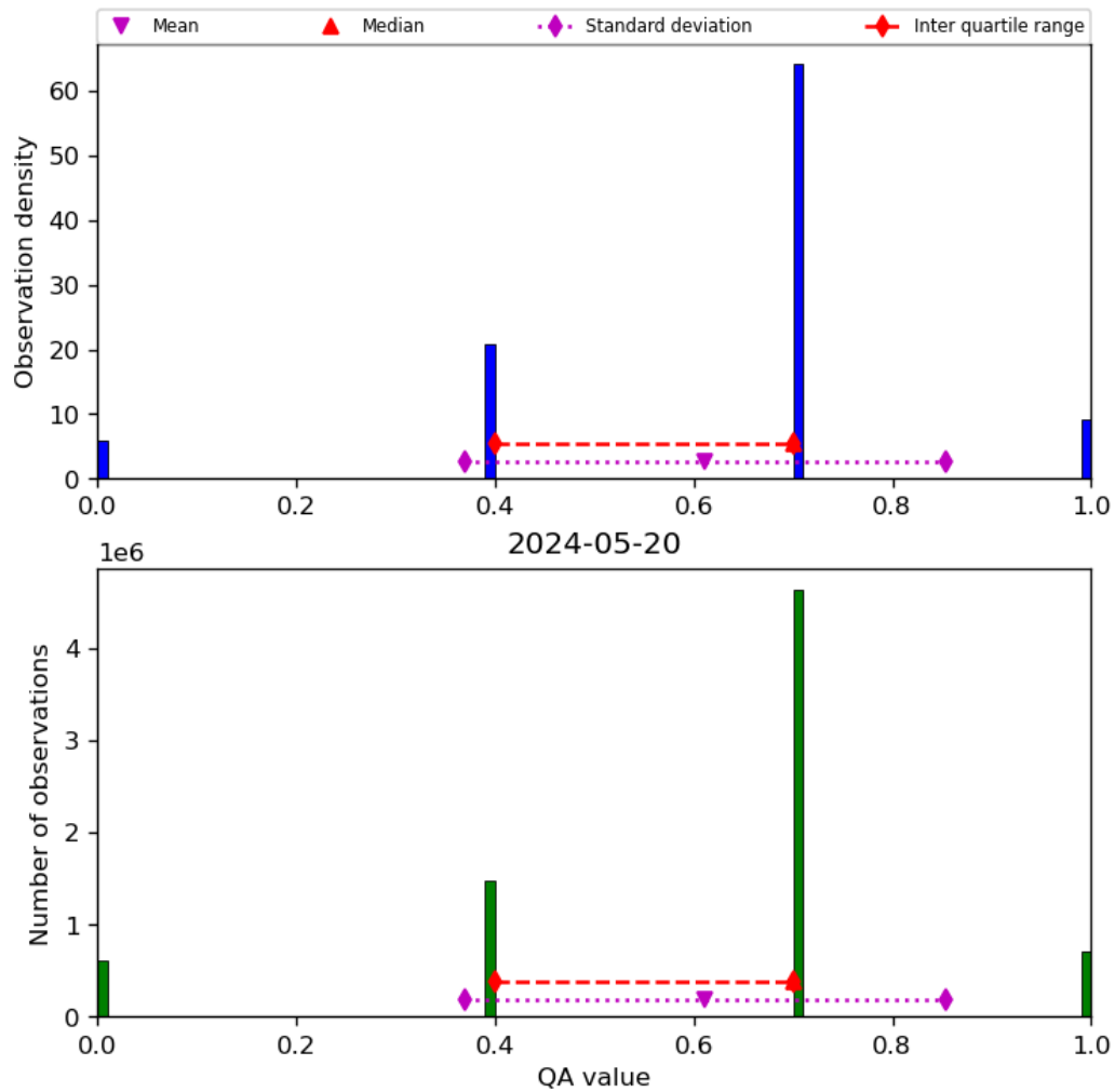
Figure 17: Histogram of “QA value” for 2024-05-19 to 2024-05-21
