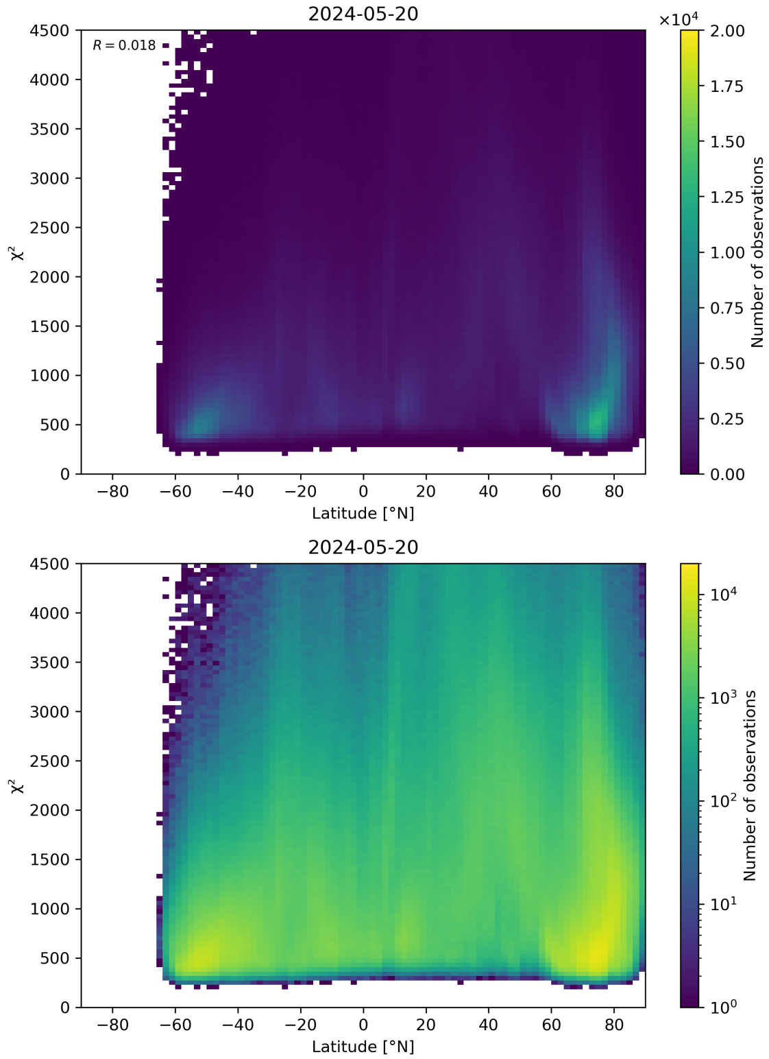
Figure 54: Scatter density plot of “Latitude” against “ \chi^2 ” for 2024-05-19 to 2024-05-21.
