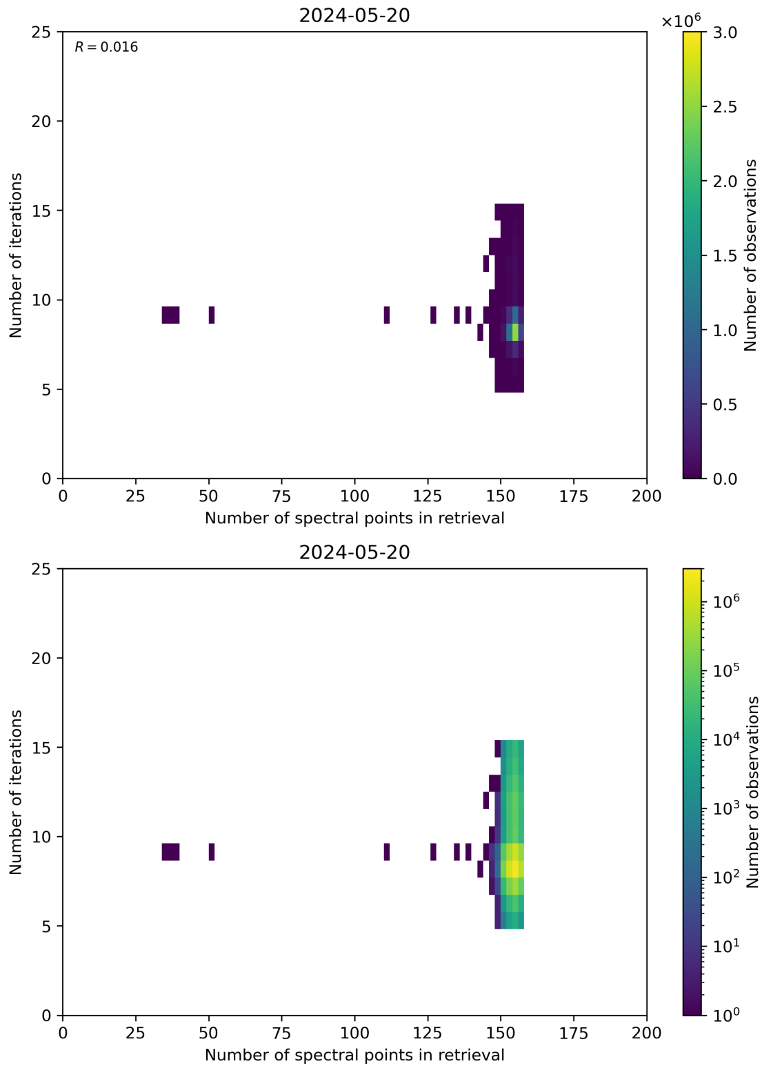
Figure 60: Scatter density plot of “Number of spectral points in retrieval” against “Number of iterations” for 2024-05-19 to 2024-05-21.
