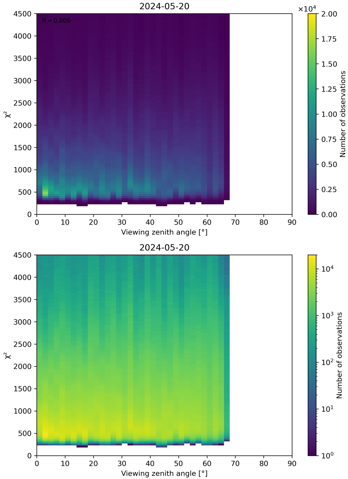
Figure 72: Scatter density plot of “Viewing zenith angle” against “ \chi^2 ” for 2024-05-19 to 2024-05-21.
