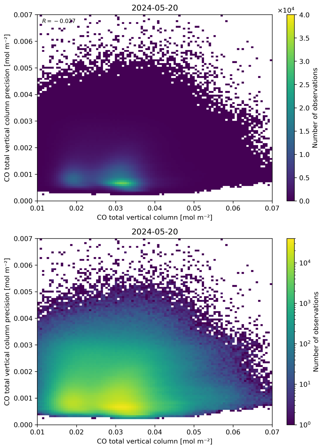
Figure 34: Scatter density plot of “CO total vertical column” against “CO total vertical column precision” for 2024-05-19 to 2024-05-21.
