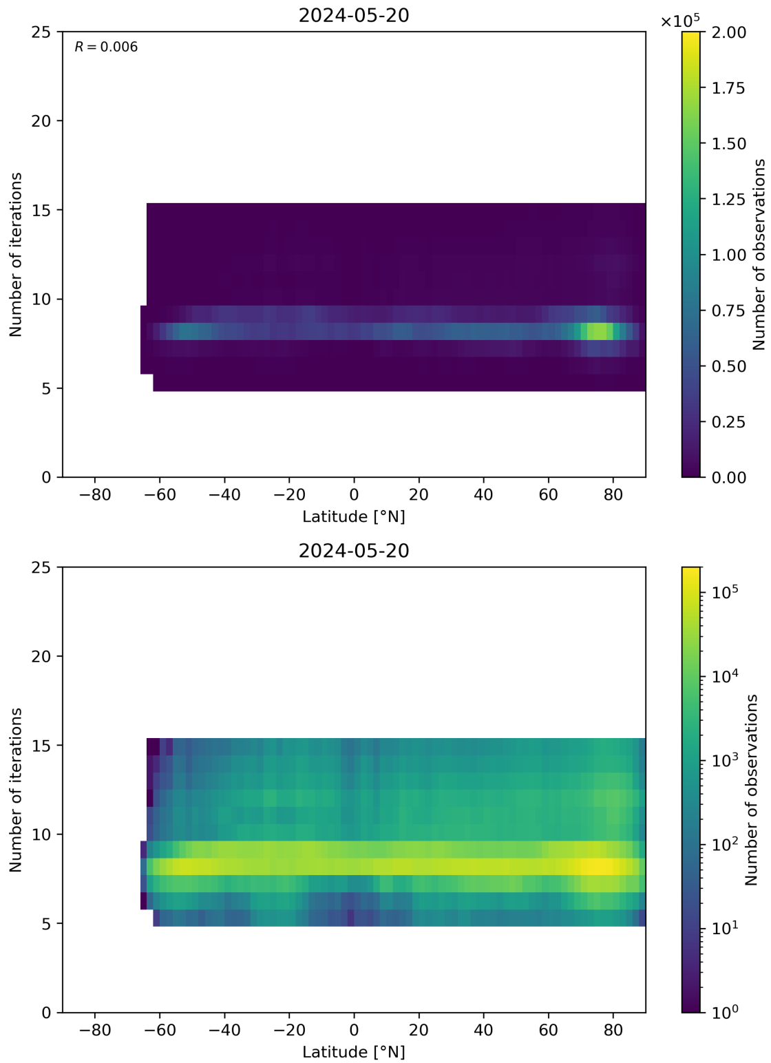
Figure 56: Scatter density plot of “Latitude” against “Number of iterations” for 2024-05-19 to 2024-05-21.
