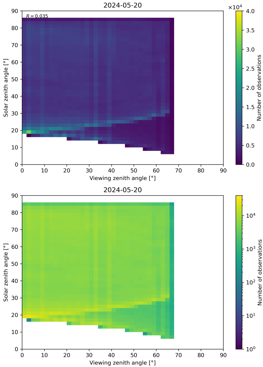
Figure 77: Scatter density plot of “Viewing zenith angle” against “Solar zenith angle” for 2024-05-19 to 2024-05-21.
