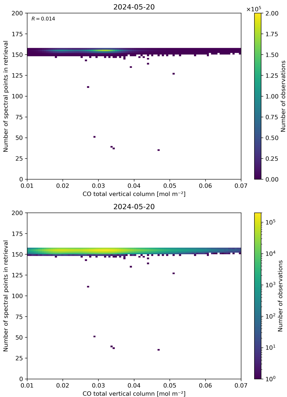
Figure 43: Scatter density plot of “CO total vertical column” against “Number of spectral points in retrieval” for 2024-05-19 to 2024-05-21.
