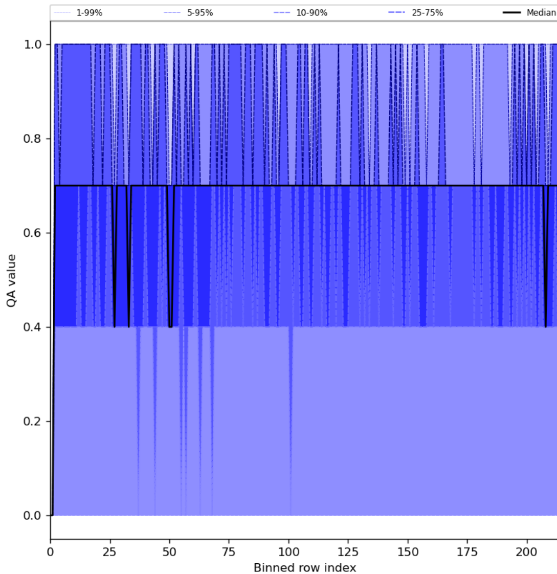
Figure 25: Along track statistics of “QA value” for 2024-05-19 to 2024-05-21
