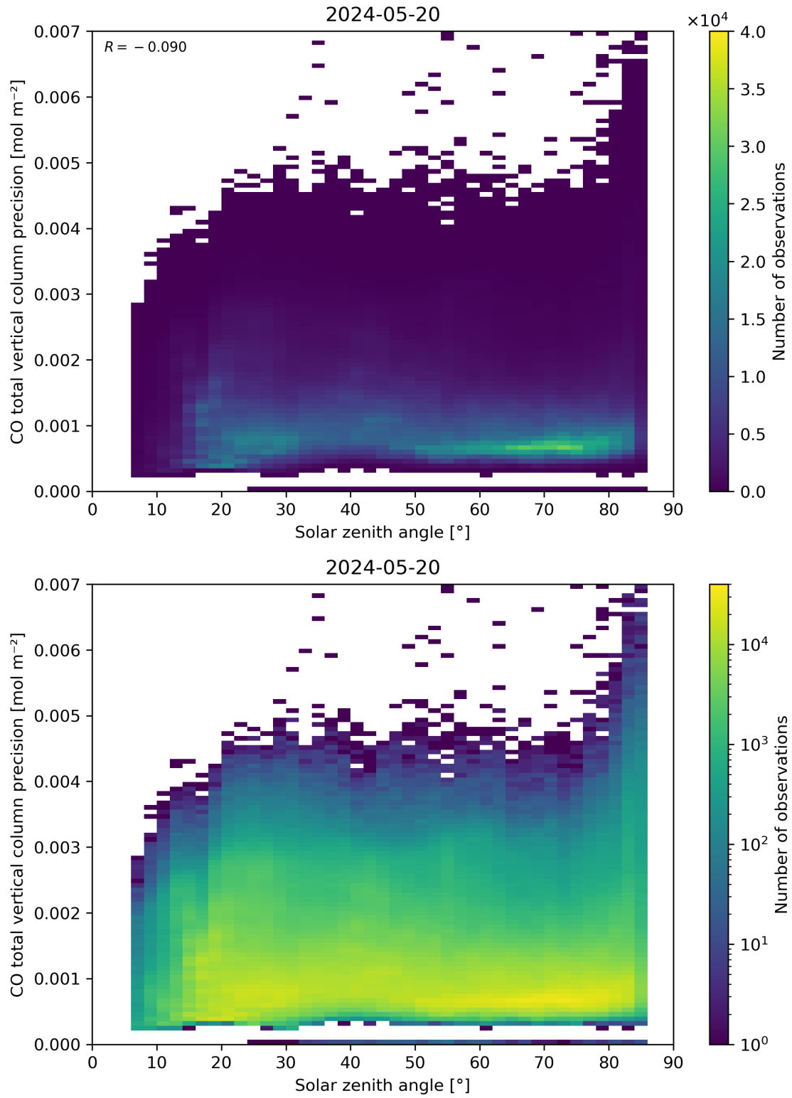
Figure 63: Scatter density plot of “Solar zenith angle” against “CO total vertical column precision” for 2024-05-19 to 2024-05-21.
