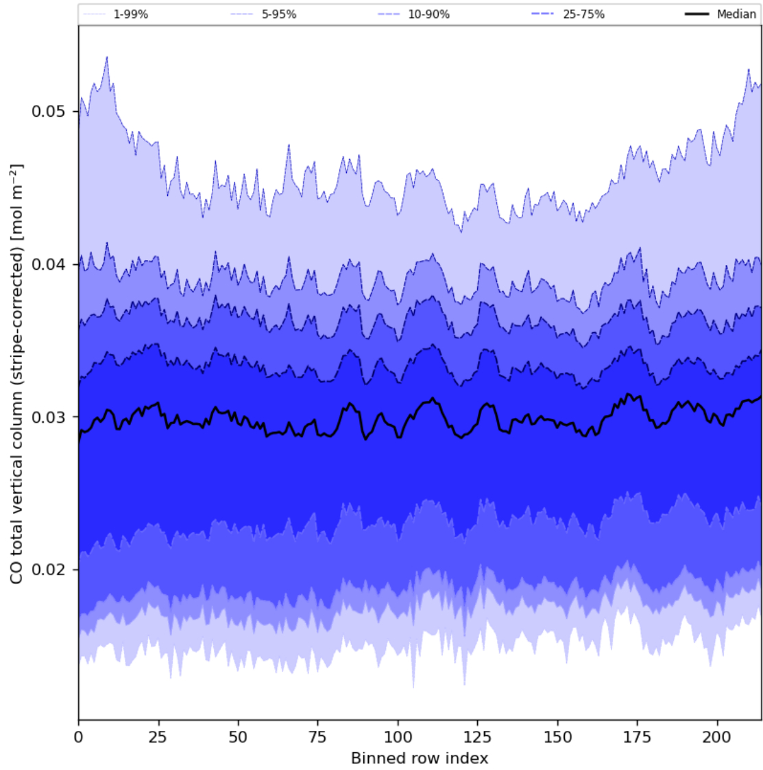
Figure 27: Along track statistics of “CO total vertical column (stripe-corrected)” for 2024-05-19 to 2024-05-21
