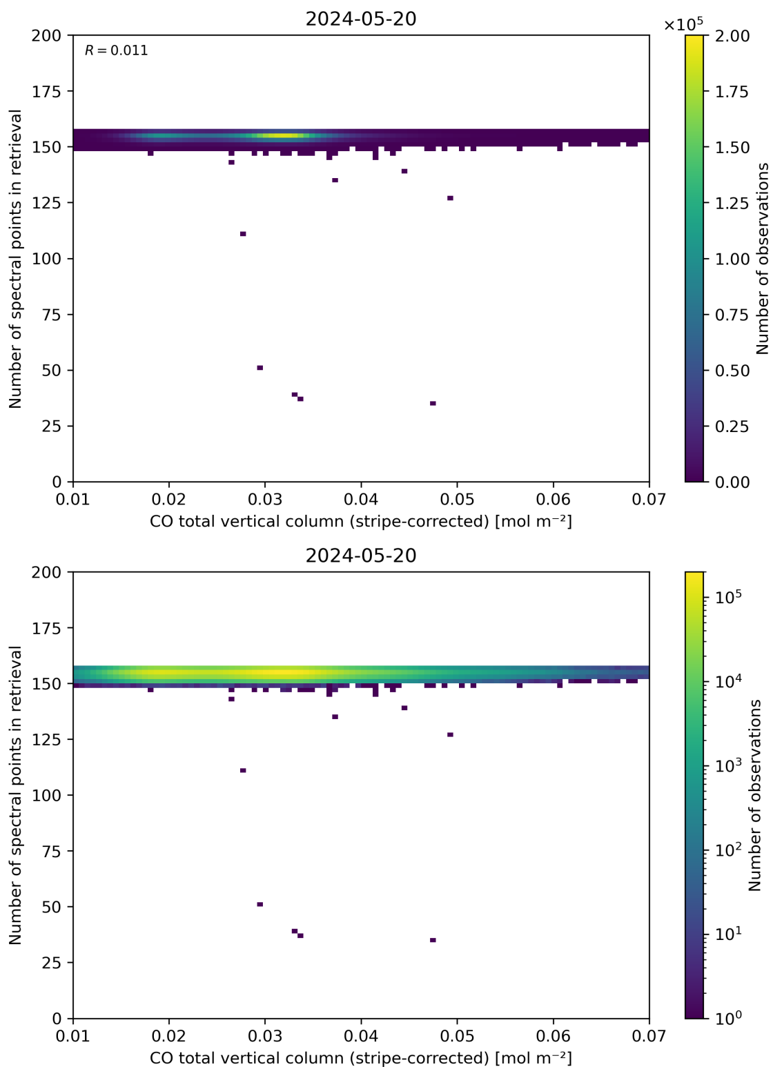
Figure 40: Scatter density plot of “CO total vertical column (stripe-corrected)” against “Number of spectral points in retrieval” for 2024-05-19 to 2024-05-21.
