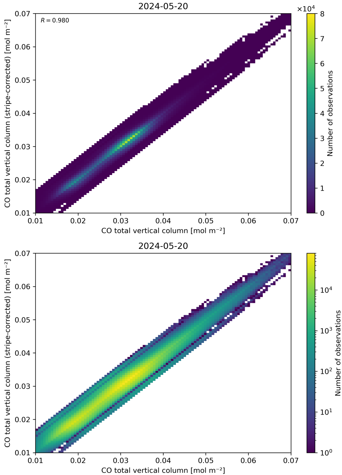
Figure 33: Scatter density plot of “CO total vertical column” against “CO total vertical column (stripe-corrected)” for 2024-05-19 to 2024-05-21.
