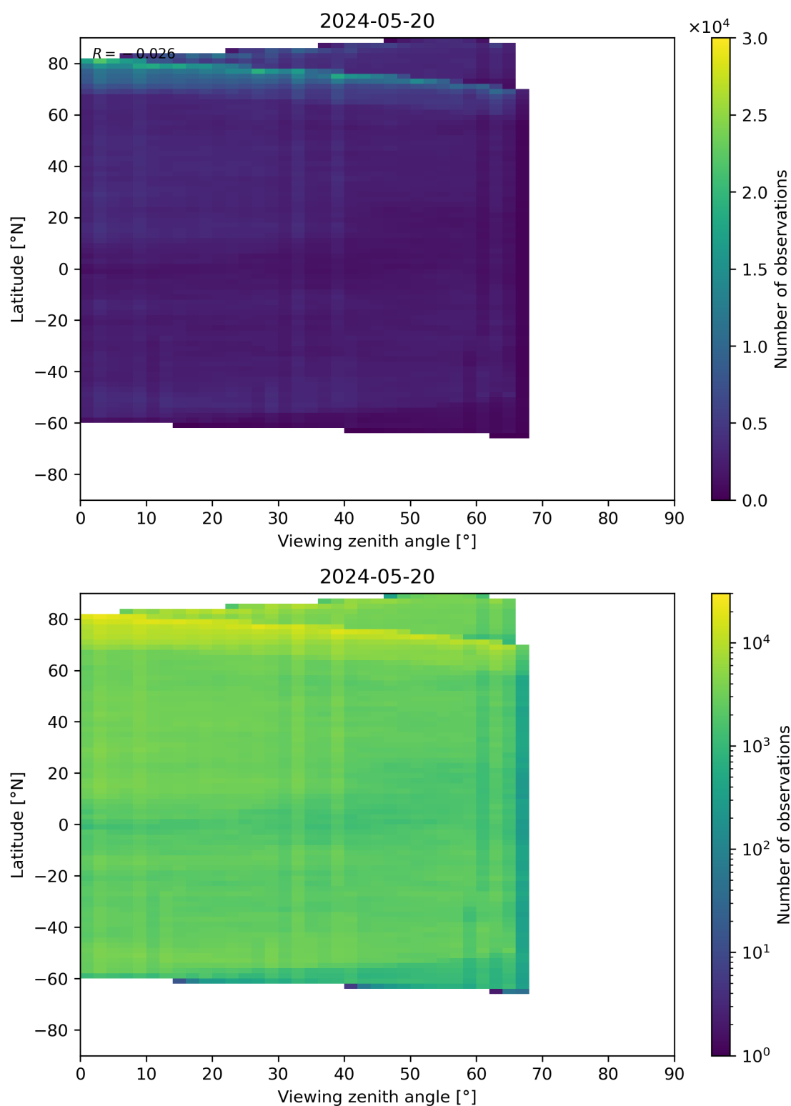
Figure 74: Scatter density plot of “Viewing zenith angle” against “Latitude” for 2024-05-19 to 2024-05-21.
