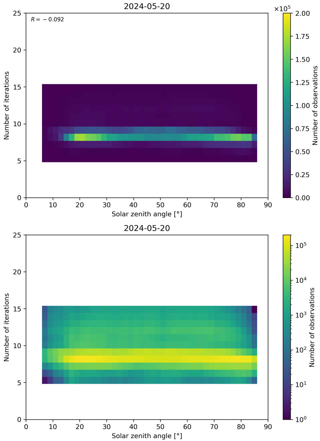
Figure 67: Scatter density plot of “Solar zenith angle” against “Number of iterations” for 2024-05-19 to 2024-05-21.
