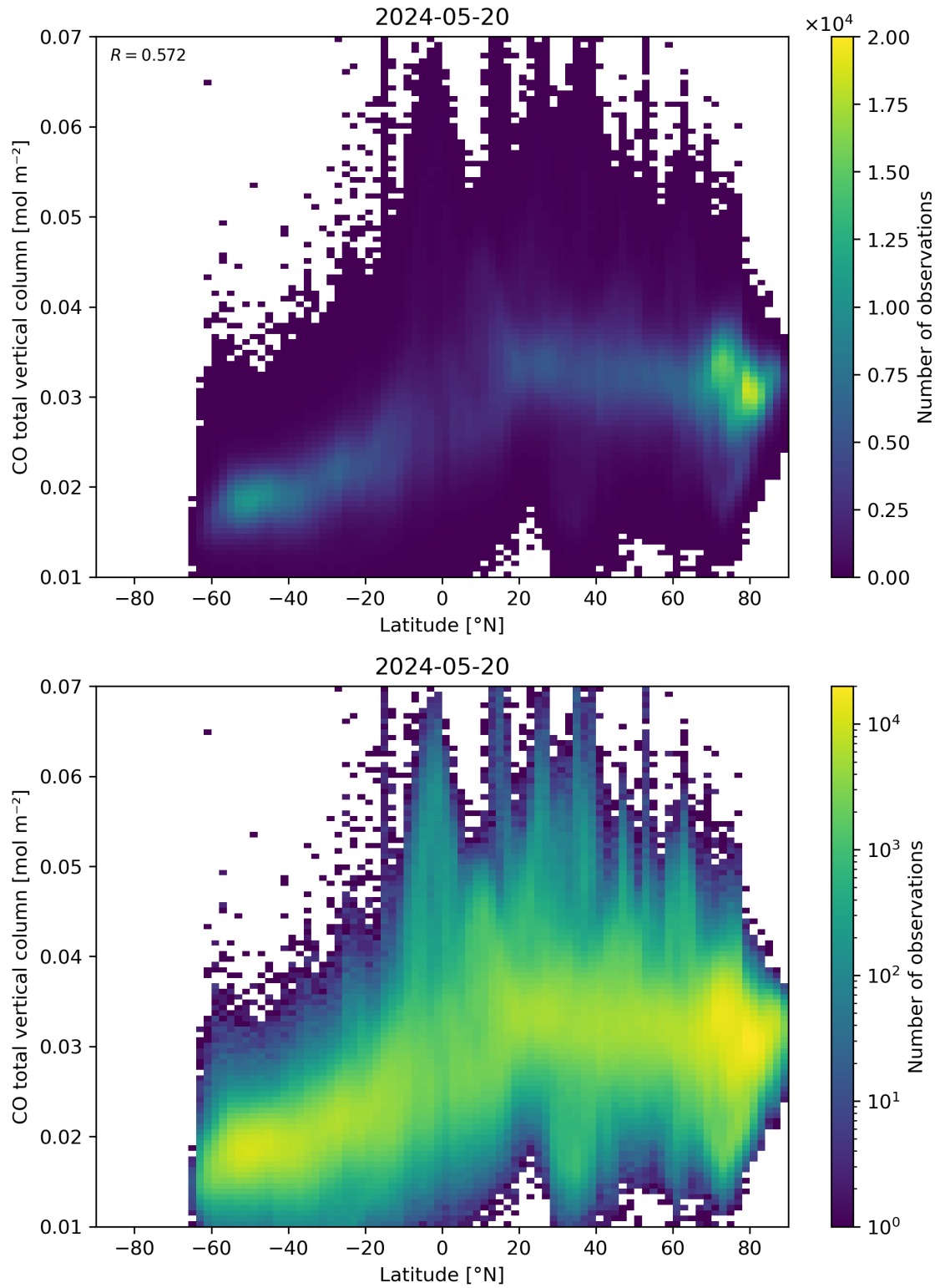
Figure 51: Scatter density plot of “Latitude” against “CO total vertical column” for 2024-05-19 to 2024-05-21.
