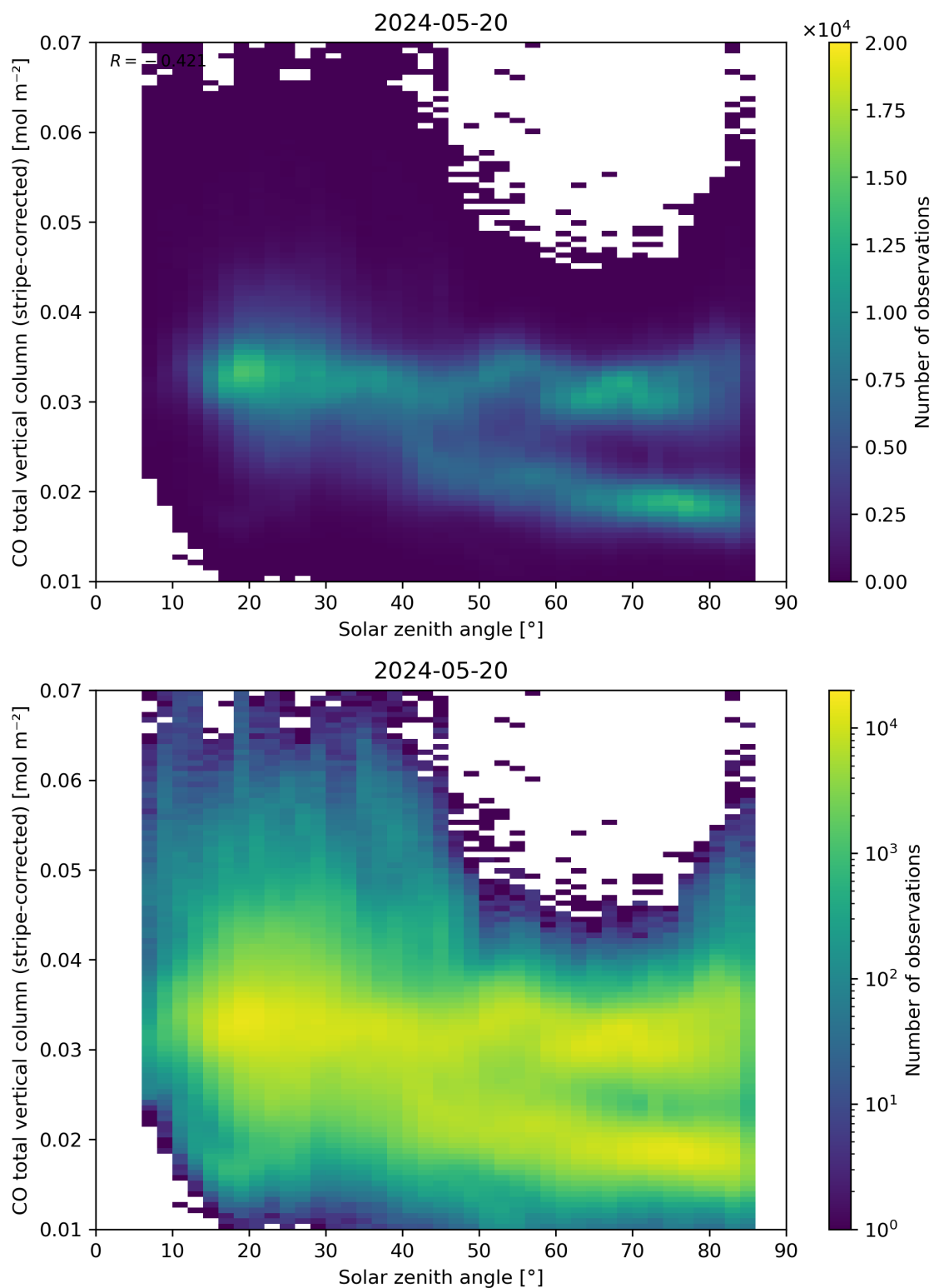
Figure 62: Scatter density plot of “Solar zenith angle” against “CO total vertical column (stripe-corrected)” for 2024-05-19 to 2024-05-21.
