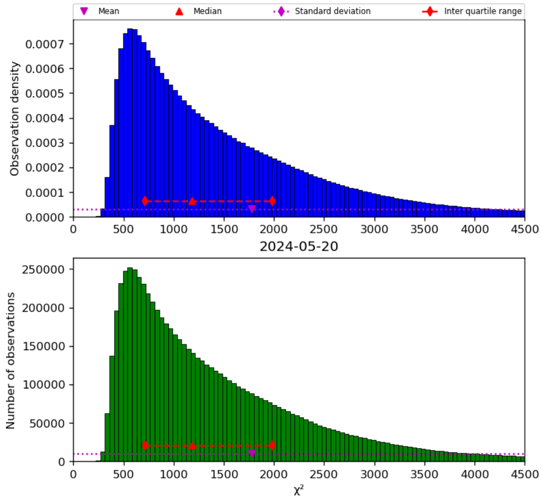
Figure 22: Histogram of “ \chi^2 ” for 2024-05-19 to 2024-05-21
