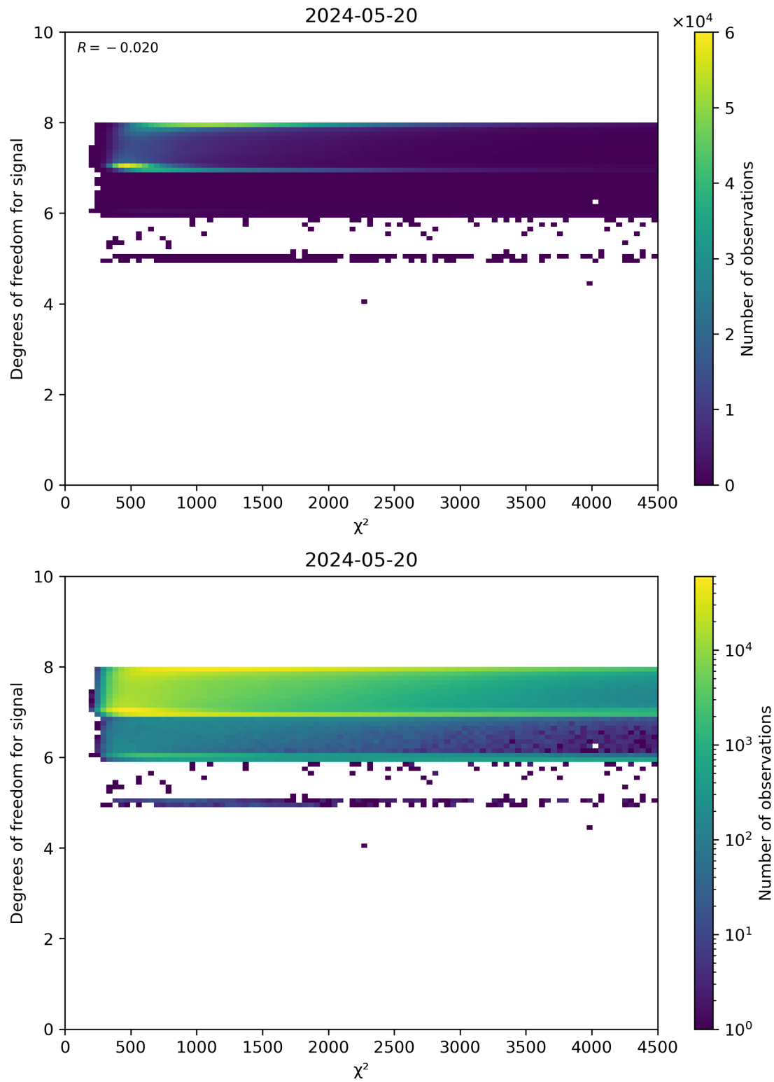
Figure 48: Scatter density plot of “ \chi^2 ” against “Degrees of freedom for signal” for 2024-05-19 to 2024-05-21.
