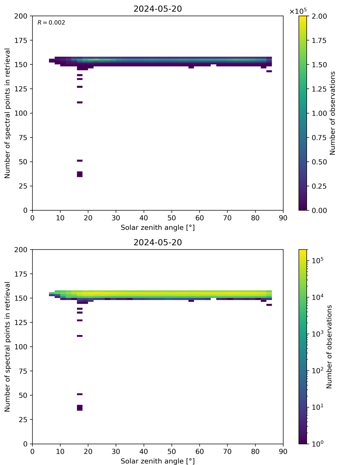
Figure 68: Scatter density plot of “Solar zenith angle” against “Number of spectral points in retrieval” for 2024-05-19 to 2024-05-21.
