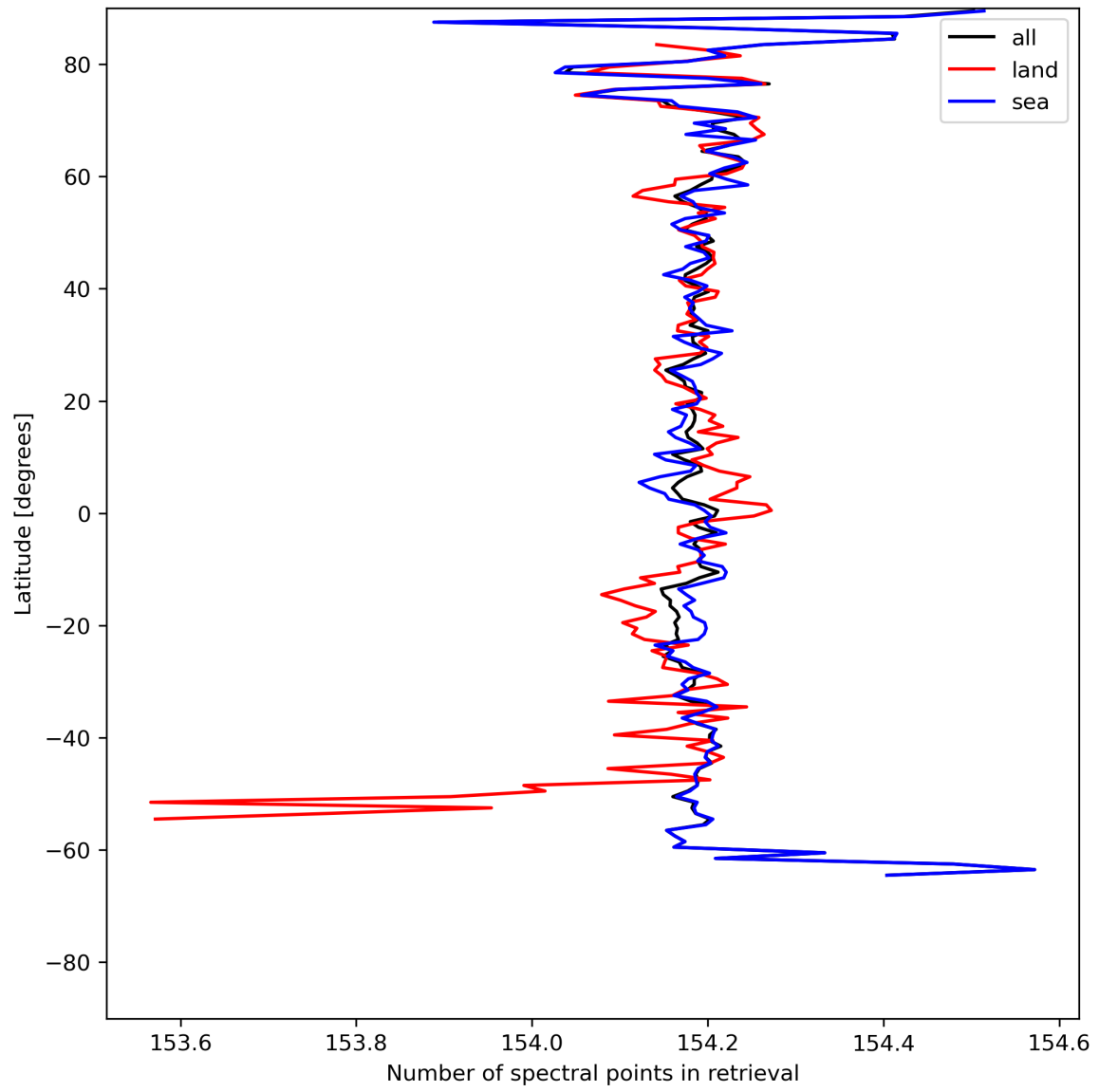
Figure 13: Zonal average of “Number of spectral points in retrieval” for 2024-05-19 to 2024-05-21.
