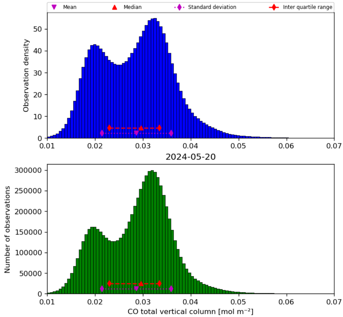
Figure 18: Histogram of “CO total vertical column” for 2024-05-19 to 2024-05-21
