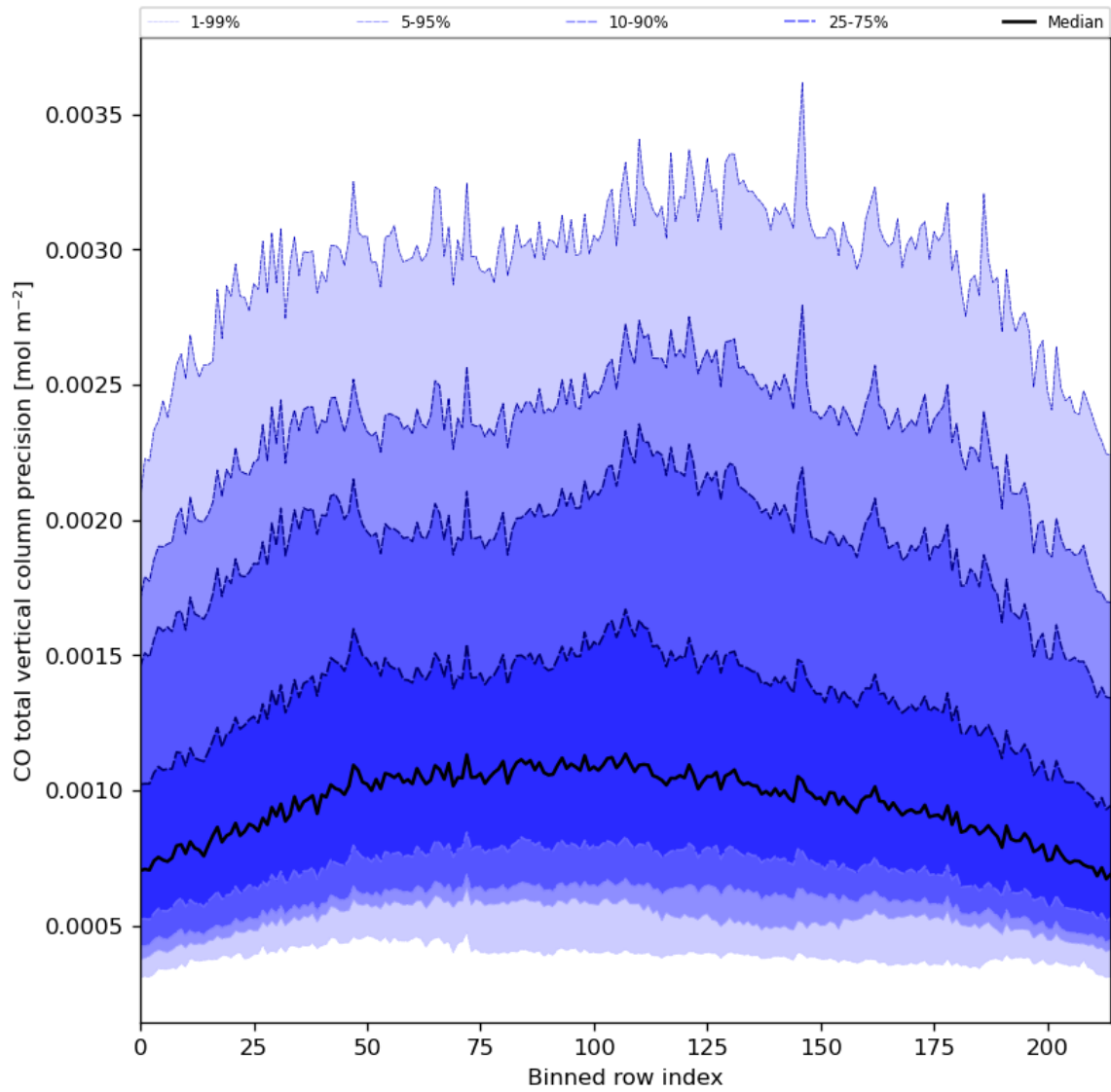
Figure 28: Along track statistics of “CO total vertical column precision” for 2024-05-19 to 2024-05-21
