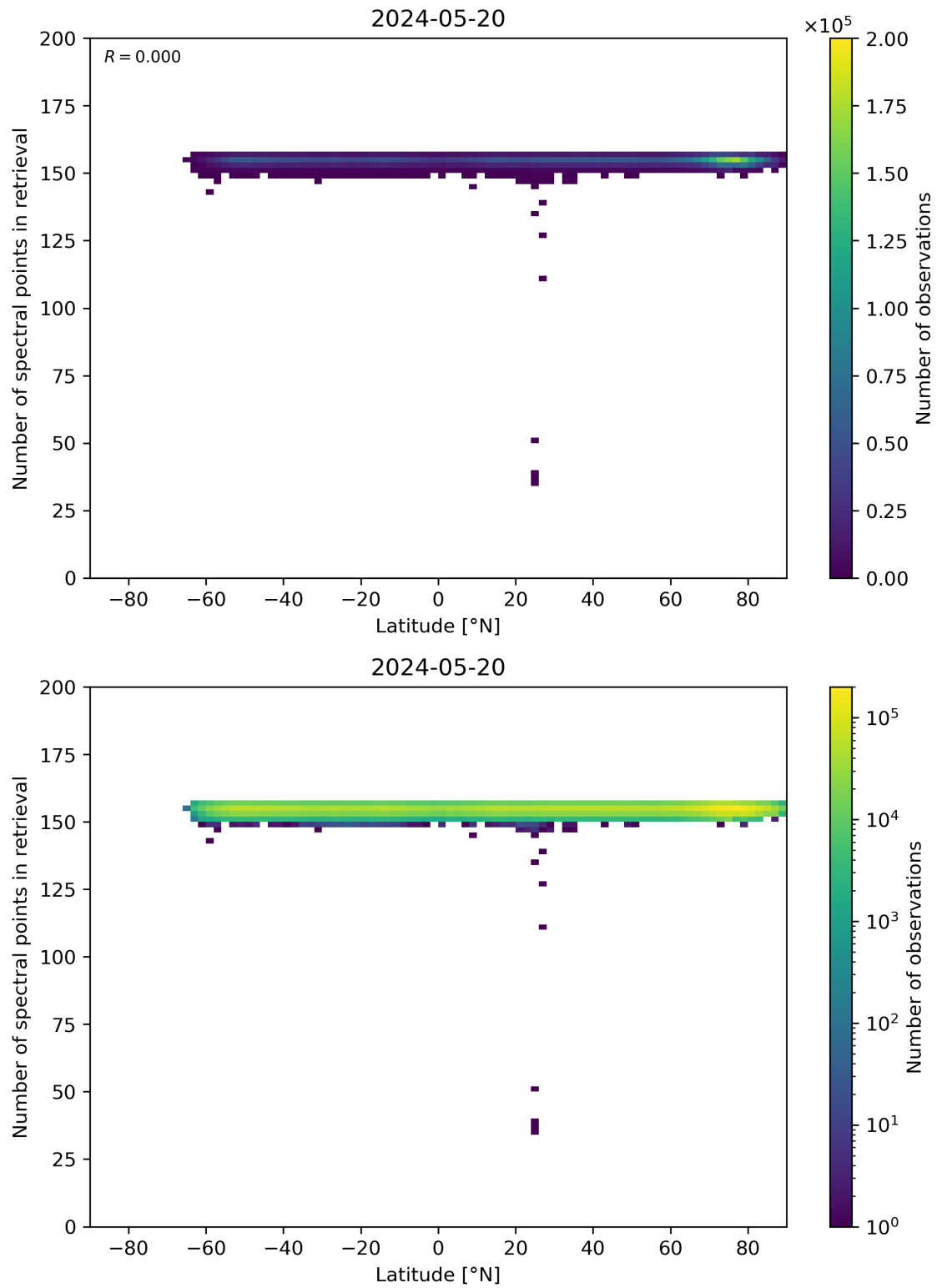
Figure 57: Scatter density plot of “Latitude” against “Number of spectral points in retrieval” for 2024-05-19 to 2024-05-21.
