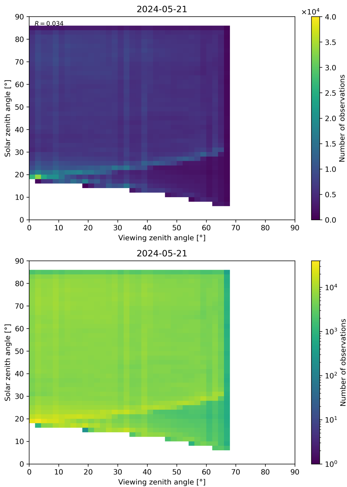
Figure 77: Scatter density plot of “Viewing zenith angle” against “Solar zenith angle” for 2024-05-20 to 2024-05-22.
