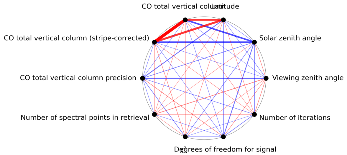
Figure 1: Map of correlation graph for 2024-05-20 to 2024-05-22.
