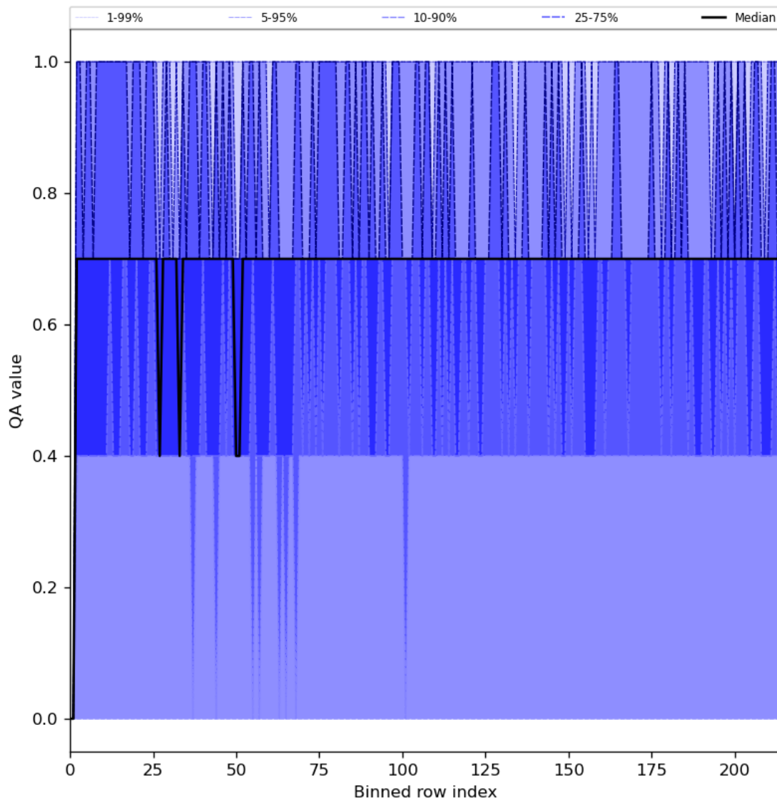
Figure 25: Along track statistics of “QA value” for 2024-05-20 to 2024-05-22
