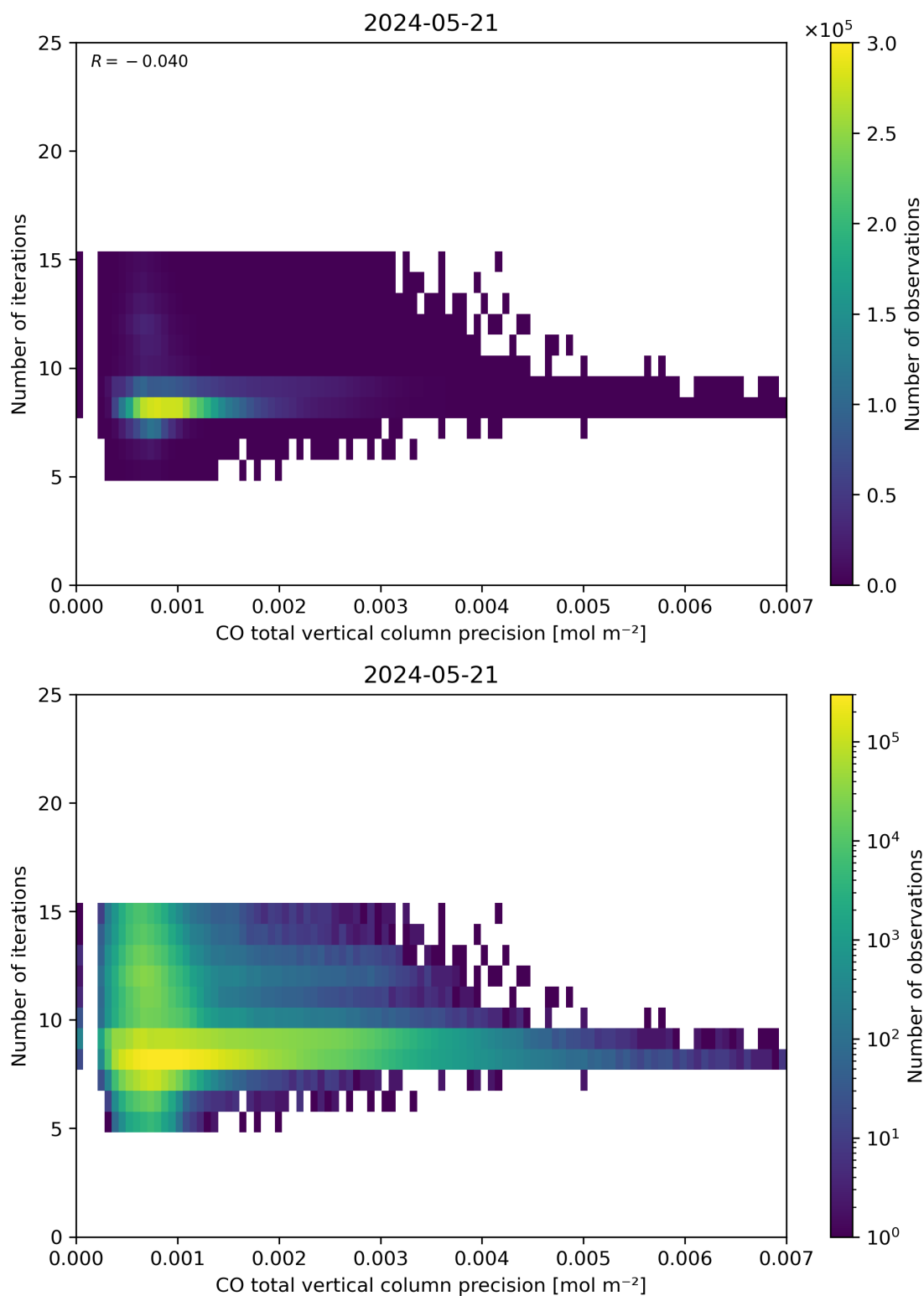
Figure 46: Scatter density plot of “CO total vertical column precision” against “Number of iterations” for 2024-05-20 to 2024-05-22.
