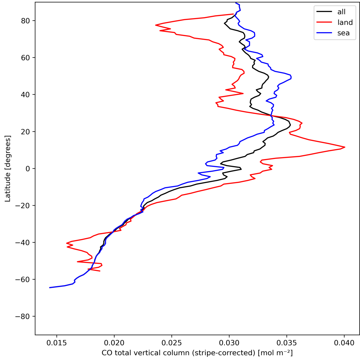
Figure 11: Zonal average of “CO total vertical column (stripe-corrected)” for 2024-05-20 to 2024-05-22.
