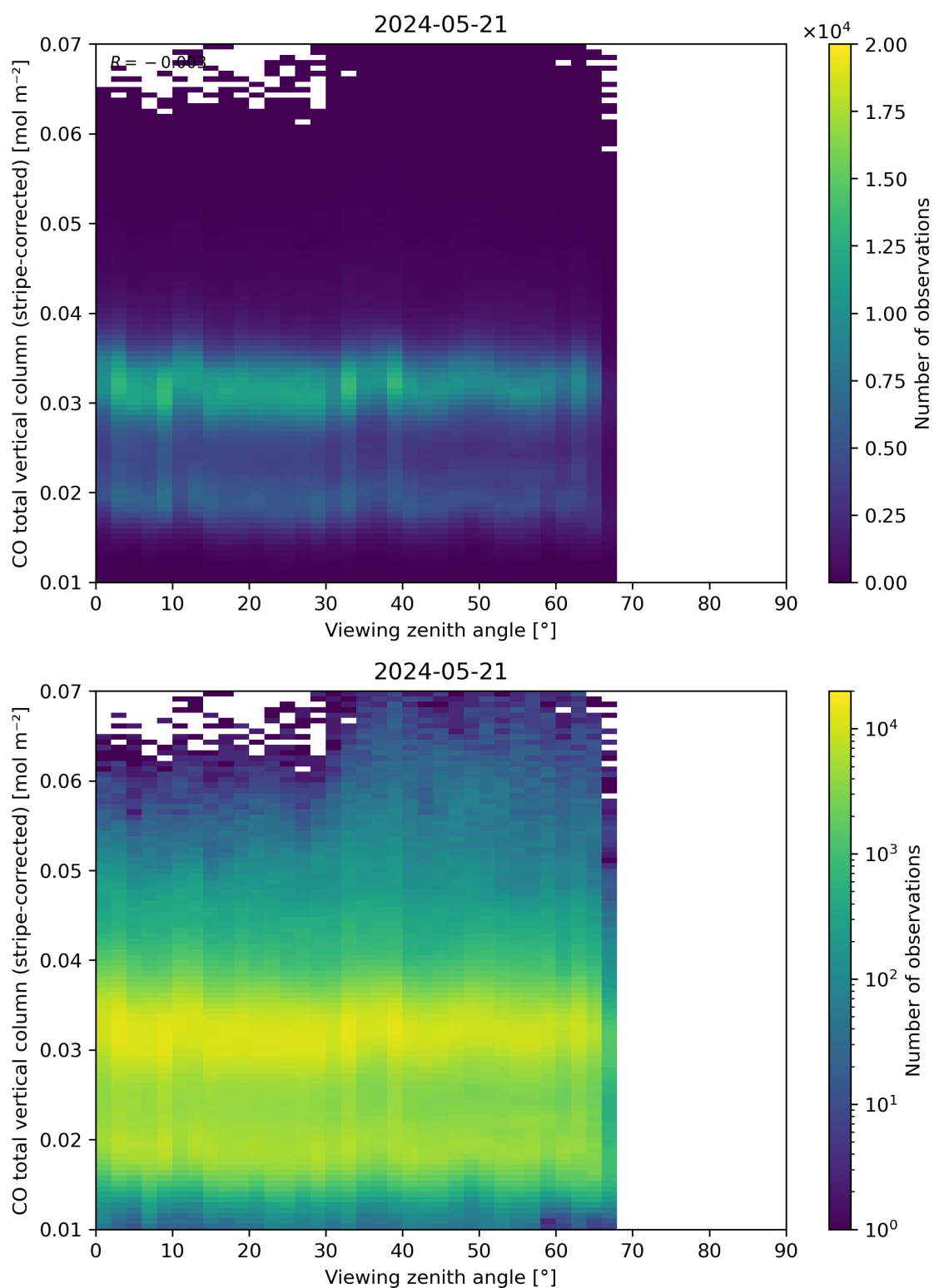
Figure 70: Scatter density plot of “Viewing zenith angle” against “CO total vertical column (stripe-corrected)” for 2024-05-20 to 2024-05-22.
