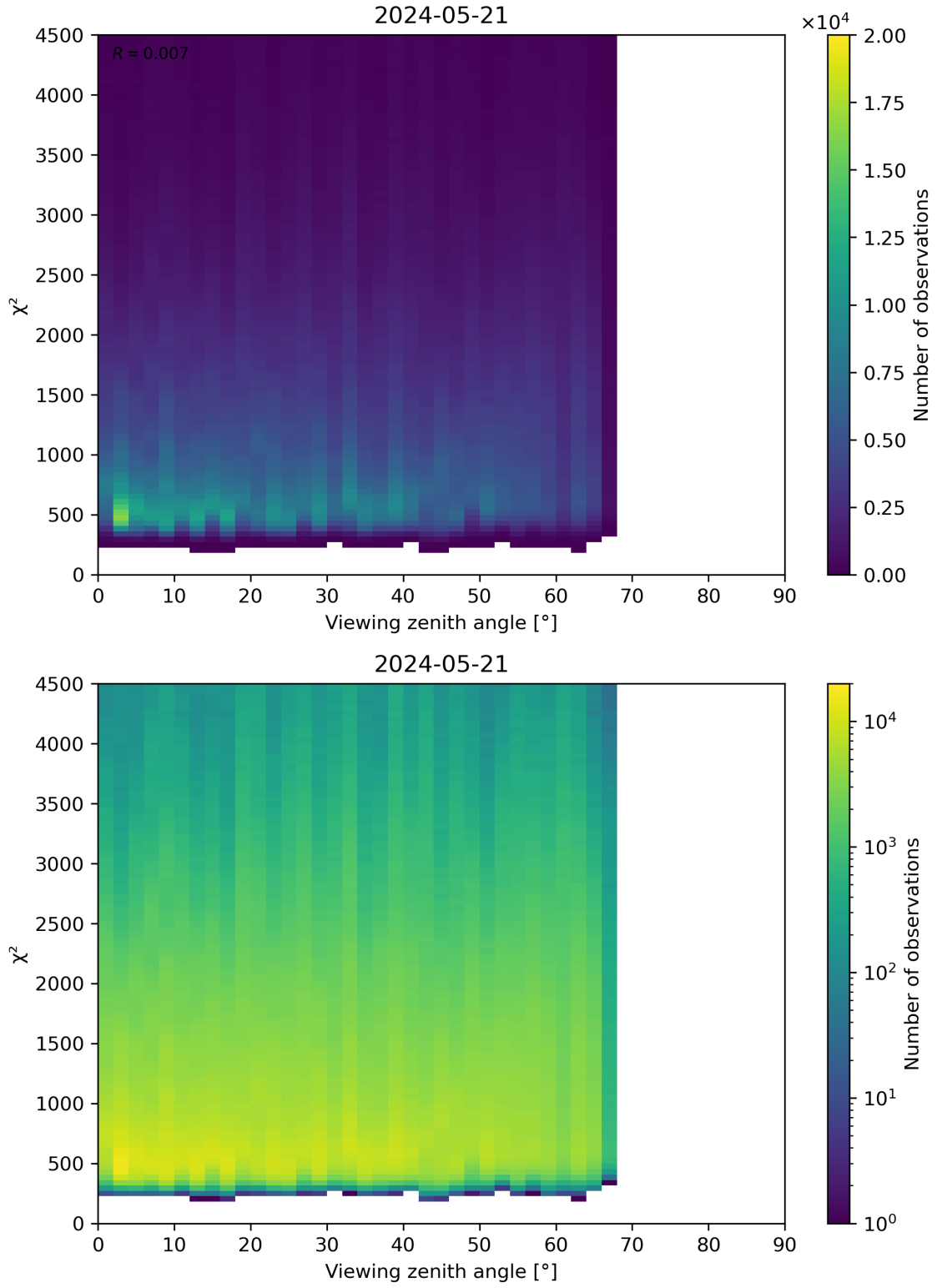
Figure 72: Scatter density plot of “Viewing zenith angle” against “ \chi^2 ” for 2024-05-20 to 2024-05-22.
