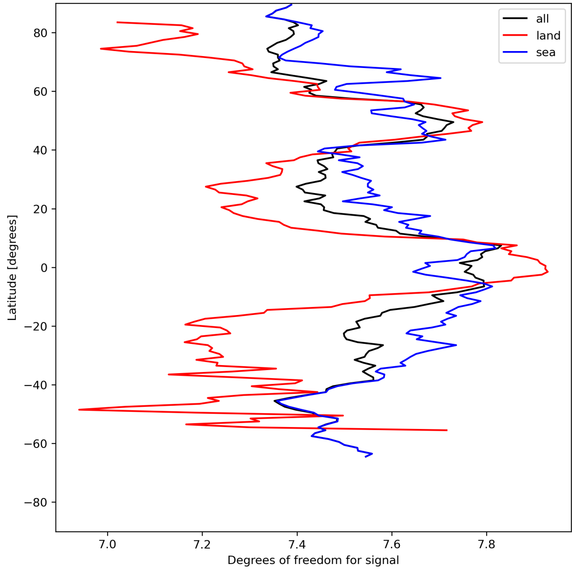
Figure 15: Zonal average of “Degrees of freedom for signal” for 2024-05-20 to 2024-05-22.
