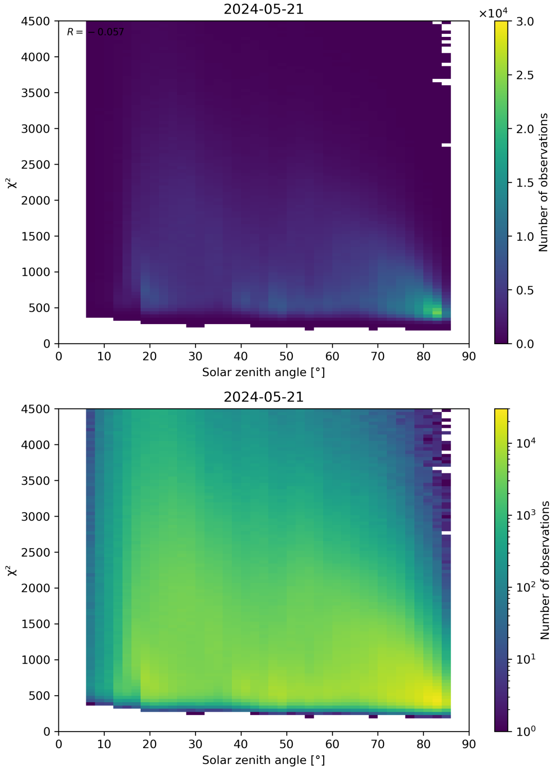
Figure 64: Scatter density plot of “Solar zenith angle” against “ \chi^2 ” for 2024-05-20 to 2024-05-22.
