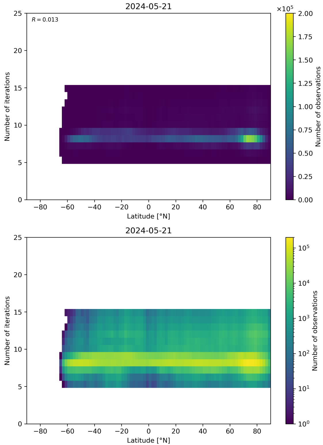
Figure 56: Scatter density plot of “Latitude” against “Number of iterations” for 2024-05-20 to 2024-05-22.
