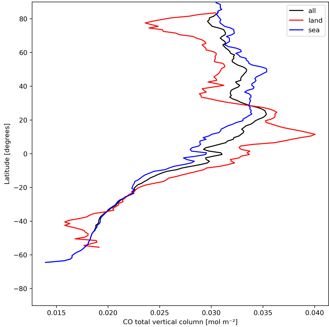
Figure 10: Zonal average of “CO total vertical column” for 2024-05-20 to 2024-05-22.
