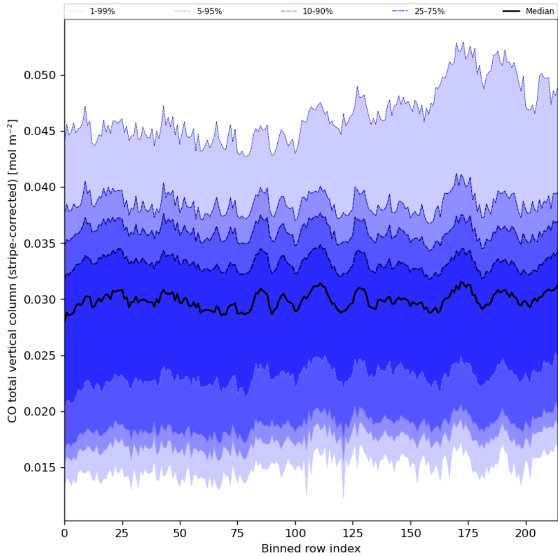
Figure 27: Along track statistics of “CO total vertical column (stripe-corrected)” for 2024-05-20 to 2024-05-22
