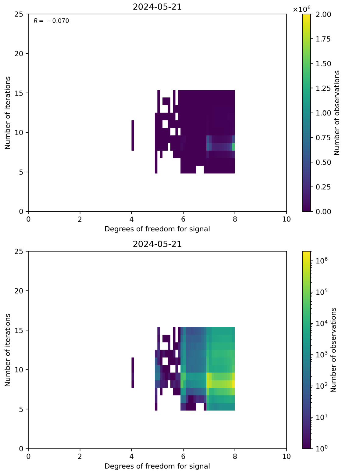
Figure 50: Scatter density plot of “Degrees of freedom for signal” against “Number of iterations” for 2024-05-20 to 2024-05-22.
