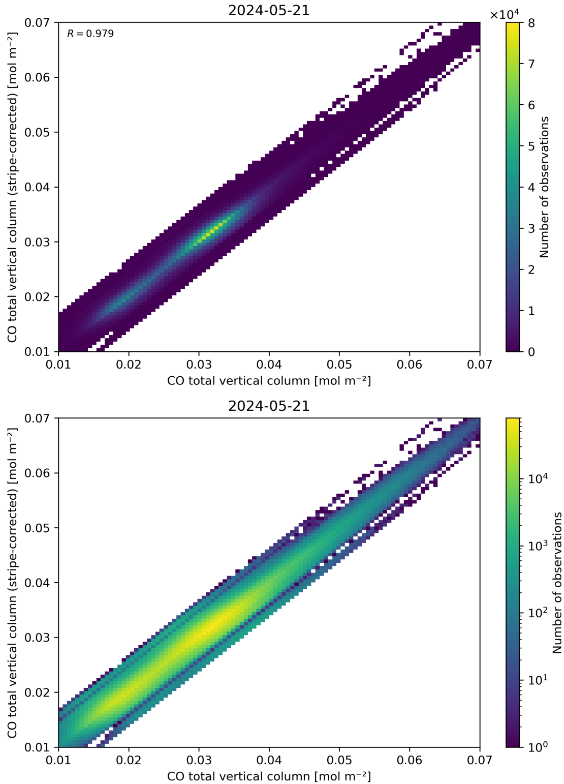
Figure 33: Scatter density plot of “CO total vertical column” against “CO total vertical column (stripe-corrected)” for 2024-05-20 to 2024-05-22.
