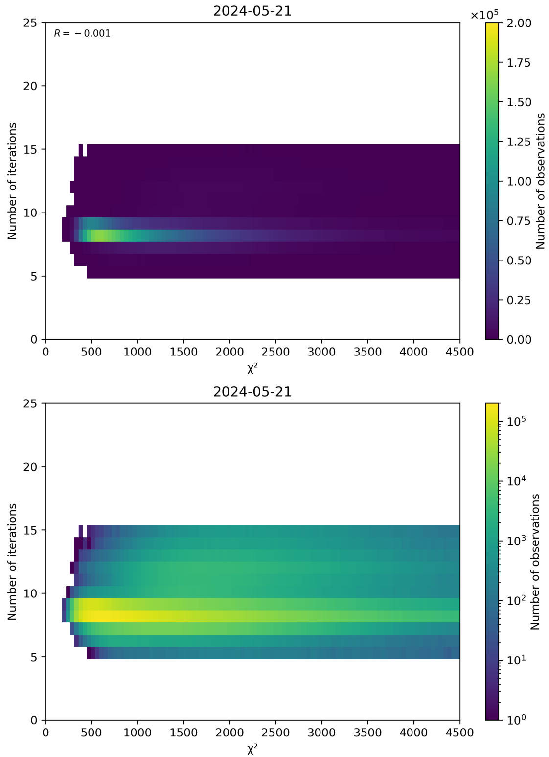
Figure 49: Scatter density plot of “ \chi^2 ” against “Number of iterations” for 2024-05-20 to 2024-05-22.
