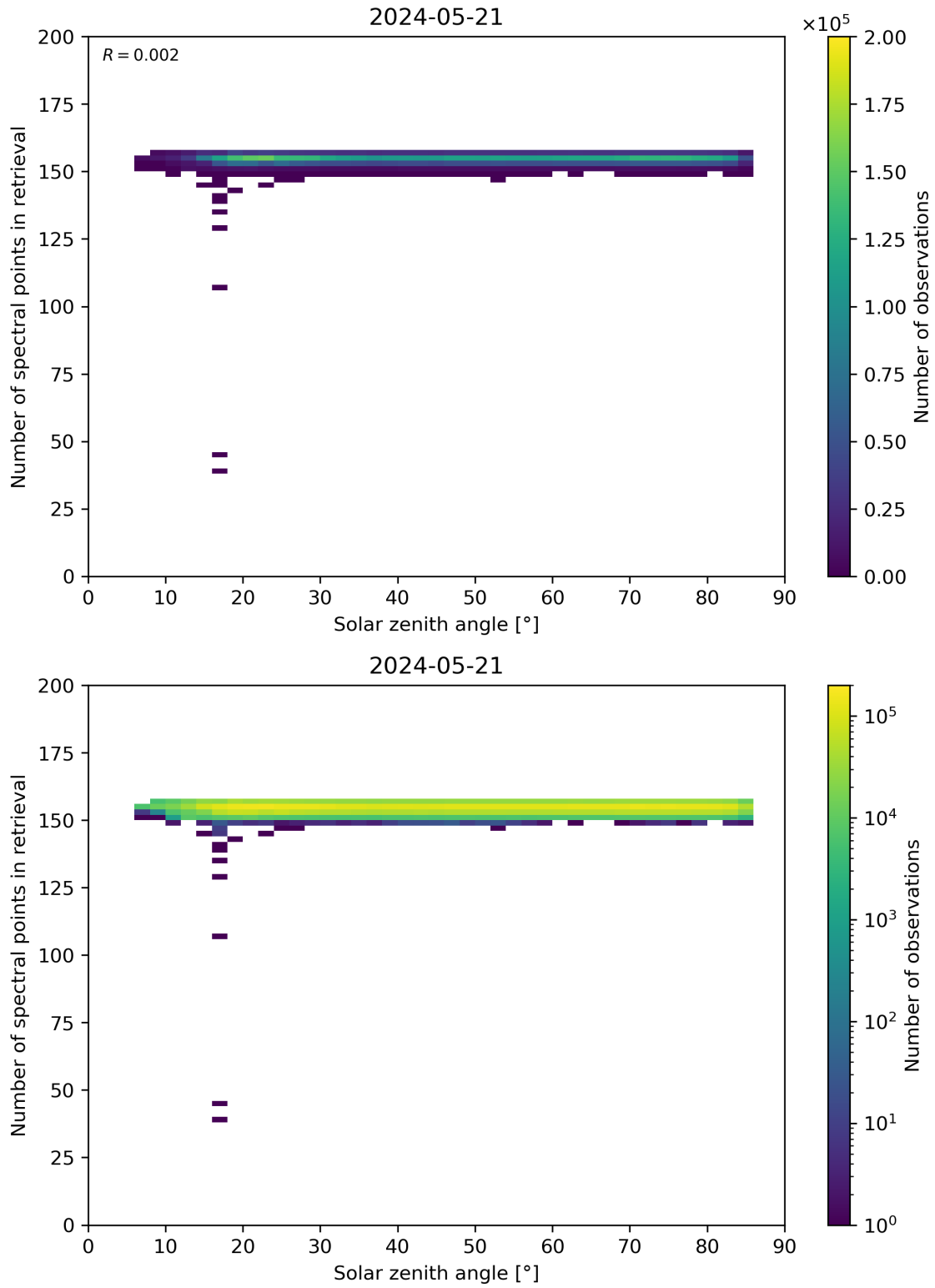
Figure 68: Scatter density plot of “Solar zenith angle” against “Number of spectral points in retrieval” for 2024-05-20 to 2024-05-22.
