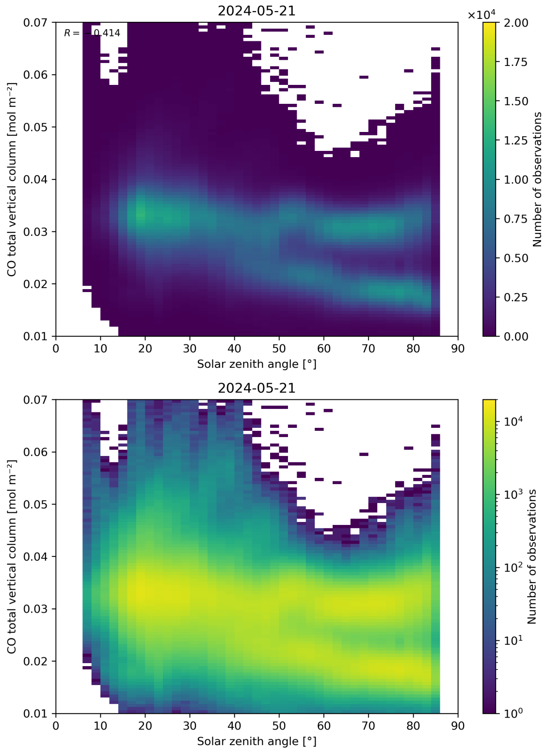
Figure 61: Scatter density plot of “Solar zenith angle” against “CO total vertical column” for 2024-05-20 to 2024-05-22.
