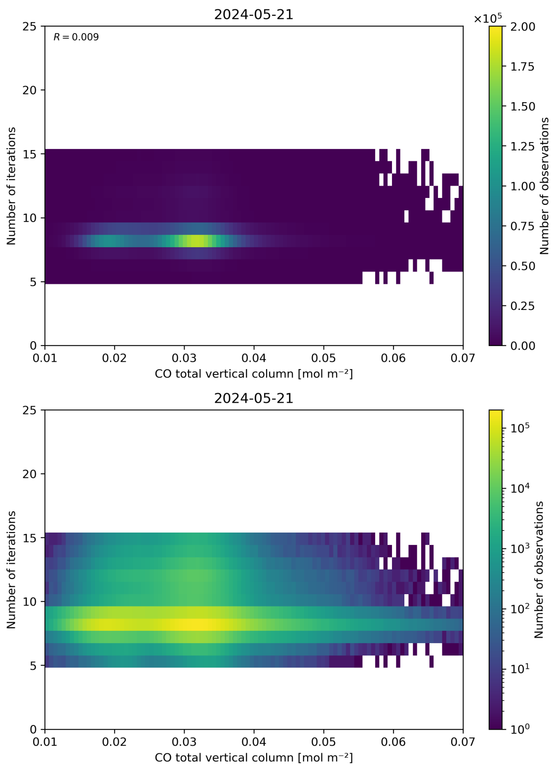
Figure 42: Scatter density plot of “CO total vertical column” against “Number of iterations” for 2024-05-20 to 2024-05-22.
