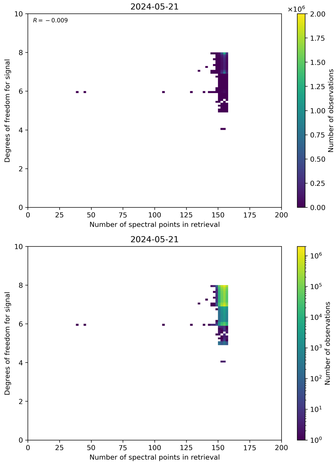
Figure 59: Scatter density plot of “Number of spectral points in retrieval” against “Degrees of freedom for signal” for 2024-05-20 to 2024-05-22.
