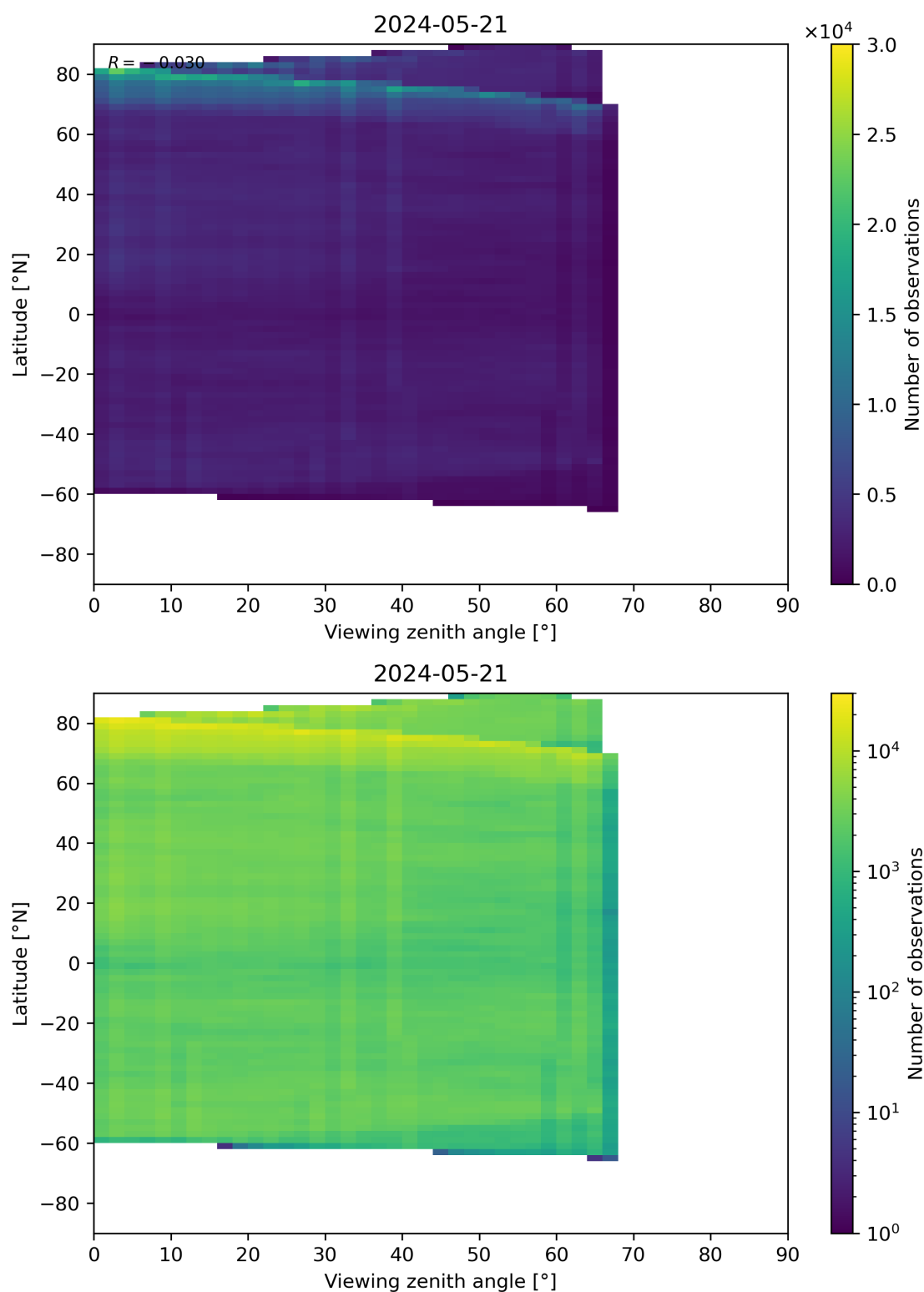
Figure 74: Scatter density plot of “Viewing zenith angle” against “Latitude” for 2024-05-20 to 2024-05-22.
