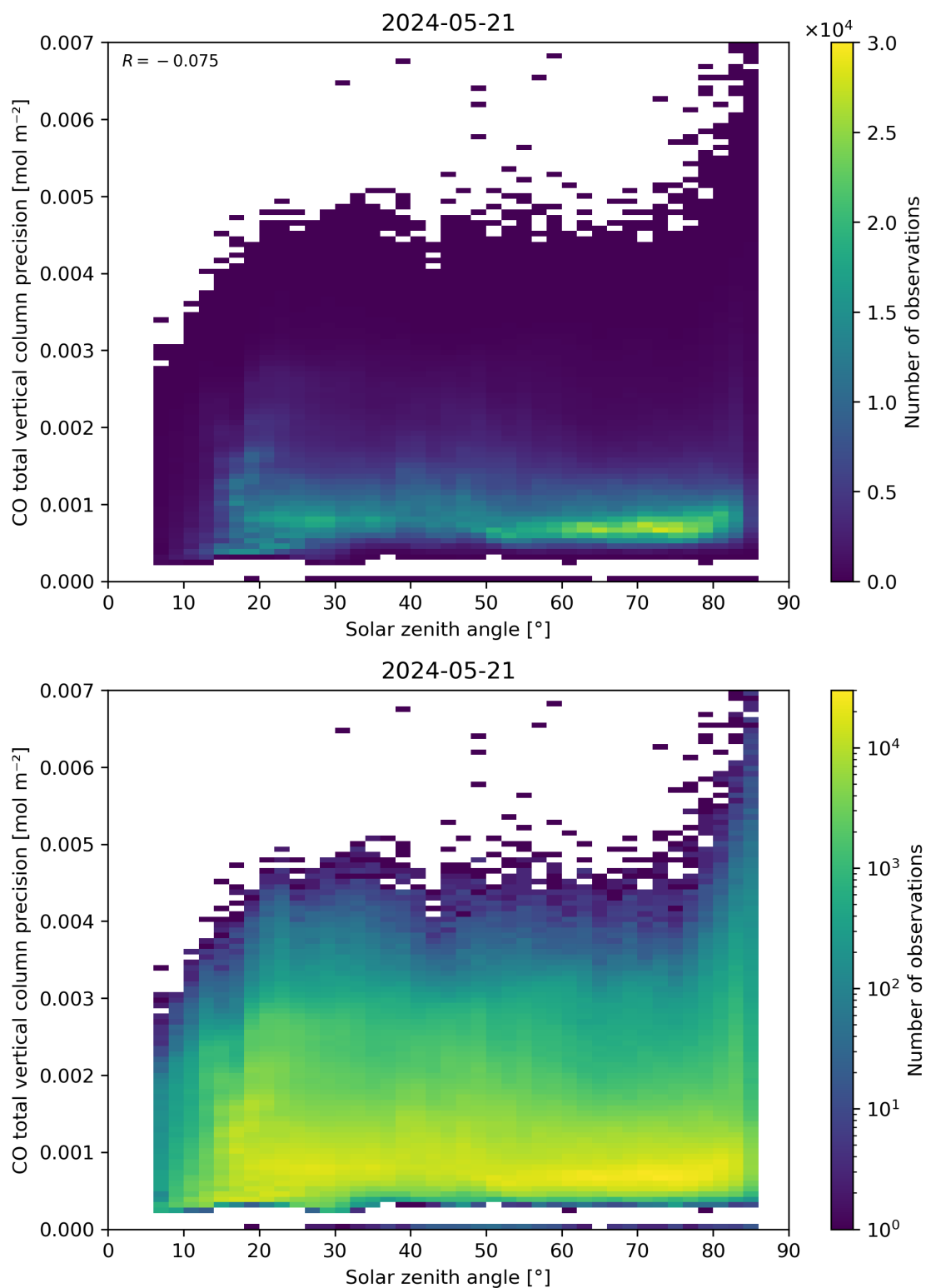
Figure 63: Scatter density plot of “Solar zenith angle” against “CO total vertical column precision” for 2024-05-20 to 2024-05-22.
