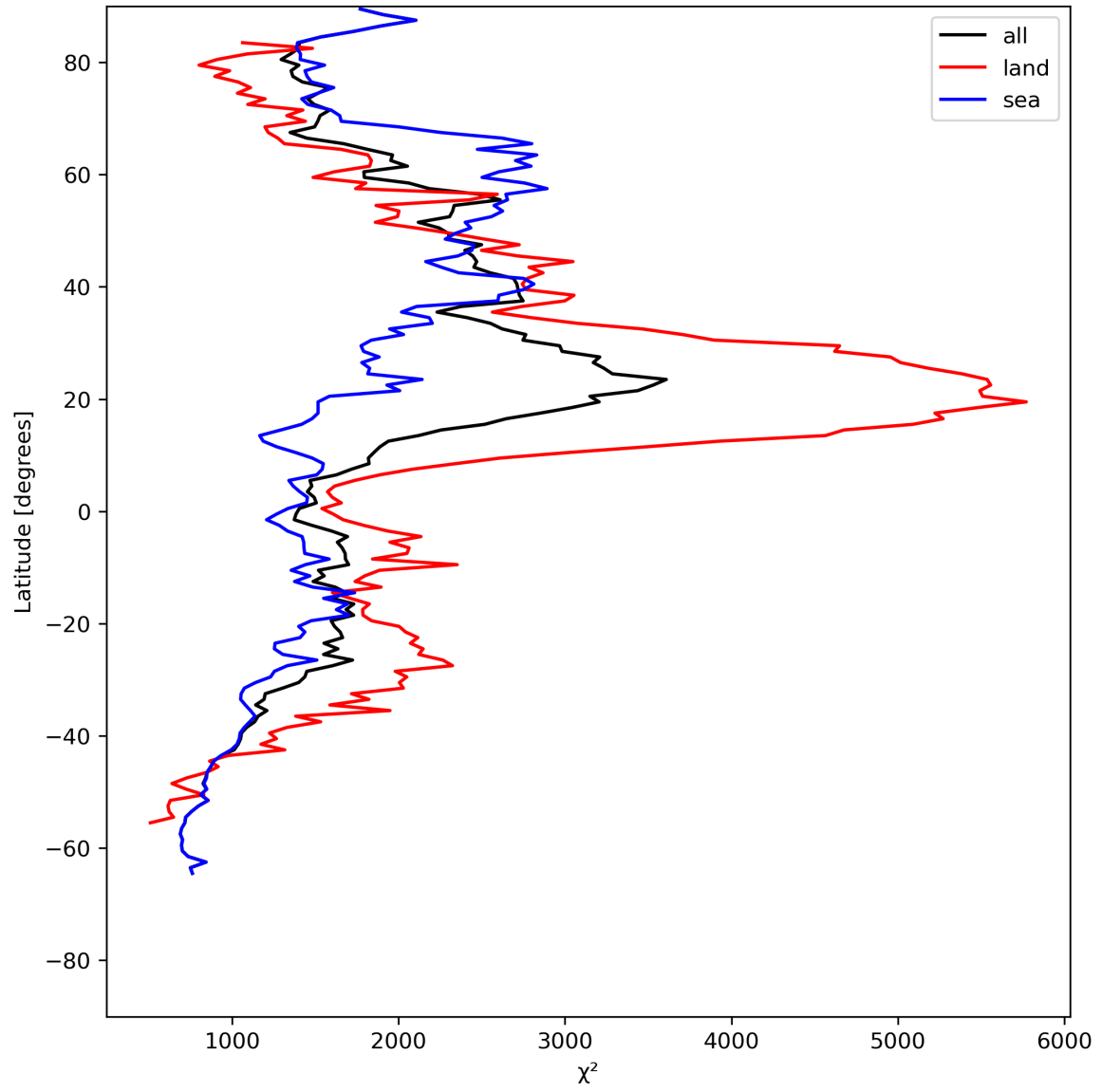
Figure 14: Zonal average of “ \chi^2 ” for 2024-05-20 to 2024-05-22.
