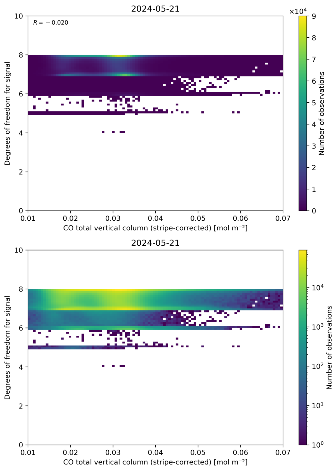
Figure 38: Scatter density plot of “CO total vertical column (stripe-corrected)” against “Degrees of freedom for signal” for 2024-05-20 to 2024-05-22.
