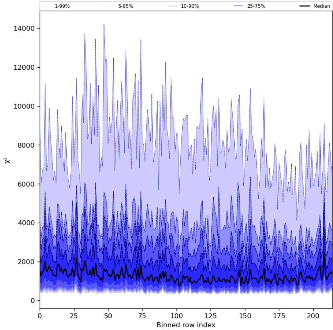
Figure 30: Along track statistics of “ \chi^2 ” for 2024-05-20 to 2024-05-22
