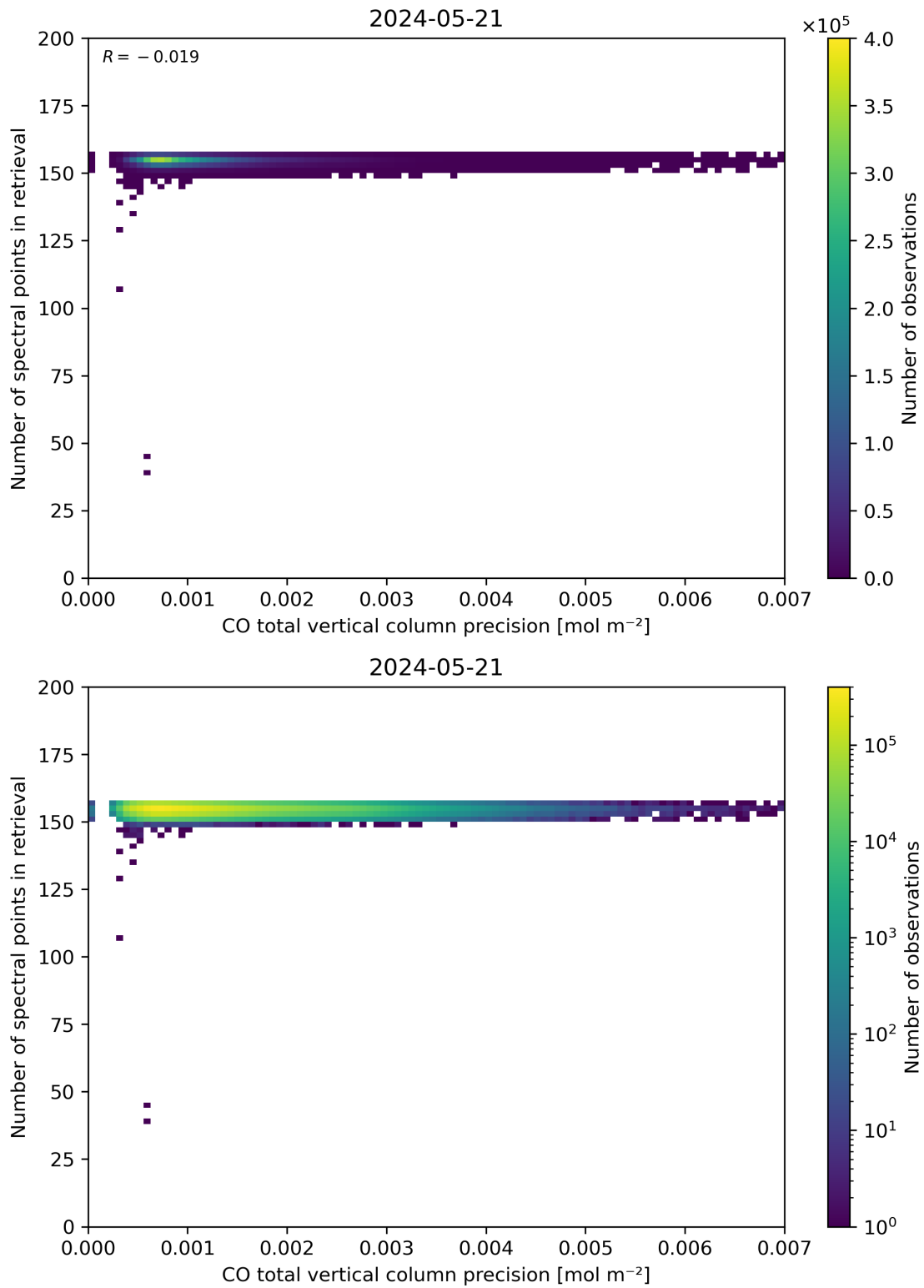
Figure 47: Scatter density plot of “CO total vertical column precision” against “Number of spectral points in retrieval” for 2024-05-20 to 2024-05-22.
