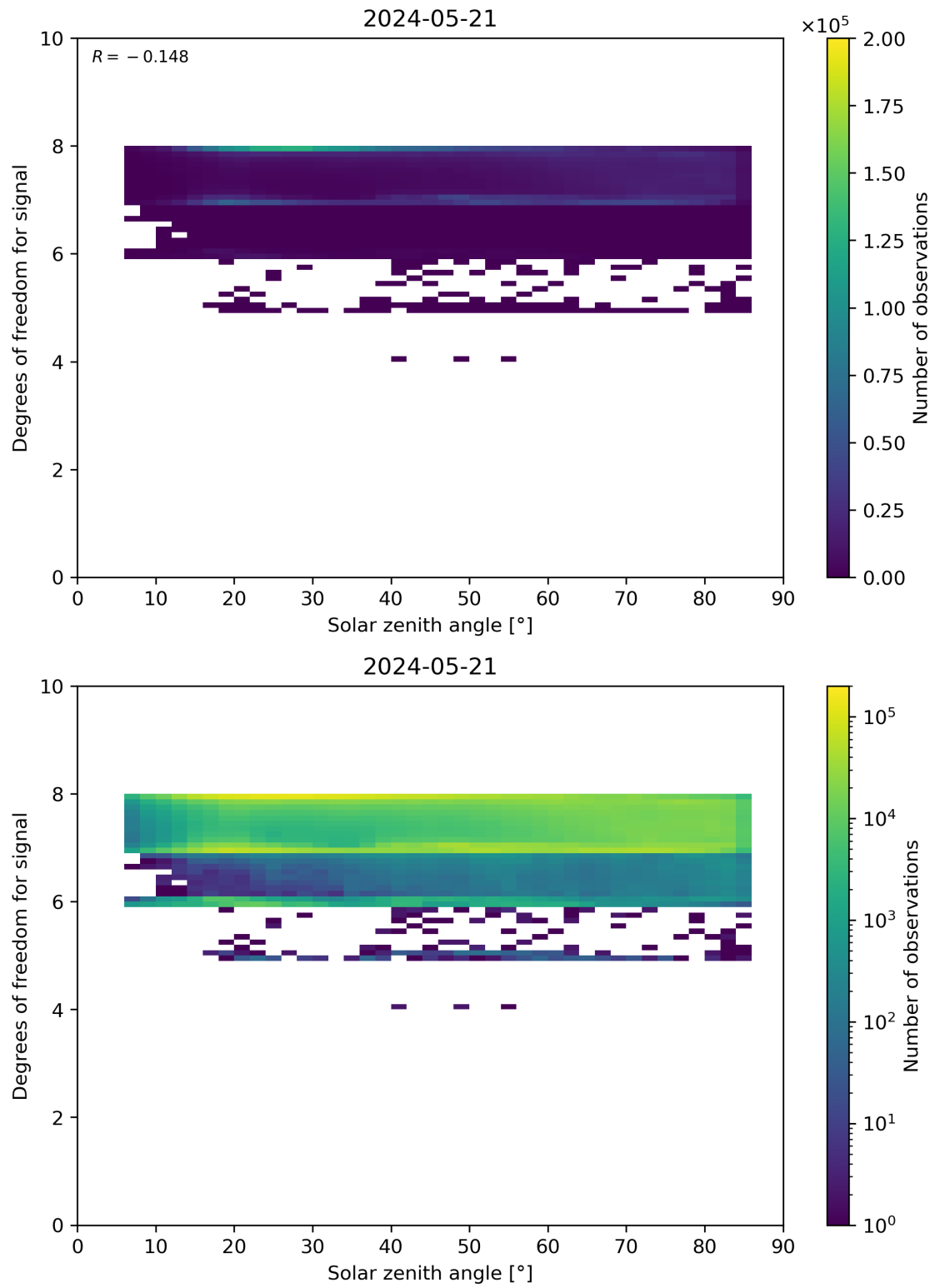
Figure 65: Scatter density plot of “Solar zenith angle” against “Degrees of freedom for signal” for 2024-05-20 to 2024-05-22.
