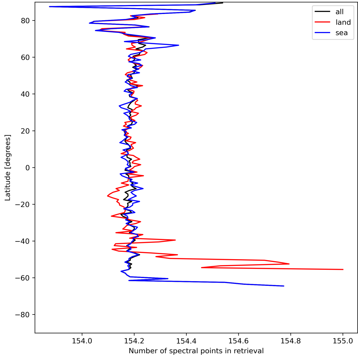
Figure 13: Zonal average of “Number of spectral points in retrieval” for 2024-05-20 to 2024-05-22.
