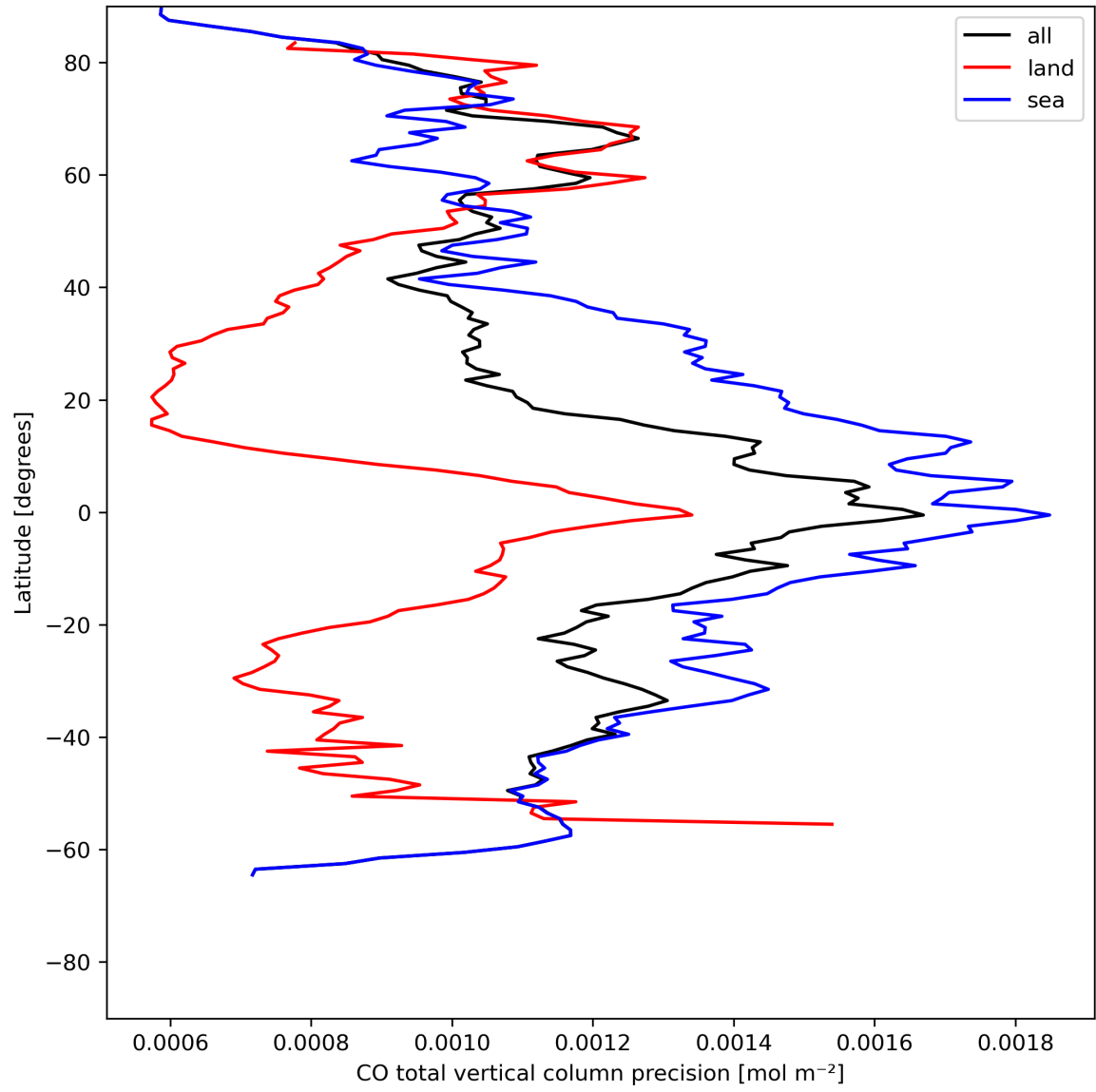
Figure 12: Zonal average of “CO total vertical column precision” for 2024-05-20 to 2024-05-22.
