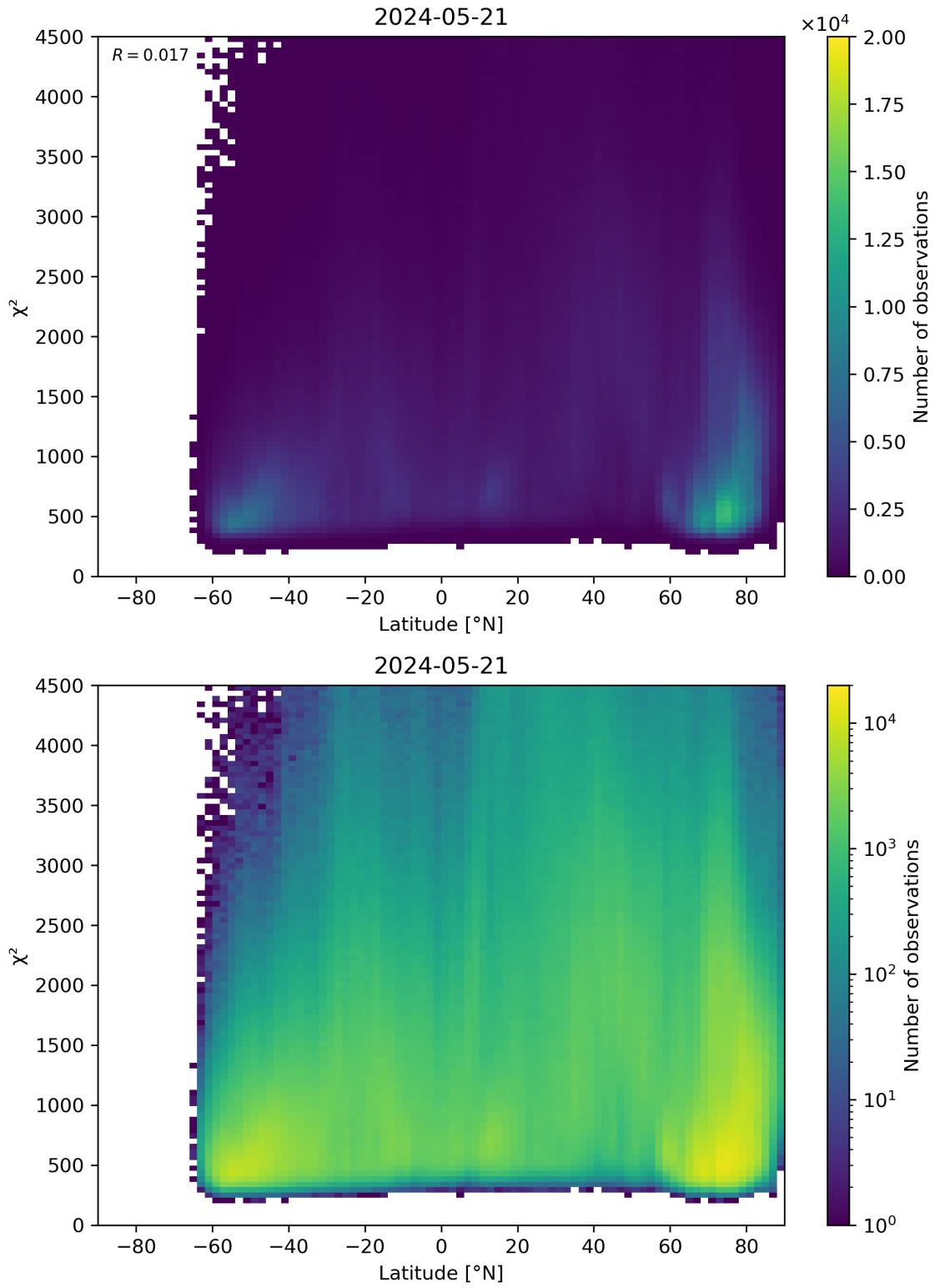
Figure 54: Scatter density plot of “Latitude” against “ \chi^2 ” for 2024-05-20 to 2024-05-22.
