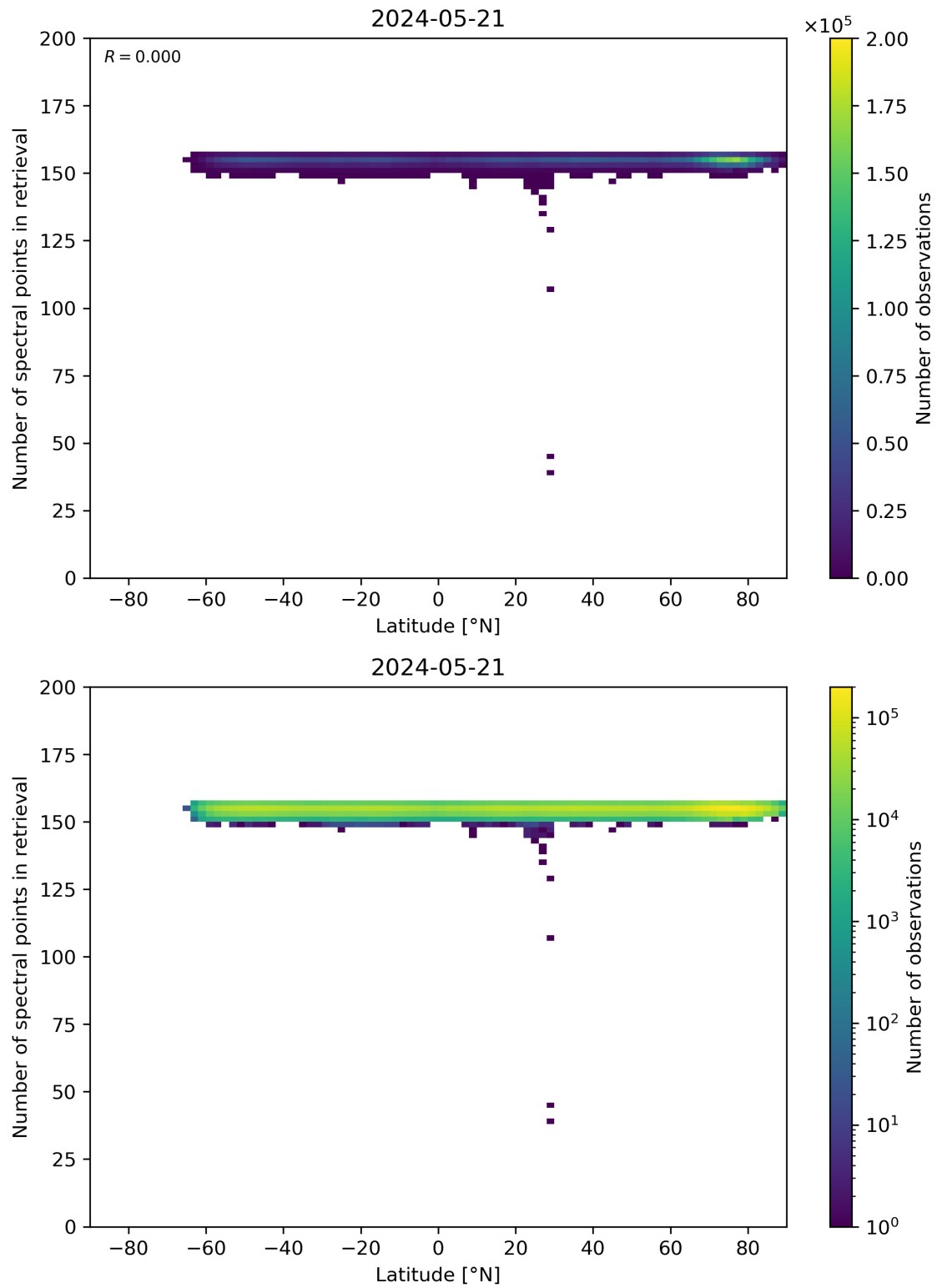
Figure 57: Scatter density plot of “Latitude” against “Number of spectral points in retrieval” for 2024-05-20 to 2024-05-22.
