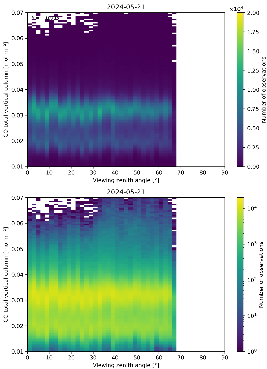
Figure 69: Scatter density plot of “Viewing zenith angle” against “CO total vertical column” for 2024-05-20 to 2024-05-22.
