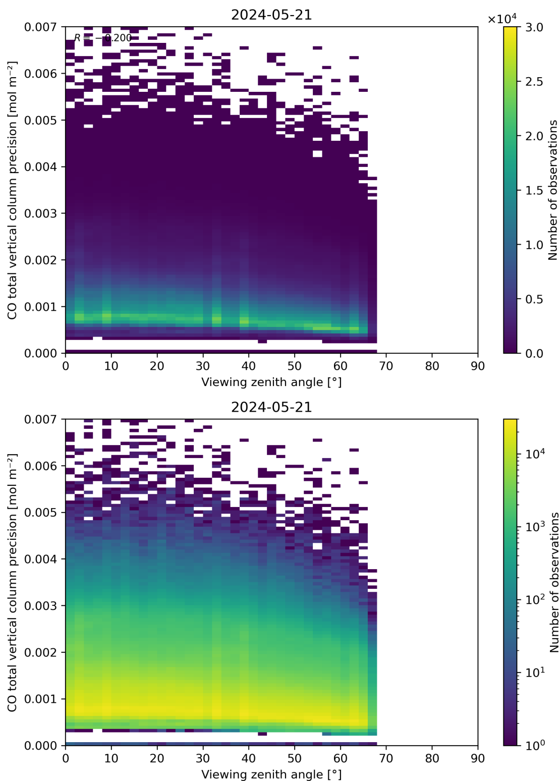
Figure 71: Scatter density plot of “Viewing zenith angle” against “CO total vertical column precision” for 2024-05-20 to 2024-05-22.
