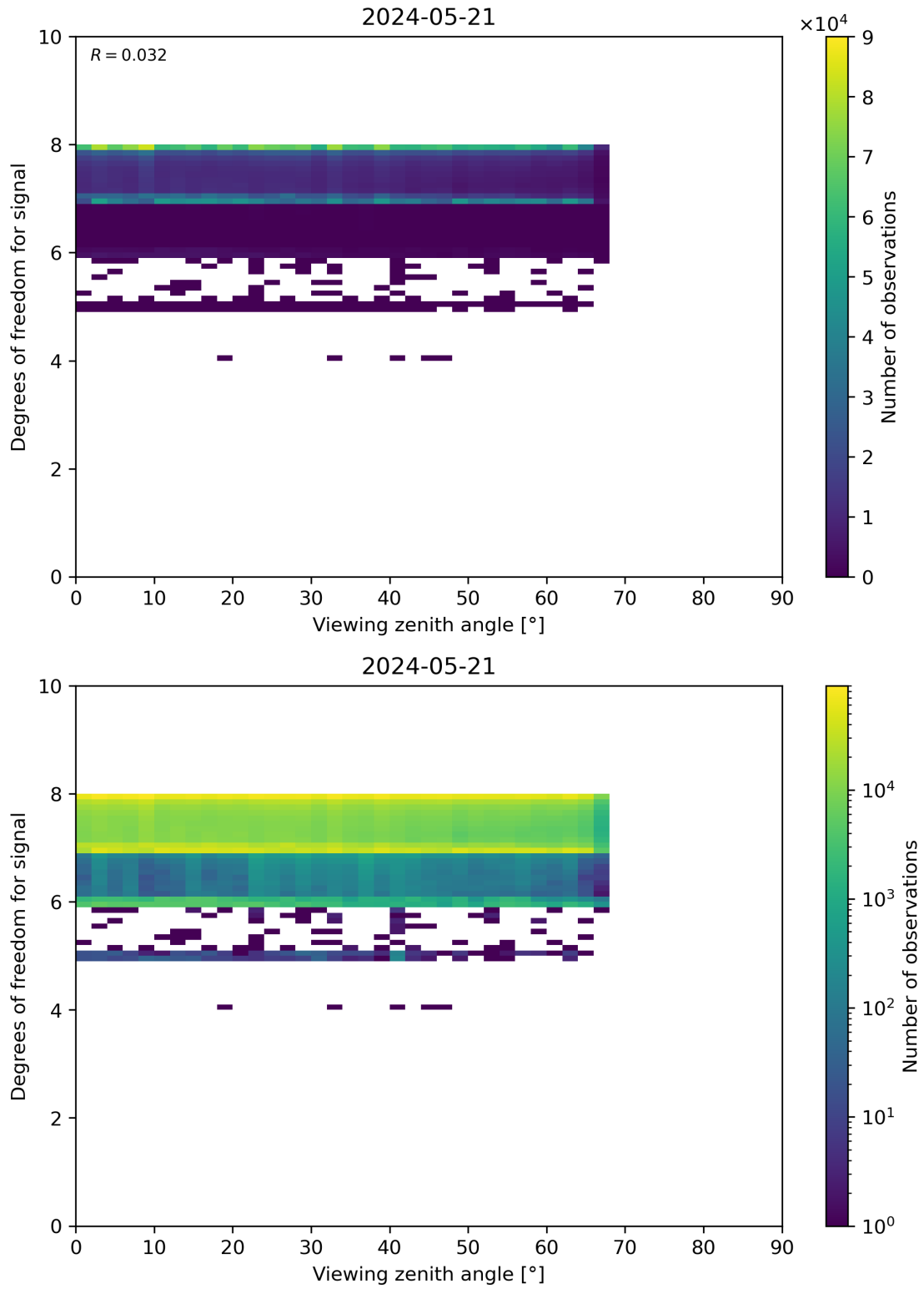
Figure 73: Scatter density plot of “Viewing zenith angle” against “Degrees of freedom for signal” for 2024-05-20 to 2024-05-22.
