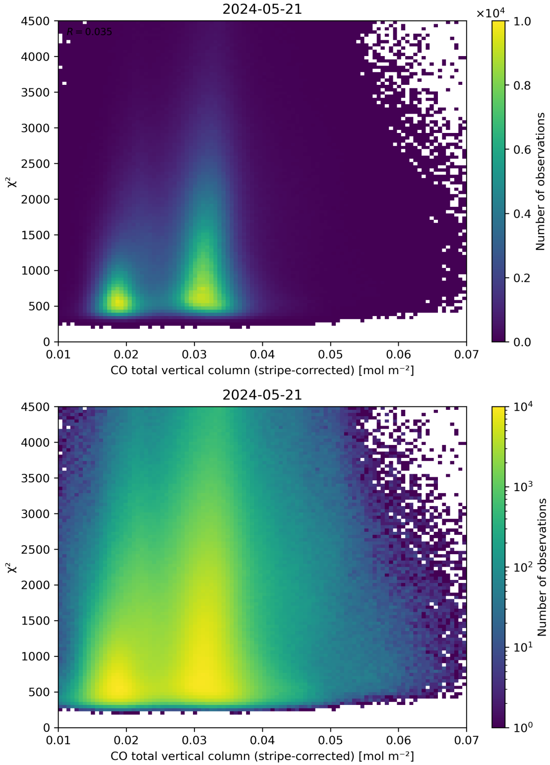
Figure 37: Scatter density plot of “CO total vertical column (stripe-corrected)” against “ \chi^2 ” for 2024-05-20 to 2024-05-22.
