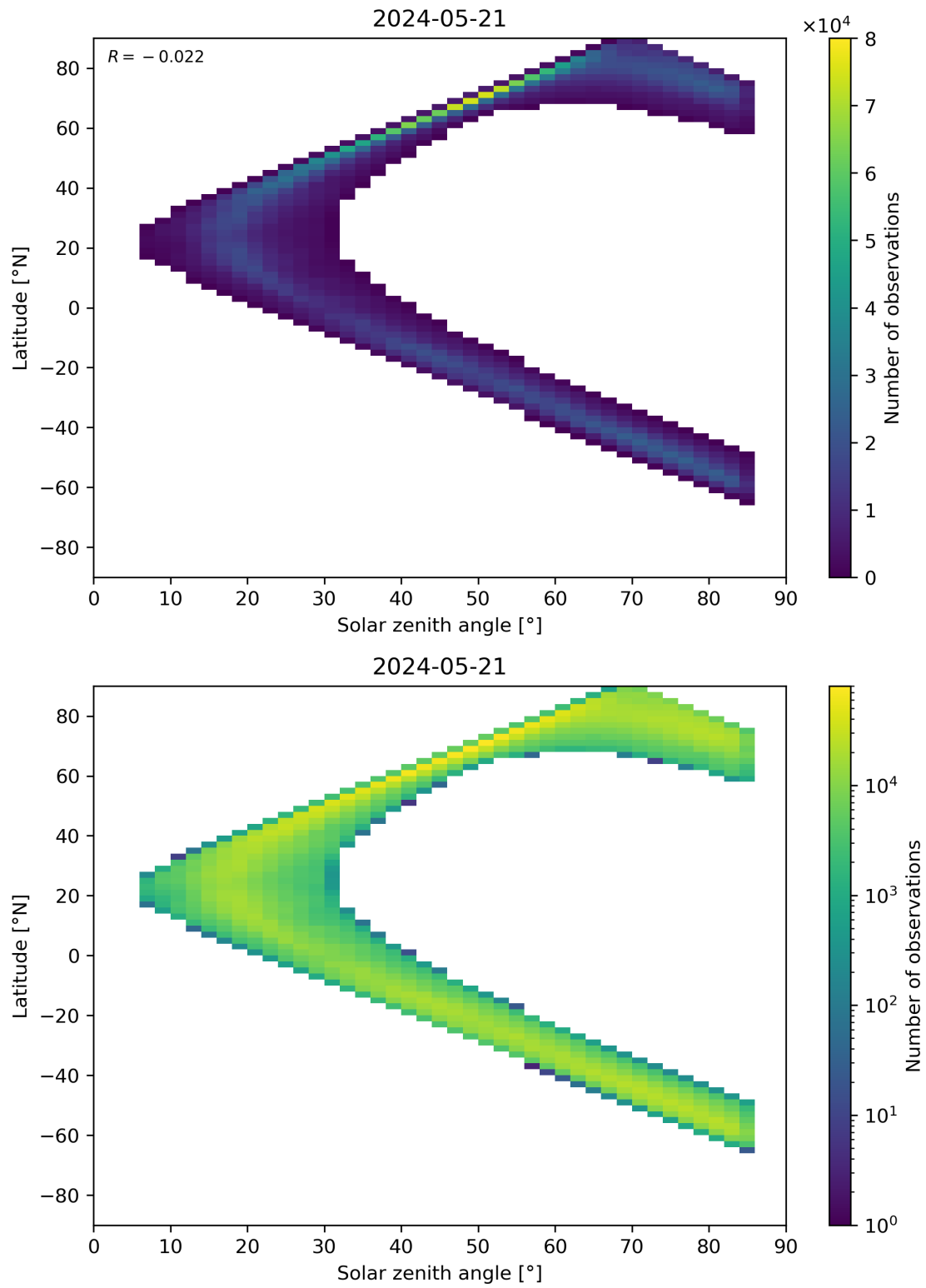
Figure 66: Scatter density plot of “Solar zenith angle” against “Latitude” for 2024-05-20 to 2024-05-22.
