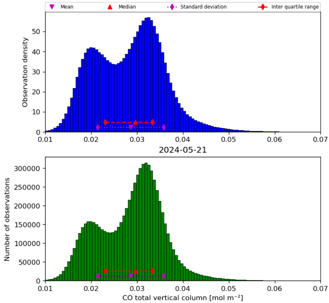
Figure 18: Histogram of “CO total vertical column” for 2024-05-20 to 2024-05-22
