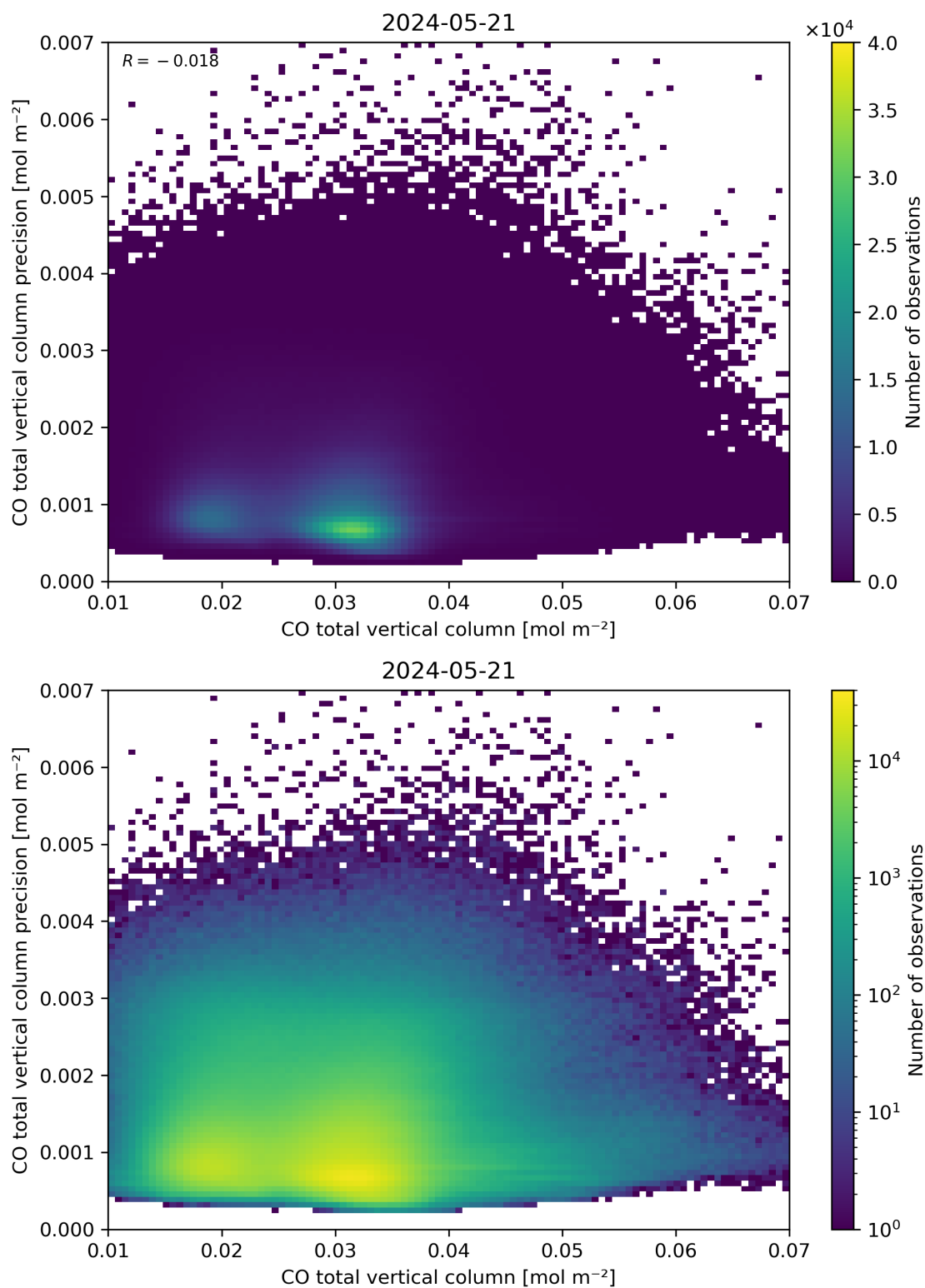
Figure 34: Scatter density plot of “CO total vertical column” against “CO total vertical column precision” for 2024-05-20 to 2024-05-22.
