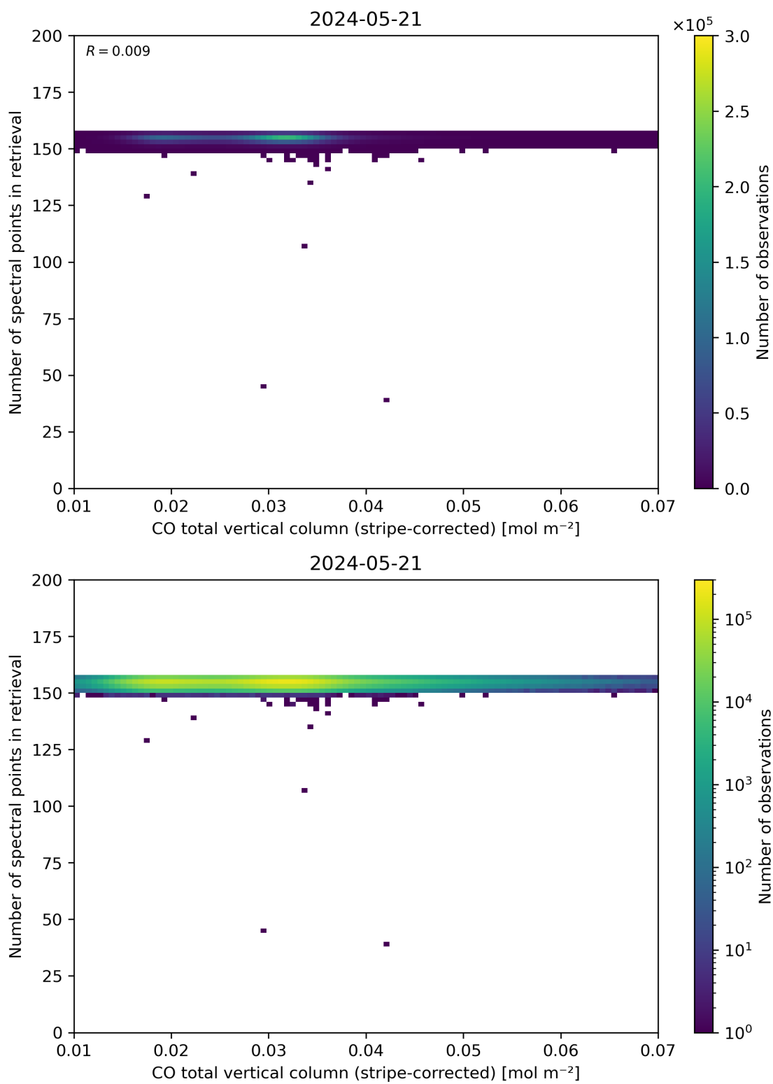
Figure 40: Scatter density plot of “CO total vertical column (stripe-corrected)” against “Number of spectral points in retrieval” for 2024-05-20 to 2024-05-22.
