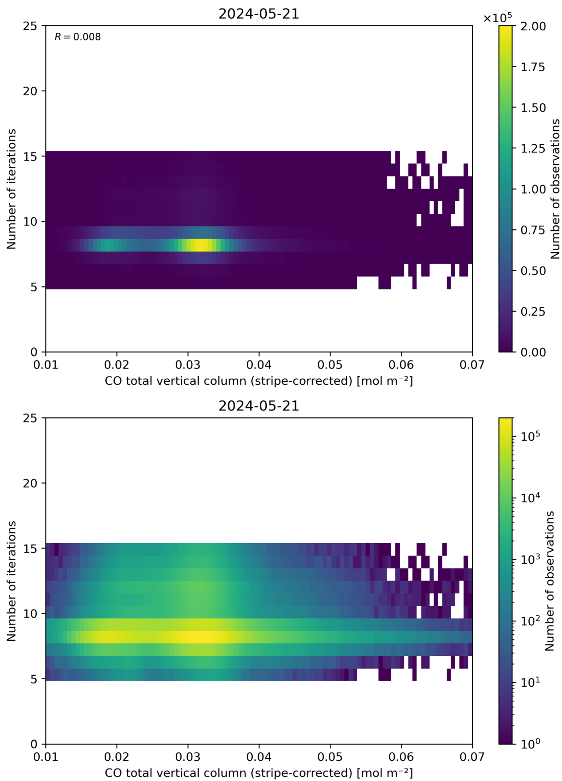
Figure 39: Scatter density plot of “CO total vertical column (stripe-corrected)” against “Number of iterations” for 2024-05-20 to 2024-05-22.
