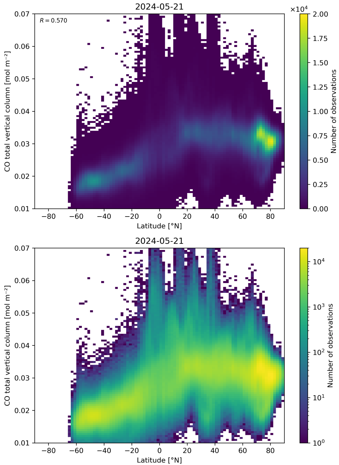
Figure 51: Scatter density plot of “Latitude” against “CO total vertical column” for 2024-05-20 to 2024-05-22.
