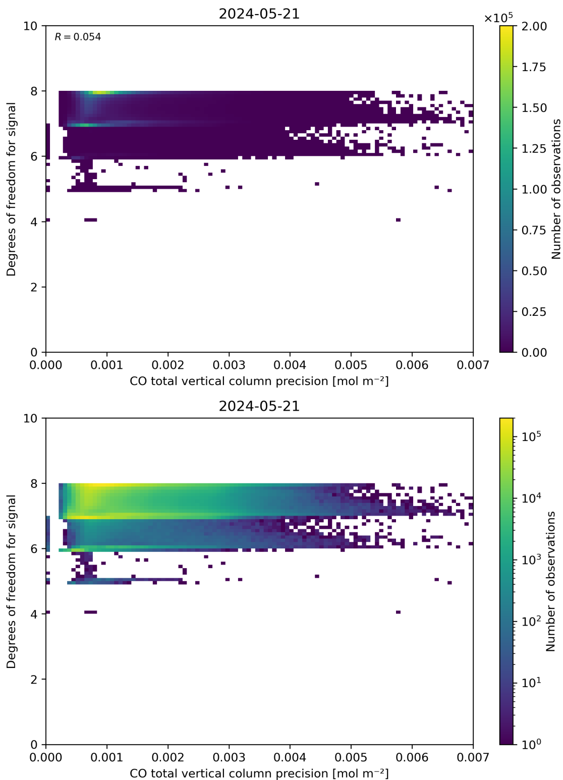
Figure 45: Scatter density plot of “CO total vertical column precision” against “Degrees of freedom for signal” for 2024-05-20 to 2024-05-22.
