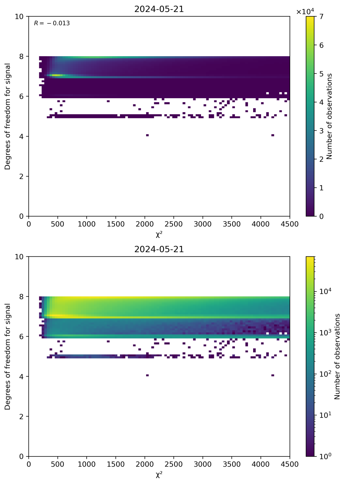
Figure 48: Scatter density plot of “ \chi^2 ” against “Degrees of freedom for signal” for 2024-05-20 to 2024-05-22.
