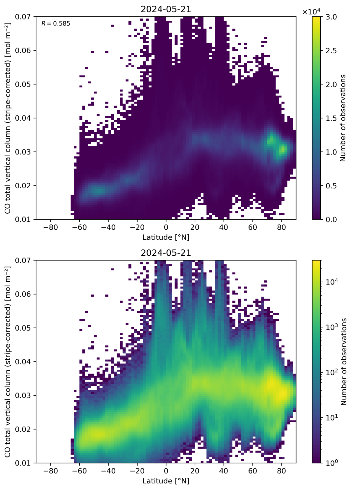
Figure 52: Scatter density plot of “Latitude” against “CO total vertical column (stripe-corrected)” for 2024-05-20 to 2024-05-22.
