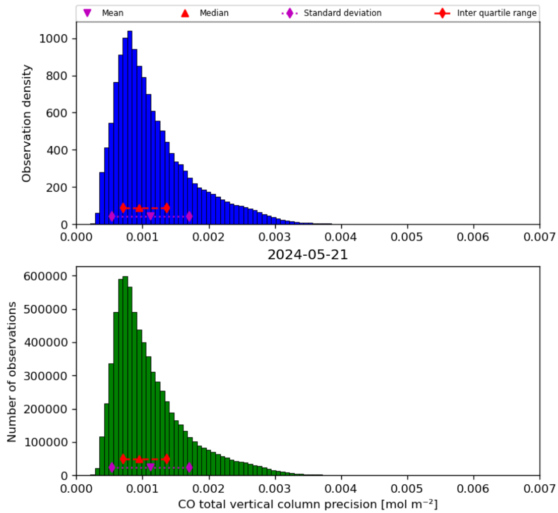
Figure 20: Histogram of “CO total vertical column precision” for 2024-05-20 to 2024-05-22
