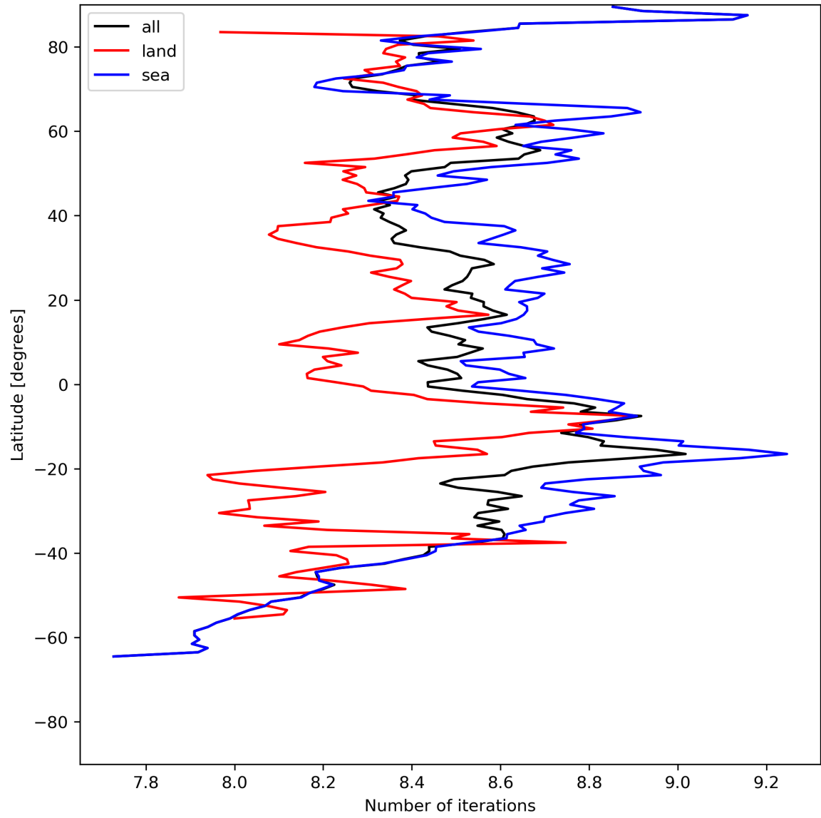
Figure 16: Zonal average of “Number of iterations” for 2024-05-20 to 2024-05-22.
