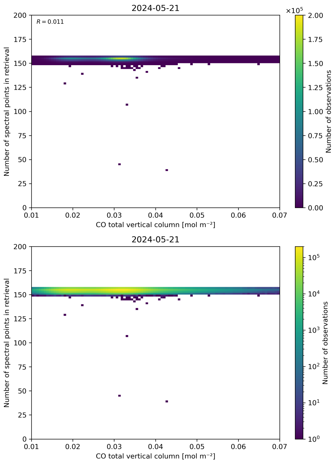
Figure 43: Scatter density plot of “CO total vertical column” against “Number of spectral points in retrieval” for 2024-05-20 to 2024-05-22.
