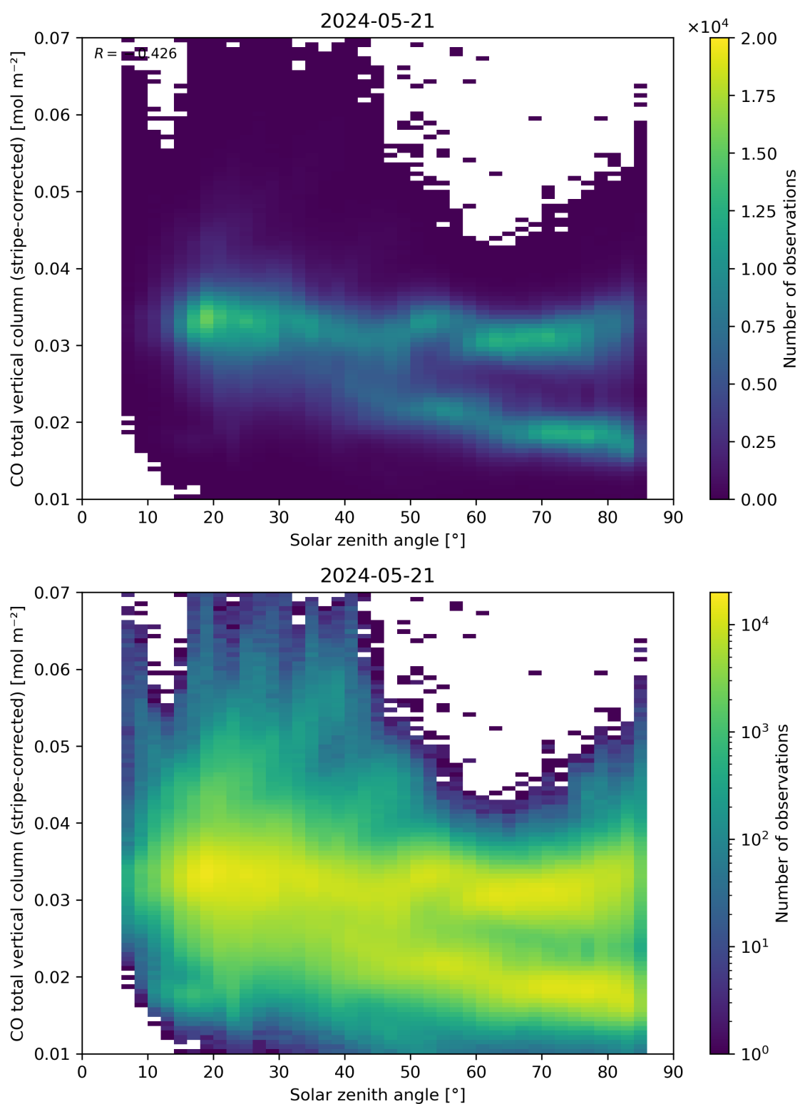
Figure 62: Scatter density plot of “Solar zenith angle” against “CO total vertical column (stripe-corrected)” for 2024-05-20 to 2024-05-22.
