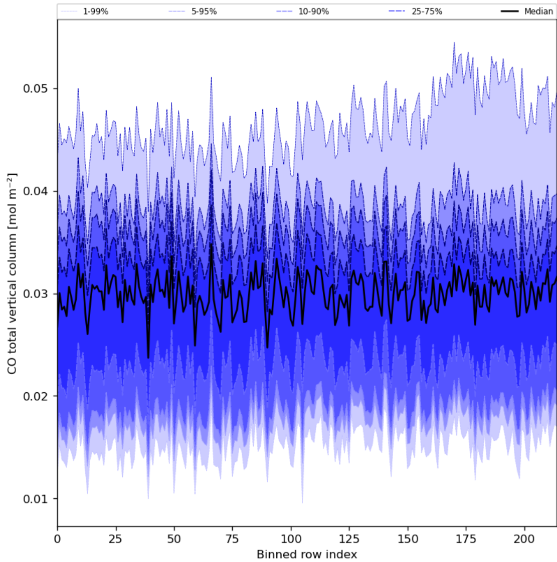
Figure 26: Along track statistics of “CO total vertical column” for 2024-05-20 to 2024-05-22
