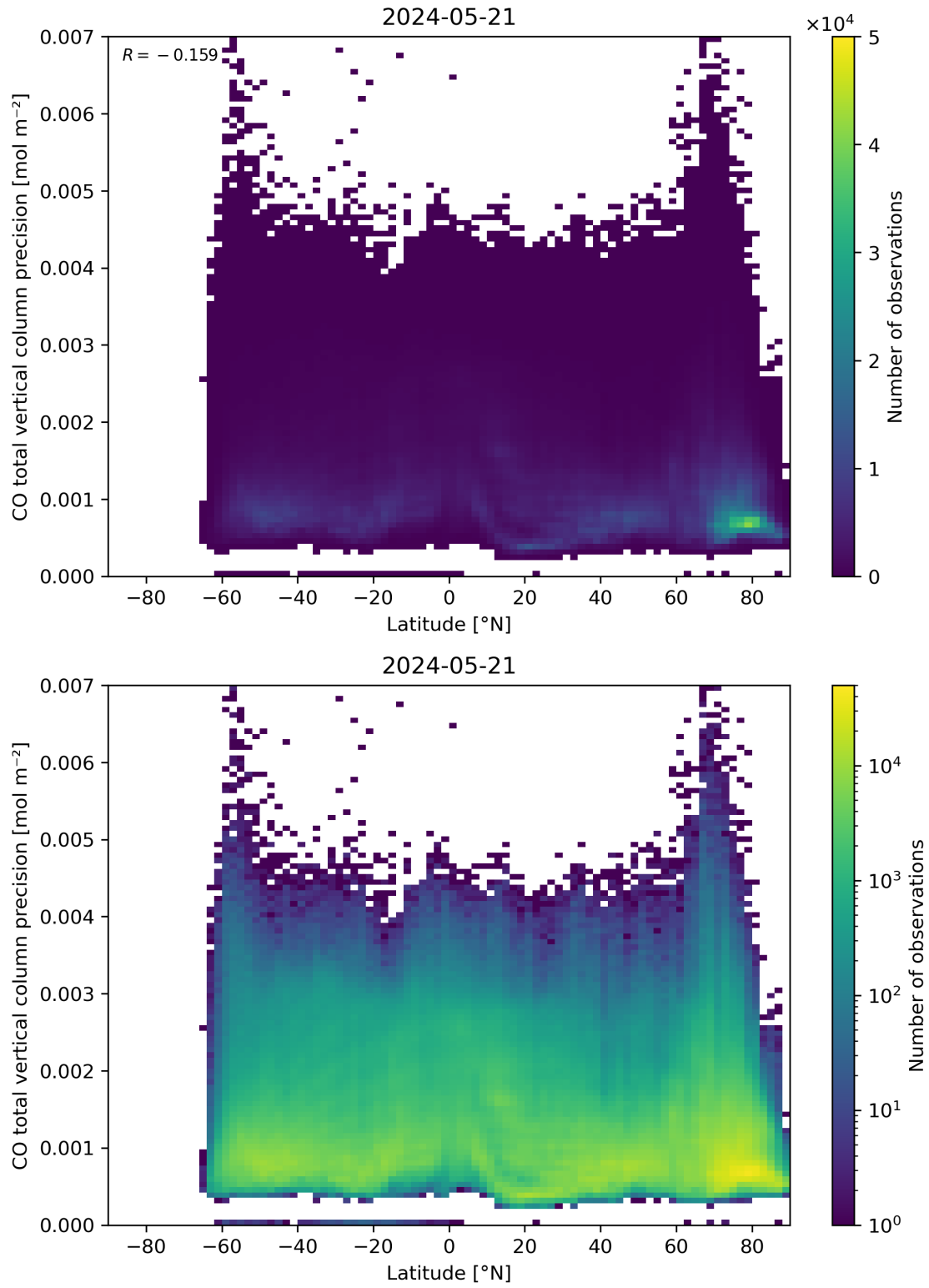
Figure 53: Scatter density plot of “Latitude” against “CO total vertical column precision” for 2024-05-20 to 2024-05-22.
