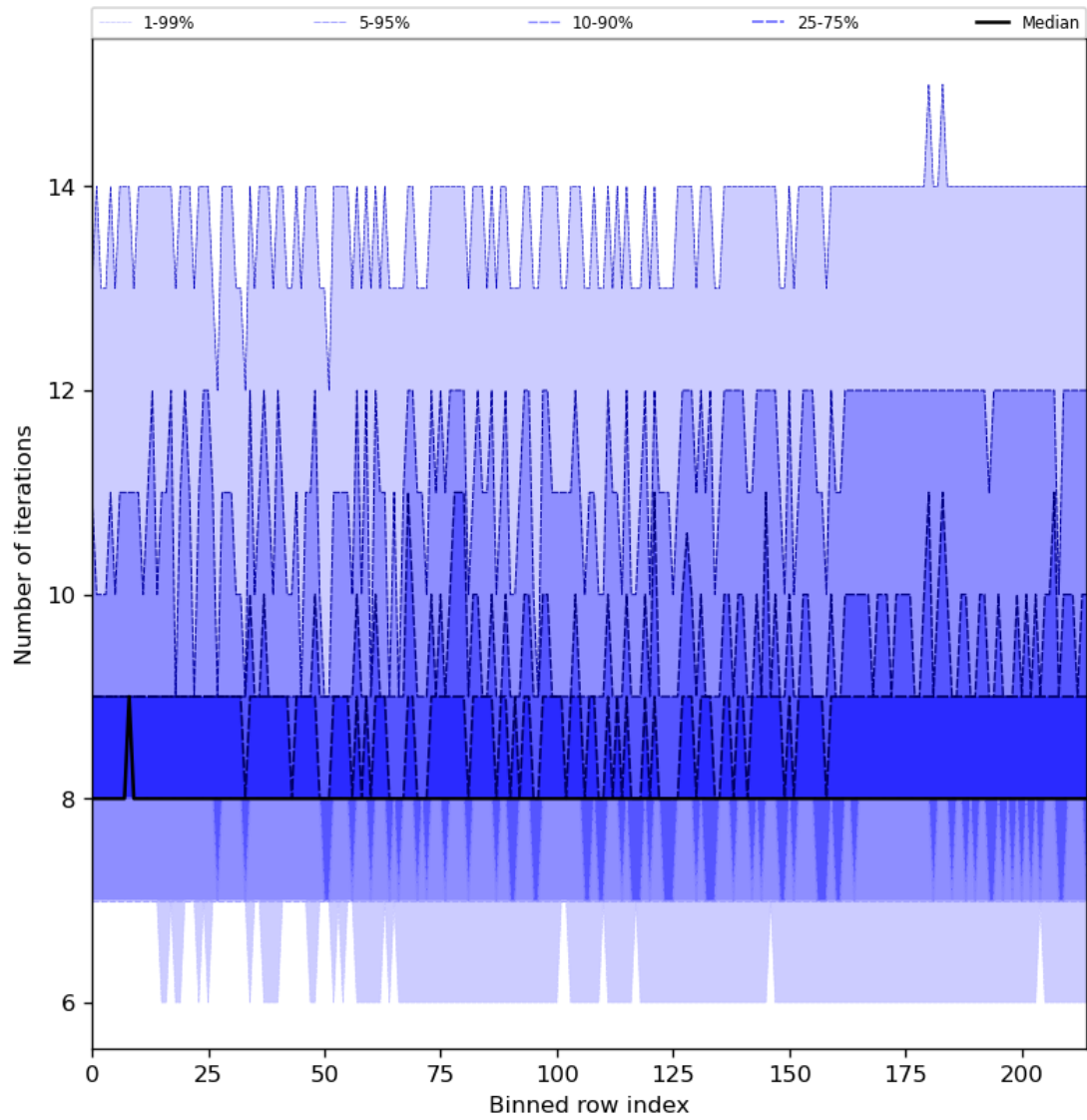
Figure 32: Along track statistics of “Number of iterations” for 2024-05-20 to 2024-05-22
