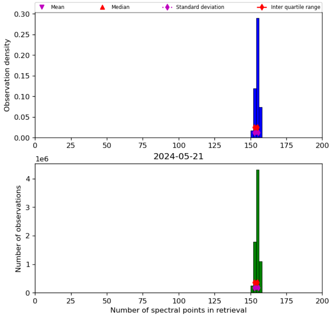
Figure 21: Histogram of “Number of spectral points in retrieval” for 2024-05-20 to 2024-05-22
