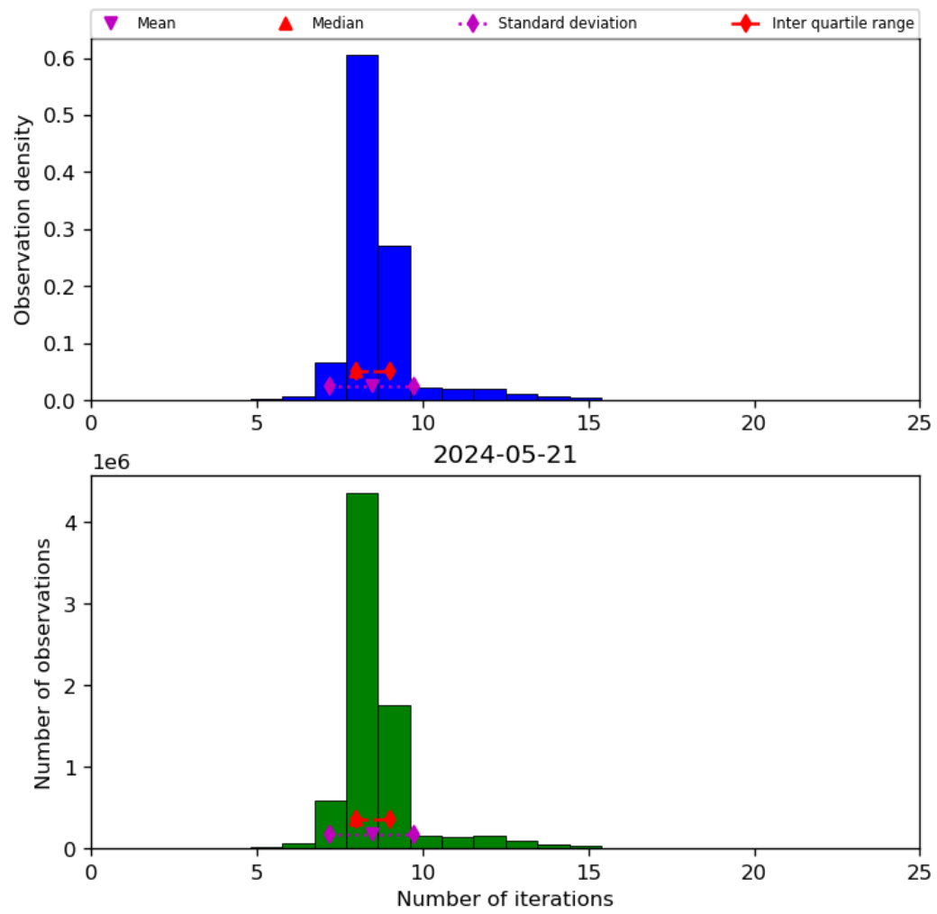
Figure 24: Histogram of “Number of iterations” for 2024-05-20 to 2024-05-22
