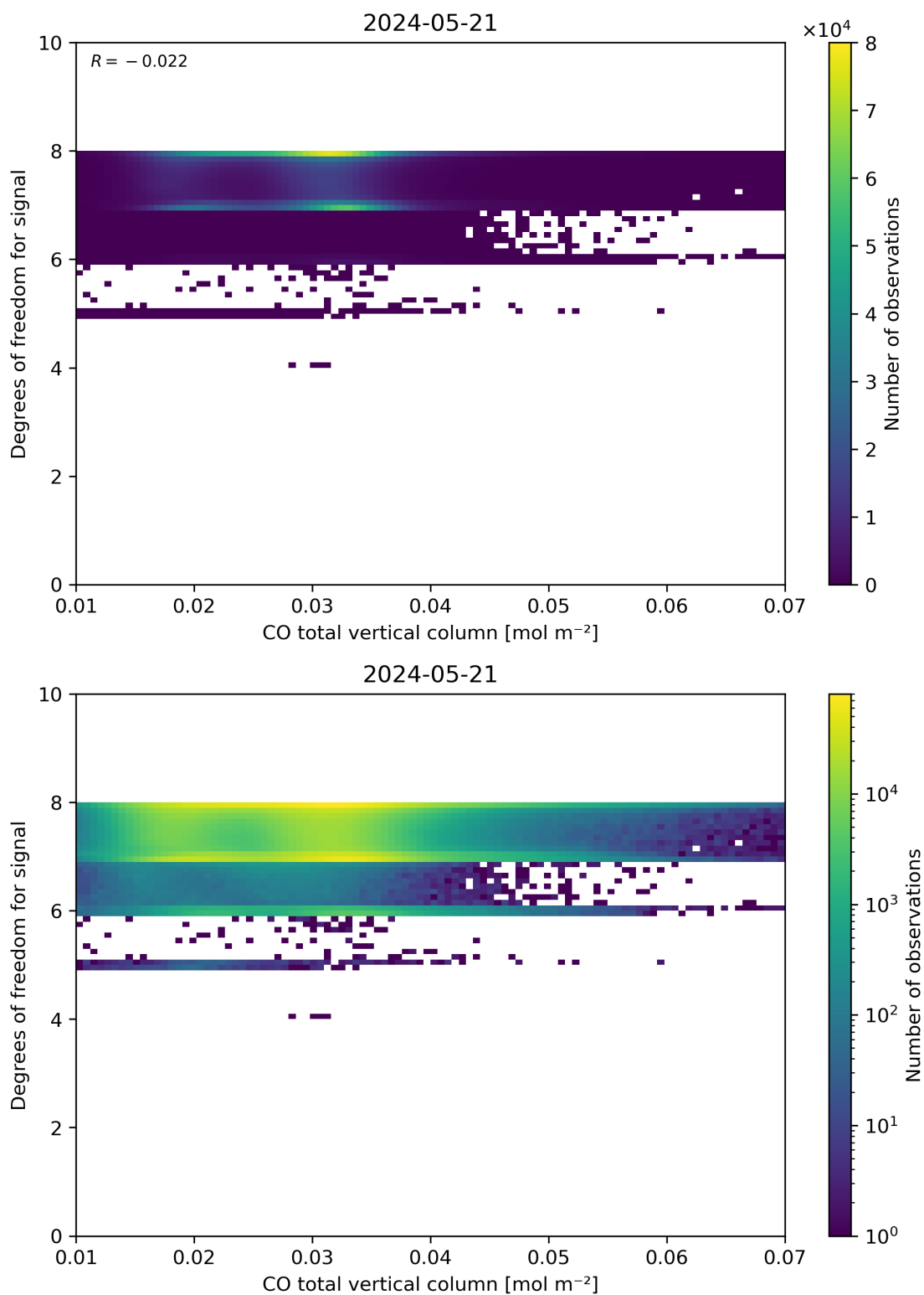
Figure 41: Scatter density plot of “CO total vertical column” against “Degrees of freedom for signal” for 2024-05-20 to 2024-05-22.
