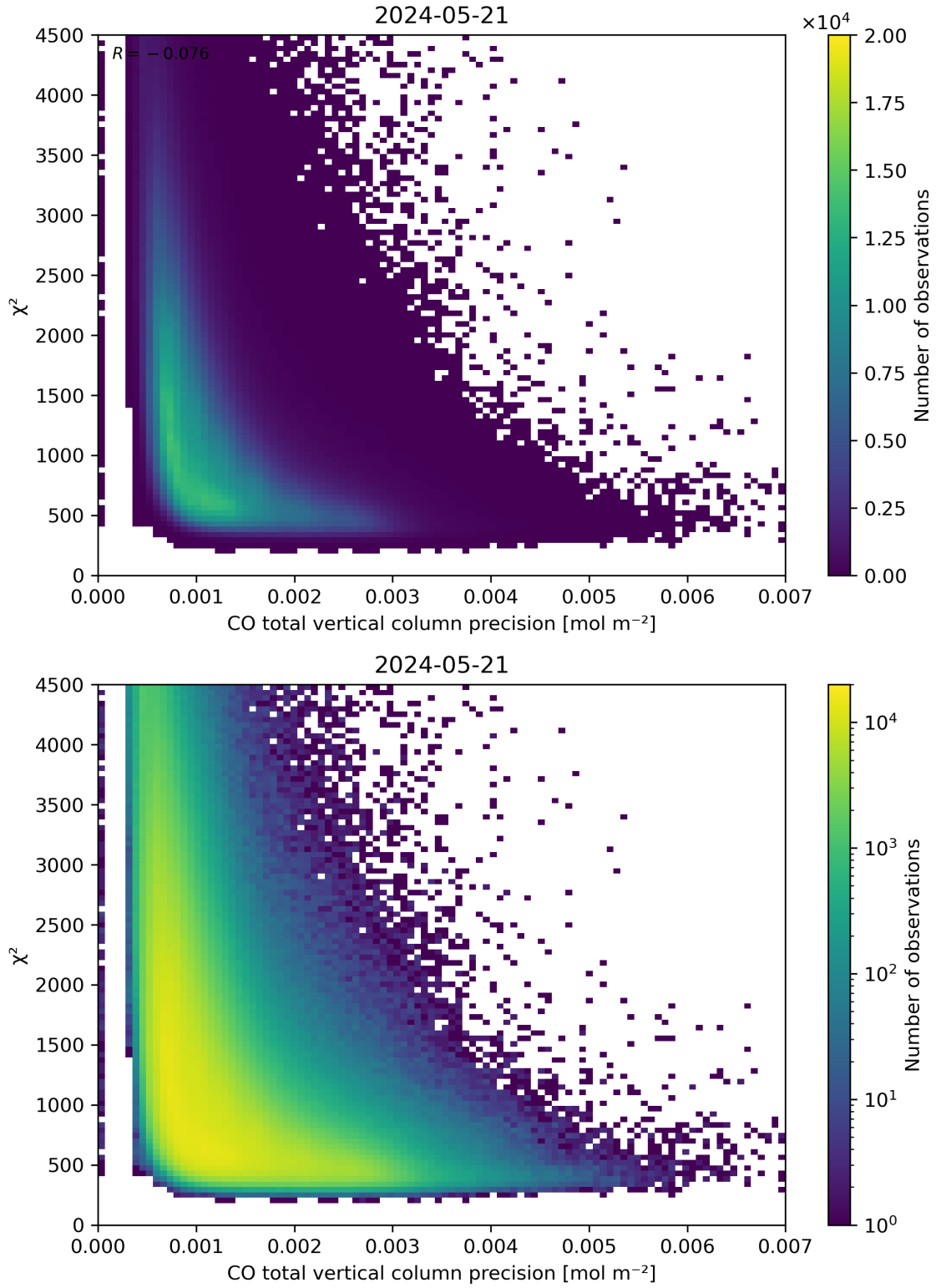
Figure 44: Scatter density plot of “CO total vertical column precision” against “ \chi^2 ” for 2024-05-20 to 2024-05-22.
