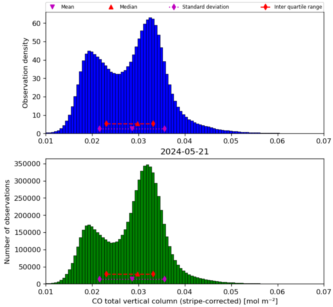
Figure 19: Histogram of “CO total vertical column (stripe-corrected)” for 2024-05-20 to 2024-05-22
