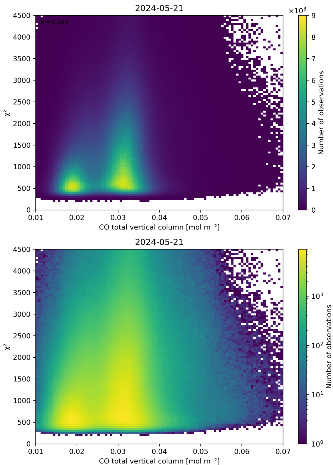
Figure 35: Scatter density plot of “CO total vertical column” against “ \chi^2 ” for 2024-05-20 to 2024-05-22.
