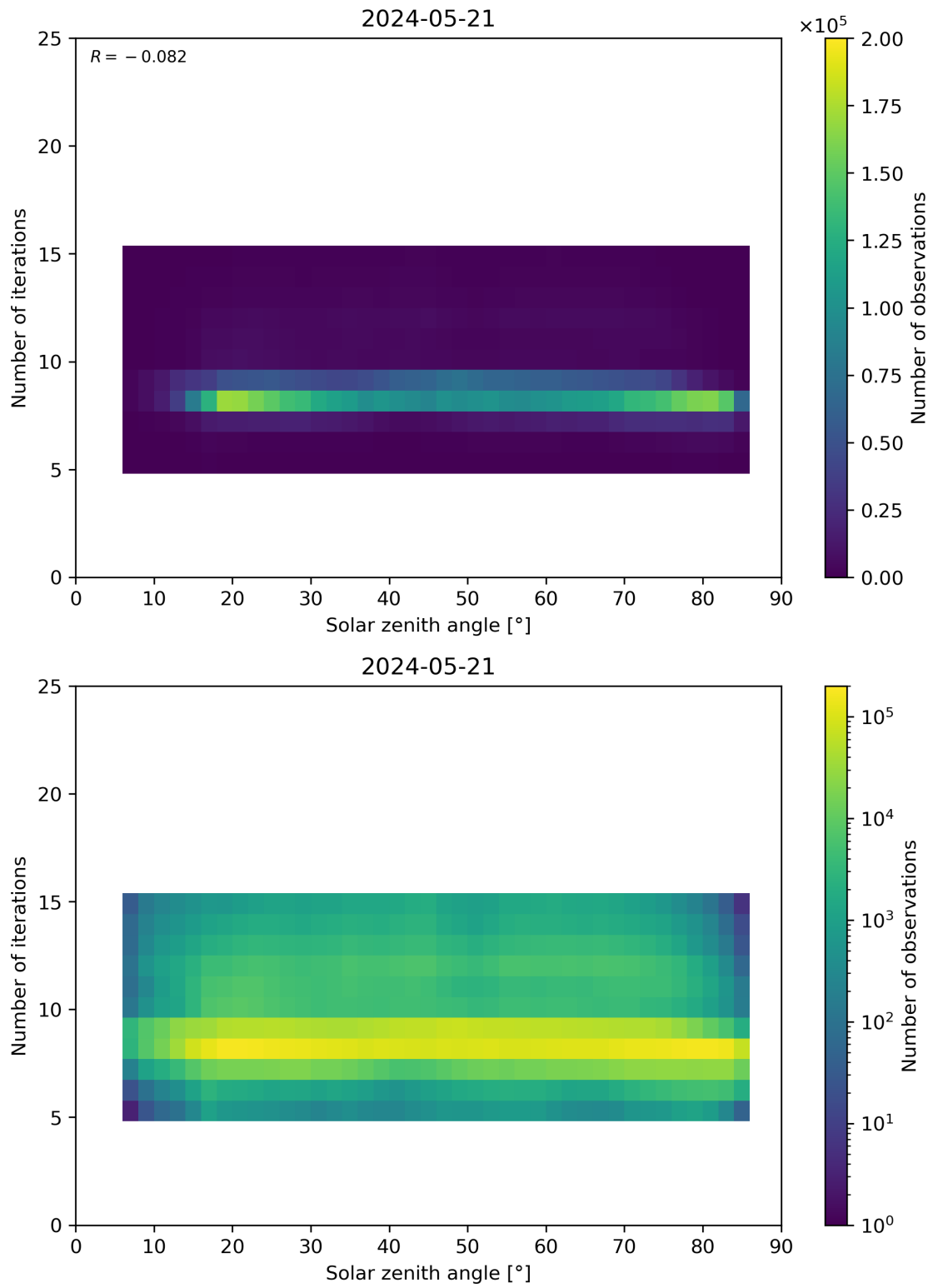
Figure 67: Scatter density plot of “Solar zenith angle” against “Number of iterations” for 2024-05-20 to 2024-05-22.
