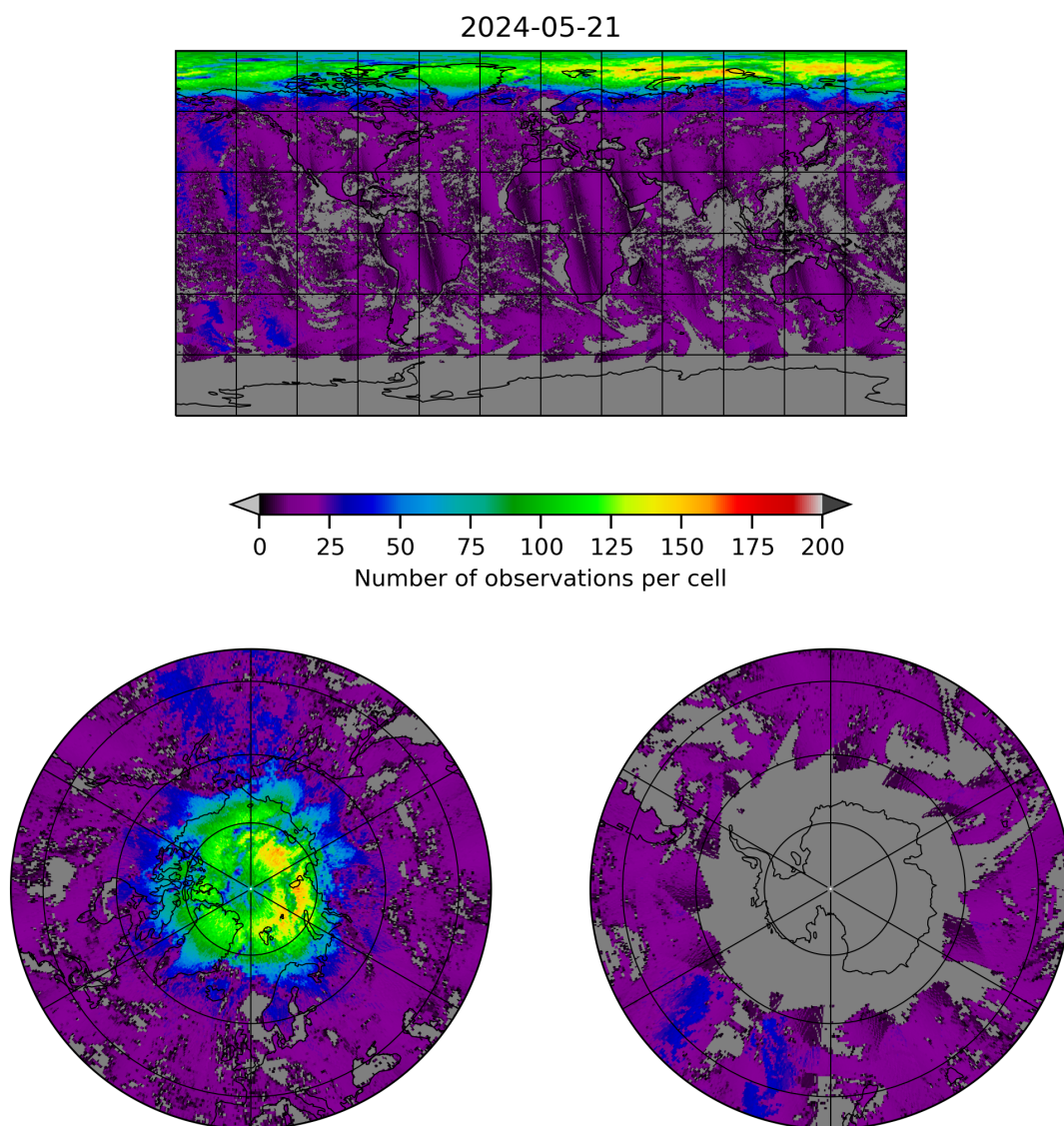
Figure 8: Map of the number of observations for 2024-05-20 to 2024-05-22
