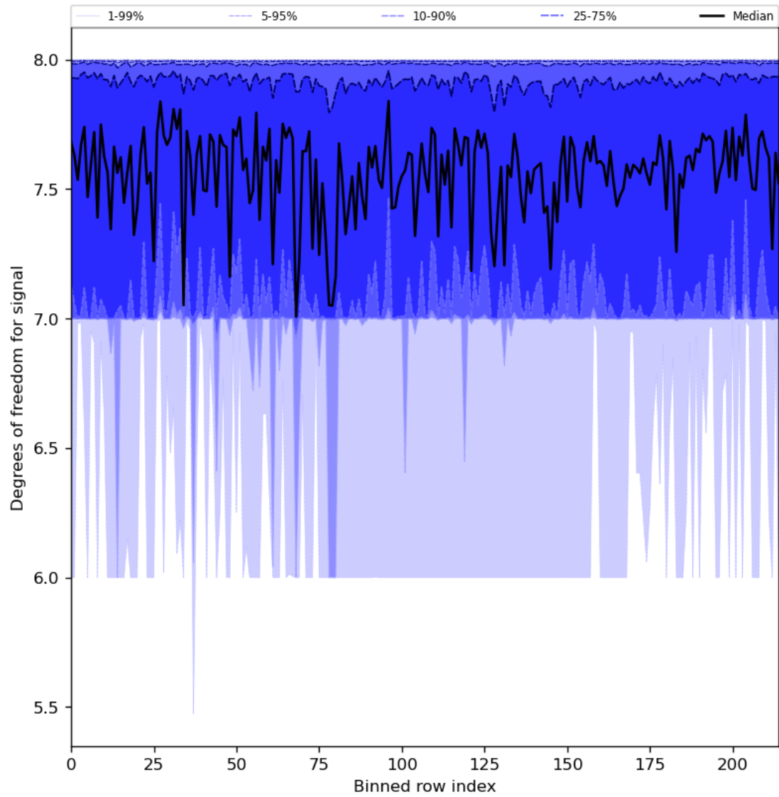
Figure 31: Along track statistics of “Degrees of freedom for signal” for 2024-05-20 to 2024-05-22
