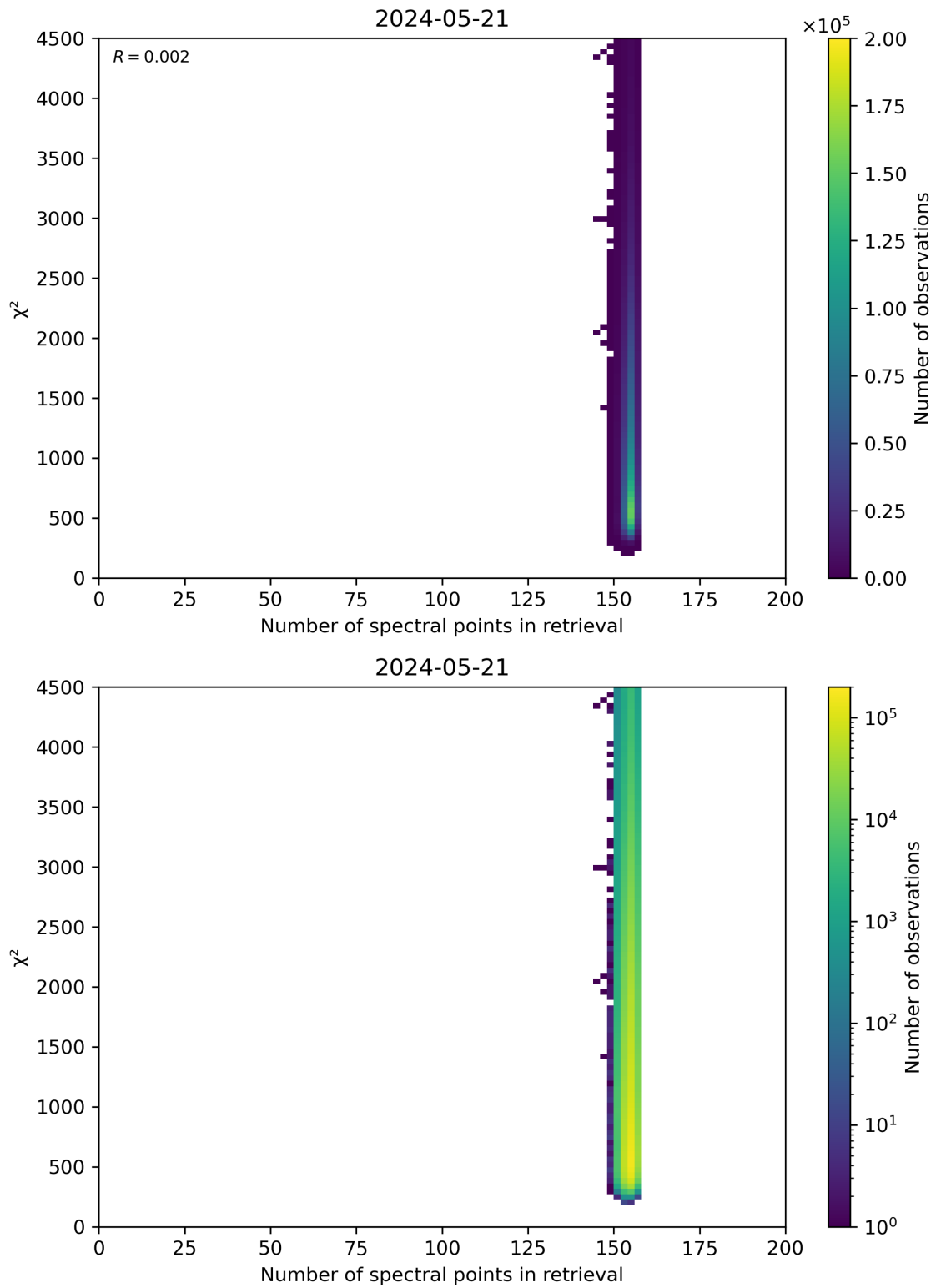
Figure 58: Scatter density plot of “Number of spectral points in retrieval” against “ \chi^2 ” for 2024-05-20 to 2024-05-22.
