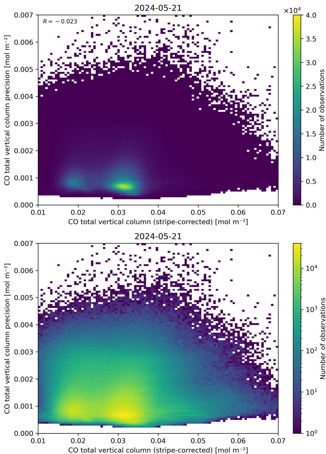
Figure 36: Scatter density plot of “CO total vertical column (stripe-corrected)” against “CO total vertical column precision” for 2024-05-20 to 2024-05-22.
