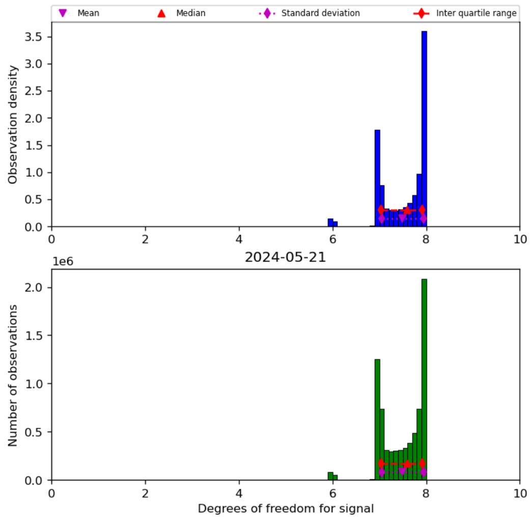
Figure 23: Histogram of “Degrees of freedom for signal” for 2024-05-20 to 2024-05-22
