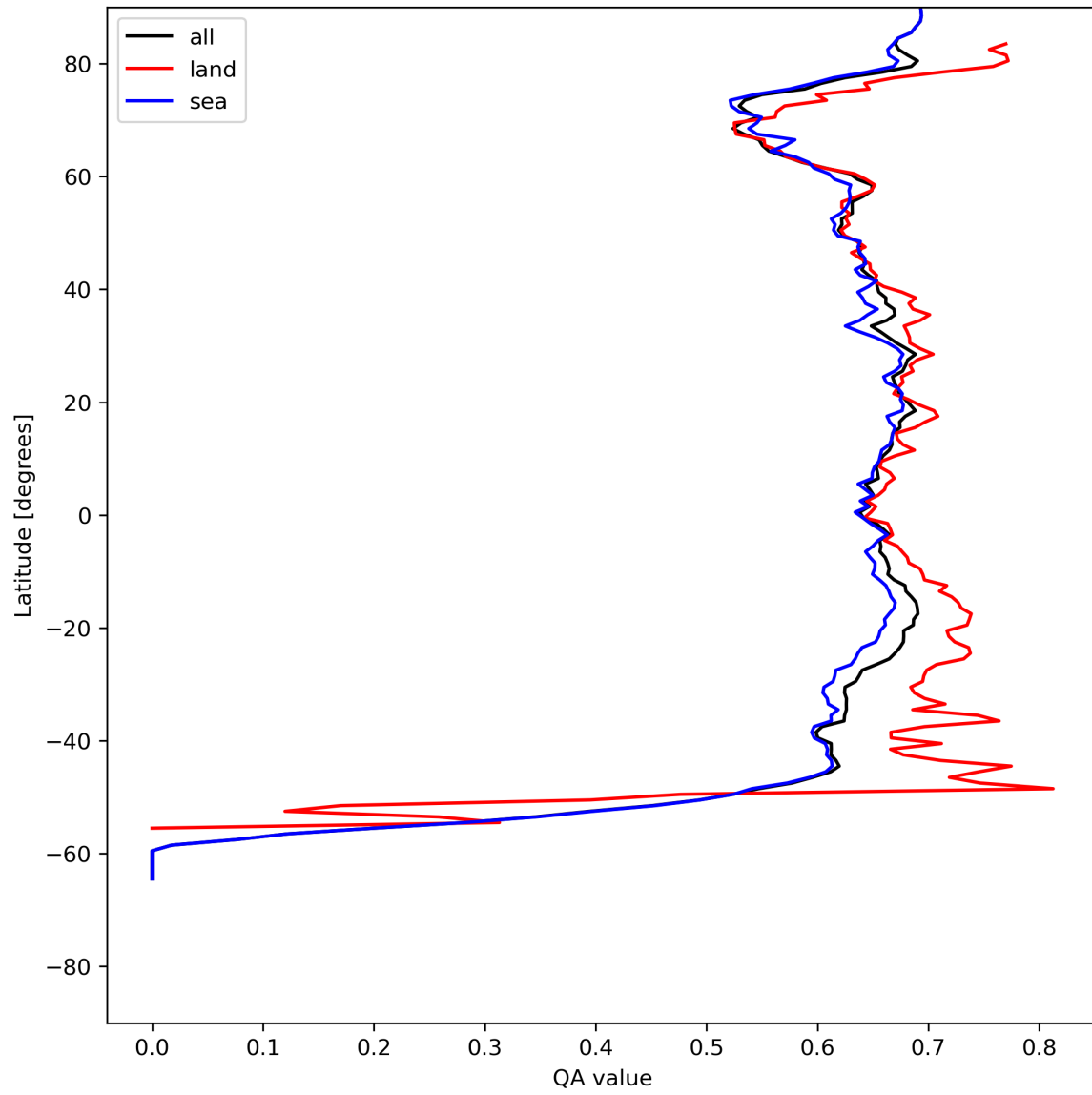
Figure 9: Zonal average of “QA value” for 2024-05-20 to 2024-05-22.
