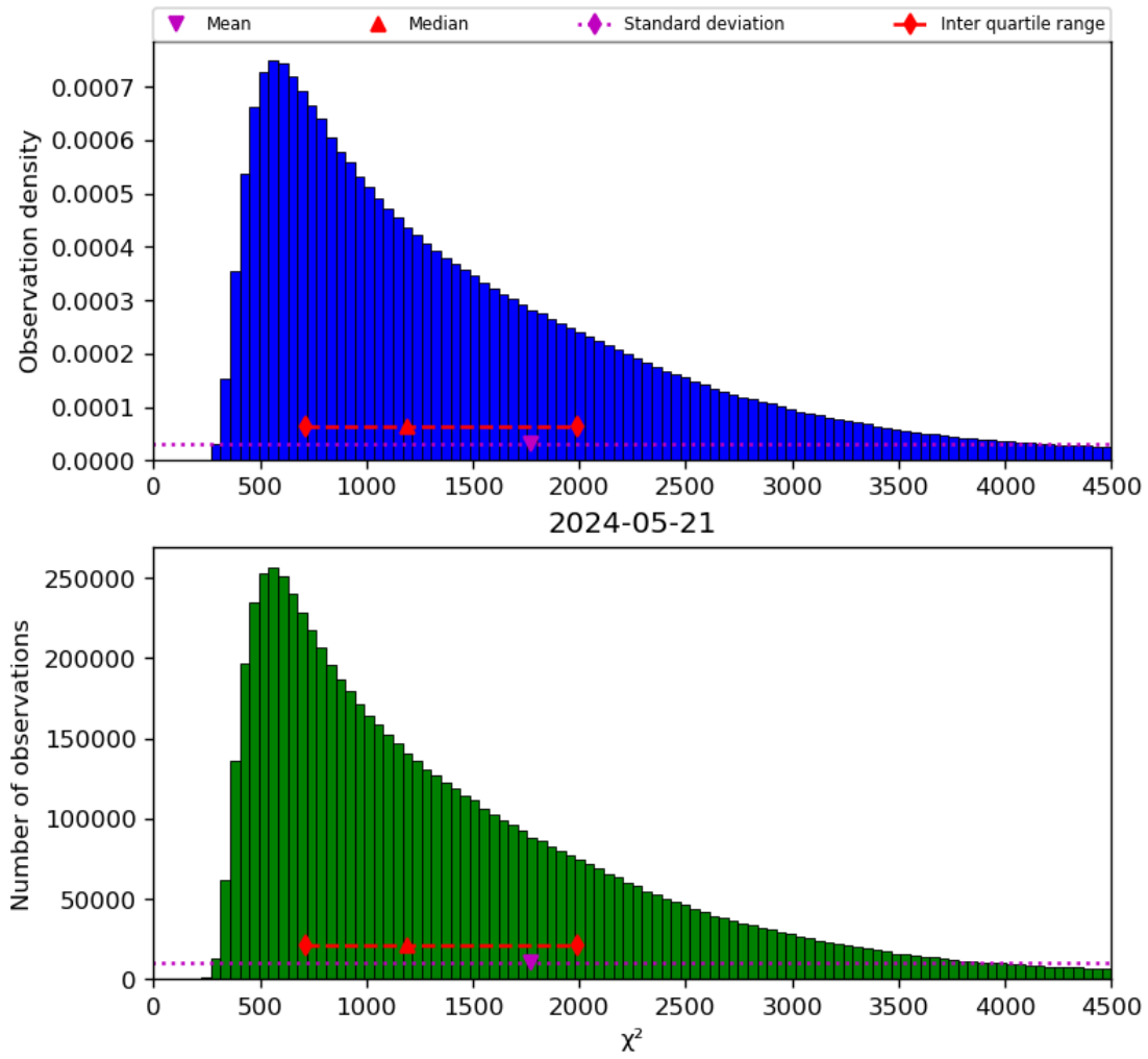
Figure 22: Histogram of “ \chi^2 ” for 2024-05-20 to 2024-05-22
