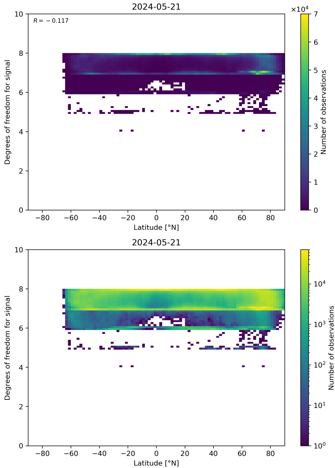
Figure 55: Scatter density plot of “Latitude” against “Degrees of freedom for signal” for 2024-05-20 to 2024-05-22.
