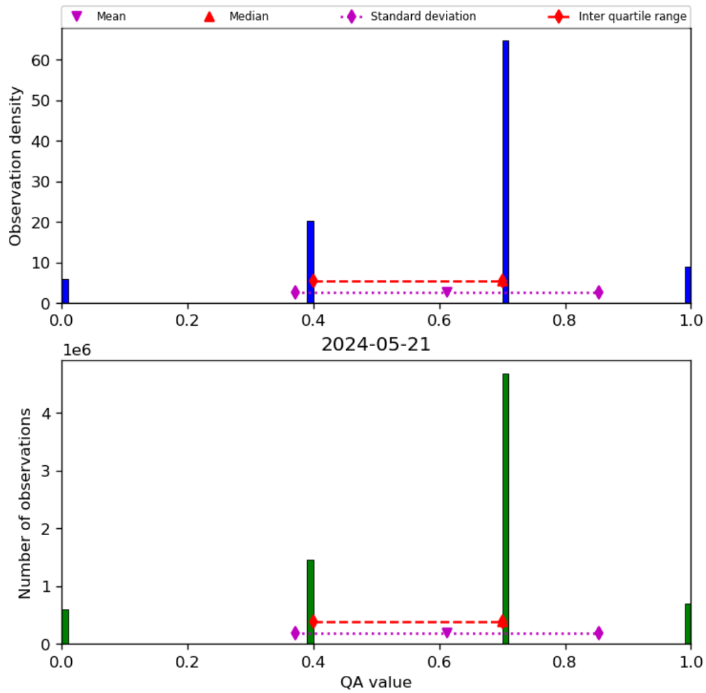
Figure 17: Histogram of “QA value” for 2024-05-20 to 2024-05-22
