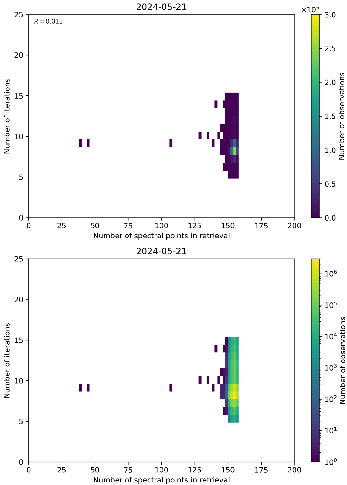
Figure 60: Scatter density plot of “Number of spectral points in retrieval” against “Number of iterations” for 2024-05-20 to 2024-05-22.
