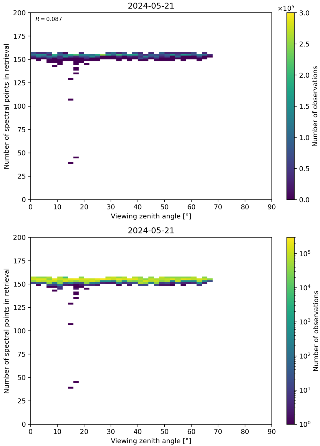
Figure 76: Scatter density plot of “Viewing zenith angle” against “Number of spectral points in retrieval” for 2024-05-20 to 2024-05-22.
