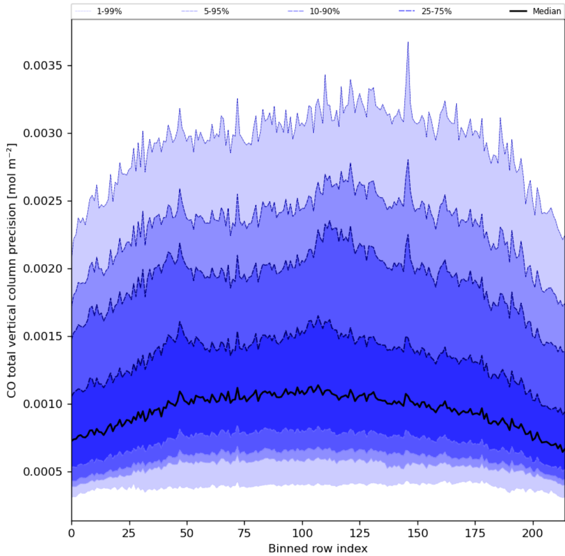
Figure 28: Along track statistics of “CO total vertical column precision” for 2024-05-20 to 2024-05-22
