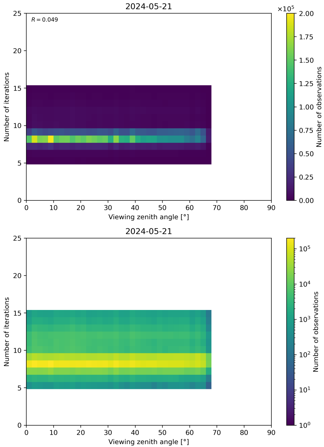
Figure 75: Scatter density plot of “Viewing zenith angle” against “Number of iterations” for 2024-05-20 to 2024-05-22.
