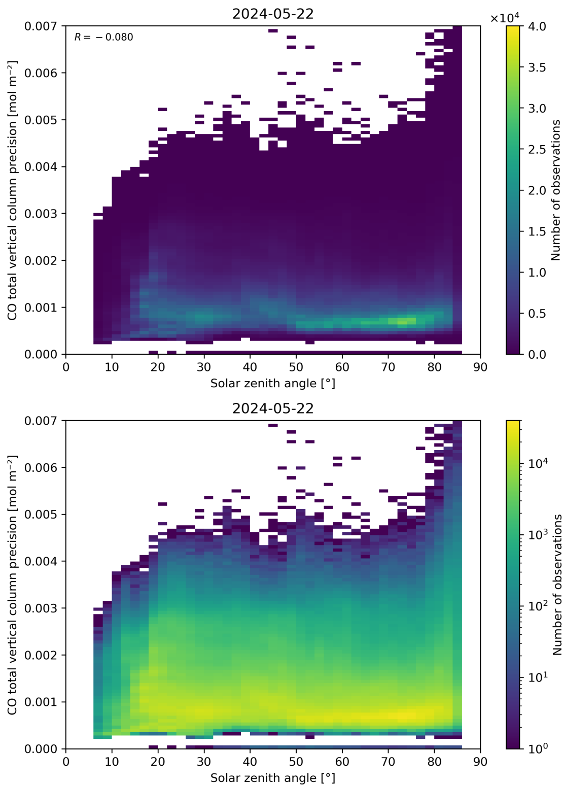
Figure 63: Scatter density plot of “Solar zenith angle” against “CO total vertical column precision” for 2024-05-21 to 2024-05-23.
