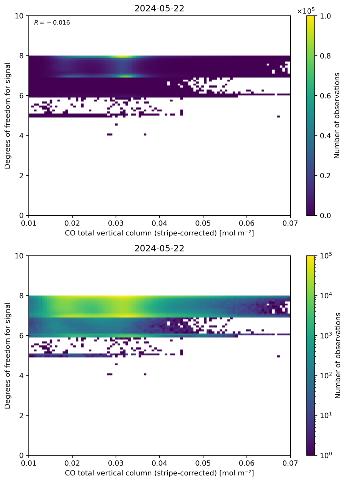
Figure 38: Scatter density plot of “CO total vertical column (stripe-corrected)” against “Degrees of freedom for signal” for 2024-05-21 to 2024-05-23.
