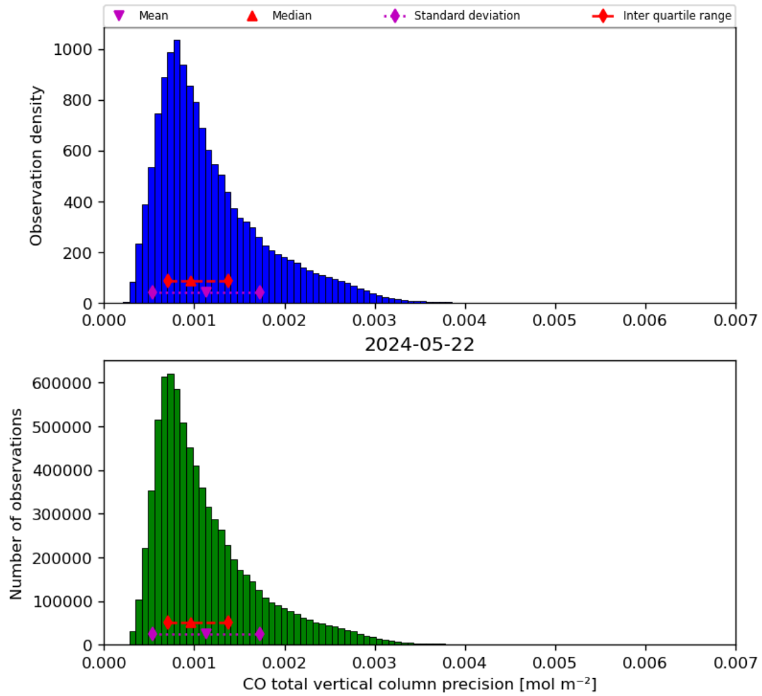
Figure 20: Histogram of “CO total vertical column precision” for 2024-05-21 to 2024-05-23
