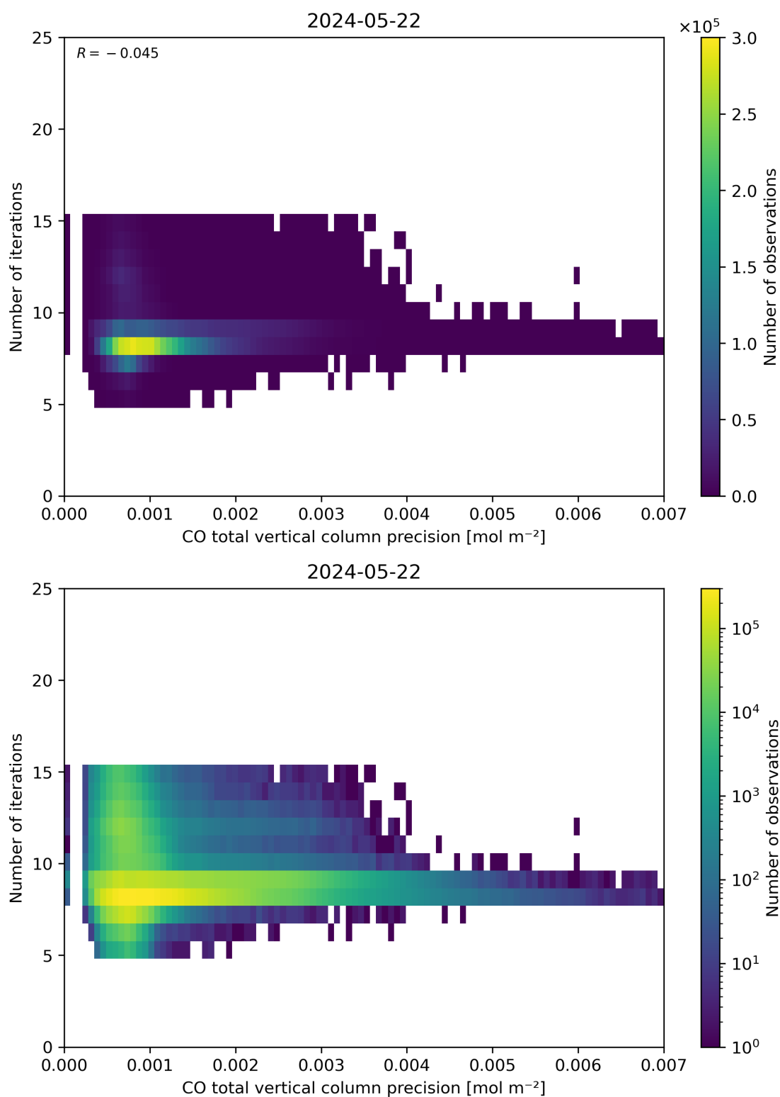
Figure 46: Scatter density plot of “CO total vertical column precision” against “Number of iterations” for 2024-05-21 to 2024-05-23.
