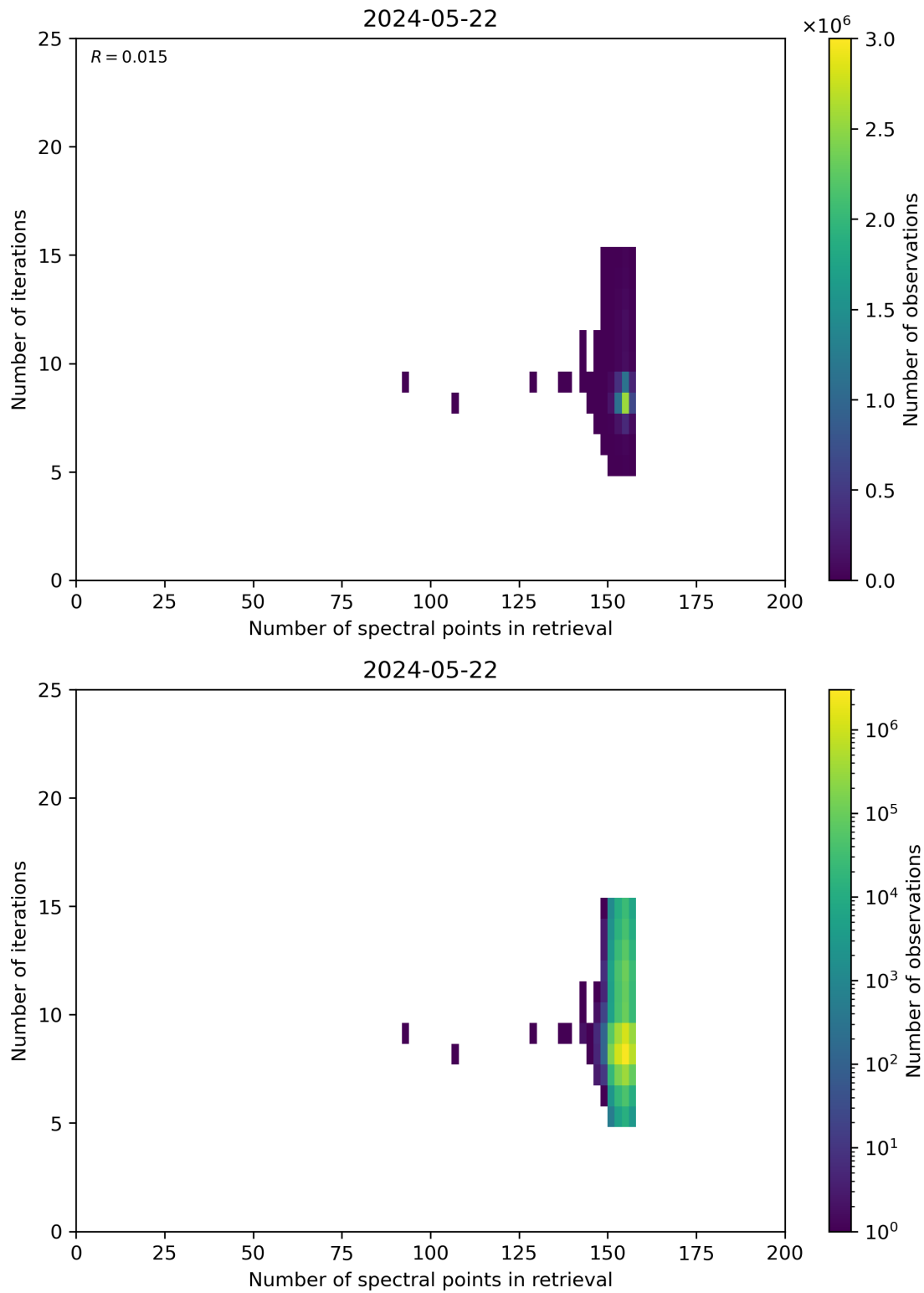
Figure 60: Scatter density plot of “Number of spectral points in retrieval” against “Number of iterations” for 2024-05-21 to 2024-05-23.
