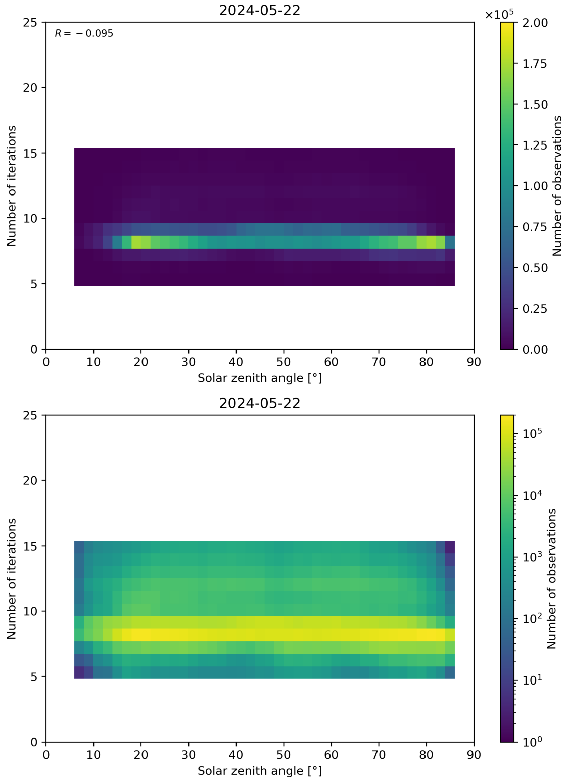
Figure 67: Scatter density plot of “Solar zenith angle” against “Number of iterations” for 2024-05-21 to 2024-05-23.
