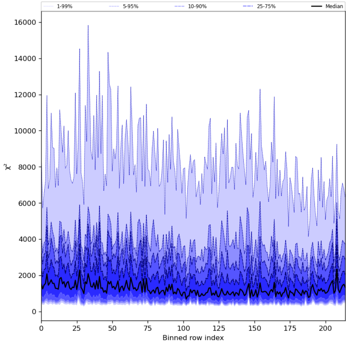
Figure 30: Along track statistics of “ \chi^2 ” for 2024-05-21 to 2024-05-23
