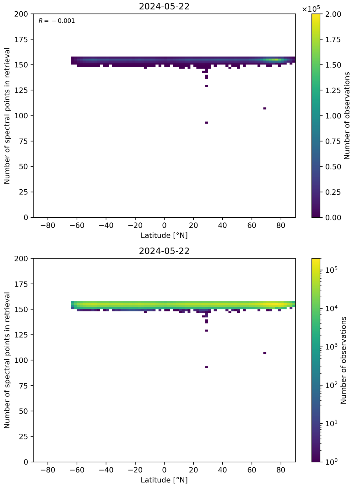
Figure 57: Scatter density plot of “Latitude” against “Number of spectral points in retrieval” for 2024-05-21 to 2024-05-23.
