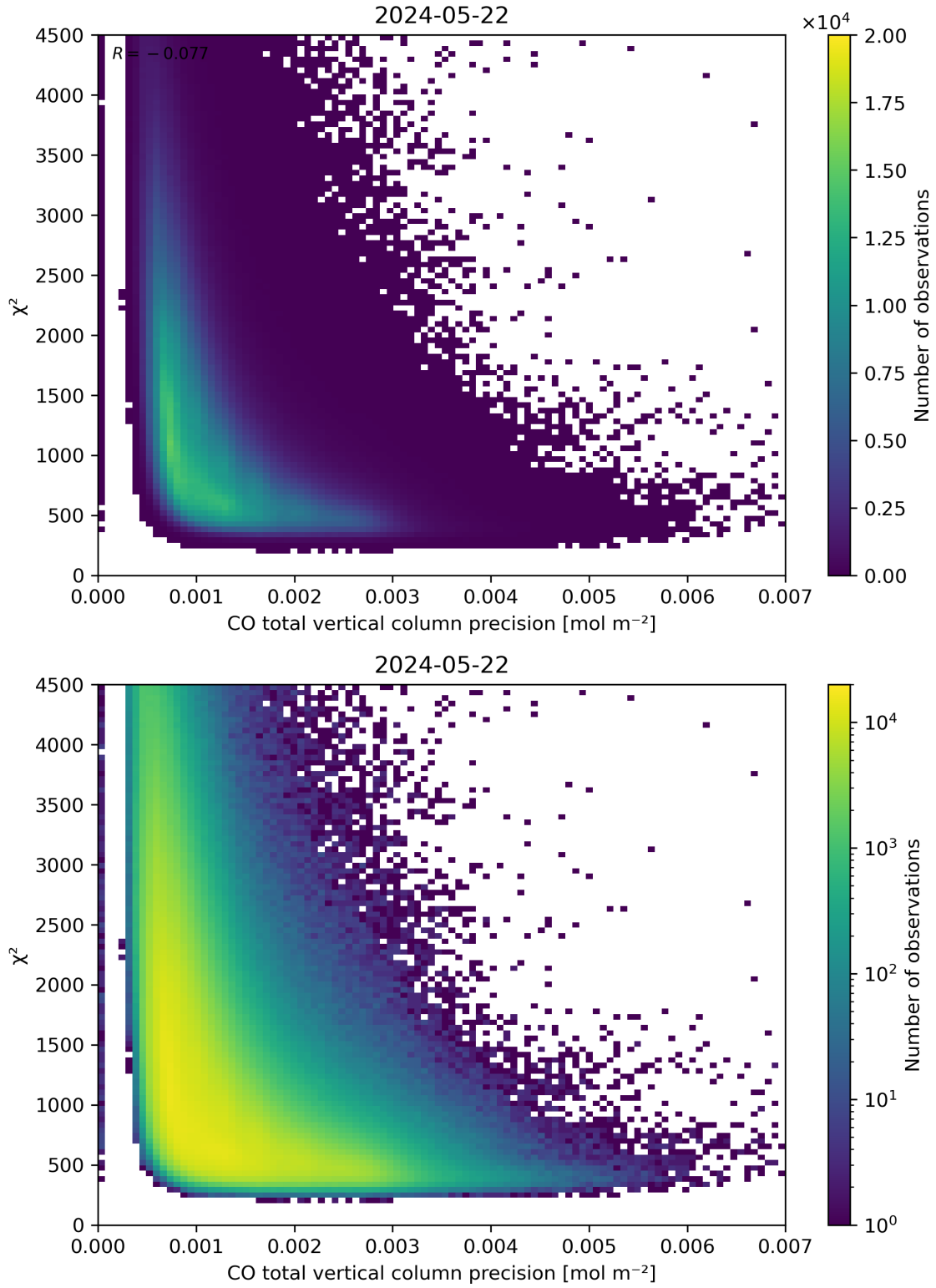
Figure 44: Scatter density plot of “CO total vertical column precision” against “ \chi^2 ” for 2024-05-21 to 2024-05-23.
