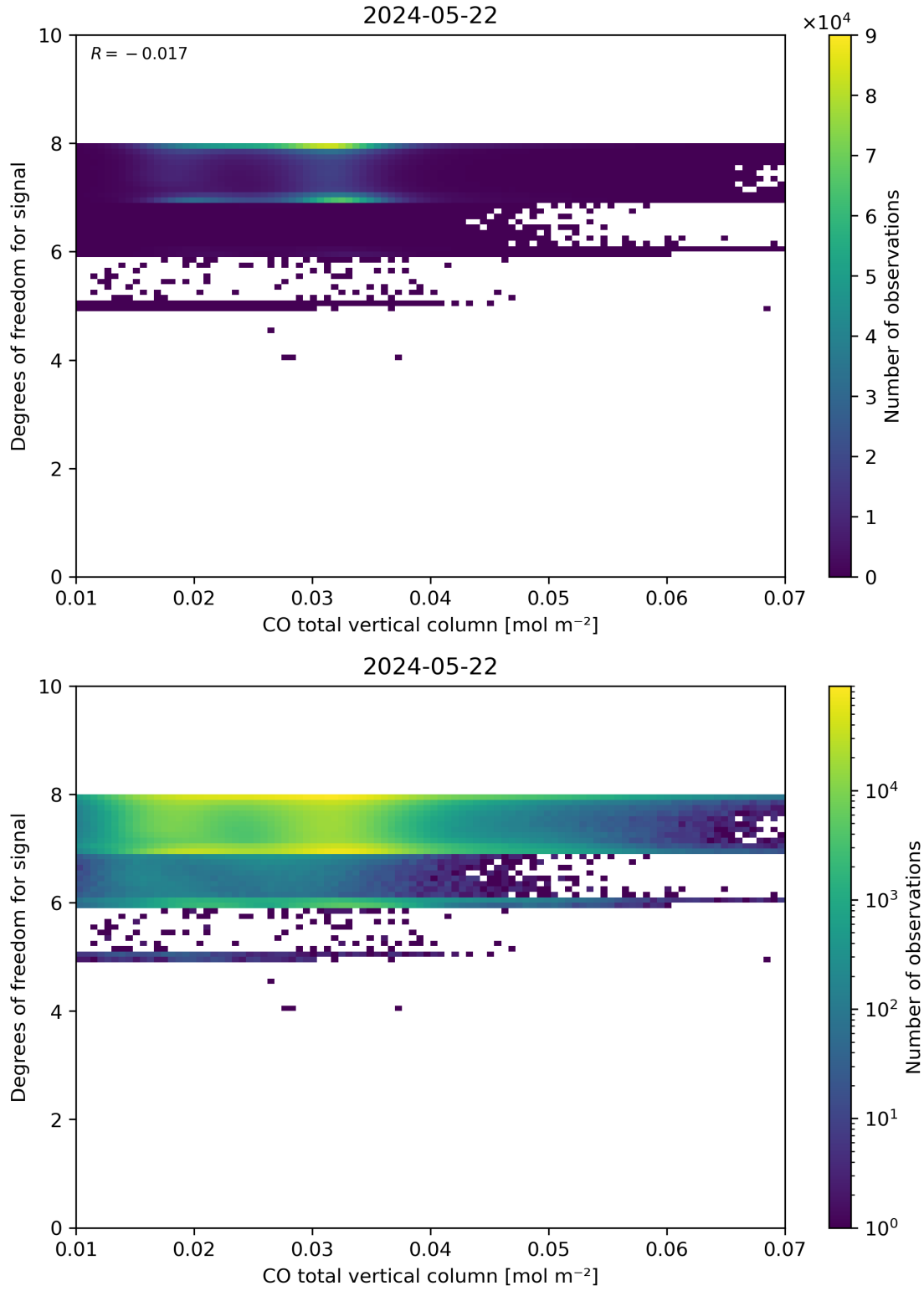
Figure 41: Scatter density plot of “CO total vertical column” against “Degrees of freedom for signal” for 2024-05-21 to 2024-05-23.
