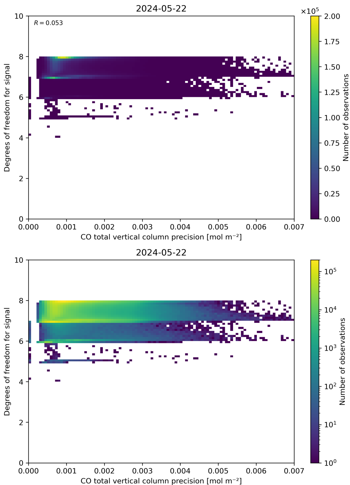
Figure 45: Scatter density plot of “CO total vertical column precision” against “Degrees of freedom for signal” for 2024-05-21 to 2024-05-23.
