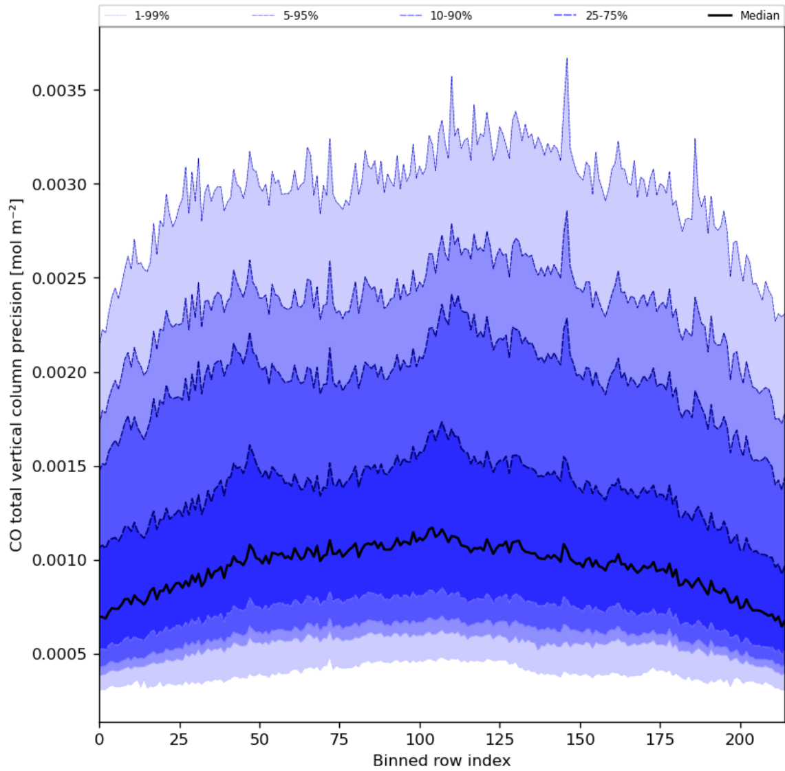
Figure 28: Along track statistics of “CO total vertical column precision” for 2024-05-21 to 2024-05-23
