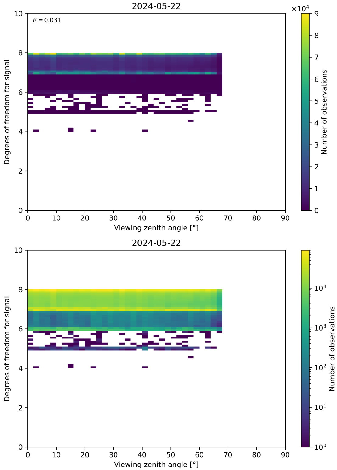
Figure 73: Scatter density plot of “Viewing zenith angle” against “Degrees of freedom for signal” for 2024-05-21 to 2024-05-23.
