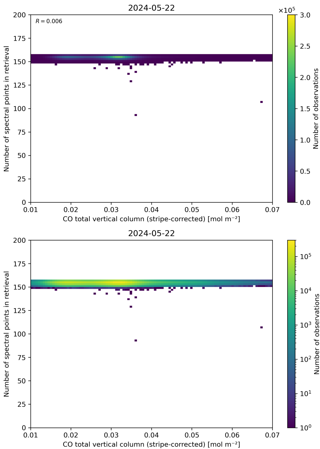
Figure 40: Scatter density plot of “CO total vertical column (stripe-corrected)” against “Number of spectral points in retrieval” for 2024-05-21 to 2024-05-23.
