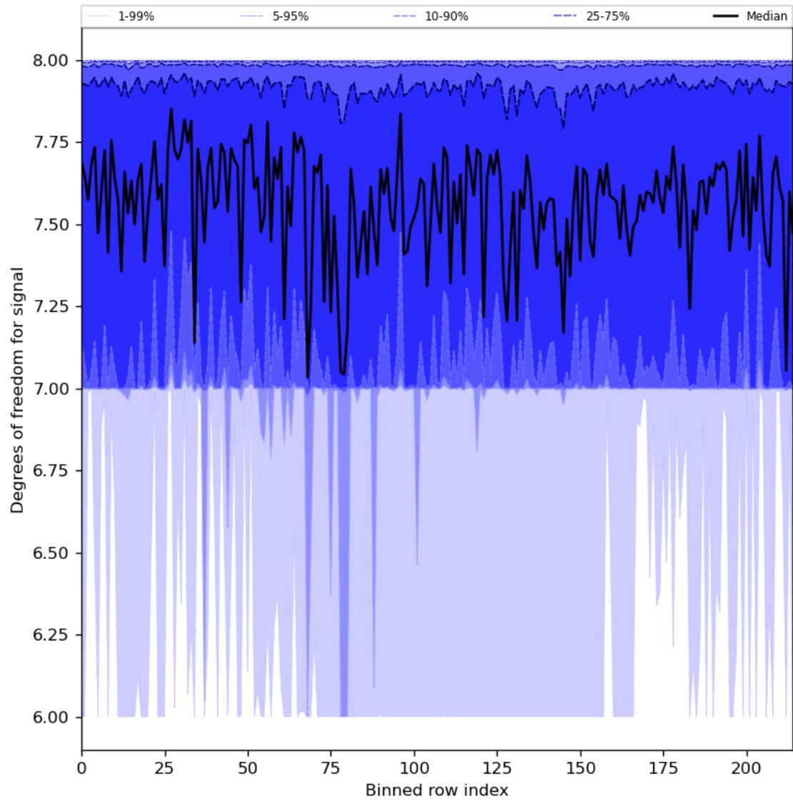
Figure 31: Along track statistics of “Degrees of freedom for signal” for 2024-05-21 to 2024-05-23
