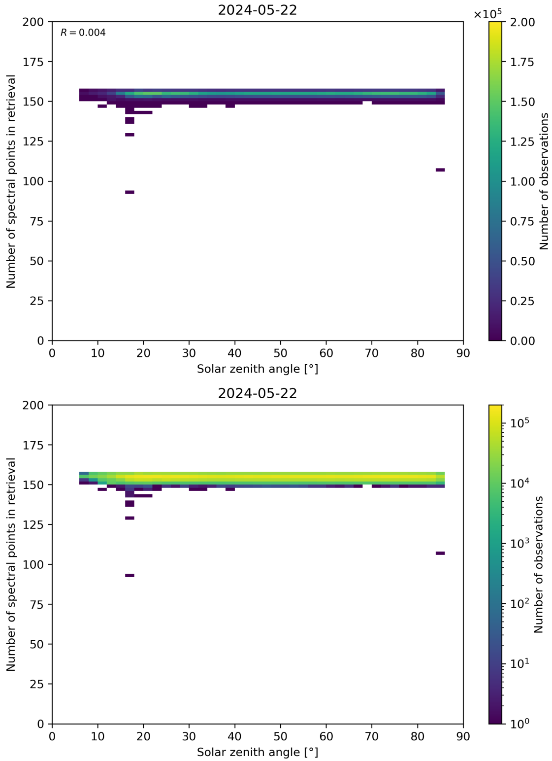
Figure 68: Scatter density plot of “Solar zenith angle” against “Number of spectral points in retrieval” for 2024-05-21 to 2024-05-23.
