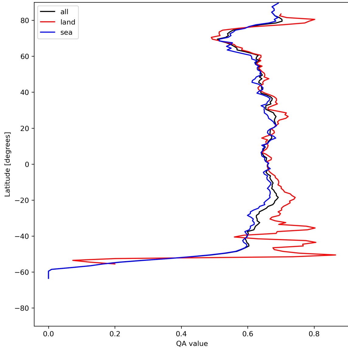
Figure 9: Zonal average of “QA value” for 2024-05-21 to 2024-05-23.
