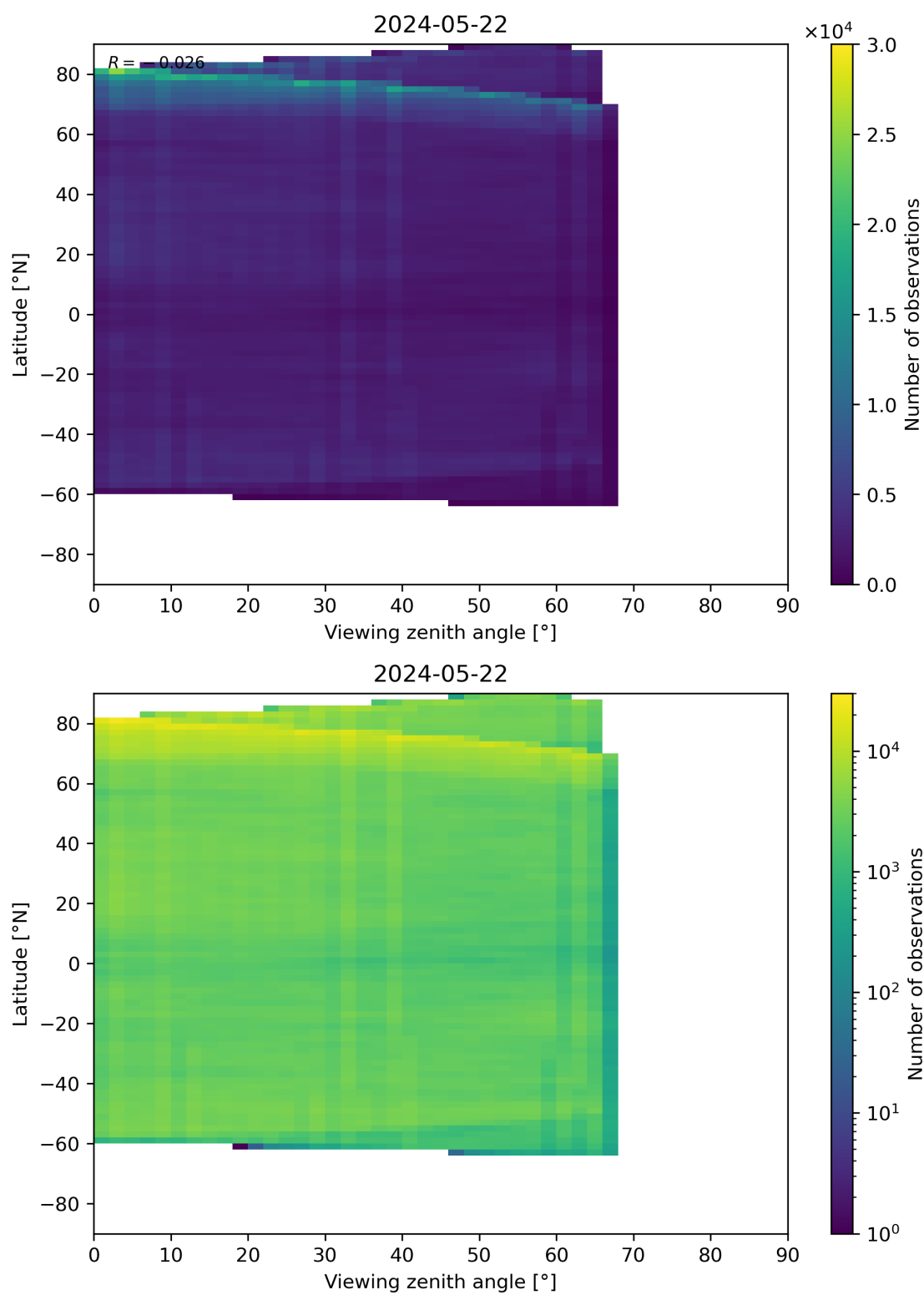
Figure 74: Scatter density plot of “Viewing zenith angle” against “Latitude” for 2024-05-21 to 2024-05-23.
