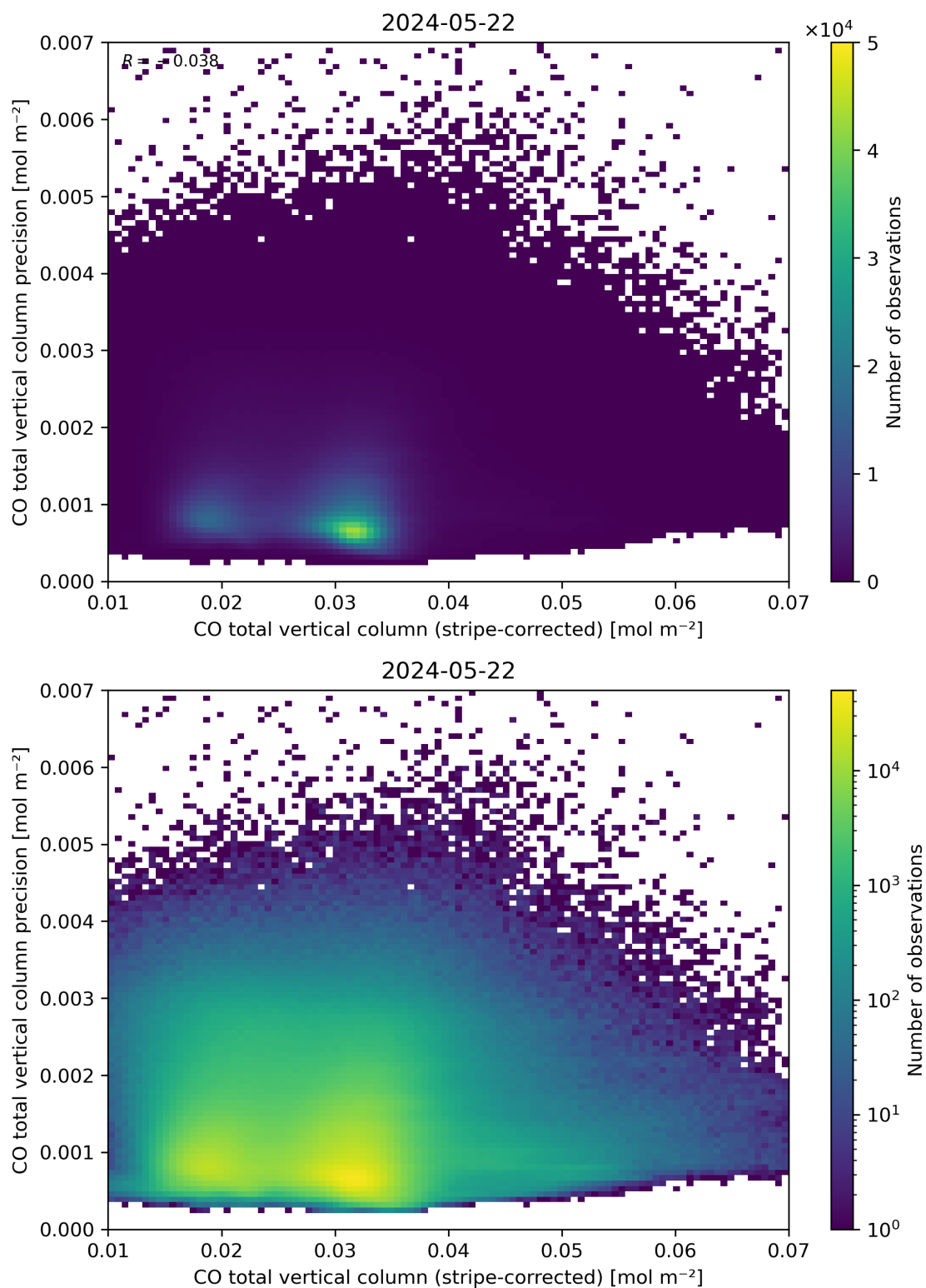
Figure 36: Scatter density plot of “CO total vertical column (stripe-corrected)” against “CO total vertical column precision” for 2024-05-21 to 2024-05-23.
