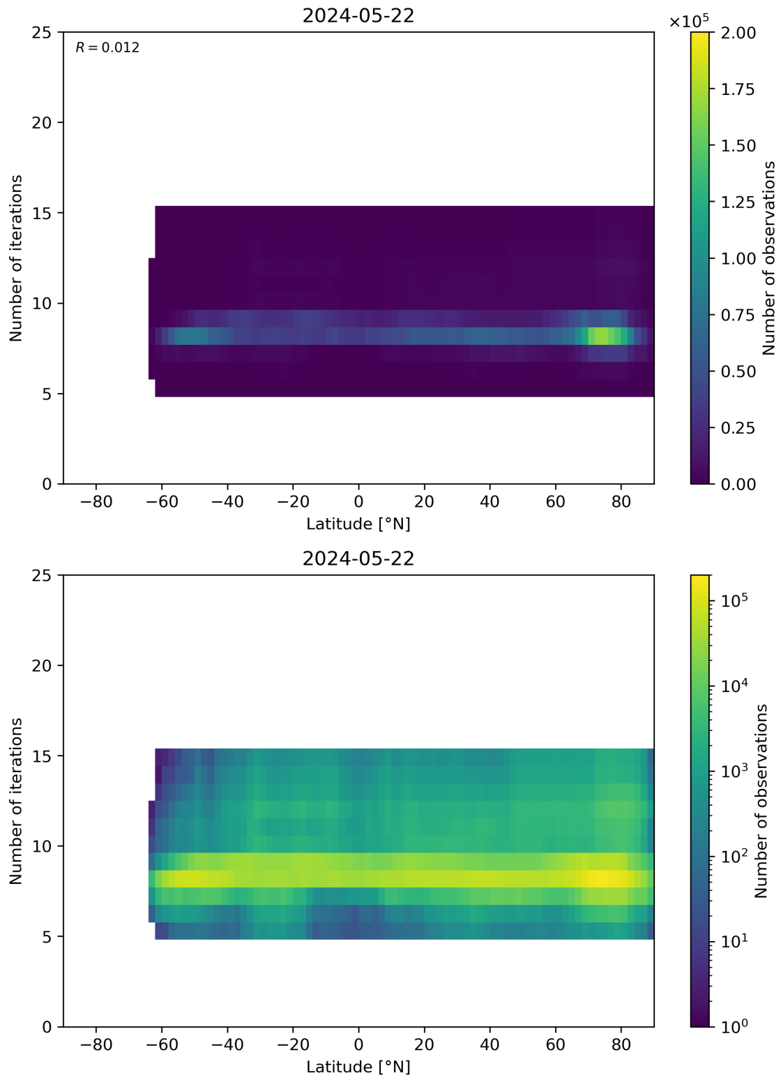
Figure 56: Scatter density plot of “Latitude” against “Number of iterations” for 2024-05-21 to 2024-05-23.
