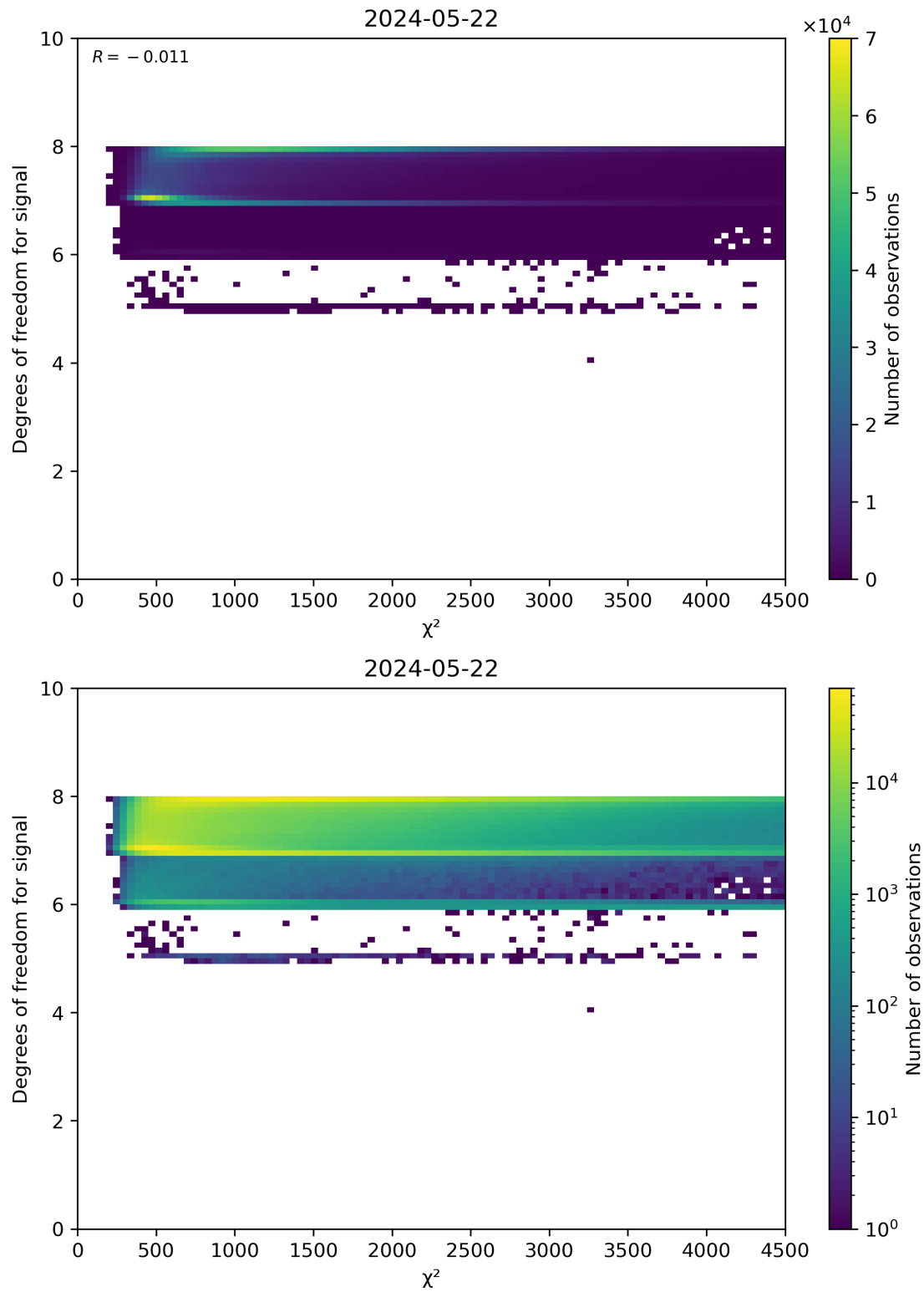
Figure 48: Scatter density plot of “ \chi^2 ” against “Degrees of freedom for signal” for 2024-05-21 to 2024-05-23.
