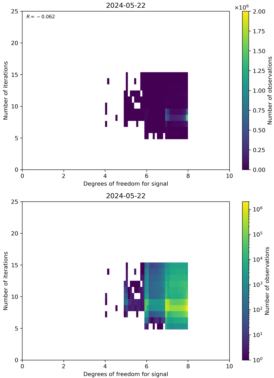
Figure 50: Scatter density plot of “Degrees of freedom for signal” against “Number of iterations” for 2024-05-21 to 2024-05-23.
