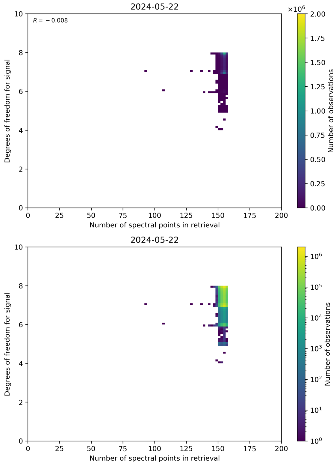
Figure 59: Scatter density plot of “Number of spectral points in retrieval” against “Degrees of freedom for signal” for 2024-05-21 to 2024-05-23.
