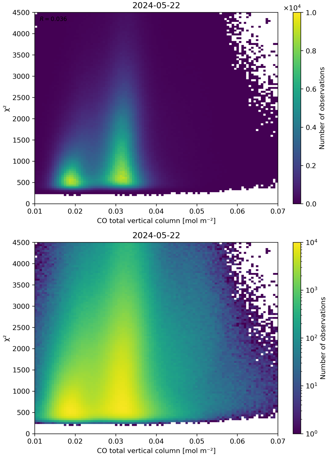
Figure 35: Scatter density plot of “CO total vertical column” against “ \chi^2 ” for 2024-05-21 to 2024-05-23.
