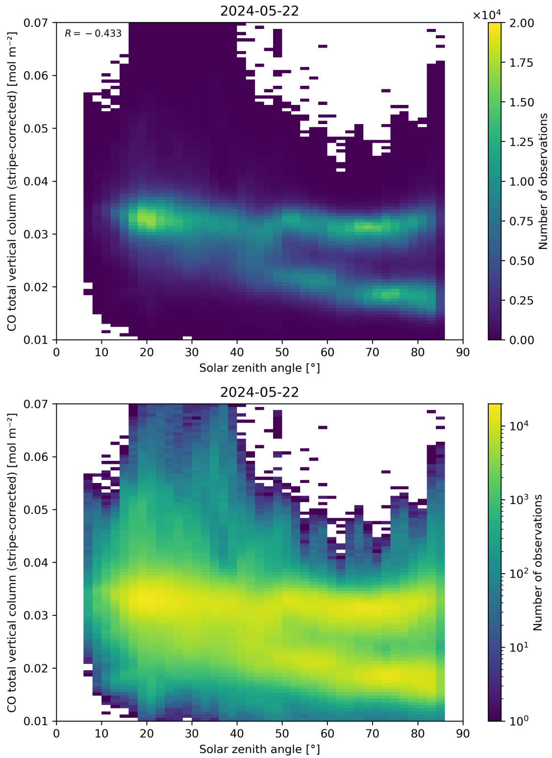
Figure 62: Scatter density plot of “Solar zenith angle” against “CO total vertical column (stripe-corrected)” for 2024-05-21 to 2024-05-23.
