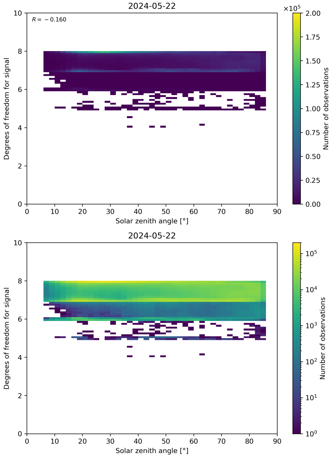
Figure 65: Scatter density plot of “Solar zenith angle” against “Degrees of freedom for signal” for 2024-05-21 to 2024-05-23.
