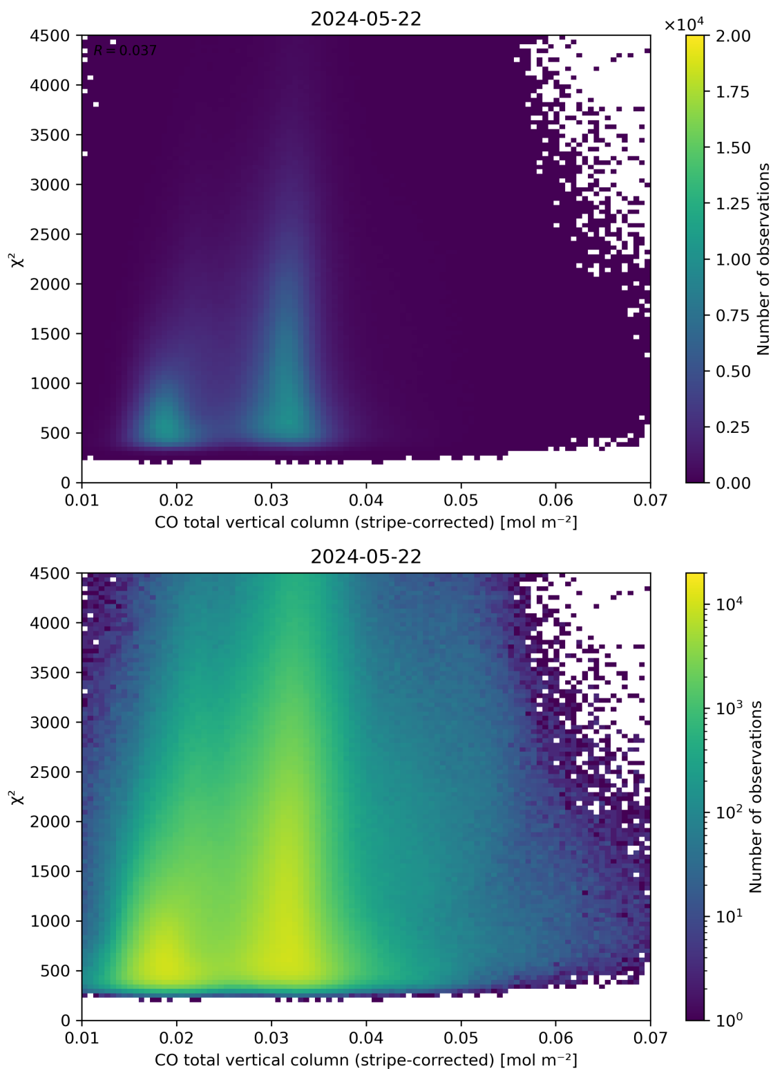
Figure 37: Scatter density plot of “CO total vertical column (stripe-corrected)” against “ \chi^2 ” for 2024-05-21 to 2024-05-23.
