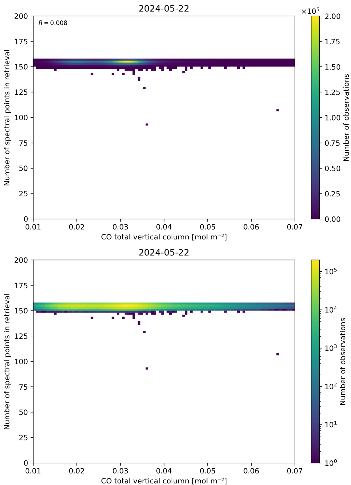
Figure 43: Scatter density plot of “CO total vertical column” against “Number of spectral points in retrieval” for 2024-05-21 to 2024-05-23.
