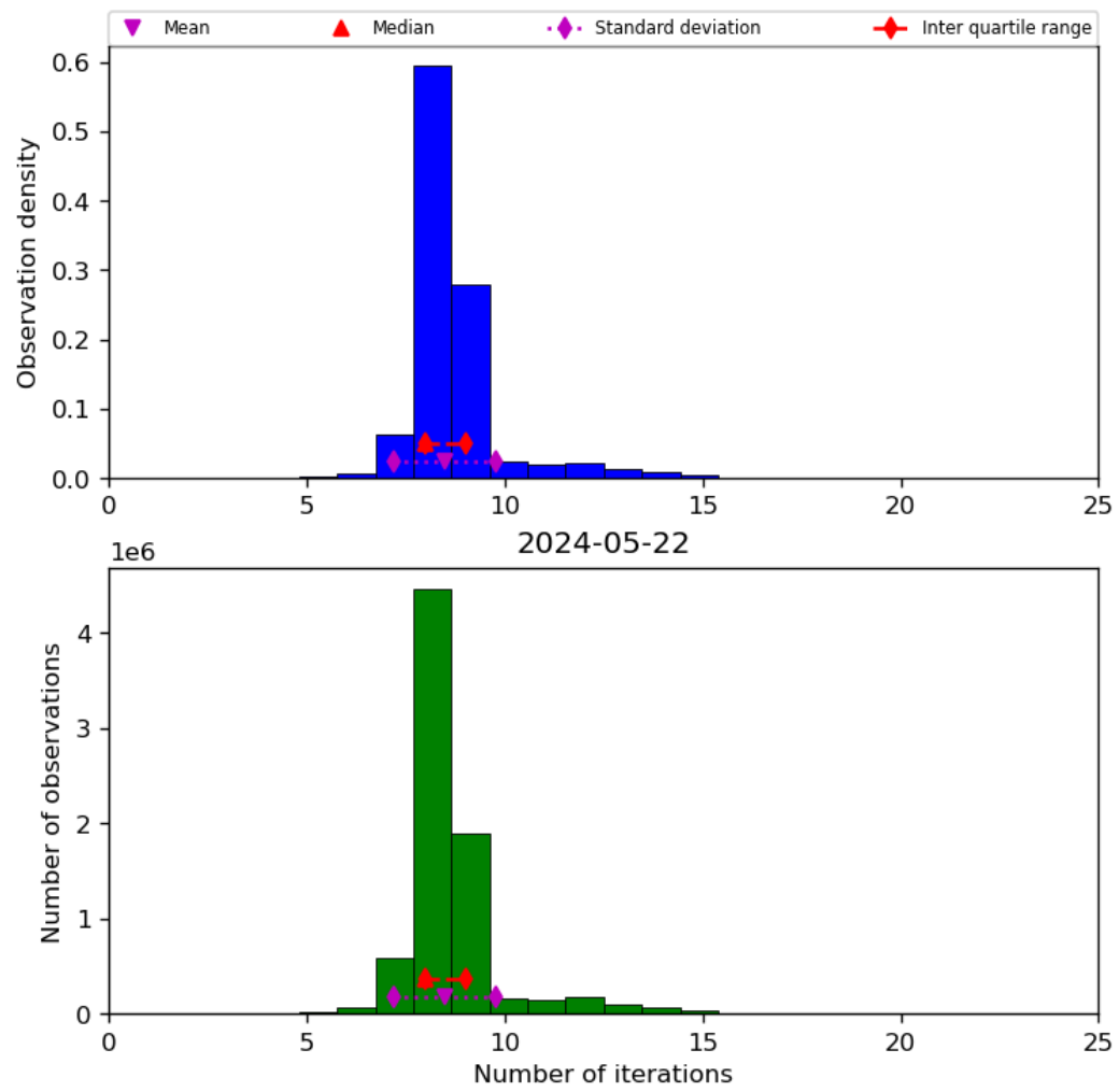
Figure 24: Histogram of “Number of iterations” for 2024-05-21 to 2024-05-23
