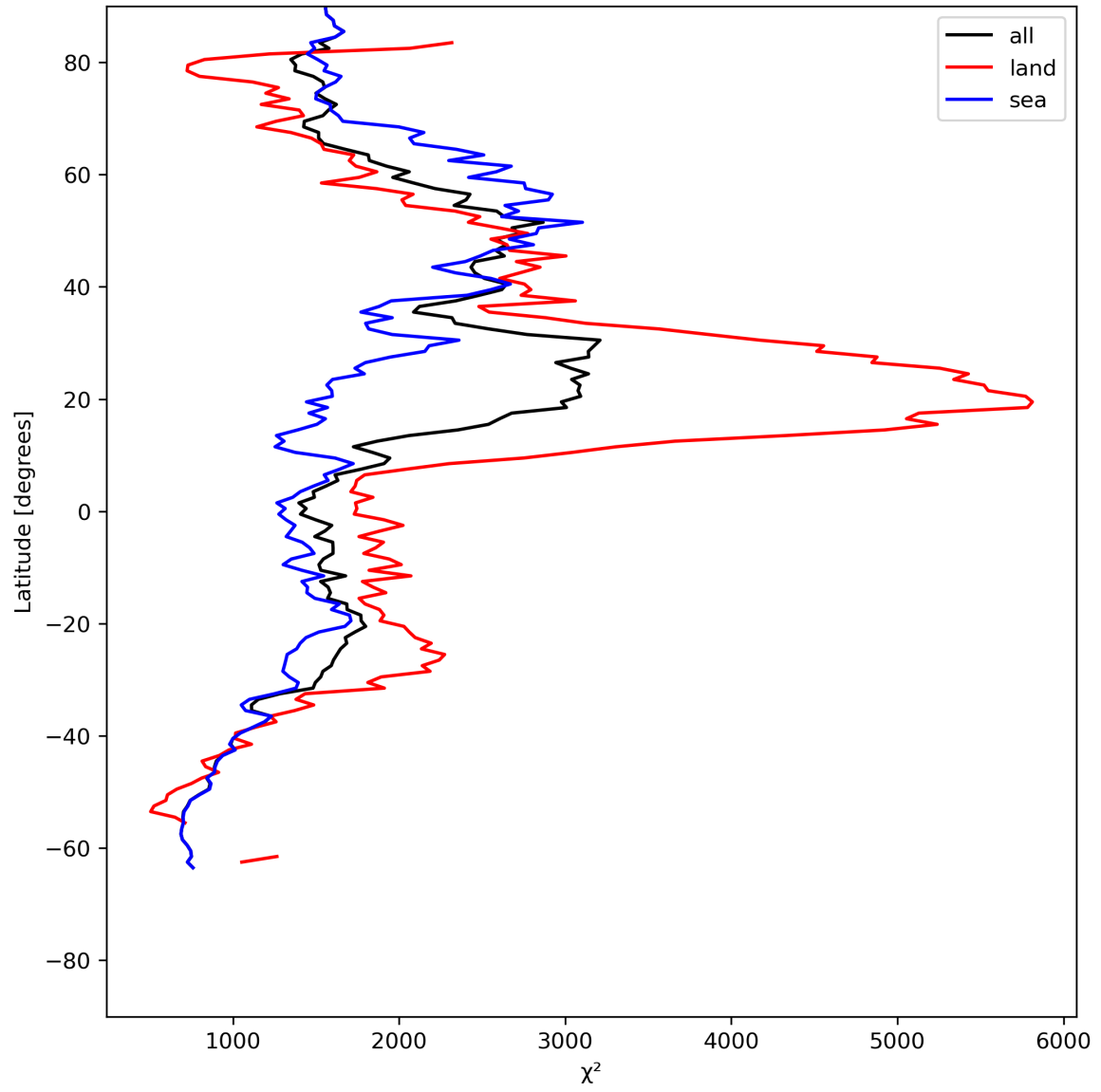
Figure 14: Zonal average of “ \chi^2 ” for 2024-05-21 to 2024-05-23.
