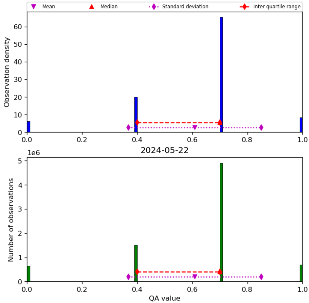
Figure 17: Histogram of “QA value” for 2024-05-21 to 2024-05-23
