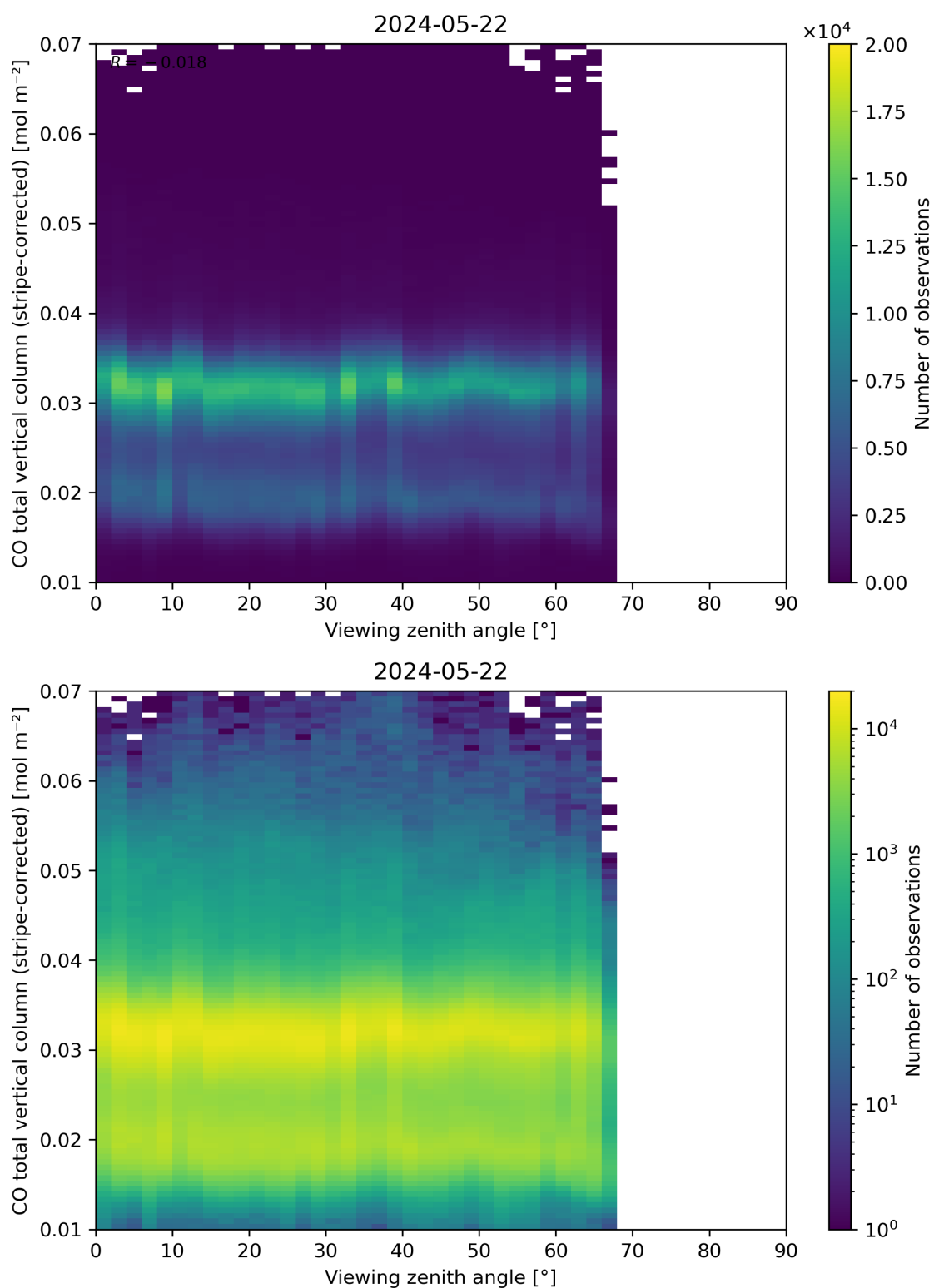
Figure 70: Scatter density plot of “Viewing zenith angle” against “CO total vertical column (stripe-corrected)” for 2024-05-21 to 2024-05-23.
