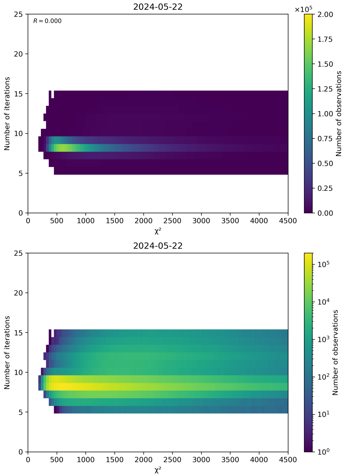
Figure 49: Scatter density plot of “ \chi^2 ” against “Number of iterations” for 2024-05-21 to 2024-05-23.
