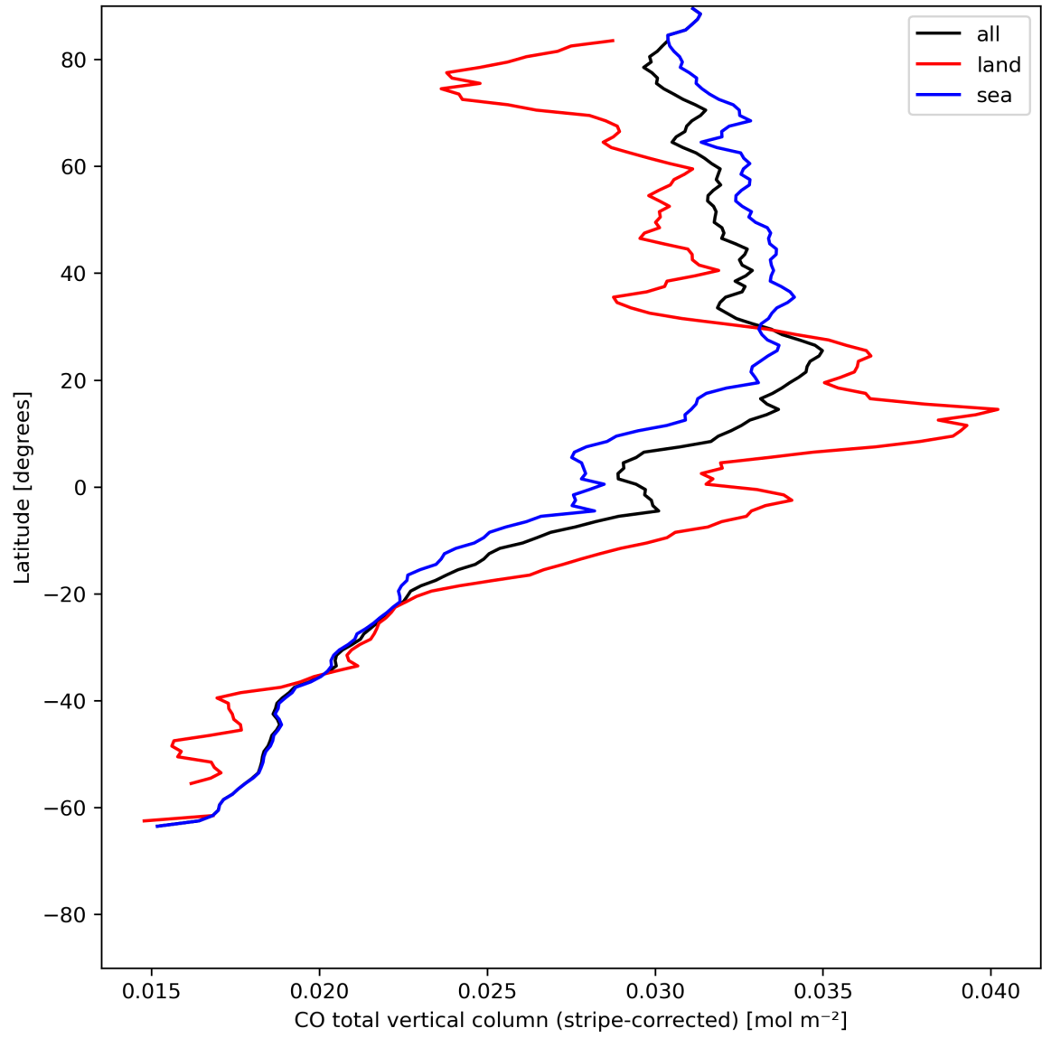
Figure 11: Zonal average of “CO total vertical column (stripe-corrected)” for 2024-05-21 to 2024-05-23.
