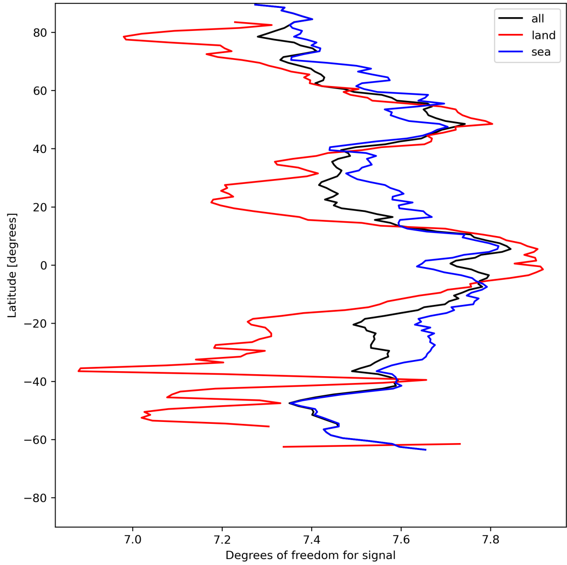
Figure 15: Zonal average of “Degrees of freedom for signal” for 2024-05-21 to 2024-05-23.
