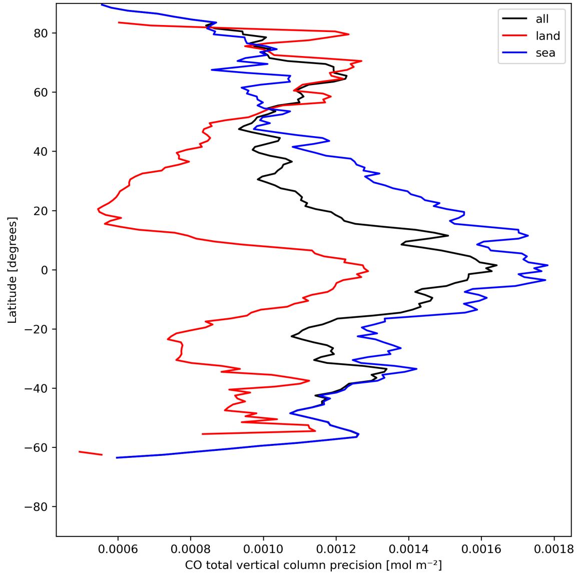
Figure 12: Zonal average of “CO total vertical column precision” for 2024-05-21 to 2024-05-23.
