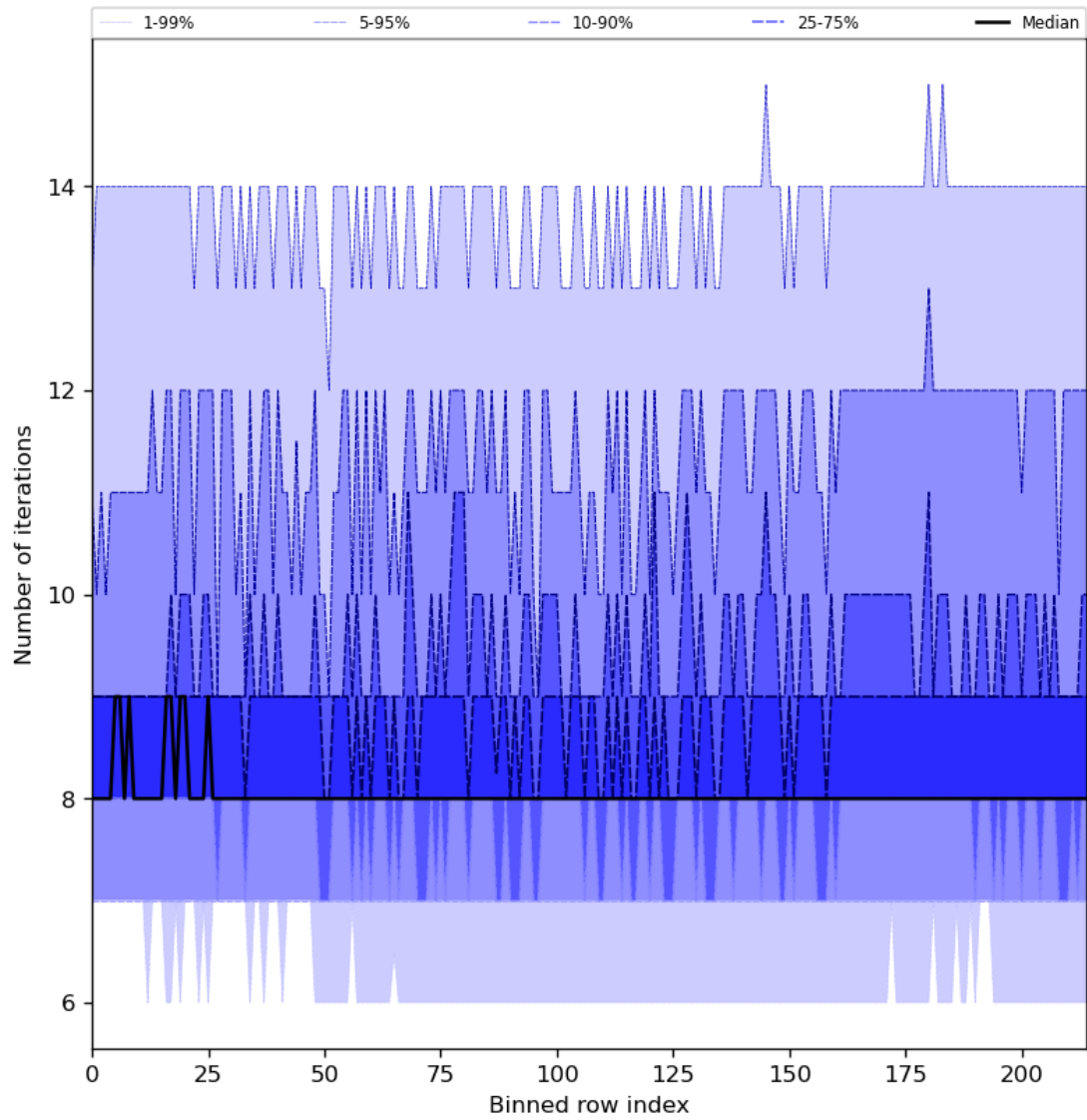
Figure 32: Along track statistics of “Number of iterations” for 2024-05-21 to 2024-05-23
