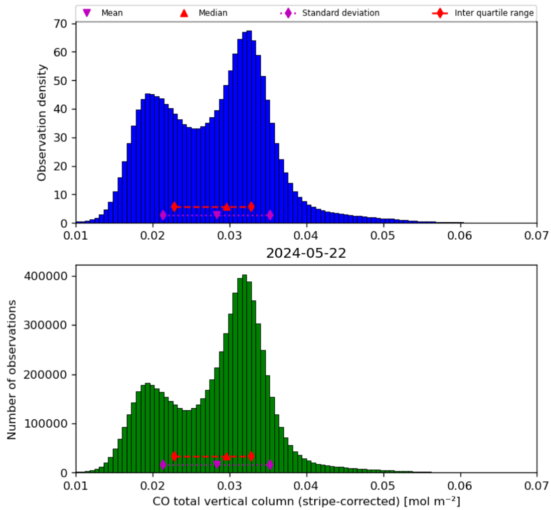
Figure 19: Histogram of “CO total vertical column (stripe-corrected)” for 2024-05-21 to 2024-05-23
