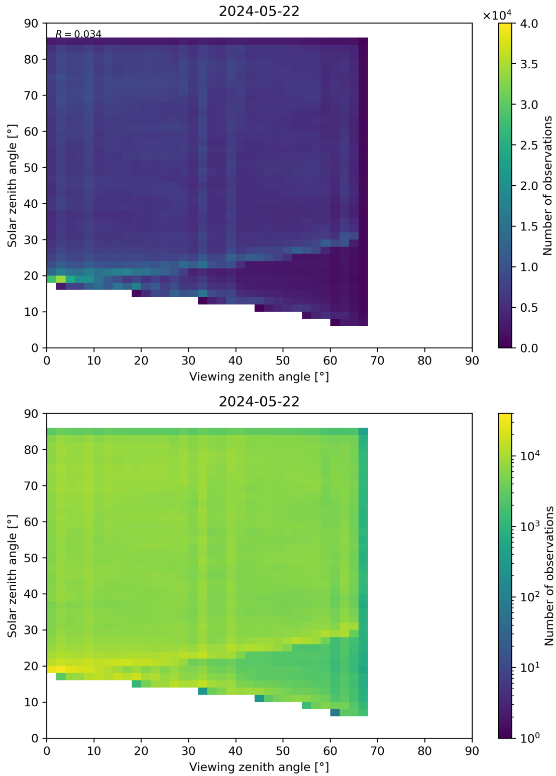
Figure 77: Scatter density plot of “Viewing zenith angle” against “Solar zenith angle” for 2024-05-21 to 2024-05-23.
