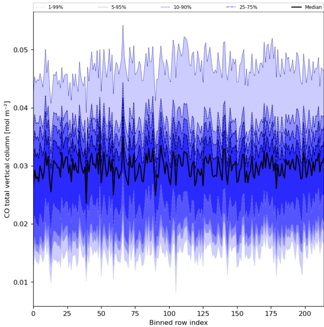
Figure 26: Along track statistics of “CO total vertical column” for 2024-05-21 to 2024-05-23
