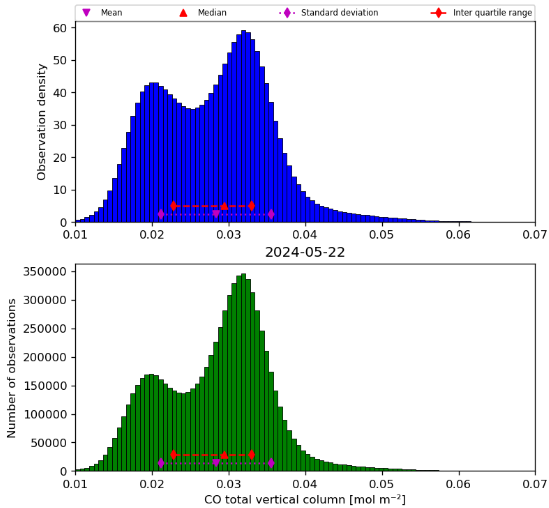
Figure 18: Histogram of “CO total vertical column” for 2024-05-21 to 2024-05-23
