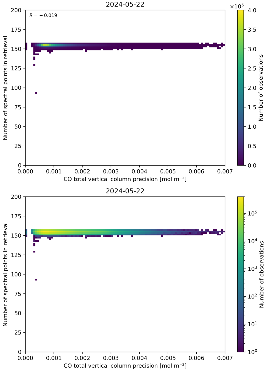
Figure 47: Scatter density plot of “CO total vertical column precision” against “Number of spectral points in retrieval” for 2024-05-21 to 2024-05-23.
