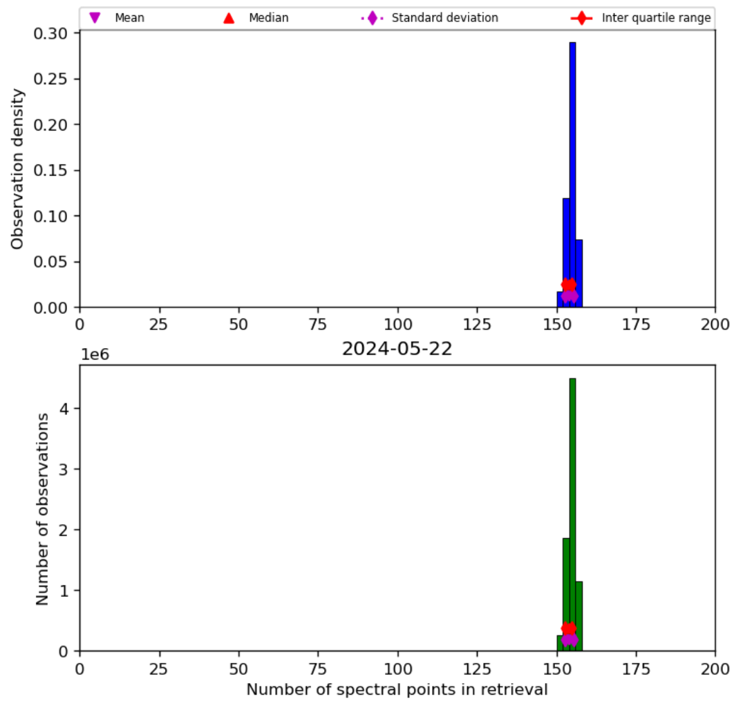
Figure 21: Histogram of “Number of spectral points in retrieval” for 2024-05-21 to 2024-05-23
