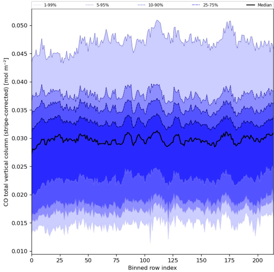
Figure 27: Along track statistics of “CO total vertical column (stripe-corrected)” for 2024-05-21 to 2024-05-23
