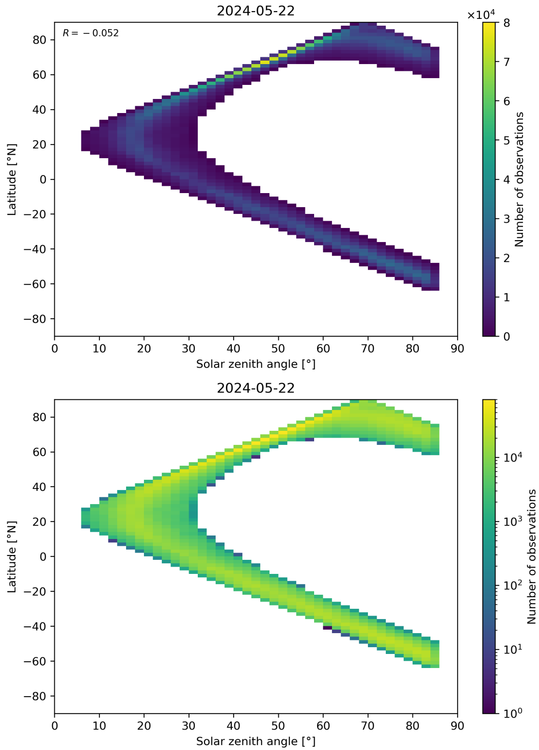
Figure 66: Scatter density plot of “Solar zenith angle” against “Latitude” for 2024-05-21 to 2024-05-23.
