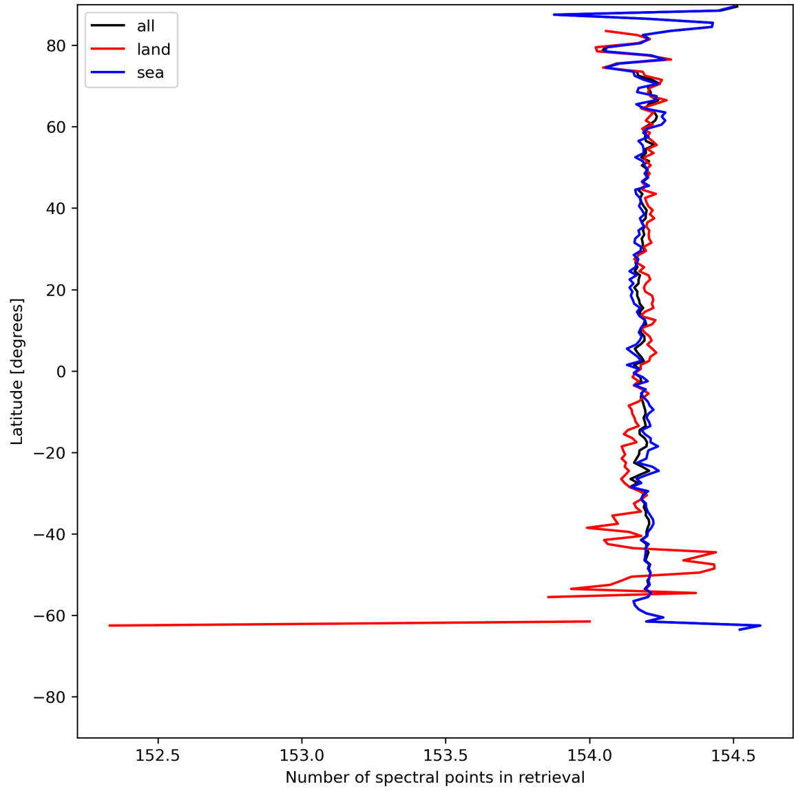
Figure 13: Zonal average of “Number of spectral points in retrieval” for 2024-05-21 to 2024-05-23.
