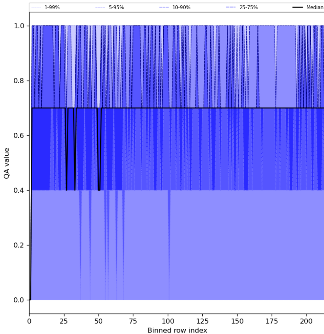
Figure 25: Along track statistics of “QA value” for 2024-05-21 to 2024-05-23
