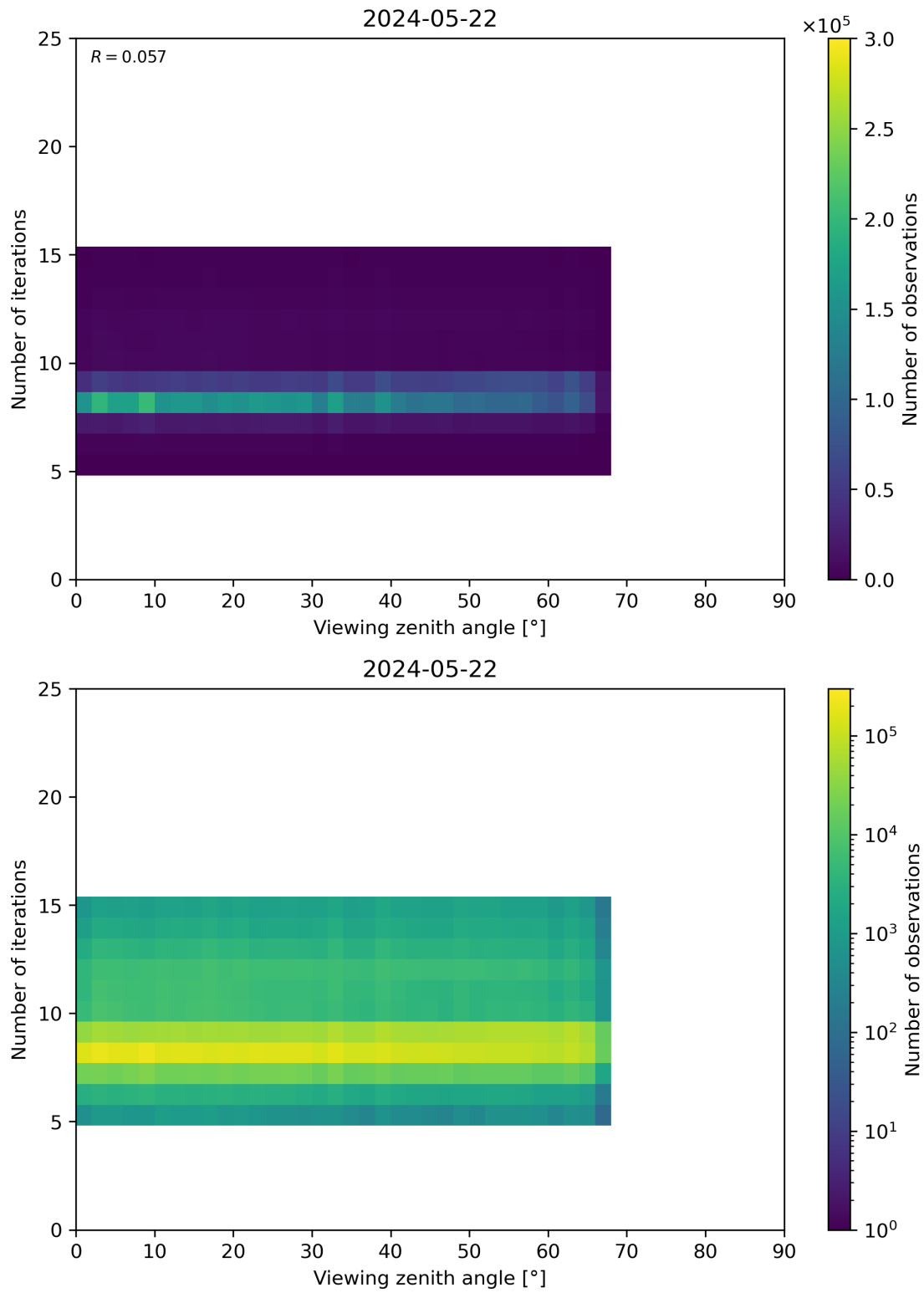
Figure 75: Scatter density plot of “Viewing zenith angle” against “Number of iterations” for 2024-05-21 to 2024-05-23.
