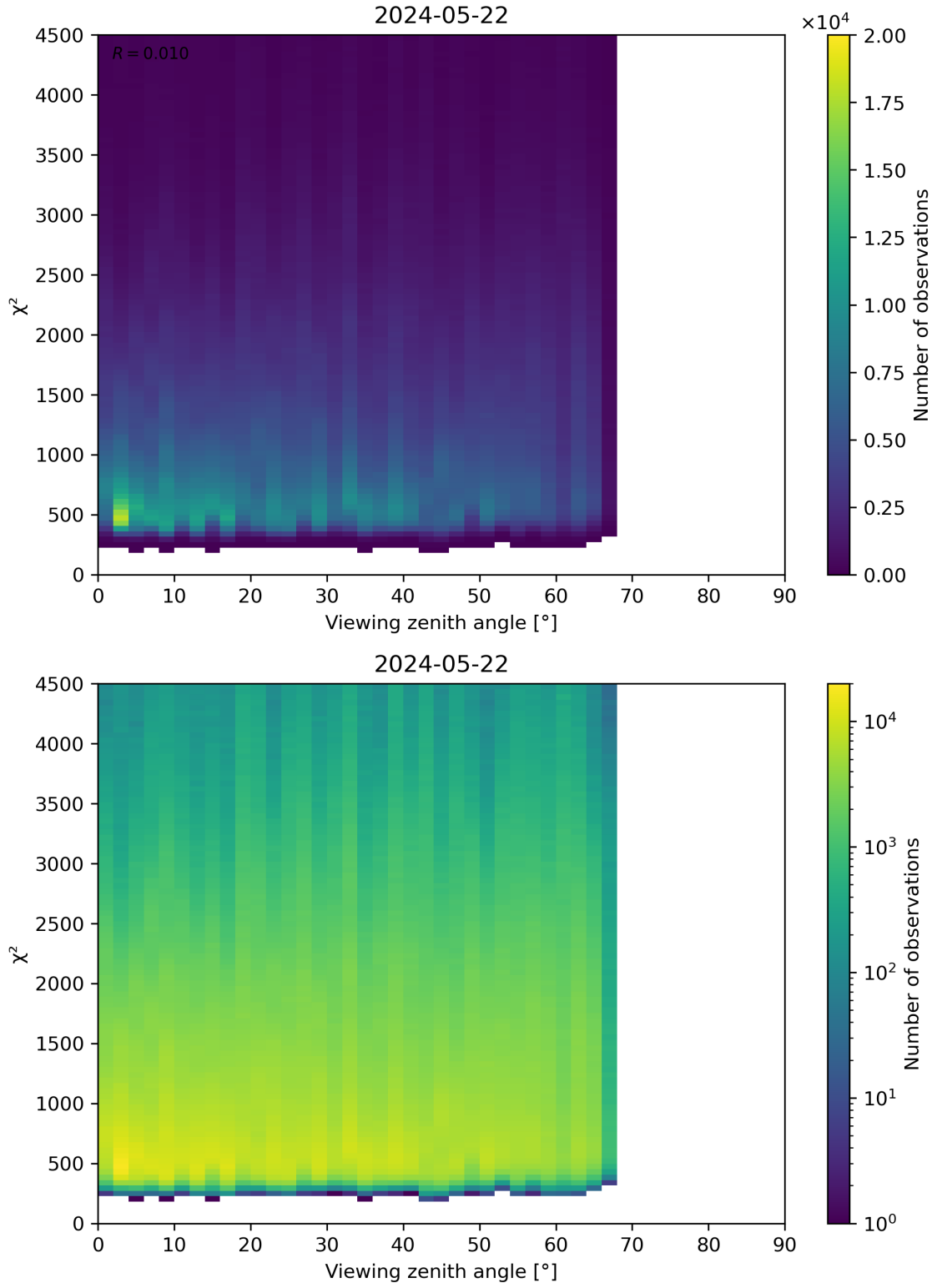
Figure 72: Scatter density plot of “Viewing zenith angle” against “ \chi^2 ” for 2024-05-21 to 2024-05-23.
