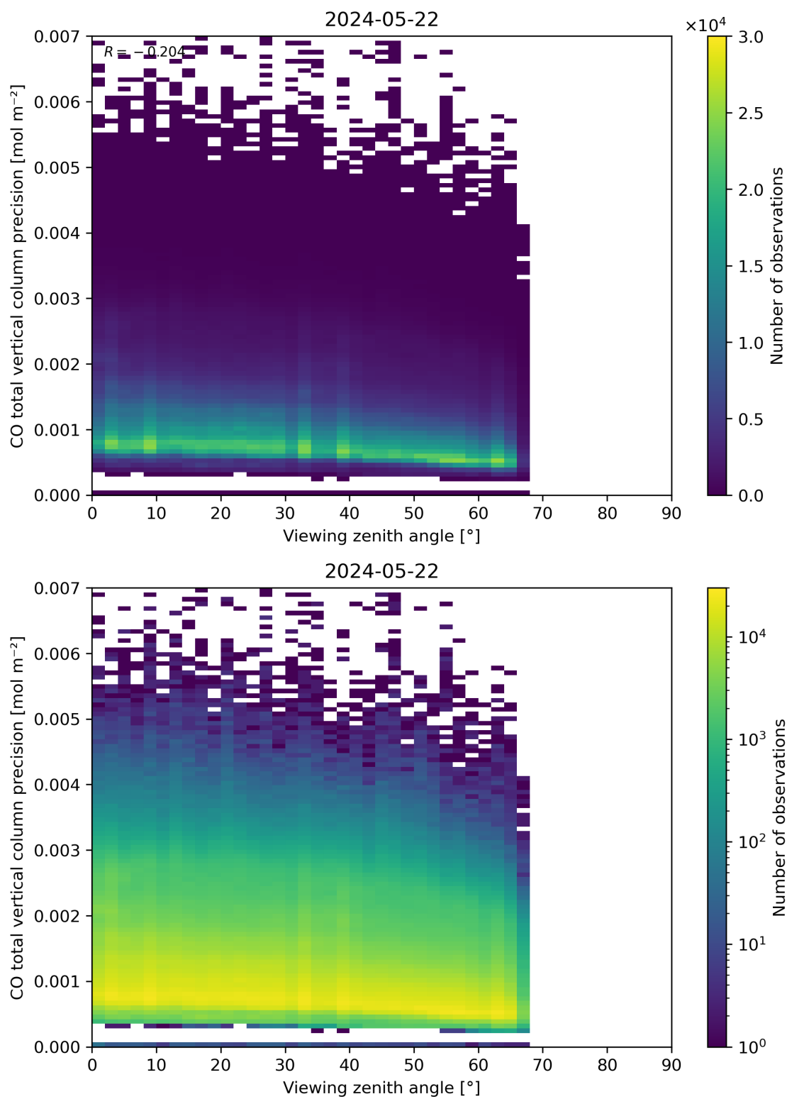
Figure 71: Scatter density plot of “Viewing zenith angle” against “CO total vertical column precision” for 2024-05-21 to 2024-05-23.
