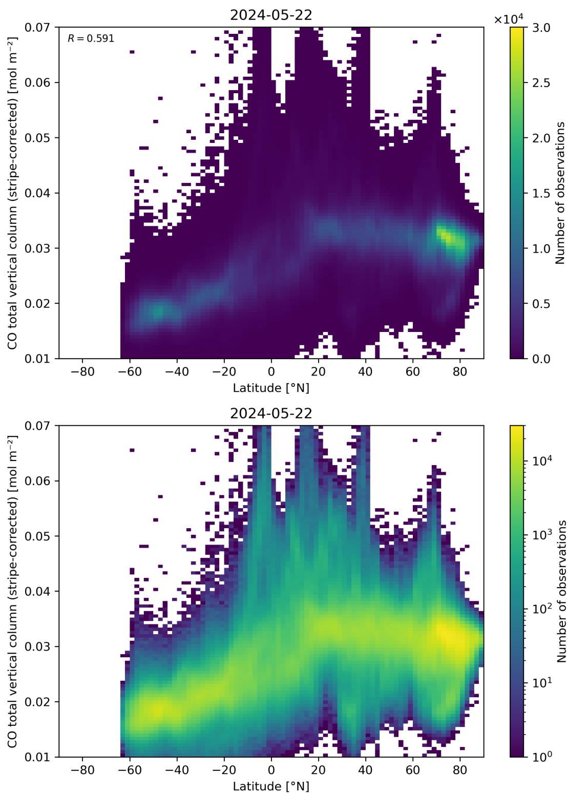
Figure 52: Scatter density plot of “Latitude” against “CO total vertical column (stripe-corrected)” for 2024-05-21 to 2024-05-23.
