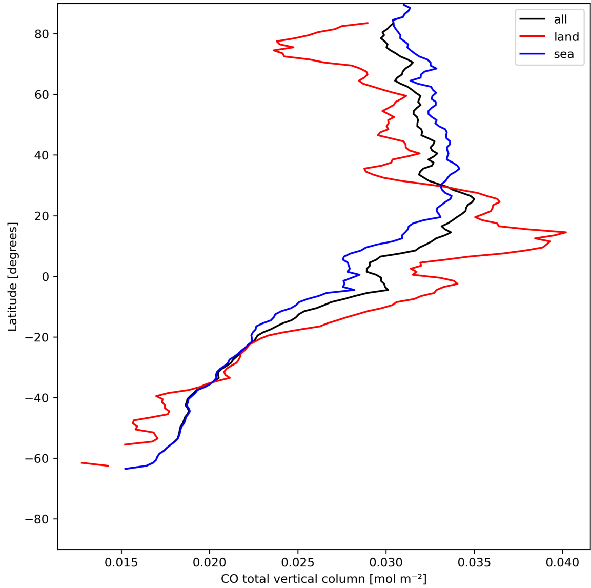
Figure 10: Zonal average of “CO total vertical column” for 2024-05-21 to 2024-05-23.
