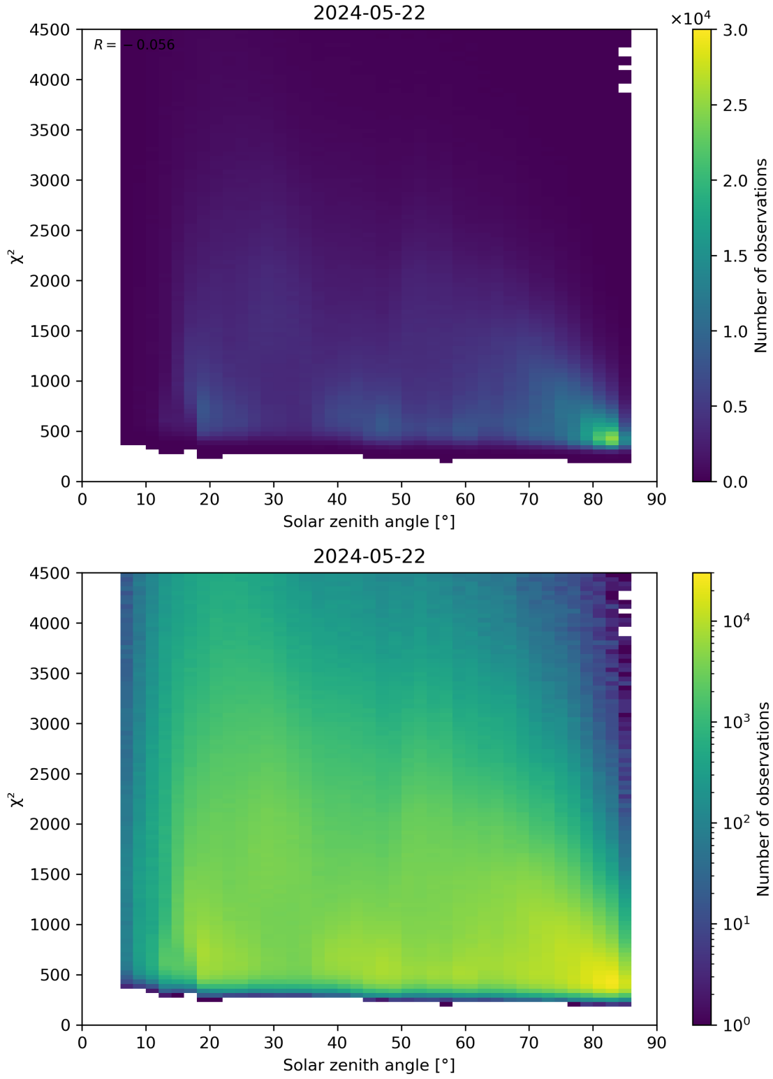
Figure 64: Scatter density plot of “Solar zenith angle” against “ \chi^2 ” for 2024-05-21 to 2024-05-23.
