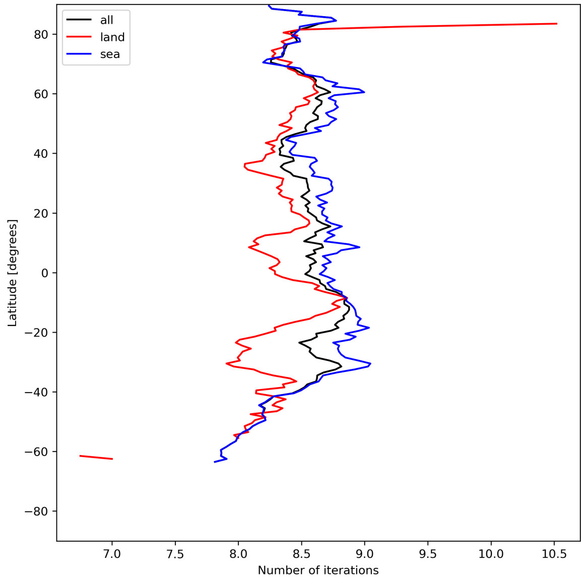
Figure 16: Zonal average of “Number of iterations” for 2024-05-21 to 2024-05-23.
