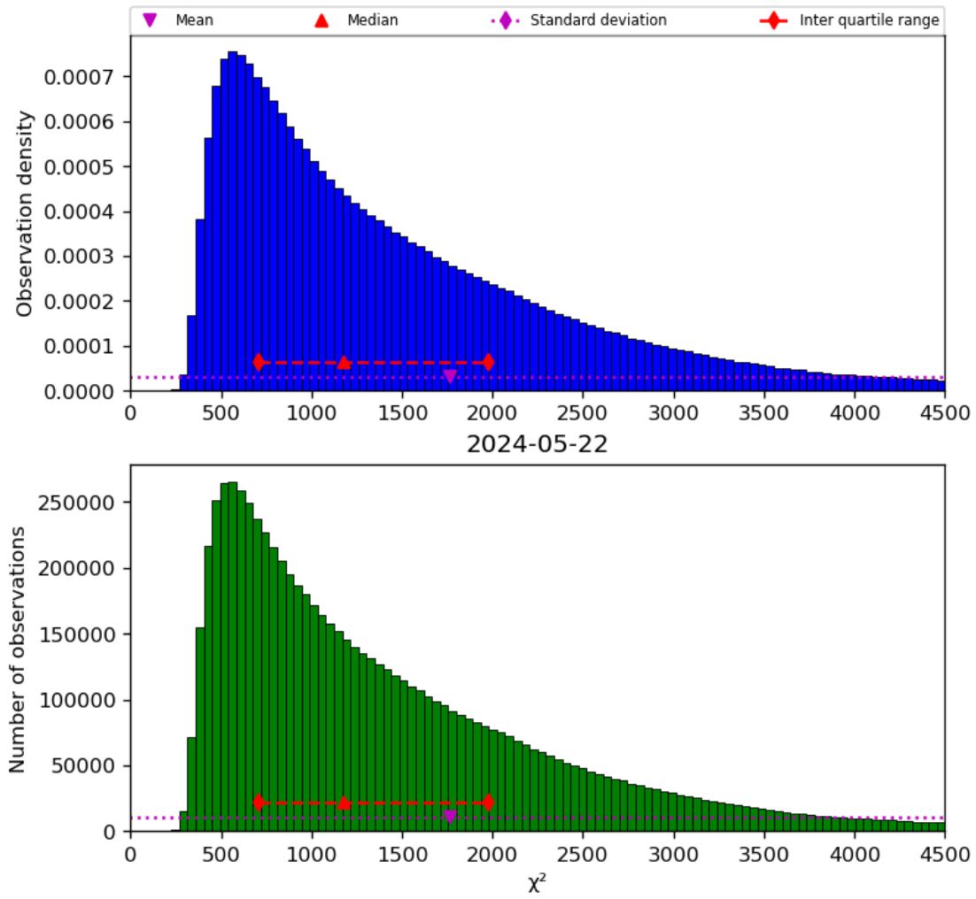
Figure 22: Histogram of “ \chi^2 ” for 2024-05-21 to 2024-05-23
