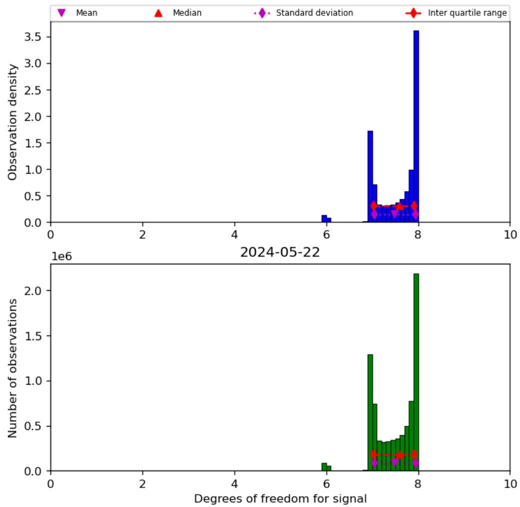
Figure 23: Histogram of “Degrees of freedom for signal” for 2024-05-21 to 2024-05-23
