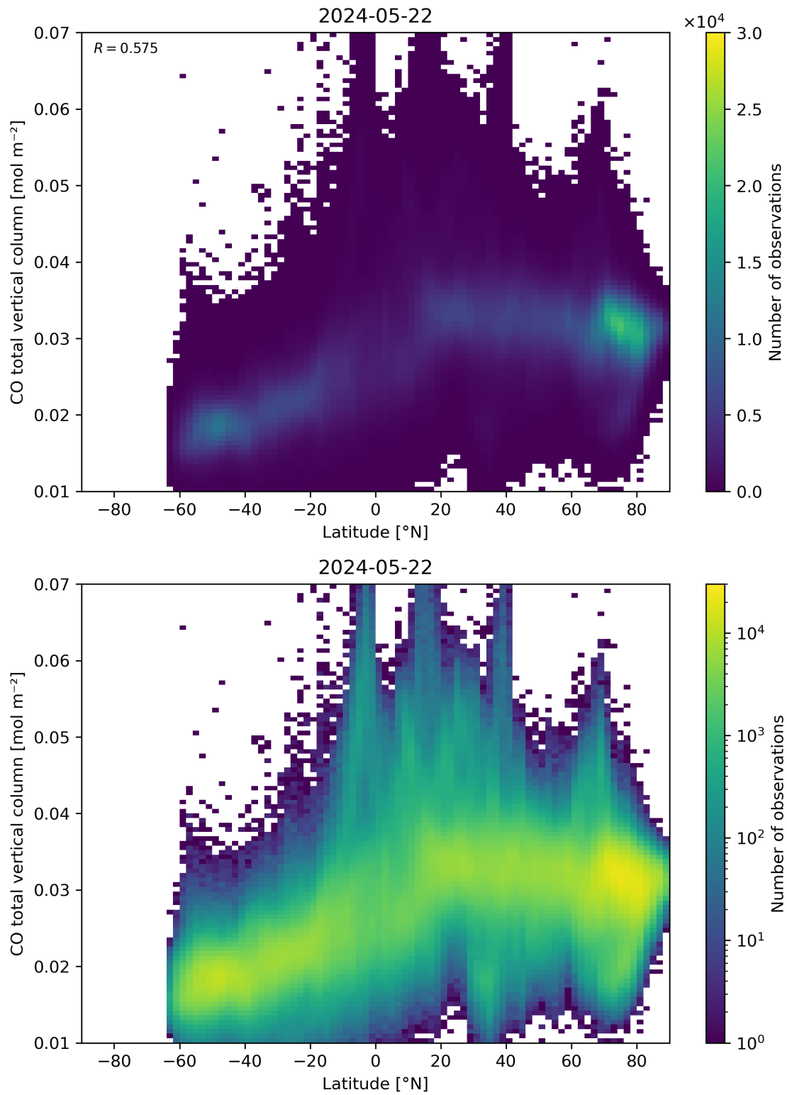
Figure 51: Scatter density plot of “Latitude” against “CO total vertical column” for 2024-05-21 to 2024-05-23.
