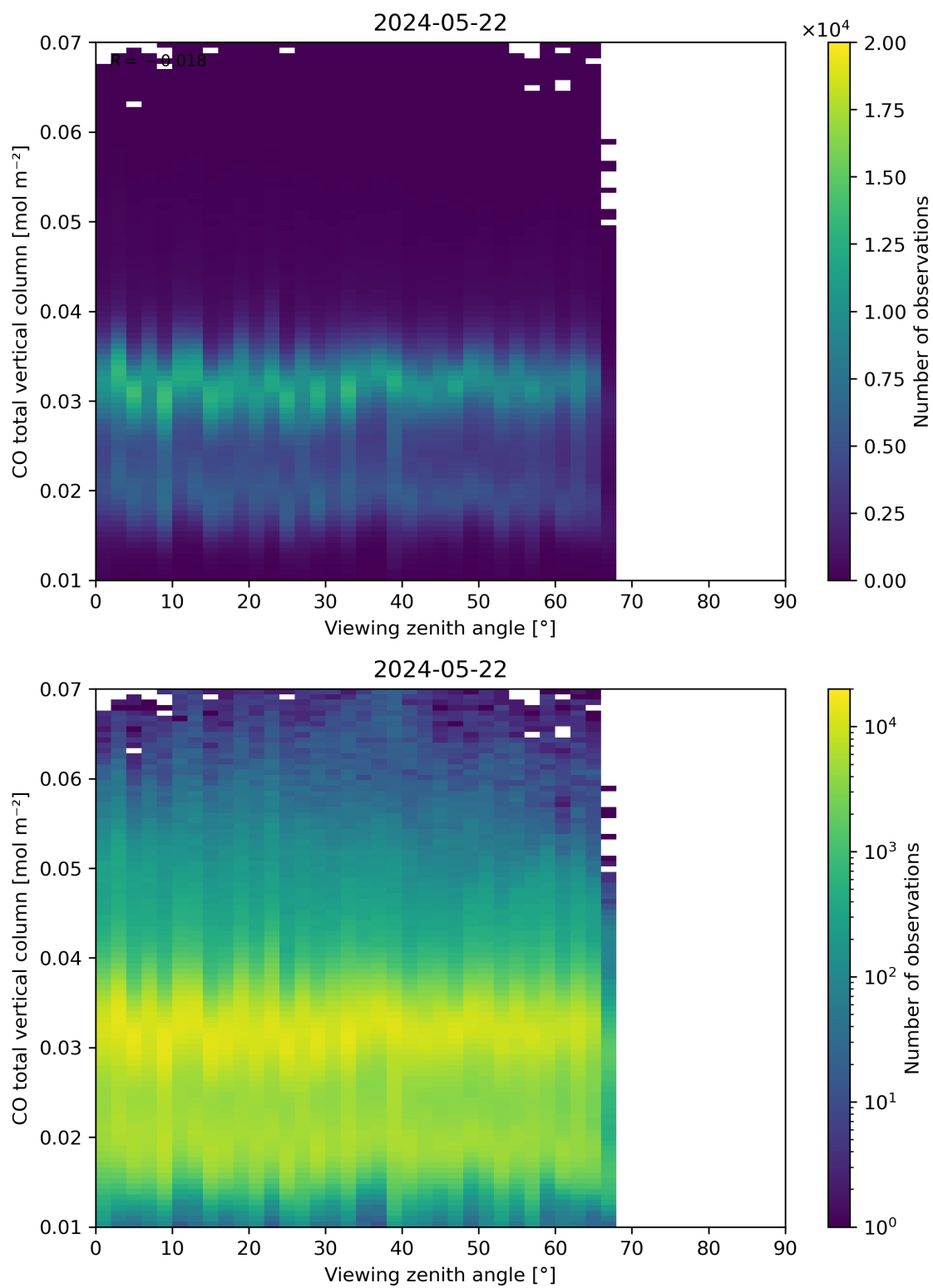
Figure 69: Scatter density plot of “Viewing zenith angle” against “CO total vertical column” for 2024-05-21 to 2024-05-23.
