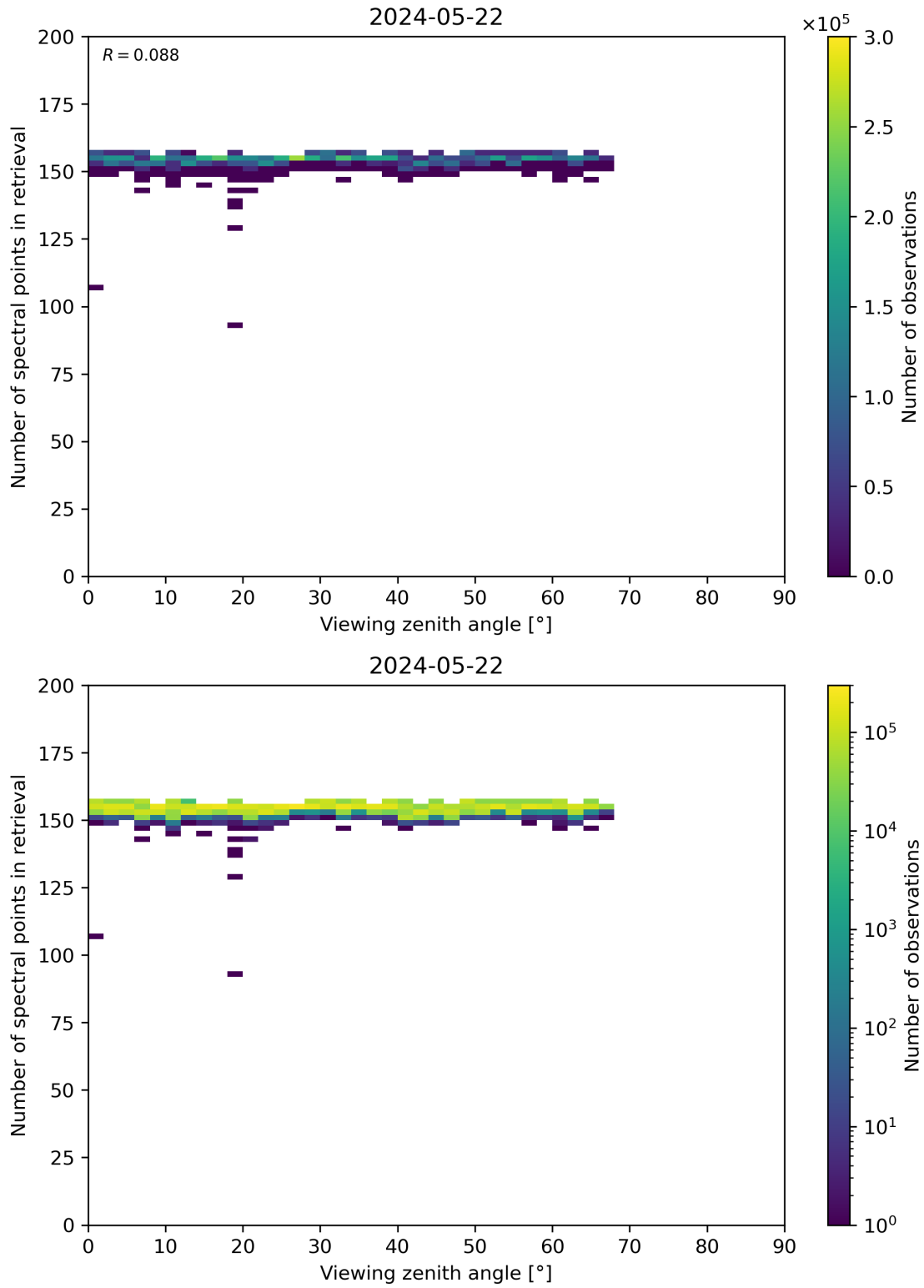
Figure 76: Scatter density plot of “Viewing zenith angle” against “Number of spectral points in retrieval” for 2024-05-21 to 2024-05-23.
