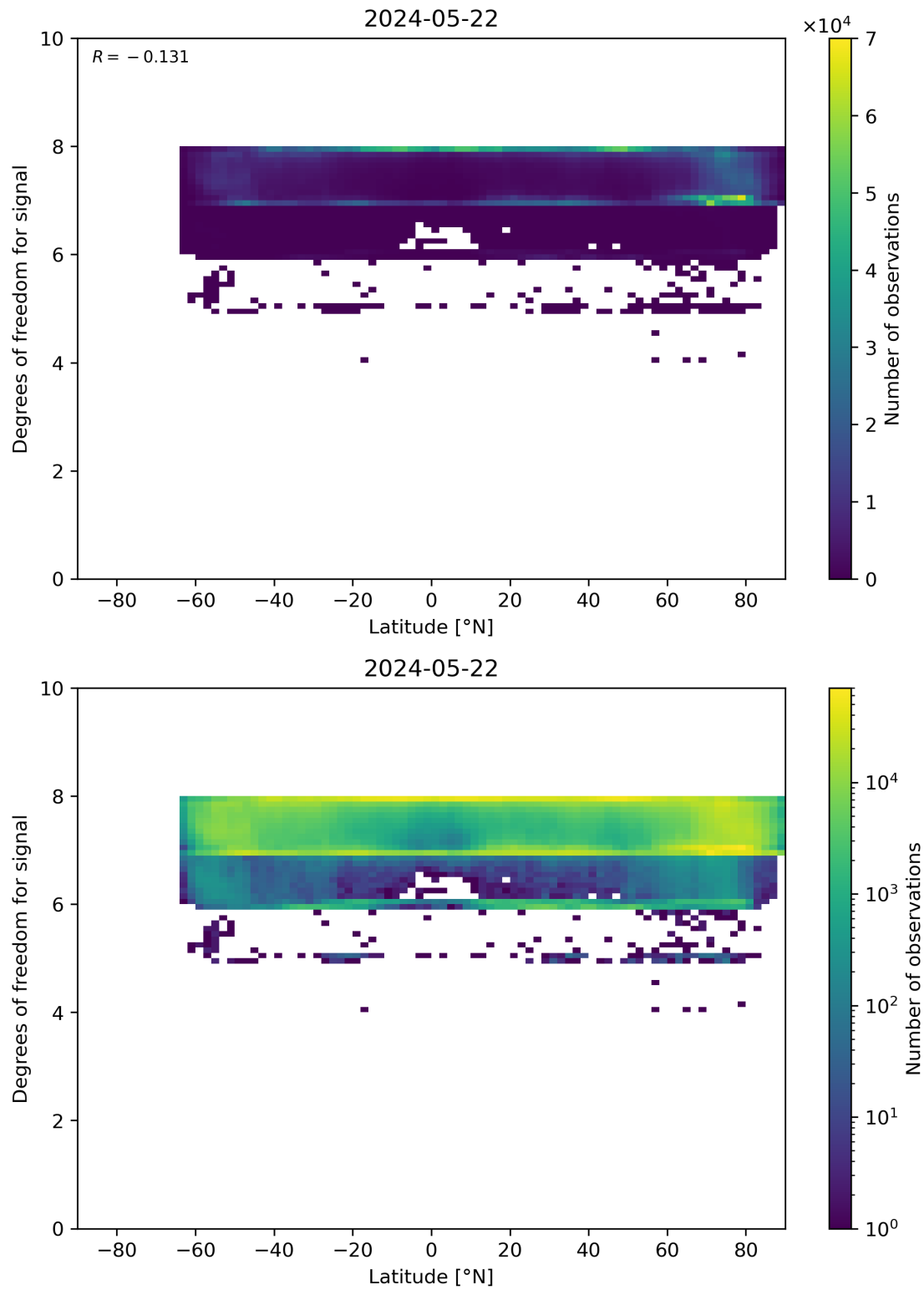
Figure 55: Scatter density plot of “Latitude” against “Degrees of freedom for signal” for 2024-05-21 to 2024-05-23.
