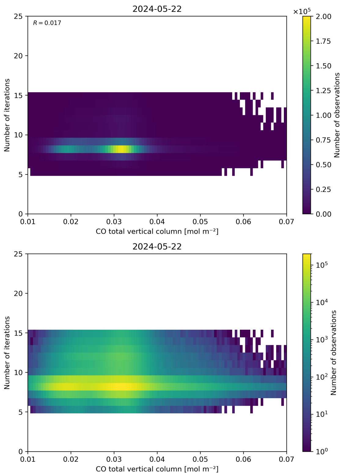
Figure 42: Scatter density plot of “CO total vertical column” against “Number of iterations” for 2024-05-21 to 2024-05-23.
