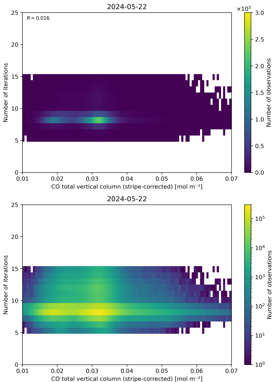
Figure 39: Scatter density plot of “CO total vertical column (stripe-corrected)” against “Number of iterations” for 2024-05-21 to 2024-05-23.
