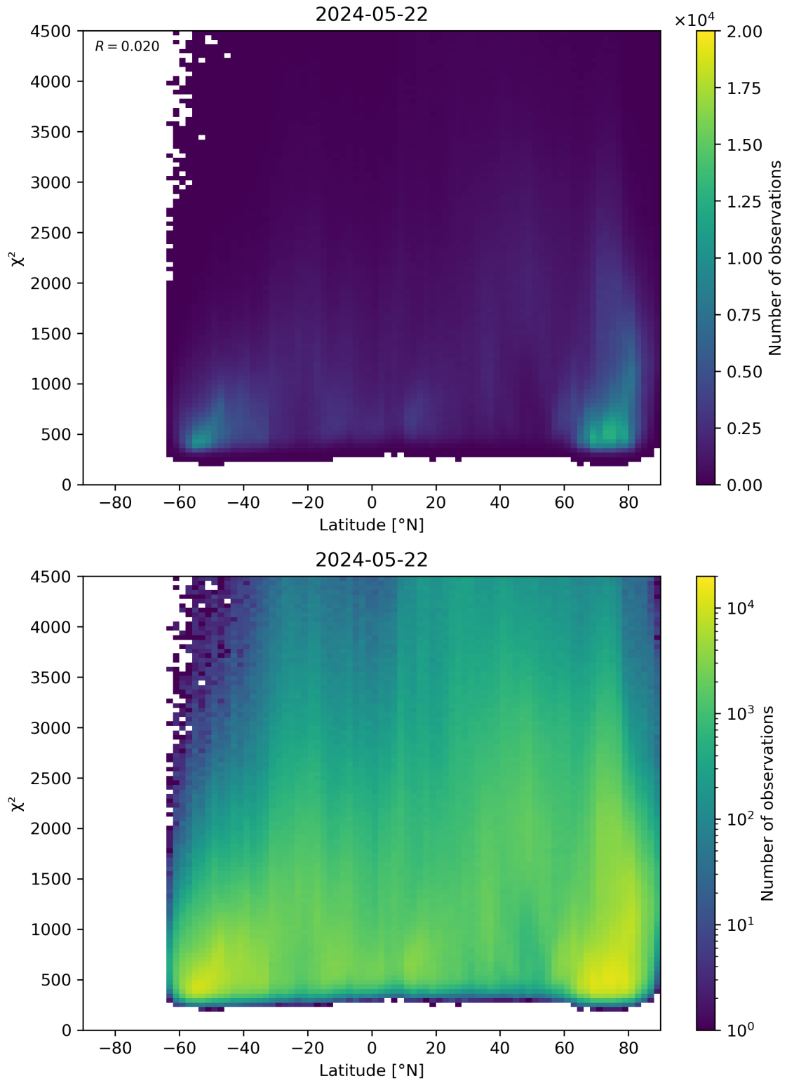
Figure 54: Scatter density plot of “Latitude” against “ \chi^2 ” for 2024-05-21 to 2024-05-23.
