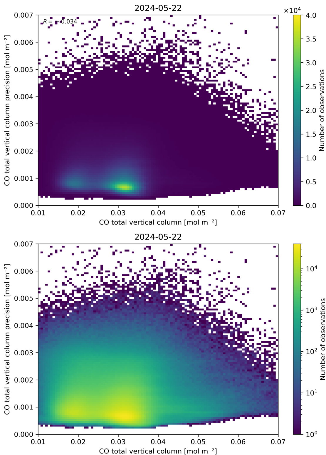
Figure 34: Scatter density plot of “CO total vertical column” against “CO total vertical column precision” for 2024-05-21 to 2024-05-23.
