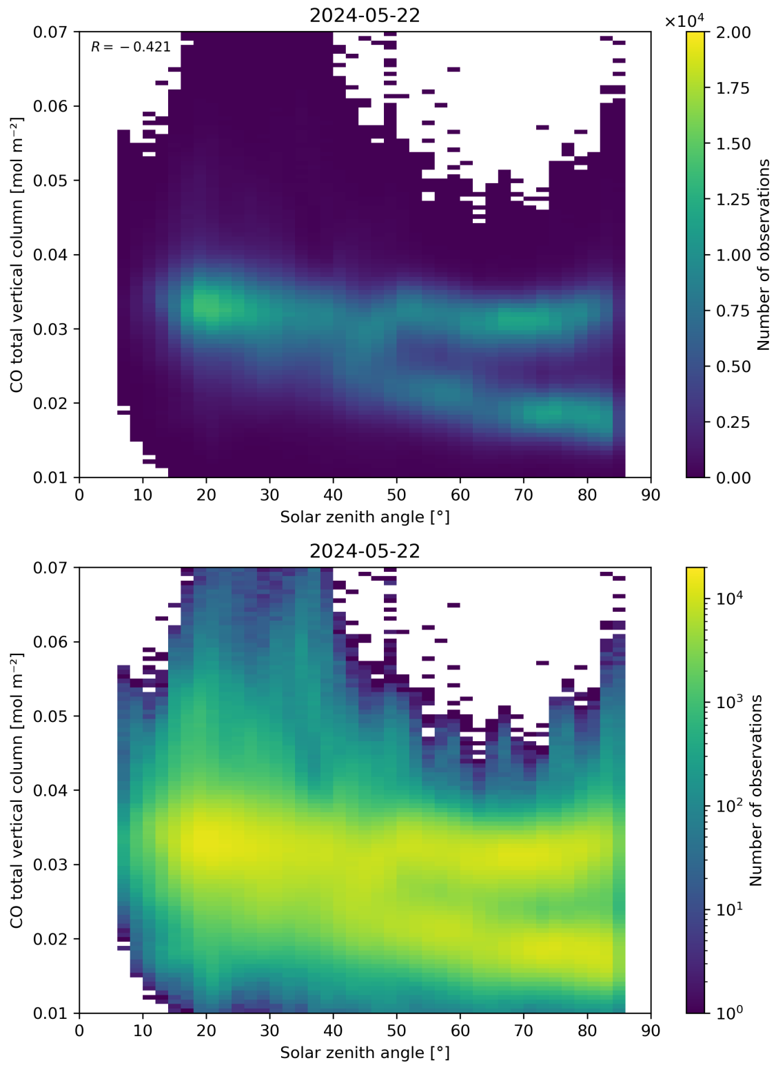
Figure 61: Scatter density plot of “Solar zenith angle” against “CO total vertical column” for 2024-05-21 to 2024-05-23.
