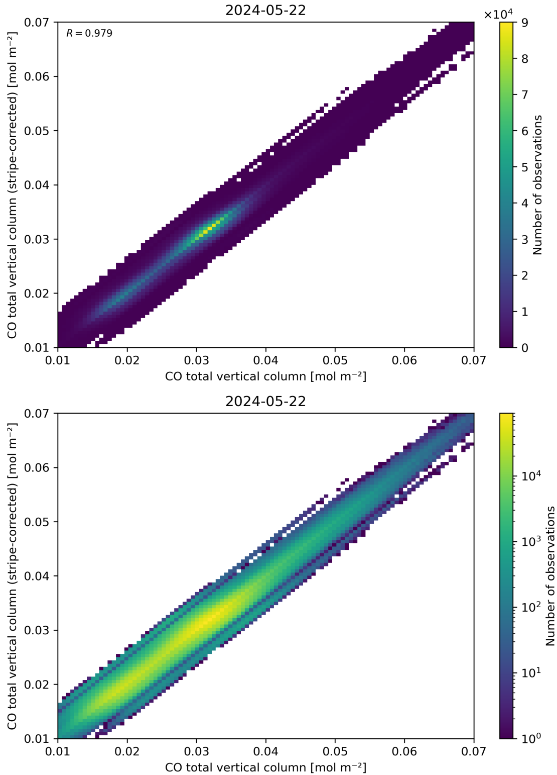
Figure 33: Scatter density plot of “CO total vertical column” against “CO total vertical column (stripe-corrected)” for 2024-05-21 to 2024-05-23.
