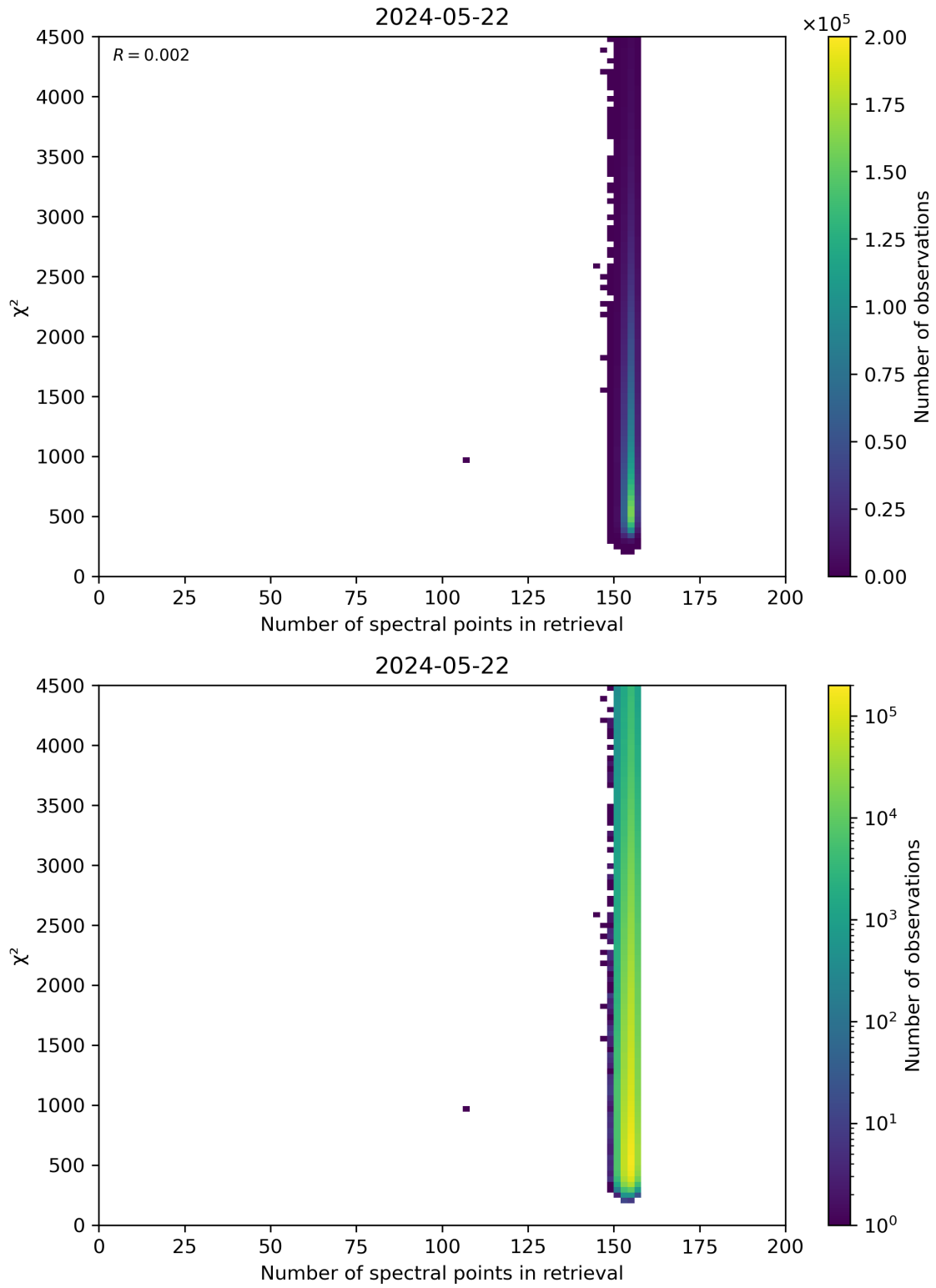
Figure 58: Scatter density plot of “Number of spectral points in retrieval” against “ \chi^2 ” for 2024-05-21 to 2024-05-23.
