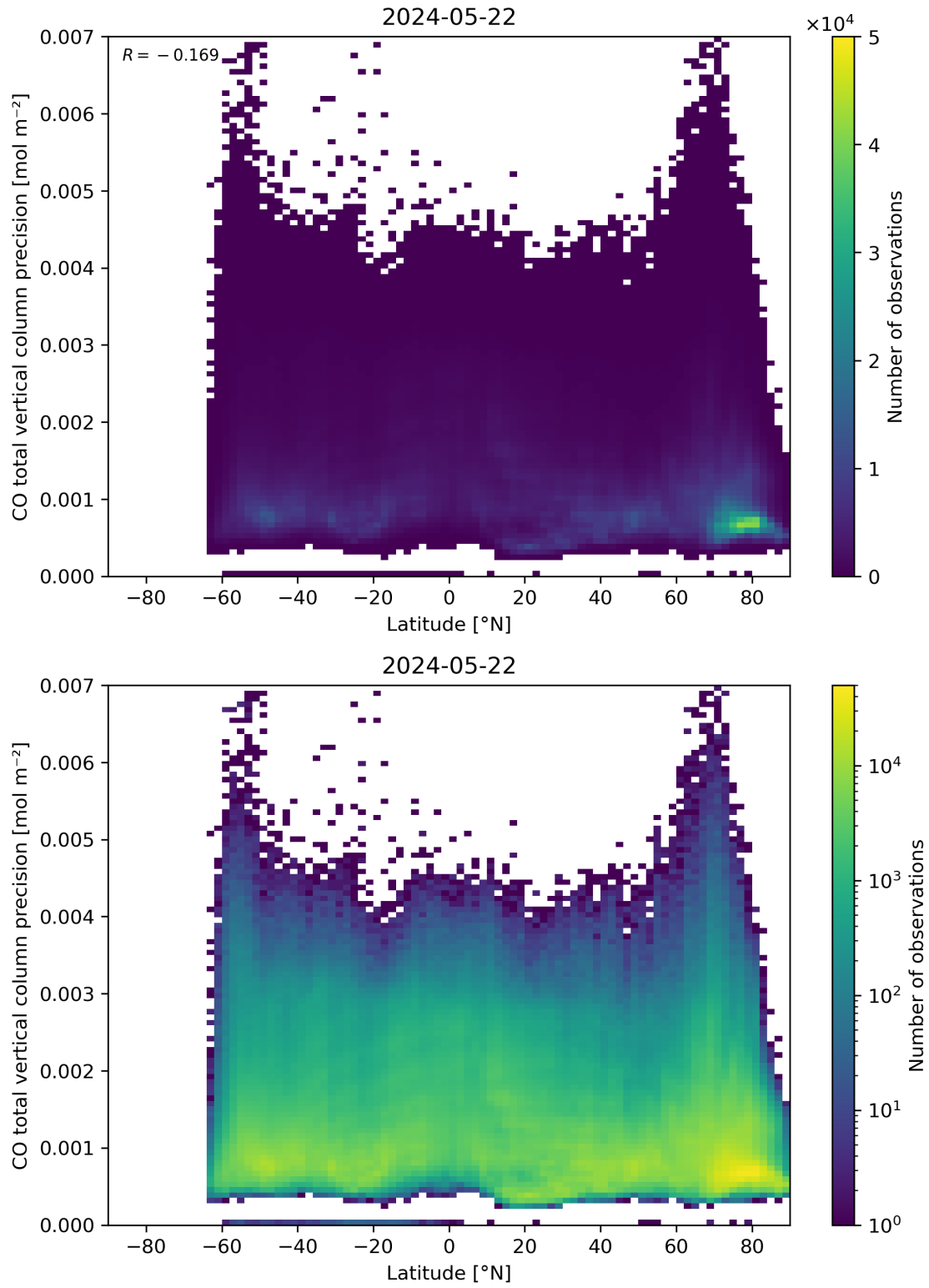
Figure 53: Scatter density plot of “Latitude” against “CO total vertical column precision” for 2024-05-21 to 2024-05-23.
