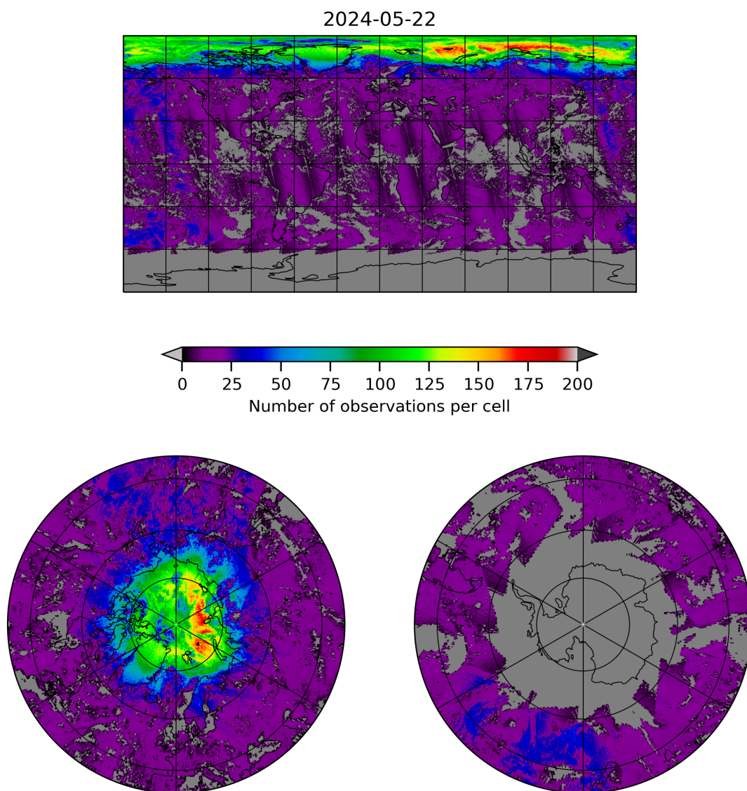
Figure 8: Map of the number of observations for 2024-05-21 to 2024-05-23
