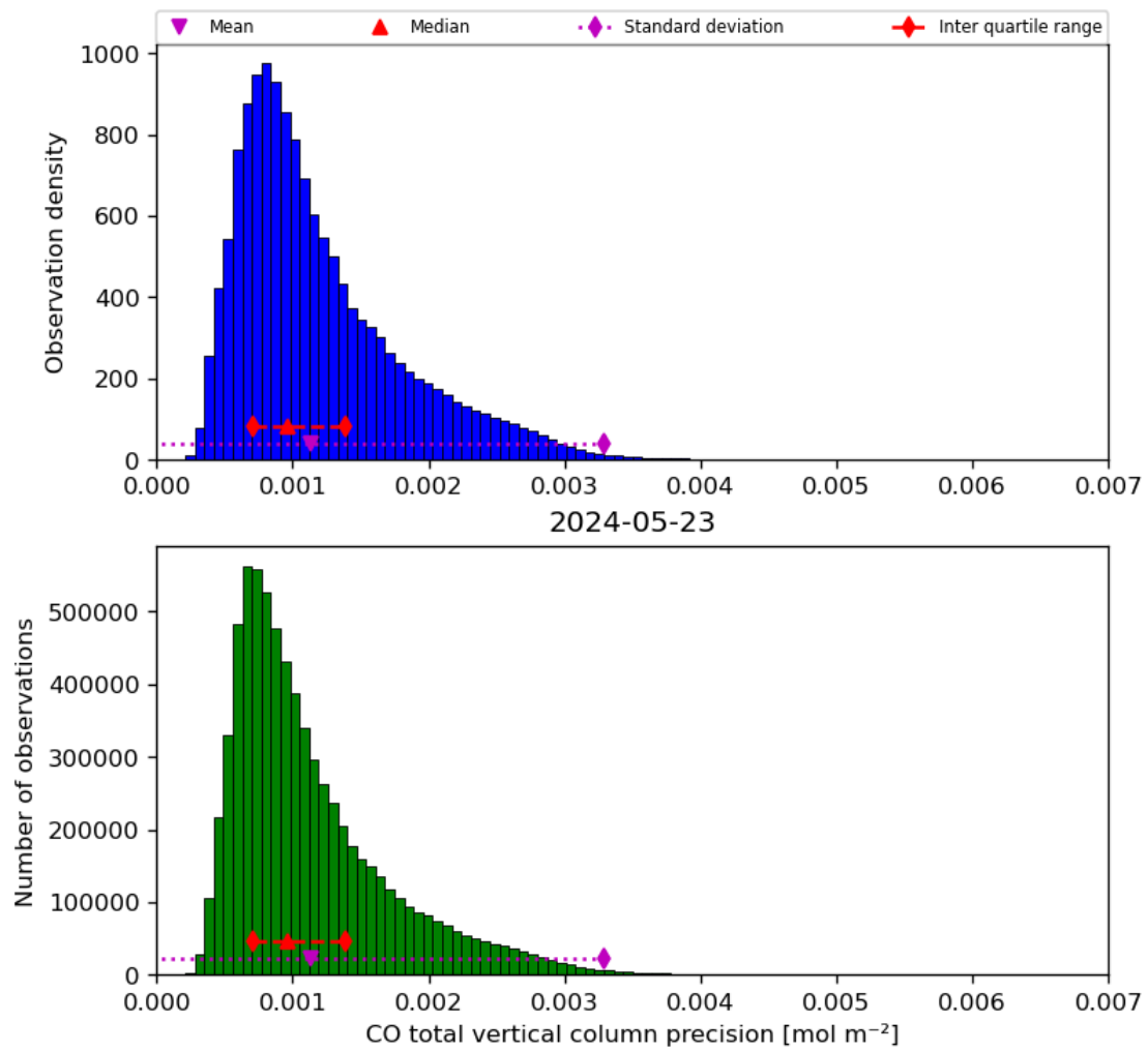
Figure 20: Histogram of “CO total vertical column precision” for 2024-05-23 to 2024-05-24
