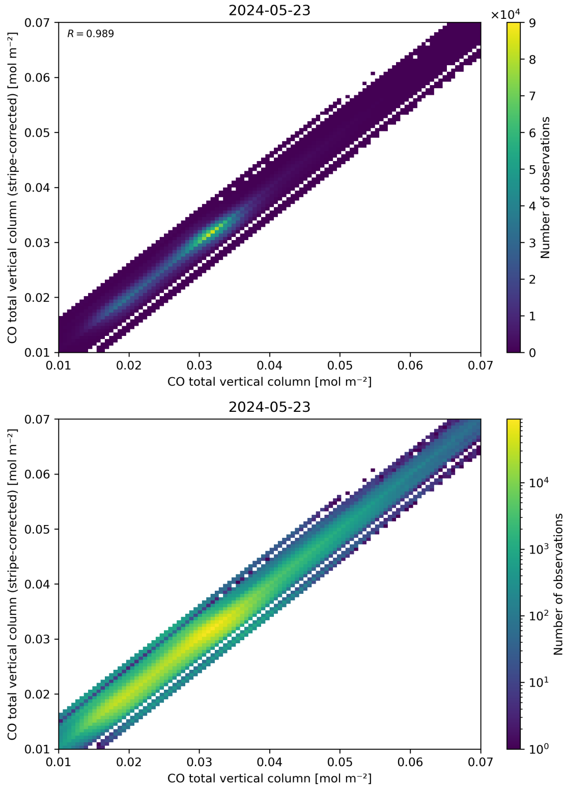
Figure 33: Scatter density plot of “CO total vertical column” against “CO total vertical column (stripe-corrected)” for 2024-05-23 to 2024-05-24.
