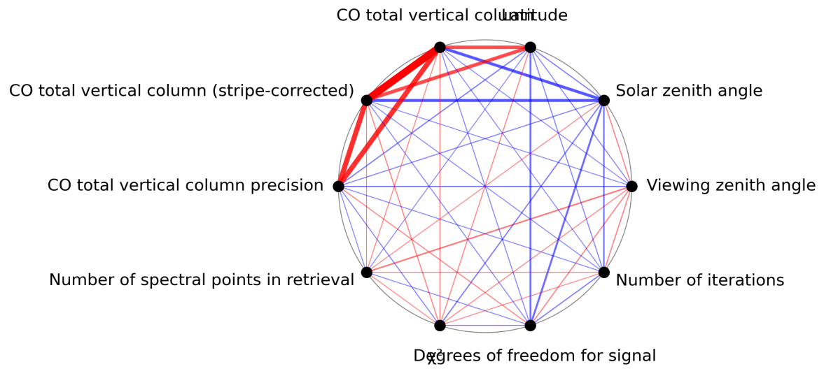
Figure 1: Map of correlation graph for 2024-05-23 to 2024-05-24.
