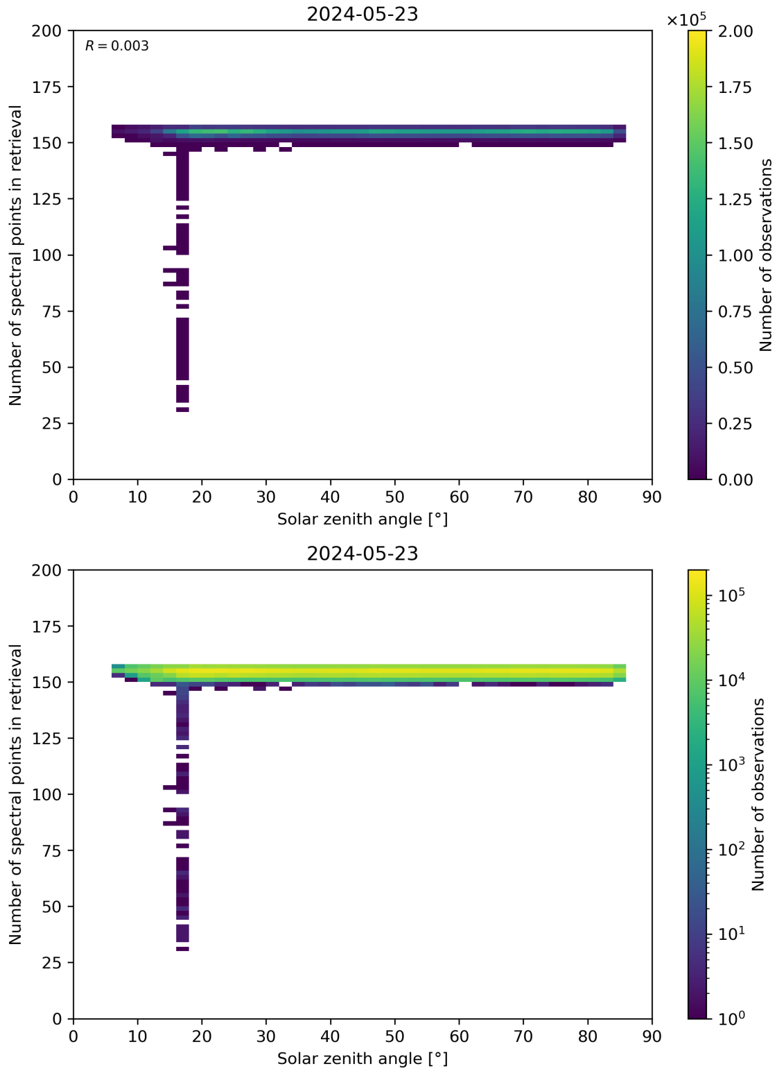
Figure 68: Scatter density plot of “Solar zenith angle” against “Number of spectral points in retrieval” for 2024-05-23 to 2024-05-24.
