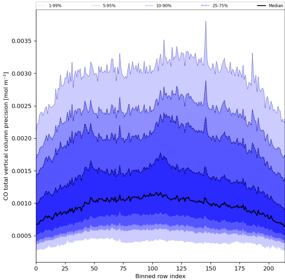
Figure 28: Along track statistics of “CO total vertical column precision” for 2024-05-23 to 2024-05-24
