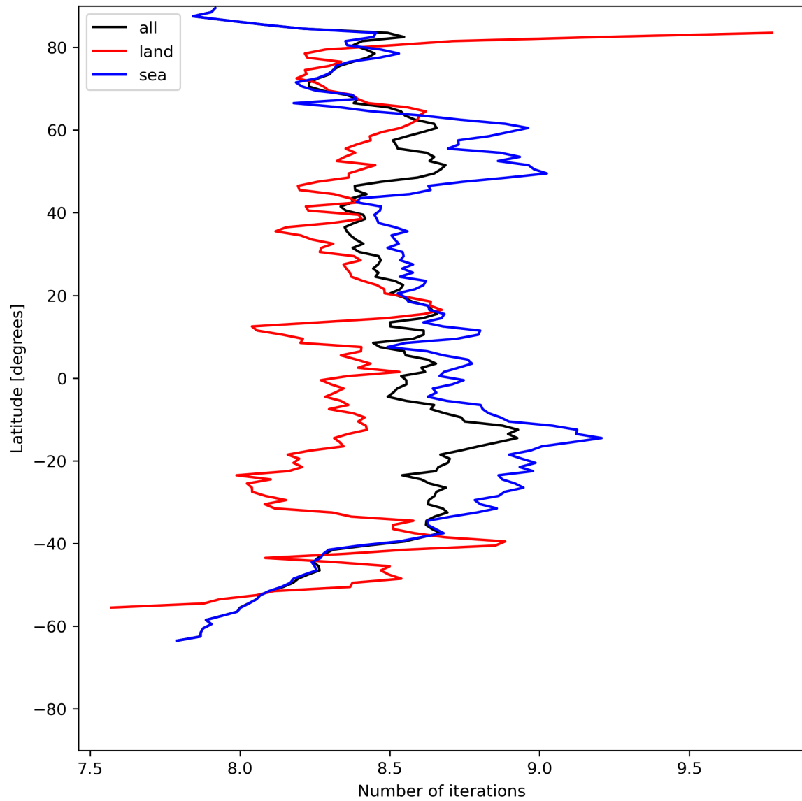
Figure 16: Zonal average of “Number of iterations” for 2024-05-23 to 2024-05-24.
