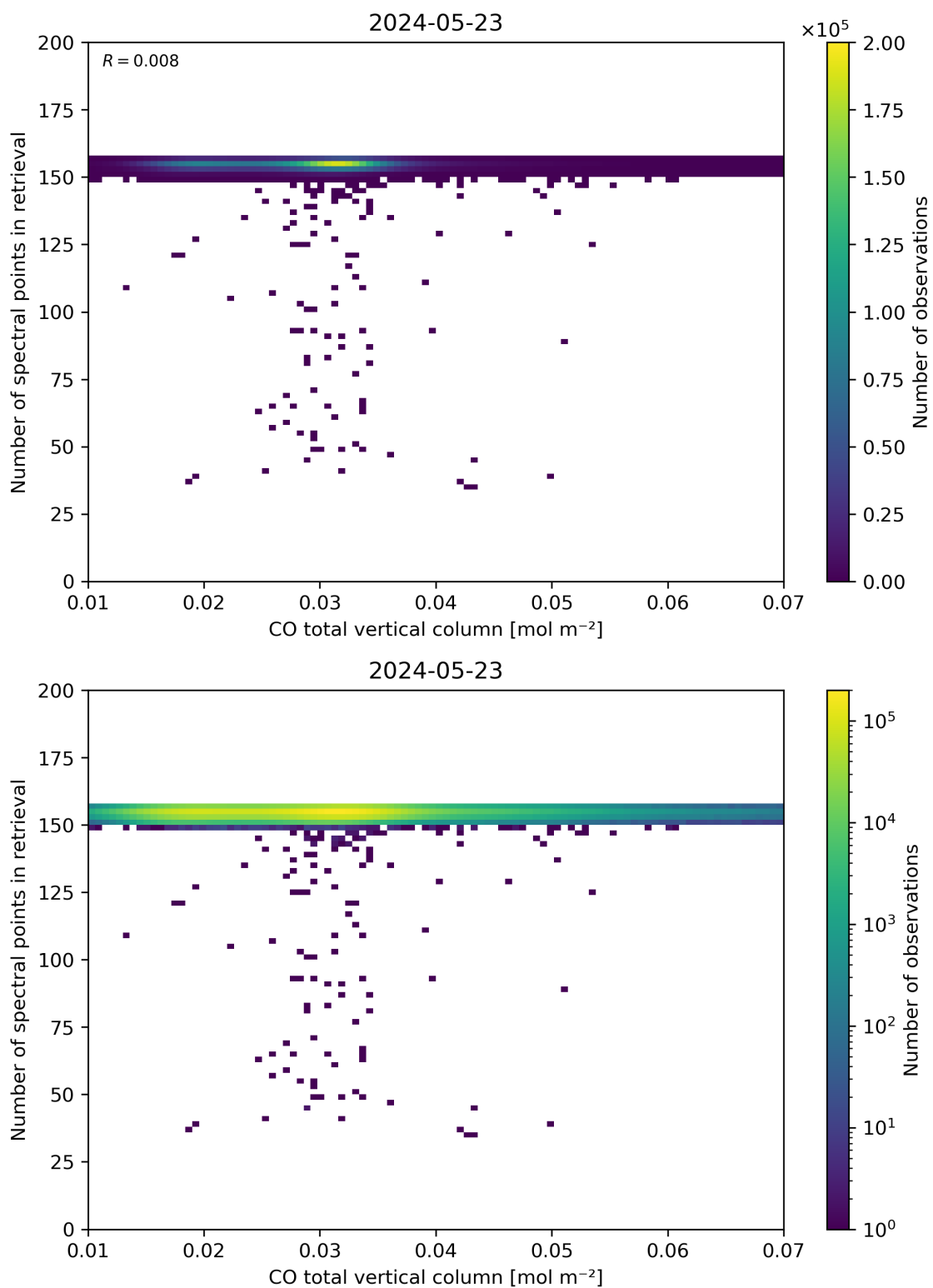
Figure 43: Scatter density plot of “CO total vertical column” against “Number of spectral points in retrieval” for 2024-05-23 to 2024-05-24.
