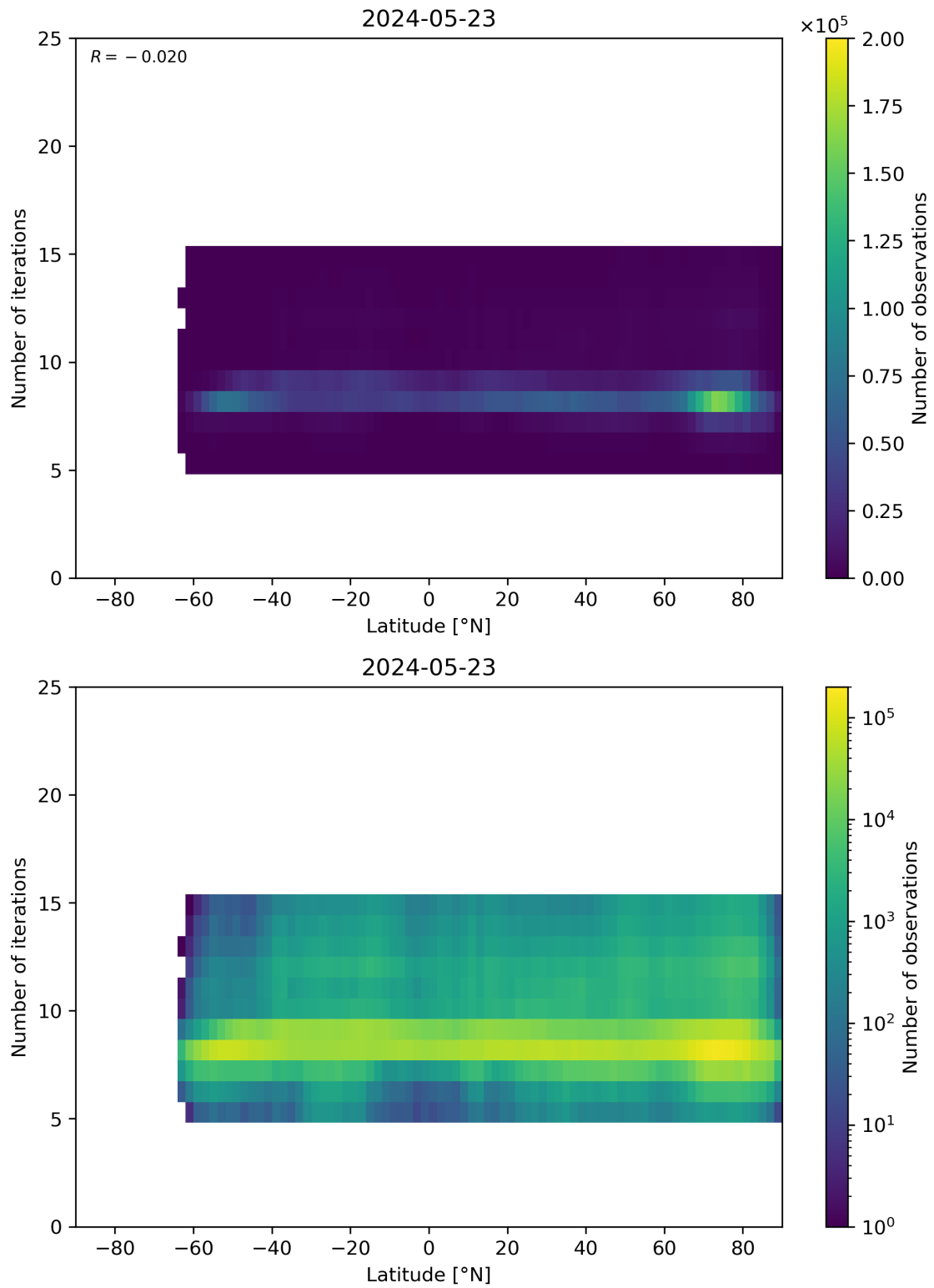
Figure 56: Scatter density plot of “Latitude” against “Number of iterations” for 2024-05-23 to 2024-05-24.
