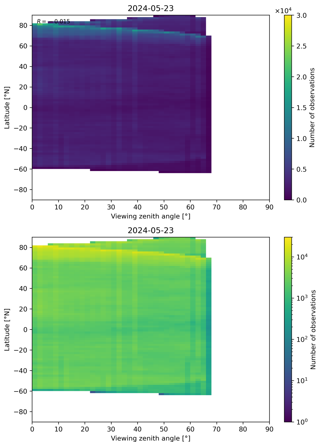
Figure 74: Scatter density plot of “Viewing zenith angle” against “Latitude” for 2024-05-23 to 2024-05-24.
