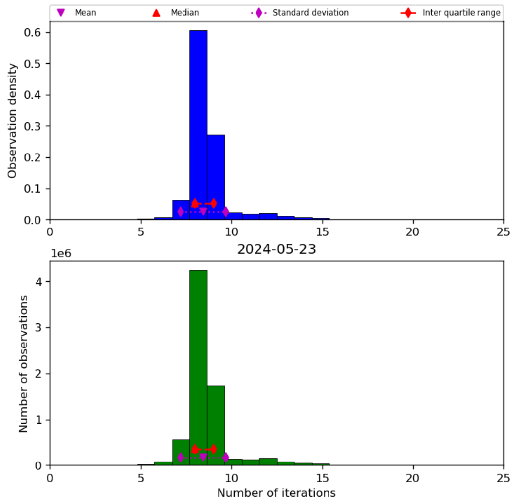
Figure 24: Histogram of “Number of iterations” for 2024-05-23 to 2024-05-24
