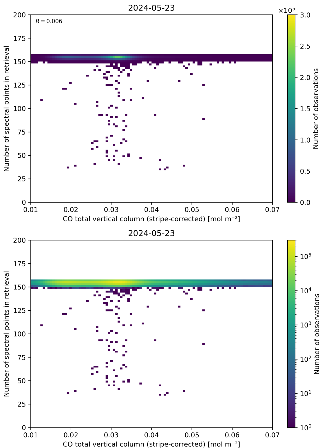
Figure 40: Scatter density plot of “CO total vertical column (stripe-corrected)” against “Number of spectral points in retrieval” for 2024-05-23 to 2024-05-24.
