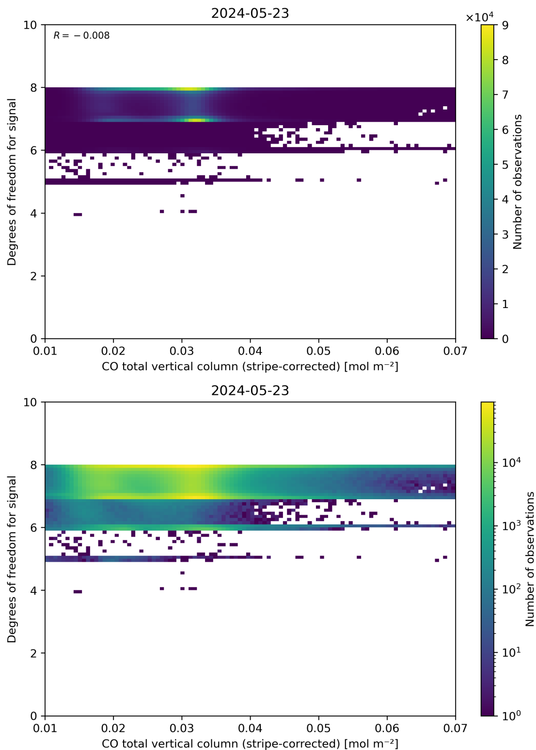
Figure 38: Scatter density plot of “CO total vertical column (stripe-corrected)” against “Degrees of freedom for signal” for 2024-05-23 to 2024-05-24.
