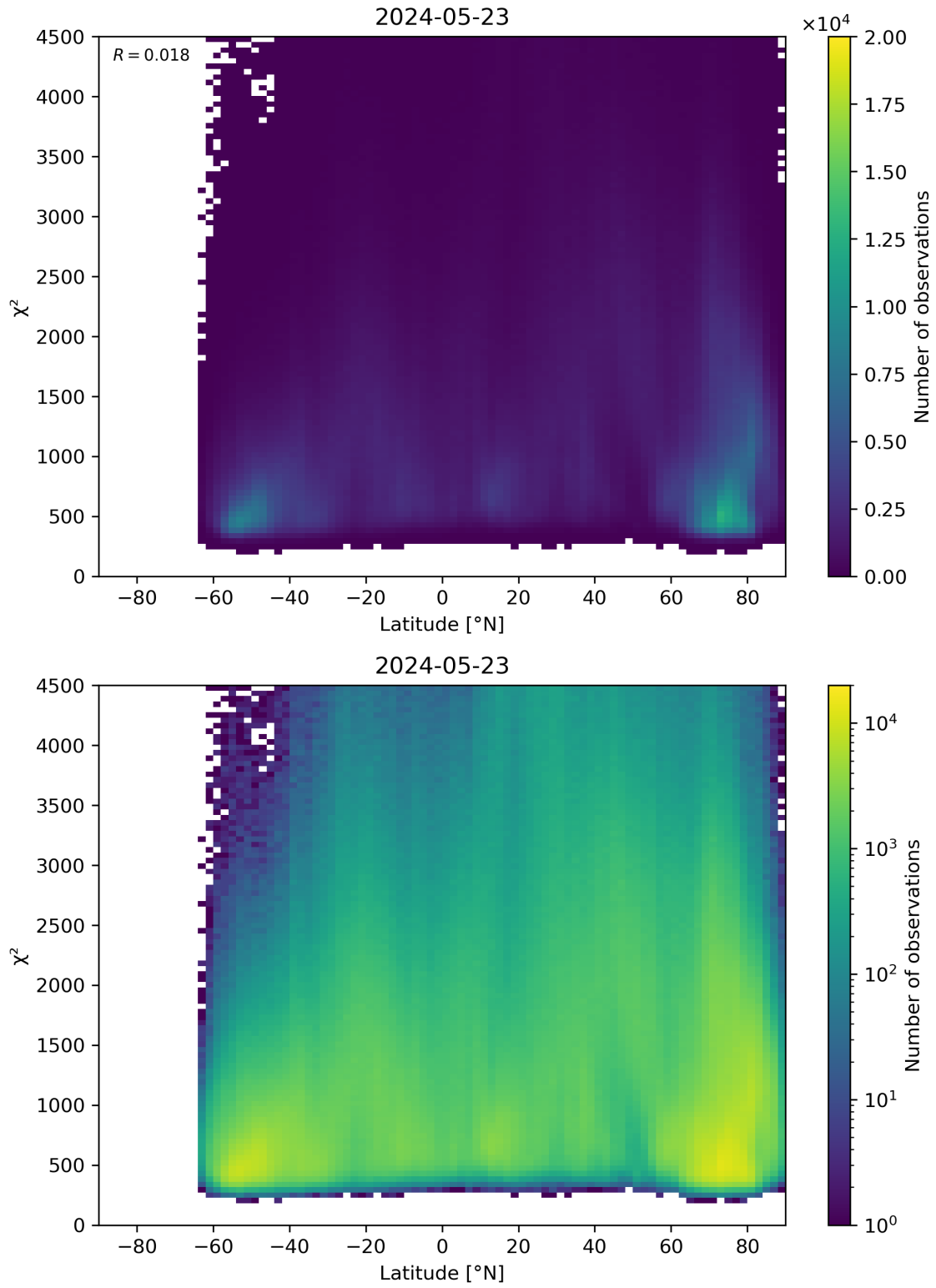
Figure 54: Scatter density plot of “Latitude” against “ \chi^2 ” for 2024-05-23 to 2024-05-24.
