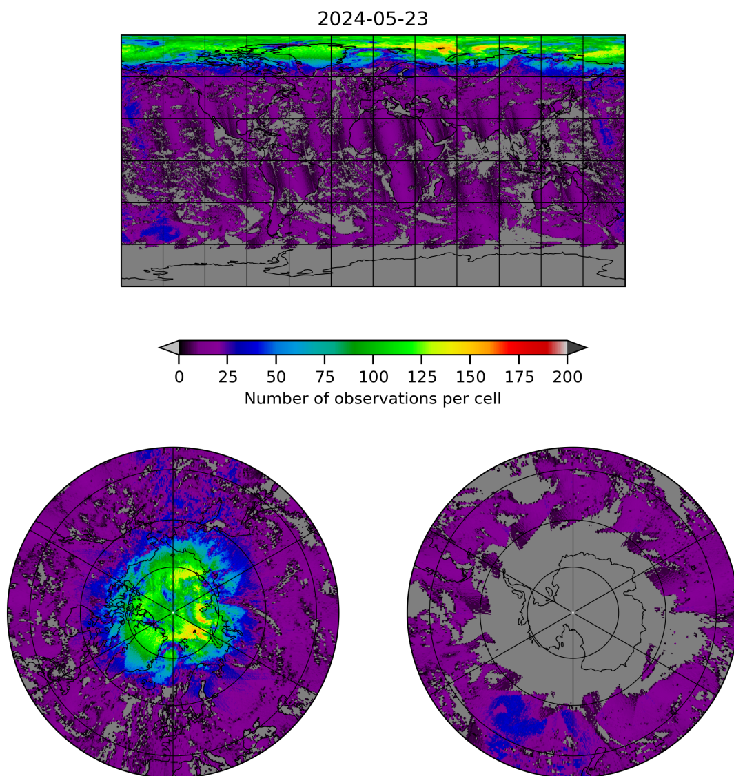
Figure 8: Map of the number of observations for 2024-05-23 to 2024-05-24
