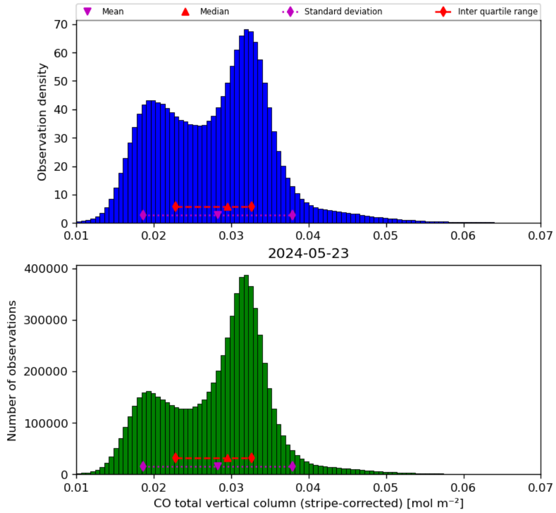
Figure 19: Histogram of “CO total vertical column (stripe-corrected)” for 2024-05-23 to 2024-05-24
