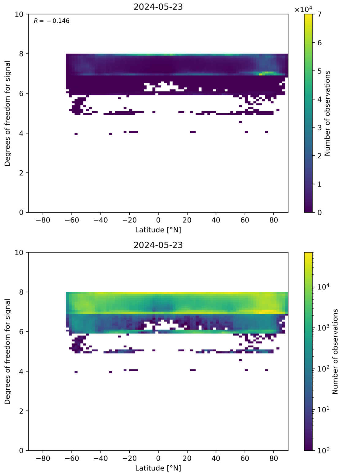
Figure 55: Scatter density plot of “Latitude” against “Degrees of freedom for signal” for 2024-05-23 to 2024-05-24.
