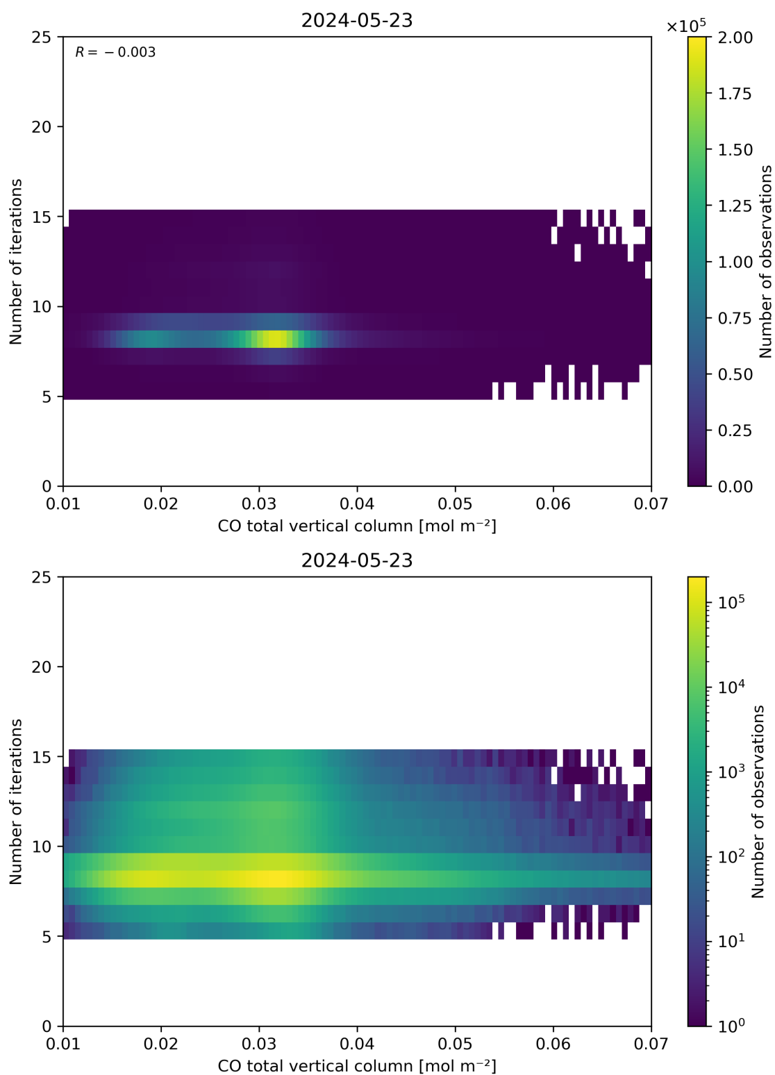
Figure 42: Scatter density plot of “CO total vertical column” against “Number of iterations” for 2024-05-23 to 2024-05-24.
