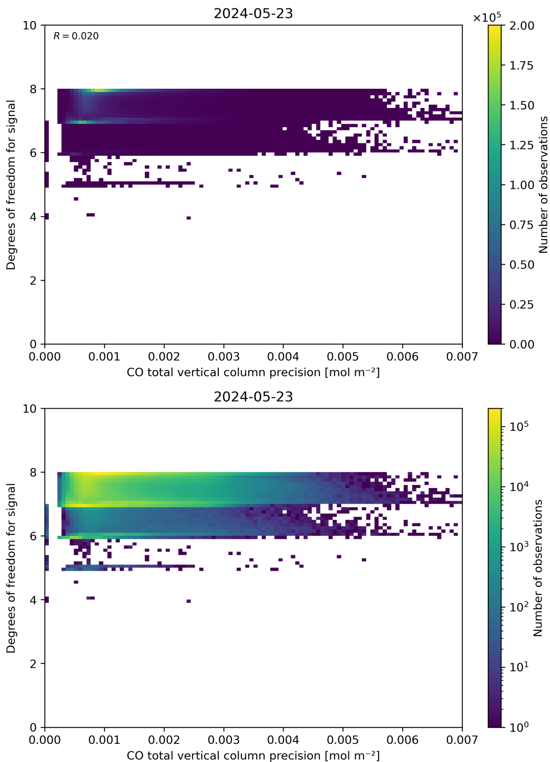
Figure 45: Scatter density plot of “CO total vertical column precision” against “Degrees of freedom for signal” for 2024-05-23 to 2024-05-24.
