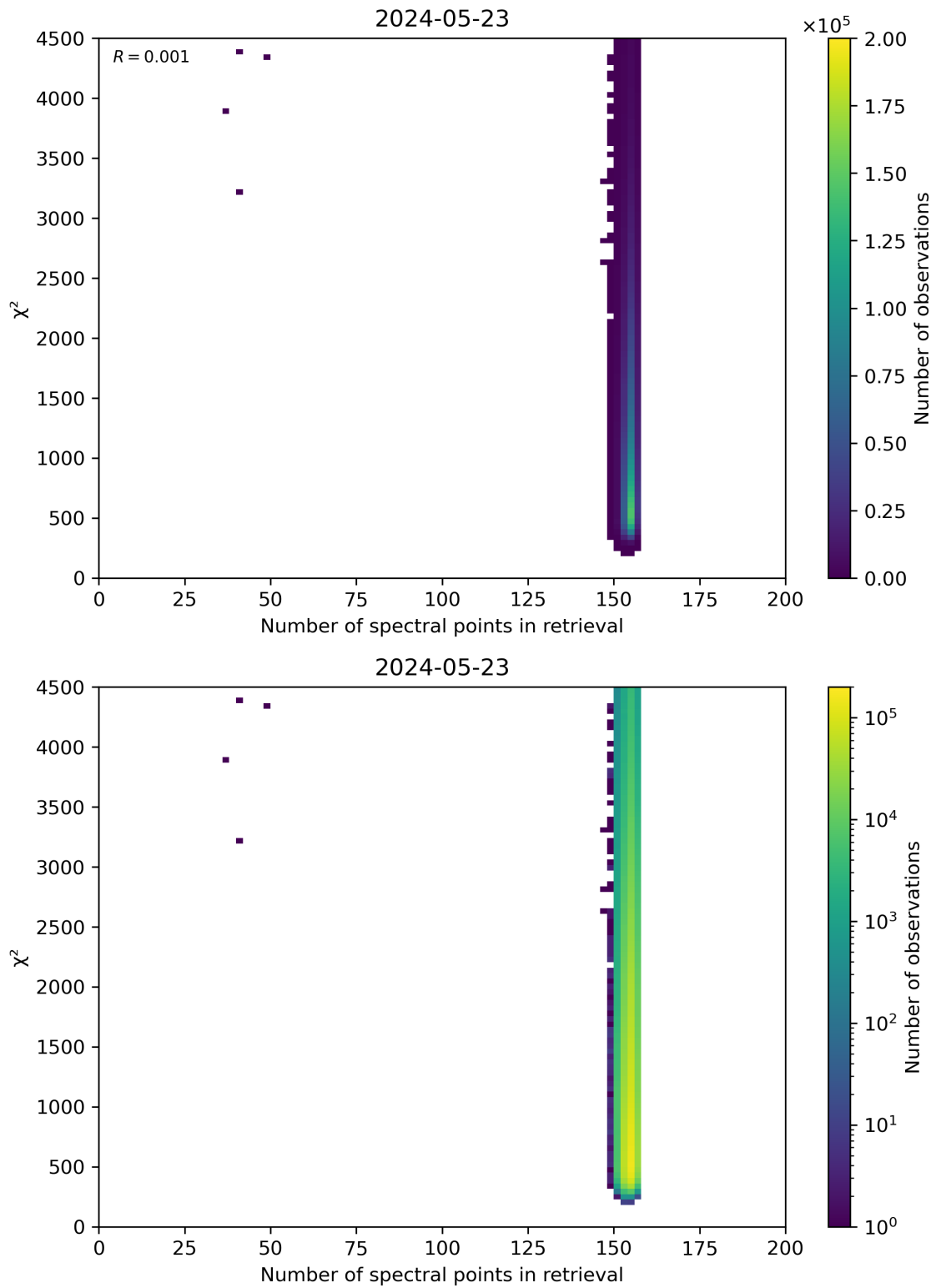
Figure 58: Scatter density plot of “Number of spectral points in retrieval” against “ \chi^2 ” for 2024-05-23 to 2024-05-24.
