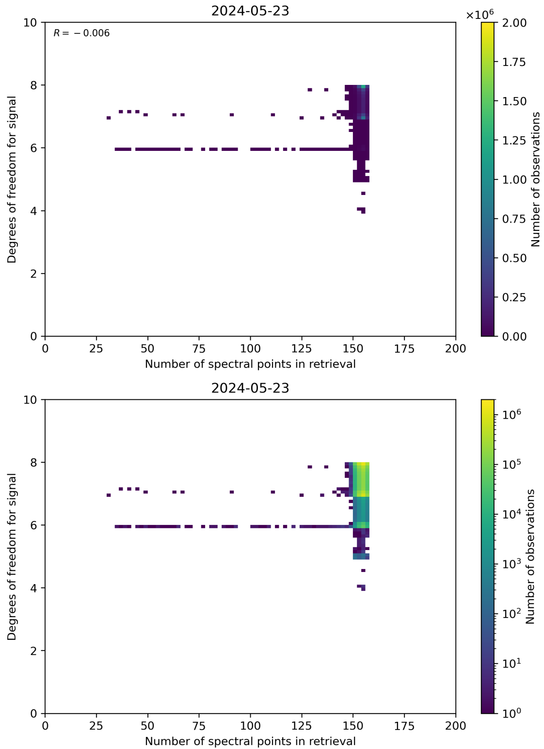
Figure 59: Scatter density plot of “Number of spectral points in retrieval” against “Degrees of freedom for signal” for 2024-05-23 to 2024-05-24.
