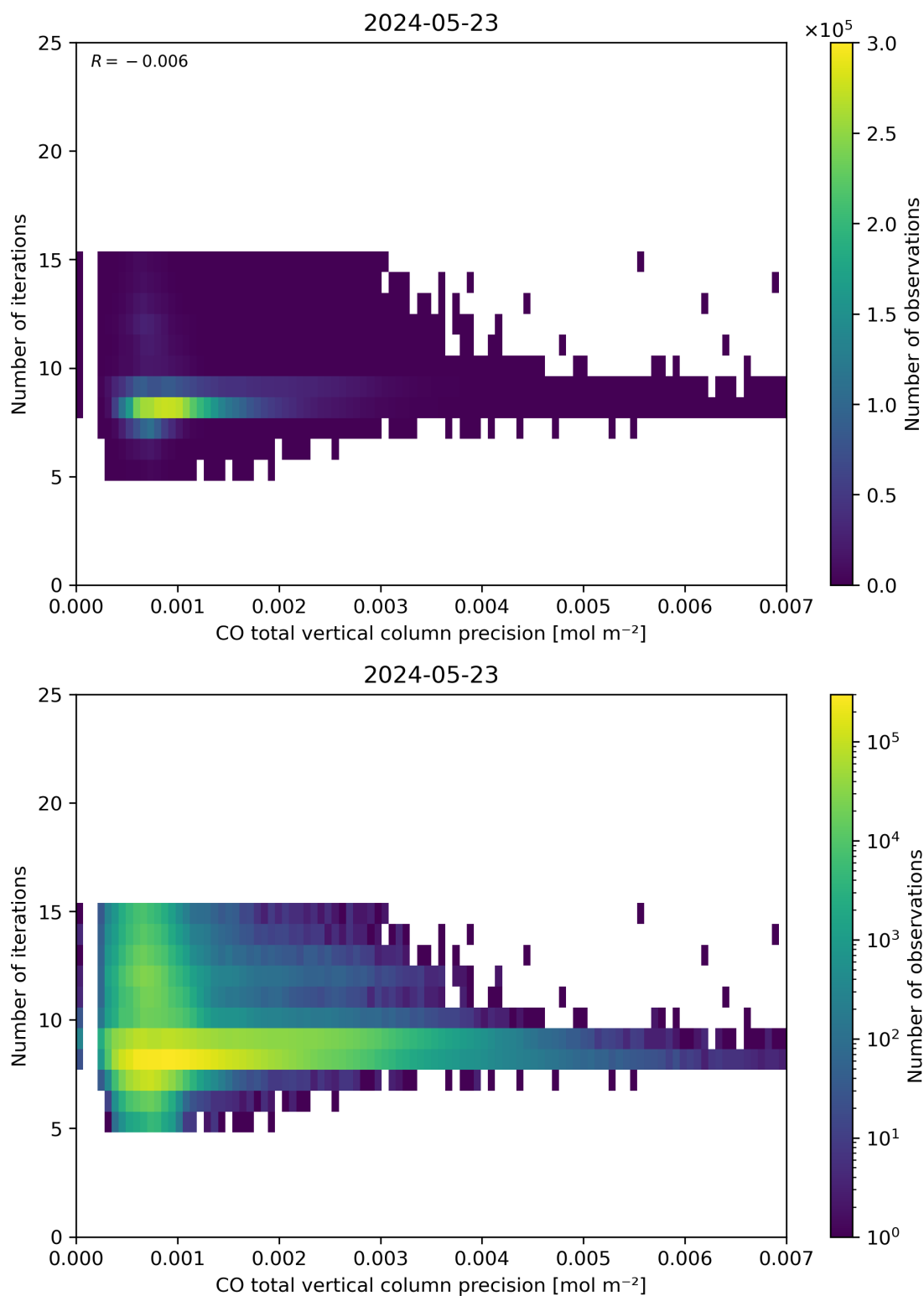
Figure 46: Scatter density plot of “CO total vertical column precision” against “Number of iterations” for 2024-05-23 to 2024-05-24.
