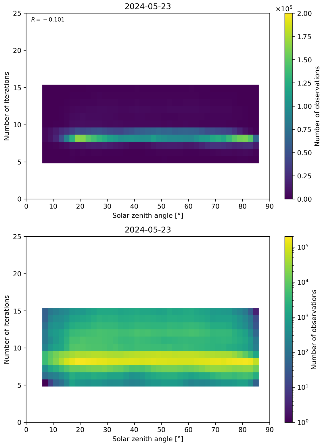
Figure 67: Scatter density plot of “Solar zenith angle” against “Number of iterations” for 2024-05-23 to 2024-05-24.
