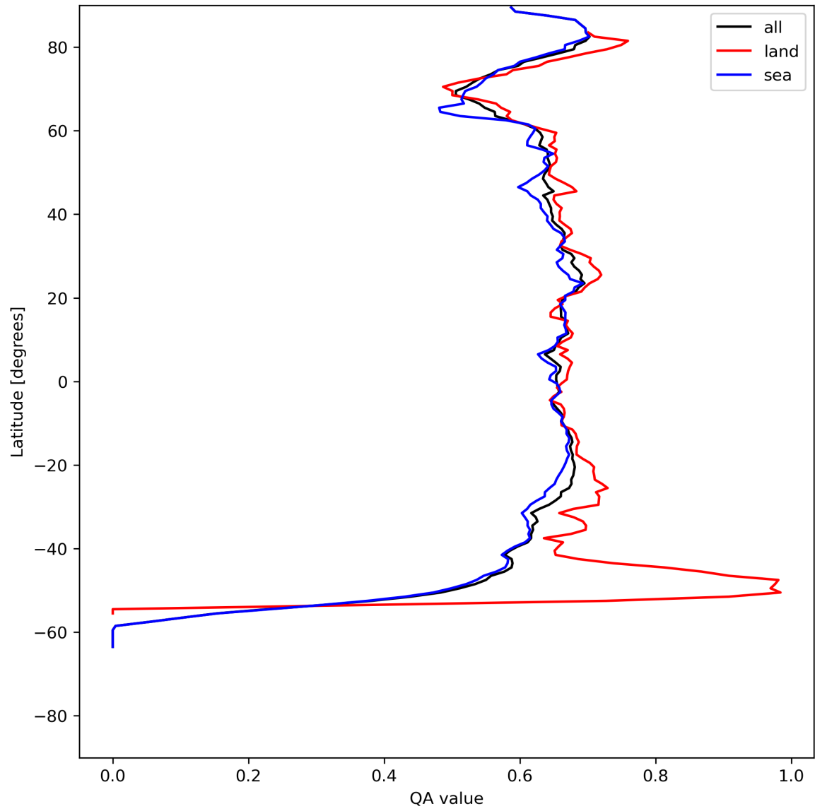
Figure 9: Zonal average of “QA value” for 2024-05-23 to 2024-05-24.
