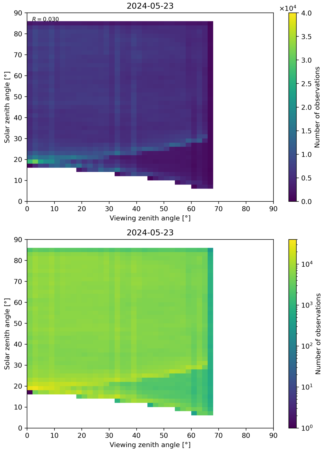
Figure 77: Scatter density plot of “Viewing zenith angle” against “Solar zenith angle” for 2024-05-23 to 2024-05-24.
