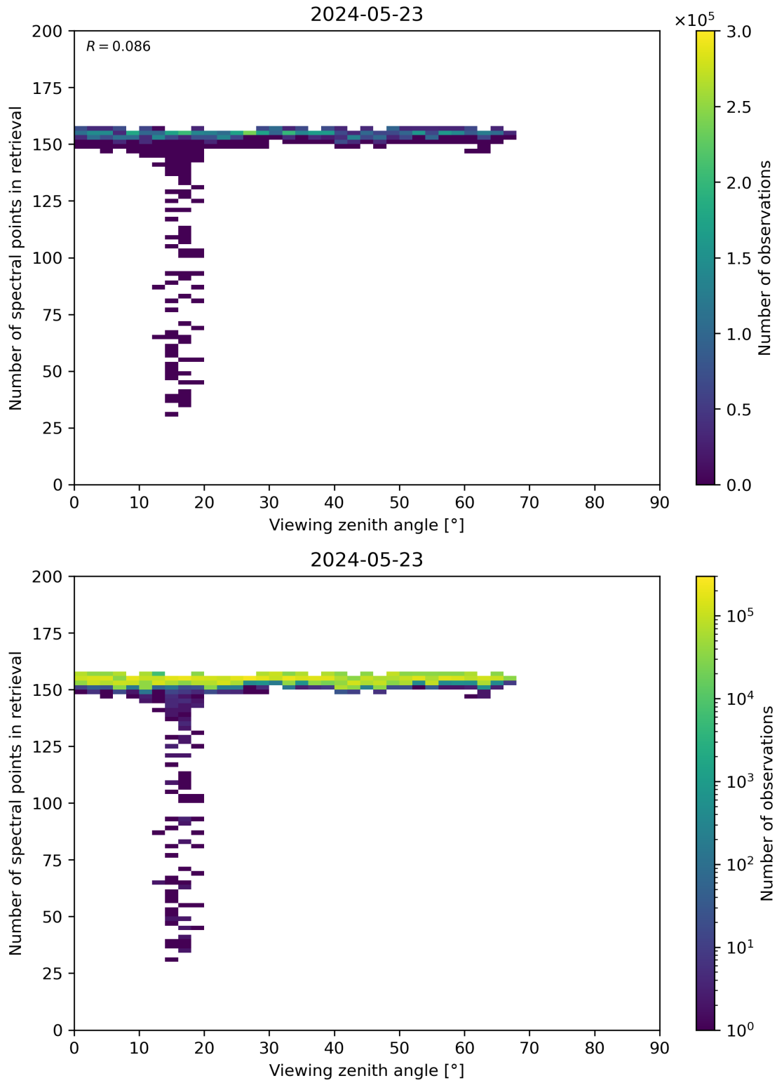
Figure 76: Scatter density plot of “Viewing zenith angle” against “Number of spectral points in retrieval” for 2024-05-23 to 2024-05-24.
