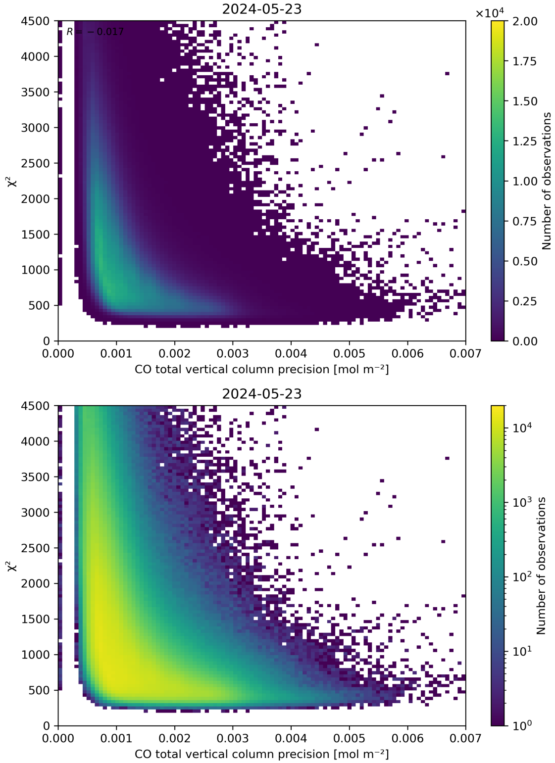
Figure 44: Scatter density plot of “CO total vertical column precision” against “ \chi^2 ” for 2024-05-23 to 2024-05-24.
