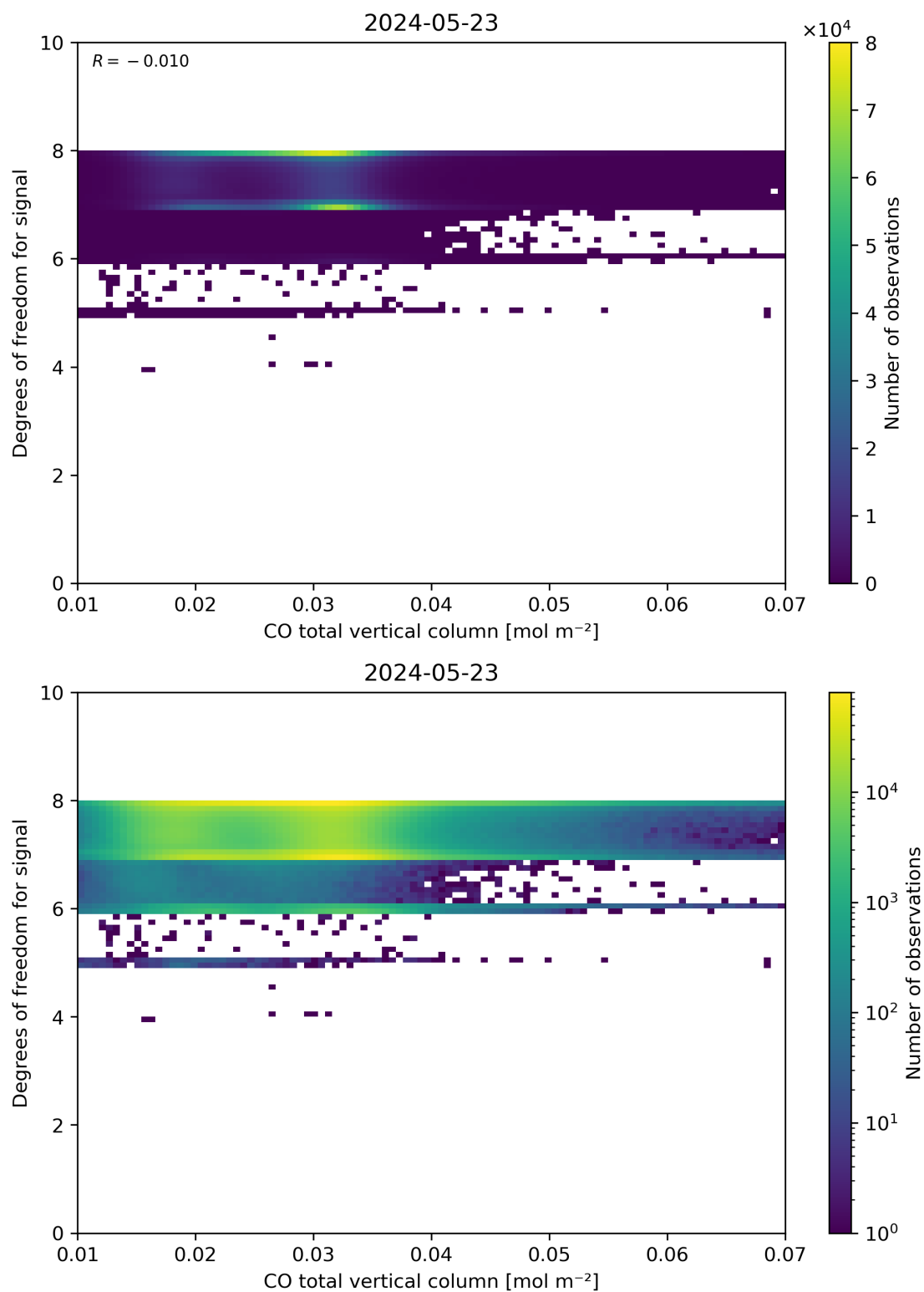
Figure 41: Scatter density plot of “CO total vertical column” against “Degrees of freedom for signal” for 2024-05-23 to 2024-05-24.
