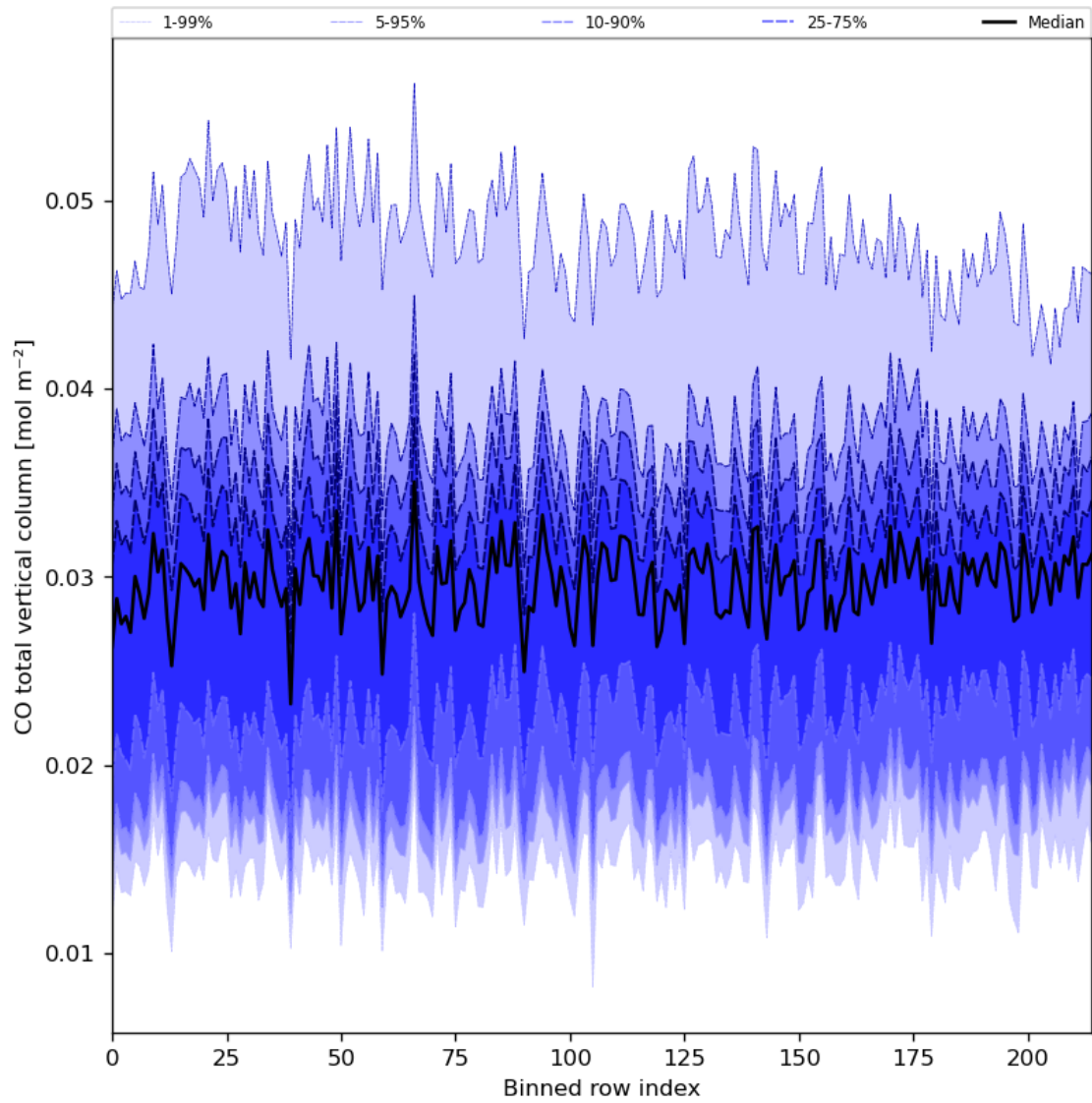
Figure 26: Along track statistics of “CO total vertical column” for 2024-05-23 to 2024-05-24
