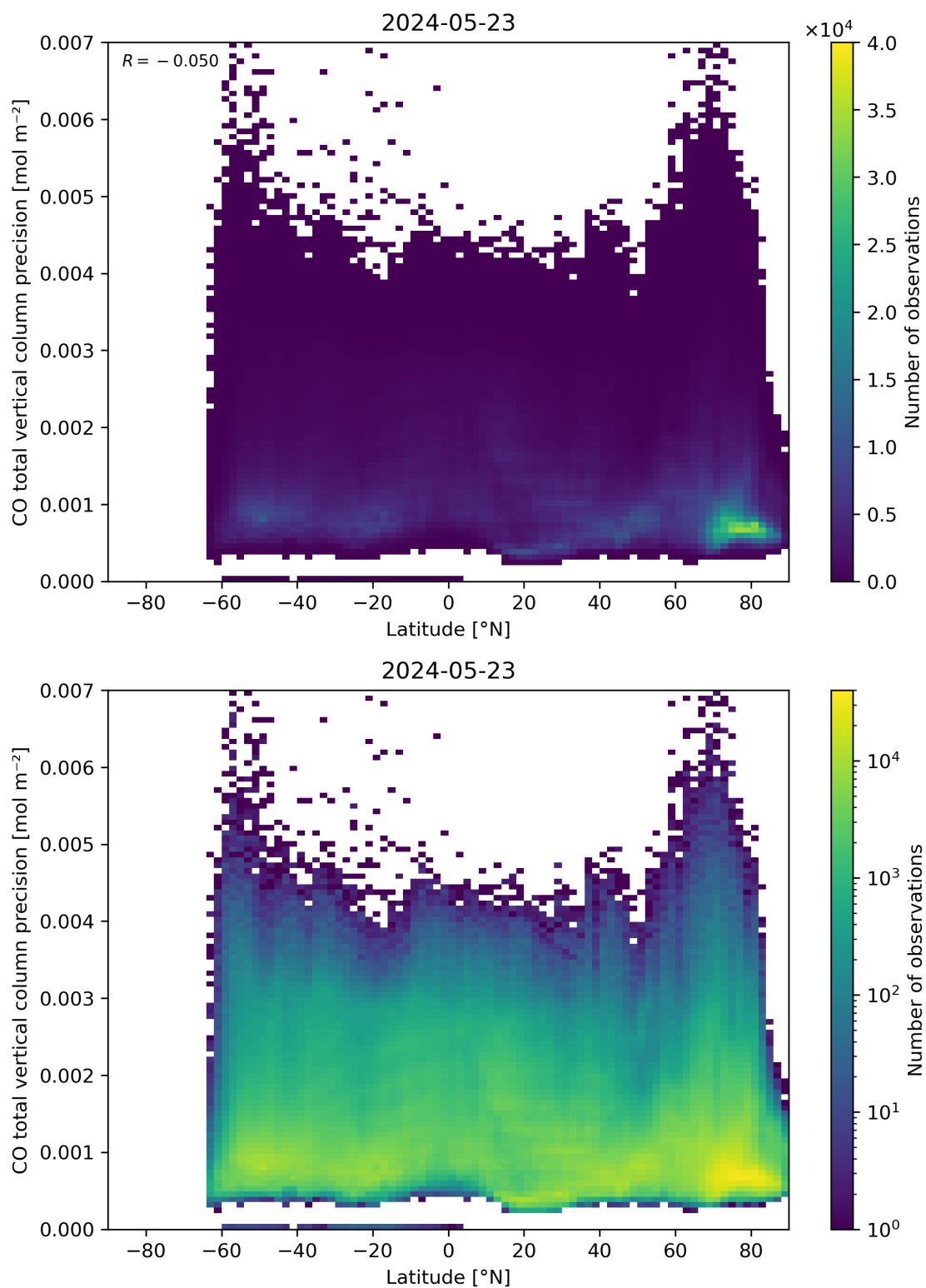
Figure 53: Scatter density plot of “Latitude” against “CO total vertical column precision” for 2024-05-23 to 2024-05-24.
