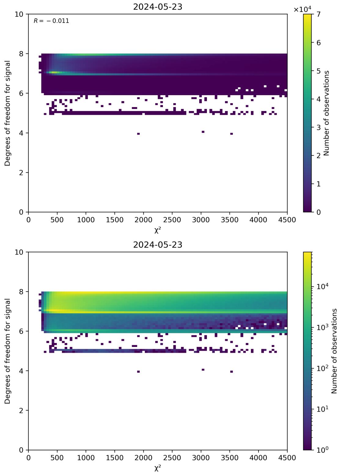
Figure 48: Scatter density plot of “ \chi^2 ” against “Degrees of freedom for signal” for 2024-05-23 to 2024-05-24.
