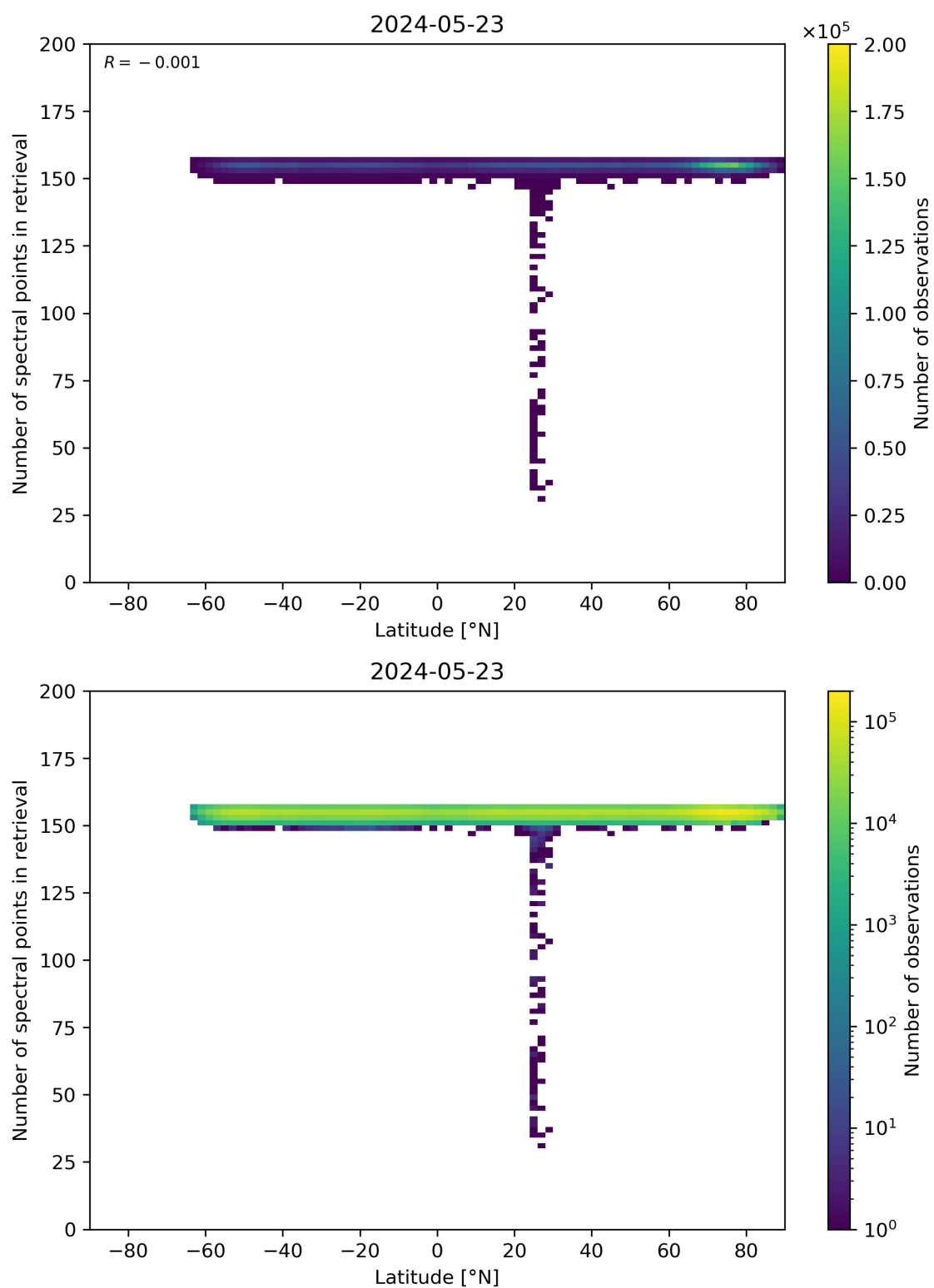
Figure 57: Scatter density plot of “Latitude” against “Number of spectral points in retrieval” for 2024-05-23 to 2024-05-24.
