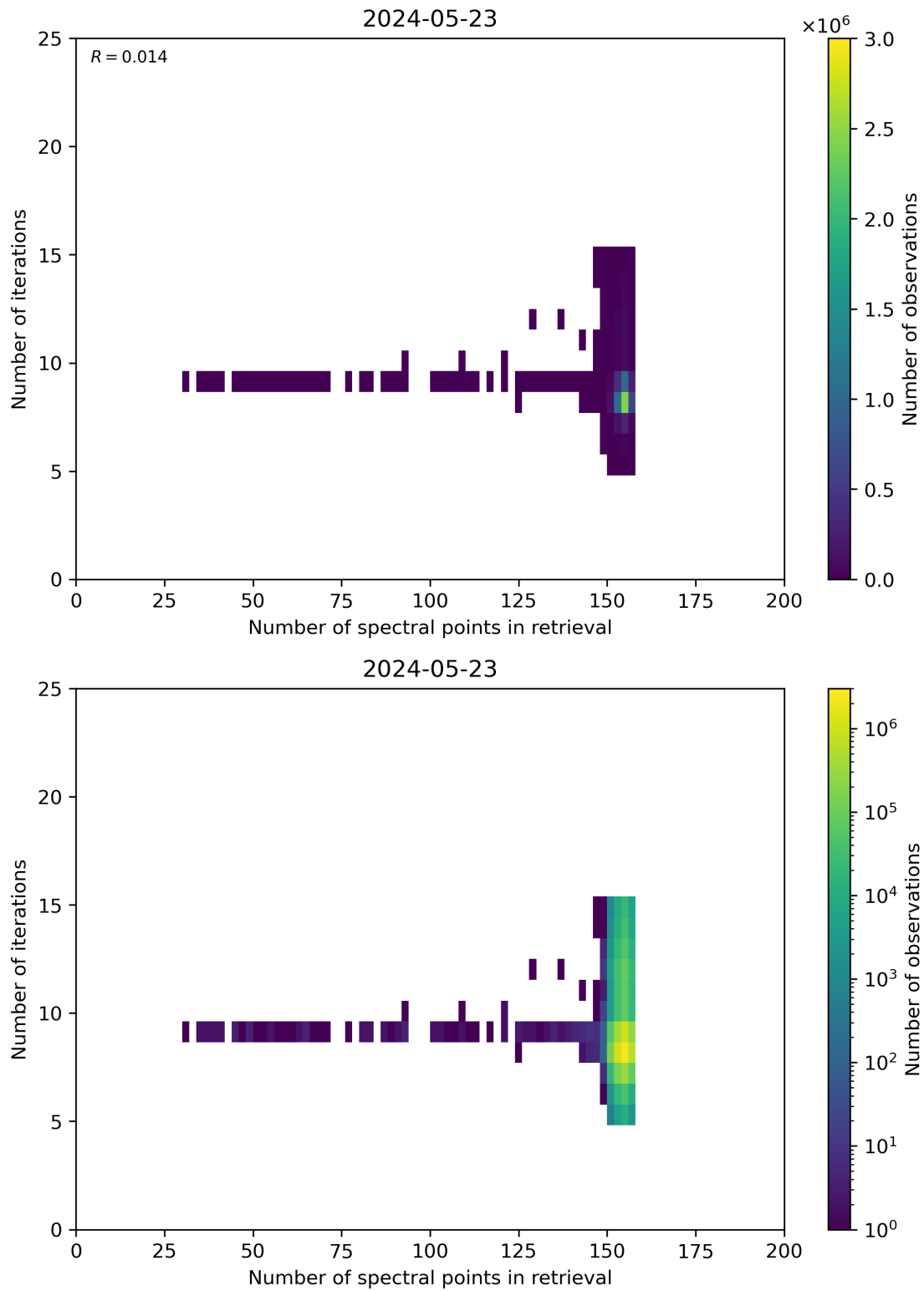
Figure 60: Scatter density plot of “Number of spectral points in retrieval” against “Number of iterations” for 2024-05-23 to 2024-05-24.
