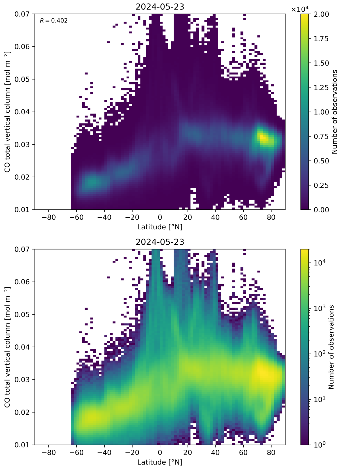
Figure 51: Scatter density plot of “Latitude” against “CO total vertical column” for 2024-05-23 to 2024-05-24.
