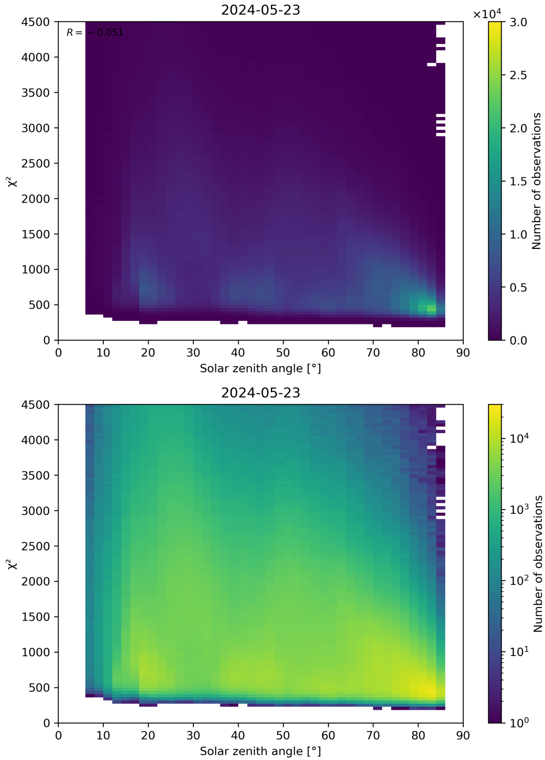
Figure 64: Scatter density plot of “Solar zenith angle” against “ \chi^2 ” for 2024-05-23 to 2024-05-24.
