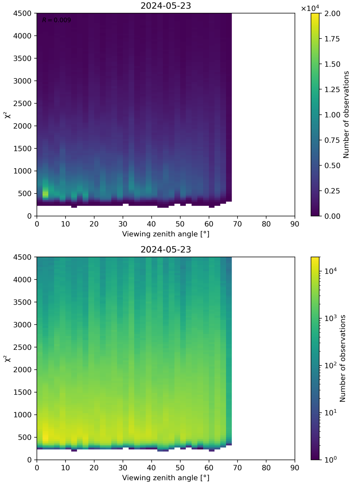
Figure 72: Scatter density plot of “Viewing zenith angle” against “ \chi^2 ” for 2024-05-23 to 2024-05-24.
