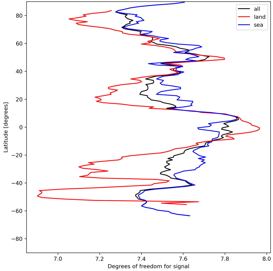
Figure 15: Zonal average of “Degrees of freedom for signal” for 2024-05-23 to 2024-05-24.
