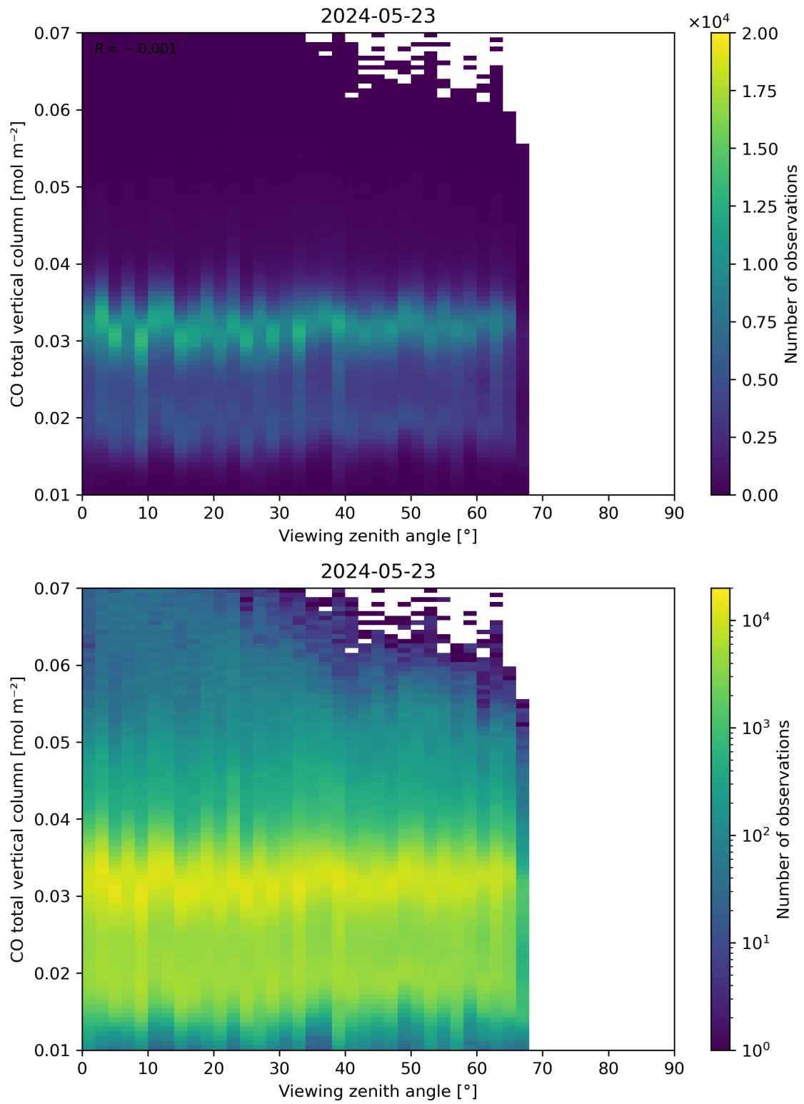
Figure 69: Scatter density plot of “Viewing zenith angle” against “CO total vertical column” for 2024-05-23 to 2024-05-24.
