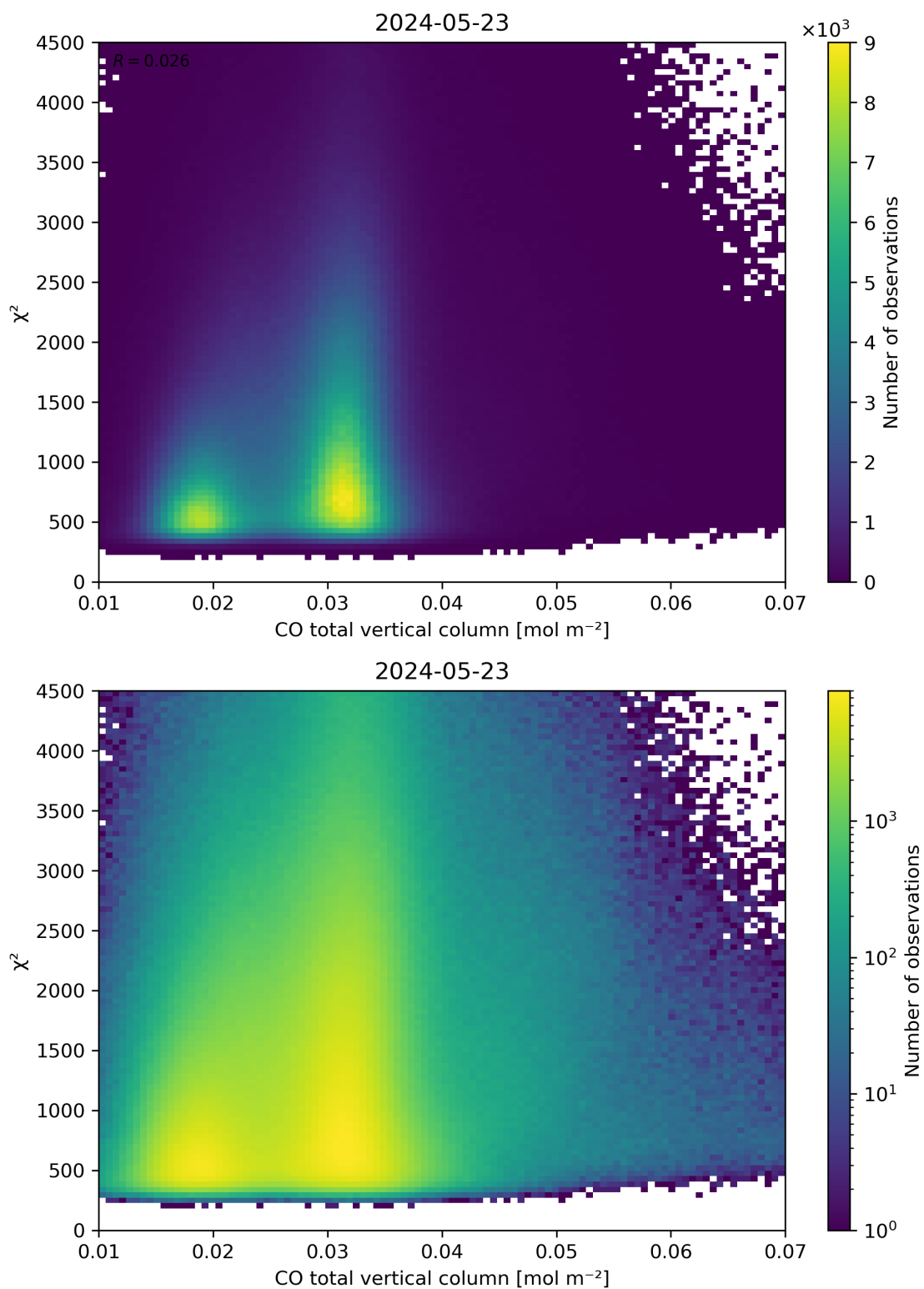
Figure 35: Scatter density plot of “CO total vertical column” against “ \chi^2 ” for 2024-05-23 to 2024-05-24.
