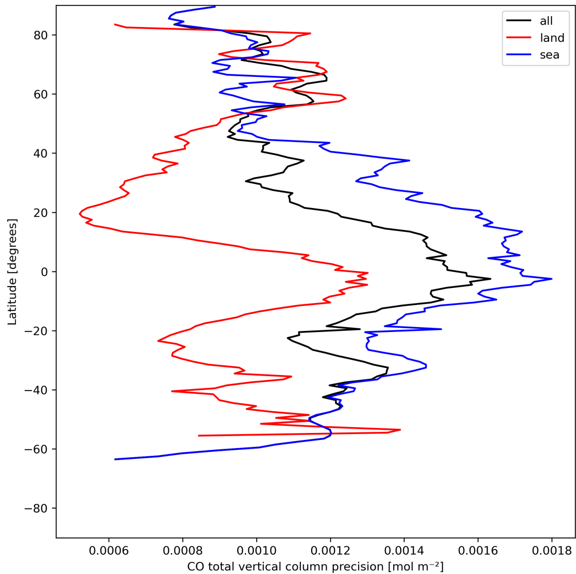
Figure 12: Zonal average of “CO total vertical column precision” for 2024-05-23 to 2024-05-24.
