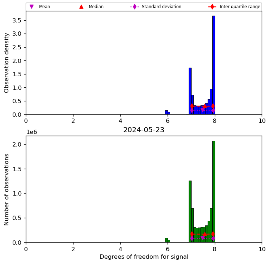
Figure 23: Histogram of “Degrees of freedom for signal” for 2024-05-23 to 2024-05-24
