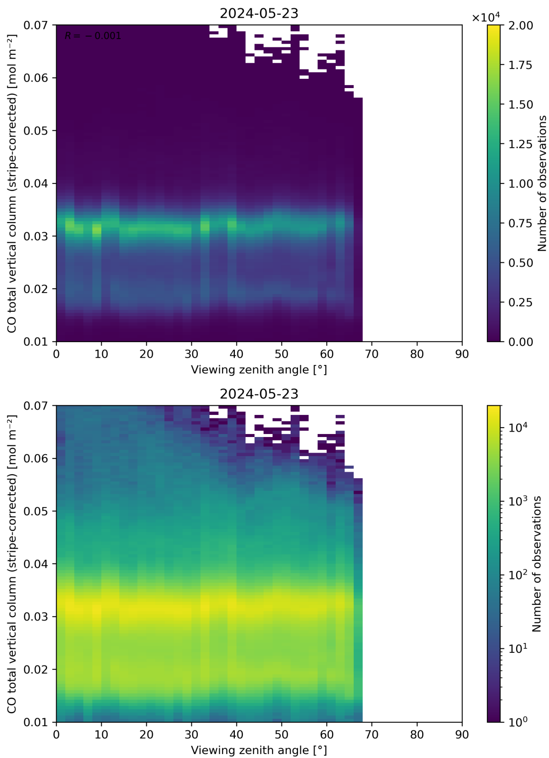
Figure 70: Scatter density plot of “Viewing zenith angle” against “CO total vertical column (stripe-corrected)” for 2024-05-23 to 2024-05-24.
