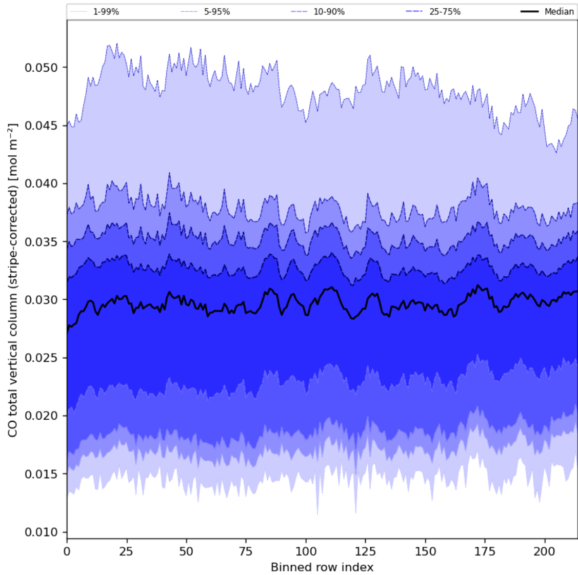
Figure 27: Along track statistics of “CO total vertical column (stripe-corrected)” for 2024-05-23 to 2024-05-24
