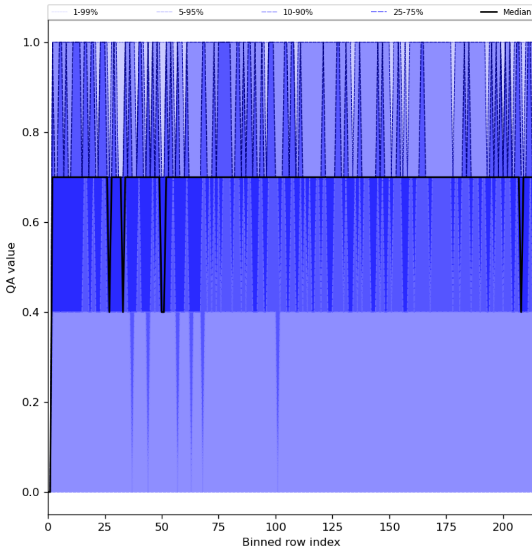
Figure 25: Along track statistics of “QA value” for 2024-05-23 to 2024-05-24
