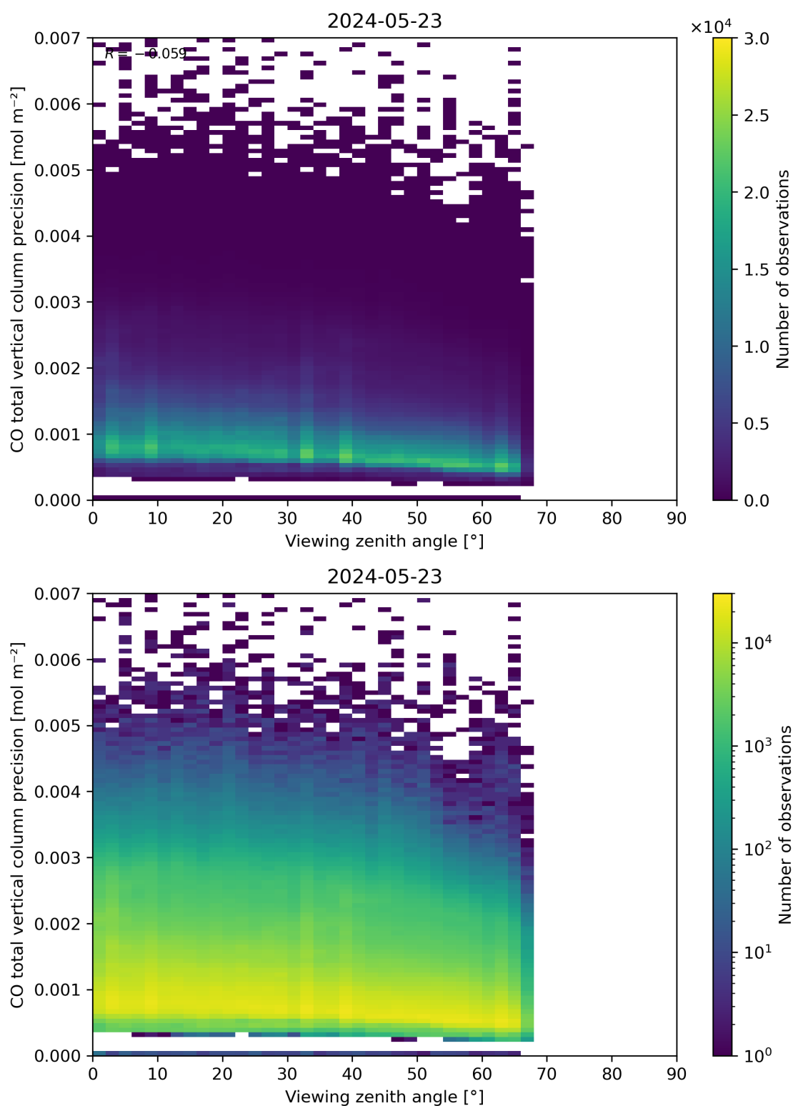
Figure 71: Scatter density plot of “Viewing zenith angle” against “CO total vertical column precision” for 2024-05-23 to 2024-05-24.
