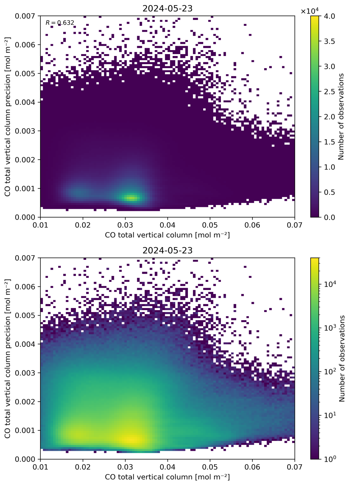
Figure 34: Scatter density plot of “CO total vertical column” against “CO total vertical column precision” for 2024-05-23 to 2024-05-24.
