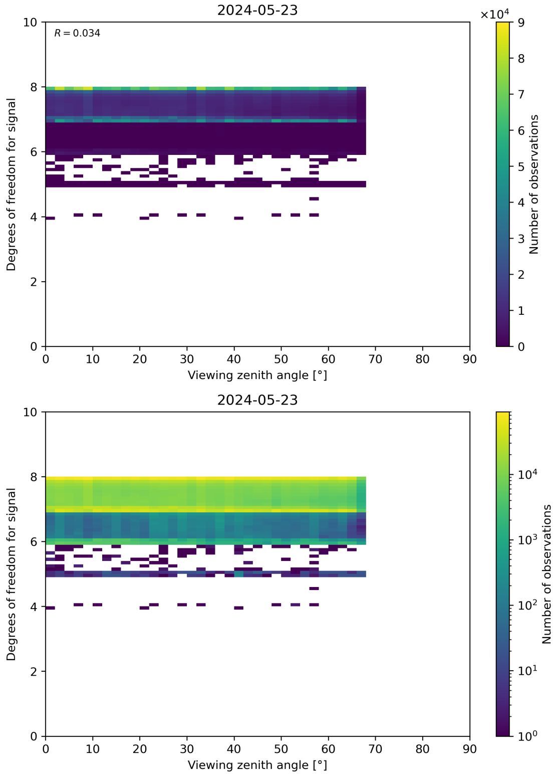
Figure 73: Scatter density plot of “Viewing zenith angle” against “Degrees of freedom for signal” for 2024-05-23 to 2024-05-24.
