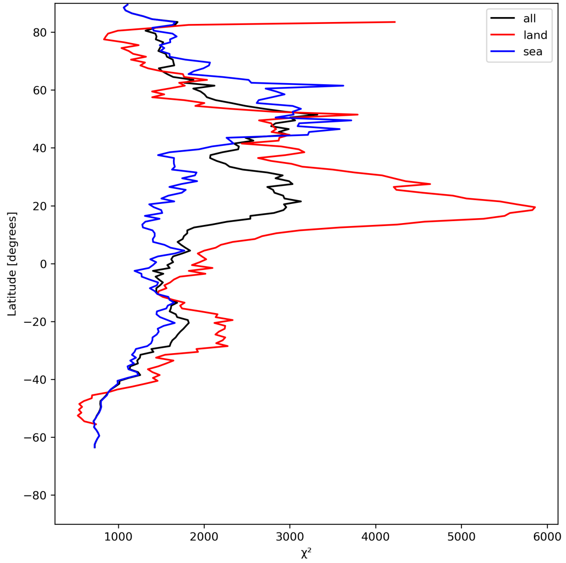
Figure 14: Zonal average of “ \chi^2 ” for 2024-05-23 to 2024-05-24.
