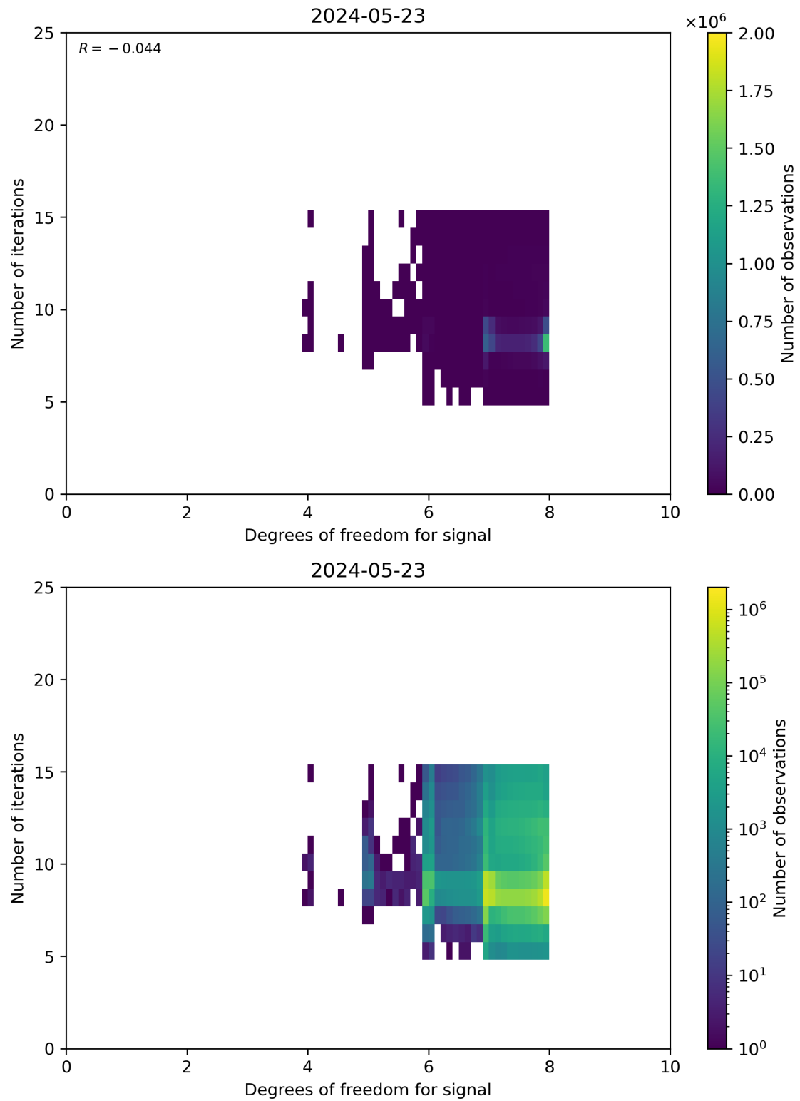
Figure 50: Scatter density plot of “Degrees of freedom for signal” against “Number of iterations” for 2024-05-23 to 2024-05-24.
