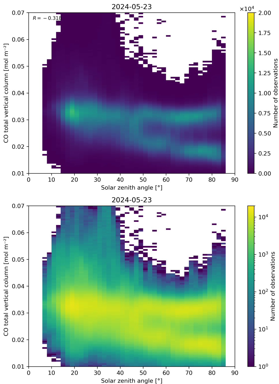
Figure 61: Scatter density plot of “Solar zenith angle” against “CO total vertical column” for 2024-05-23 to 2024-05-24.
