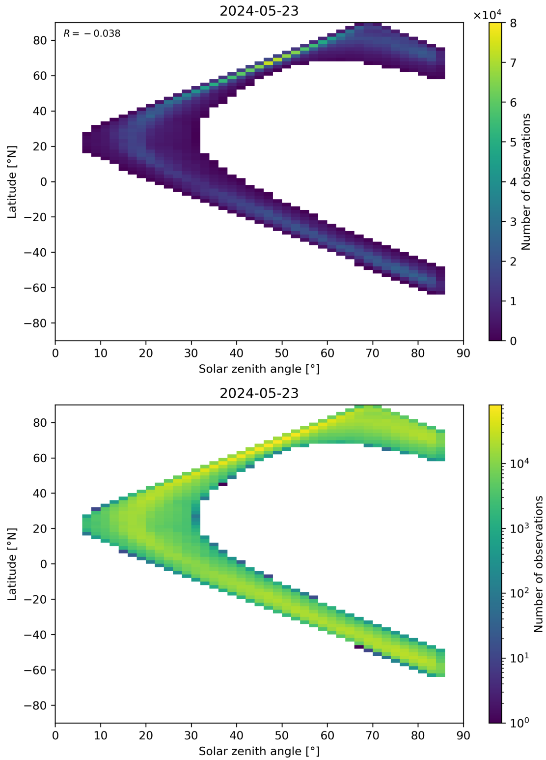
Figure 66: Scatter density plot of “Solar zenith angle” against “Latitude” for 2024-05-23 to 2024-05-24.
