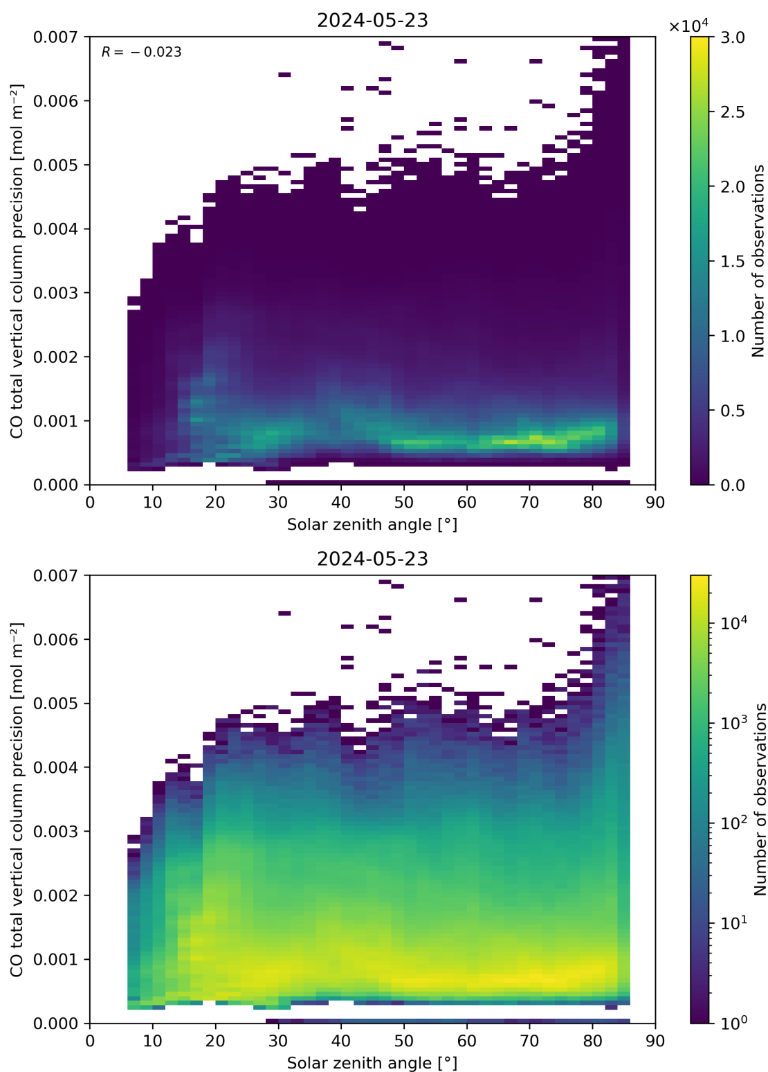
Figure 63: Scatter density plot of “Solar zenith angle” against “CO total vertical column precision” for 2024-05-23 to 2024-05-24.
