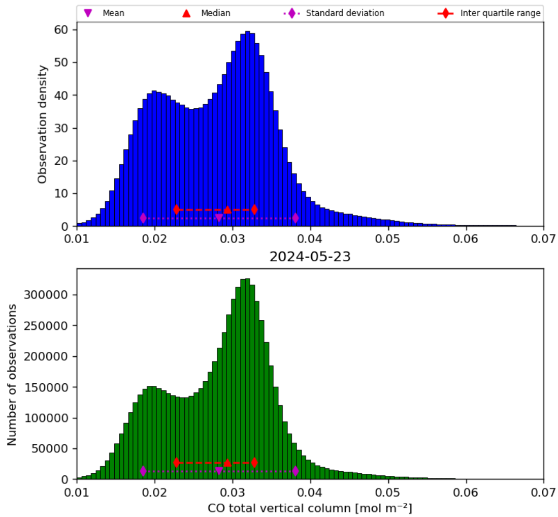
Figure 18: Histogram of “CO total vertical column” for 2024-05-23 to 2024-05-24
