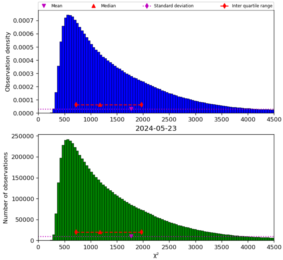
Figure 22: Histogram of “ \chi^2 ” for 2024-05-23 to 2024-05-24
