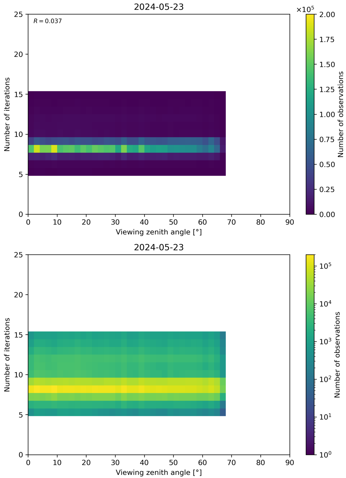
Figure 75: Scatter density plot of “Viewing zenith angle” against “Number of iterations” for 2024-05-23 to 2024-05-24.
