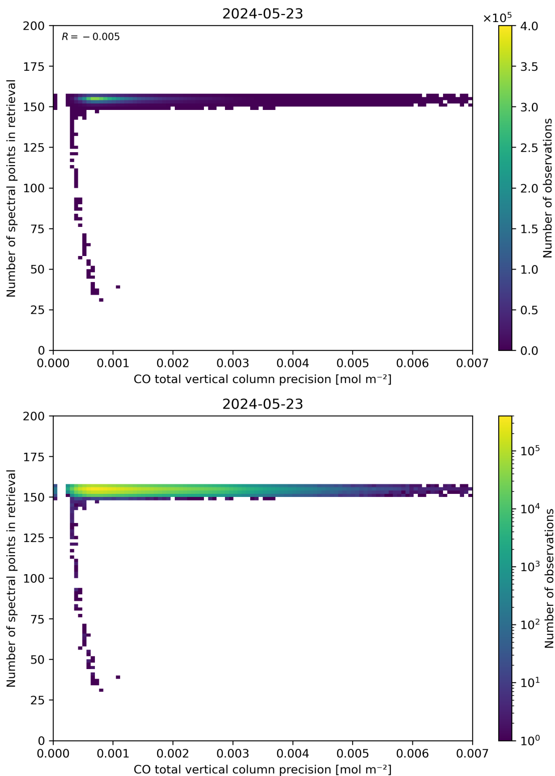
Figure 47: Scatter density plot of “CO total vertical column precision” against “Number of spectral points in retrieval” for 2024-05-23 to 2024-05-24.
