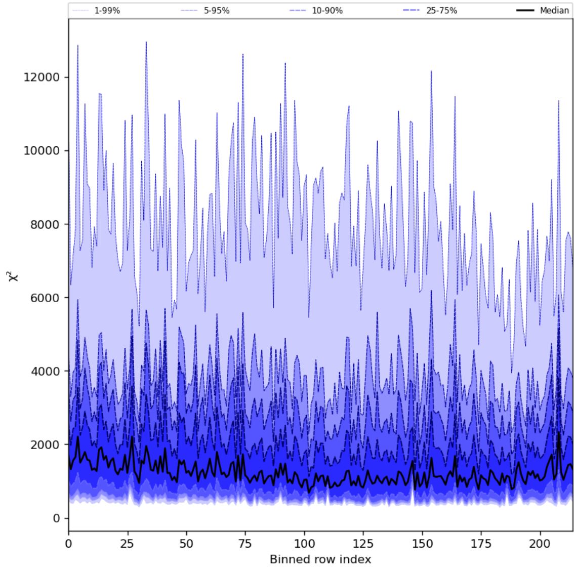
Figure 30: Along track statistics of “ \chi^2 ” for 2024-05-23 to 2024-05-24
