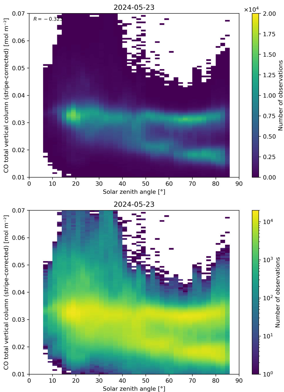
Figure 62: Scatter density plot of “Solar zenith angle” against “CO total vertical column (stripe-corrected)” for 2024-05-23 to 2024-05-24.
