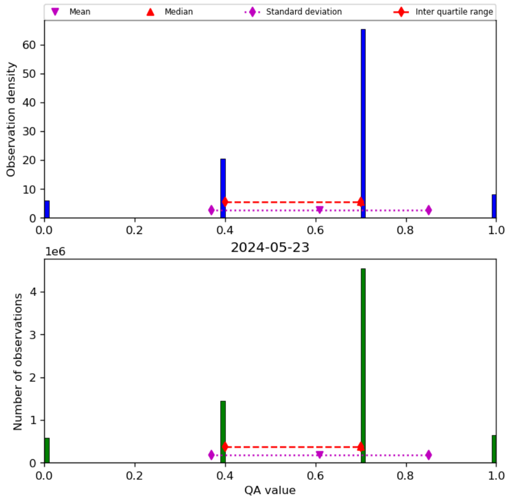
Figure 17: Histogram of “QA value” for 2024-05-23 to 2024-05-24
