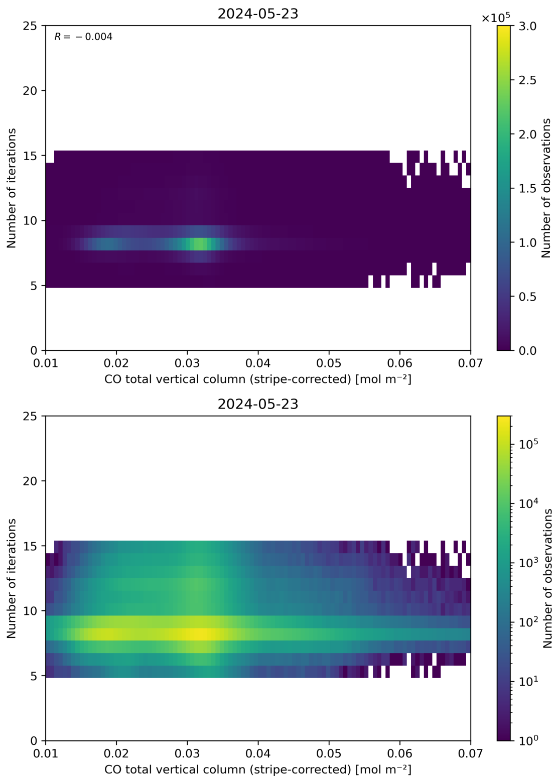
Figure 39: Scatter density plot of “CO total vertical column (stripe-corrected)” against “Number of iterations” for 2024-05-23 to 2024-05-24.
