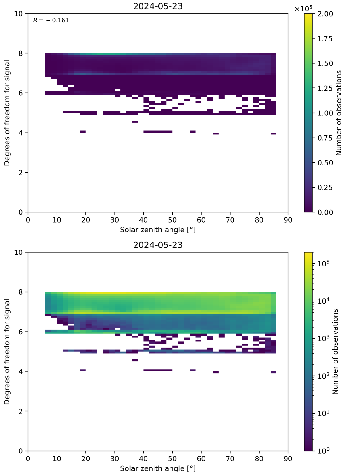
Figure 65: Scatter density plot of “Solar zenith angle” against “Degrees of freedom for signal” for 2024-05-23 to 2024-05-24.
