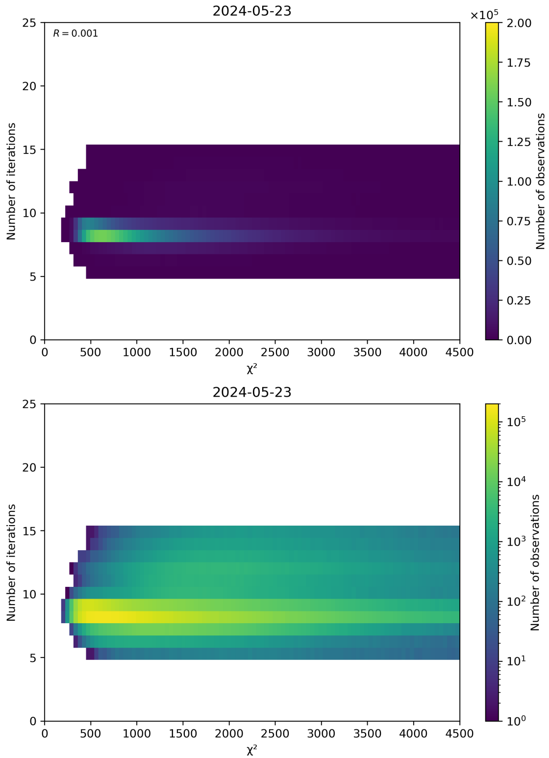
Figure 49: Scatter density plot of “ \chi^2 ” against “Number of iterations” for 2024-05-23 to 2024-05-24.
