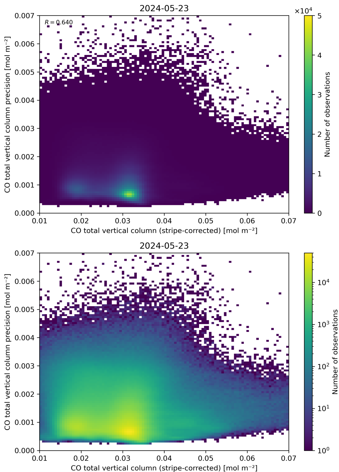
Figure 36: Scatter density plot of “CO total vertical column (stripe-corrected)” against “CO total vertical column precision” for 2024-05-23 to 2024-05-24.
