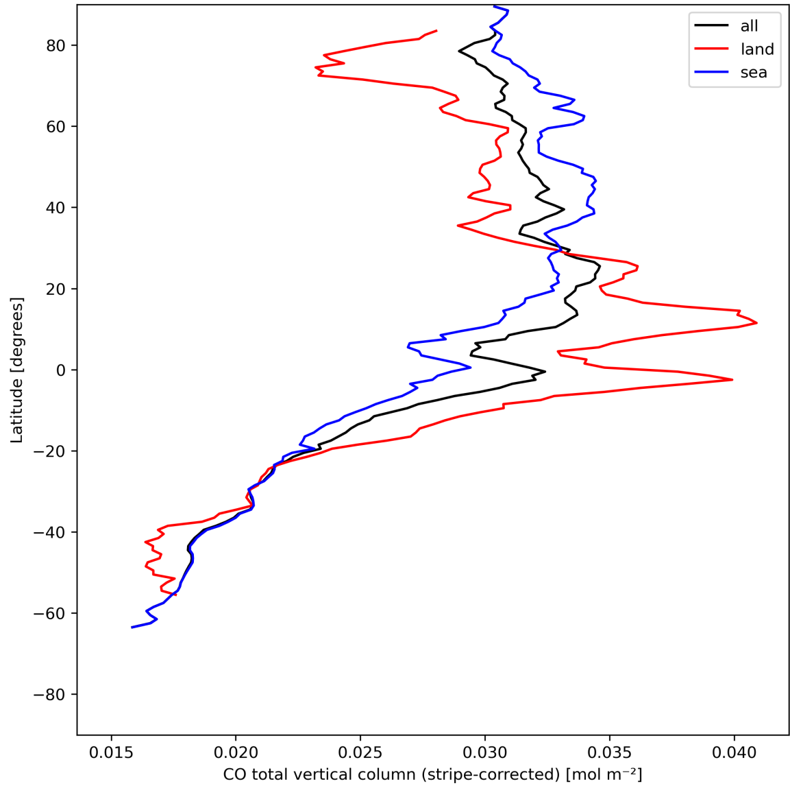
Figure 11: Zonal average of “CO total vertical column (stripe-corrected)” for 2024-05-23 to 2024-05-24.
