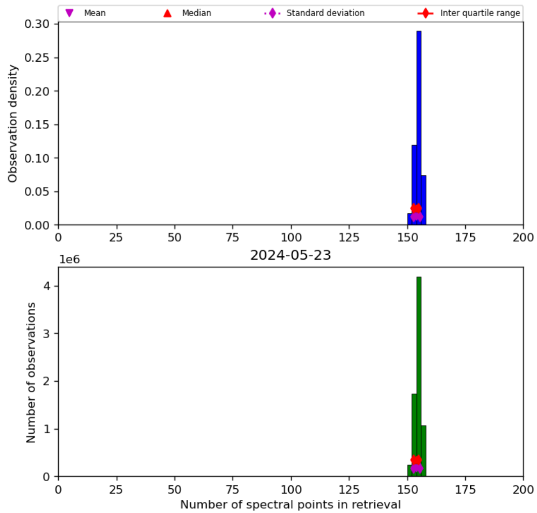
Figure 21: Histogram of “Number of spectral points in retrieval” for 2024-05-23 to 2024-05-24
