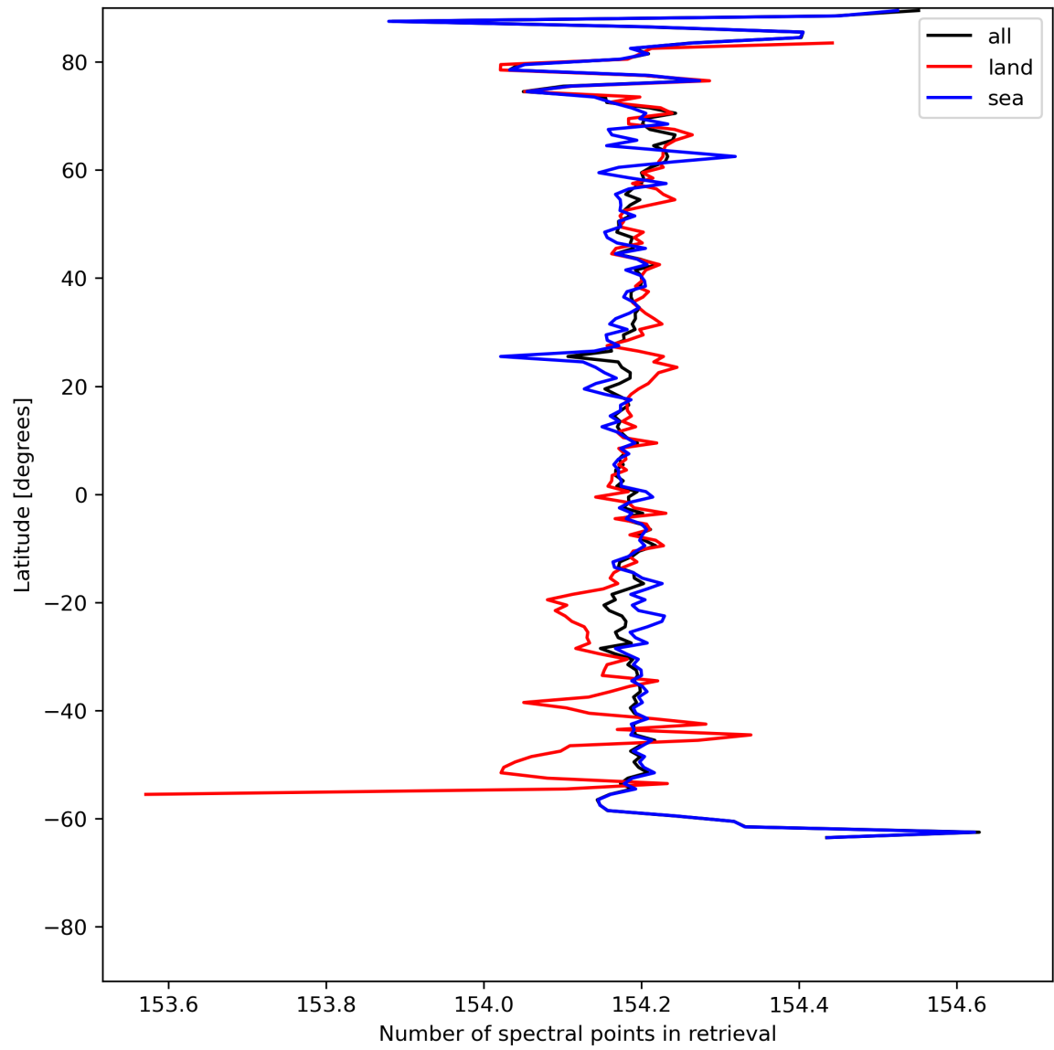
Figure 13: Zonal average of “Number of spectral points in retrieval” for 2024-05-23 to 2024-05-24.
