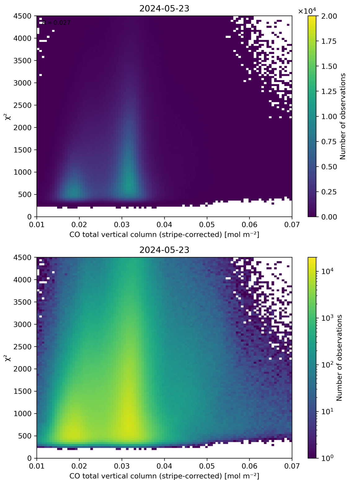
Figure 37: Scatter density plot of “CO total vertical column (stripe-corrected)” against “ \chi^2 ” for 2024-05-23 to 2024-05-24.
