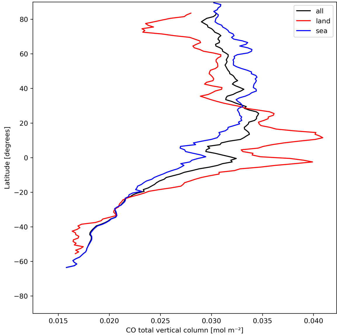
Figure 10: Zonal average of “CO total vertical column” for 2024-05-23 to 2024-05-24.
