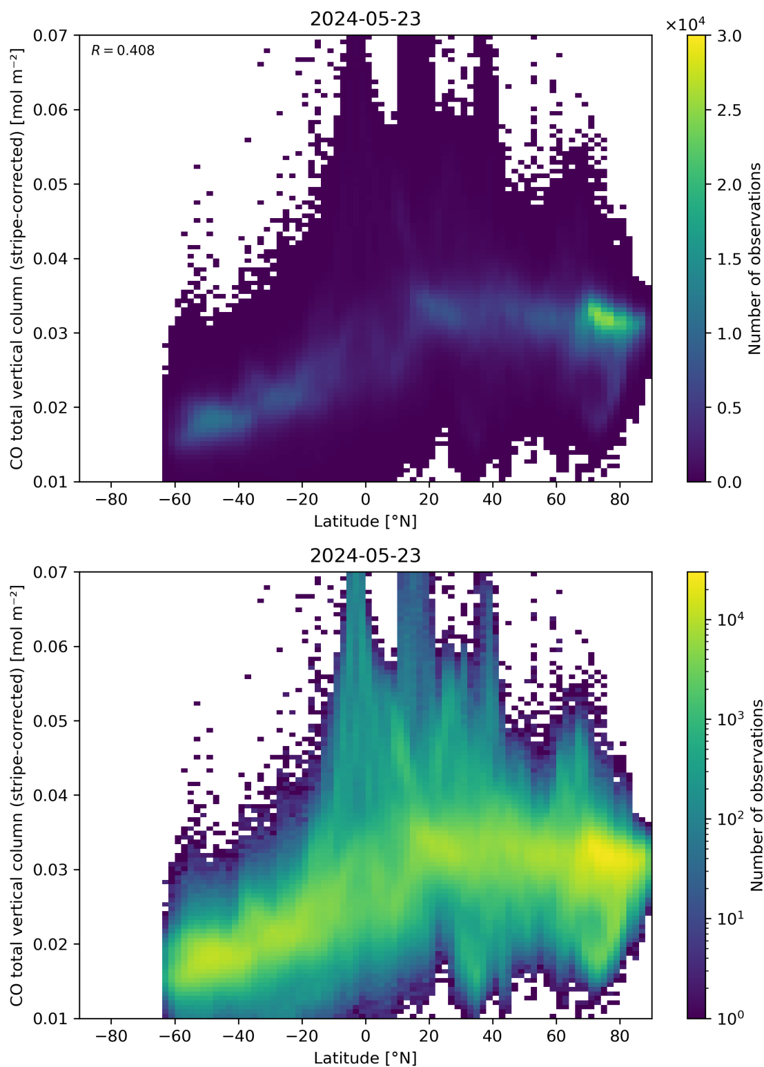
Figure 52: Scatter density plot of “Latitude” against “CO total vertical column (stripe-corrected)” for 2024-05-23 to 2024-05-24.
