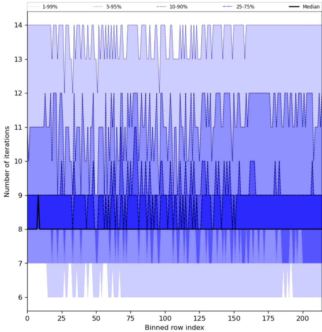
Figure 32: Along track statistics of “Number of iterations” for 2024-05-23 to 2024-05-24
