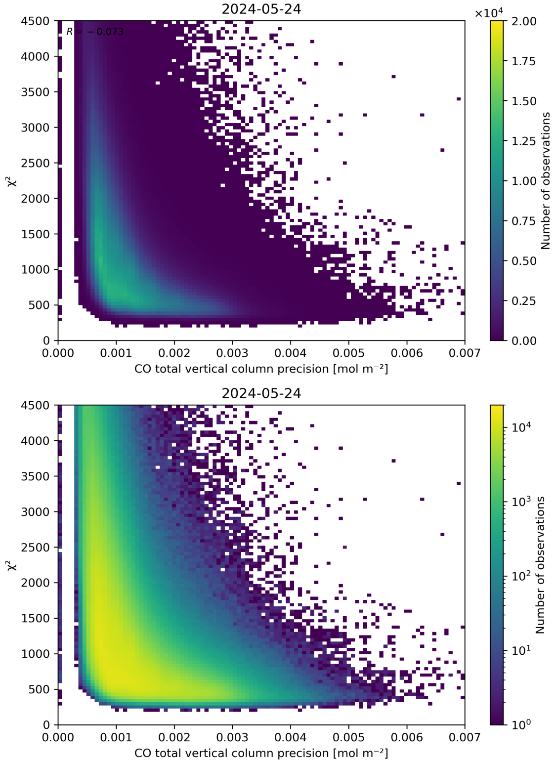
Figure 44: Scatter density plot of “CO total vertical column precision” against “ \chi^2 ” for 2024-05-23 to 2024-05-25.
