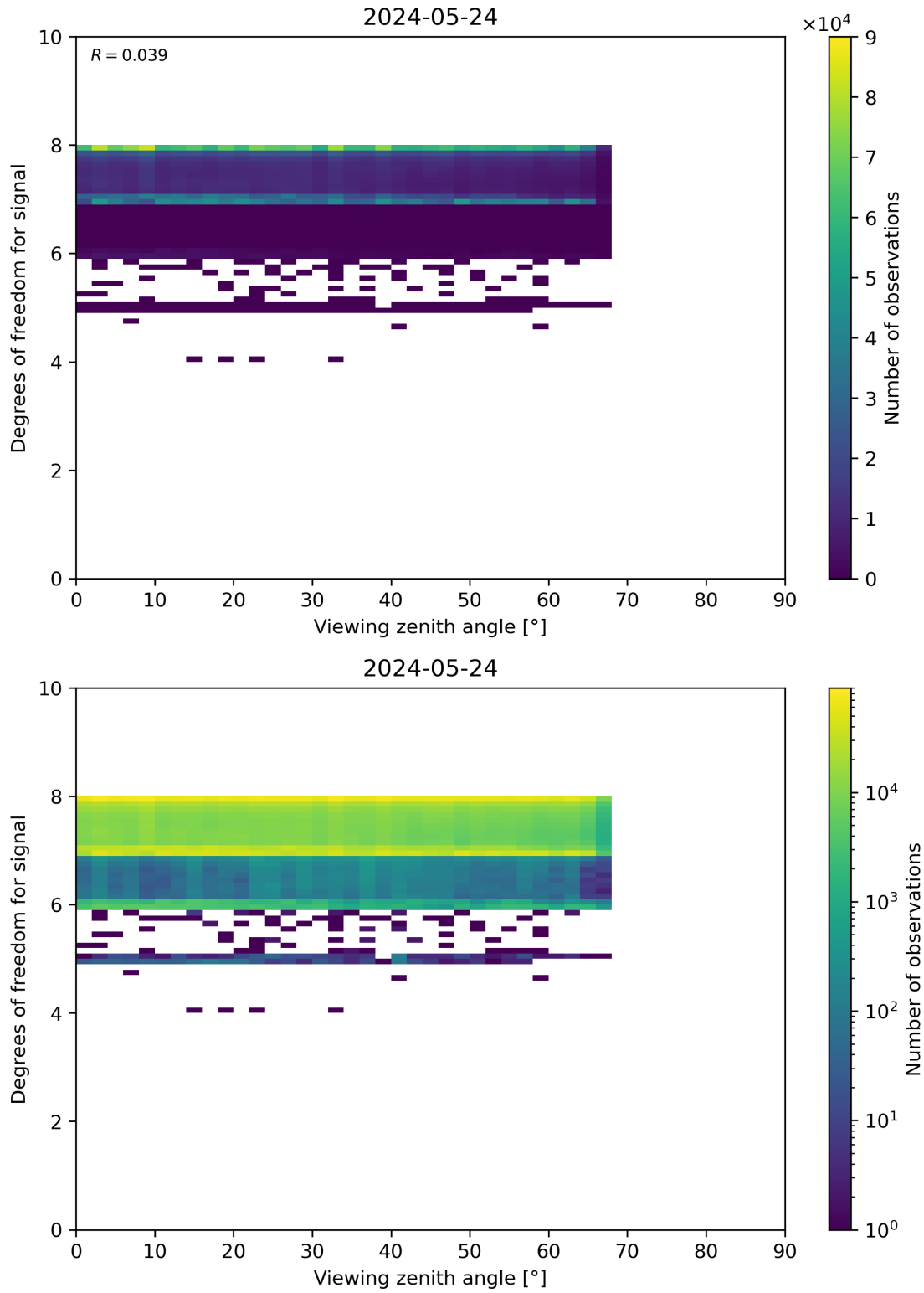
Figure 73: Scatter density plot of “Viewing zenith angle” against “Degrees of freedom for signal” for 2024-05-23 to 2024-05-25.
