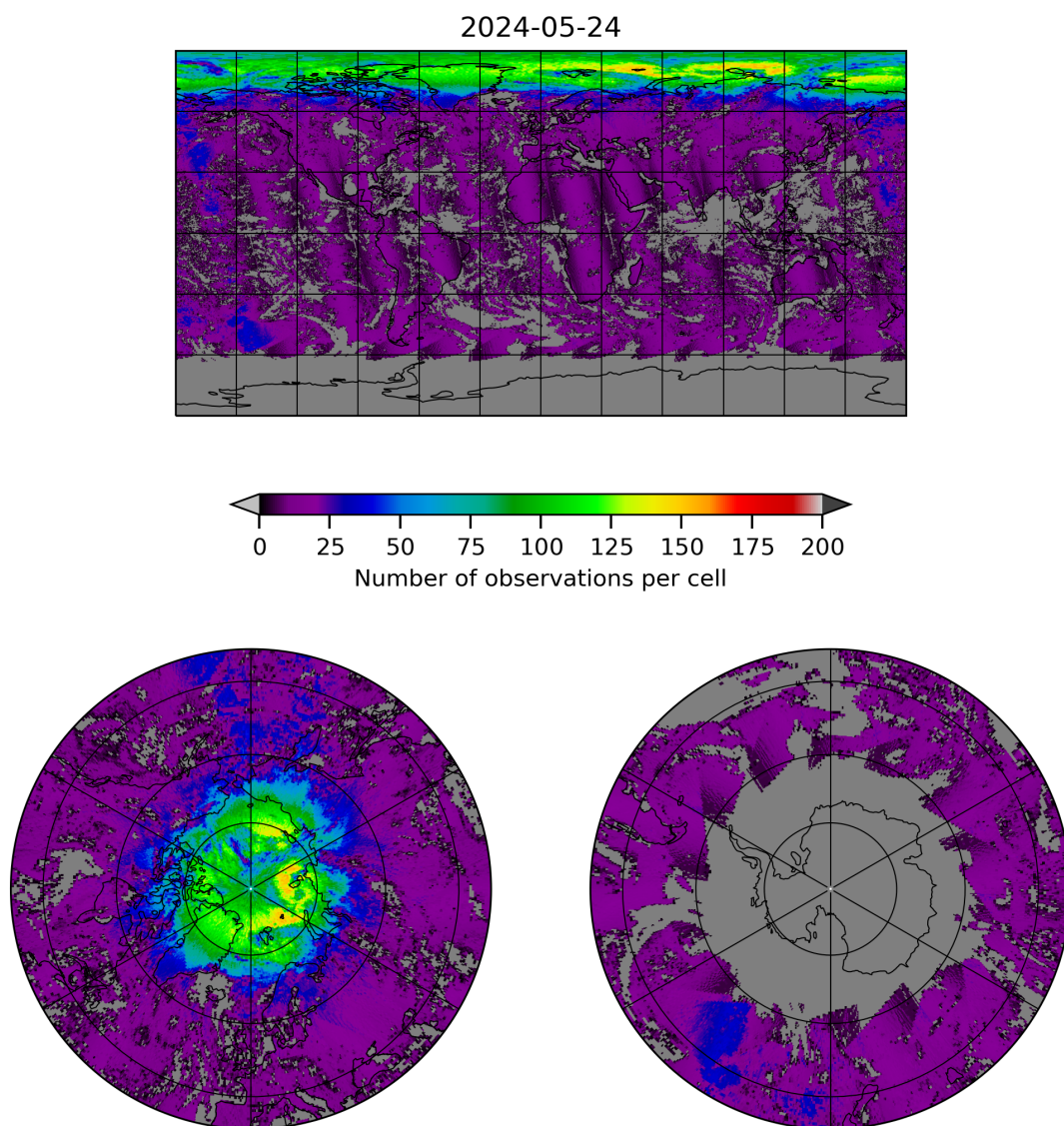
Figure 8: Map of the number of observations for 2024-05-23 to 2024-05-25
