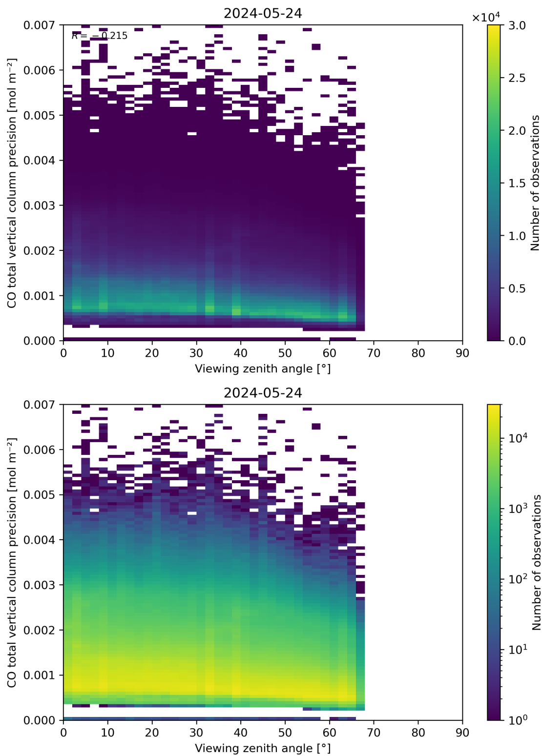
Figure 71: Scatter density plot of “Viewing zenith angle” against “CO total vertical column precision” for 2024-05-23 to 2024-05-25.
