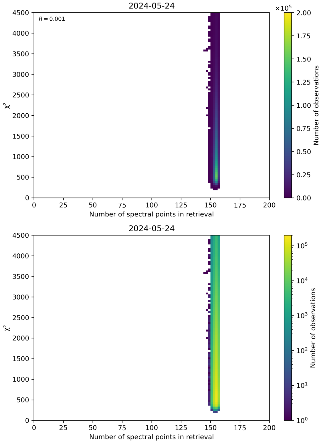
Figure 58: Scatter density plot of “Number of spectral points in retrieval” against “ \chi^2 ” for 2024-05-23 to 2024-05-25.
