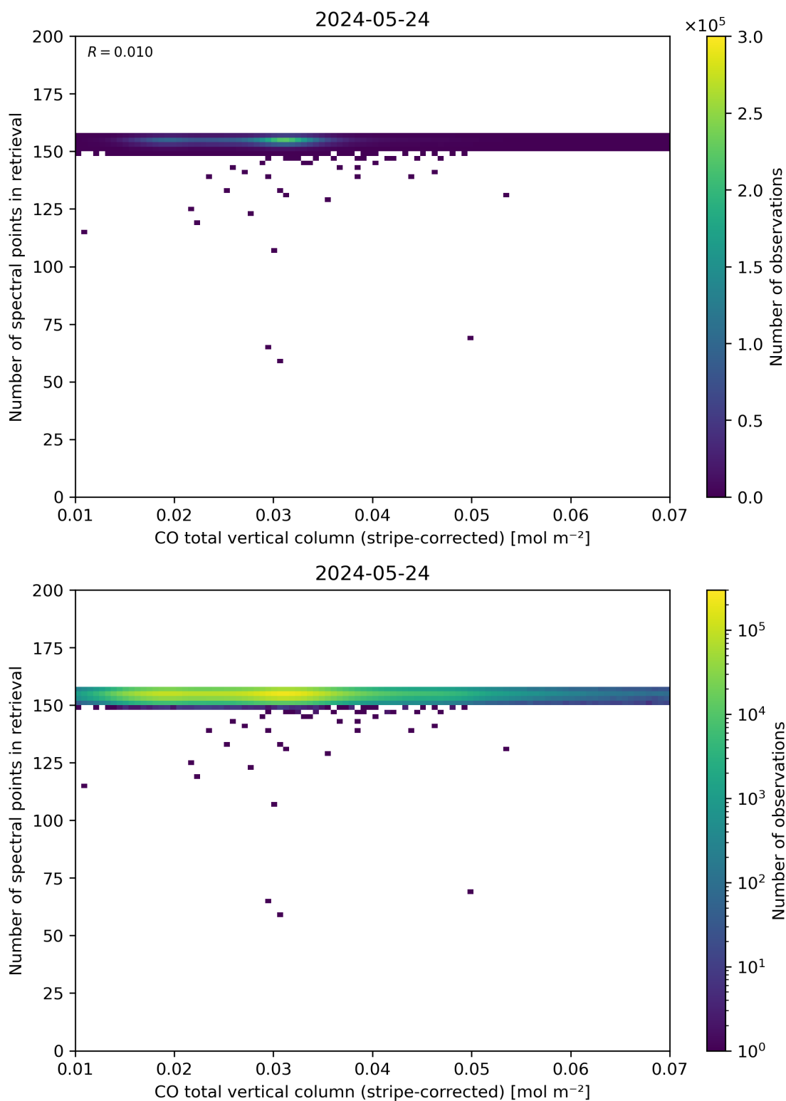
Figure 40: Scatter density plot of “CO total vertical column (stripe-corrected)” against “Number of spectral points in retrieval” for 2024-05-23 to 2024-05-25.
