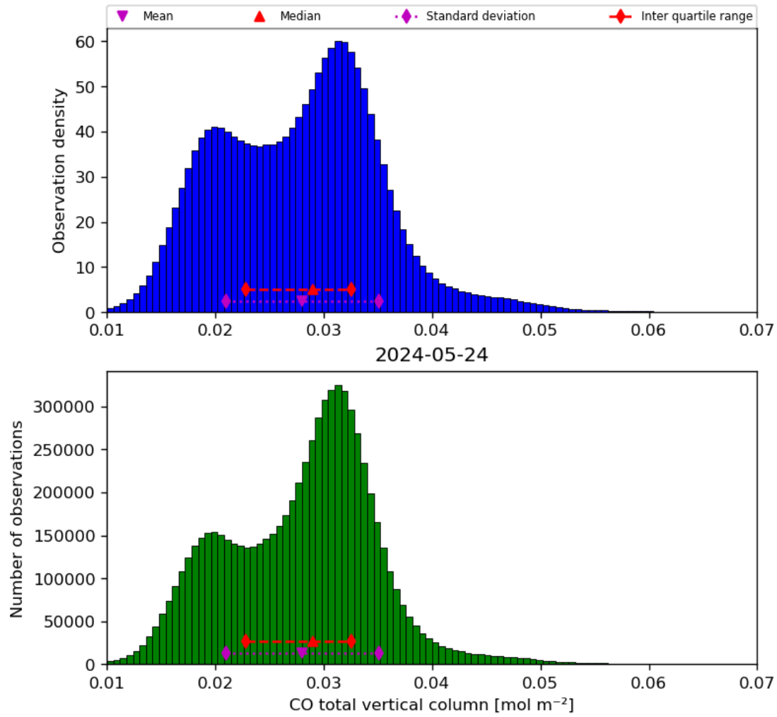
Figure 18: Histogram of “CO total vertical column” for 2024-05-23 to 2024-05-25
