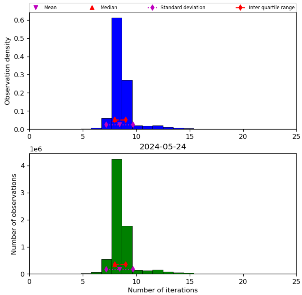
Figure 24: Histogram of “Number of iterations” for 2024-05-23 to 2024-05-25
