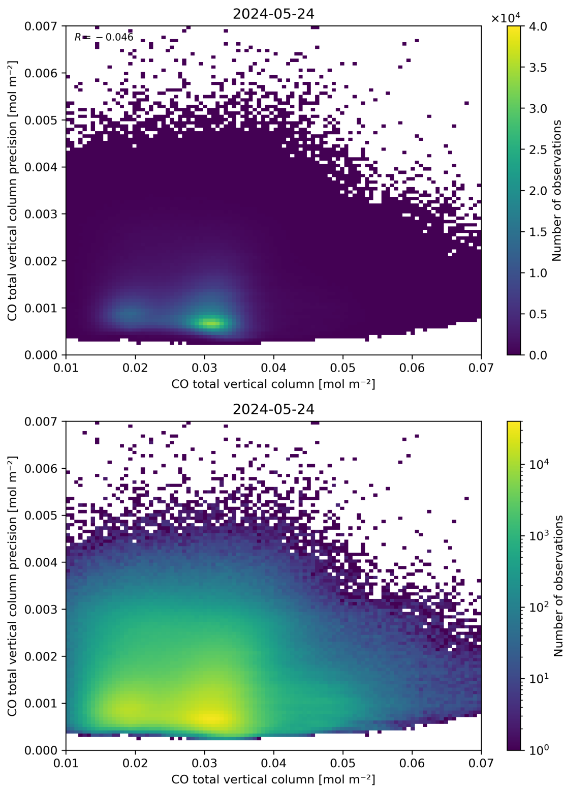
Figure 34: Scatter density plot of “CO total vertical column” against “CO total vertical column precision” for 2024-05-23 to 2024-05-25.
