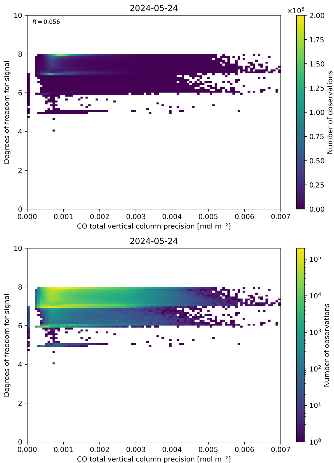
Figure 45: Scatter density plot of “CO total vertical column precision” against “Degrees of freedom for signal” for 2024-05-23 to 2024-05-25.
