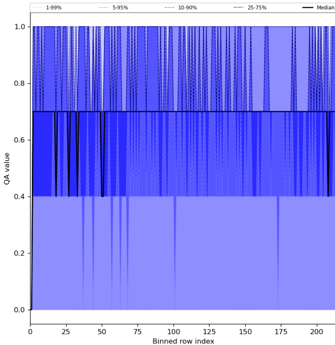
Figure 25: Along track statistics of “QA value” for 2024-05-23 to 2024-05-25
