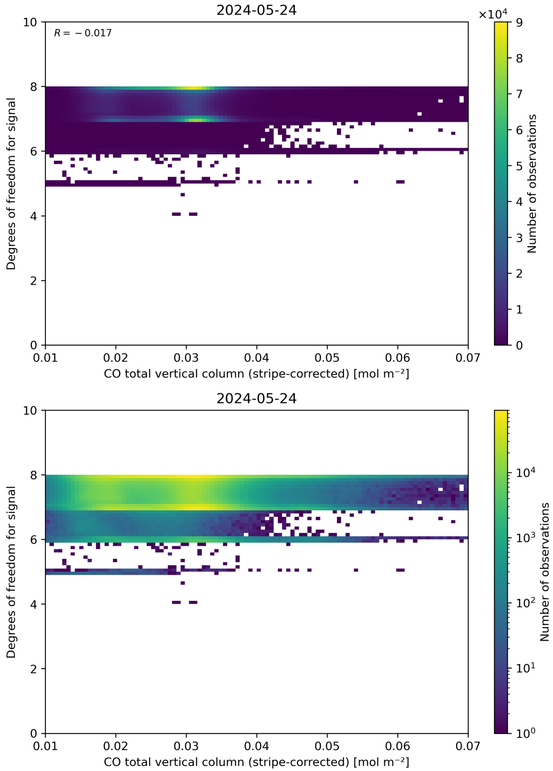
Figure 38: Scatter density plot of “CO total vertical column (stripe-corrected)” against “Degrees of freedom for signal” for 2024-05-23 to 2024-05-25.
