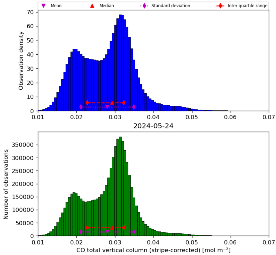
Figure 19: Histogram of “CO total vertical column (stripe-corrected)” for 2024-05-23 to 2024-05-25
