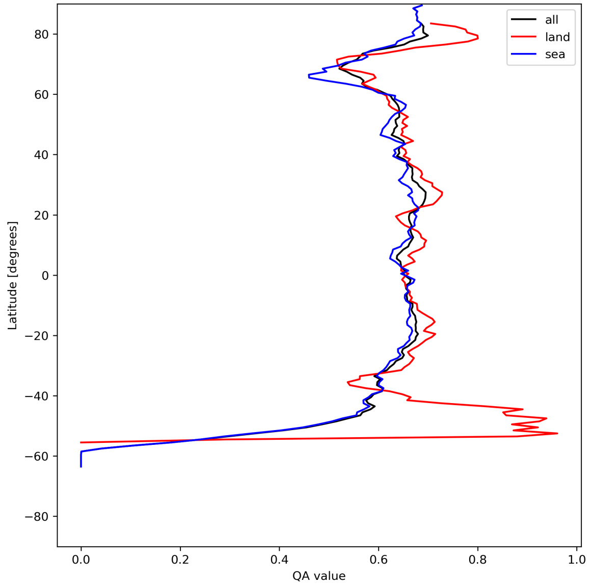
Figure 9: Zonal average of “QA value” for 2024-05-23 to 2024-05-25.
