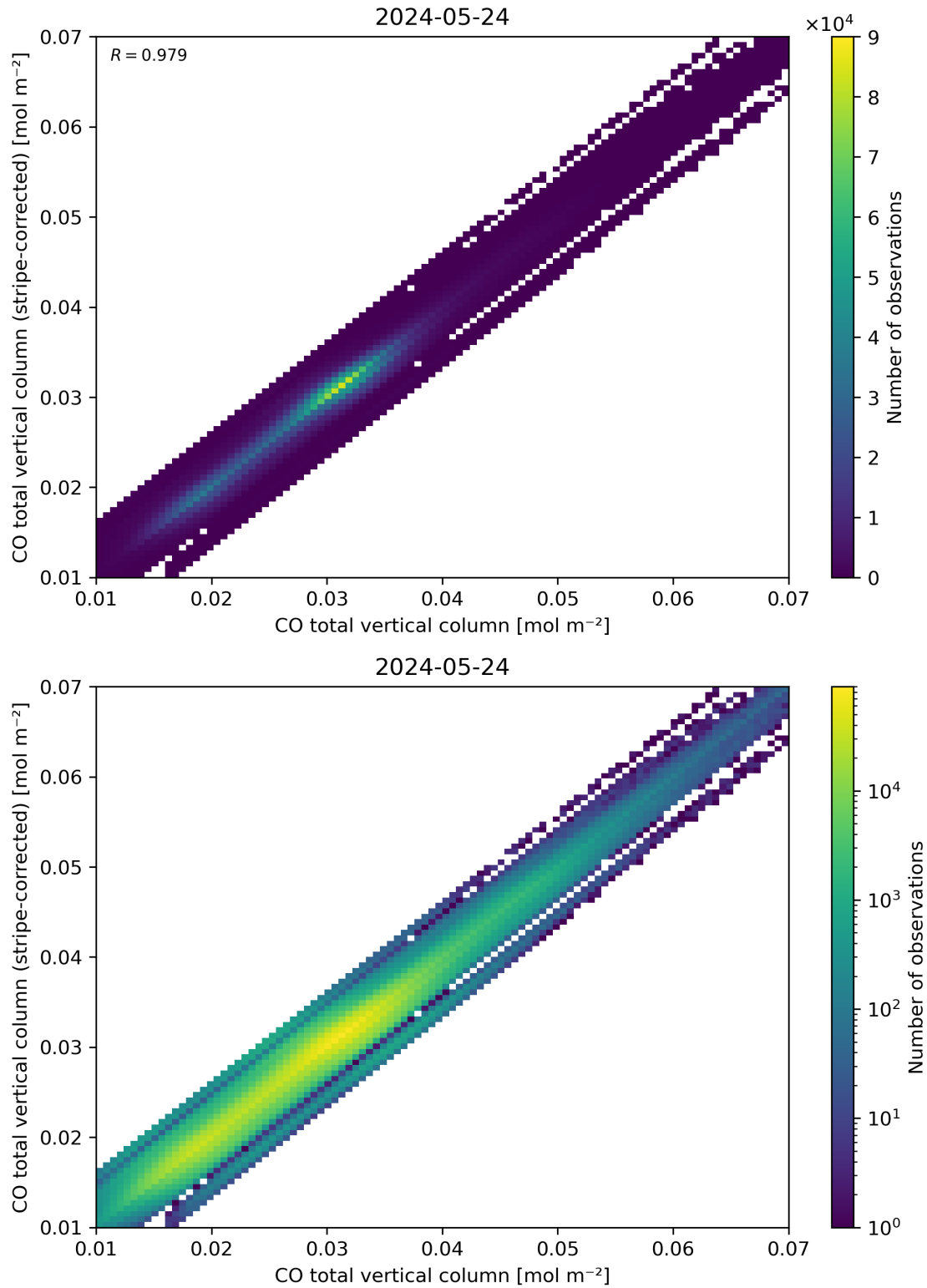
Figure 33: Scatter density plot of “CO total vertical column” against “CO total vertical column (stripe-corrected)” for 2024-05-23 to 2024-05-25.
