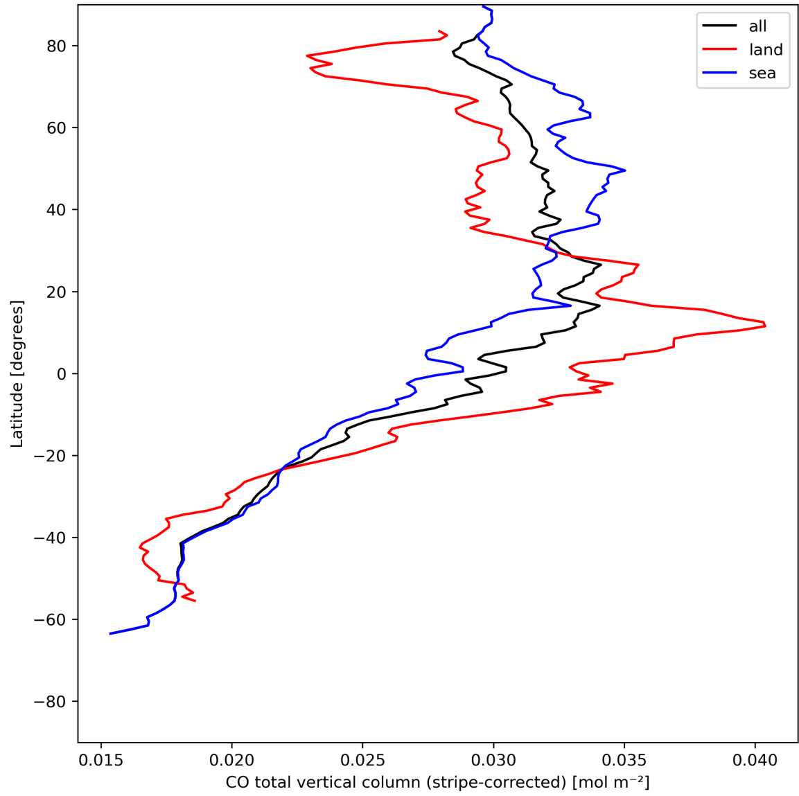
Figure 11: Zonal average of “CO total vertical column (stripe-corrected)” for 2024-05-23 to 2024-05-25.
