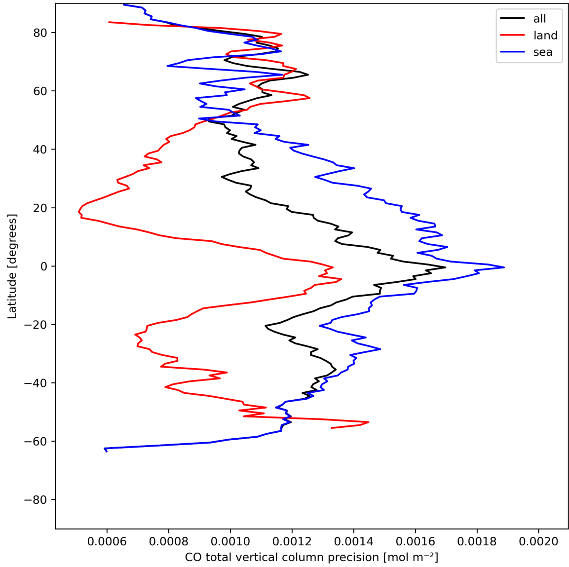
Figure 12: Zonal average of “CO total vertical column precision” for 2024-05-23 to 2024-05-25.
