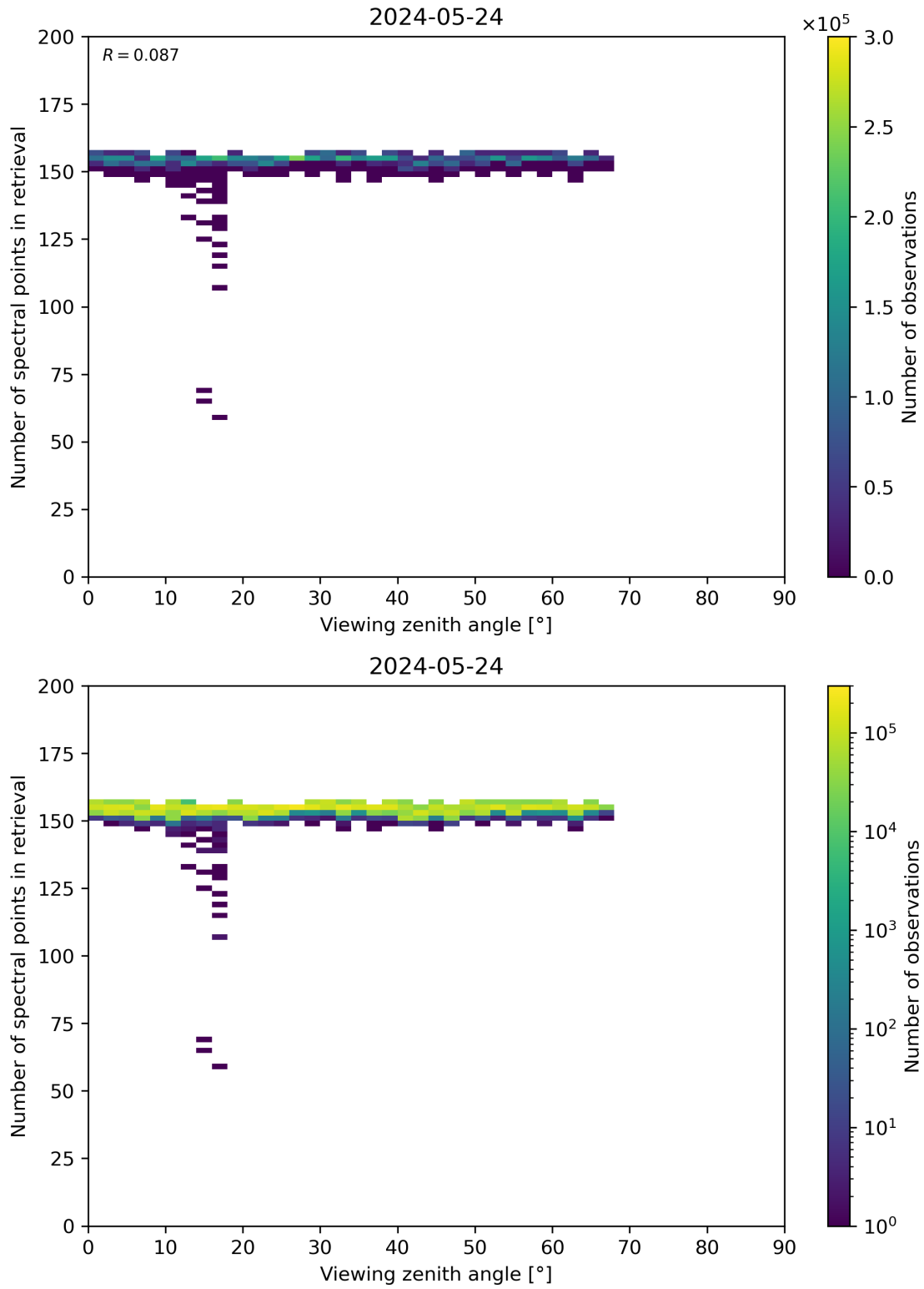
Figure 76: Scatter density plot of “Viewing zenith angle” against “Number of spectral points in retrieval” for 2024-05-23 to 2024-05-25.
