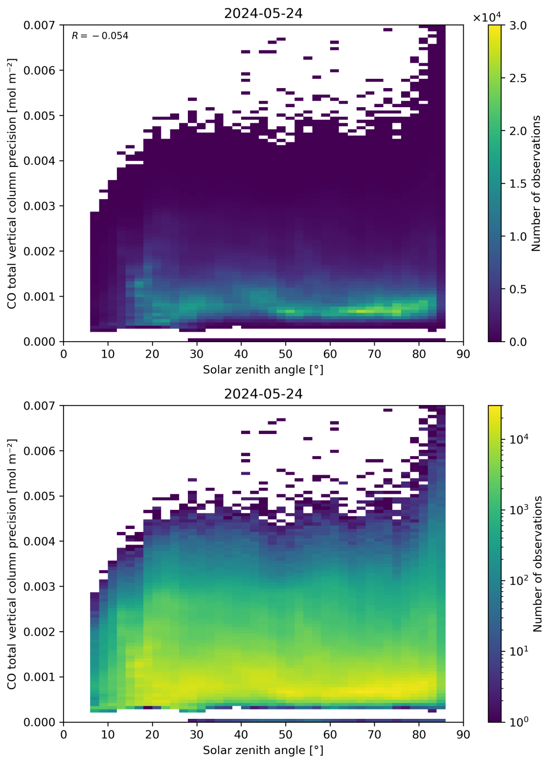
Figure 63: Scatter density plot of “Solar zenith angle” against “CO total vertical column precision” for 2024-05-23 to 2024-05-25.
