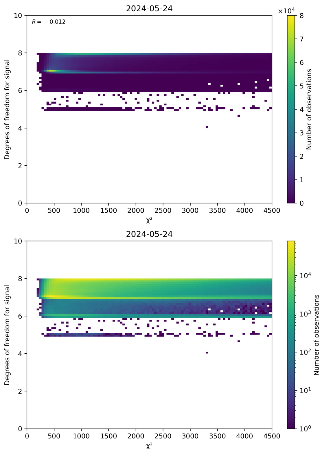
Figure 48: Scatter density plot of “ \chi^2 ” against “Degrees of freedom for signal” for 2024-05-23 to 2024-05-25.
