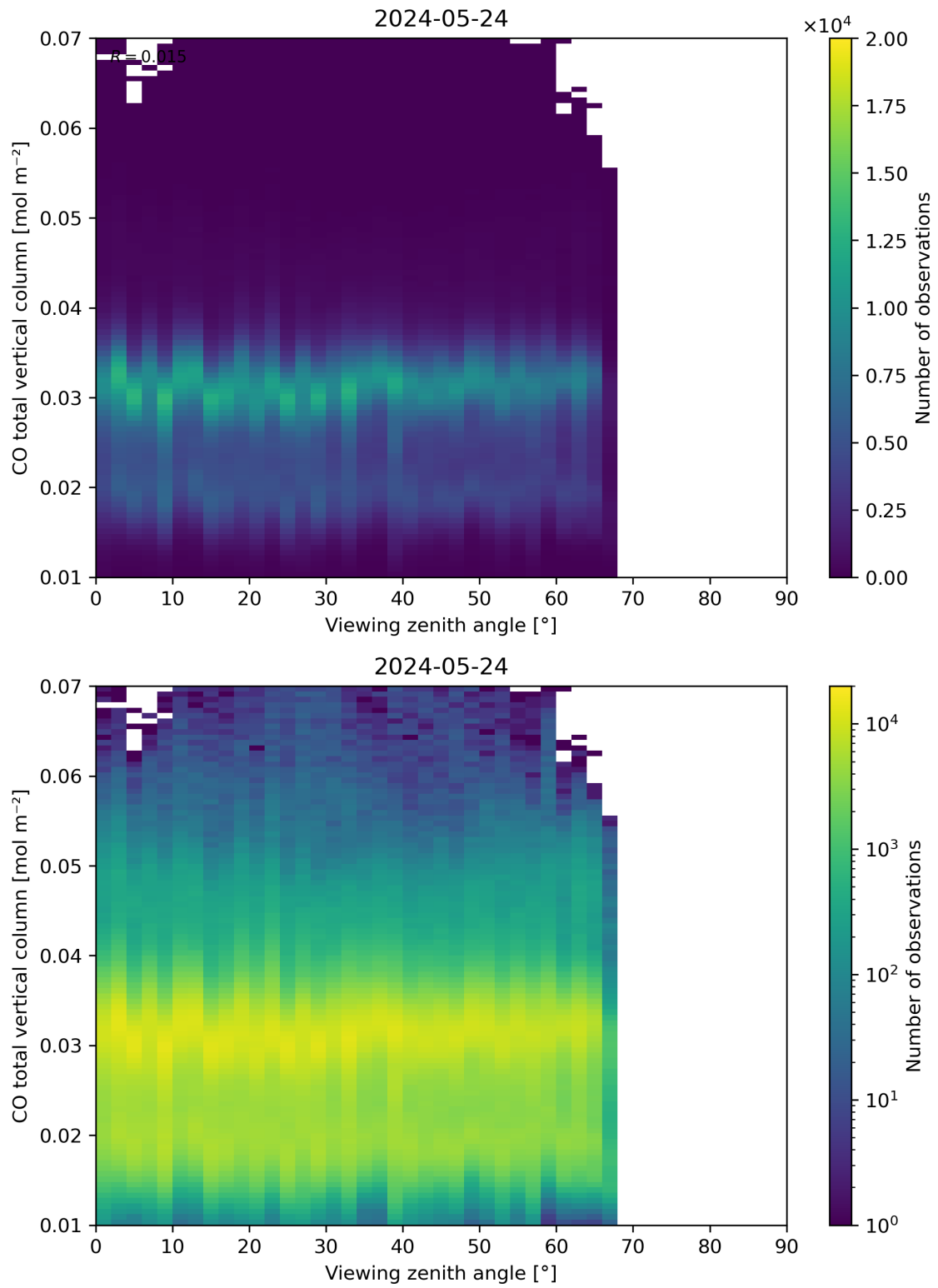
Figure 69: Scatter density plot of “Viewing zenith angle” against “CO total vertical column” for 2024-05-23 to 2024-05-25.
