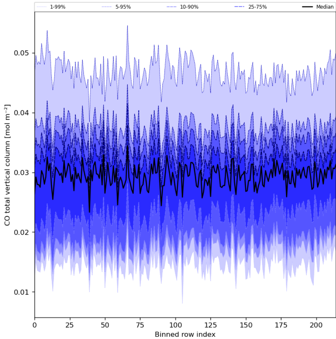
Figure 26: Along track statistics of “CO total vertical column” for 2024-05-23 to 2024-05-25
