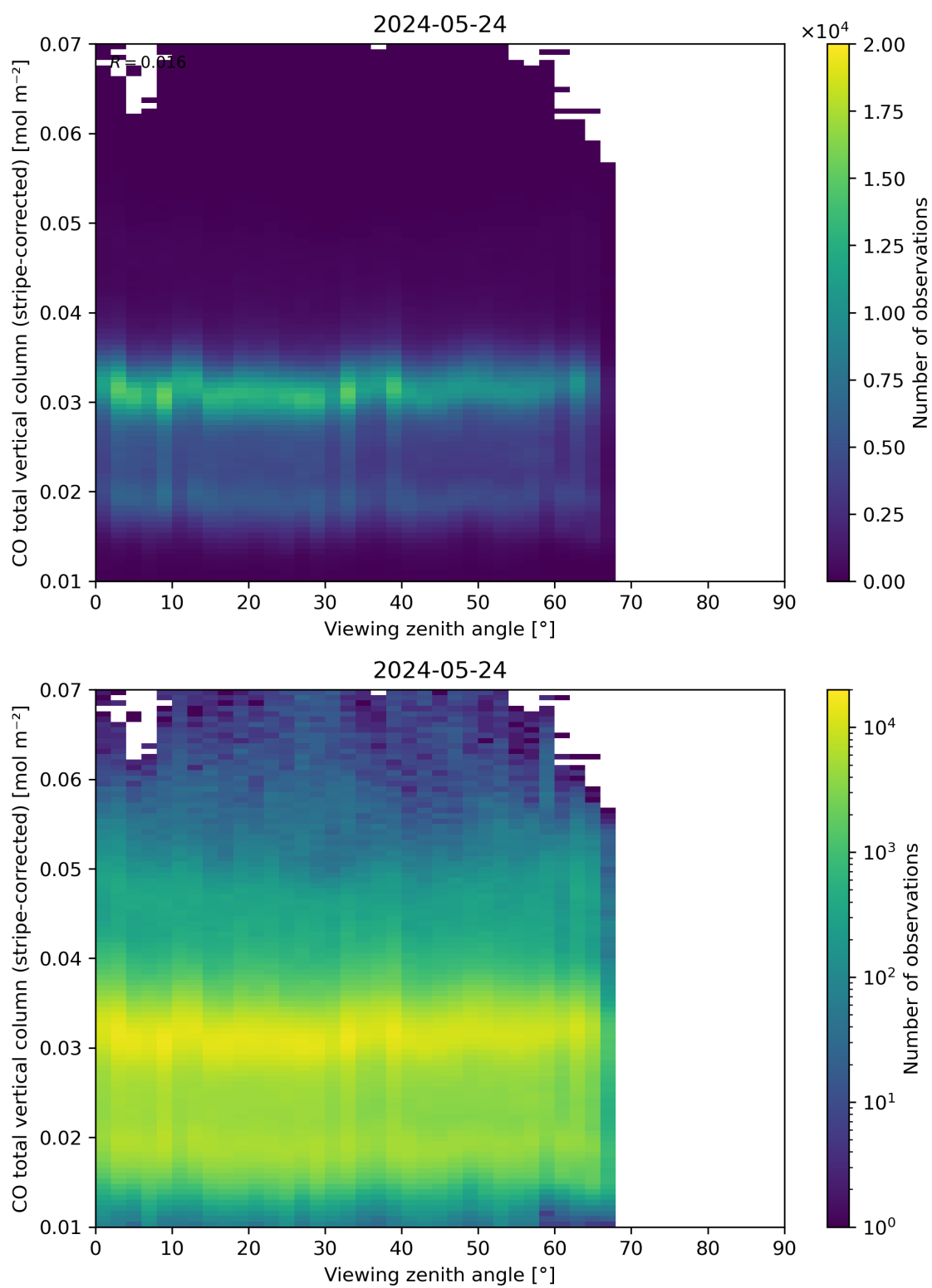
Figure 70: Scatter density plot of “Viewing zenith angle” against “CO total vertical column (stripe-corrected)” for 2024-05-23 to 2024-05-25.
