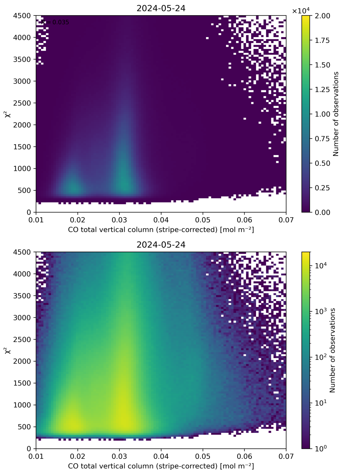
Figure 37: Scatter density plot of “CO total vertical column (stripe-corrected)” against “ \chi^2 ” for 2024-05-23 to 2024-05-25.
