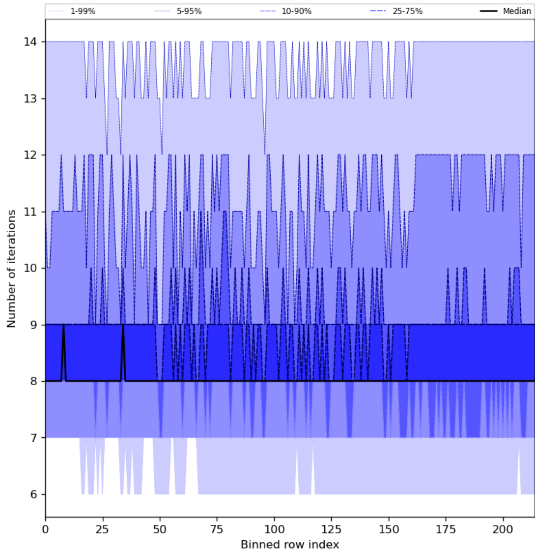
Figure 32: Along track statistics of “Number of iterations” for 2024-05-23 to 2024-05-25
