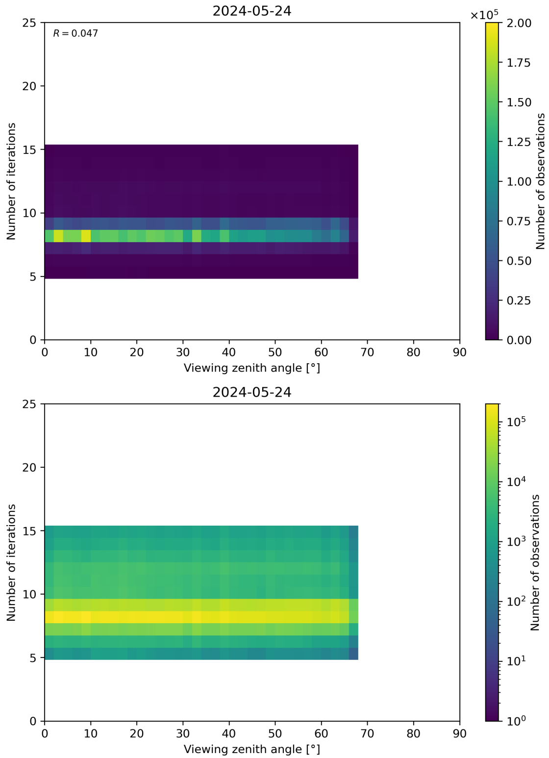
Figure 75: Scatter density plot of “Viewing zenith angle” against “Number of iterations” for 2024-05-23 to 2024-05-25.
