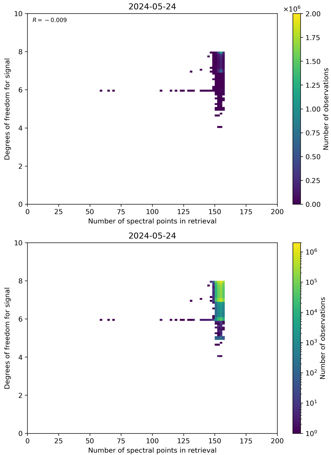
Figure 59: Scatter density plot of “Number of spectral points in retrieval” against “Degrees of freedom for signal” for 2024-05-23 to 2024-05-25.
