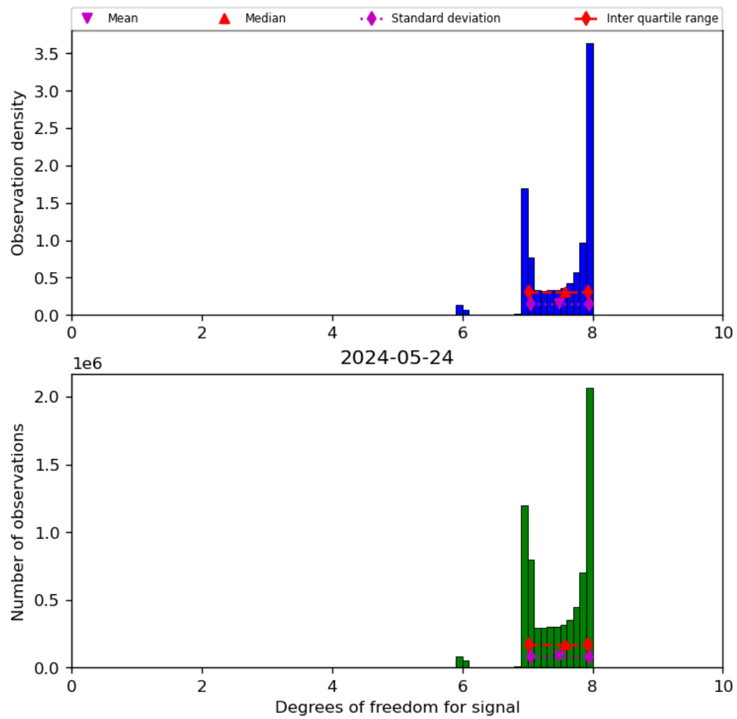
Figure 23: Histogram of “Degrees of freedom for signal” for 2024-05-23 to 2024-05-25
