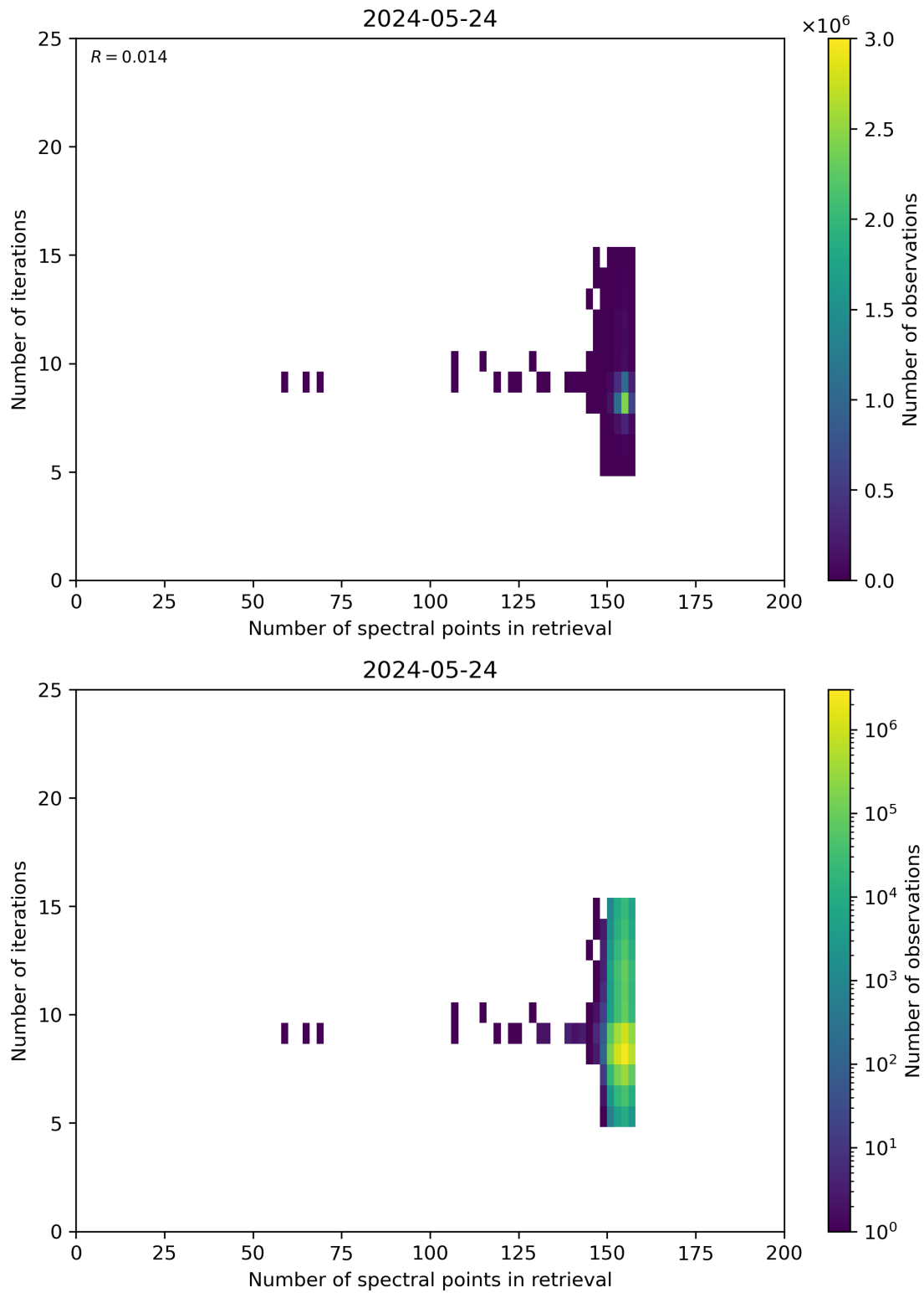
Figure 60: Scatter density plot of “Number of spectral points in retrieval” against “Number of iterations” for 2024-05-23 to 2024-05-25.
