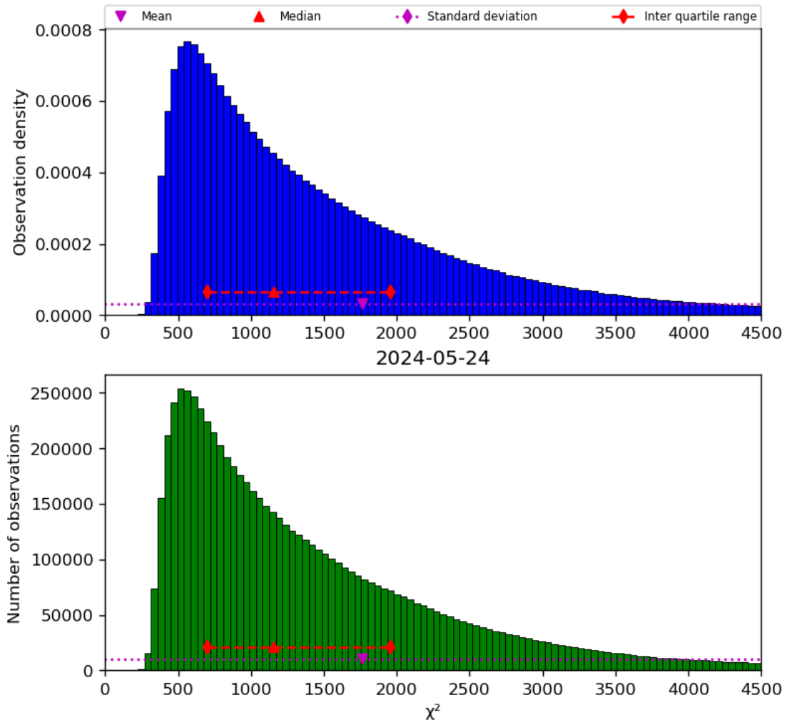
Figure 22: Histogram of “ \chi^2 ” for 2024-05-23 to 2024-05-25
