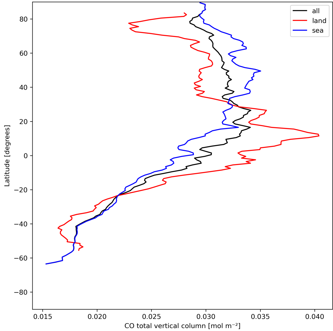
Figure 10: Zonal average of “CO total vertical column” for 2024-05-23 to 2024-05-25.
