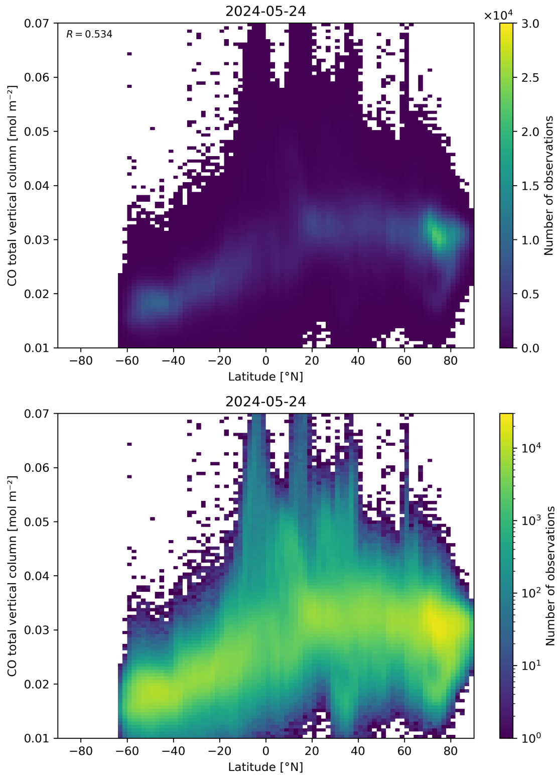
Figure 51: Scatter density plot of “Latitude” against “CO total vertical column” for 2024-05-23 to 2024-05-25.
