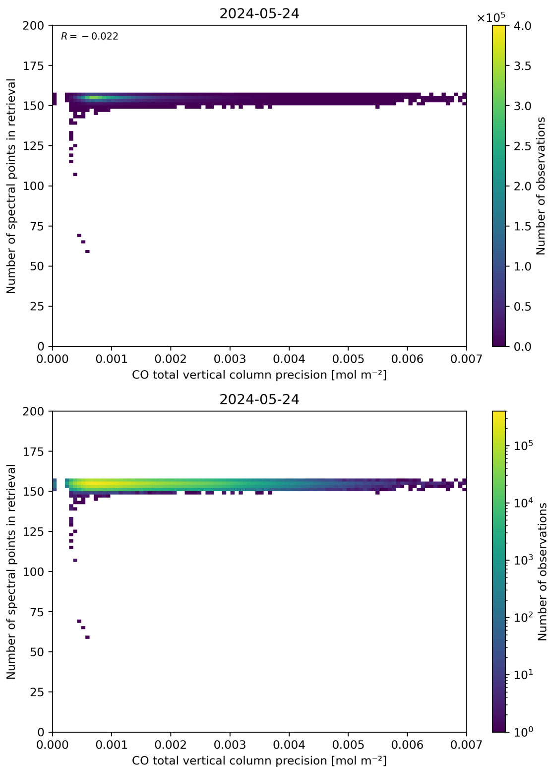
Figure 47: Scatter density plot of “CO total vertical column precision” against “Number of spectral points in retrieval” for 2024-05-23 to 2024-05-25.
