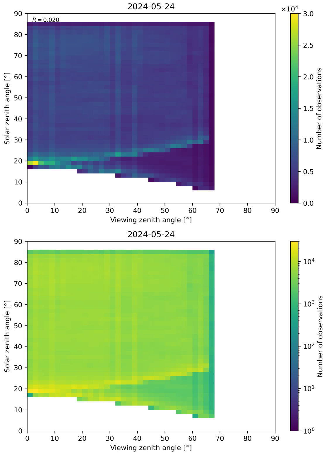
Figure 77: Scatter density plot of “Viewing zenith angle” against “Solar zenith angle” for 2024-05-23 to 2024-05-25.
