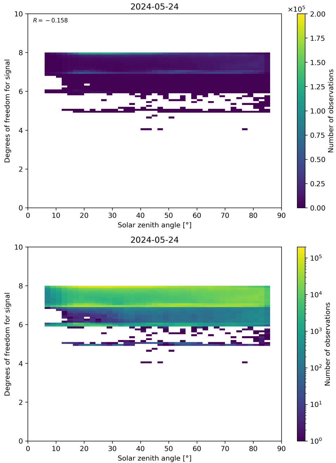
Figure 65: Scatter density plot of “Solar zenith angle” against “Degrees of freedom for signal” for 2024-05-23 to 2024-05-25.
