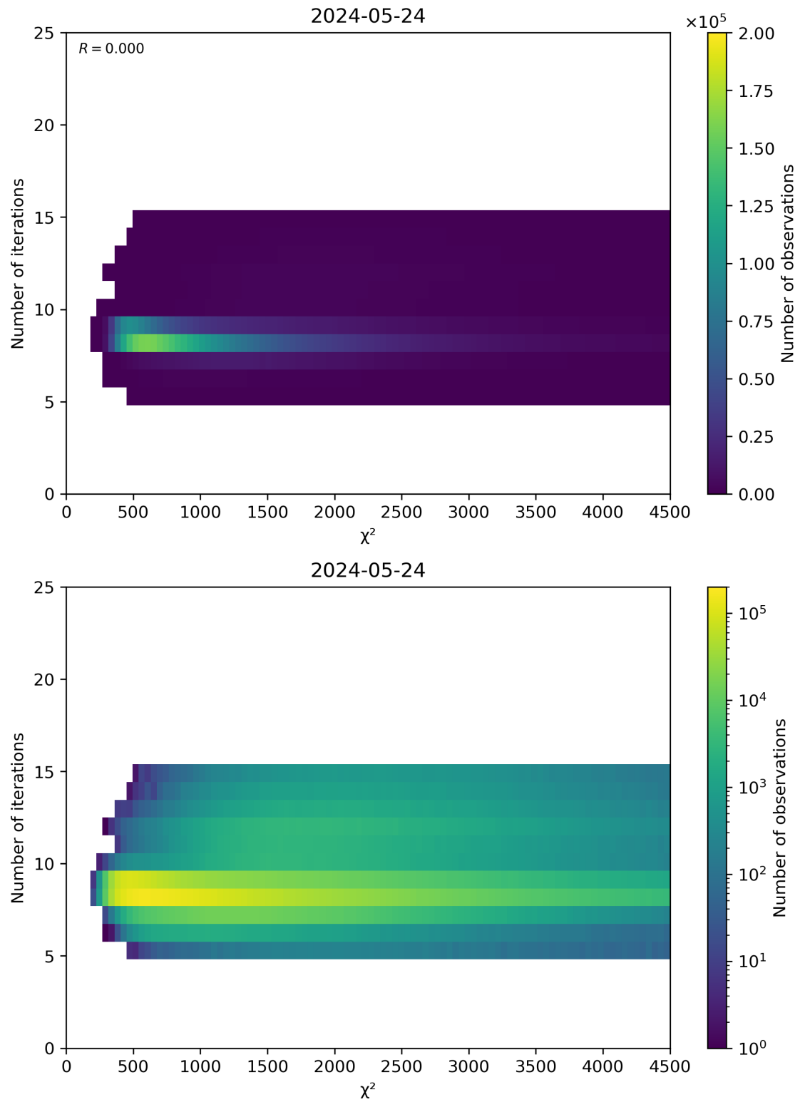
Figure 49: Scatter density plot of “ \chi^2 ” against “Number of iterations” for 2024-05-23 to 2024-05-25.
