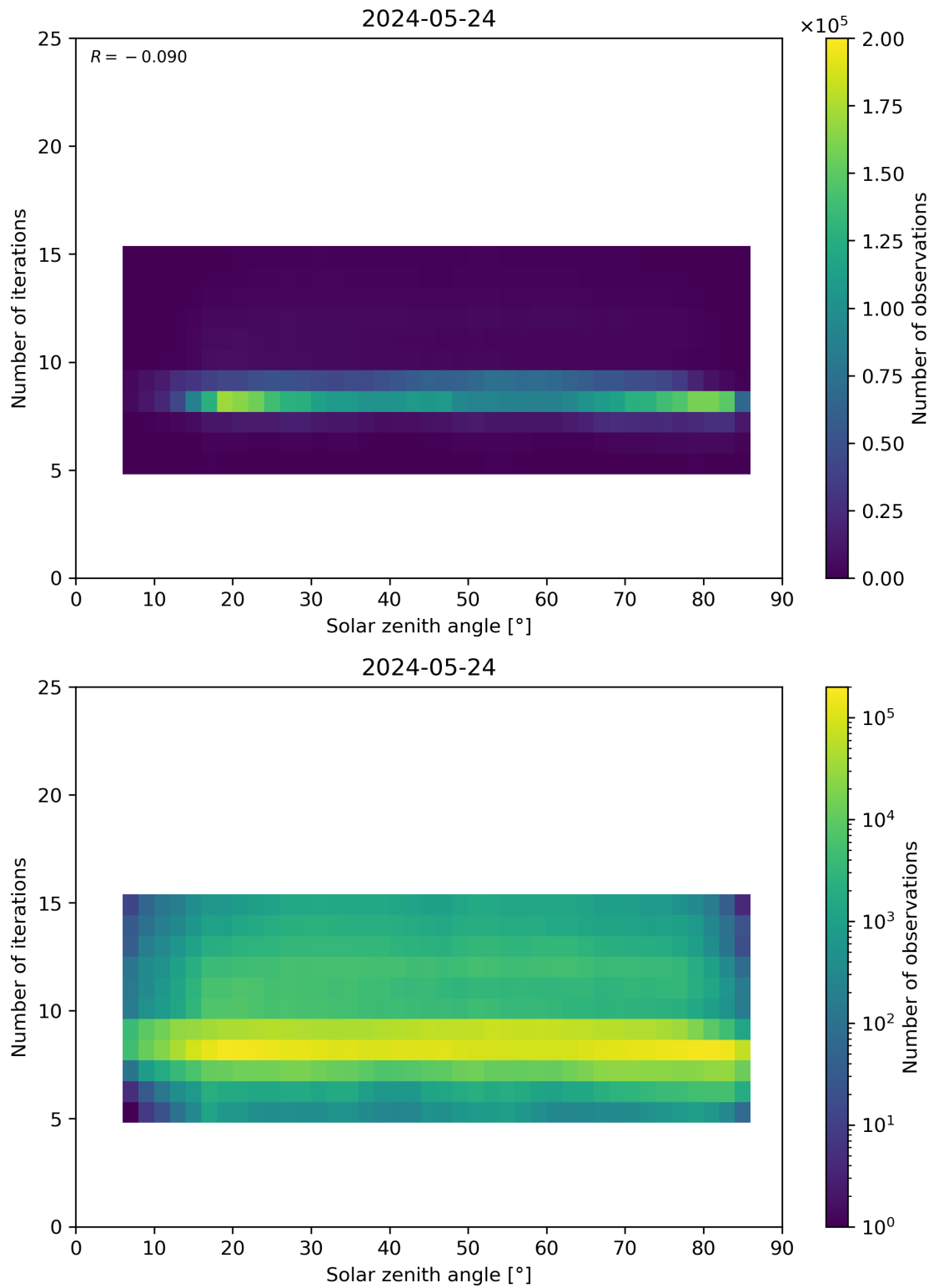
Figure 67: Scatter density plot of “Solar zenith angle” against “Number of iterations” for 2024-05-23 to 2024-05-25.
