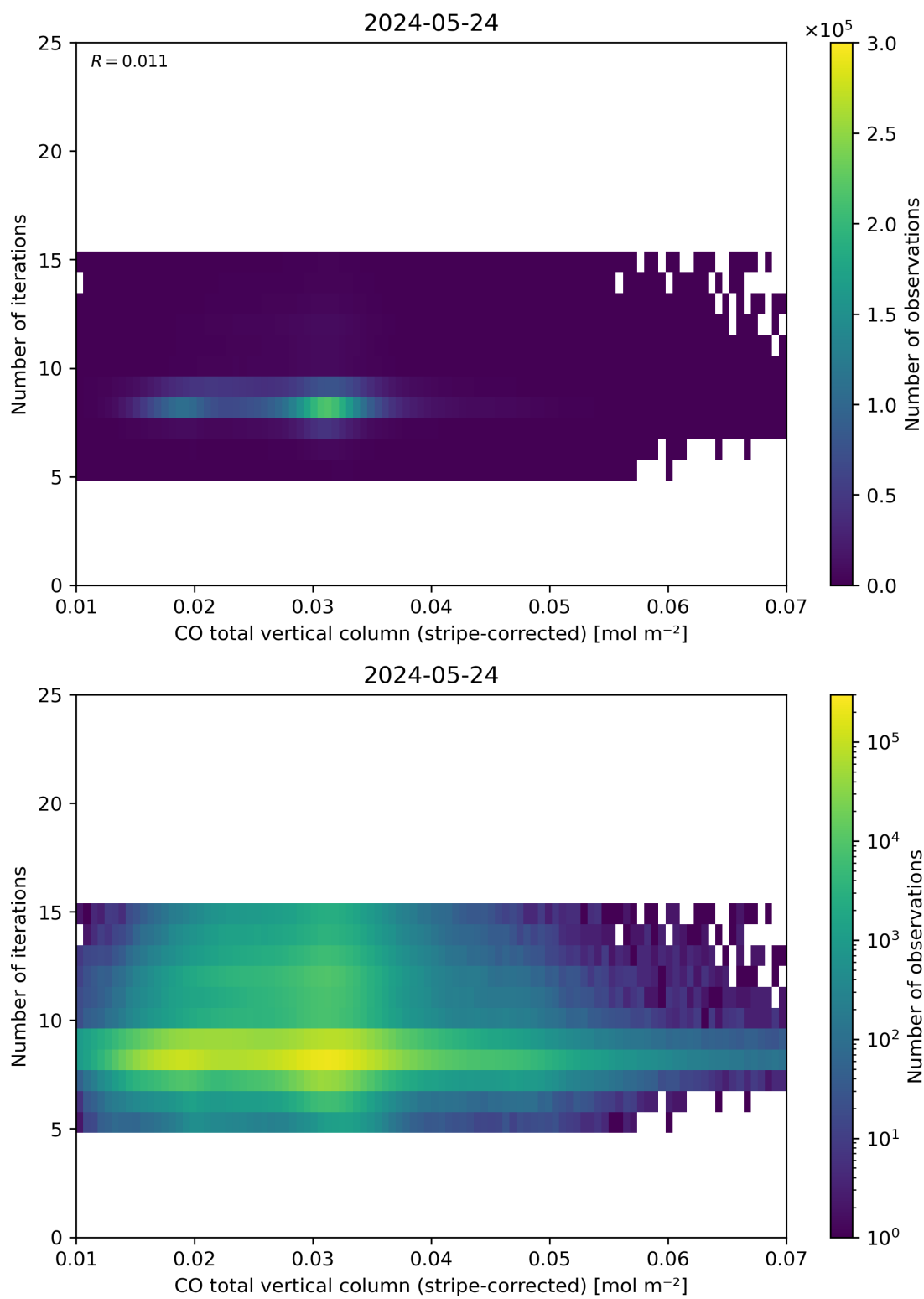
Figure 39: Scatter density plot of “CO total vertical column (stripe-corrected)” against “Number of iterations” for 2024-05-23 to 2024-05-25.
