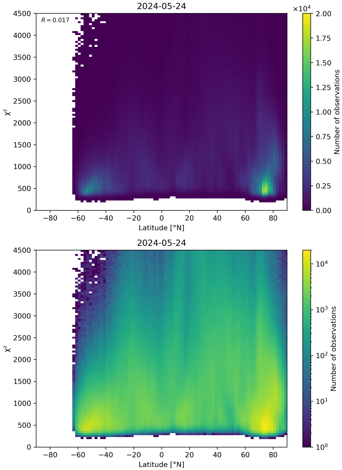
Figure 54: Scatter density plot of “Latitude” against “ \chi^2 ” for 2024-05-23 to 2024-05-25.
