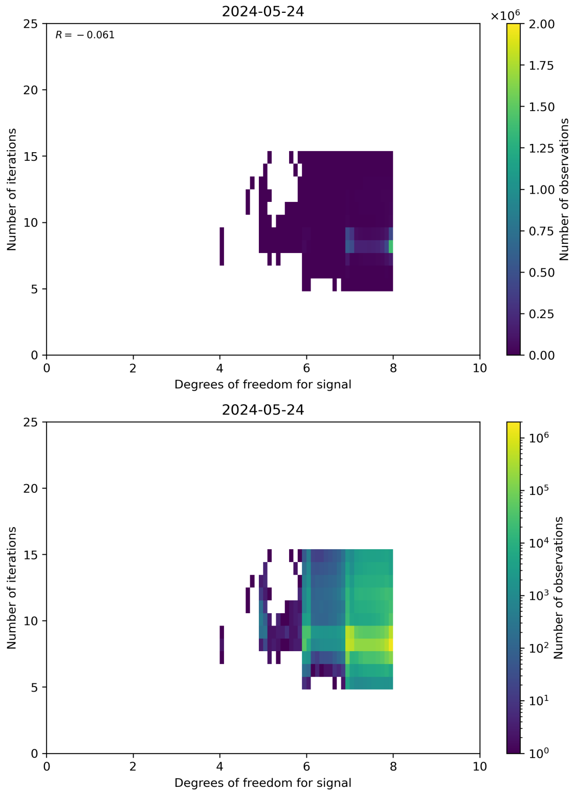
Figure 50: Scatter density plot of “Degrees of freedom for signal” against “Number of iterations” for 2024-05-23 to 2024-05-25.
