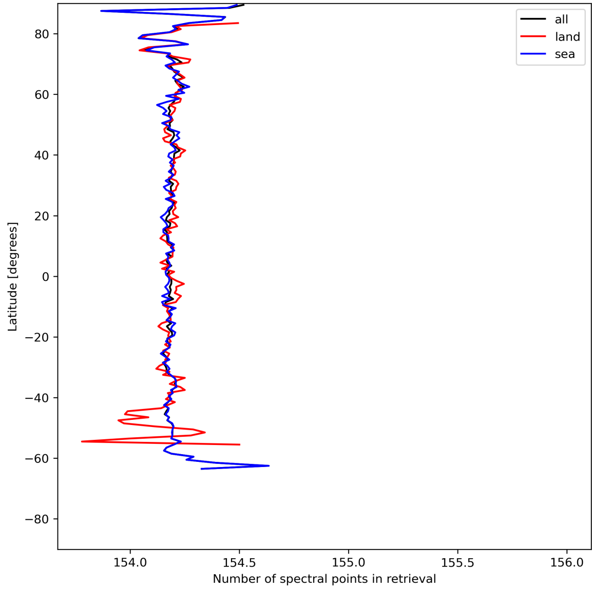
Figure 13: Zonal average of “Number of spectral points in retrieval” for 2024-05-23 to 2024-05-25.
