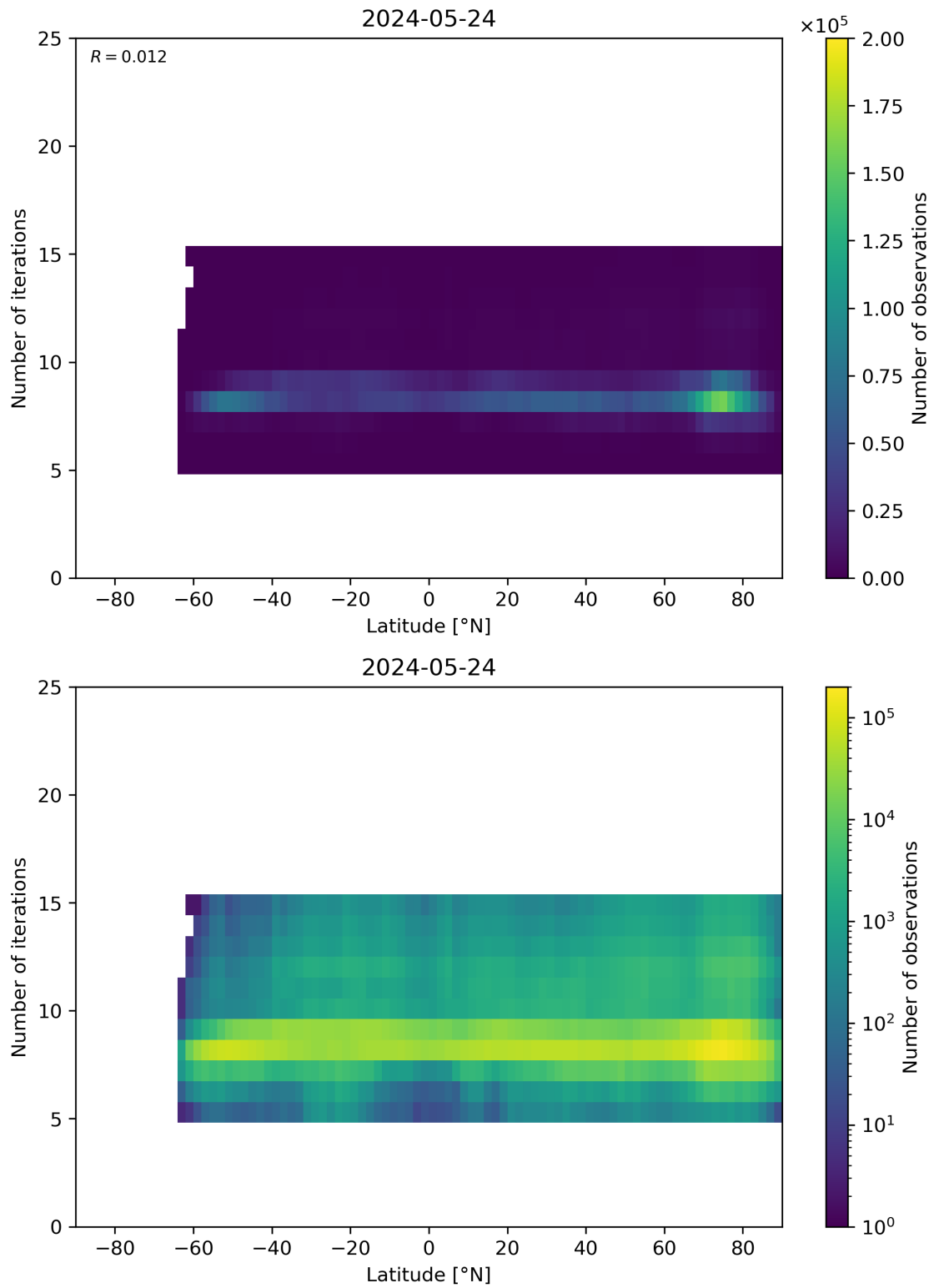
Figure 56: Scatter density plot of “Latitude” against “Number of iterations” for 2024-05-23 to 2024-05-25.
