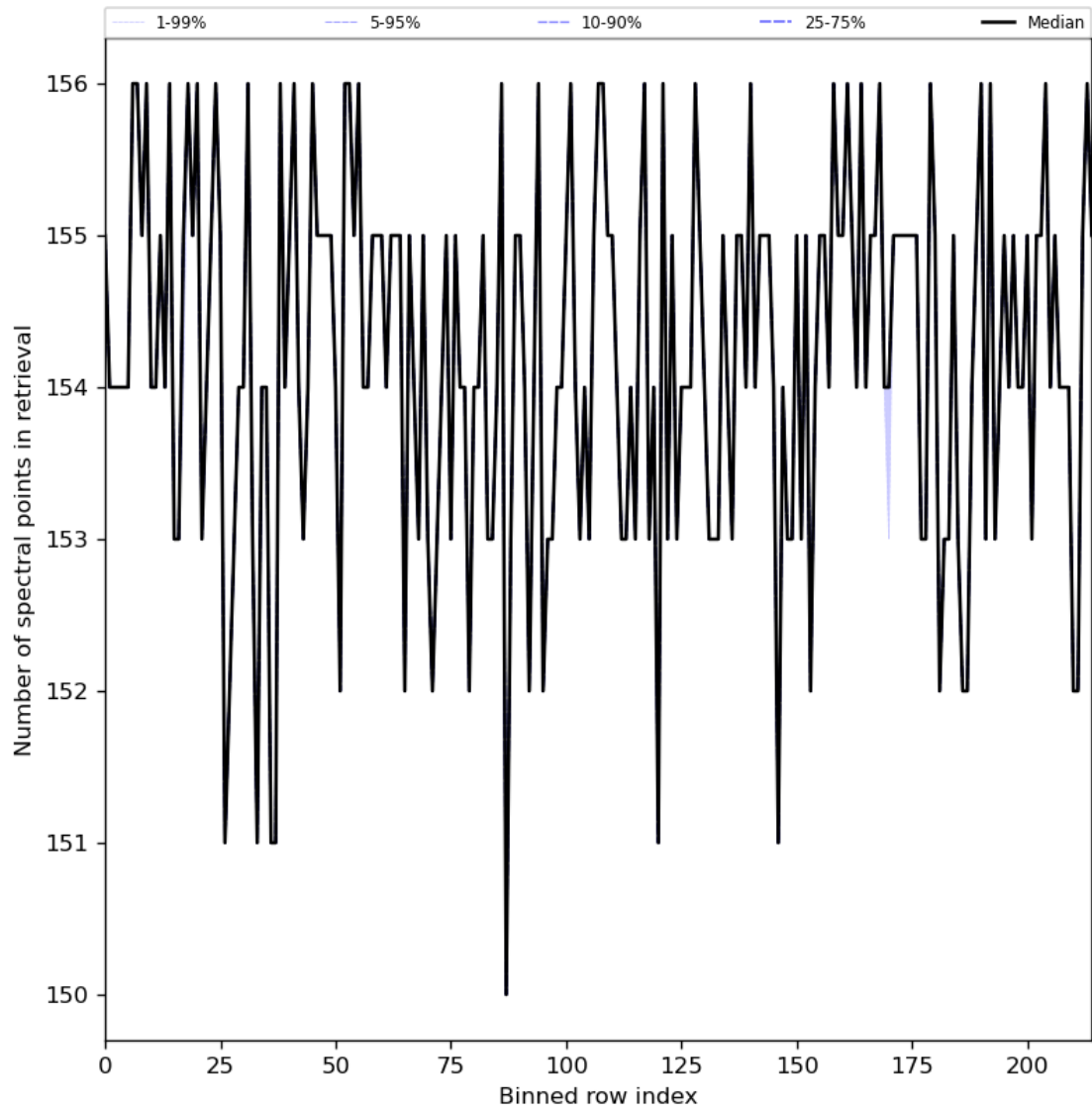
Figure 29: Along track statistics of “Number of spectral points in retrieval” for 2024-05-23 to 2024-05-25
