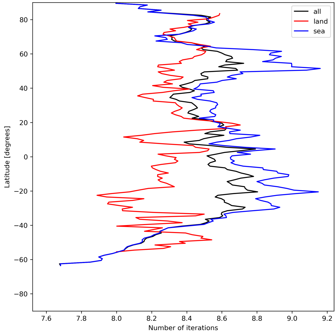
Figure 16: Zonal average of “Number of iterations” for 2024-05-23 to 2024-05-25.
