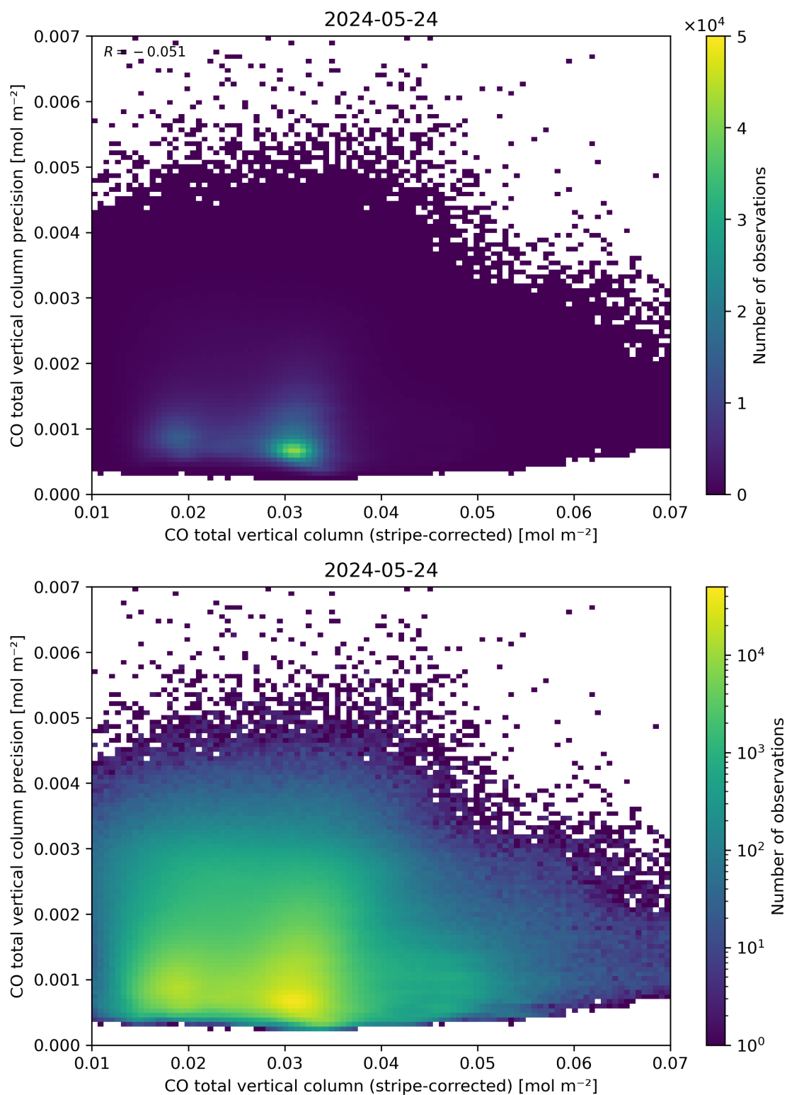
Figure 36: Scatter density plot of “CO total vertical column (stripe-corrected)” against “CO total vertical column precision” for 2024-05-23 to 2024-05-25.
