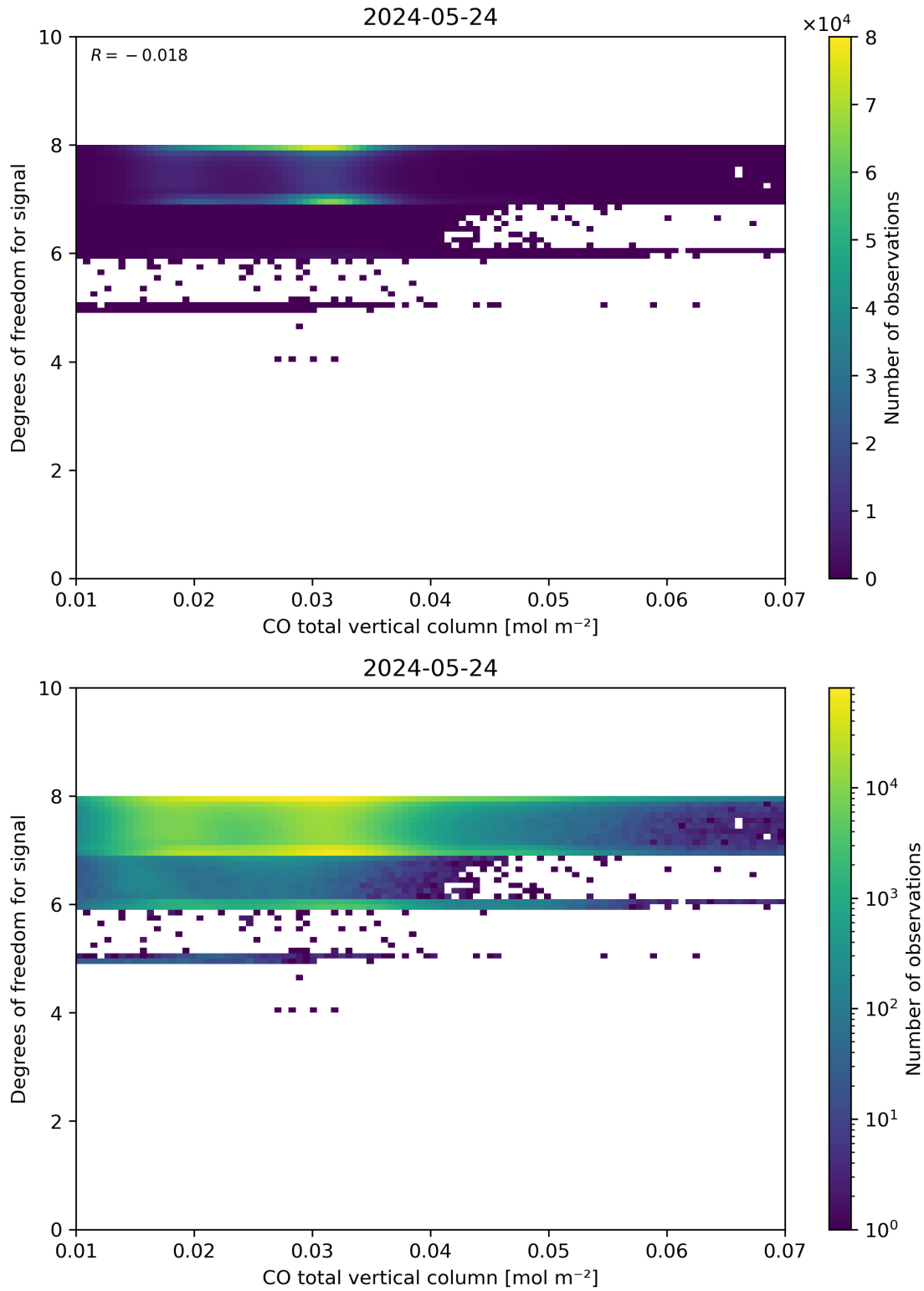
Figure 41: Scatter density plot of “CO total vertical column” against “Degrees of freedom for signal” for 2024-05-23 to 2024-05-25.
