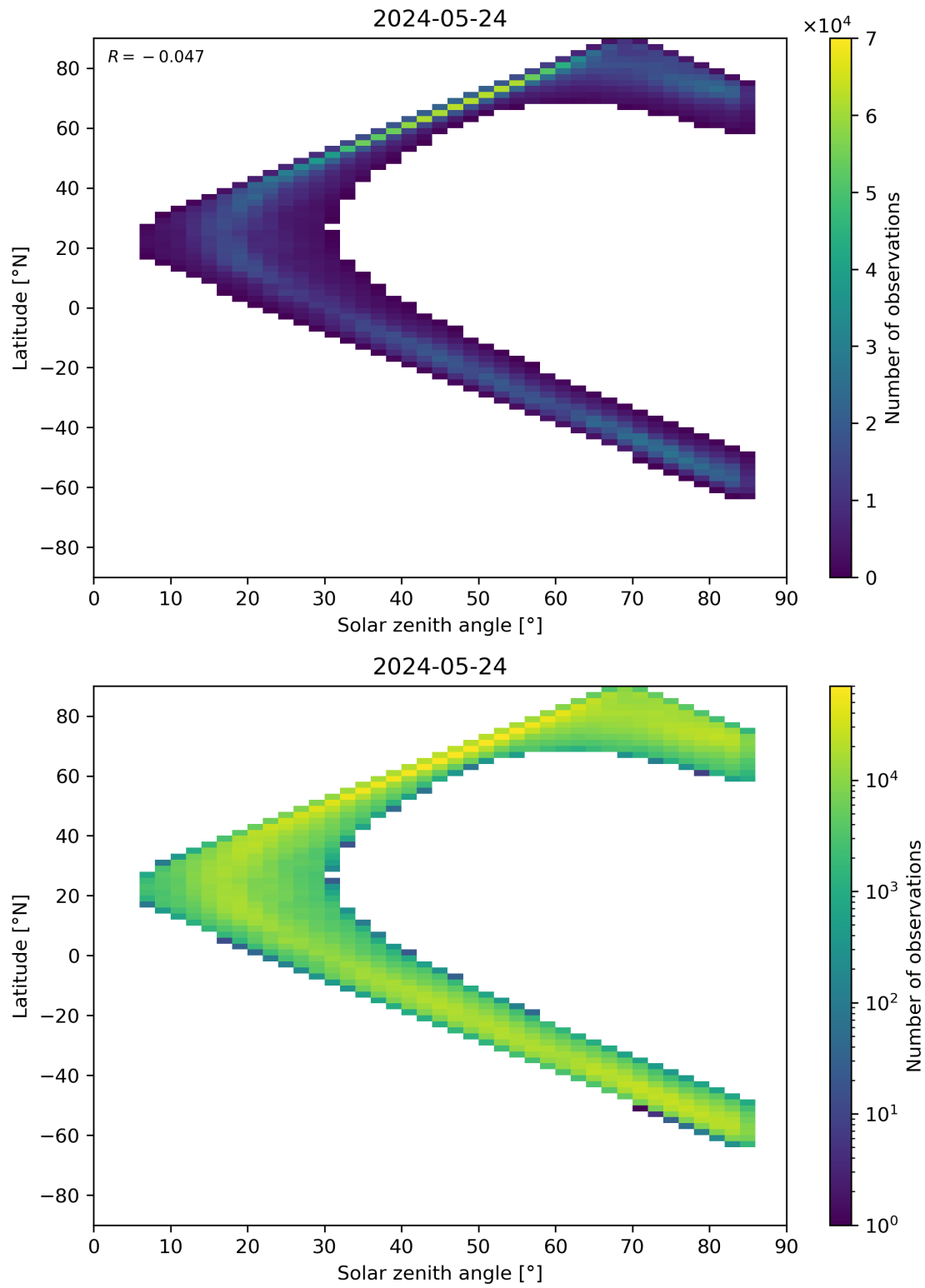
Figure 66: Scatter density plot of “Solar zenith angle” against “Latitude” for 2024-05-23 to 2024-05-25.
