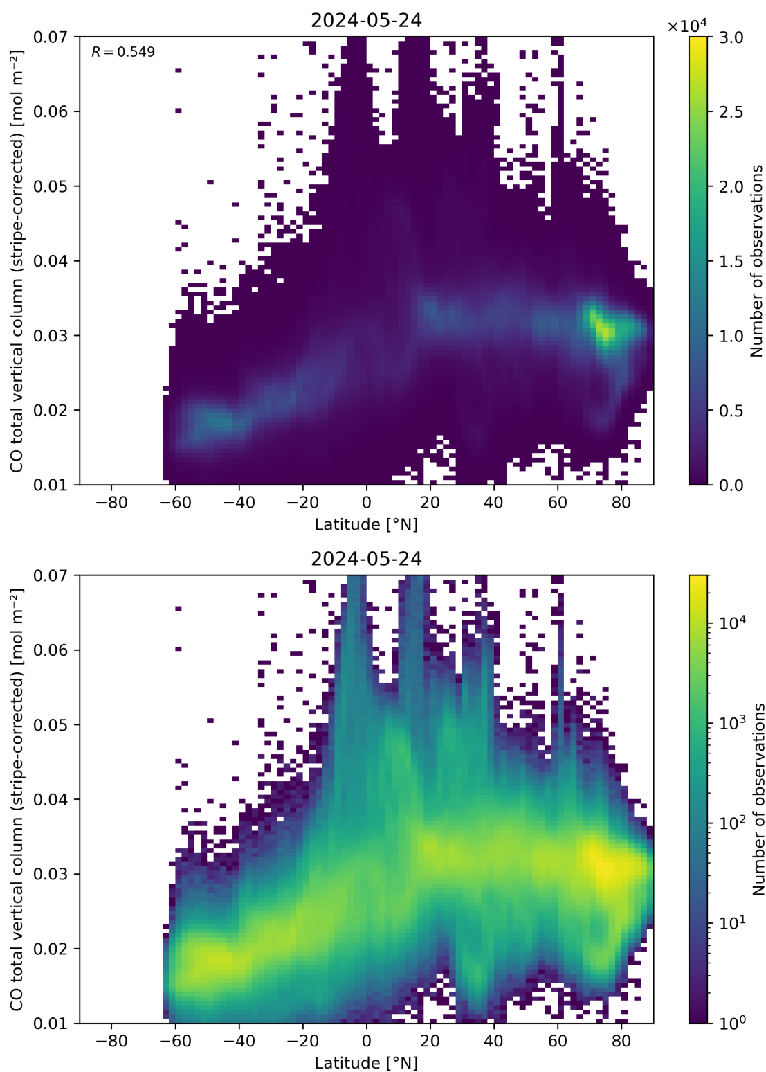
Figure 52: Scatter density plot of “Latitude” against “CO total vertical column (stripe-corrected)” for 2024-05-23 to 2024-05-25.
