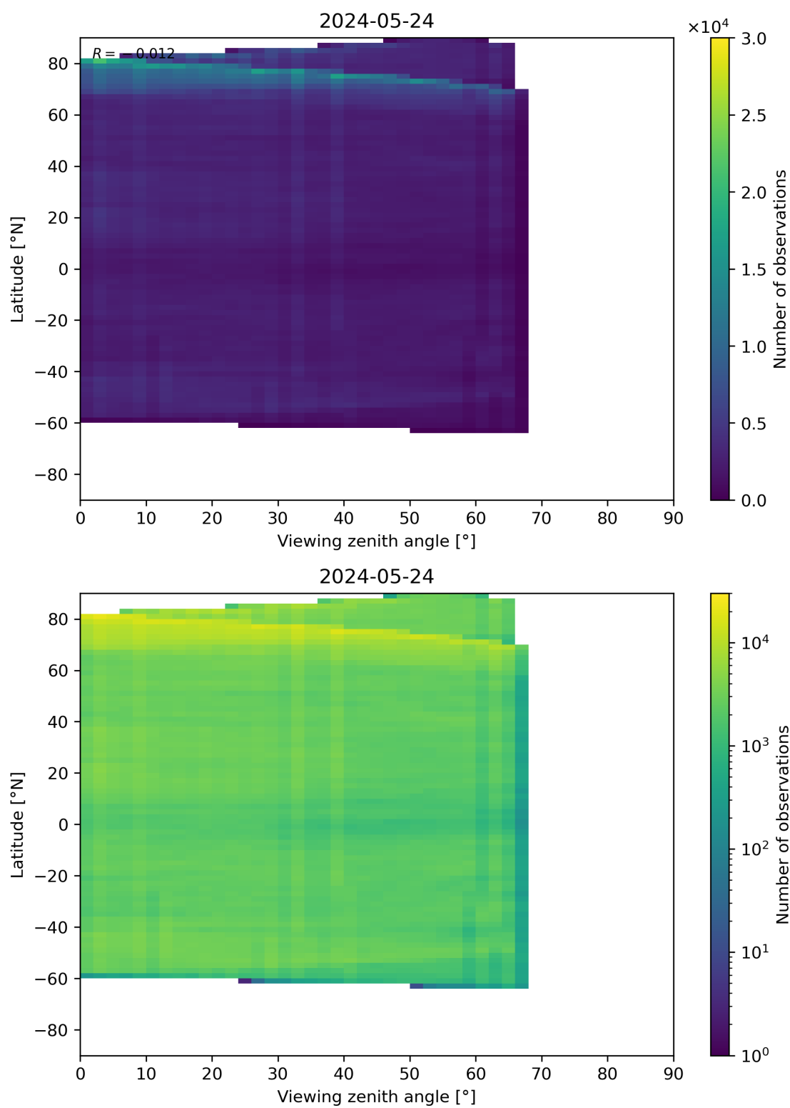
Figure 74: Scatter density plot of “Viewing zenith angle” against “Latitude” for 2024-05-23 to 2024-05-25.
