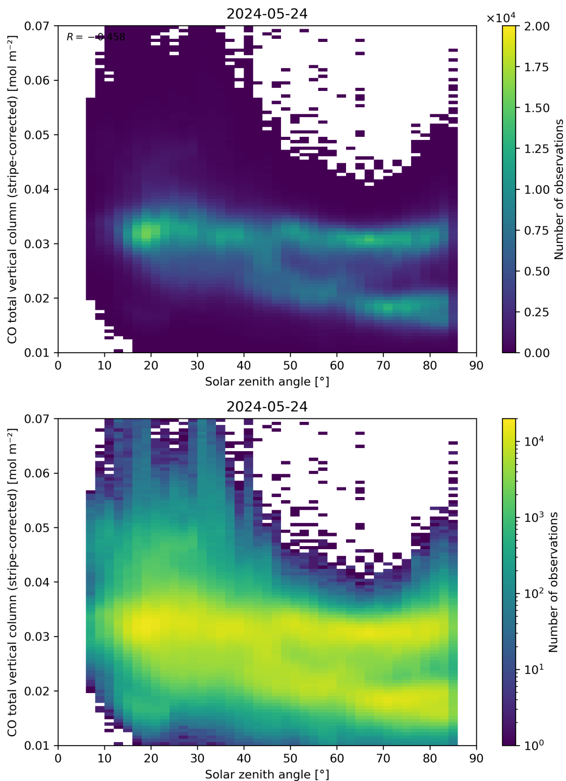
Figure 62: Scatter density plot of “Solar zenith angle” against “CO total vertical column (stripe-corrected)” for 2024-05-23 to 2024-05-25.
