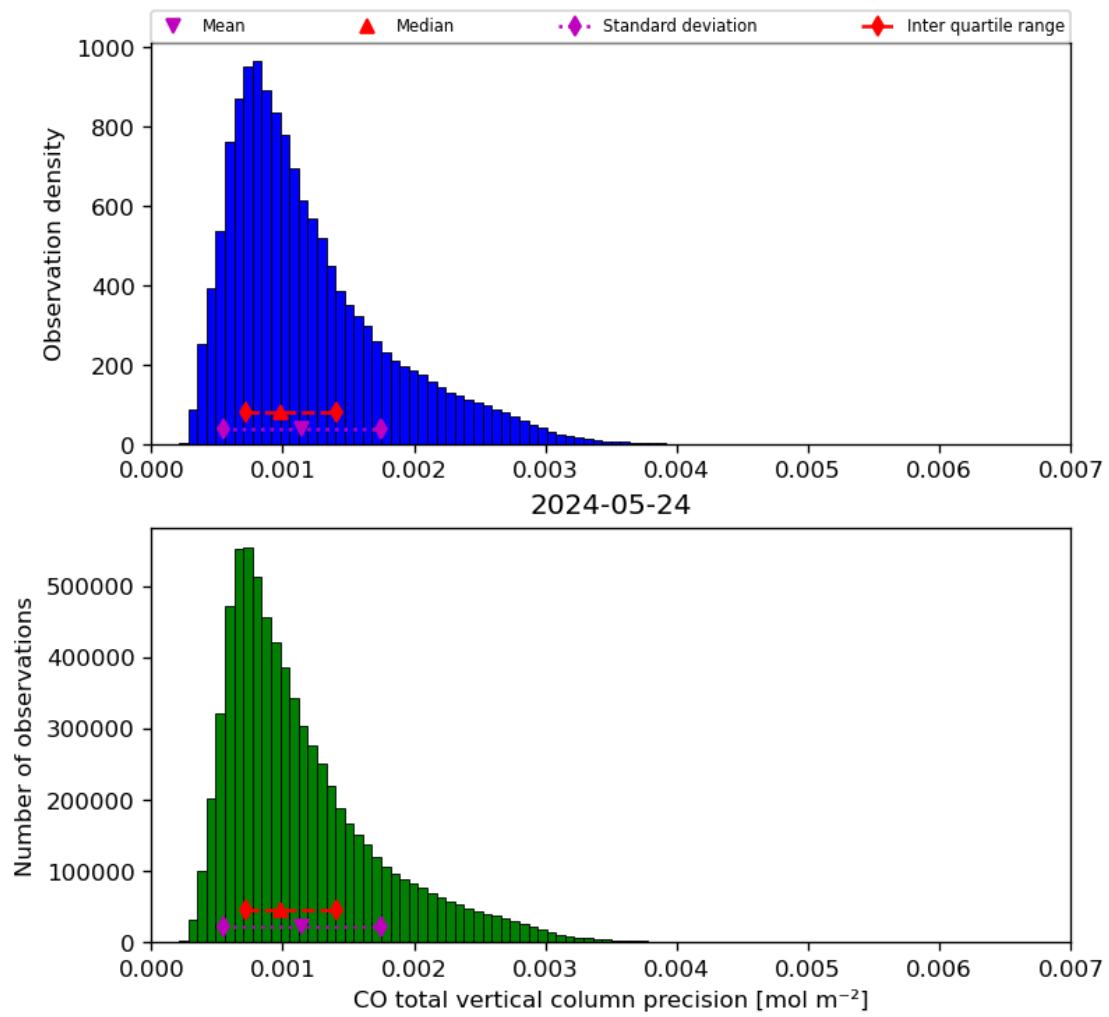
Figure 20: Histogram of “CO total vertical column precision” for 2024-05-23 to 2024-05-25
