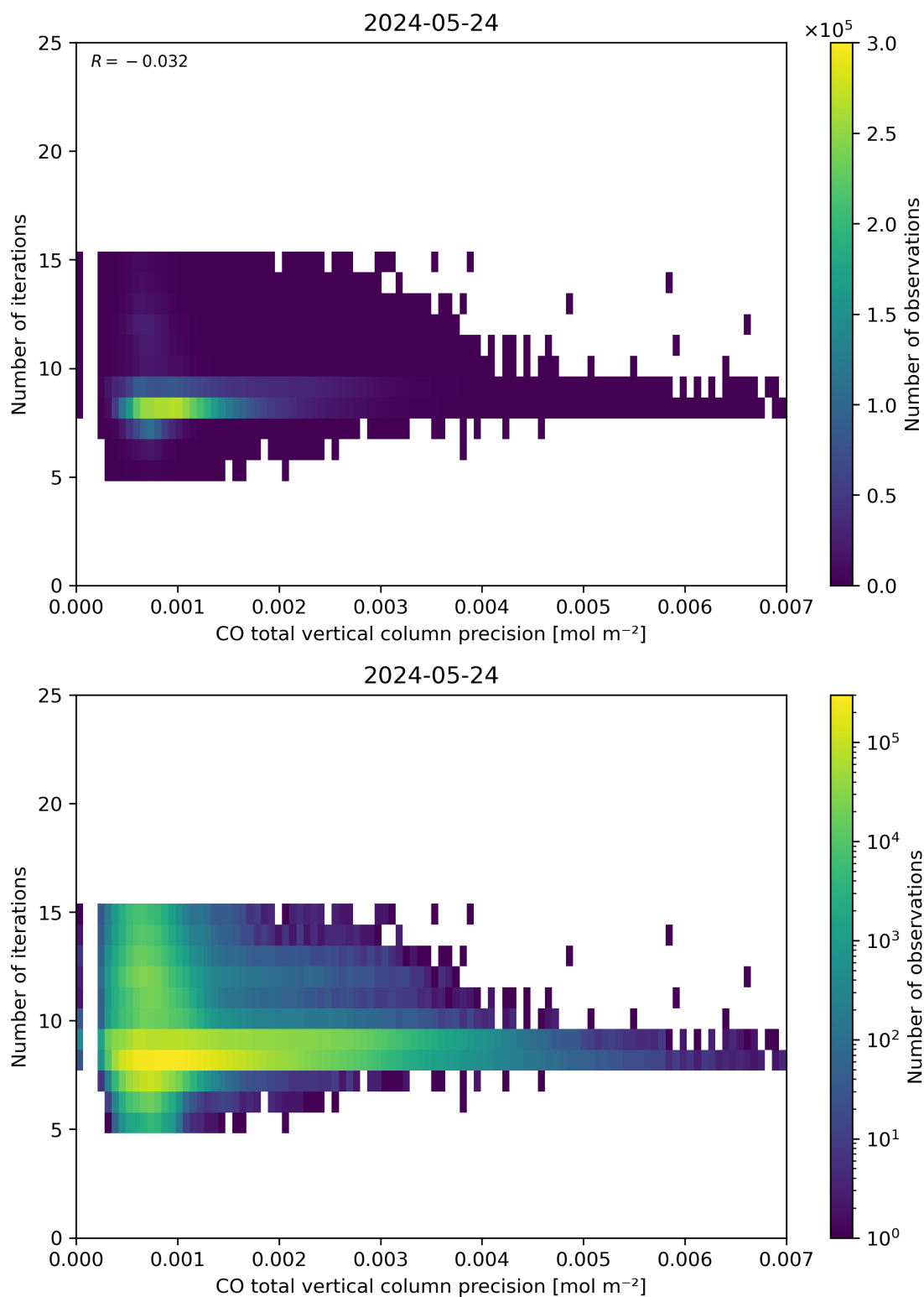
Figure 46: Scatter density plot of “CO total vertical column precision” against “Number of iterations” for 2024-05-23 to 2024-05-25.
