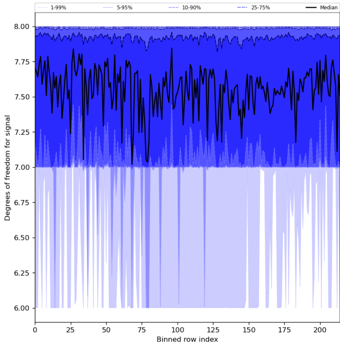
Figure 31: Along track statistics of “Degrees of freedom for signal” for 2024-05-23 to 2024-05-25
