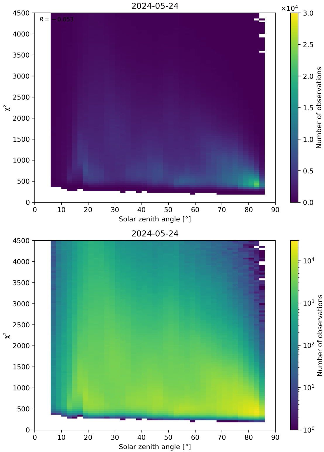
Figure 64: Scatter density plot of “Solar zenith angle” against “ \chi^2 ” for 2024-05-23 to 2024-05-25.
