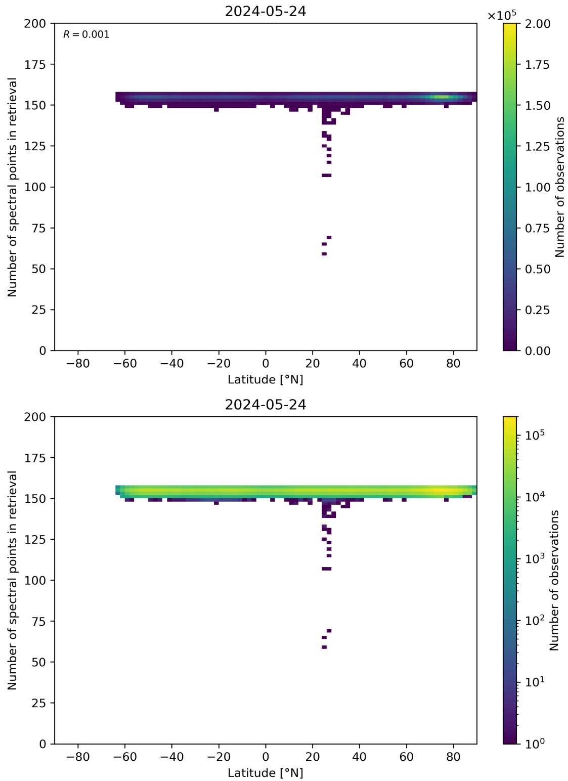
Figure 57: Scatter density plot of “Latitude” against “Number of spectral points in retrieval” for 2024-05-23 to 2024-05-25.
