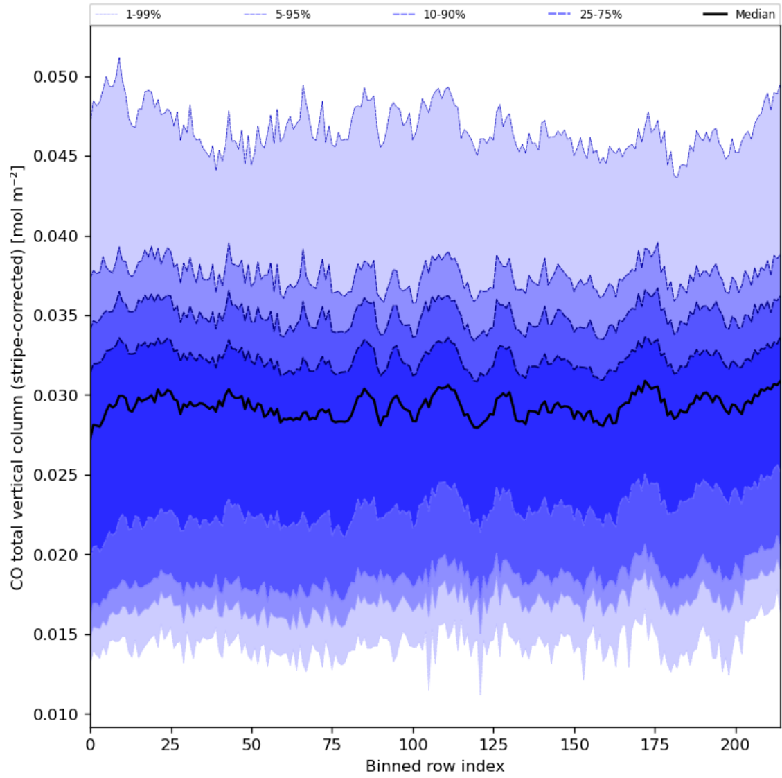
Figure 27: Along track statistics of “CO total vertical column (stripe-corrected)” for 2024-05-23 to 2024-05-25
