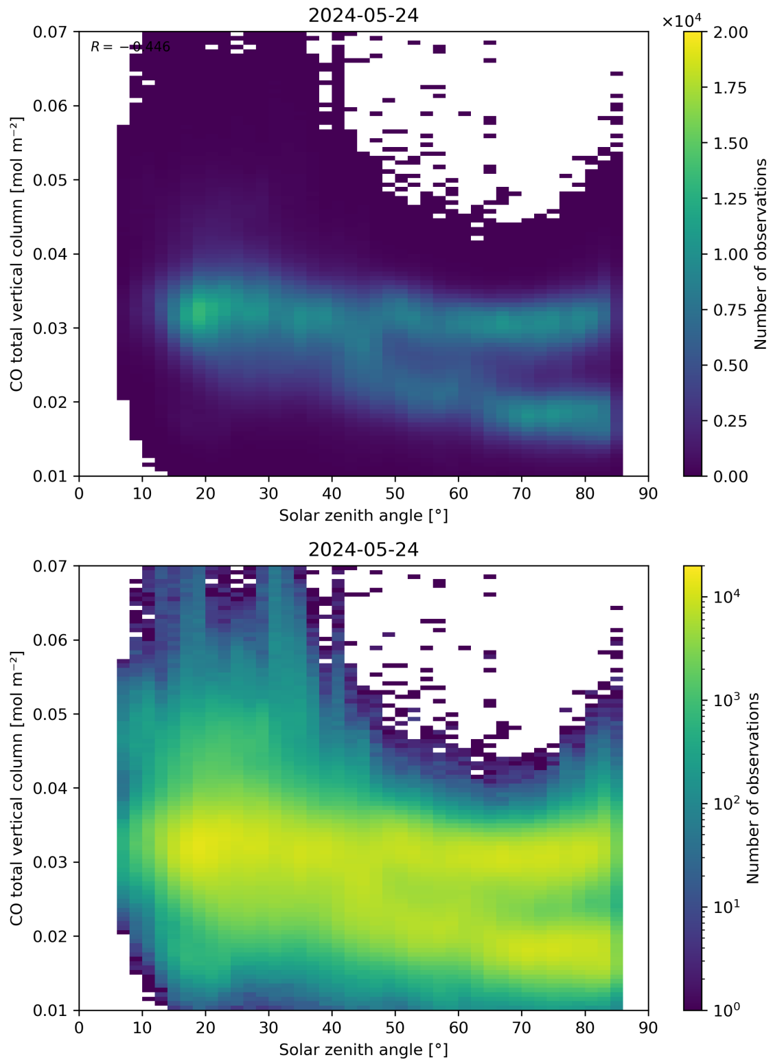
Figure 61: Scatter density plot of “Solar zenith angle” against “CO total vertical column” for 2024-05-23 to 2024-05-25.
