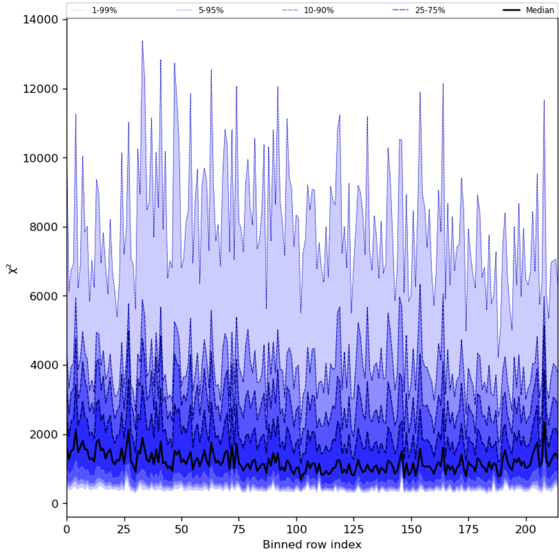
Figure 30: Along track statistics of “ \chi^2 ” for 2024-05-23 to 2024-05-25
