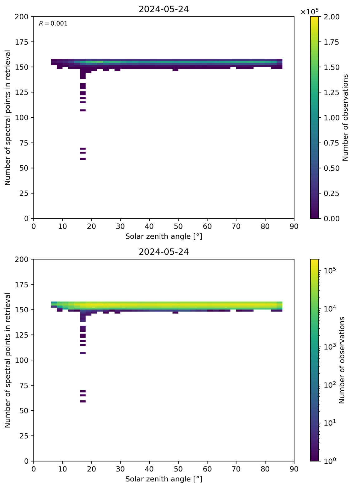
Figure 68: Scatter density plot of “Solar zenith angle” against “Number of spectral points in retrieval” for 2024-05-23 to 2024-05-25.
