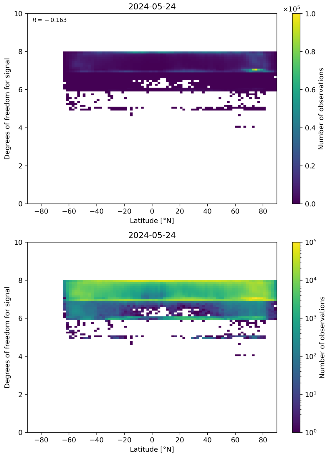
Figure 55: Scatter density plot of “Latitude” against “Degrees of freedom for signal” for 2024-05-23 to 2024-05-25.
