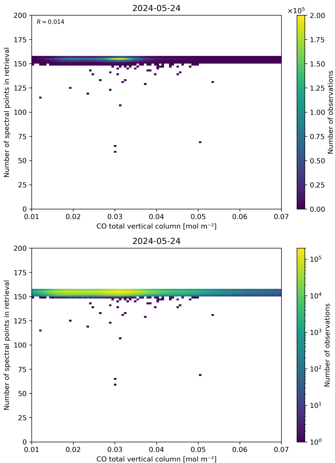
Figure 43: Scatter density plot of “CO total vertical column” against “Number of spectral points in retrieval” for 2024-05-23 to 2024-05-25.
