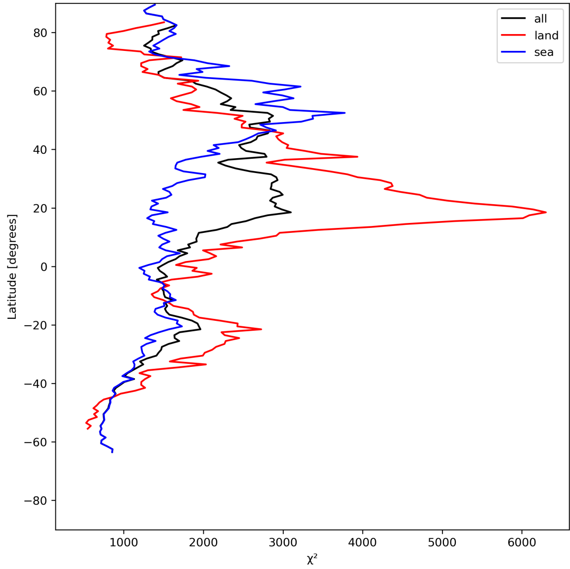
Figure 14: Zonal average of “ \chi^2 ” for 2024-05-23 to 2024-05-25.
