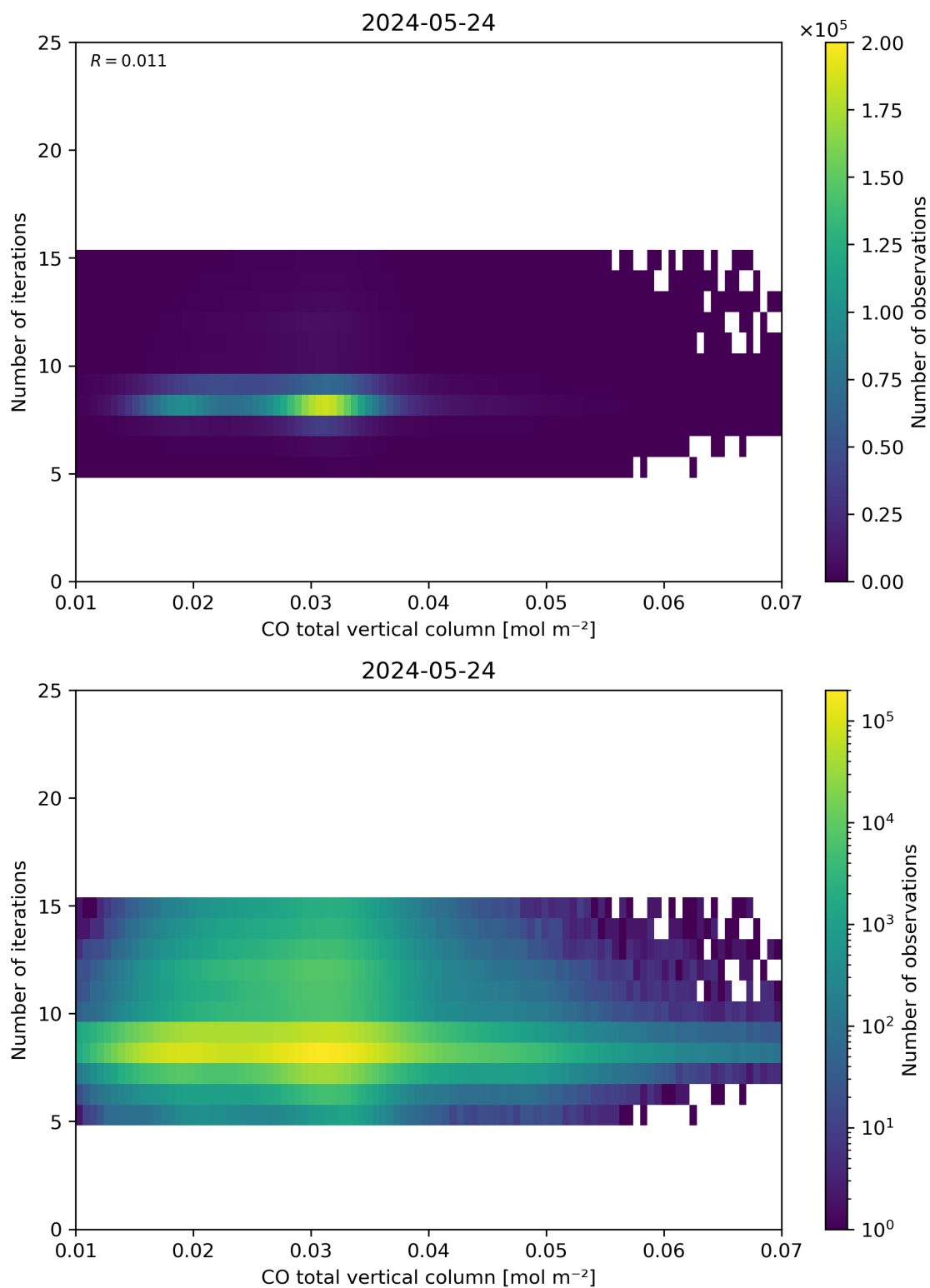
Figure 42: Scatter density plot of “CO total vertical column” against “Number of iterations” for 2024-05-23 to 2024-05-25.
