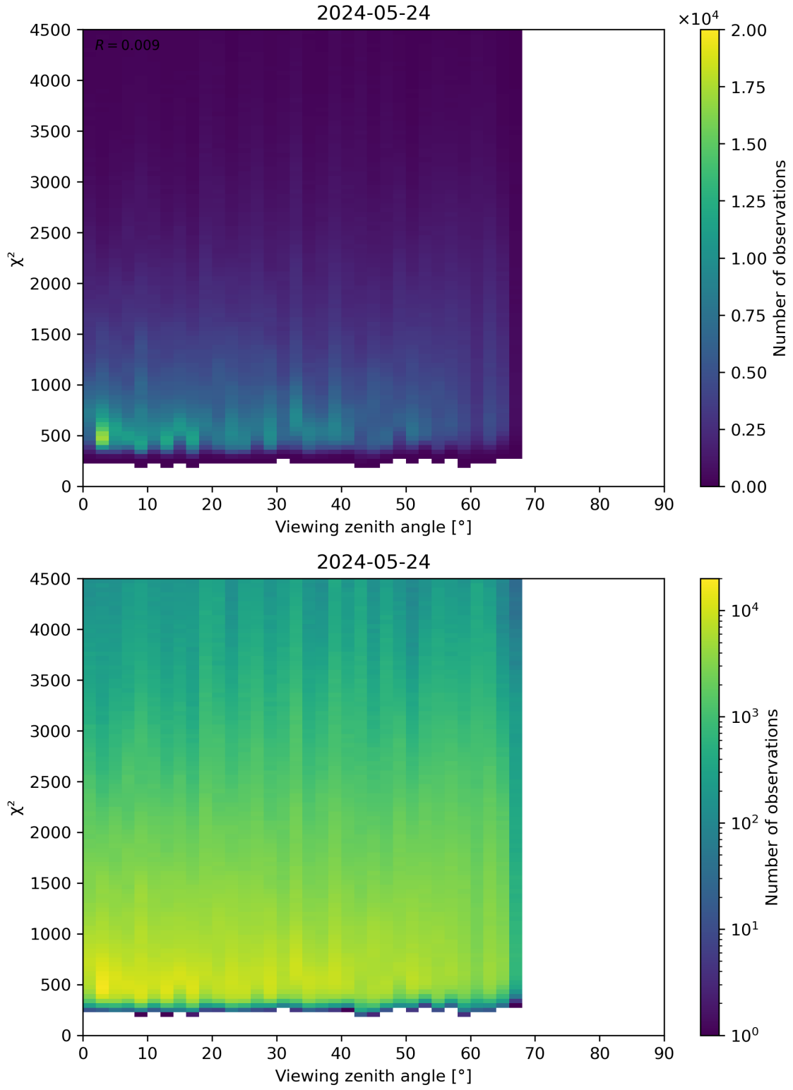
Figure 72: Scatter density plot of “Viewing zenith angle” against “ \chi^2 ” for 2024-05-23 to 2024-05-25.
