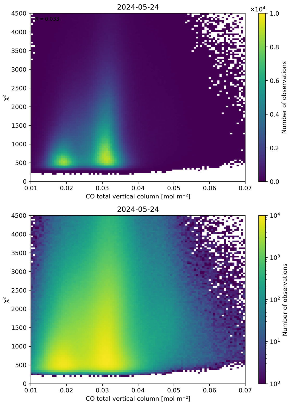
Figure 35: Scatter density plot of “CO total vertical column” against “ \chi^2 ” for 2024-05-23 to 2024-05-25.
