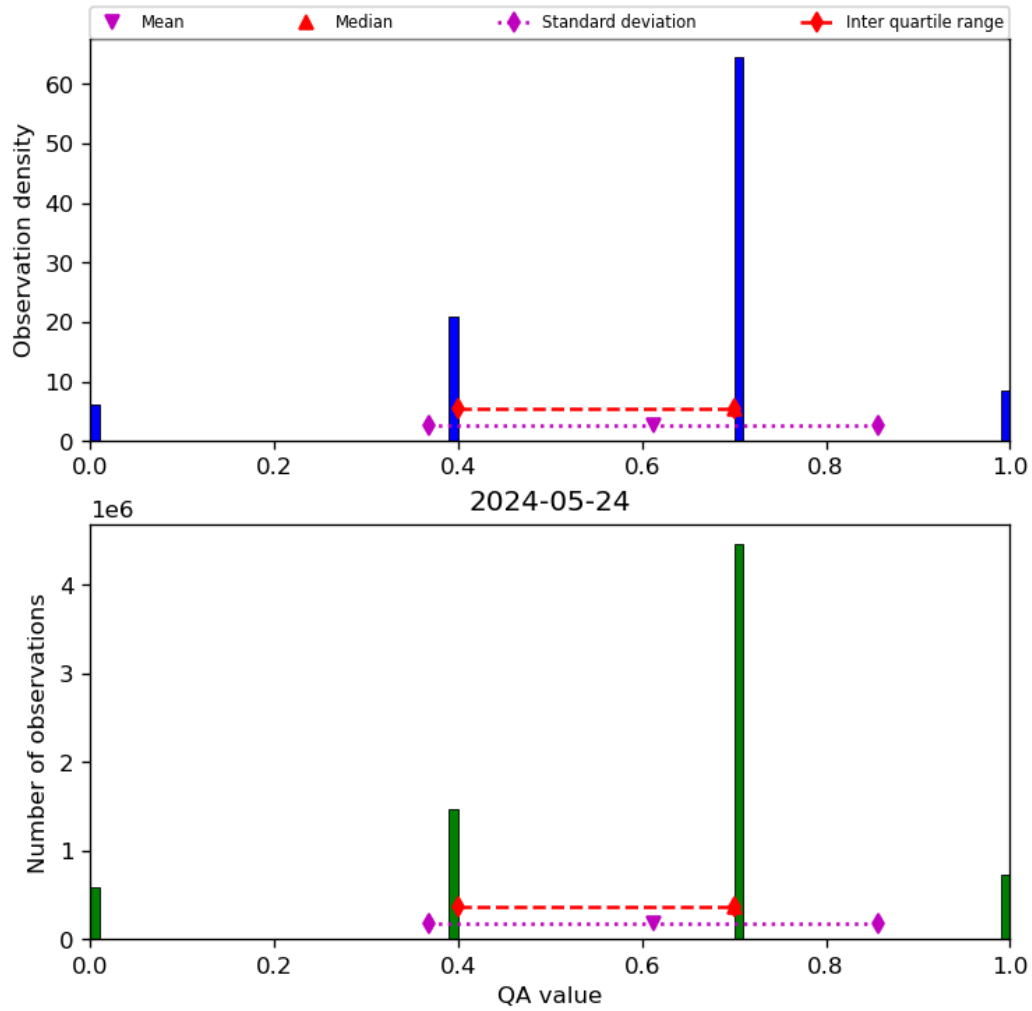
Figure 17: Histogram of “QA value” for 2024-05-23 to 2024-05-25
