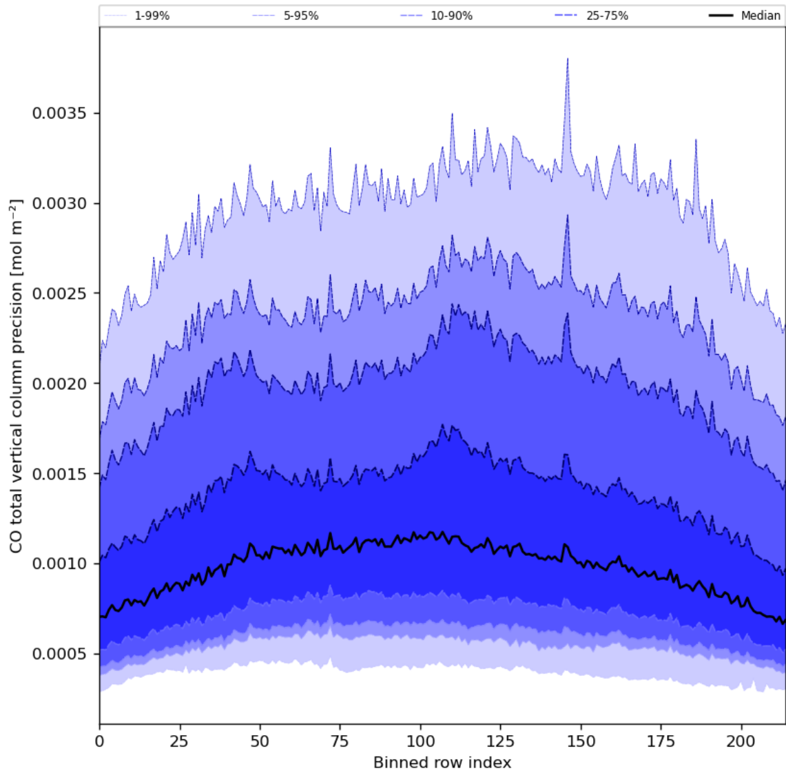
Figure 28: Along track statistics of “CO total vertical column precision” for 2024-05-23 to 2024-05-25
