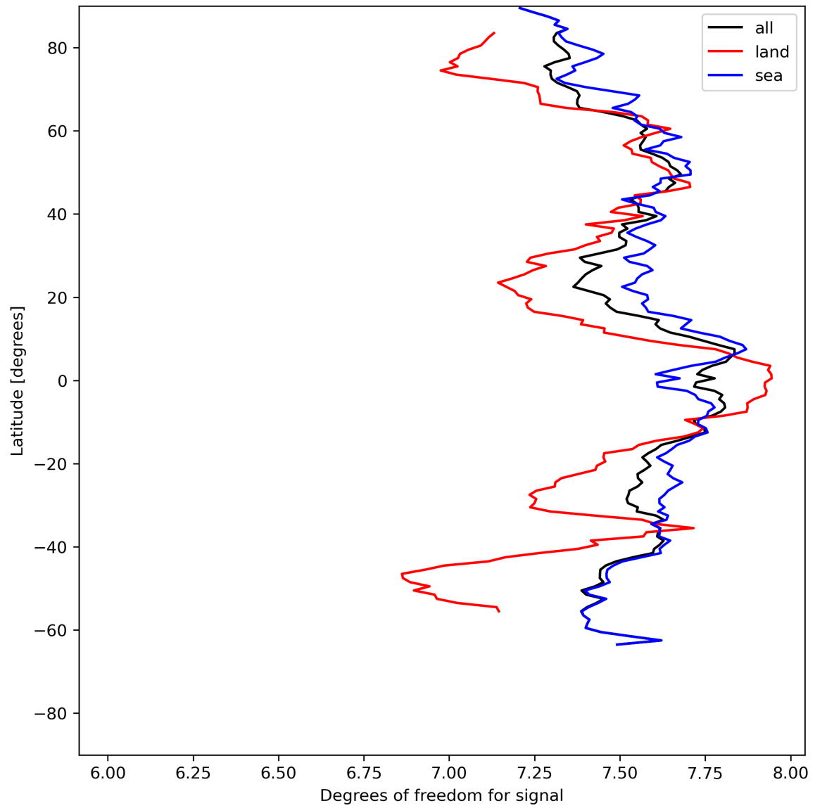
Figure 15: Zonal average of “Degrees of freedom for signal” for 2024-05-23 to 2024-05-25.
