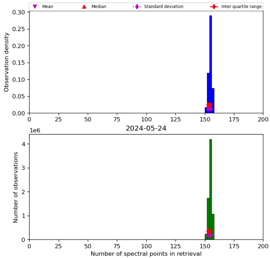
Figure 21: Histogram of “Number of spectral points in retrieval” for 2024-05-23 to 2024-05-25
