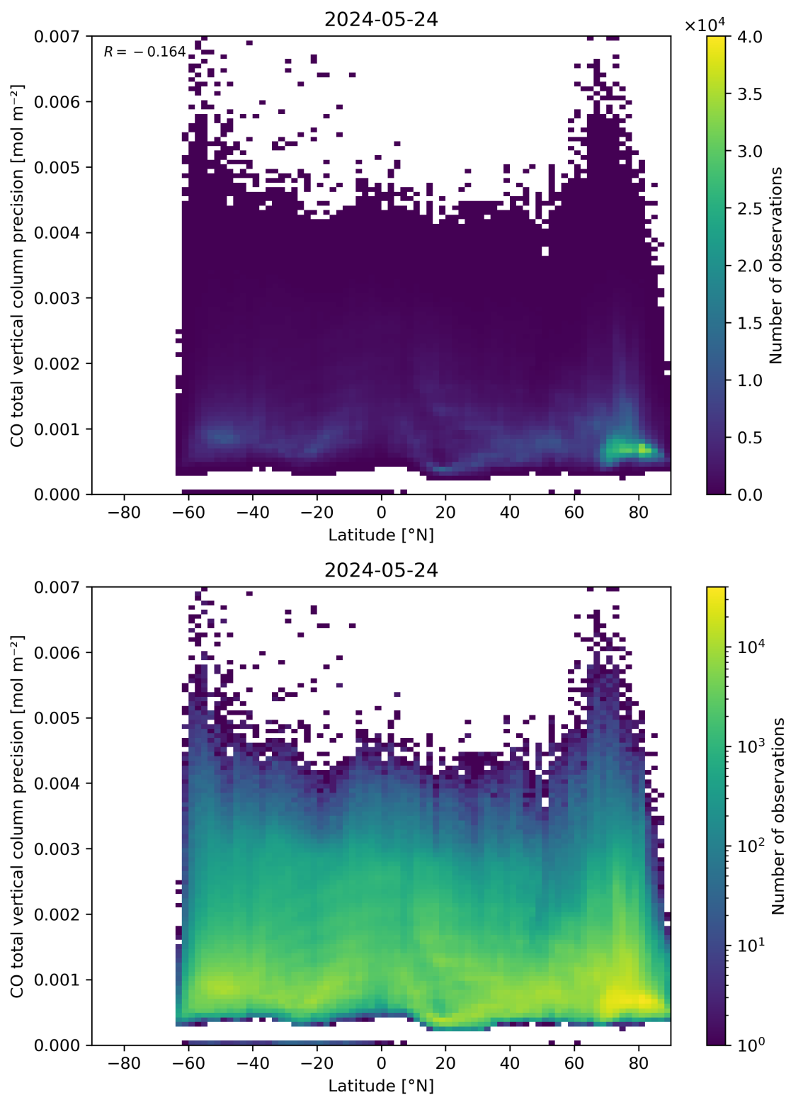
Figure 53: Scatter density plot of “Latitude” against “CO total vertical column precision” for 2024-05-23 to 2024-05-25.
