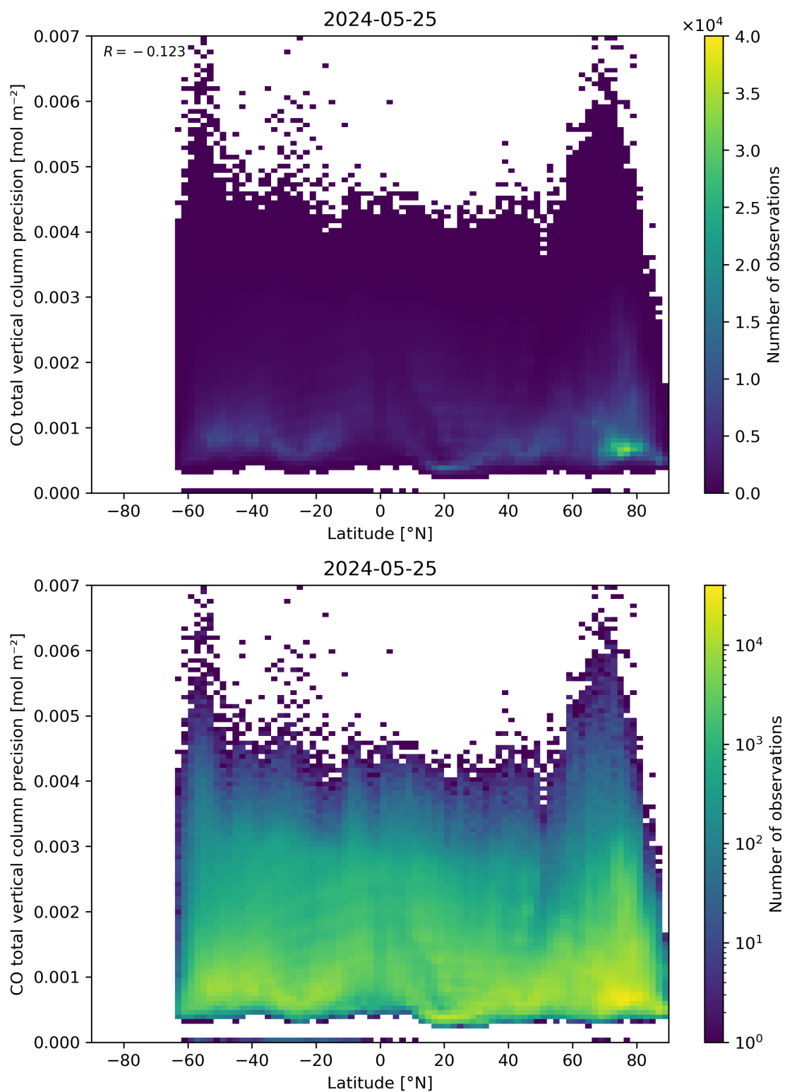
Figure 53: Scatter density plot of “Latitude” against “CO total vertical column precision” for 2024-05-24 to 2024-05-26.
