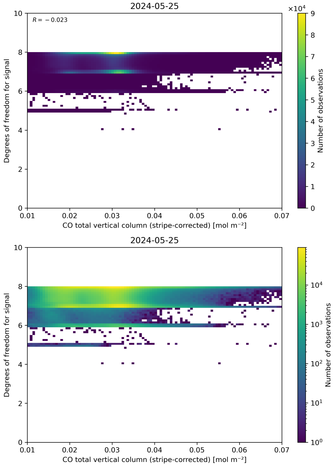
Figure 38: Scatter density plot of “CO total vertical column (stripe-corrected)” against “Degrees of freedom for signal” for 2024-05-24 to 2024-05-26.
