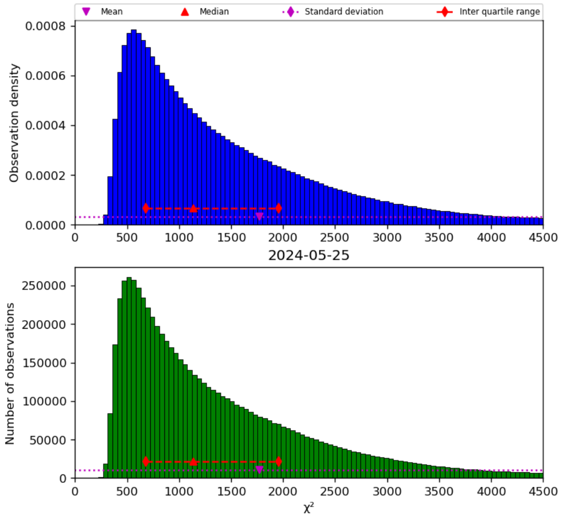
Figure 22: Histogram of “ \chi^2 ” for 2024-05-24 to 2024-05-26
