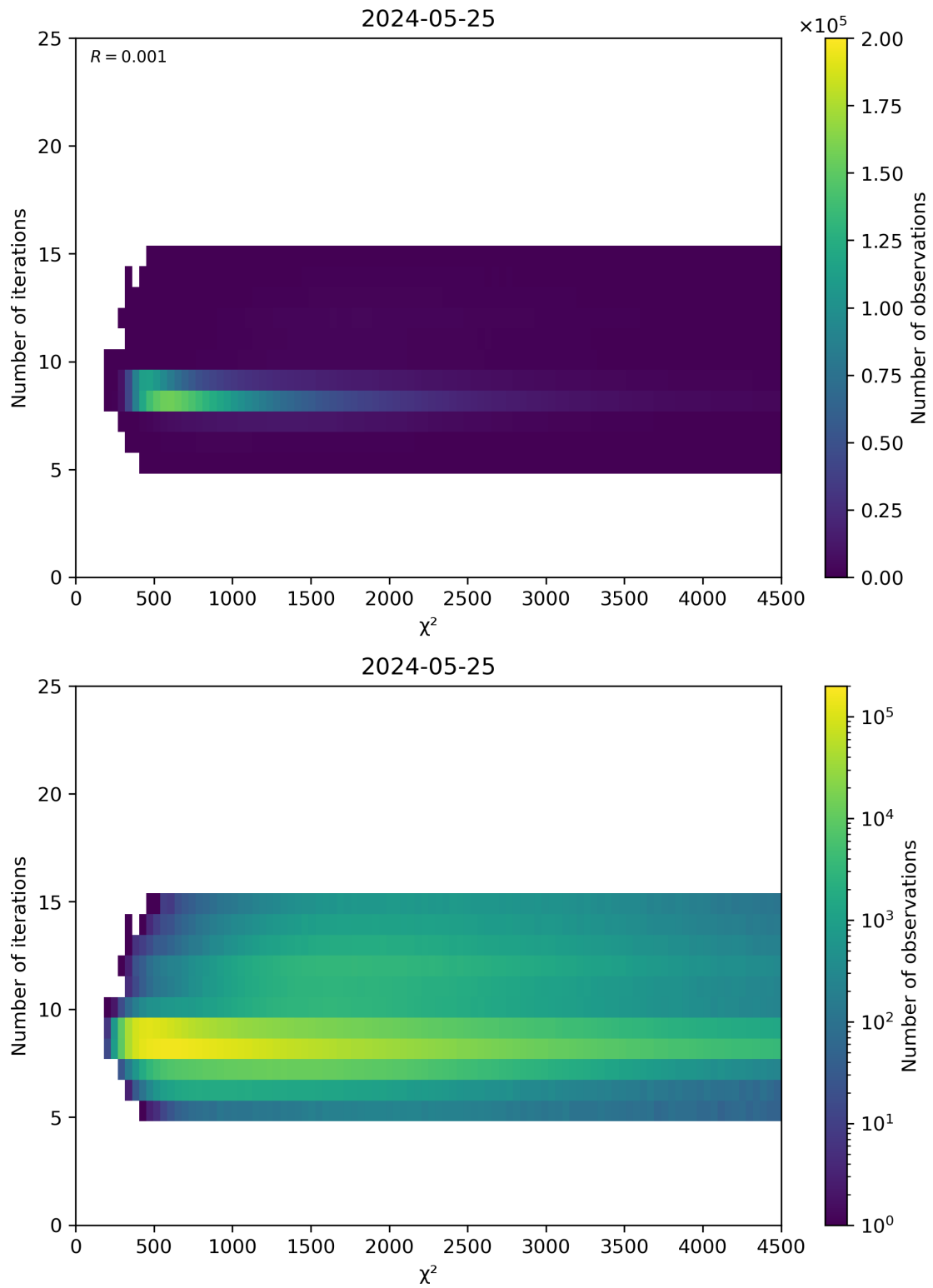
Figure 49: Scatter density plot of “ \chi^2 ” against “Number of iterations” for 2024-05-24 to 2024-05-26.
