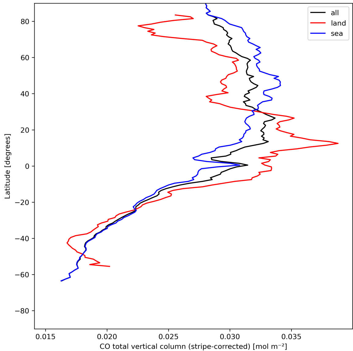
Figure 11: Zonal average of “CO total vertical column (stripe-corrected)” for 2024-05-24 to 2024-05-26.
