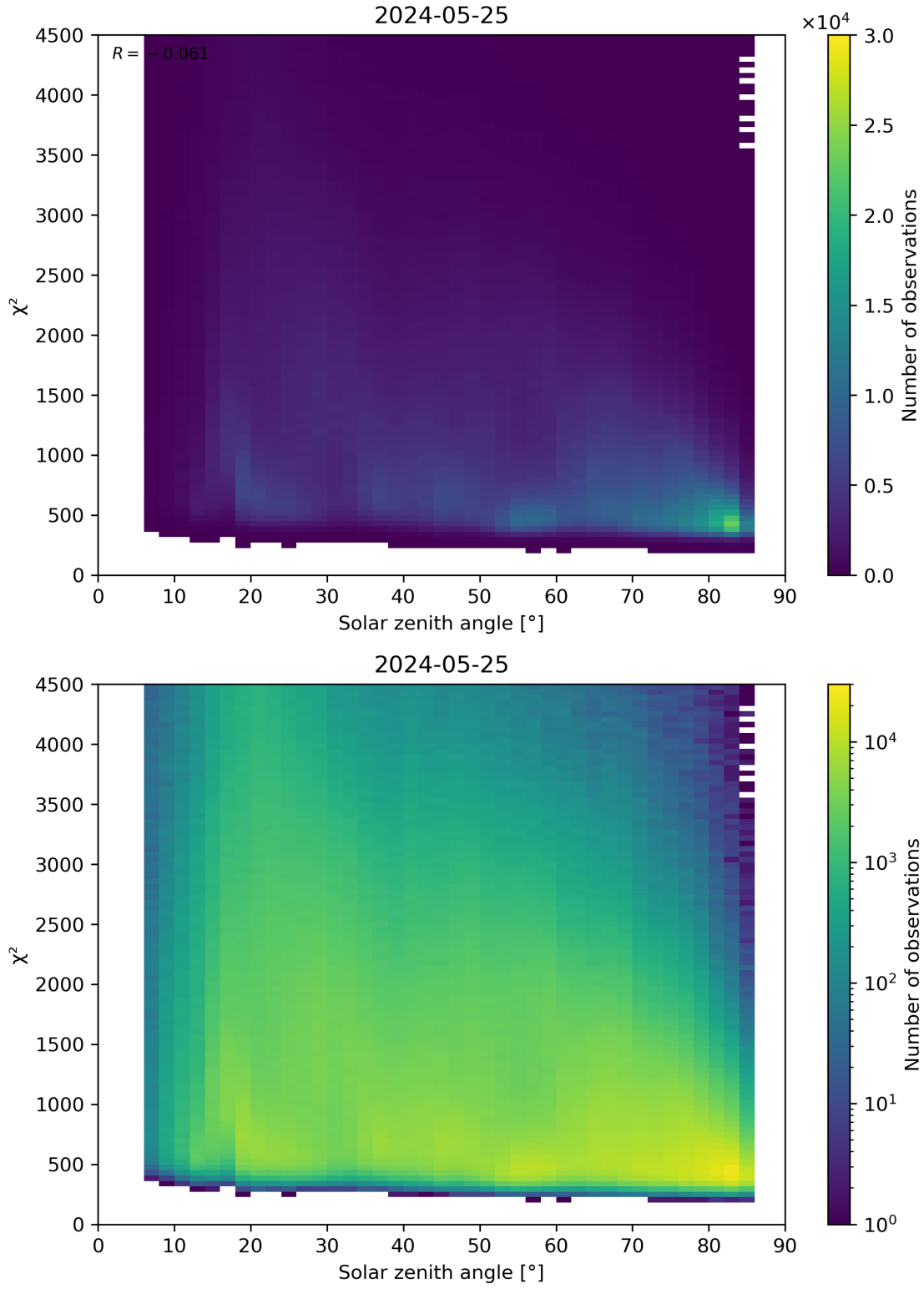
Figure 64: Scatter density plot of “Solar zenith angle” against “ \chi^2 ” for 2024-05-24 to 2024-05-26.
