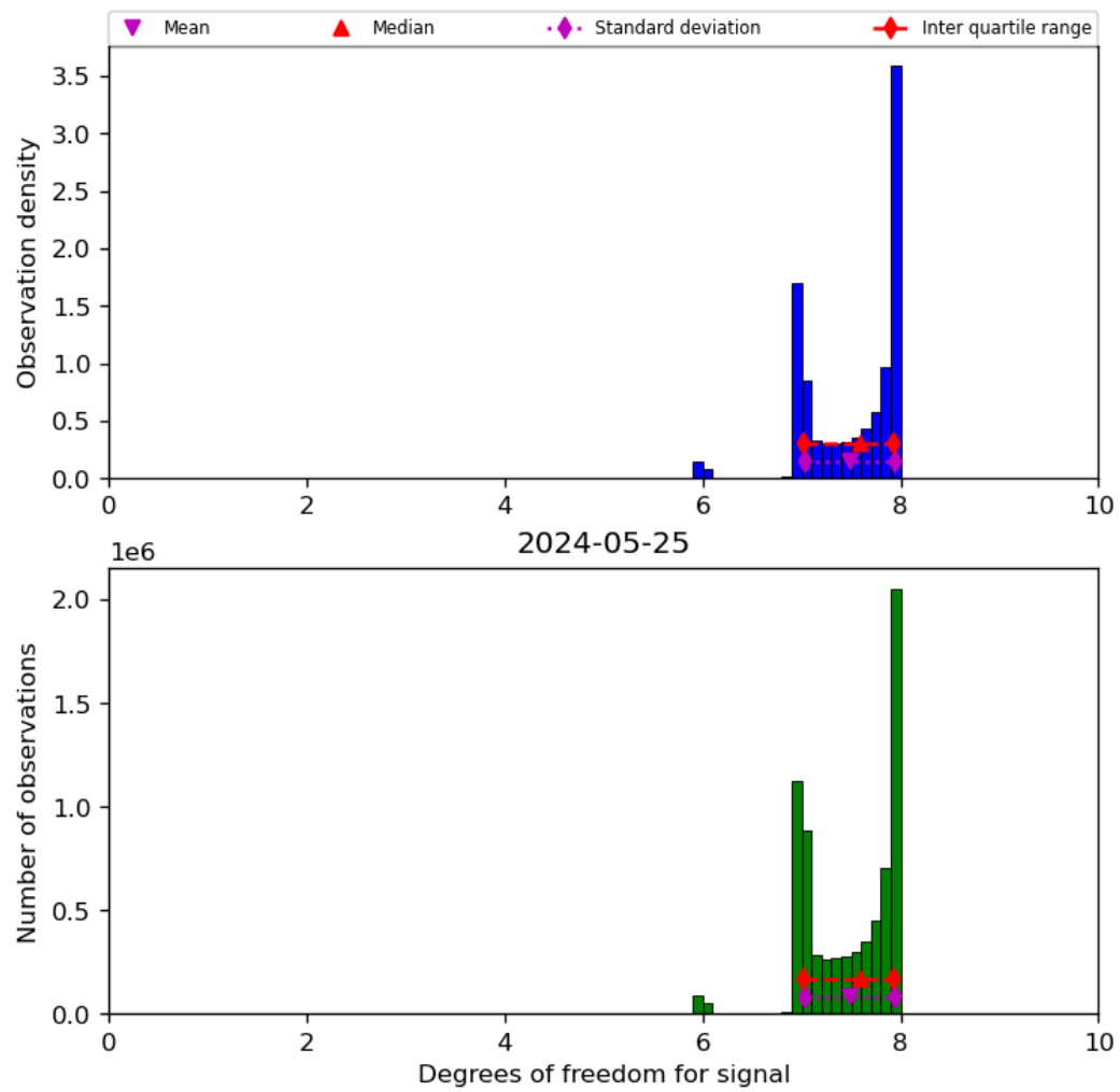
Figure 23: Histogram of “Degrees of freedom for signal” for 2024-05-24 to 2024-05-26
