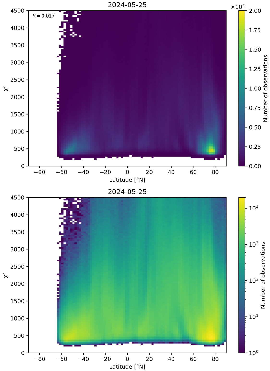
Figure 54: Scatter density plot of “Latitude” against “ \chi^2 ” for 2024-05-24 to 2024-05-26.
