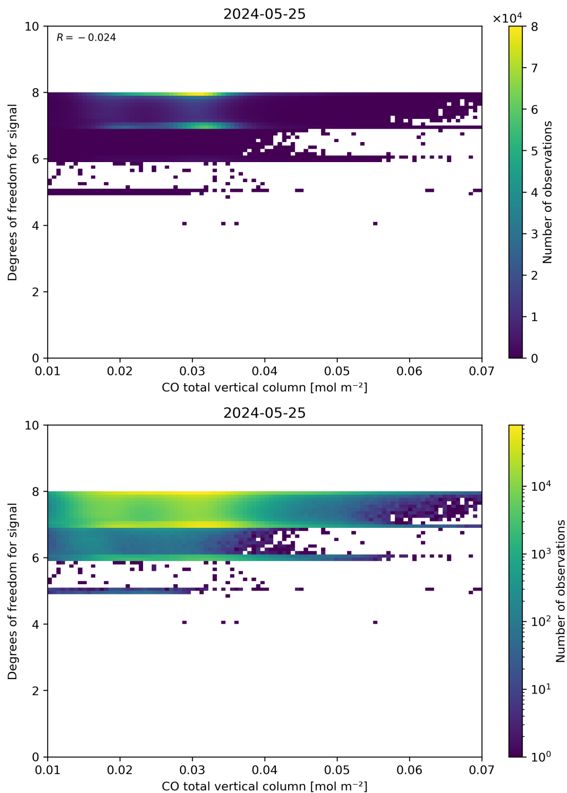
Figure 41: Scatter density plot of “CO total vertical column” against “Degrees of freedom for signal” for 2024-05-24 to 2024-05-26.
