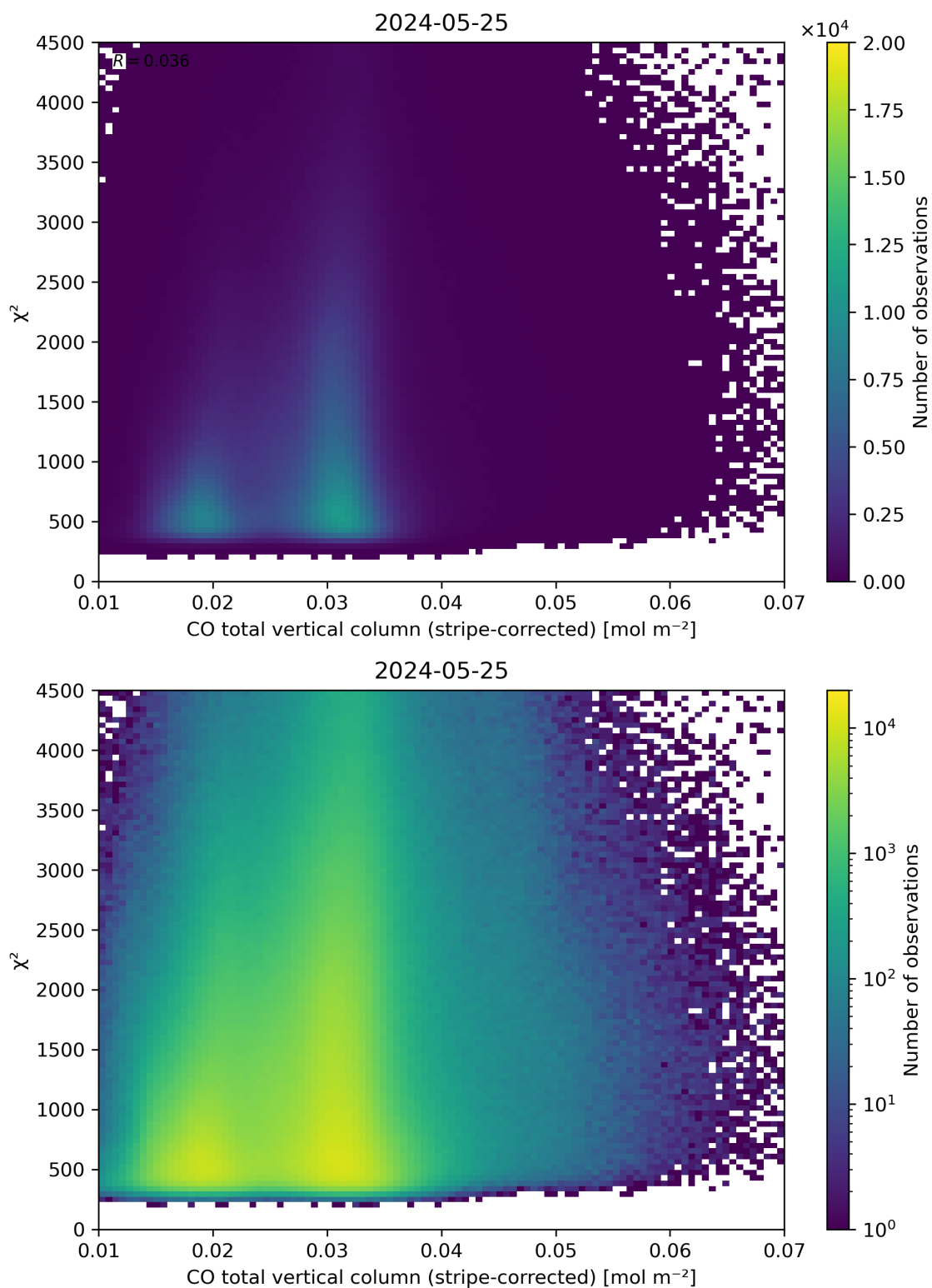
Figure 37: Scatter density plot of “CO total vertical column (stripe-corrected)” against “ \chi^2 ” for 2024-05-24 to 2024-05-26.
