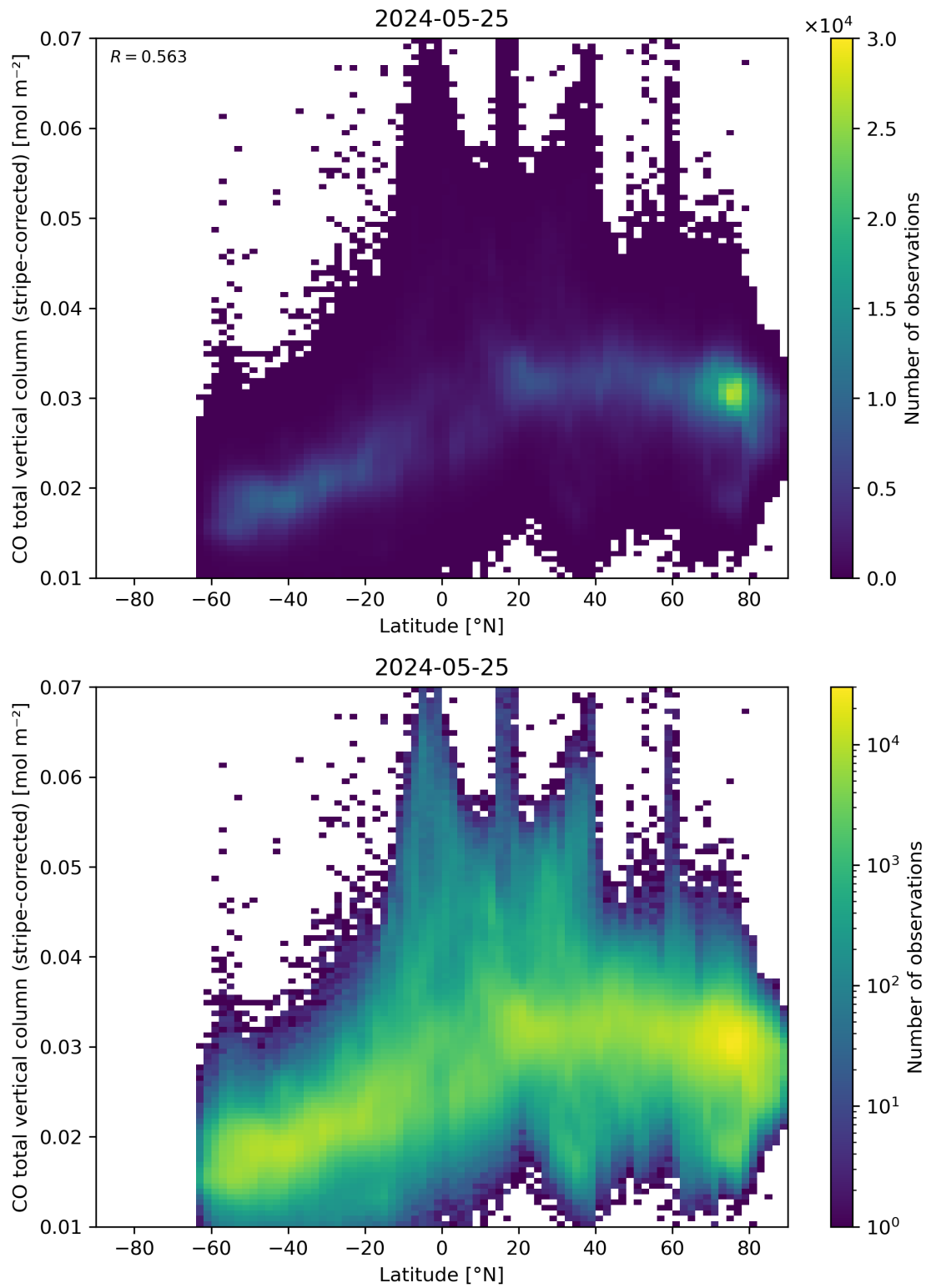
Figure 52: Scatter density plot of “Latitude” against “CO total vertical column (stripe-corrected)” for 2024-05-24 to 2024-05-26.
