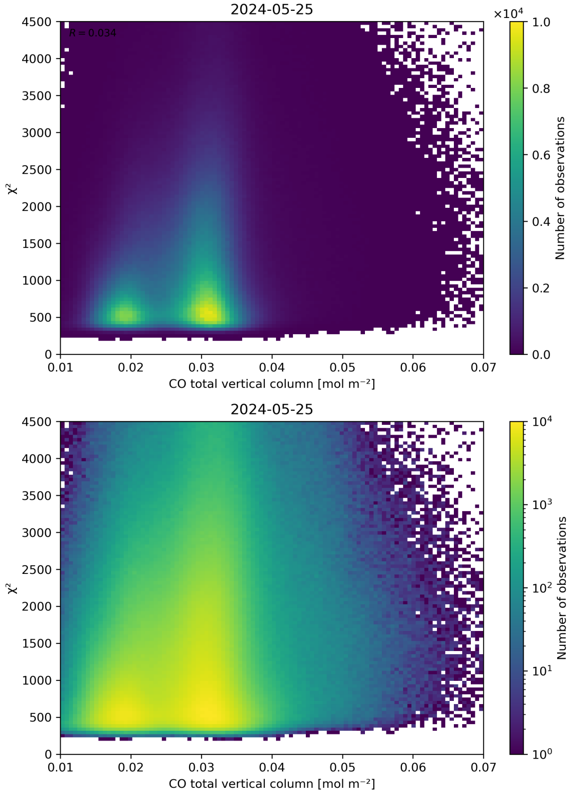
Figure 35: Scatter density plot of “CO total vertical column” against “ \chi^2 ” for 2024-05-24 to 2024-05-26.
