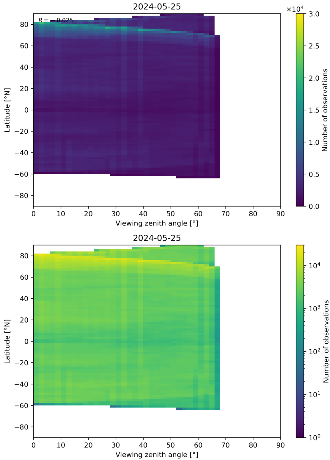
Figure 74: Scatter density plot of “Viewing zenith angle” against “Latitude” for 2024-05-24 to 2024-05-26.
