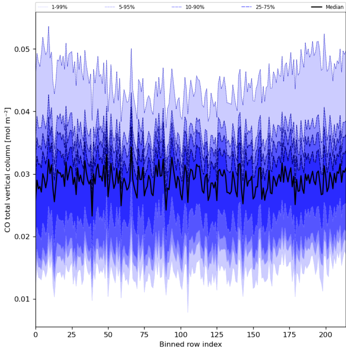
Figure 26: Along track statistics of “CO total vertical column” for 2024-05-24 to 2024-05-26
