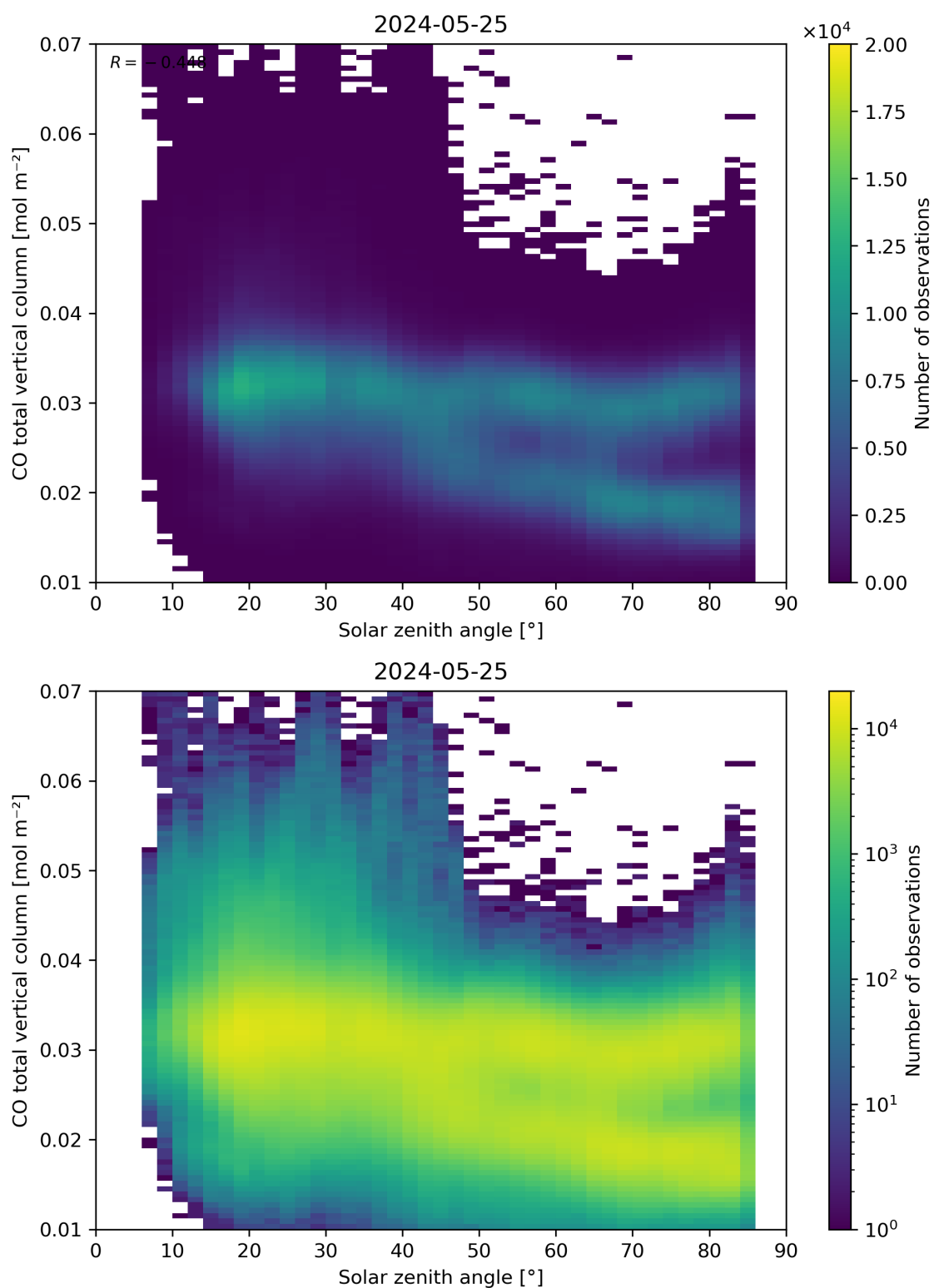
Figure 61: Scatter density plot of “Solar zenith angle” against “CO total vertical column” for 2024-05-24 to 2024-05-26.
