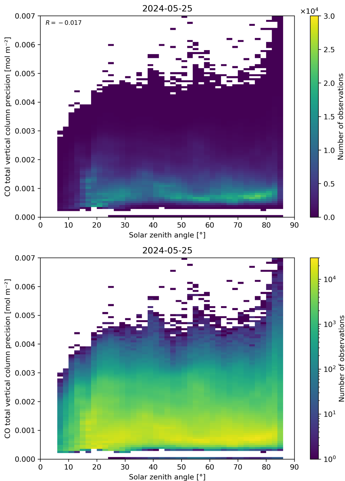
Figure 63: Scatter density plot of “Solar zenith angle” against “CO total vertical column precision” for 2024-05-24 to 2024-05-26.
