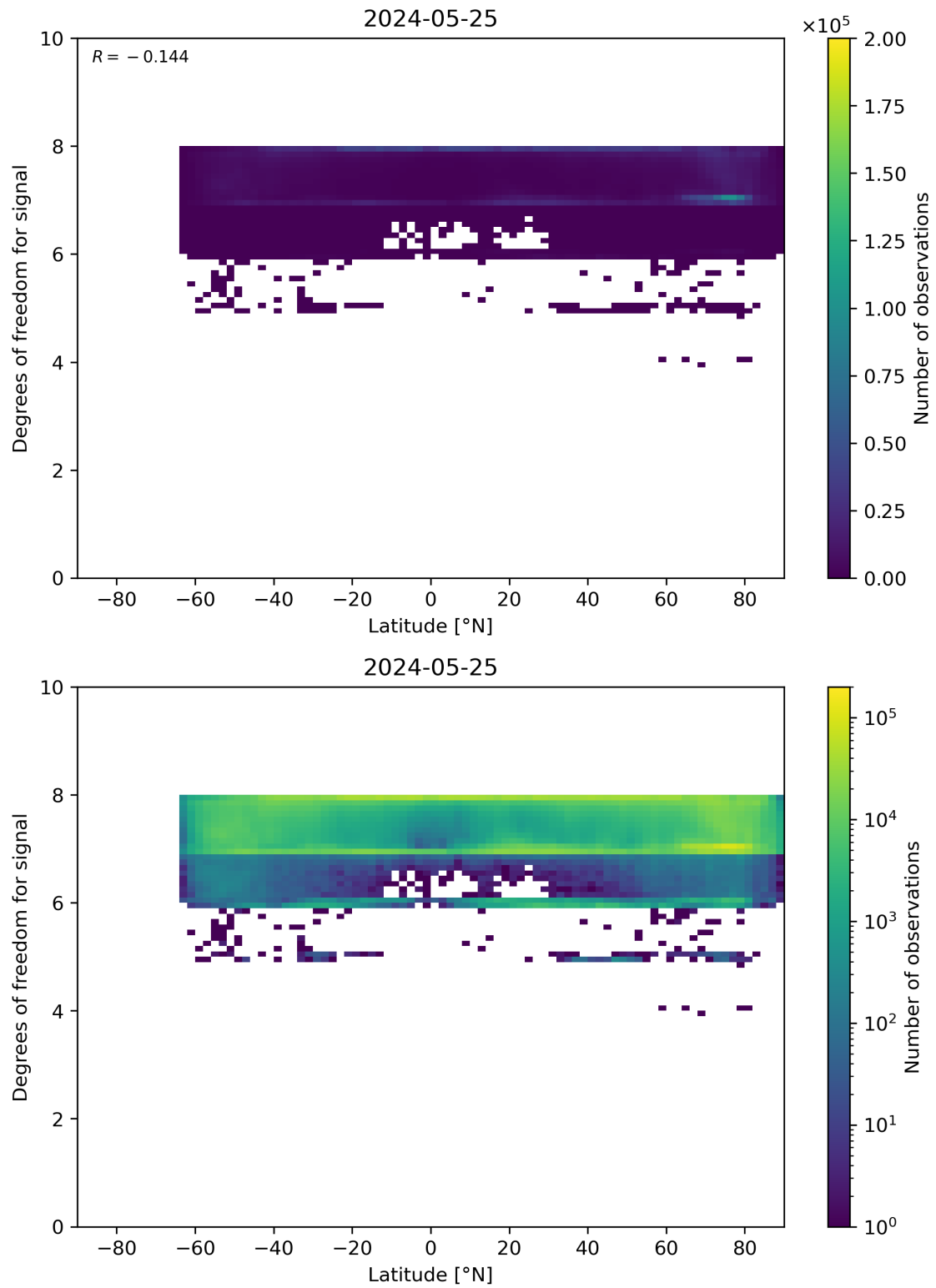
Figure 55: Scatter density plot of “Latitude” against “Degrees of freedom for signal” for 2024-05-24 to 2024-05-26.
