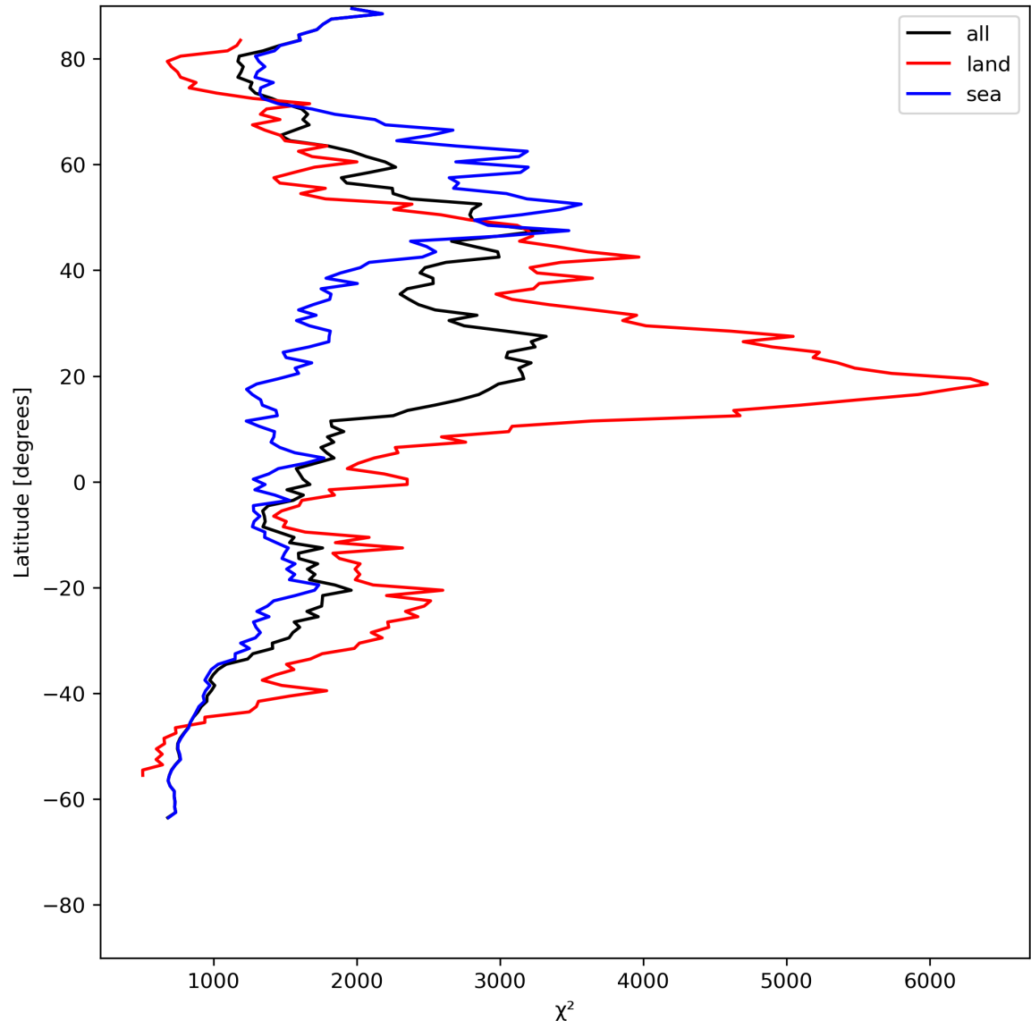
Figure 14: Zonal average of “ \chi^2 ” for 2024-05-24 to 2024-05-26.
