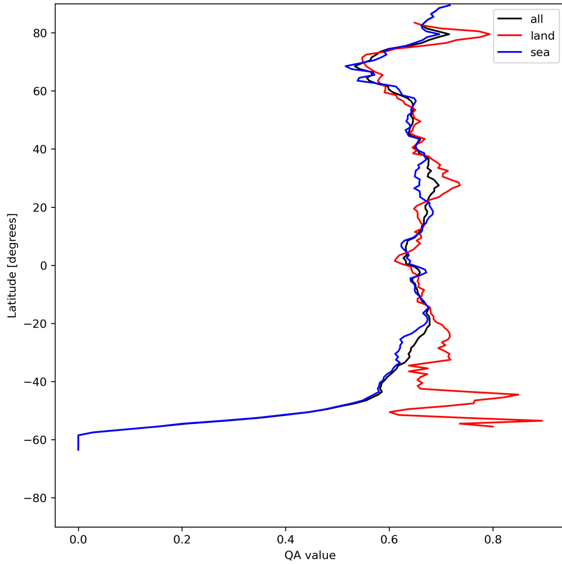
Figure 9: Zonal average of “QA value” for 2024-05-24 to 2024-05-26.
