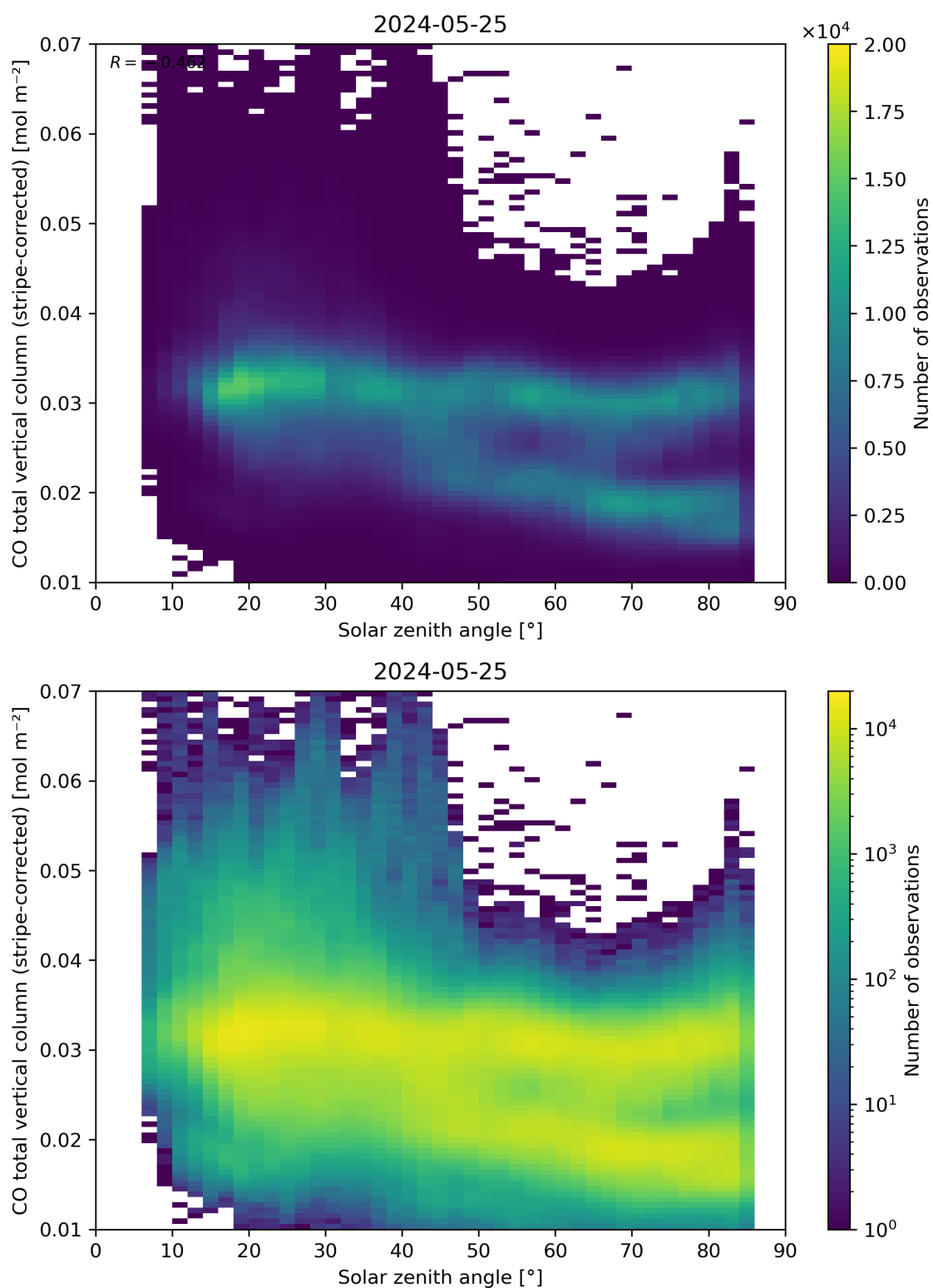
Figure 62: Scatter density plot of “Solar zenith angle” against “CO total vertical column (stripe-corrected)” for 2024-05-24 to 2024-05-26.
