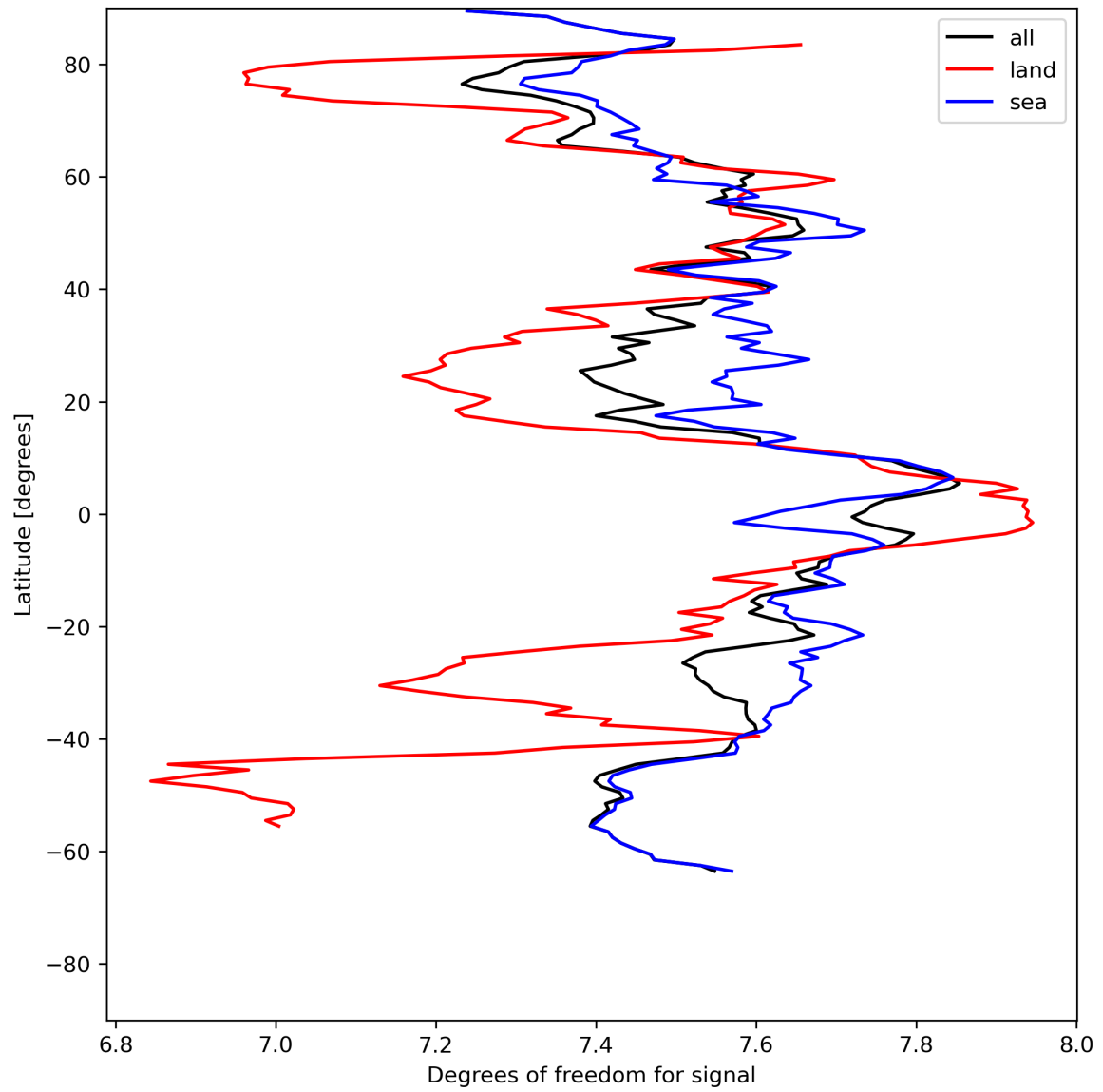
Figure 15: Zonal average of “Degrees of freedom for signal” for 2024-05-24 to 2024-05-26.
