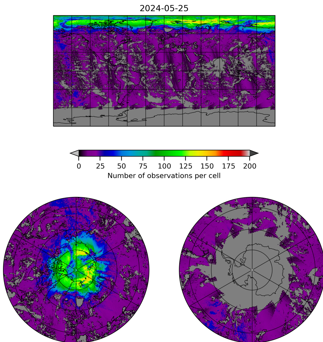
Figure 8: Map of the number of observations for 2024-05-24 to 2024-05-26
