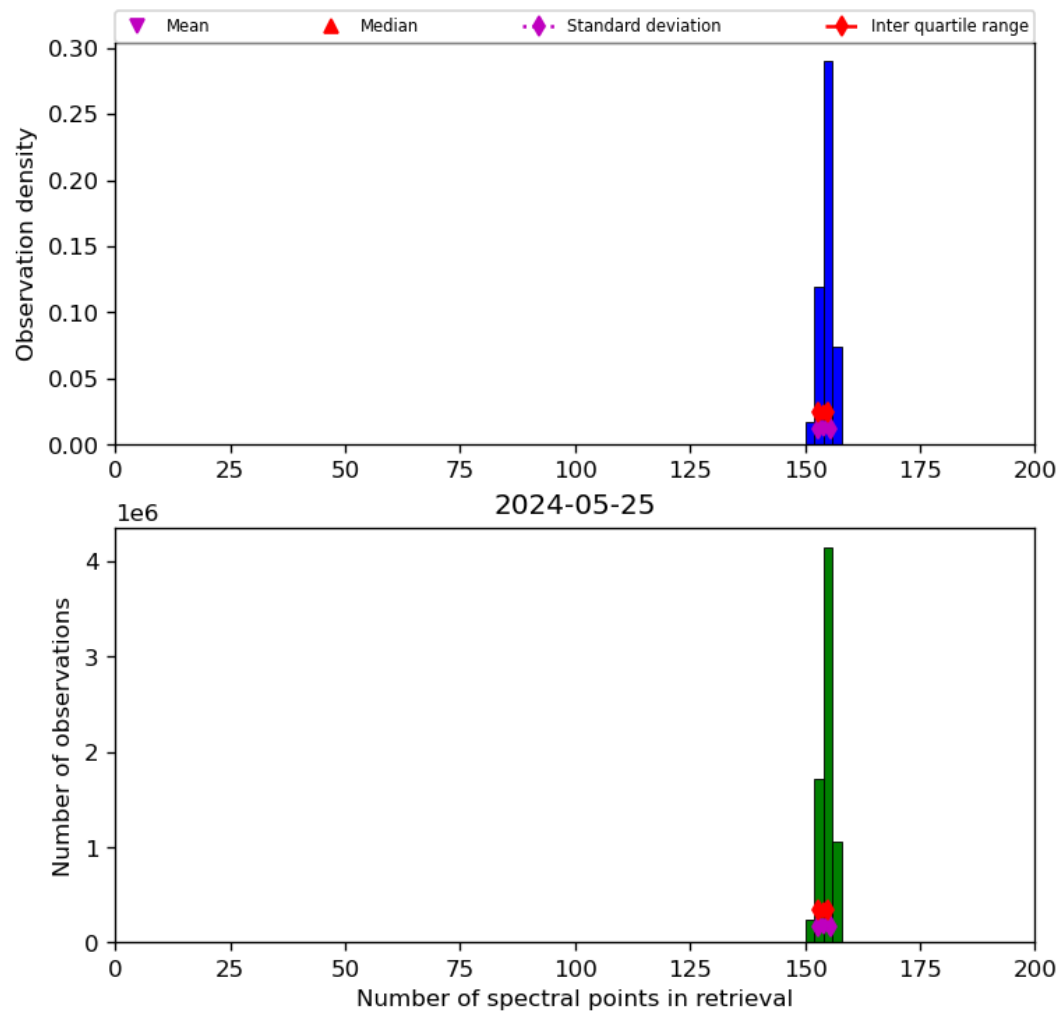
Figure 21: Histogram of “Number of spectral points in retrieval” for 2024-05-24 to 2024-05-26
