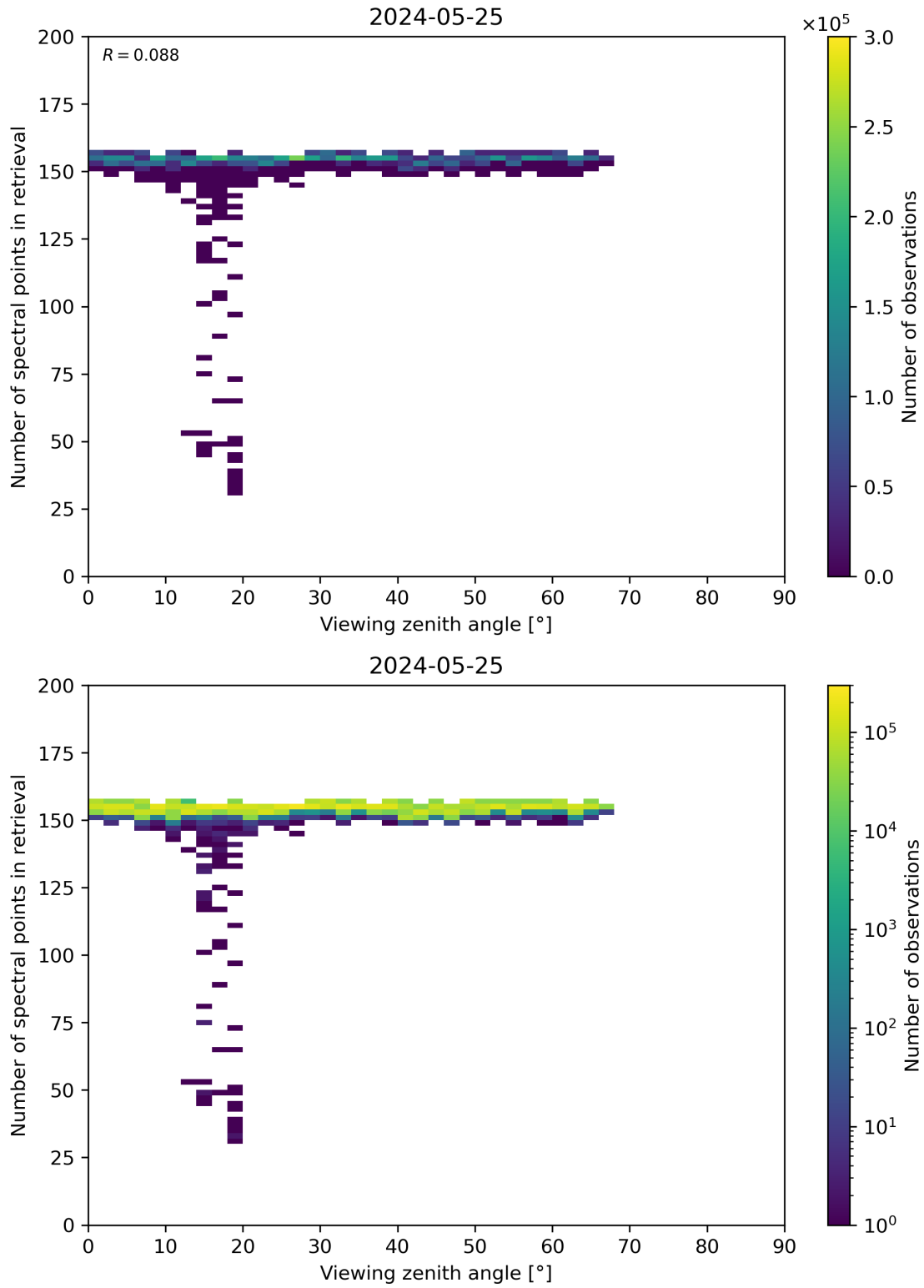
Figure 76: Scatter density plot of “Viewing zenith angle” against “Number of spectral points in retrieval” for 2024-05-24 to 2024-05-26.
