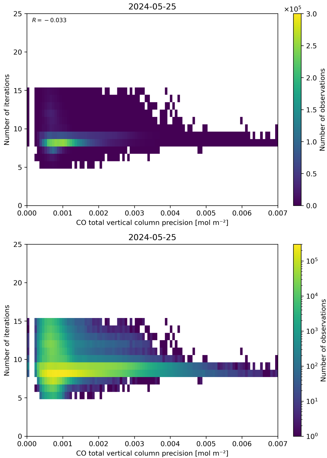
Figure 46: Scatter density plot of “CO total vertical column precision” against “Number of iterations” for 2024-05-24 to 2024-05-26.
