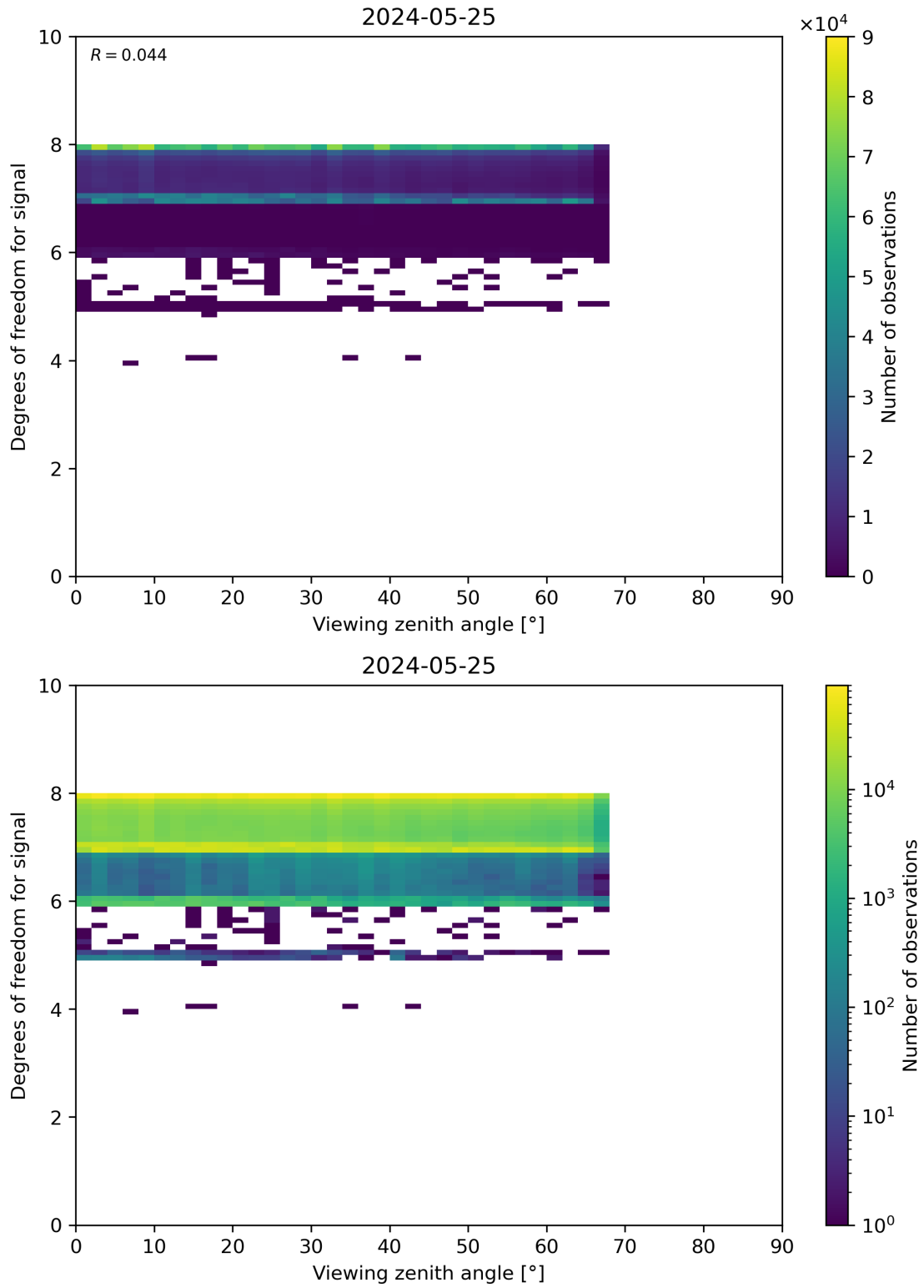
Figure 73: Scatter density plot of “Viewing zenith angle” against “Degrees of freedom for signal” for 2024-05-24 to 2024-05-26.
