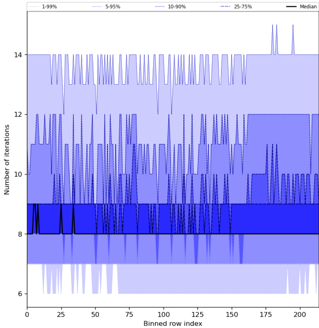
Figure 32: Along track statistics of “Number of iterations” for 2024-05-24 to 2024-05-26
