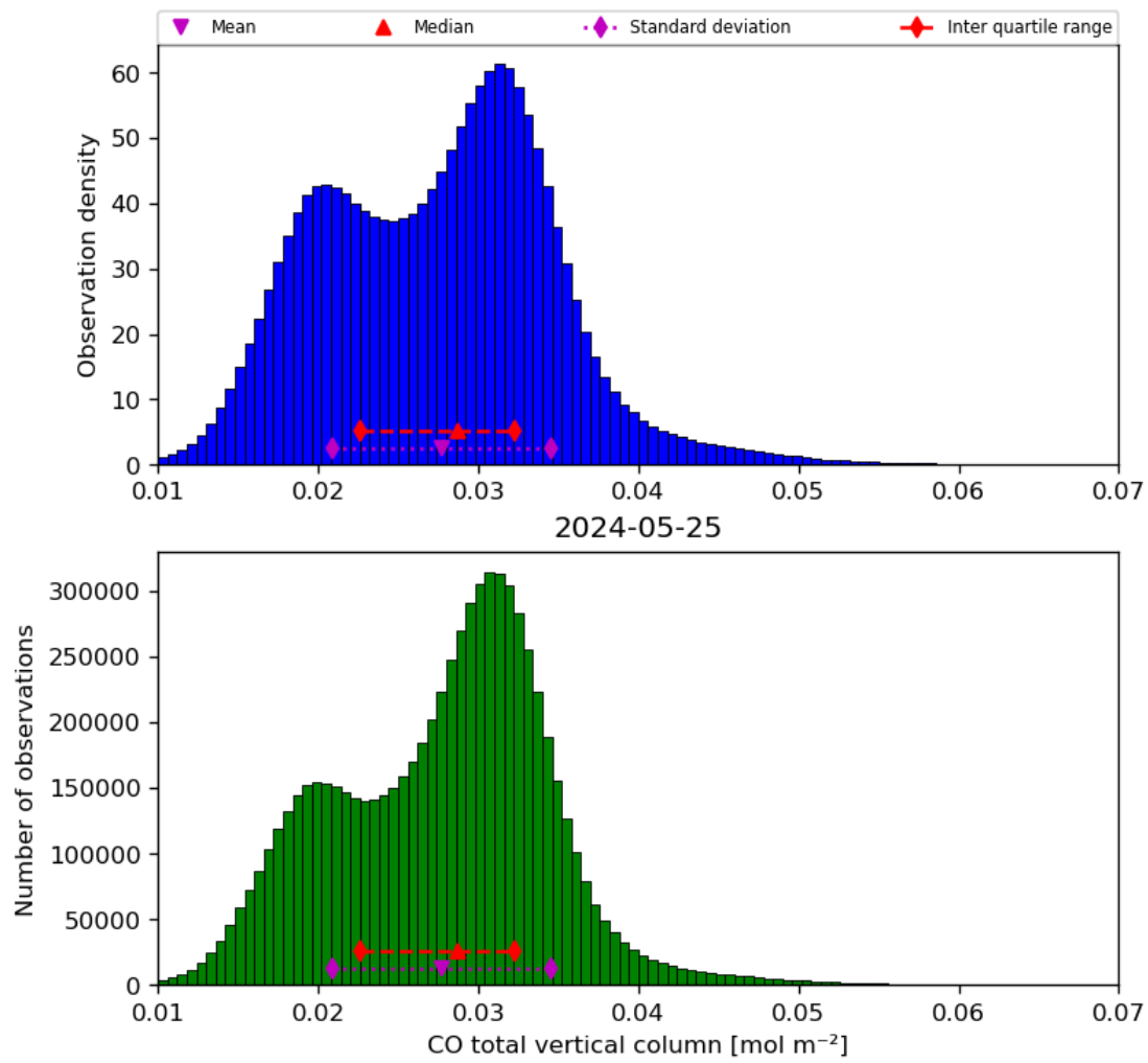
Figure 18: Histogram of “CO total vertical column” for 2024-05-24 to 2024-05-26
