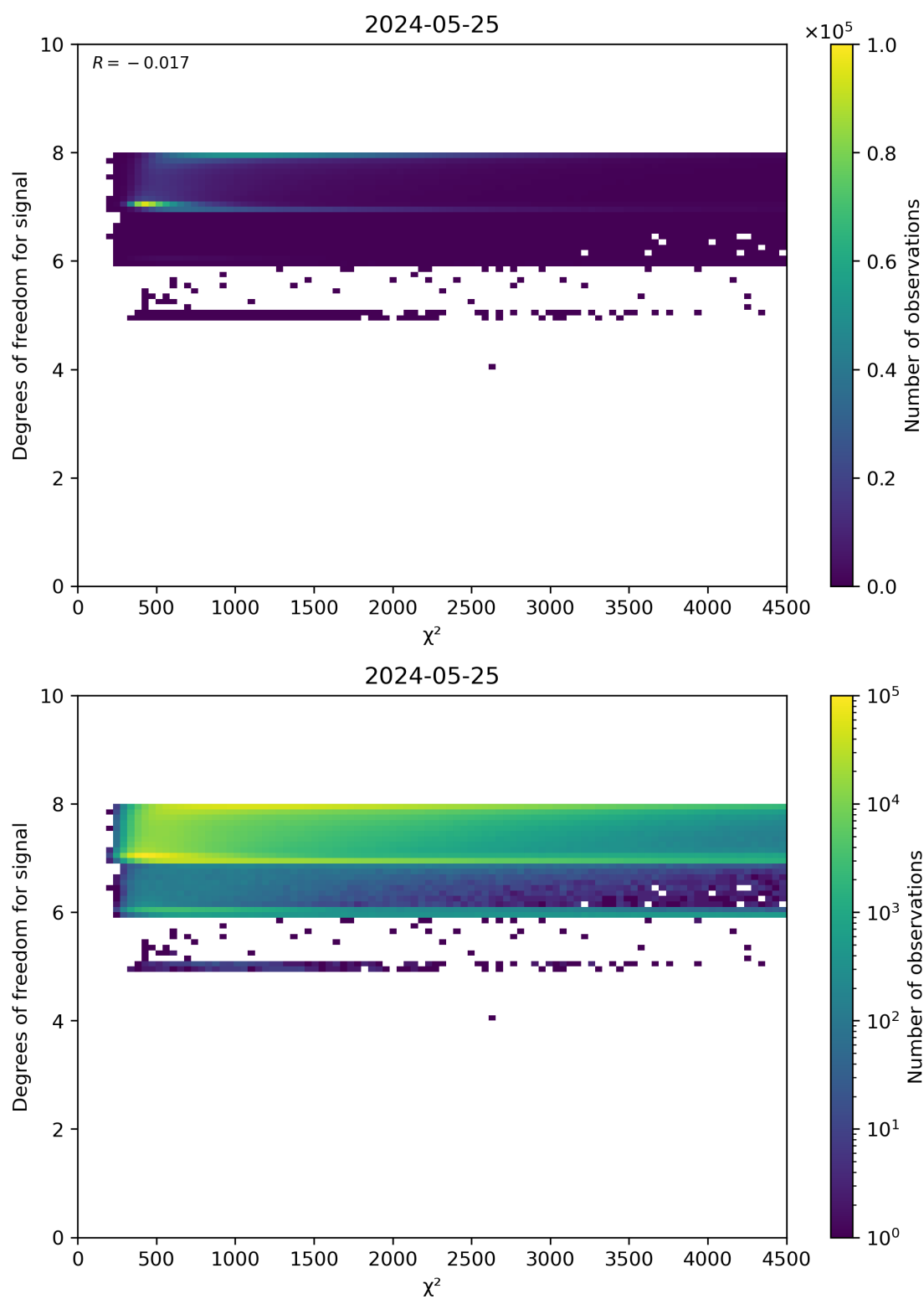
Figure 48: Scatter density plot of “ \chi^2 ” against “Degrees of freedom for signal” for 2024-05-24 to 2024-05-26.
