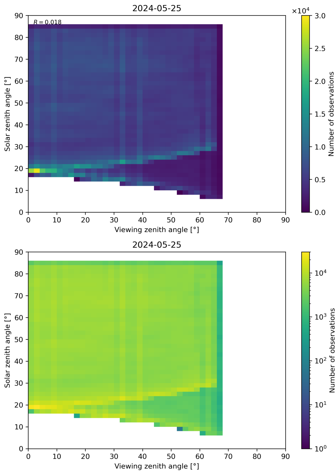
Figure 77: Scatter density plot of “Viewing zenith angle” against “Solar zenith angle” for 2024-05-24 to 2024-05-26.
