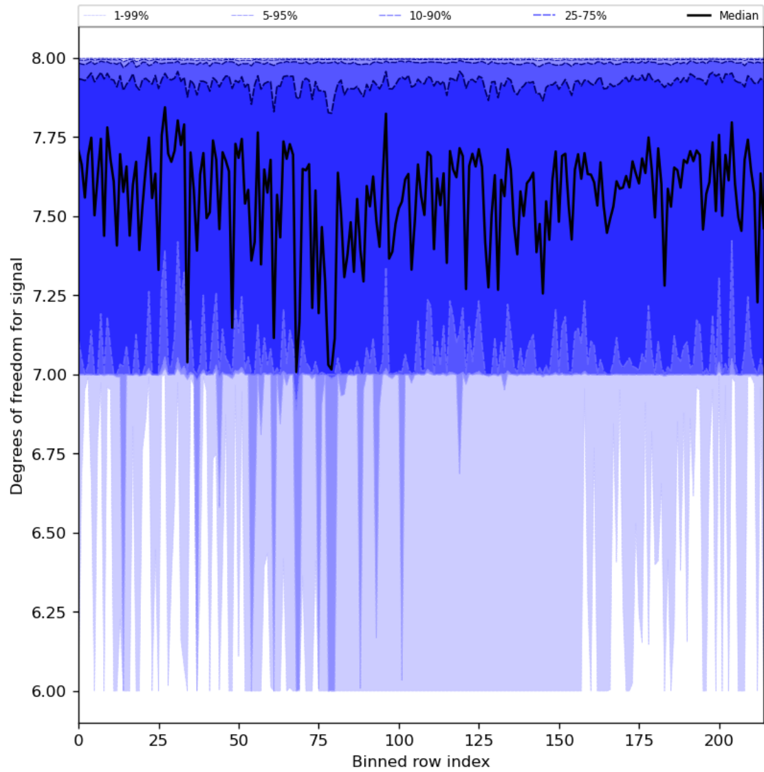
Figure 31: Along track statistics of “Degrees of freedom for signal” for 2024-05-24 to 2024-05-26
