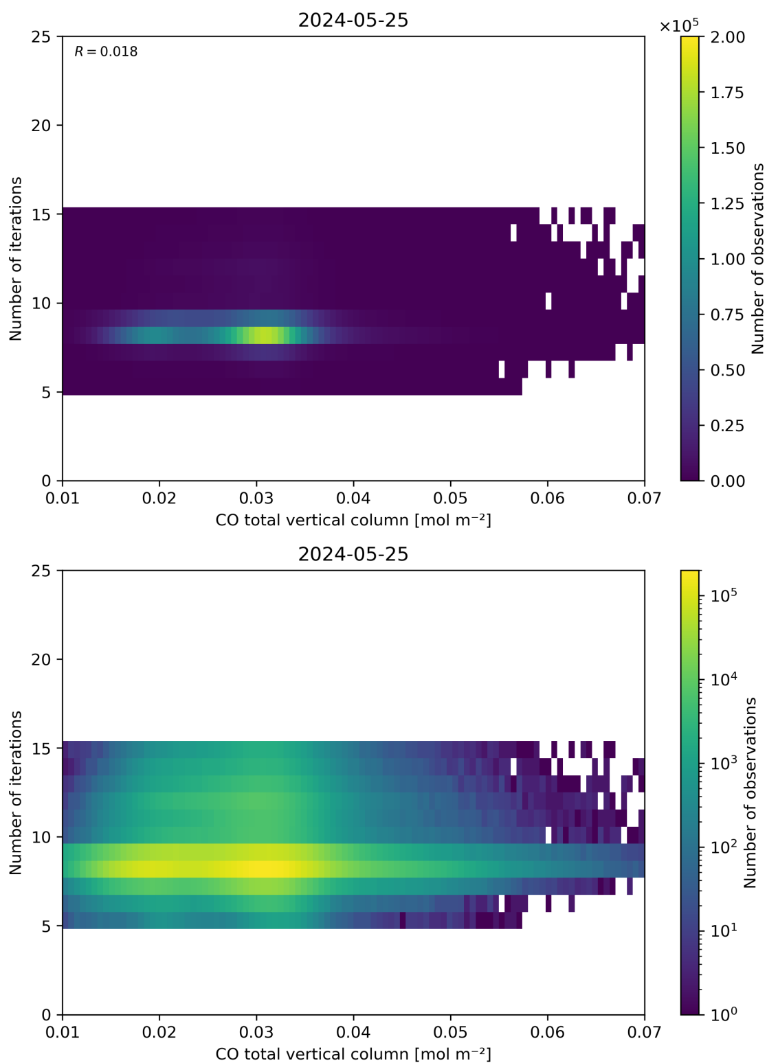
Figure 42: Scatter density plot of “CO total vertical column” against “Number of iterations” for 2024-05-24 to 2024-05-26.
