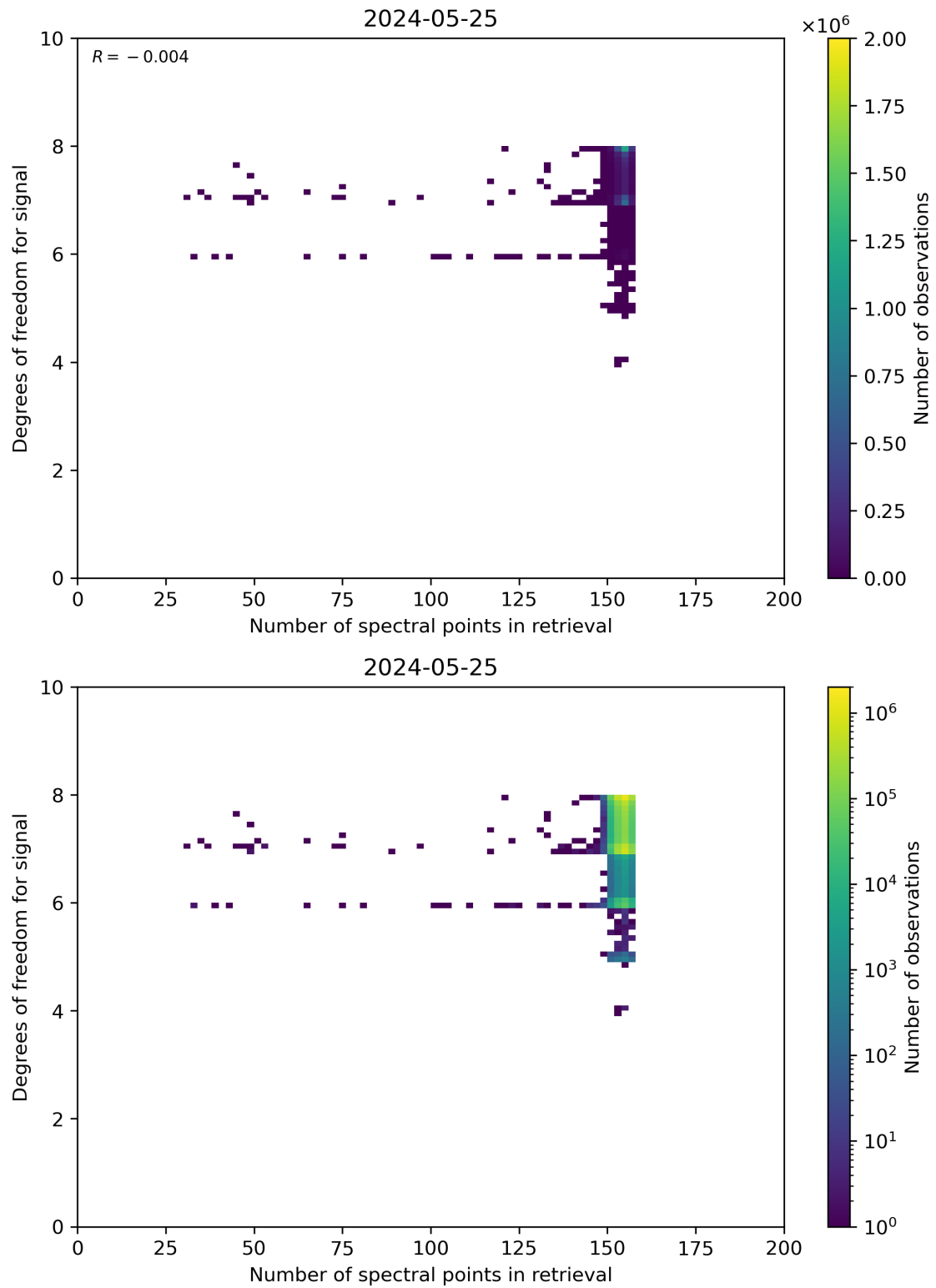
Figure 59: Scatter density plot of “Number of spectral points in retrieval” against “Degrees of freedom for signal” for 2024-05-24 to 2024-05-26.
