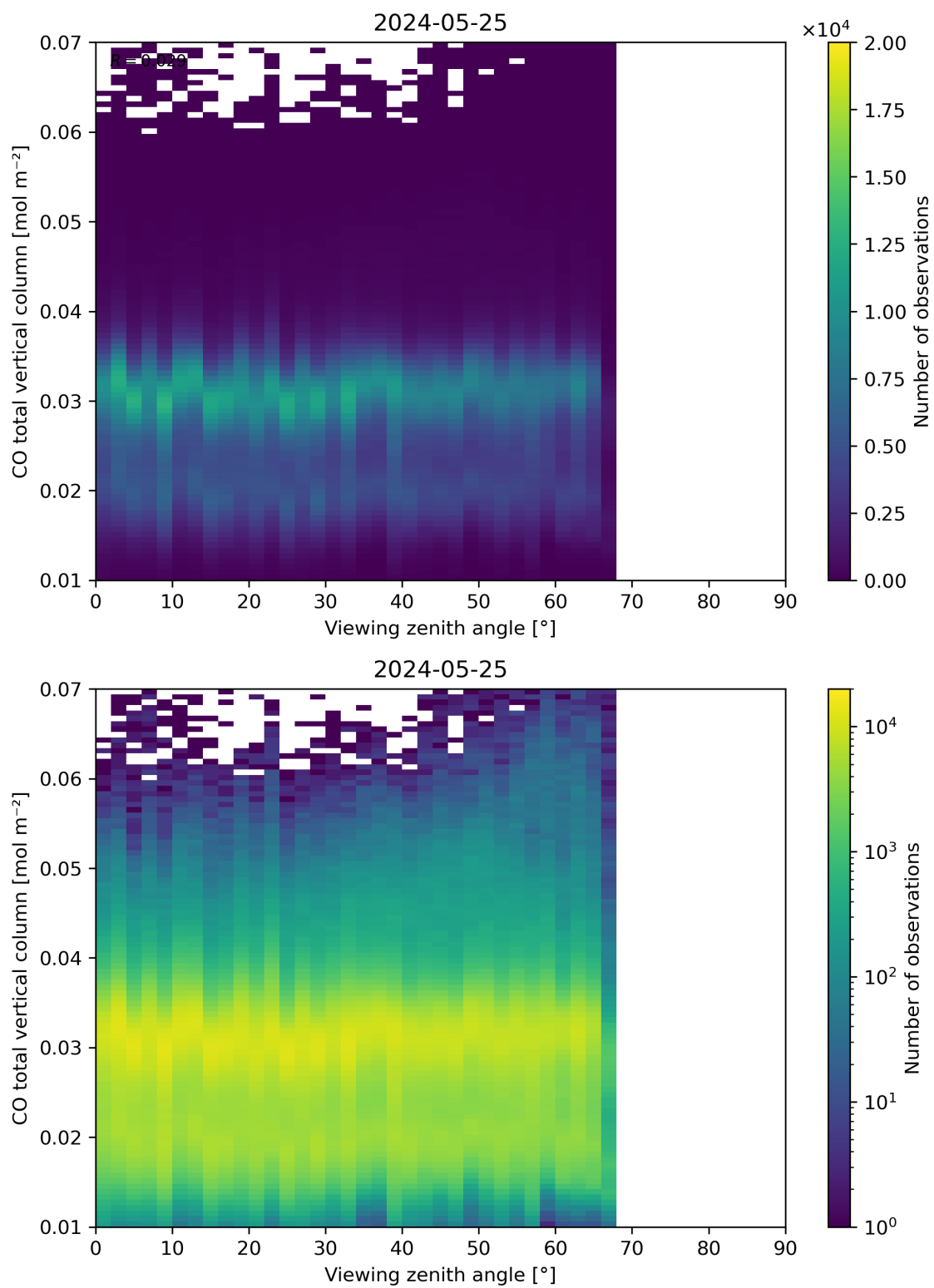
Figure 69: Scatter density plot of “Viewing zenith angle” against “CO total vertical column” for 2024-05-24 to 2024-05-26.
