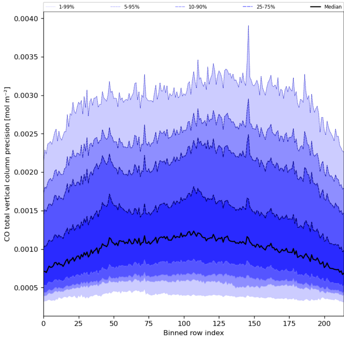
Figure 28: Along track statistics of “CO total vertical column precision” for 2024-05-24 to 2024-05-26
