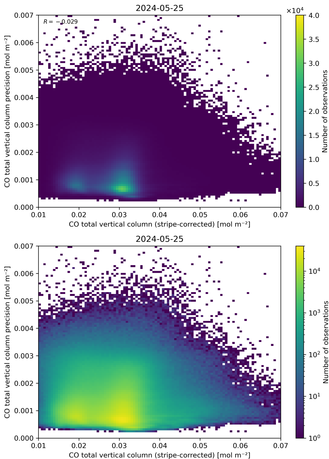
Figure 36: Scatter density plot of “CO total vertical column (stripe-corrected)” against “CO total vertical column precision” for 2024-05-24 to 2024-05-26.
