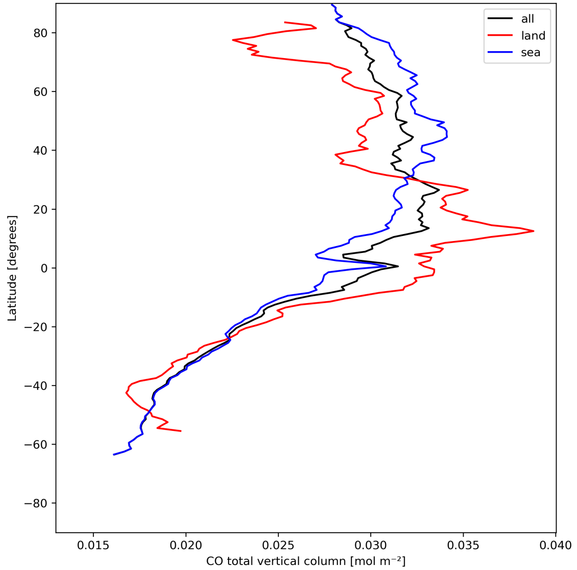
Figure 10: Zonal average of “CO total vertical column” for 2024-05-24 to 2024-05-26.
