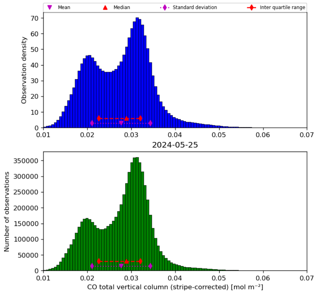
Figure 19: Histogram of “CO total vertical column (stripe-corrected)” for 2024-05-24 to 2024-05-26
