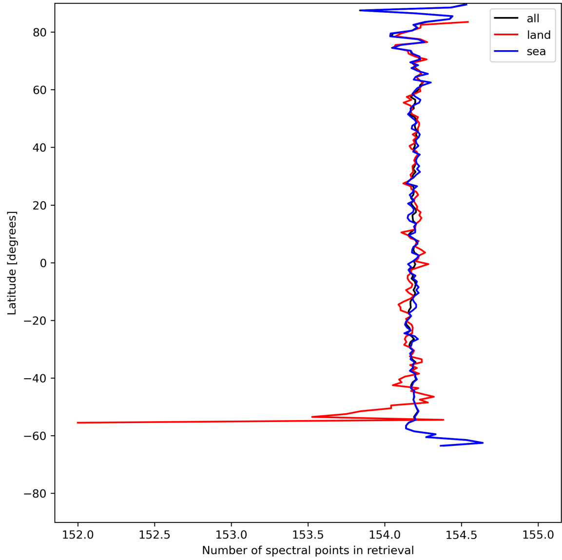
Figure 13: Zonal average of “Number of spectral points in retrieval” for 2024-05-24 to 2024-05-26.
