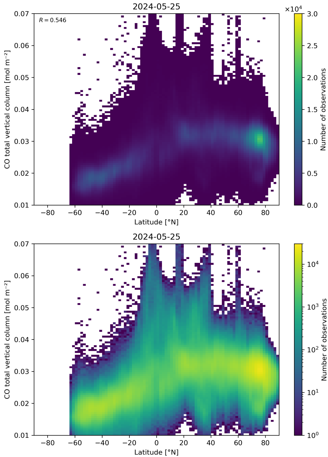
Figure 51: Scatter density plot of “Latitude” against “CO total vertical column” for 2024-05-24 to 2024-05-26.
