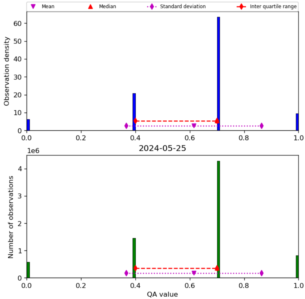
Figure 17: Histogram of “QA value” for 2024-05-24 to 2024-05-26
