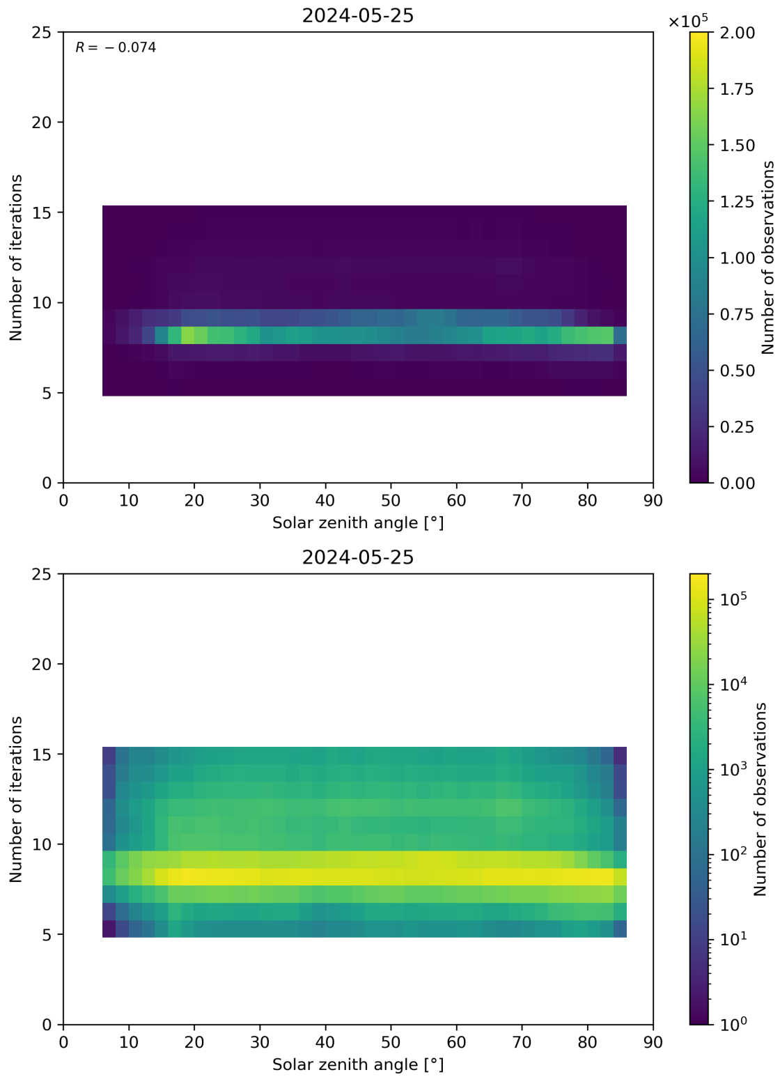
Figure 67: Scatter density plot of “Solar zenith angle” against “Number of iterations” for 2024-05-24 to 2024-05-26.
