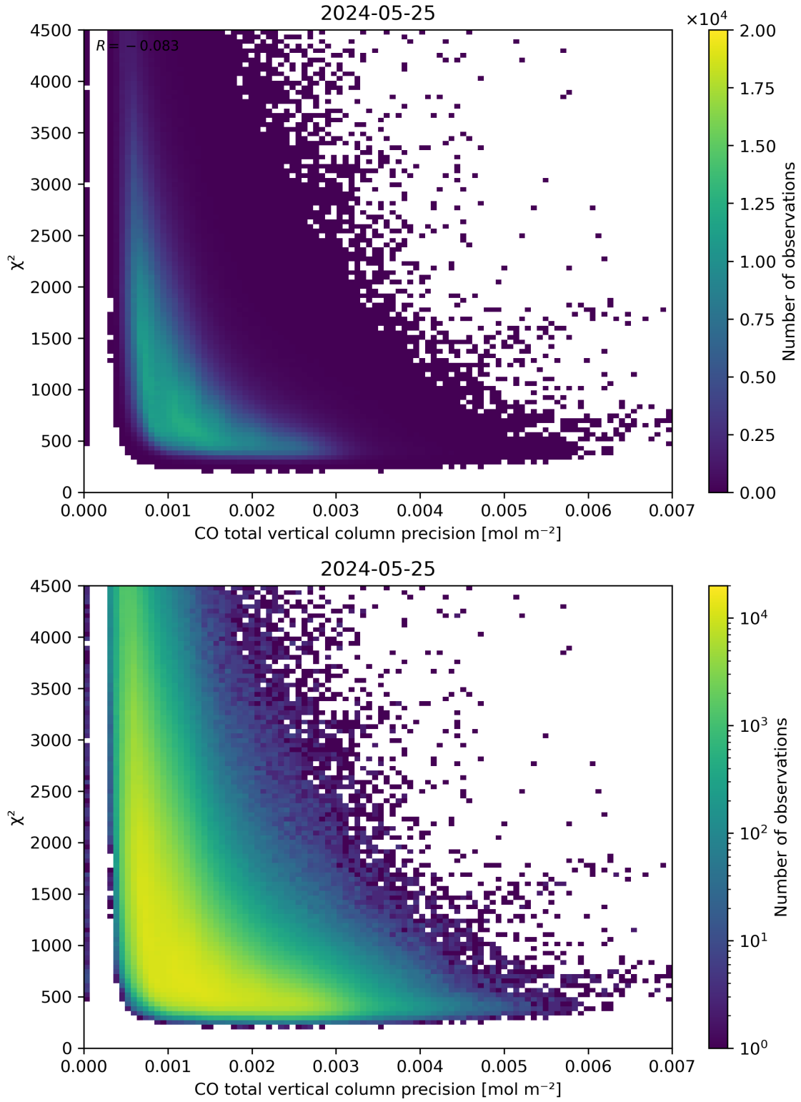
Figure 44: Scatter density plot of “CO total vertical column precision” against “ \chi^2 ” for 2024-05-24 to 2024-05-26.
