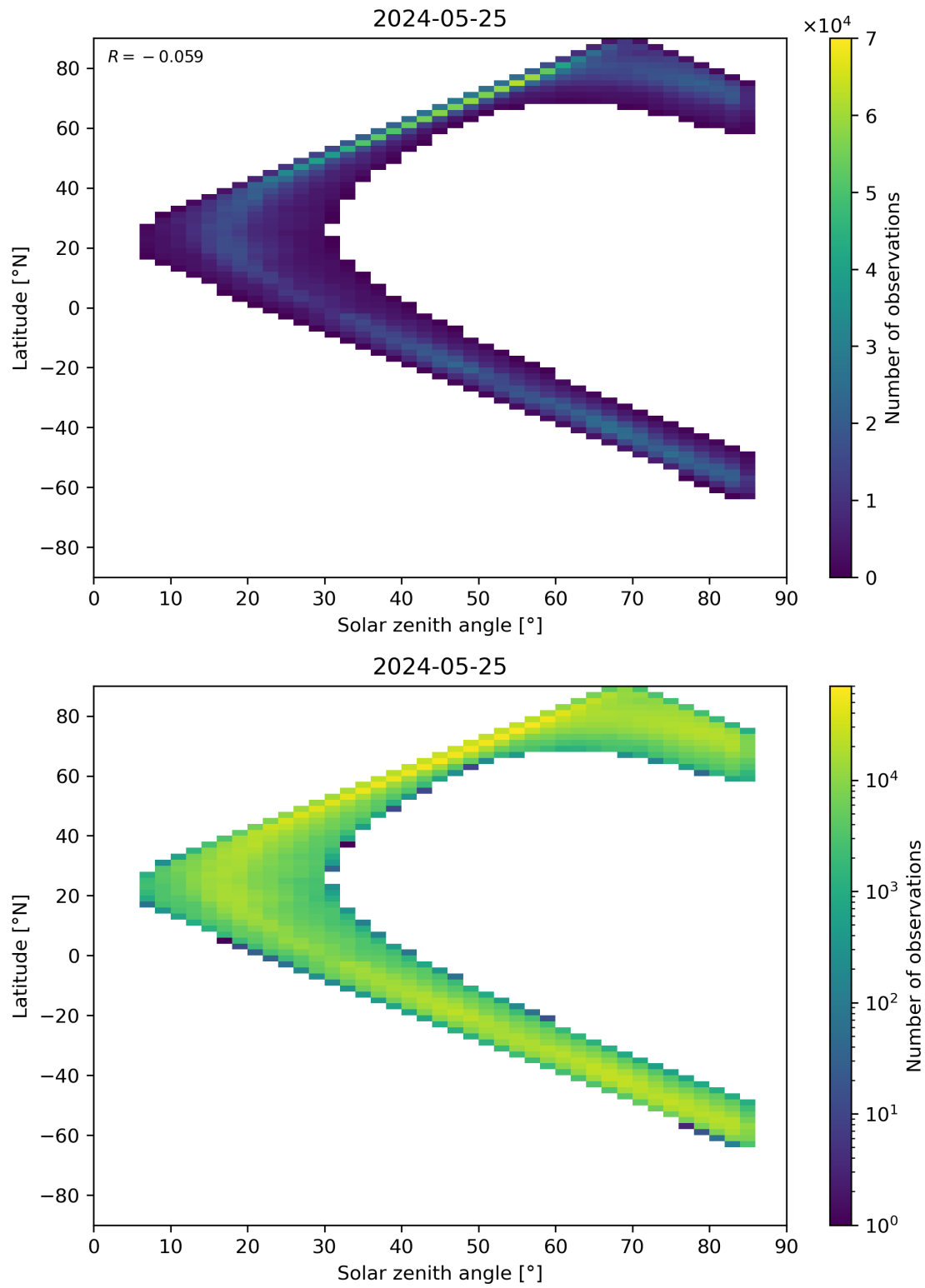
Figure 66: Scatter density plot of “Solar zenith angle” against “Latitude” for 2024-05-24 to 2024-05-26.
