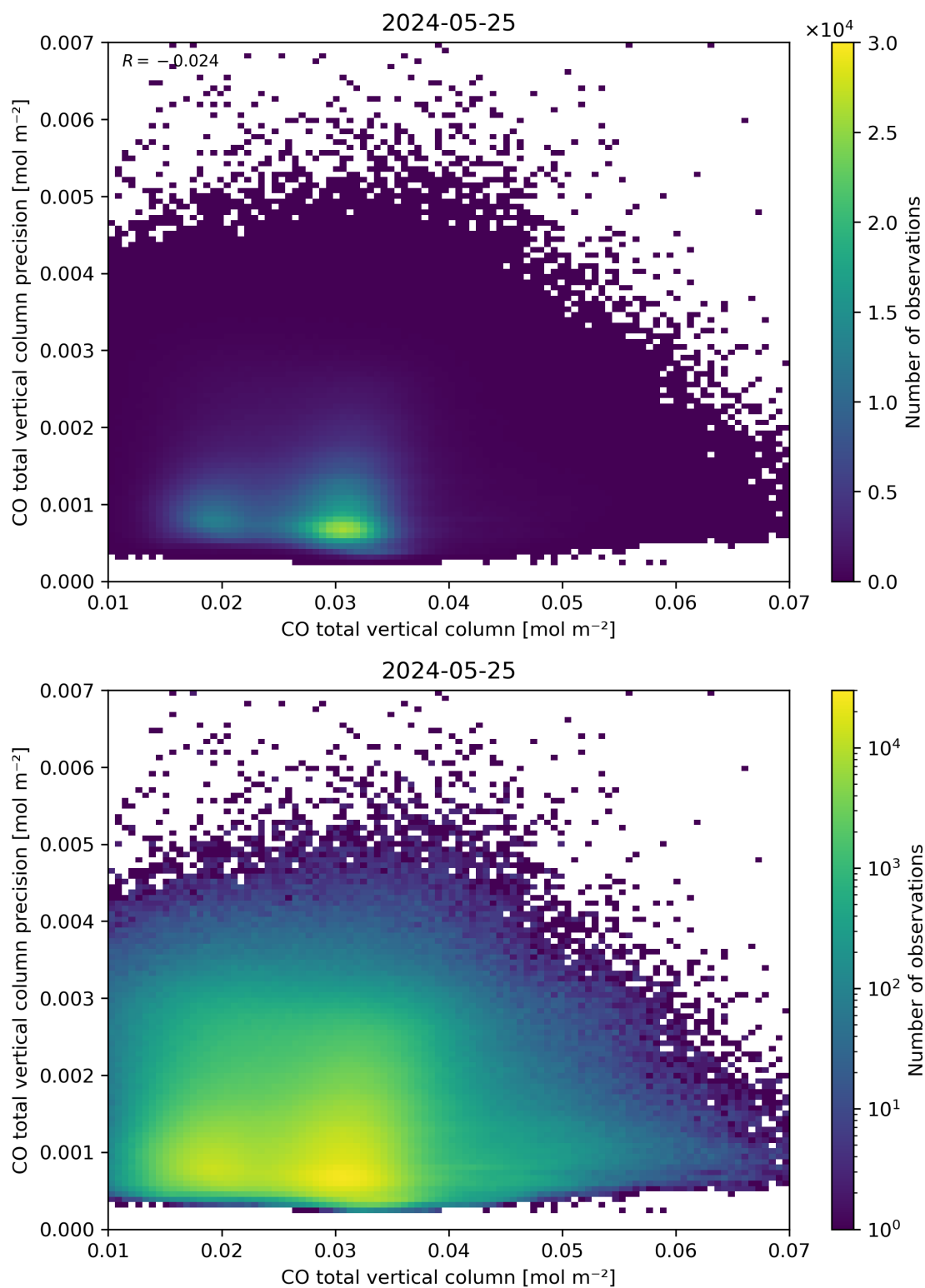
Figure 34: Scatter density plot of “CO total vertical column” against “CO total vertical column precision” for 2024-05-24 to 2024-05-26.
