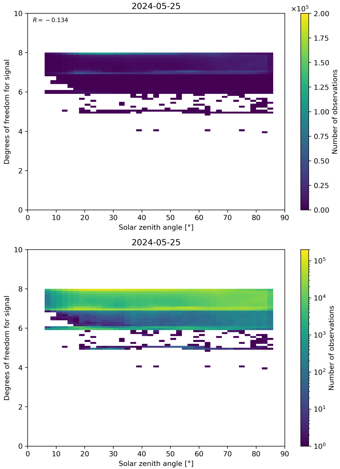
Figure 65: Scatter density plot of “Solar zenith angle” against “Degrees of freedom for signal” for 2024-05-24 to 2024-05-26.
