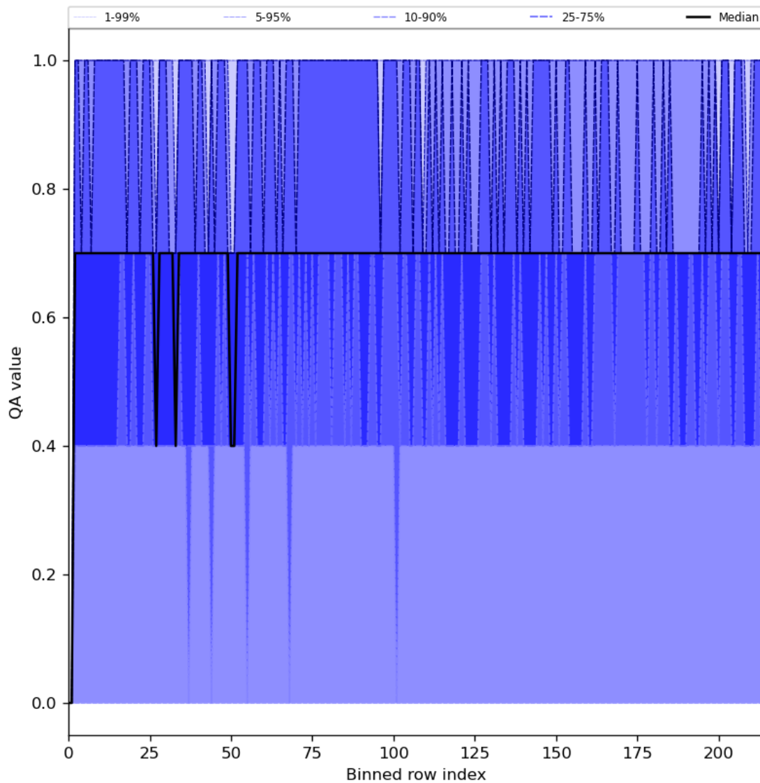
Figure 25: Along track statistics of “QA value” for 2024-05-24 to 2024-05-26
