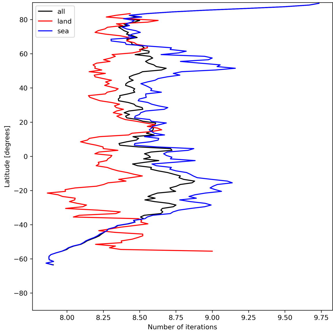
Figure 16: Zonal average of “Number of iterations” for 2024-05-24 to 2024-05-26.
