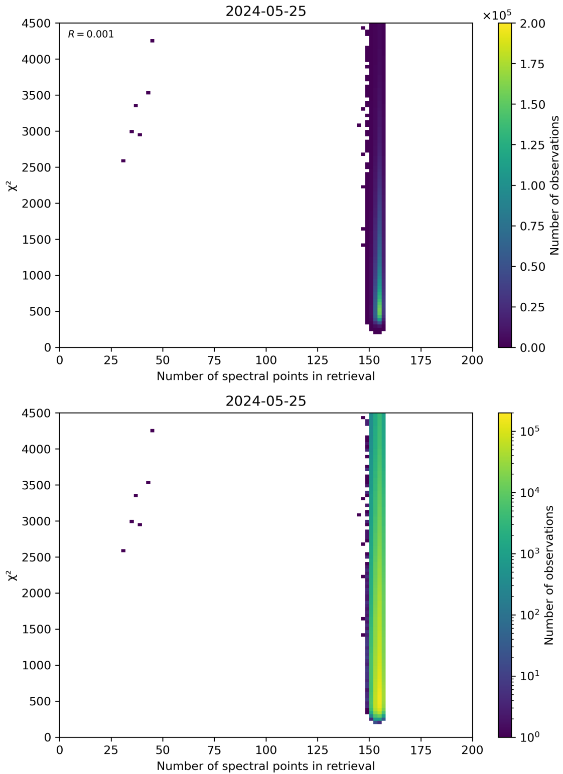
Figure 58: Scatter density plot of “Number of spectral points in retrieval” against “ \chi^2 ” for 2024-05-24 to 2024-05-26.
