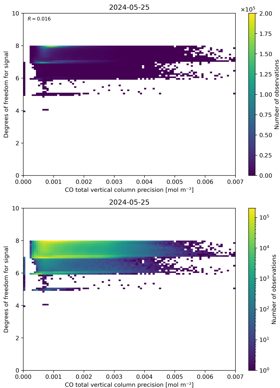
Figure 45: Scatter density plot of “CO total vertical column precision” against “Degrees of freedom for signal” for 2024-05-24 to 2024-05-26.
