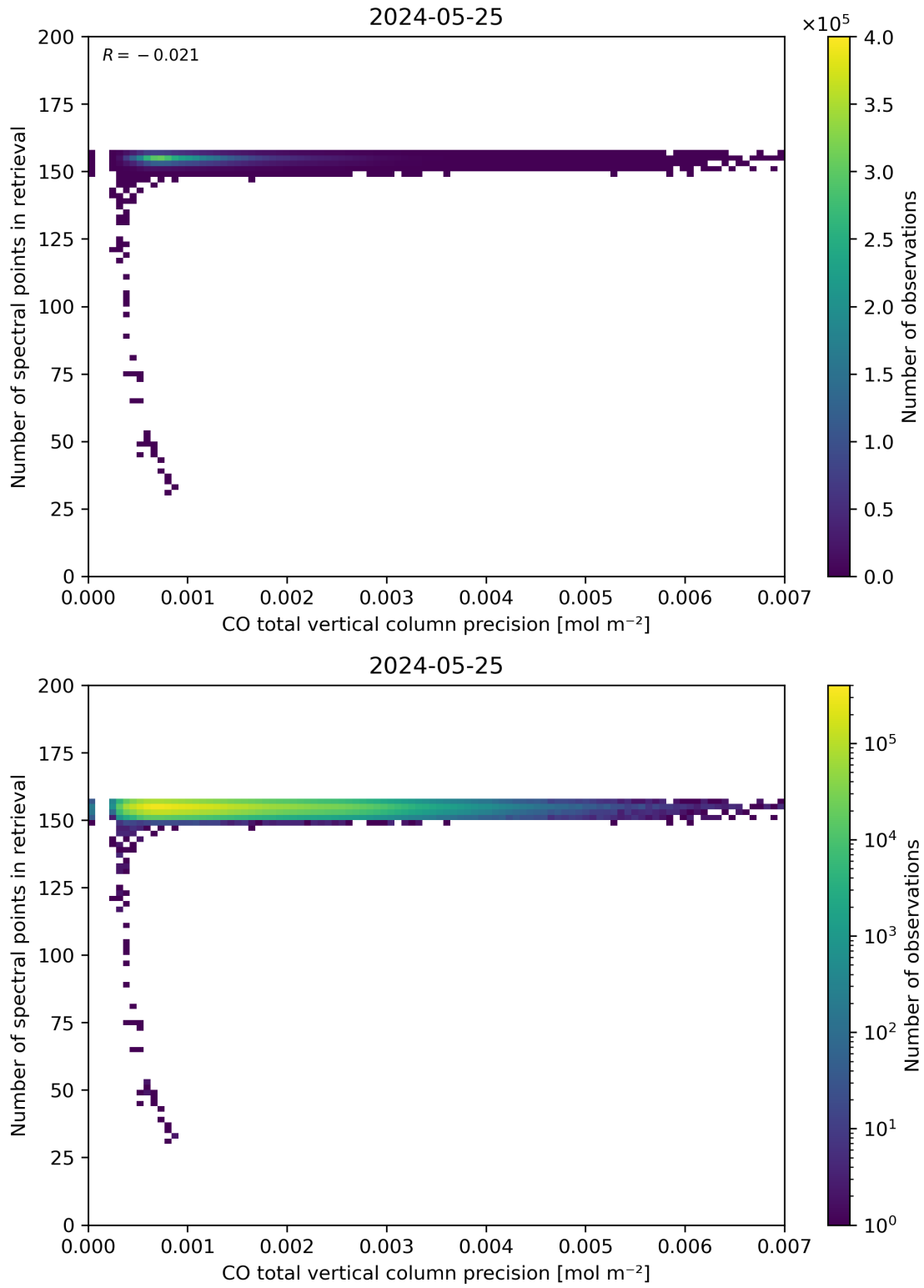
Figure 47: Scatter density plot of “CO total vertical column precision” against “Number of spectral points in retrieval” for 2024-05-24 to 2024-05-26.
