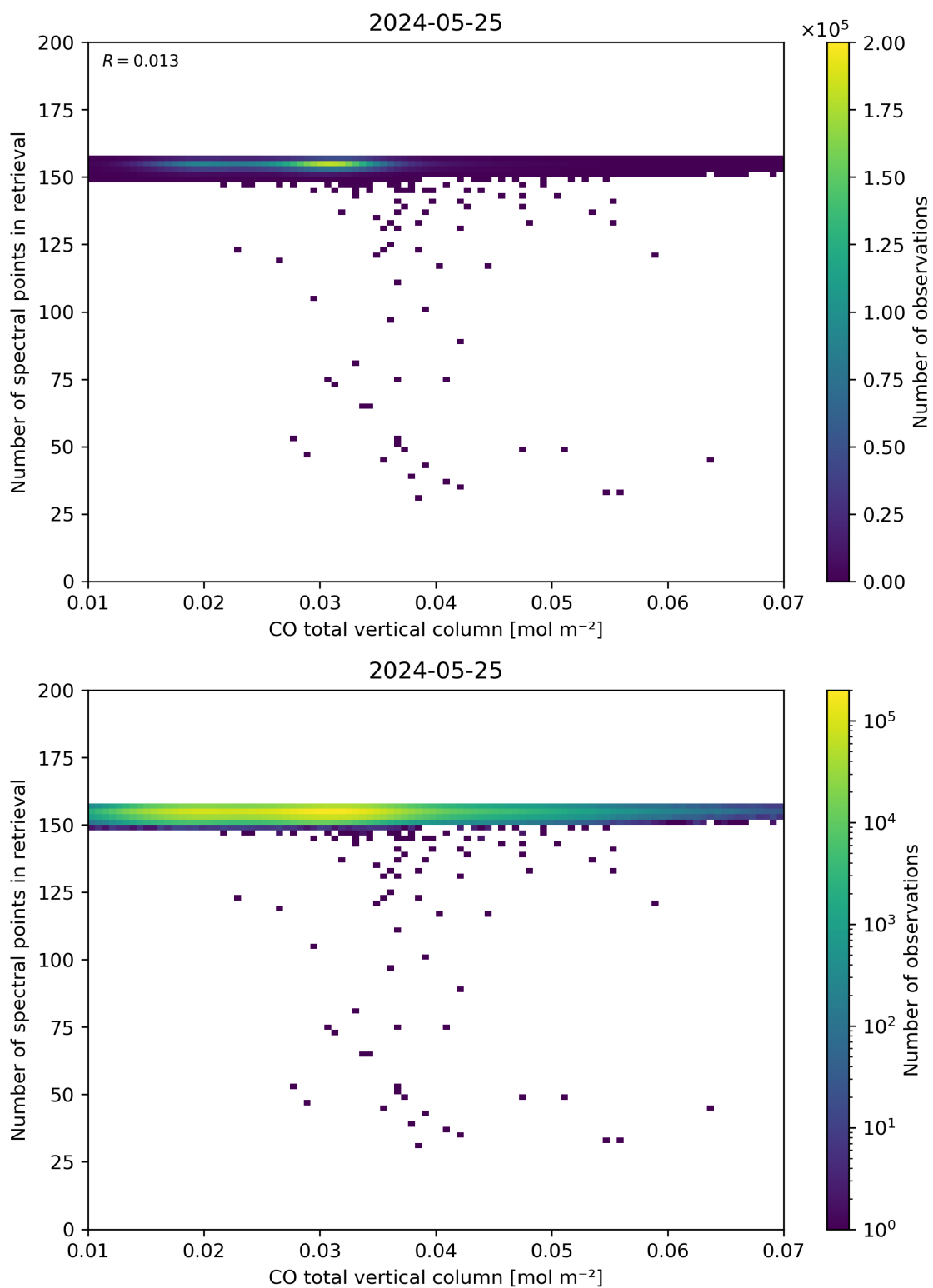
Figure 43: Scatter density plot of “CO total vertical column” against “Number of spectral points in retrieval” for 2024-05-24 to 2024-05-26.
