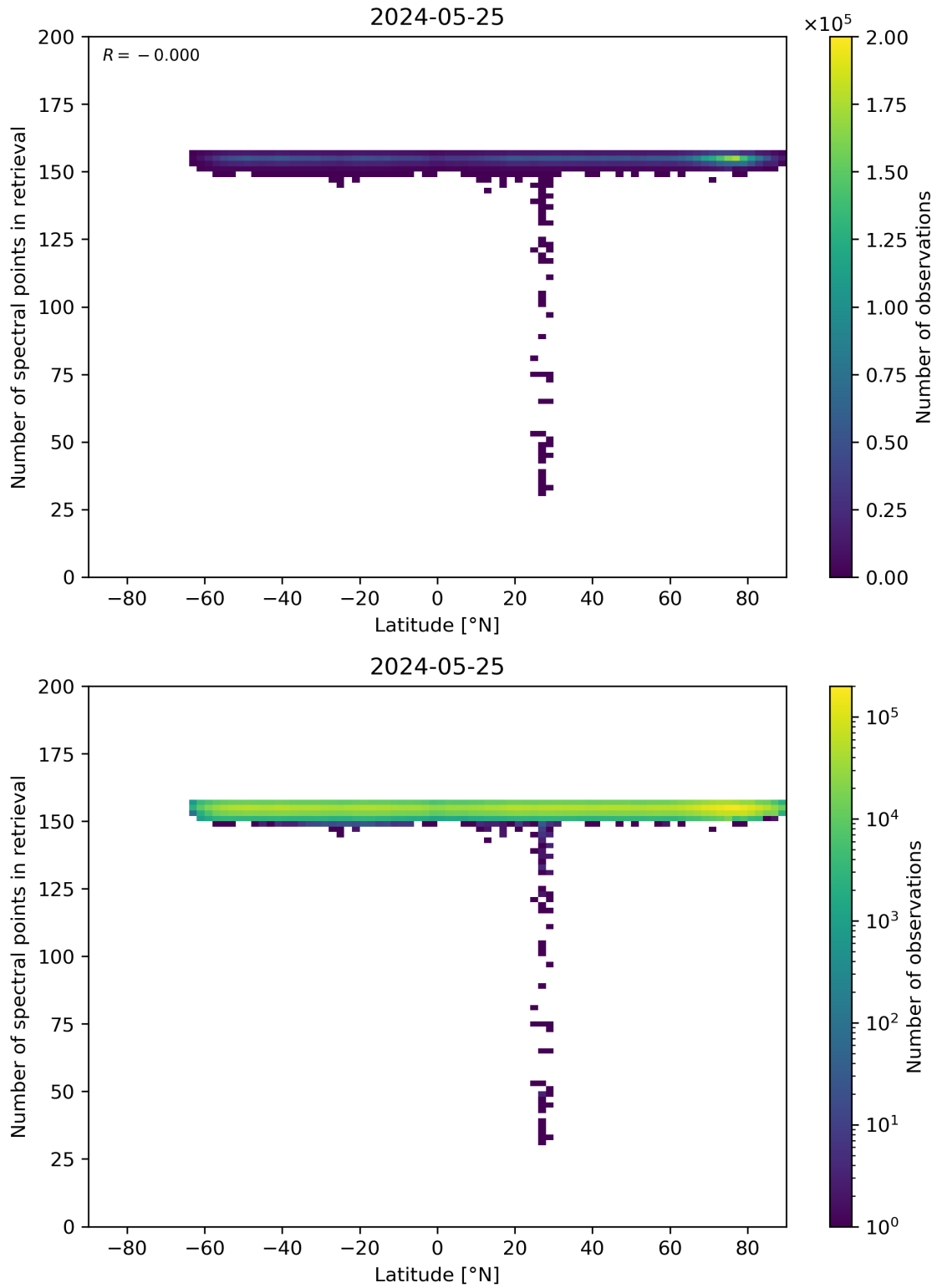
Figure 57: Scatter density plot of “Latitude” against “Number of spectral points in retrieval” for 2024-05-24 to 2024-05-26.
