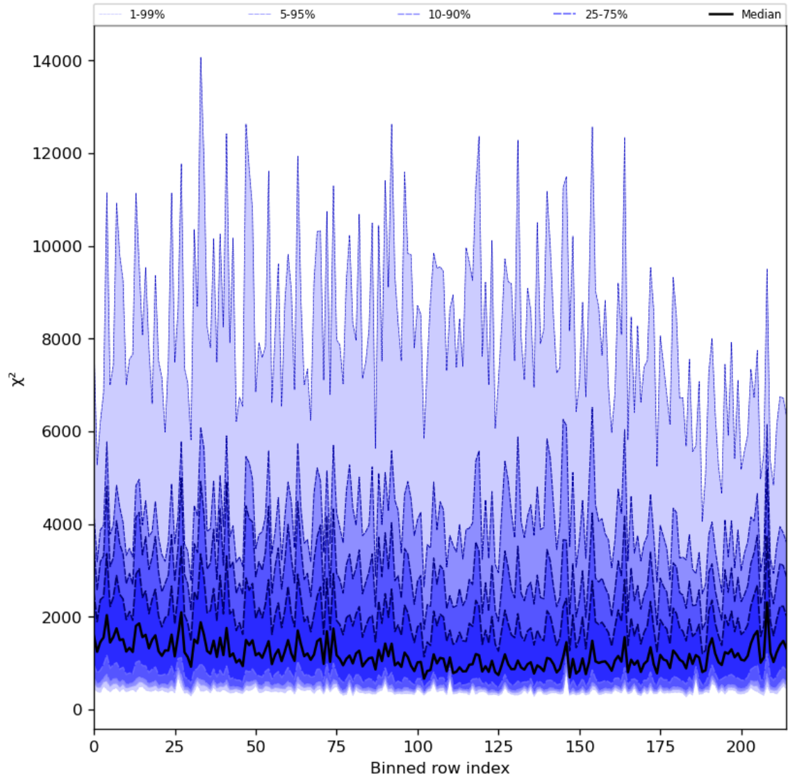
Figure 30: Along track statistics of “ \chi^2 ” for 2024-05-24 to 2024-05-26
