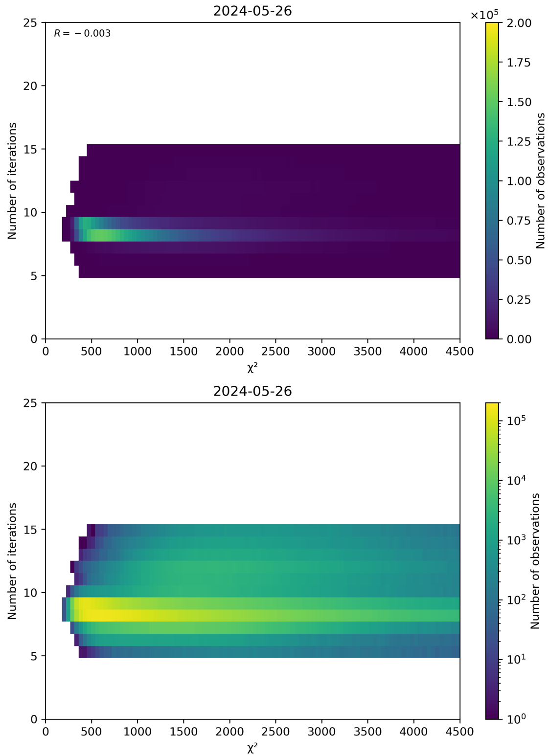
Figure 49: Scatter density plot of “ \chi^2 ” against “Number of iterations” for 2024-05-25 to 2024-05-27.
