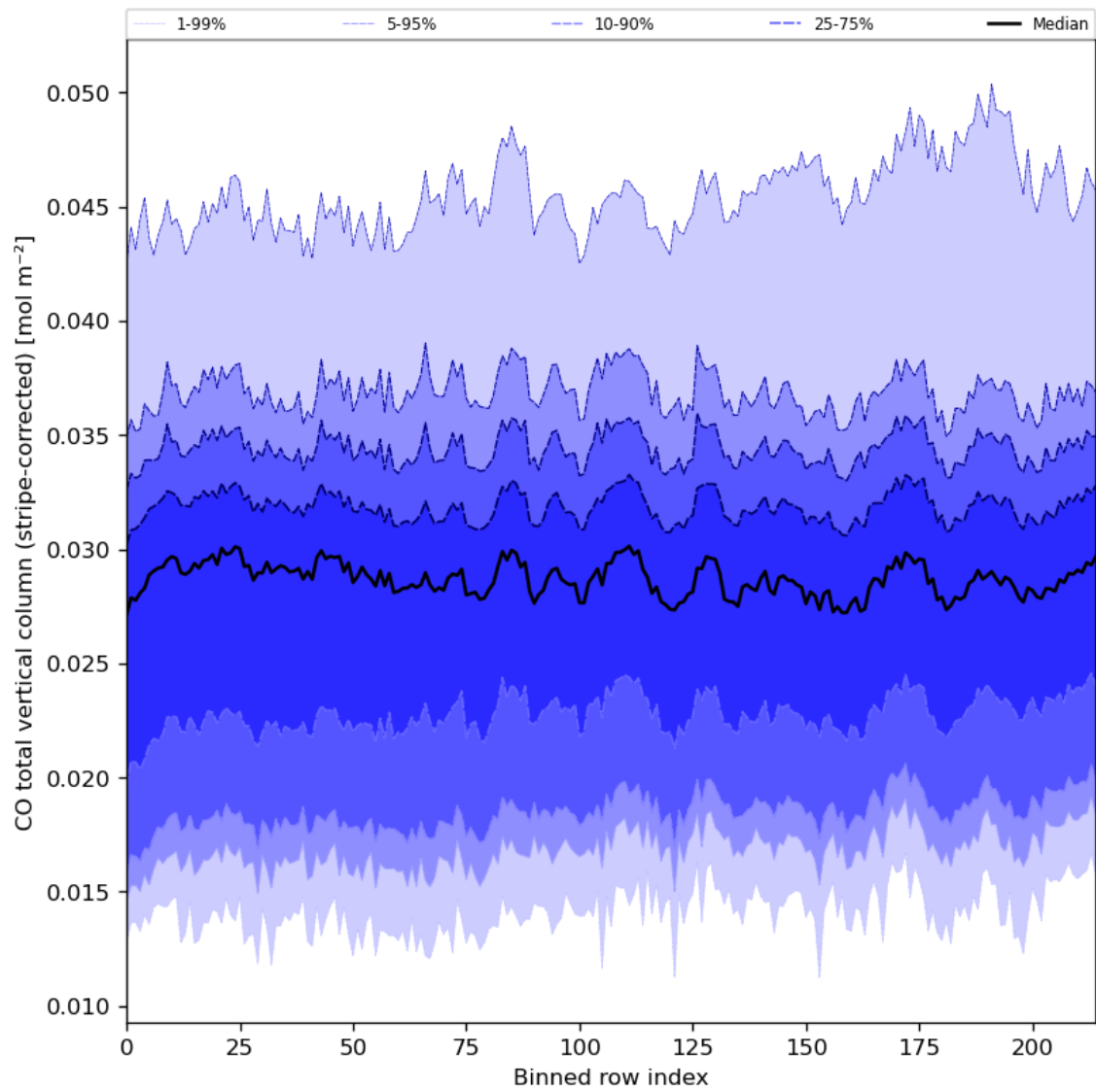
Figure 27: Along track statistics of “CO total vertical column (stripe-corrected)” for 2024-05-25 to 2024-05-27
