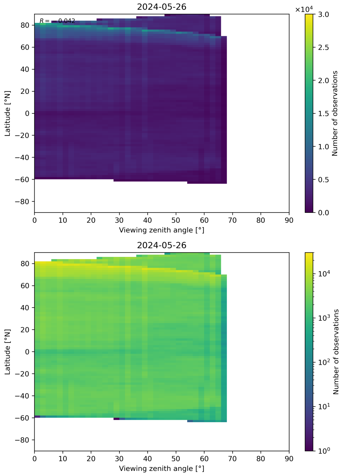
Figure 74: Scatter density plot of “Viewing zenith angle” against “Latitude” for 2024-05-25 to 2024-05-27.
