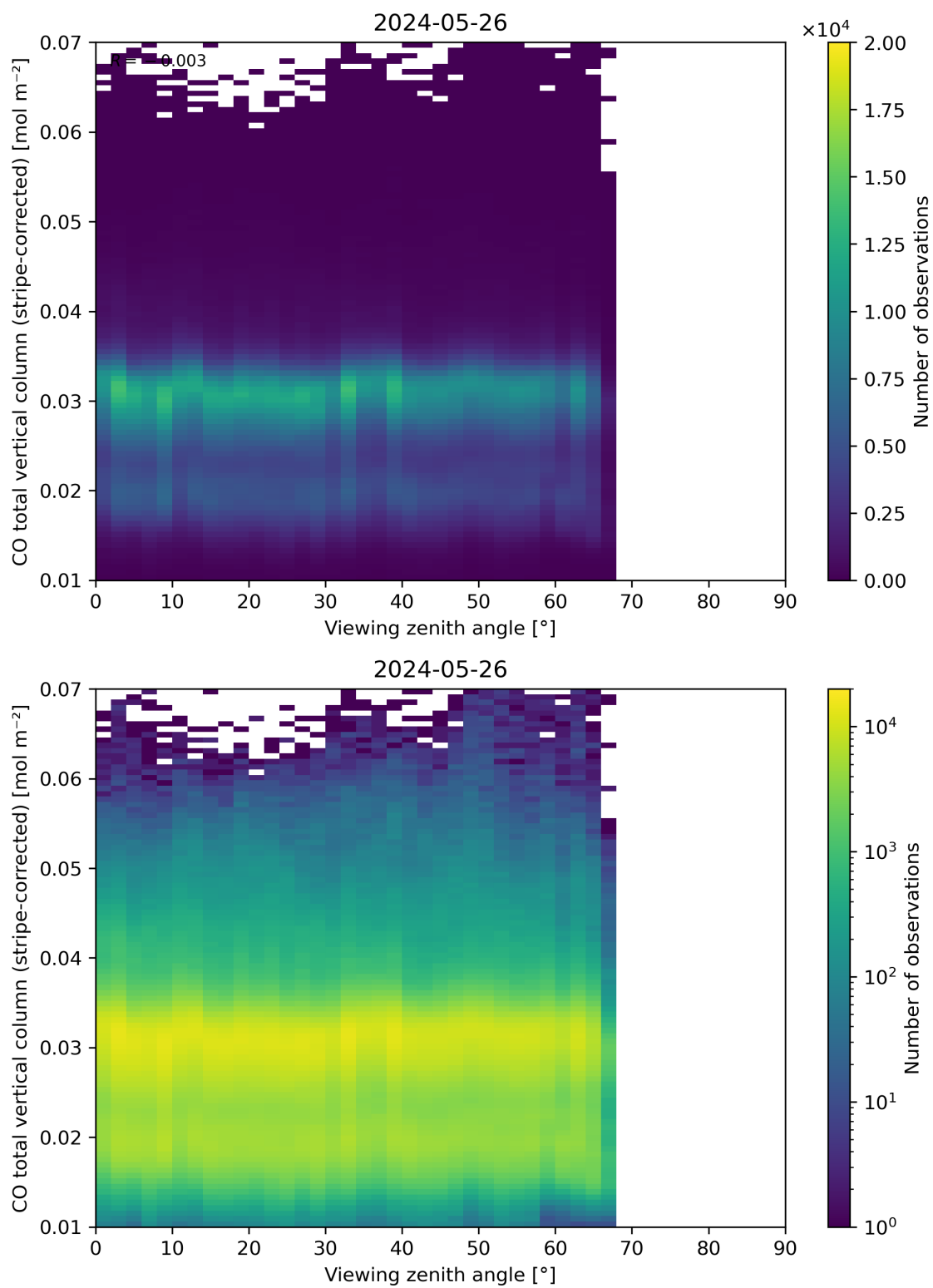
Figure 70: Scatter density plot of “Viewing zenith angle” against “CO total vertical column (stripe-corrected)” for 2024-05-25 to 2024-05-27.
