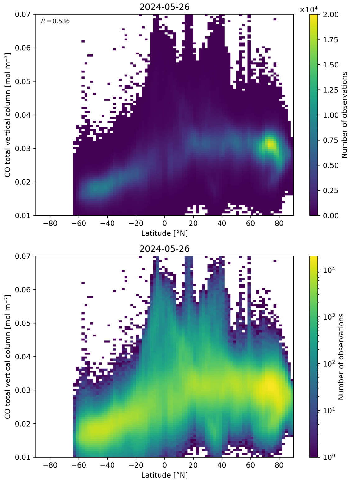
Figure 51: Scatter density plot of “Latitude” against “CO total vertical column” for 2024-05-25 to 2024-05-27.
