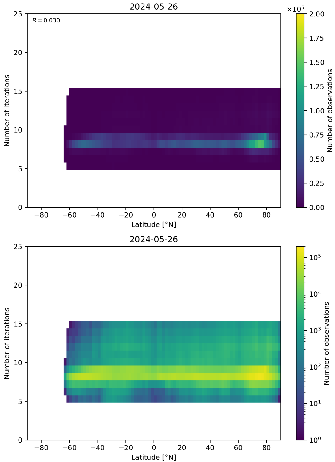
Figure 56: Scatter density plot of “Latitude” against “Number of iterations” for 2024-05-25 to 2024-05-27.
