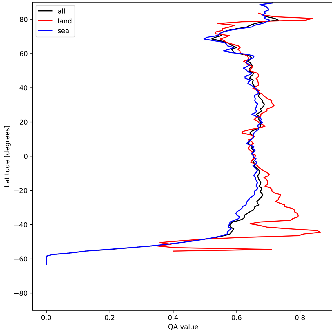
Figure 9: Zonal average of “QA value” for 2024-05-25 to 2024-05-27.
