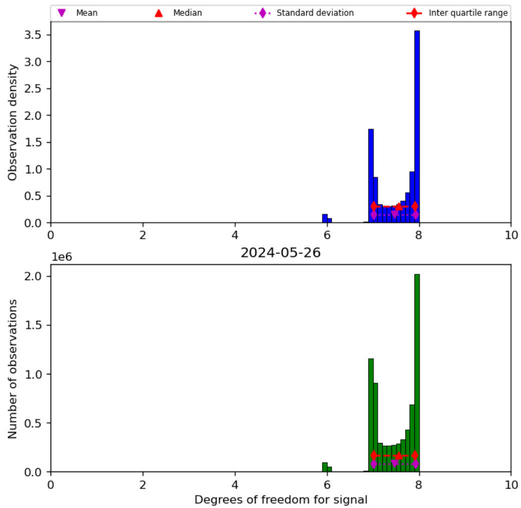
Figure 23: Histogram of “Degrees of freedom for signal” for 2024-05-25 to 2024-05-27
