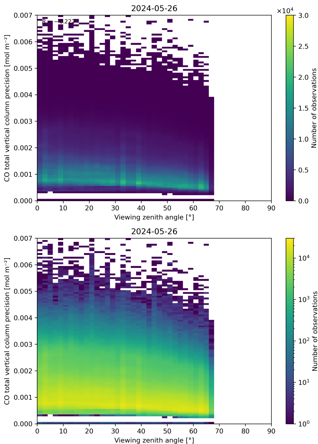
Figure 71: Scatter density plot of “Viewing zenith angle” against “CO total vertical column precision” for 2024-05-25 to 2024-05-27.
