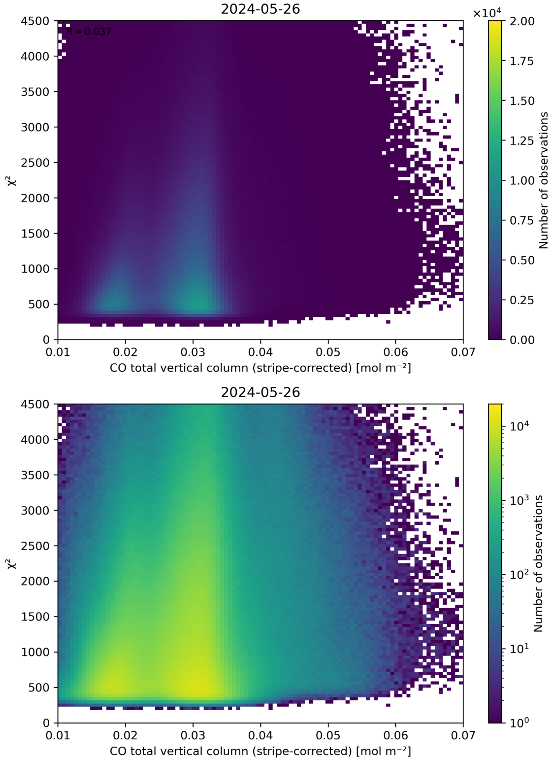
Figure 37: Scatter density plot of “CO total vertical column (stripe-corrected)” against “ \chi^2 ” for 2024-05-25 to 2024-05-27.
