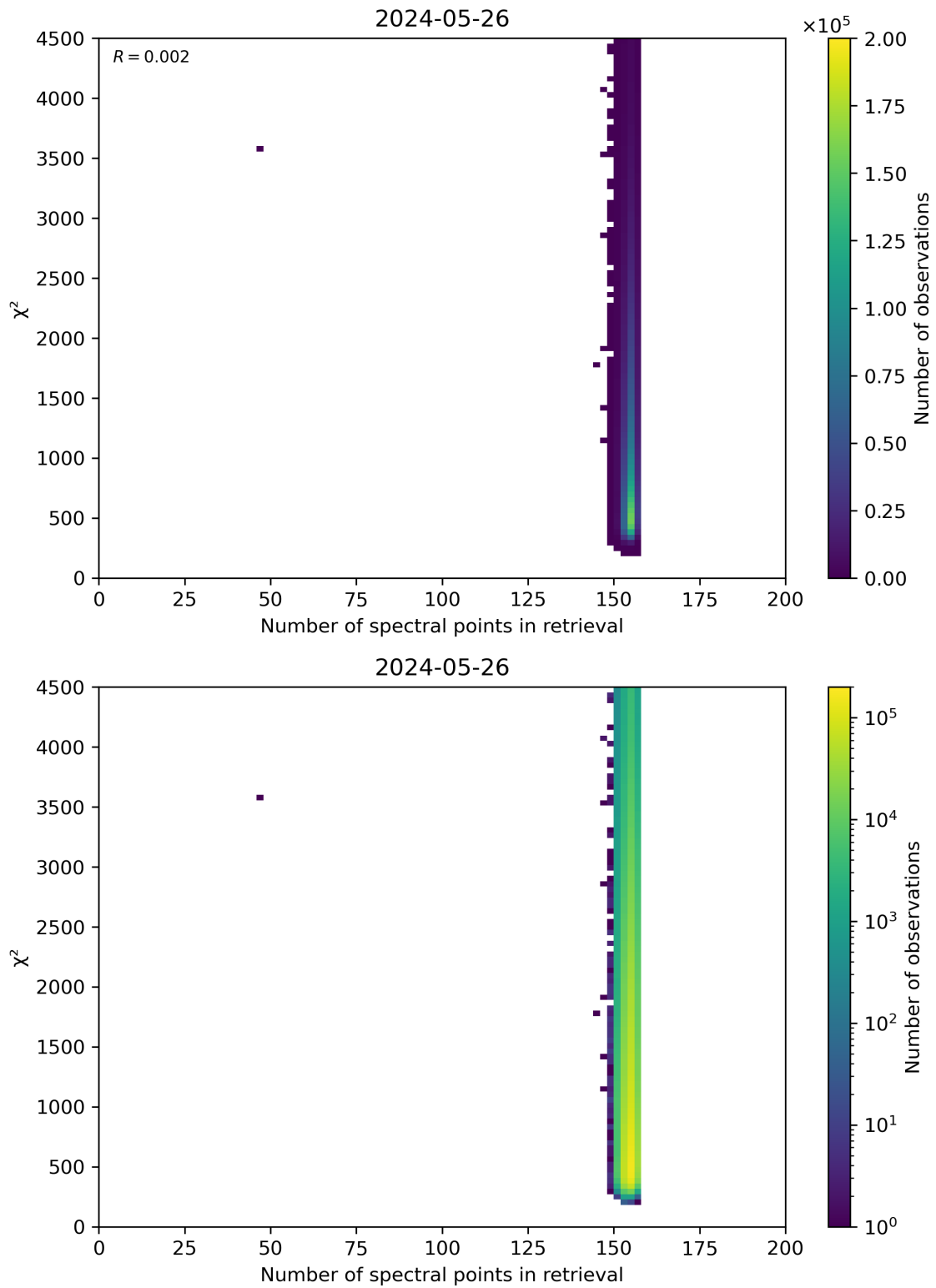
Figure 58: Scatter density plot of “Number of spectral points in retrieval” against “ \chi^2 ” for 2024-05-25 to 2024-05-27.
