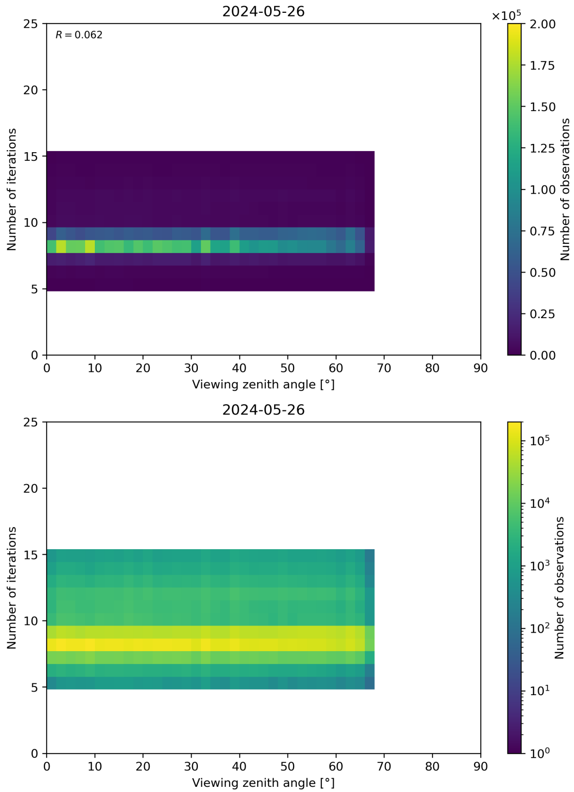
Figure 75: Scatter density plot of “Viewing zenith angle” against “Number of iterations” for 2024-05-25 to 2024-05-27.
