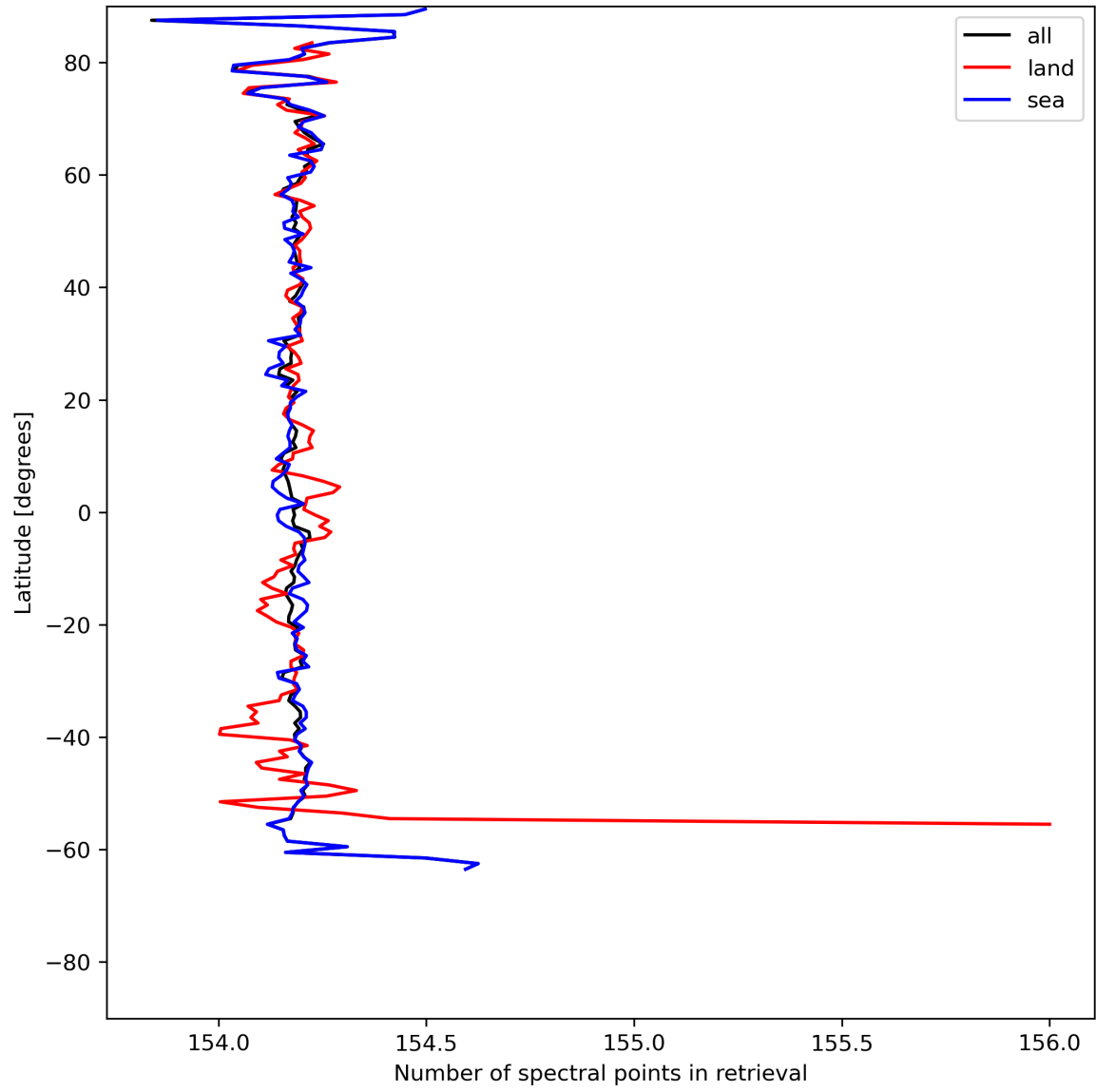
Figure 13: Zonal average of “Number of spectral points in retrieval” for 2024-05-25 to 2024-05-27.
