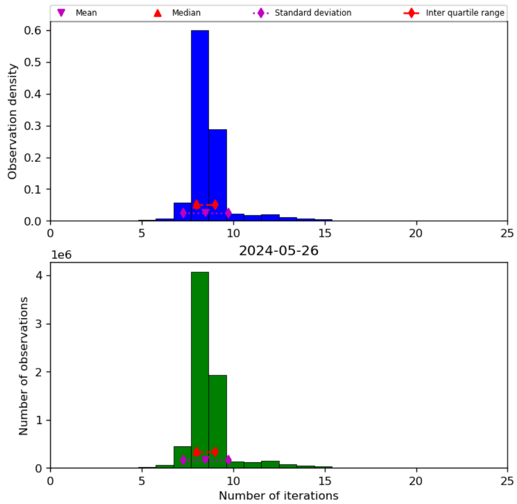
Figure 24: Histogram of “Number of iterations” for 2024-05-25 to 2024-05-27
