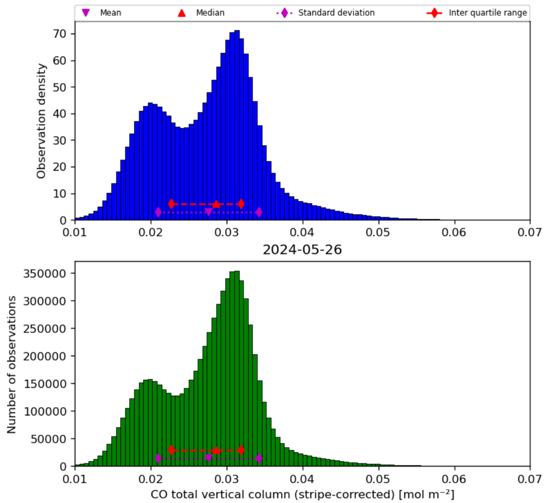
Figure 19: Histogram of “CO total vertical column (stripe-corrected)” for 2024-05-25 to 2024-05-27
