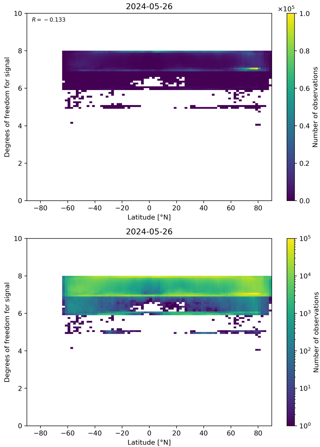
Figure 55: Scatter density plot of “Latitude” against “Degrees of freedom for signal” for 2024-05-25 to 2024-05-27.
