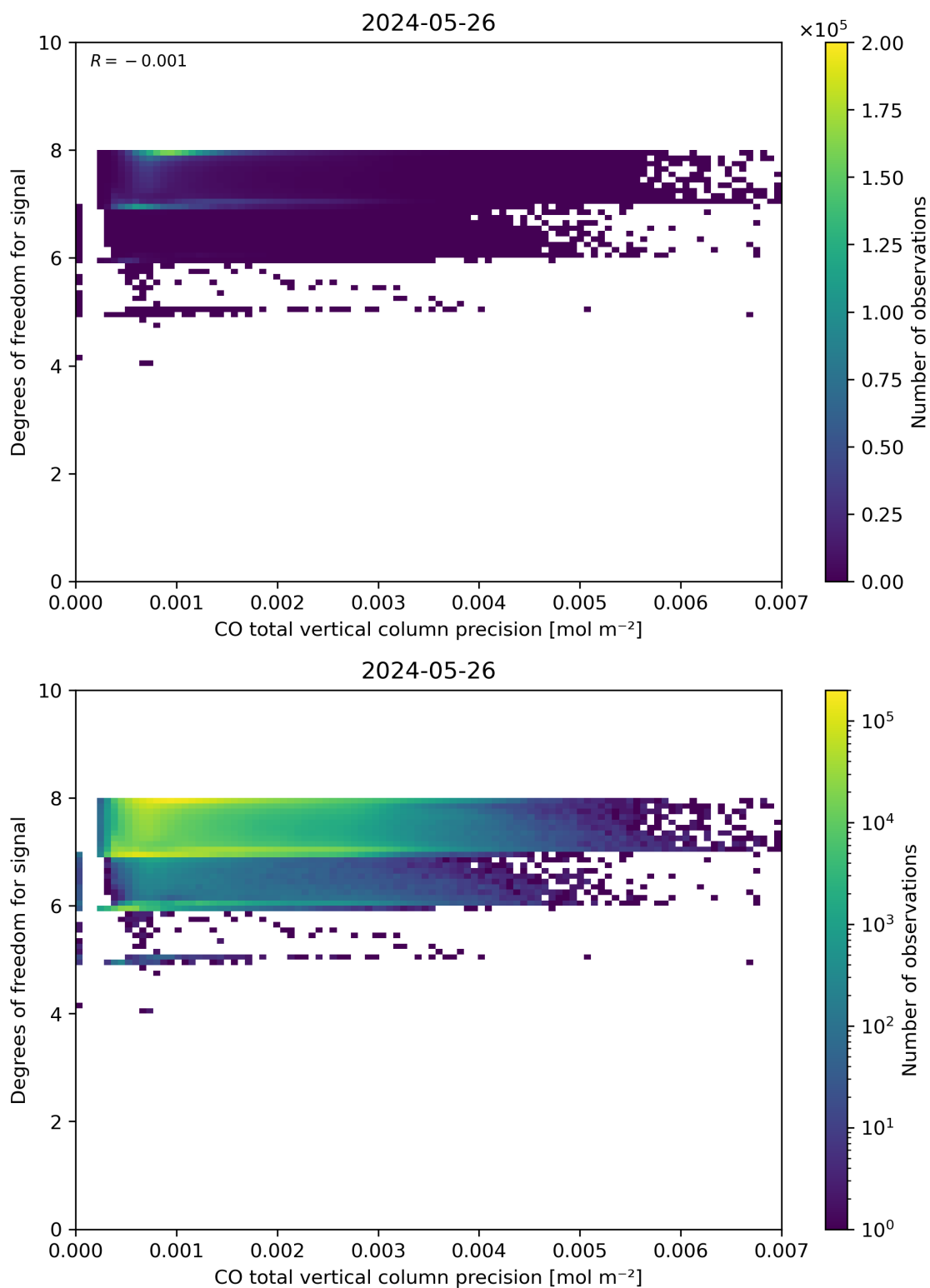
Figure 45: Scatter density plot of “CO total vertical column precision” against “Degrees of freedom for signal” for 2024-05-25 to 2024-05-27.
