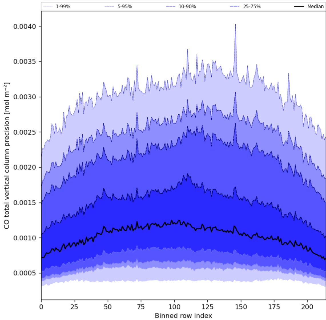
Figure 28: Along track statistics of “CO total vertical column precision” for 2024-05-25 to 2024-05-27
