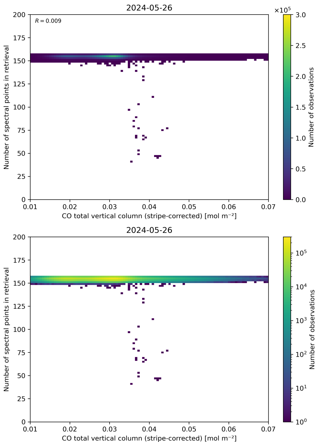
Figure 40: Scatter density plot of “CO total vertical column (stripe-corrected)” against “Number of spectral points in retrieval” for 2024-05-25 to 2024-05-27.
