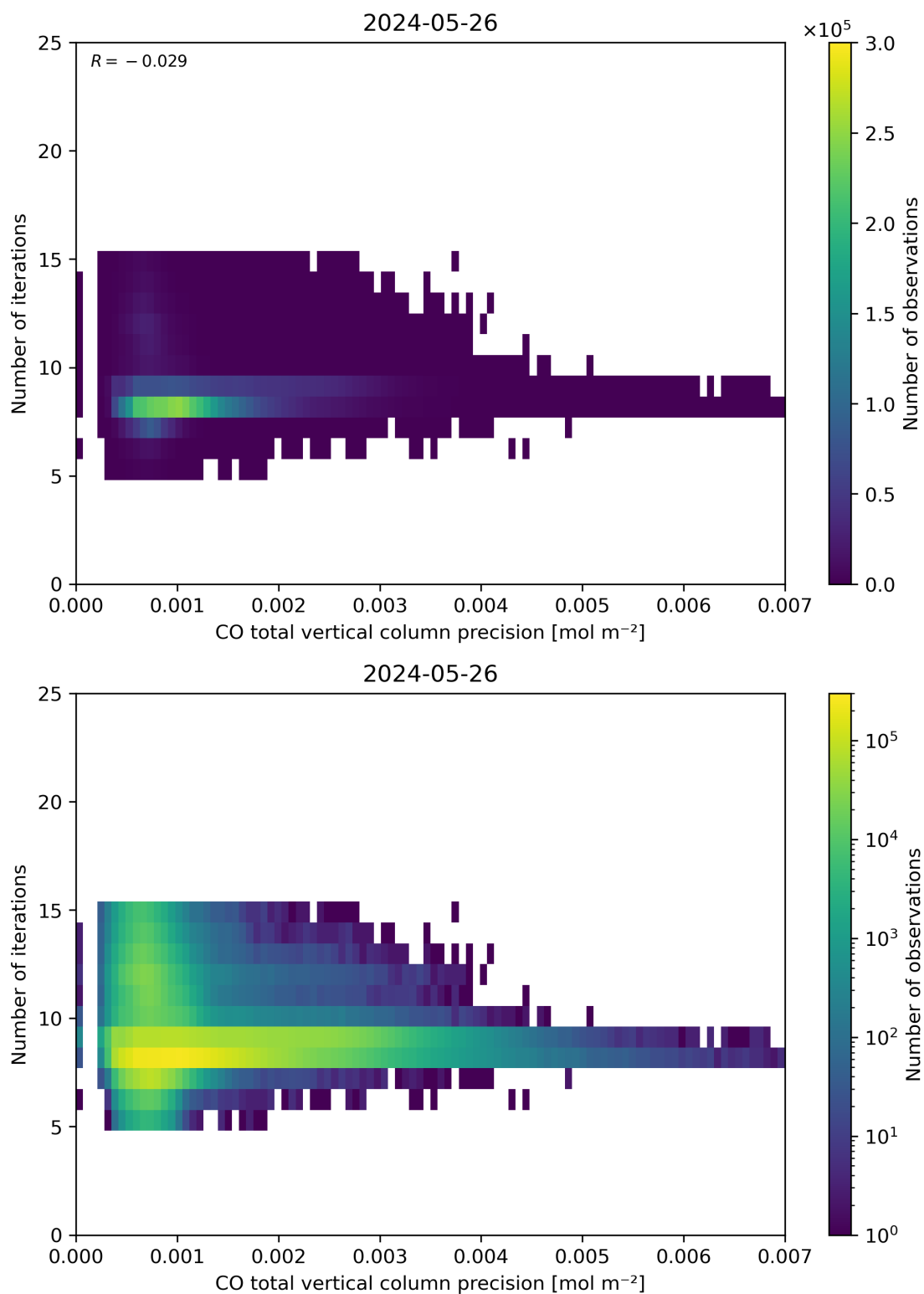
Figure 46: Scatter density plot of “CO total vertical column precision” against “Number of iterations” for 2024-05-25 to 2024-05-27.
