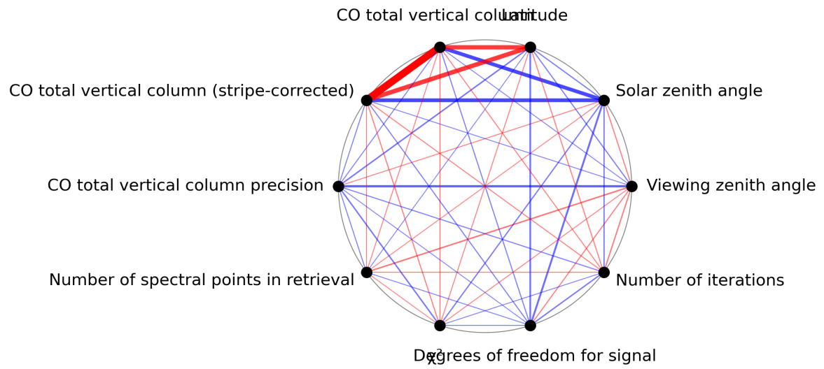
Figure 1: Map of correlation graph for 2024-05-25 to 2024-05-27.
