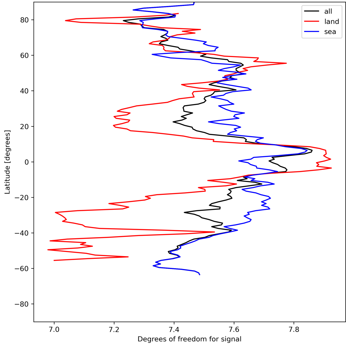
Figure 15: Zonal average of “Degrees of freedom for signal” for 2024-05-25 to 2024-05-27.
