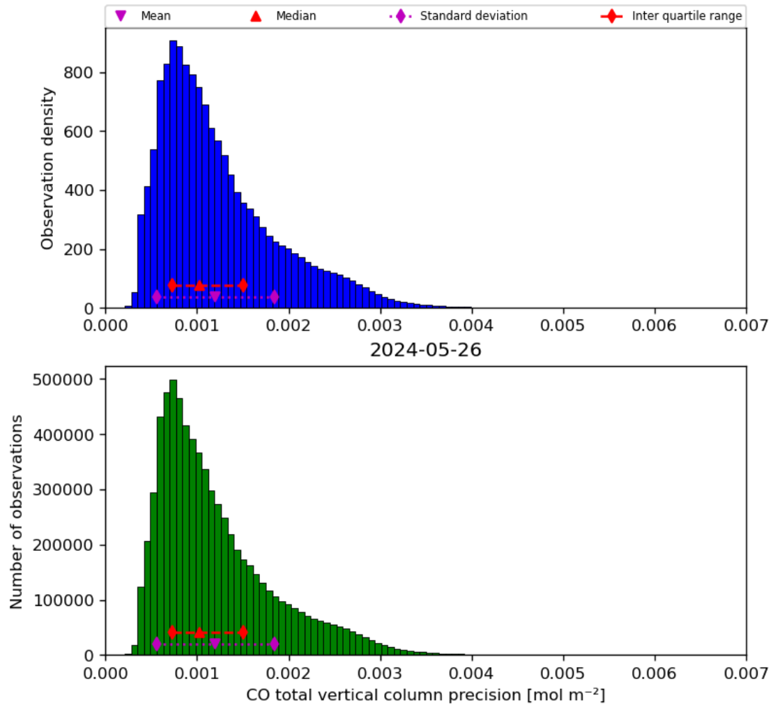
Figure 20: Histogram of “CO total vertical column precision” for 2024-05-25 to 2024-05-27
