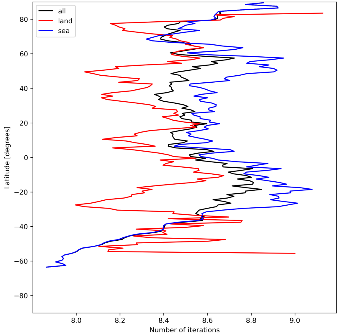
Figure 16: Zonal average of “Number of iterations” for 2024-05-25 to 2024-05-27.
