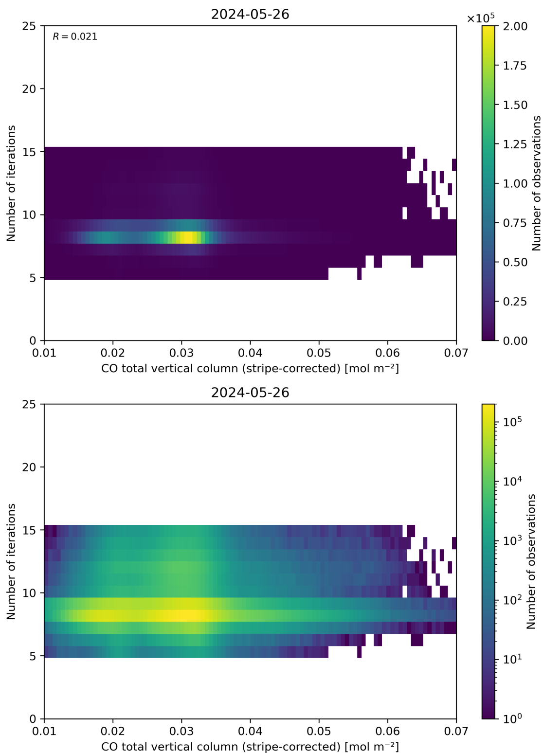
Figure 39: Scatter density plot of “CO total vertical column (stripe-corrected)” against “Number of iterations” for 2024-05-25 to 2024-05-27.
