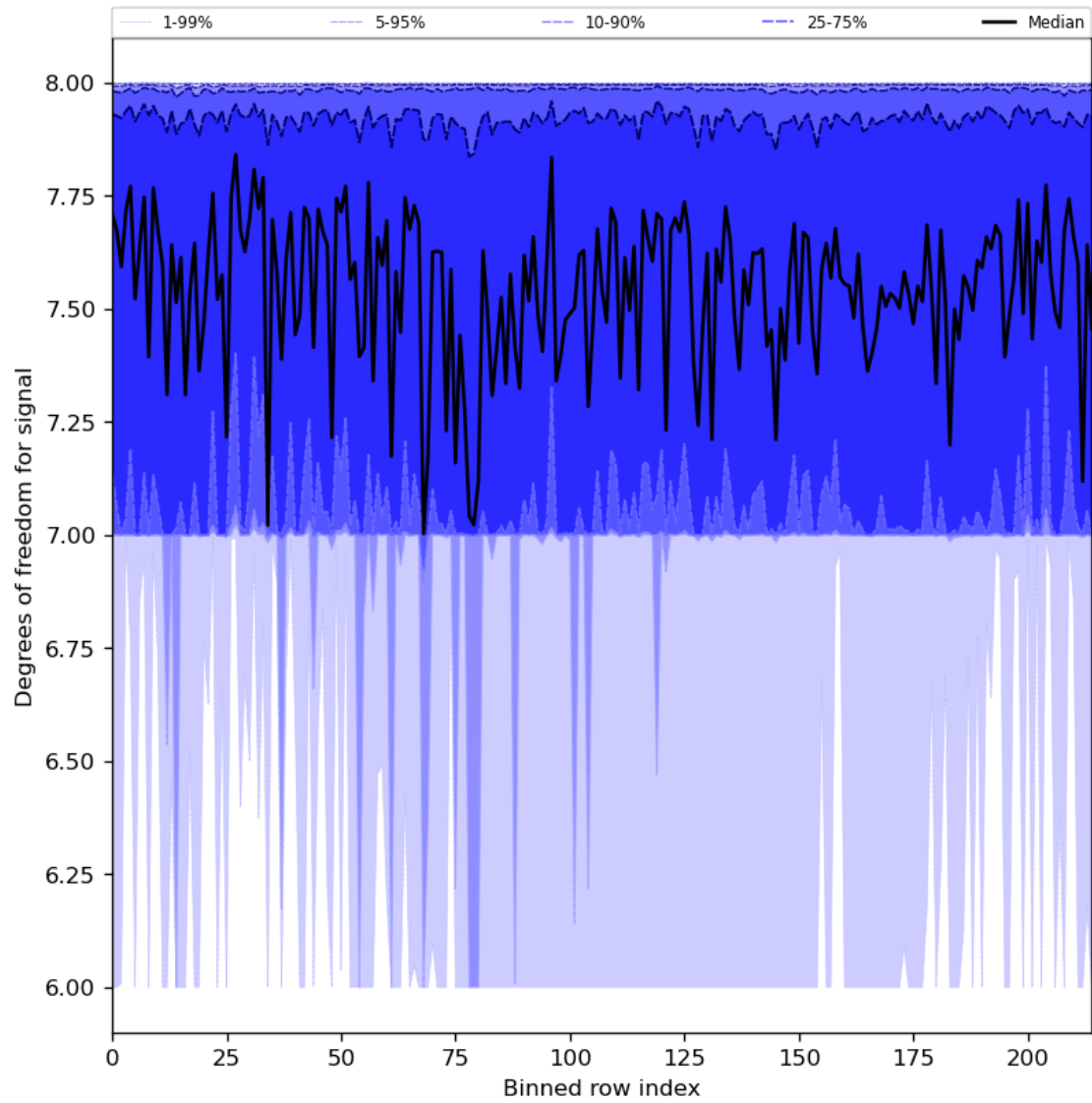
Figure 31: Along track statistics of “Degrees of freedom for signal” for 2024-05-25 to 2024-05-27
