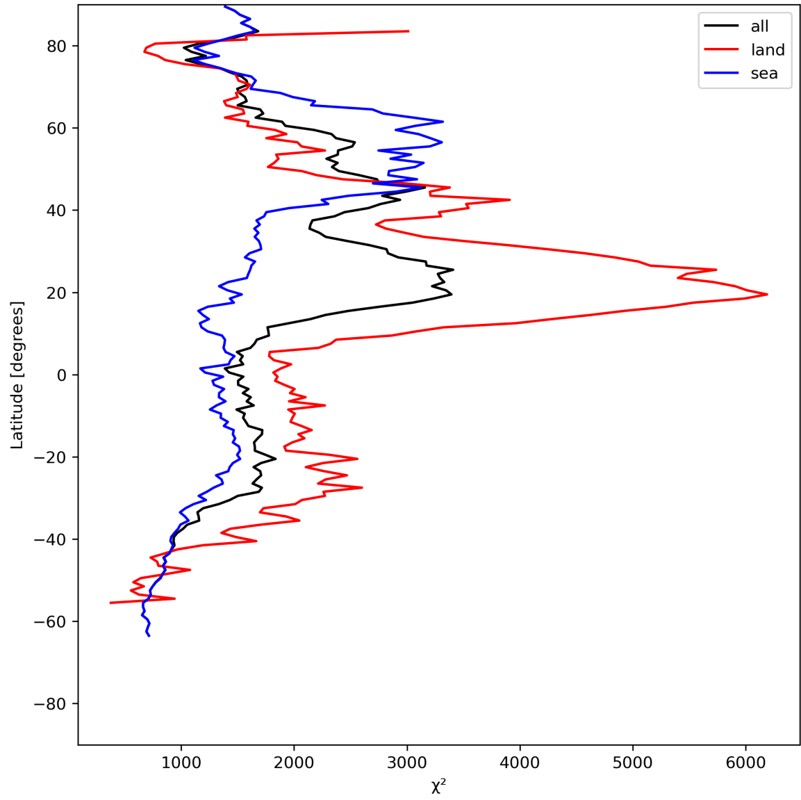
Figure 14: Zonal average of “ \chi^2 ” for 2024-05-25 to 2024-05-27.
