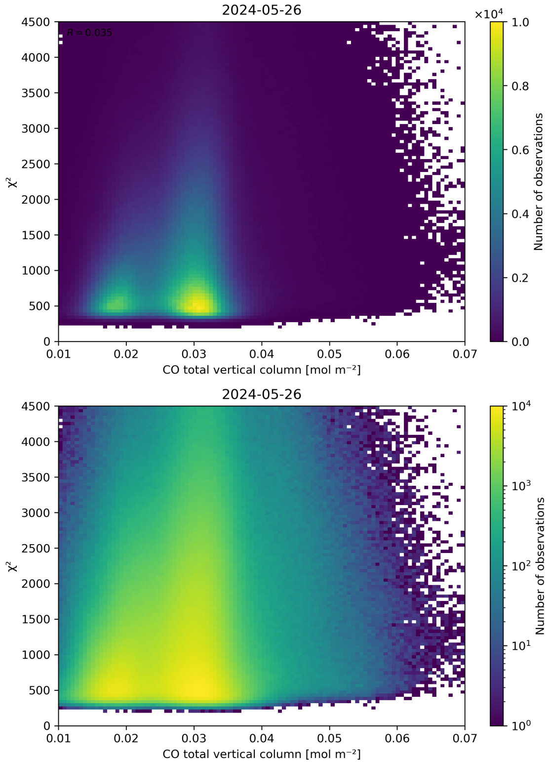
Figure 35: Scatter density plot of “CO total vertical column” against “ \chi^2 ” for 2024-05-25 to 2024-05-27.
