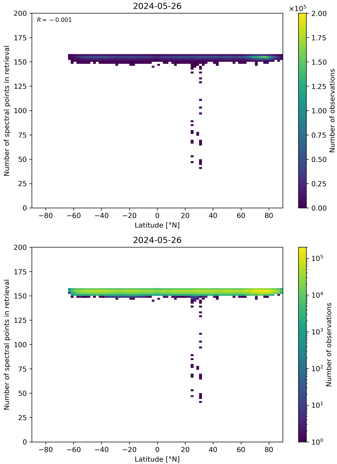
Figure 57: Scatter density plot of “Latitude” against “Number of spectral points in retrieval” for 2024-05-25 to 2024-05-27.
