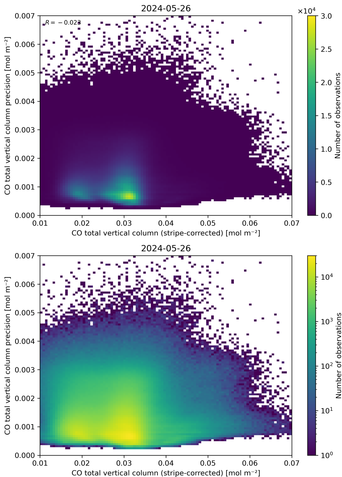
Figure 36: Scatter density plot of “CO total vertical column (stripe-corrected)” against “CO total vertical column precision” for 2024-05-25 to 2024-05-27.
