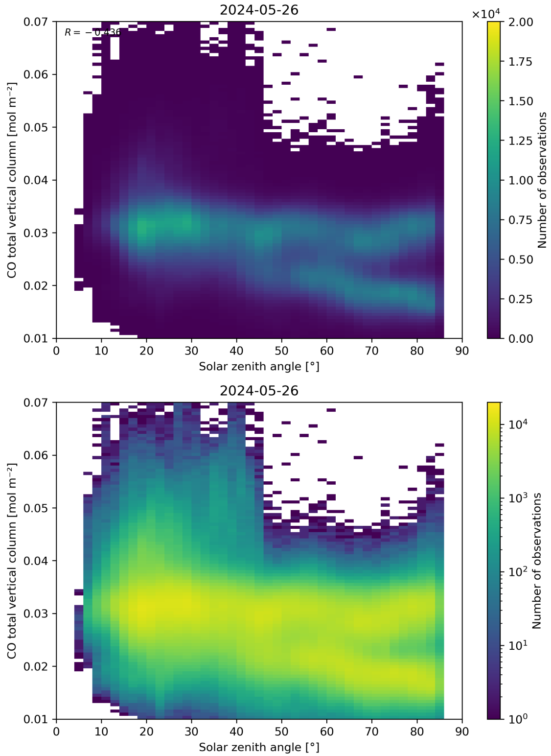
Figure 61: Scatter density plot of “Solar zenith angle” against “CO total vertical column” for 2024-05-25 to 2024-05-27.
