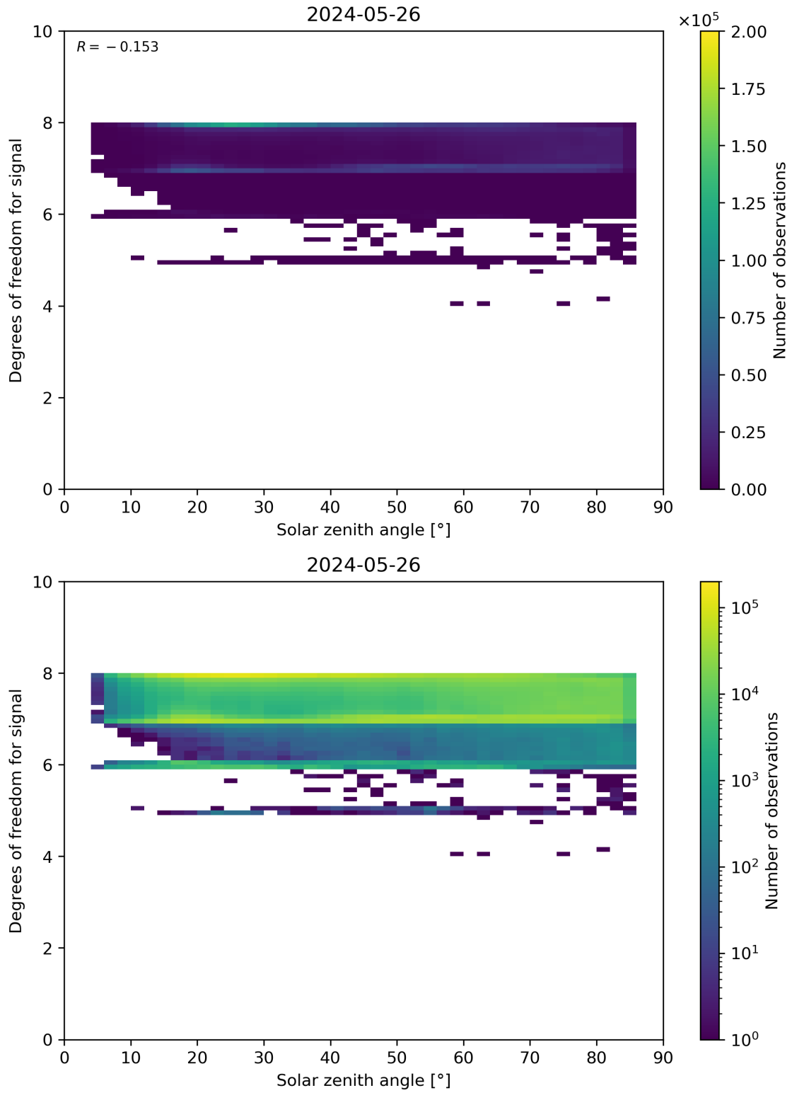
Figure 65: Scatter density plot of “Solar zenith angle” against “Degrees of freedom for signal” for 2024-05-25 to 2024-05-27.
