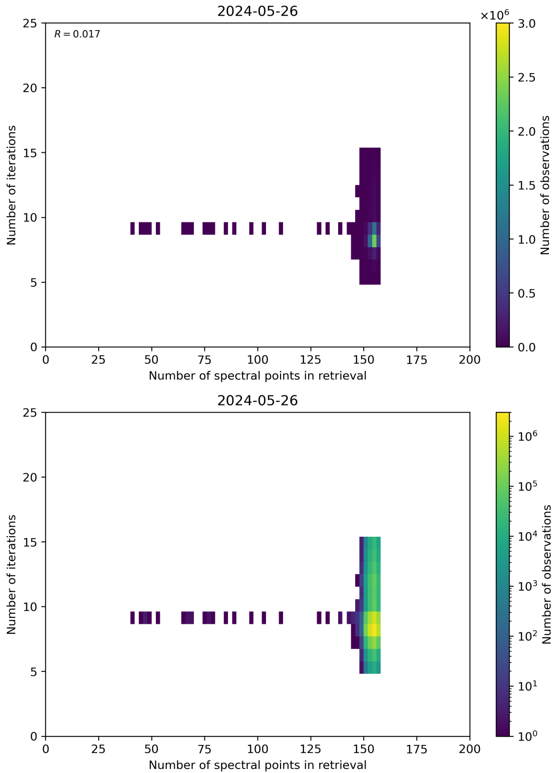
Figure 60: Scatter density plot of “Number of spectral points in retrieval” against “Number of iterations” for 2024-05-25 to 2024-05-27.
