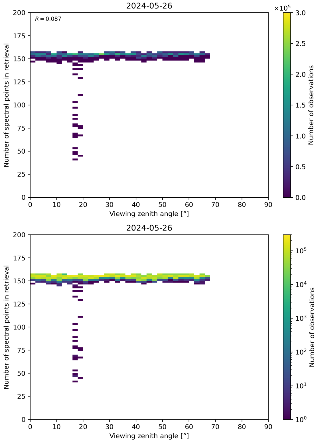
Figure 76: Scatter density plot of “Viewing zenith angle” against “Number of spectral points in retrieval” for 2024-05-25 to 2024-05-27.
