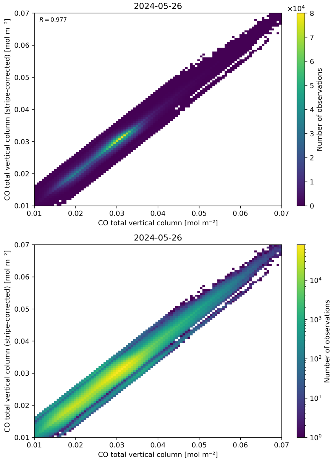
Figure 33: Scatter density plot of “CO total vertical column” against “CO total vertical column (stripe-corrected)” for 2024-05-25 to 2024-05-27.
