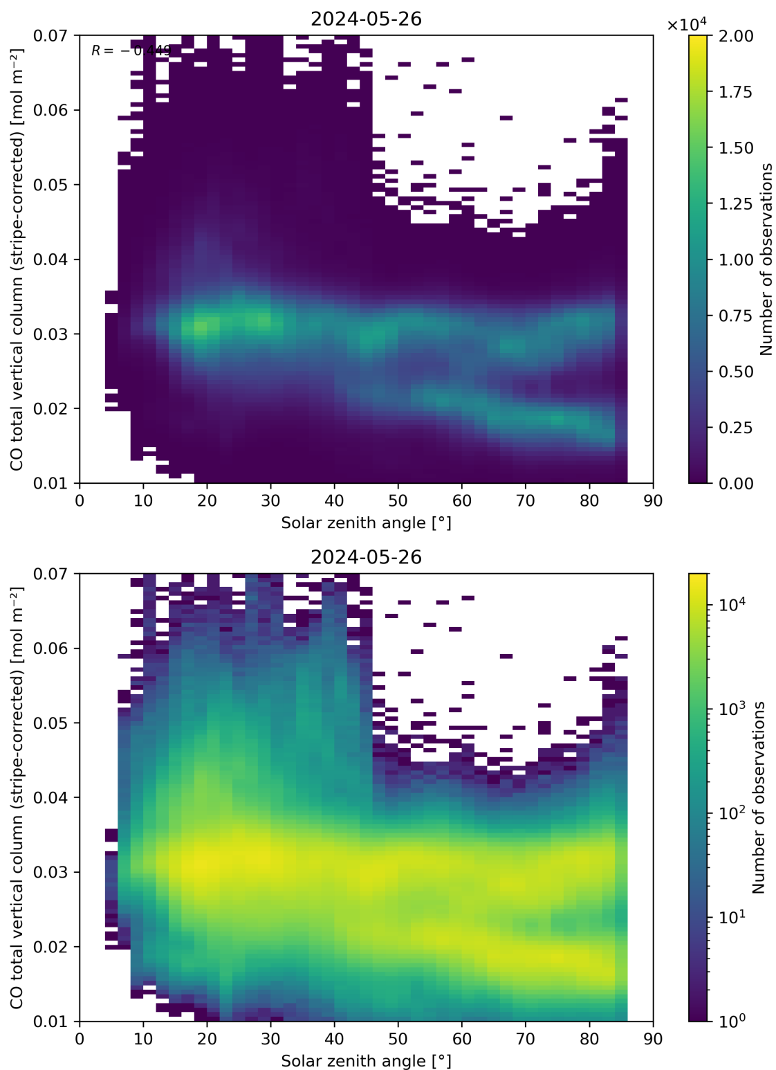
Figure 62: Scatter density plot of “Solar zenith angle” against “CO total vertical column (stripe-corrected)” for 2024-05-25 to 2024-05-27.
