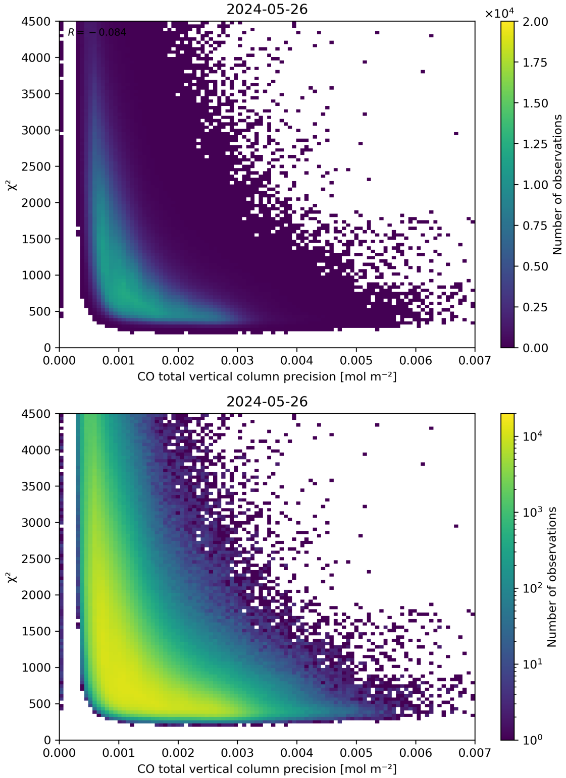
Figure 44: Scatter density plot of “CO total vertical column precision” against “ \chi^2 ” for 2024-05-25 to 2024-05-27.
