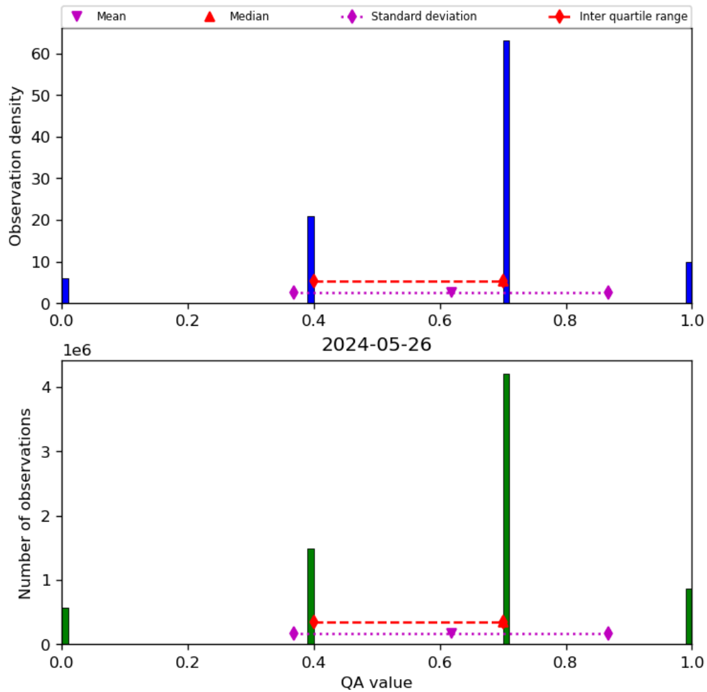
Figure 17: Histogram of “QA value” for 2024-05-25 to 2024-05-27
