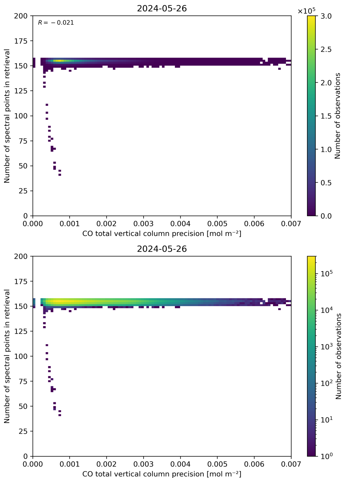
Figure 47: Scatter density plot of “CO total vertical column precision” against “Number of spectral points in retrieval” for 2024-05-25 to 2024-05-27.
