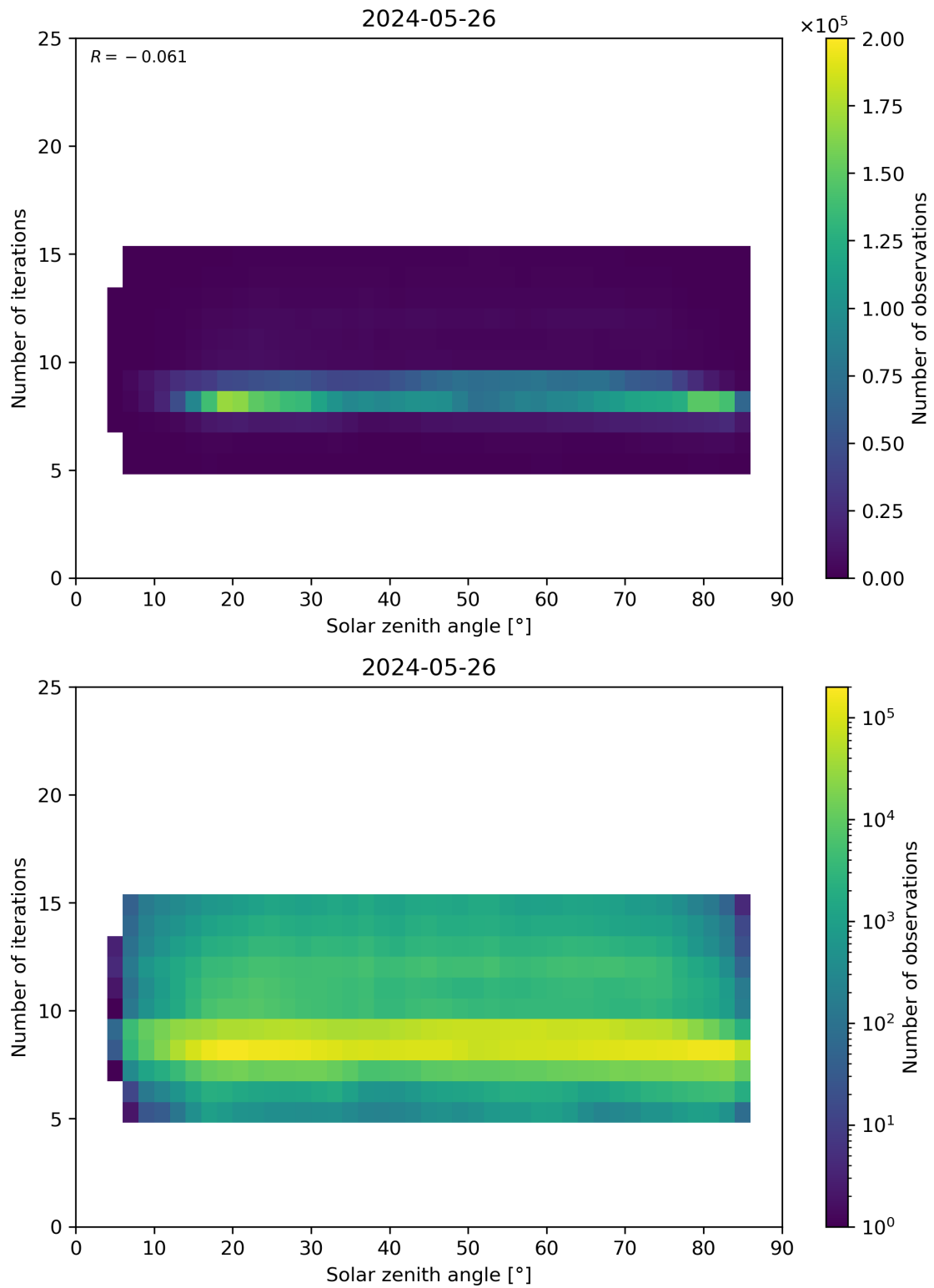
Figure 67: Scatter density plot of “Solar zenith angle” against “Number of iterations” for 2024-05-25 to 2024-05-27.
