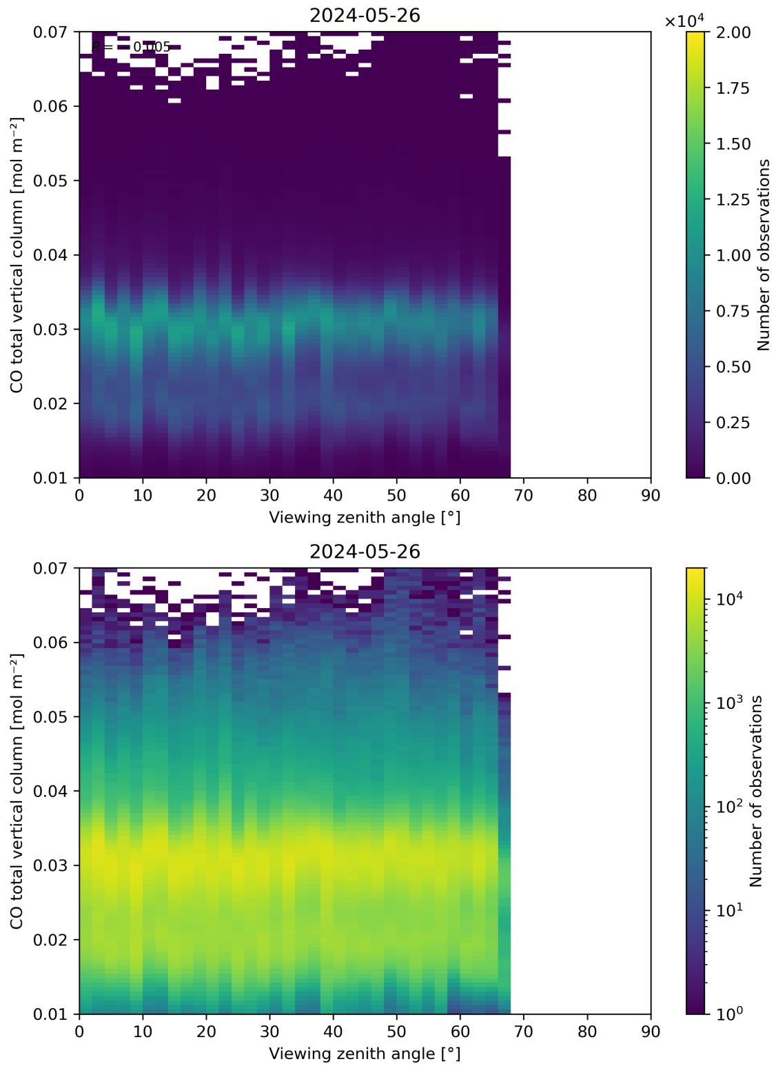
Figure 69: Scatter density plot of “Viewing zenith angle” against “CO total vertical column” for 2024-05-25 to 2024-05-27.
