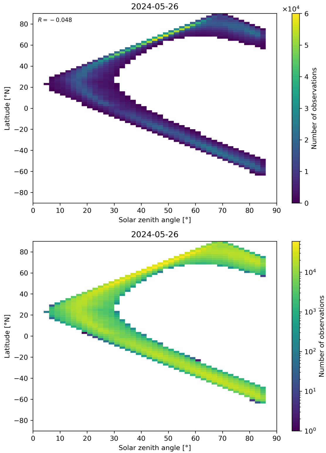
Figure 66: Scatter density plot of “Solar zenith angle” against “Latitude” for 2024-05-25 to 2024-05-27.
