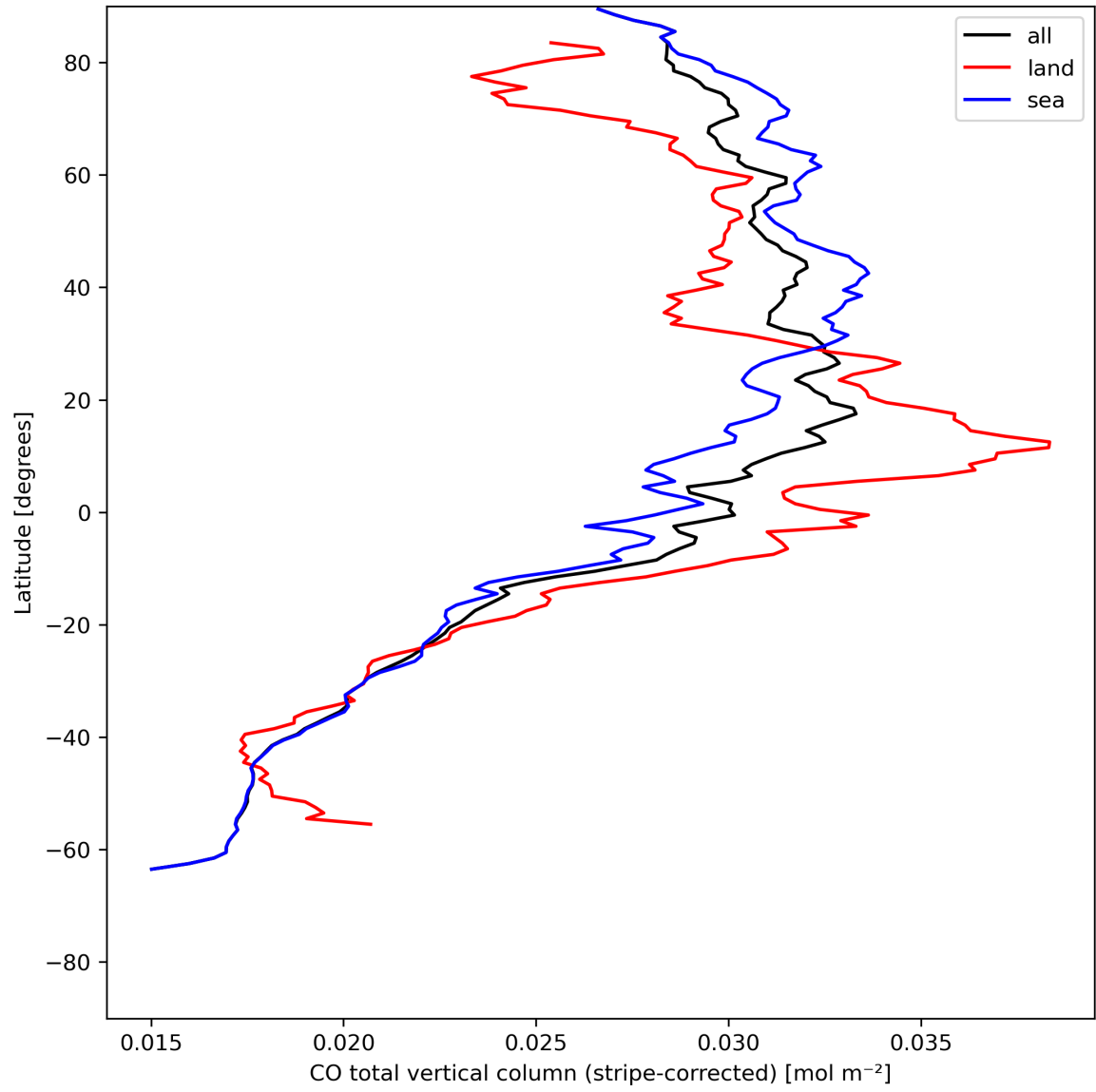
Figure 11: Zonal average of “CO total vertical column (stripe-corrected)” for 2024-05-25 to 2024-05-27.
