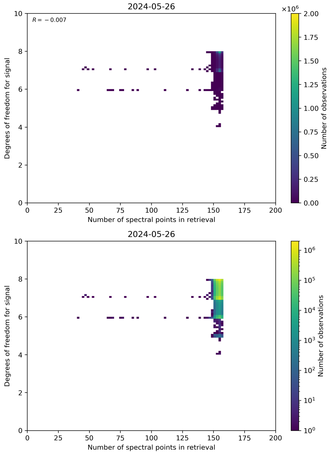
Figure 59: Scatter density plot of “Number of spectral points in retrieval” against “Degrees of freedom for signal” for 2024-05-25 to 2024-05-27.
