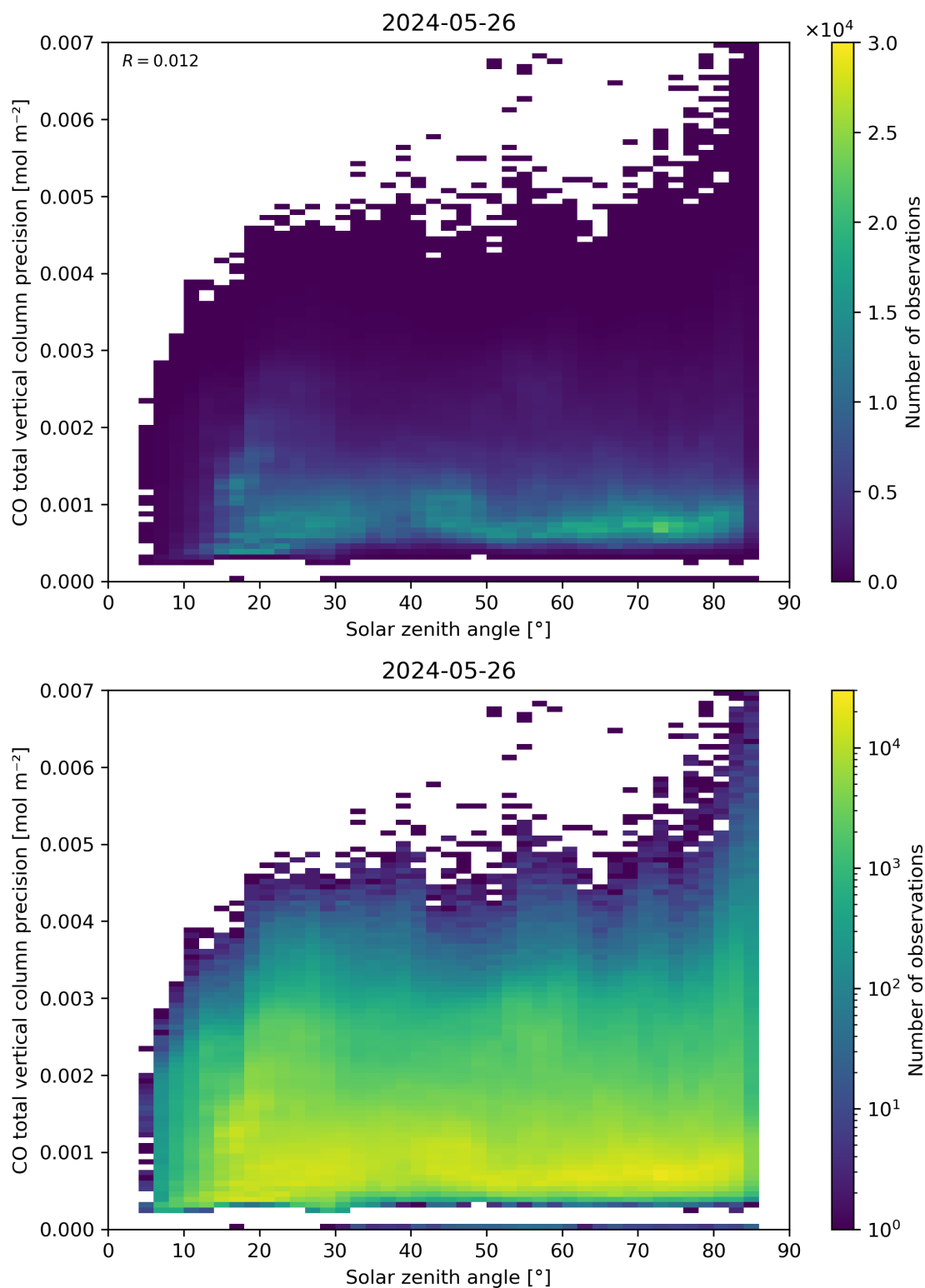
Figure 63: Scatter density plot of “Solar zenith angle” against “CO total vertical column precision” for 2024-05-25 to 2024-05-27.
