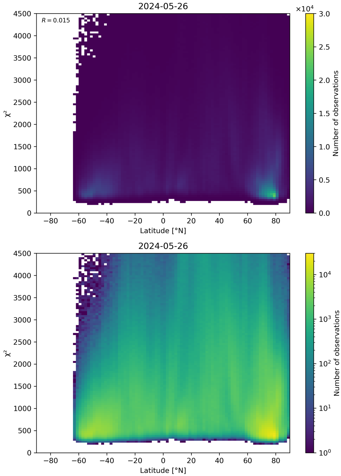
Figure 54: Scatter density plot of “Latitude” against “ \chi^2 ” for 2024-05-25 to 2024-05-27.
