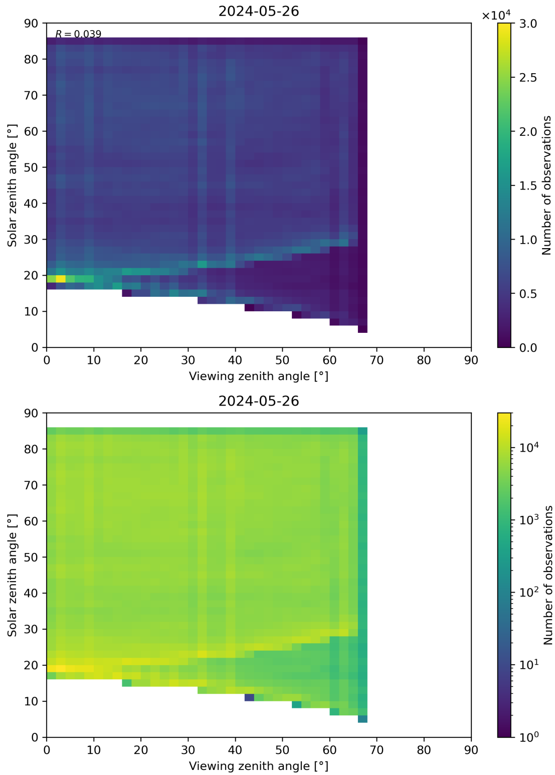
Figure 77: Scatter density plot of “Viewing zenith angle” against “Solar zenith angle” for 2024-05-25 to 2024-05-27.
