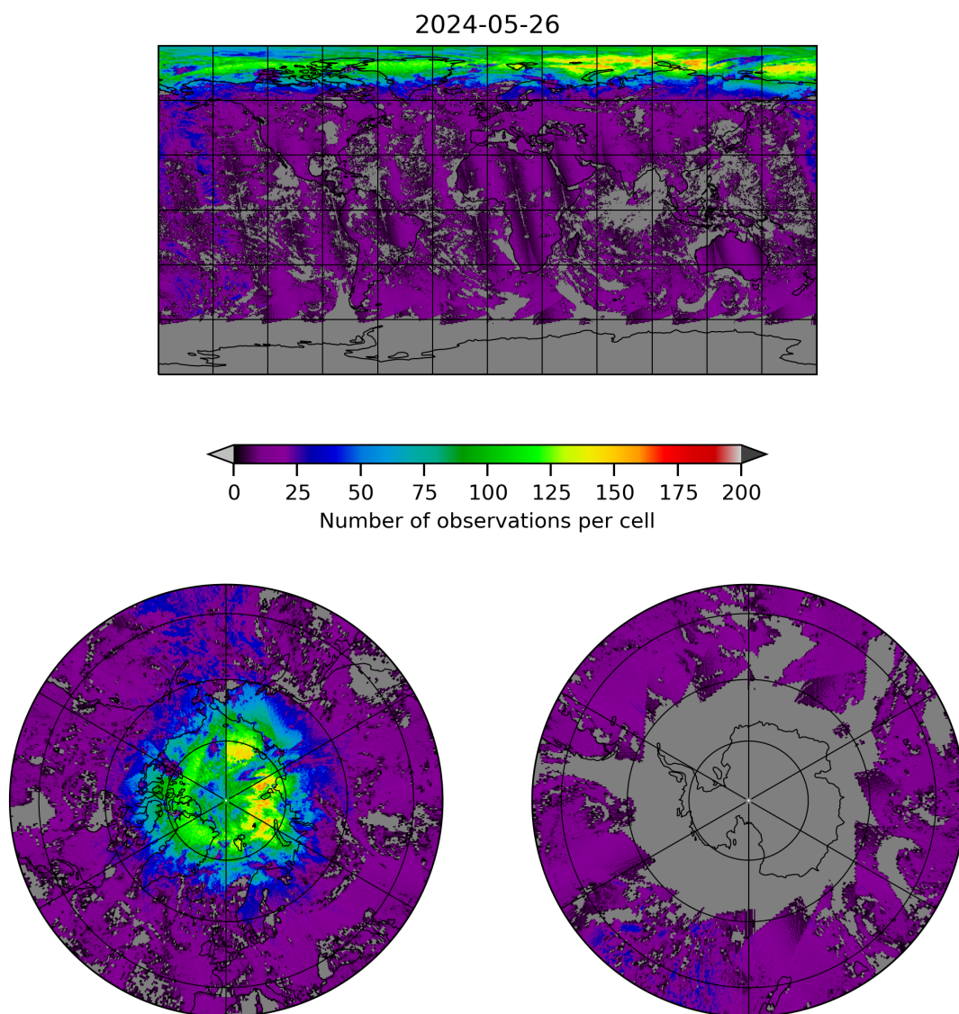
Figure 8: Map of the number of observations for 2024-05-25 to 2024-05-27
