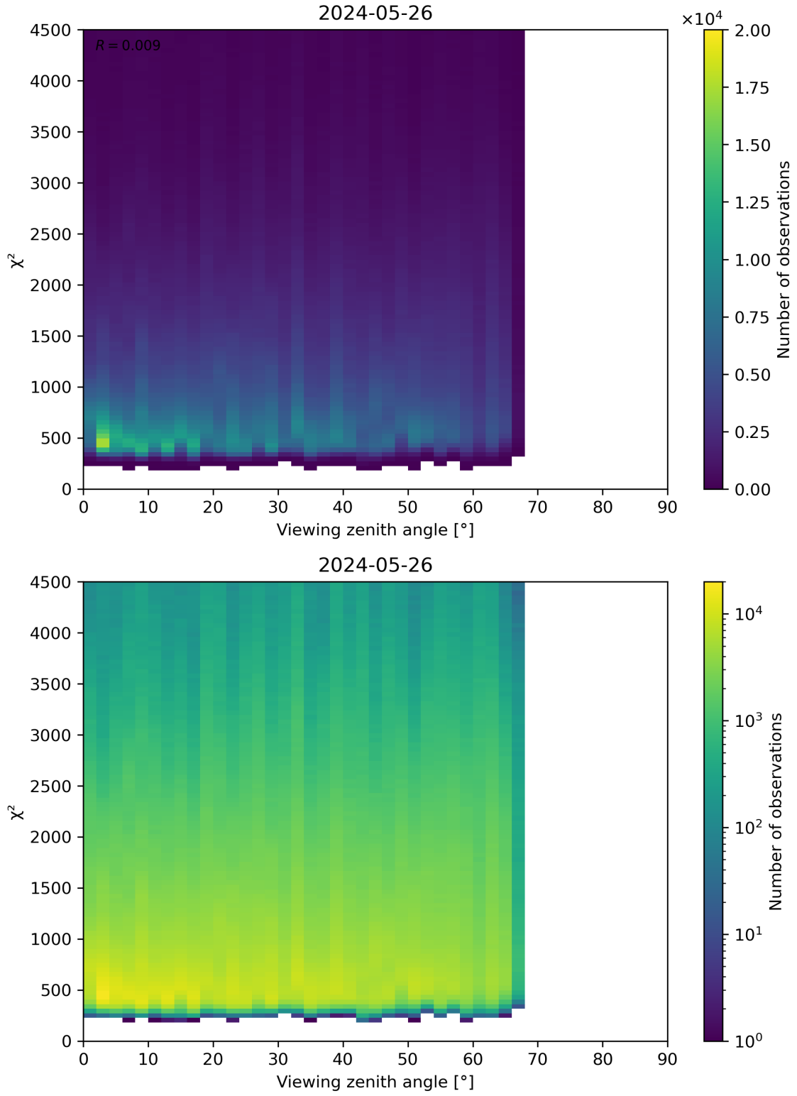
Figure 72: Scatter density plot of “Viewing zenith angle” against “ \chi^2 ” for 2024-05-25 to 2024-05-27.
