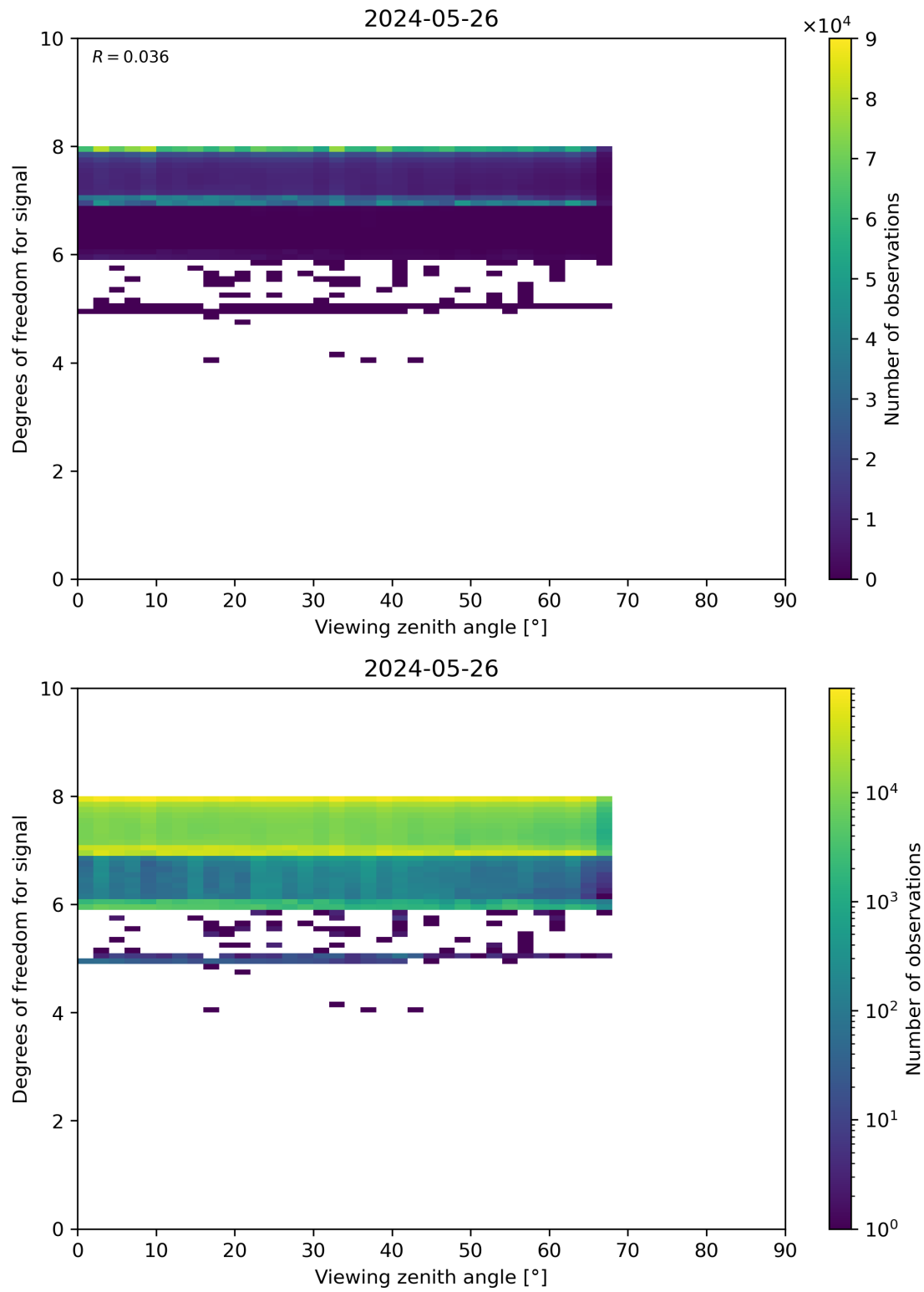
Figure 73: Scatter density plot of “Viewing zenith angle” against “Degrees of freedom for signal” for 2024-05-25 to 2024-05-27.
