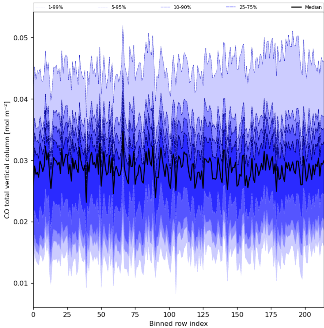
Figure 26: Along track statistics of “CO total vertical column” for 2024-05-25 to 2024-05-27
