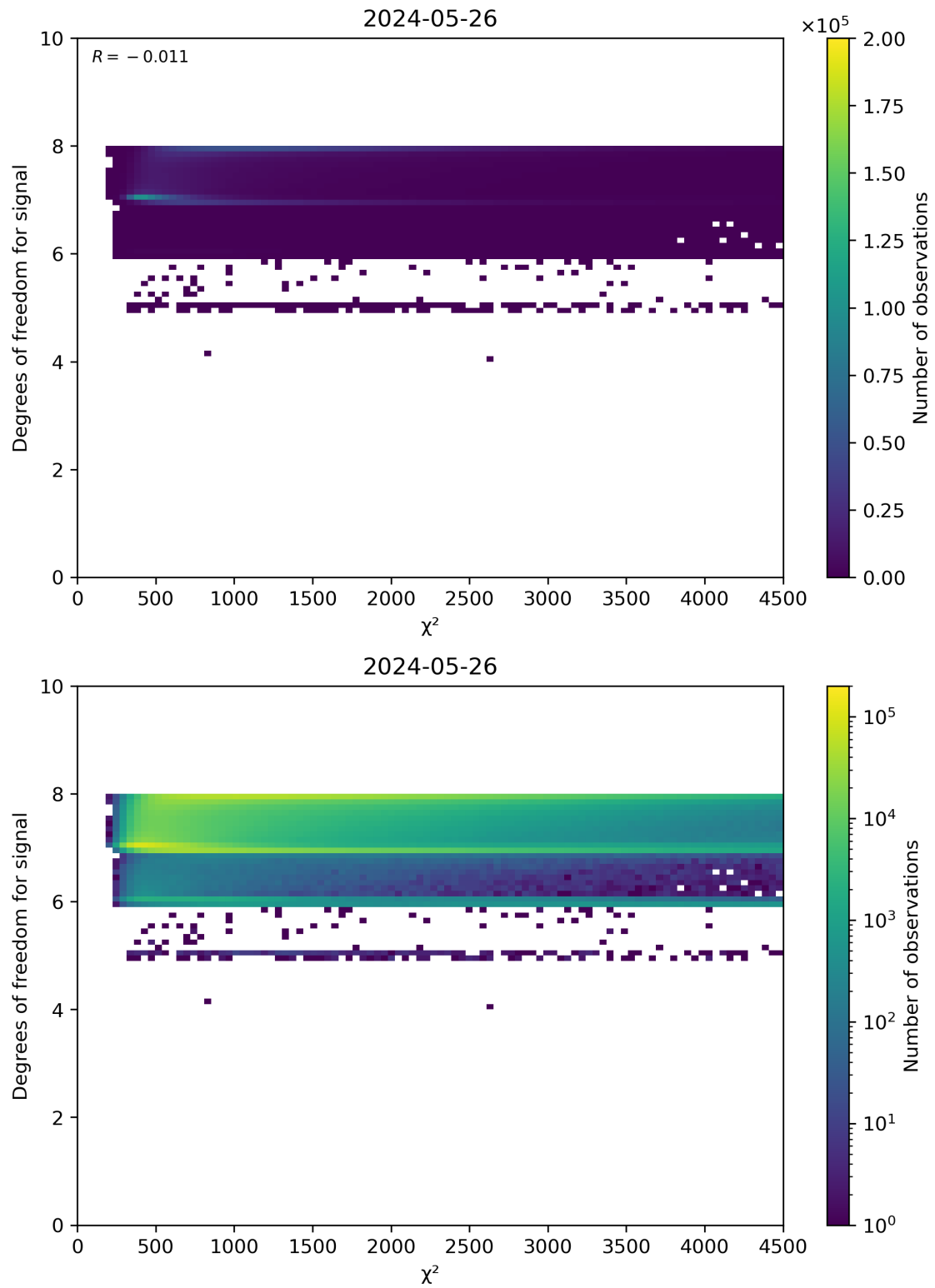
Figure 48: Scatter density plot of “ \chi^2 ” against “Degrees of freedom for signal” for 2024-05-25 to 2024-05-27.
