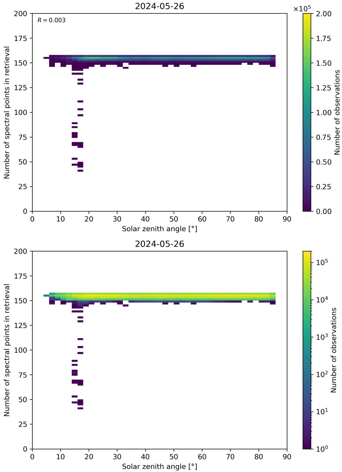
Figure 68: Scatter density plot of “Solar zenith angle” against “Number of spectral points in retrieval” for 2024-05-25 to 2024-05-27.
