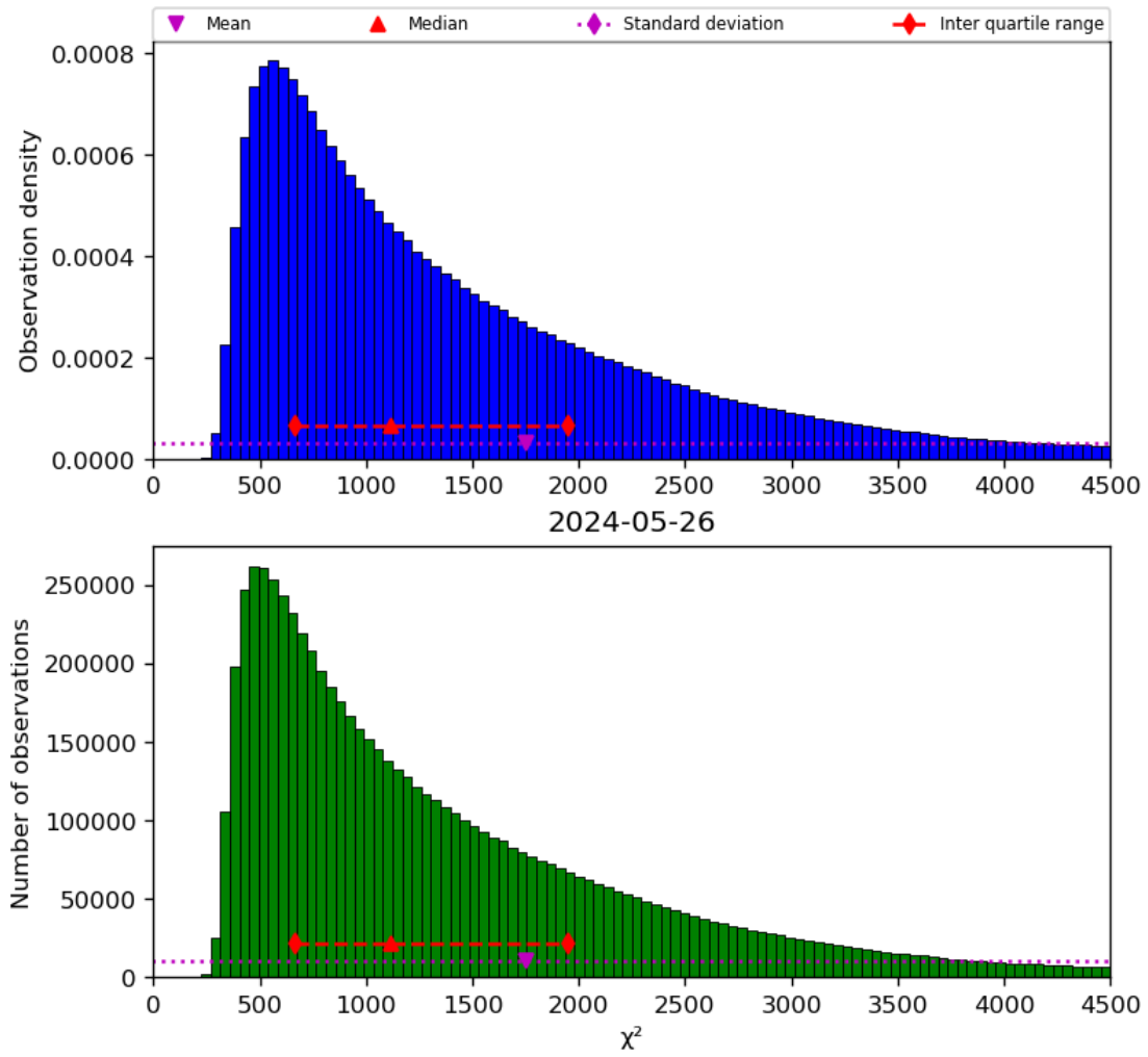
Figure 22: Histogram of “ \chi^2 ” for 2024-05-25 to 2024-05-27
