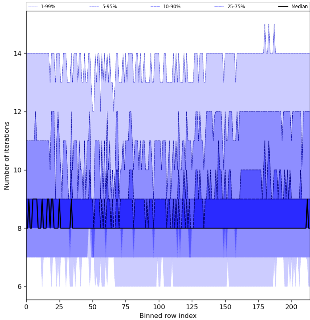
Figure 32: Along track statistics of “Number of iterations” for 2024-05-25 to 2024-05-27
