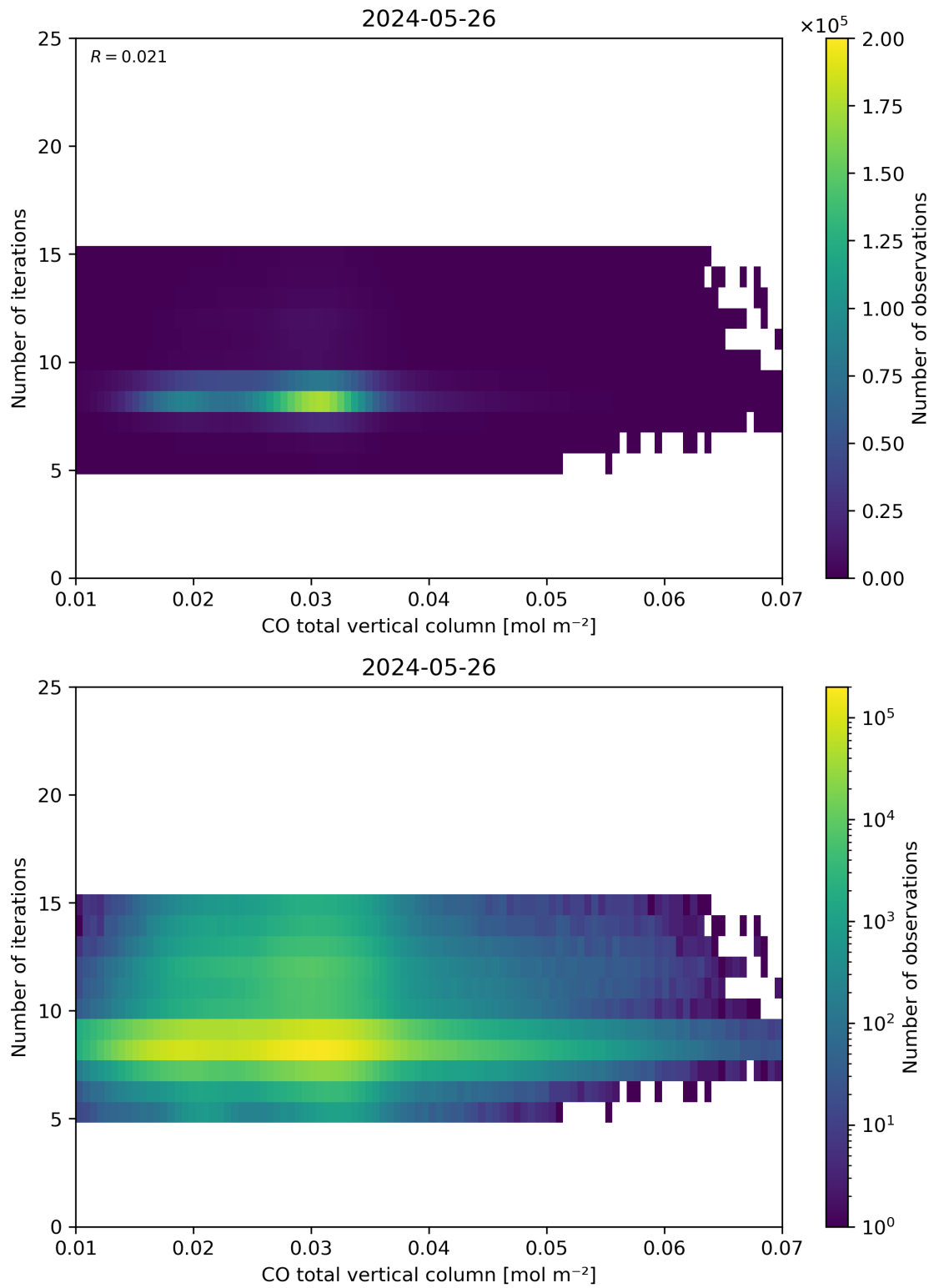
Figure 42: Scatter density plot of “CO total vertical column” against “Number of iterations” for 2024-05-25 to 2024-05-27.
