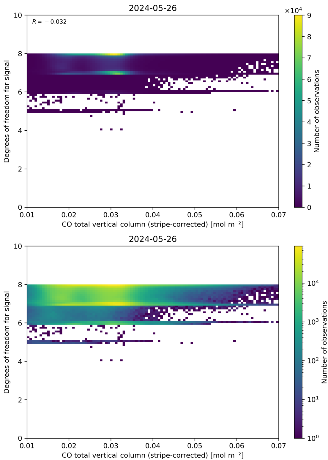
Figure 38: Scatter density plot of “CO total vertical column (stripe-corrected)” against “Degrees of freedom for signal” for 2024-05-25 to 2024-05-27.
