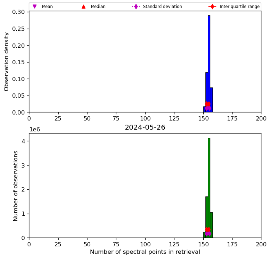
Figure 21: Histogram of “Number of spectral points in retrieval” for 2024-05-25 to 2024-05-27
