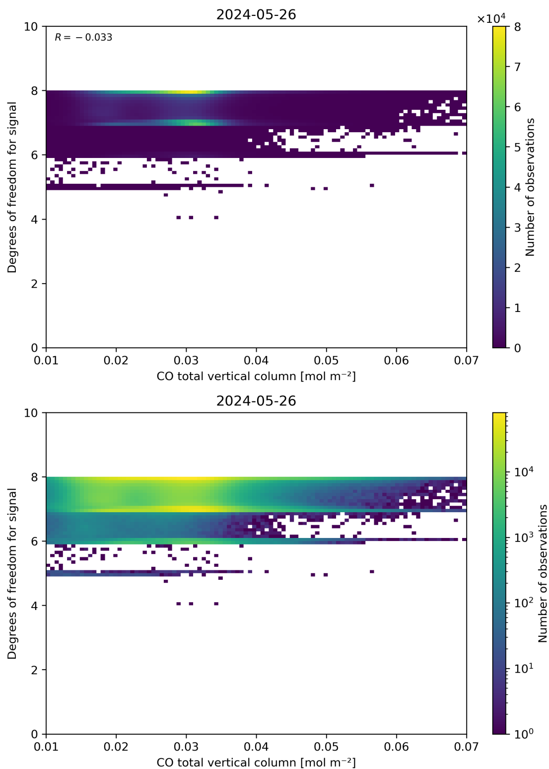
Figure 41: Scatter density plot of “CO total vertical column” against “Degrees of freedom for signal” for 2024-05-25 to 2024-05-27.
