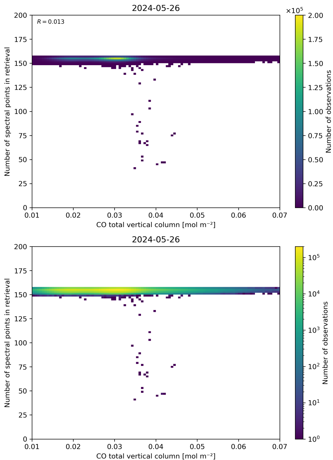
Figure 43: Scatter density plot of “CO total vertical column” against “Number of spectral points in retrieval” for 2024-05-25 to 2024-05-27.
