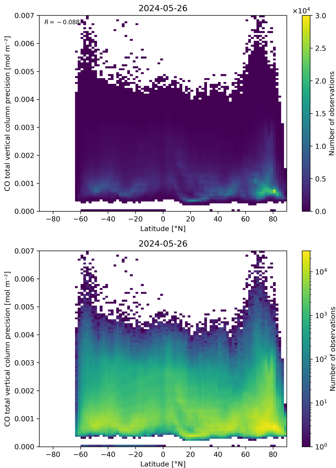
Figure 53: Scatter density plot of “Latitude” against “CO total vertical column precision” for 2024-05-25 to 2024-05-27.
