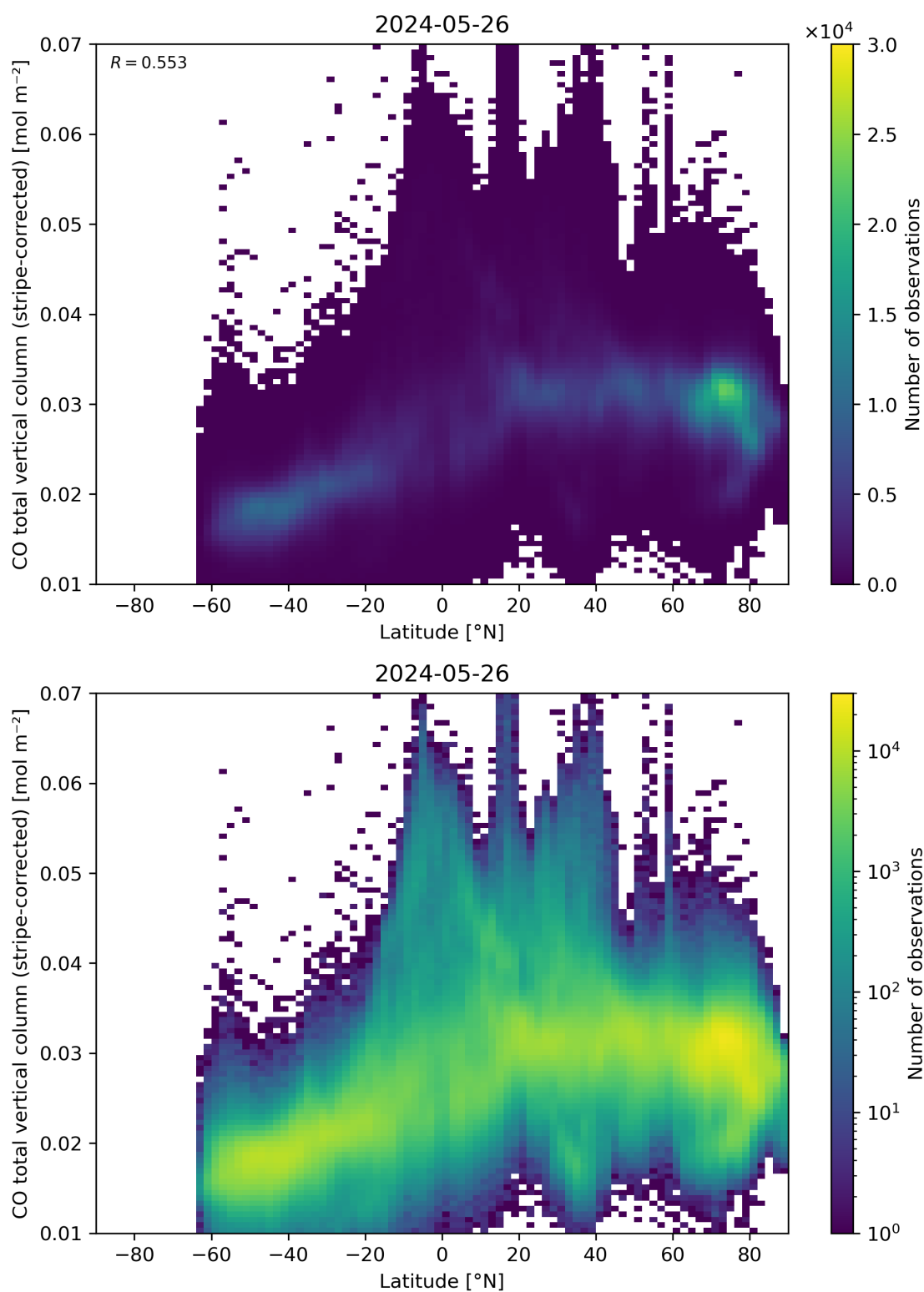
Figure 52: Scatter density plot of “Latitude” against “CO total vertical column (stripe-corrected)” for 2024-05-25 to 2024-05-27.
