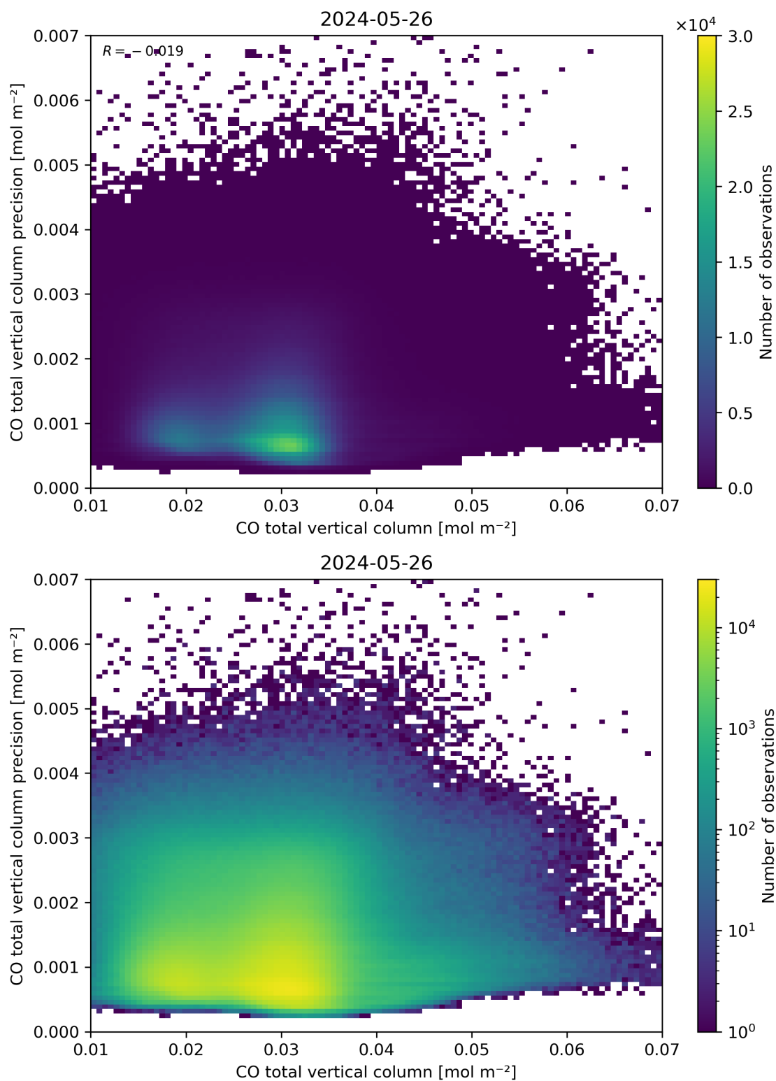
Figure 34: Scatter density plot of “CO total vertical column” against “CO total vertical column precision” for 2024-05-25 to 2024-05-27.
