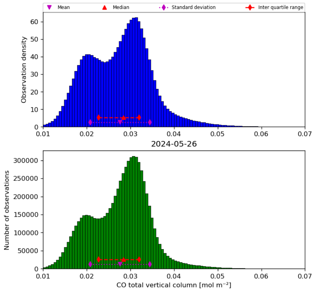
Figure 18: Histogram of “CO total vertical column” for 2024-05-25 to 2024-05-27
