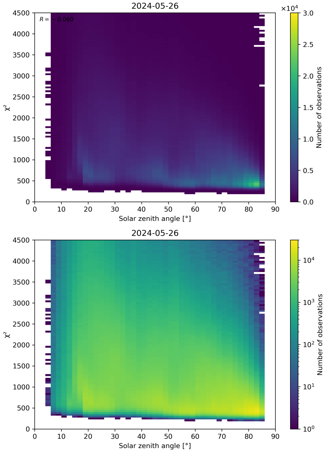
Figure 64: Scatter density plot of “Solar zenith angle” against “ \chi^2 ” for 2024-05-25 to 2024-05-27.
