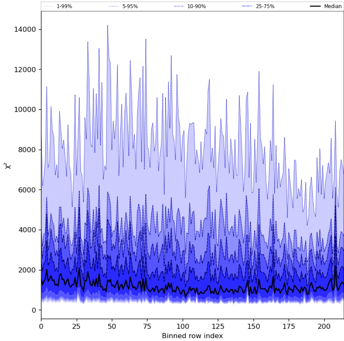
Figure 30: Along track statistics of “ \chi^2 ” for 2024-05-25 to 2024-05-27
