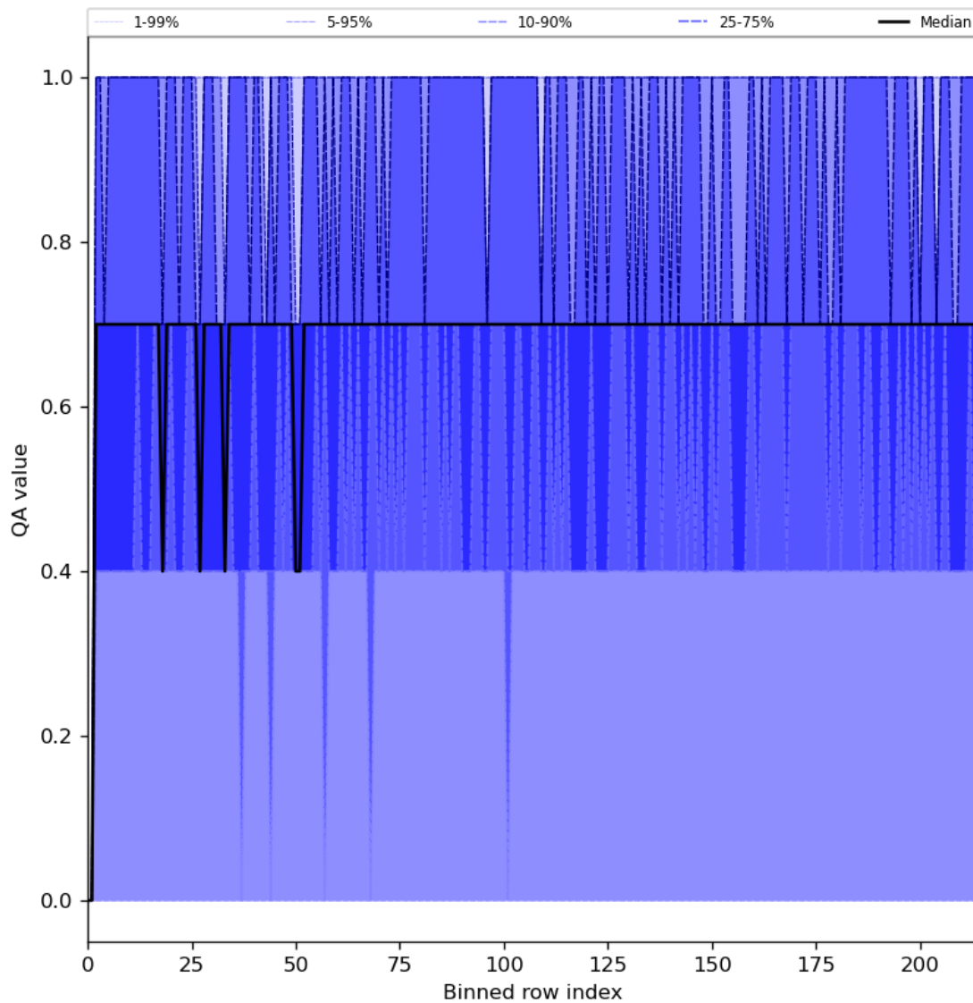
Figure 25: Along track statistics of "QA value" for 2024-05-25 to 2024-05-27
