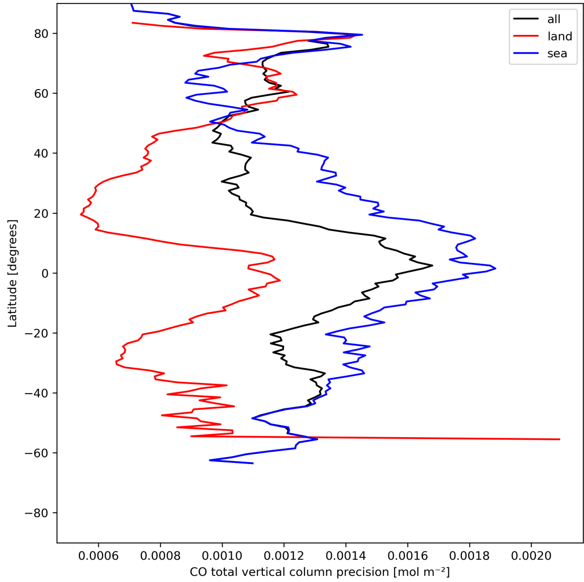
Figure 12: Zonal average of “CO total vertical column precision” for 2024-05-25 to 2024-05-27.
