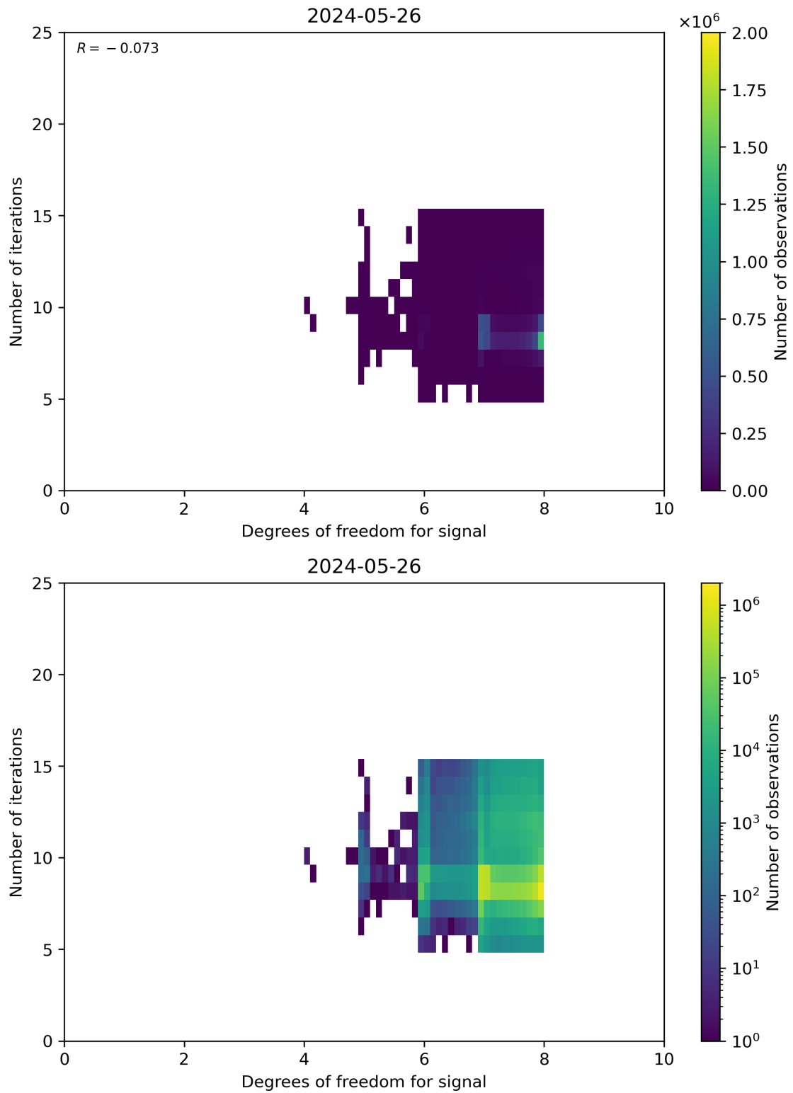
Figure 50: Scatter density plot of “Degrees of freedom for signal” against “Number of iterations” for 2024-05-25 to 2024-05-27.
