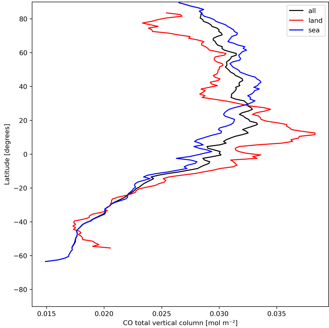
Figure 10: Zonal average of “CO total vertical column” for 2024-05-25 to 2024-05-27.
