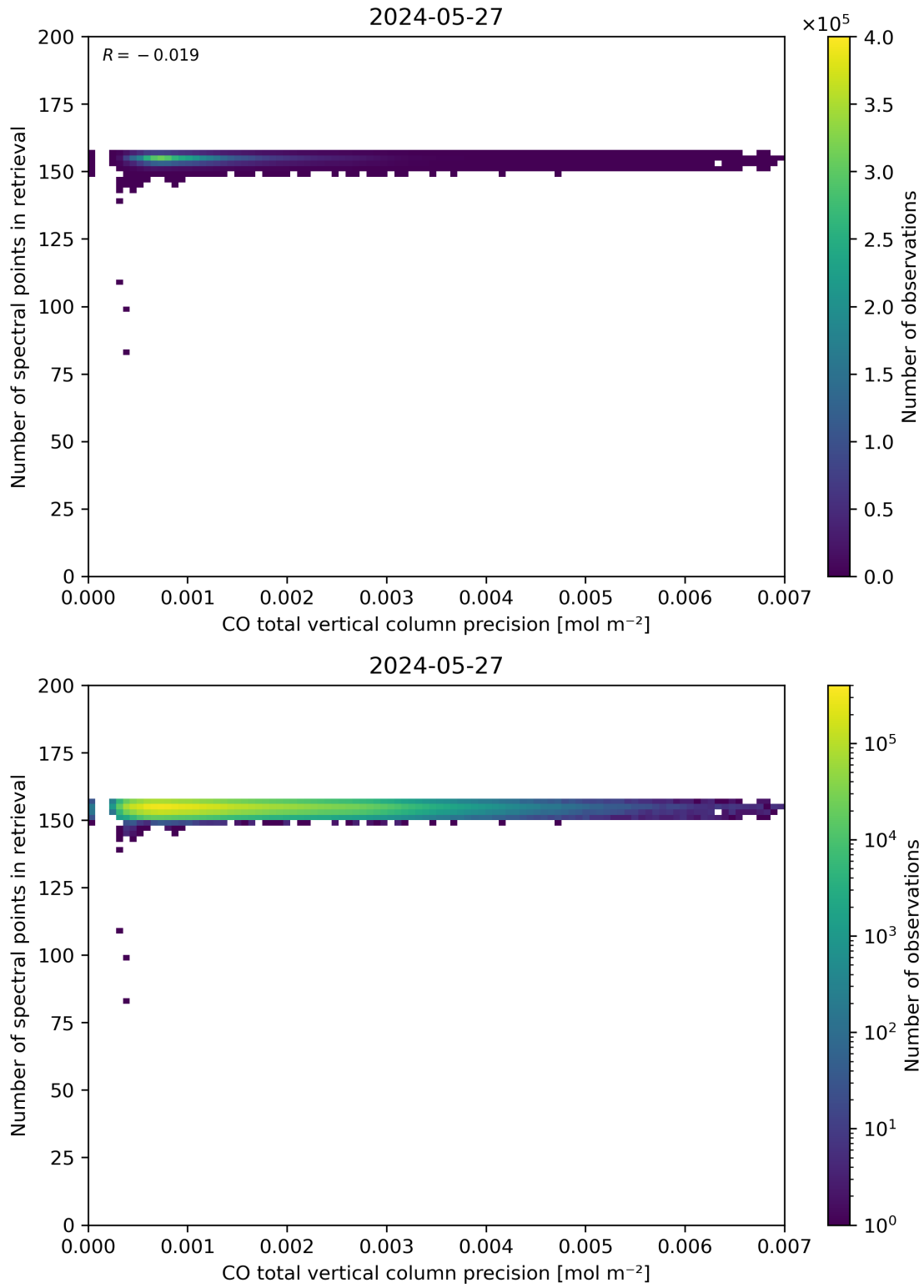
Figure 47: Scatter density plot of “CO total vertical column precision” against “Number of spectral points in retrieval” for 2024-05-26 to 2024-05-28.
