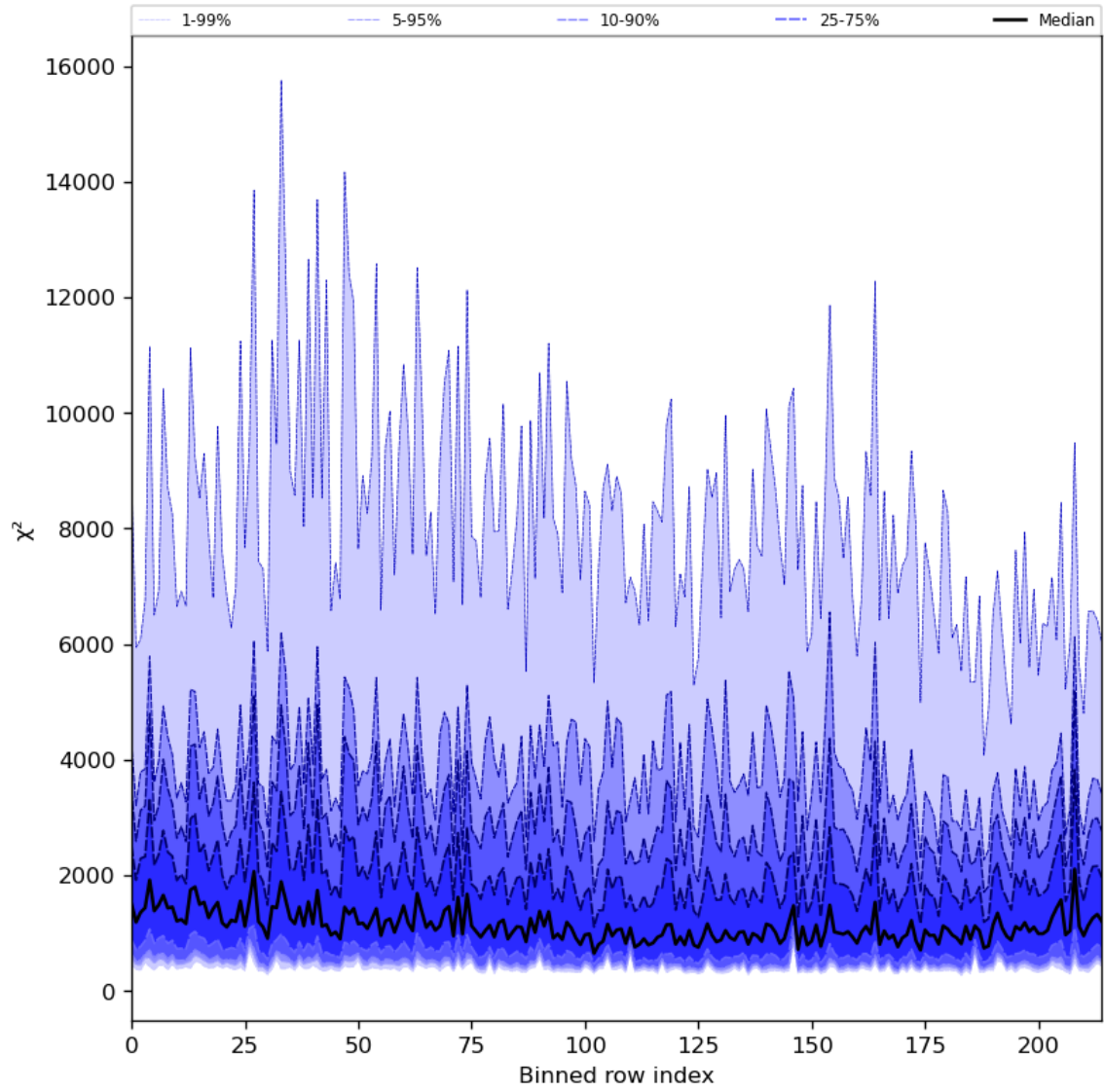
Figure 30: Along track statistics of “ \chi^2 ” for 2024-05-26 to 2024-05-28
