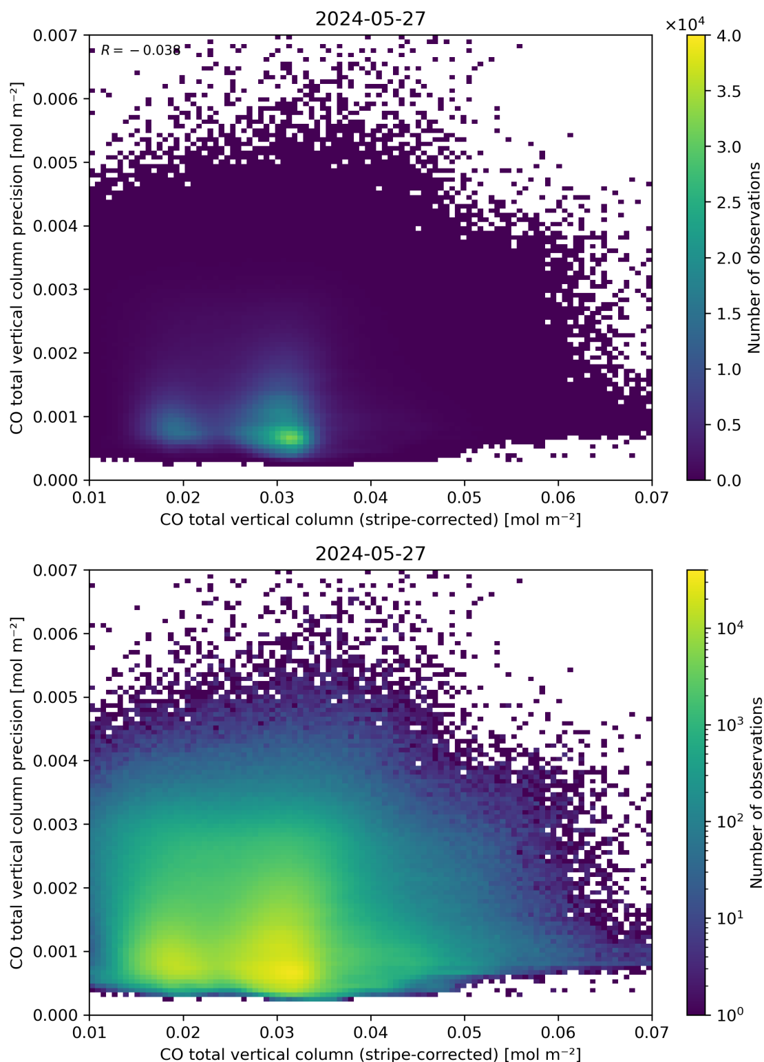
Figure 36: Scatter density plot of “CO total vertical column (stripe-corrected)” against “CO total vertical column precision” for 2024-05-26 to 2024-05-28.
