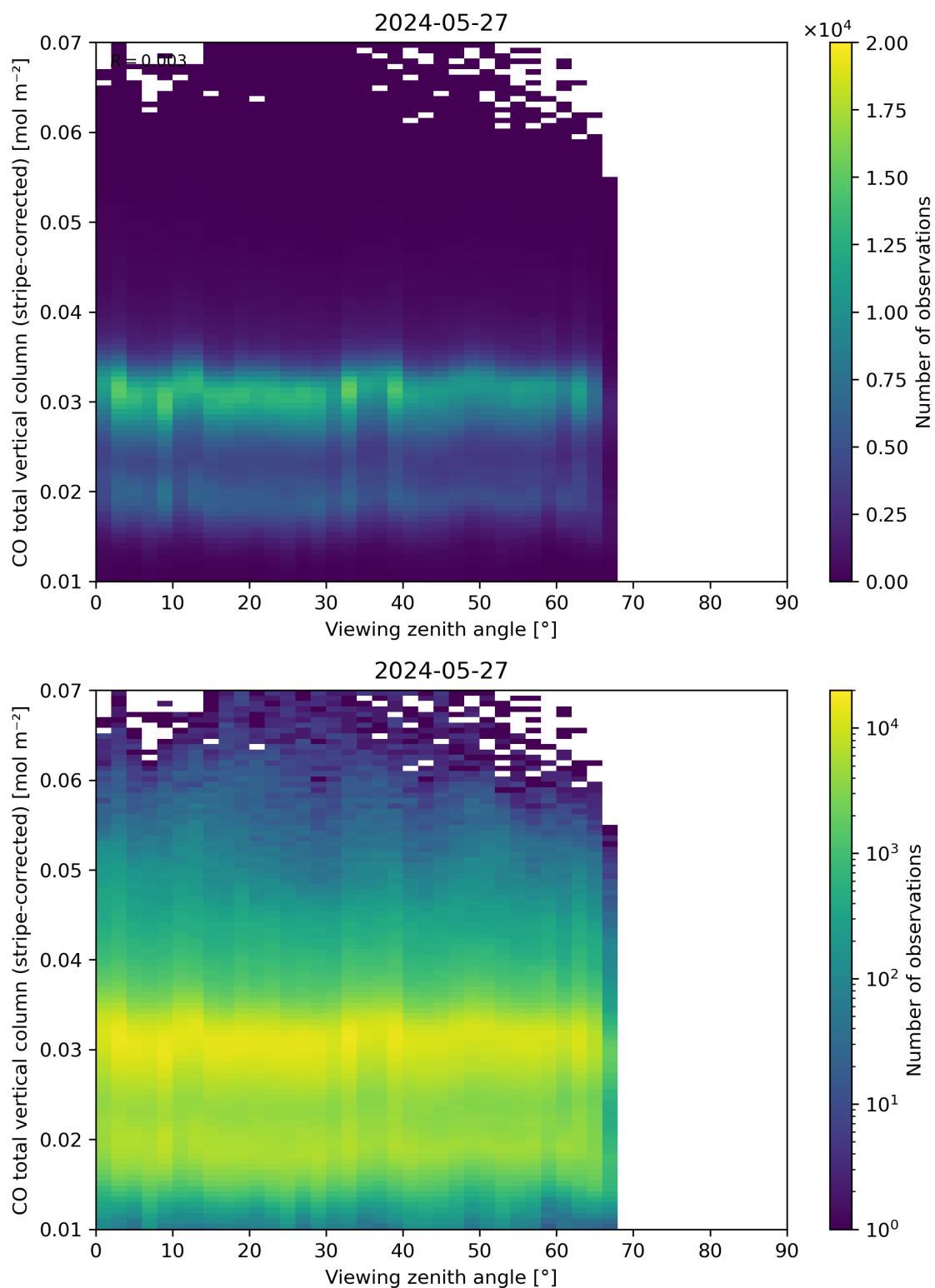
Figure 70: Scatter density plot of “Viewing zenith angle” against “CO total vertical column (stripe-corrected)” for 2024-05-26 to 2024-05-28.
