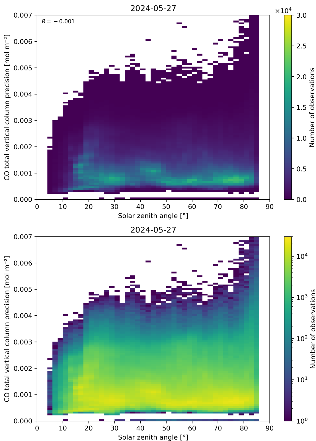
Figure 63: Scatter density plot of “Solar zenith angle” against “CO total vertical column precision” for 2024-05-26 to 2024-05-28.
