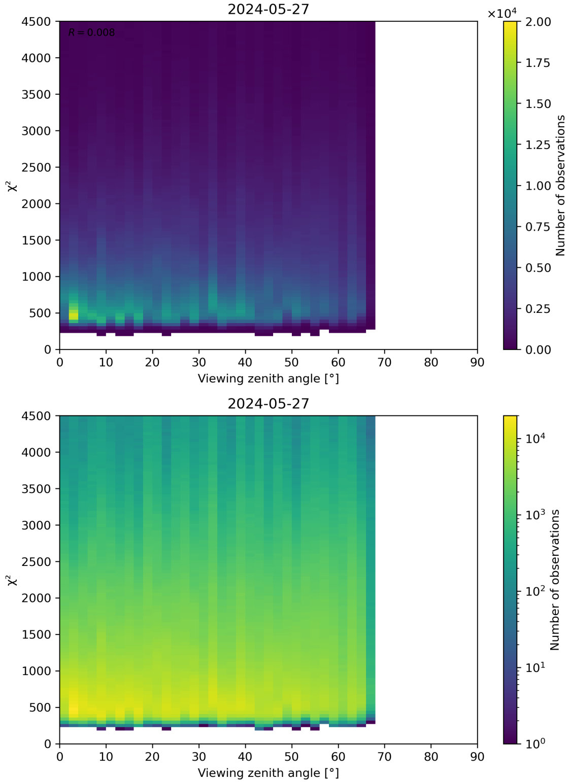
Figure 72: Scatter density plot of “Viewing zenith angle” against “ \chi^2 ” for 2024-05-26 to 2024-05-28.
