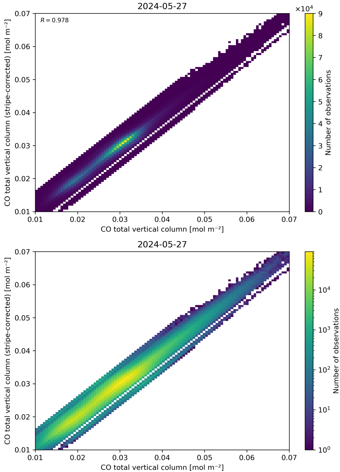
Figure 33: Scatter density plot of “CO total vertical column” against “CO total vertical column (stripe-corrected)” for 2024-05-26 to 2024-05-28.
