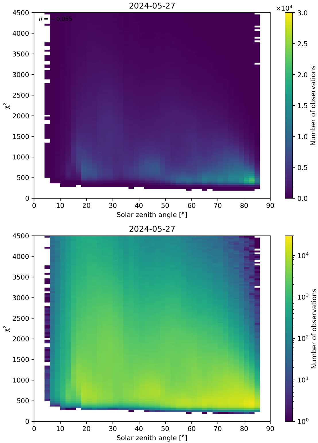
Figure 64: Scatter density plot of “Solar zenith angle” against “ \chi^2 ” for 2024-05-26 to 2024-05-28.
