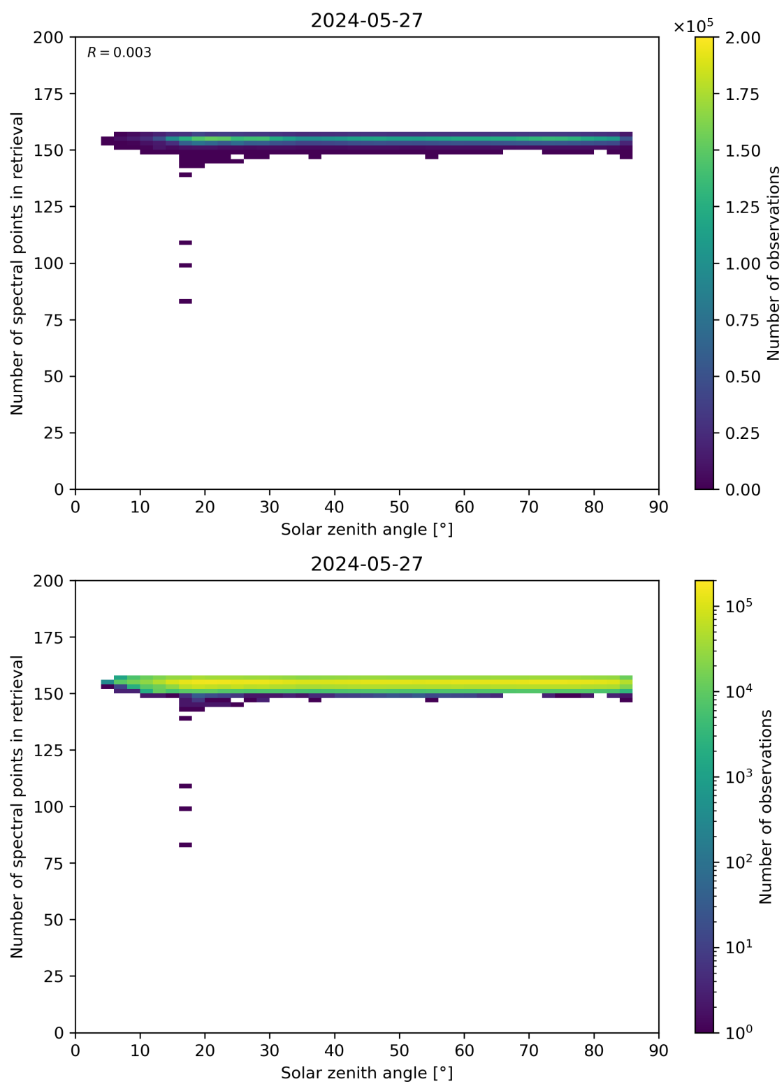
Figure 68: Scatter density plot of “Solar zenith angle” against “Number of spectral points in retrieval” for 2024-05-26 to 2024-05-28.
