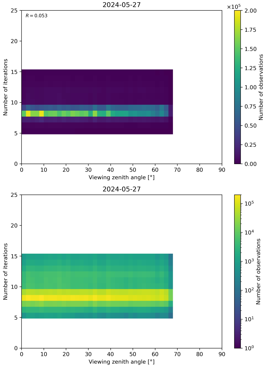
Figure 75: Scatter density plot of “Viewing zenith angle” against “Number of iterations” for 2024-05-26 to 2024-05-28.
