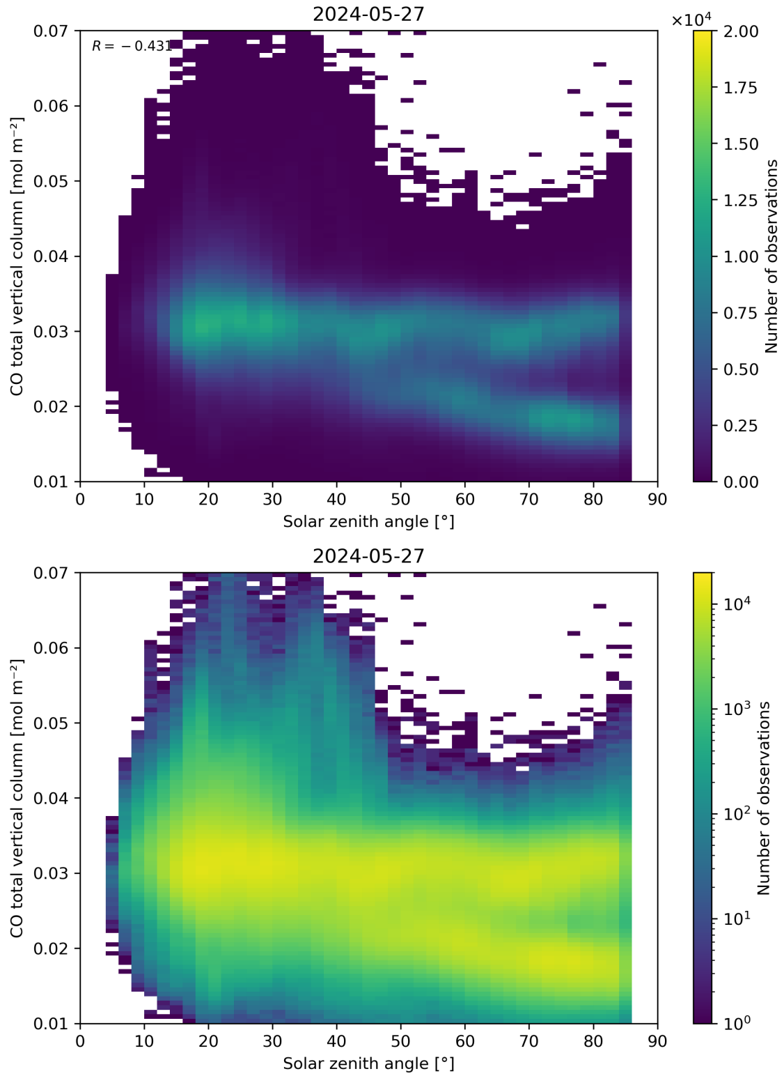
Figure 61: Scatter density plot of “Solar zenith angle” against “CO total vertical column” for 2024-05-26 to 2024-05-28.
