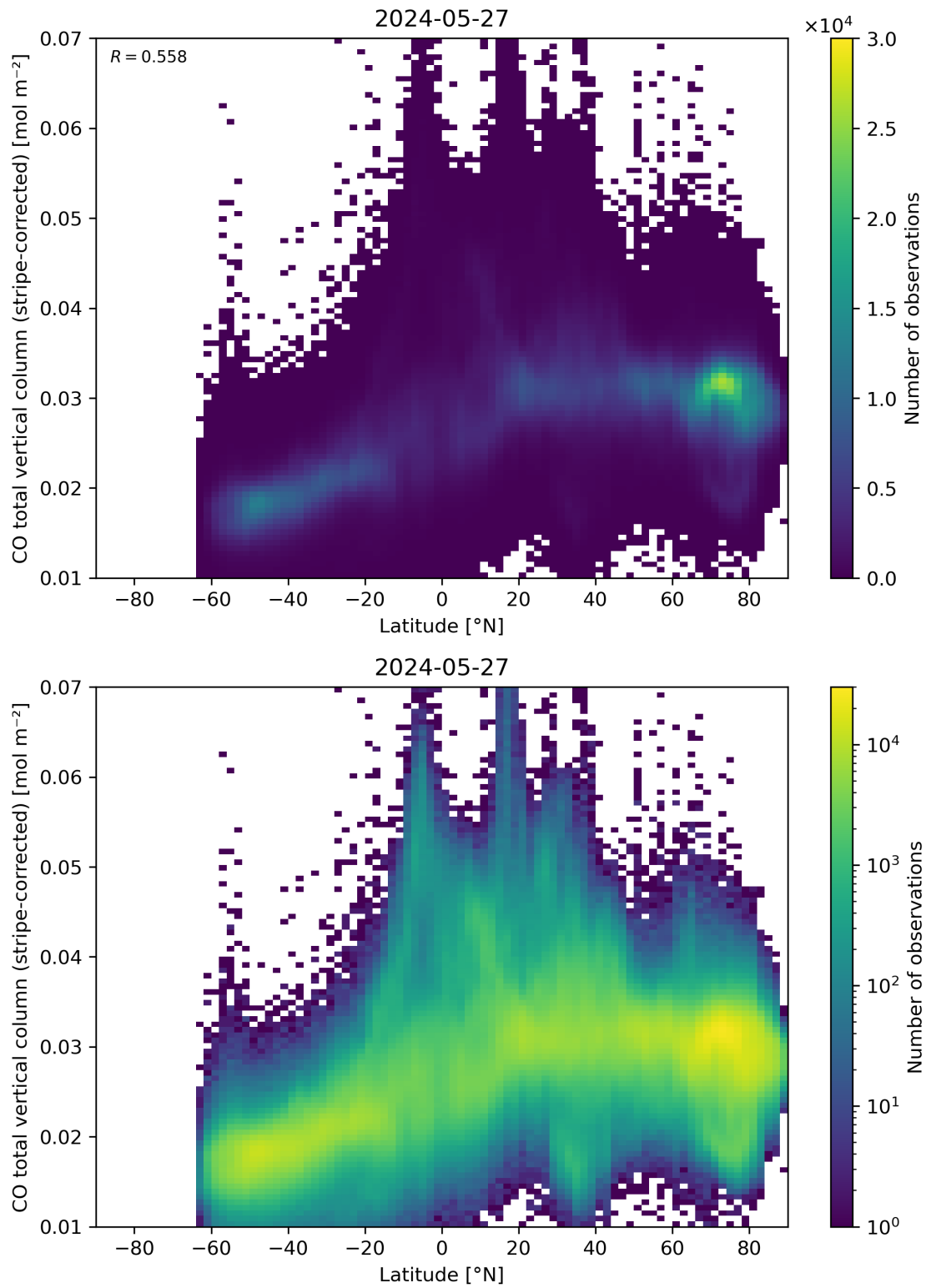
Figure 52: Scatter density plot of “Latitude” against “CO total vertical column (stripe-corrected)” for 2024-05-26 to 2024-05-28.
