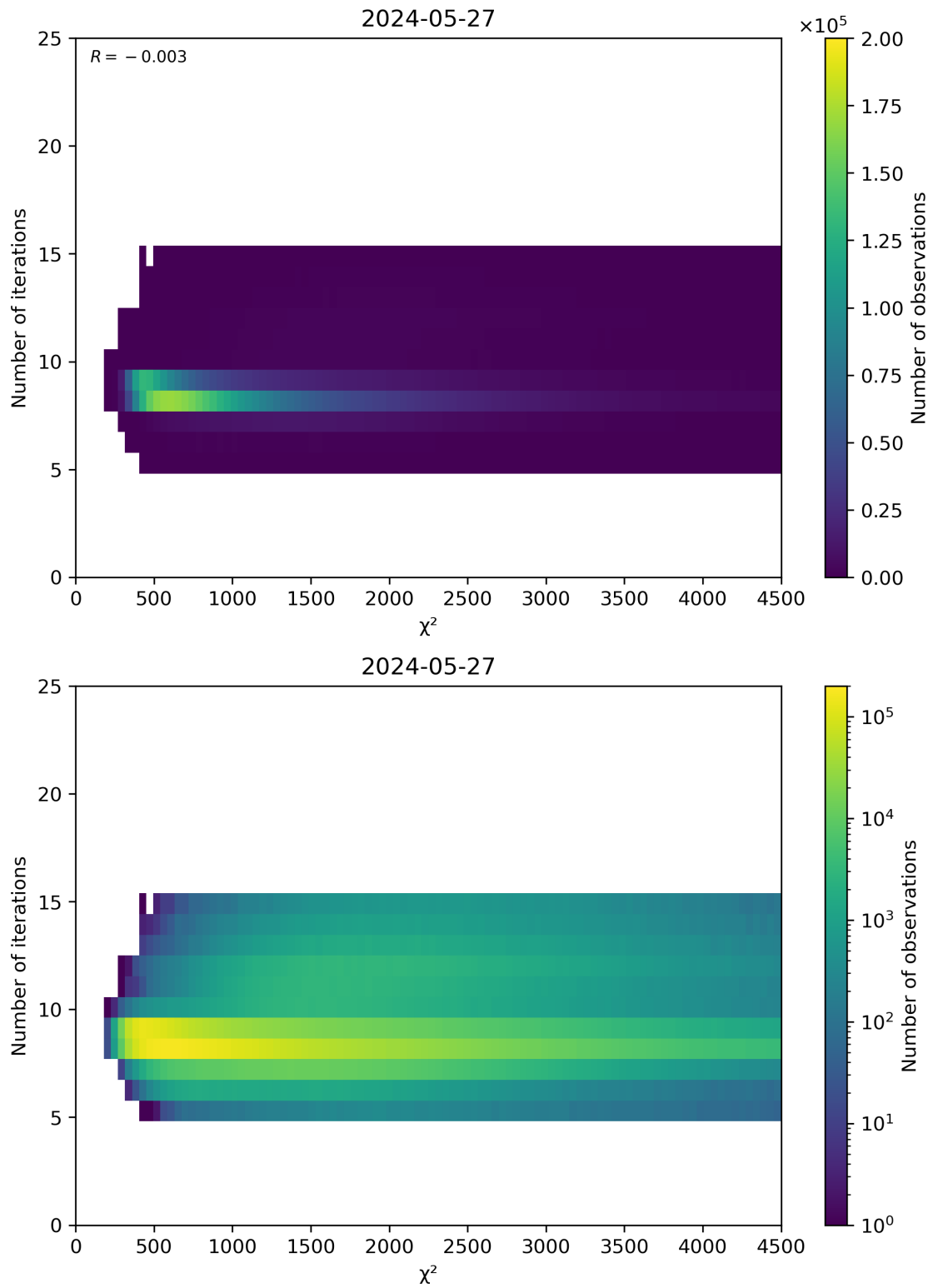
Figure 49: Scatter density plot of “ \chi^2 ” against “Number of iterations” for 2024-05-26 to 2024-05-28.
