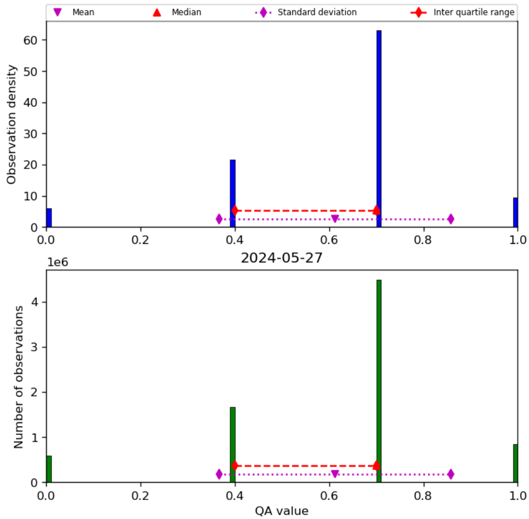
Figure 17: Histogram of “QA value” for 2024-05-26 to 2024-05-28
