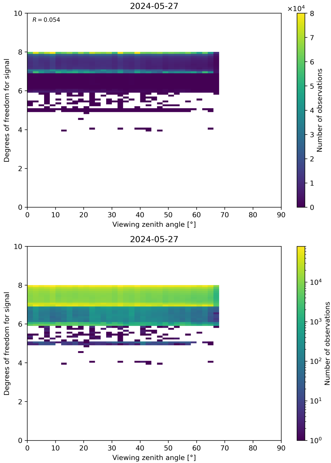
Figure 73: Scatter density plot of “Viewing zenith angle” against “Degrees of freedom for signal” for 2024-05-26 to 2024-05-28.
