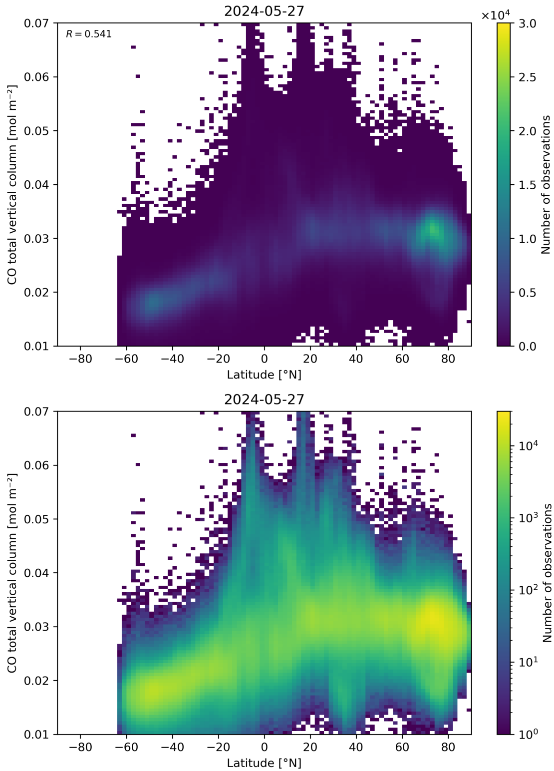
Figure 51: Scatter density plot of “Latitude” against “CO total vertical column” for 2024-05-26 to 2024-05-28.
