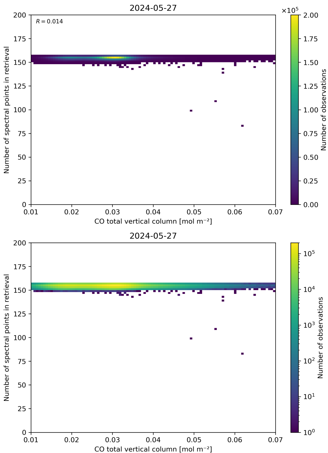
Figure 43: Scatter density plot of “CO total vertical column” against “Number of spectral points in retrieval” for 2024-05-26 to 2024-05-28.
