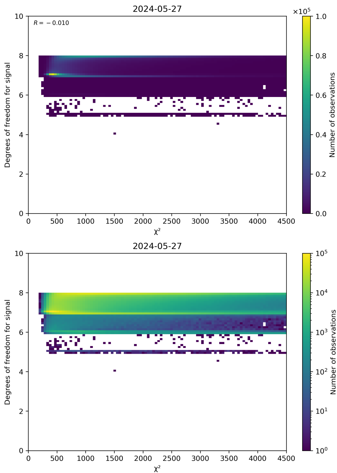
Figure 48: Scatter density plot of “ \chi^2 ” against “Degrees of freedom for signal” for 2024-05-26 to 2024-05-28.
