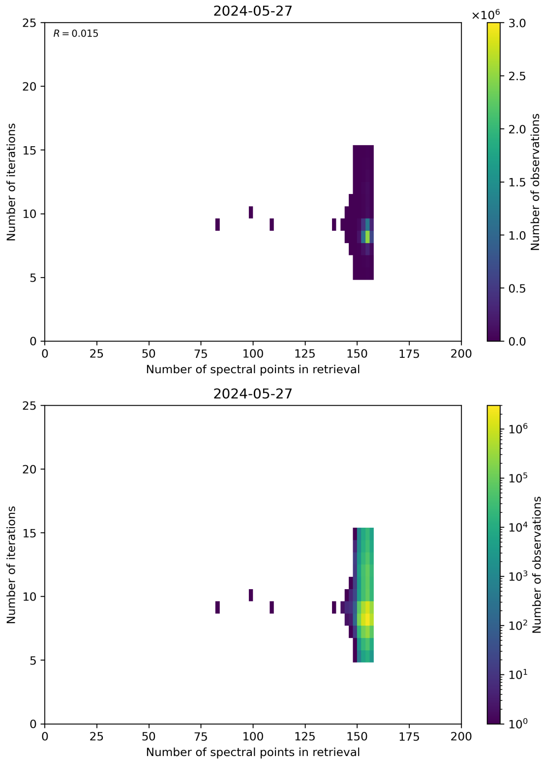
Figure 60: Scatter density plot of “Number of spectral points in retrieval” against “Number of iterations” for 2024-05-26 to 2024-05-28.
