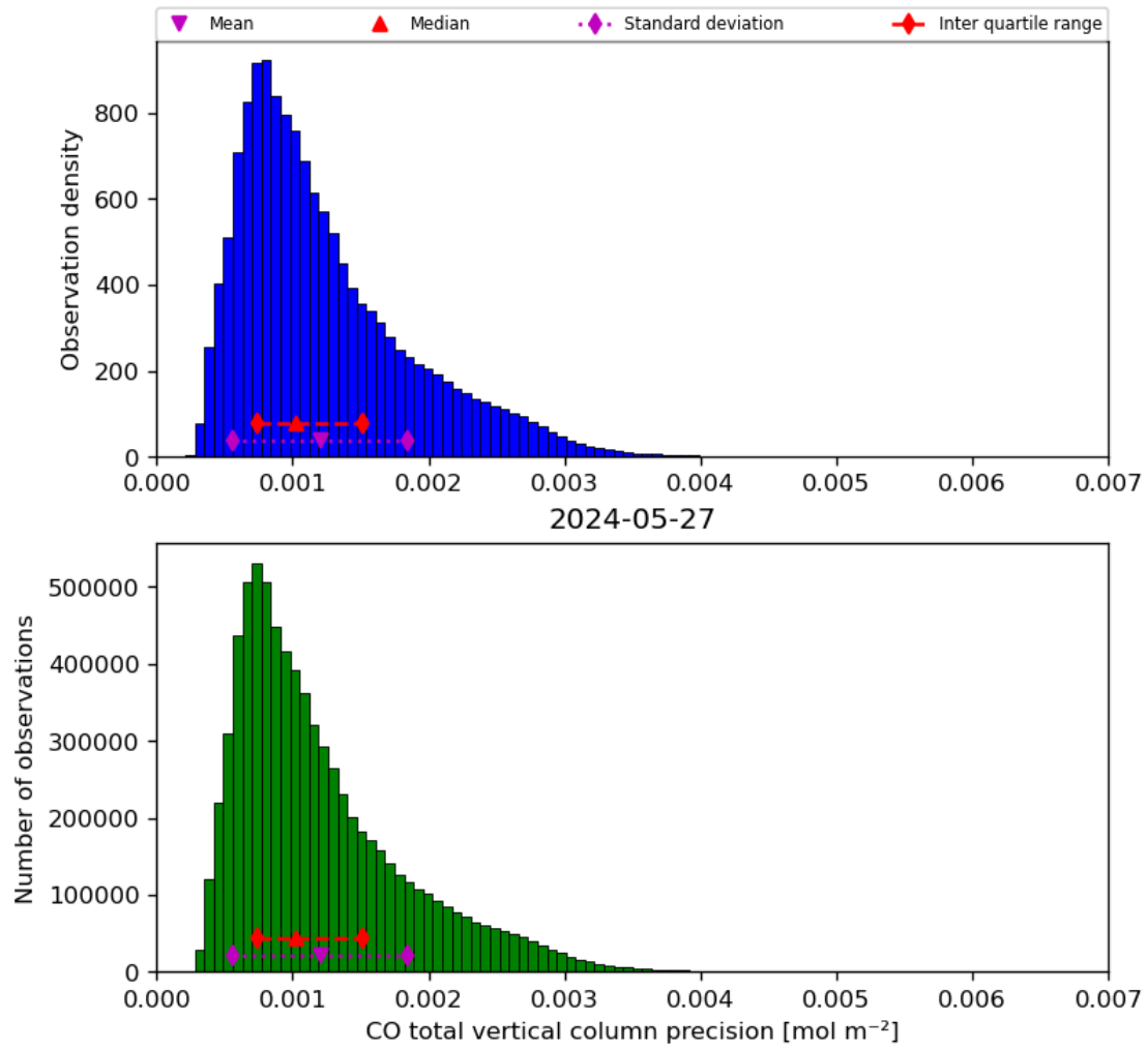
Figure 20: Histogram of “CO total vertical column precision” for 2024-05-26 to 2024-05-28
