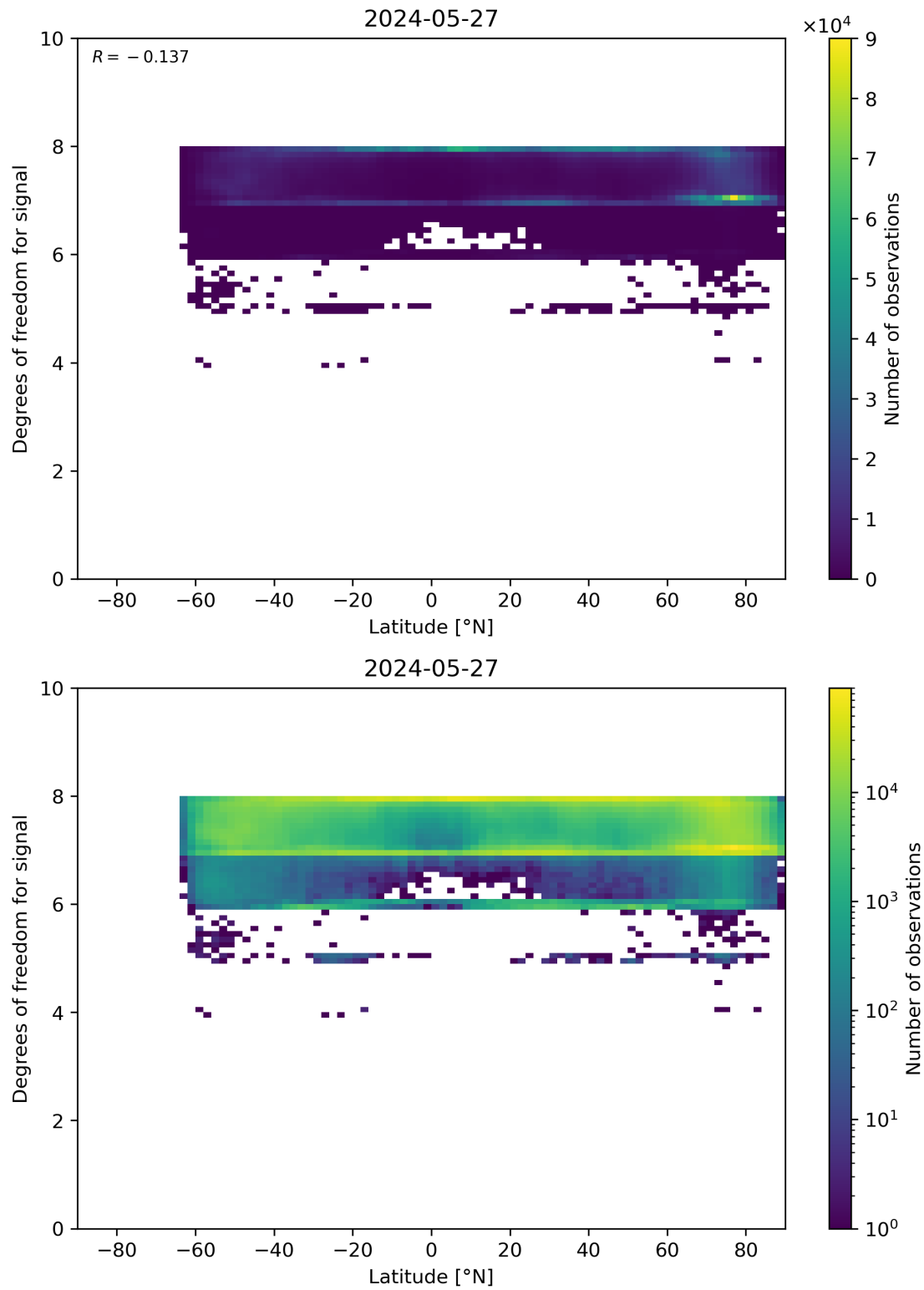
Figure 55: Scatter density plot of “Latitude” against “Degrees of freedom for signal” for 2024-05-26 to 2024-05-28.
