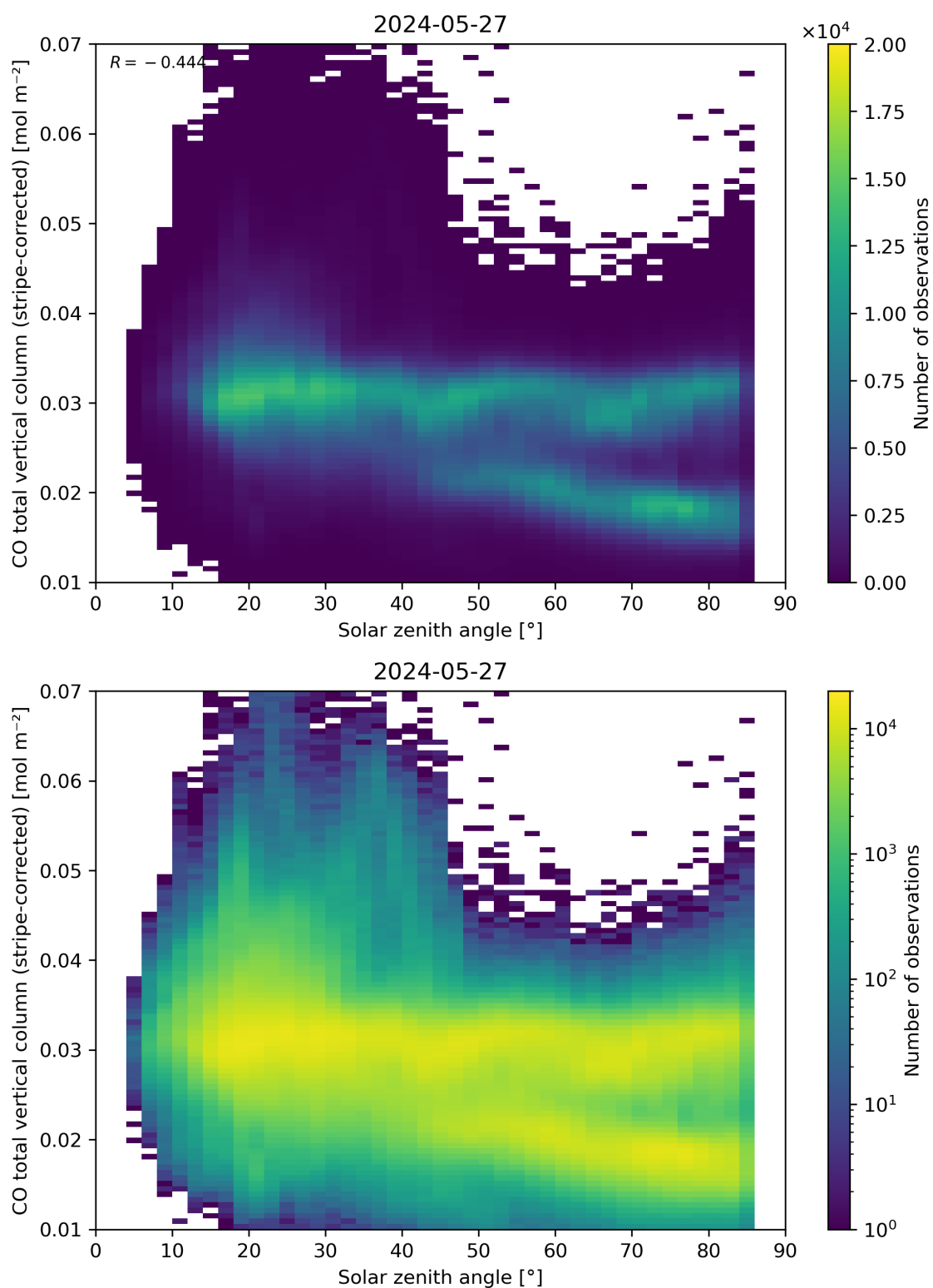
Figure 62: Scatter density plot of “Solar zenith angle” against “CO total vertical column (stripe-corrected)” for 2024-05-26 to 2024-05-28.
