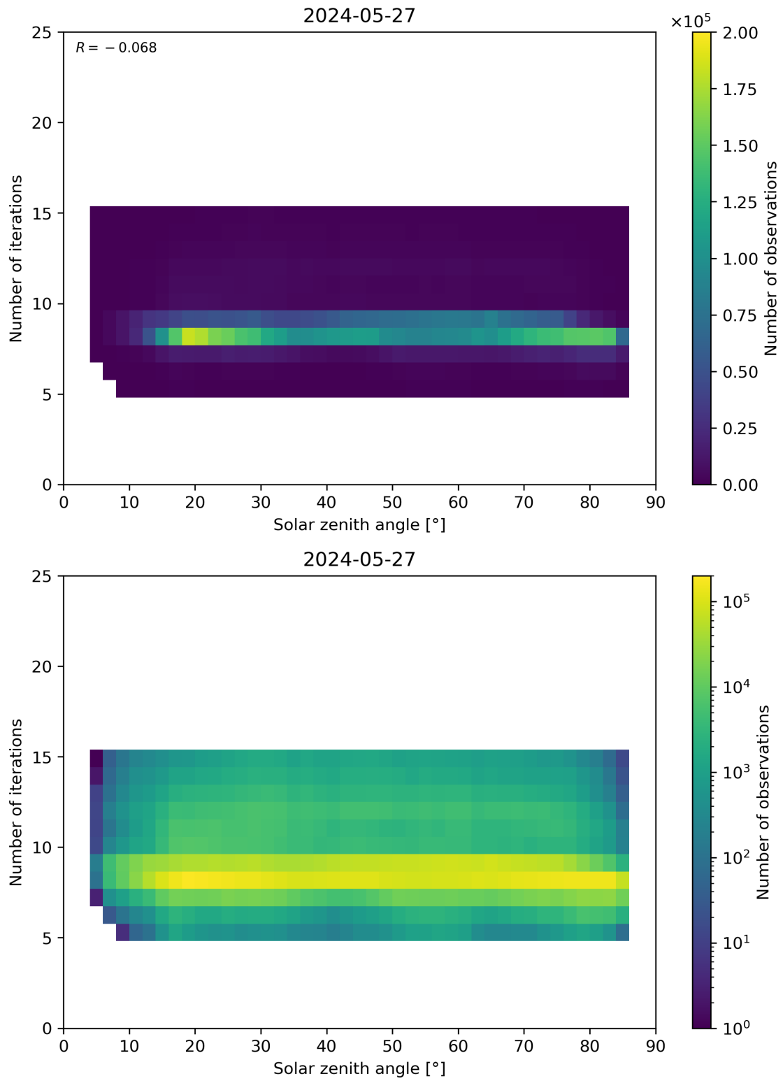
Figure 67: Scatter density plot of “Solar zenith angle” against “Number of iterations” for 2024-05-26 to 2024-05-28.
