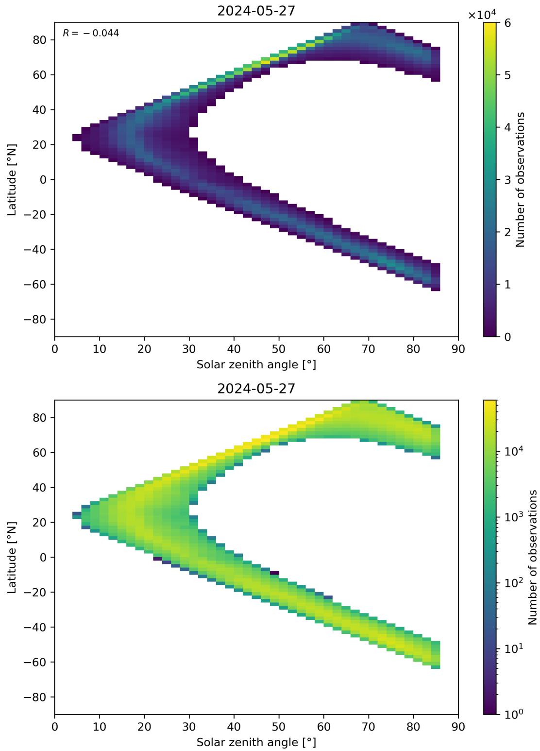
Figure 66: Scatter density plot of “Solar zenith angle” against “Latitude” for 2024-05-26 to 2024-05-28.
