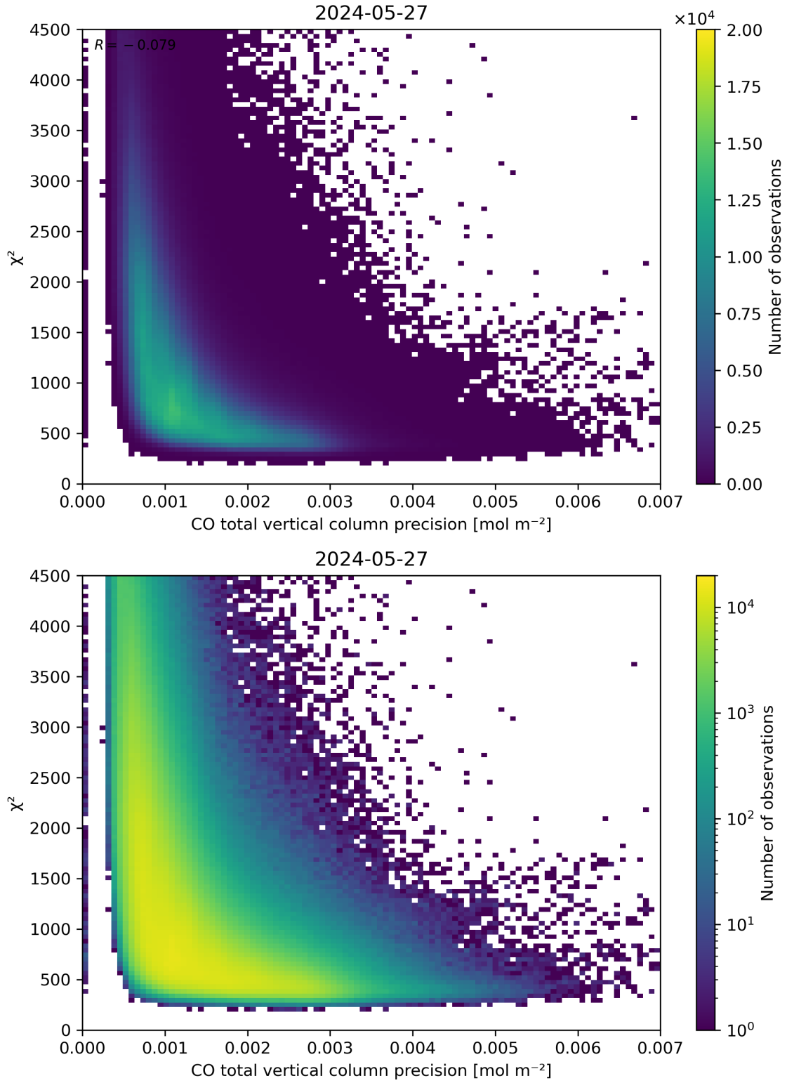
Figure 44: Scatter density plot of “CO total vertical column precision” against “ \chi^2 ” for 2024-05-26 to 2024-05-28.
