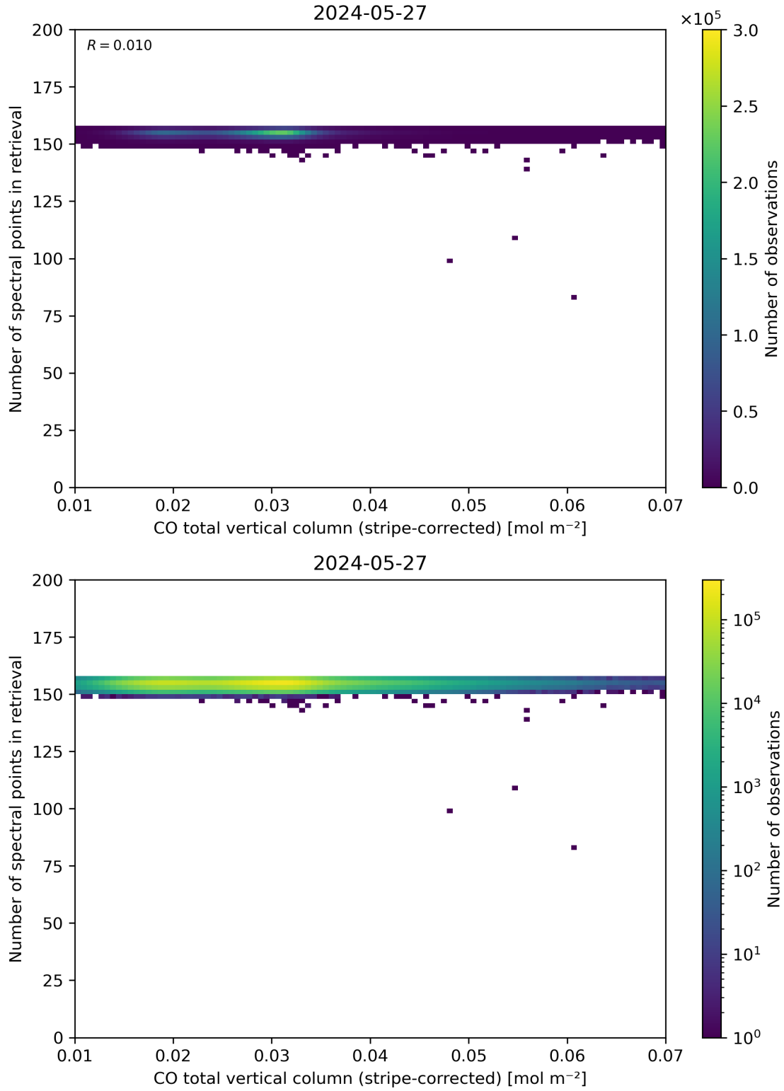
Figure 40: Scatter density plot of “CO total vertical column (stripe-corrected)” against “Number of spectral points in retrieval” for 2024-05-26 to 2024-05-28.
