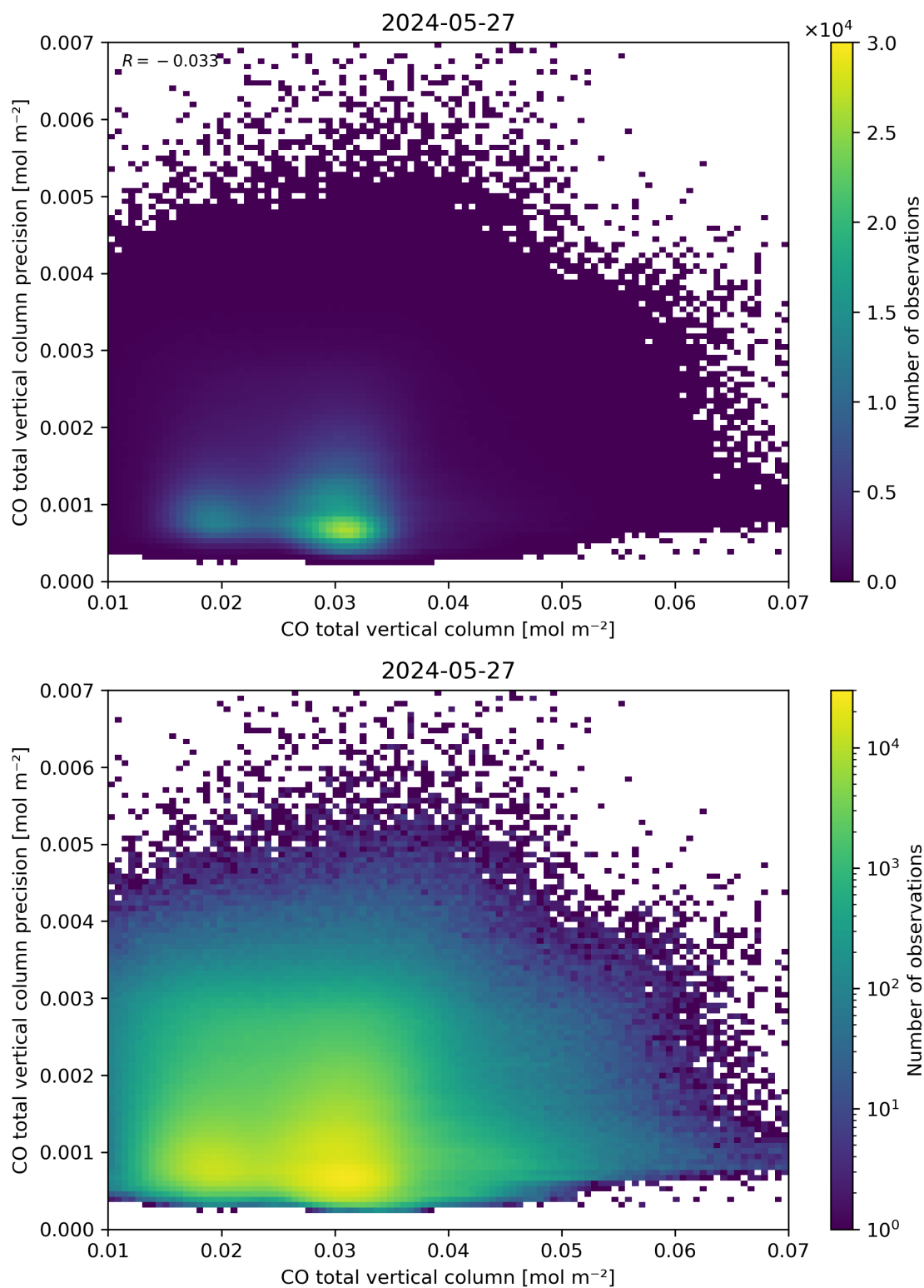
Figure 34: Scatter density plot of “CO total vertical column” against “CO total vertical column precision” for 2024-05-26 to 2024-05-28.
