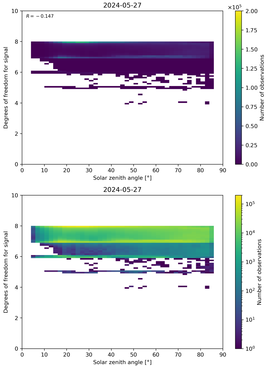
Figure 65: Scatter density plot of “Solar zenith angle” against “Degrees of freedom for signal” for 2024-05-26 to 2024-05-28.
