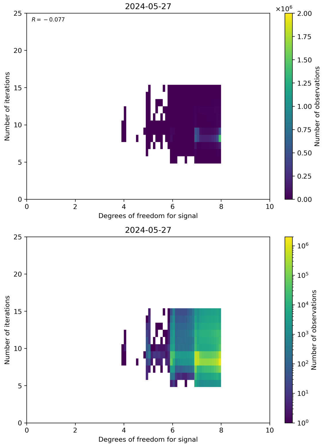
Figure 50: Scatter density plot of “Degrees of freedom for signal” against “Number of iterations” for 2024-05-26 to 2024-05-28.
