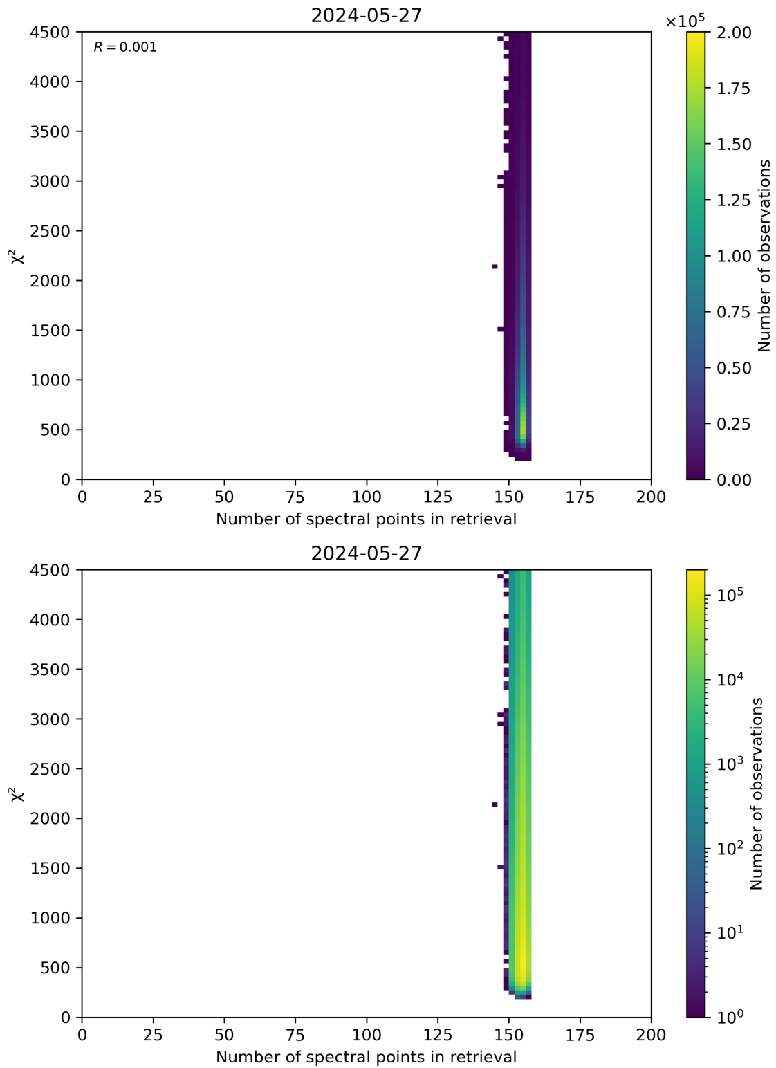
Figure 58: Scatter density plot of “Number of spectral points in retrieval” against “ \chi^2 ” for 2024-05-26 to 2024-05-28.
