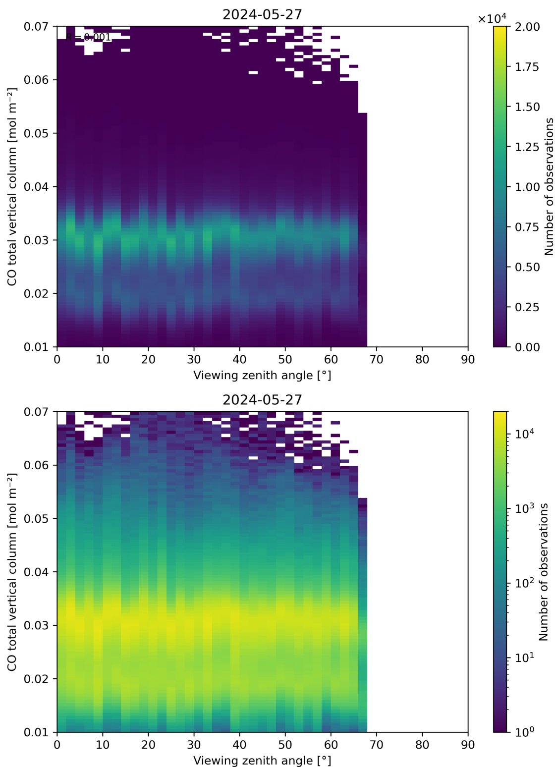
Figure 69: Scatter density plot of “Viewing zenith angle” against “CO total vertical column” for 2024-05-26 to 2024-05-28.
