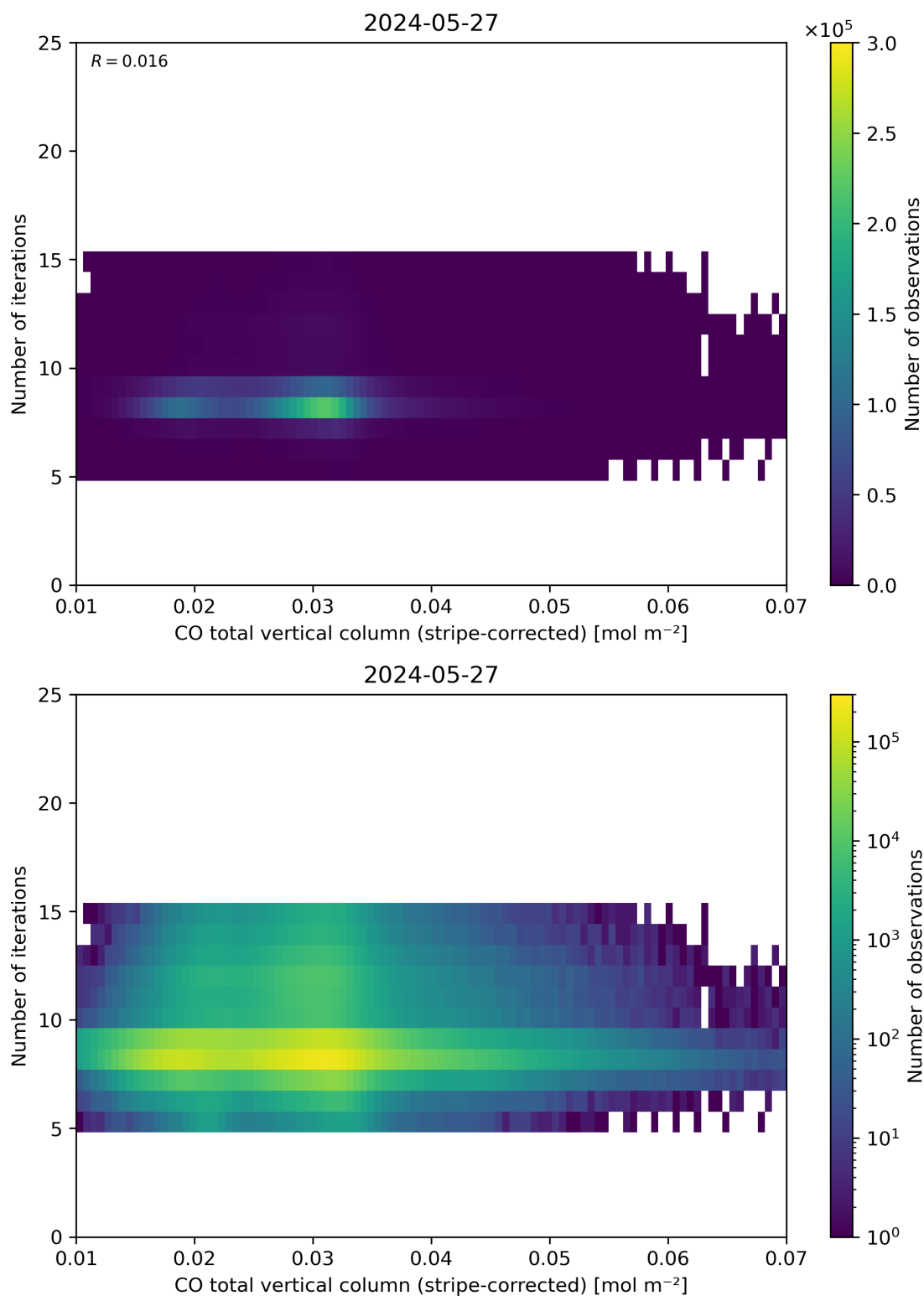
Figure 39: Scatter density plot of “CO total vertical column (stripe-corrected)” against “Number of iterations” for 2024-05-26 to 2024-05-28.
