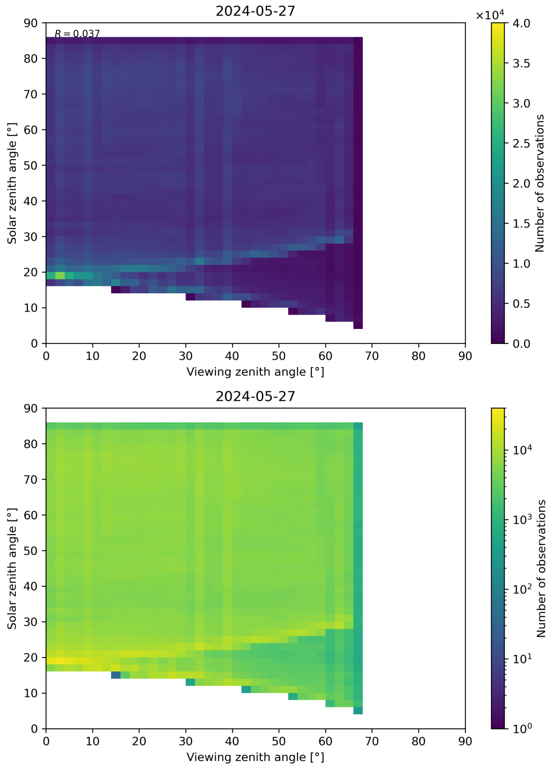
Figure 77: Scatter density plot of “Viewing zenith angle” against “Solar zenith angle” for 2024-05-26 to 2024-05-28.
