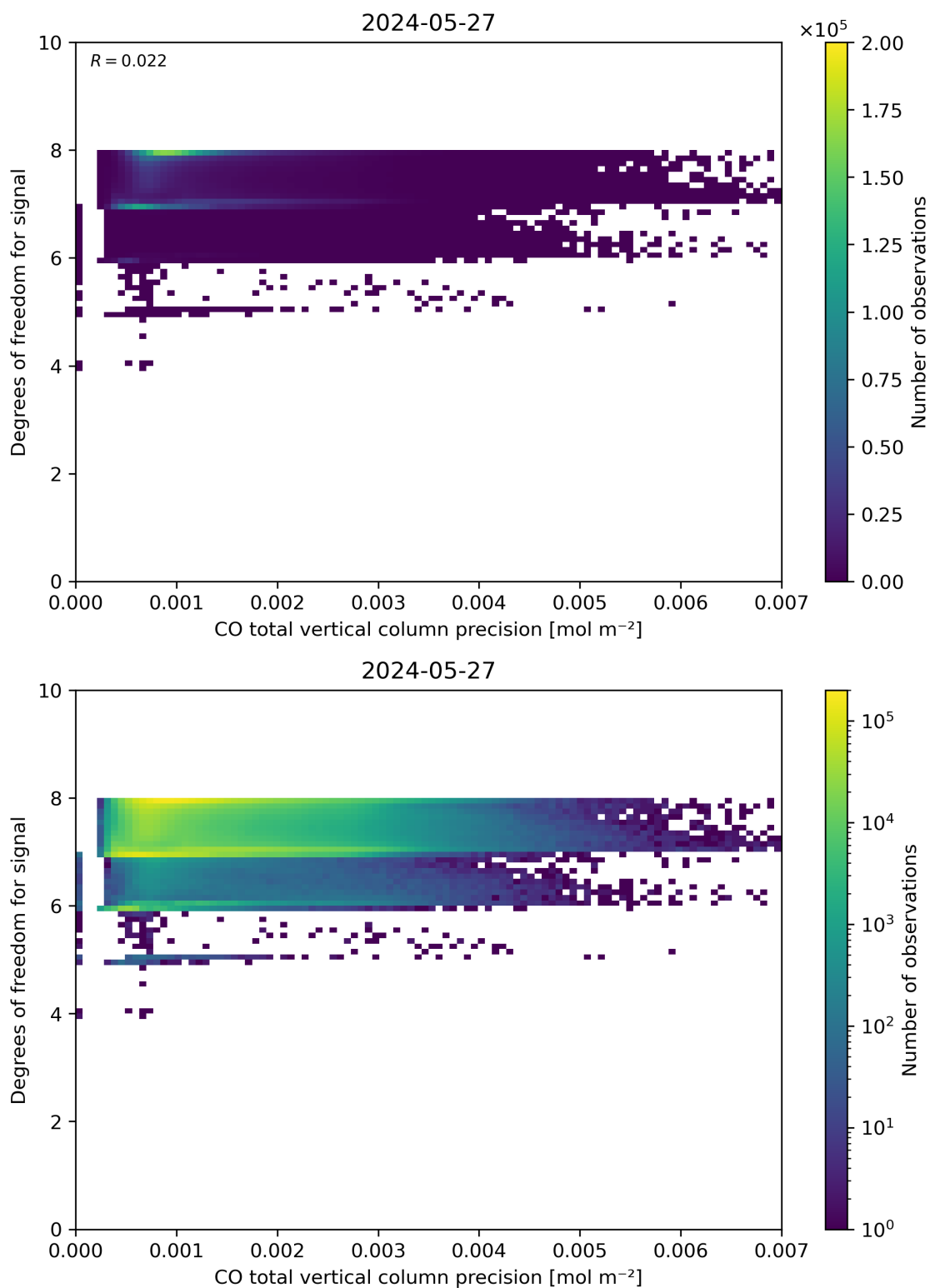
Figure 45: Scatter density plot of “CO total vertical column precision” against “Degrees of freedom for signal” for 2024-05-26 to 2024-05-28.
