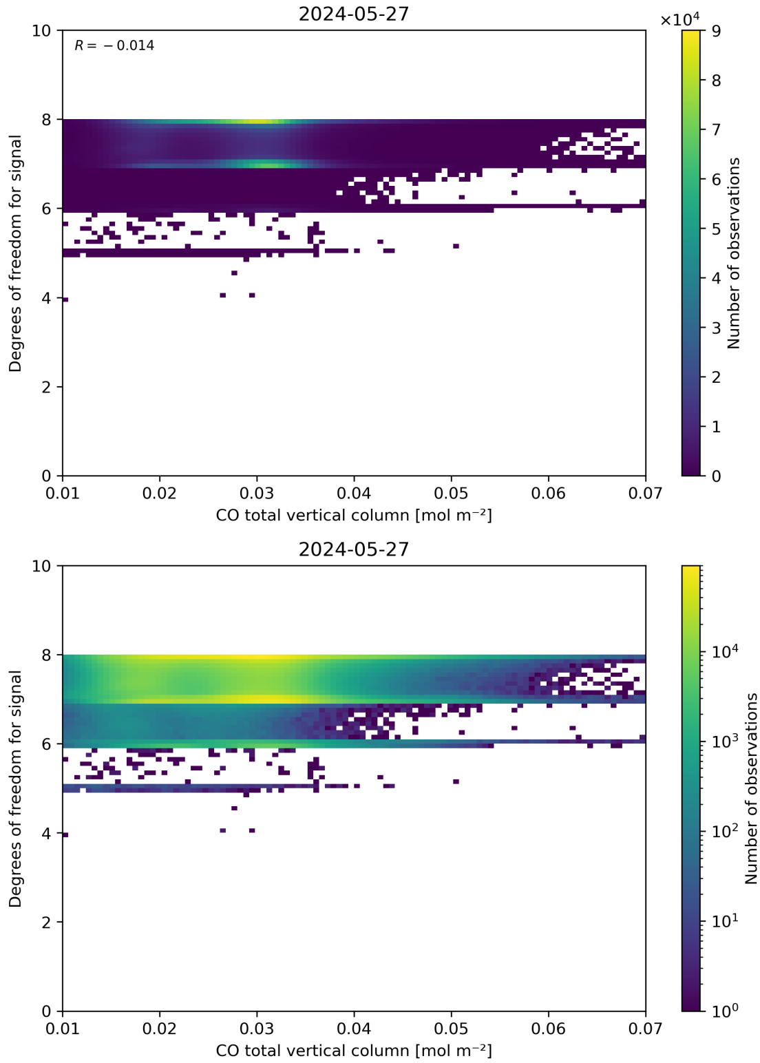
Figure 41: Scatter density plot of “CO total vertical column” against “Degrees of freedom for signal” for 2024-05-26 to 2024-05-28.
