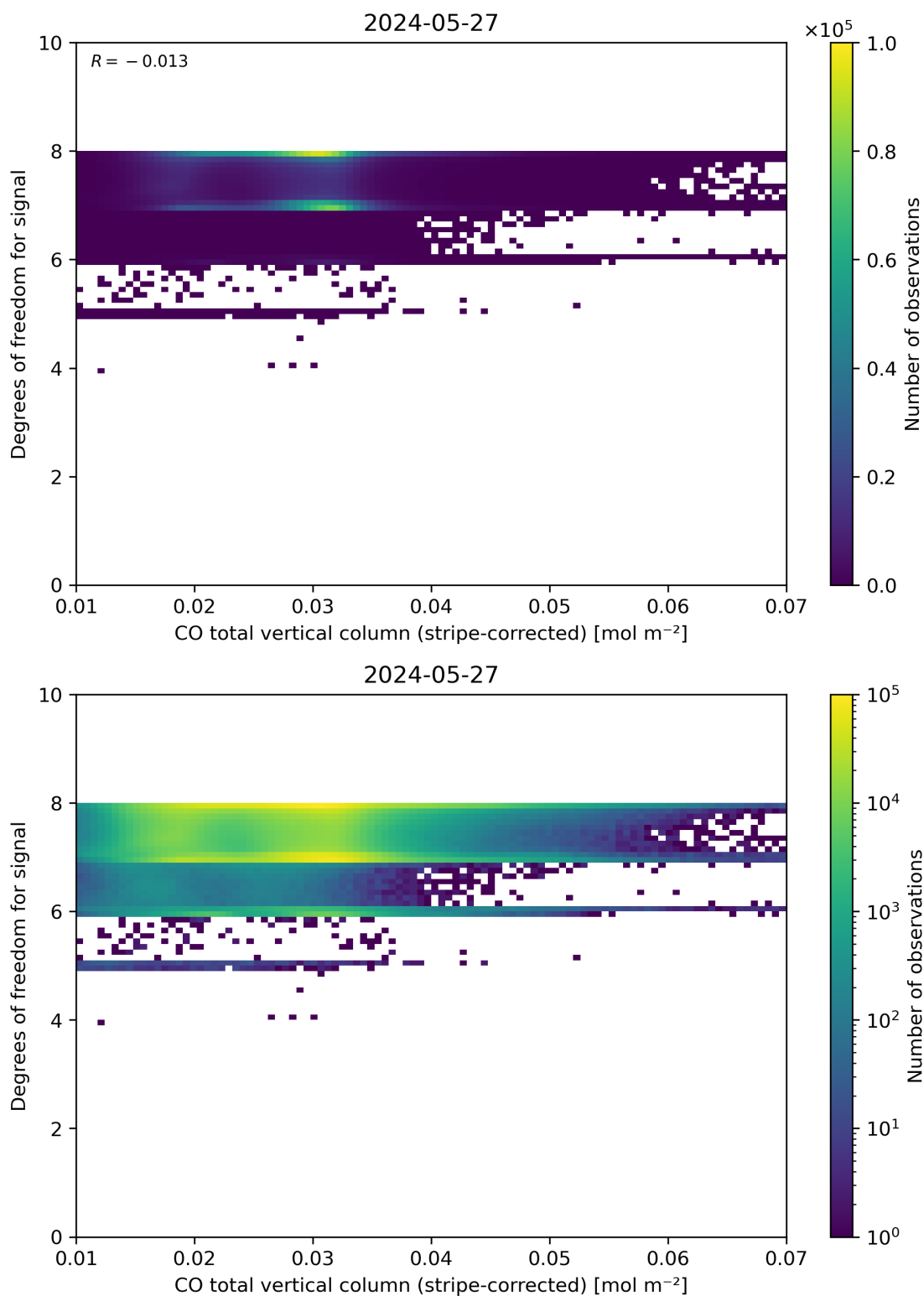
Figure 38: Scatter density plot of “CO total vertical column (stripe-corrected)” against “Degrees of freedom for signal” for 2024-05-26 to 2024-05-28.
