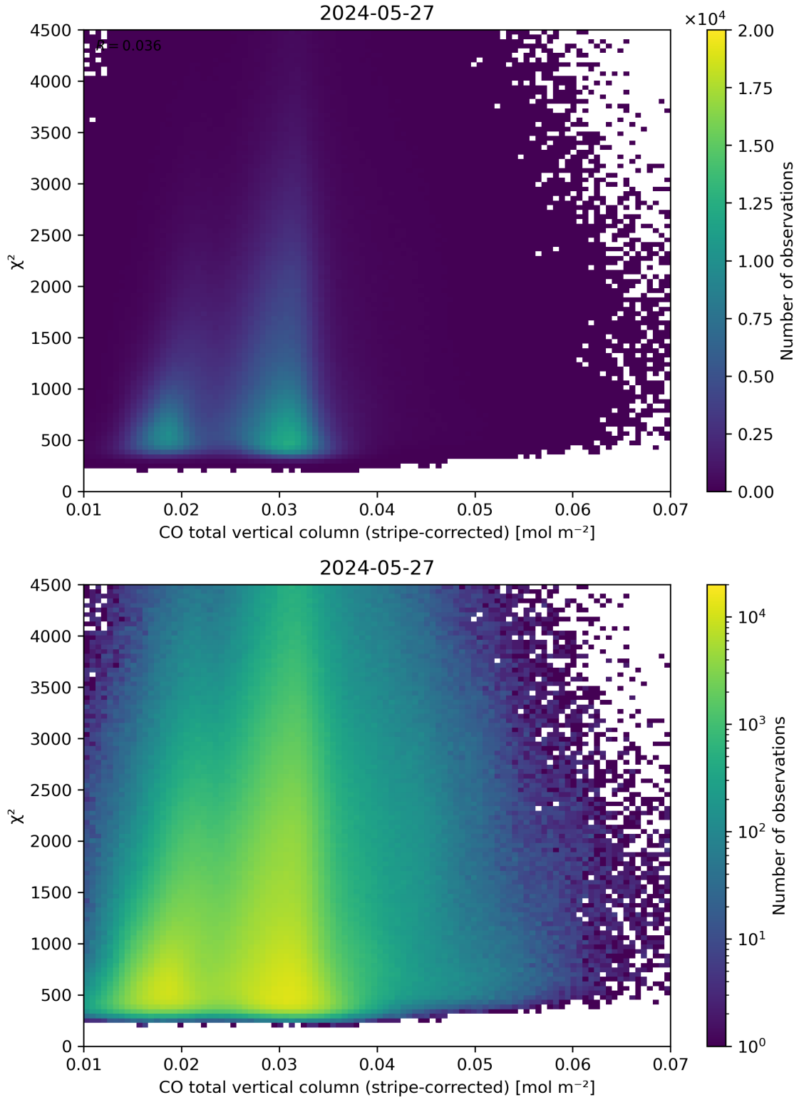
Figure 37: Scatter density plot of “CO total vertical column (stripe-corrected)” against “ \chi^2 ” for 2024-05-26 to 2024-05-28.
