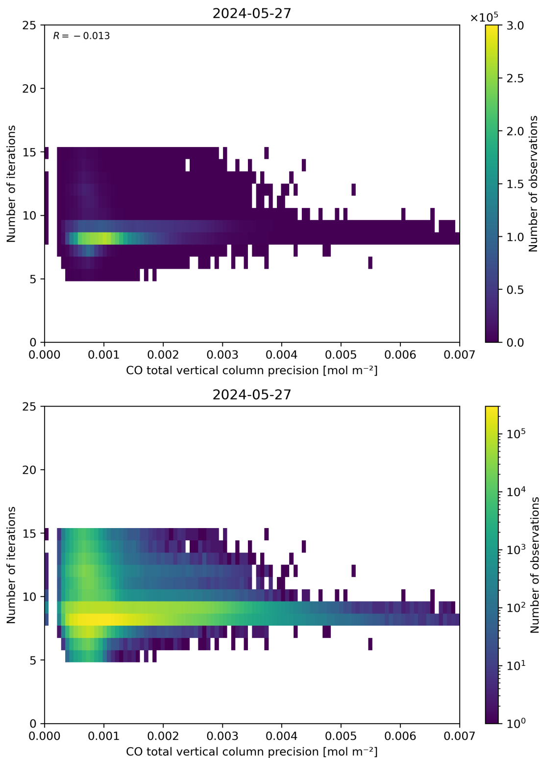
Figure 46: Scatter density plot of “CO total vertical column precision” against “Number of iterations” for 2024-05-26 to 2024-05-28.
