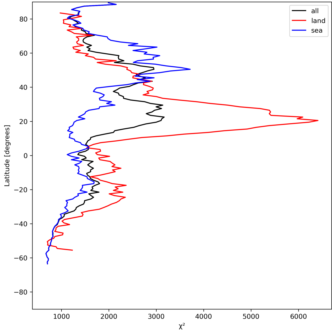
Figure 14: Zonal average of “ \chi^2 ” for 2024-05-26 to 2024-05-28.
