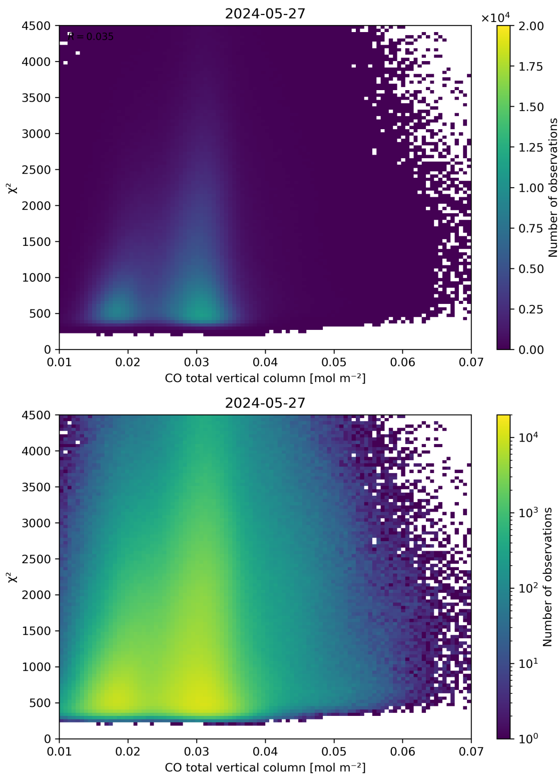
Figure 35: Scatter density plot of “CO total vertical column” against “ \chi^2 ” for 2024-05-26 to 2024-05-28.
