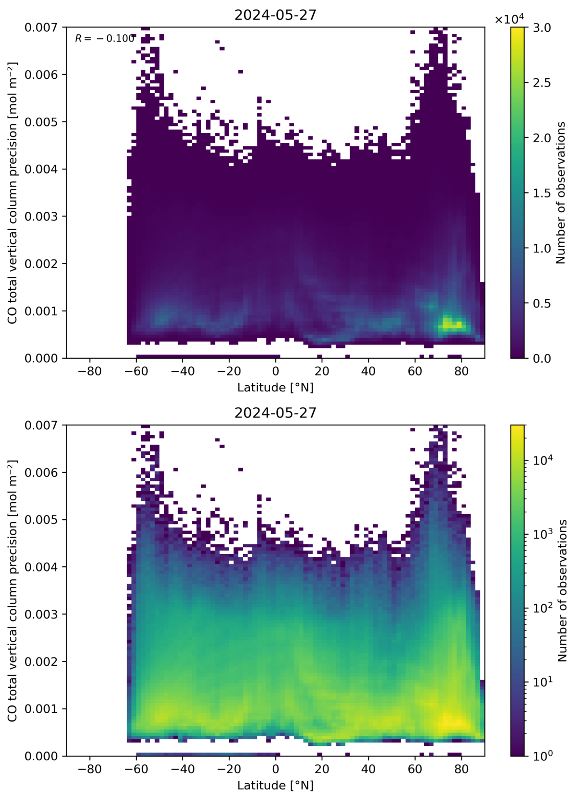
Figure 53: Scatter density plot of “Latitude” against “CO total vertical column precision” for 2024-05-26 to 2024-05-28.
