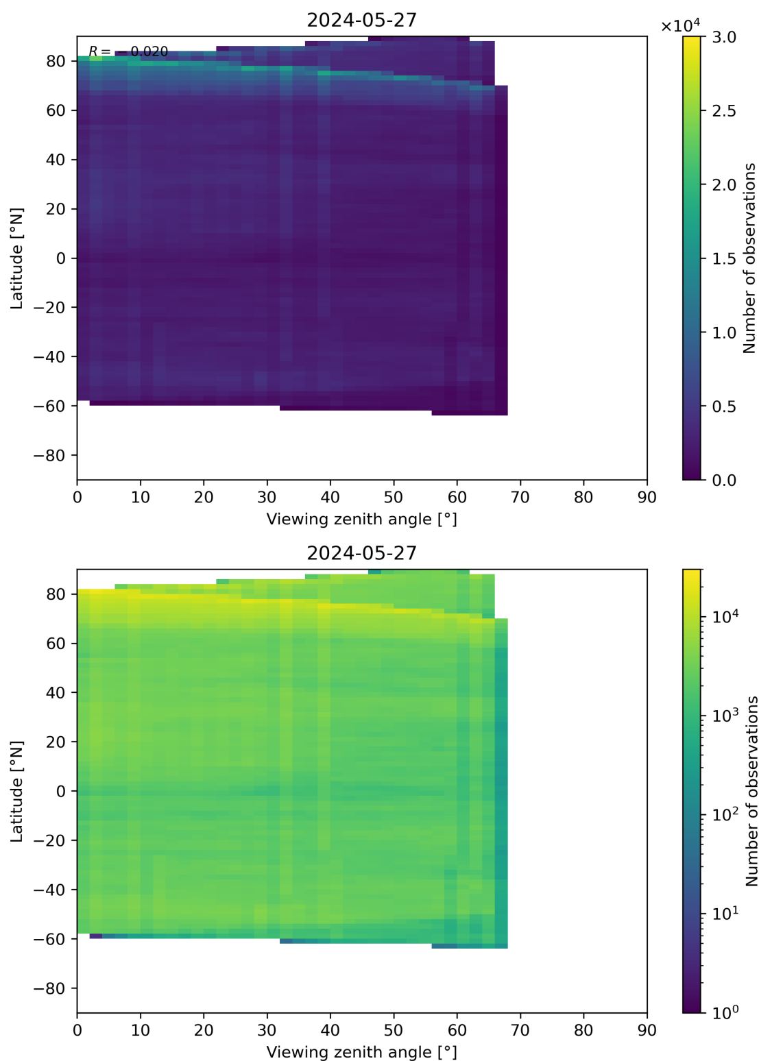
Figure 74: Scatter density plot of “Viewing zenith angle” against “Latitude” for 2024-05-26 to 2024-05-28.
