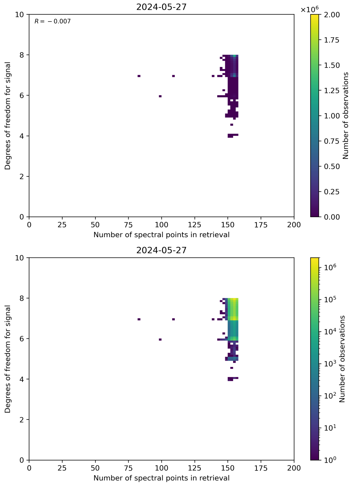
Figure 59: Scatter density plot of “Number of spectral points in retrieval” against “Degrees of freedom for signal” for 2024-05-26 to 2024-05-28.
