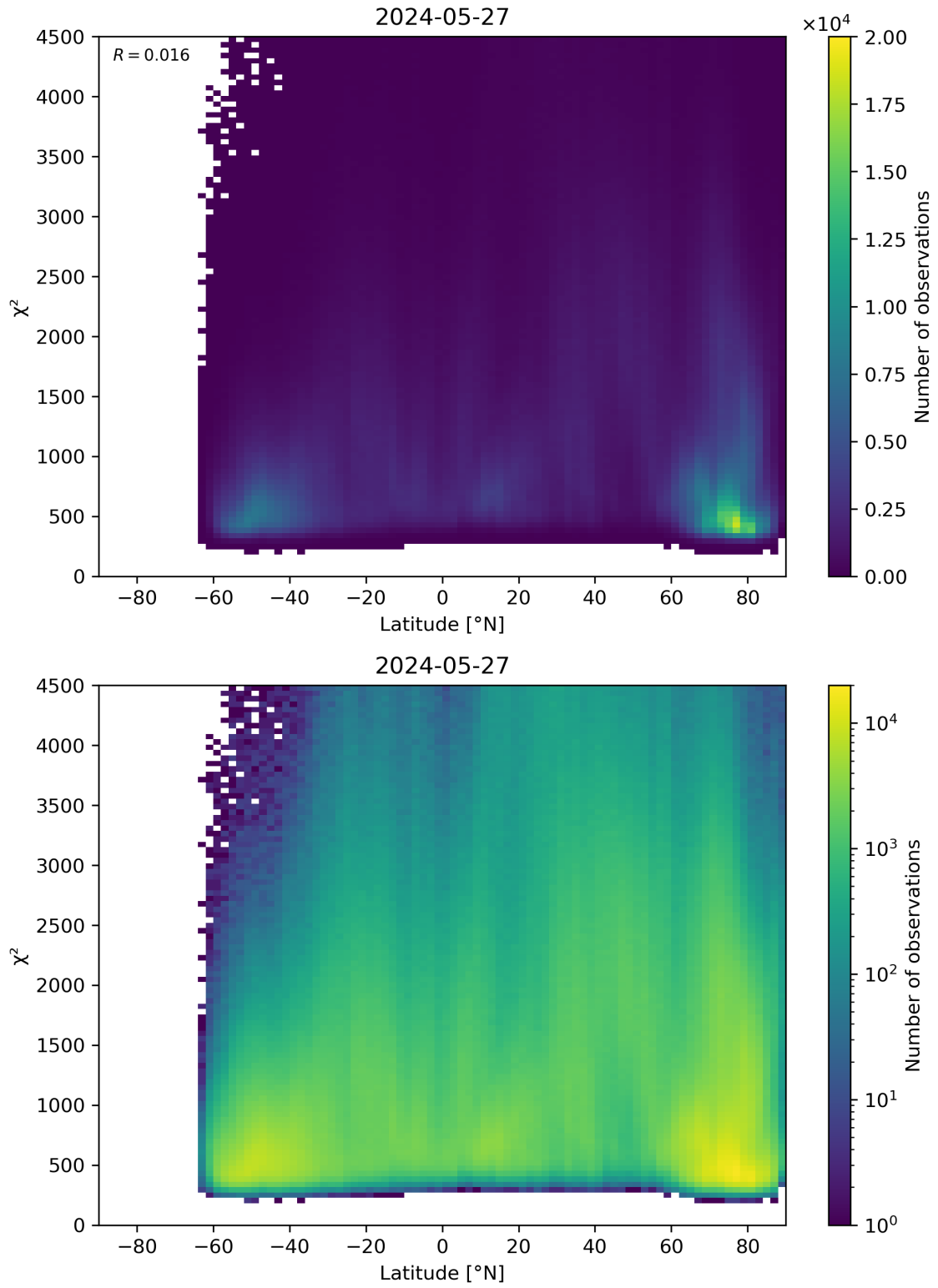
Figure 54: Scatter density plot of “Latitude” against “ \chi^2 ” for 2024-05-26 to 2024-05-28.
