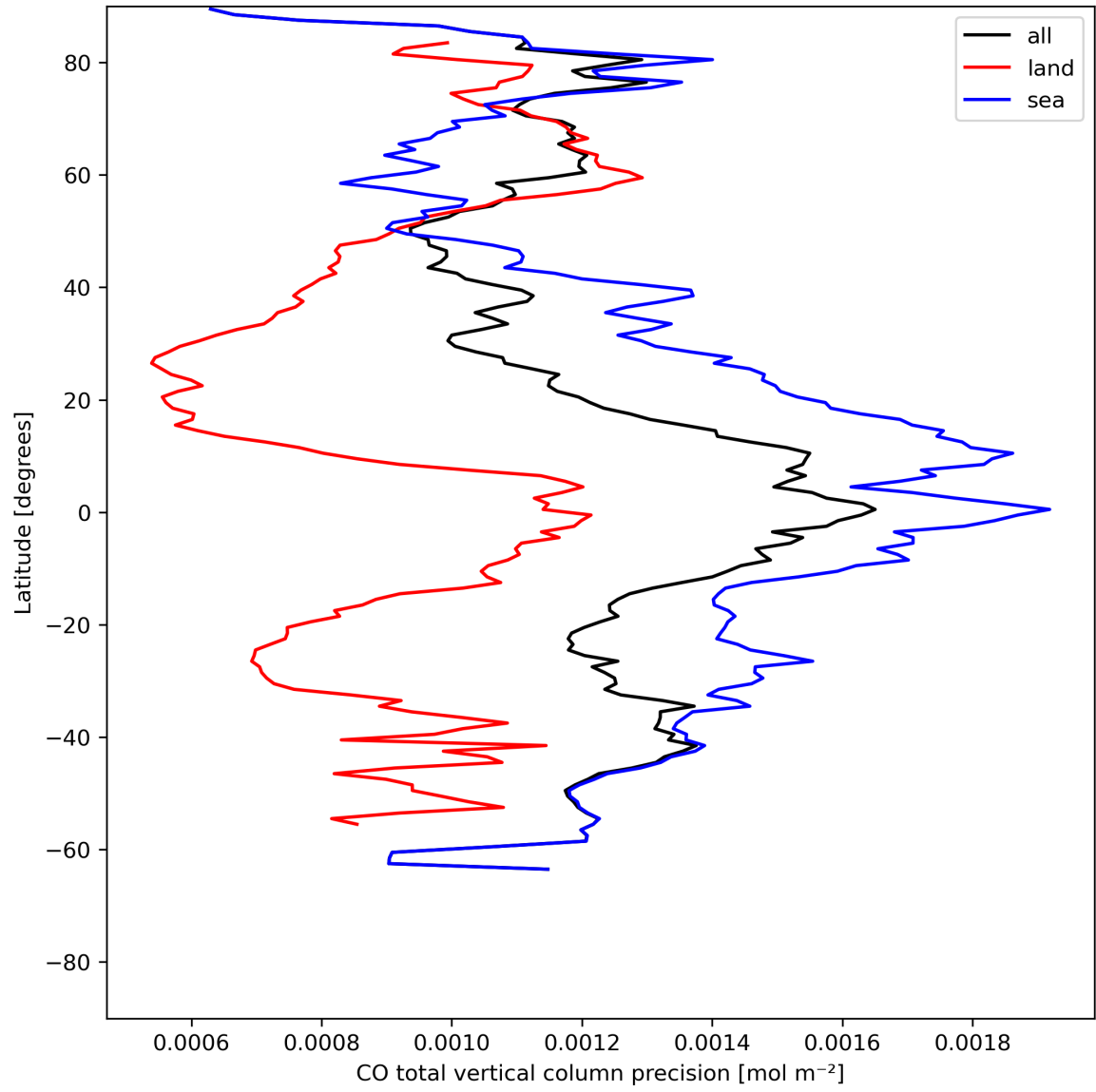
Figure 12: Zonal average of “CO total vertical column precision” for 2024-05-26 to 2024-05-28.
