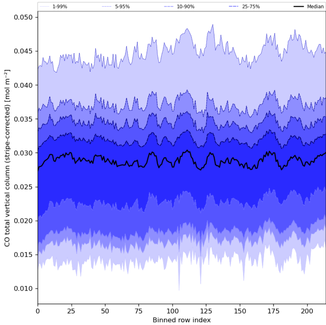
Figure 27: Along track statistics of "CO total vertical column (stripe-corrected)" for 2024-05-26 to 2024-05-28
