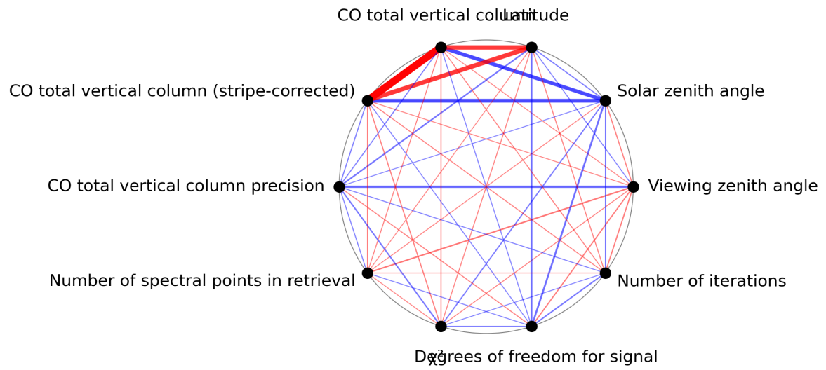
Figure 1: Map of correlation graph for 2024-05-26 to 2024-05-28.
