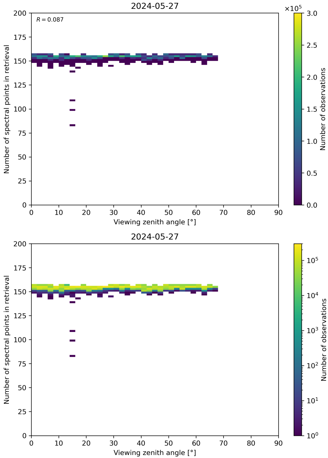
Figure 76: Scatter density plot of “Viewing zenith angle” against “Number of spectral points in retrieval” for 2024-05-26 to 2024-05-28.
