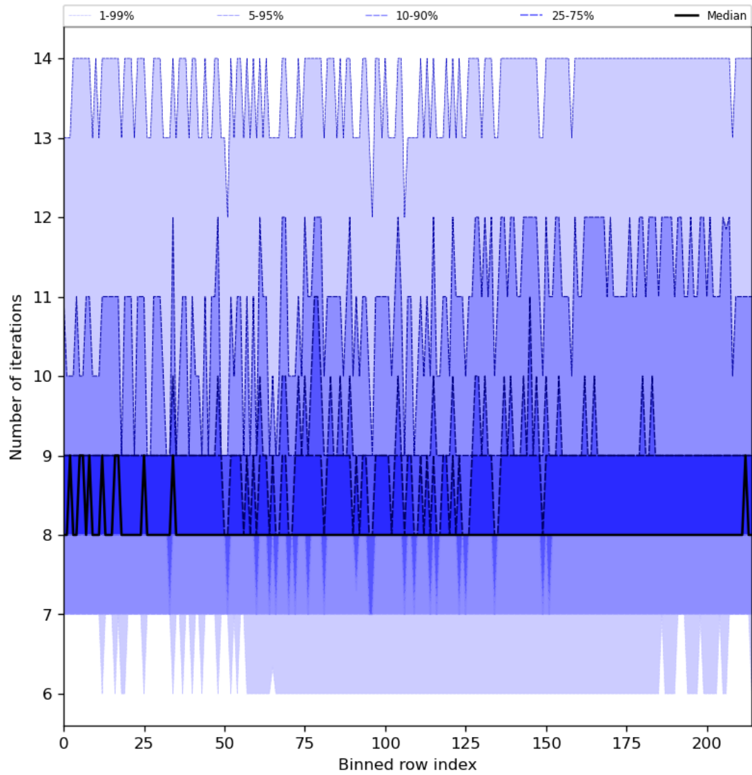
Figure 32: Along track statistics of “Number of iterations” for 2024-05-26 to 2024-05-28
