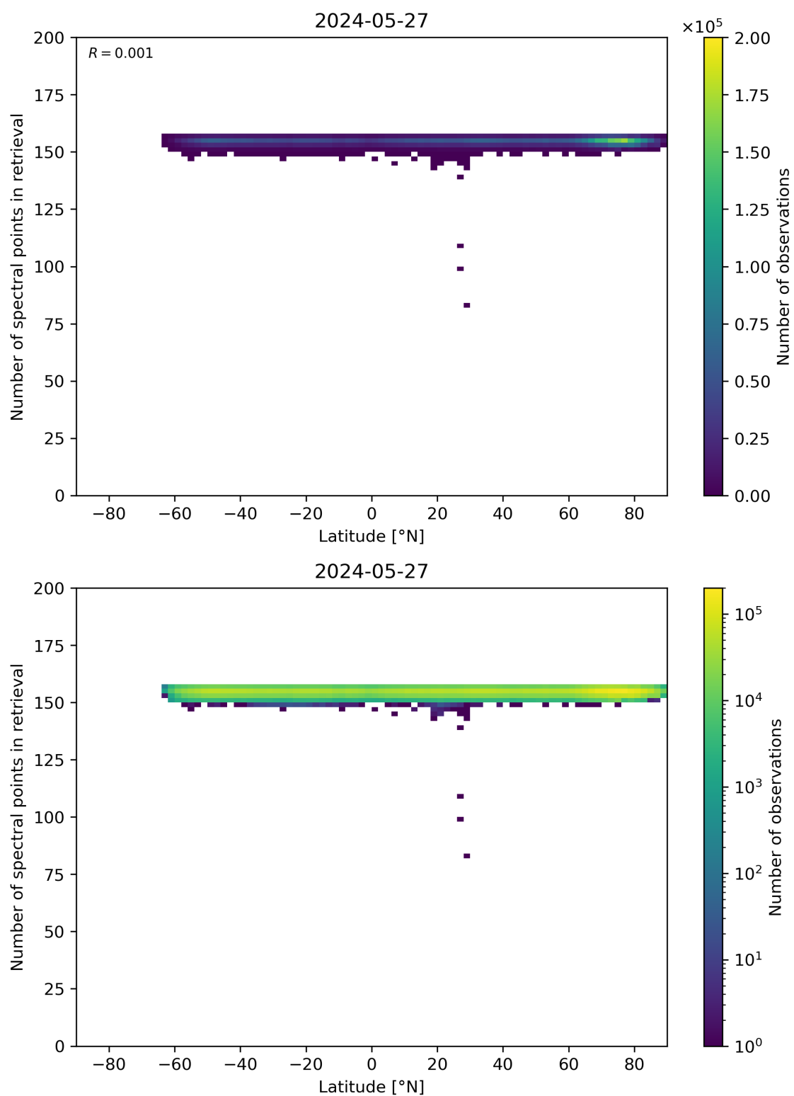
Figure 57: Scatter density plot of “Latitude” against “Number of spectral points in retrieval” for 2024-05-26 to 2024-05-28.
