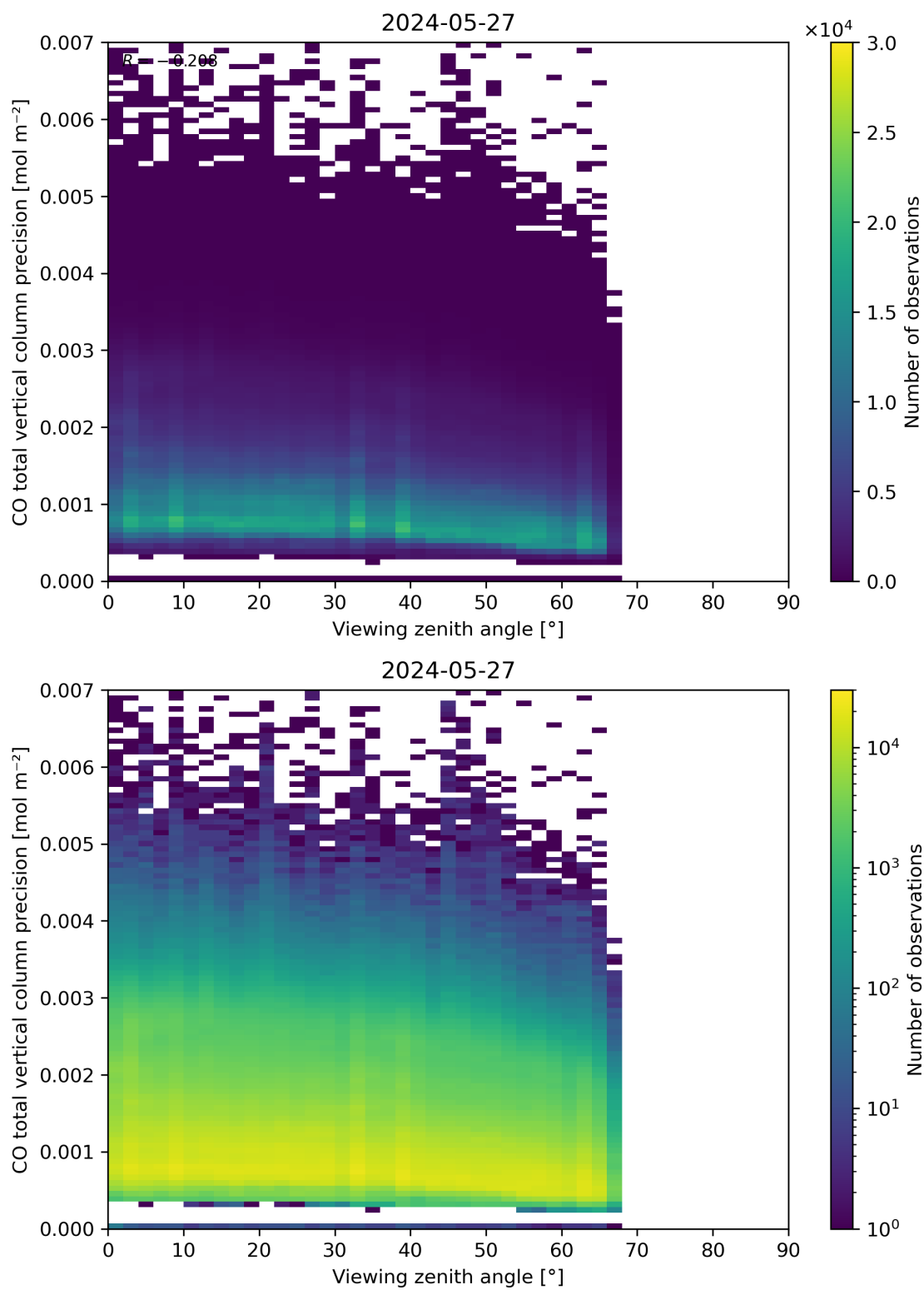
Figure 71: Scatter density plot of “Viewing zenith angle” against “CO total vertical column precision” for 2024-05-26 to 2024-05-28.
