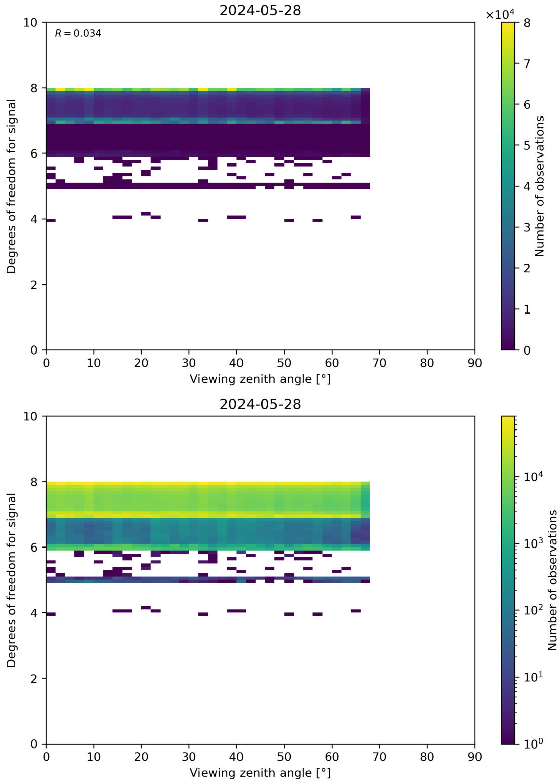
Figure 73: Scatter density plot of “Viewing zenith angle” against “Degrees of freedom for signal” for 2024-05-28 to 2024-05-29.
