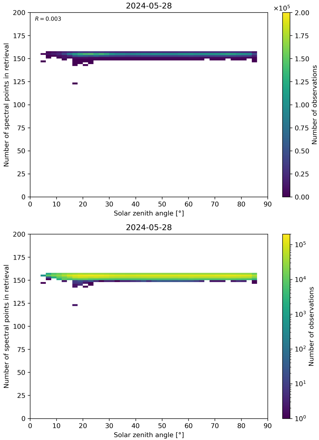
Figure 68: Scatter density plot of “Solar zenith angle” against “Number of spectral points in retrieval” for 2024-05-28 to 2024-05-29.
