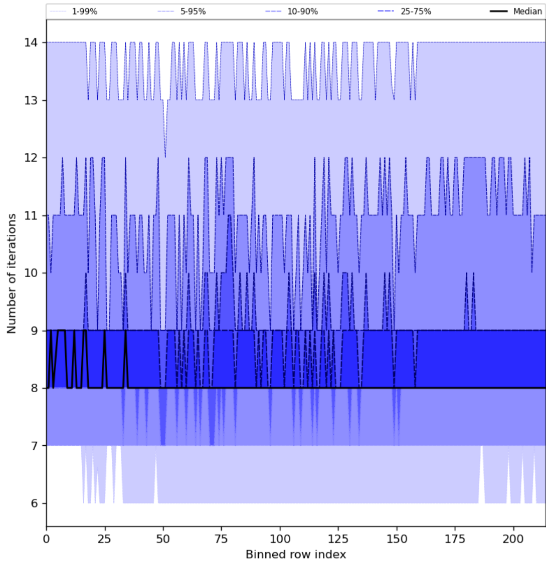
Figure 32: Along track statistics of “Number of iterations” for 2024-05-28 to 2024-05-29
