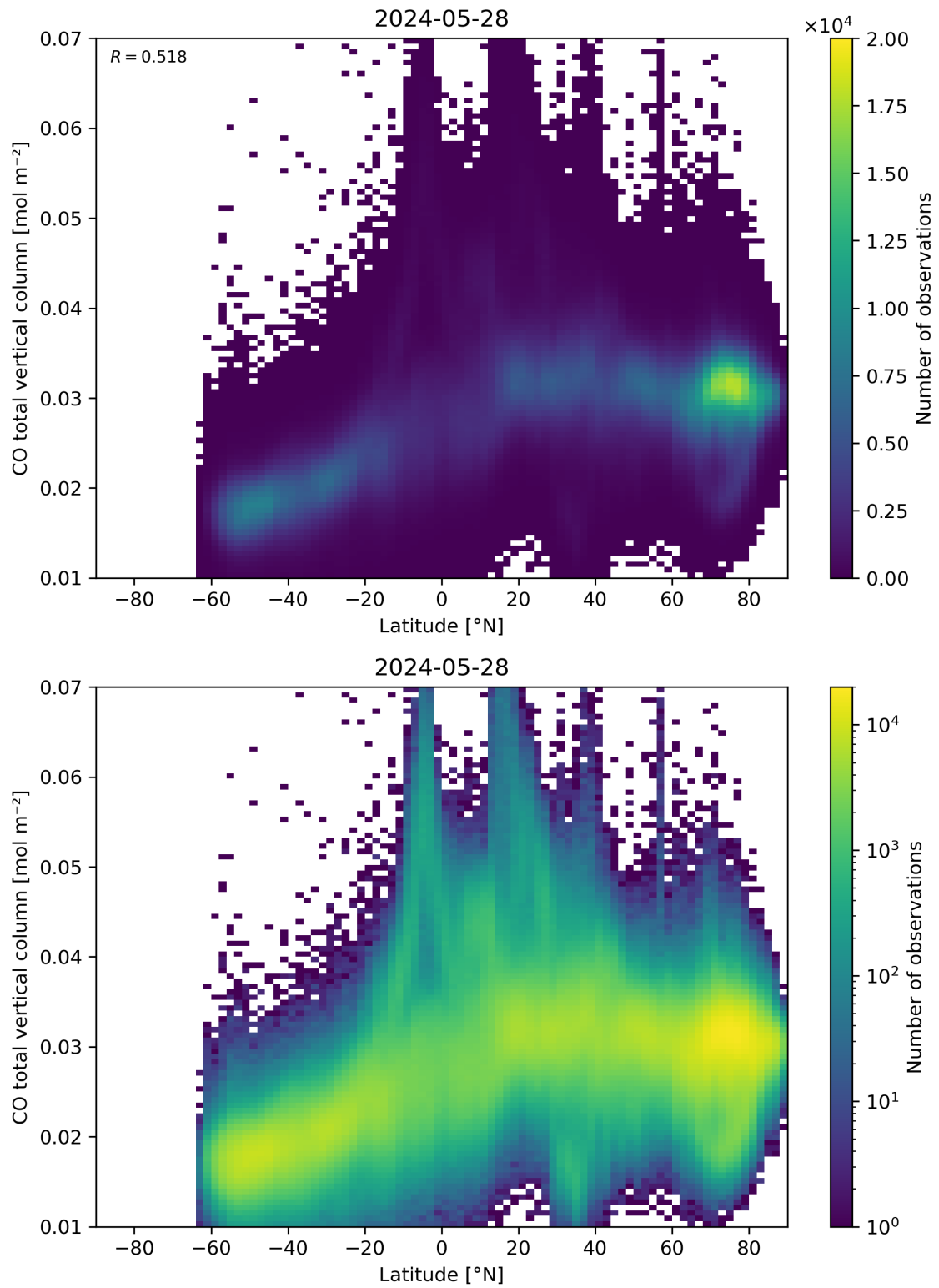
Figure 51: Scatter density plot of “Latitude” against “CO total vertical column” for 2024-05-28 to 2024-05-29.
