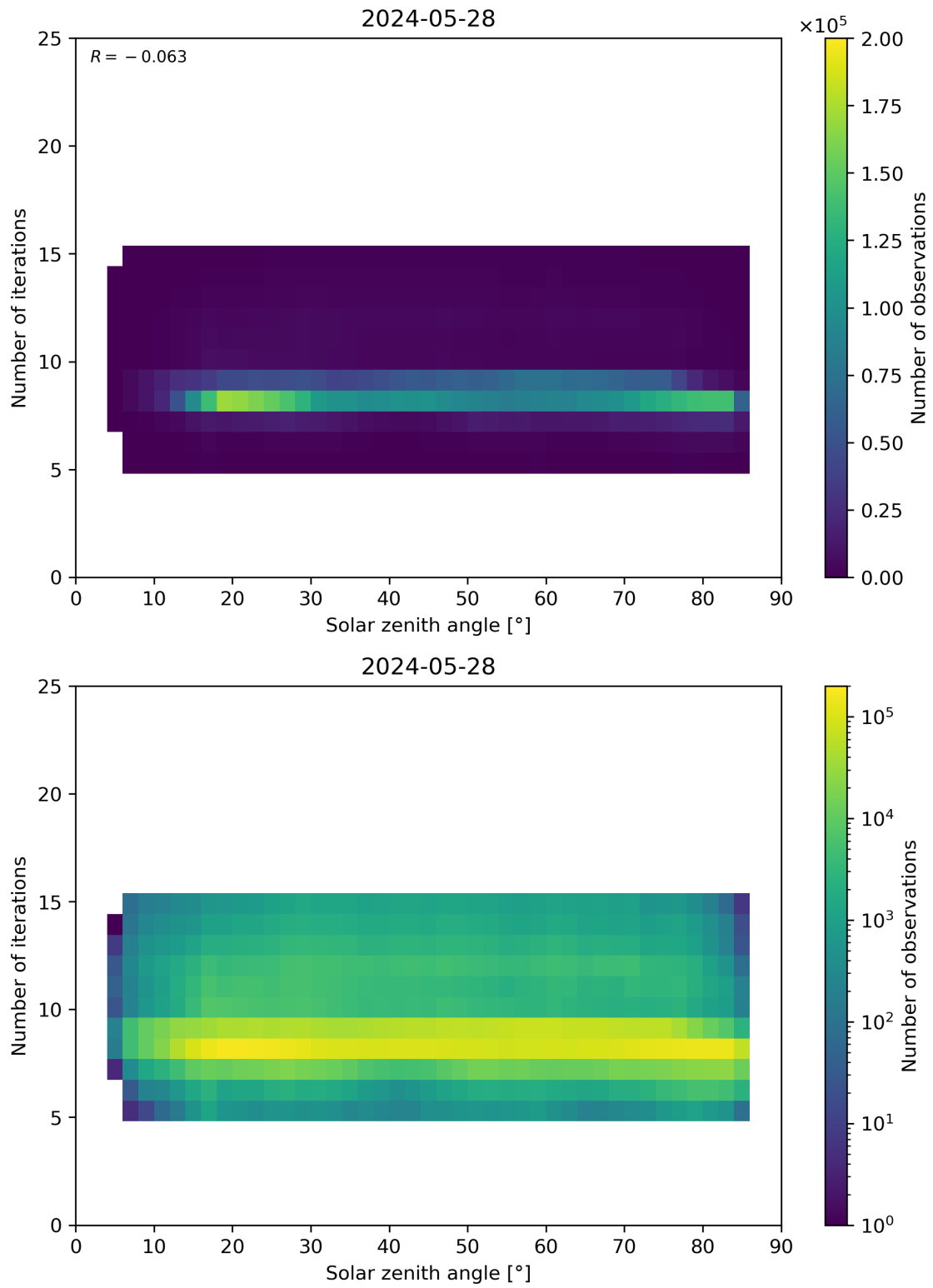
Figure 67: Scatter density plot of “Solar zenith angle” against “Number of iterations” for 2024-05-28 to 2024-05-29.
