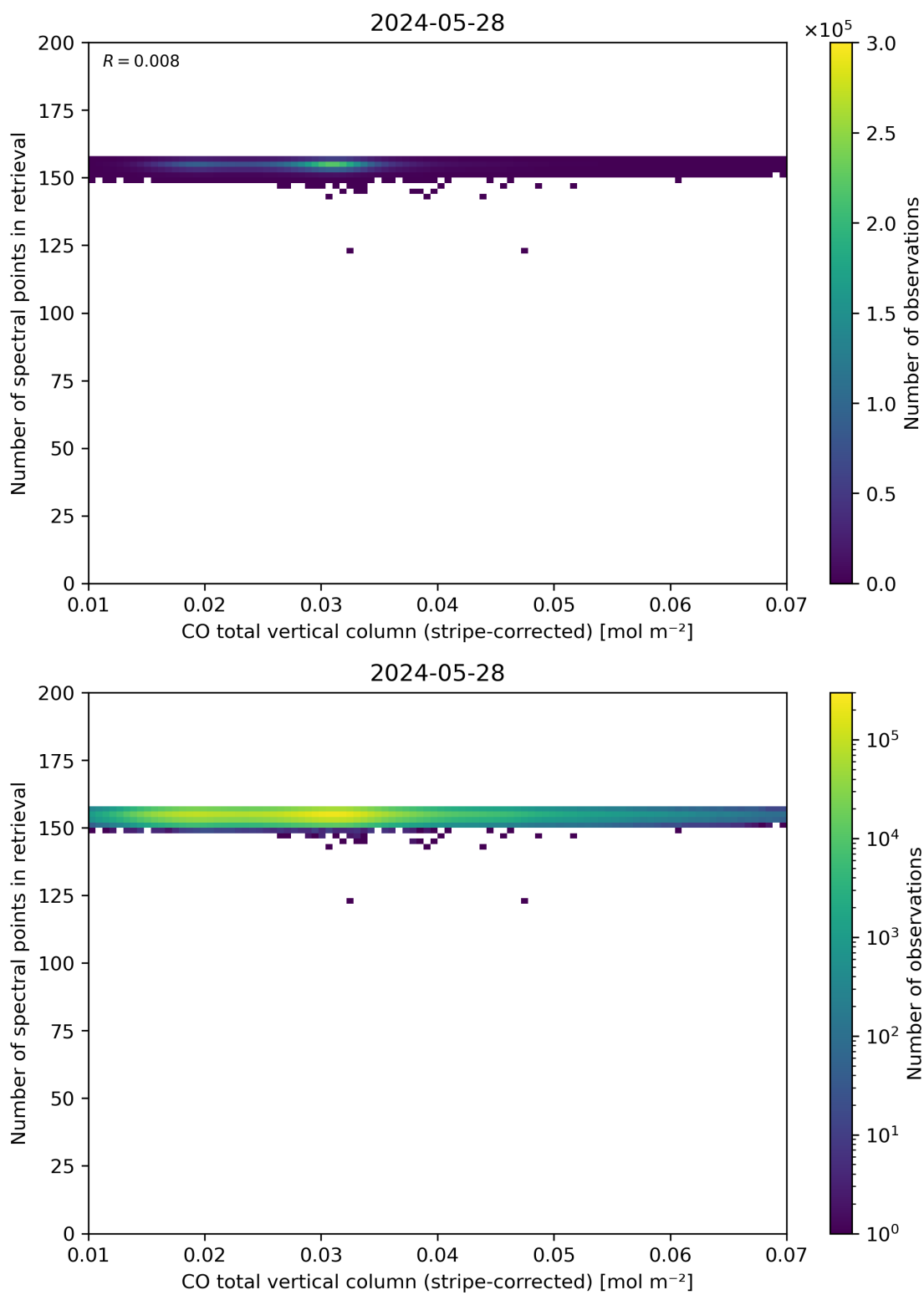
Figure 40: Scatter density plot of “CO total vertical column (stripe-corrected)” against “Number of spectral points in retrieval” for 2024-05-28 to 2024-05-29.
