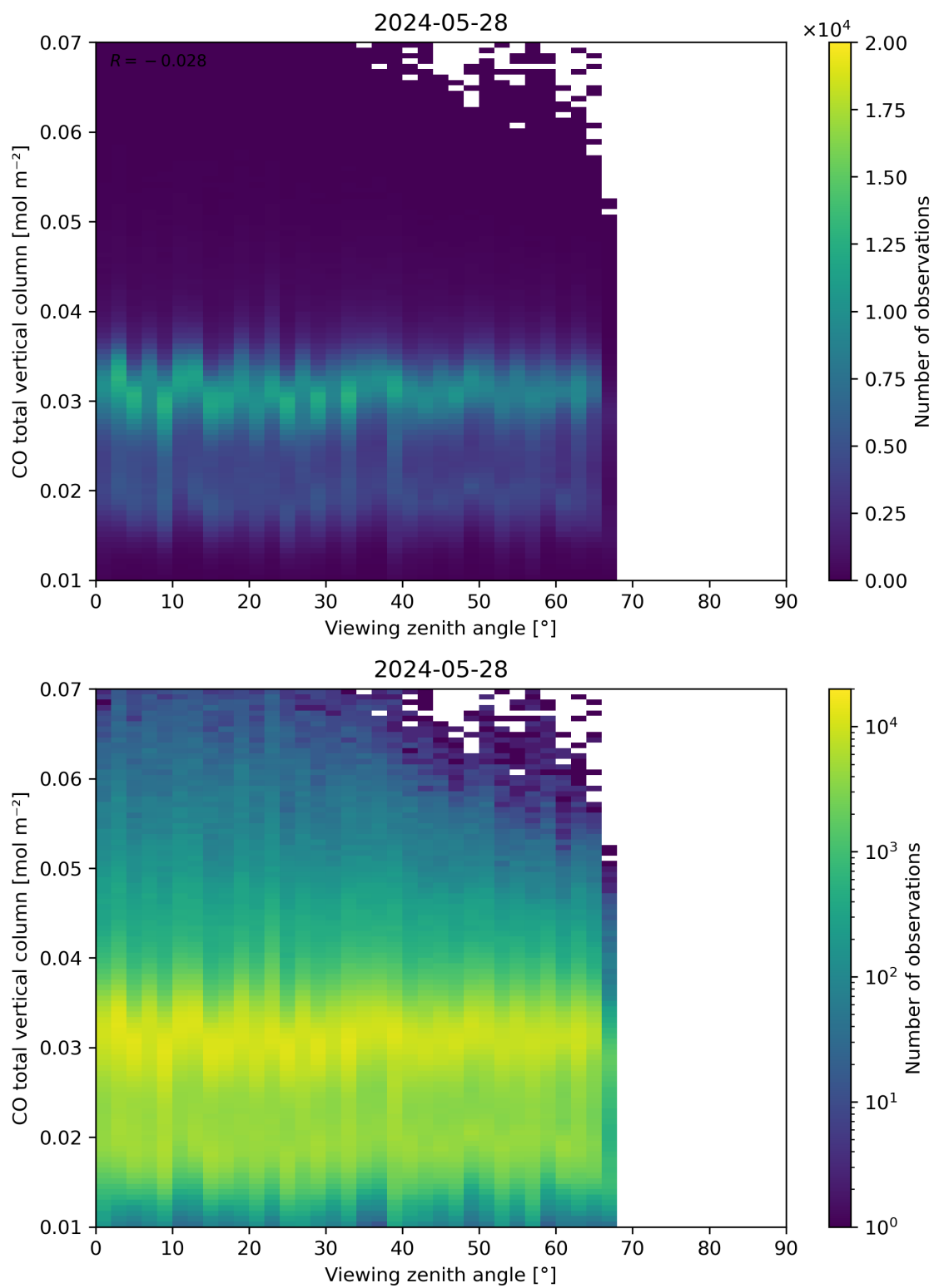
Figure 69: Scatter density plot of “Viewing zenith angle” against “CO total vertical column” for 2024-05-28 to 2024-05-29.
