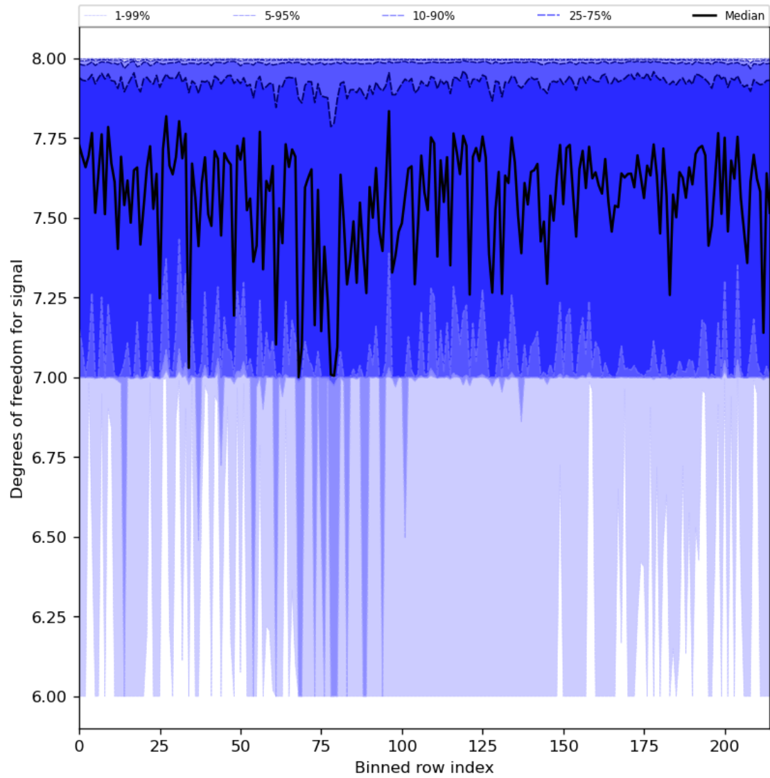
Figure 31: Along track statistics of “Degrees of freedom for signal” for 2024-05-28 to 2024-05-29
