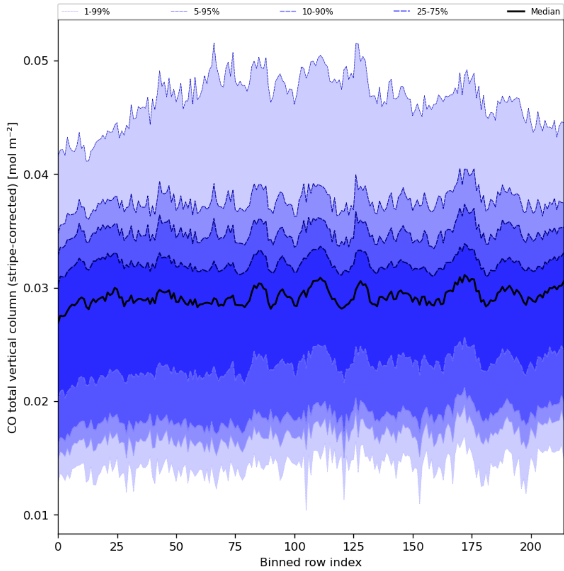
Figure 27: Along track statistics of “CO total vertical column (stripe-corrected)” for 2024-05-28 to 2024-05-29
