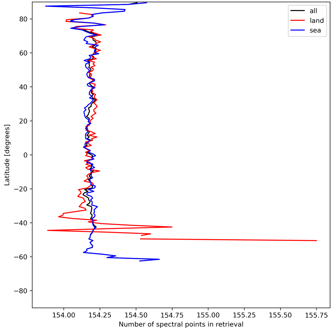
Figure 13: Zonal average of “Number of spectral points in retrieval” for 2024-05-28 to 2024-05-29.
