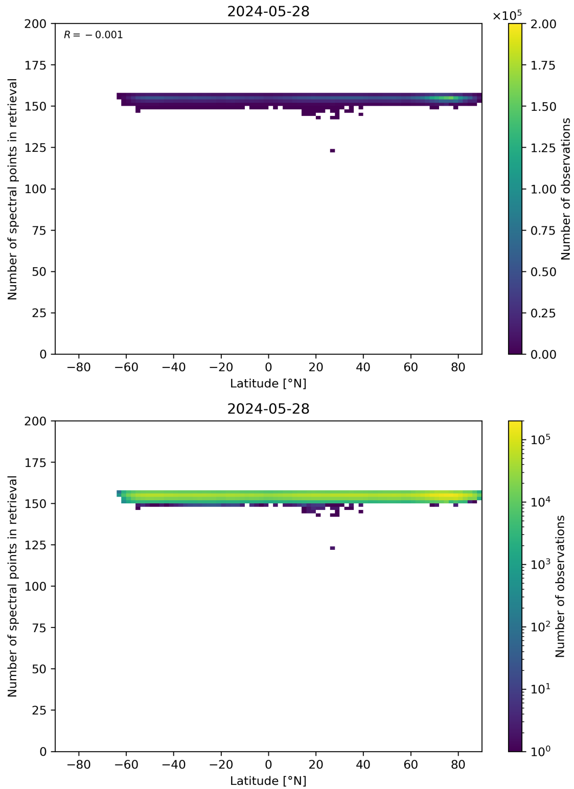
Figure 57: Scatter density plot of “Latitude” against “Number of spectral points in retrieval” for 2024-05-28 to 2024-05-29.
