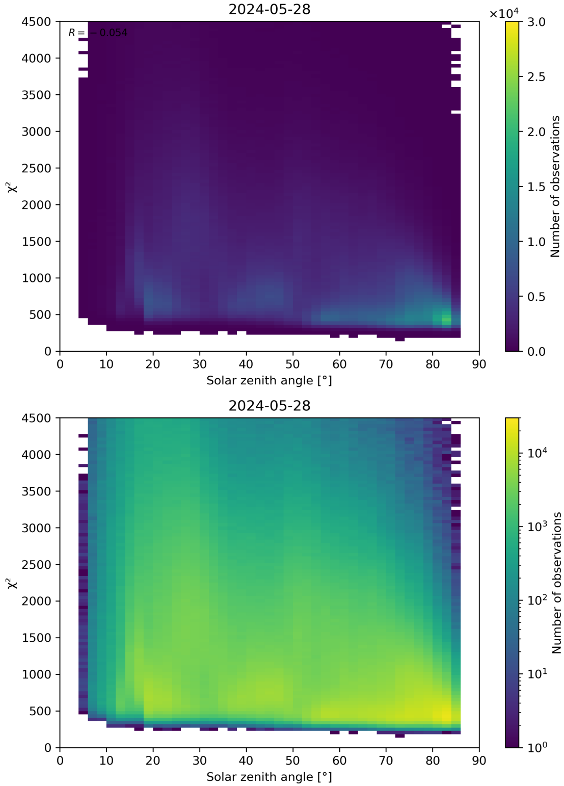
Figure 64: Scatter density plot of “Solar zenith angle” against “ \chi^2 ” for 2024-05-28 to 2024-05-29.
