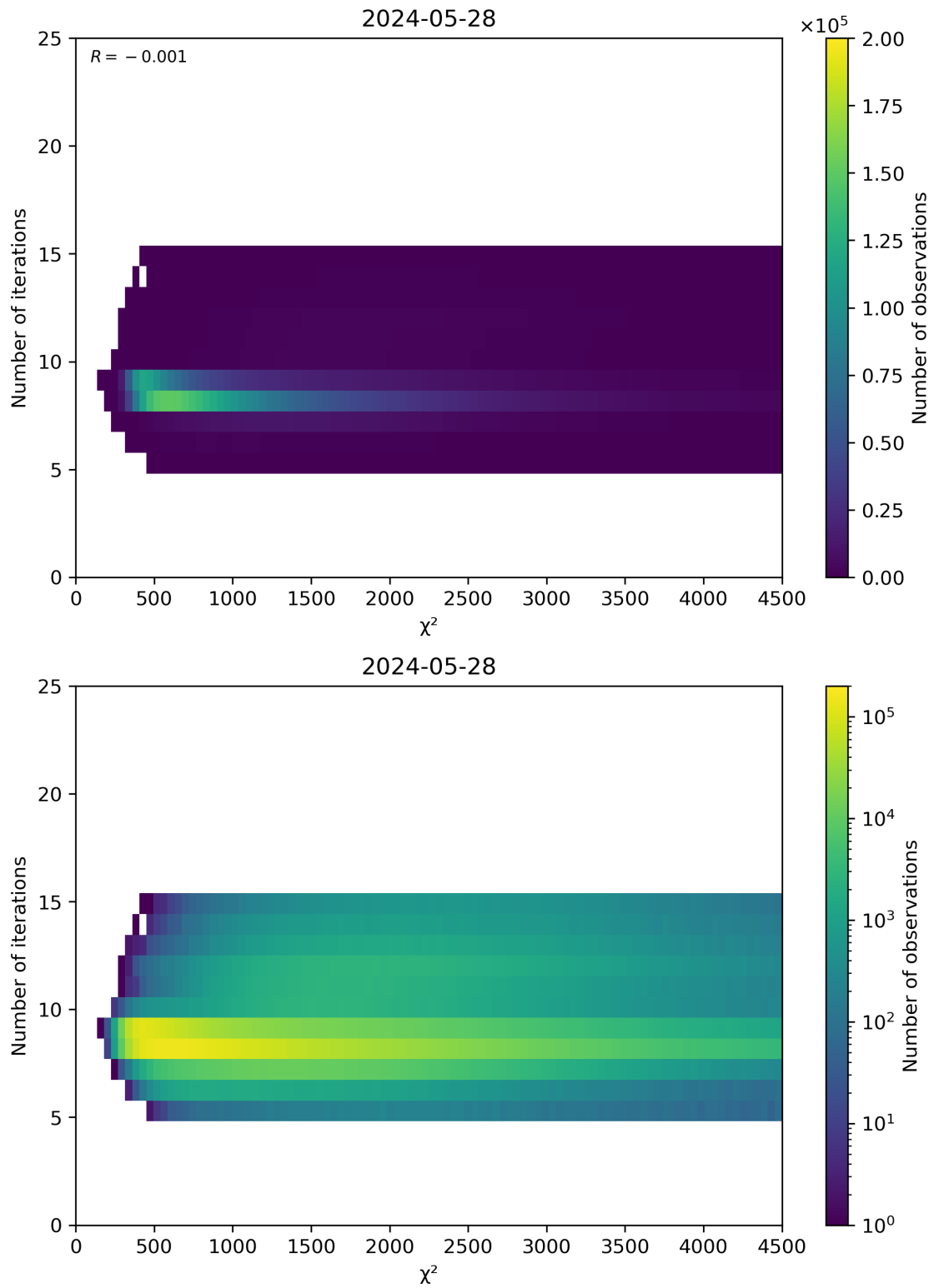
Figure 49: Scatter density plot of “ \chi^2 ” against “Number of iterations” for 2024-05-28 to 2024-05-29.
