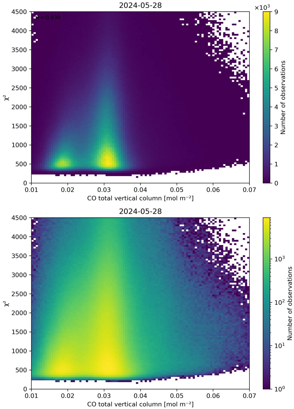
Figure 35: Scatter density plot of “CO total vertical column” against “ \chi^2 ” for 2024-05-28 to 2024-05-29.
