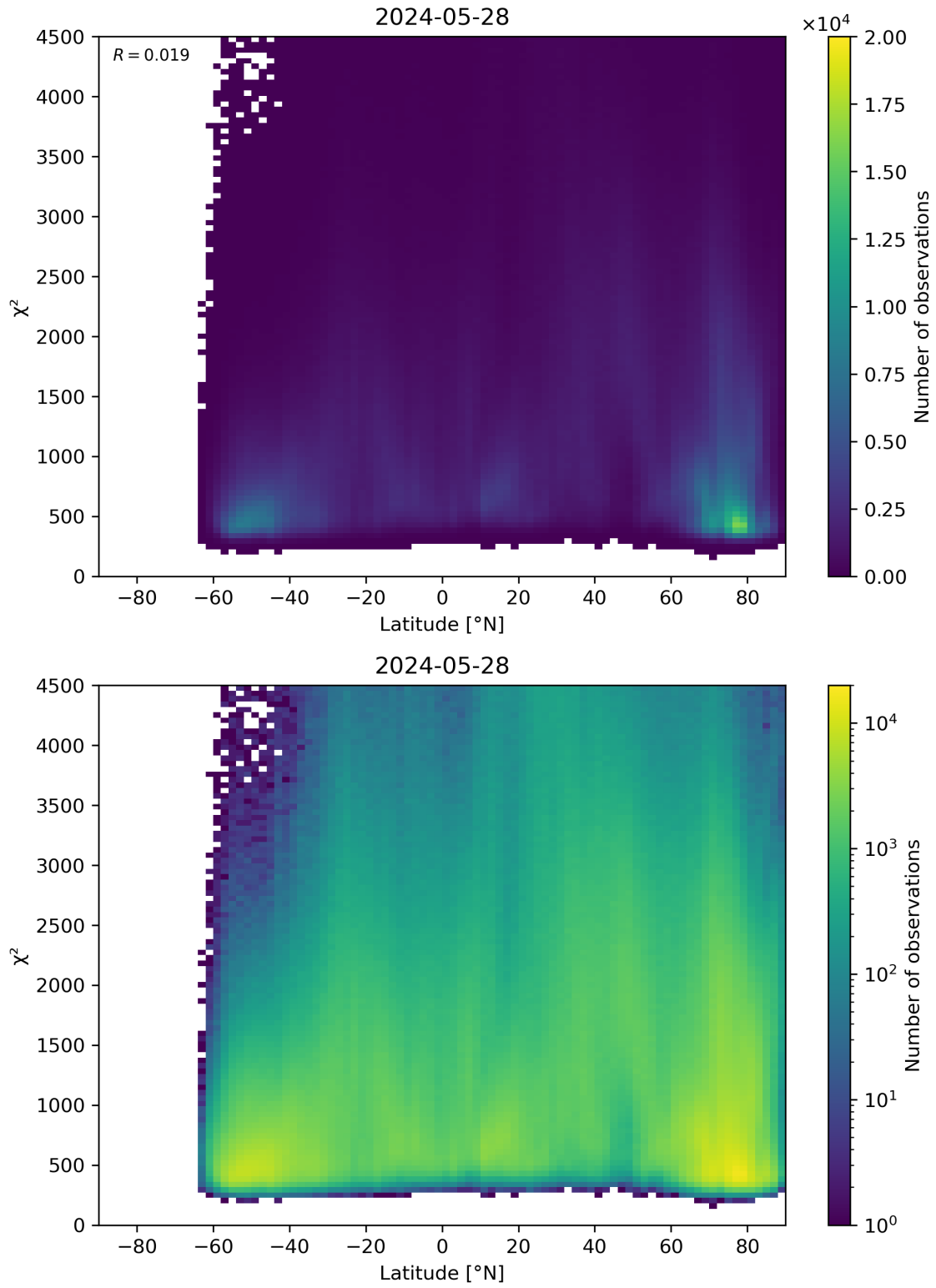
Figure 54: Scatter density plot of “Latitude” against “ \chi^2 ” for 2024-05-28 to 2024-05-29.
