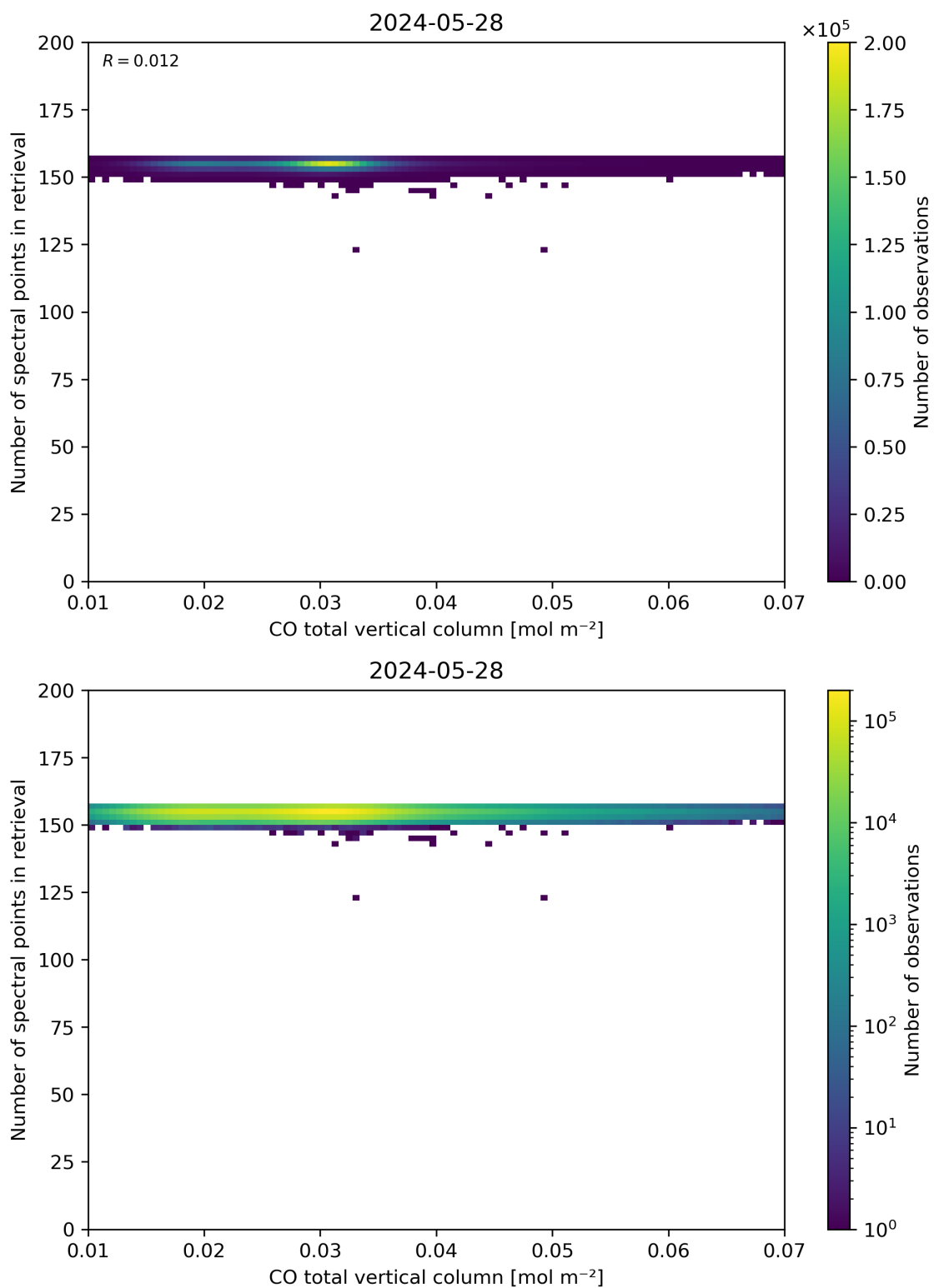
Figure 43: Scatter density plot of “CO total vertical column” against “Number of spectral points in retrieval” for 2024-05-28 to 2024-05-29.
