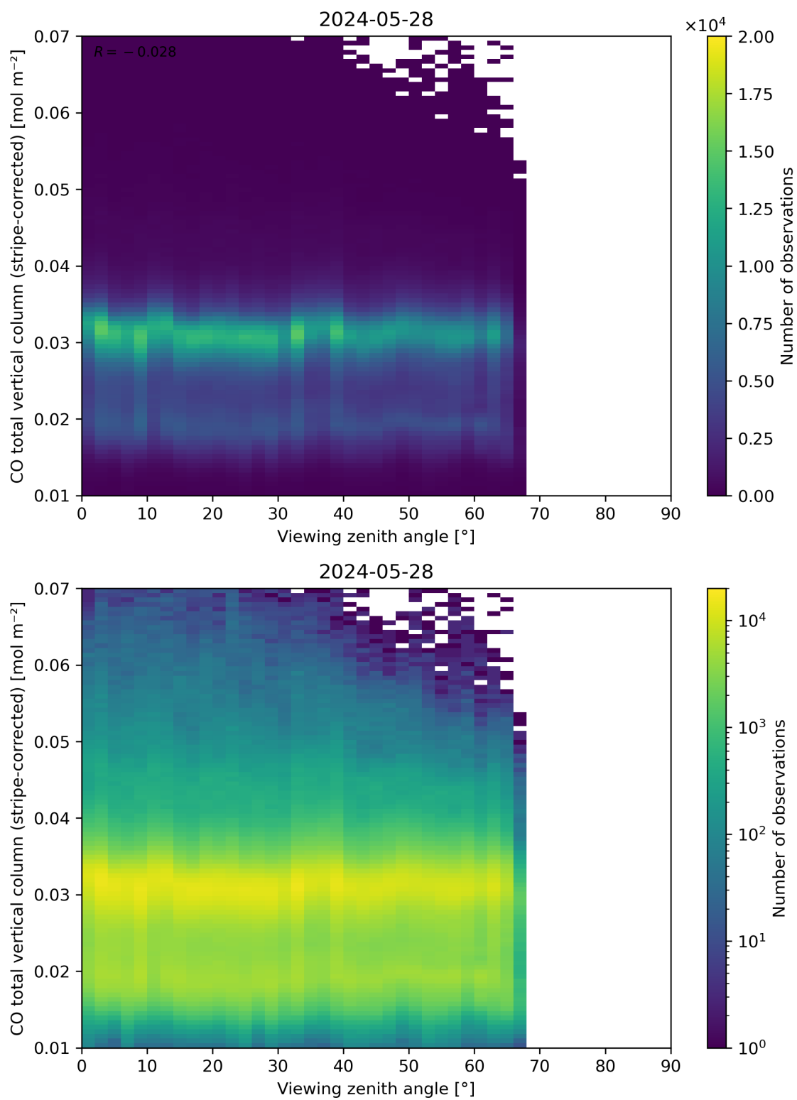
Figure 70: Scatter density plot of “Viewing zenith angle” against “CO total vertical column (stripe-corrected)” for 2024-05-28 to 2024-05-29.
