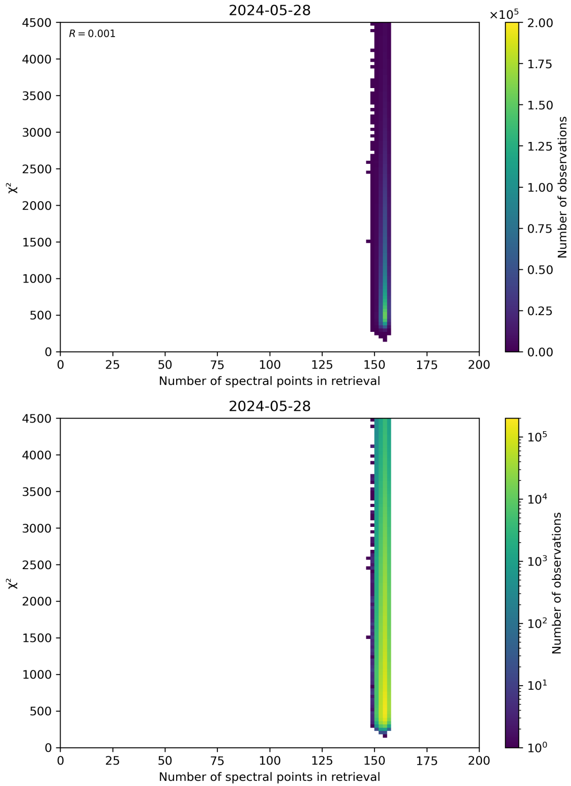
Figure 58: Scatter density plot of “Number of spectral points in retrieval” against “ \chi^2 ” for 2024-05-28 to 2024-05-29.
