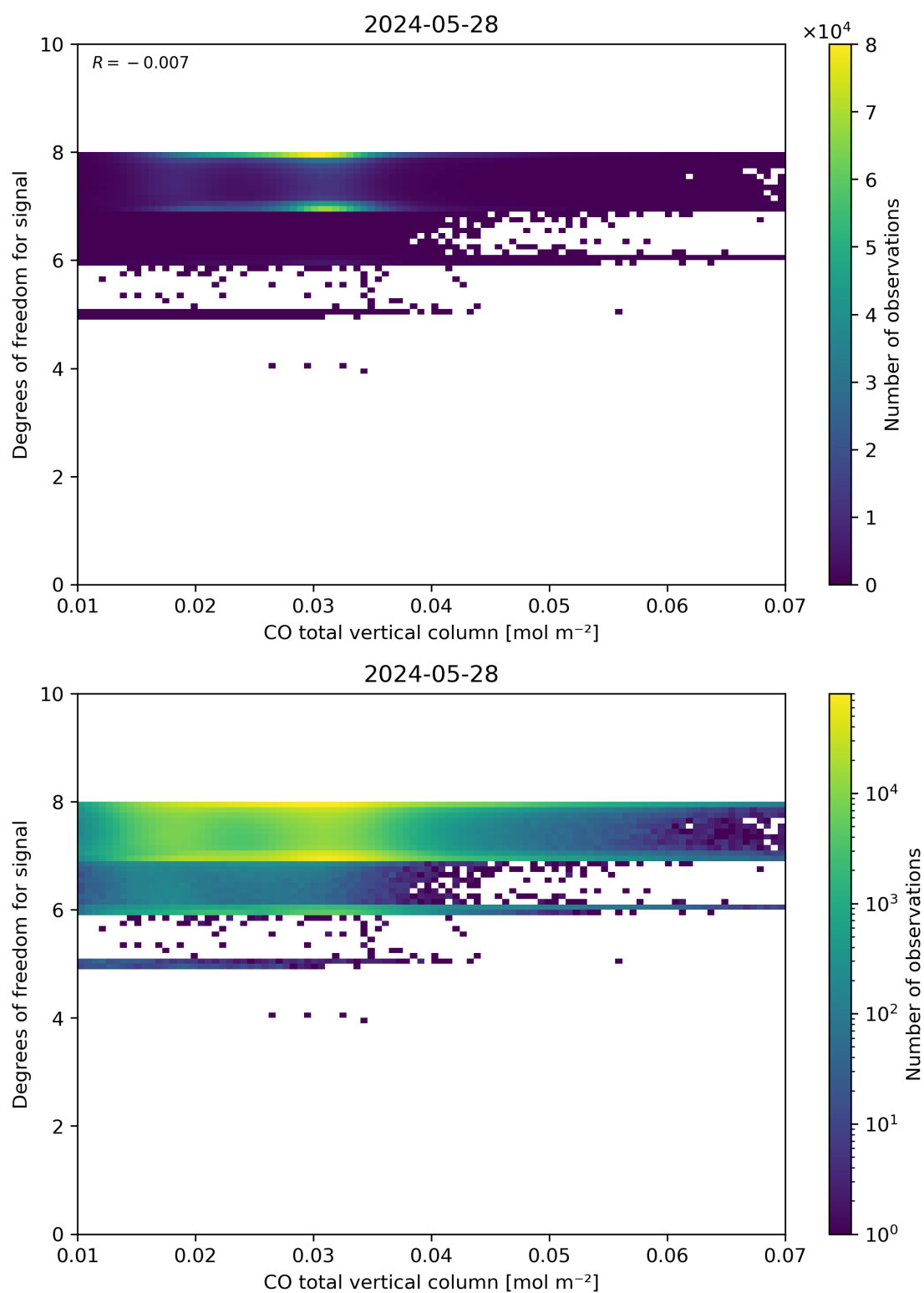
Figure 41: Scatter density plot of “CO total vertical column” against “Degrees of freedom for signal” for 2024-05-28 to 2024-05-29.
