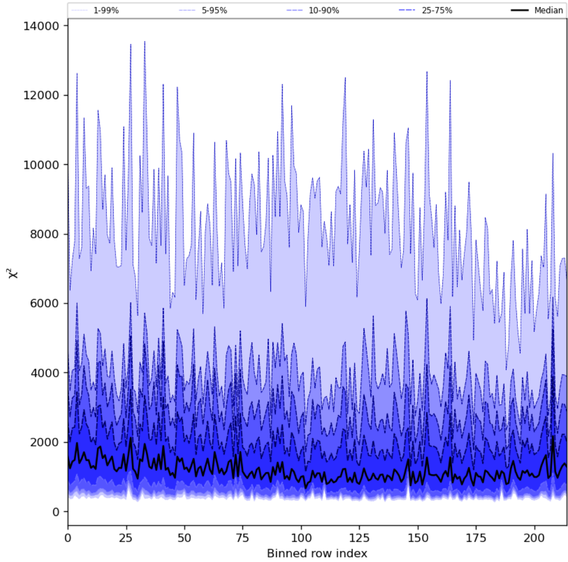
Figure 30: Along track statistics of “ \chi^2 ” for 2024-05-28 to 2024-05-29
