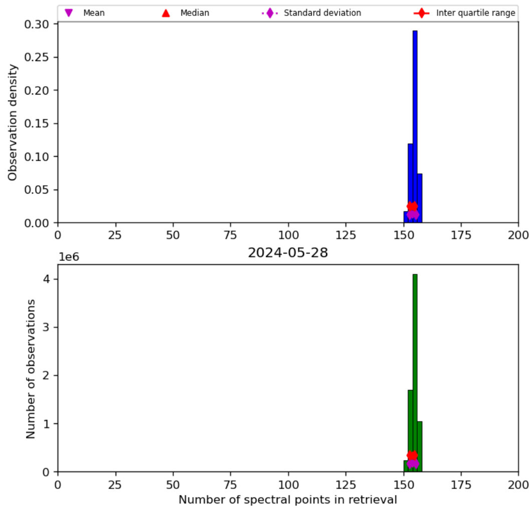
Figure 21: Histogram of “Number of spectral points in retrieval” for 2024-05-28 to 2024-05-29
