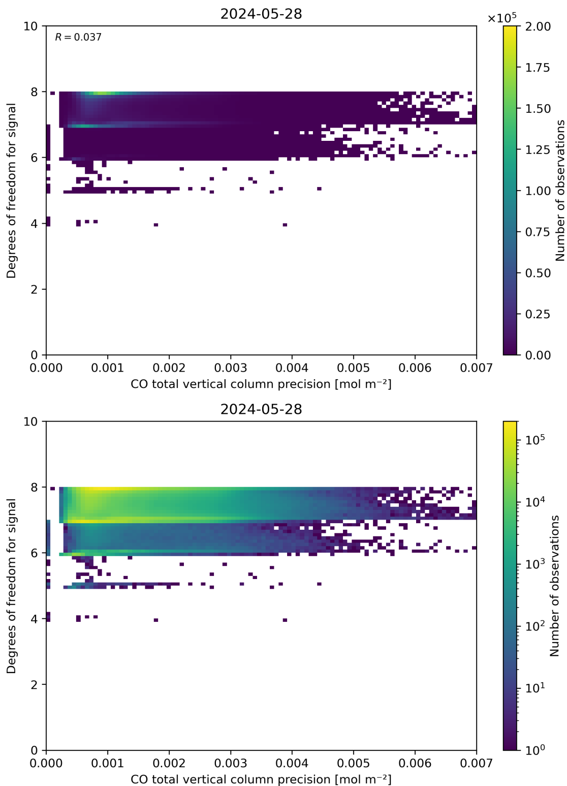
Figure 45: Scatter density plot of “CO total vertical column precision” against “Degrees of freedom for signal” for 2024-05-28 to 2024-05-29.
