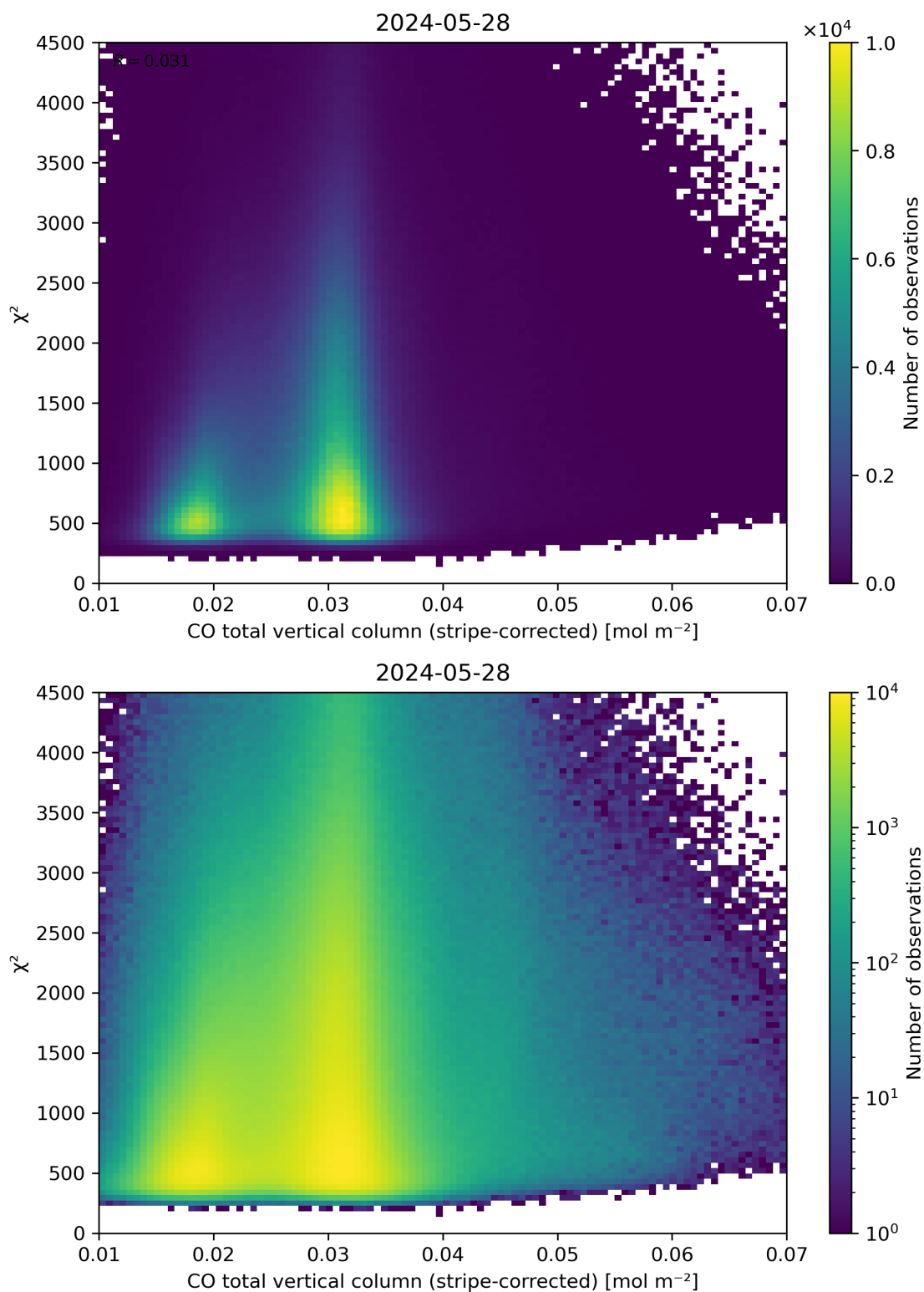
Figure 37: Scatter density plot of “CO total vertical column (stripe-corrected)” against “ \chi^2 ” for 2024-05-28 to 2024-05-29.
