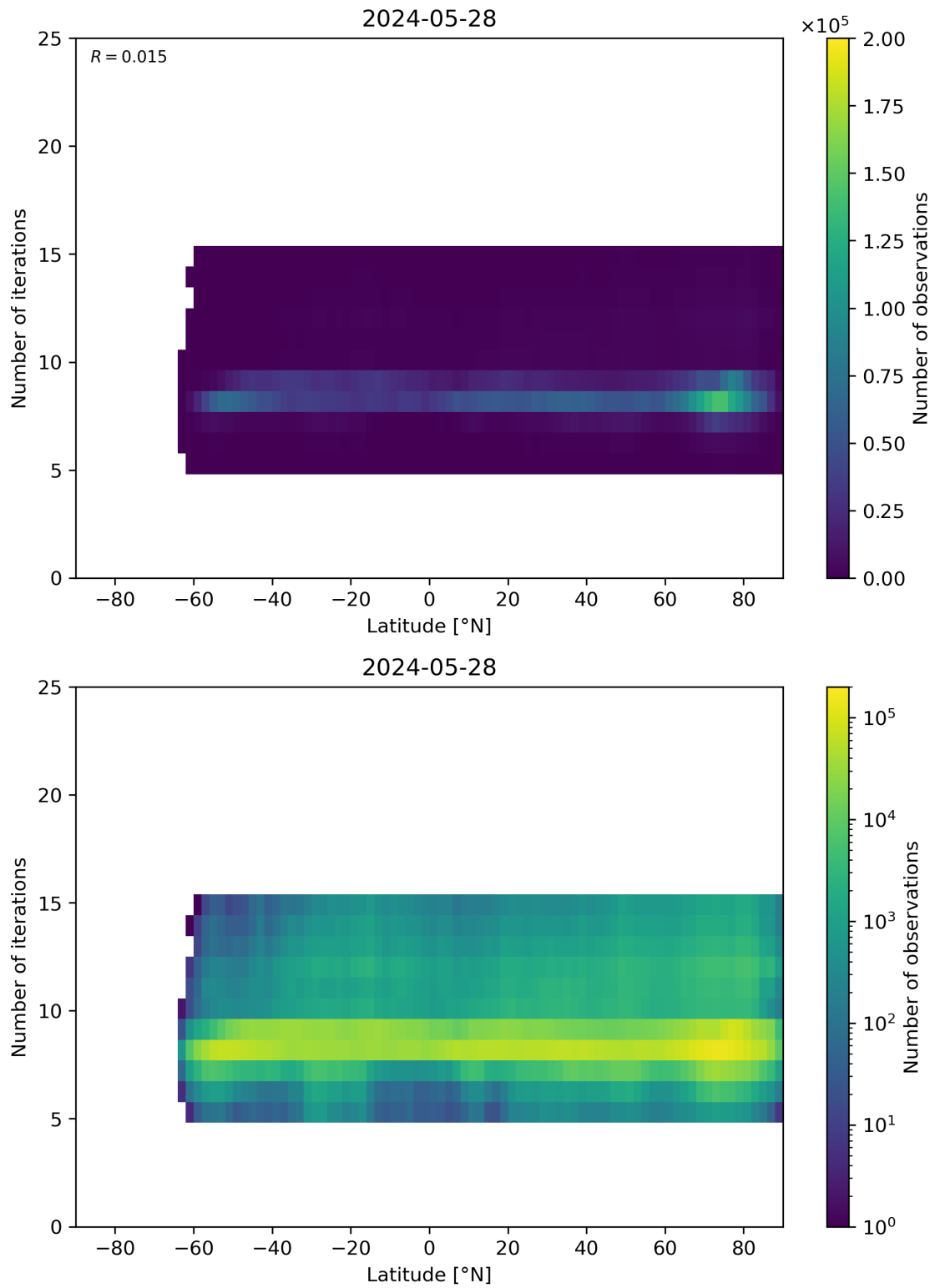
Figure 56: Scatter density plot of “Latitude” against “Number of iterations” for 2024-05-28 to 2024-05-29.
