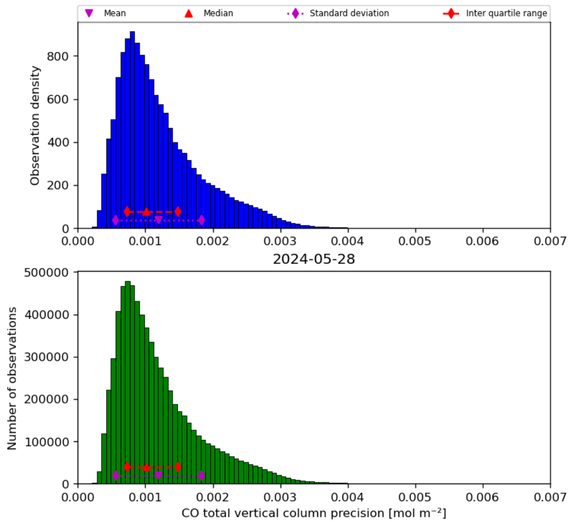
Figure 20: Histogram of “CO total vertical column precision” for 2024-05-28 to 2024-05-29
