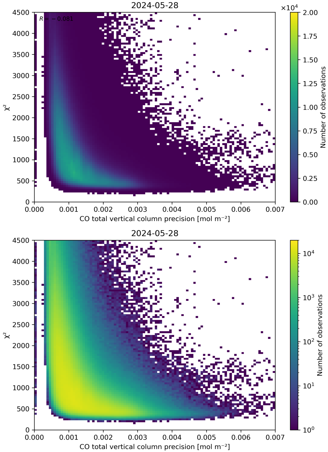
Figure 44: Scatter density plot of “CO total vertical column precision” against “ \chi^2 ” for 2024-05-28 to 2024-05-29.
