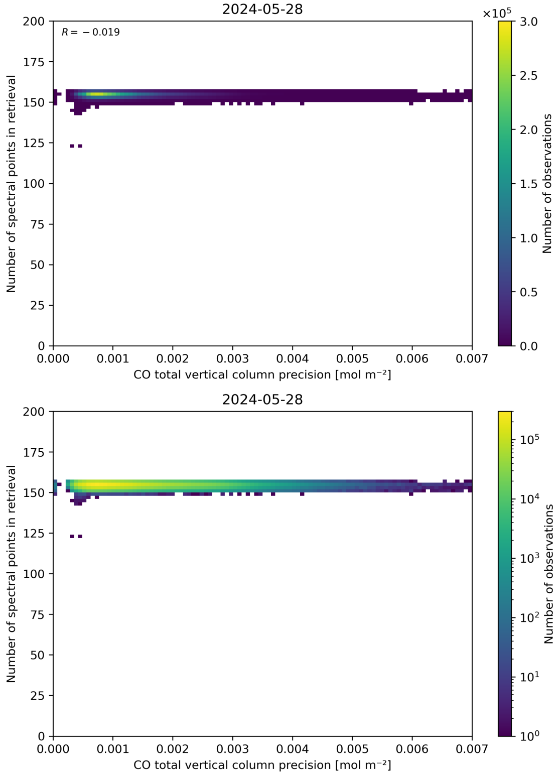
Figure 47: Scatter density plot of “CO total vertical column precision” against “Number of spectral points in retrieval” for 2024-05-28 to 2024-05-29.
