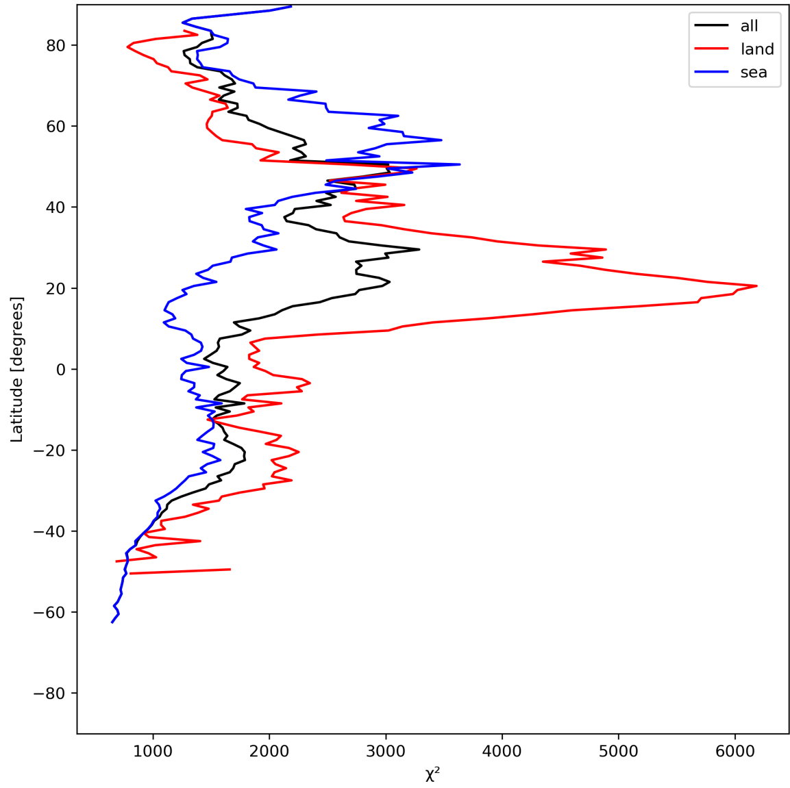
Figure 14: Zonal average of “ \chi^2 ” for 2024-05-28 to 2024-05-29.
