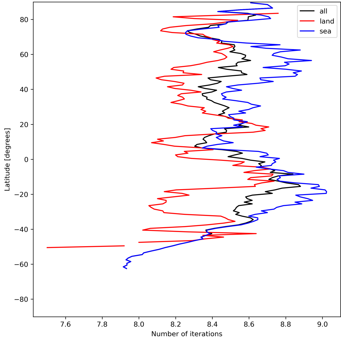
Figure 16: Zonal average of “Number of iterations” for 2024-05-28 to 2024-05-29.
