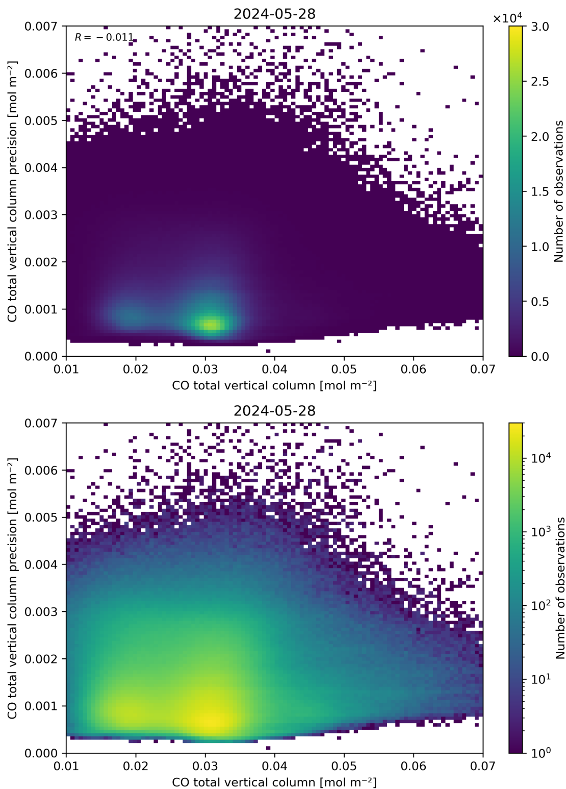
Figure 34: Scatter density plot of “CO total vertical column” against “CO total vertical column precision” for 2024-05-28 to 2024-05-29.
