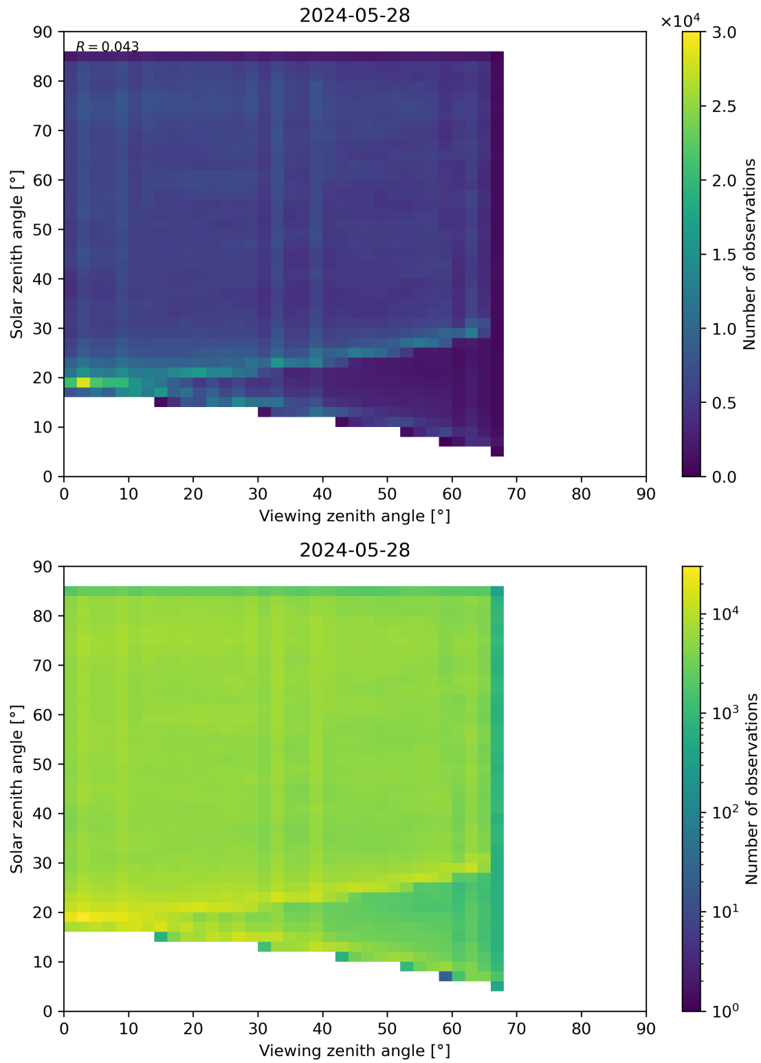
Figure 77: Scatter density plot of “Viewing zenith angle” against “Solar zenith angle” for 2024-05-28 to 2024-05-29.
