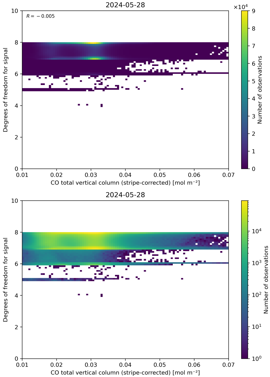
Figure 38: Scatter density plot of “CO total vertical column (stripe-corrected)” against “Degrees of freedom for signal” for 2024-05-28 to 2024-05-29.
