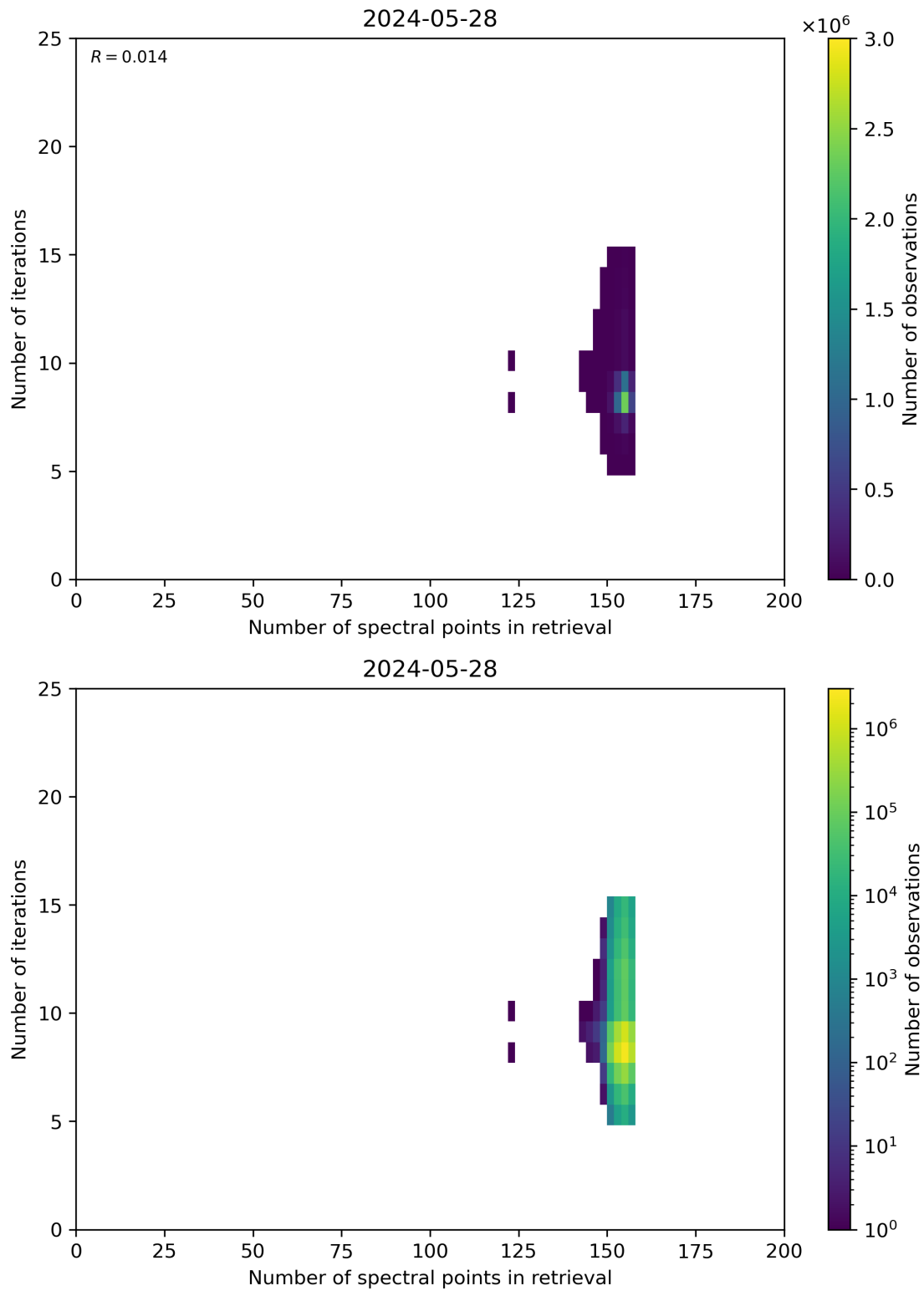
Figure 60: Scatter density plot of “Number of spectral points in retrieval” against “Number of iterations” for 2024-05-28 to 2024-05-29.
