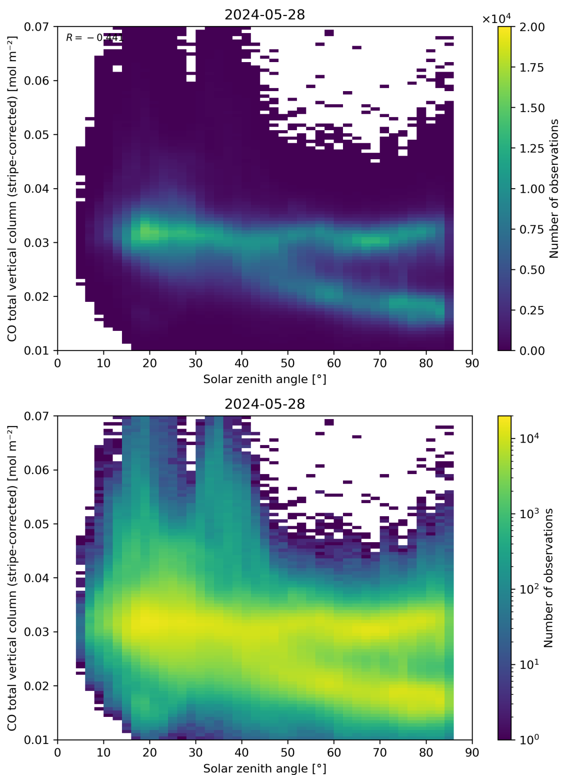
Figure 62: Scatter density plot of “Solar zenith angle” against “CO total vertical column (stripe-corrected)” for 2024-05-28 to 2024-05-29.
