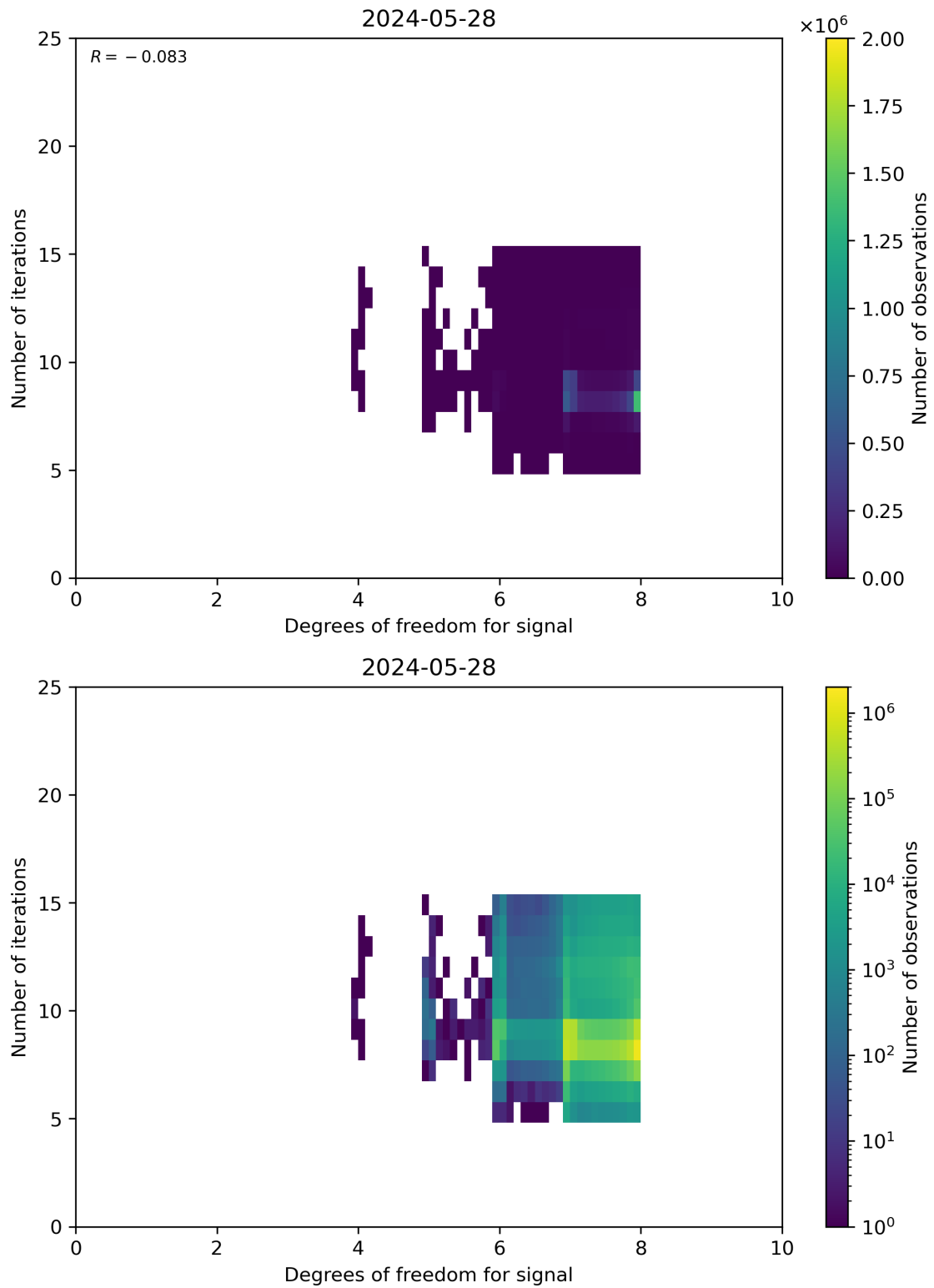
Figure 50: Scatter density plot of “Degrees of freedom for signal” against “Number of iterations” for 2024-05-28 to 2024-05-29.
