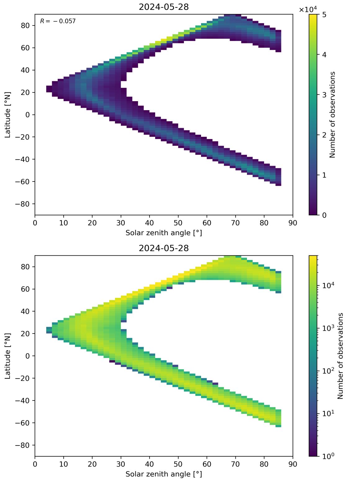
Figure 66: Scatter density plot of “Solar zenith angle” against “Latitude” for 2024-05-28 to 2024-05-29.
