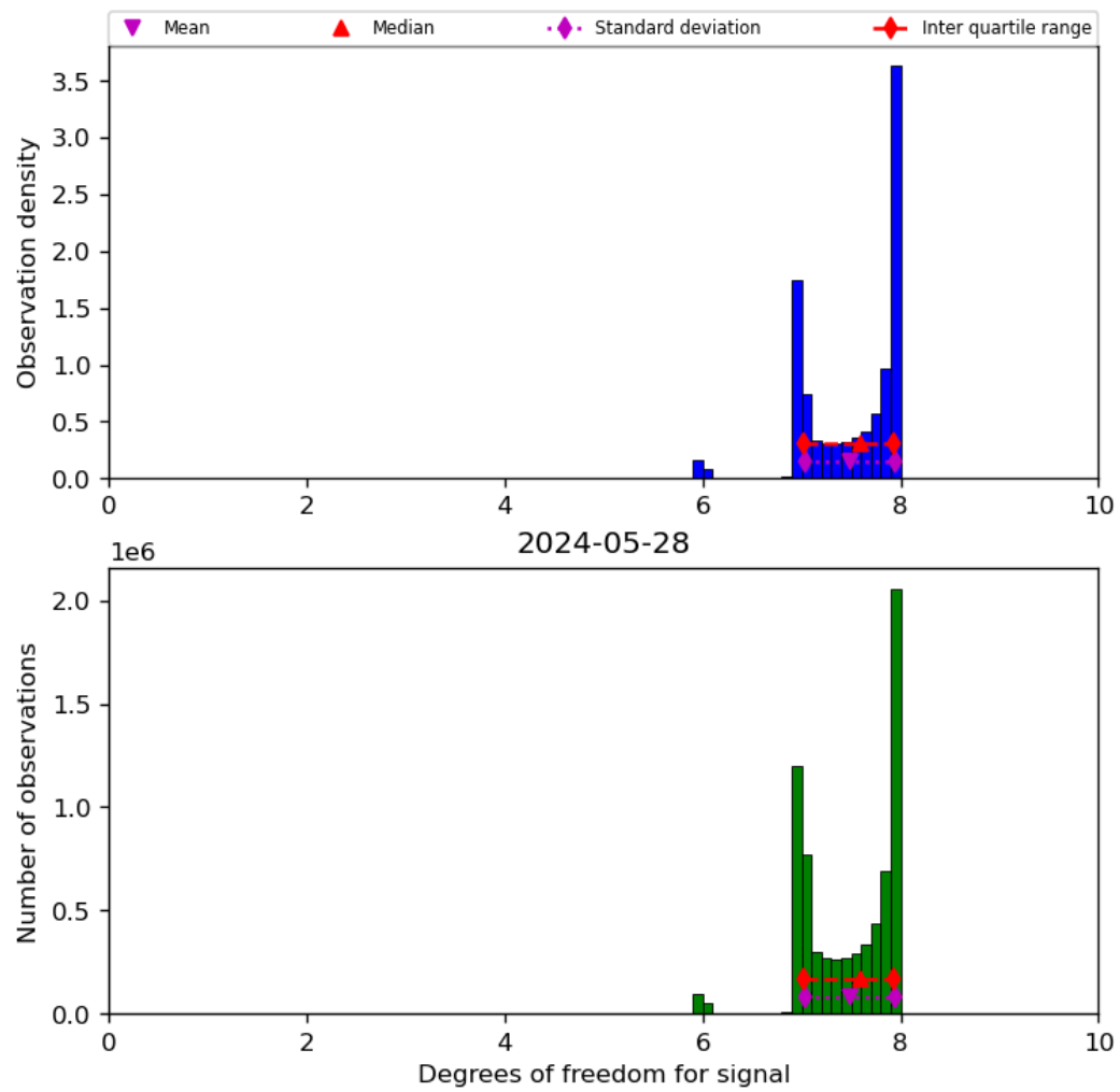
Figure 23: Histogram of “Degrees of freedom for signal” for 2024-05-28 to 2024-05-29
