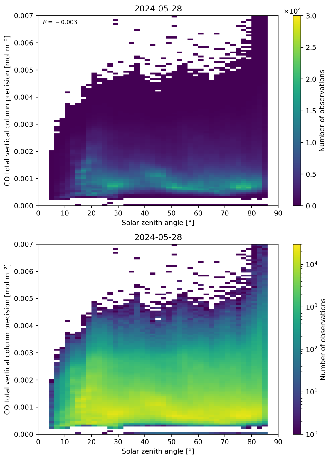
Figure 63: Scatter density plot of “Solar zenith angle” against “CO total vertical column precision” for 2024-05-28 to 2024-05-29.
