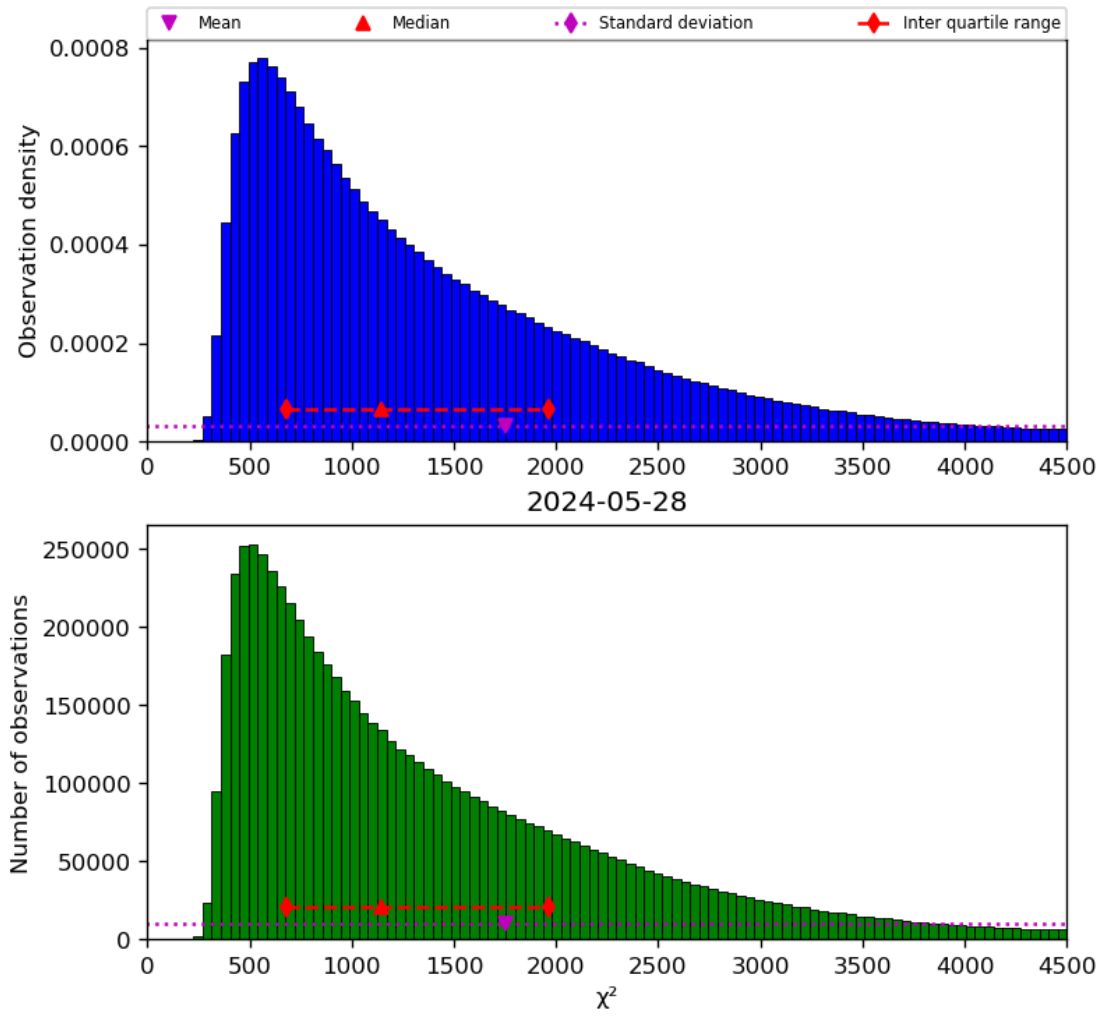
Figure 22: Histogram of “ \chi^2 ” for 2024-05-28 to 2024-05-29
