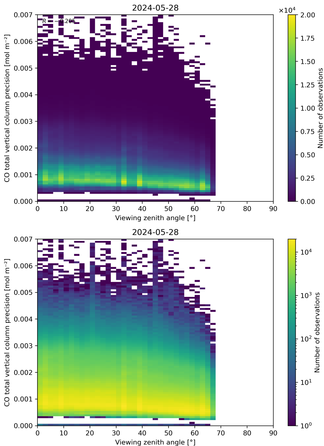
Figure 71: Scatter density plot of “Viewing zenith angle” against “CO total vertical column precision” for 2024-05-28 to 2024-05-29.
