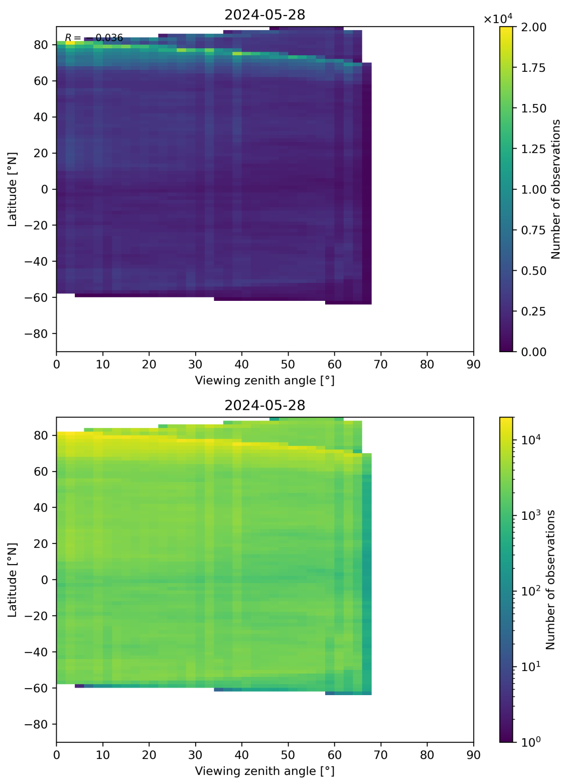
Figure 74: Scatter density plot of “Viewing zenith angle” against “Latitude” for 2024-05-28 to 2024-05-29.
