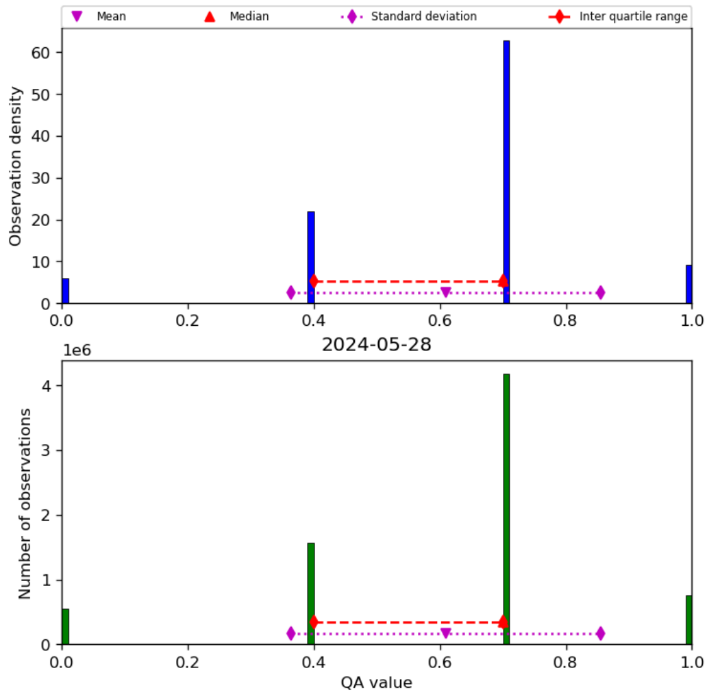
Figure 17: Histogram of “QA value” for 2024-05-28 to 2024-05-29
