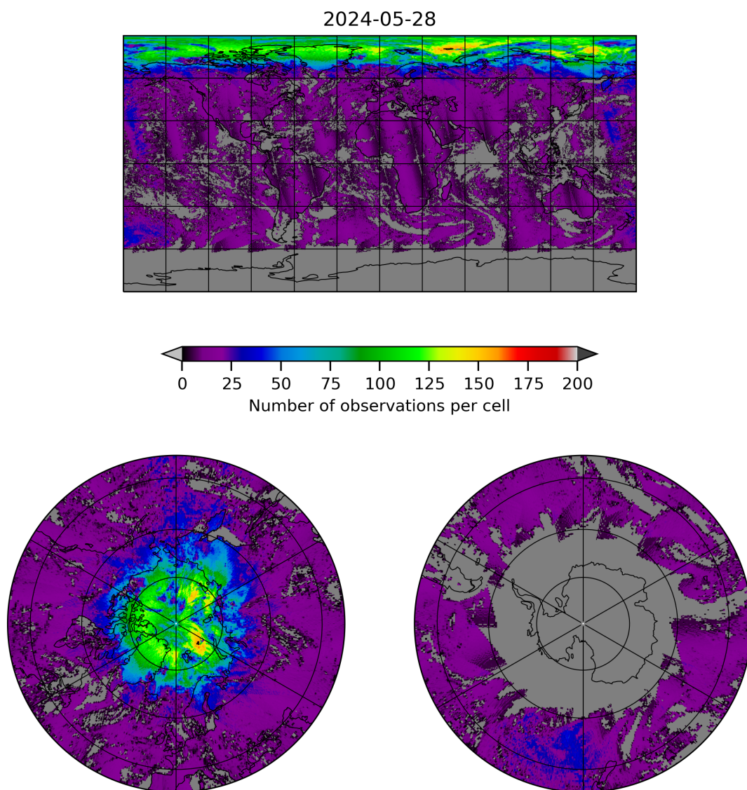
Figure 8: Map of the number of observations for 2024-05-28 to 2024-05-29
