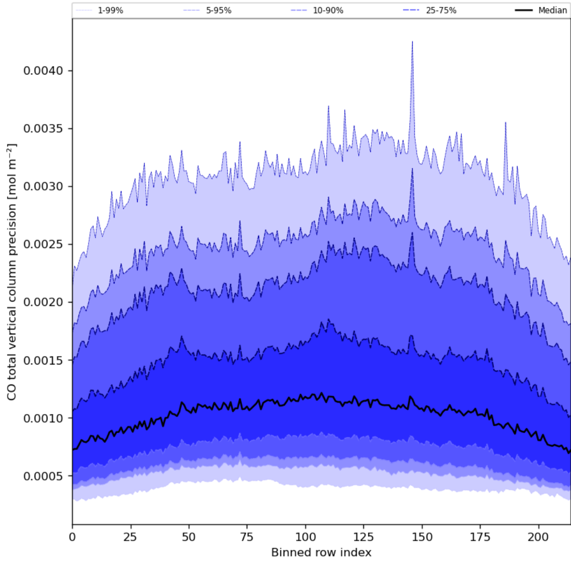
Figure 28: Along track statistics of “CO total vertical column precision” for 2024-05-28 to 2024-05-29
