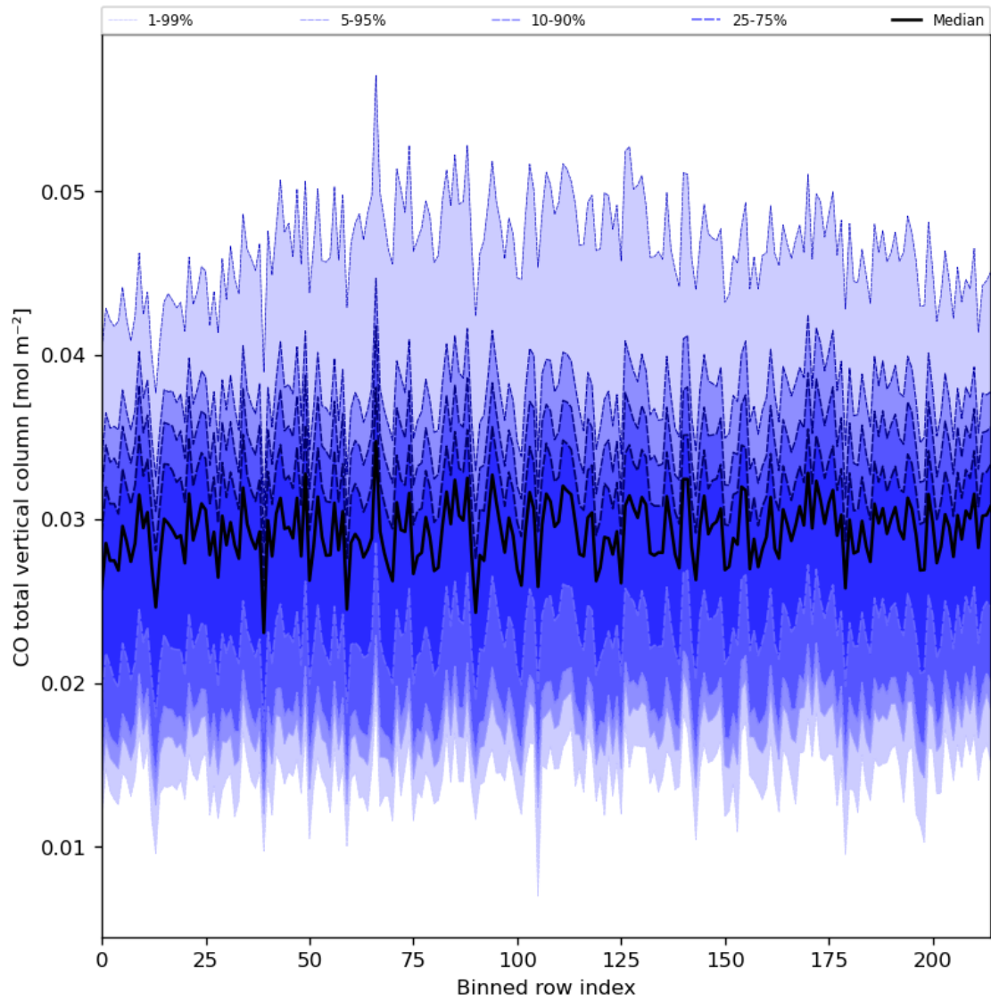
Figure 26: Along track statistics of “CO total vertical column” for 2024-05-28 to 2024-05-29
