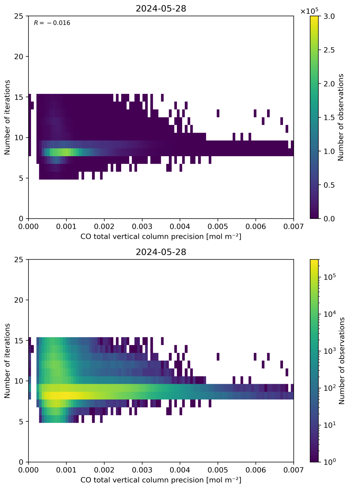
Figure 46: Scatter density plot of “CO total vertical column precision” against “Number of iterations” for 2024-05-28 to 2024-05-29.
