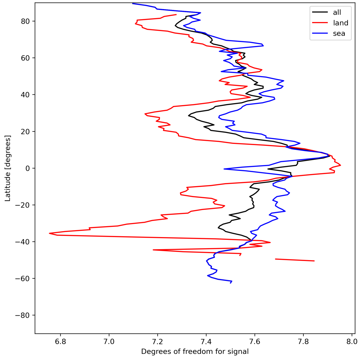
Figure 15: Zonal average of “Degrees of freedom for signal” for 2024-05-28 to 2024-05-29.
