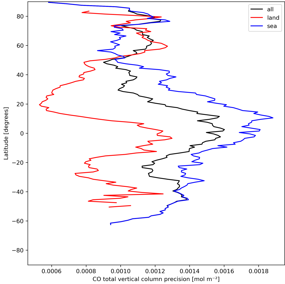
Figure 12: Zonal average of “CO total vertical column precision” for 2024-05-28 to 2024-05-29.
