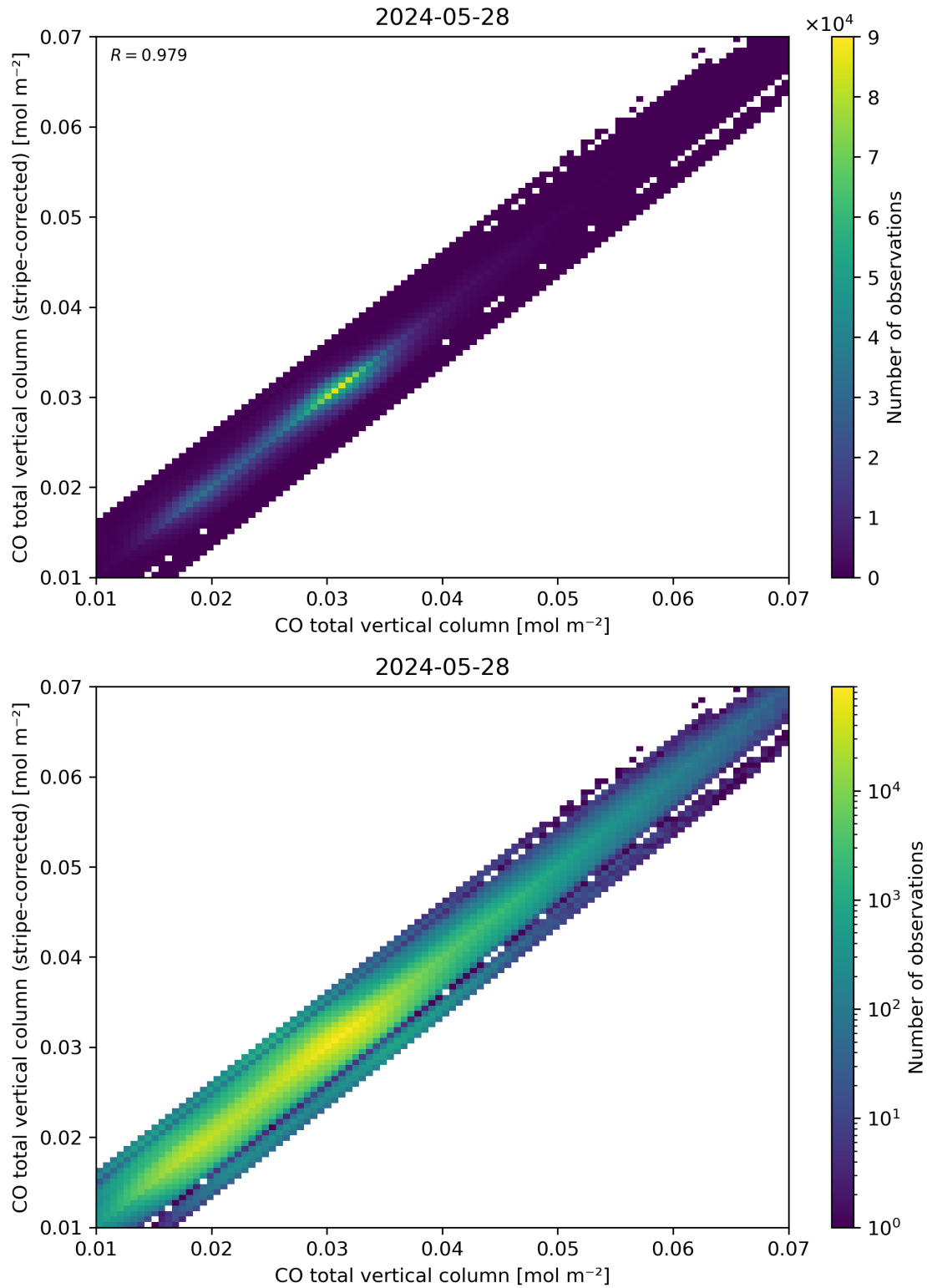
Figure 33: Scatter density plot of “CO total vertical column” against “CO total vertical column (stripe-corrected)” for 2024-05-28 to 2024-05-29.
