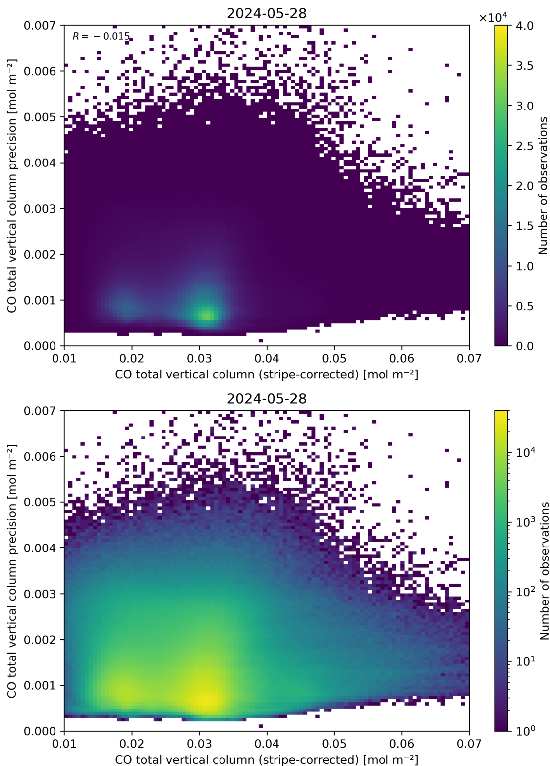
Figure 36: Scatter density plot of “CO total vertical column (stripe-corrected)” against “CO total vertical column precision” for 2024-05-28 to 2024-05-29.
