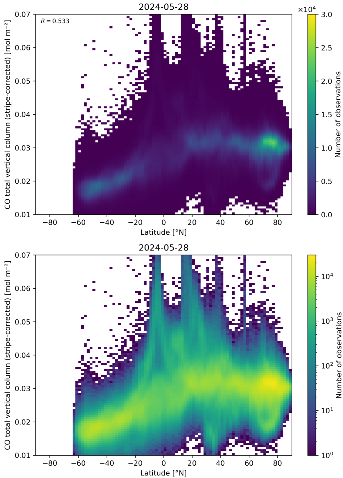
Figure 52: Scatter density plot of “Latitude” against “CO total vertical column (stripe-corrected)” for 2024-05-28 to 2024-05-29.
