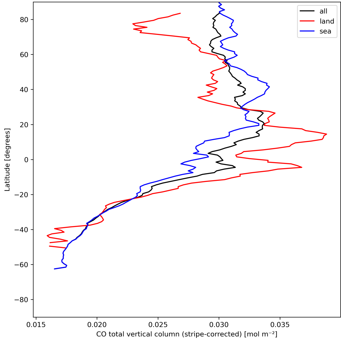
Figure 11: Zonal average of “CO total vertical column (stripe-corrected)” for 2024-05-28 to 2024-05-29.
