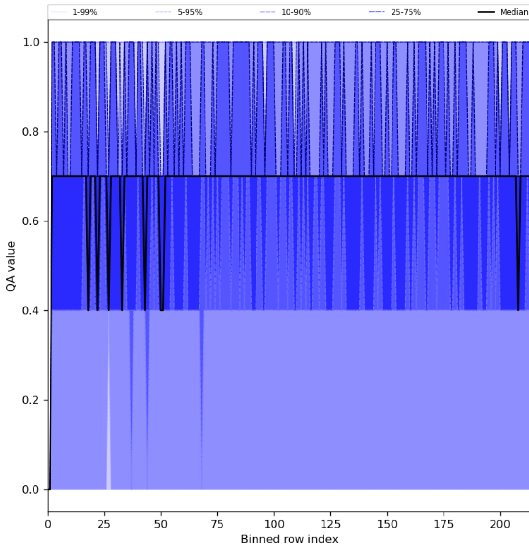
Figure 25: Along track statistics of “QA value” for 2024-05-28 to 2024-05-29
