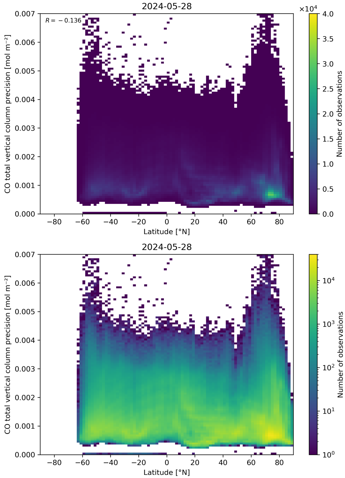
Figure 53: Scatter density plot of “Latitude” against “CO total vertical column precision” for 2024-05-28 to 2024-05-29.
