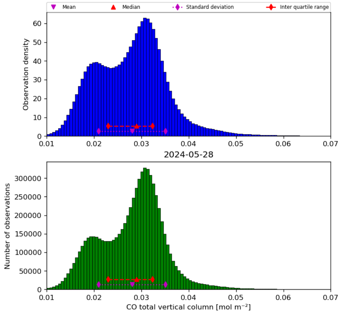
Figure 18: Histogram of “CO total vertical column” for 2024-05-28 to 2024-05-29
