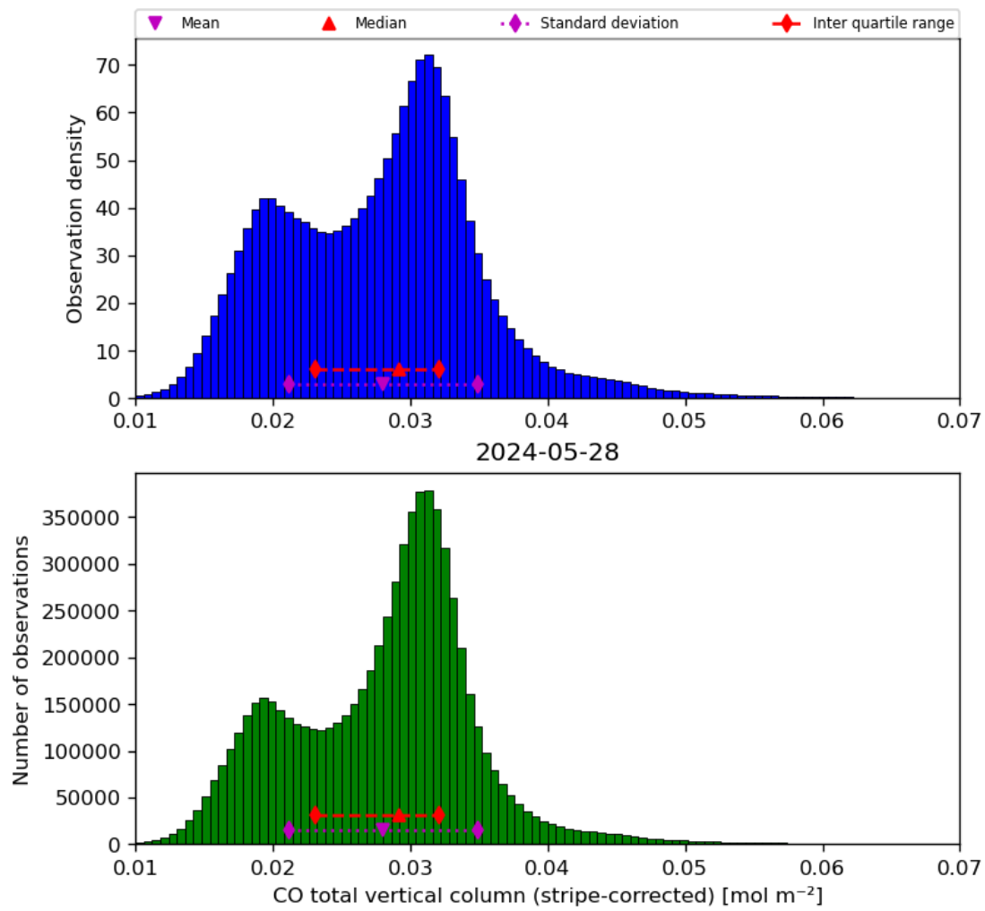
Figure 19: Histogram of “CO total vertical column (stripe-corrected)” for 2024-05-28 to 2024-05-29
