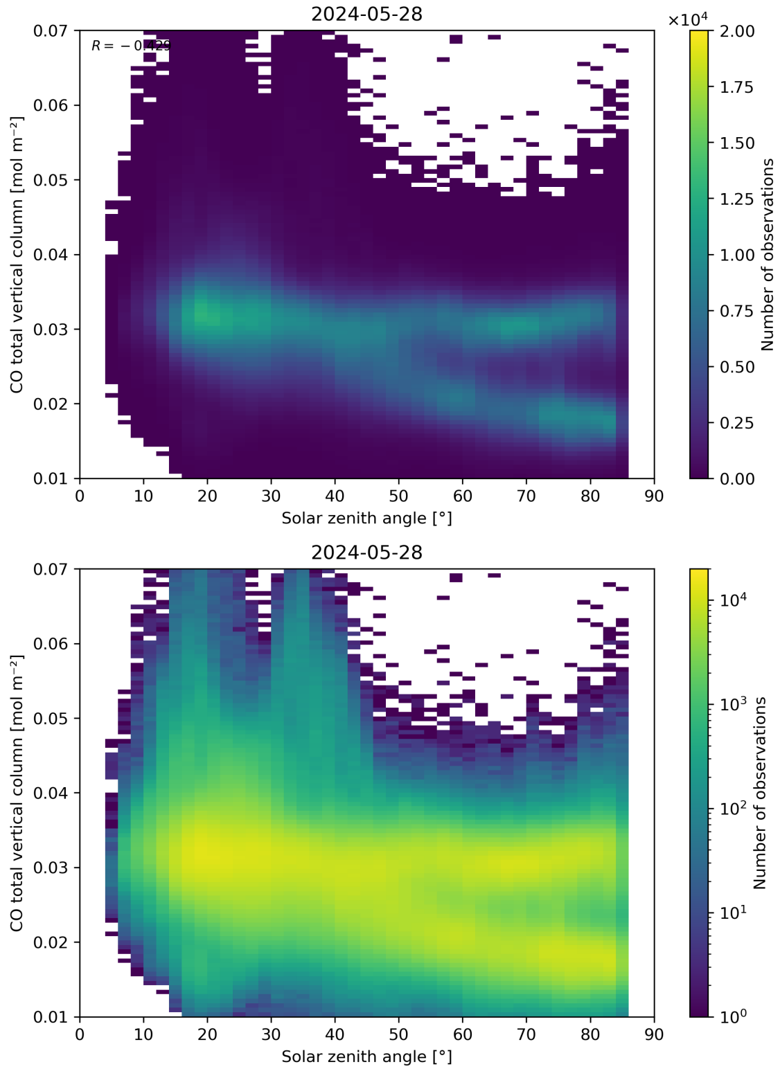
Figure 61: Scatter density plot of “Solar zenith angle” against “CO total vertical column” for 2024-05-28 to 2024-05-29.
