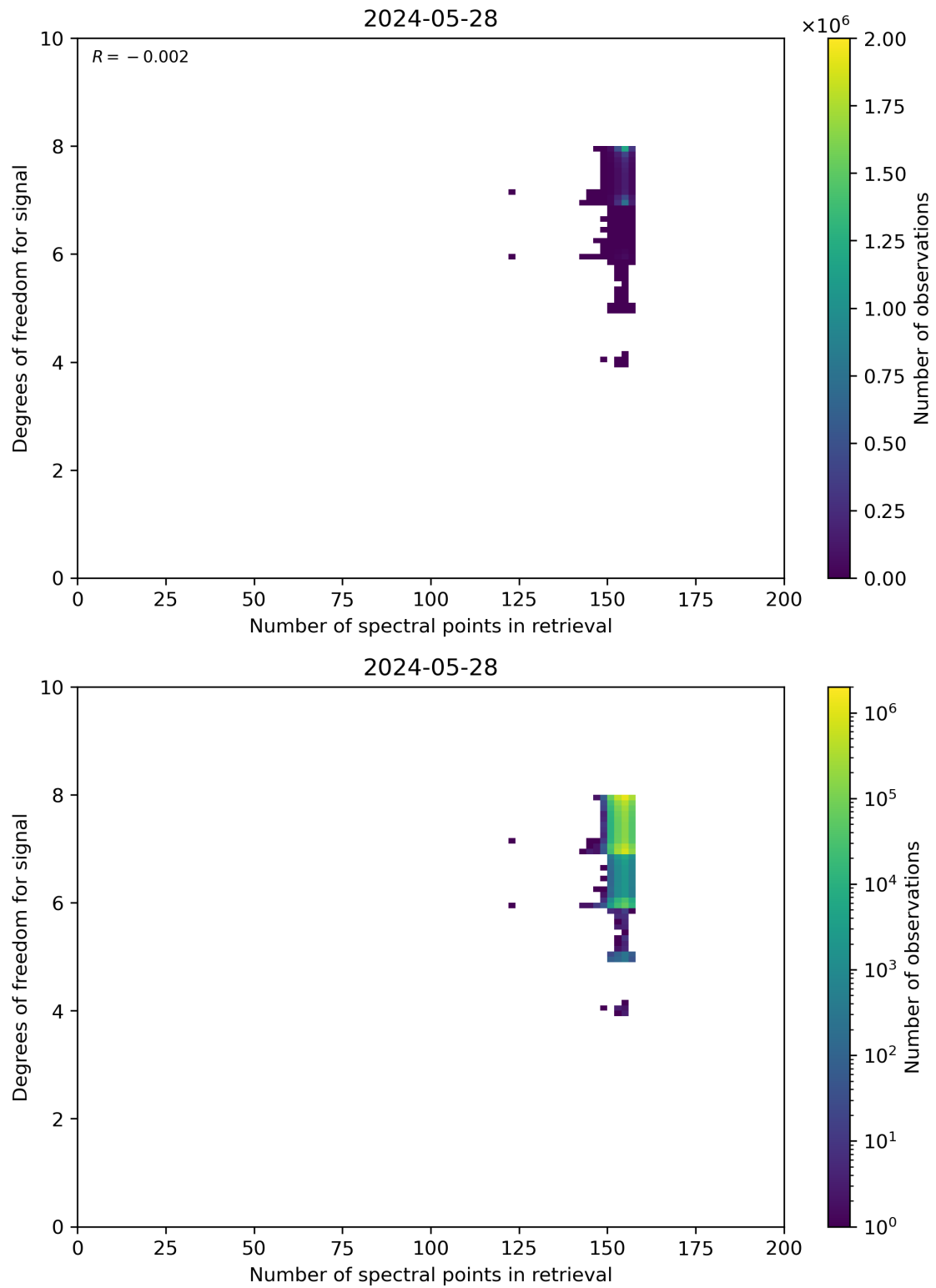
Figure 59: Scatter density plot of “Number of spectral points in retrieval” against “Degrees of freedom for signal” for 2024-05-28 to 2024-05-29.
