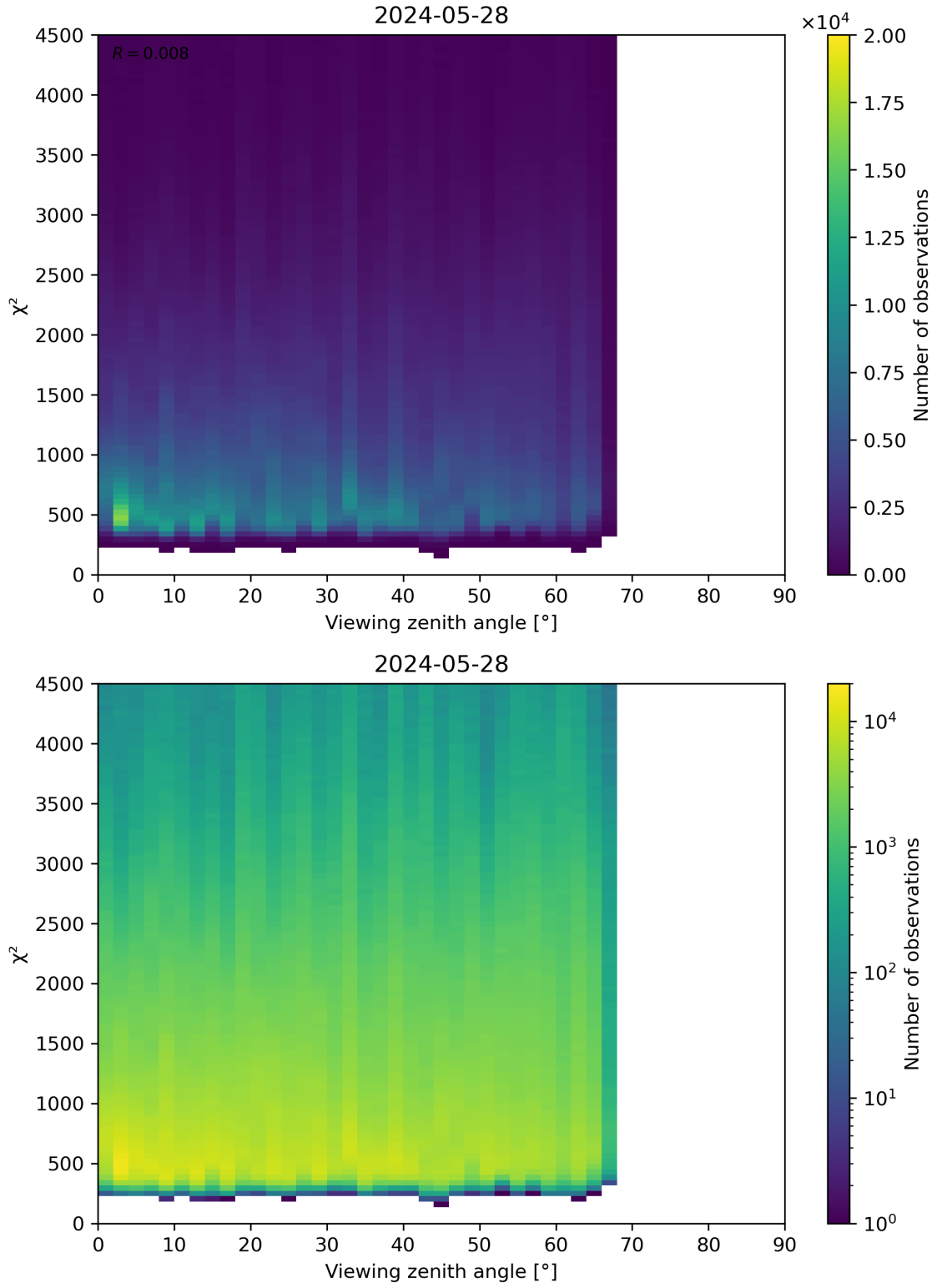
Figure 72: Scatter density plot of “Viewing zenith angle” against “ \chi^2 ” for 2024-05-28 to 2024-05-29.
