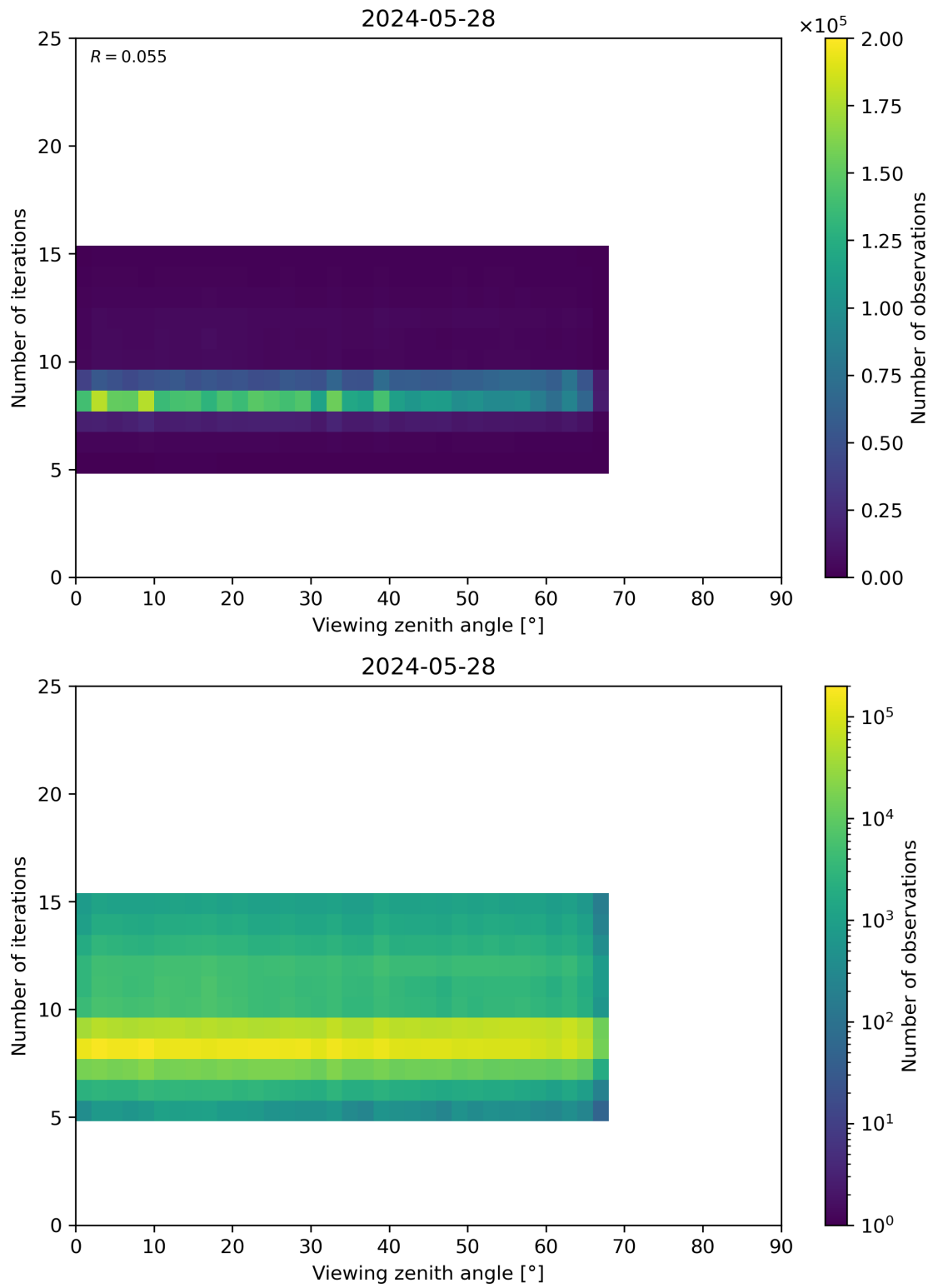
Figure 75: Scatter density plot of “Viewing zenith angle” against “Number of iterations” for 2024-05-28 to 2024-05-29.
