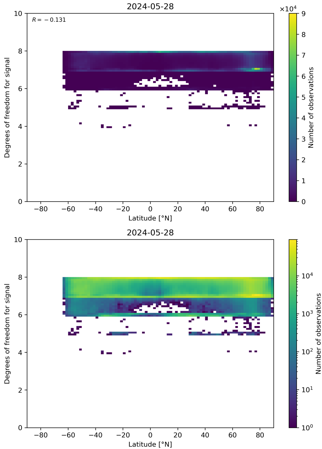
Figure 55: Scatter density plot of “Latitude” against “Degrees of freedom for signal” for 2024-05-28 to 2024-05-29.
