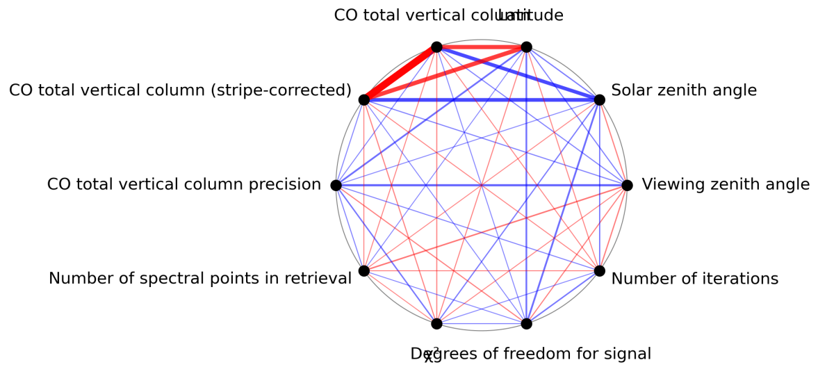
Figure 1: Map of correlation graph for 2024-05-28 to 2024-05-29.
