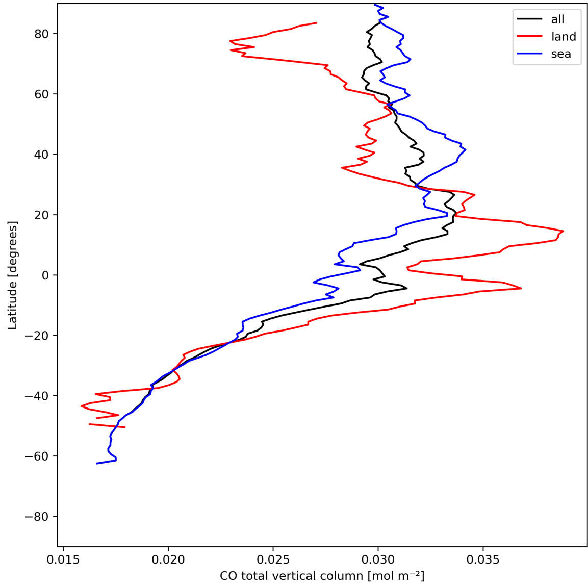
Figure 10: Zonal average of “CO total vertical column” for 2024-05-28 to 2024-05-29.
