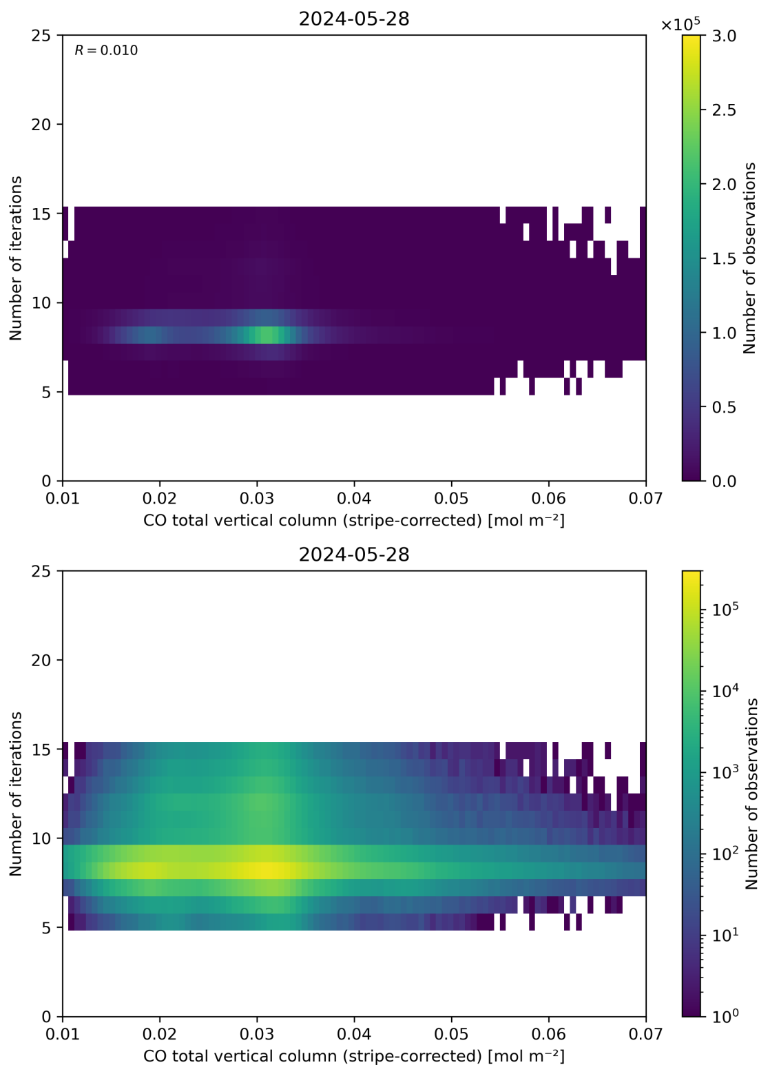
Figure 39: Scatter density plot of “CO total vertical column (stripe-corrected)” against “Number of iterations” for 2024-05-28 to 2024-05-29.
