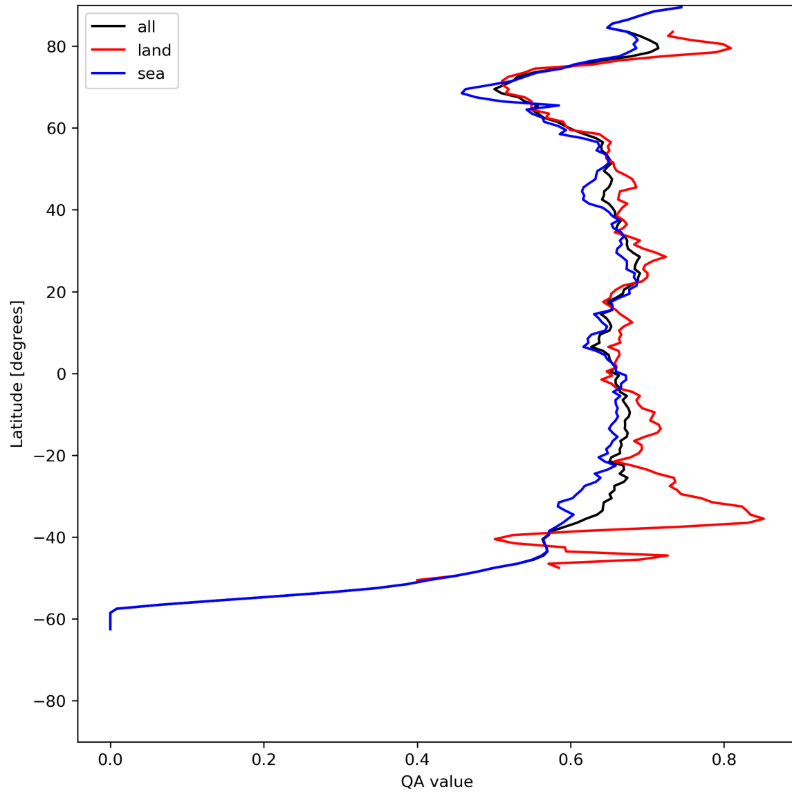
Figure 9: Zonal average of “QA value” for 2024-05-28 to 2024-05-29.
