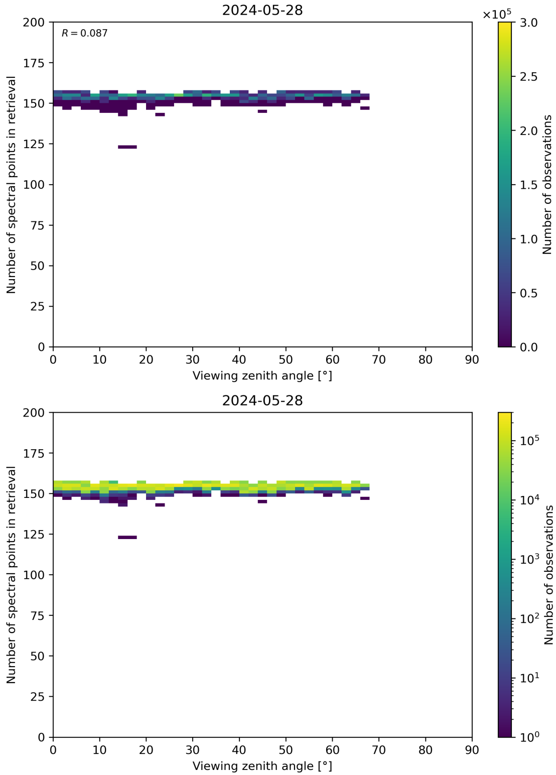
Figure 76: Scatter density plot of “Viewing zenith angle” against “Number of spectral points in retrieval” for 2024-05-28 to 2024-05-29.
