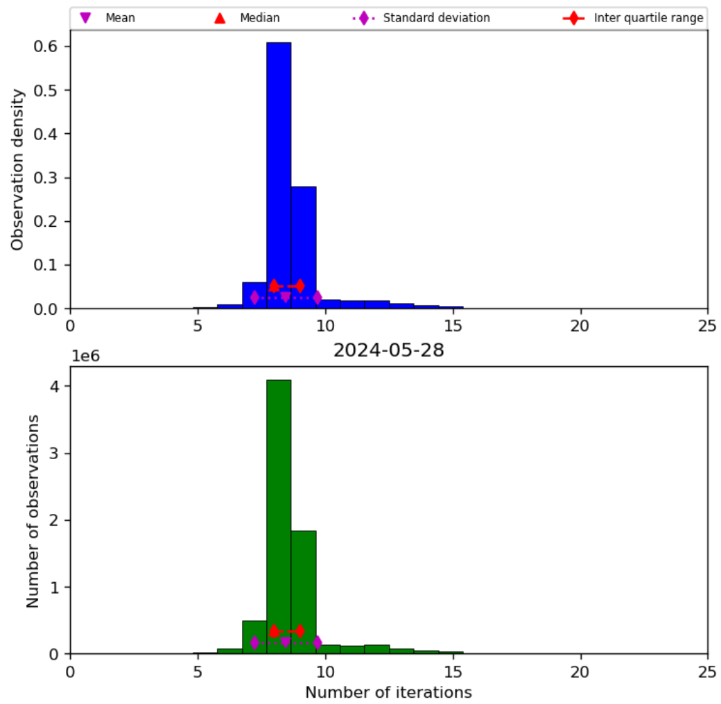
Figure 24: Histogram of “Number of iterations” for 2024-05-28 to 2024-05-29
