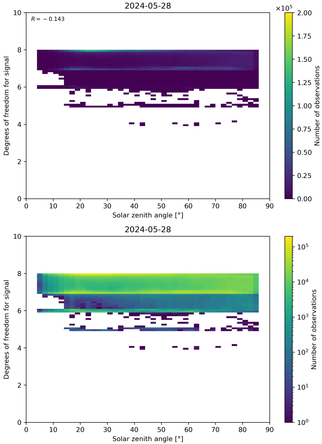
Figure 65: Scatter density plot of “Solar zenith angle” against “Degrees of freedom for signal” for 2024-05-28 to 2024-05-29.
