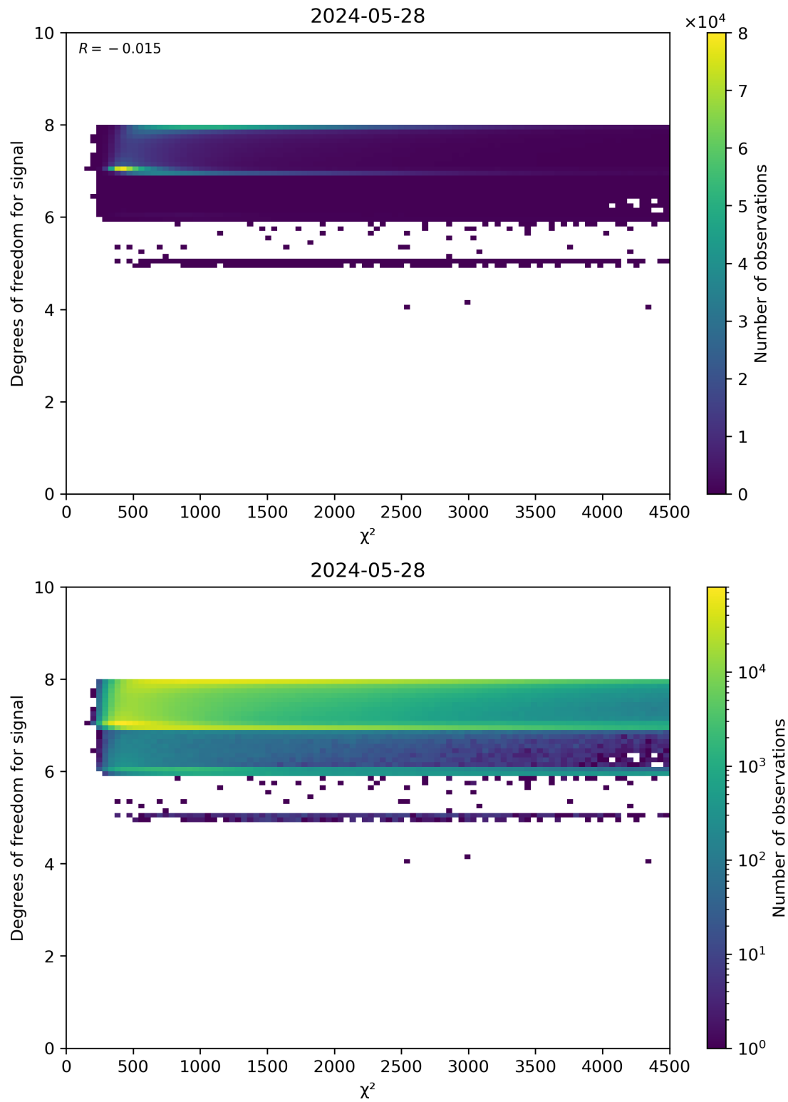
Figure 48: Scatter density plot of “ \chi^2 ” against “Degrees of freedom for signal” for 2024-05-28 to 2024-05-29.
