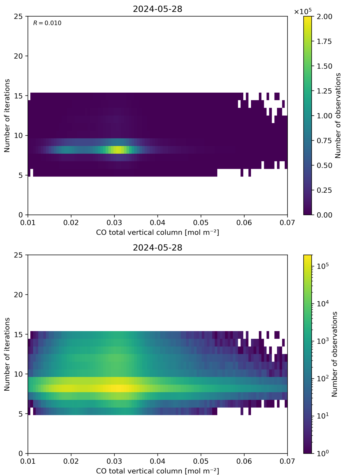
Figure 42: Scatter density plot of “CO total vertical column” against “Number of iterations” for 2024-05-28 to 2024-05-29.
