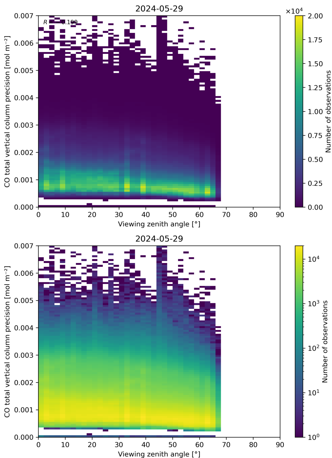
Figure 71: Scatter density plot of “Viewing zenith angle” against “CO total vertical column precision” for 2024-05-28 to 2024-05-30.
