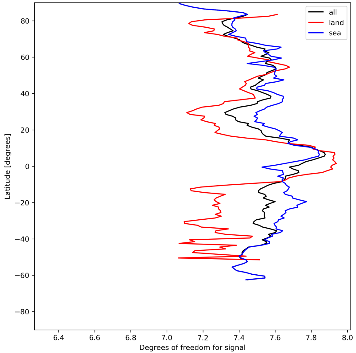
Figure 15: Zonal average of “Degrees of freedom for signal” for 2024-05-28 to 2024-05-30.
