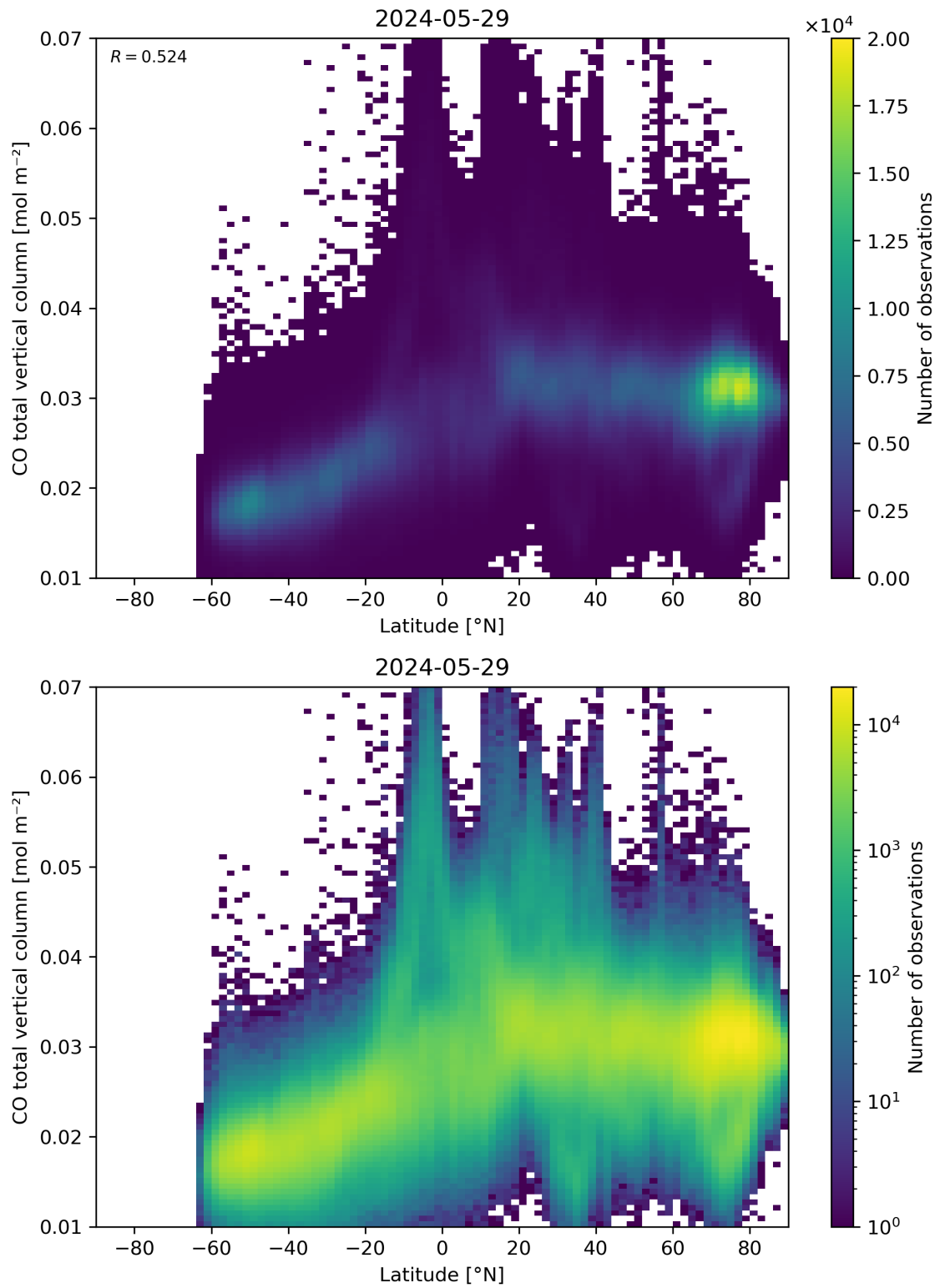
Figure 51: Scatter density plot of “Latitude” against “CO total vertical column” for 2024-05-28 to 2024-05-30.
