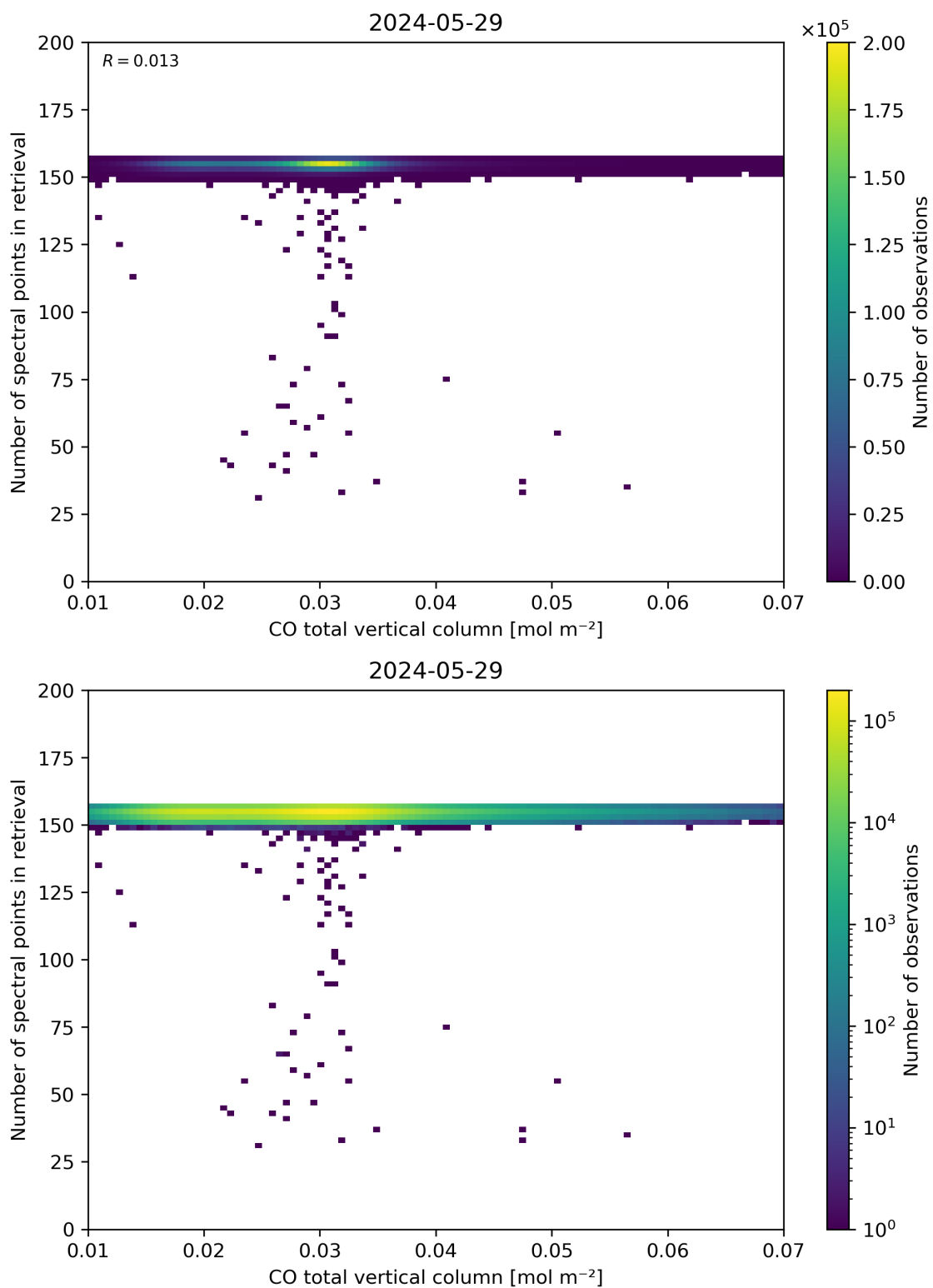
Figure 43: Scatter density plot of “CO total vertical column” against “Number of spectral points in retrieval” for 2024-05-28 to 2024-05-30.
