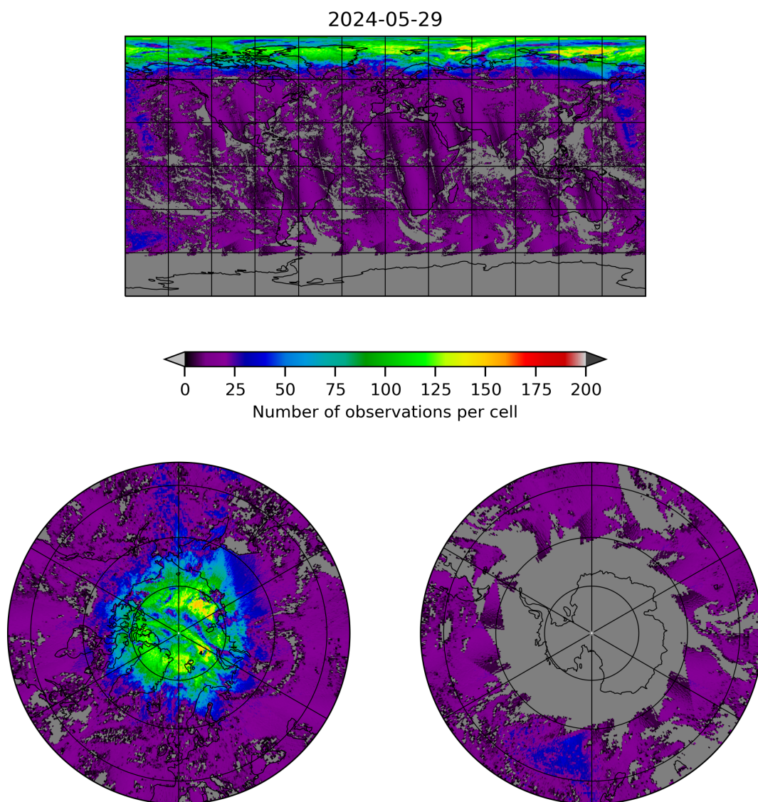
Figure 8: Map of the number of observations for 2024-05-28 to 2024-05-30
