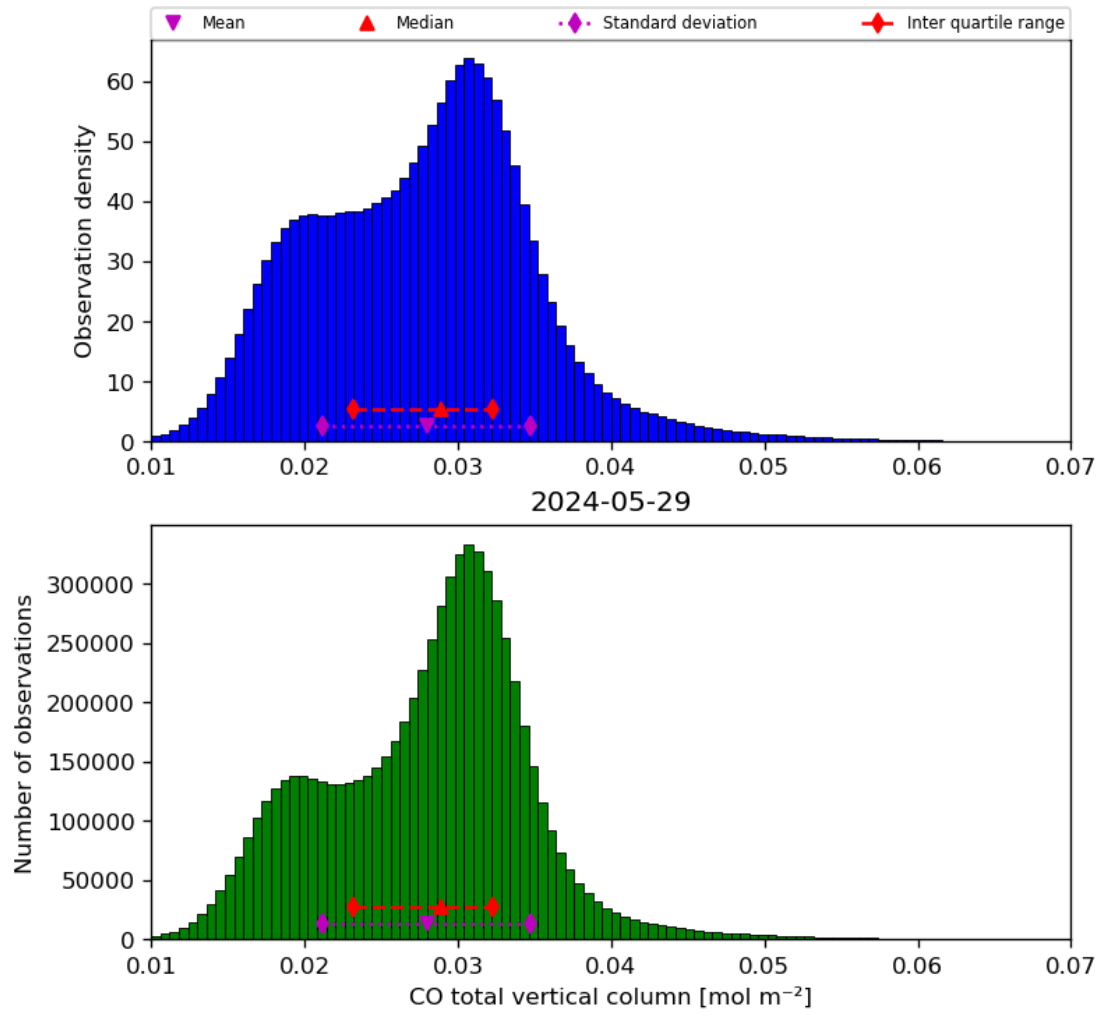
Figure 18: Histogram of “CO total vertical column” for 2024-05-28 to 2024-05-30
