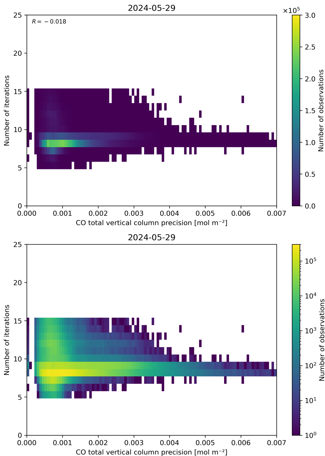
Figure 46: Scatter density plot of “CO total vertical column precision” against “Number of iterations” for 2024-05-28 to 2024-05-30.
