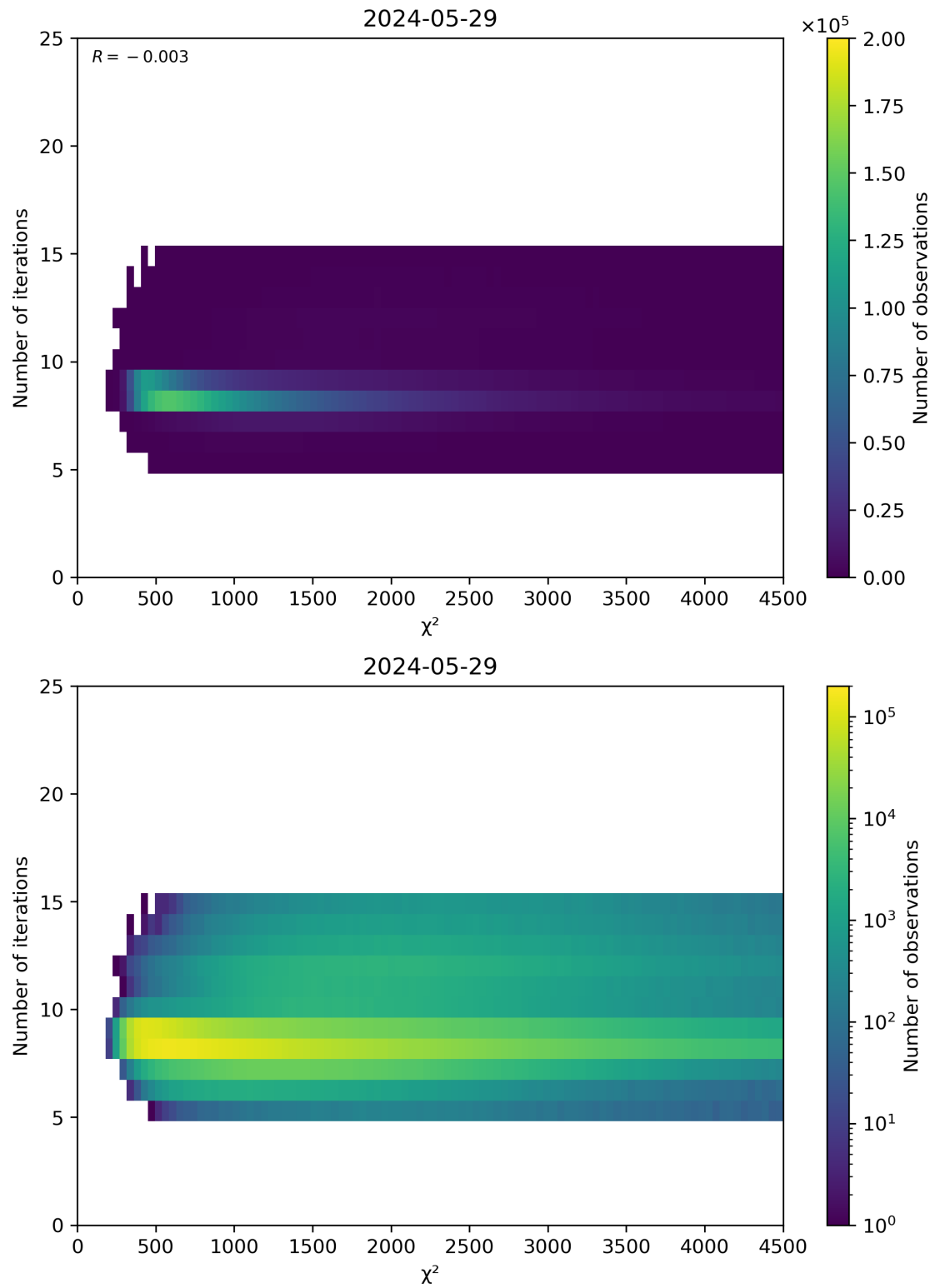
Figure 49: Scatter density plot of “ \chi^2 ” against “Number of iterations” for 2024-05-28 to 2024-05-30.
