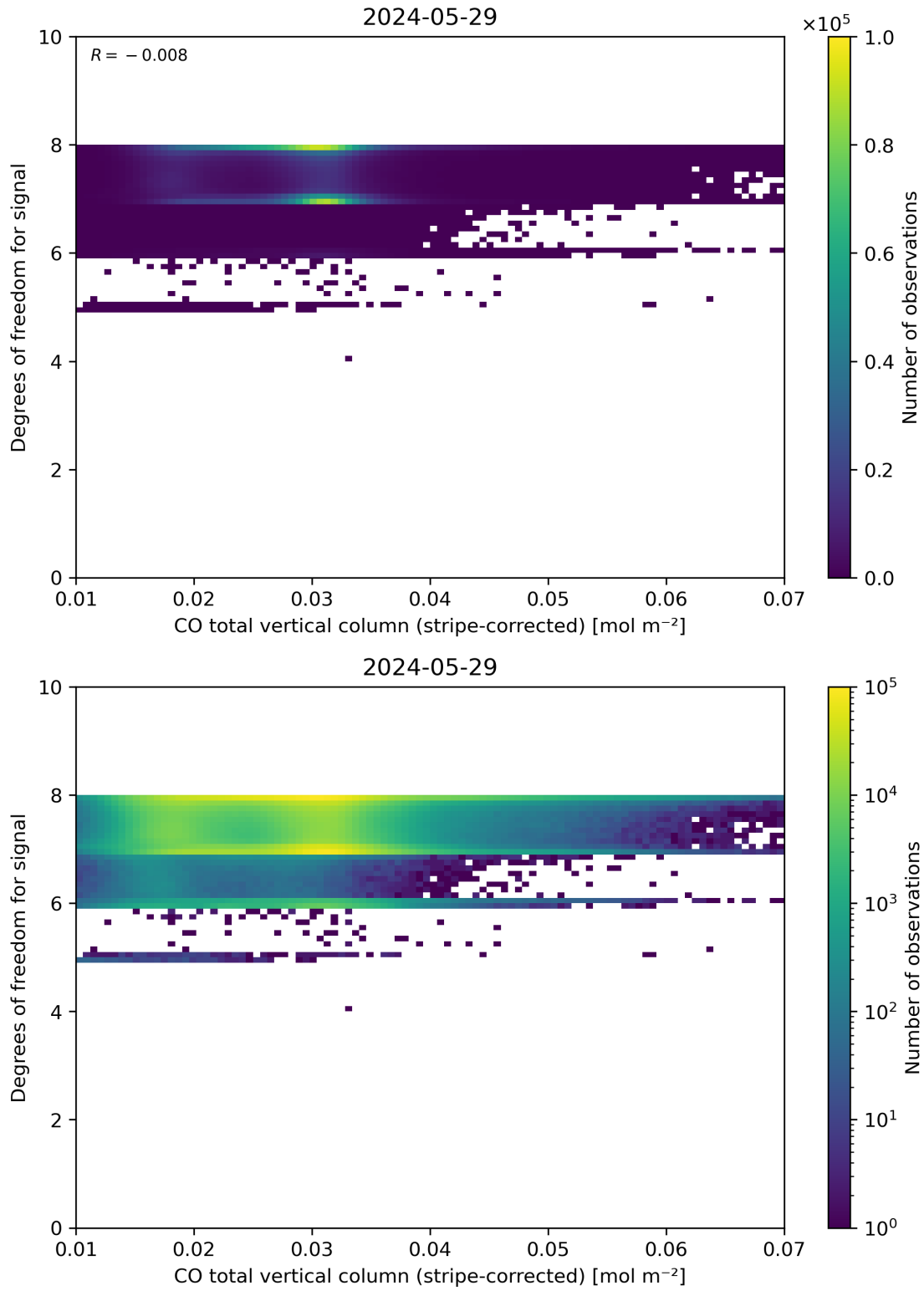
Figure 38: Scatter density plot of “CO total vertical column (stripe-corrected)” against “Degrees of freedom for signal” for 2024-05-28 to 2024-05-30.
