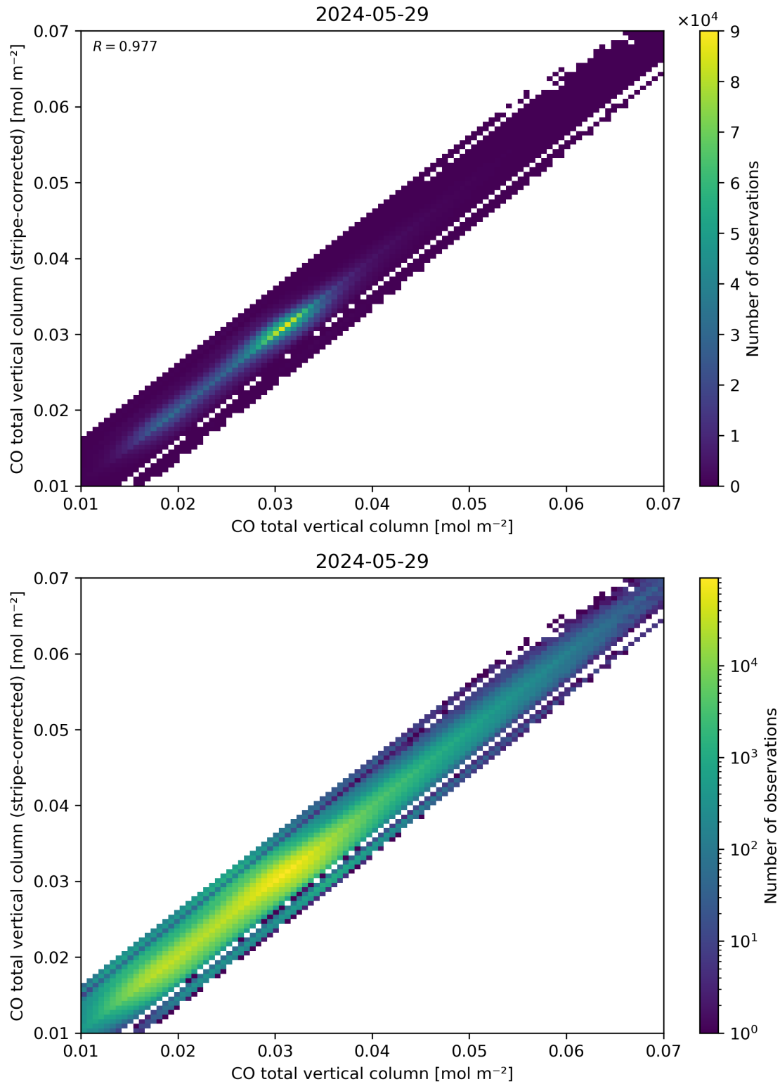
Figure 33: Scatter density plot of “CO total vertical column” against “CO total vertical column (stripe-corrected)” for 2024-05-28 to 2024-05-30.
