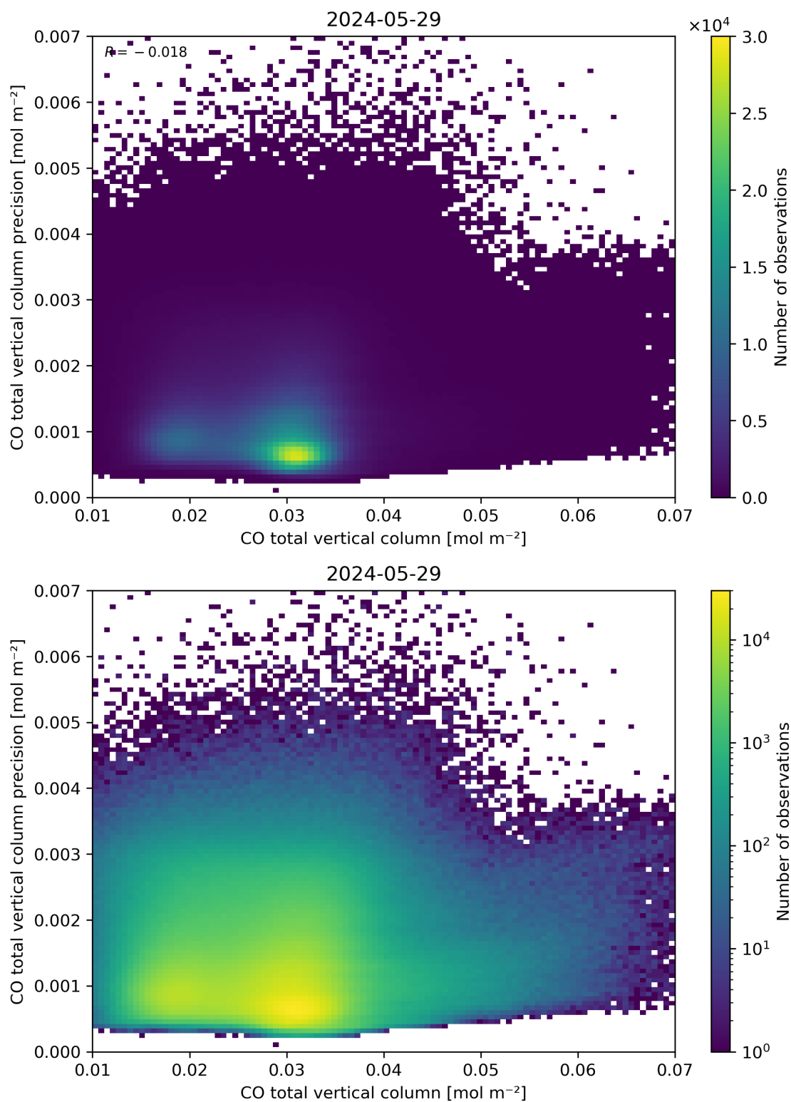
Figure 34: Scatter density plot of “CO total vertical column” against “CO total vertical column precision” for 2024-05-28 to 2024-05-30.
