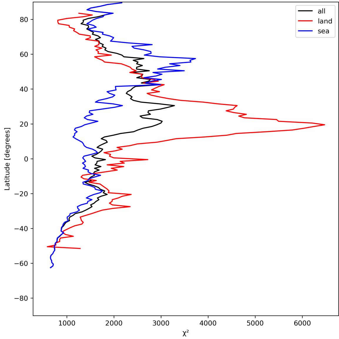
Figure 14: Zonal average of “ \chi^2 ” for 2024-05-28 to 2024-05-30.
