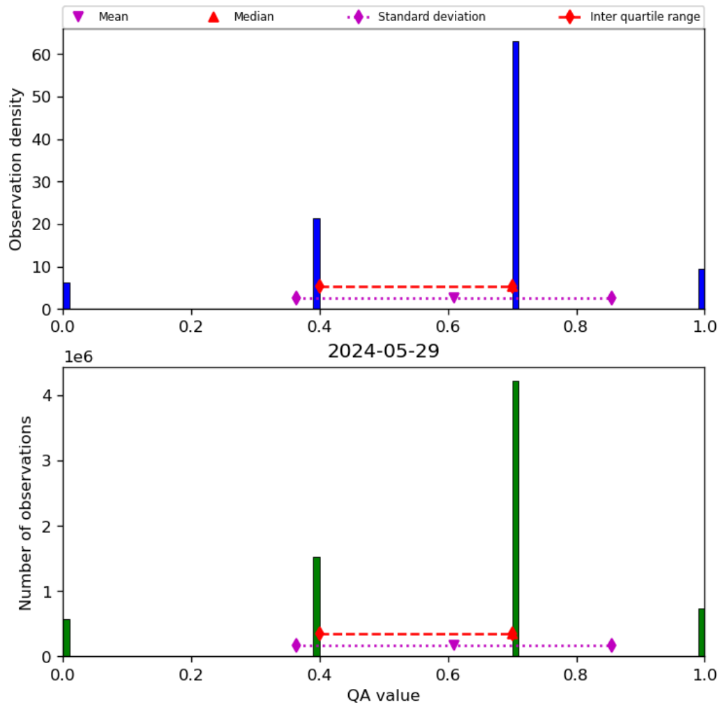
Figure 17: Histogram of “QA value” for 2024-05-28 to 2024-05-30
