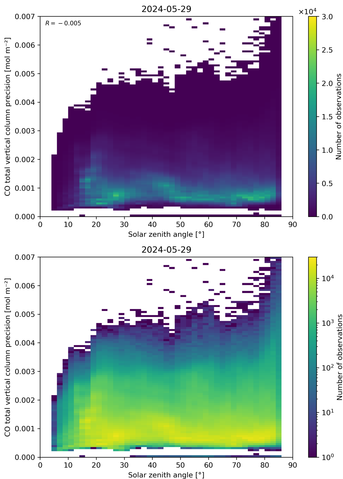
Figure 63: Scatter density plot of “Solar zenith angle” against “CO total vertical column precision” for 2024-05-28 to 2024-05-30.
