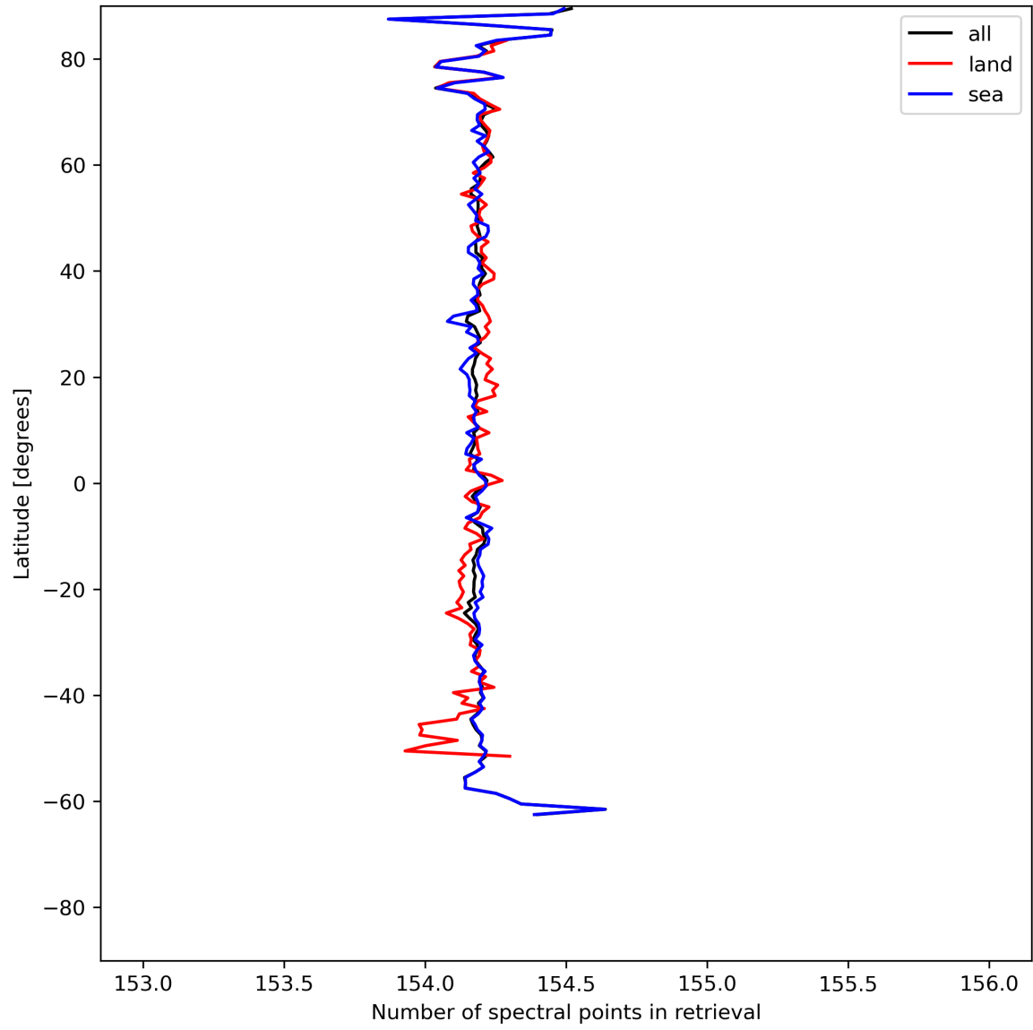
Figure 13: Zonal average of “Number of spectral points in retrieval” for 2024-05-28 to 2024-05-30.
