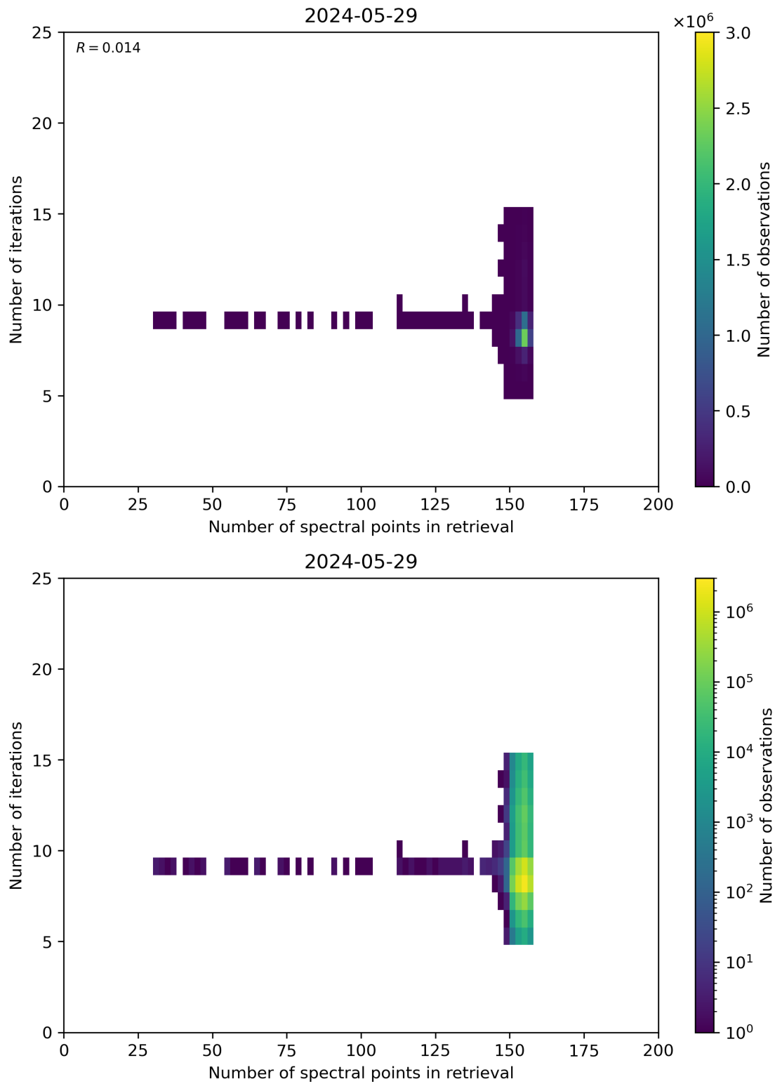
Figure 60: Scatter density plot of “Number of spectral points in retrieval” against “Number of iterations” for 2024-05-28 to 2024-05-30.
