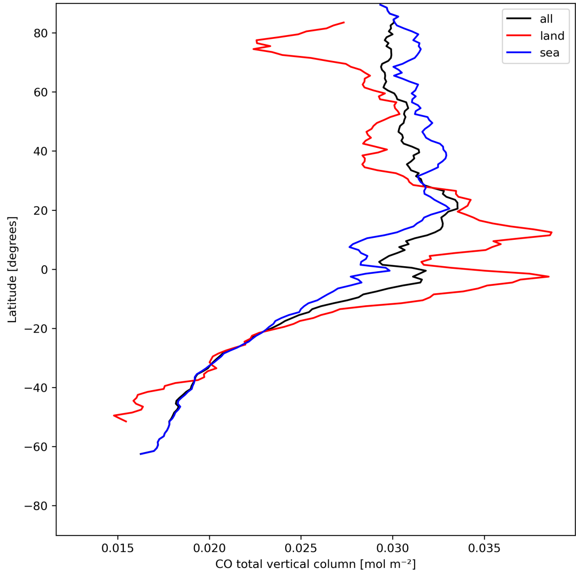
Figure 10: Zonal average of “CO total vertical column” for 2024-05-28 to 2024-05-30.
