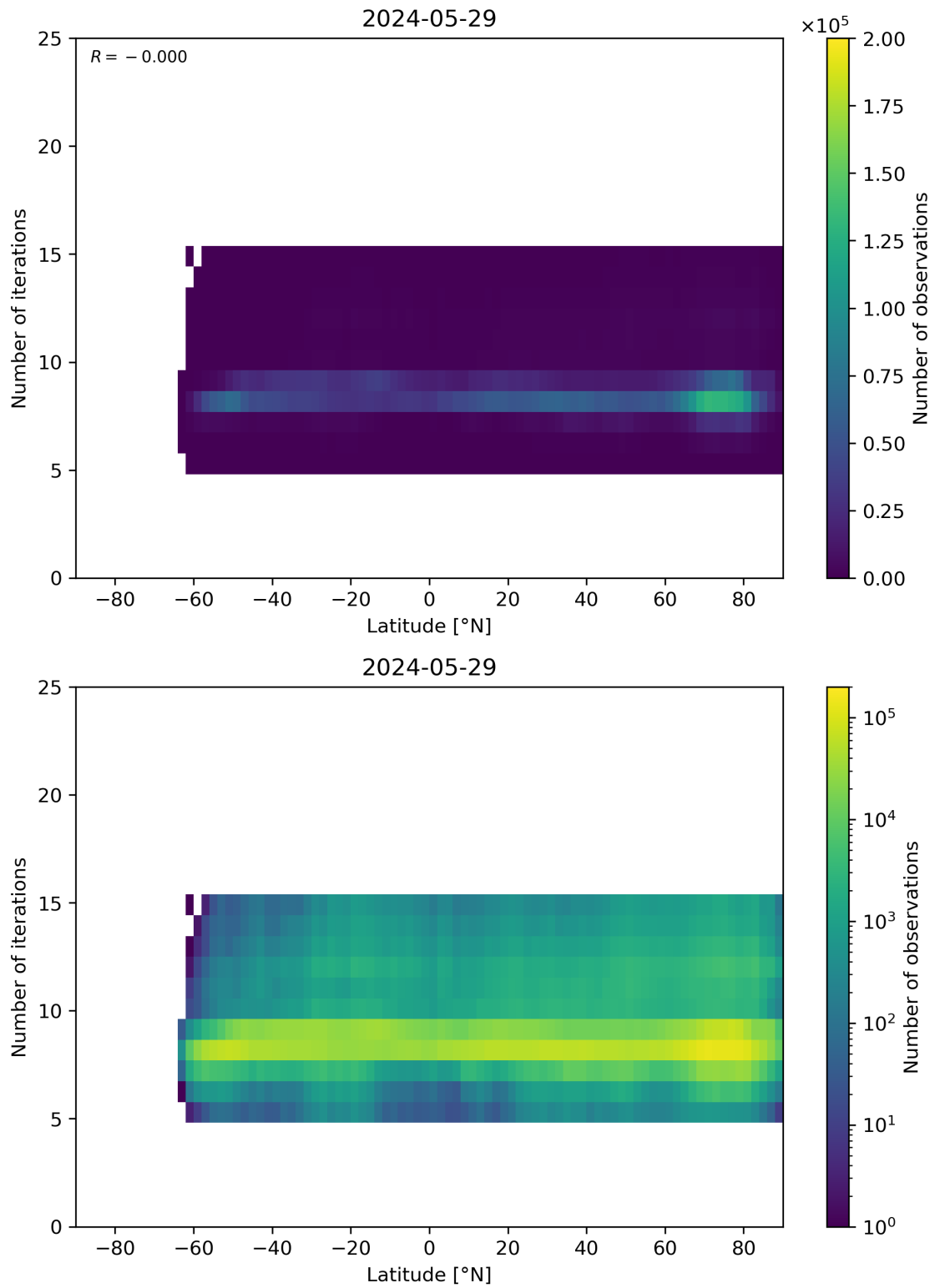
Figure 56: Scatter density plot of “Latitude” against “Number of iterations” for 2024-05-28 to 2024-05-30.
