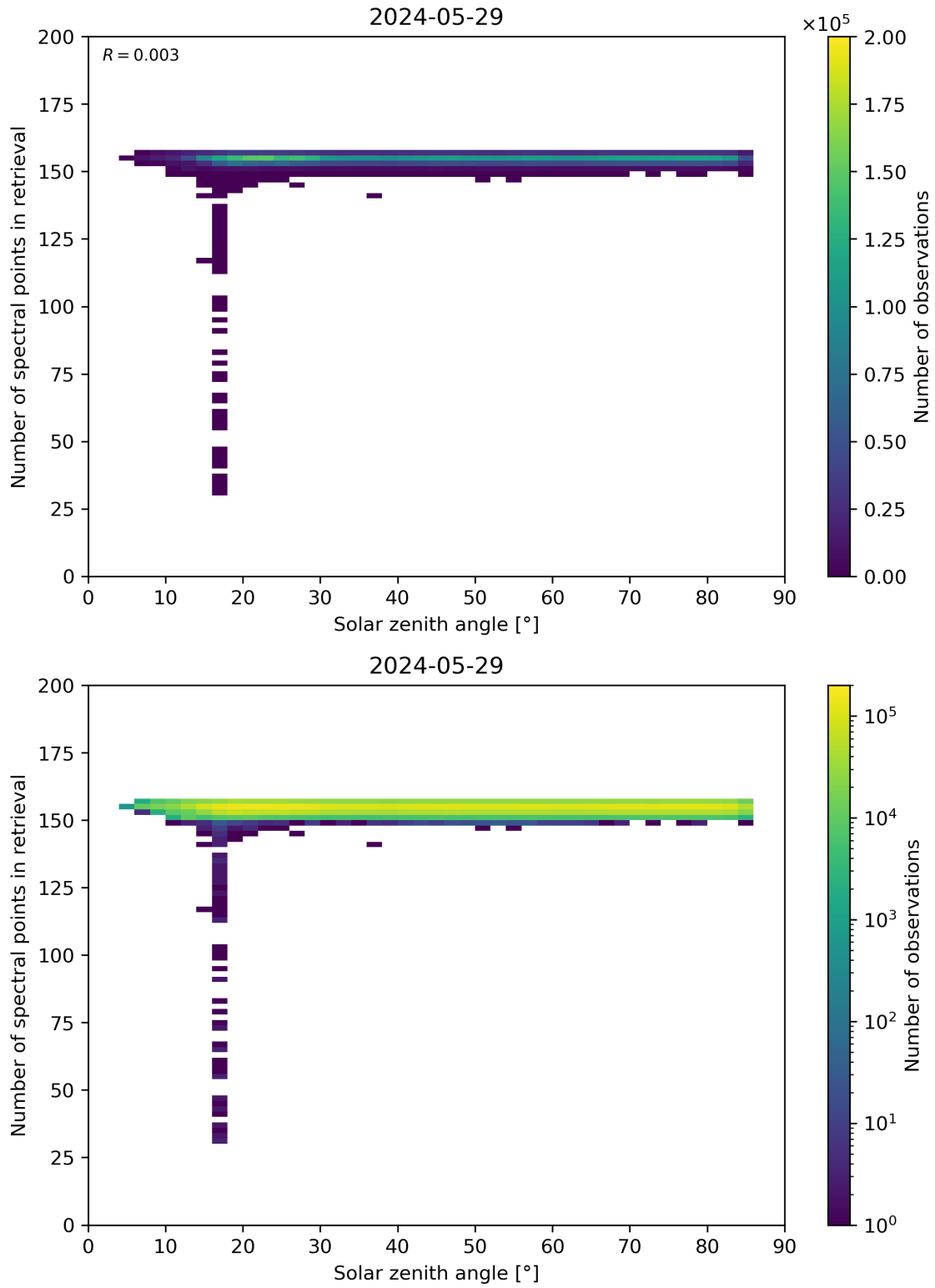
Figure 68: Scatter density plot of “Solar zenith angle” against “Number of spectral points in retrieval” for 2024-05-28 to 2024-05-30.
