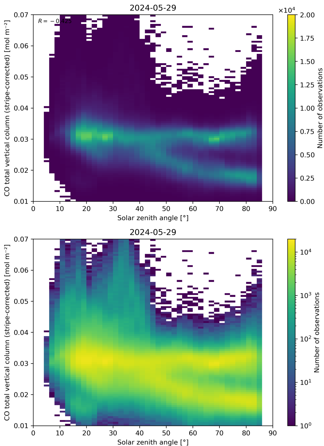
Figure 62: Scatter density plot of “Solar zenith angle” against “CO total vertical column (stripe-corrected)” for 2024-05-28 to 2024-05-30.
