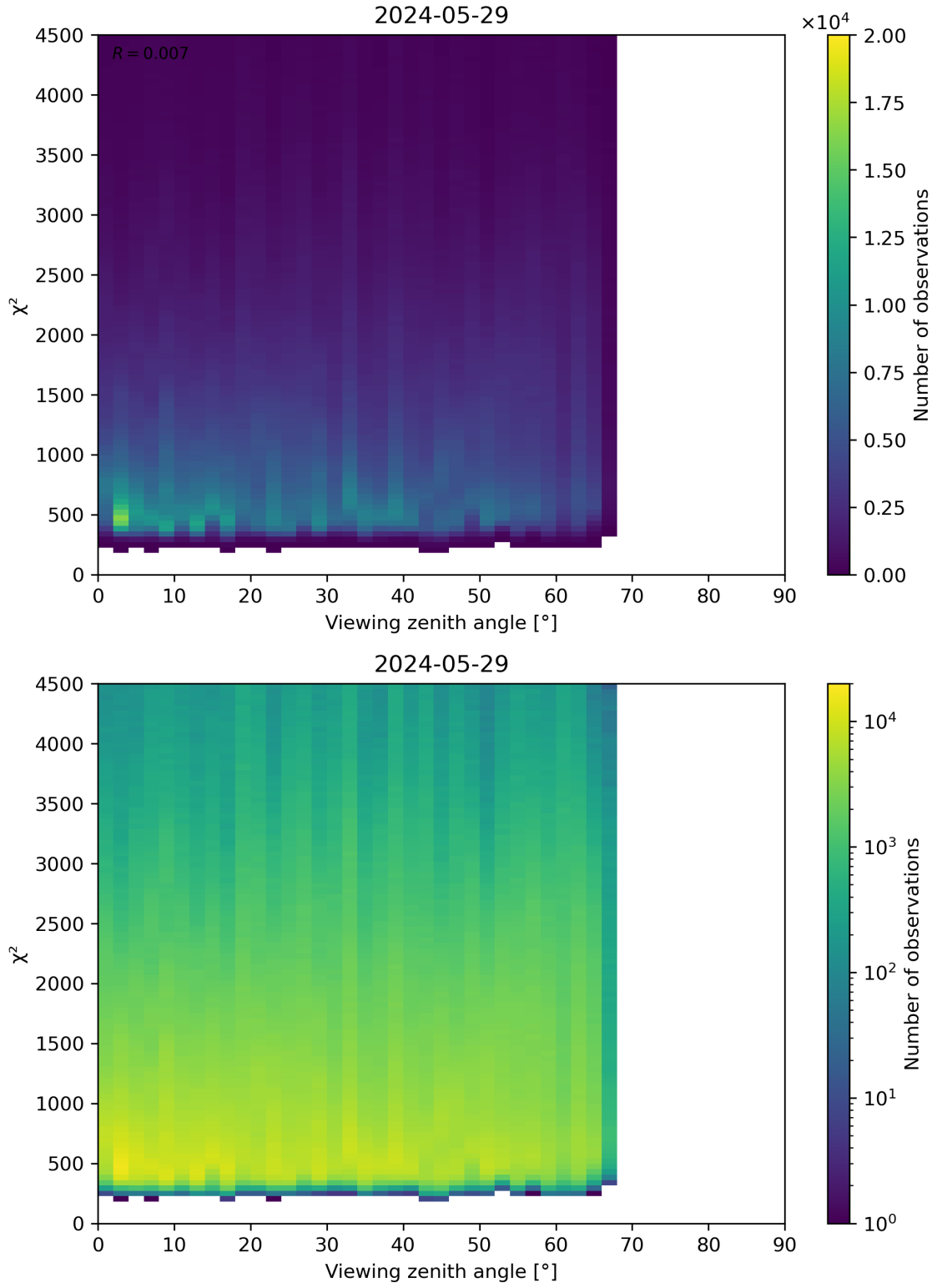
Figure 72: Scatter density plot of “Viewing zenith angle” against “ \chi^2 ” for 2024-05-28 to 2024-05-30.
