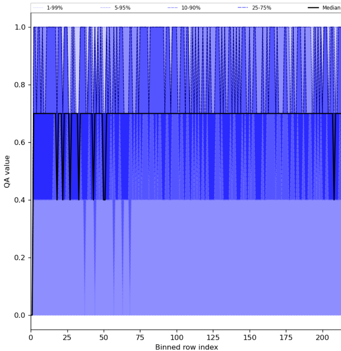
Figure 25: Along track statistics of “QA value” for 2024-05-28 to 2024-05-30
