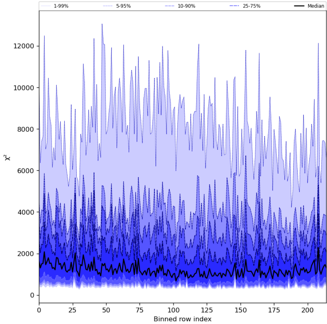
Figure 30: Along track statistics of “ \chi^2 ” for 2024-05-28 to 2024-05-30
