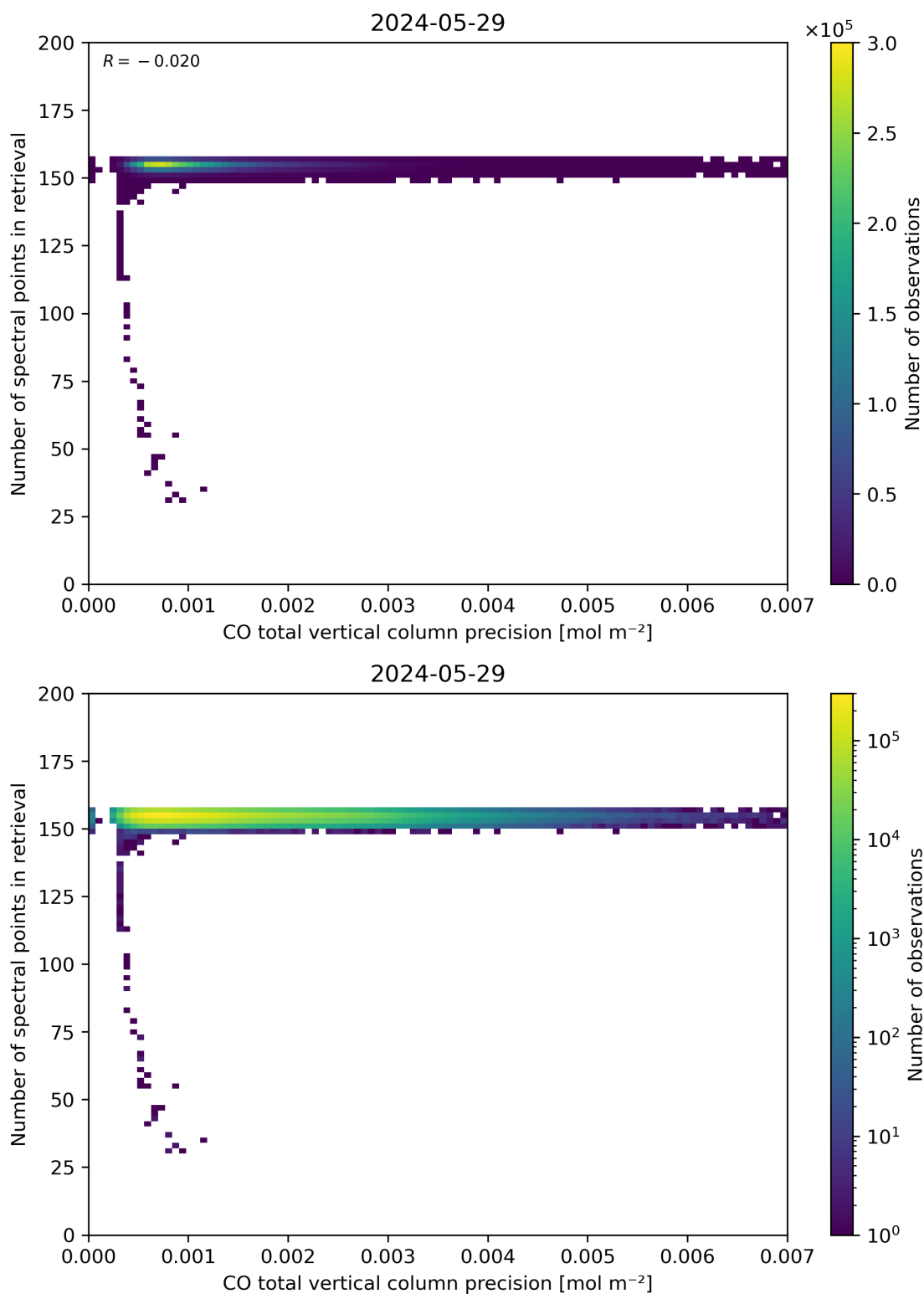
Figure 47: Scatter density plot of “CO total vertical column precision” against “Number of spectral points in retrieval” for 2024-05-28 to 2024-05-30.
