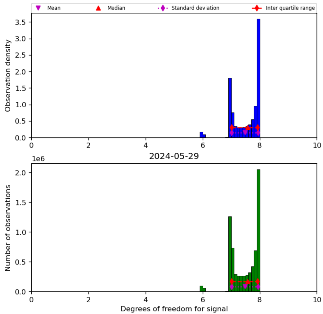
Figure 23: Histogram of “Degrees of freedom for signal” for 2024-05-28 to 2024-05-30
