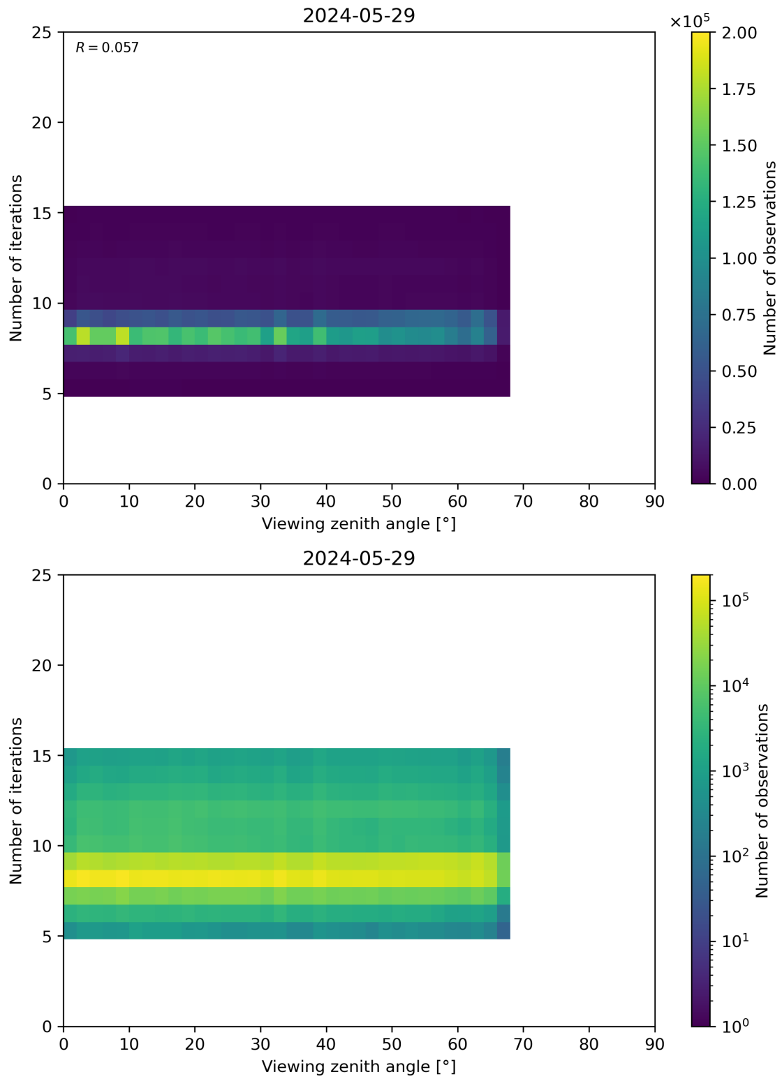
Figure 75: Scatter density plot of “Viewing zenith angle” against “Number of iterations” for 2024-05-28 to 2024-05-30.
