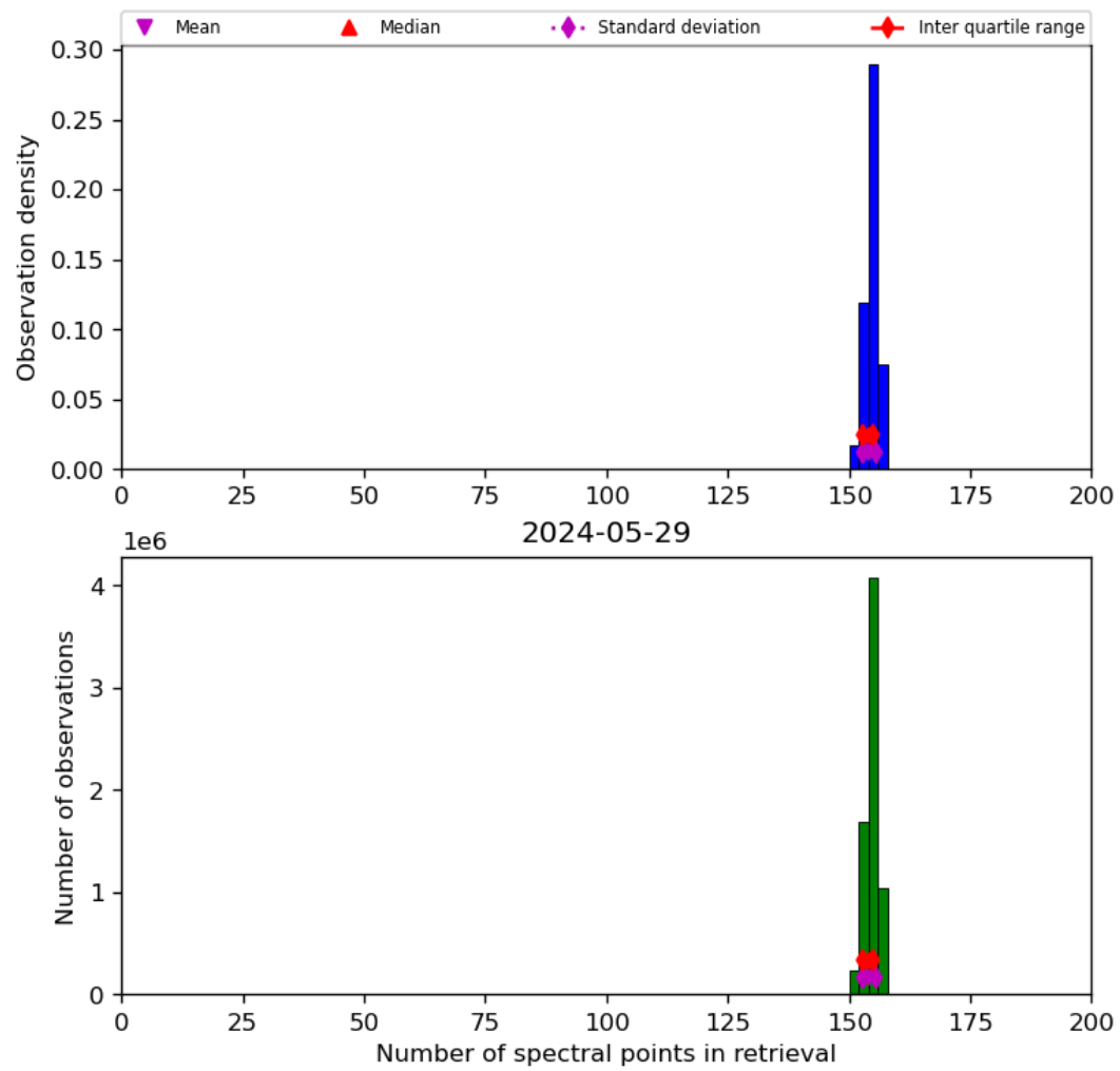
Figure 21: Histogram of “Number of spectral points in retrieval” for 2024-05-28 to 2024-05-30
