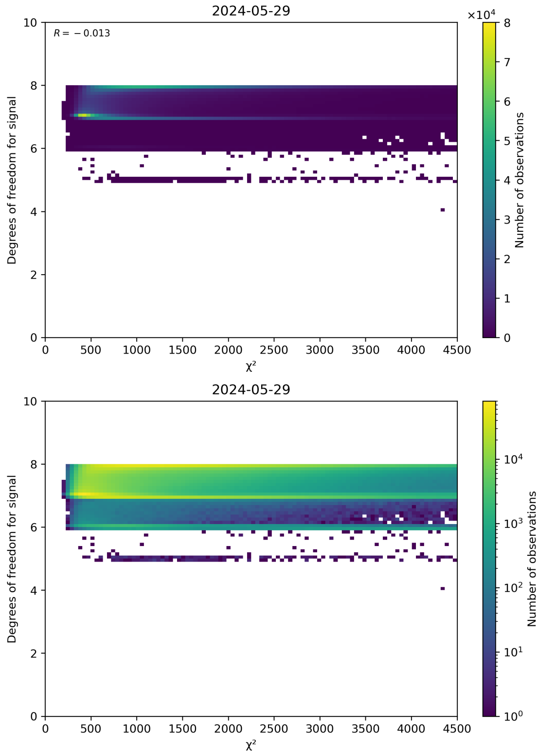
Figure 48: Scatter density plot of “ \chi^2 ” against “Degrees of freedom for signal” for 2024-05-28 to 2024-05-30.
