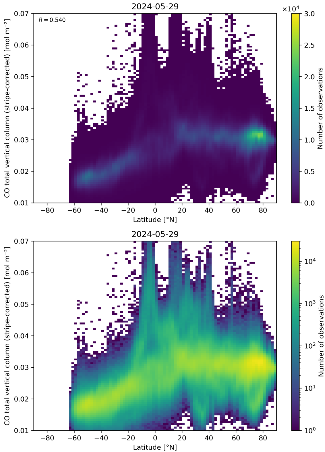
Figure 52: Scatter density plot of “Latitude” against “CO total vertical column (stripe-corrected)” for 2024-05-28 to 2024-05-30.
