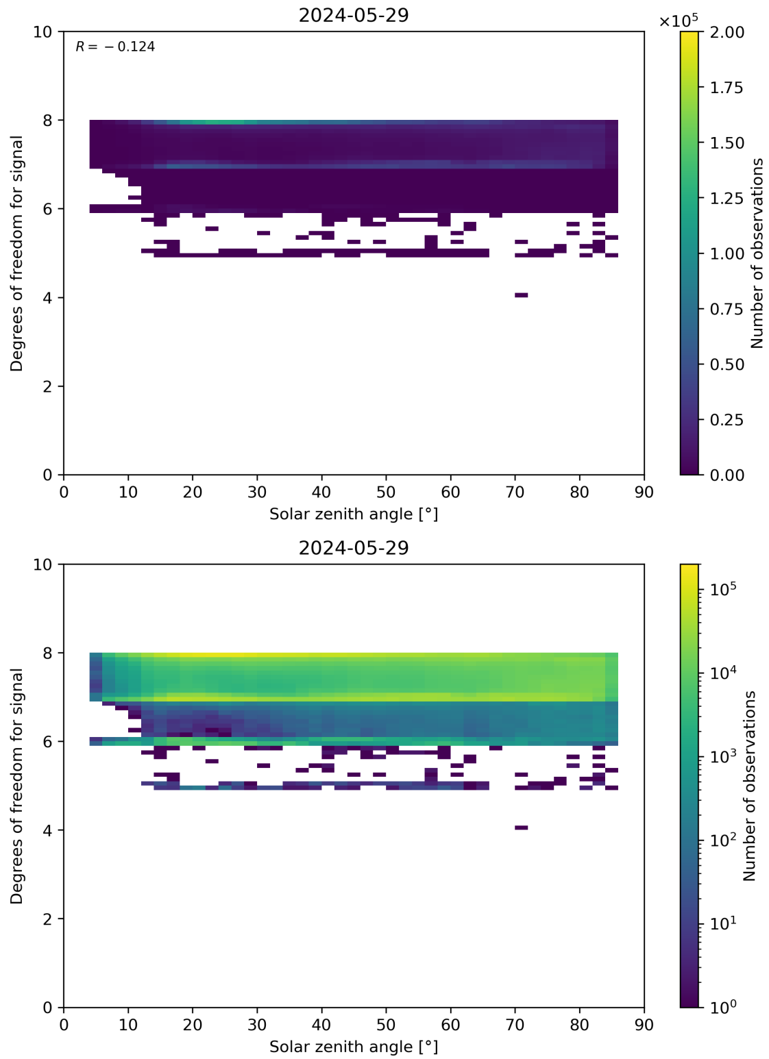
Figure 65: Scatter density plot of “Solar zenith angle” against “Degrees of freedom for signal” for 2024-05-28 to 2024-05-30.
