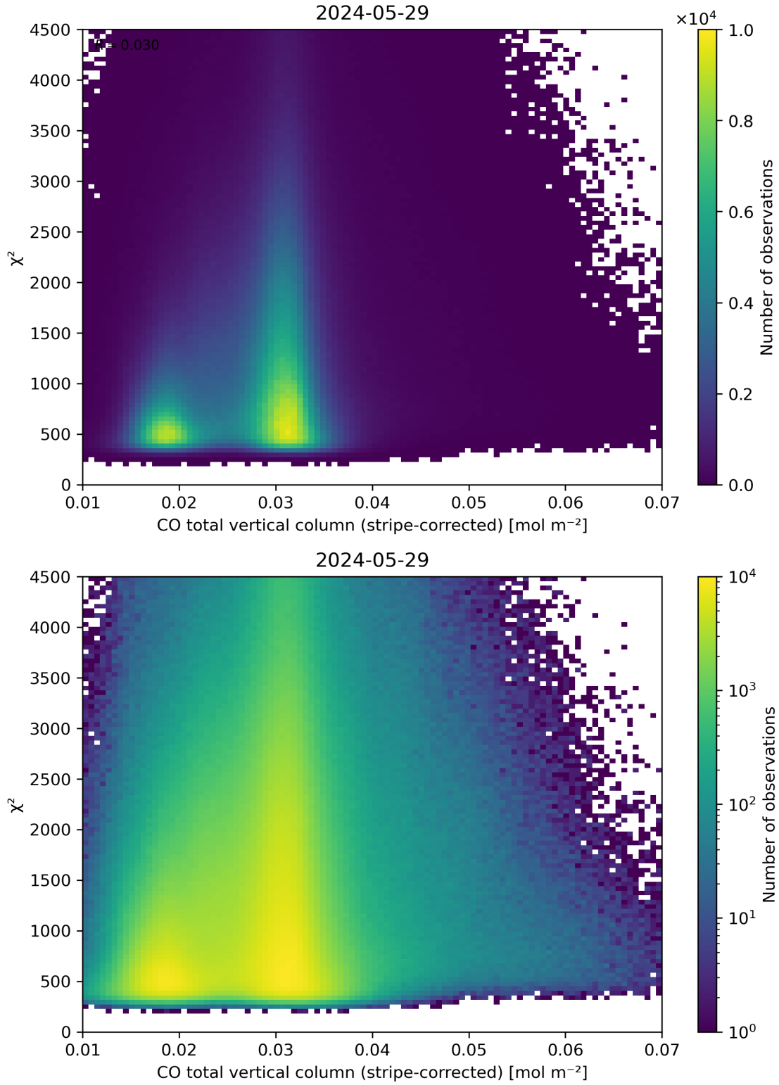
Figure 37: Scatter density plot of “CO total vertical column (stripe-corrected)” against “ \chi^2 ” for 2024-05-28 to 2024-05-30.
