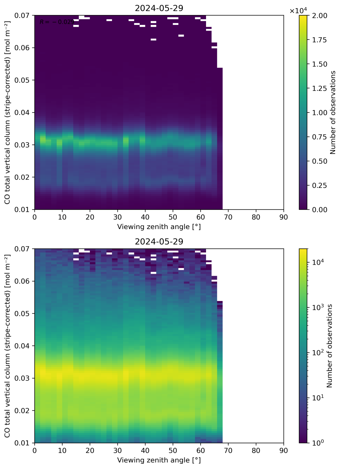
Figure 70: Scatter density plot of “Viewing zenith angle” against “CO total vertical column (stripe-corrected)” for 2024-05-28 to 2024-05-30.
