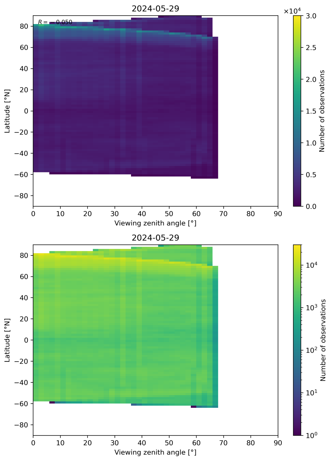
Figure 74: Scatter density plot of “Viewing zenith angle” against “Latitude” for 2024-05-28 to 2024-05-30.
