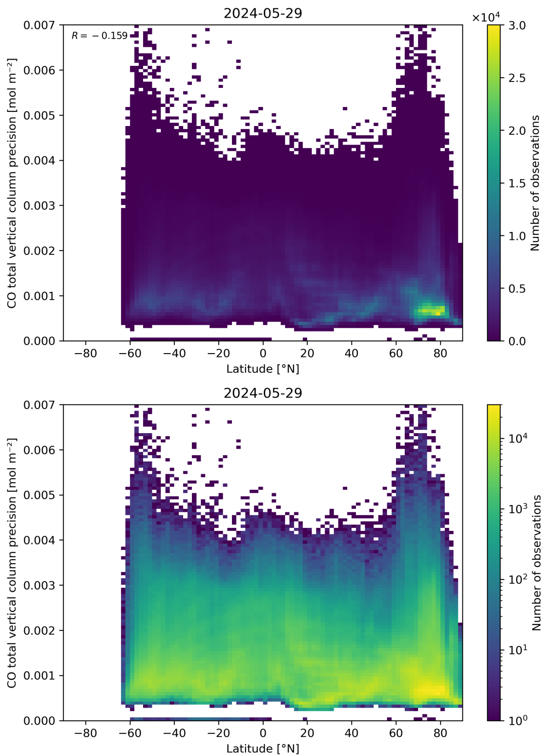
Figure 53: Scatter density plot of “Latitude” against “CO total vertical column precision” for 2024-05-28 to 2024-05-30.
