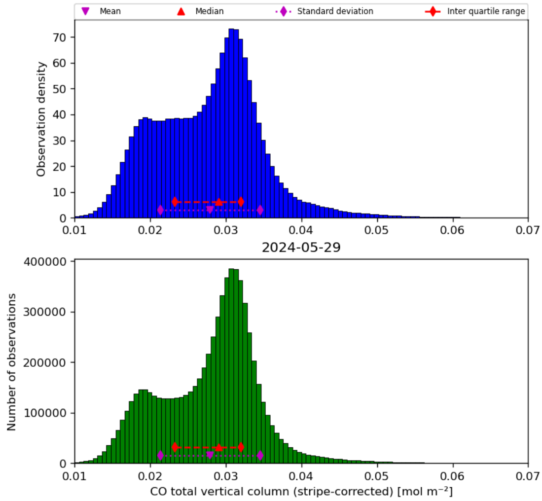
Figure 19: Histogram of “CO total vertical column (stripe-corrected)” for 2024-05-28 to 2024-05-30
