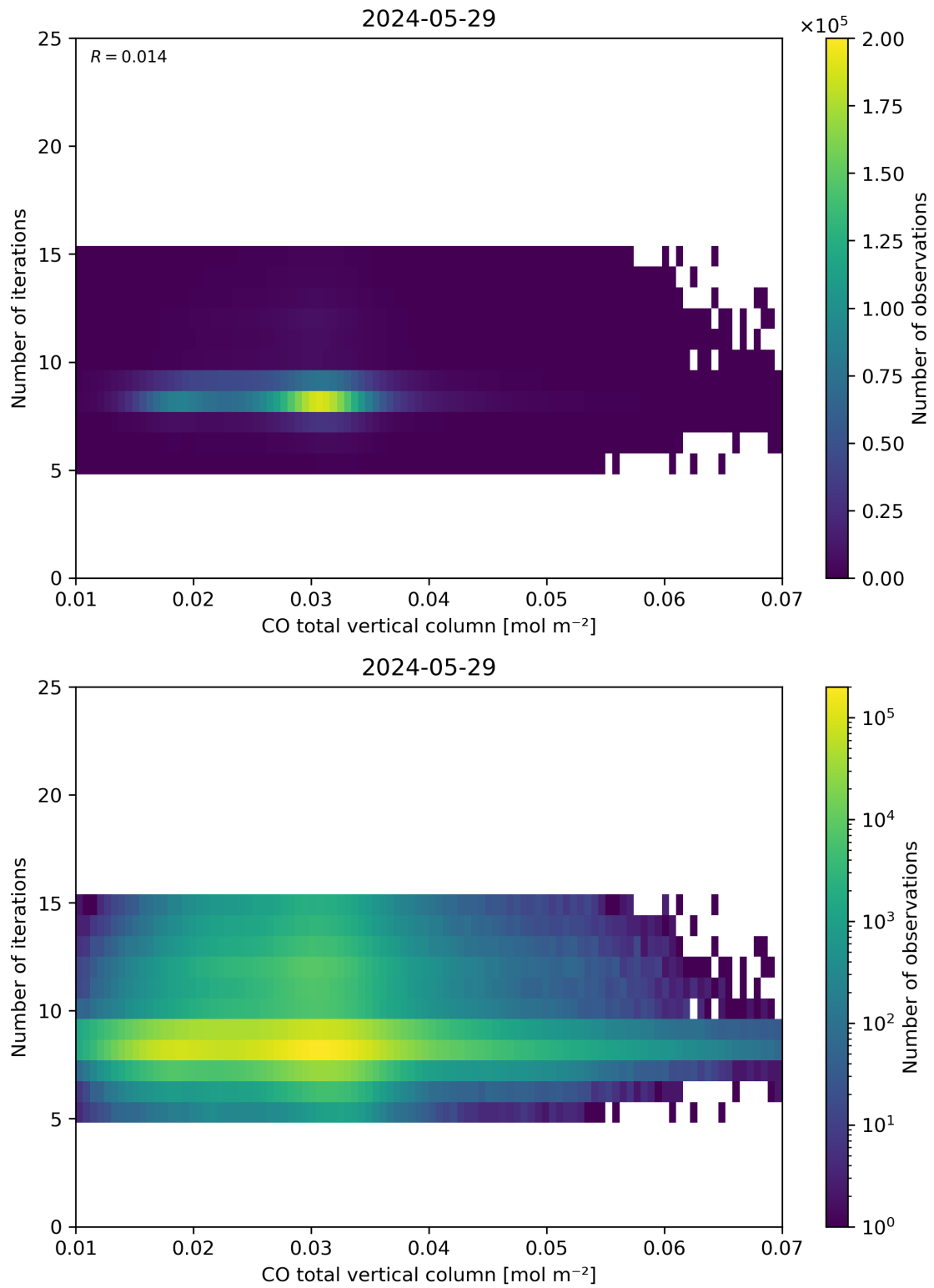
Figure 42: Scatter density plot of “CO total vertical column” against “Number of iterations” for 2024-05-28 to 2024-05-30.
