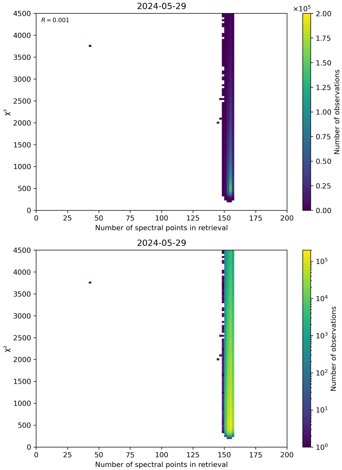
Figure 58: Scatter density plot of “Number of spectral points in retrieval” against “ \chi^2 ” for 2024-05-28 to 2024-05-30.
