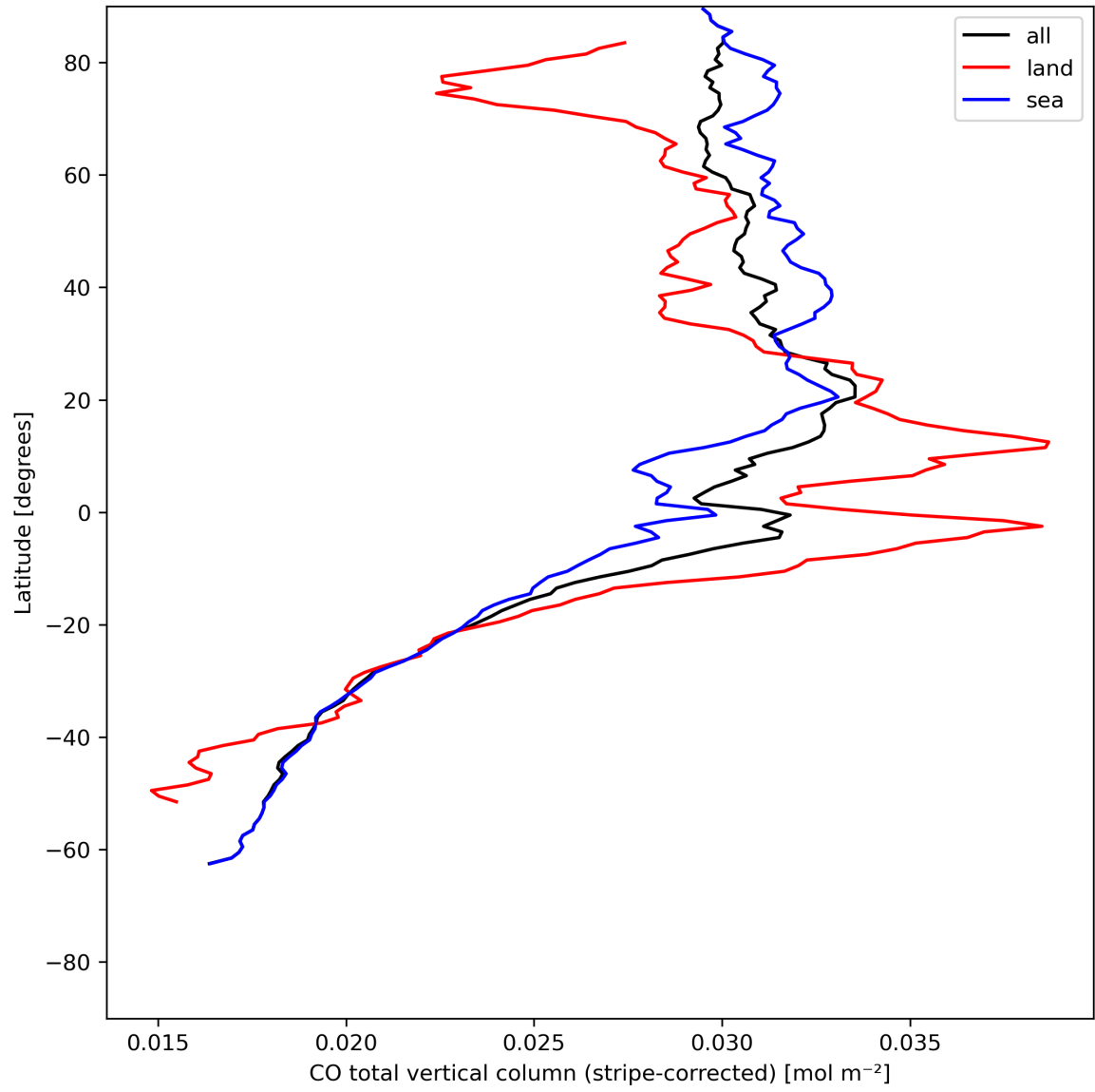
Figure 11: Zonal average of “CO total vertical column (stripe-corrected)” for 2024-05-28 to 2024-05-30.
