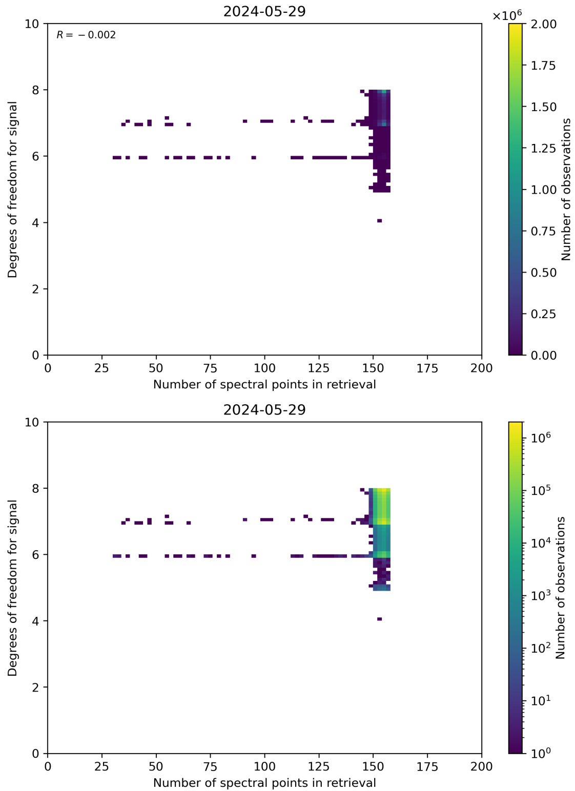
Figure 59: Scatter density plot of “Number of spectral points in retrieval” against “Degrees of freedom for signal” for 2024-05-28 to 2024-05-30.
