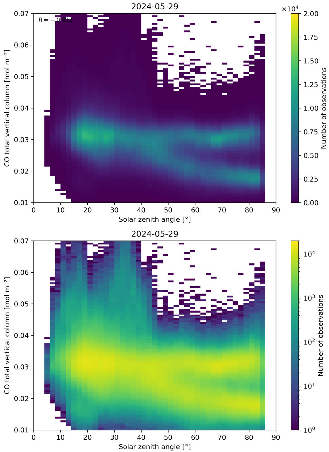
Figure 61: Scatter density plot of “Solar zenith angle” against “CO total vertical column” for 2024-05-28 to 2024-05-30.
