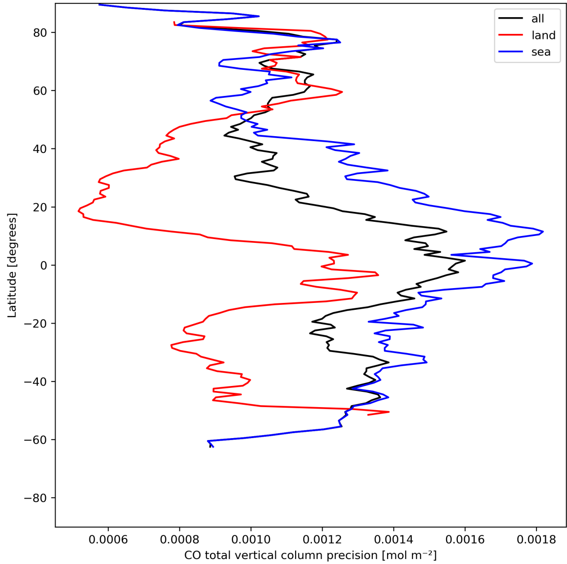
Figure 12: Zonal average of “CO total vertical column precision” for 2024-05-28 to 2024-05-30.
