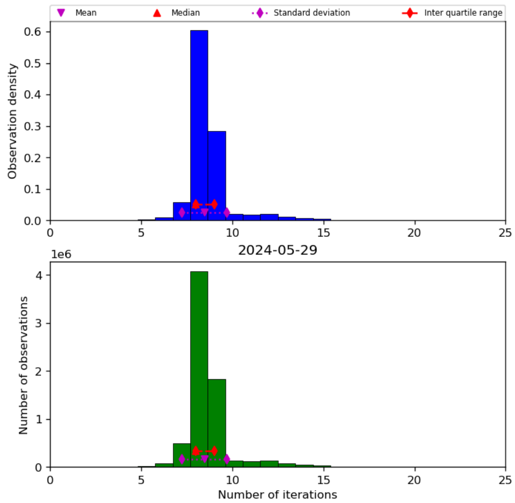
Figure 24: Histogram of “Number of iterations” for 2024-05-28 to 2024-05-30
