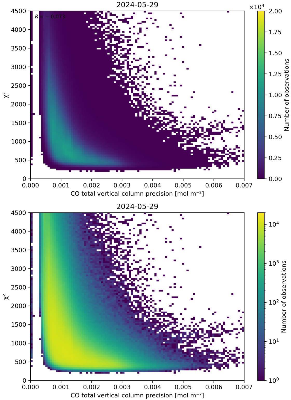
Figure 44: Scatter density plot of “CO total vertical column precision” against “ \chi^2 ” for 2024-05-28 to 2024-05-30.
