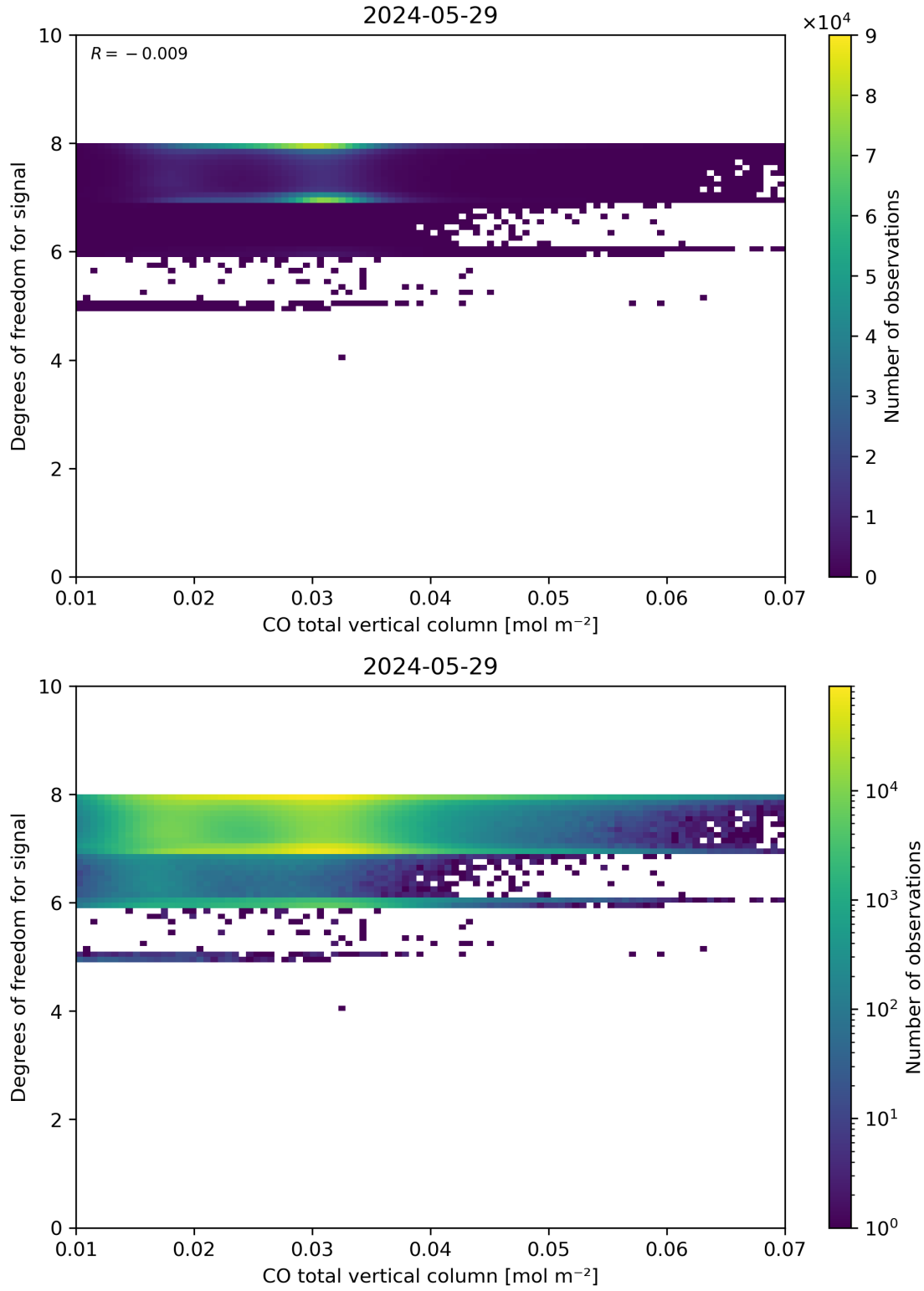
Figure 41: Scatter density plot of “CO total vertical column” against “Degrees of freedom for signal” for 2024-05-28 to 2024-05-30.
