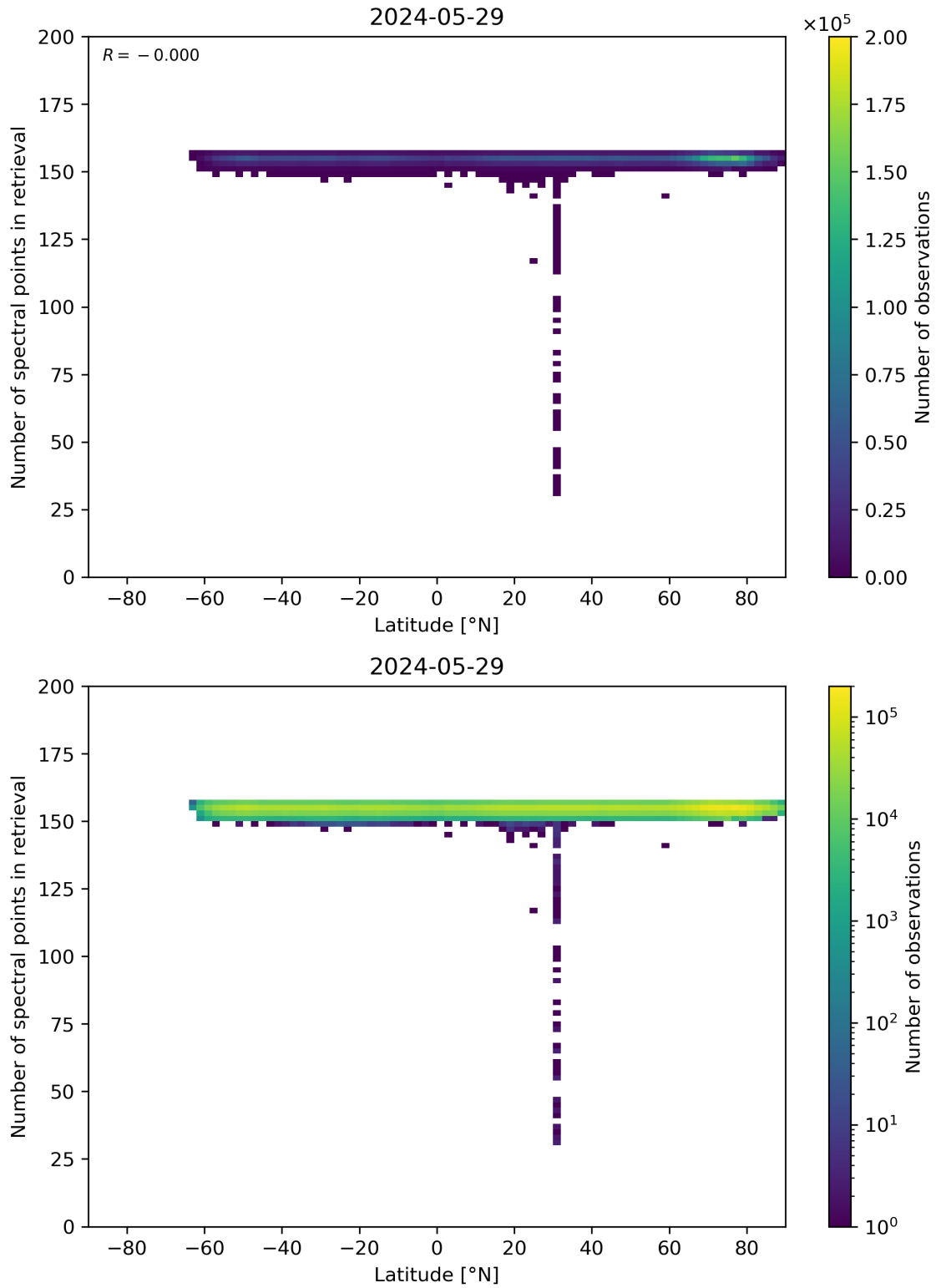
Figure 57: Scatter density plot of “Latitude” against “Number of spectral points in retrieval” for 2024-05-28 to 2024-05-30.
