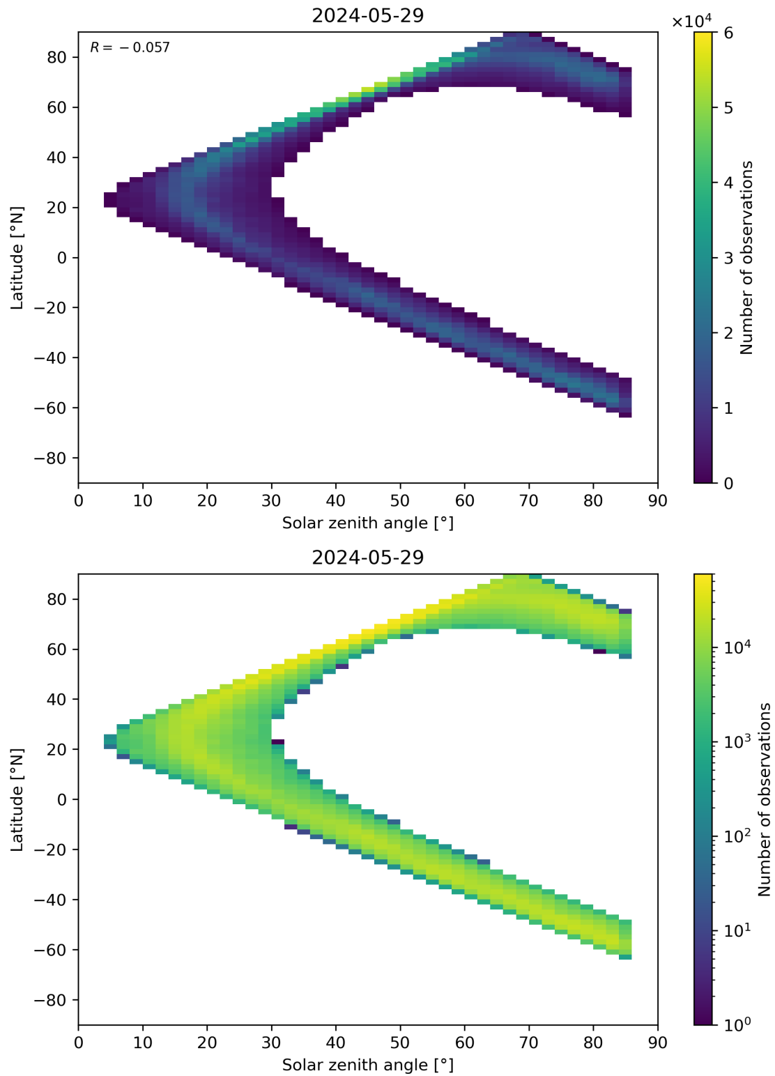
Figure 66: Scatter density plot of “Solar zenith angle” against “Latitude” for 2024-05-28 to 2024-05-30.
