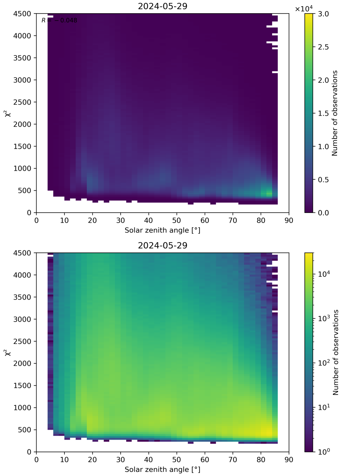
Figure 64: Scatter density plot of “Solar zenith angle” against “ \chi^2 ” for 2024-05-28 to 2024-05-30.
