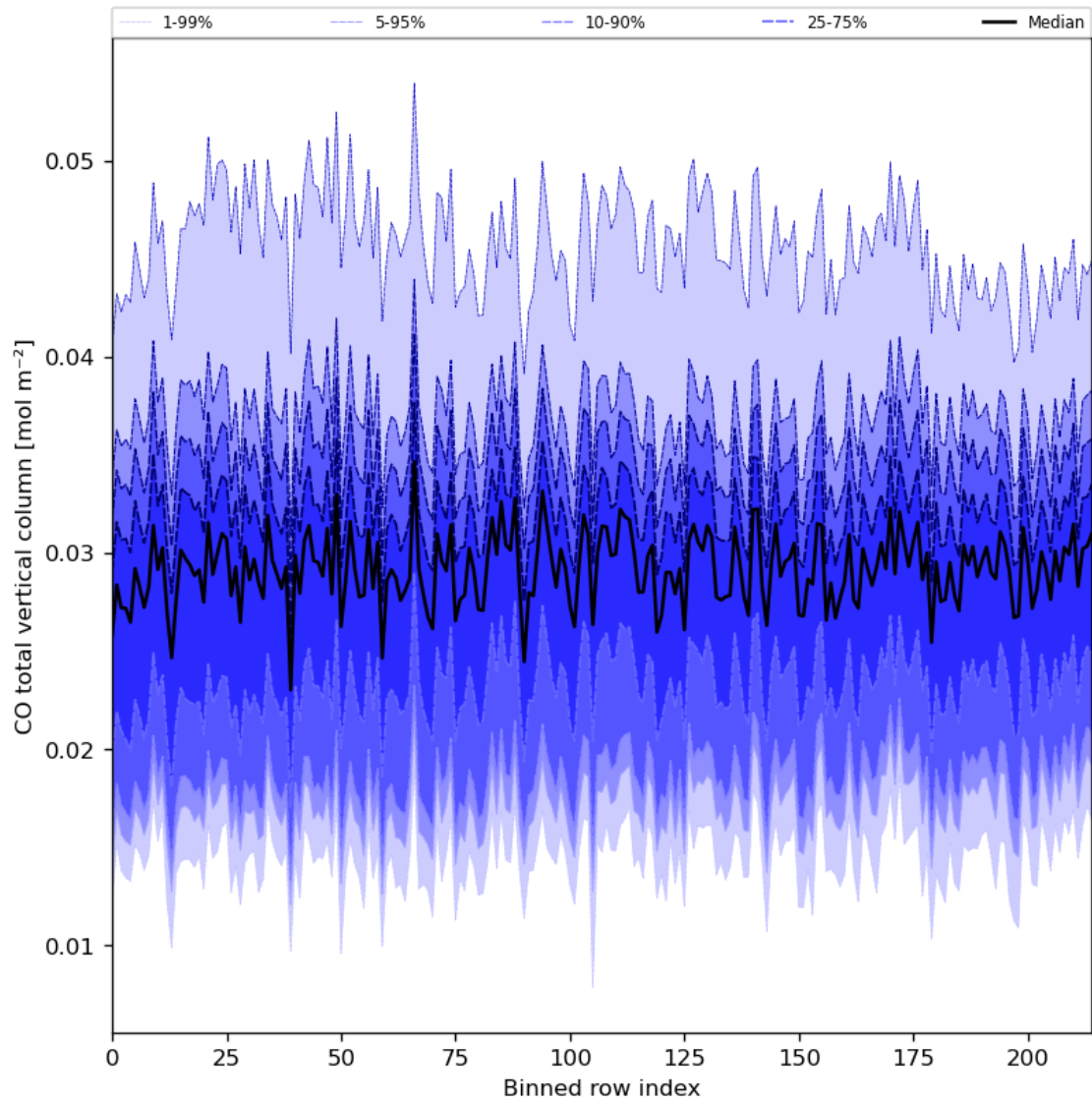
Figure 26: Along track statistics of “CO total vertical column” for 2024-05-28 to 2024-05-30
