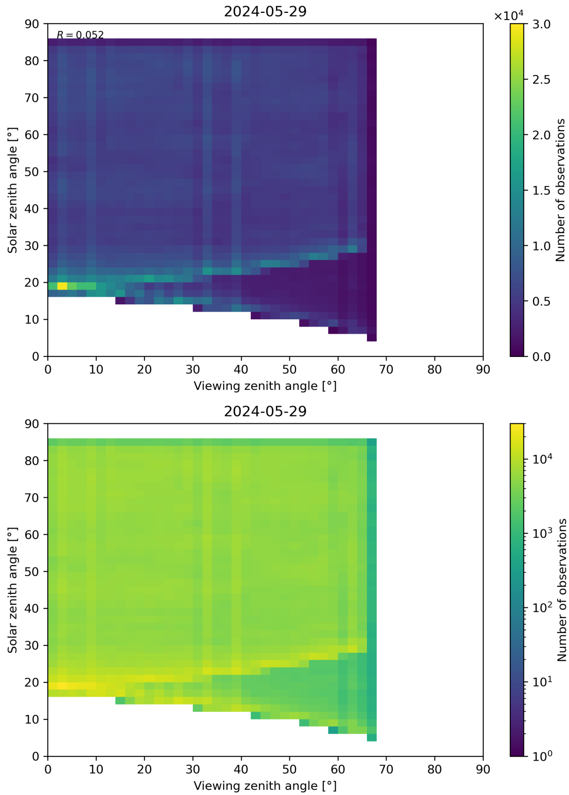
Figure 77: Scatter density plot of “Viewing zenith angle” against “Solar zenith angle” for 2024-05-28 to 2024-05-30.
