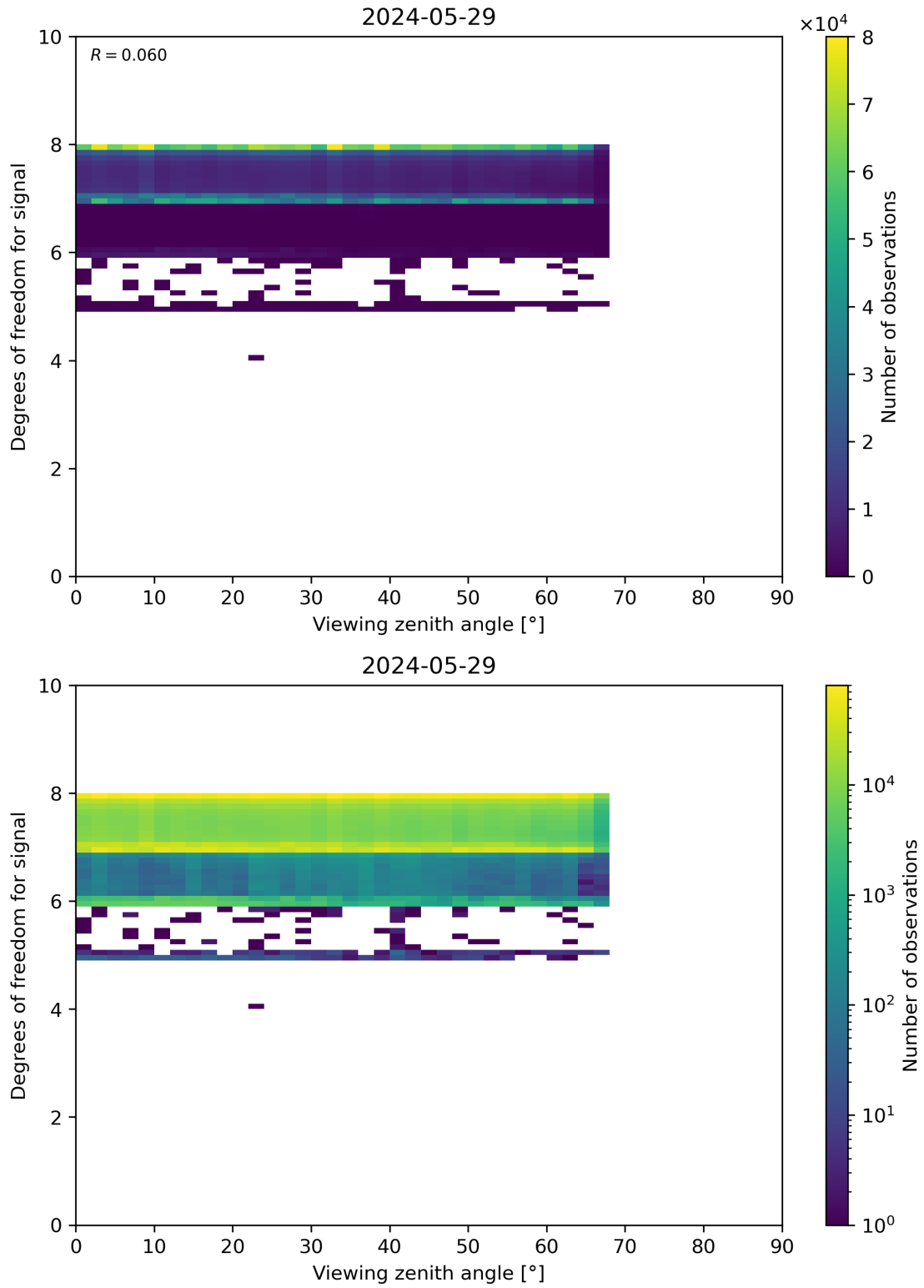
Figure 73: Scatter density plot of “Viewing zenith angle” against “Degrees of freedom for signal” for 2024-05-28 to 2024-05-30.
