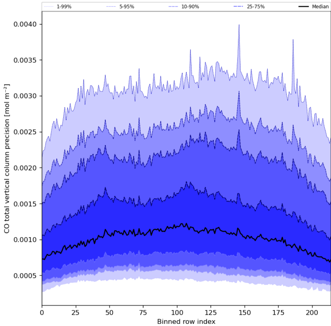
Figure 28: Along track statistics of “CO total vertical column precision” for 2024-05-28 to 2024-05-30
