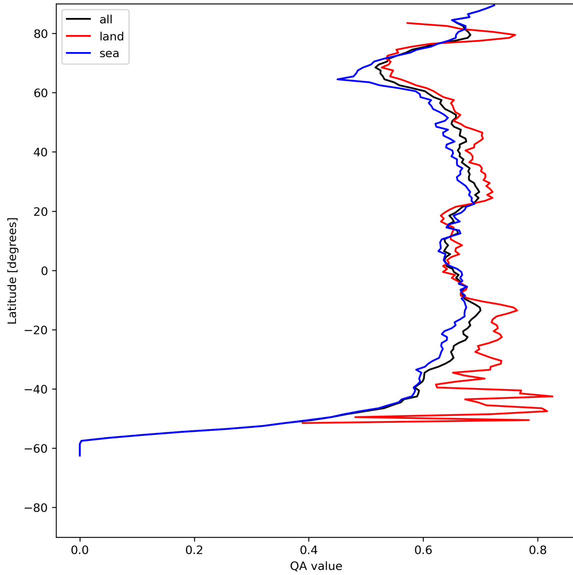
Figure 9: Zonal average of “QA value” for 2024-05-28 to 2024-05-30.
