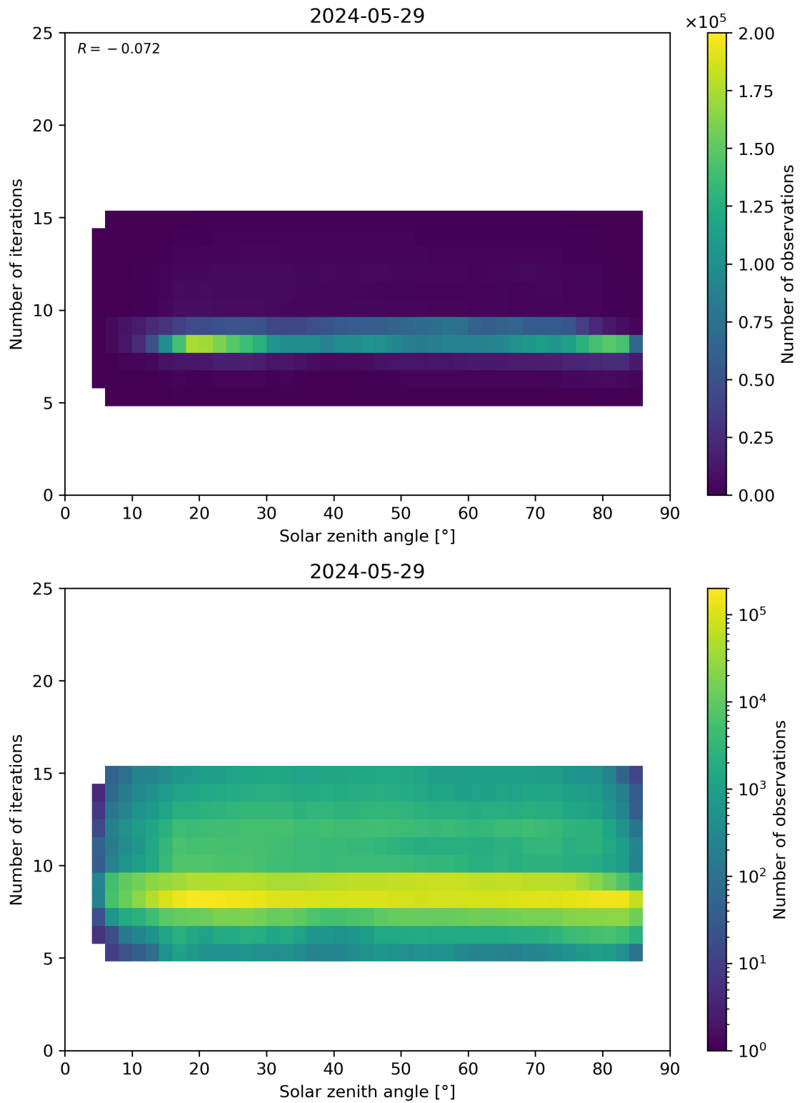
Figure 67: Scatter density plot of “Solar zenith angle” against “Number of iterations” for 2024-05-28 to 2024-05-30.
