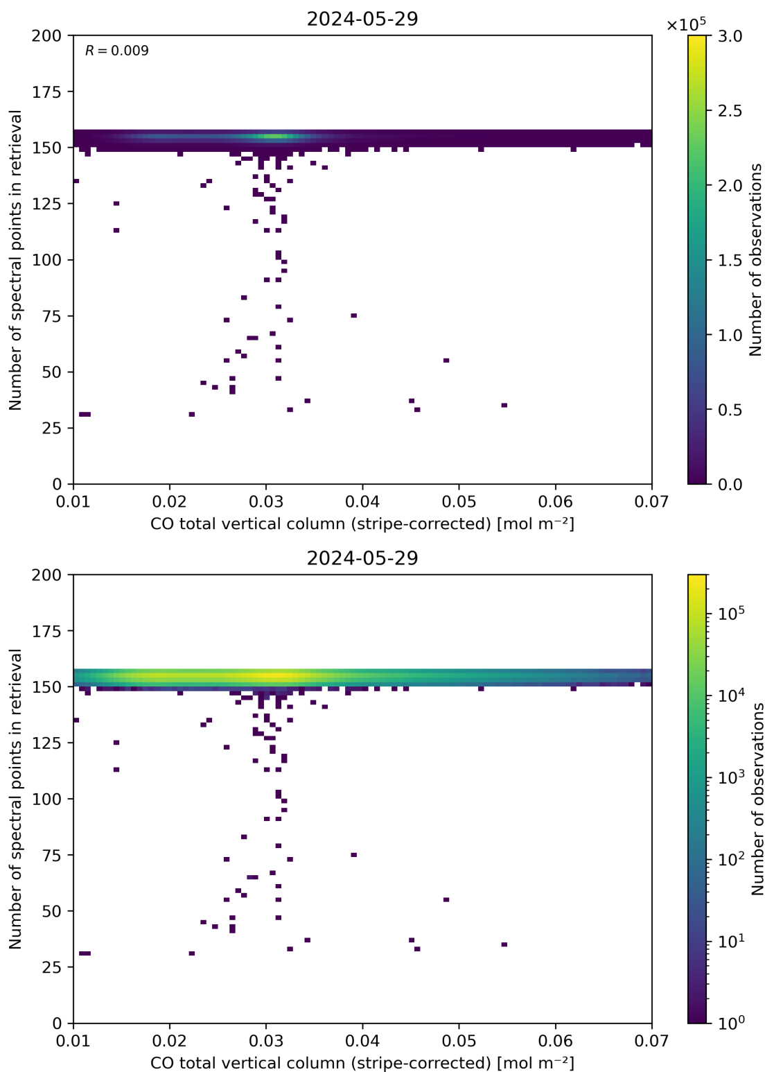
Figure 40: Scatter density plot of “CO total vertical column (stripe-corrected)” against “Number of spectral points in retrieval” for 2024-05-28 to 2024-05-30.
