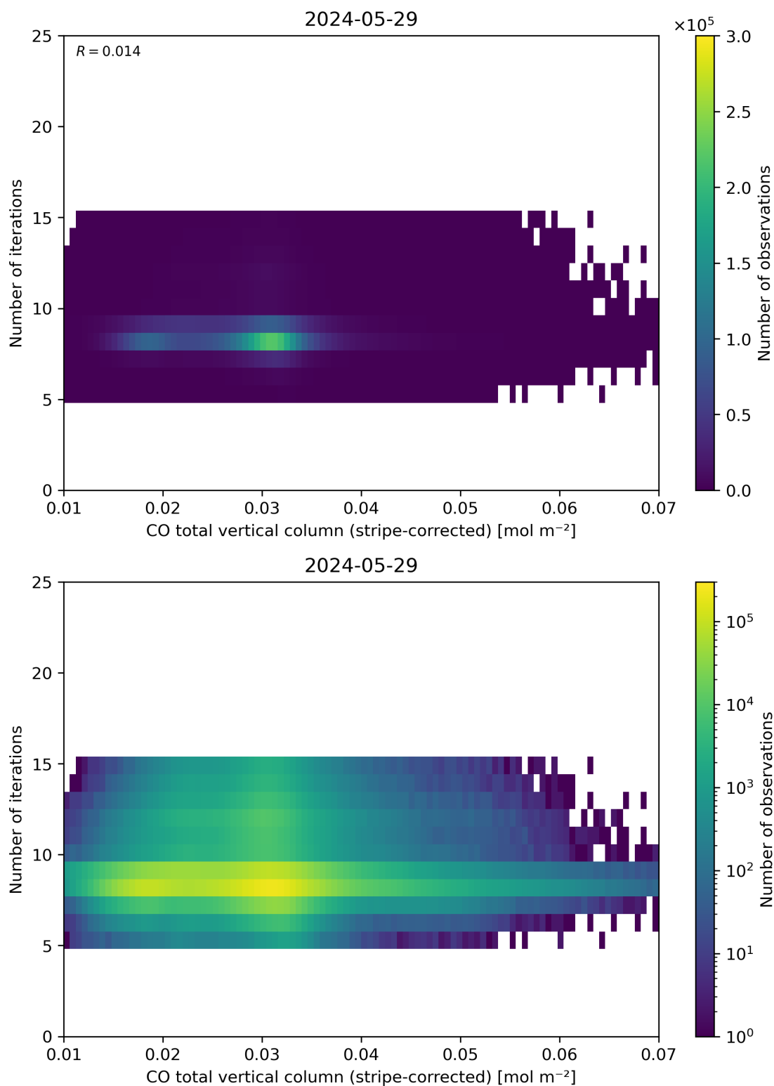
Figure 39: Scatter density plot of “CO total vertical column (stripe-corrected)” against “Number of iterations” for 2024-05-28 to 2024-05-30.
