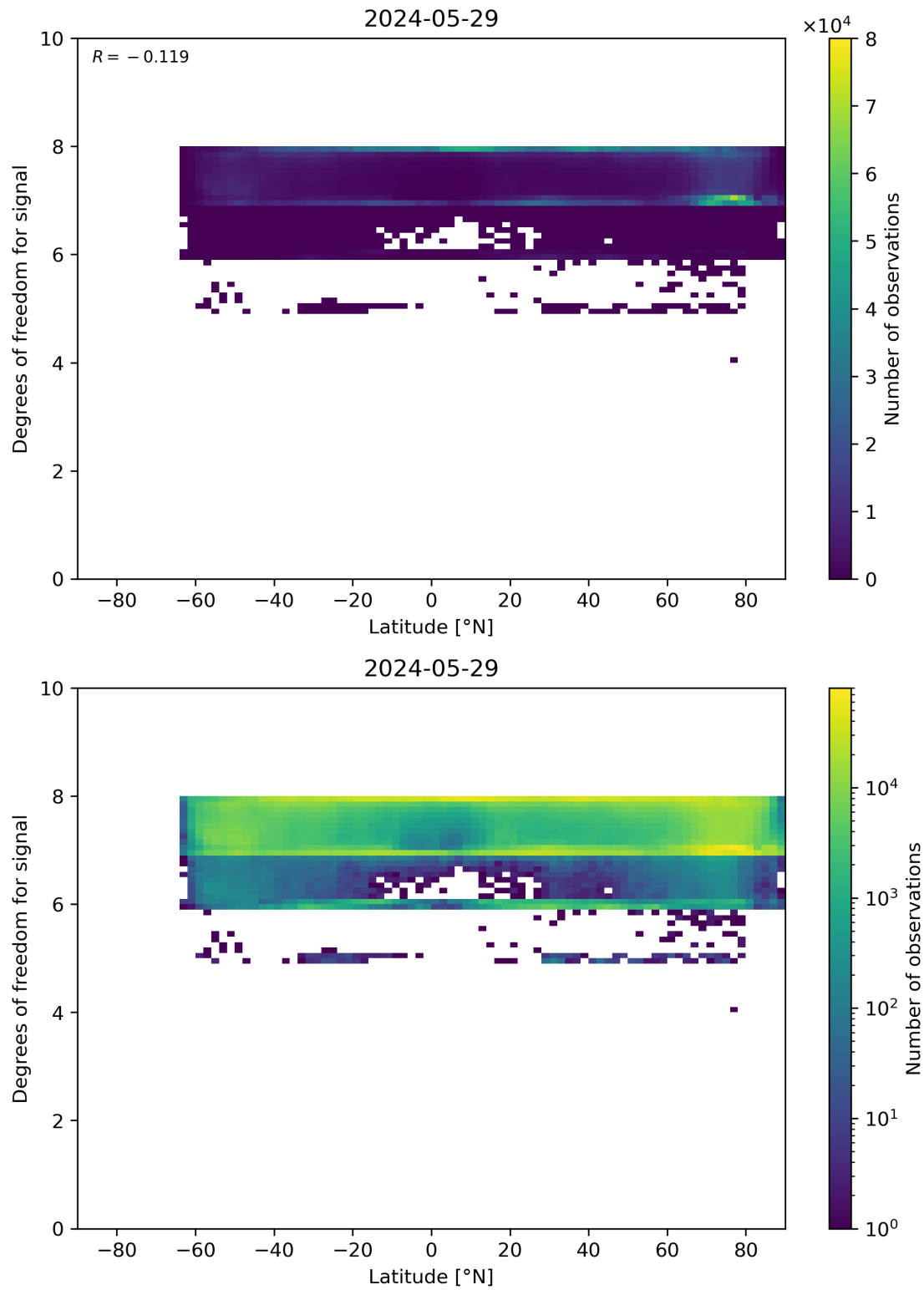
Figure 55: Scatter density plot of “Latitude” against “Degrees of freedom for signal” for 2024-05-28 to 2024-05-30.
