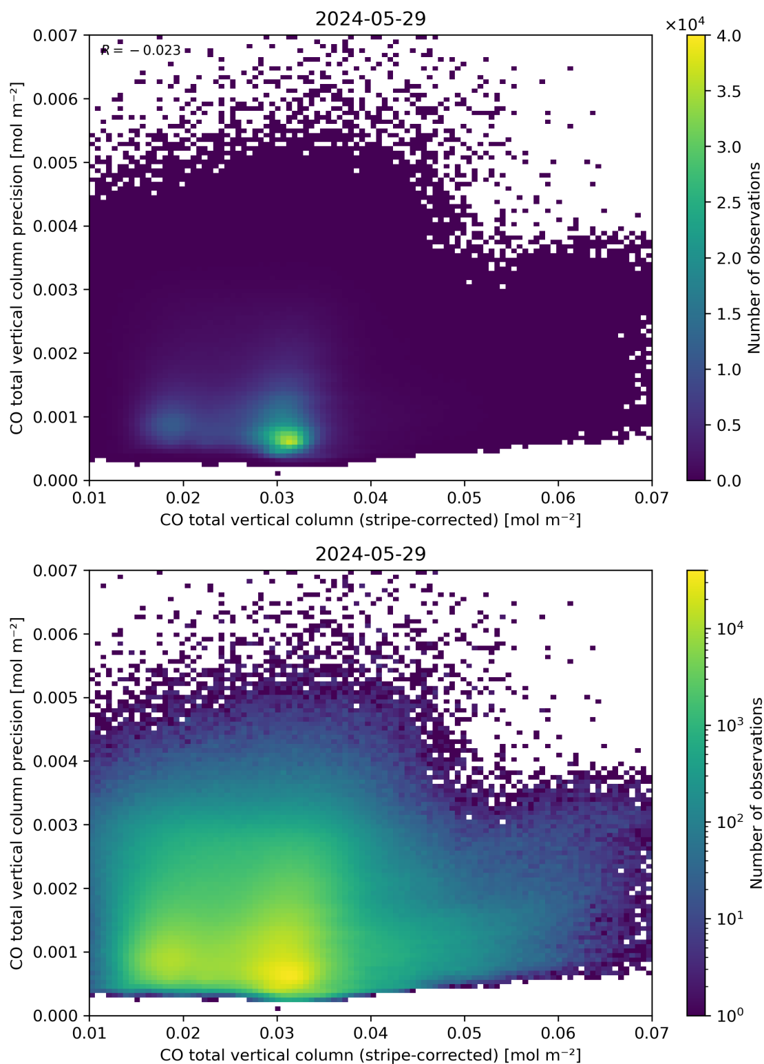
Figure 36: Scatter density plot of “CO total vertical column (stripe-corrected)” against “CO total vertical column precision” for 2024-05-28 to 2024-05-30.
