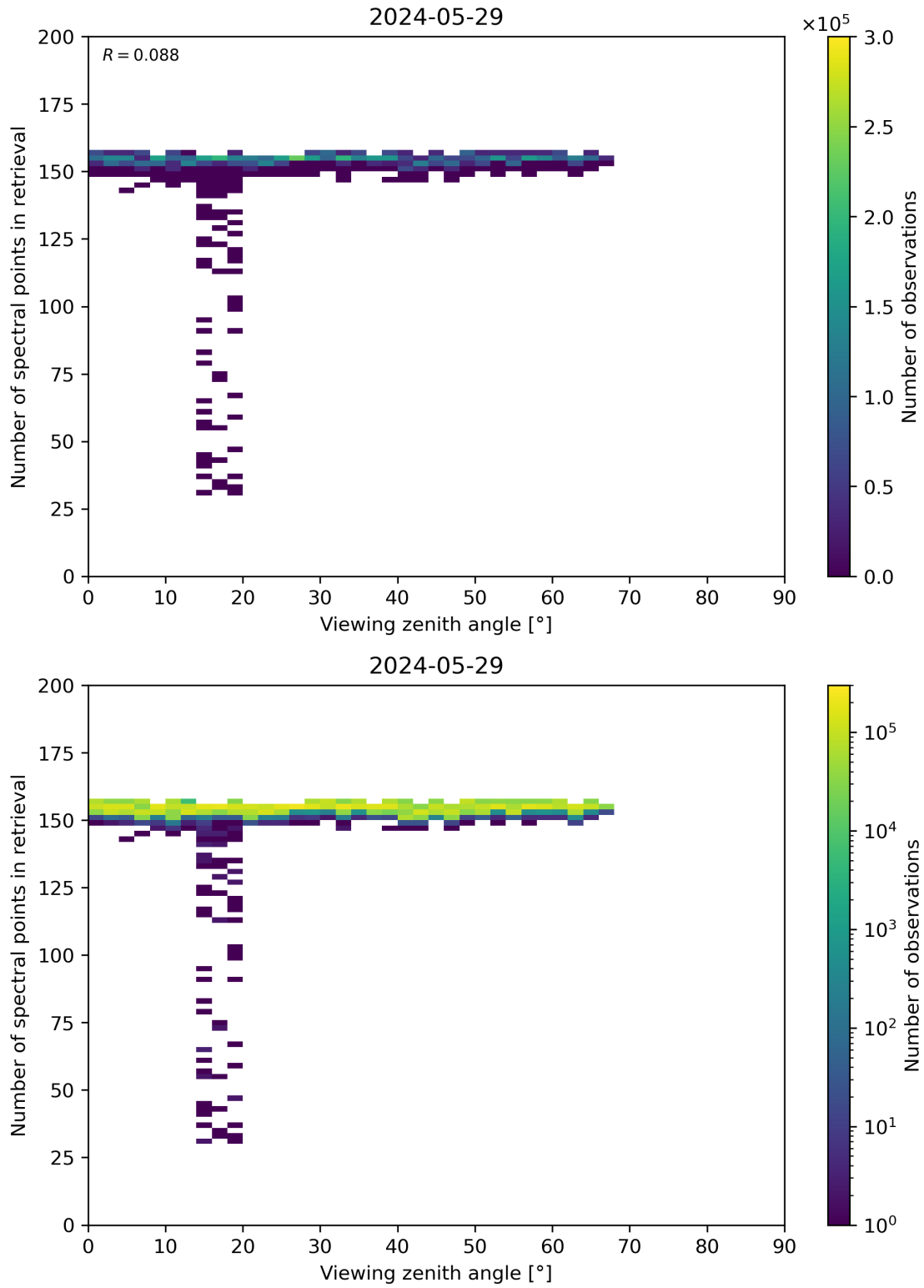
Figure 76: Scatter density plot of “Viewing zenith angle” against “Number of spectral points in retrieval” for 2024-05-28 to 2024-05-30.
