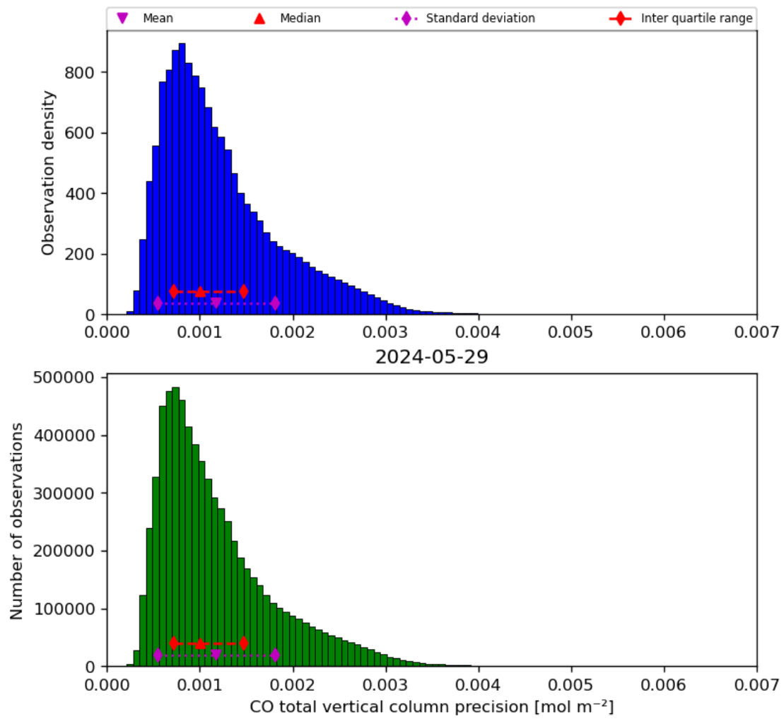
Figure 20: Histogram of “CO total vertical column precision” for 2024-05-28 to 2024-05-30
