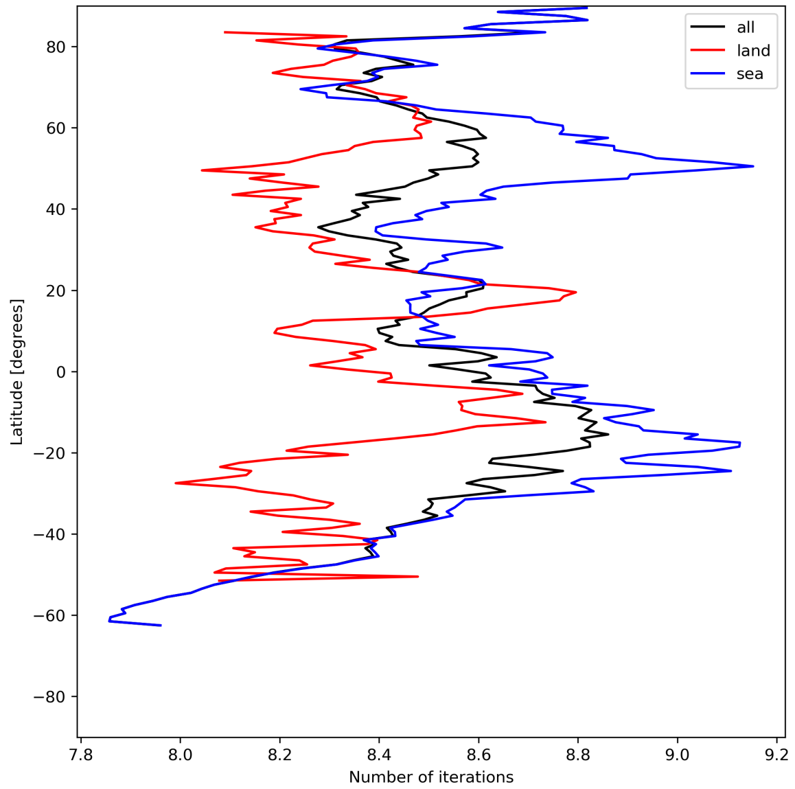
Figure 16: Zonal average of “Number of iterations” for 2024-05-28 to 2024-05-30.
