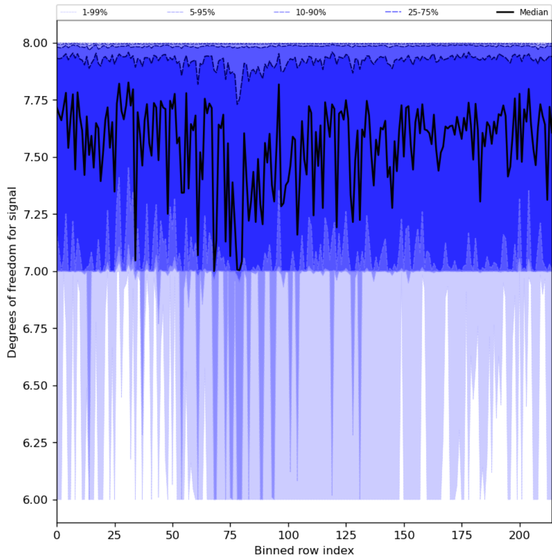
Figure 31: Along track statistics of “Degrees of freedom for signal” for 2024-05-28 to 2024-05-30
