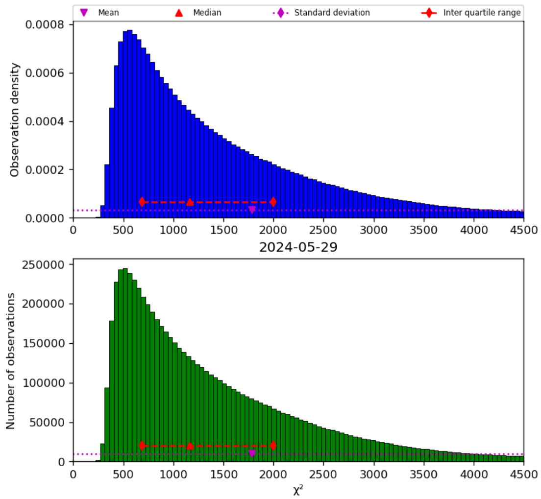
Figure 22: Histogram of “ \chi^2 ” for 2024-05-28 to 2024-05-30
