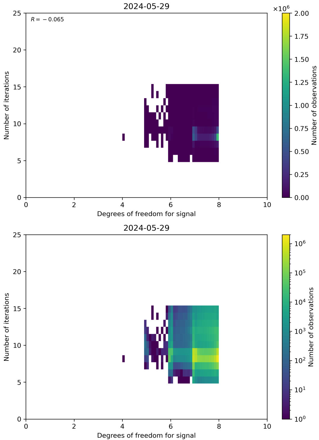
Figure 50: Scatter density plot of “Degrees of freedom for signal” against “Number of iterations” for 2024-05-28 to 2024-05-30.
