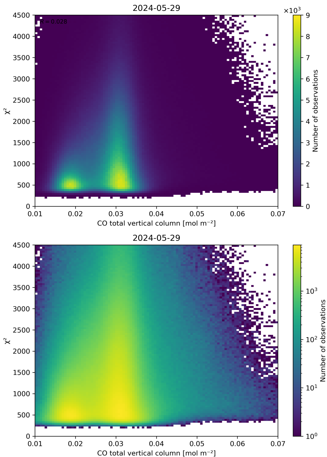
Figure 35: Scatter density plot of “CO total vertical column” against “ \chi^2 ” for 2024-05-28 to 2024-05-30.
