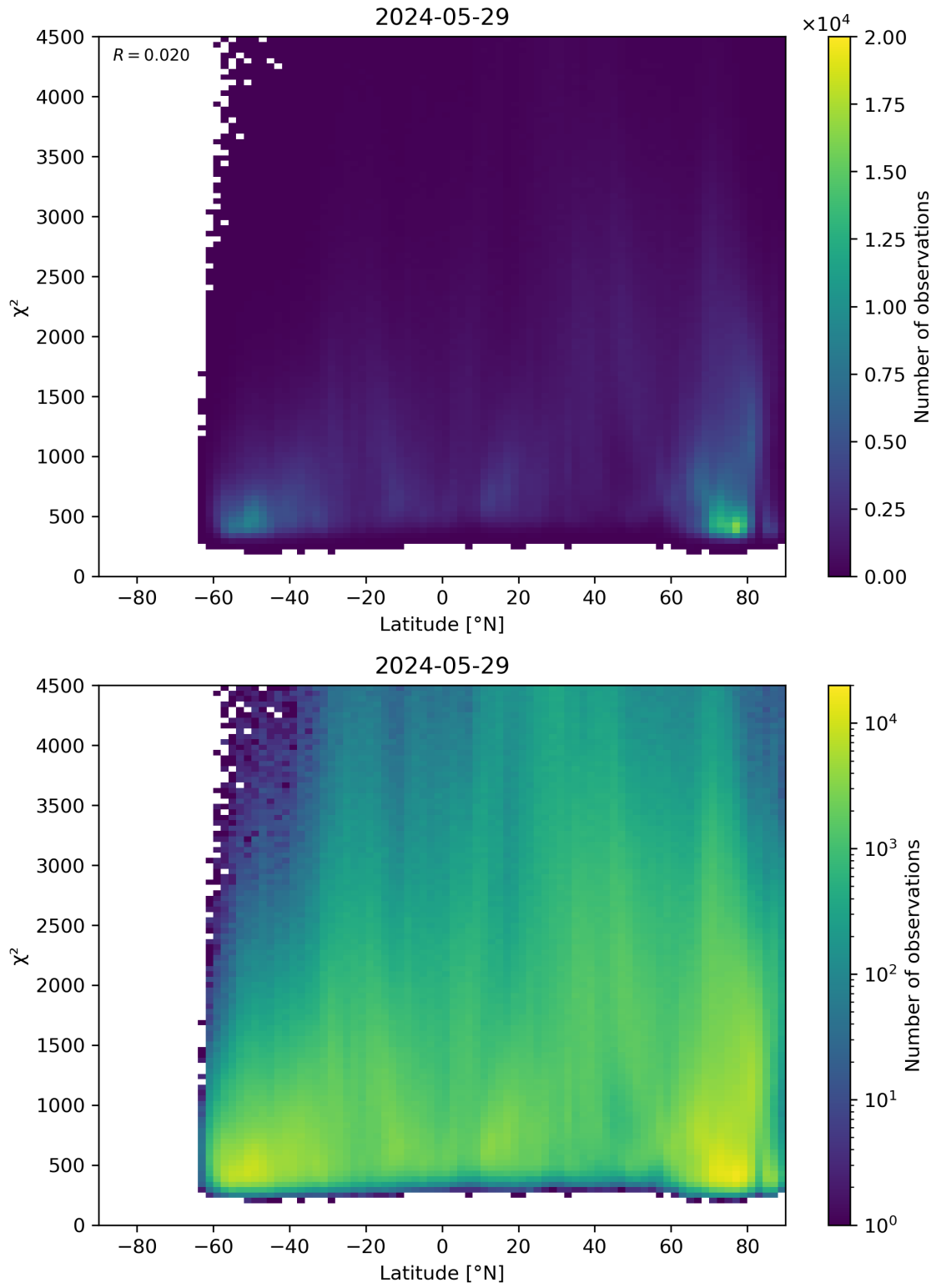
Figure 54: Scatter density plot of “Latitude” against “ \chi^2 ” for 2024-05-28 to 2024-05-30.
