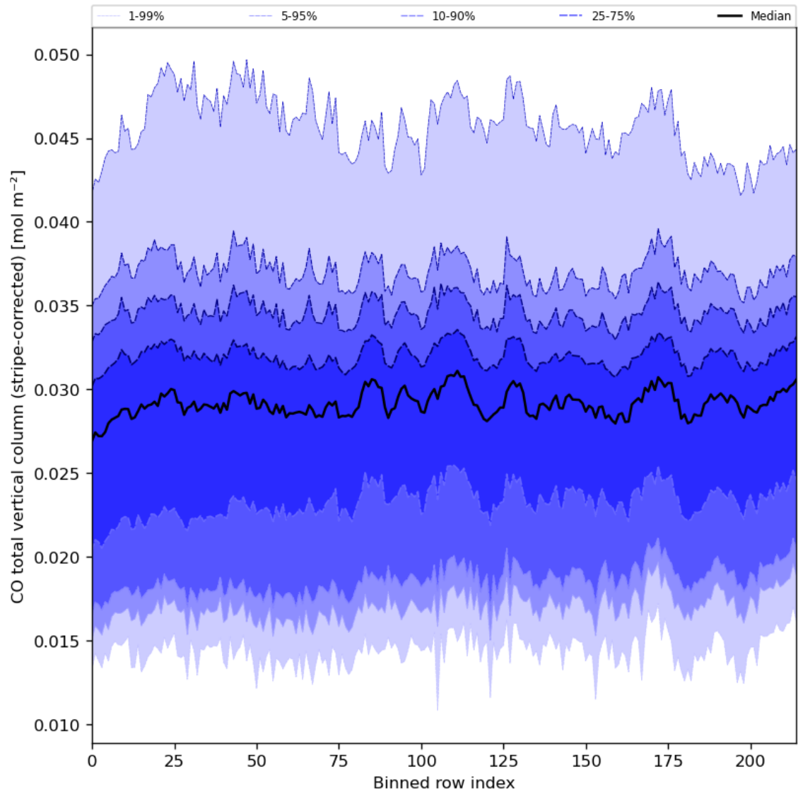
Figure 27: Along track statistics of “CO total vertical column (stripe-corrected)” for 2024-05-28 to 2024-05-30
