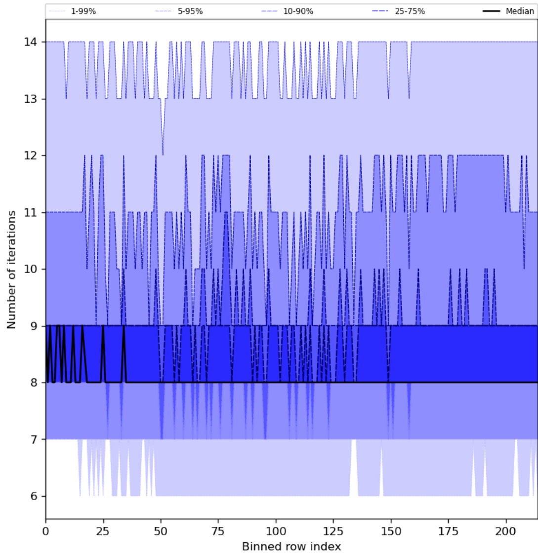
Figure 32: Along track statistics of “Number of iterations” for 2024-05-28 to 2024-05-30
