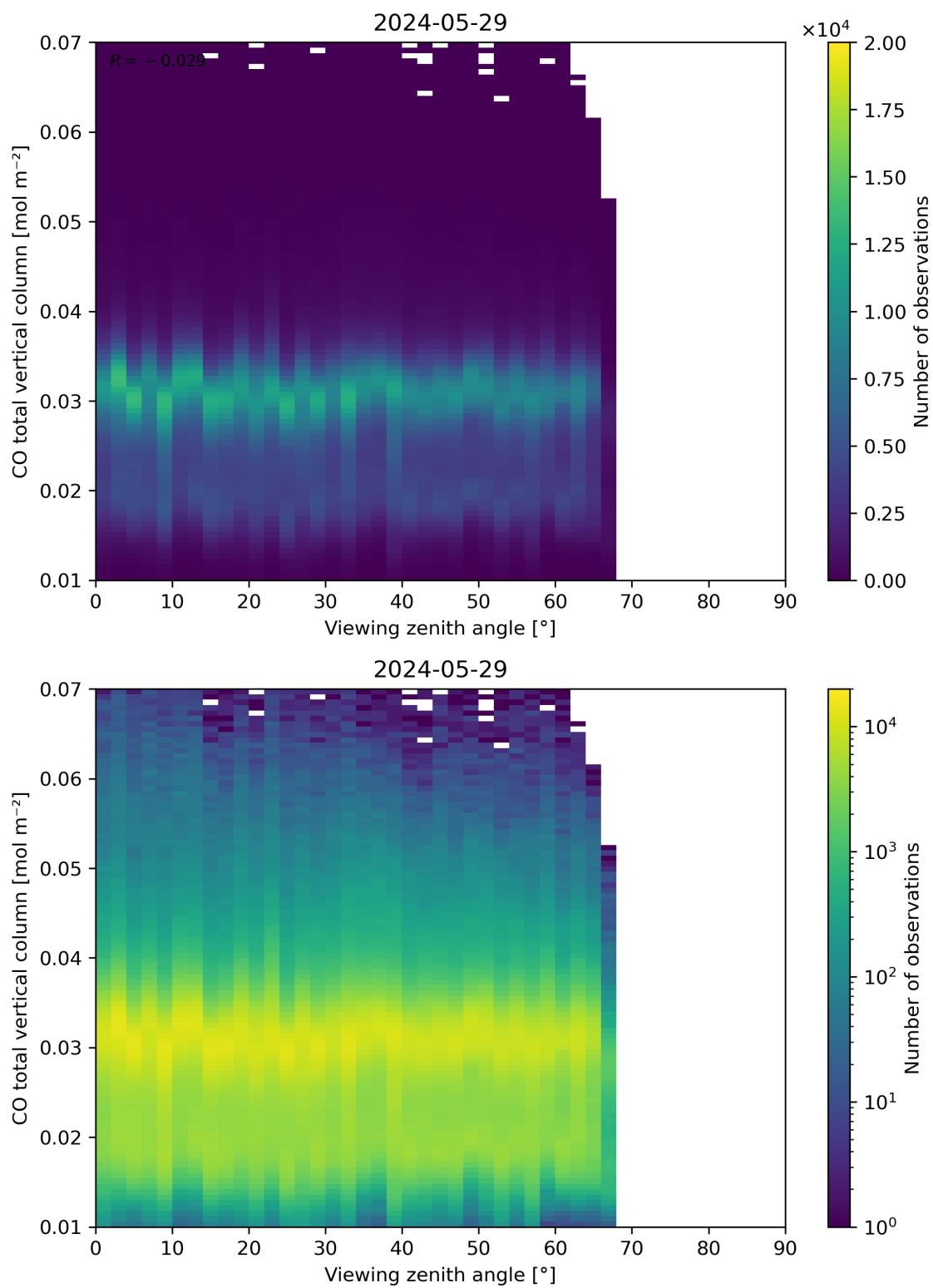
Figure 69: Scatter density plot of “Viewing zenith angle” against “CO total vertical column” for 2024-05-28 to 2024-05-30.
