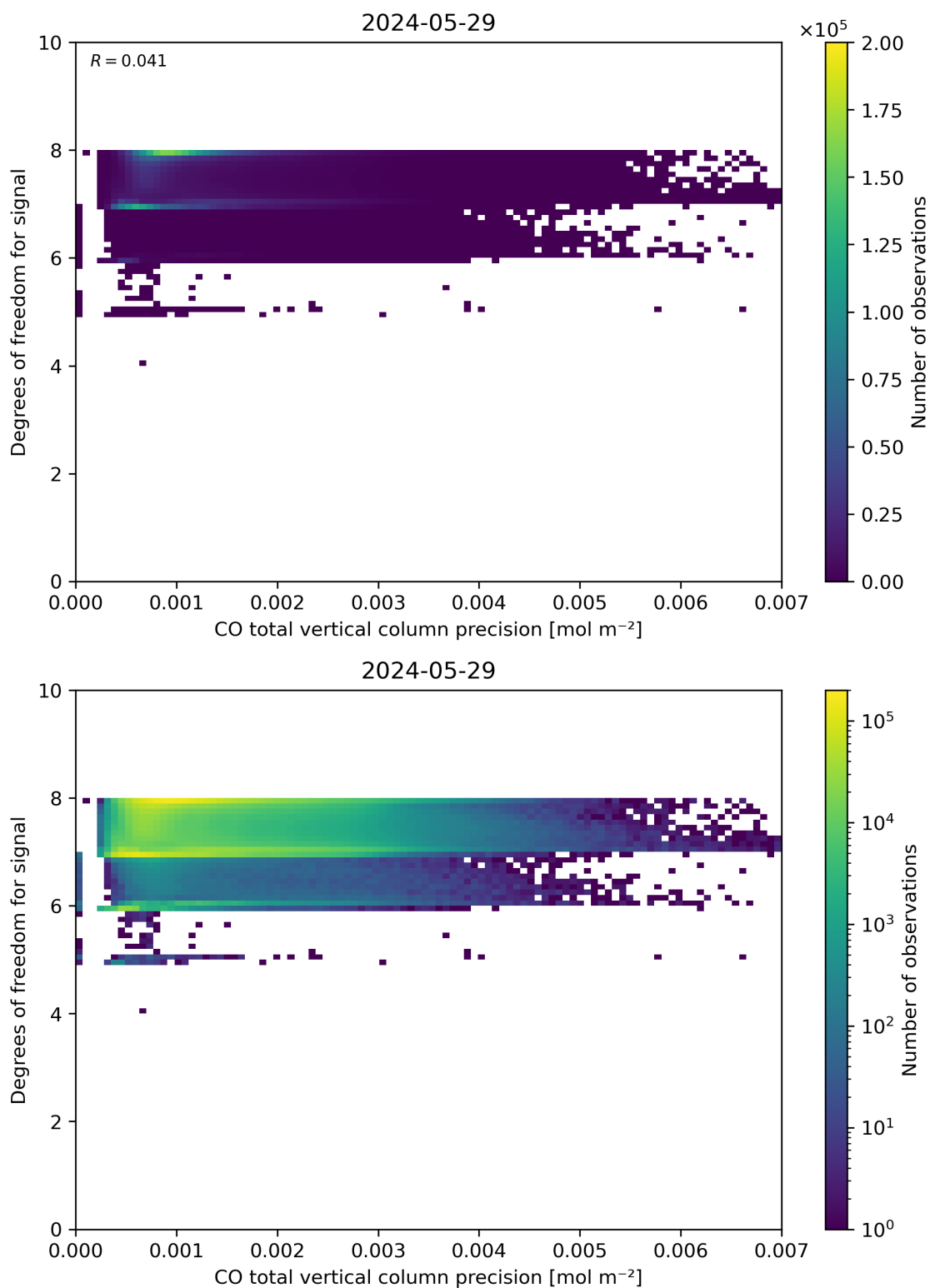
Figure 45: Scatter density plot of “CO total vertical column precision” against “Degrees of freedom for signal” for 2024-05-28 to 2024-05-30.
