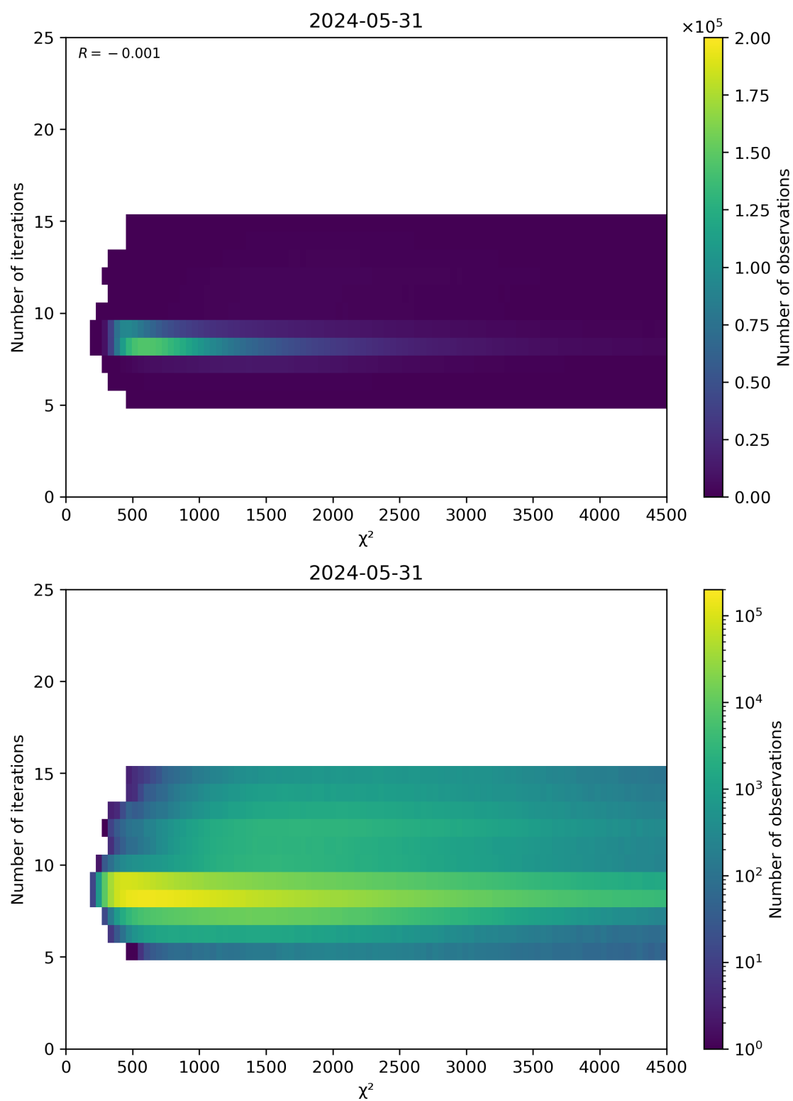
Figure 49: Scatter density plot of “ \chi^2 ” against “Number of iterations” for 2024-05-30 to 2024-06-01.
