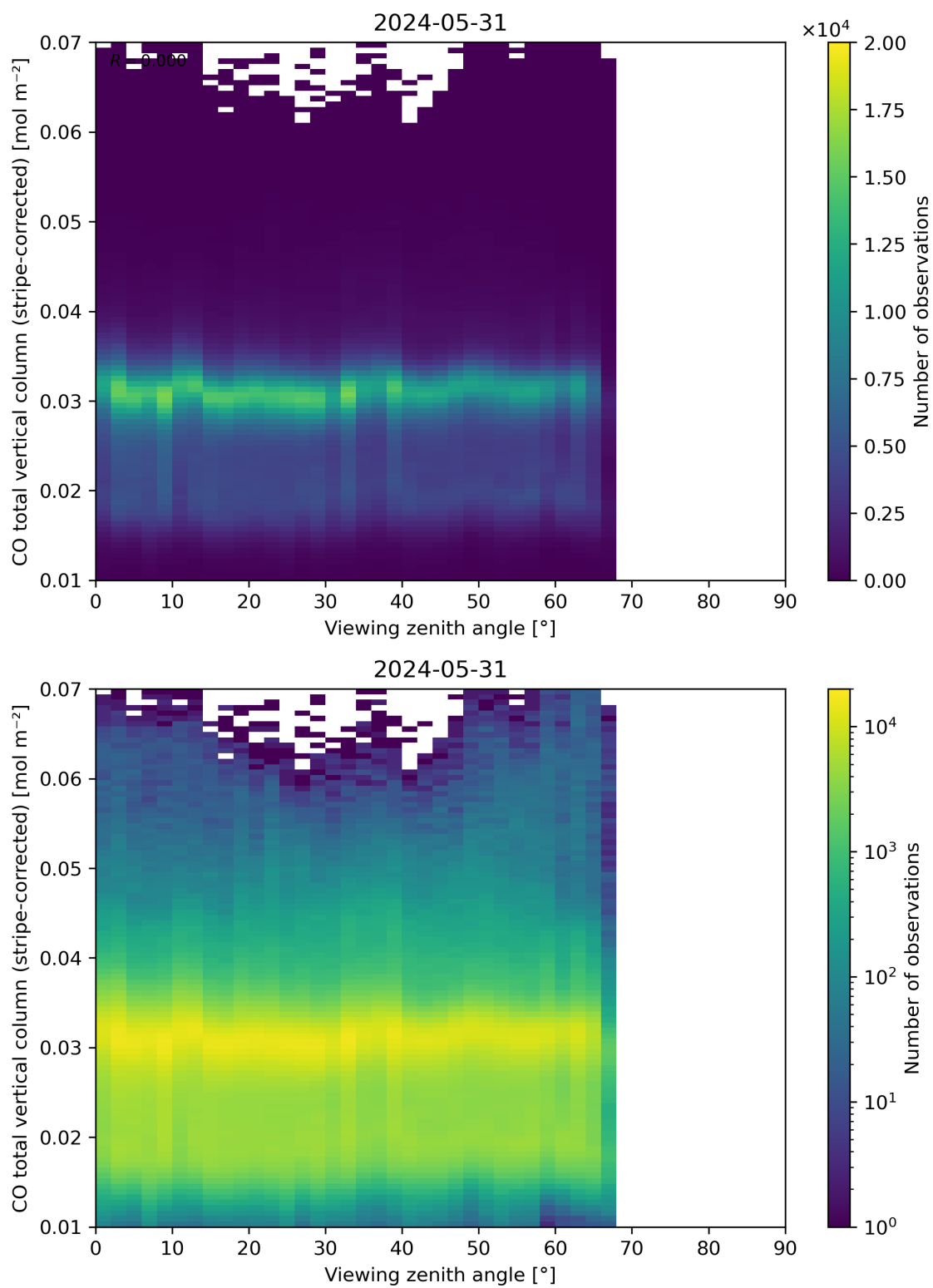
Figure 70: Scatter density plot of “Viewing zenith angle” against “CO total vertical column (stripe-corrected)” for 2024-05-30 to 2024-06-01.
