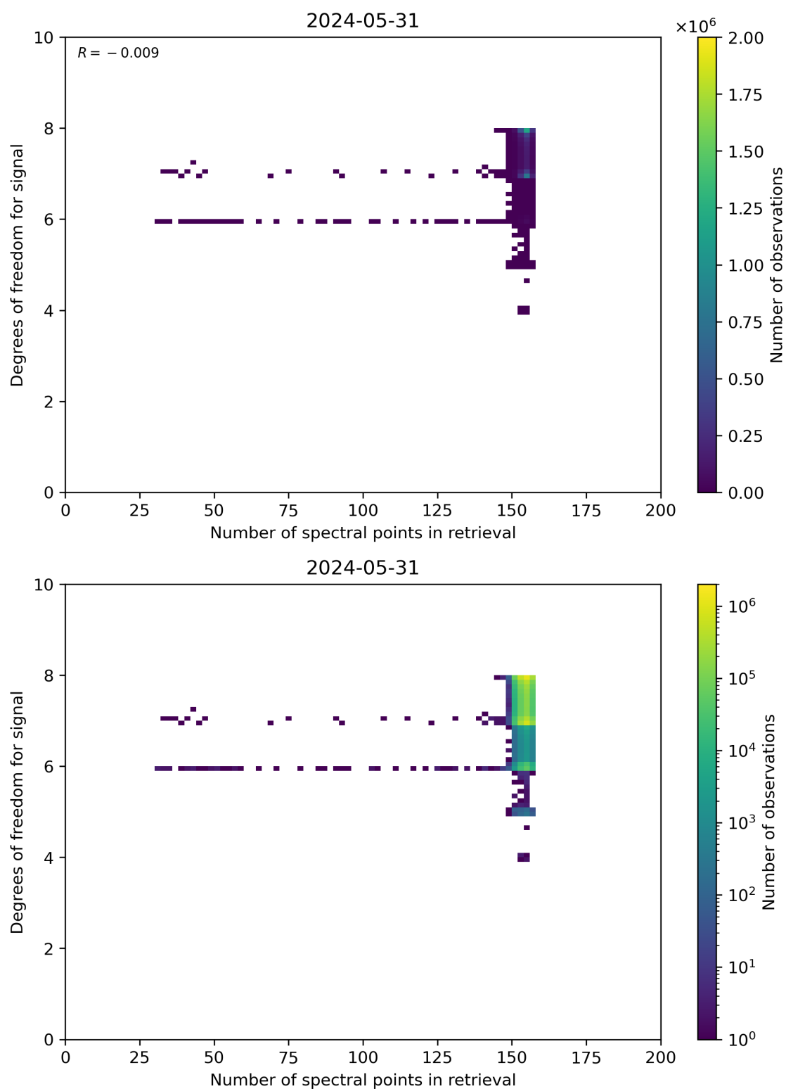
Figure 59: Scatter density plot of “Number of spectral points in retrieval” against “Degrees of freedom for signal” for 2024-05-30 to 2024-06-01.
