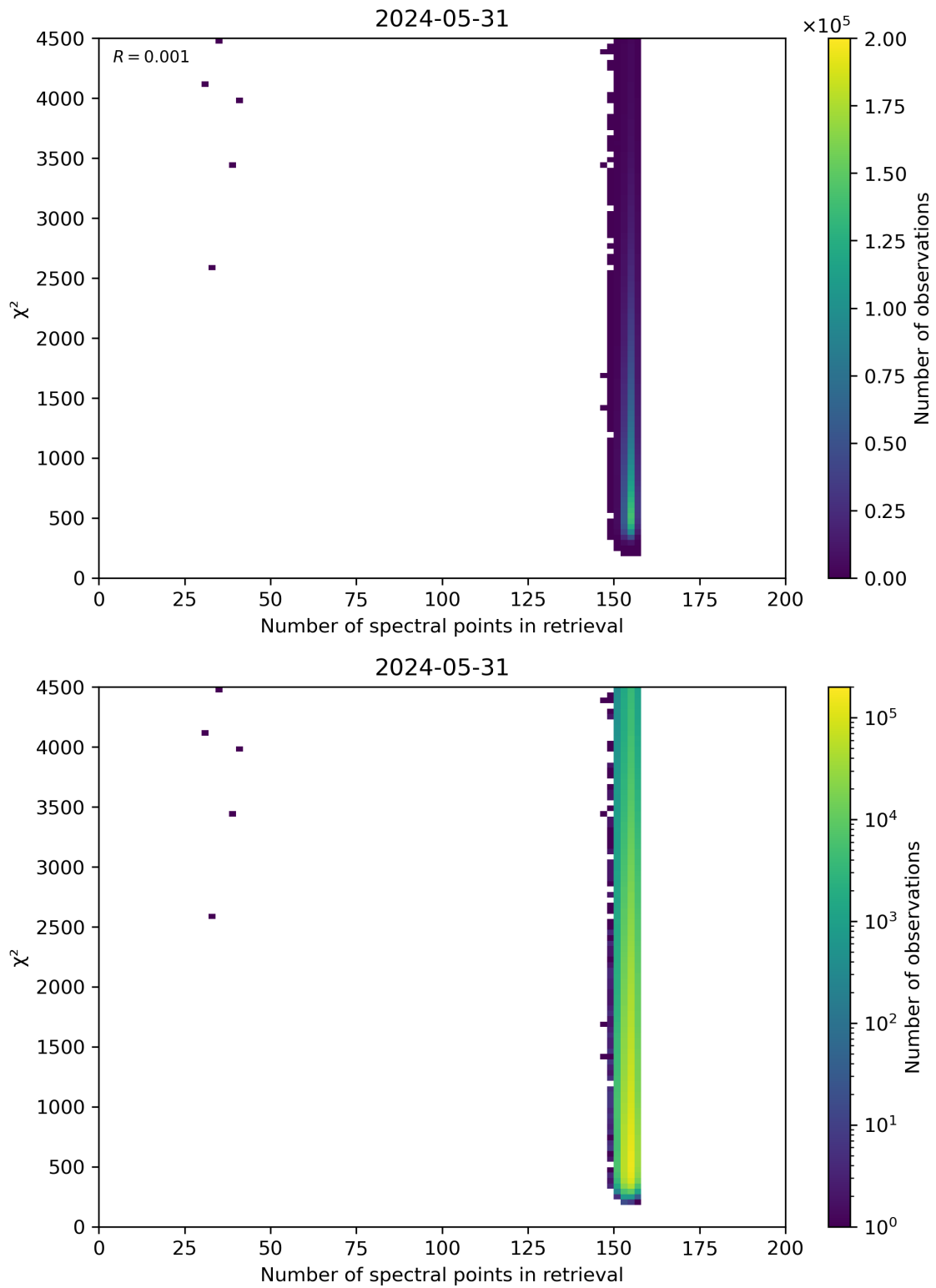
Figure 58: Scatter density plot of “Number of spectral points in retrieval” against “ \chi^2 ” for 2024-05-30 to 2024-06-01.
