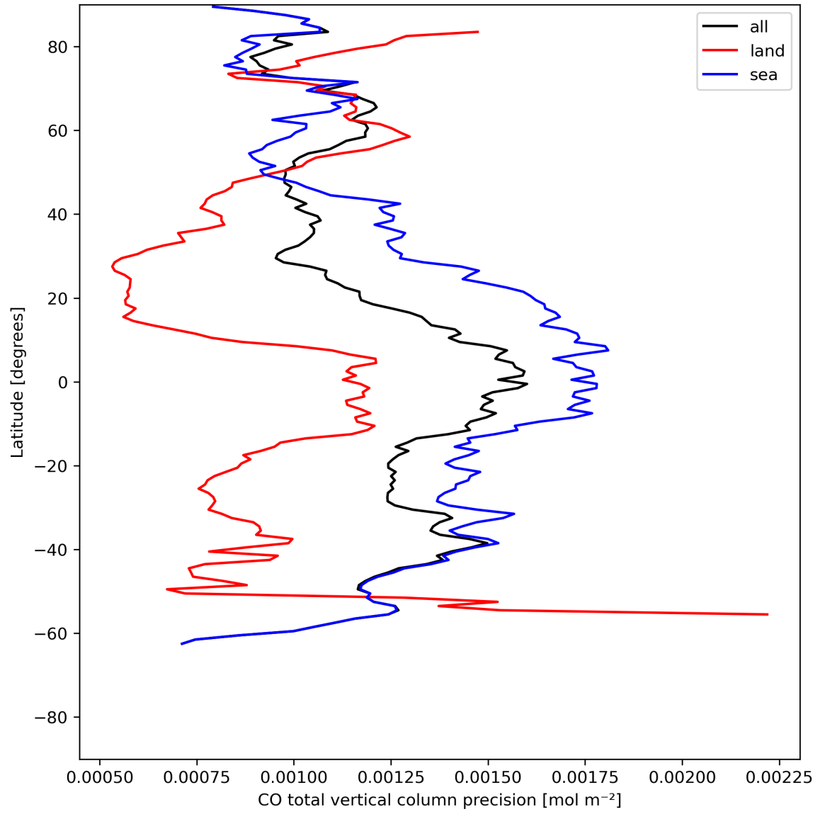
Figure 12: Zonal average of “CO total vertical column precision” for 2024-05-30 to 2024-06-01.
