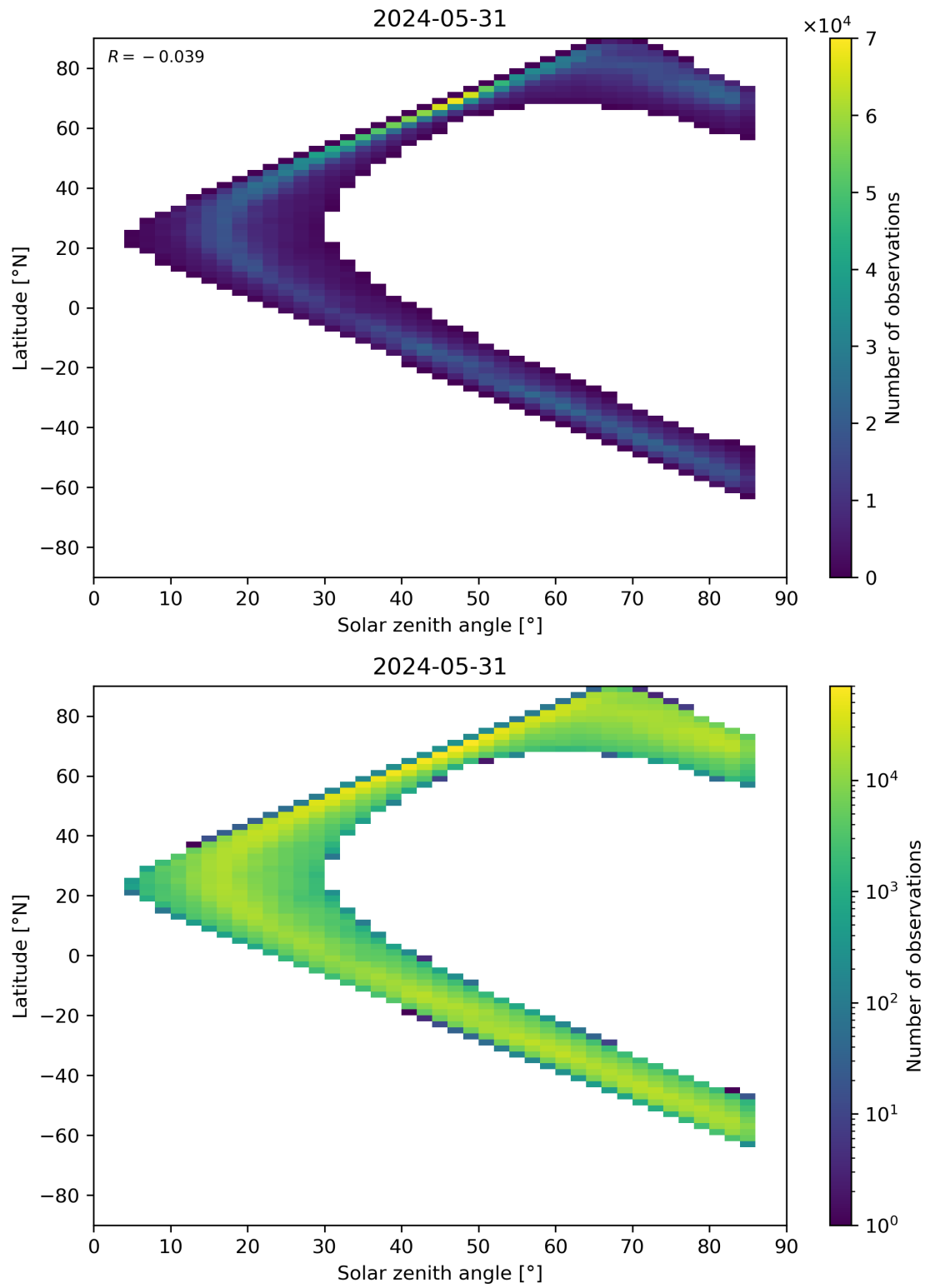
Figure 66: Scatter density plot of “Solar zenith angle” against “Latitude” for 2024-05-30 to 2024-06-01.
