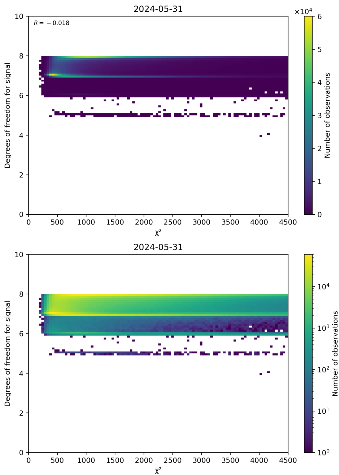
Figure 48: Scatter density plot of “ \chi^2 ” against “Degrees of freedom for signal” for 2024-05-30 to 2024-06-01.
