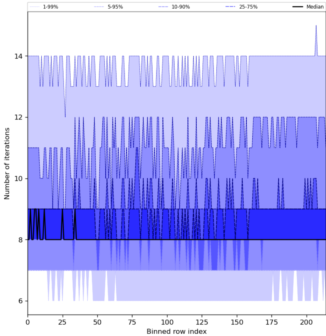
Figure 32: Along track statistics of “Number of iterations” for 2024-05-30 to 2024-06-01
