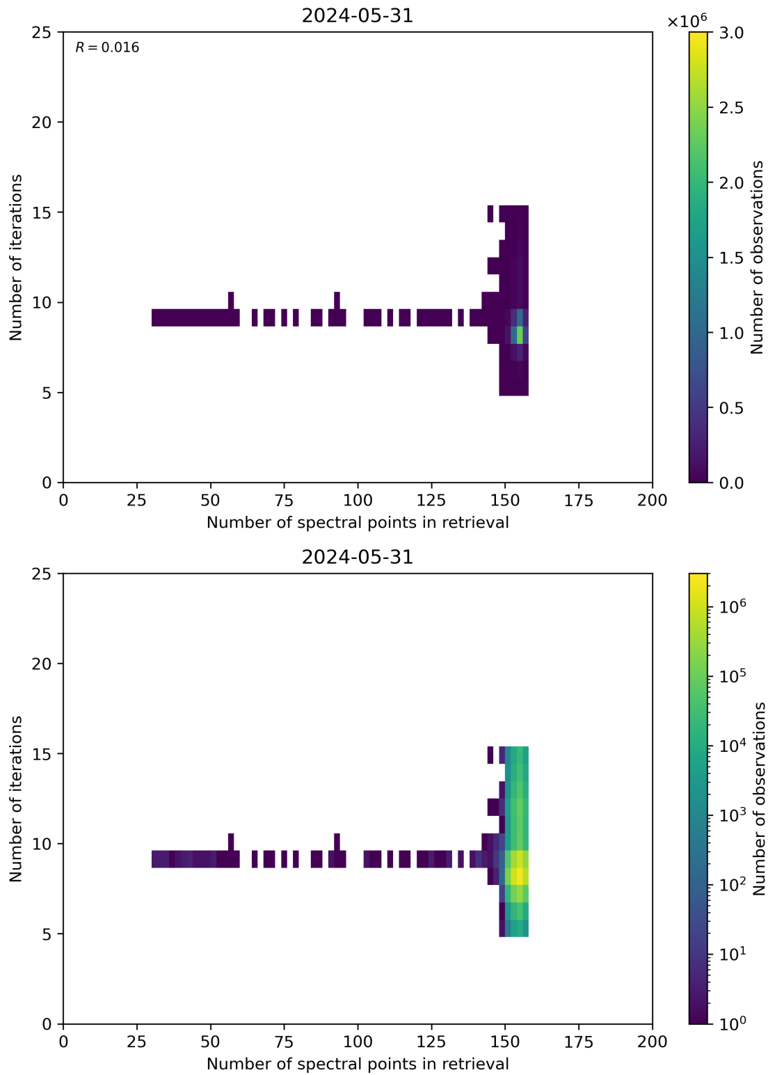
Figure 60: Scatter density plot of “Number of spectral points in retrieval” against “Number of iterations” for 2024-05-30 to 2024-06-01.
