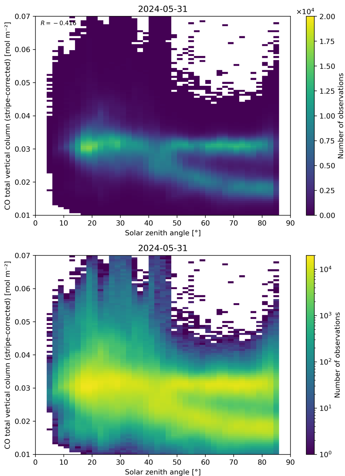
Figure 62: Scatter density plot of “Solar zenith angle” against “CO total vertical column (stripe-corrected)” for 2024-05-30 to 2024-06-01.
