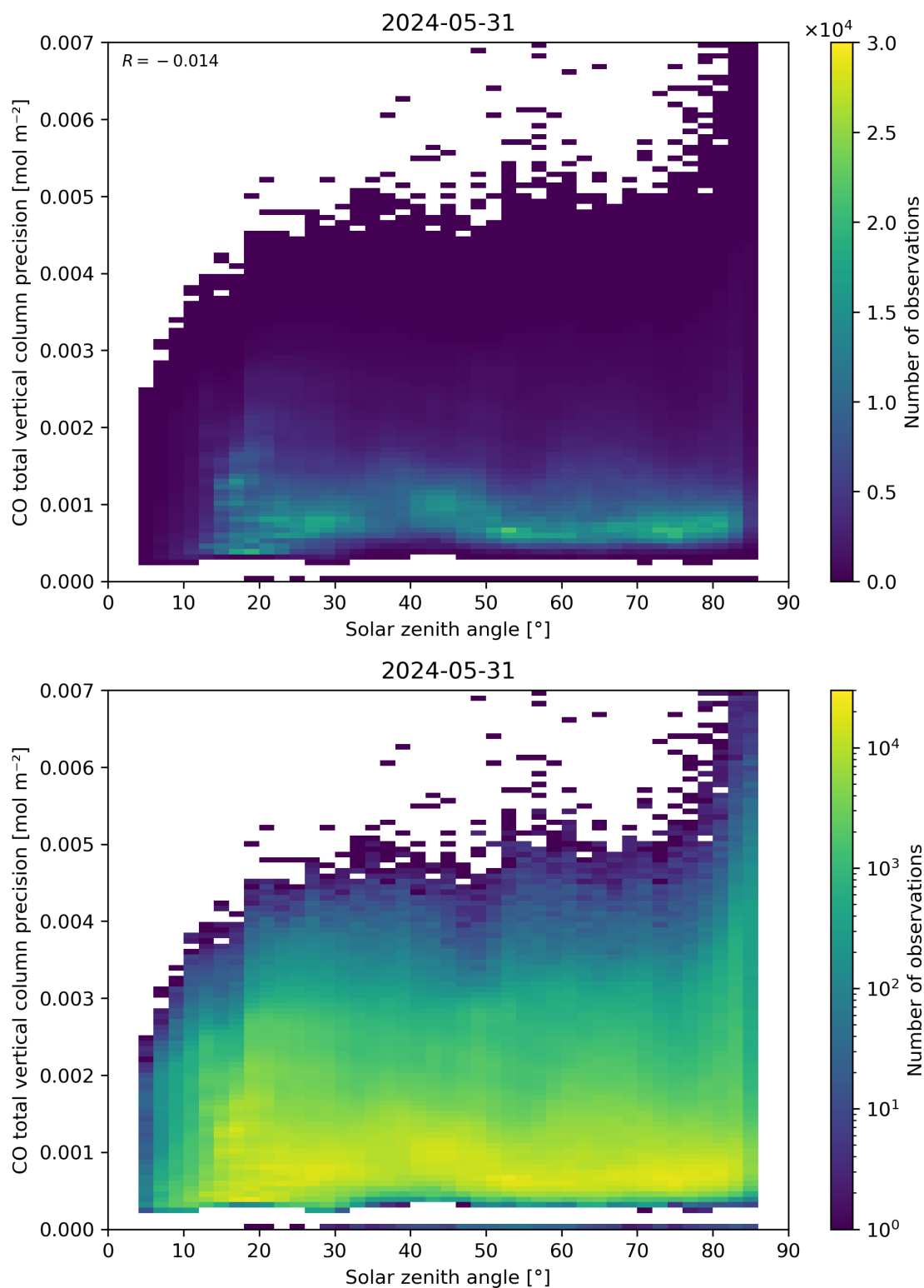
Figure 63: Scatter density plot of “Solar zenith angle” against “CO total vertical column precision” for 2024-05-30 to 2024-06-01.
