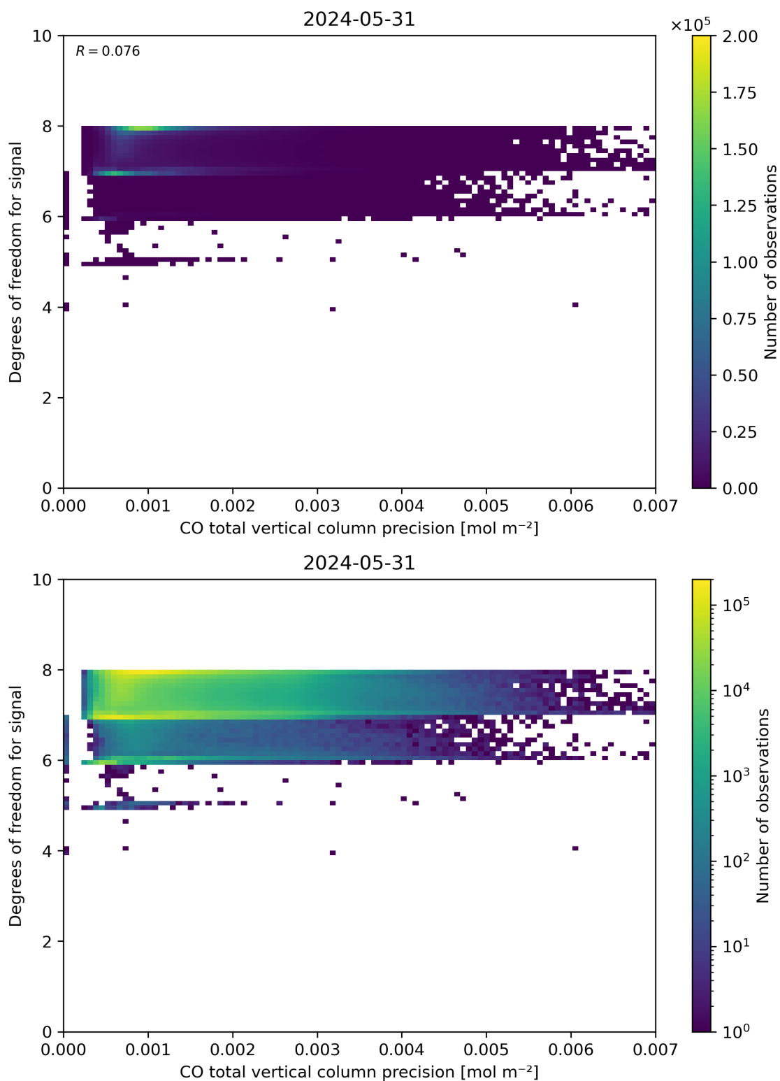
Figure 45: Scatter density plot of “CO total vertical column precision” against “Degrees of freedom for signal” for 2024-05-30 to 2024-06-01.
