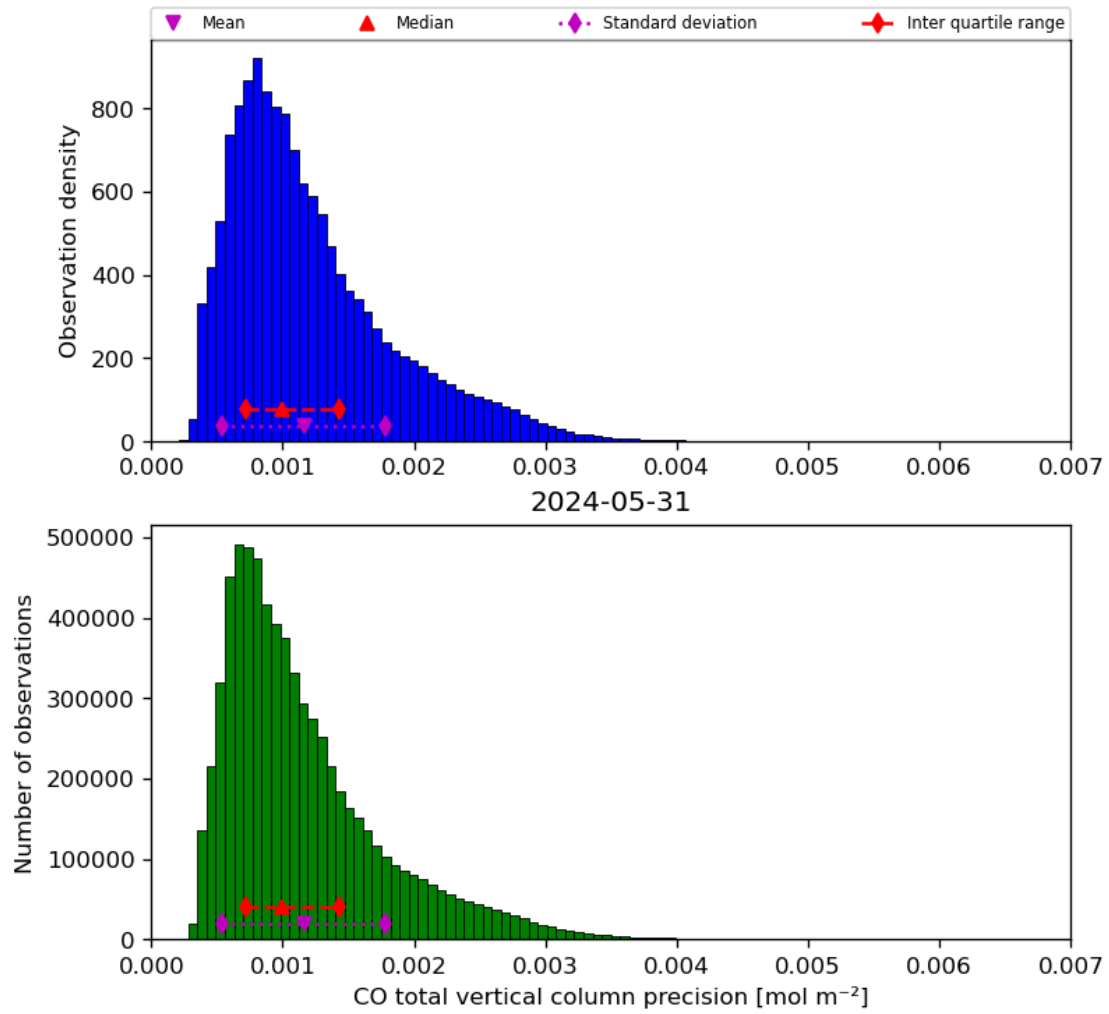
Figure 20: Histogram of “CO total vertical column precision” for 2024-05-30 to 2024-06-01
