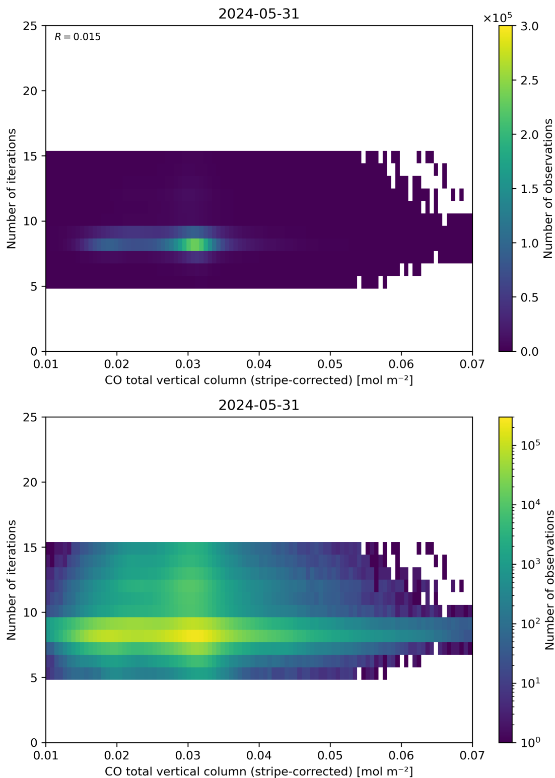
Figure 39: Scatter density plot of “CO total vertical column (stripe-corrected)” against “Number of iterations” for 2024-05-30 to 2024-06-01.
