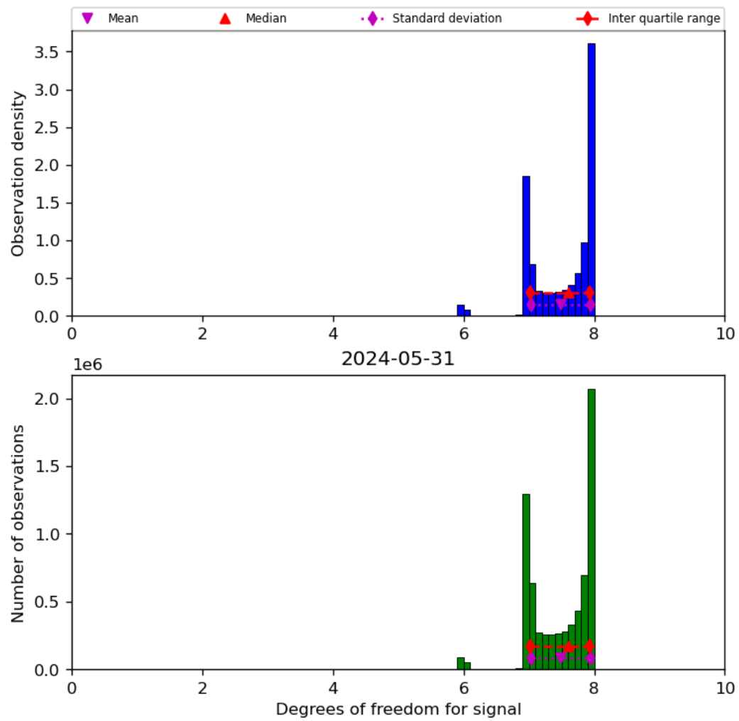
Figure 23: Histogram of “Degrees of freedom for signal” for 2024-05-30 to 2024-06-01
