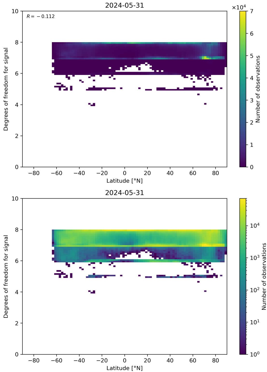
Figure 55: Scatter density plot of “Latitude” against “Degrees of freedom for signal” for 2024-05-30 to 2024-06-01.
