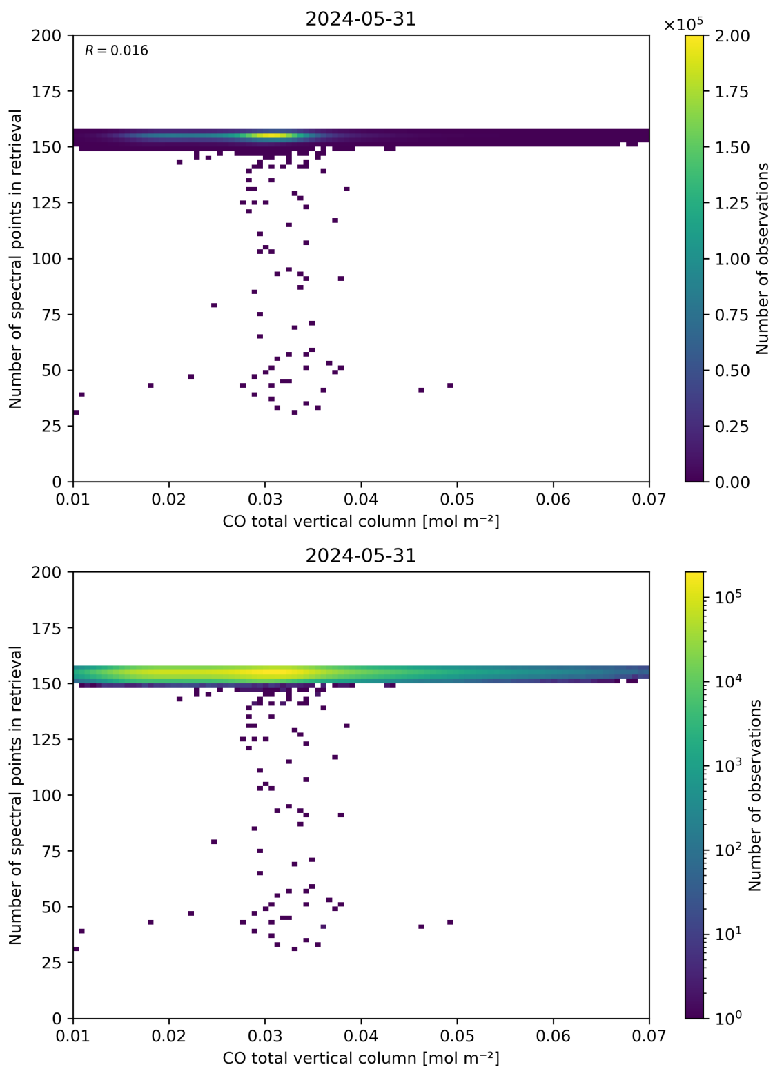
Figure 43: Scatter density plot of “CO total vertical column” against “Number of spectral points in retrieval” for 2024-05-30 to 2024-06-01.
