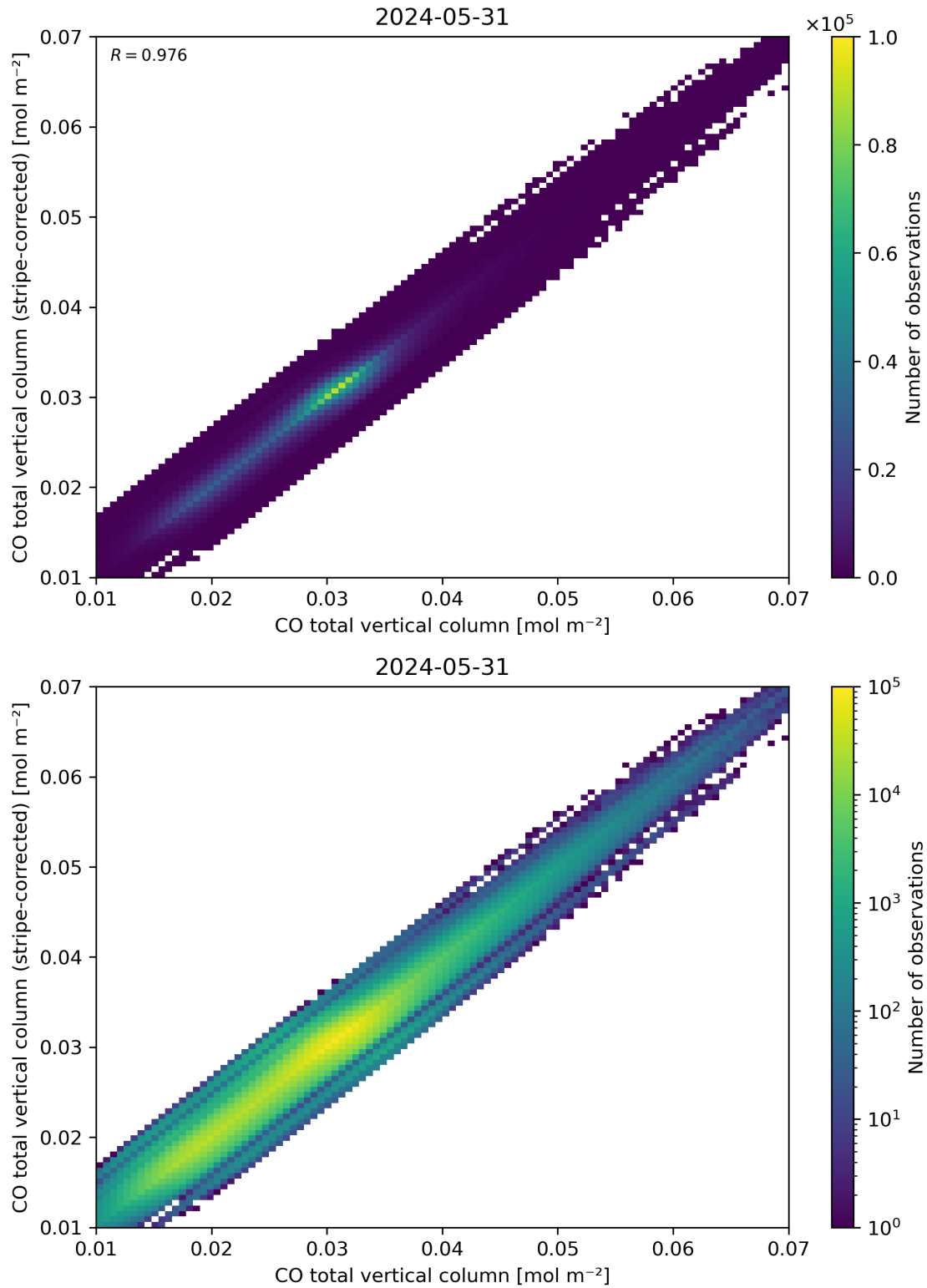
Figure 33: Scatter density plot of “CO total vertical column” against “CO total vertical column (stripe-corrected)” for 2024-05-30 to 2024-06-01.
