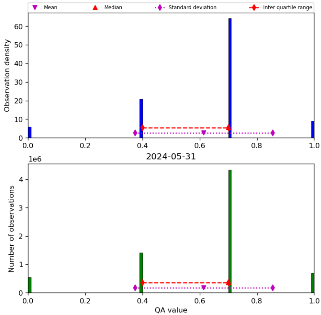
Figure 17: Histogram of “QA value” for 2024-05-30 to 2024-06-01
