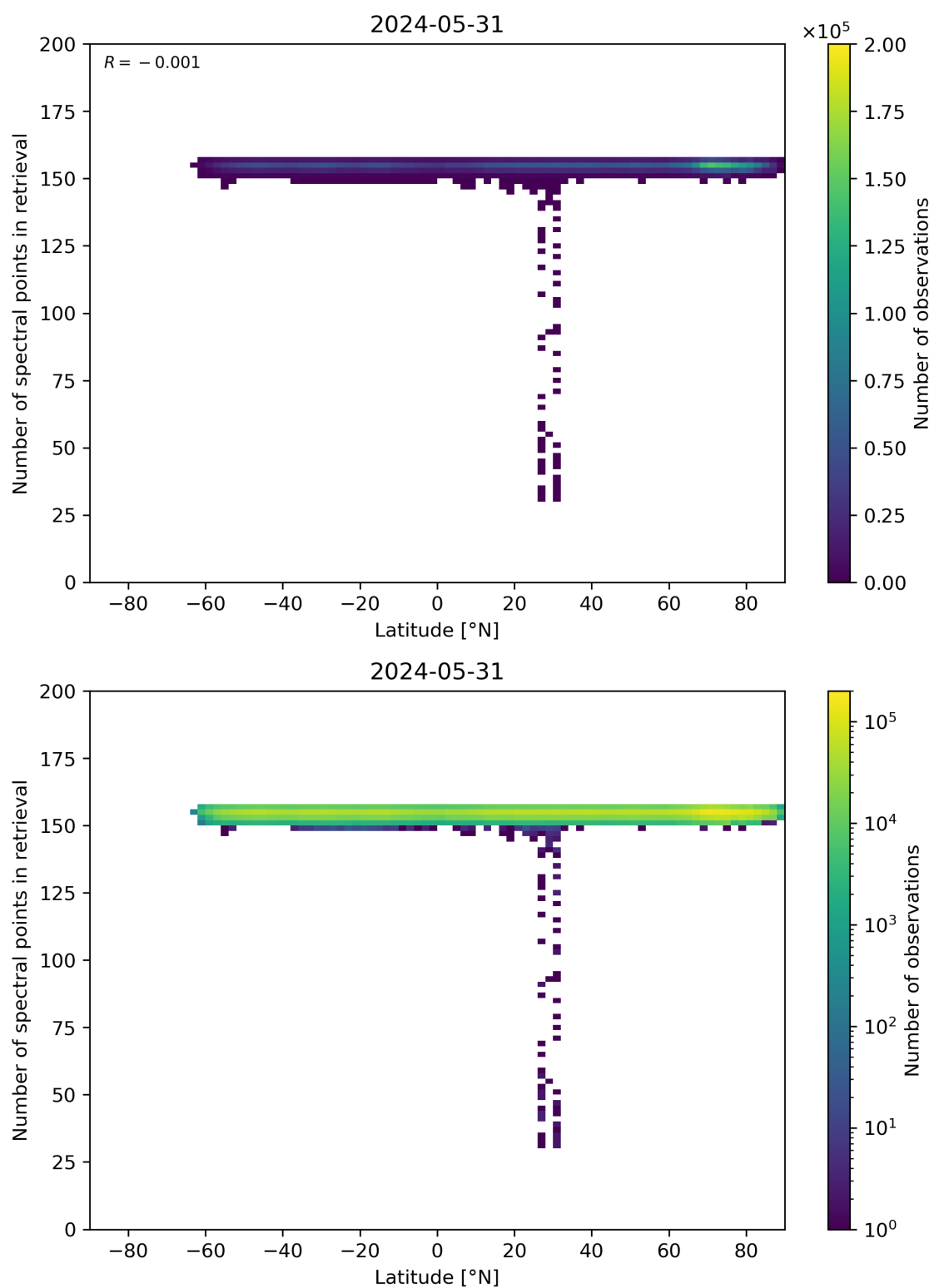
Figure 57: Scatter density plot of “Latitude” against “Number of spectral points in retrieval” for 2024-05-30 to 2024-06-01.
