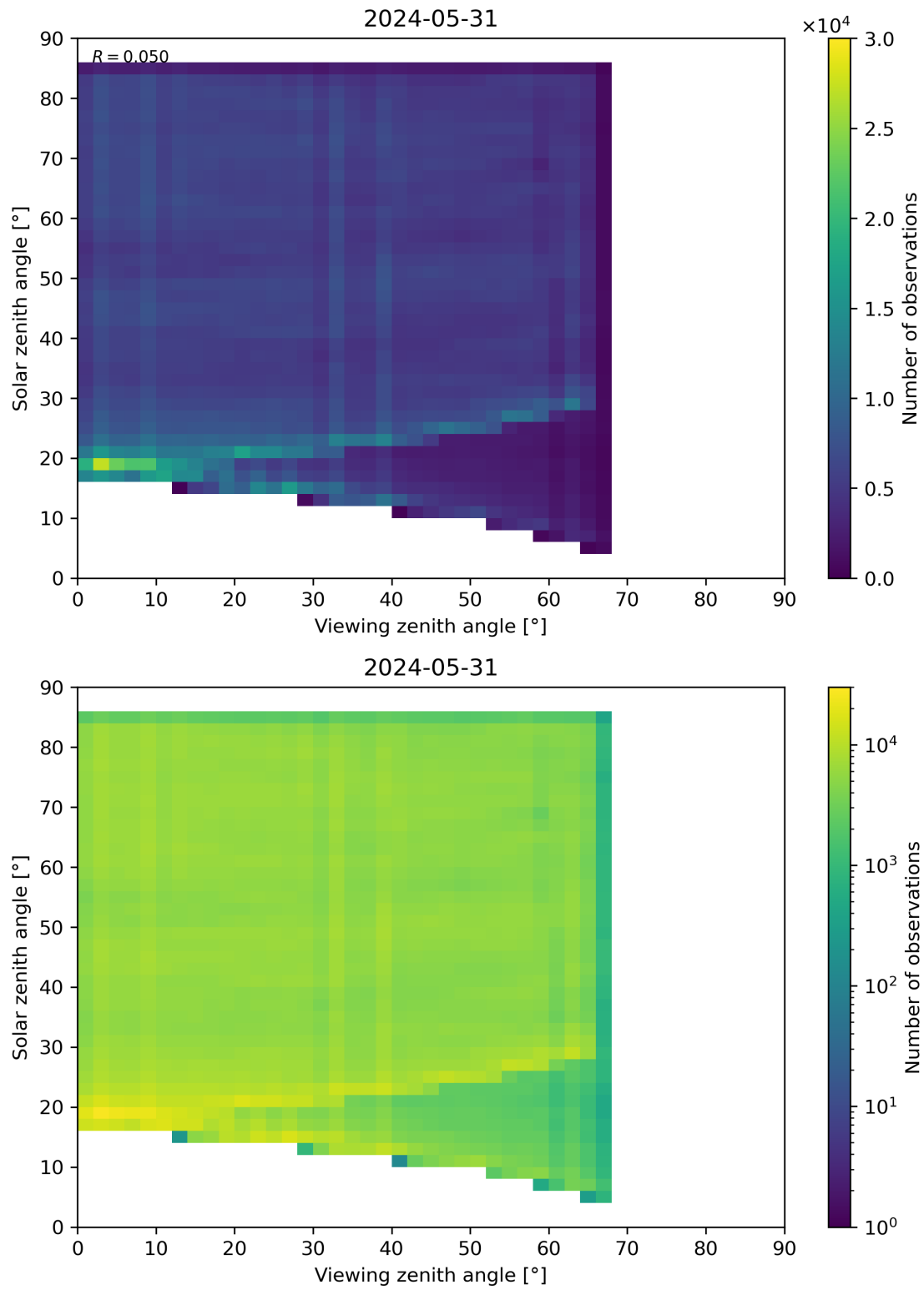
Figure 77: Scatter density plot of “Viewing zenith angle” against “Solar zenith angle” for 2024-05-30 to 2024-06-01.
