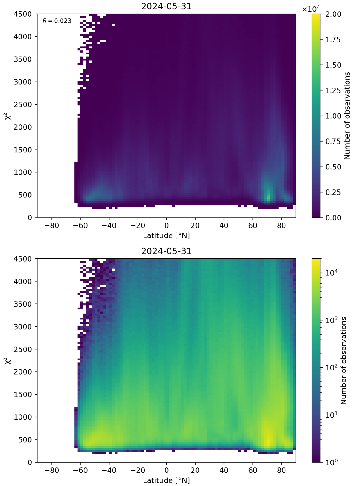
Figure 54: Scatter density plot of “Latitude” against “ \chi^2 ” for 2024-05-30 to 2024-06-01.
