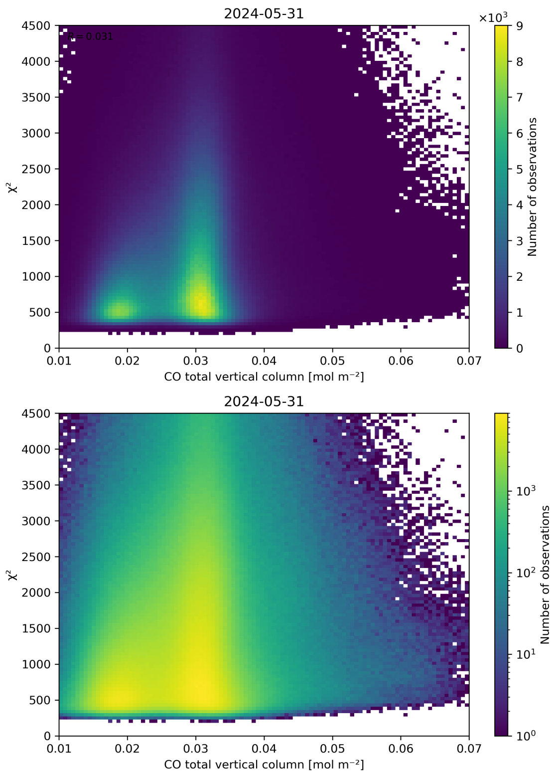
Figure 35: Scatter density plot of “CO total vertical column” against “ \chi^2 ” for 2024-05-30 to 2024-06-01.
