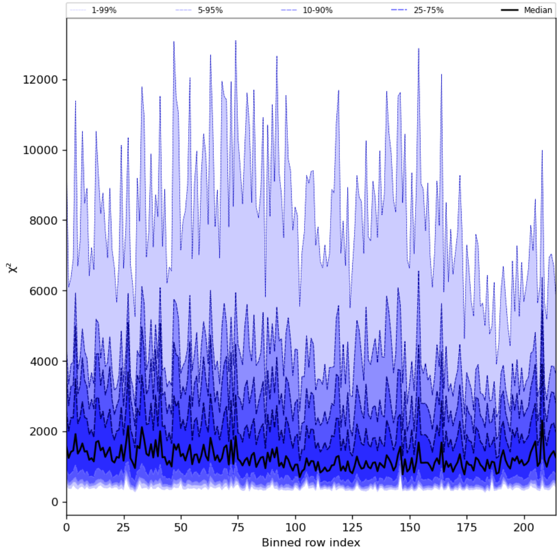
Figure 30: Along track statistics of “ \chi^2 ” for 2024-05-30 to 2024-06-01
