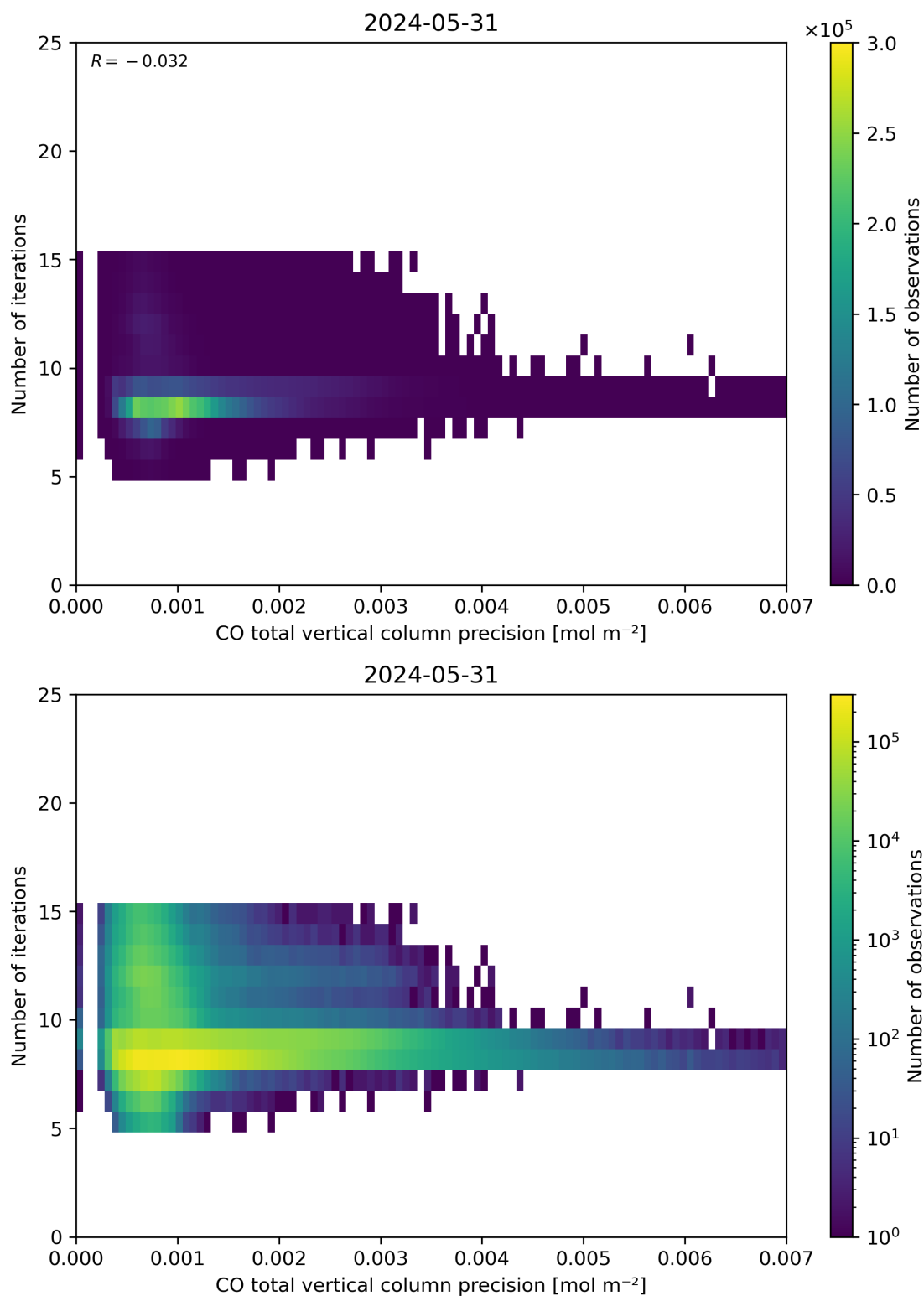
Figure 46: Scatter density plot of “CO total vertical column precision” against “Number of iterations” for 2024-05-30 to 2024-06-01.
