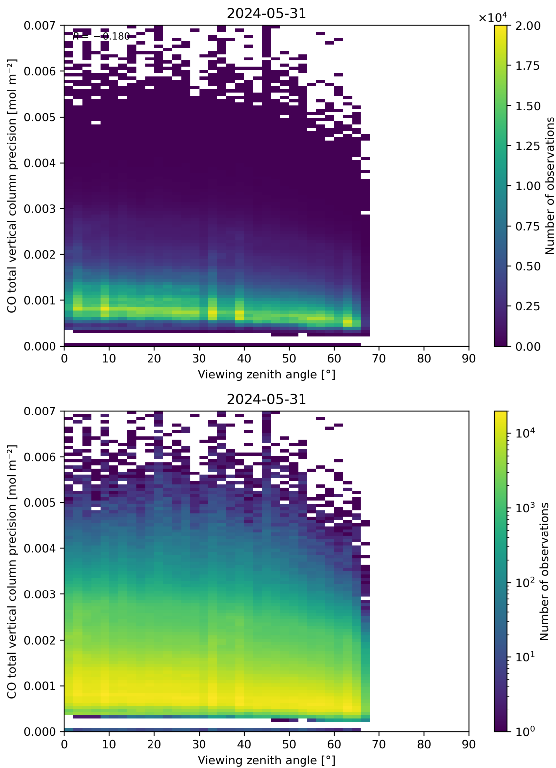
Figure 71: Scatter density plot of “Viewing zenith angle” against “CO total vertical column precision” for 2024-05-30 to 2024-06-01.
