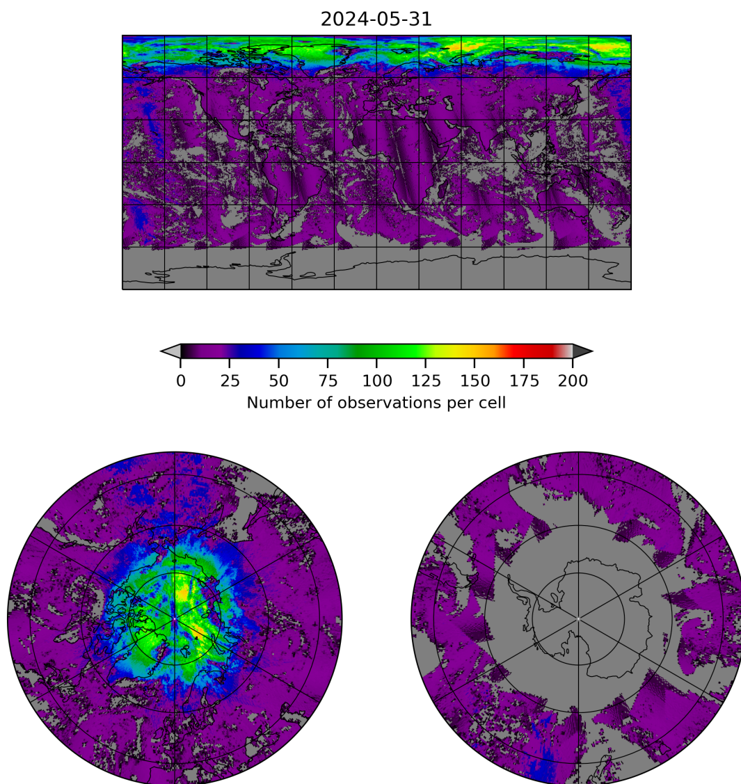
Figure 8: Map of the number of observations for 2024-05-30 to 2024-06-01
