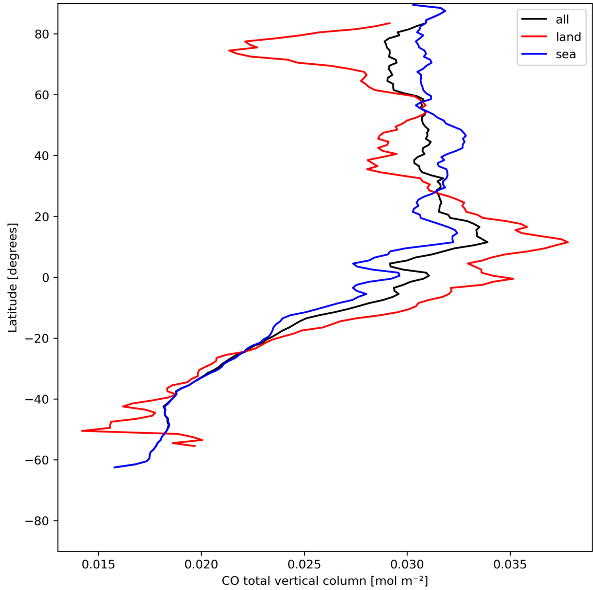
Figure 10: Zonal average of “CO total vertical column” for 2024-05-30 to 2024-06-01.
