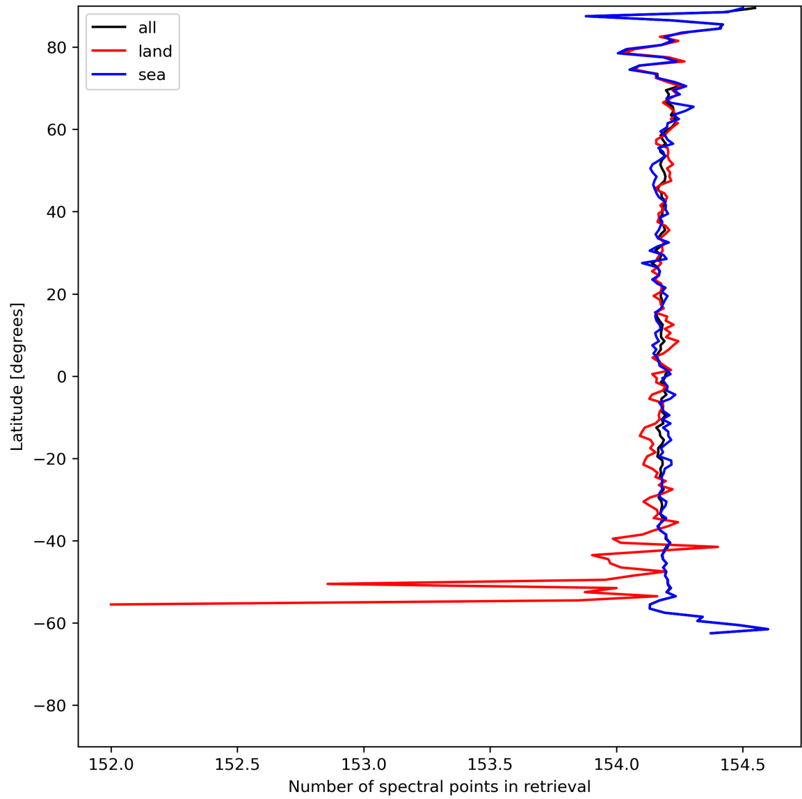
Figure 13: Zonal average of “Number of spectral points in retrieval” for 2024-05-30 to 2024-06-01.
