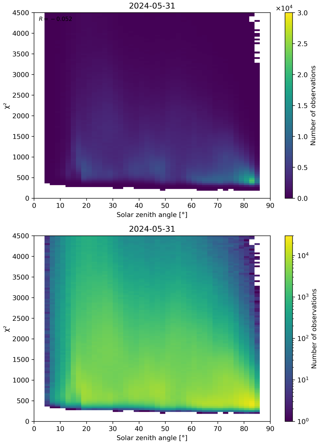
Figure 64: Scatter density plot of “Solar zenith angle” against “ \chi^2 ” for 2024-05-30 to 2024-06-01.
