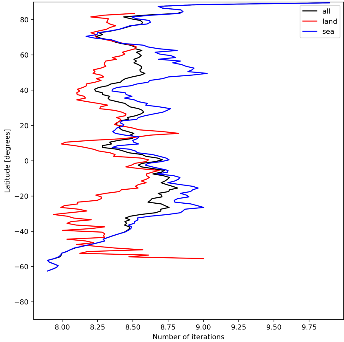
Figure 16: Zonal average of “Number of iterations” for 2024-05-30 to 2024-06-01.
