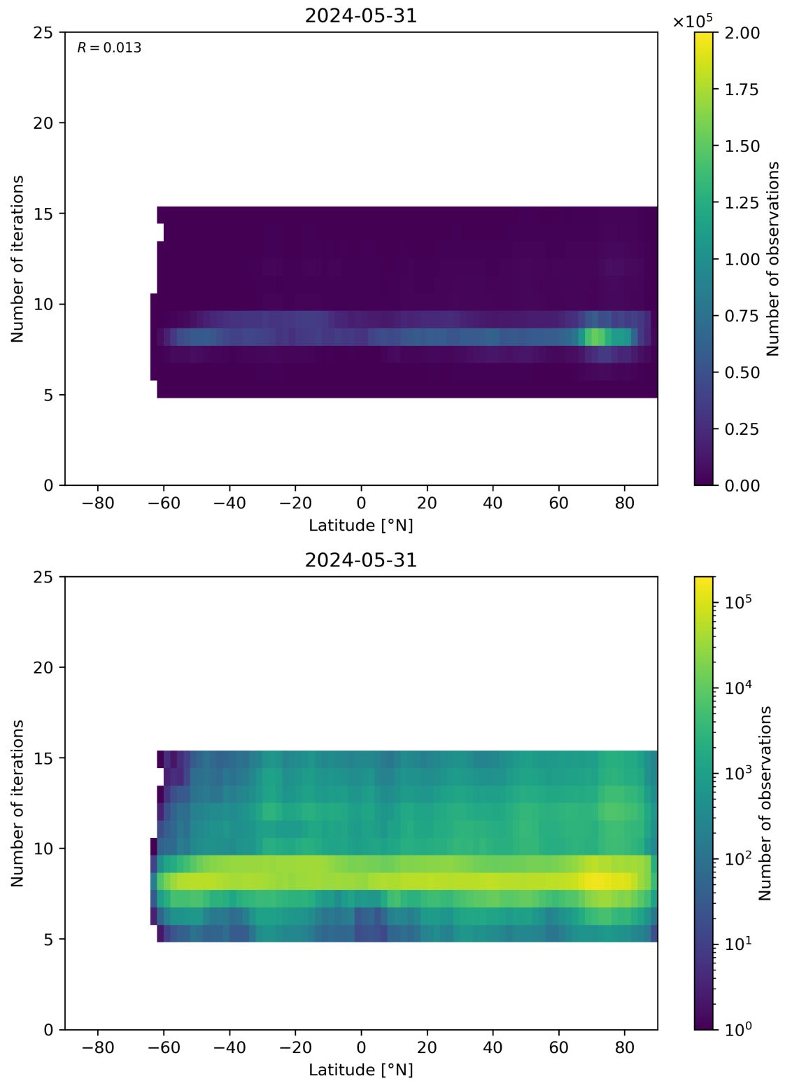
Figure 56: Scatter density plot of “Latitude” against “Number of iterations” for 2024-05-30 to 2024-06-01.
