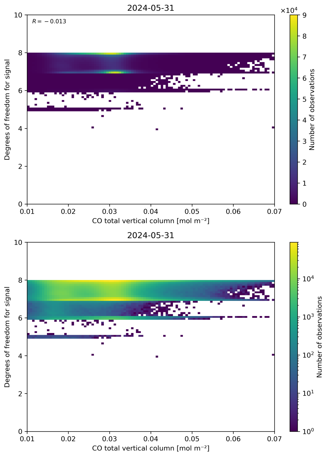
Figure 41: Scatter density plot of “CO total vertical column” against “Degrees of freedom for signal” for 2024-05-30 to 2024-06-01.
