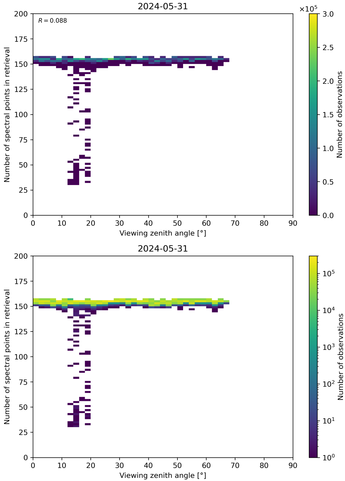
Figure 76: Scatter density plot of “Viewing zenith angle” against “Number of spectral points in retrieval” for 2024-05-30 to 2024-06-01.
