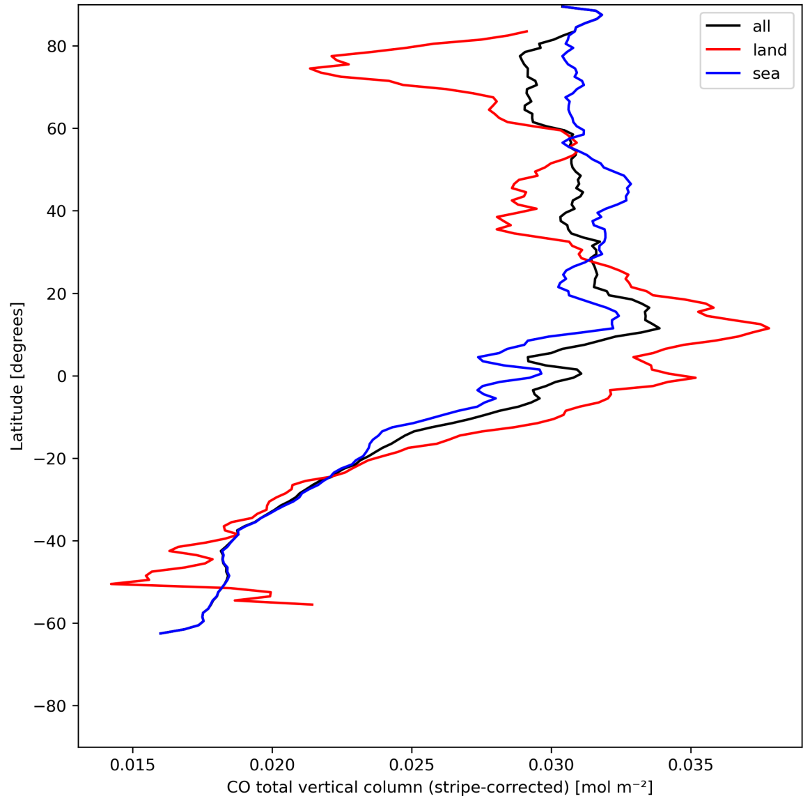
Figure 11: Zonal average of “CO total vertical column (stripe-corrected)” for 2024-05-30 to 2024-06-01.
