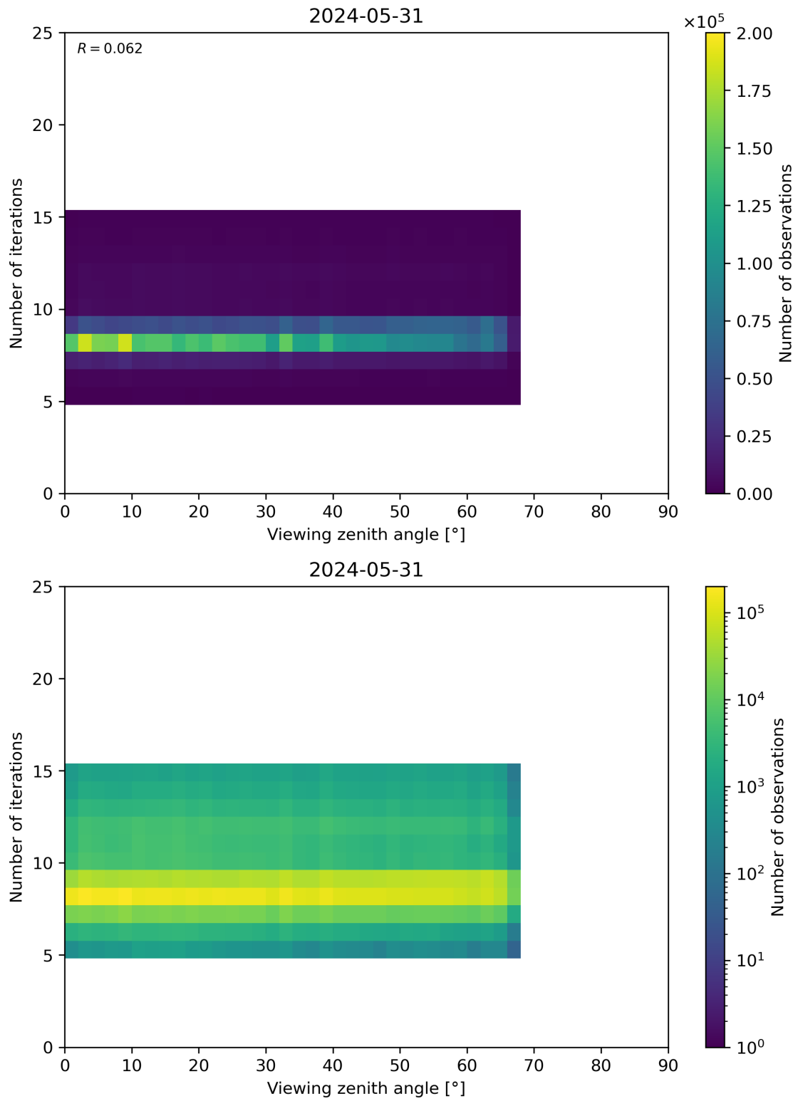
Figure 75: Scatter density plot of “Viewing zenith angle” against “Number of iterations” for 2024-05-30 to 2024-06-01.
