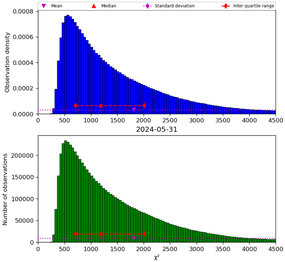
Figure 22: Histogram of “ \chi^2 ” for 2024-05-30 to 2024-06-01
