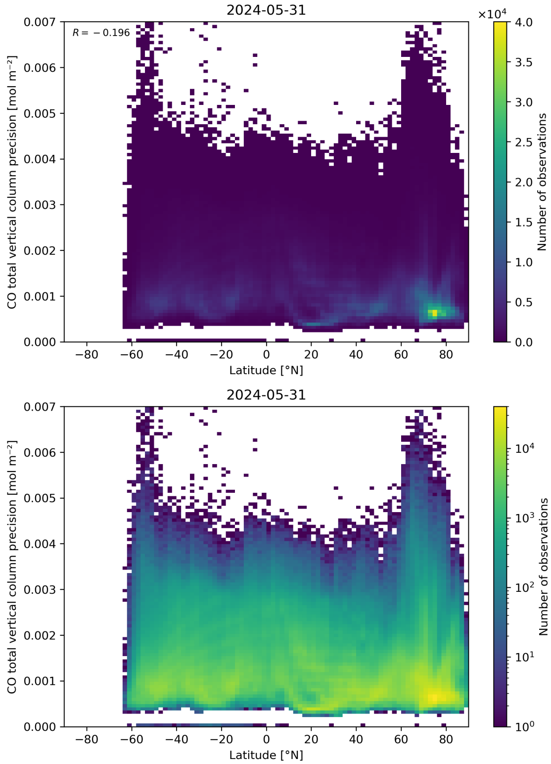
Figure 53: Scatter density plot of “Latitude” against “CO total vertical column precision” for 2024-05-30 to 2024-06-01.
