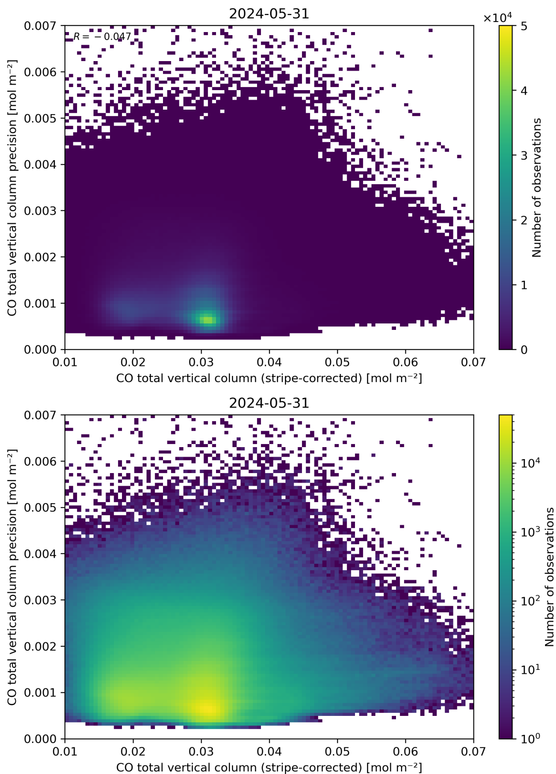
Figure 36: Scatter density plot of “CO total vertical column (stripe-corrected)” against “CO total vertical column precision” for 2024-05-30 to 2024-06-01.
