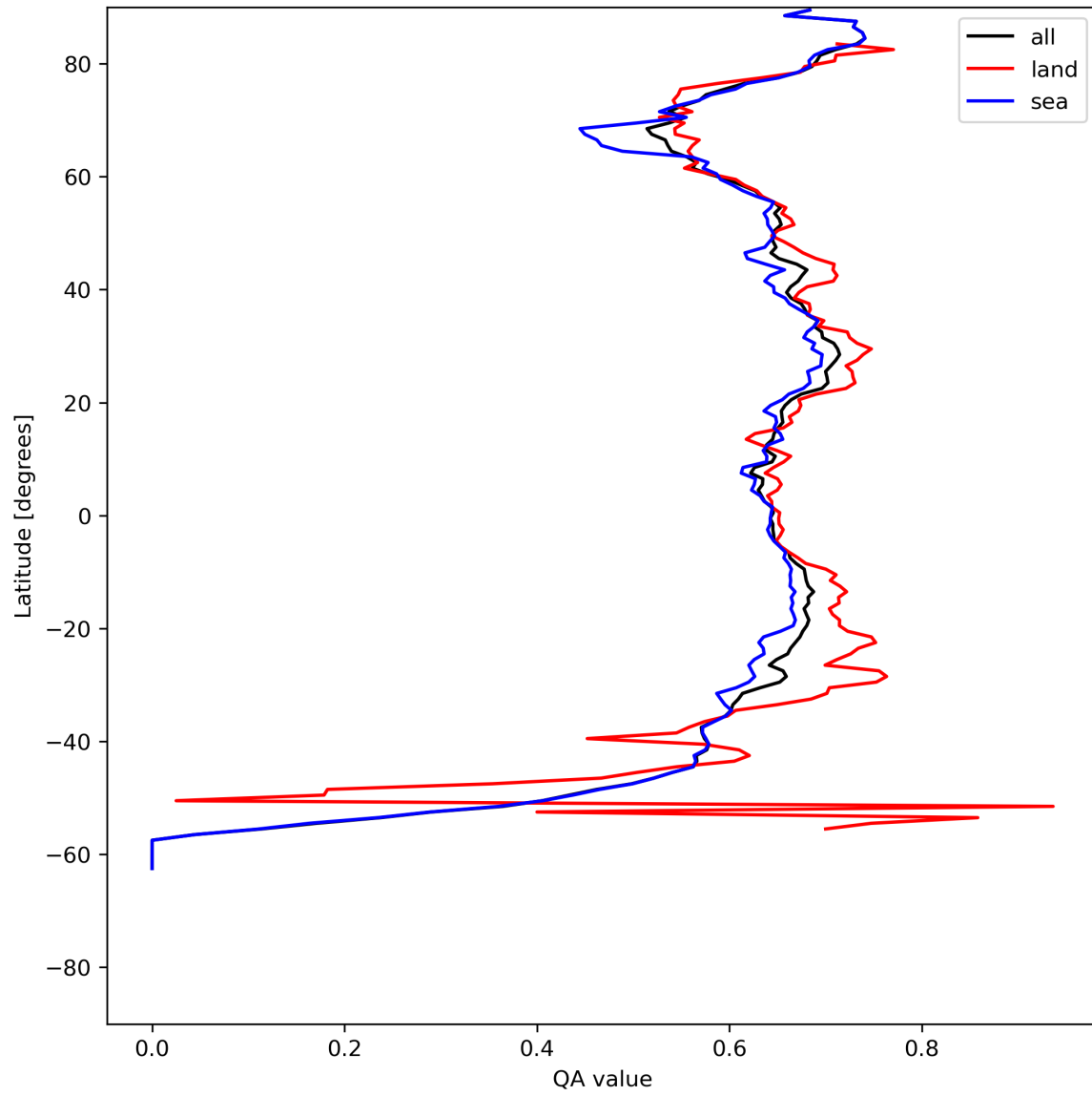
Figure 9: Zonal average of “QA value” for 2024-05-30 to 2024-06-01.
