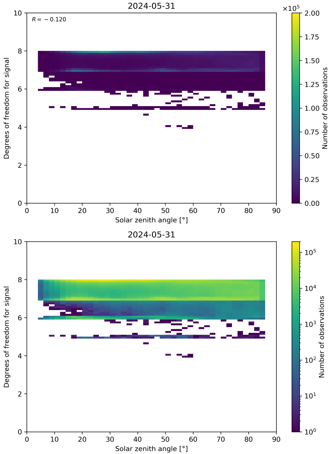
Figure 65: Scatter density plot of “Solar zenith angle” against “Degrees of freedom for signal” for 2024-05-30 to 2024-06-01.
