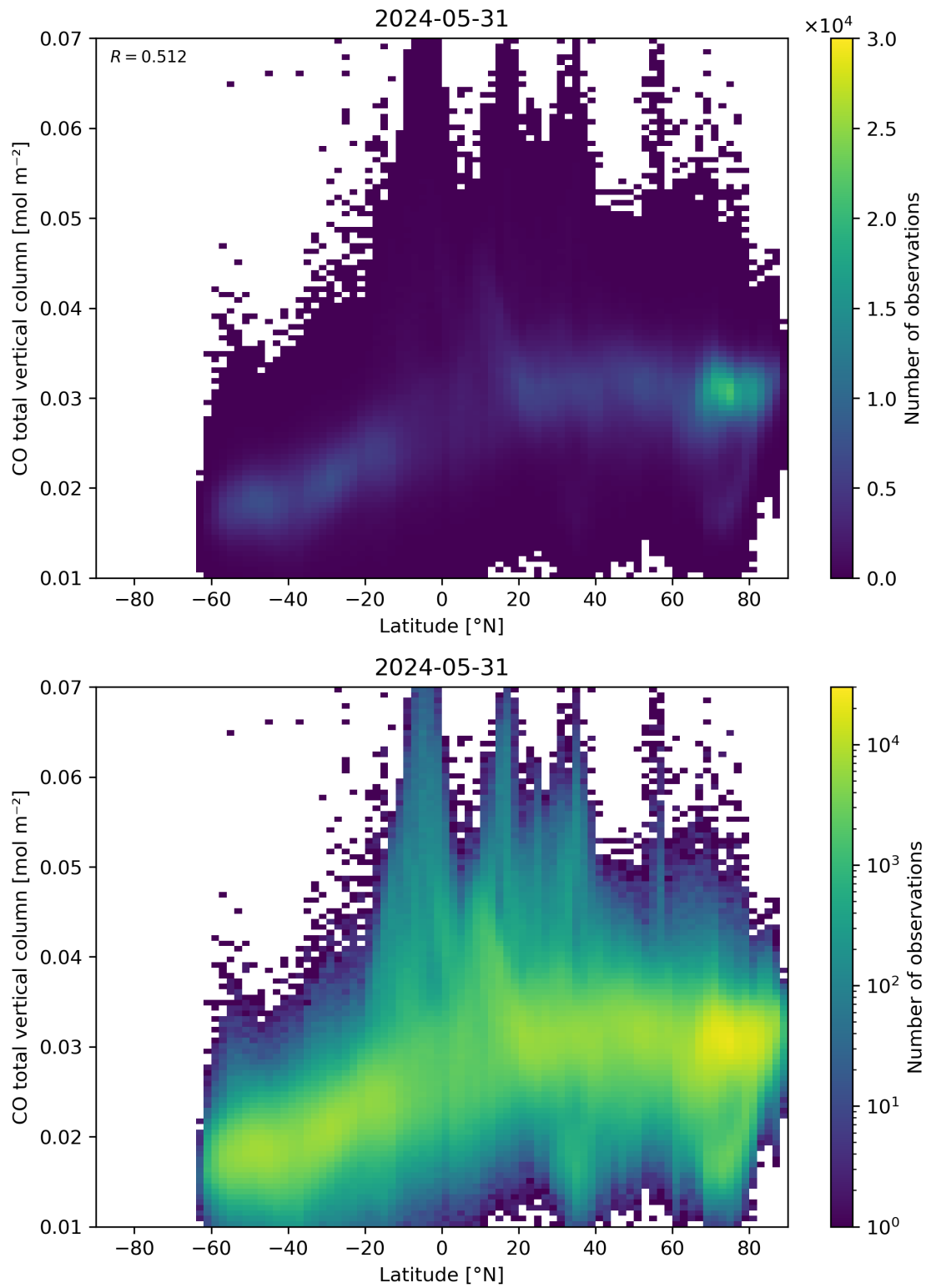
Figure 51: Scatter density plot of “Latitude” against “CO total vertical column” for 2024-05-30 to 2024-06-01.
