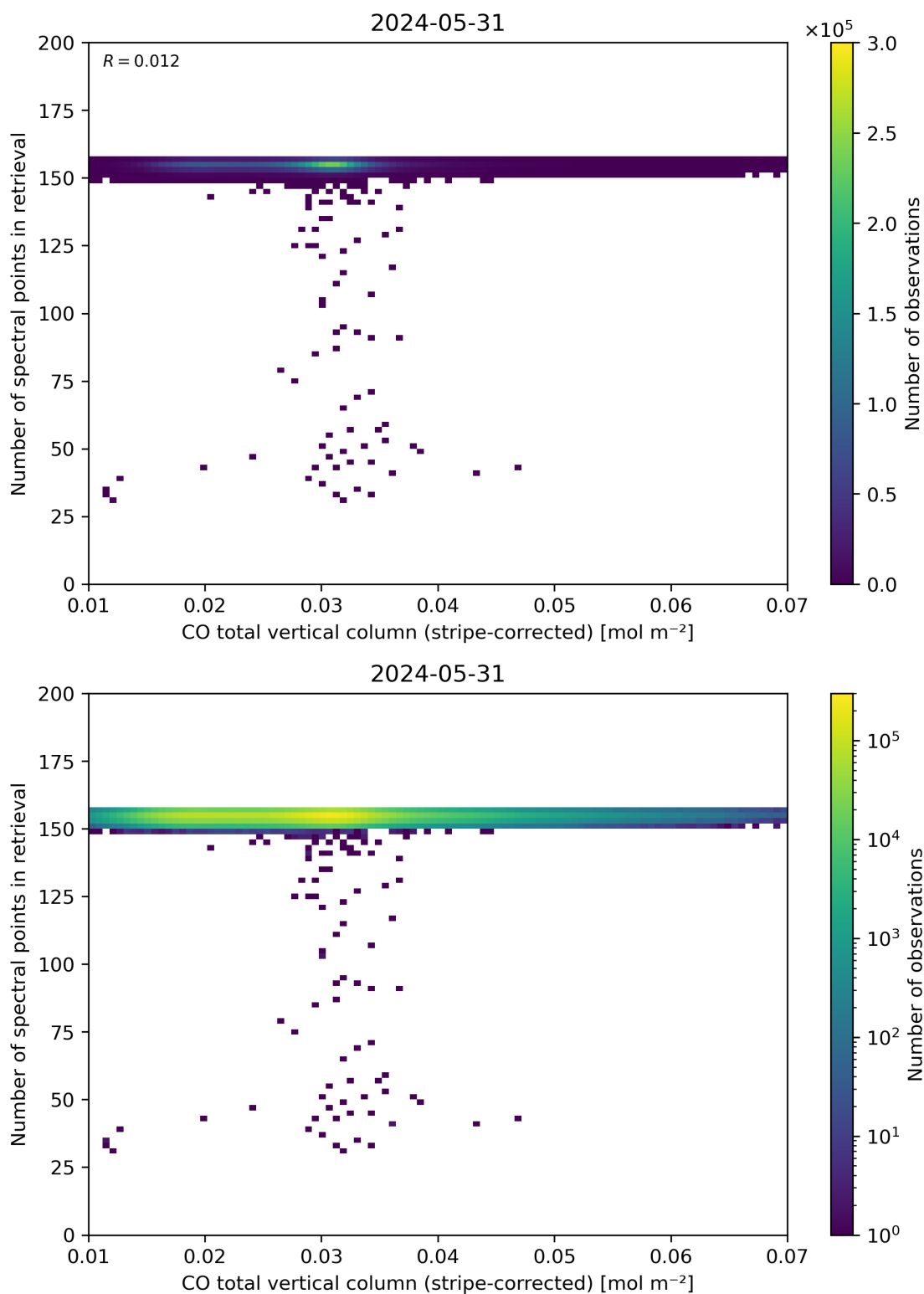
Figure 40: Scatter density plot of “CO total vertical column (stripe-corrected)” against “Number of spectral points in retrieval” for 2024-05-30 to 2024-06-01.
