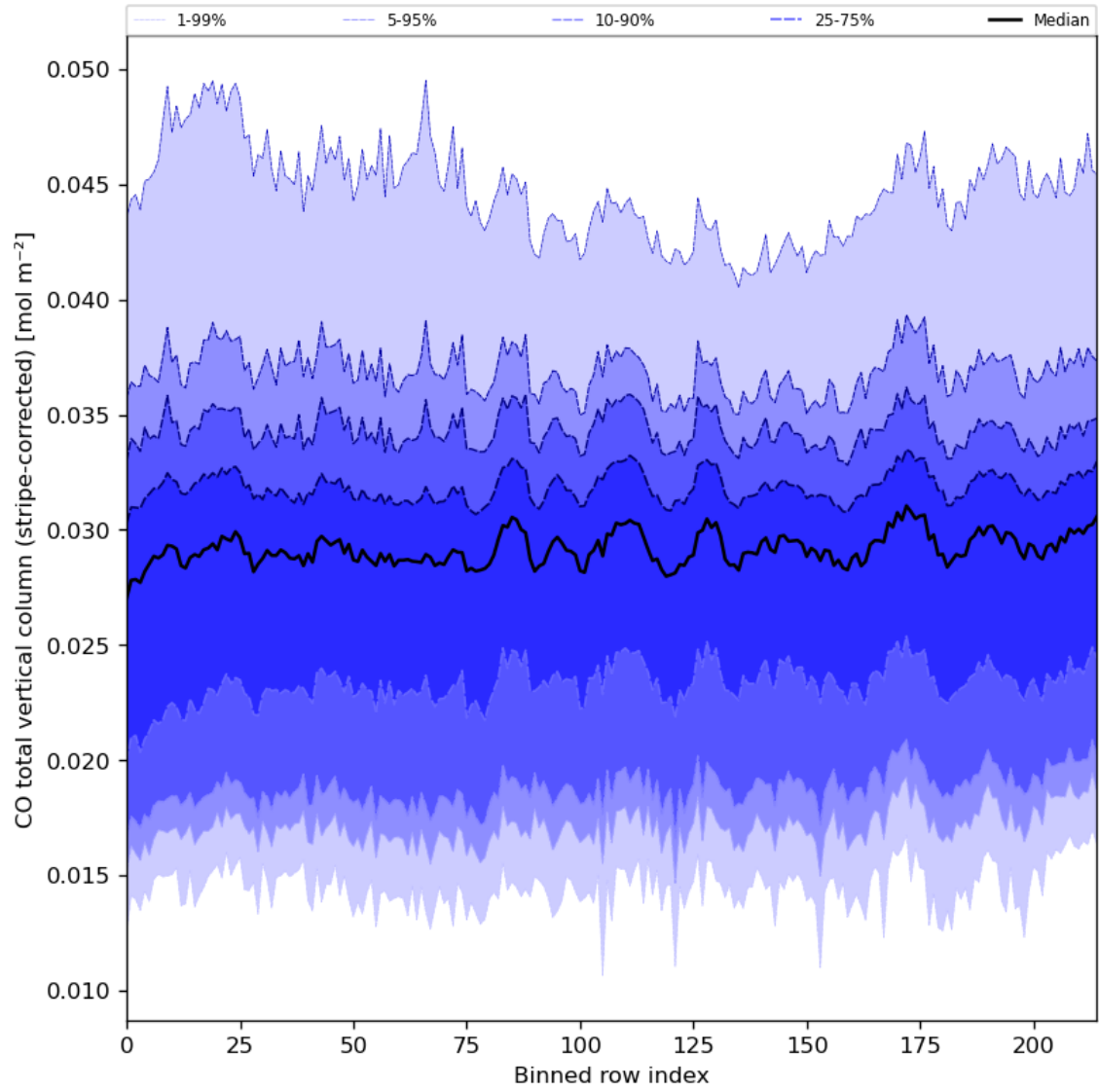
Figure 27: Along track statistics of “CO total vertical column (stripe-corrected)” for 2024-05-30 to 2024-06-01
