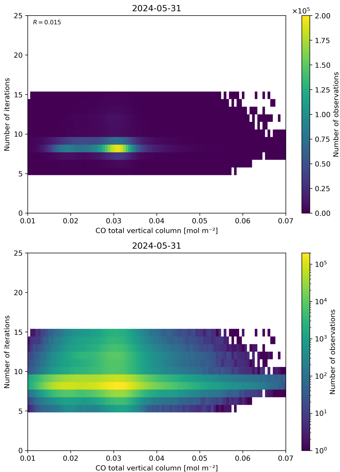
Figure 42: Scatter density plot of “CO total vertical column” against “Number of iterations” for 2024-05-30 to 2024-06-01.
