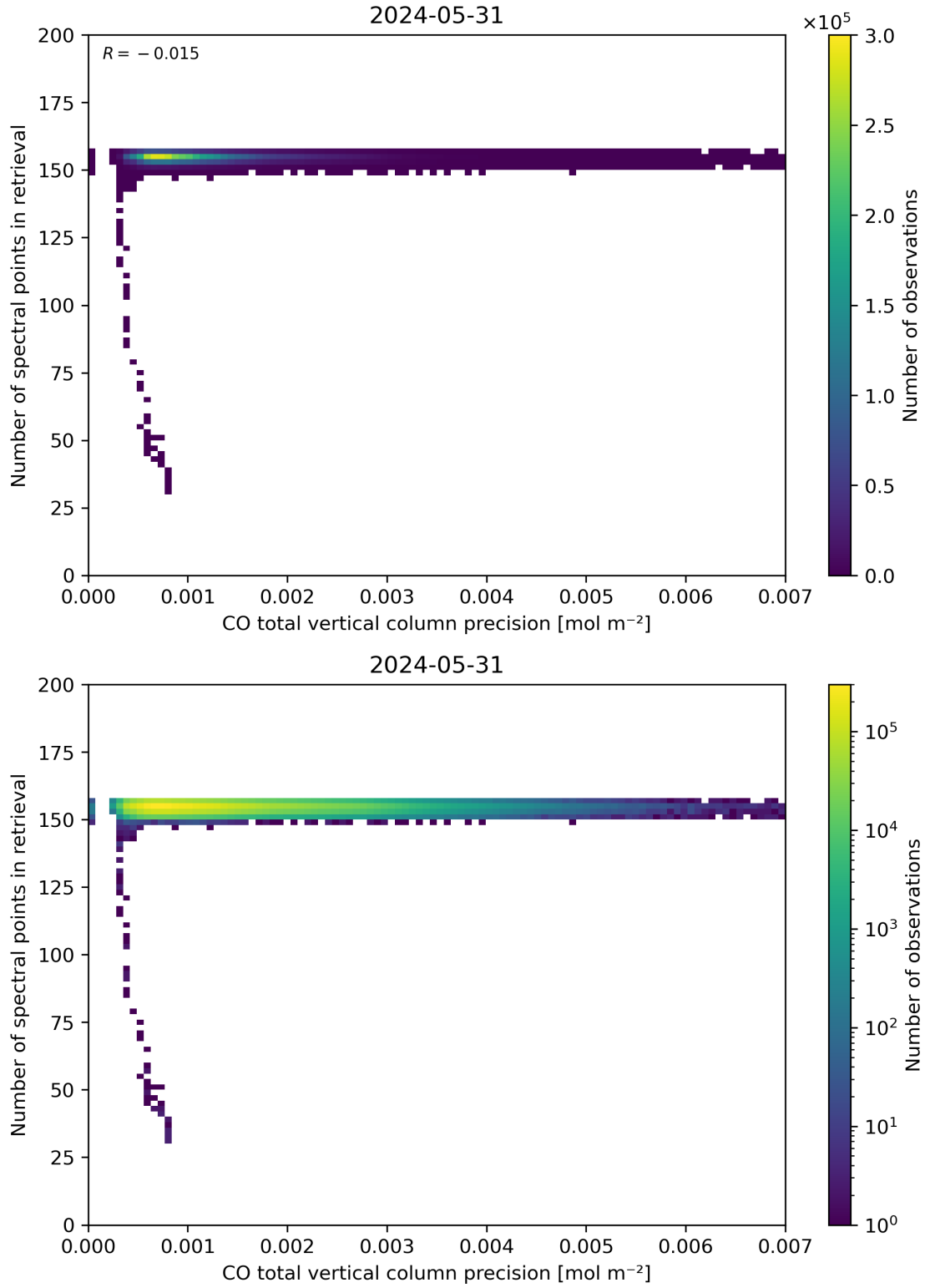
Figure 47: Scatter density plot of “CO total vertical column precision” against “Number of spectral points in retrieval” for 2024-05-30 to 2024-06-01.
