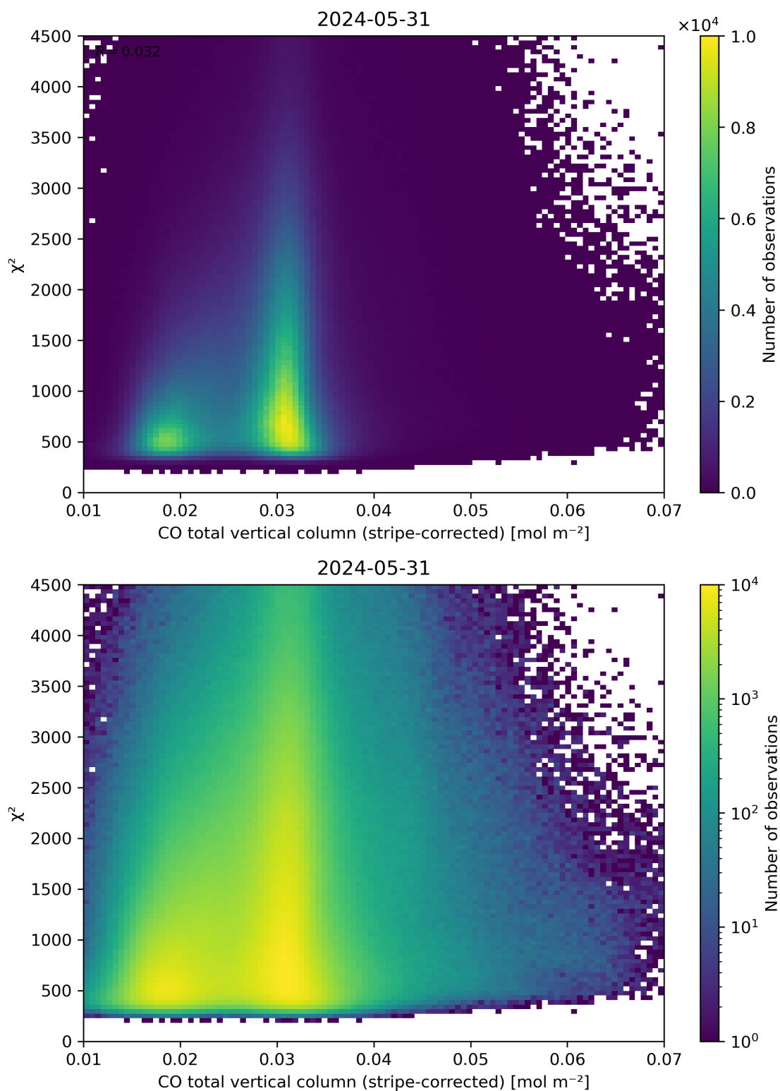
Figure 37: Scatter density plot of “CO total vertical column (stripe-corrected)” against “ \chi^2 ” for 2024-05-30 to 2024-06-01.
