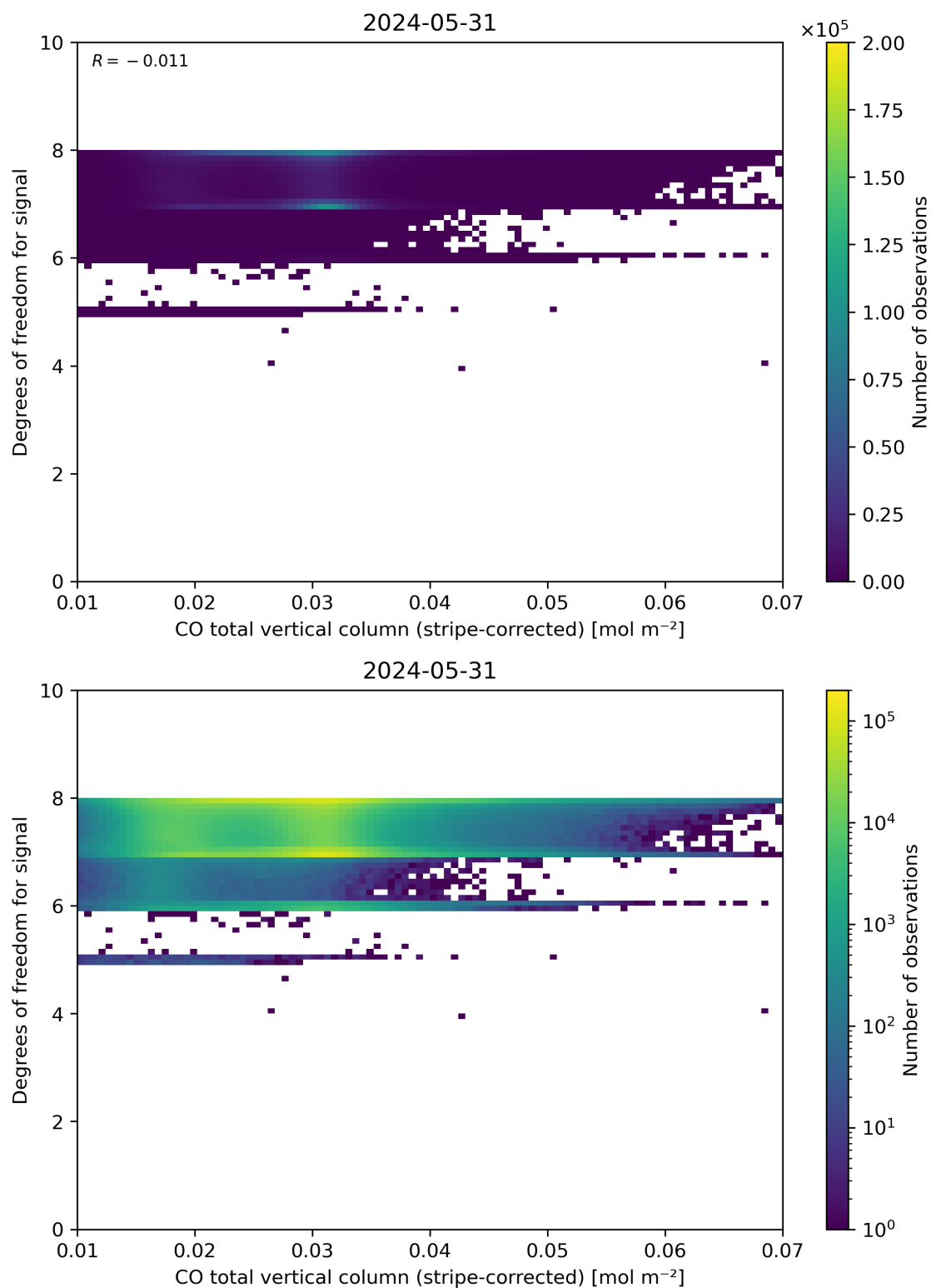
Figure 38: Scatter density plot of “CO total vertical column (stripe-corrected)” against “Degrees of freedom for signal” for 2024-05-30 to 2024-06-01.
