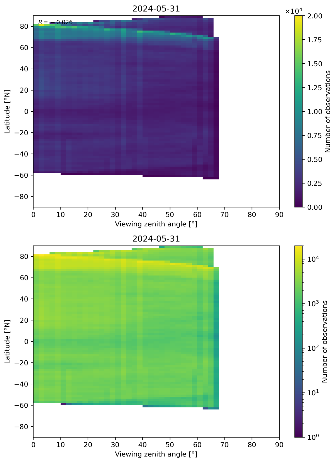
Figure 74: Scatter density plot of “Viewing zenith angle” against “Latitude” for 2024-05-30 to 2024-06-01.
