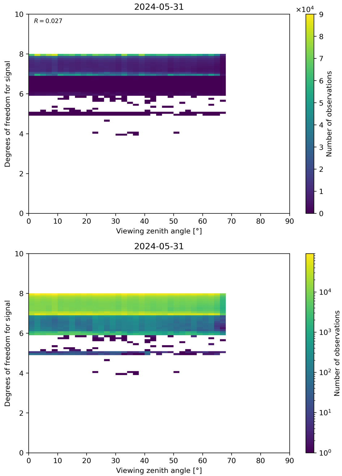
Figure 73: Scatter density plot of “Viewing zenith angle” against “Degrees of freedom for signal” for 2024-05-30 to 2024-06-01.
