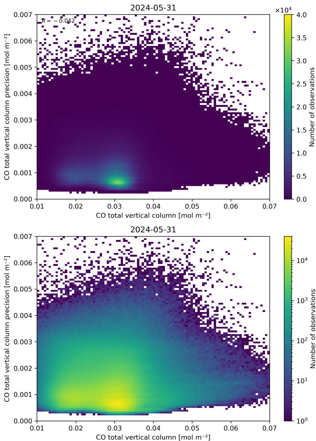
Figure 34: Scatter density plot of “CO total vertical column” against “CO total vertical column precision” for 2024-05-30 to 2024-06-01.
