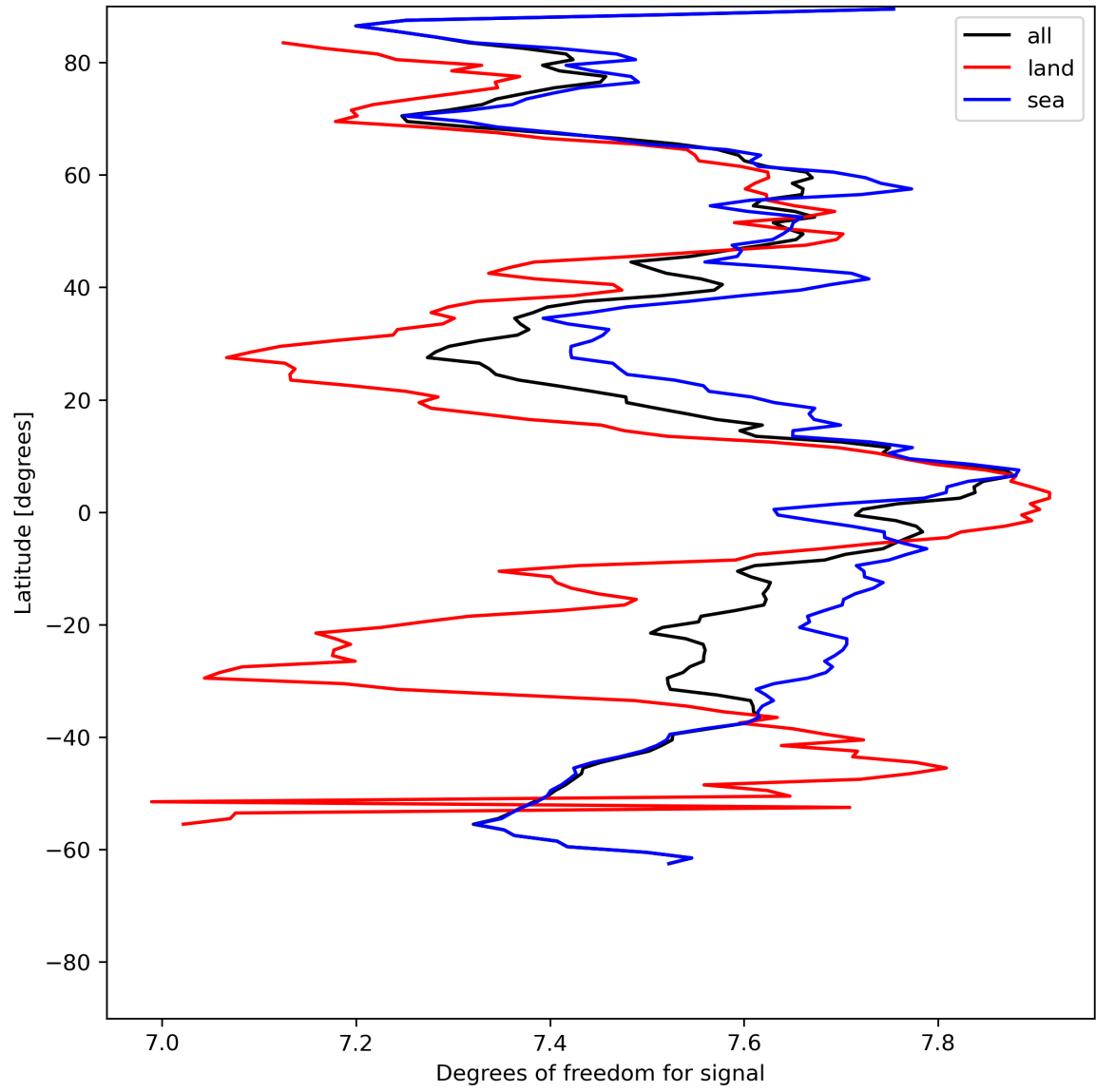
Figure 15: Zonal average of “Degrees of freedom for signal” for 2024-05-30 to 2024-06-01.
