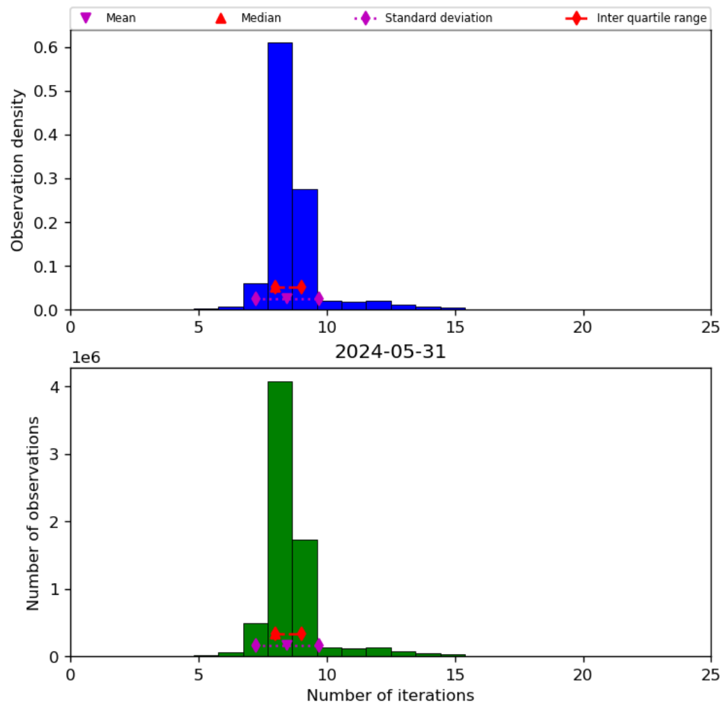
Figure 24: Histogram of “Number of iterations” for 2024-05-30 to 2024-06-01
