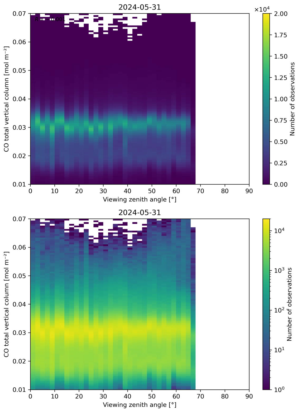
Figure 69: Scatter density plot of “Viewing zenith angle” against “CO total vertical column” for 2024-05-30 to 2024-06-01.
