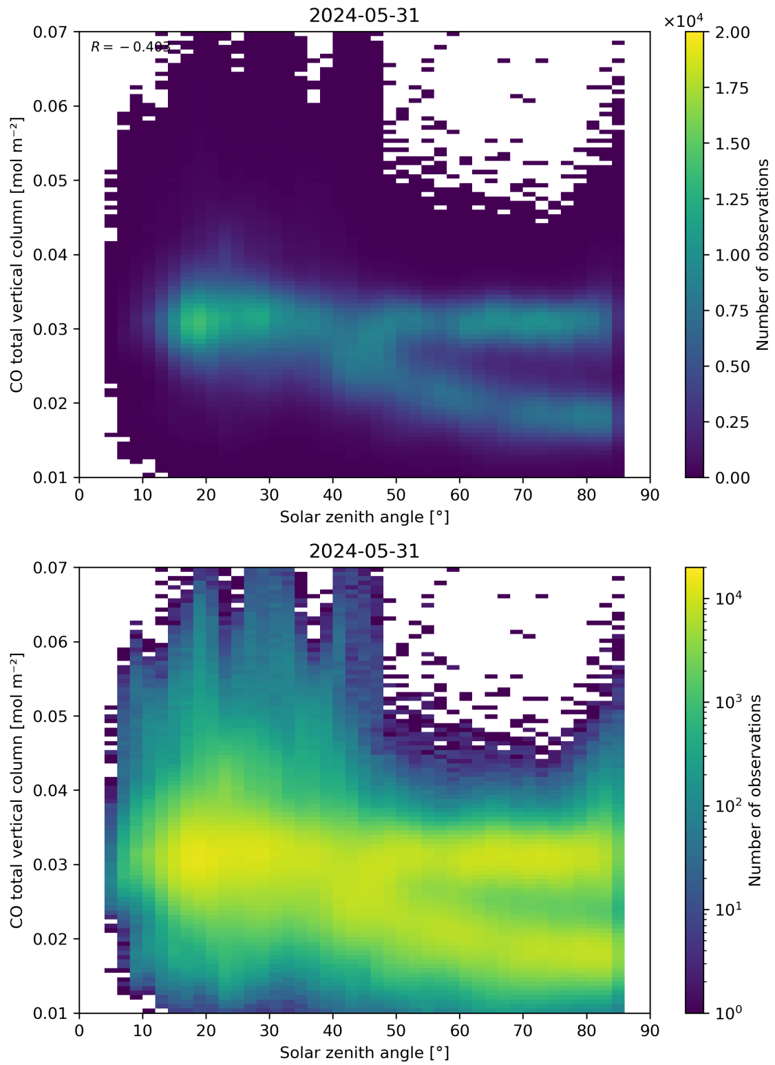
Figure 61: Scatter density plot of “Solar zenith angle” against “CO total vertical column” for 2024-05-30 to 2024-06-01.
