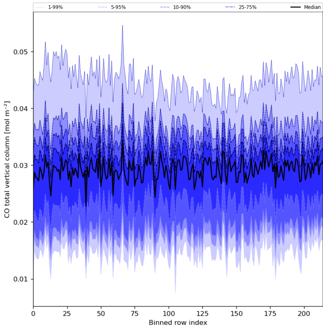
Figure 26: Along track statistics of “CO total vertical column” for 2024-05-30 to 2024-06-01
