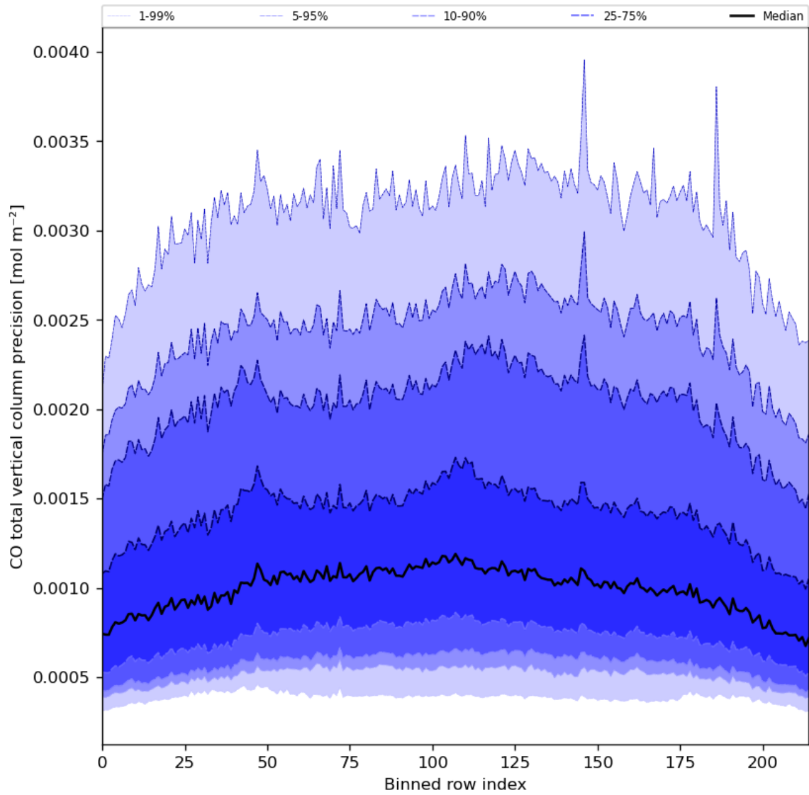
Figure 28: Along track statistics of “CO total vertical column precision” for 2024-05-30 to 2024-06-01
