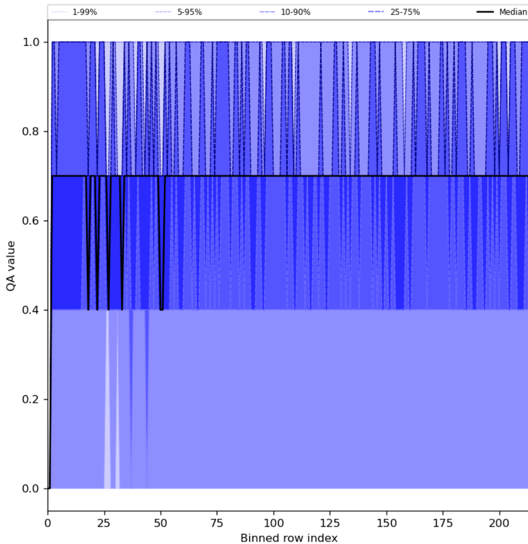
Figure 25: Along track statistics of “QA value” for 2024-05-30 to 2024-06-01
