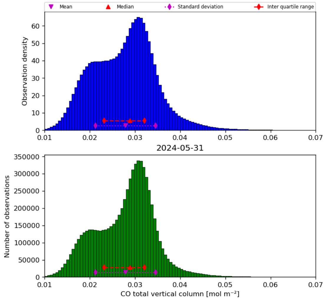
Figure 18: Histogram of “CO total vertical column” for 2024-05-30 to 2024-06-01
