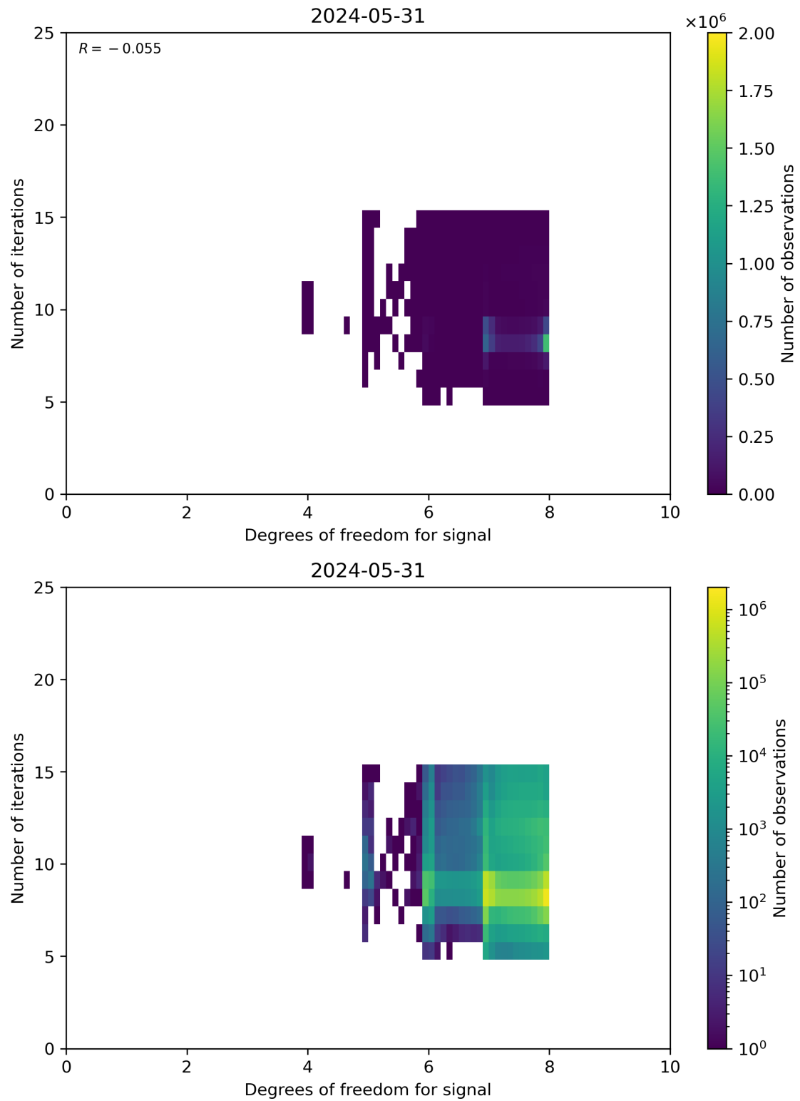
Figure 50: Scatter density plot of “Degrees of freedom for signal” against “Number of iterations” for 2024-05-30 to 2024-06-01.
