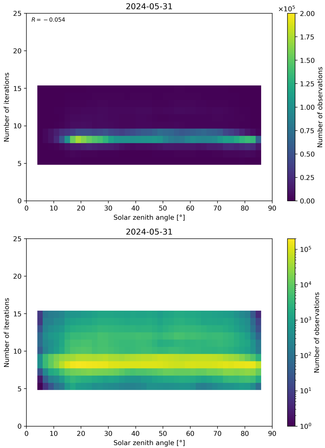
Figure 67: Scatter density plot of “Solar zenith angle” against “Number of iterations” for 2024-05-30 to 2024-06-01.
