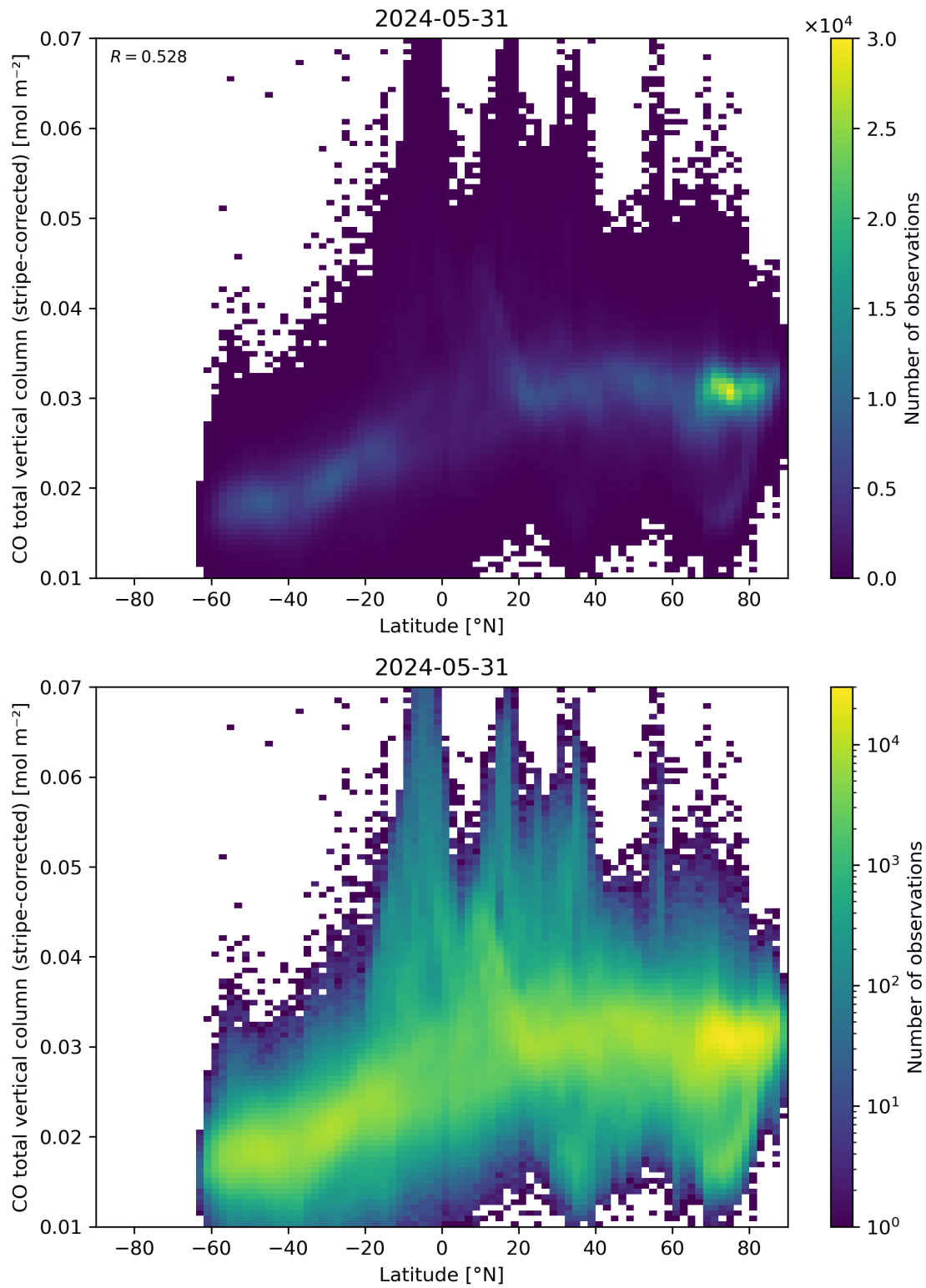
Figure 52: Scatter density plot of “Latitude” against “CO total vertical column (stripe-corrected)” for 2024-05-30 to 2024-06-01.
