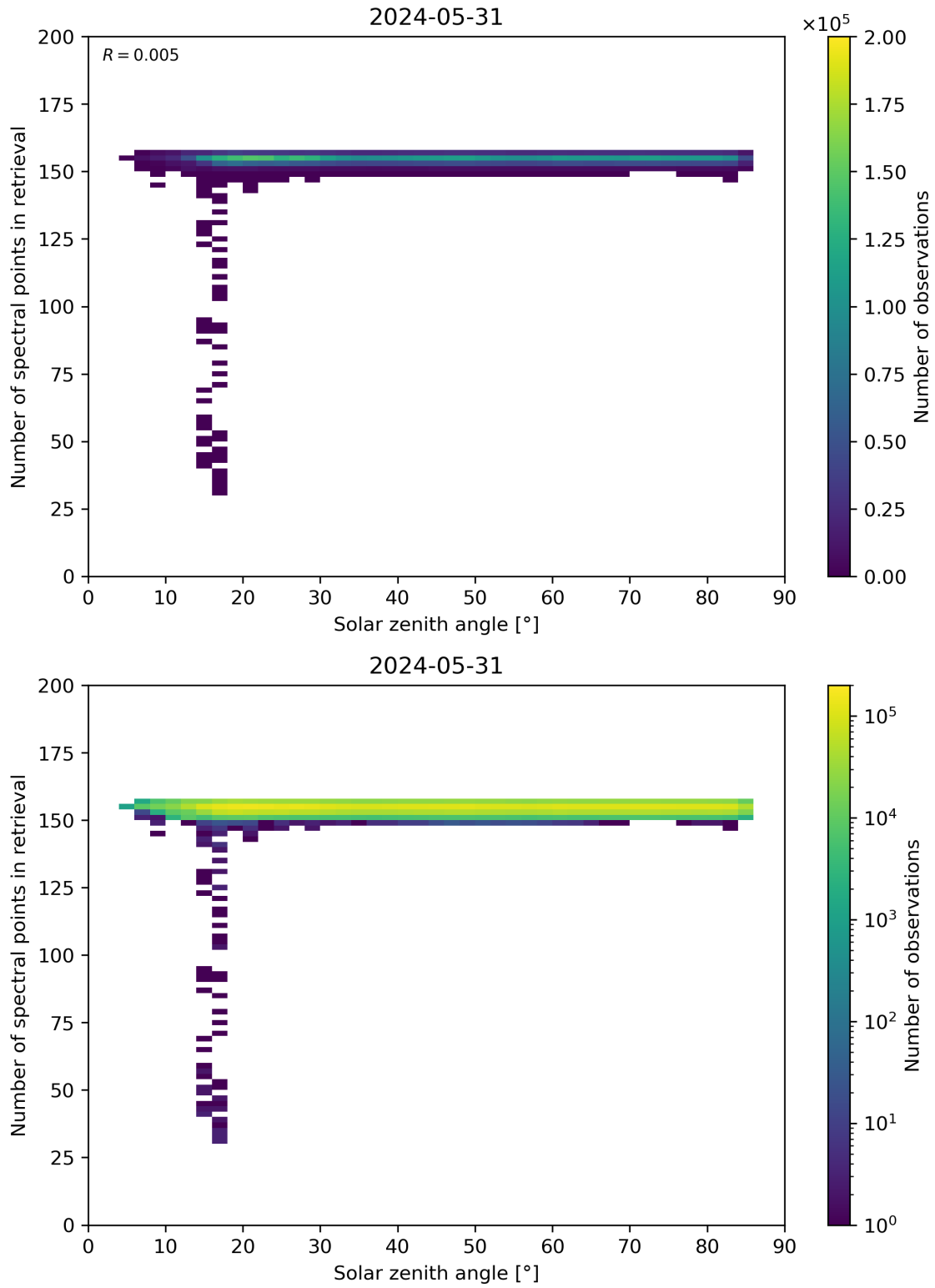
Figure 68: Scatter density plot of “Solar zenith angle” against “Number of spectral points in retrieval” for 2024-05-30 to 2024-06-01.
