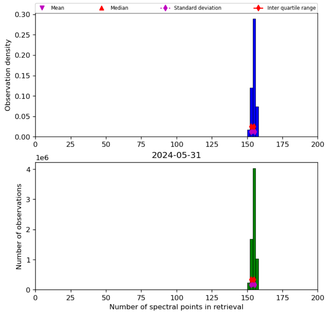
Figure 21: Histogram of “Number of spectral points in retrieval” for 2024-05-30 to 2024-06-01
