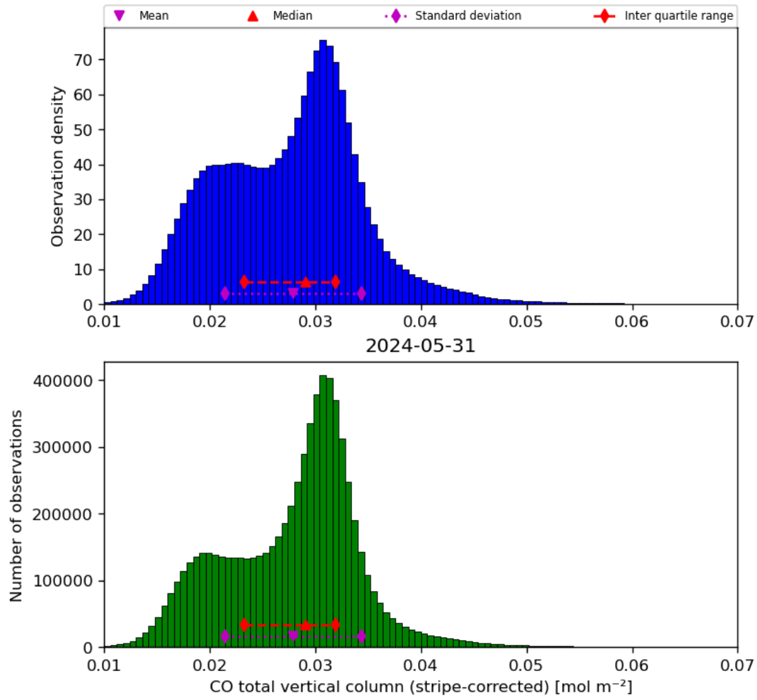
Figure 19: Histogram of “CO total vertical column (stripe-corrected)” for 2024-05-30 to 2024-06-01
