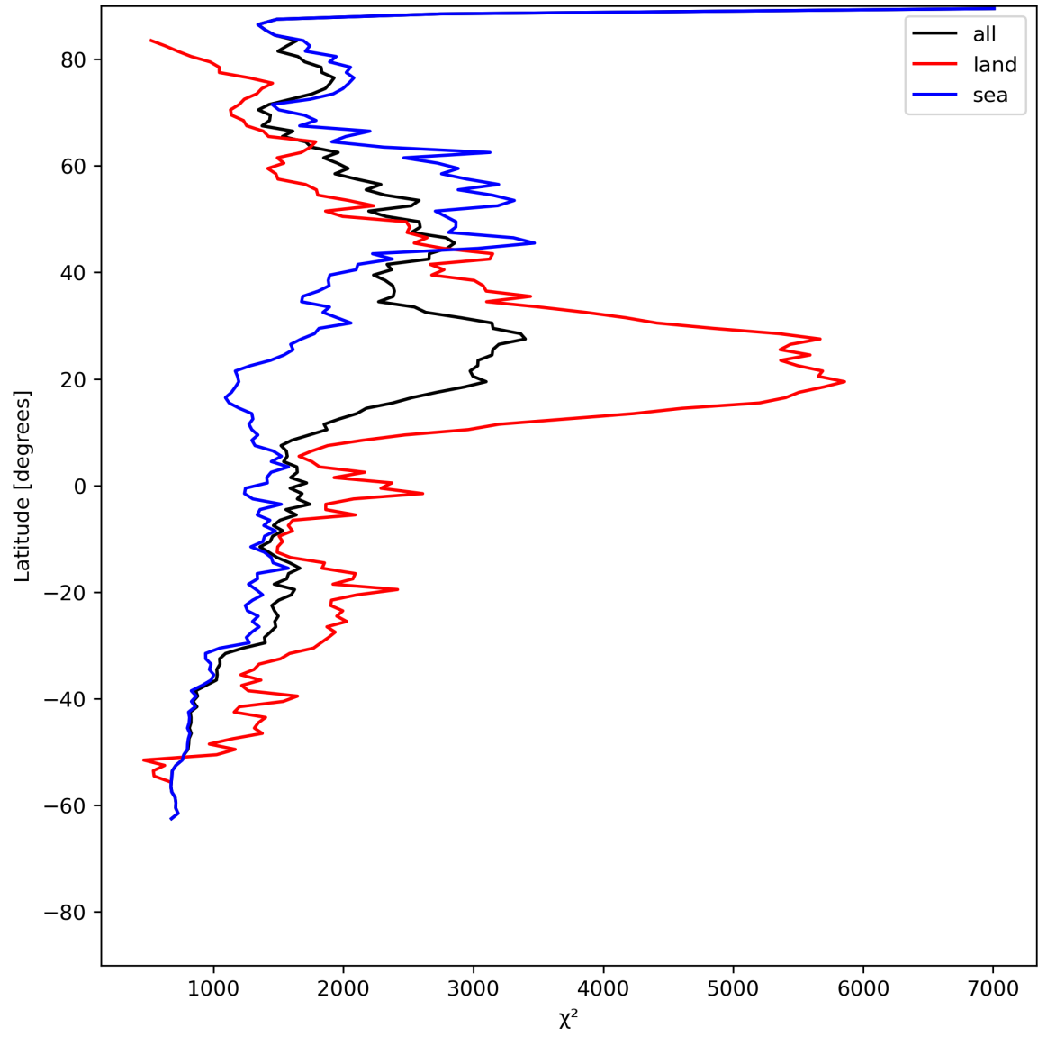
Figure 14: Zonal average of “ \chi^2 ” for 2024-05-30 to 2024-06-01.
