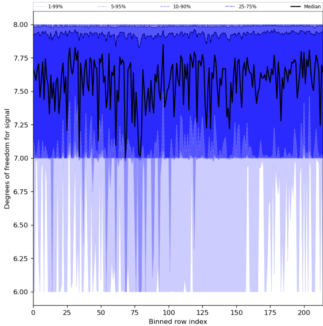
Figure 31: Along track statistics of “Degrees of freedom for signal” for 2024-05-30 to 2024-06-01
