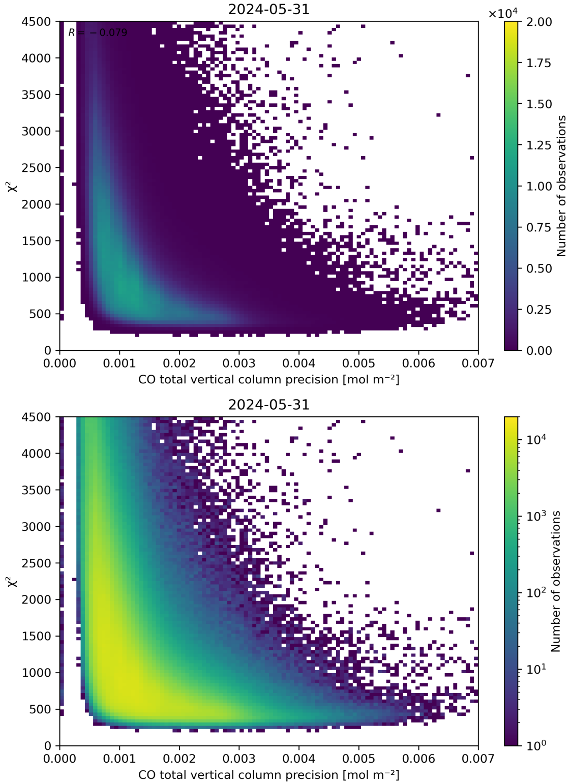
Figure 44: Scatter density plot of “CO total vertical column precision” against “ \chi^2 ” for 2024-05-30 to 2024-06-01.
