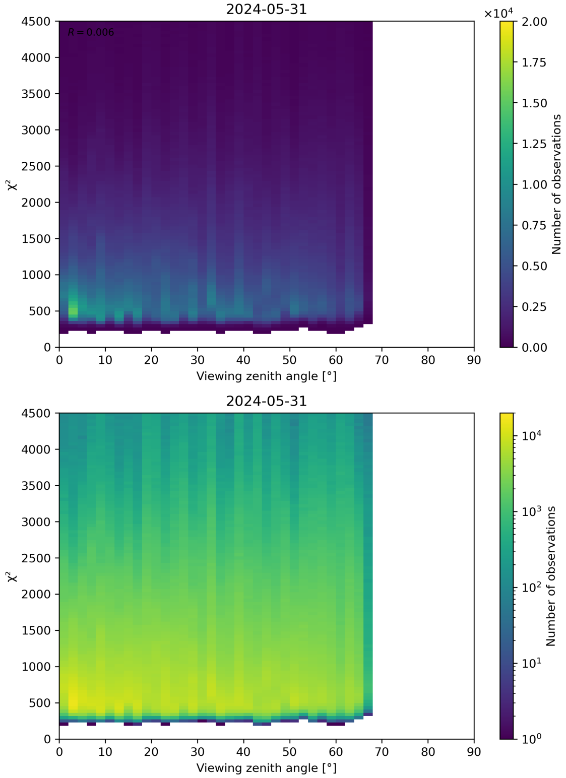
Figure 72: Scatter density plot of “Viewing zenith angle” against “ \chi^2 ” for 2024-05-30 to 2024-06-01.
