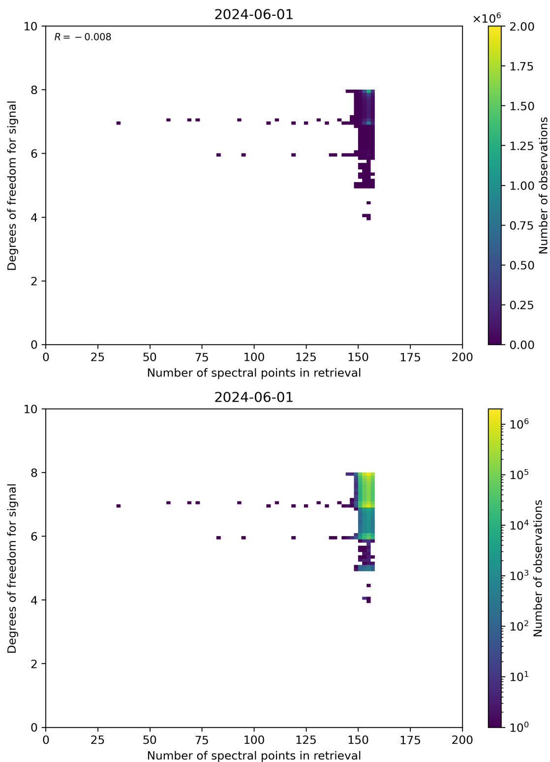
Figure 59: Scatter density plot of “Number of spectral points in retrieval” against “Degrees of freedom for signal” for 2024-05-31 to 2024-06-02.
