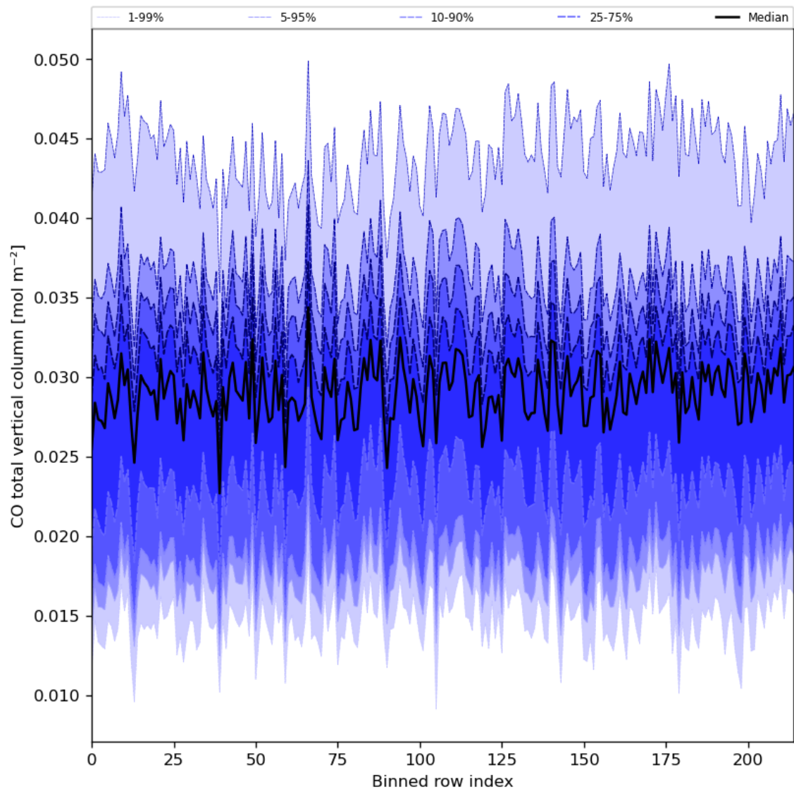
Figure 26: Along track statistics of “CO total vertical column” for 2024-05-31 to 2024-06-02
