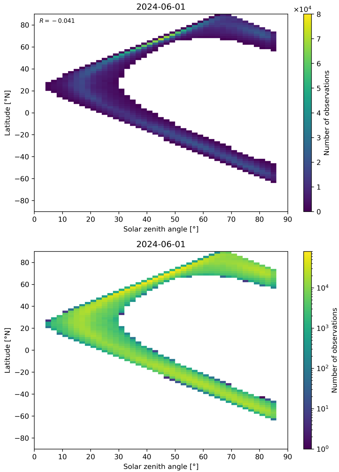
Figure 66: Scatter density plot of “Solar zenith angle” against “Latitude” for 2024-05-31 to 2024-06-02.
