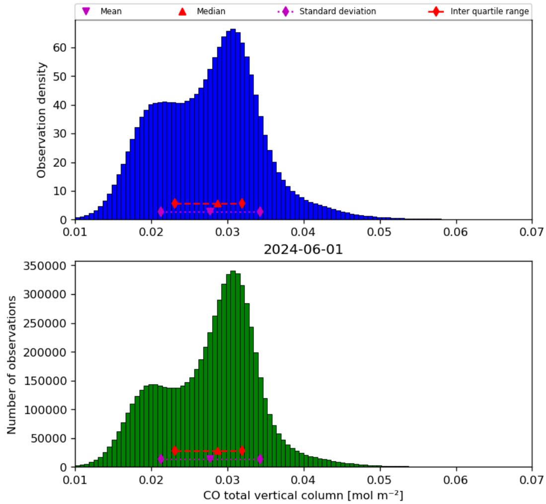
Figure 18: Histogram of “CO total vertical column” for 2024-05-31 to 2024-06-02
