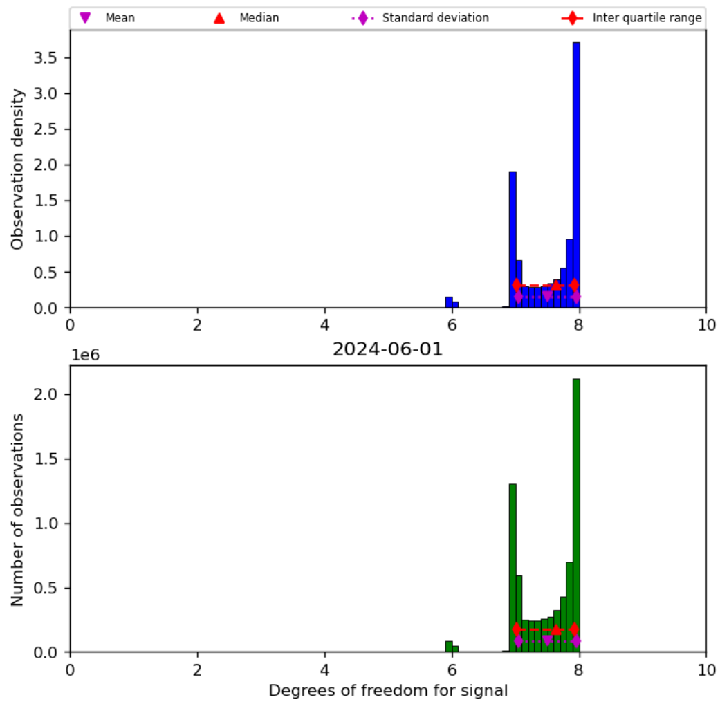
Figure 23: Histogram of “Degrees of freedom for signal” for 2024-05-31 to 2024-06-02
