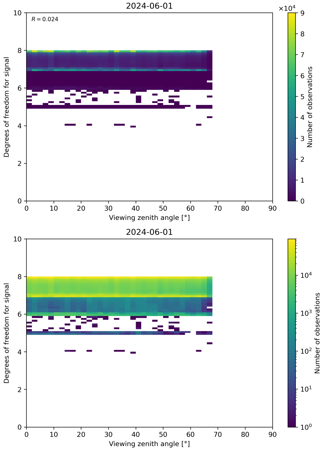
Figure 73: Scatter density plot of “Viewing zenith angle” against “Degrees of freedom for signal” for 2024-05-31 to 2024-06-02.
