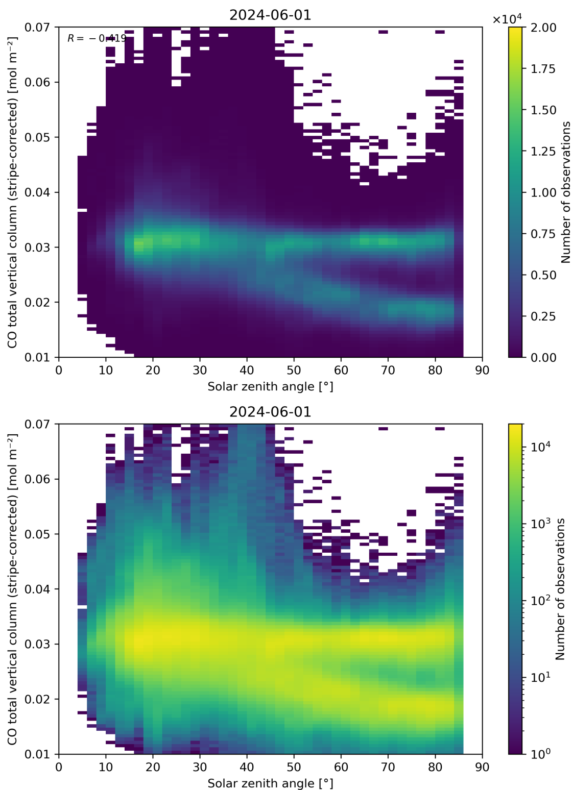
Figure 62: Scatter density plot of “Solar zenith angle” against “CO total vertical column (stripe-corrected)” for 2024-05-31 to 2024-06-02.
