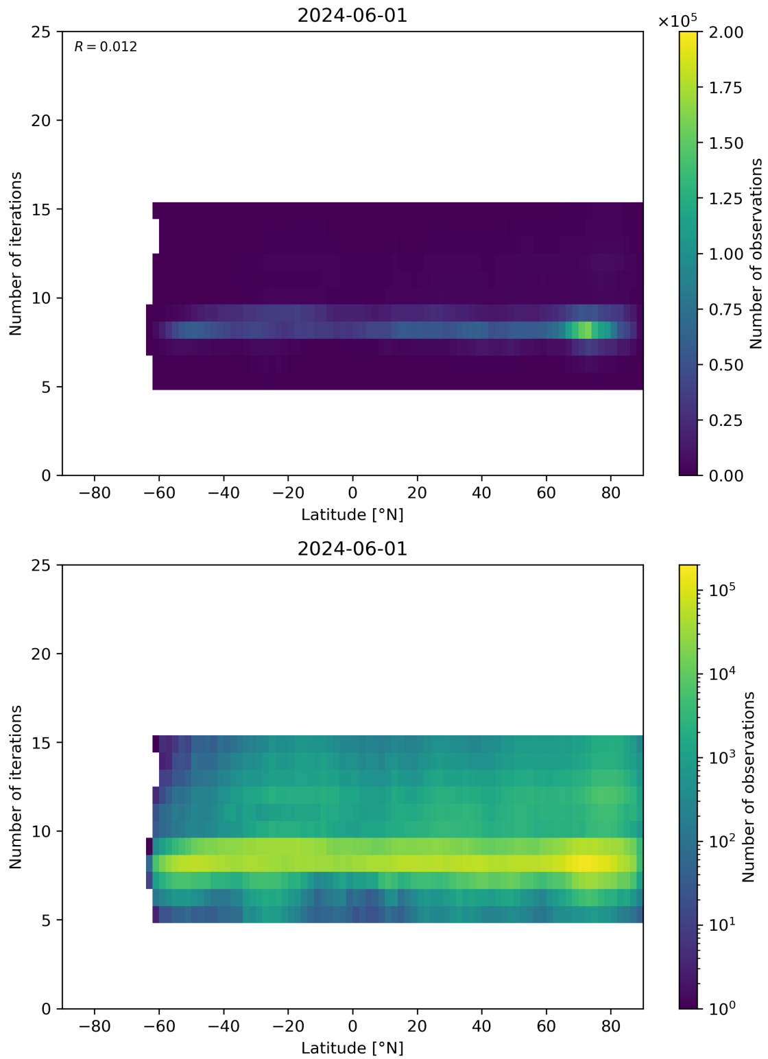
Figure 56: Scatter density plot of “Latitude” against “Number of iterations” for 2024-05-31 to 2024-06-02.
