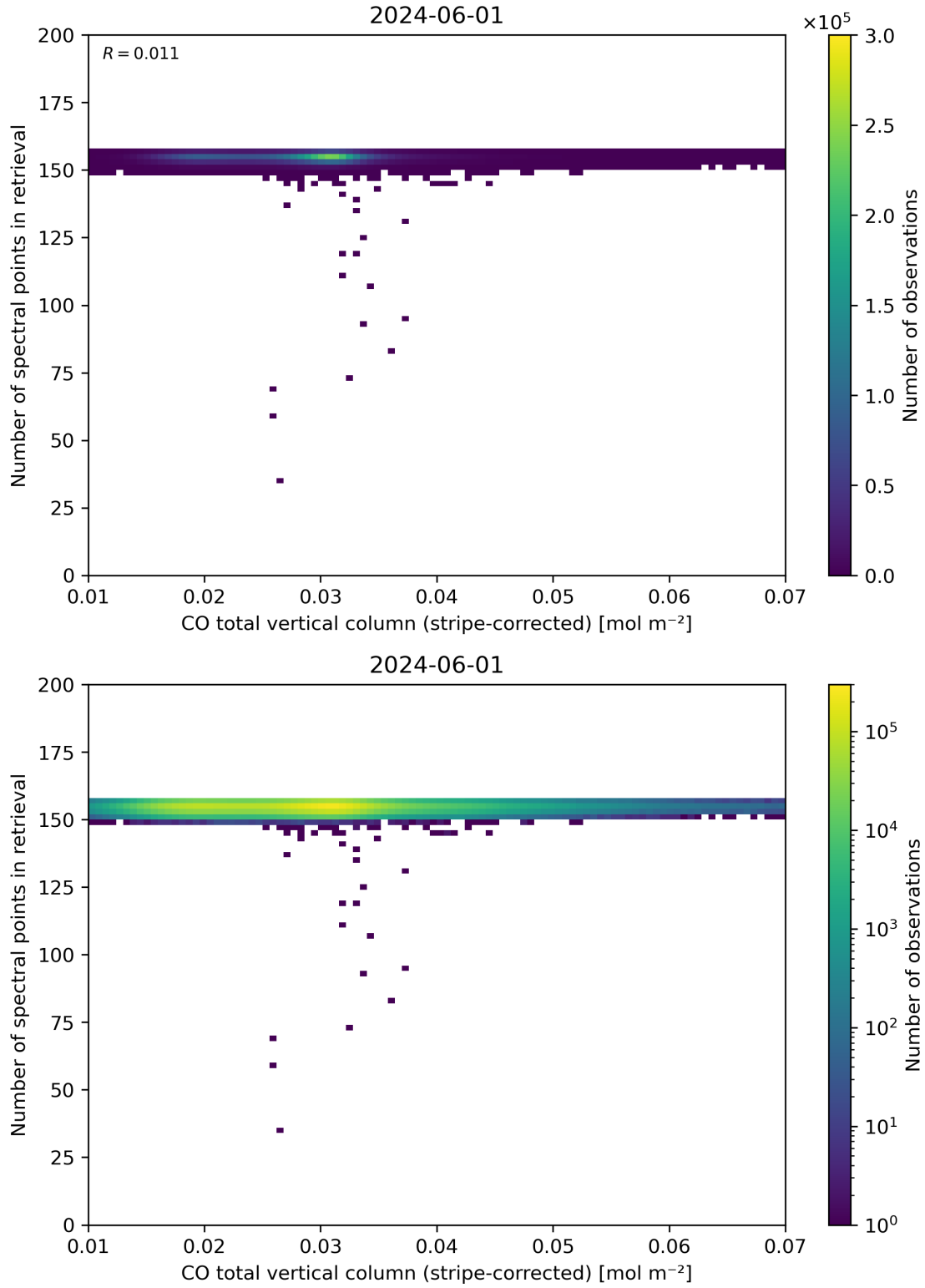
Figure 40: Scatter density plot of “CO total vertical column (stripe-corrected)” against “Number of spectral points in retrieval” for 2024-05-31 to 2024-06-02.
