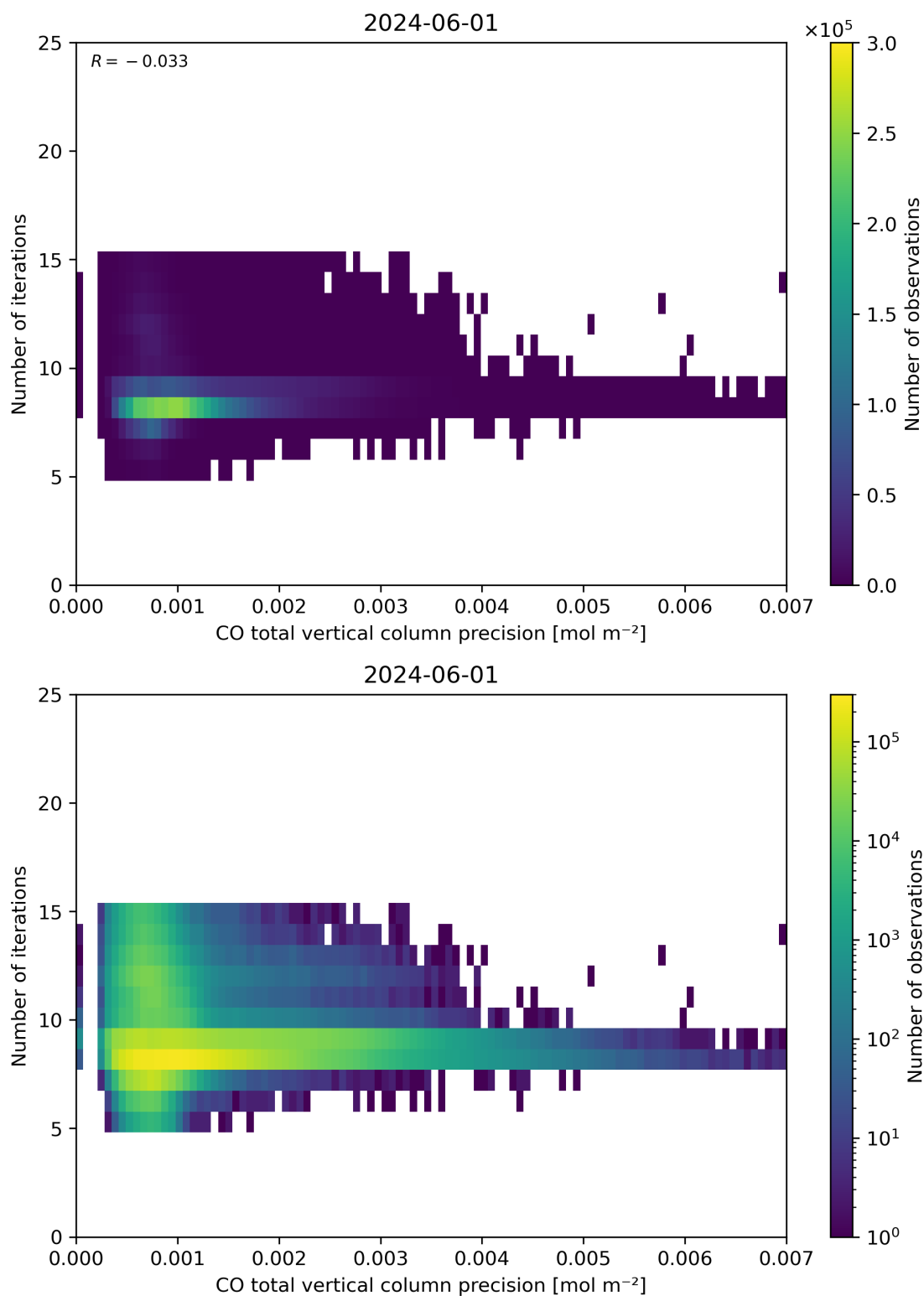
Figure 46: Scatter density plot of “CO total vertical column precision” against “Number of iterations” for 2024-05-31 to 2024-06-02.
