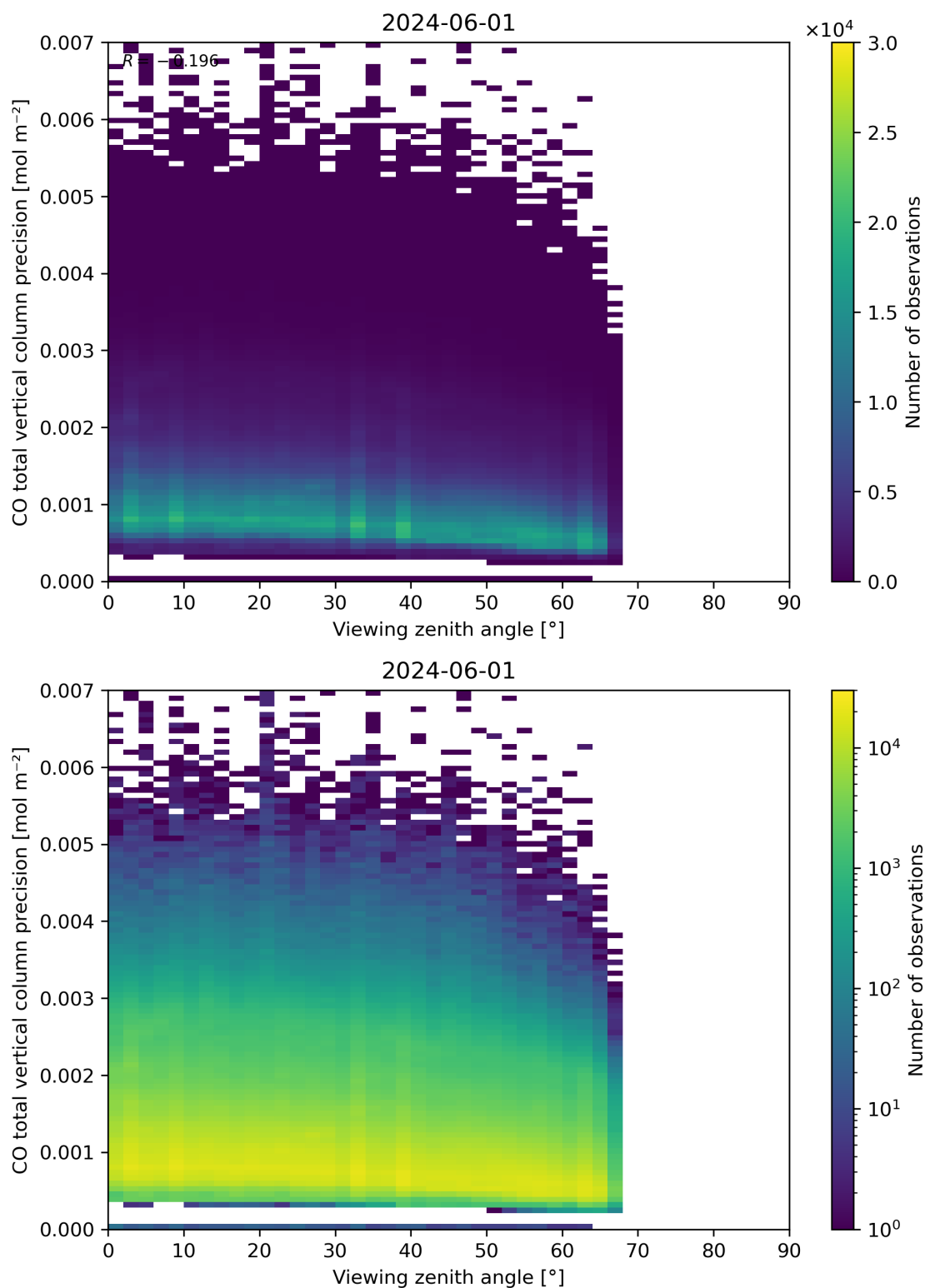
Figure 71: Scatter density plot of “Viewing zenith angle” against “CO total vertical column precision” for 2024-05-31 to 2024-06-02.
