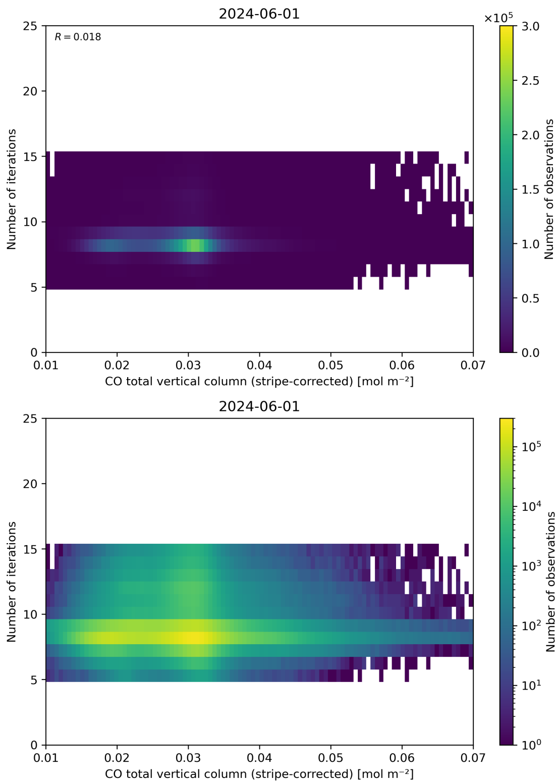
Figure 39: Scatter density plot of “CO total vertical column (stripe-corrected)” against “Number of iterations” for 2024-05-31 to 2024-06-02.
