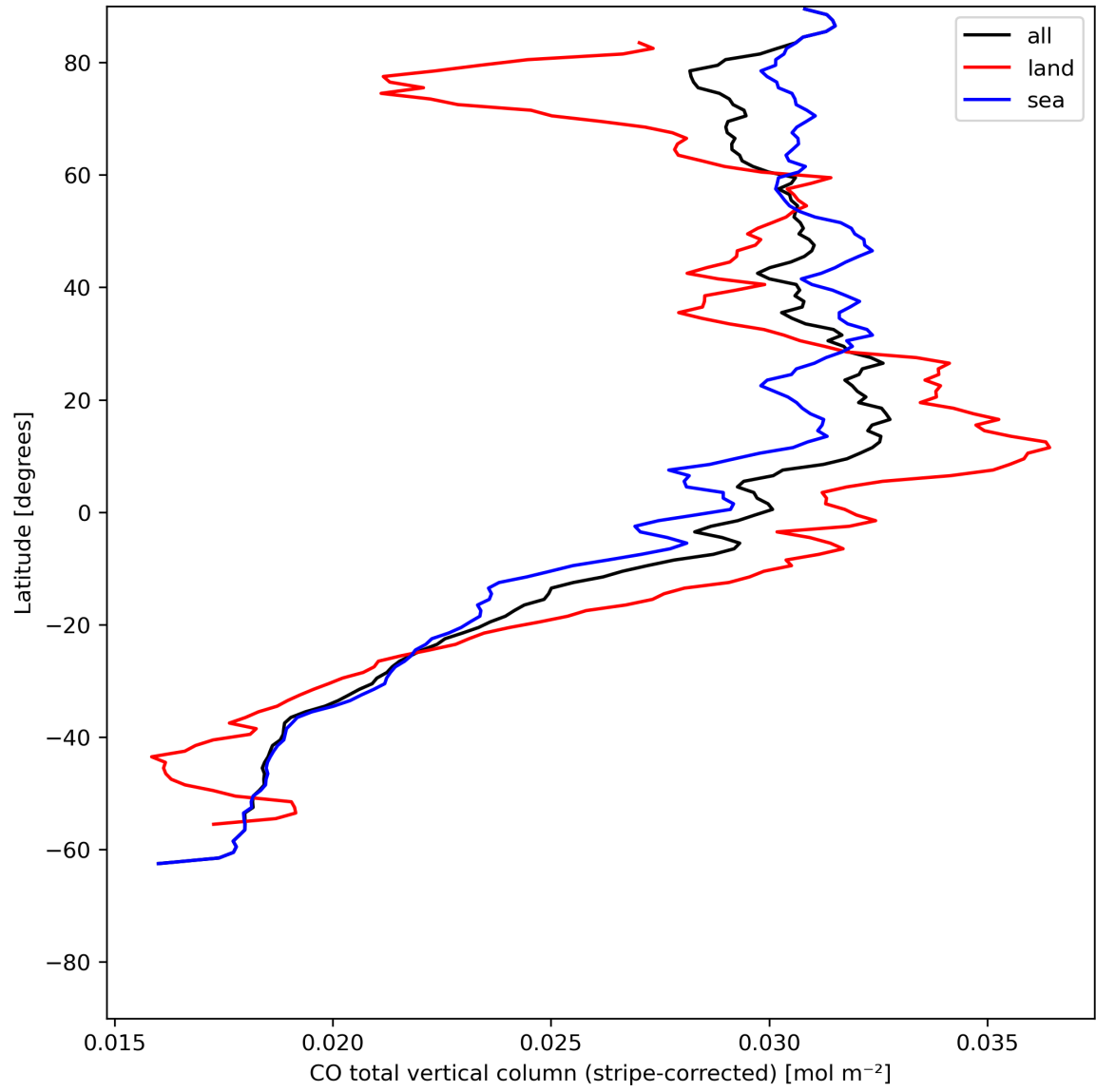
Figure 11: Zonal average of “CO total vertical column (stripe-corrected)” for 2024-05-31 to 2024-06-02.
