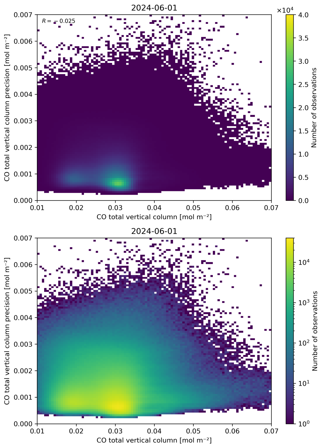
Figure 34: Scatter density plot of “CO total vertical column” against “CO total vertical column precision” for 2024-05-31 to 2024-06-02.
