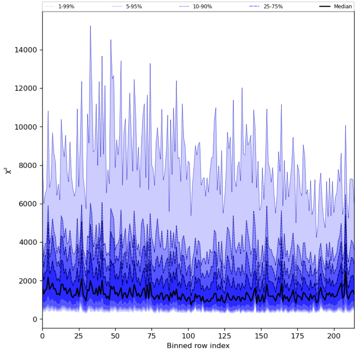
Figure 30: Along track statistics of “ \chi^2 ” for 2024-05-31 to 2024-06-02
