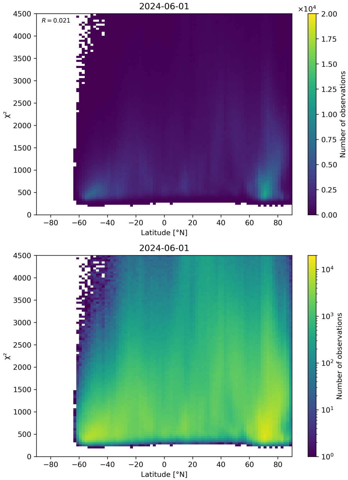
Figure 54: Scatter density plot of “Latitude” against “ \chi^2 ” for 2024-05-31 to 2024-06-02.
