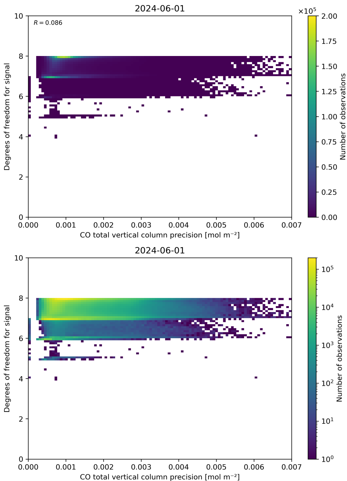
Figure 45: Scatter density plot of “CO total vertical column precision” against “Degrees of freedom for signal” for 2024-05-31 to 2024-06-02.
