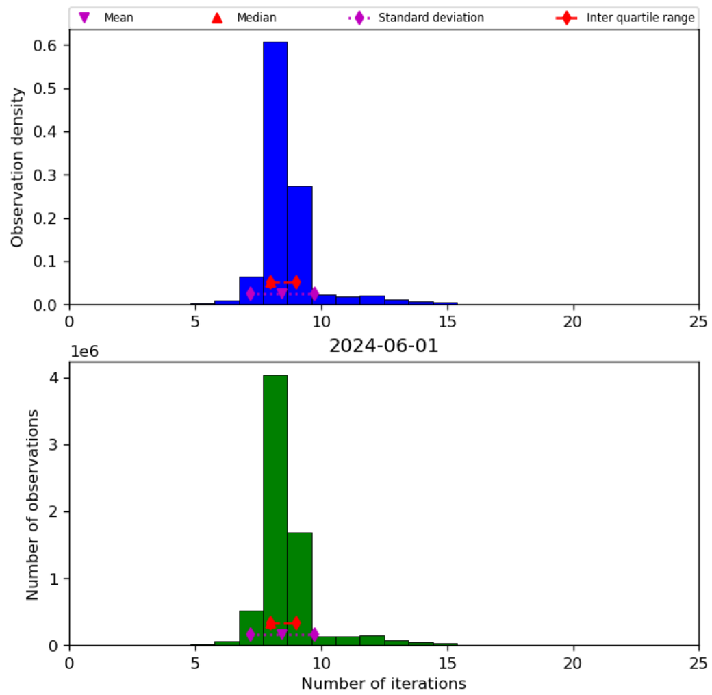
Figure 24: Histogram of “Number of iterations” for 2024-05-31 to 2024-06-02
