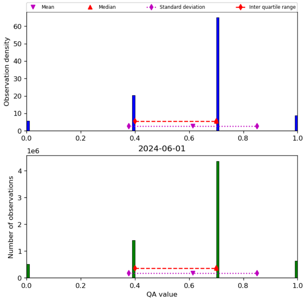
Figure 17: Histogram of “QA value” for 2024-05-31 to 2024-06-02
