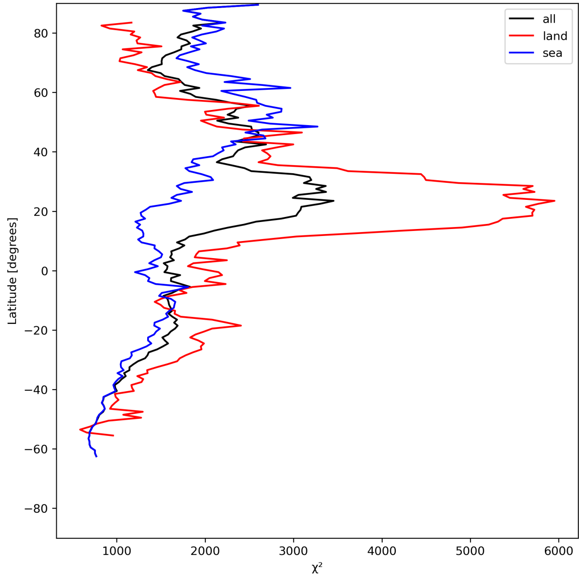
Figure 14: Zonal average of “ \chi^2 ” for 2024-05-31 to 2024-06-02.
