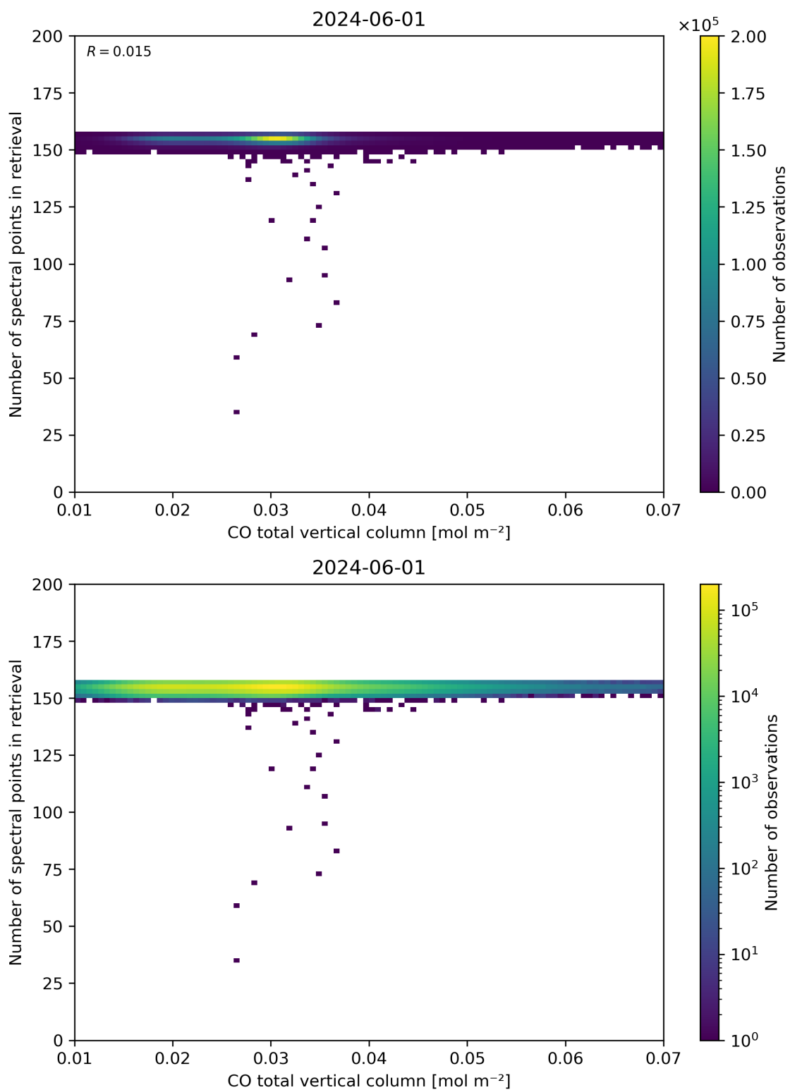
Figure 43: Scatter density plot of “CO total vertical column” against “Number of spectral points in retrieval” for 2024-05-31 to 2024-06-02.
