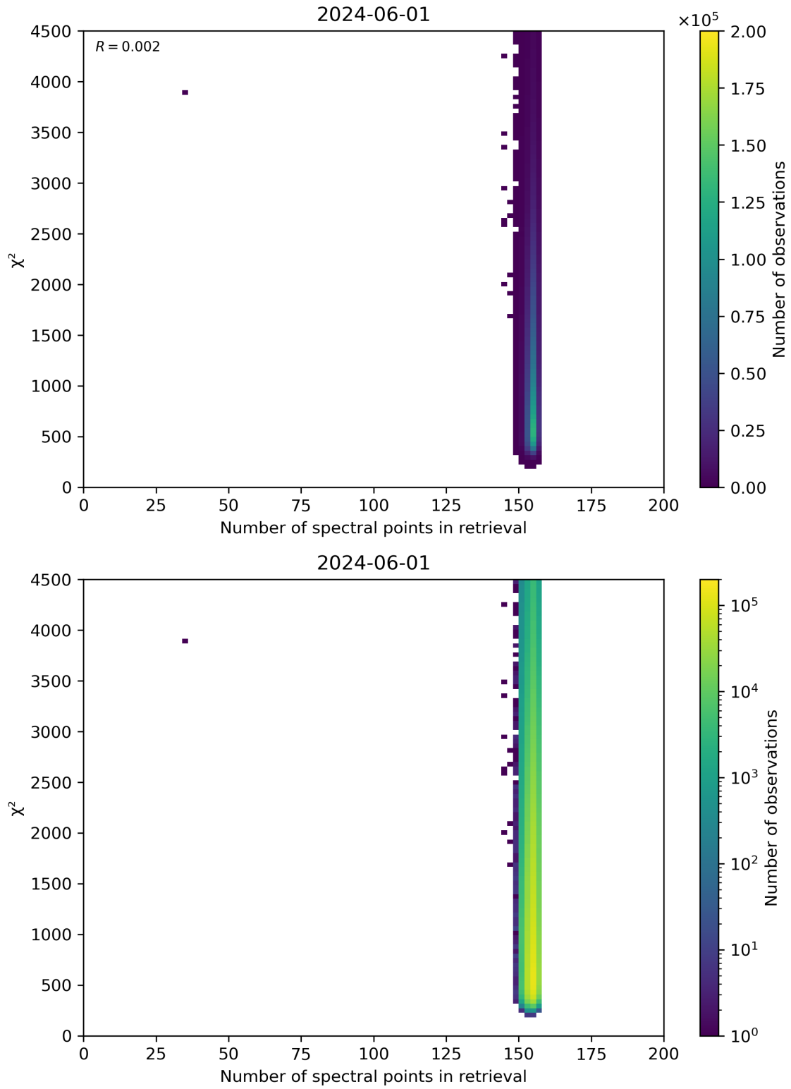
Figure 58: Scatter density plot of “Number of spectral points in retrieval” against “ \chi^2 ” for 2024-05-31 to 2024-06-02.
