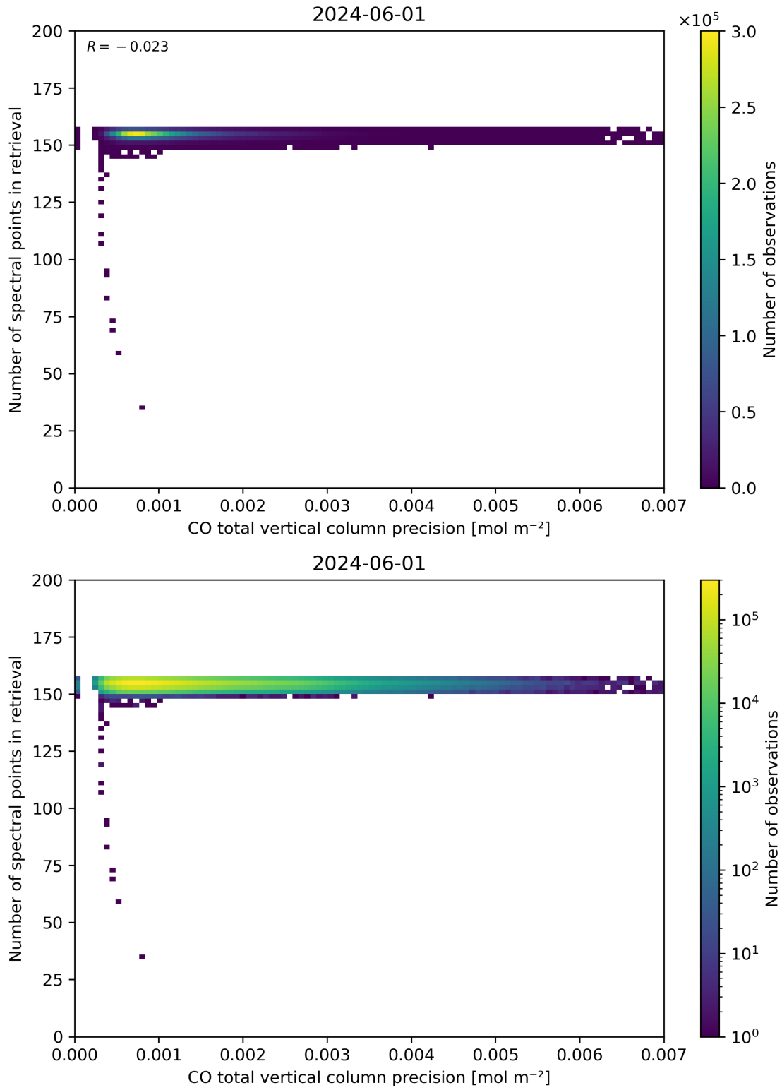
Figure 47: Scatter density plot of “CO total vertical column precision” against “Number of spectral points in retrieval” for 2024-05-31 to 2024-06-02.
