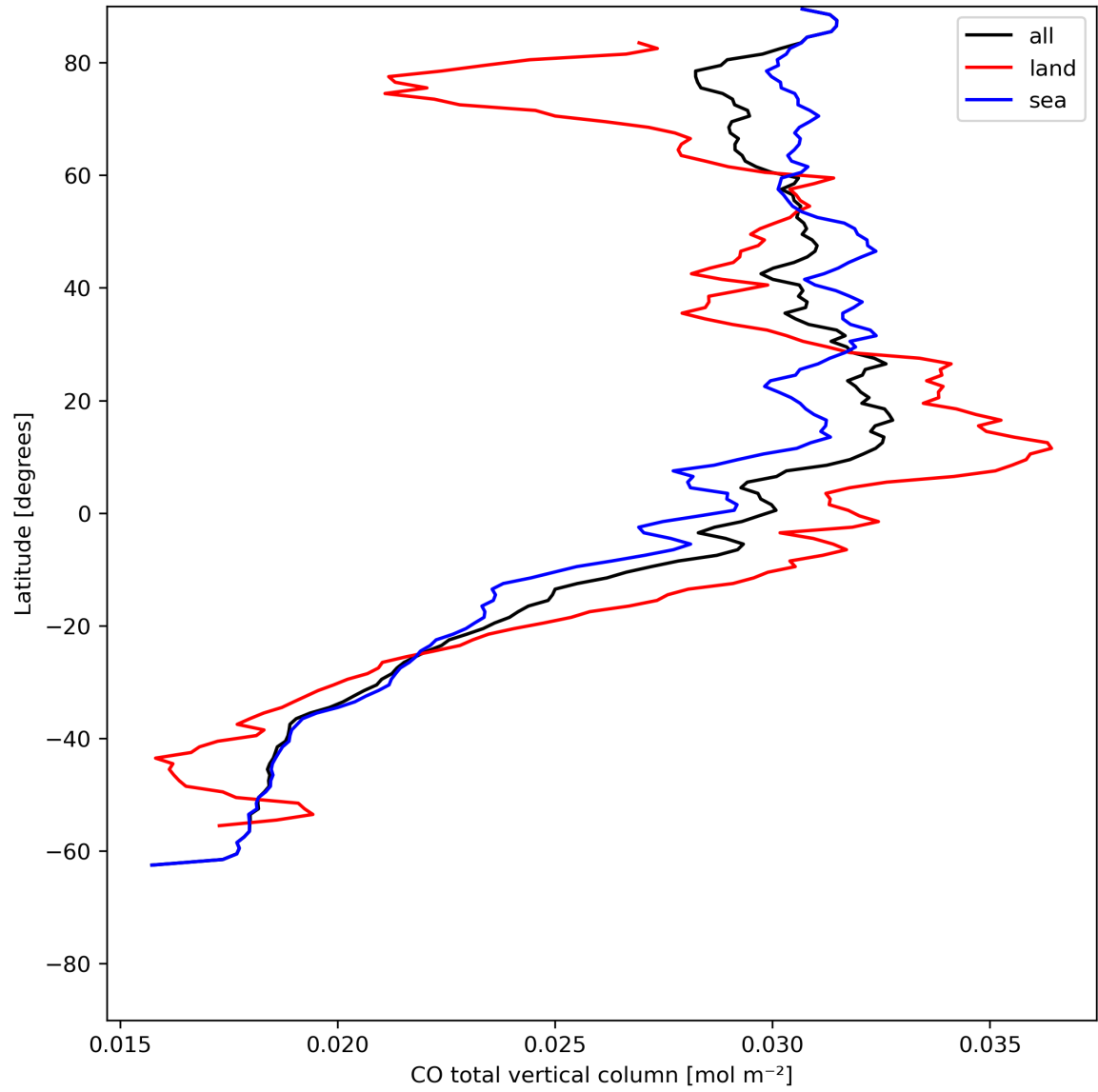
Figure 10: Zonal average of “CO total vertical column” for 2024-05-31 to 2024-06-02.
