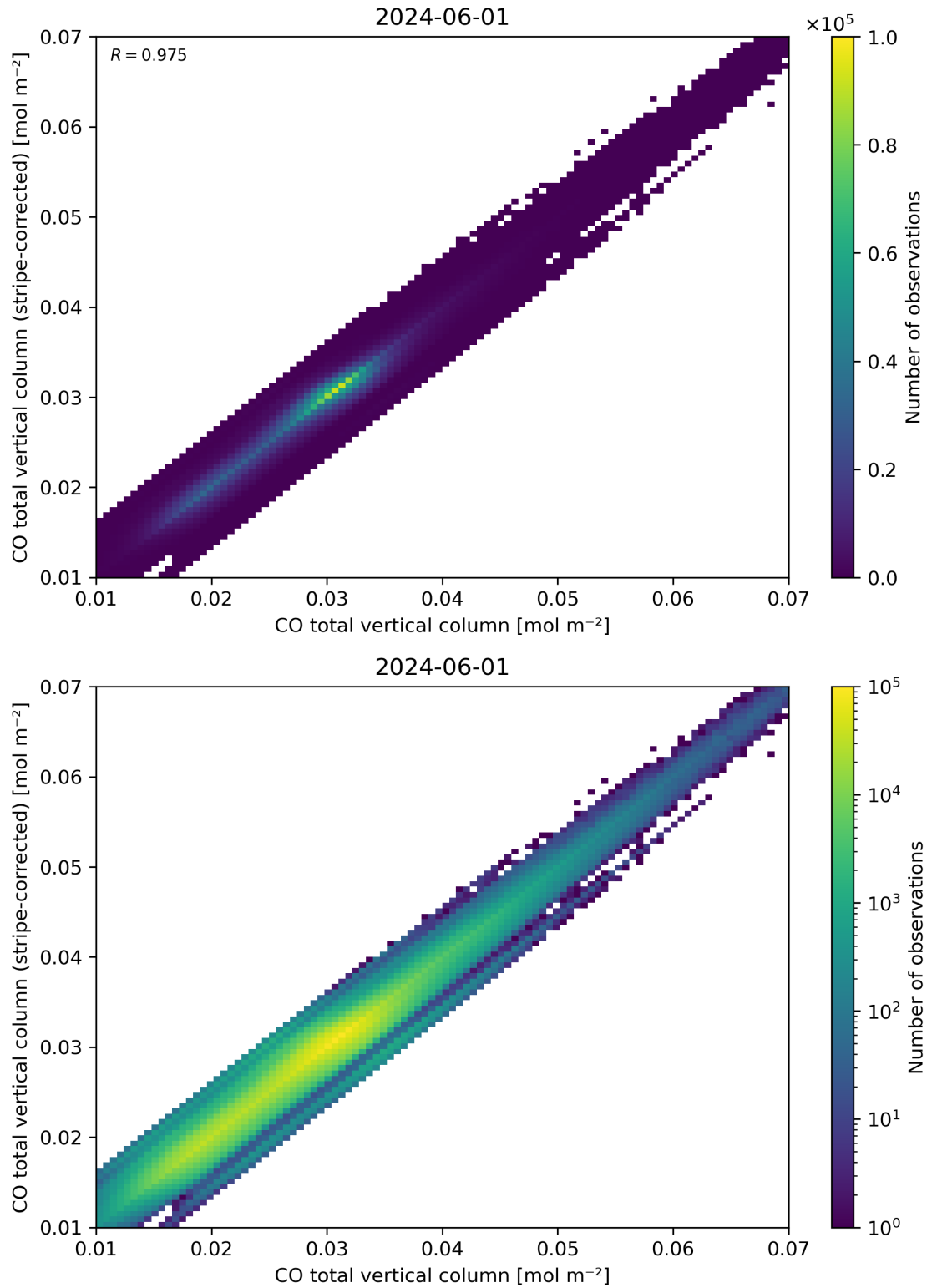
Figure 33: Scatter density plot of “CO total vertical column” against “CO total vertical column (stripe-corrected)” for 2024-05-31 to 2024-06-02.
