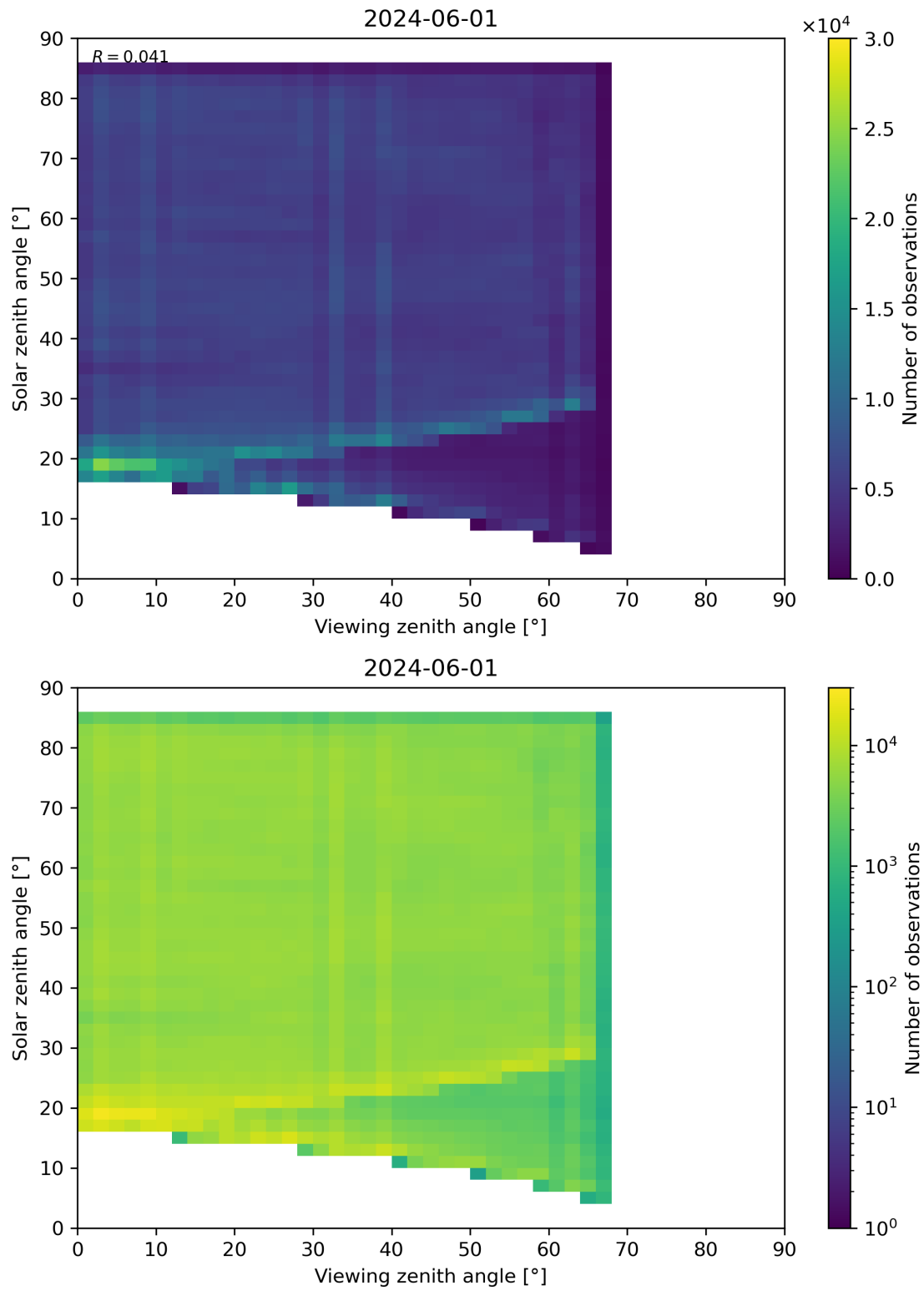
Figure 77: Scatter density plot of “Viewing zenith angle” against “Solar zenith angle” for 2024-05-31 to 2024-06-02.
