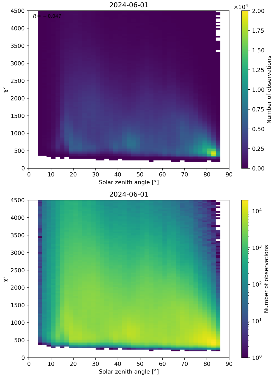
Figure 64: Scatter density plot of “Solar zenith angle” against “ \chi^2 ” for 2024-05-31 to 2024-06-02.
