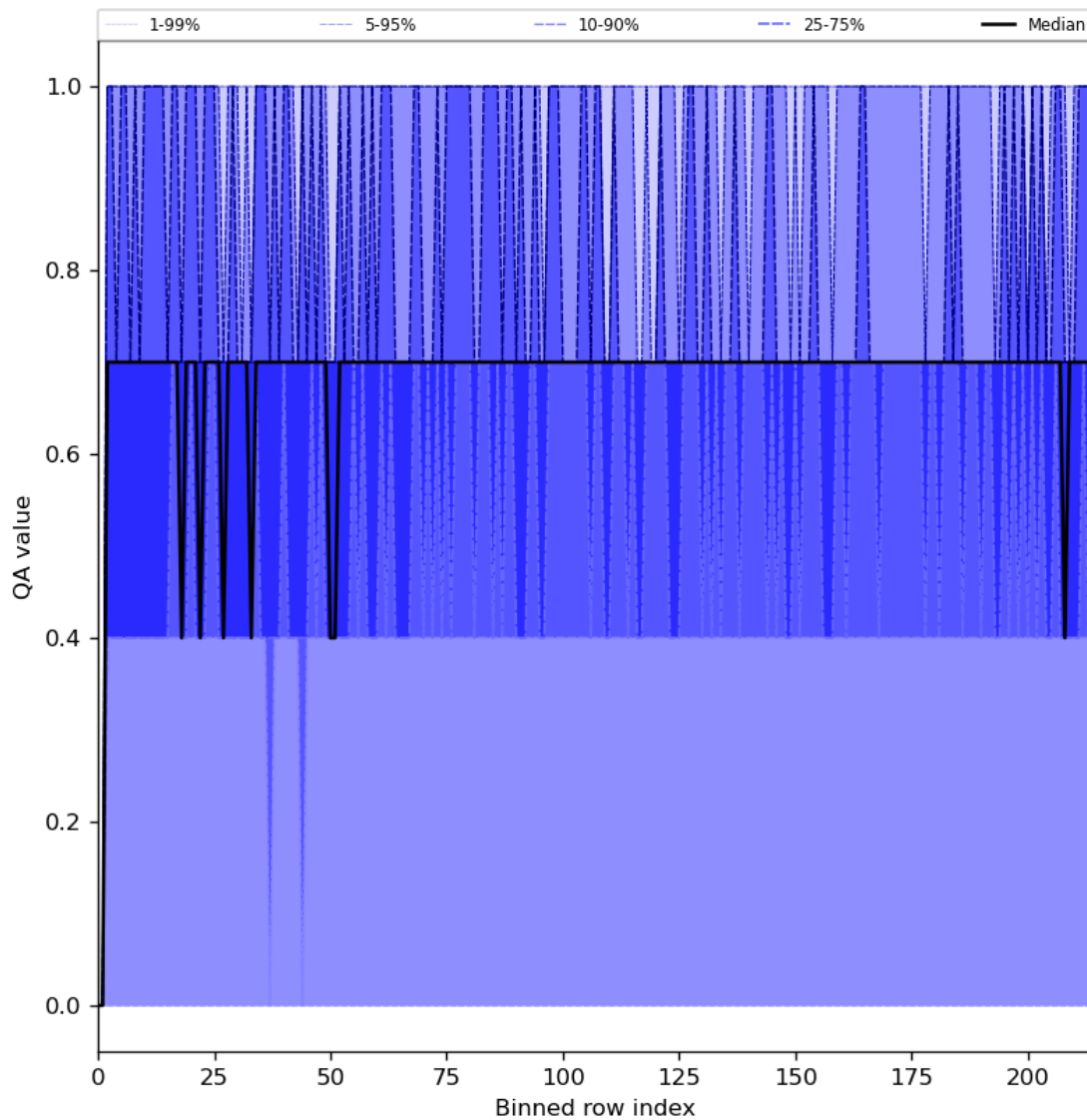
Figure 25: Along track statistics of “QA value” for 2024-05-31 to 2024-06-02
