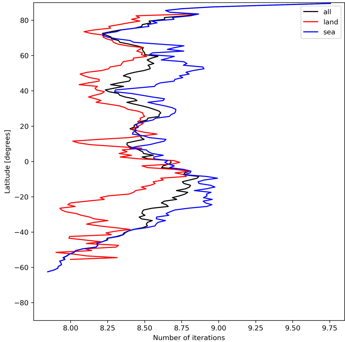
Figure 16: Zonal average of “Number of iterations” for 2024-05-31 to 2024-06-02.
