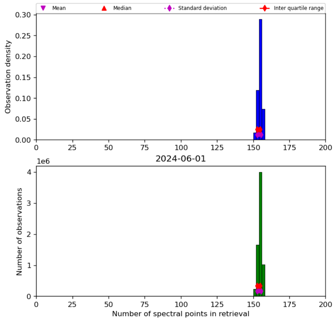
Figure 21: Histogram of “Number of spectral points in retrieval” for 2024-05-31 to 2024-06-02
