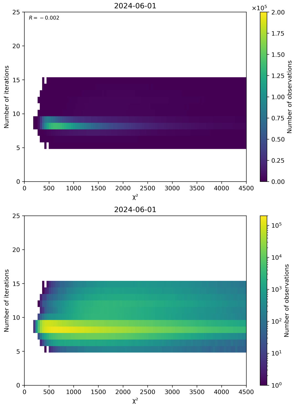
Figure 49: Scatter density plot of “ \chi^2 ” against “Number of iterations” for 2024-05-31 to 2024-06-02.
