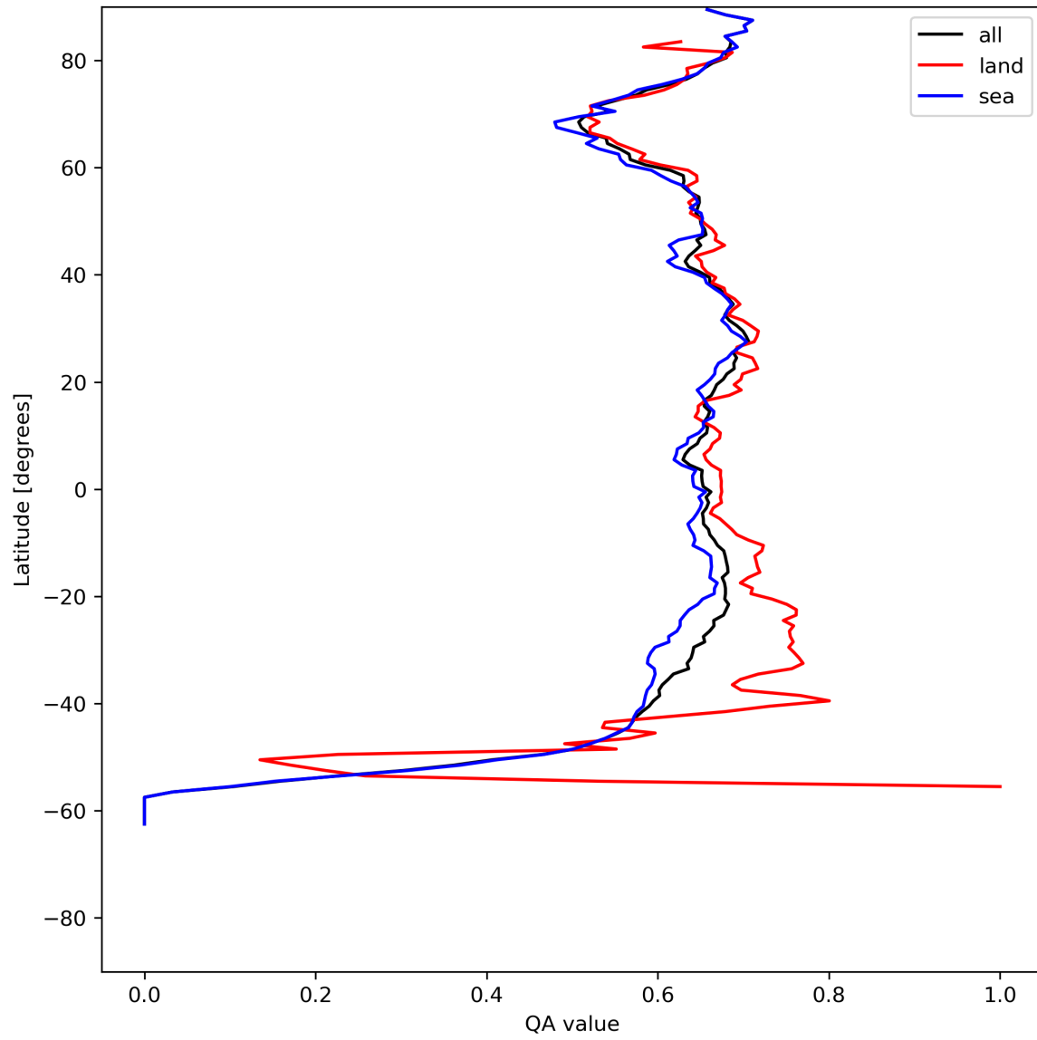
Figure 9: Zonal average of “QA value” for 2024-05-31 to 2024-06-02.
