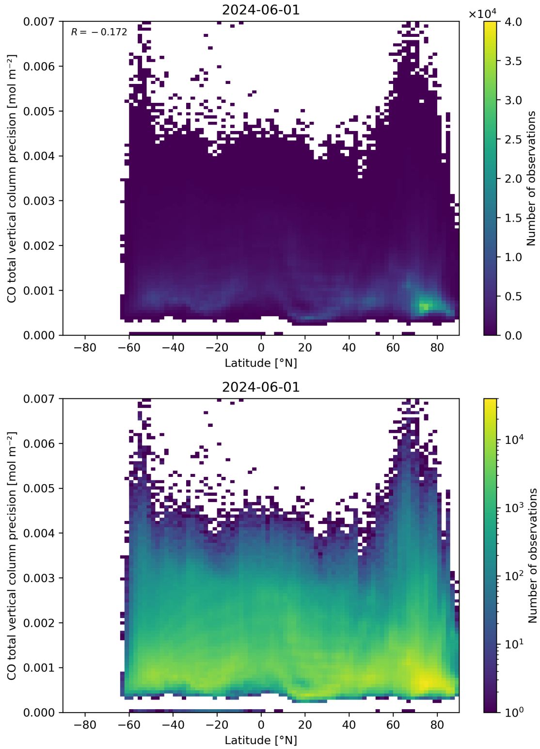
Figure 53: Scatter density plot of “Latitude” against “CO total vertical column precision” for 2024-05-31 to 2024-06-02.
