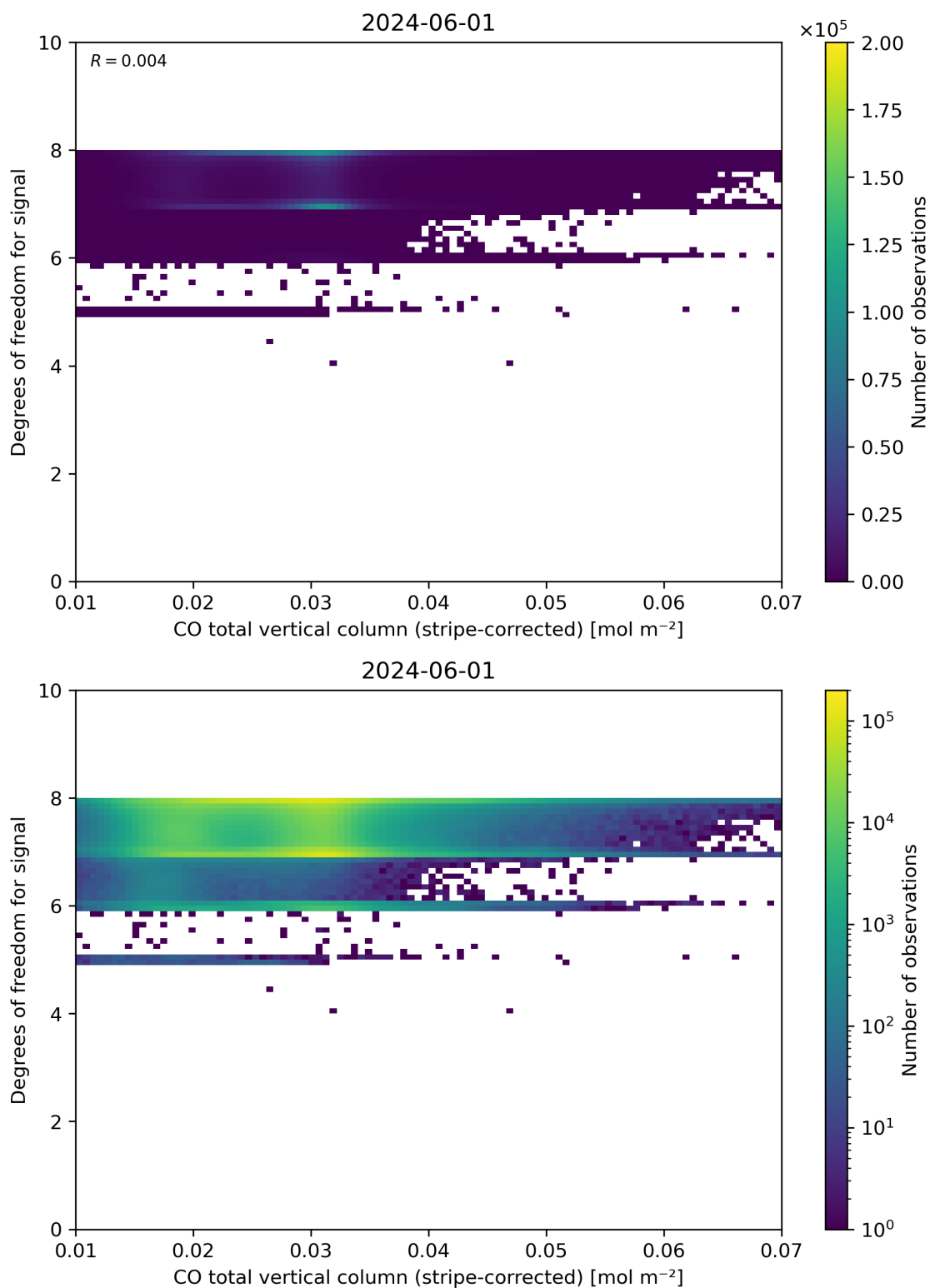
Figure 38: Scatter density plot of “CO total vertical column (stripe-corrected)” against “Degrees of freedom for signal” for 2024-05-31 to 2024-06-02.
