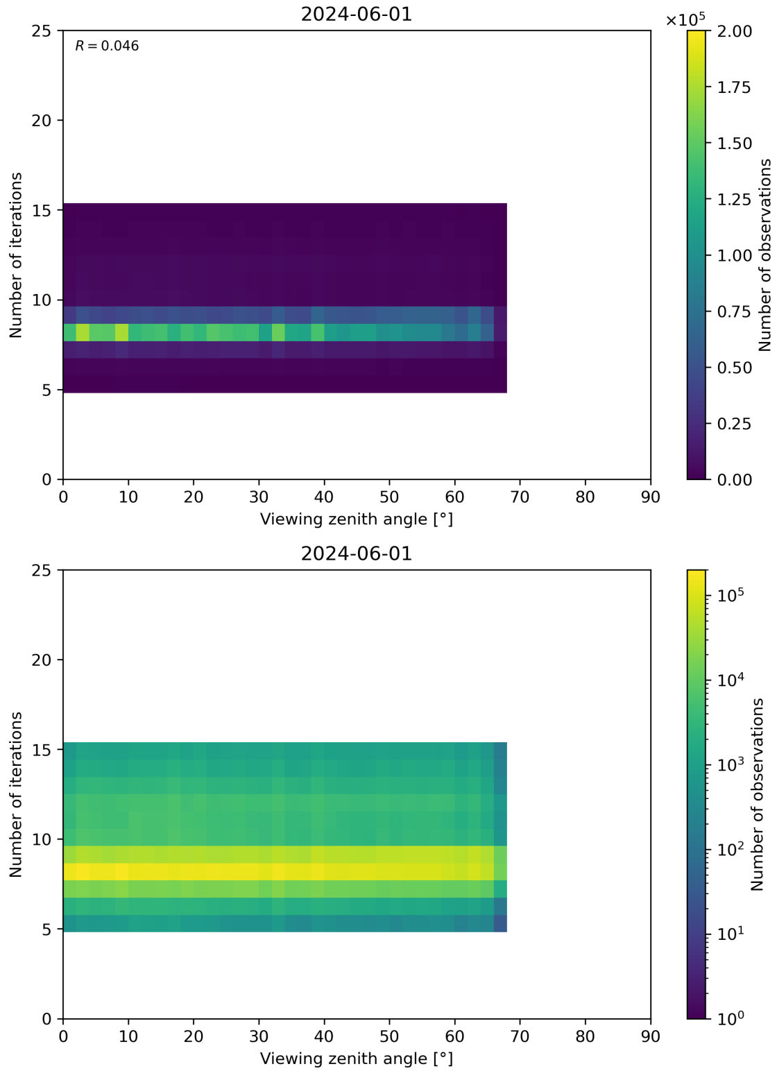
Figure 75: Scatter density plot of “Viewing zenith angle” against “Number of iterations” for 2024-05-31 to 2024-06-02.
