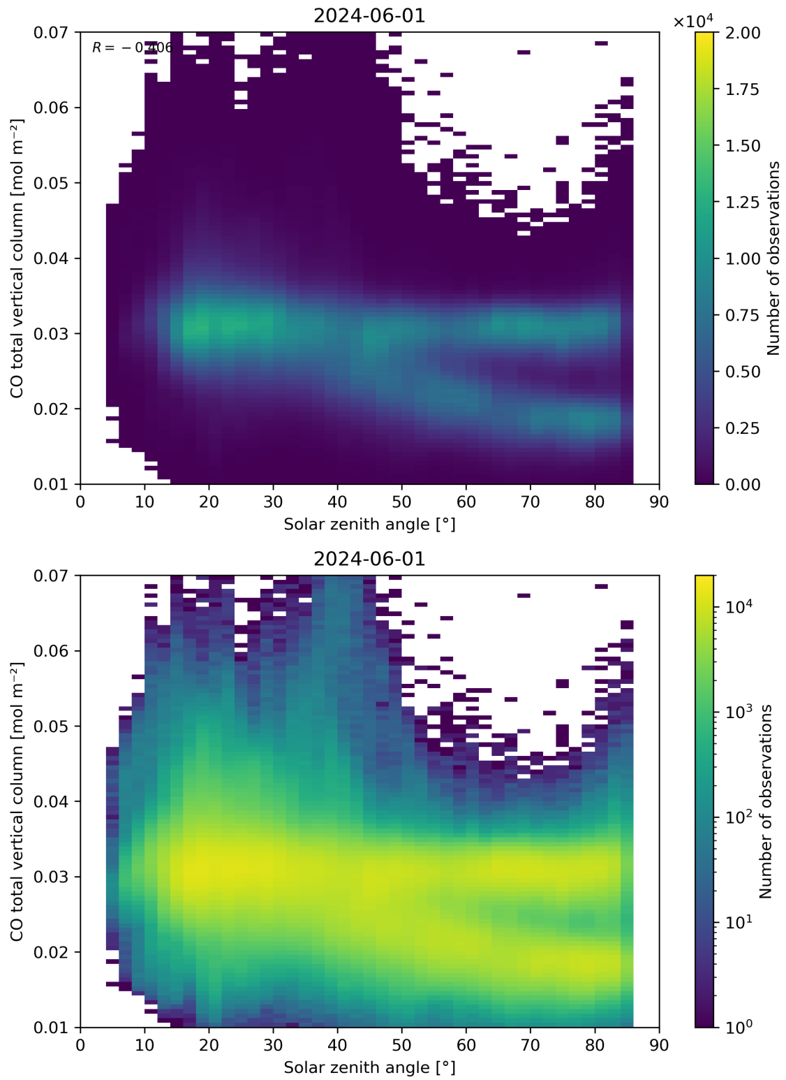
Figure 61: Scatter density plot of “Solar zenith angle” against “CO total vertical column” for 2024-05-31 to 2024-06-02.
