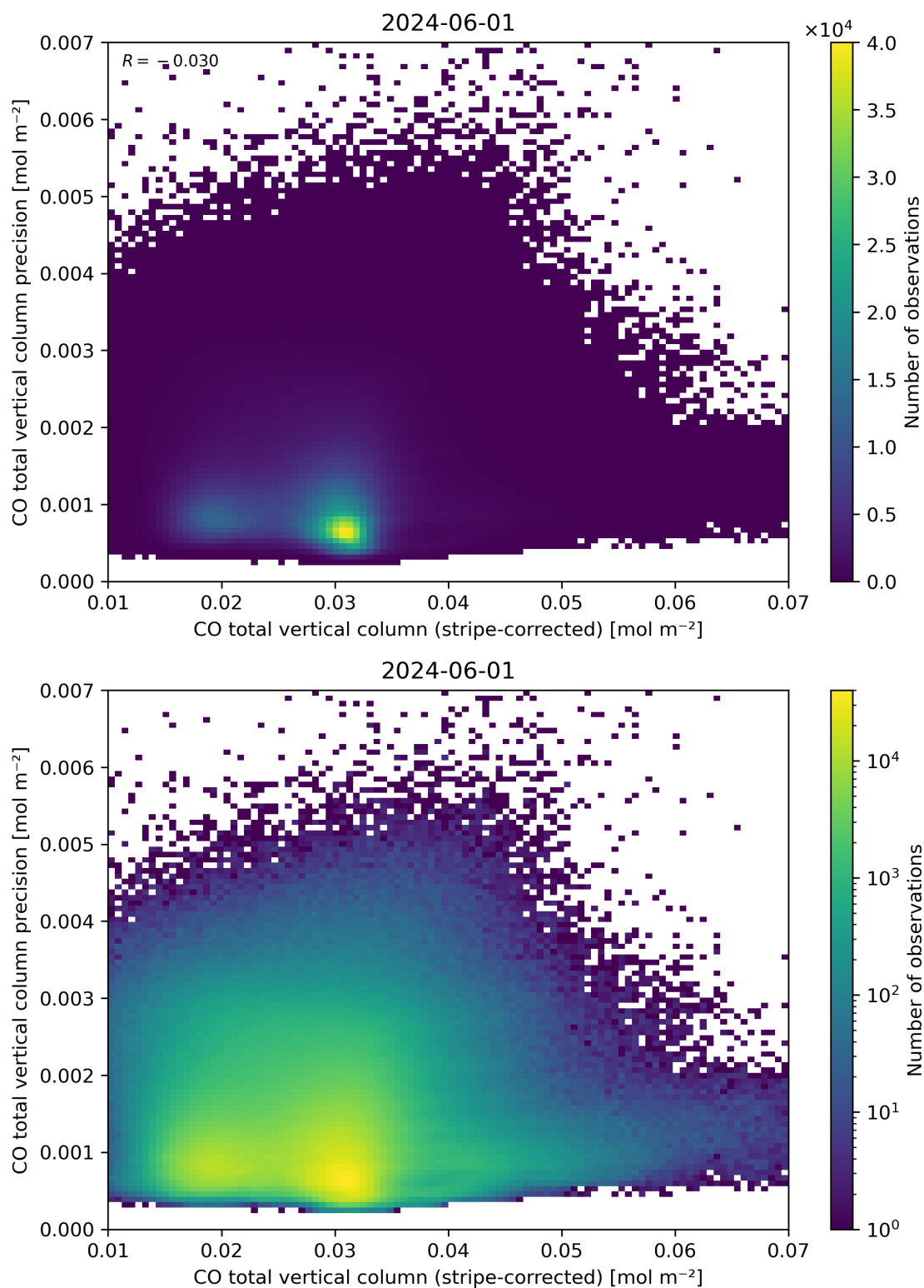
Figure 36: Scatter density plot of “CO total vertical column (stripe-corrected)” against “CO total vertical column precision” for 2024-05-31 to 2024-06-02.
