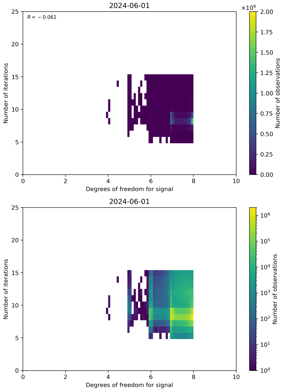
Figure 50: Scatter density plot of “Degrees of freedom for signal” against “Number of iterations” for 2024-05-31 to 2024-06-02.
