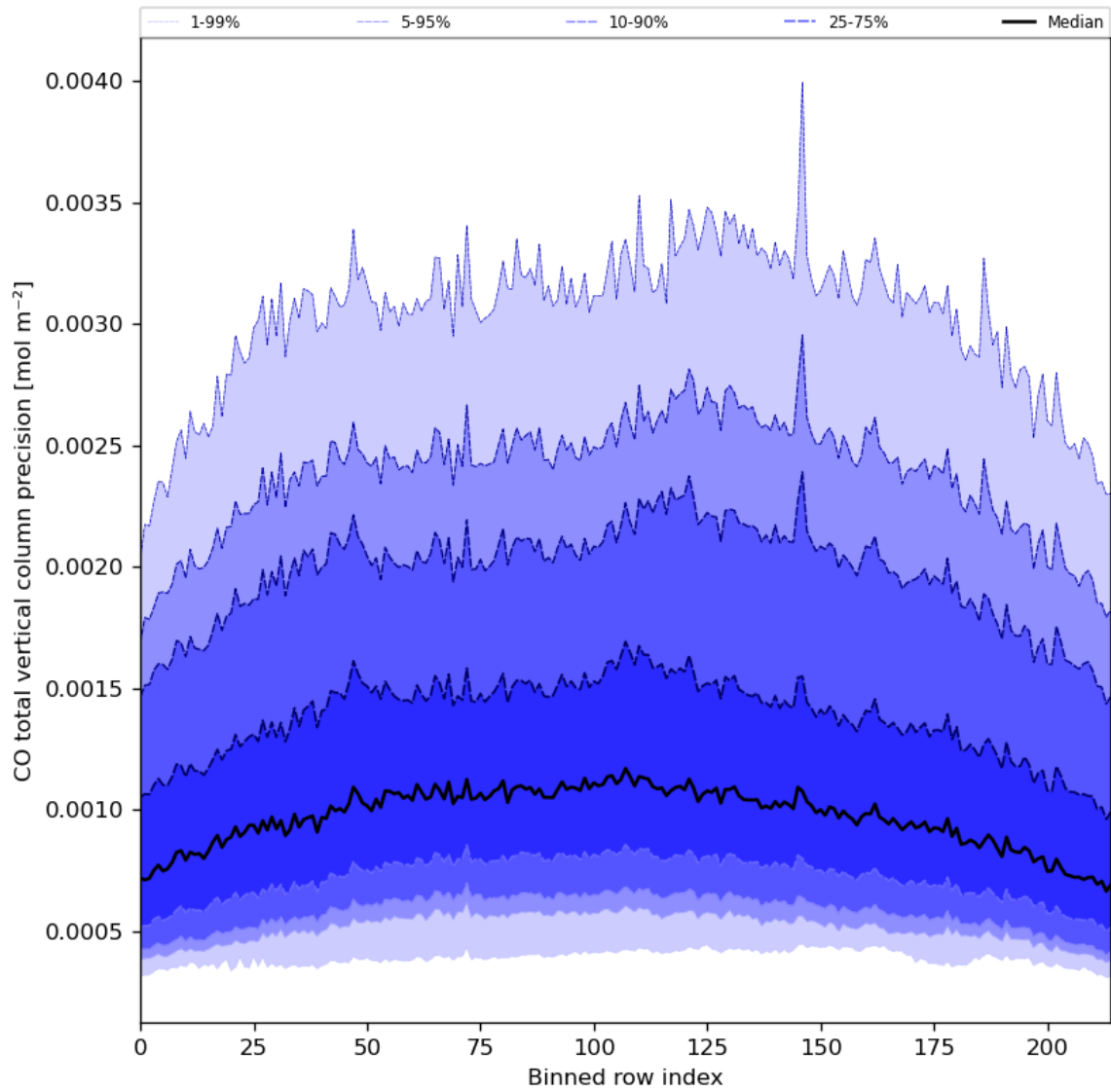
Figure 28: Along track statistics of “CO total vertical column precision” for 2024-05-31 to 2024-06-02
