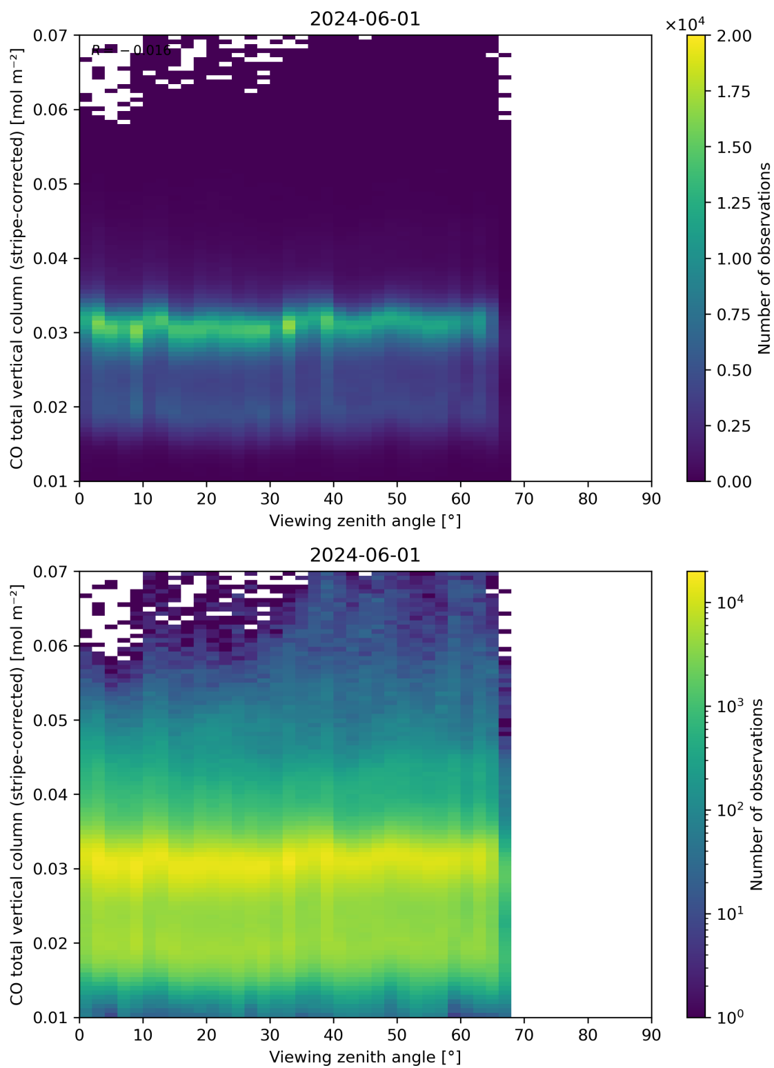
Figure 70: Scatter density plot of “Viewing zenith angle” against “CO total vertical column (stripe-corrected)” for 2024-05-31 to 2024-06-02.
