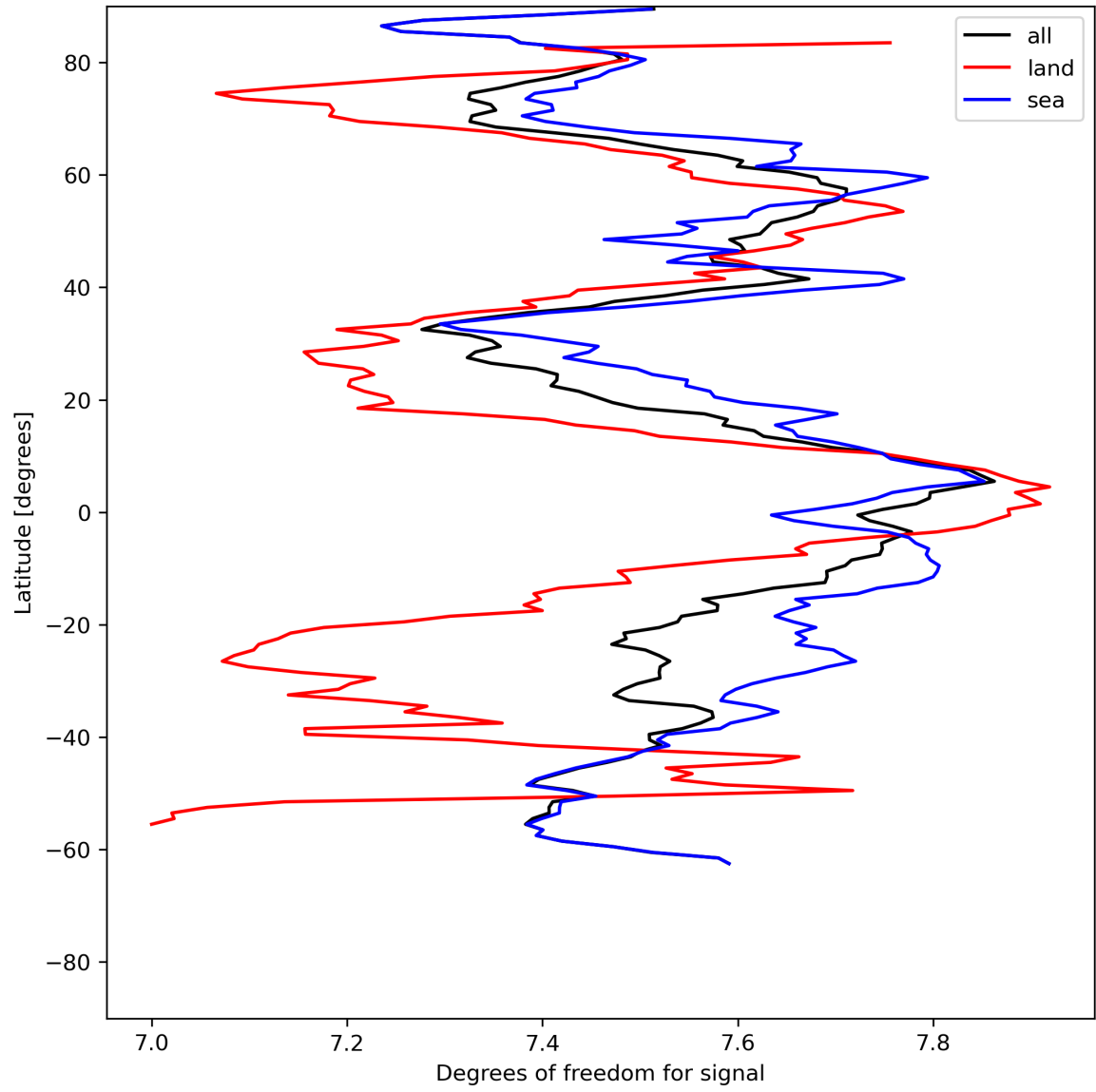
Figure 15: Zonal average of “Degrees of freedom for signal” for 2024-05-31 to 2024-06-02.
