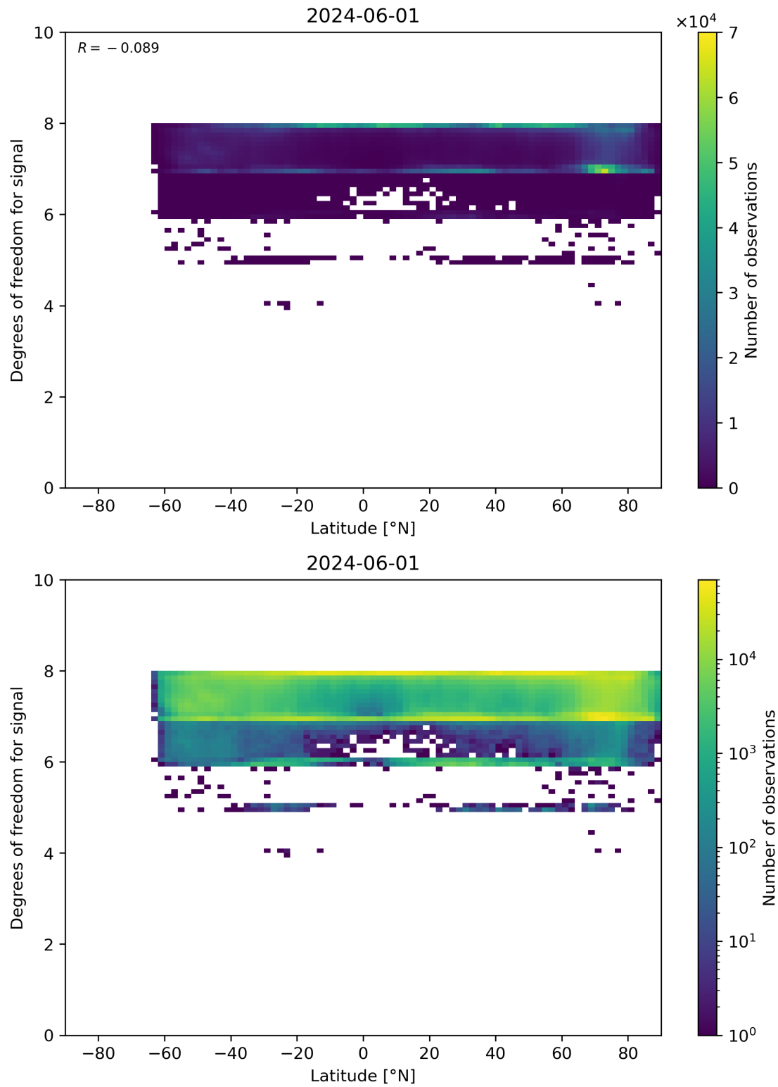
Figure 55: Scatter density plot of “Latitude” against “Degrees of freedom for signal” for 2024-05-31 to 2024-06-02.
