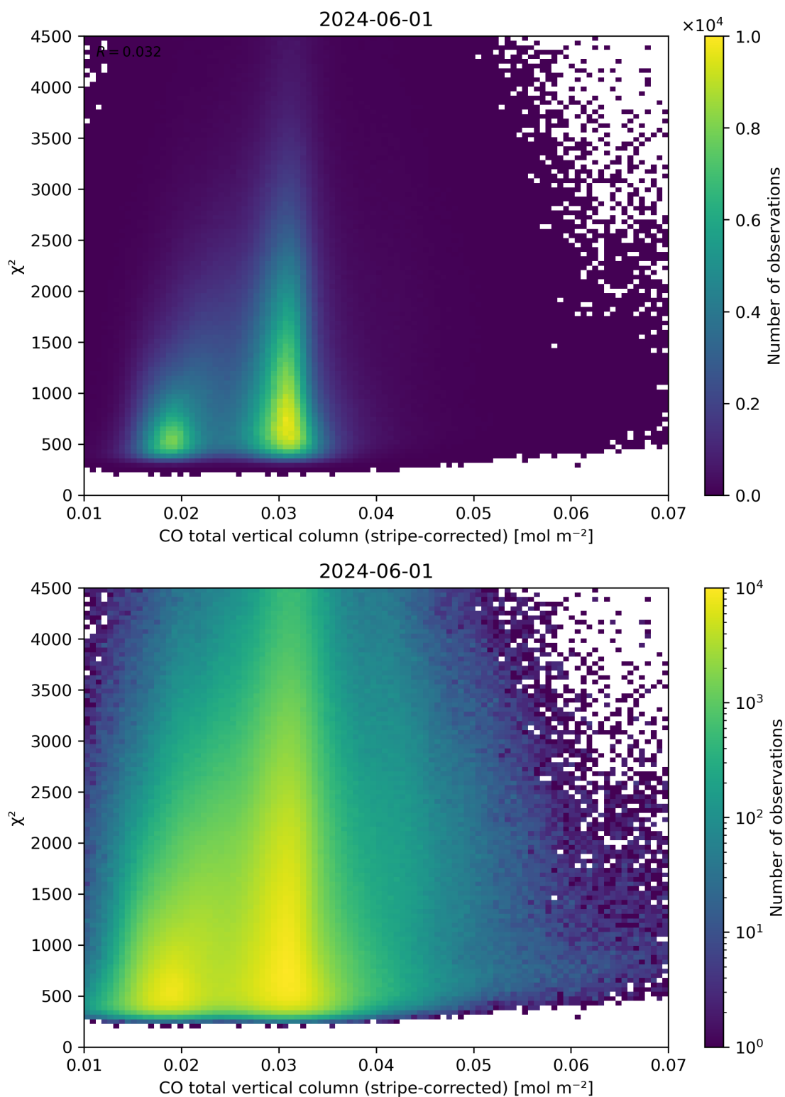
Figure 37: Scatter density plot of “CO total vertical column (stripe-corrected)” against “ \chi^2 ” for 2024-05-31 to 2024-06-02.
