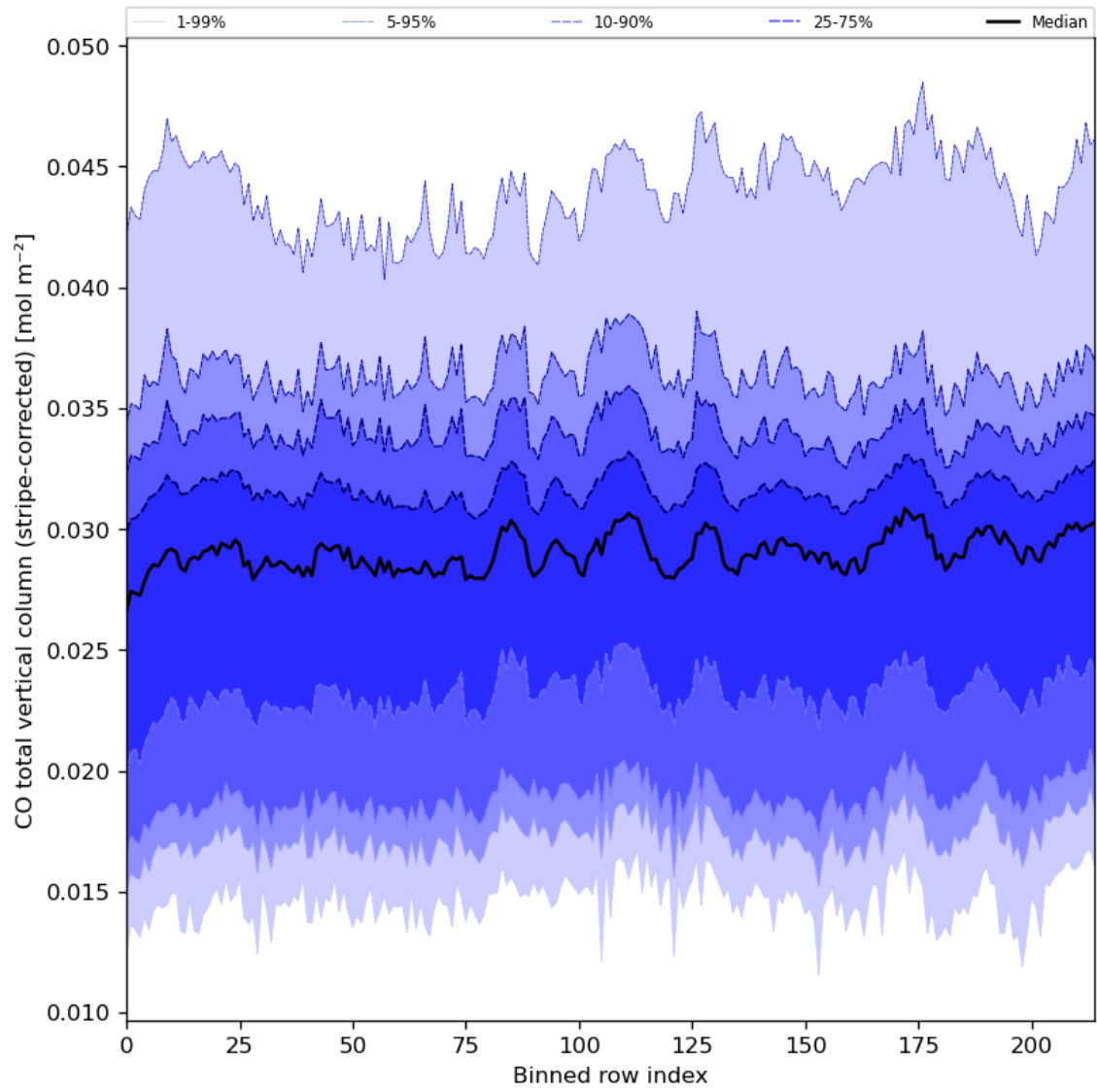
Figure 27: Along track statistics of “CO total vertical column (stripe-corrected)” for 2024-05-31 to 2024-06-02
