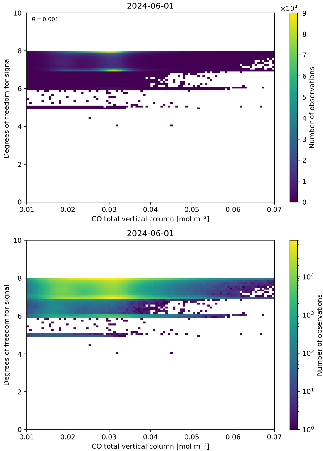
Figure 41: Scatter density plot of “CO total vertical column” against “Degrees of freedom for signal” for 2024-05-31 to 2024-06-02.
