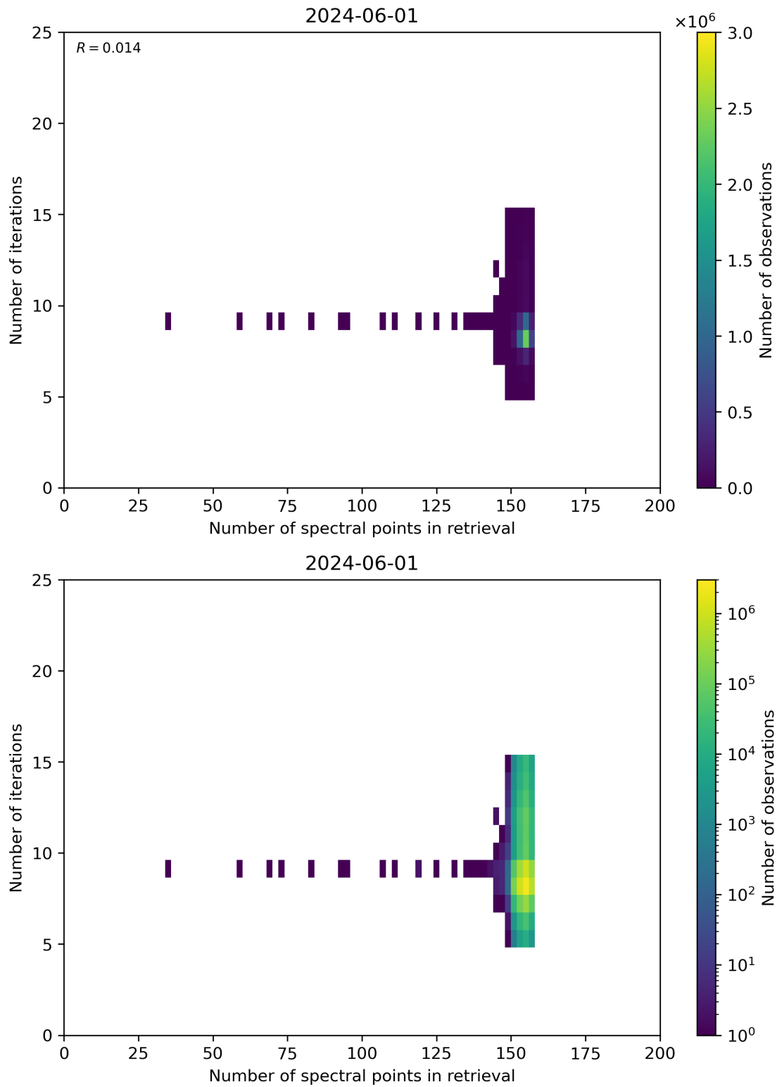
Figure 60: Scatter density plot of “Number of spectral points in retrieval” against “Number of iterations” for 2024-05-31 to 2024-06-02.
