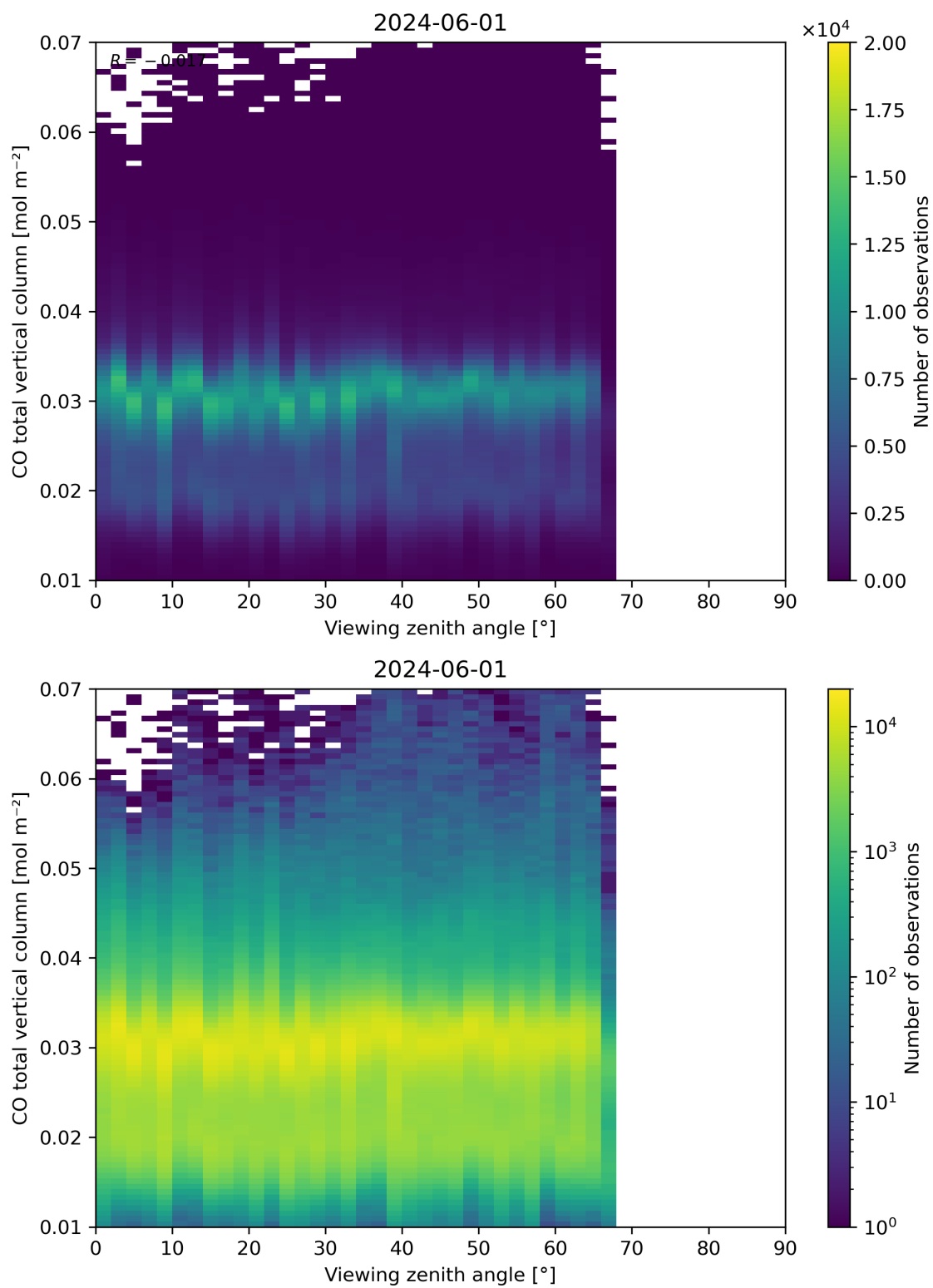
Figure 69: Scatter density plot of “Viewing zenith angle” against “CO total vertical column” for 2024-05-31 to 2024-06-02.
