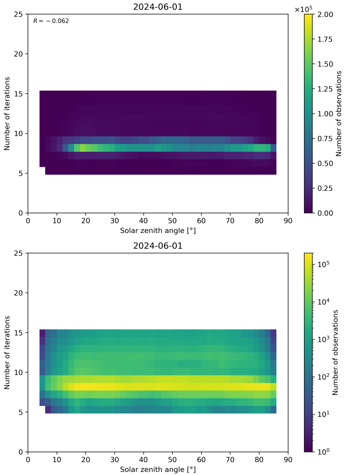
Figure 67: Scatter density plot of “Solar zenith angle” against “Number of iterations” for 2024-05-31 to 2024-06-02.
