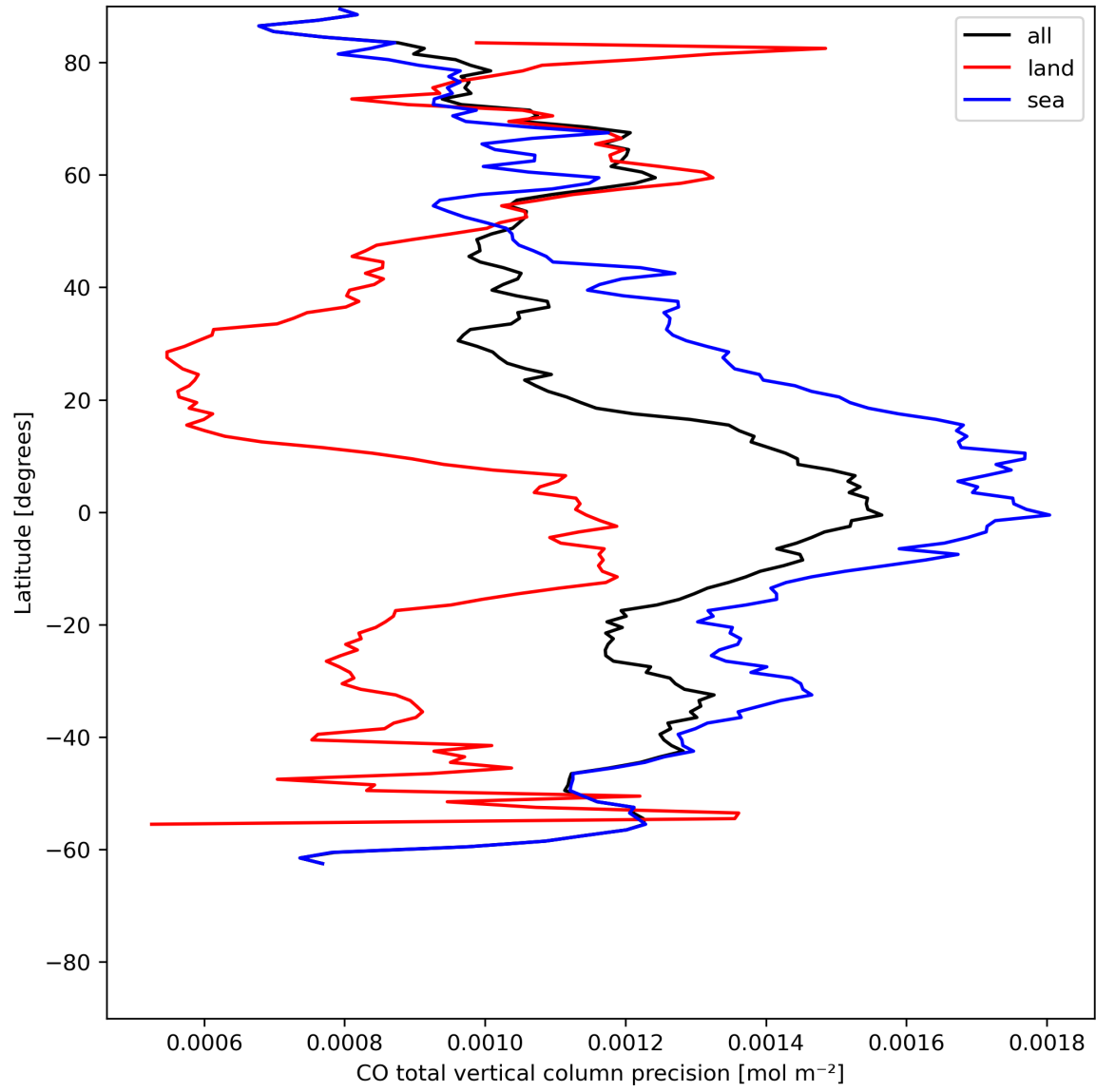
Figure 12: Zonal average of “CO total vertical column precision” for 2024-05-31 to 2024-06-02.
