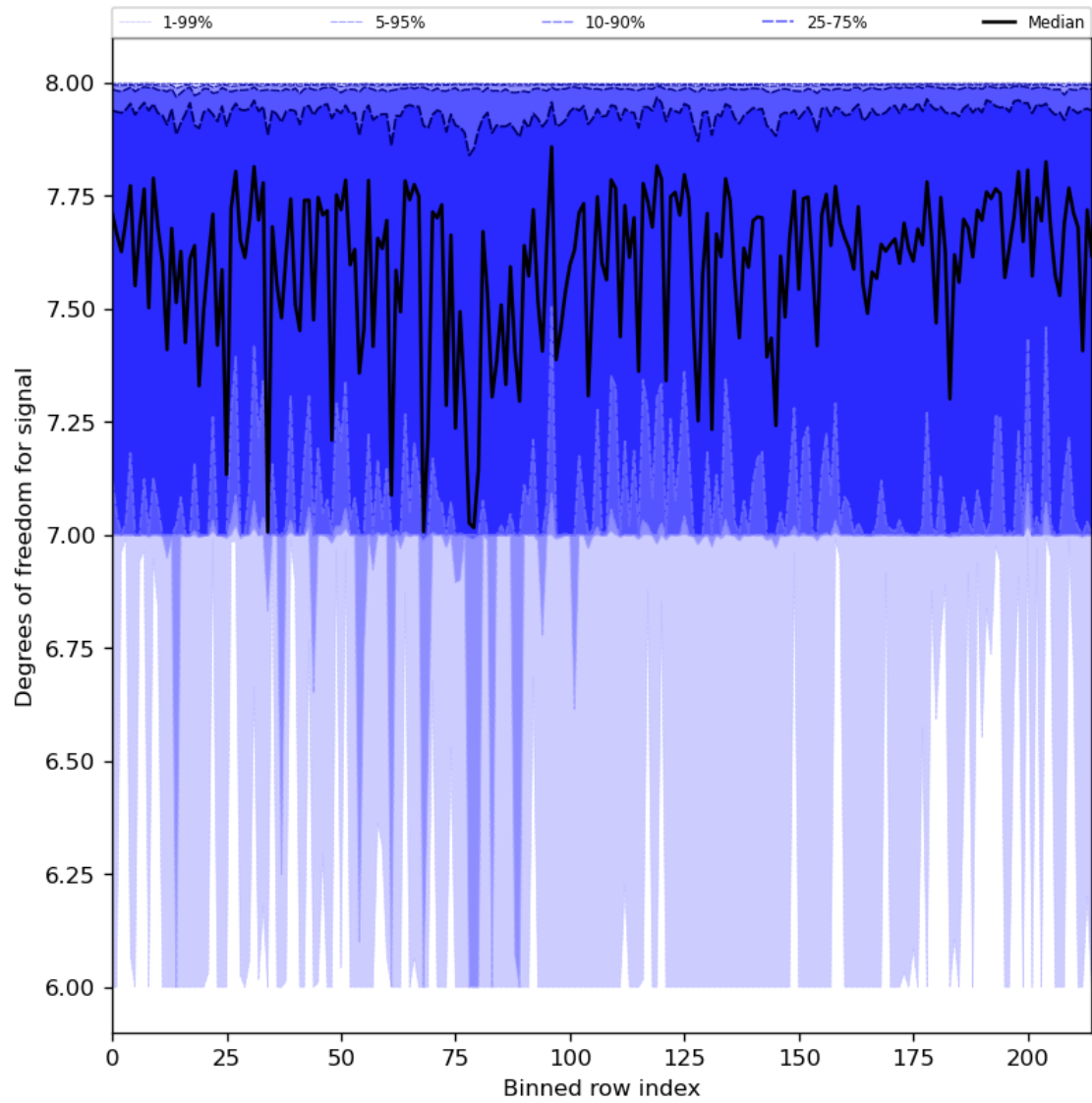
Figure 31: Along track statistics of “Degrees of freedom for signal” for 2024-05-31 to 2024-06-02
