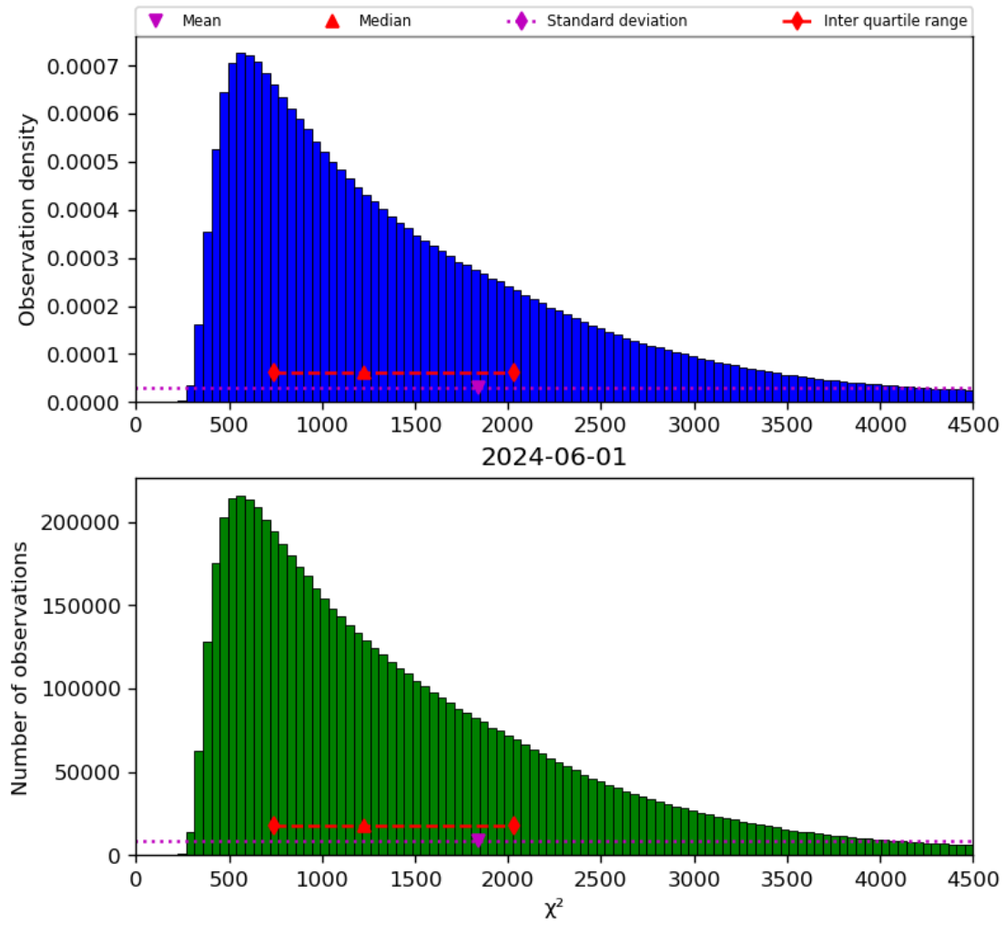
Figure 22: Histogram of “ \chi^2 ” for 2024-05-31 to 2024-06-02
