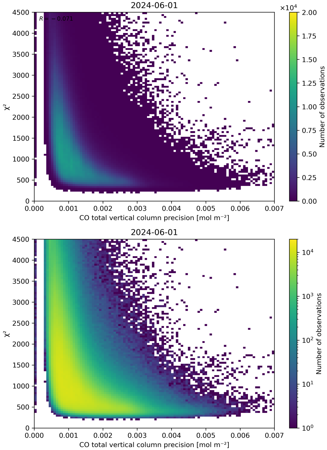
Figure 44: Scatter density plot of “CO total vertical column precision” against “ \chi^2 ” for 2024-05-31 to 2024-06-02.
