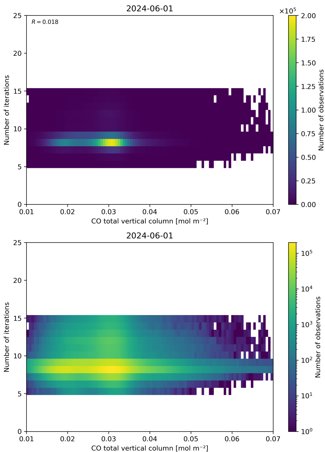
Figure 42: Scatter density plot of “CO total vertical column” against “Number of iterations” for 2024-05-31 to 2024-06-02.
