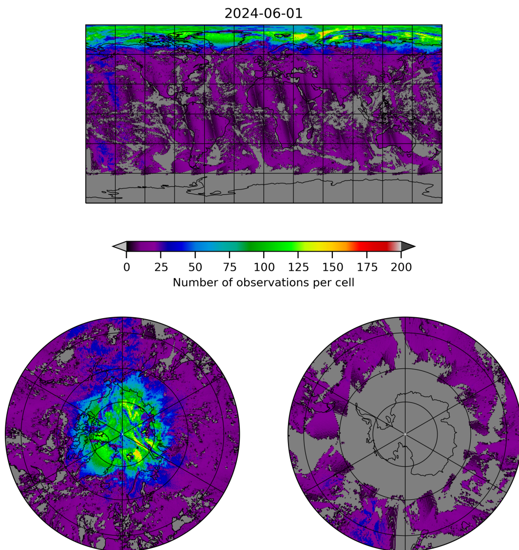
Figure 8: Map of the number of observations for 2024-05-31 to 2024-06-02
