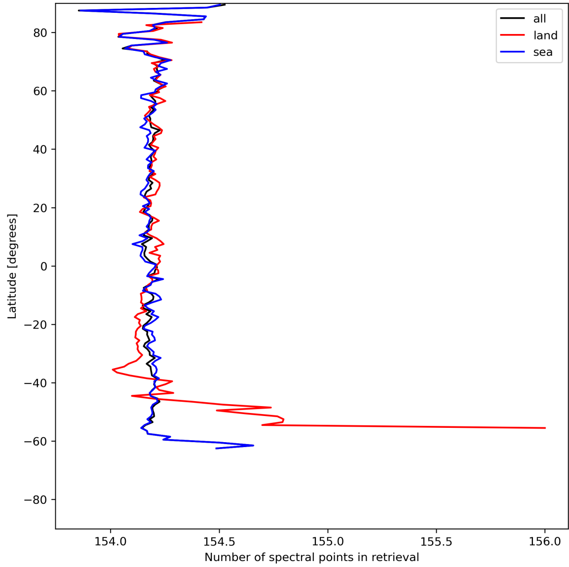
Figure 13: Zonal average of “Number of spectral points in retrieval” for 2024-05-31 to 2024-06-02.
