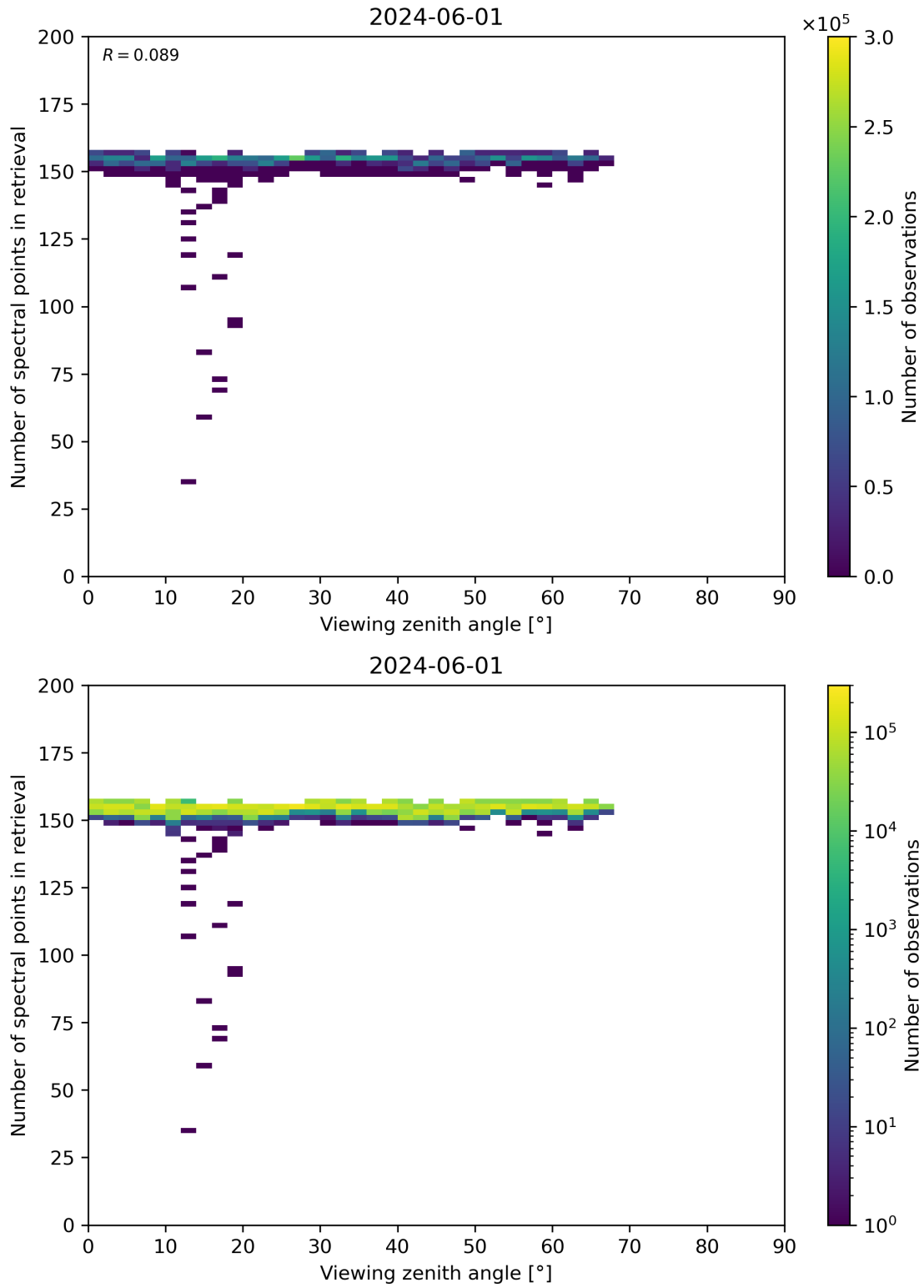
Figure 76: Scatter density plot of “Viewing zenith angle” against “Number of spectral points in retrieval” for 2024-05-31 to 2024-06-02.
