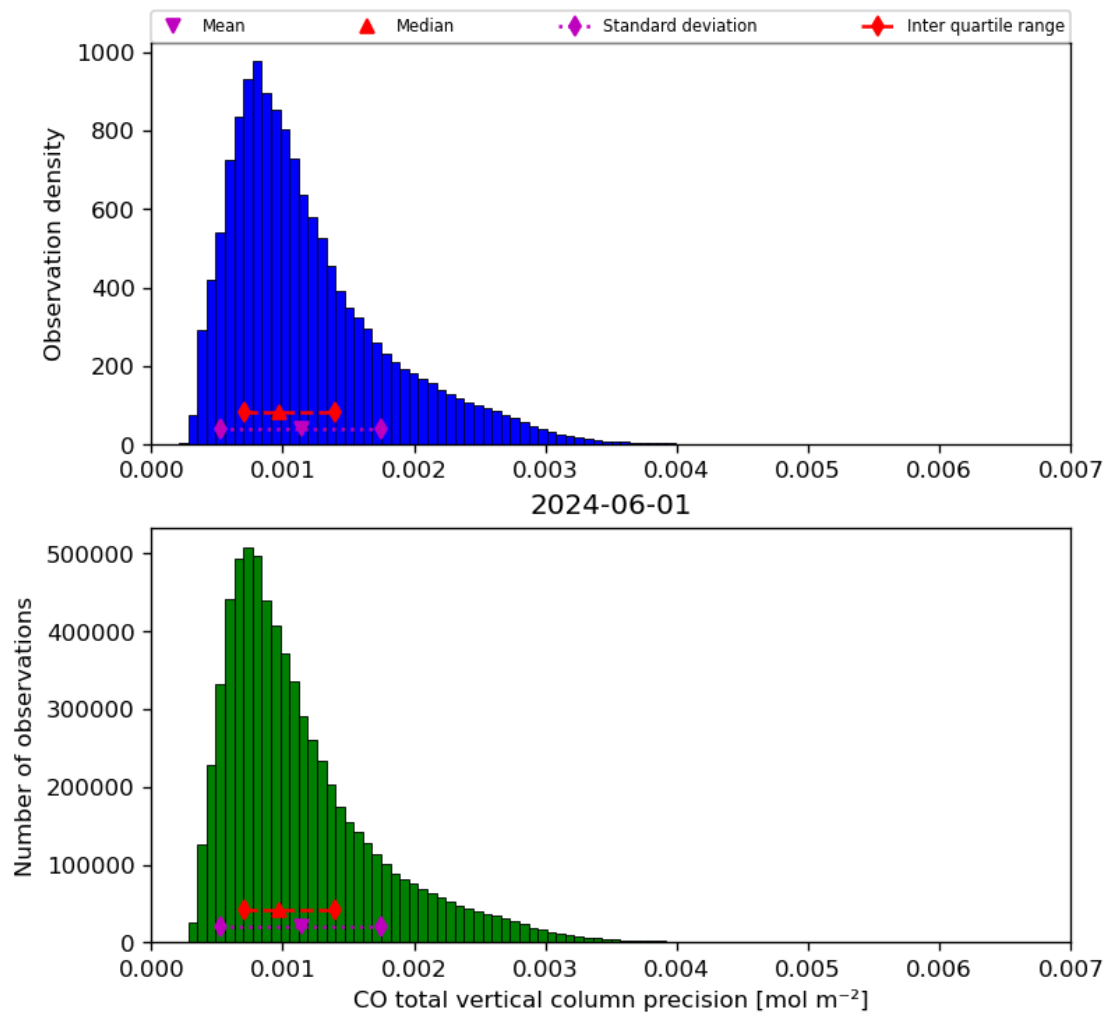
Figure 20: Histogram of “CO total vertical column precision” for 2024-05-31 to 2024-06-02
