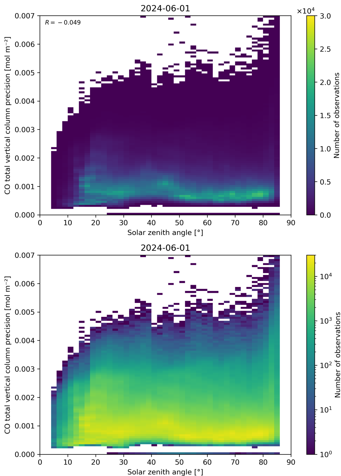
Figure 63: Scatter density plot of “Solar zenith angle” against “CO total vertical column precision” for 2024-05-31 to 2024-06-02.
