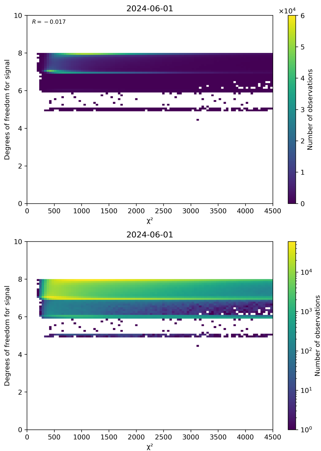
Figure 48: Scatter density plot of “ \chi^2 ” against “Degrees of freedom for signal” for 2024-05-31 to 2024-06-02.
