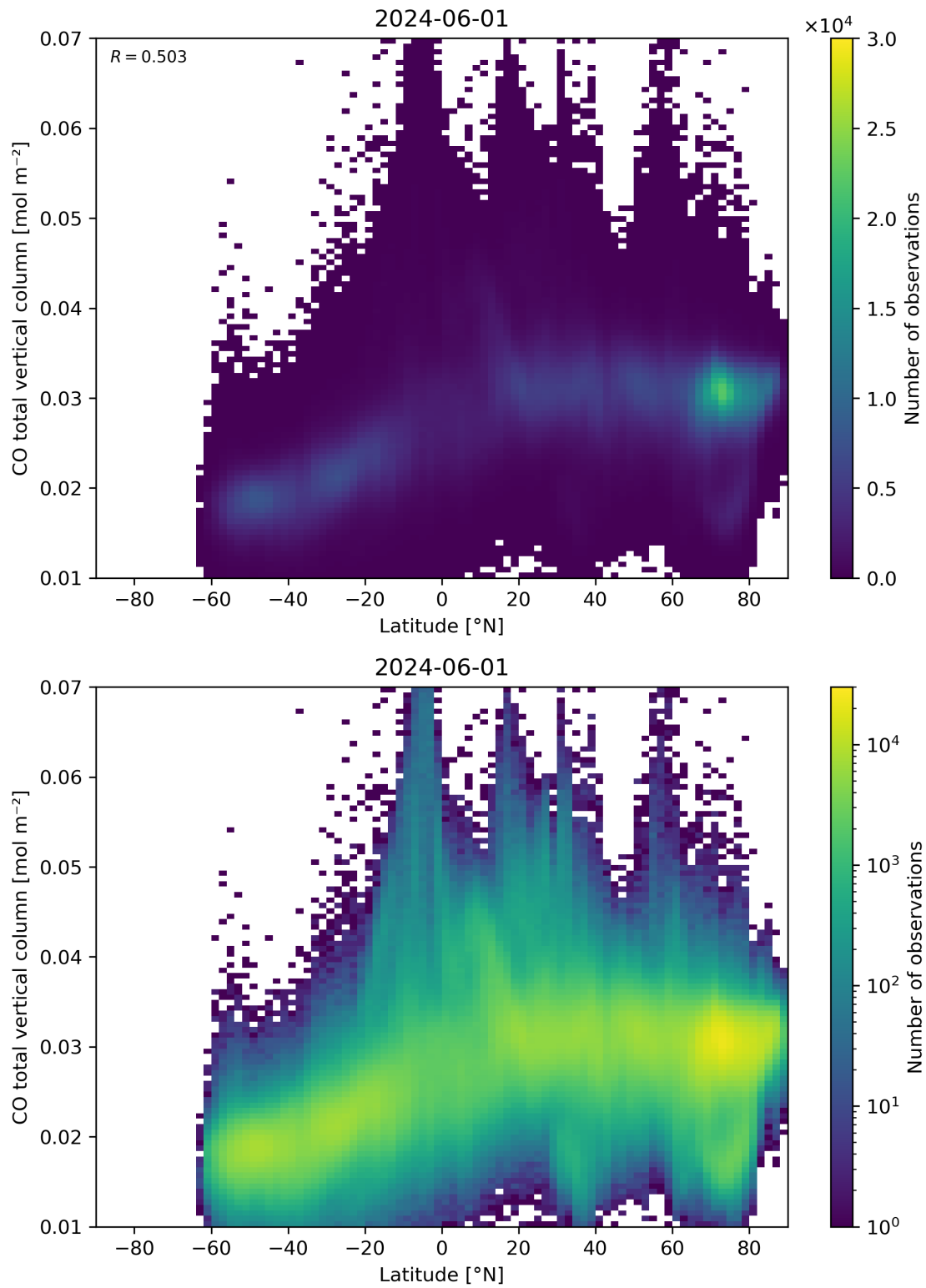
Figure 51: Scatter density plot of “Latitude” against “CO total vertical column” for 2024-05-31 to 2024-06-02.
