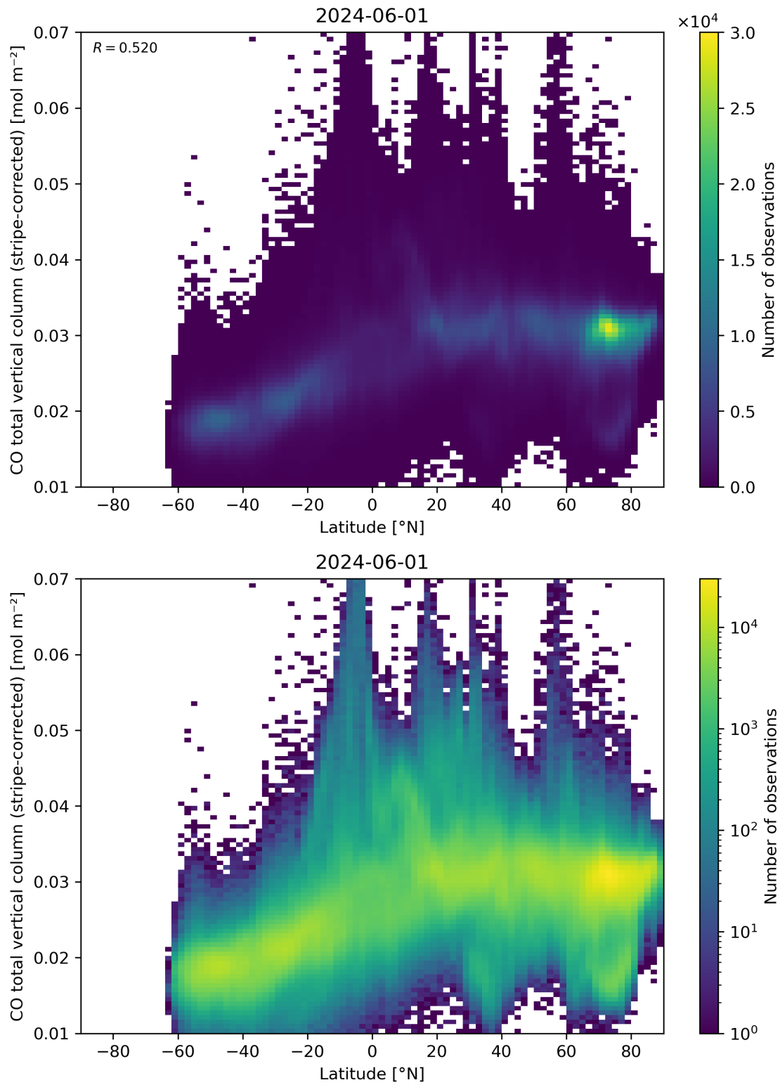
Figure 52: Scatter density plot of “Latitude” against “CO total vertical column (stripe-corrected)” for 2024-05-31 to 2024-06-02.
