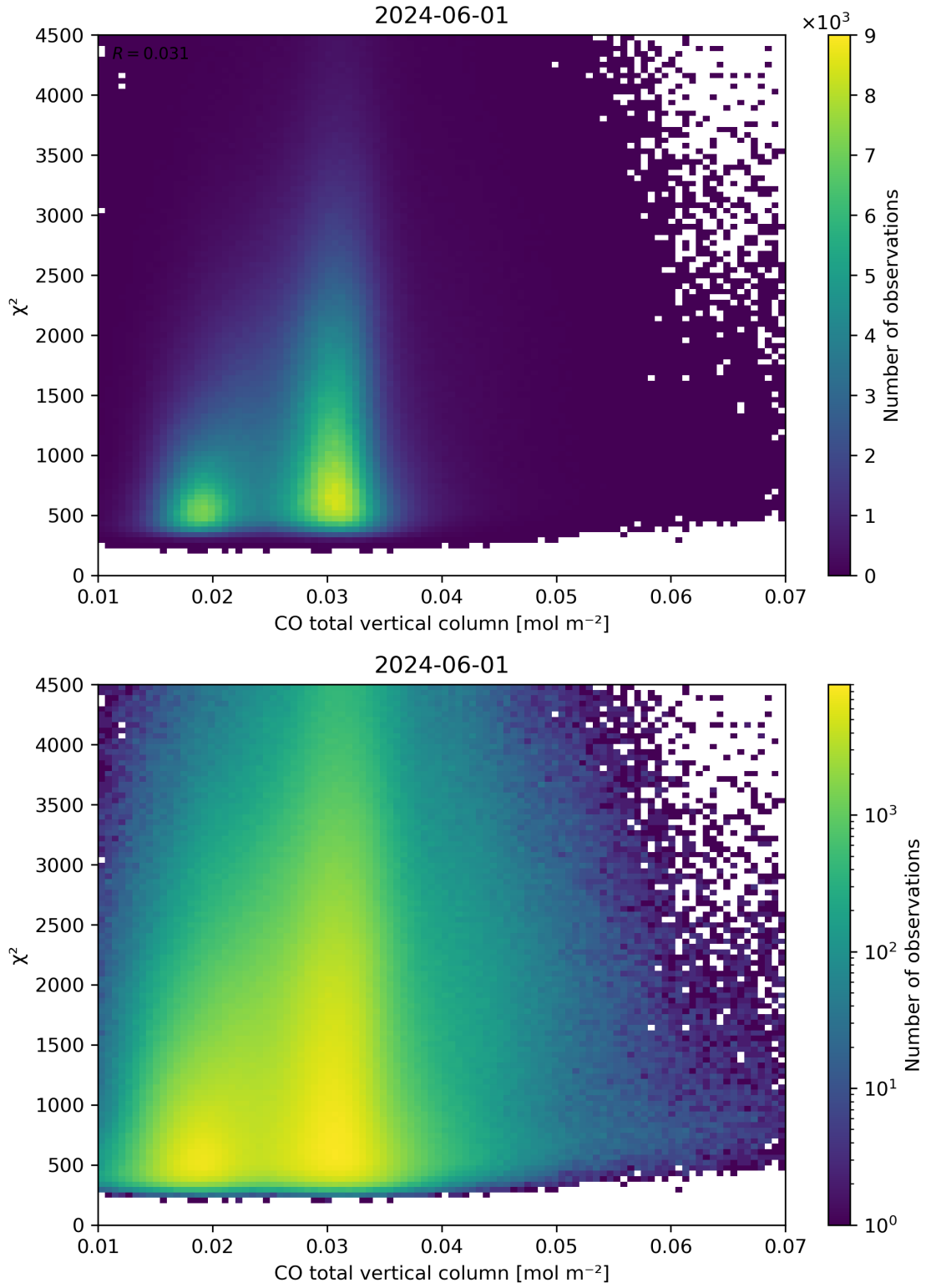
Figure 35: Scatter density plot of “CO total vertical column” against “ \chi^2 ” for 2024-05-31 to 2024-06-02.
