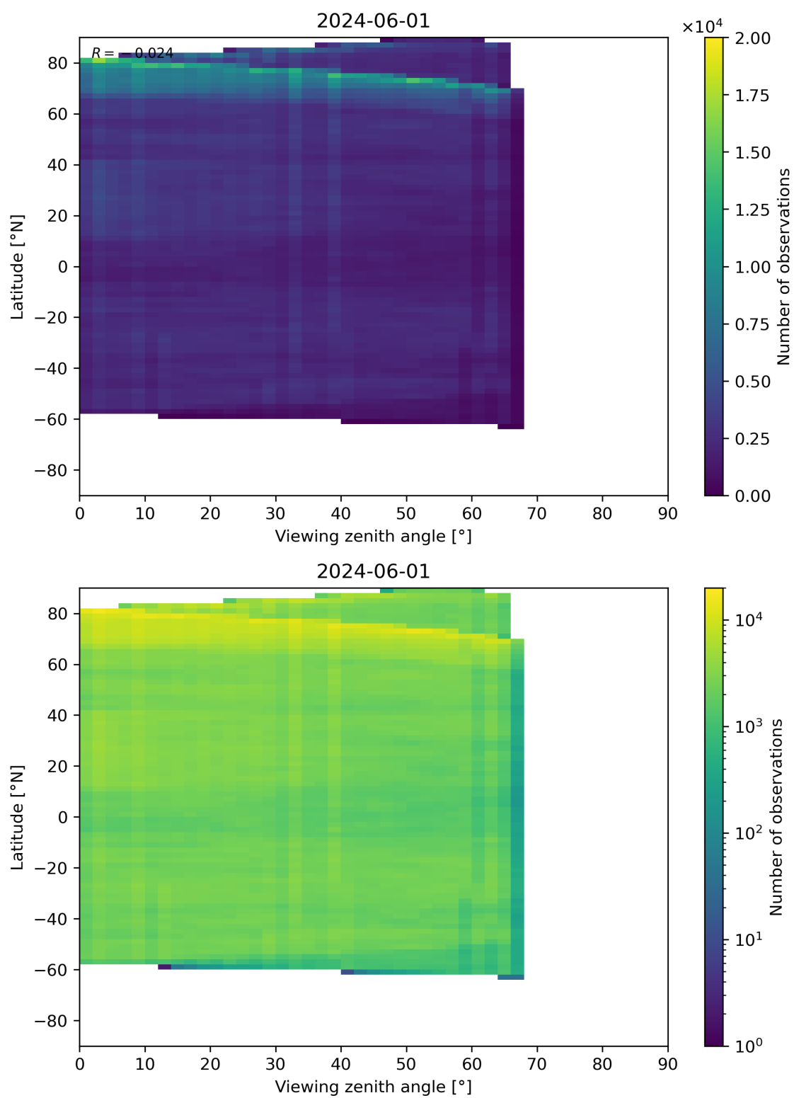
Figure 74: Scatter density plot of “Viewing zenith angle” against “Latitude” for 2024-05-31 to 2024-06-02.
