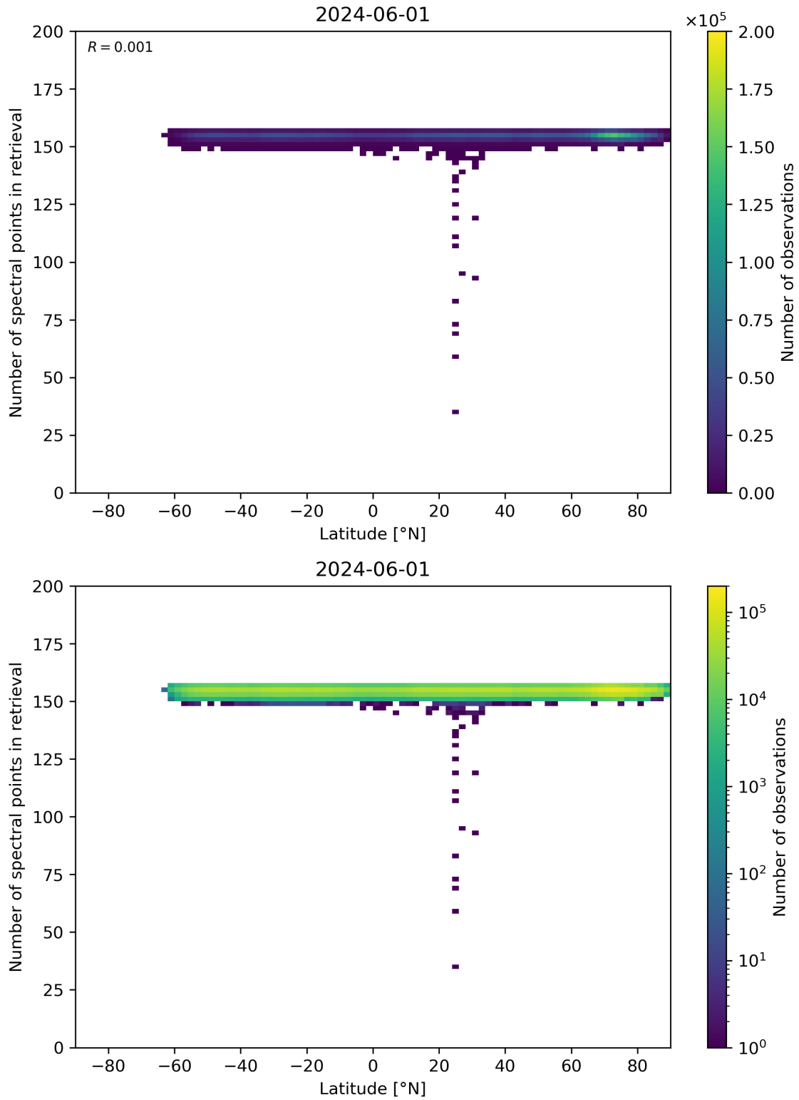
Figure 57: Scatter density plot of “Latitude” against “Number of spectral points in retrieval” for 2024-05-31 to 2024-06-02.
