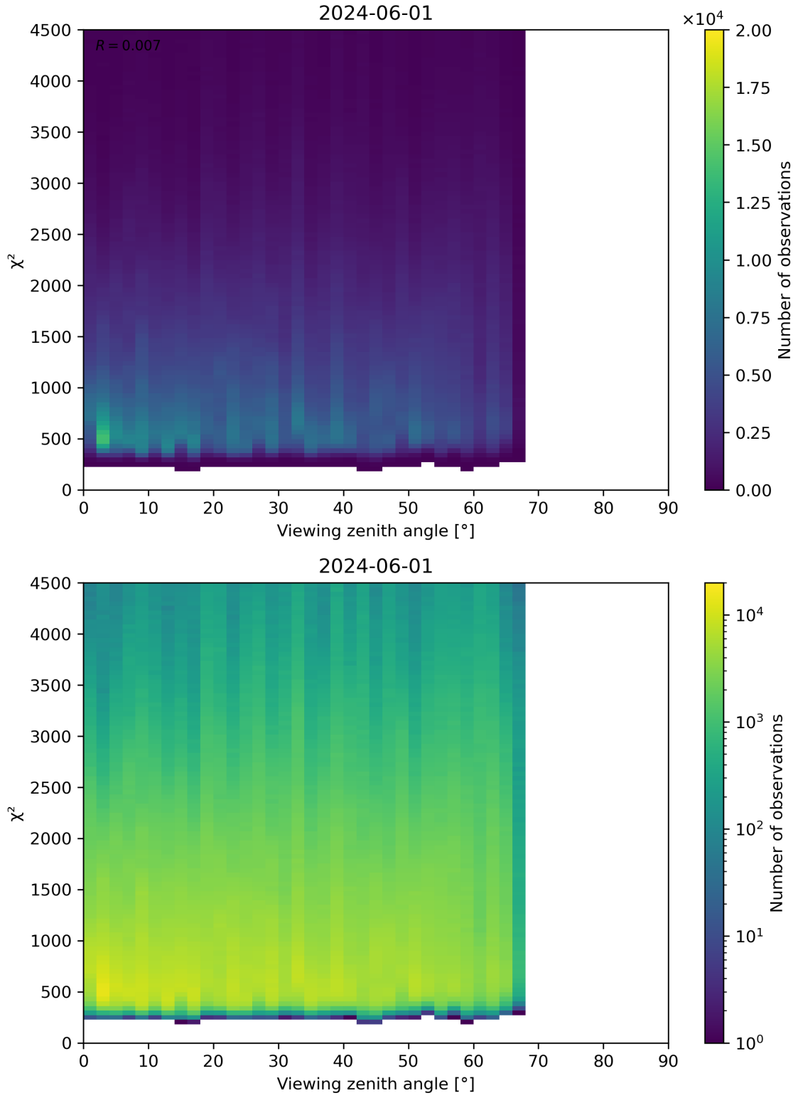
Figure 72: Scatter density plot of “Viewing zenith angle” against “ \chi^2 ” for 2024-05-31 to 2024-06-02.
