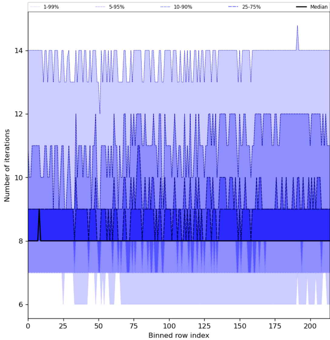
Figure 32: Along track statistics of “Number of iterations” for 2024-05-31 to 2024-06-02
