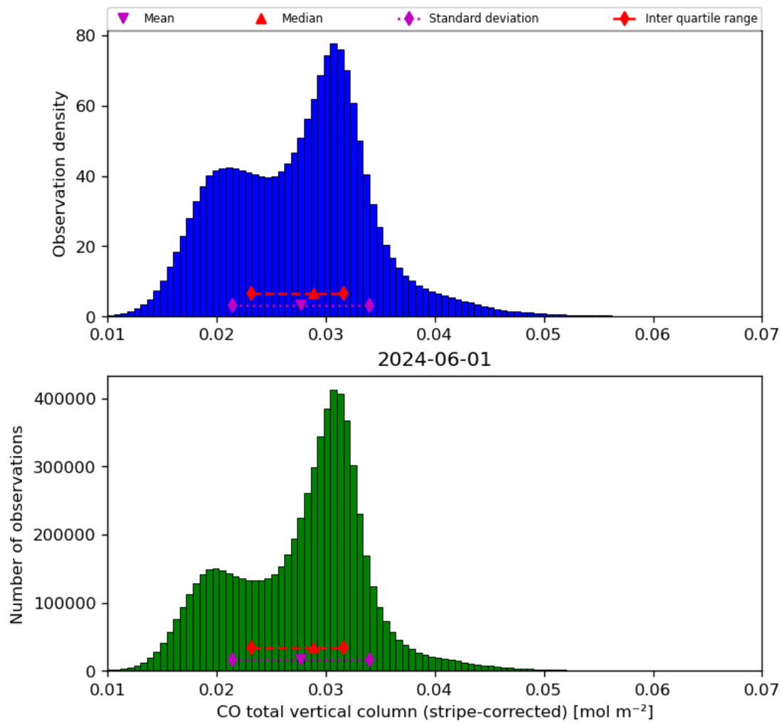
Figure 19: Histogram of “CO total vertical column (stripe-corrected)” for 2024-05-31 to 2024-06-02
