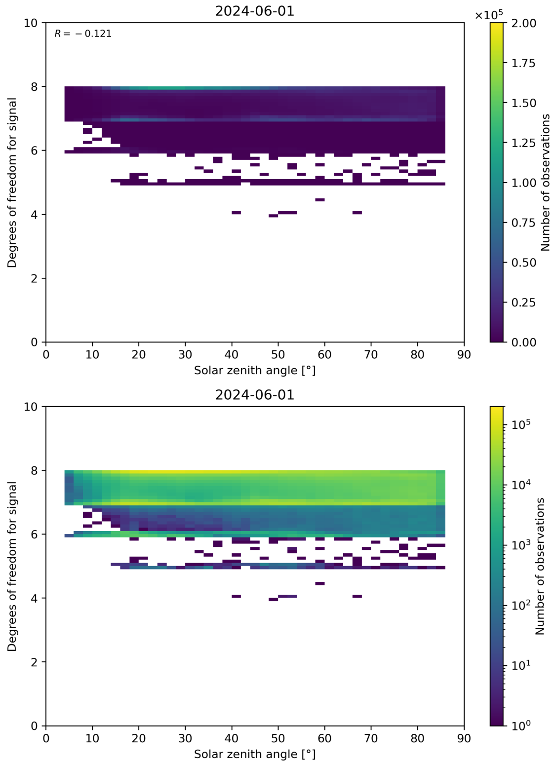
Figure 65: Scatter density plot of “Solar zenith angle” against “Degrees of freedom for signal” for 2024-05-31 to 2024-06-02.
