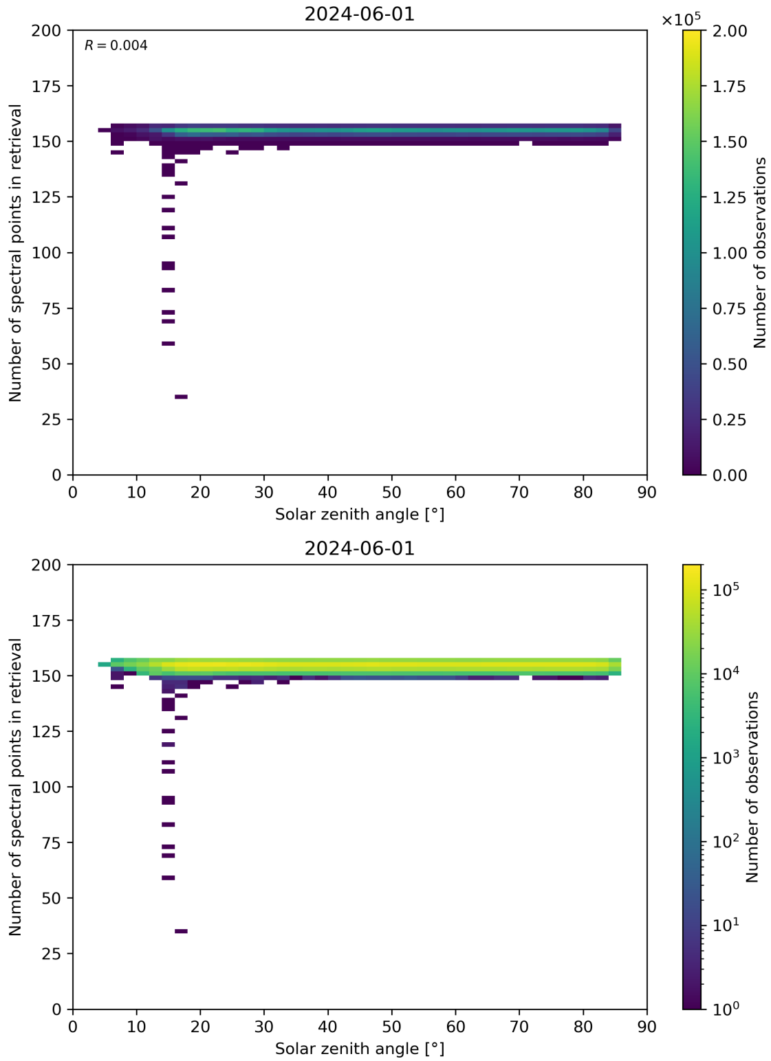
Figure 68: Scatter density plot of “Solar zenith angle” against “Number of spectral points in retrieval” for 2024-05-31 to 2024-06-02.
